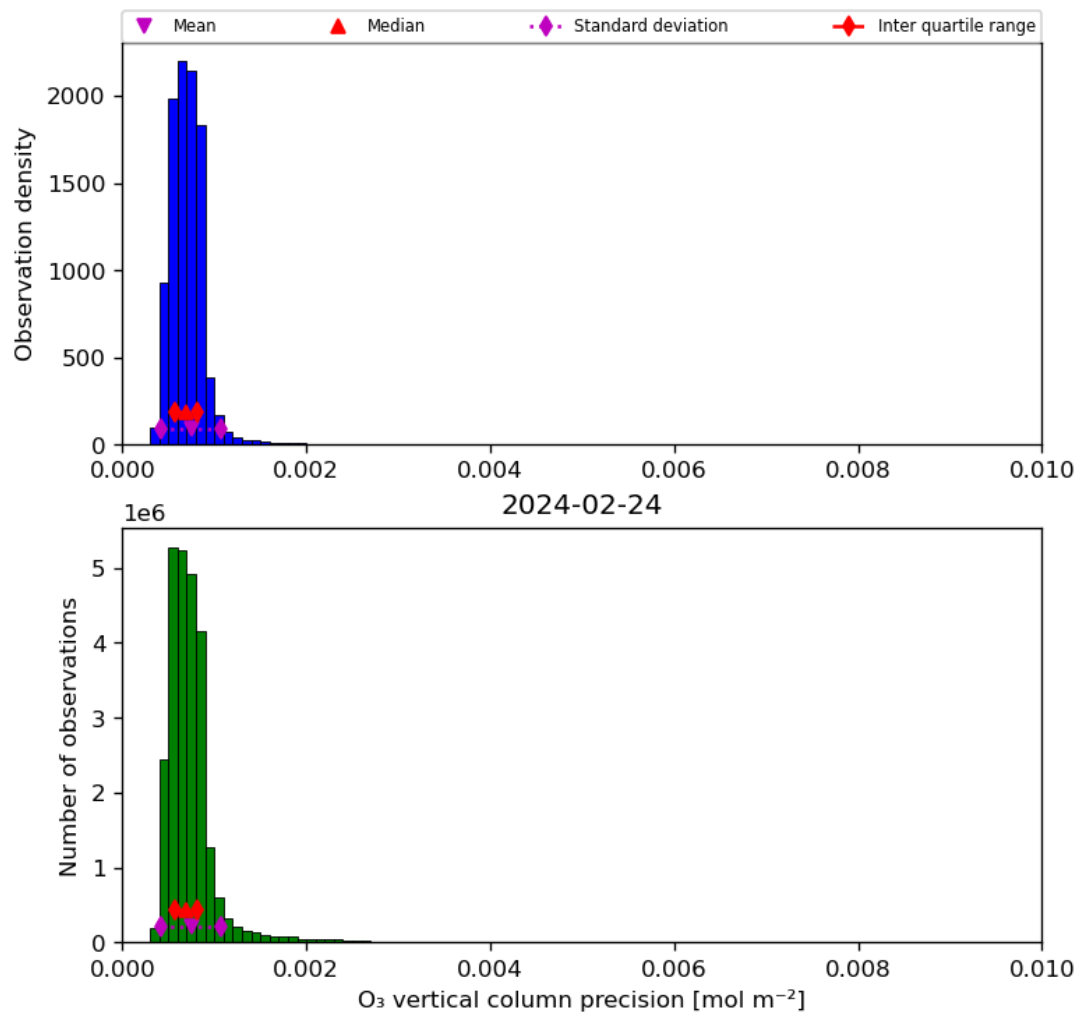
Figure 22: Histogram of “O 3 vertical column precision” for 2024-02-23 to 2024-02-25
