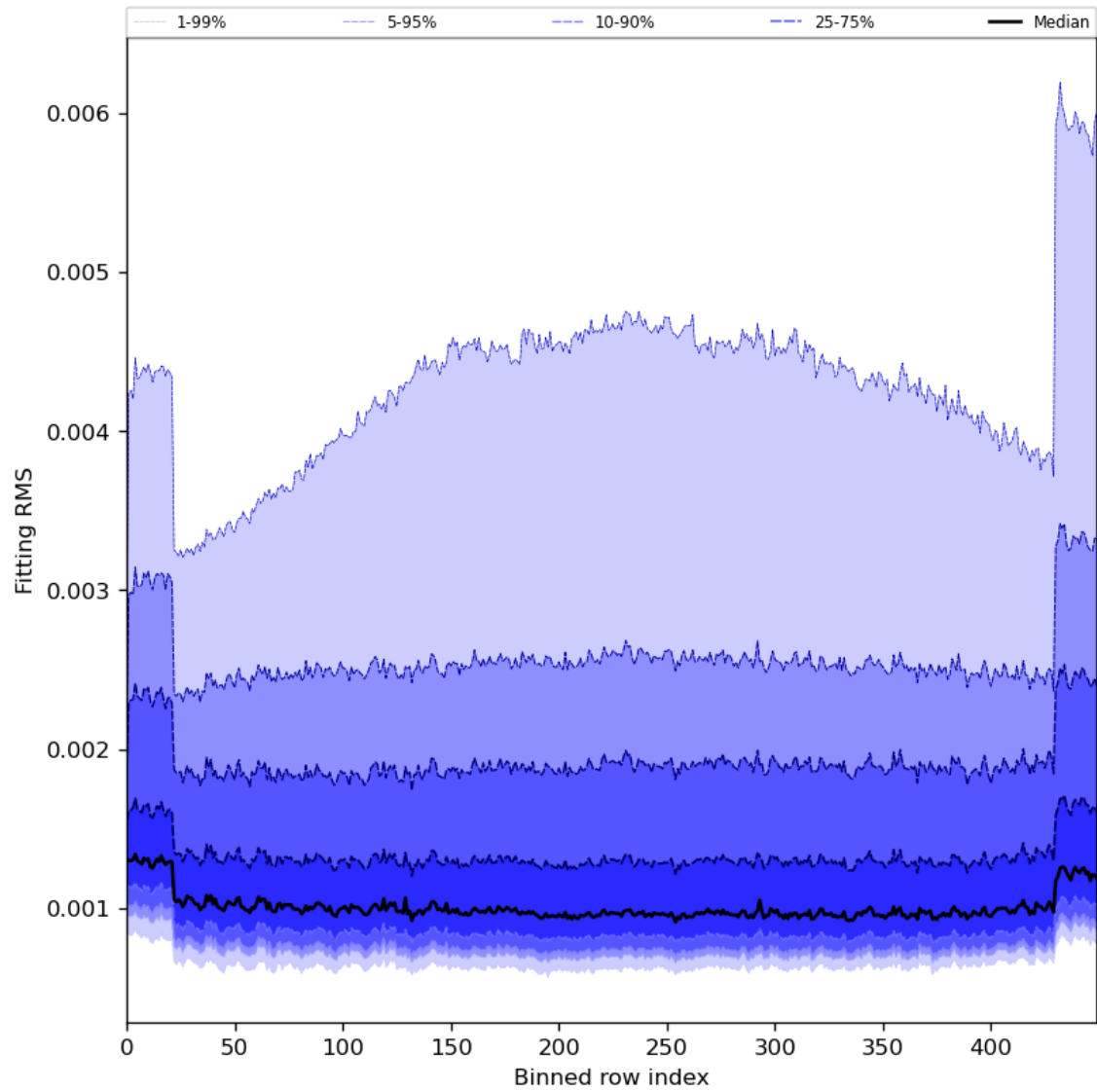
Figure 30: Along track statistics of “Fitting RMS” for 2024-02-23 to 2024-02-25
