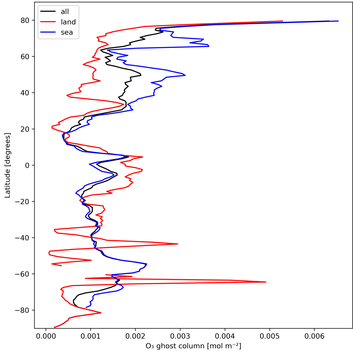
Figure 18: Zonal average of "O 3 ghost column" for 2024-02-23 to 2024-02-25.
