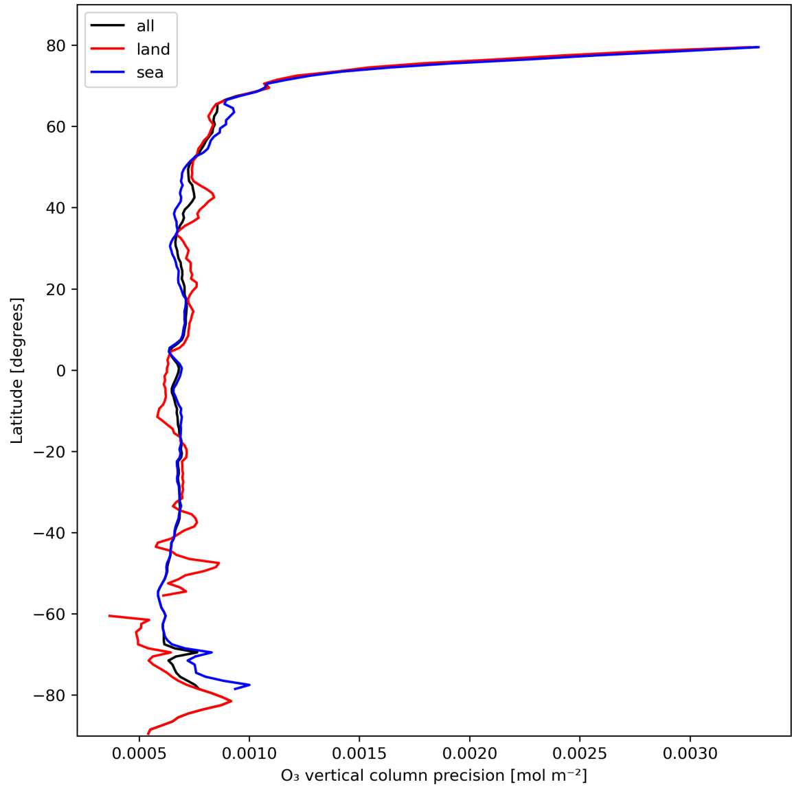
Figure 15: Zonal average of “O 3 vertical column precision” for 2024-02-23 to 2024-02-25.
