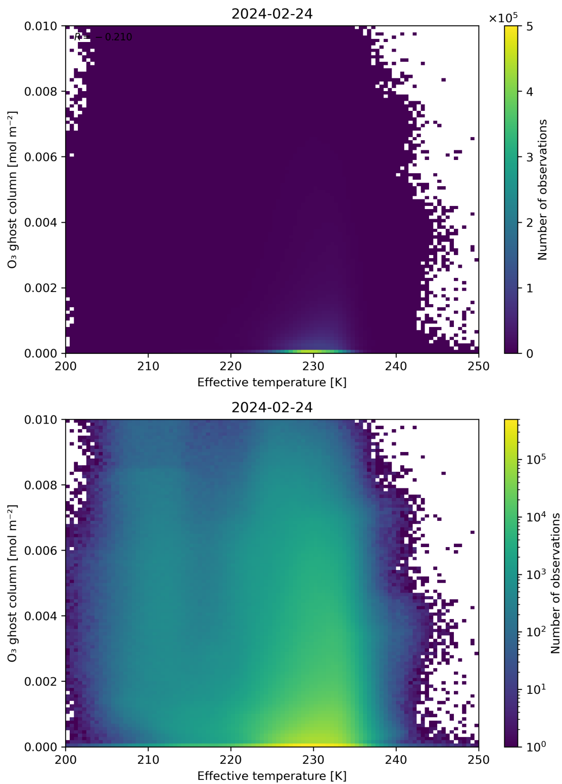
Figure 38: Scatter density plot of “Effective temperature” against “O 3 ghost column” for 2024-02-23 to 2024-02-25.
