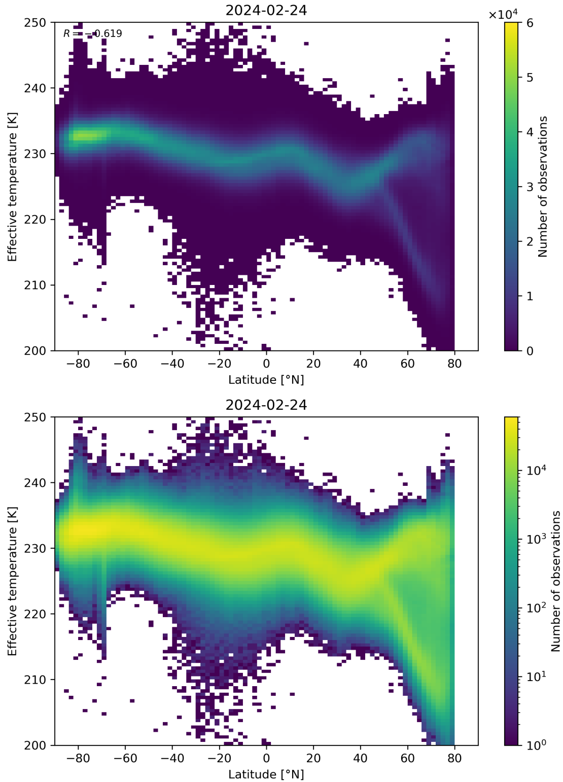
Figure 34: Scatter density plot of “Latitude” against “Effective temperature” for 2024-02-23 to 2024-02-25.
