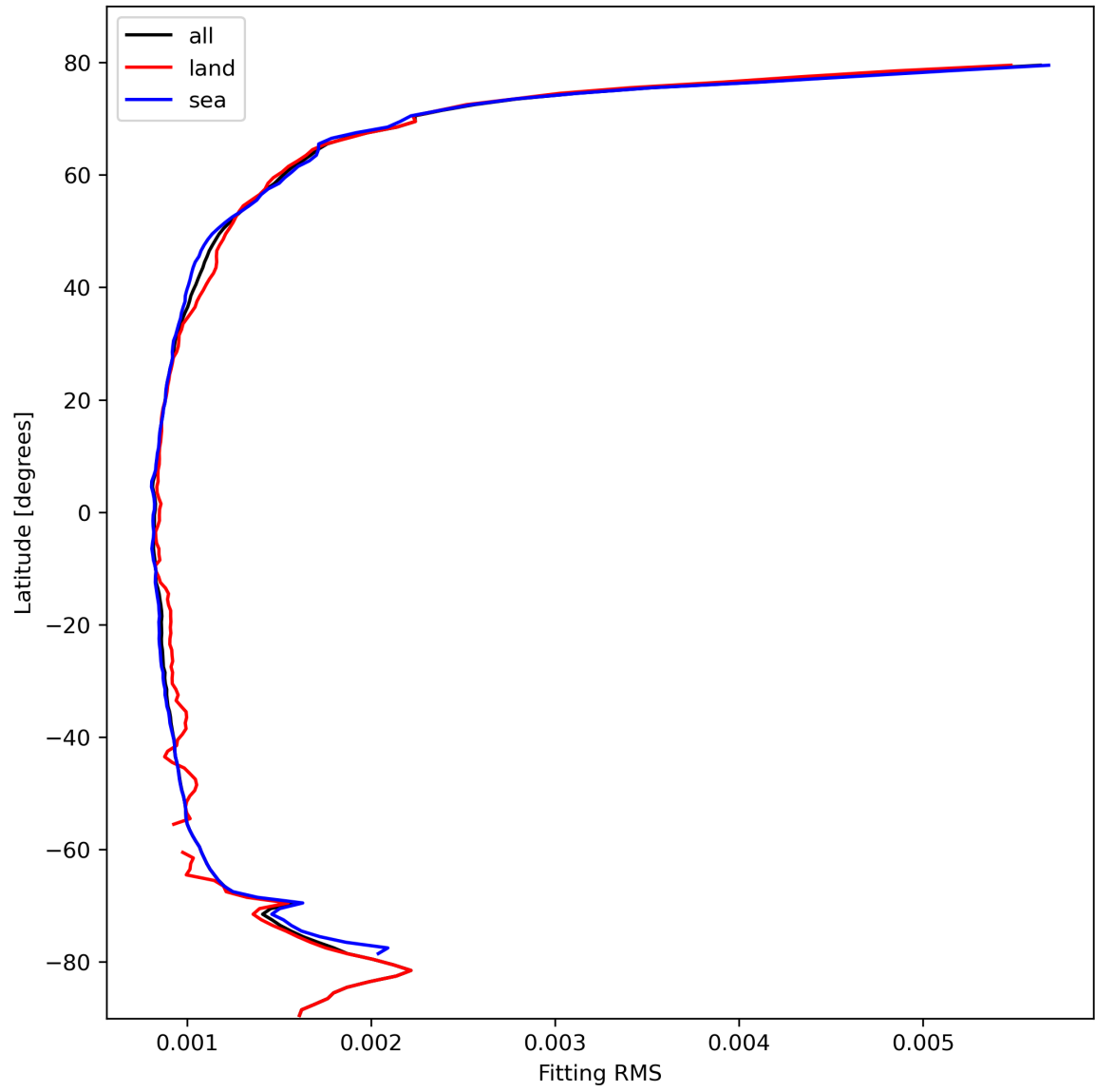
Figure 16: Zonal average of “Fitting RMS” for 2024-02-23 to 2024-02-25.
