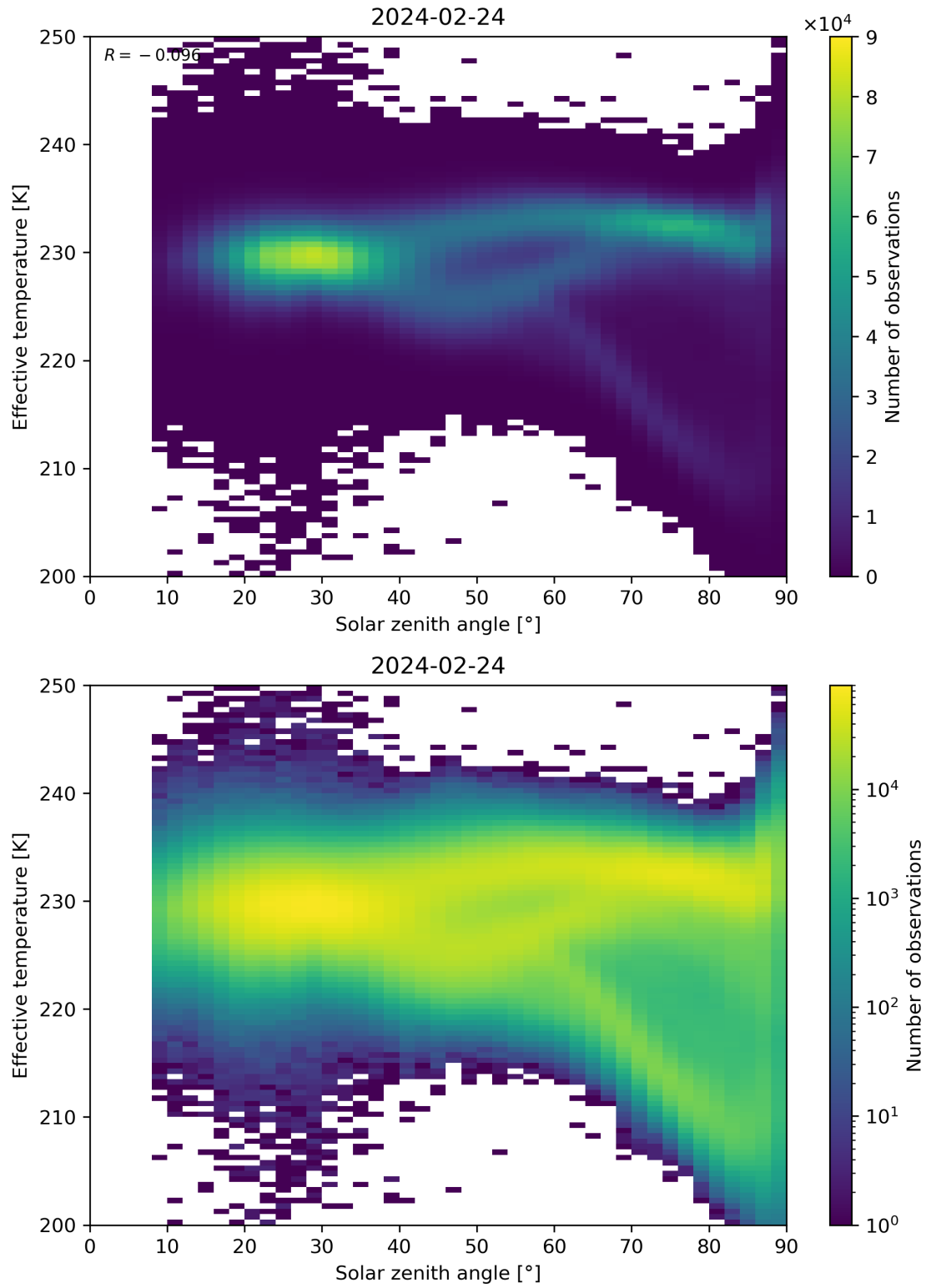
Figure 45: Scatter density plot of “Solar zenith angle” against “Effective temperature” for 2024-02-23 to 2024-02-25.
