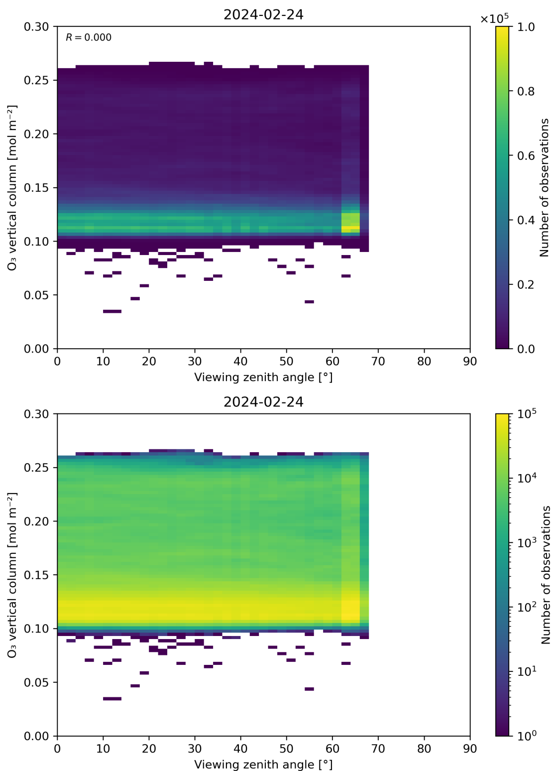
Figure 52: Scatter density plot of “Viewing zenith angle” against “O 3 vertical column” for 2024-02-23 to 2024-02-25.
