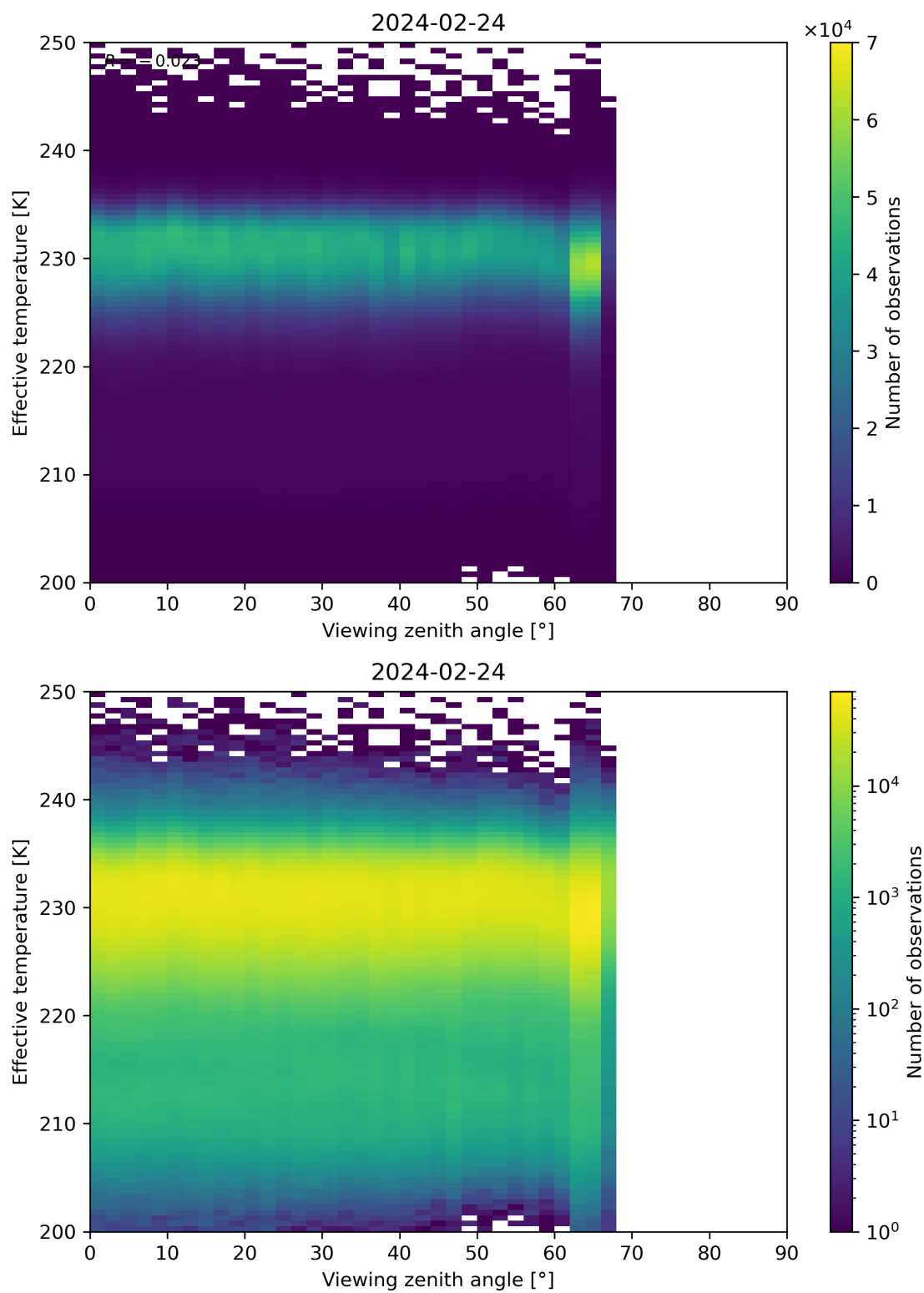
Figure 50: Scatter density plot of “Viewing zenith angle” against “Effective temperature” for 2024-02-23 to 2024-02-25.
