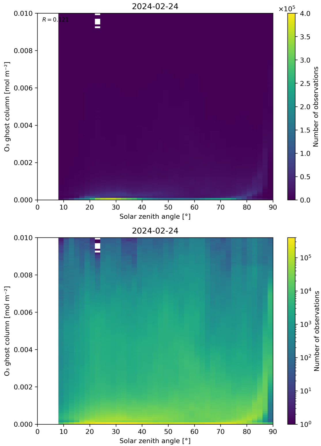
Figure 46: Scatter density plot of “Solar zenith angle” against “O 3 ghost column” for 2024-02-23 to 2024-02-25.
