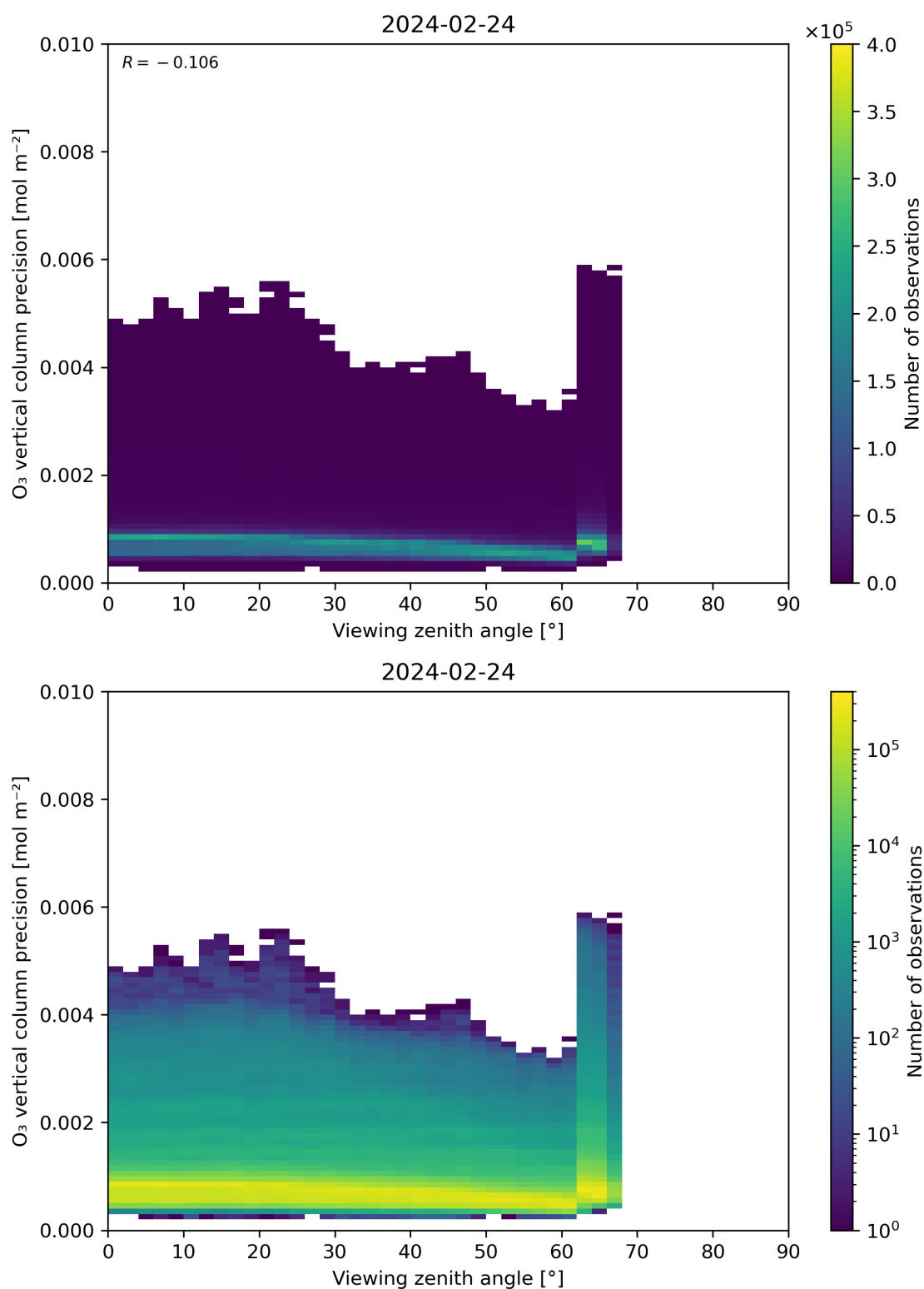
Figure 53: Scatter density plot of “Viewing zenith angle” against “O 3 vertical column precision” for 2024-02-23 to 2024-02-25.
