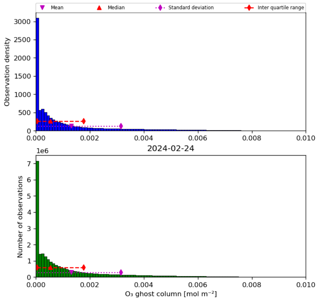
Figure 25: Histogram of “O 3 ghost column” for 2024-02-23 to 2024-02-25
