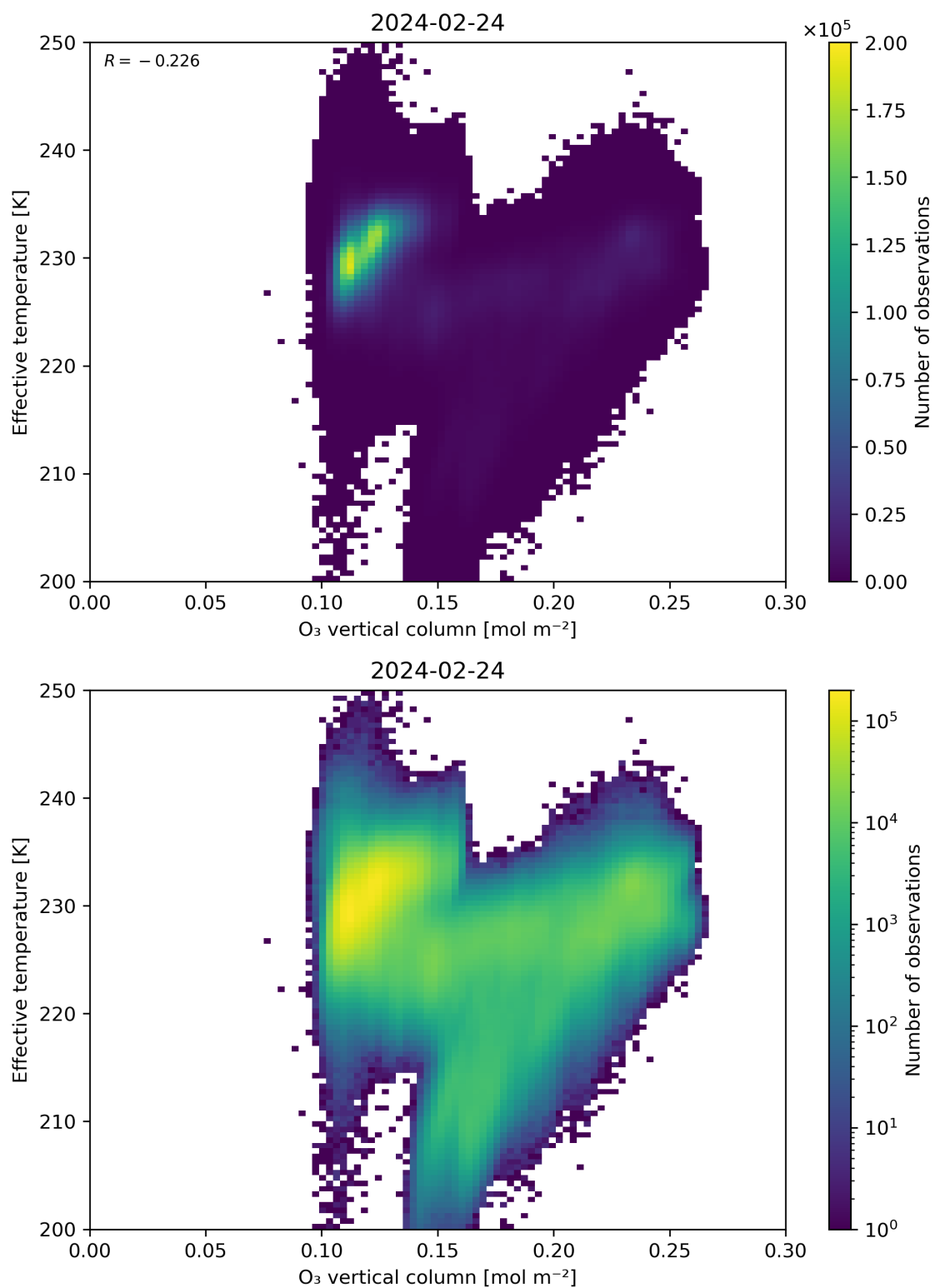
Figure 39: Scatter density plot of “O 3 vertical column” against “Effective temperature” for 2024-02-23 to 2024-02-25.
