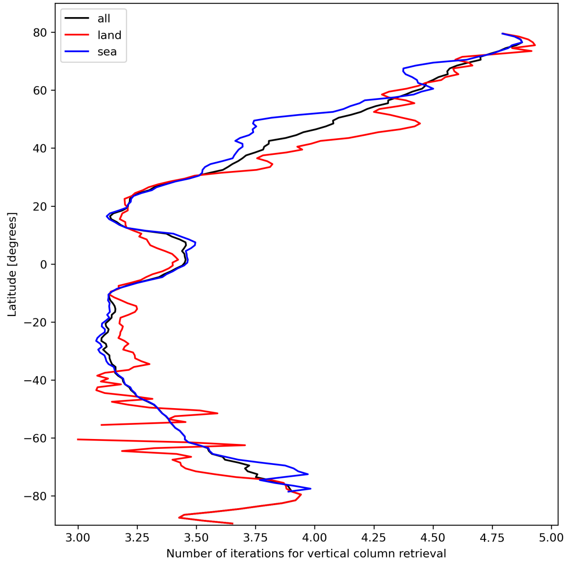
Figure 19: Zonal average of “Number of iterations for vertical column retrieval” for 2024-02-23 to 2024-02-25.
