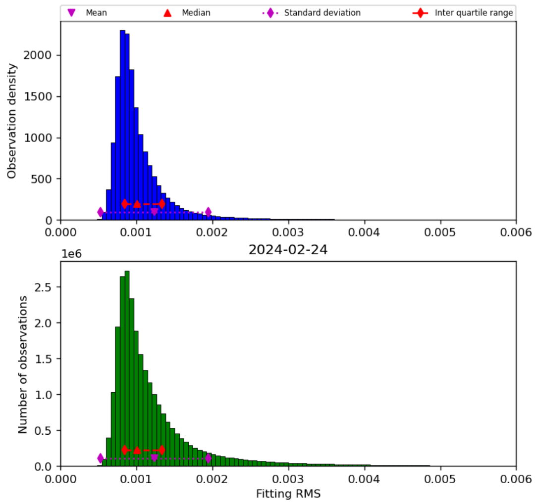
Figure 23: Histogram of “Fitting RMS” for 2024-02-23 to 2024-02-25
