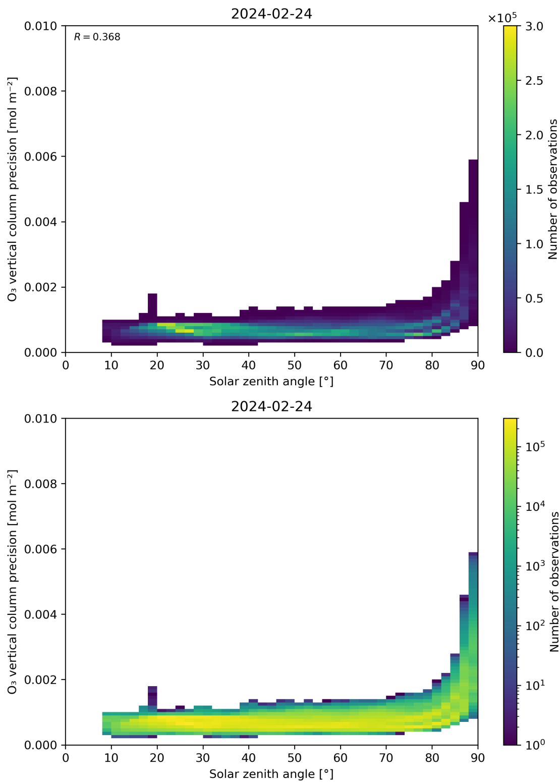
Figure 48: Scatter density plot of “Solar zenith angle” against “O 3 vertical column precision” for 2024-02-23 to 2024-02-25.
