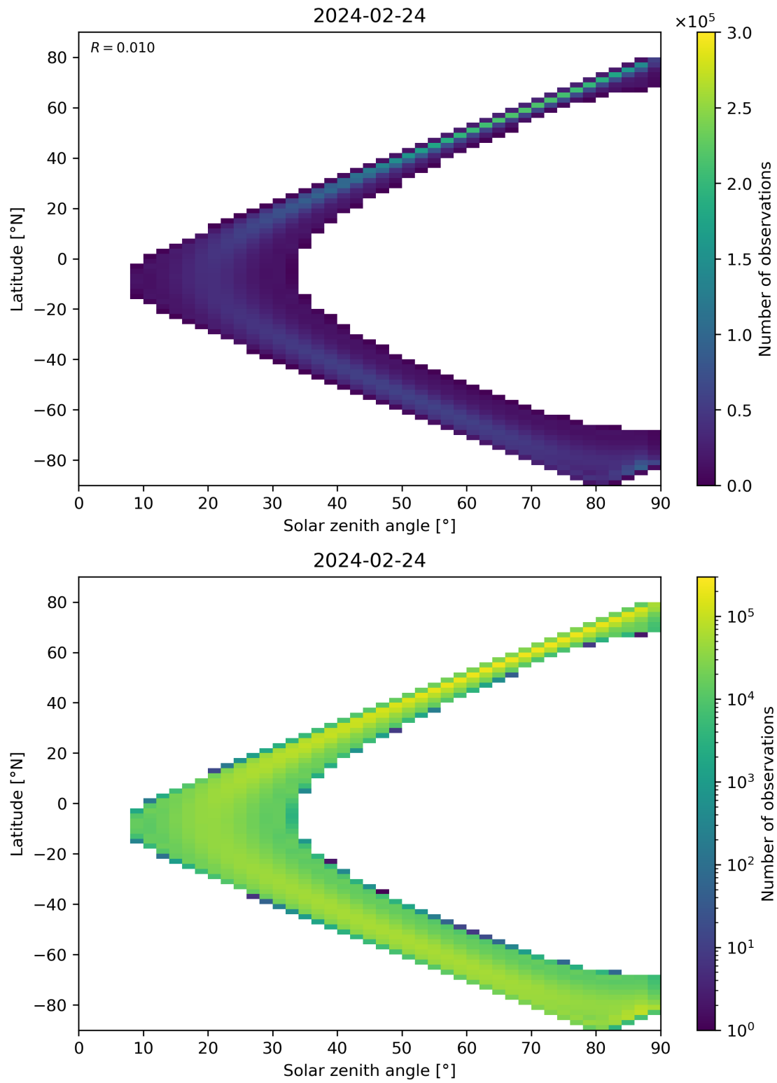
Figure 44: Scatter density plot of “Solar zenith angle” against “Latitude” for 2024-02-23 to 2024-02-25.
