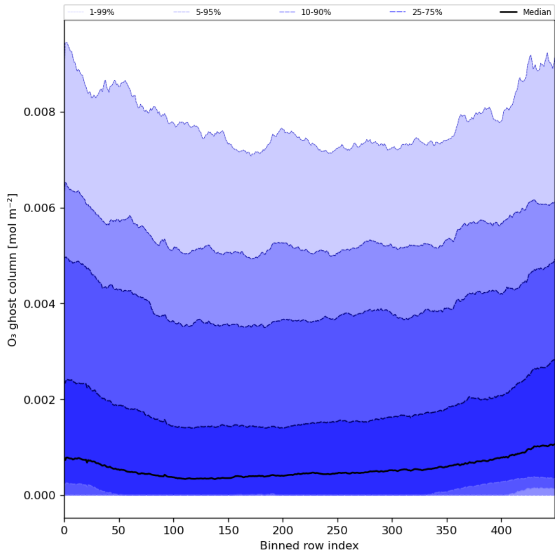
Figure 32: Along track statistics of “O 3 ghost column” for 2024-02-23 to 2024-02-25
