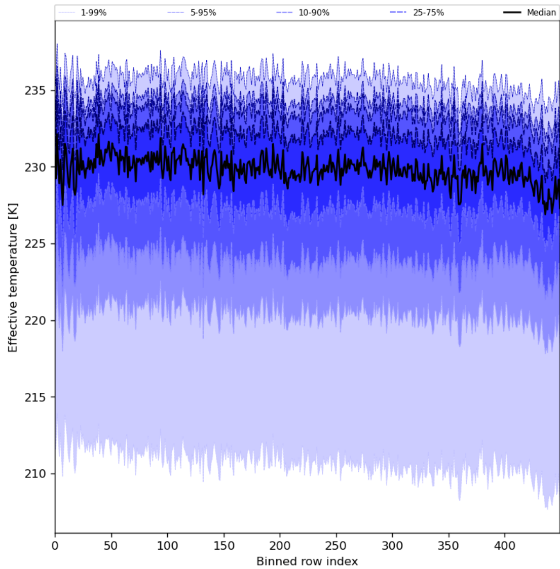
Figure 31: Along track statistics of “Effective temperature” for 2024-02-23 to 2024-02-25
