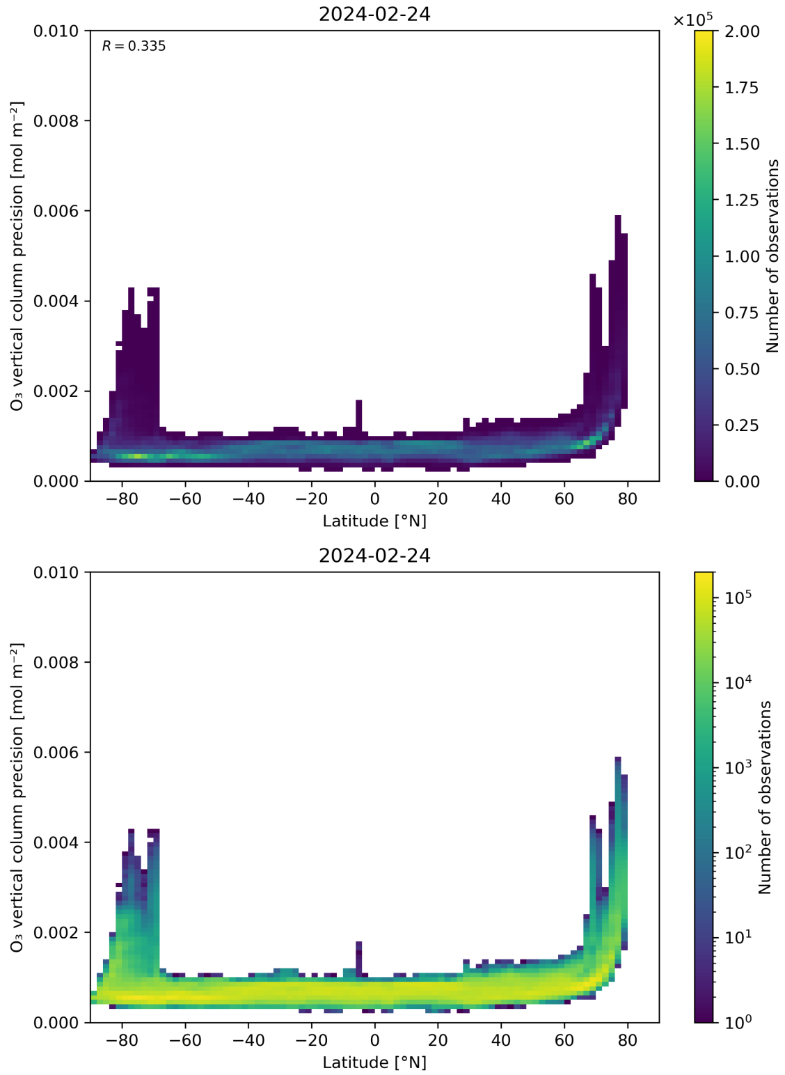
Figure 37: Scatter density plot of “Latitude” against “O 3 vertical column precision” for 2024-02-23 to 2024-02-25.
