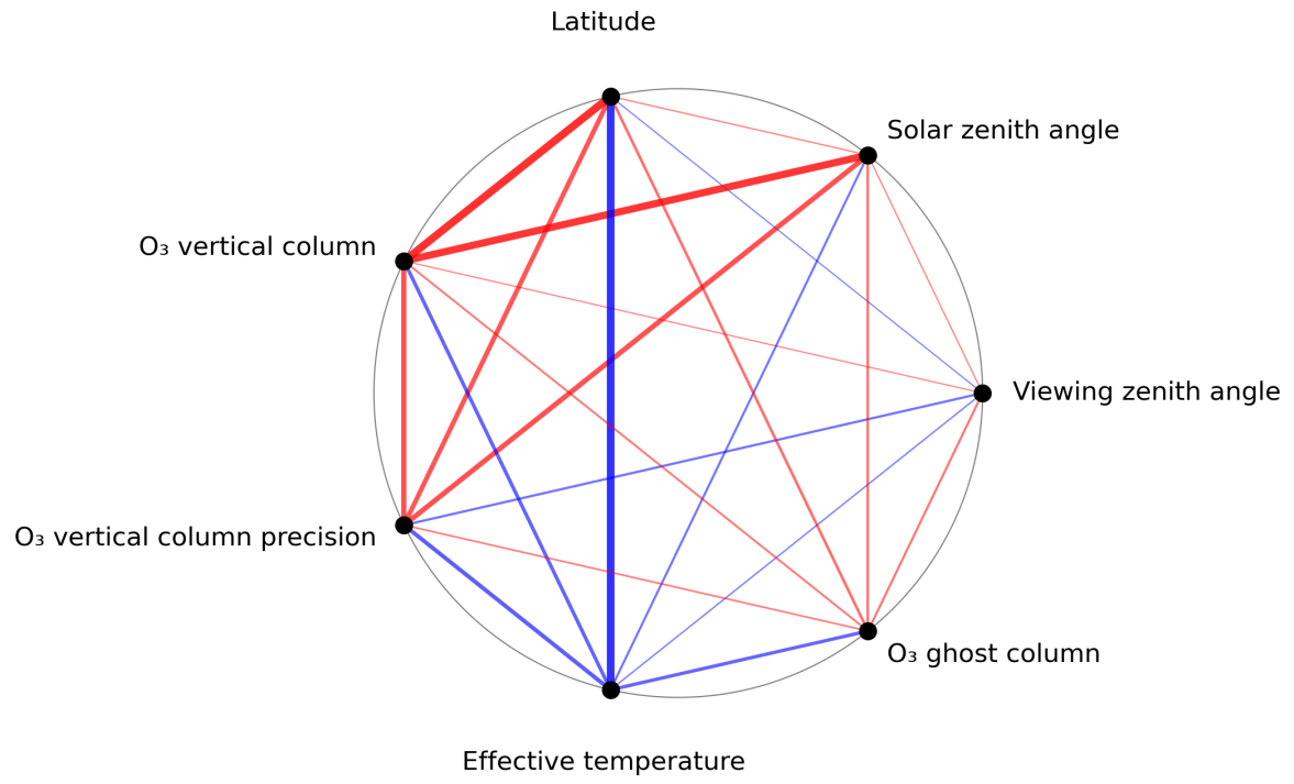
Figure 1: Map of correlation graph for 2024-02-23 to 2024-02-25.
