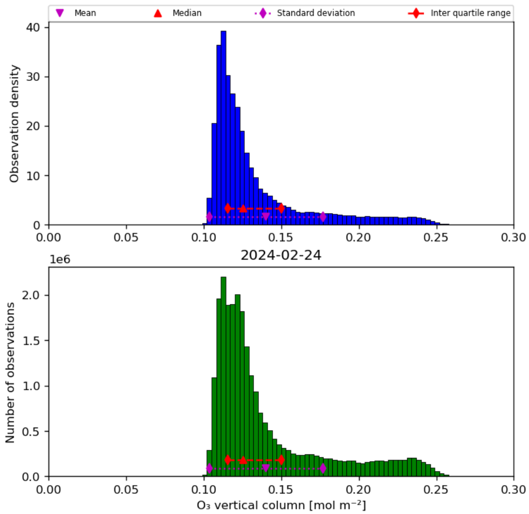
Figure 21: Histogram of “O 3 vertical column” for 2024-02-23 to 2024-02-25
