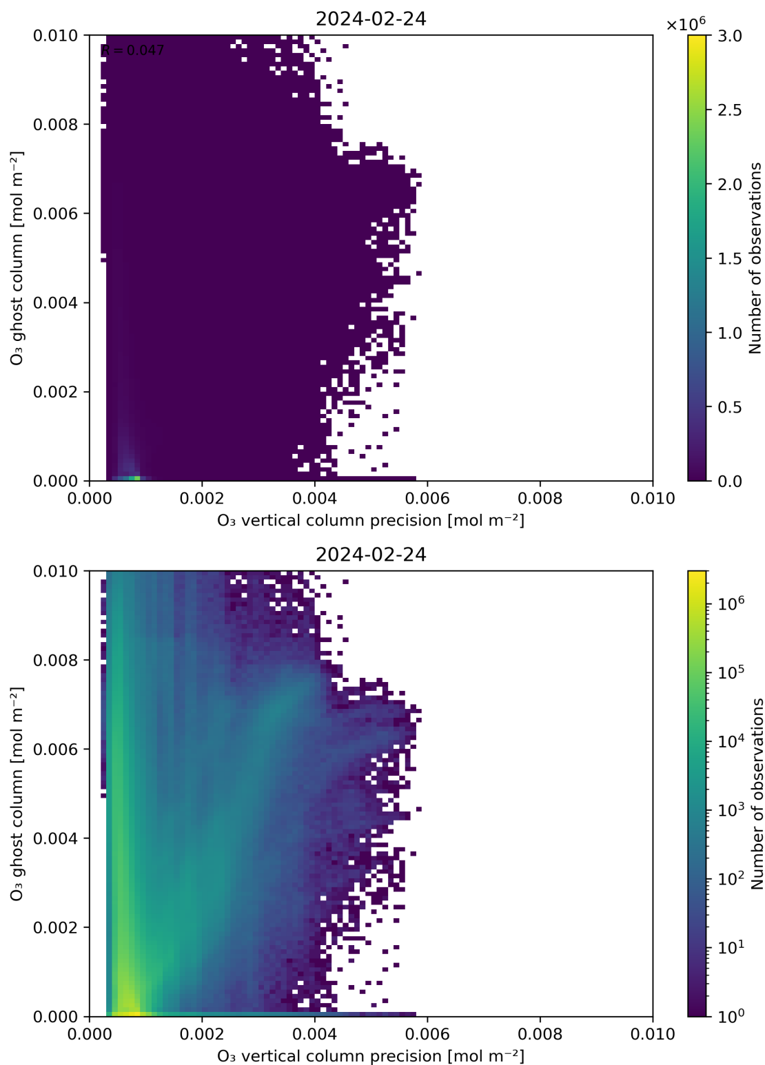
Figure 43: Scatter density plot of “O 3 vertical column precision” against “O 3 ghost column” for 2024-02-23 to 2024-02-25.
