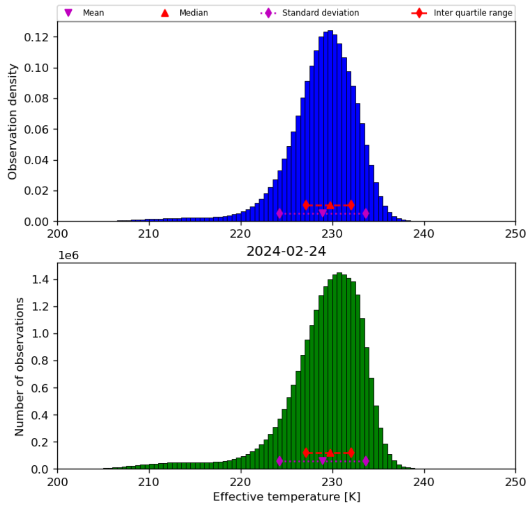
Figure 24: Histogram of “Effective temperature” for 2024-02-23 to 2024-02-25
