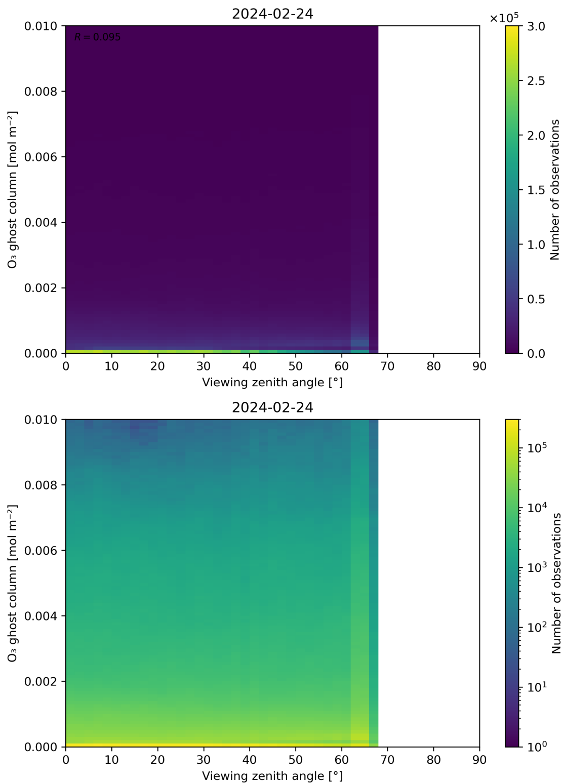
Figure 51: Scatter density plot of “Viewing zenith angle” against “O 3 ghost column” for 2024-02-23 to 2024-02-25.
