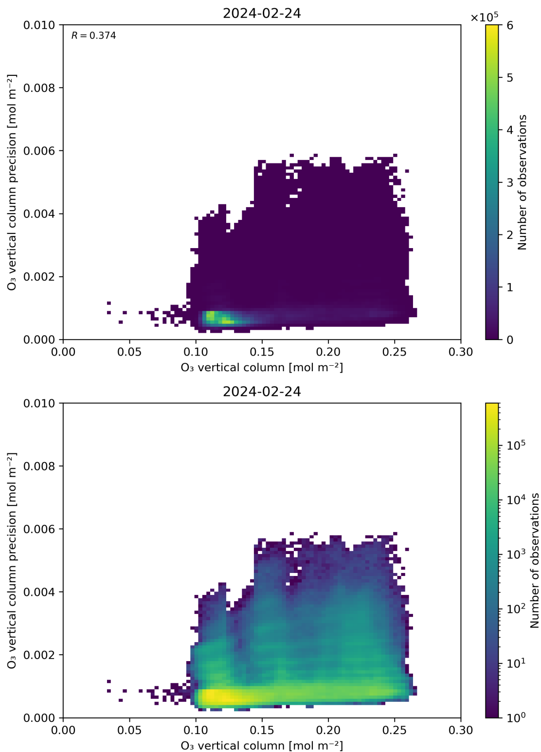
Figure 41: Scatter density plot of “O 3 vertical column” against “O 3 vertical column precision” for 2024-02-23 to 2024-02-25.
