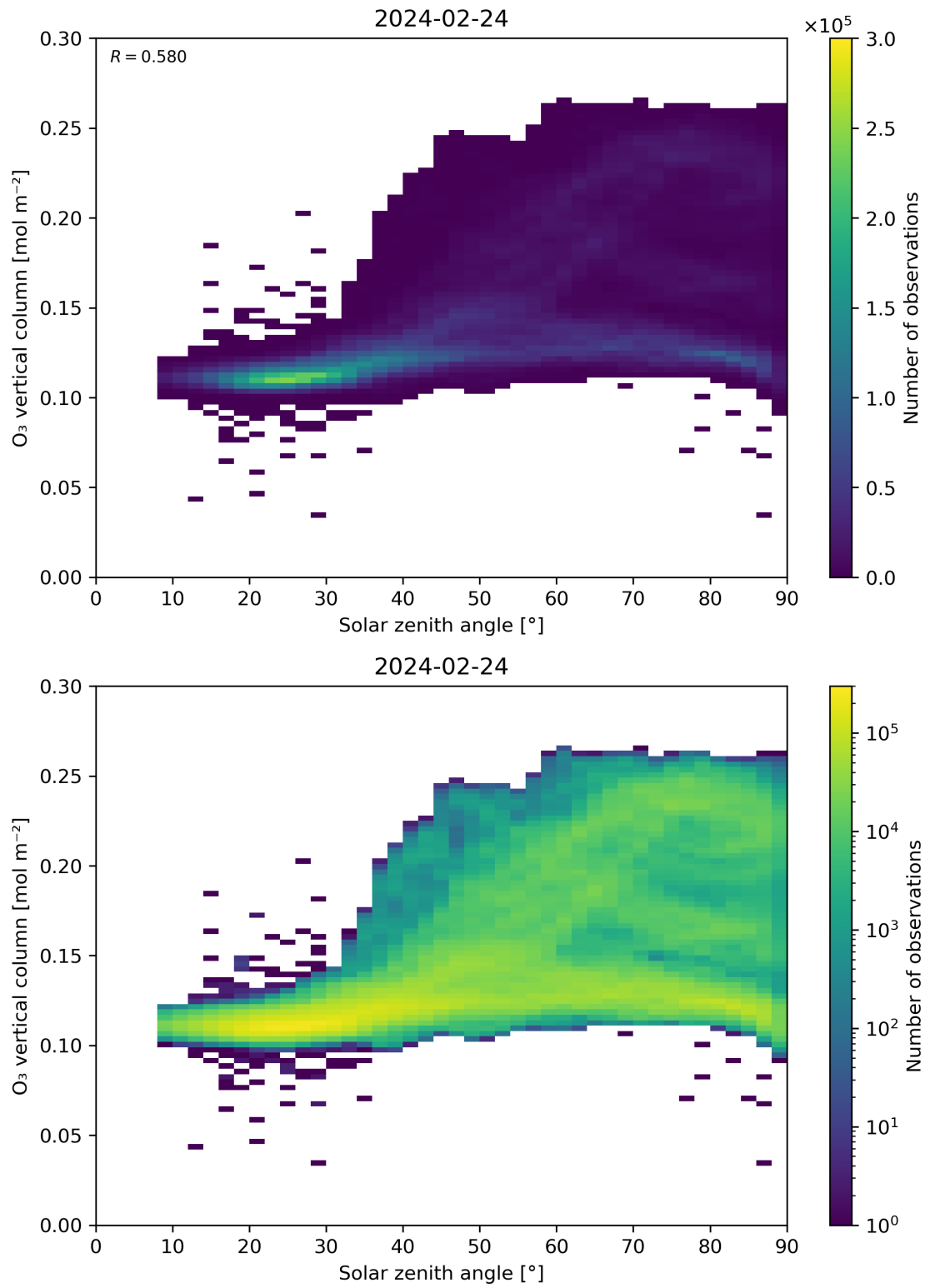
Figure 47: Scatter density plot of “Solar zenith angle” against “O 3 vertical column” for 2024-02-23 to 2024-02-25.
