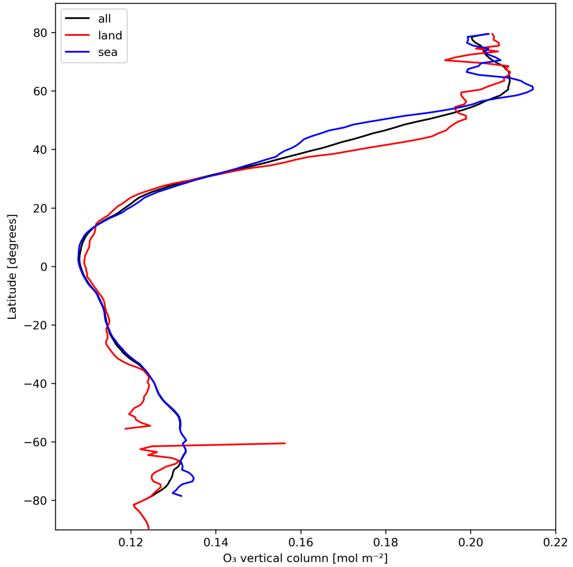
Figure 14: Zonal average of “O 3 vertical column” for 2024-02-23 to 2024-02-25.
