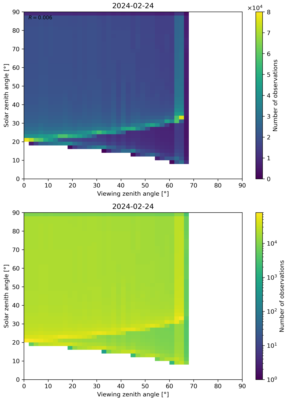
Figure 54: Scatter density plot of “Viewing zenith angle” against “Solar zenith angle” for 2024-02-23 to 2024-02-25.
