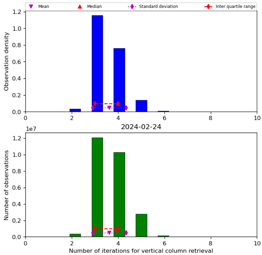
Figure 26: Histogram of “Number of iterations for vertical column retrieval” for 2024-02-23 to 2024-02-25
