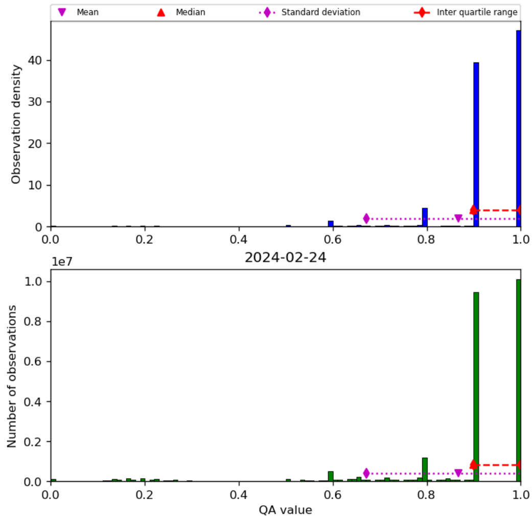
Figure 20: Histogram of “QA value” for 2024-02-23 to 2024-02-25
