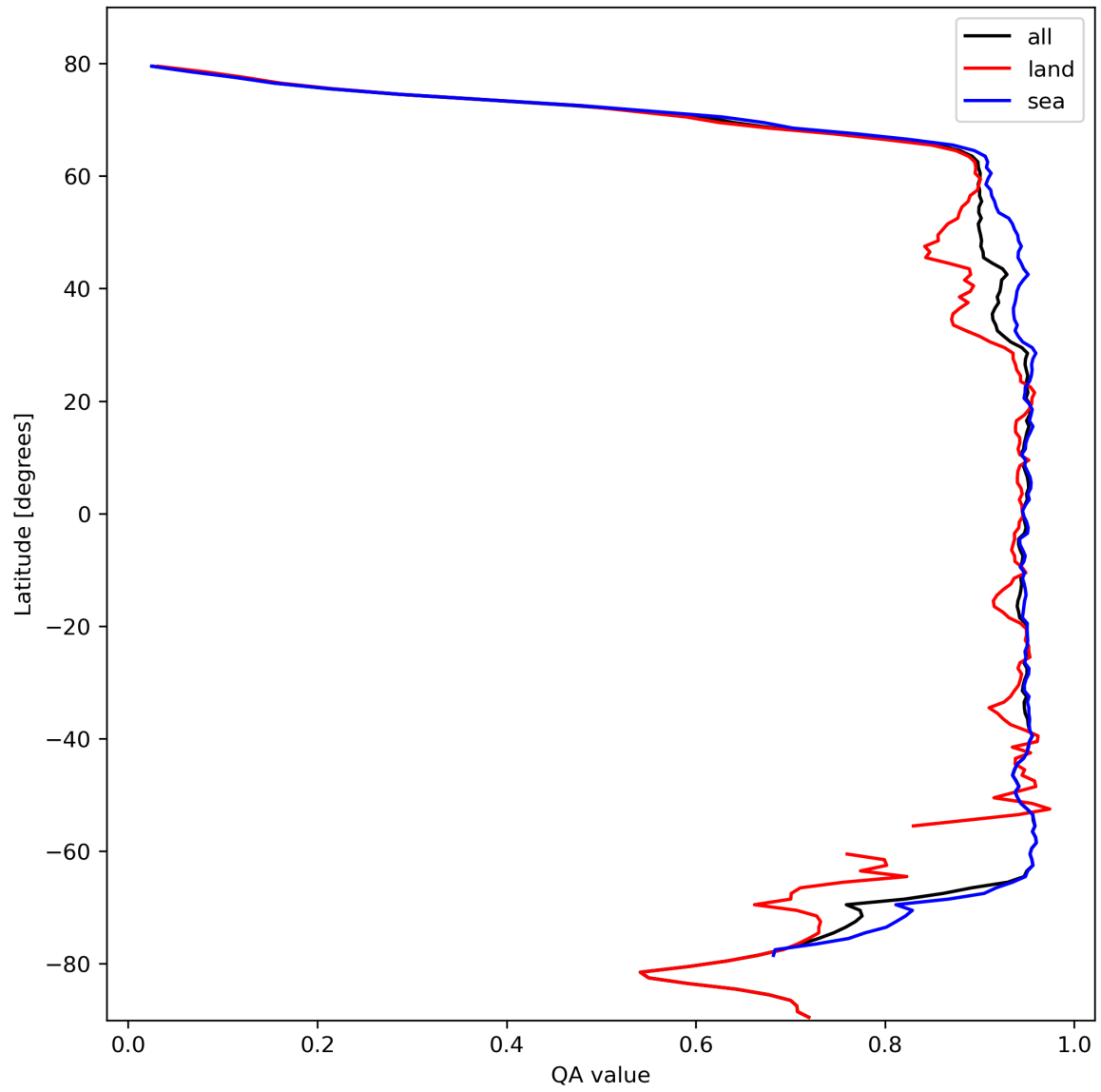
Figure 13: Zonal average of “QA value” for 2024-02-23 to 2024-02-25.
