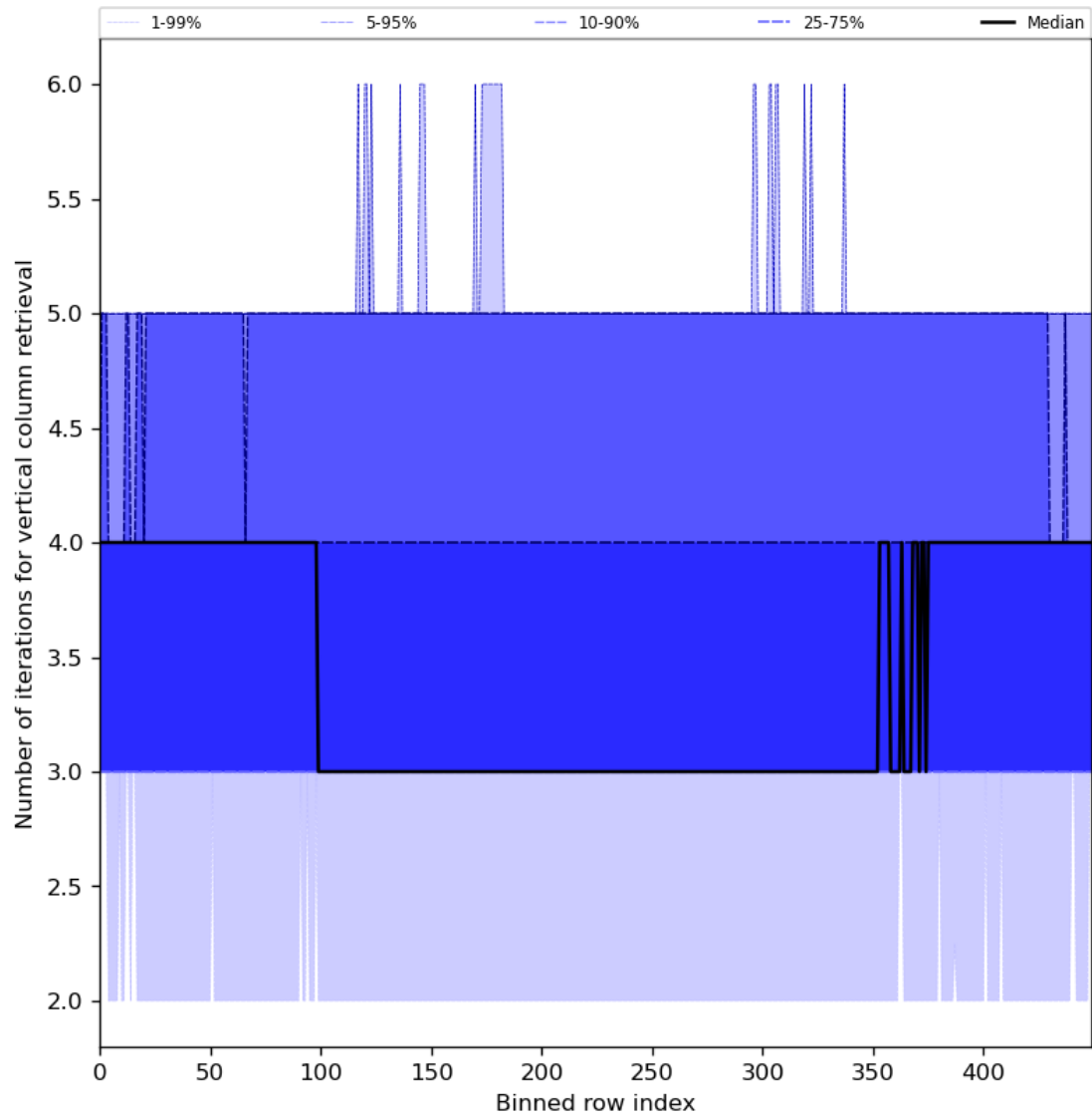
Figure 33: Along track statistics of “Number of iterations for vertical column retrieval” for 2024-02-23 to 2024-02-25
