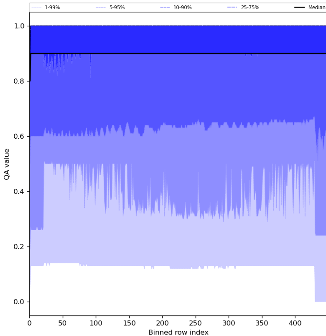
Figure 27: Along track statistics of “QA value” for 2024-02-23 to 2024-02-25
