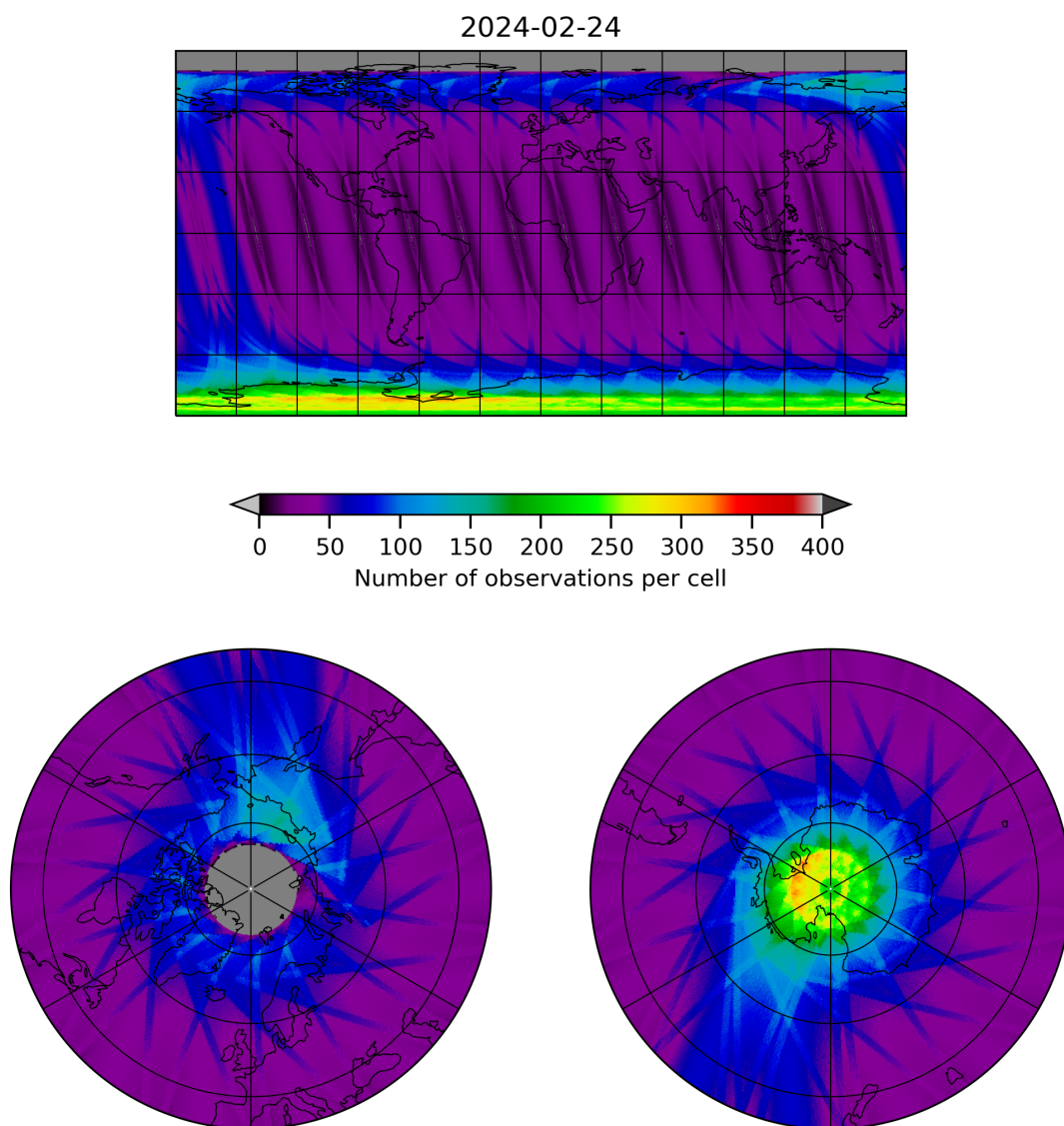
Figure 12: Map of the number of observations for 2024-02-23 to 2024-02-25
