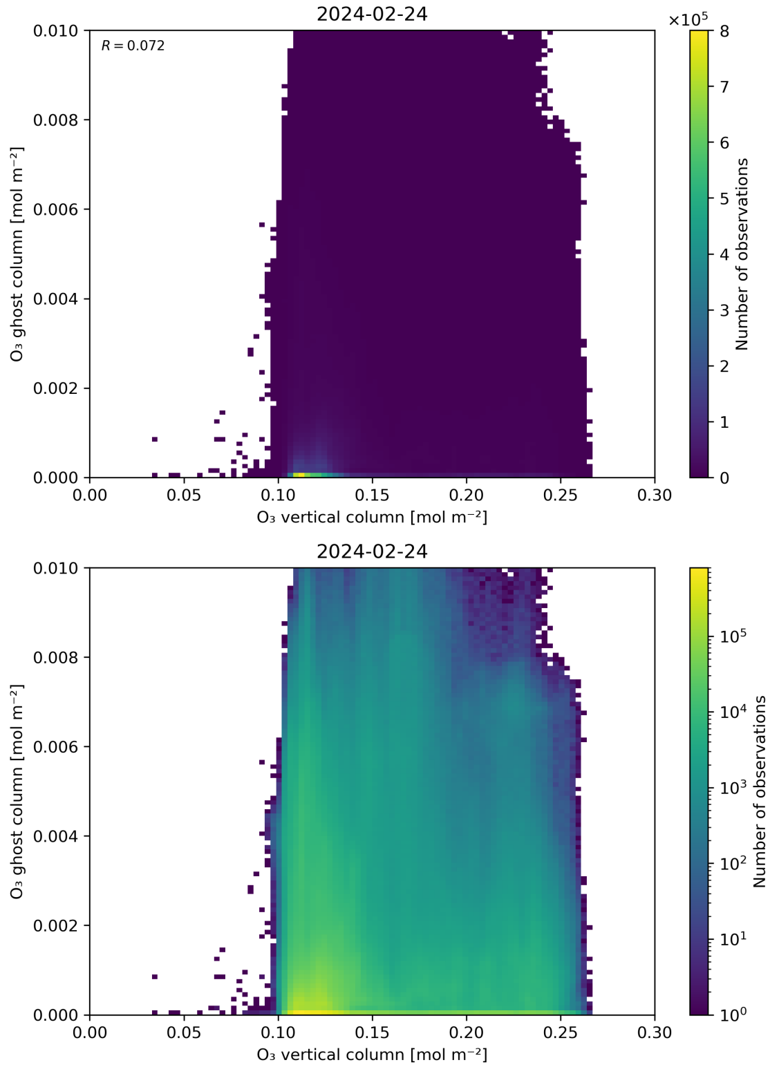
Figure 40: Scatter density plot of “O 3 vertical column” against “O 3 ghost column” for 2024-02-23 to 2024-02-25.
