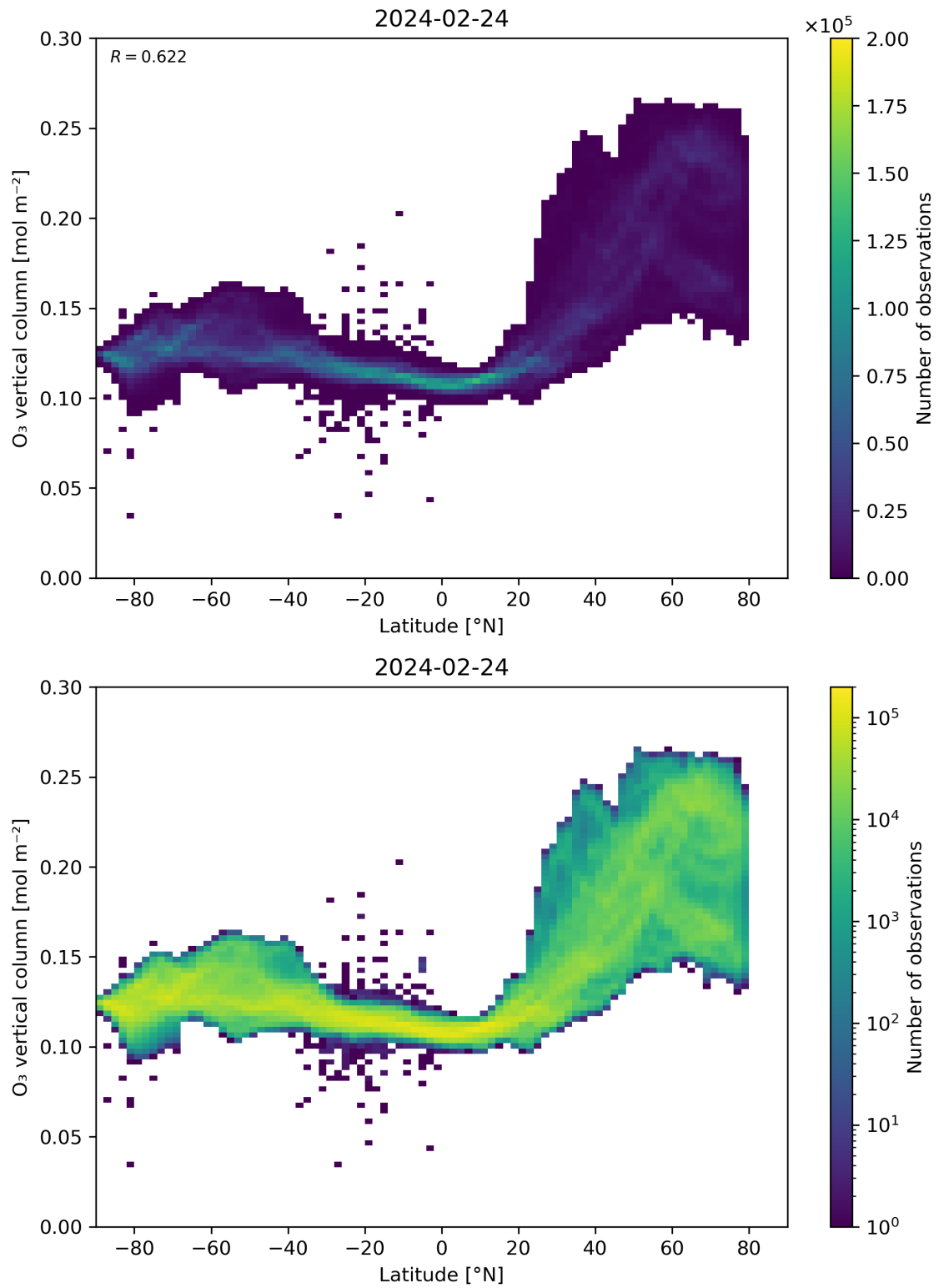
Figure 36: Scatter density plot of “Latitude” against “O 3 vertical column” for 2024-02-23 to 2024-02-25.
