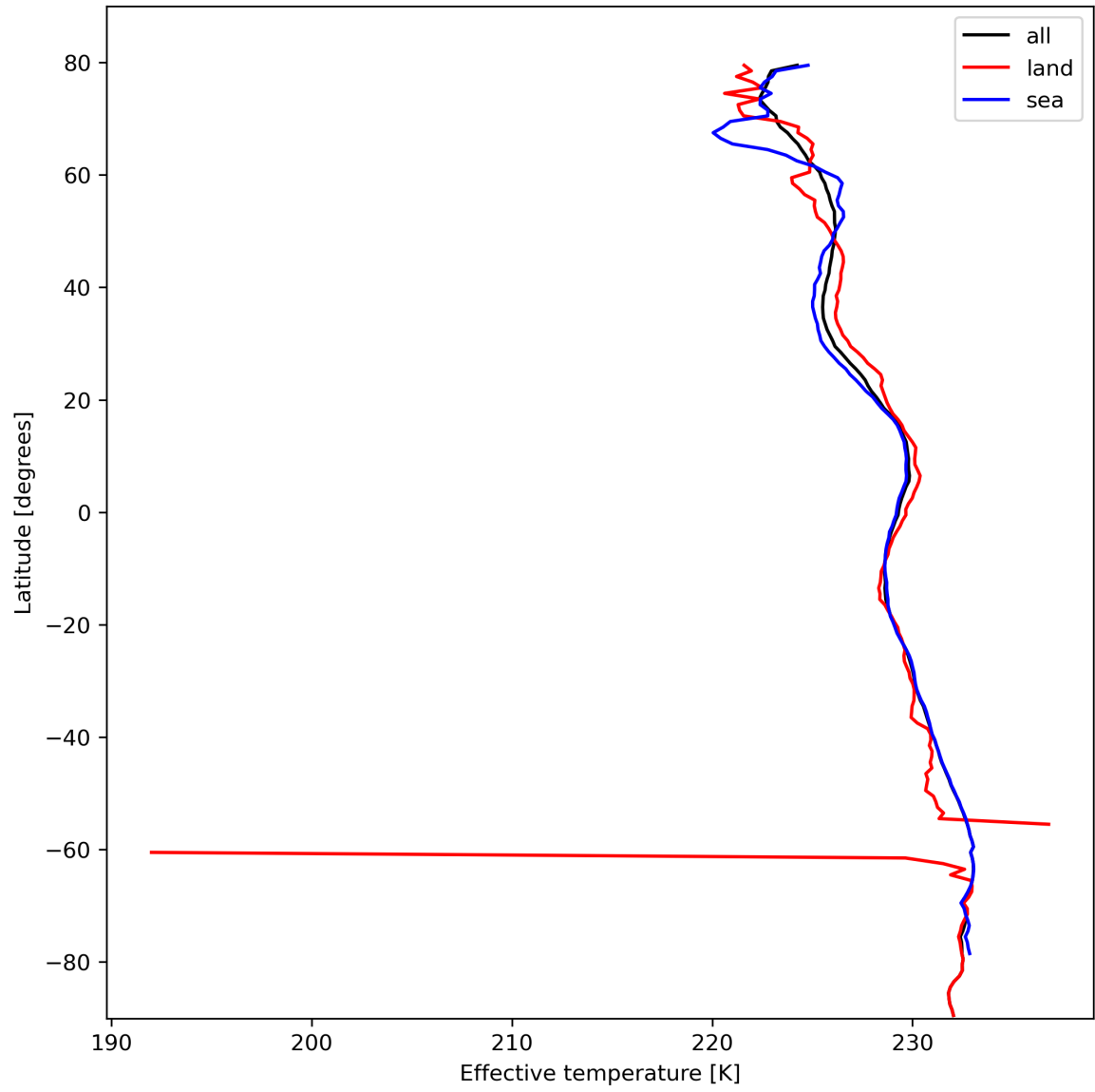
Figure 17: Zonal average of “Effective temperature” for 2024-02-23 to 2024-02-25.
