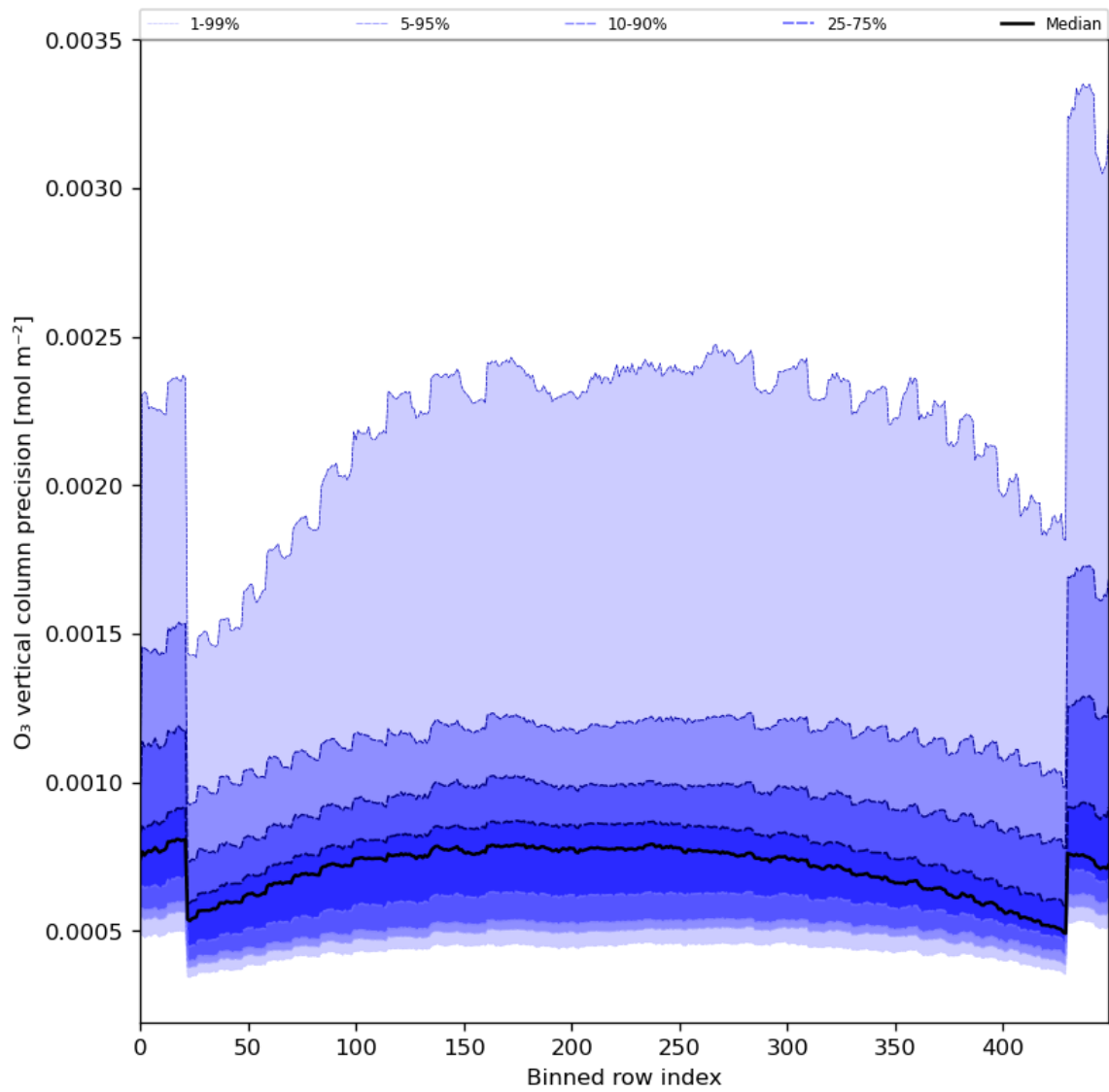
Figure 29: Along track statistics of “O 3 vertical column precision” for 2024-02-23 to 2024-02-25
