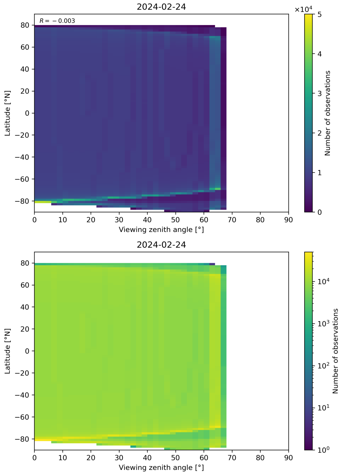
Figure 49: Scatter density plot of “Viewing zenith angle” against “Latitude” for 2024-02-23 to 2024-02-25.
