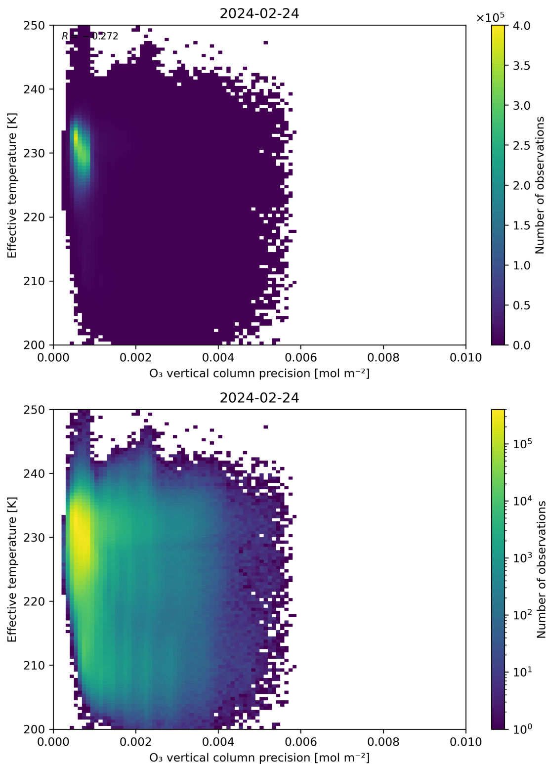
Figure 42: Scatter density plot of “O 3 vertical column precision” against “Effective temperature” for 2024-02-23 to 2024-02-25.
