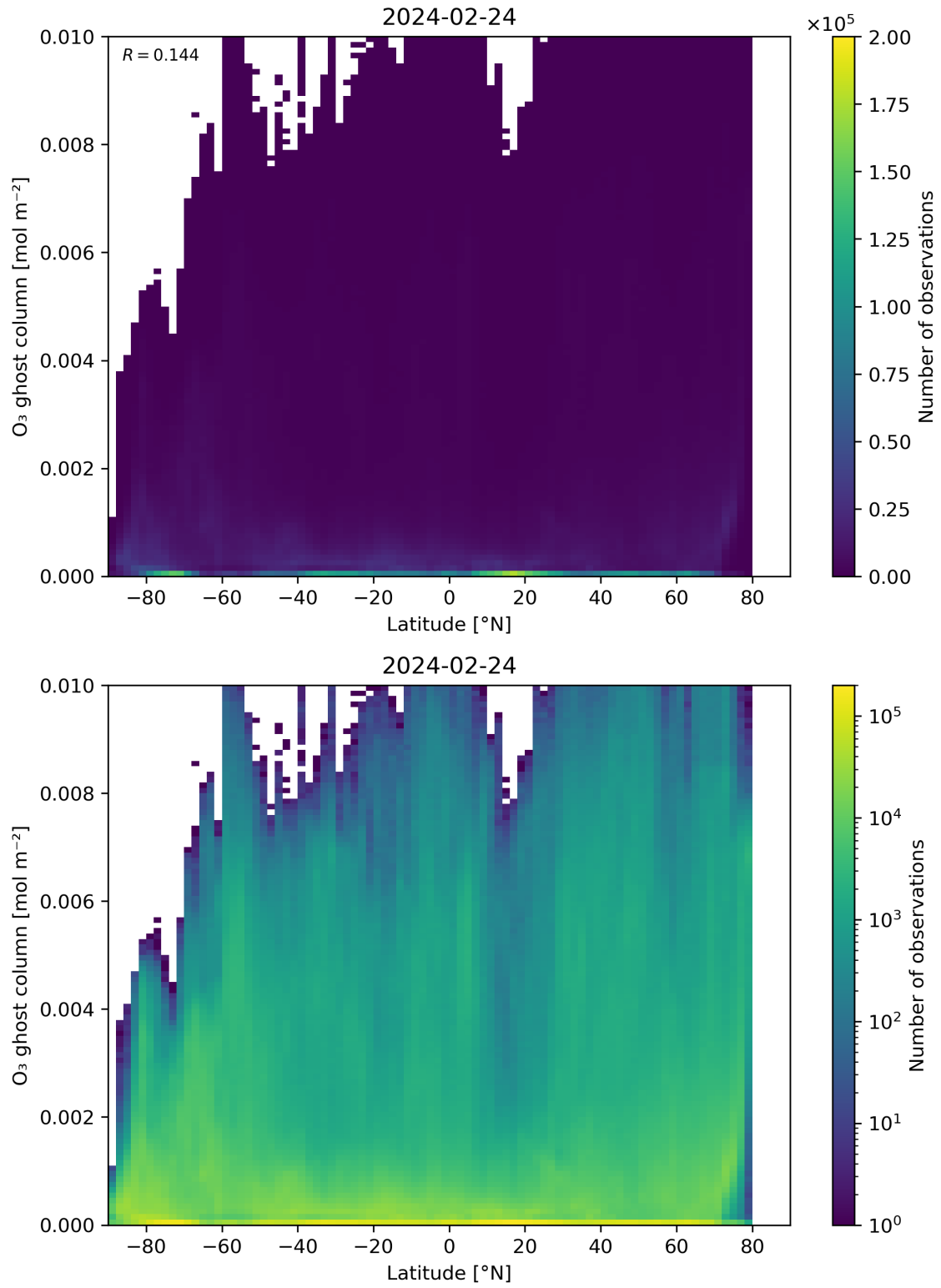
Figure 35: Scatter density plot of “Latitude” against “O 3 ghost column” for 2024-02-23 to 2024-02-25.
