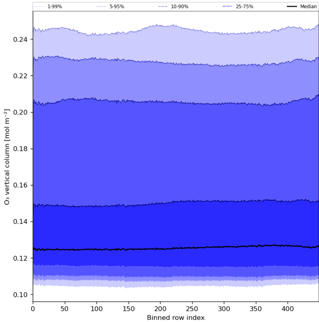
Figure 28: Along track statistics of “O 3 vertical column” for 2024-02-23 to 2024-02-25
