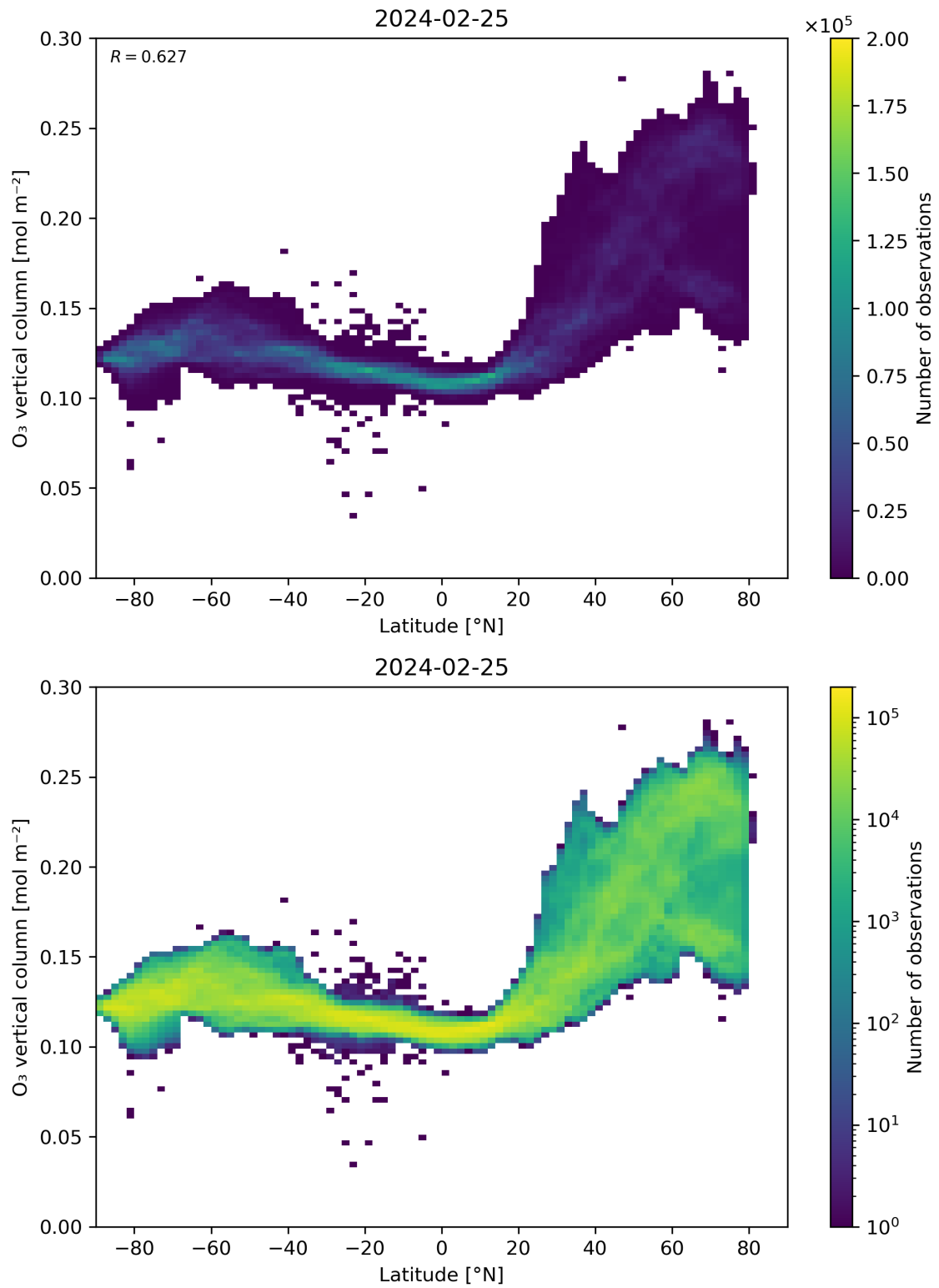
Figure 36: Scatter density plot of “Latitude” against “O 3 vertical column” for 2024-02-24 to 2024-02-26.
