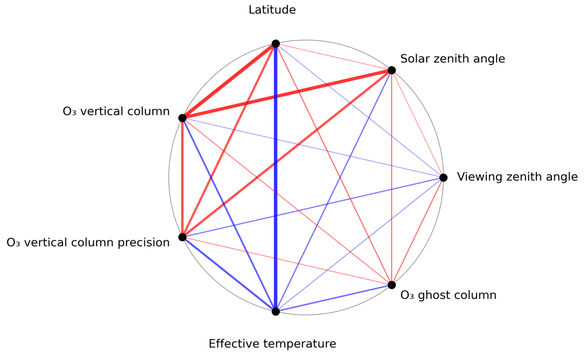
Figure 1: Map of correlation graph for 2024-02-24 to 2024-02-26.
