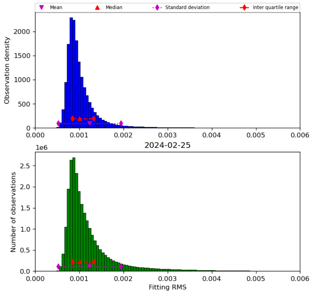
Figure 23: Histogram of “Fitting RMS” for 2024-02-24 to 2024-02-26
