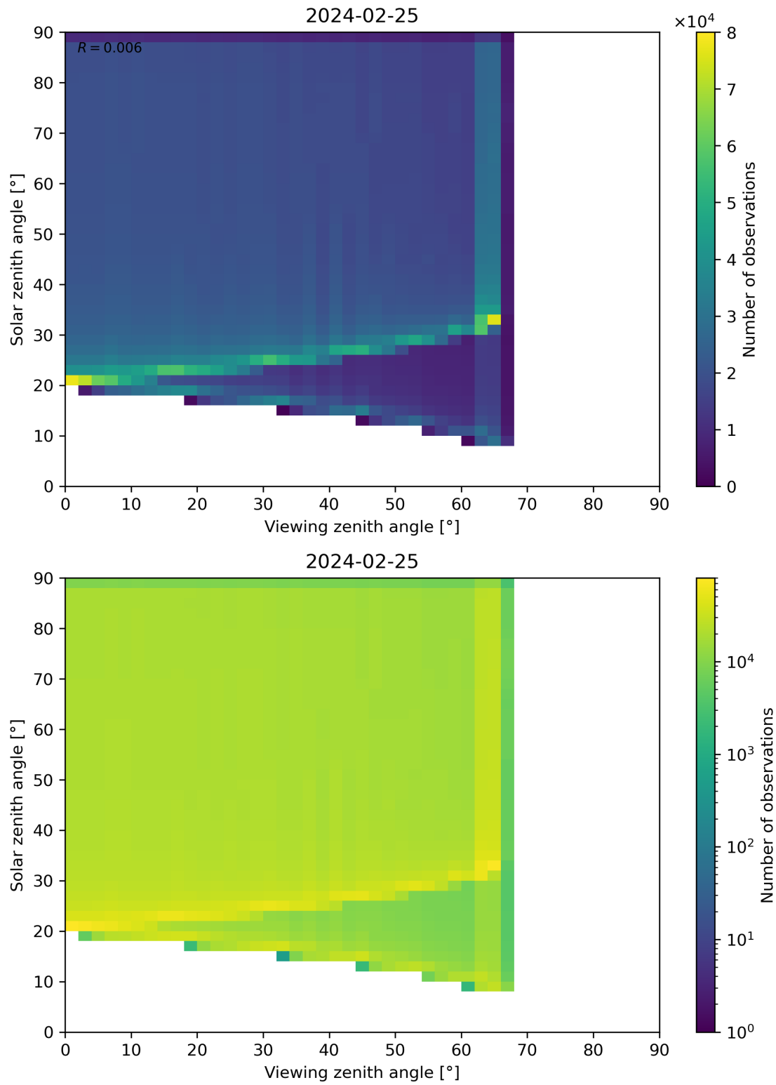
Figure 54: Scatter density plot of “Viewing zenith angle” against “Solar zenith angle” for 2024-02-24 to 2024-02-26.
