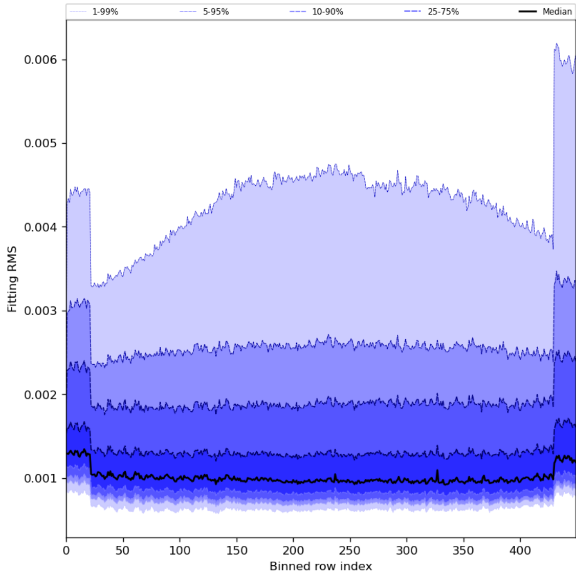
Figure 30: Along track statistics of “Fitting RMS” for 2024-02-24 to 2024-02-26
