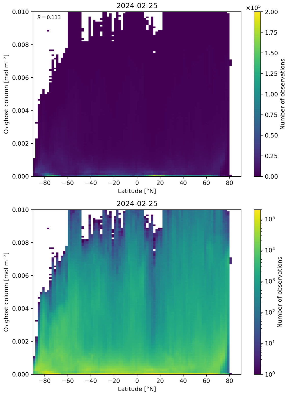
Figure 35: Scatter density plot of “Latitude” against “O 3 ghost column” for 2024-02-24 to 2024-02-26.
