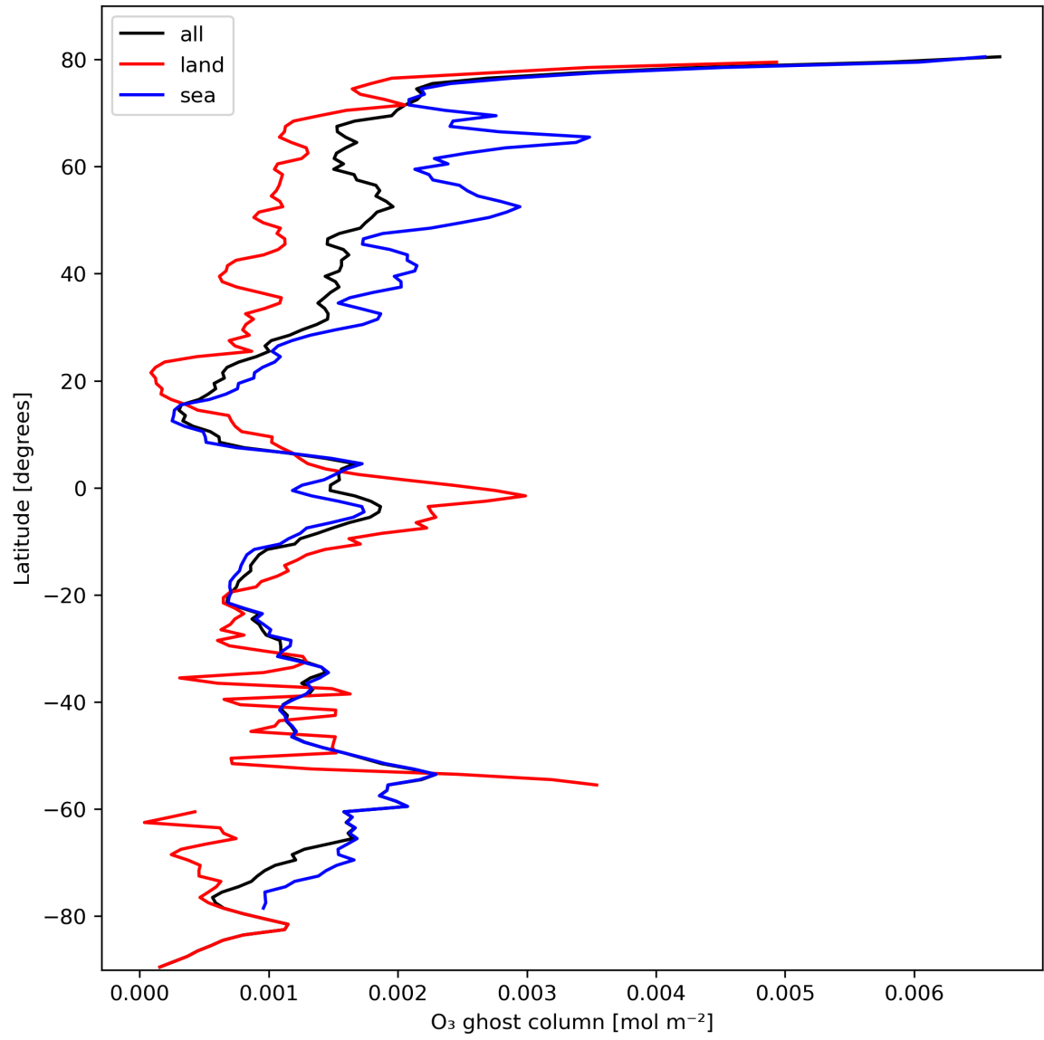
Figure 18: Zonal average of "O 3 ghost column" for 2024-02-24 to 2024-02-26.
