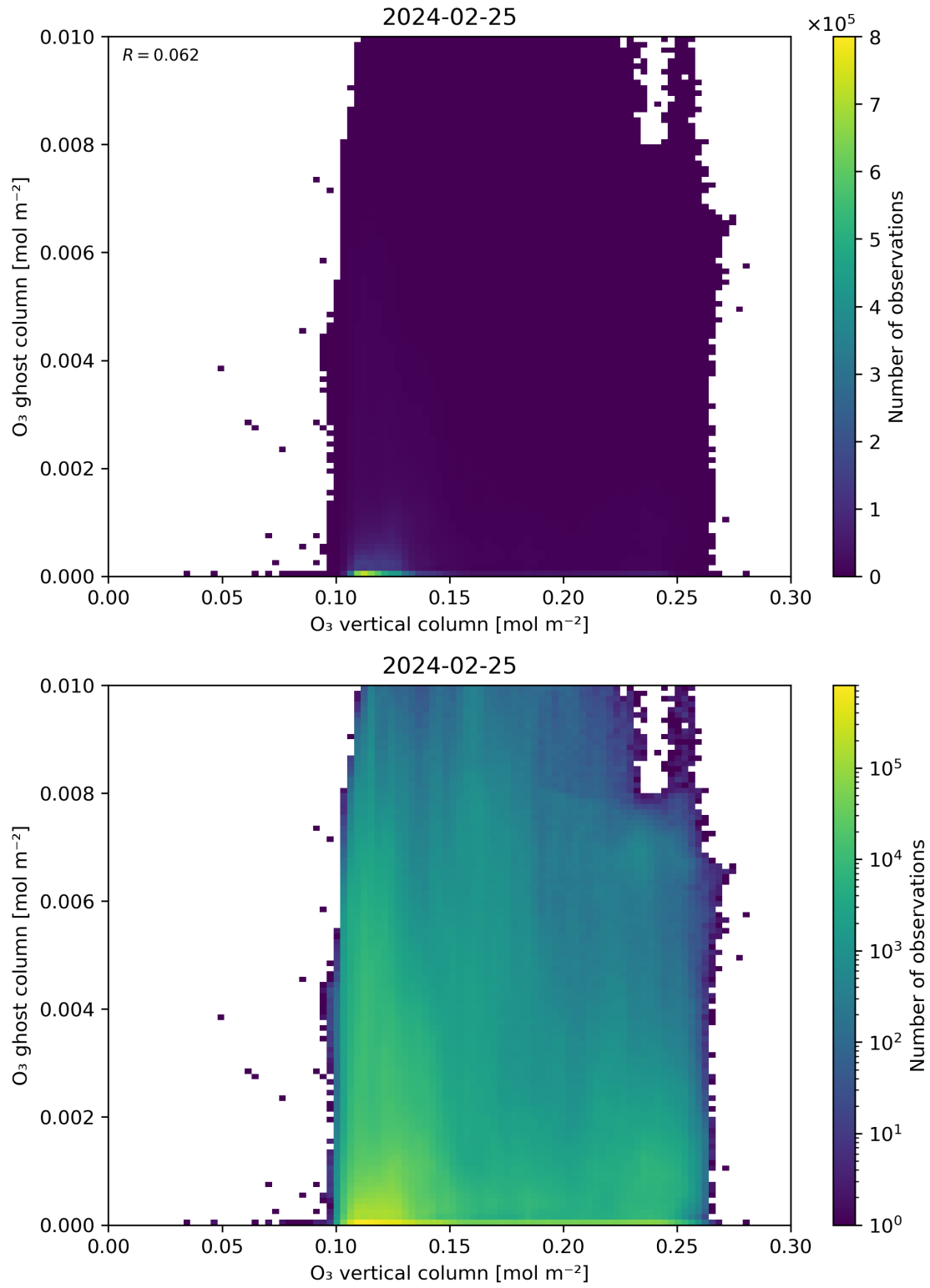
Figure 40: Scatter density plot of “O 3 vertical column” against “O 3 ghost column” for 2024-02-24 to 2024-02-26.
