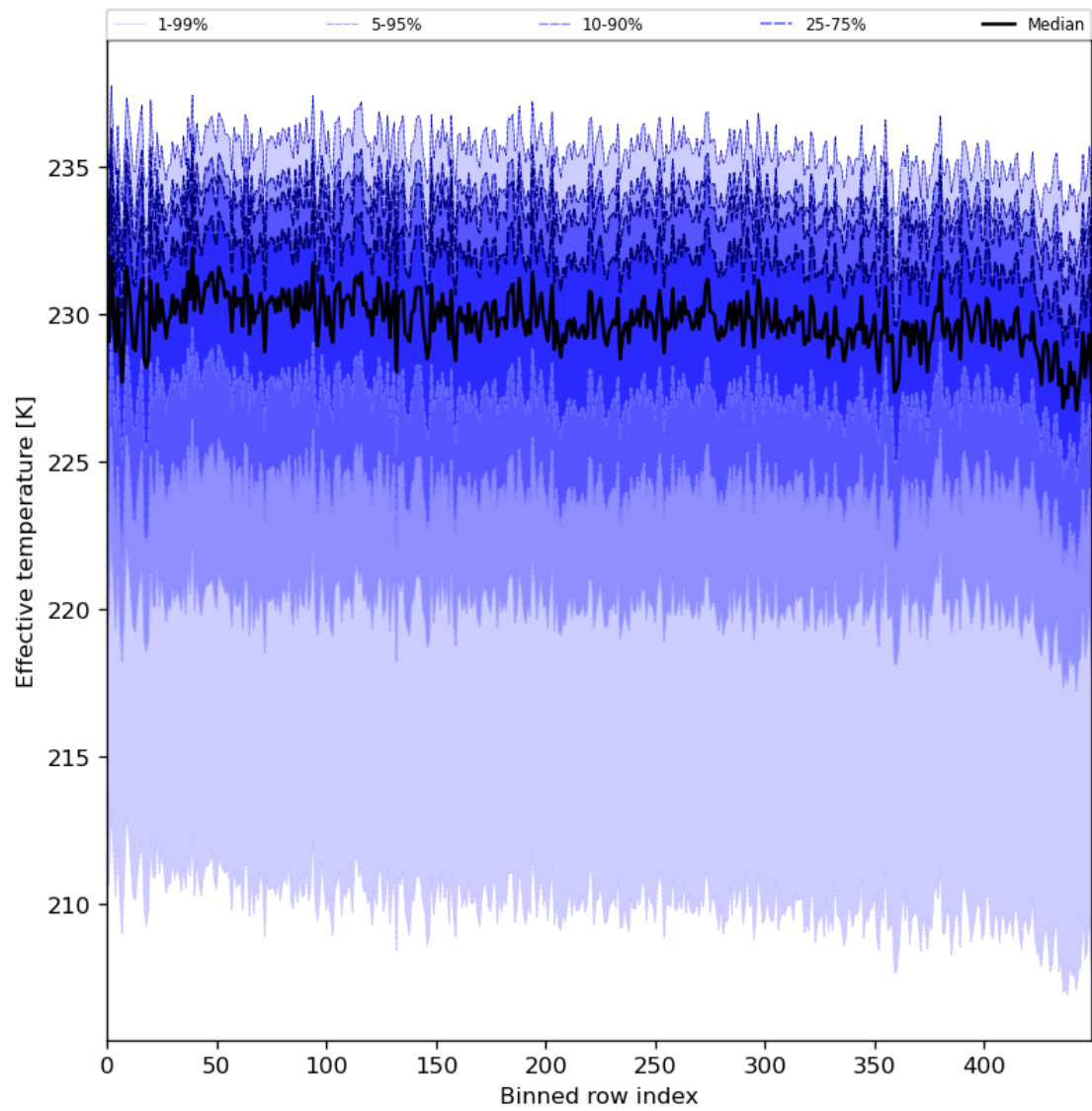
Figure 31: Along track statistics of “Effective temperature” for 2024-02-24 to 2024-02-26
