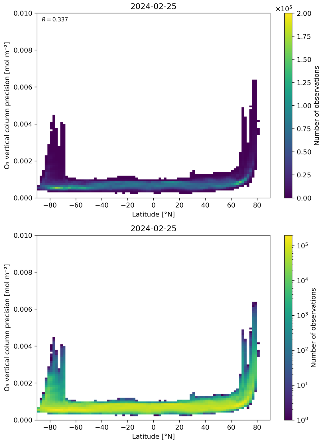
Figure 37: Scatter density plot of “Latitude” against “O 3 vertical column precision” for 2024-02-24 to 2024-02-26.
