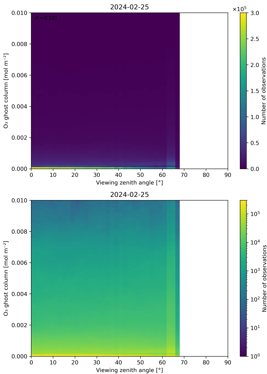
Figure 51: Scatter density plot of “Viewing zenith angle” against “O 3 ghost column” for 2024-02-24 to 2024-02-26.
