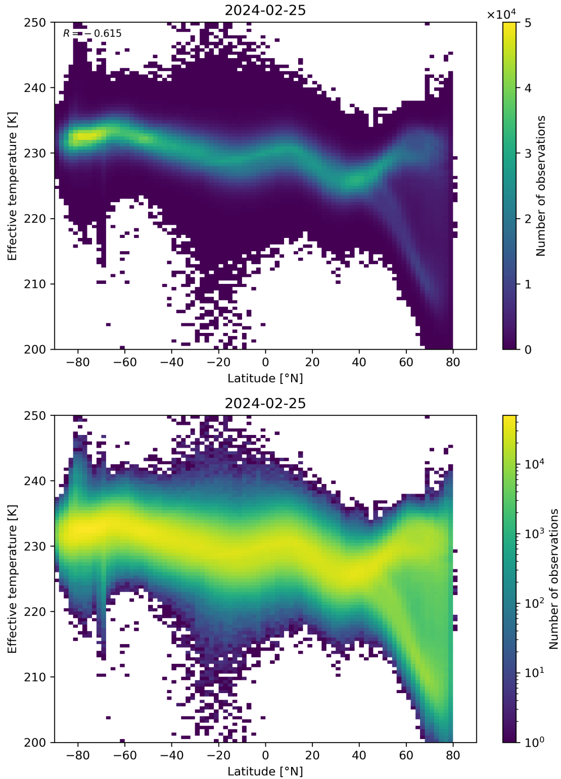
Figure 34: Scatter density plot of “Latitude” against “Effective temperature” for 2024-02-24 to 2024-02-26.
