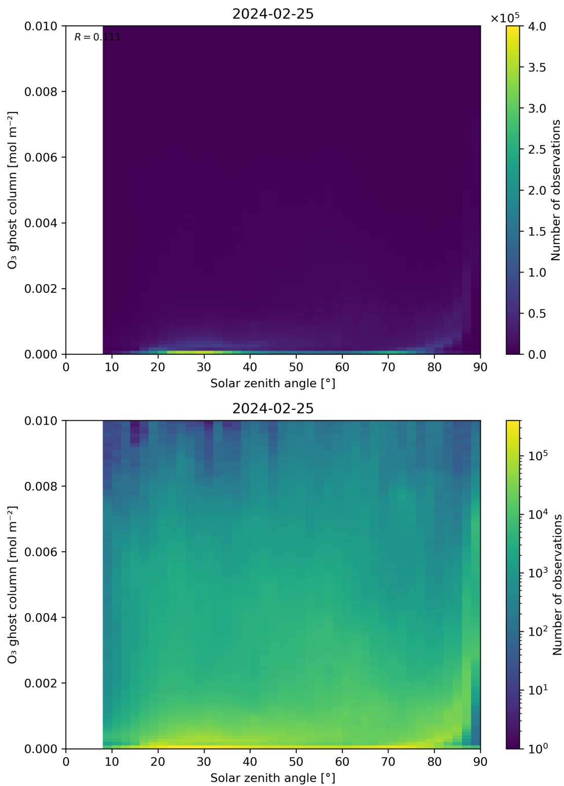
Figure 46: Scatter density plot of “Solar zenith angle” against “O 3 ghost column” for 2024-02-24 to 2024-02-26.
