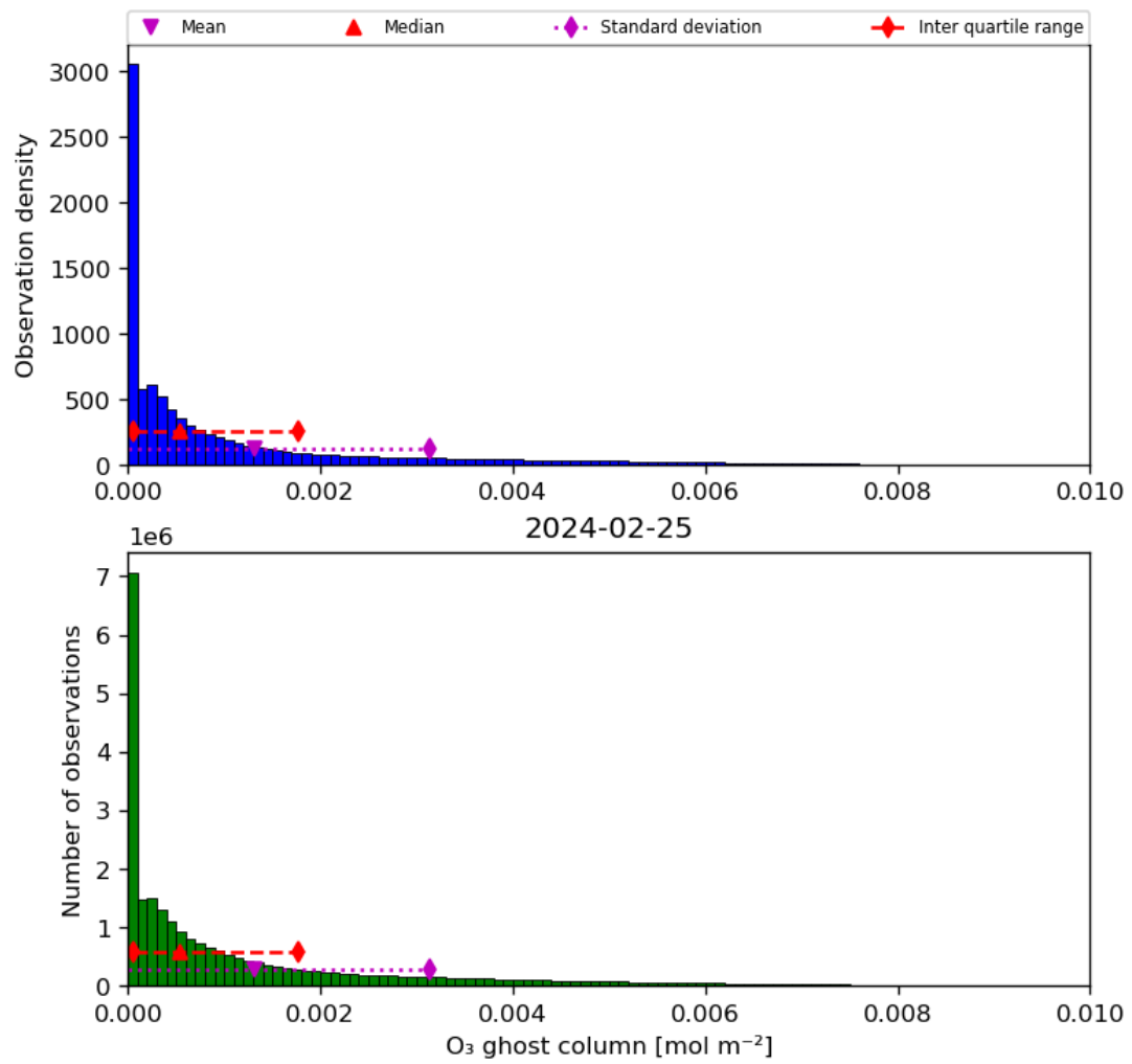
Figure 25: Histogram of “O 3 ghost column” for 2024-02-24 to 2024-02-26
