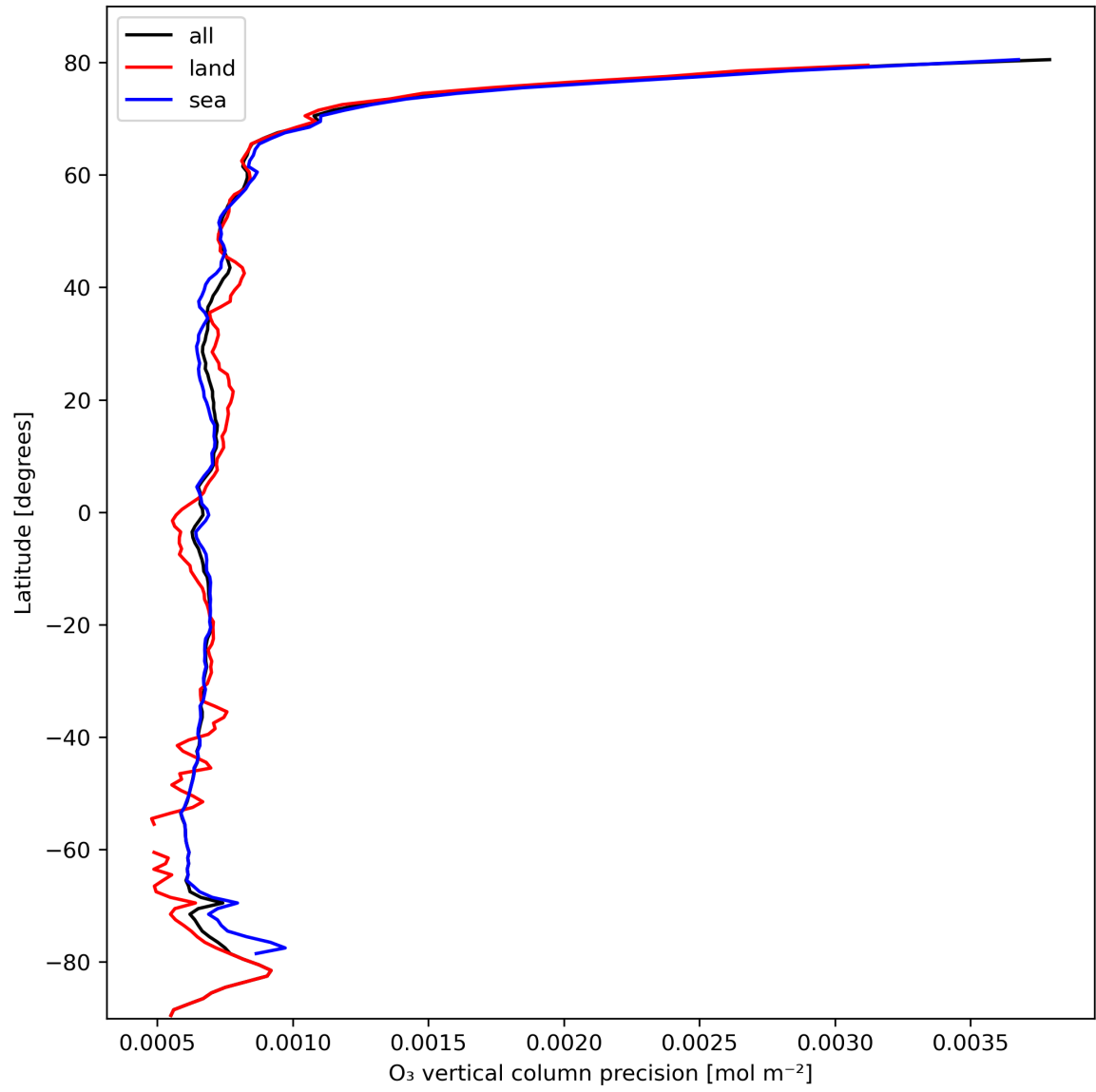
Figure 15: Zonal average of "O 3 vertical column precision" for 2024-02-24 to 2024-02-26.
