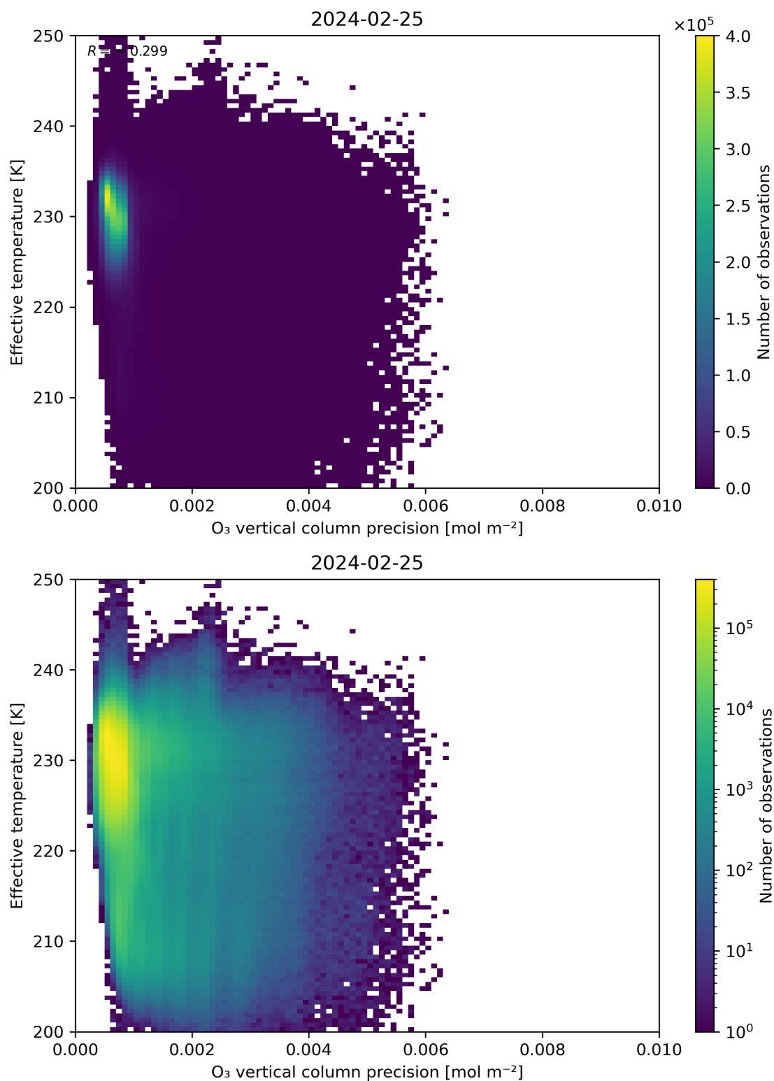
Figure 42: Scatter density plot of “ O_3 vertical column precision” against “Effective temperature” for 2024-02-24 to 2024-02-26.
