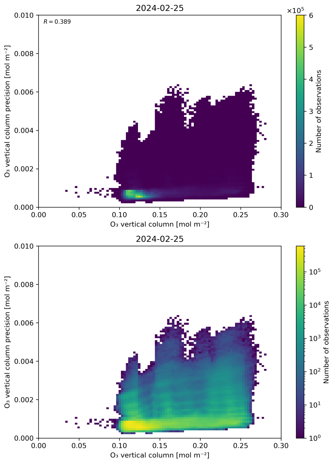
Figure 41: Scatter density plot of “O 3 vertical column” against “O 3 vertical column precision” for 2024-02-24 to 2024-02-26.
