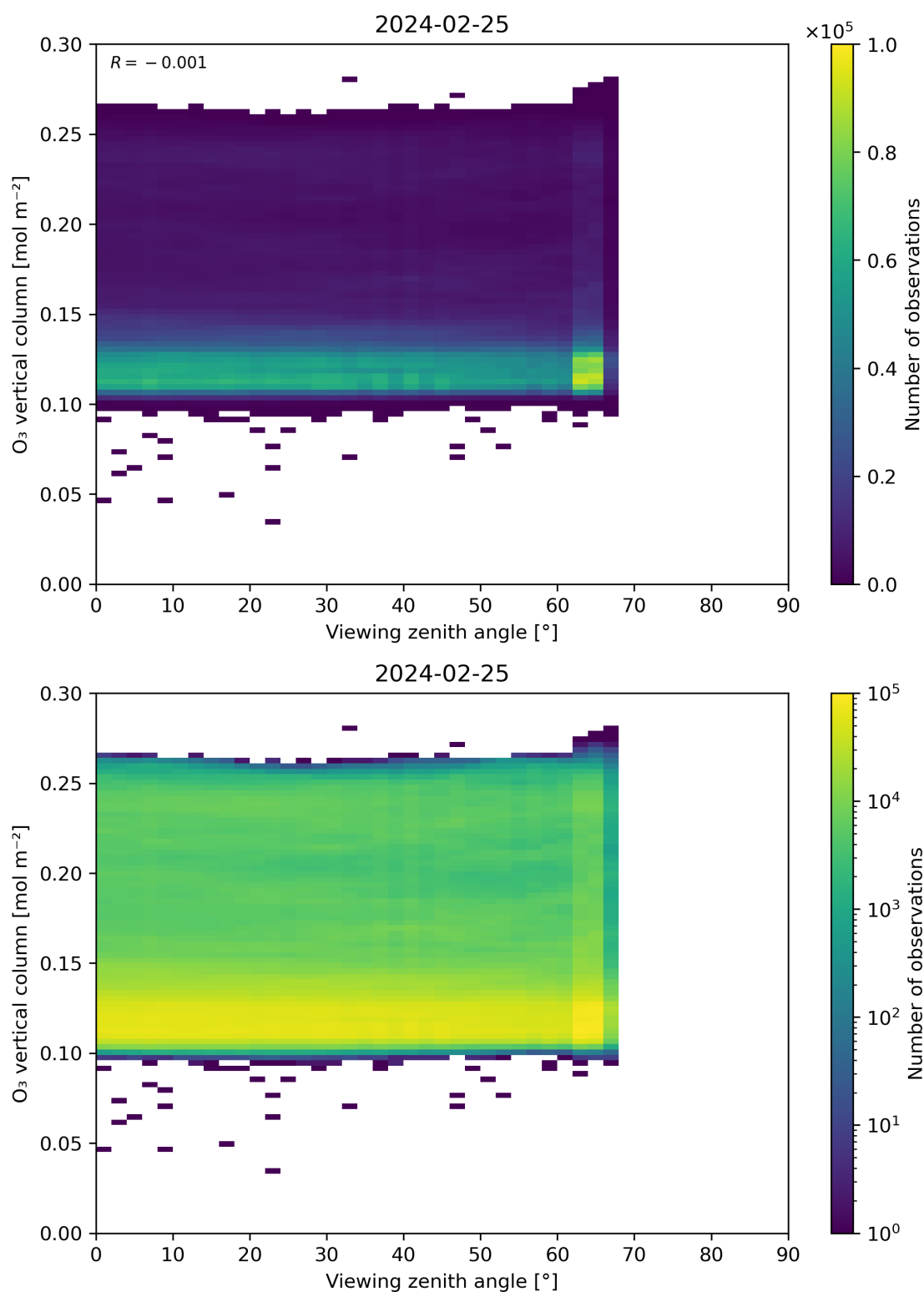
Figure 52: Scatter density plot of “Viewing zenith angle” against “O 3 vertical column” for 2024-02-24 to 2024-02-26.
