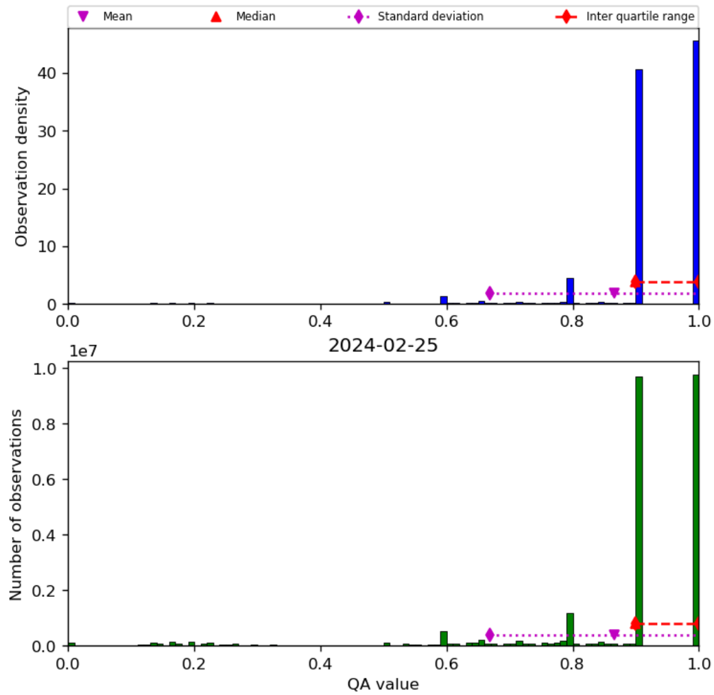
Figure 20: Histogram of “QA value” for 2024-02-24 to 2024-02-26
