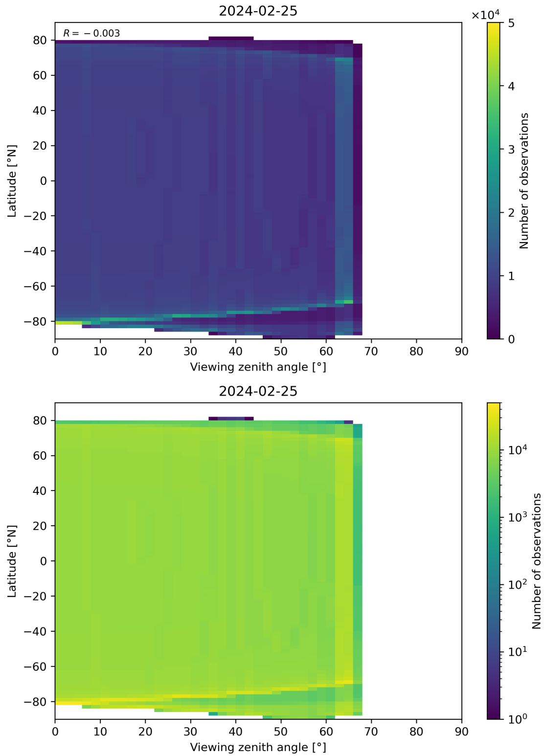
Figure 49: Scatter density plot of “Viewing zenith angle” against “Latitude” for 2024-02-24 to 2024-02-26.
