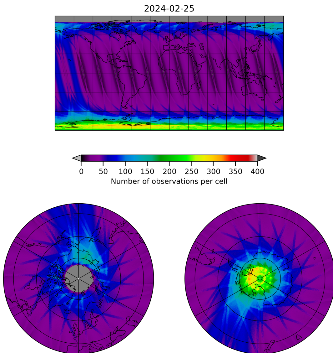
Figure 12: Map of the number of observations for 2024-02-24 to 2024-02-26
