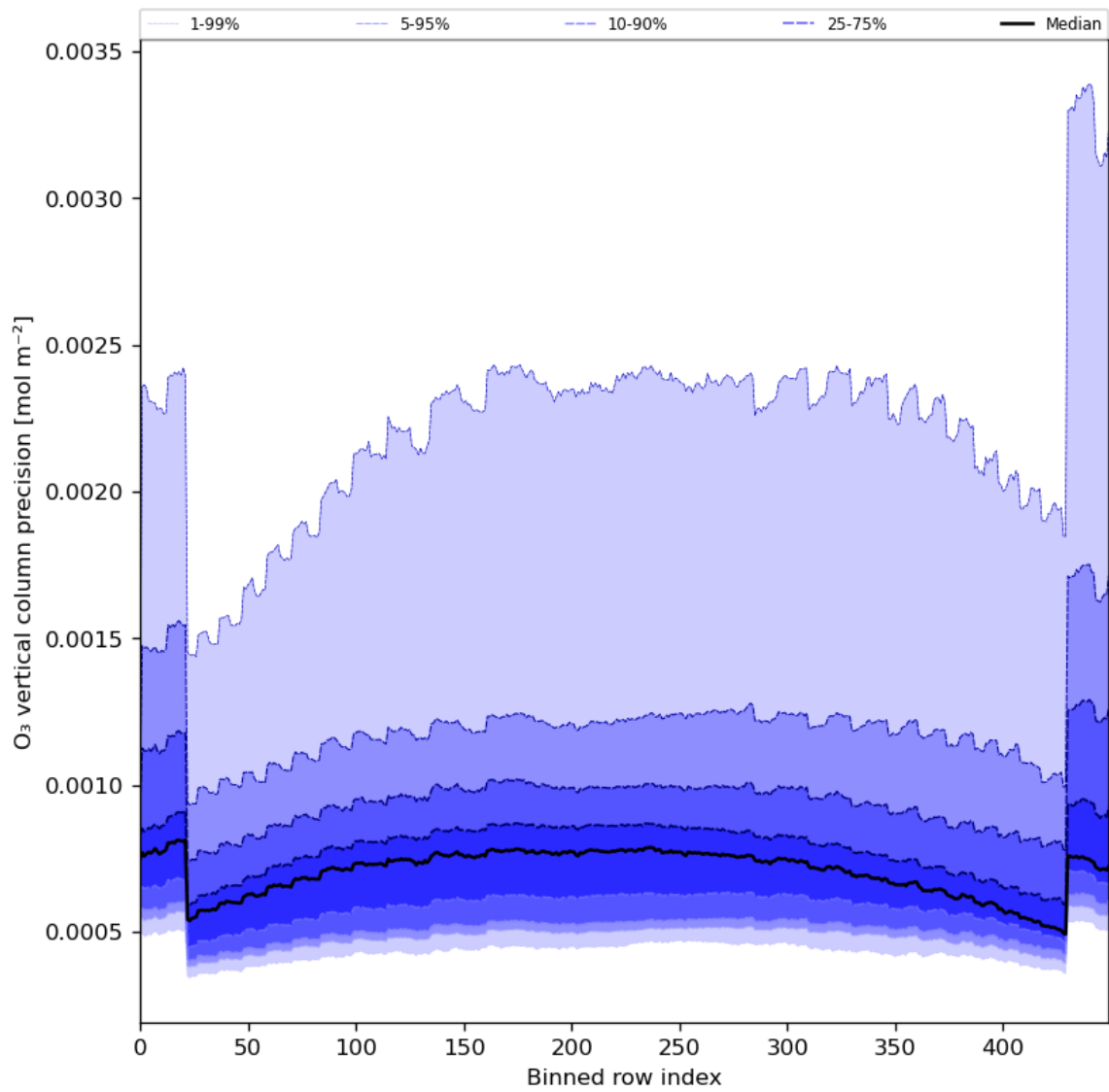
Figure 29: Along track statistics of “O 3 vertical column precision” for 2024-02-24 to 2024-02-26
