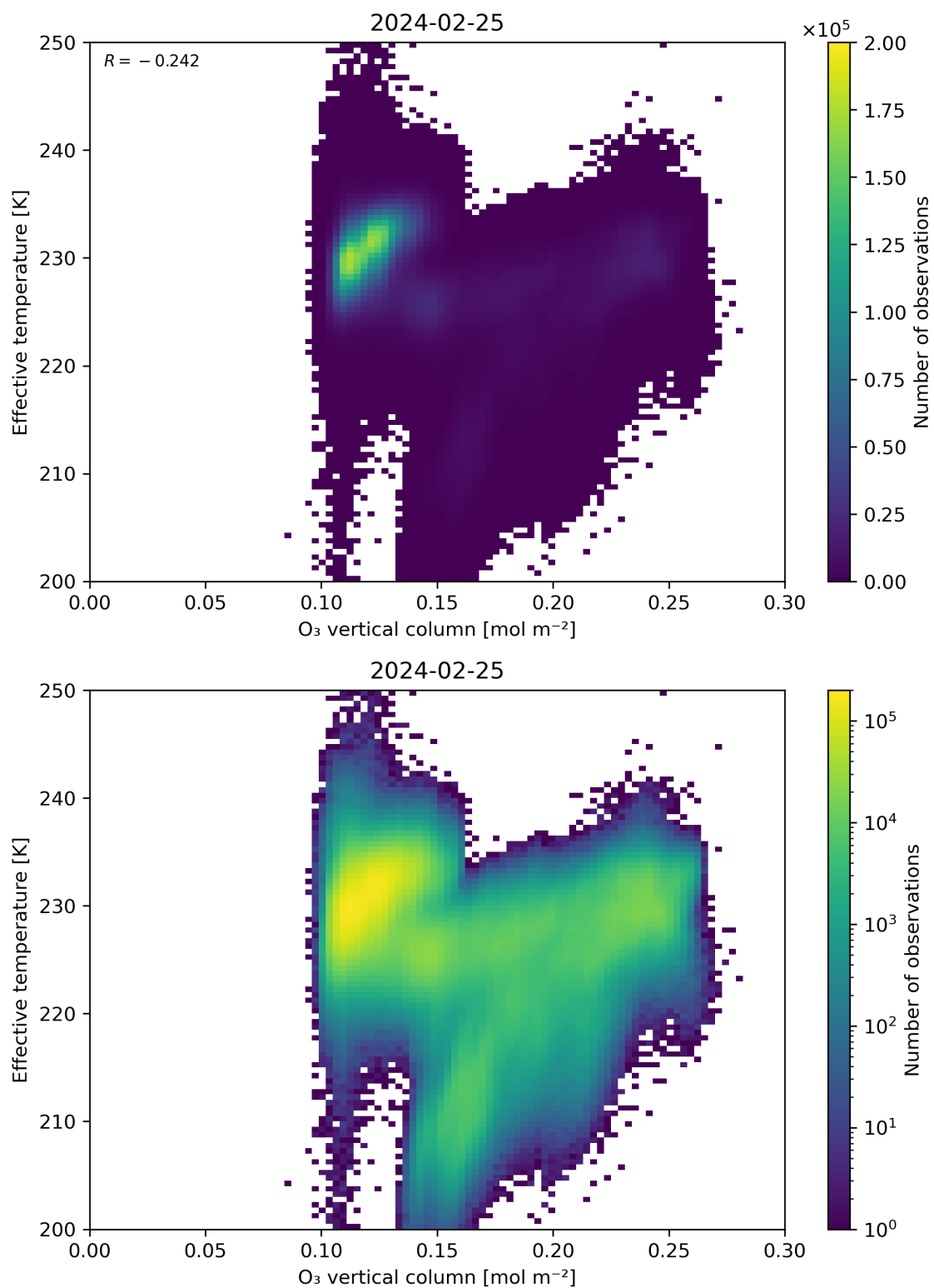
Figure 39: Scatter density plot of “O 3 vertical column” against “Effective temperature” for 2024-02-24 to 2024-02-26.
