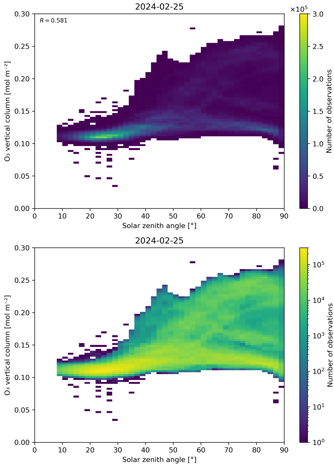
Figure 47: Scatter density plot of “Solar zenith angle” against “O 3 vertical column” for 2024-02-24 to 2024-02-26.
