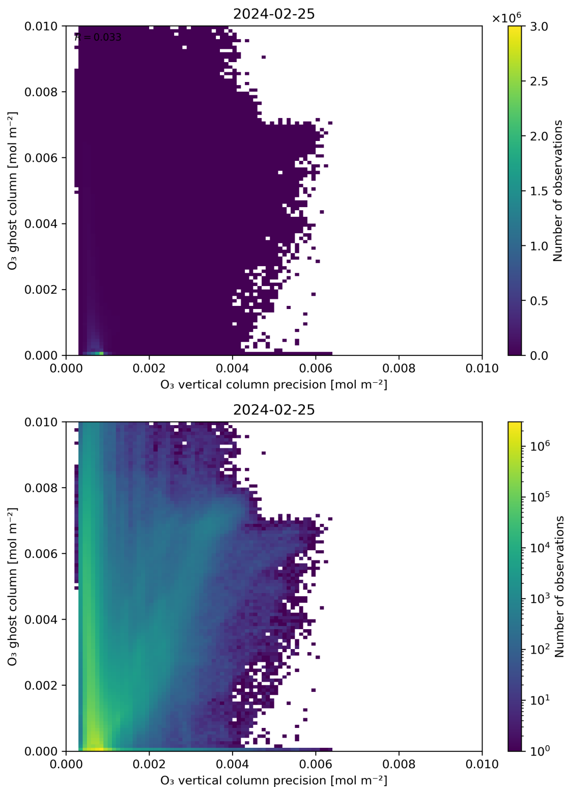
Figure 43: Scatter density plot of “O 3 vertical column precision” against “O 3 ghost column” for 2024-02-24 to 2024-02-26.
