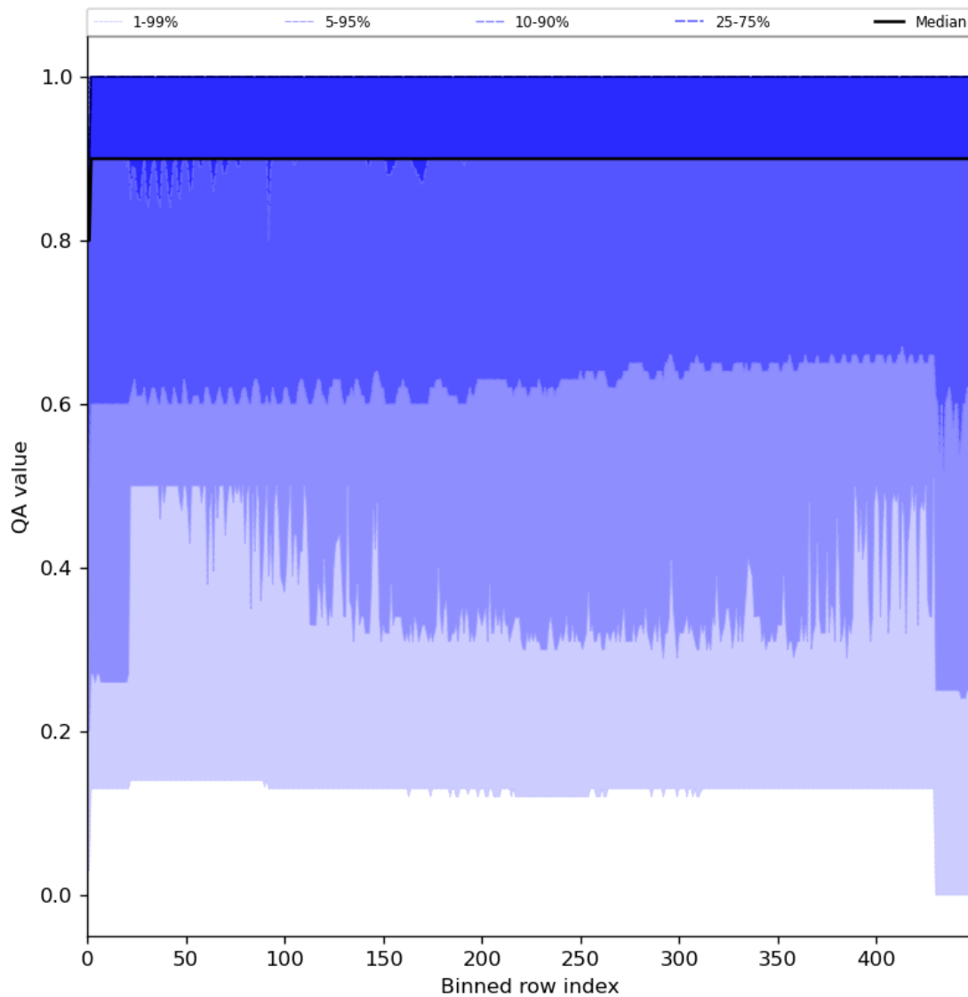
Figure 27: Along track statistics of “QA value” for 2024-02-24 to 2024-02-26
