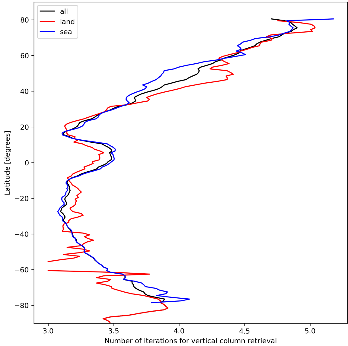
Figure 19: Zonal average of “Number of iterations for vertical column retrieval” for 2024-02-24 to 2024-02-26.
