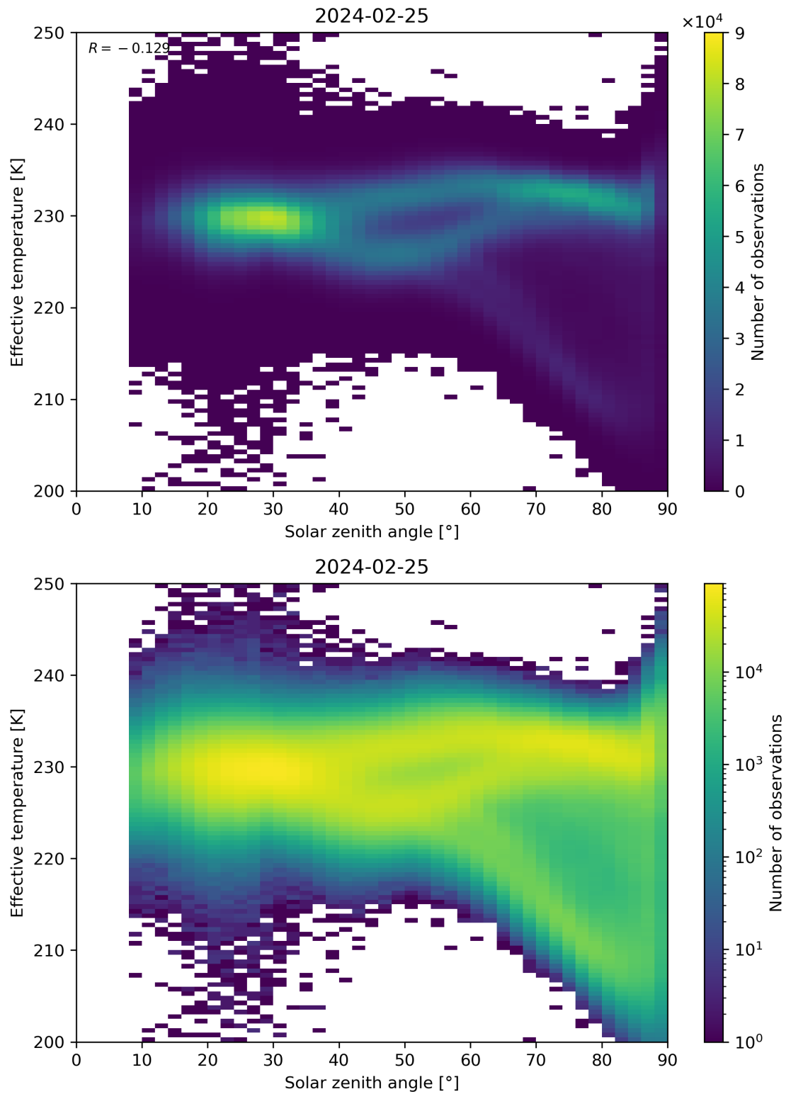
Figure 45: Scatter density plot of “Solar zenith angle” against “Effective temperature” for 2024-02-24 to 2024-02-26.
