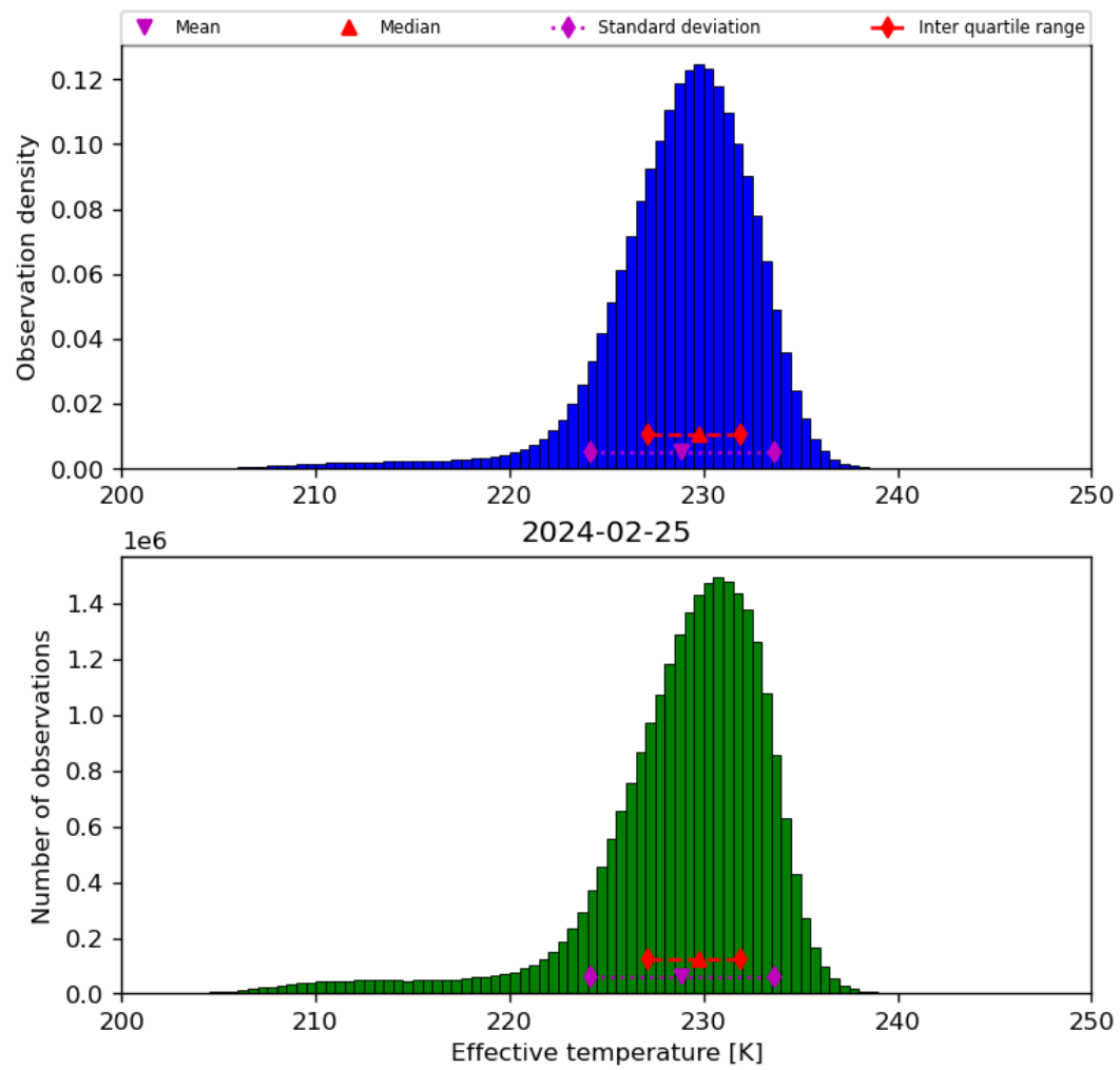
Figure 24: Histogram of “Effective temperature” for 2024-02-24 to 2024-02-26
