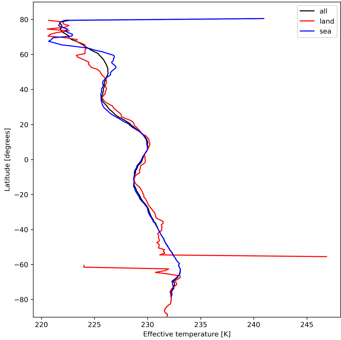
Figure 17: Zonal average of "Effective temperature" for 2024-02-24 to 2024-02-26.
