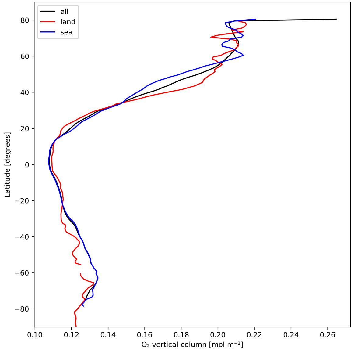
Figure 14: Zonal average of “O 3 vertical column” for 2024-02-24 to 2024-02-26.
