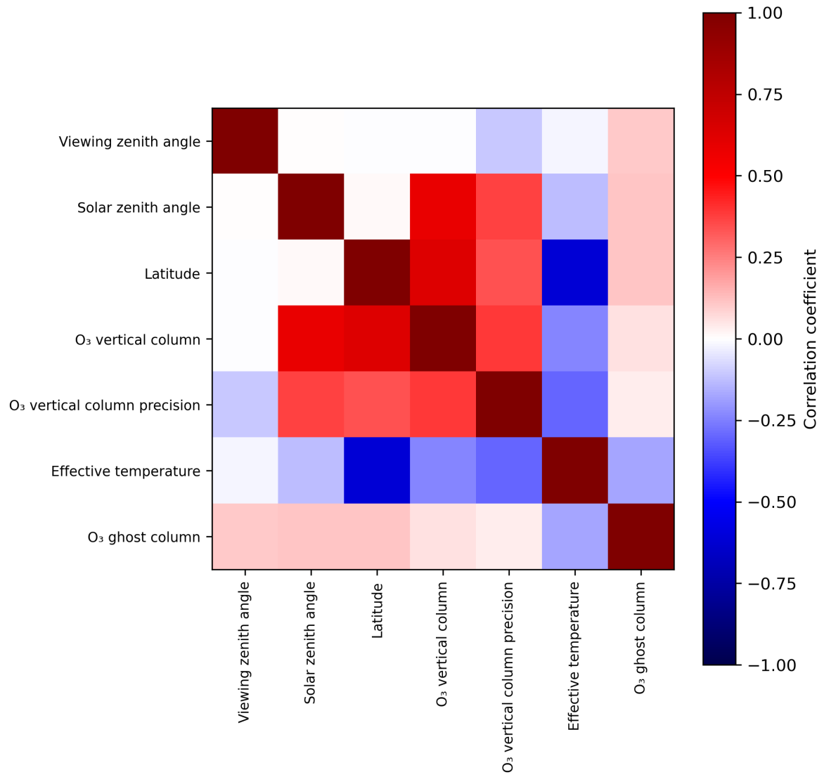
Figure 2: Map of correlation matrix for 2024-02-24 to 2024-02-26.
