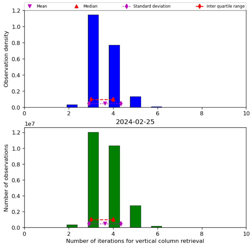
Figure 26: Histogram of “Number of iterations for vertical column retrieval” for 2024-02-24 to 2024-02-26
