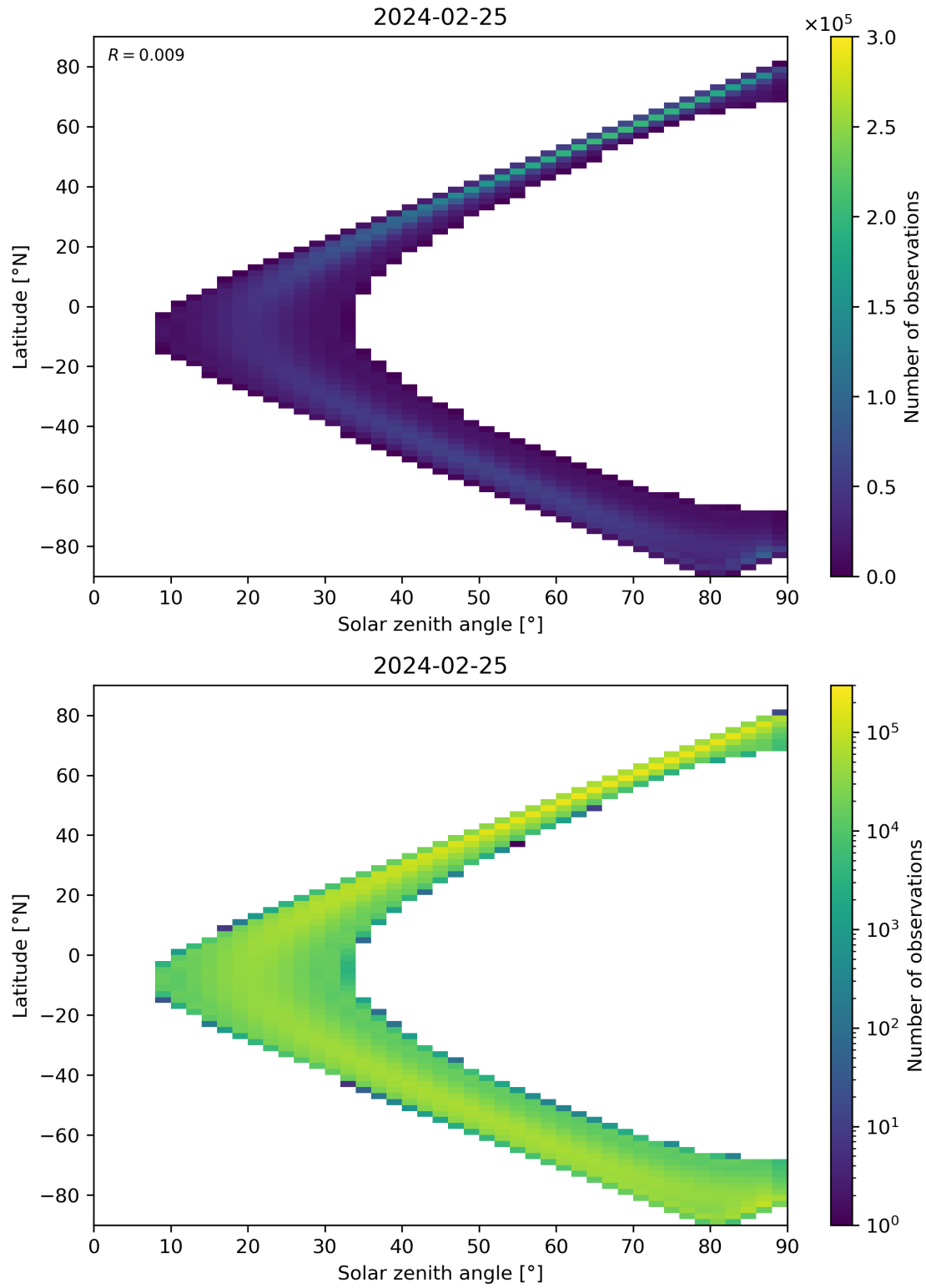
Figure 44: Scatter density plot of “Solar zenith angle” against “Latitude” for 2024-02-24 to 2024-02-26.
