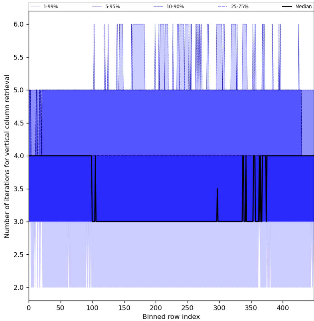
Figure 33: Along track statistics of “Number of iterations for vertical column retrieval” for 2024-02-24 to 2024-02-26
