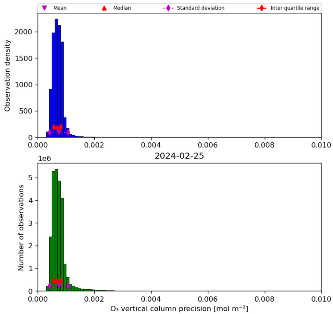
Figure 22: Histogram of “O 3 vertical column precision” for 2024-02-24 to 2024-02-26
