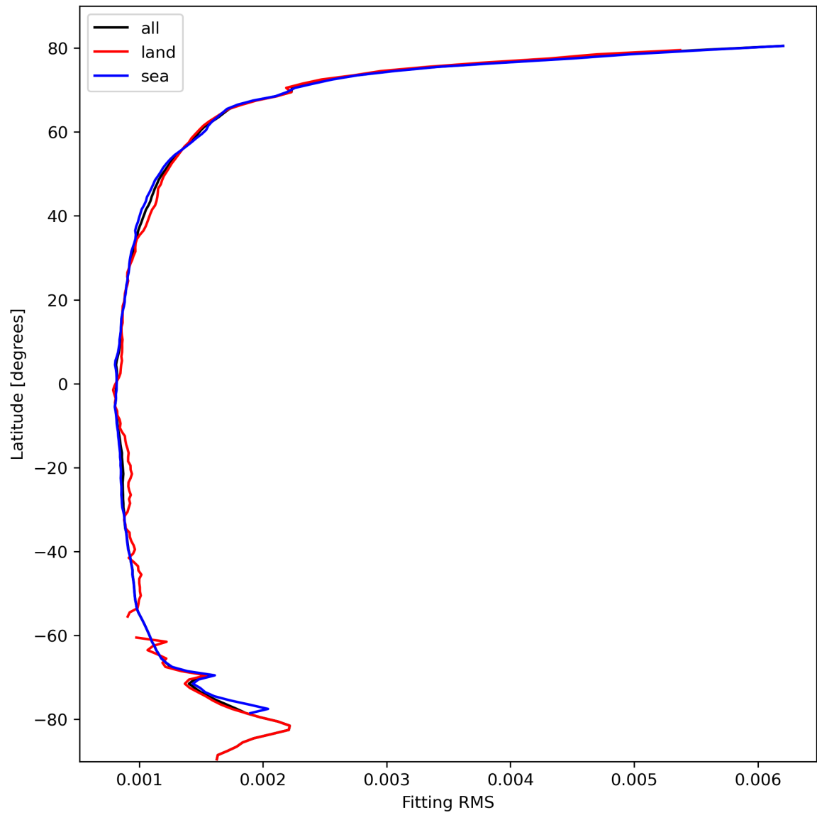
Figure 16: Zonal average of “Fitting RMS” for 2024-02-24 to 2024-02-26.
