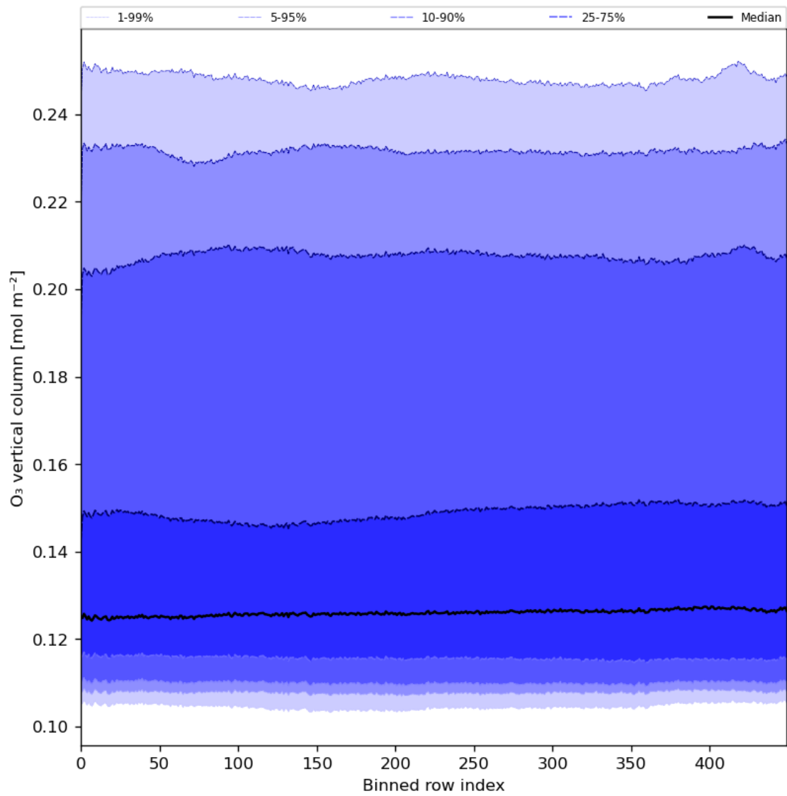
Figure 28: Along track statistics of “O 3 vertical column” for 2024-02-24 to 2024-02-26
