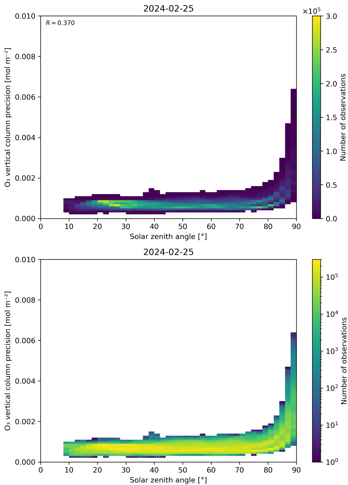
Figure 48: Scatter density plot of “Solar zenith angle” against “O 3 vertical column precision” for 2024-02-24 to 2024-02-26.
