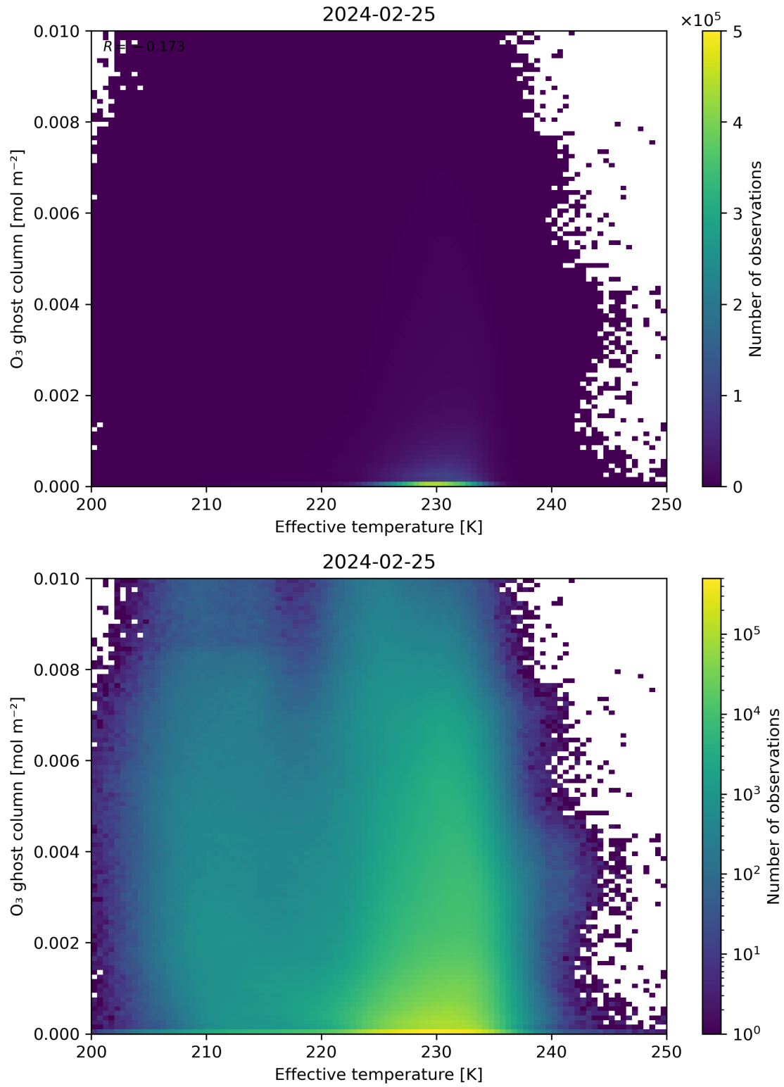
Figure 38: Scatter density plot of “Effective temperature” against “O 3 ghost column” for 2024-02-24 to 2024-02-26.
