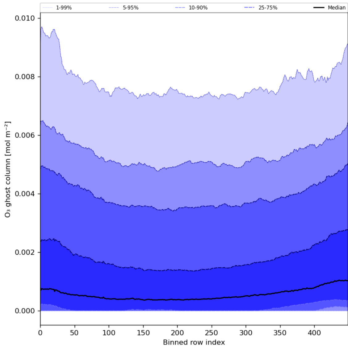
Figure 32: Along track statistics of “O 3 ghost column” for 2024-02-24 to 2024-02-26
