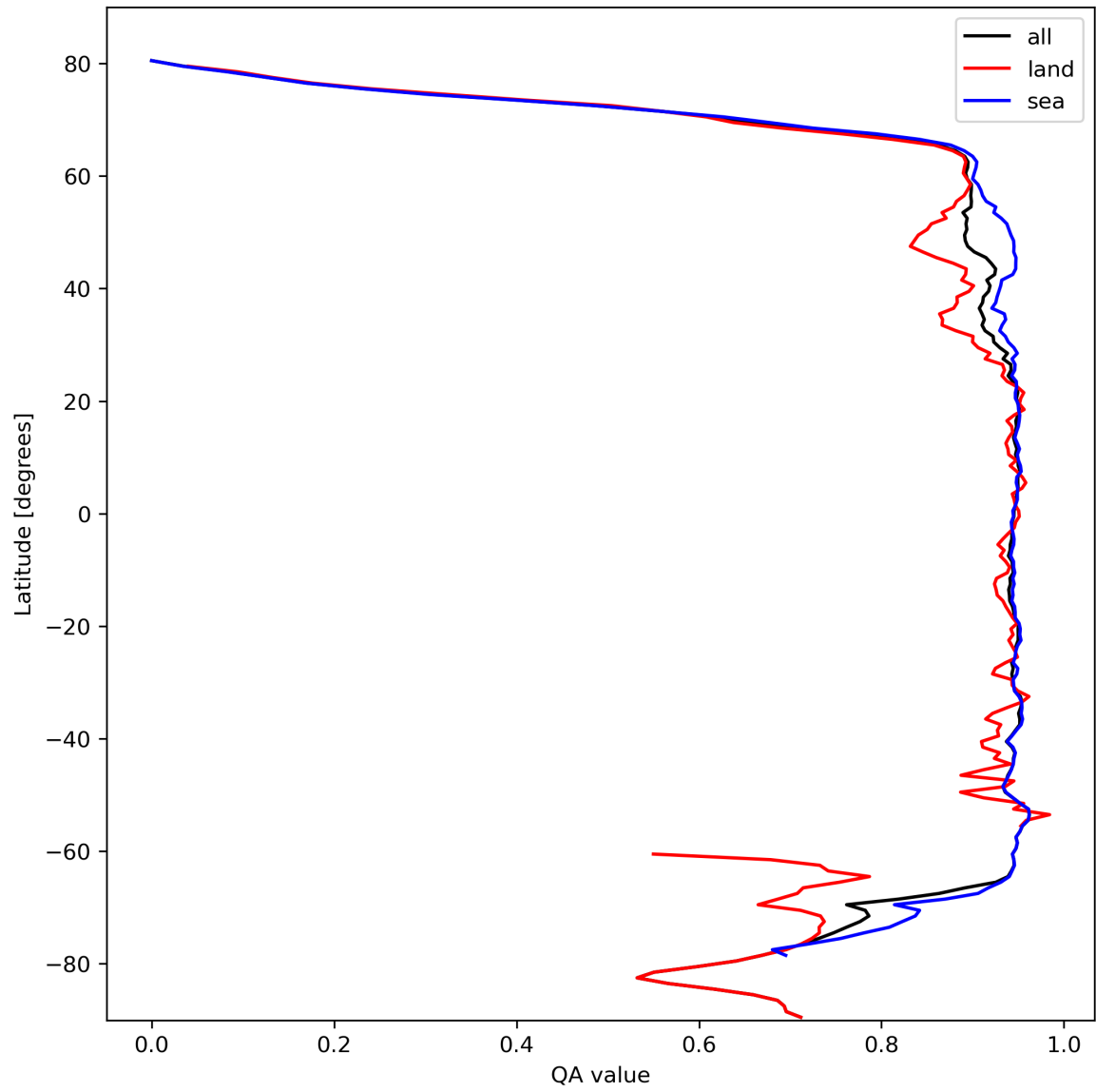
Figure 13: Zonal average of “QA value” for 2024-02-24 to 2024-02-26.
