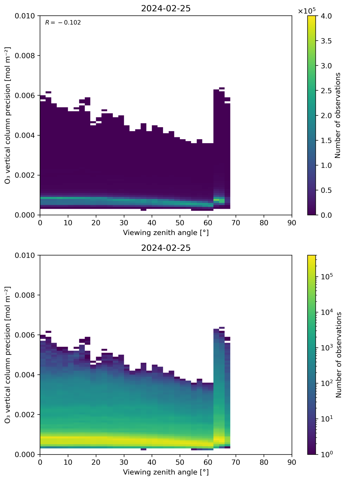
Figure 53: Scatter density plot of “Viewing zenith angle” against “O 3 vertical column precision” for 2024-02-24 to 2024-02-26.
