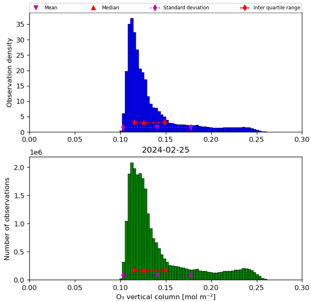
Figure 21: Histogram of “O 3 vertical column” for 2024-02-24 to 2024-02-26
