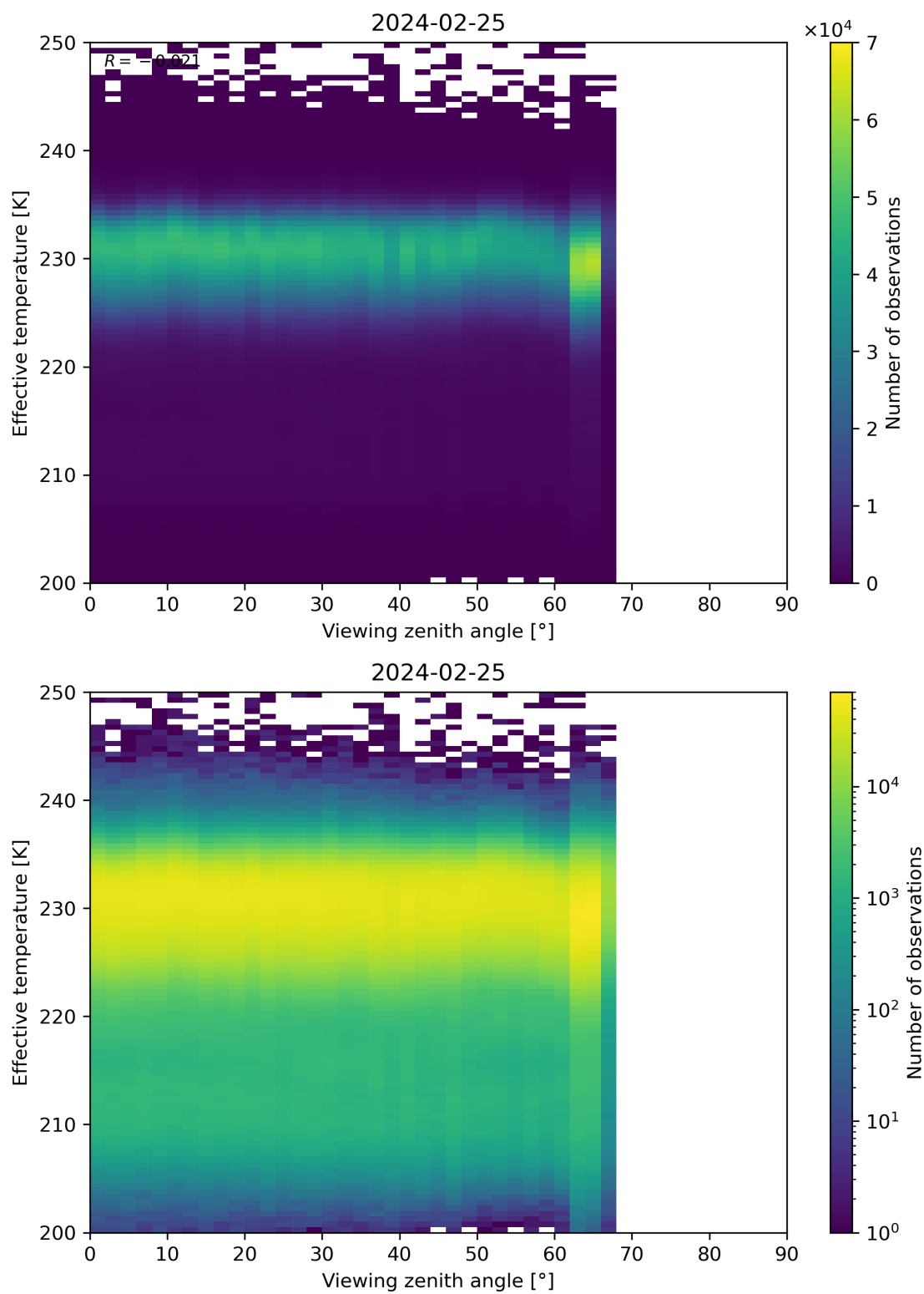
Figure 50: Scatter density plot of “Viewing zenith angle” against “Effective temperature” for 2024-02-24 to 2024-02-26.
