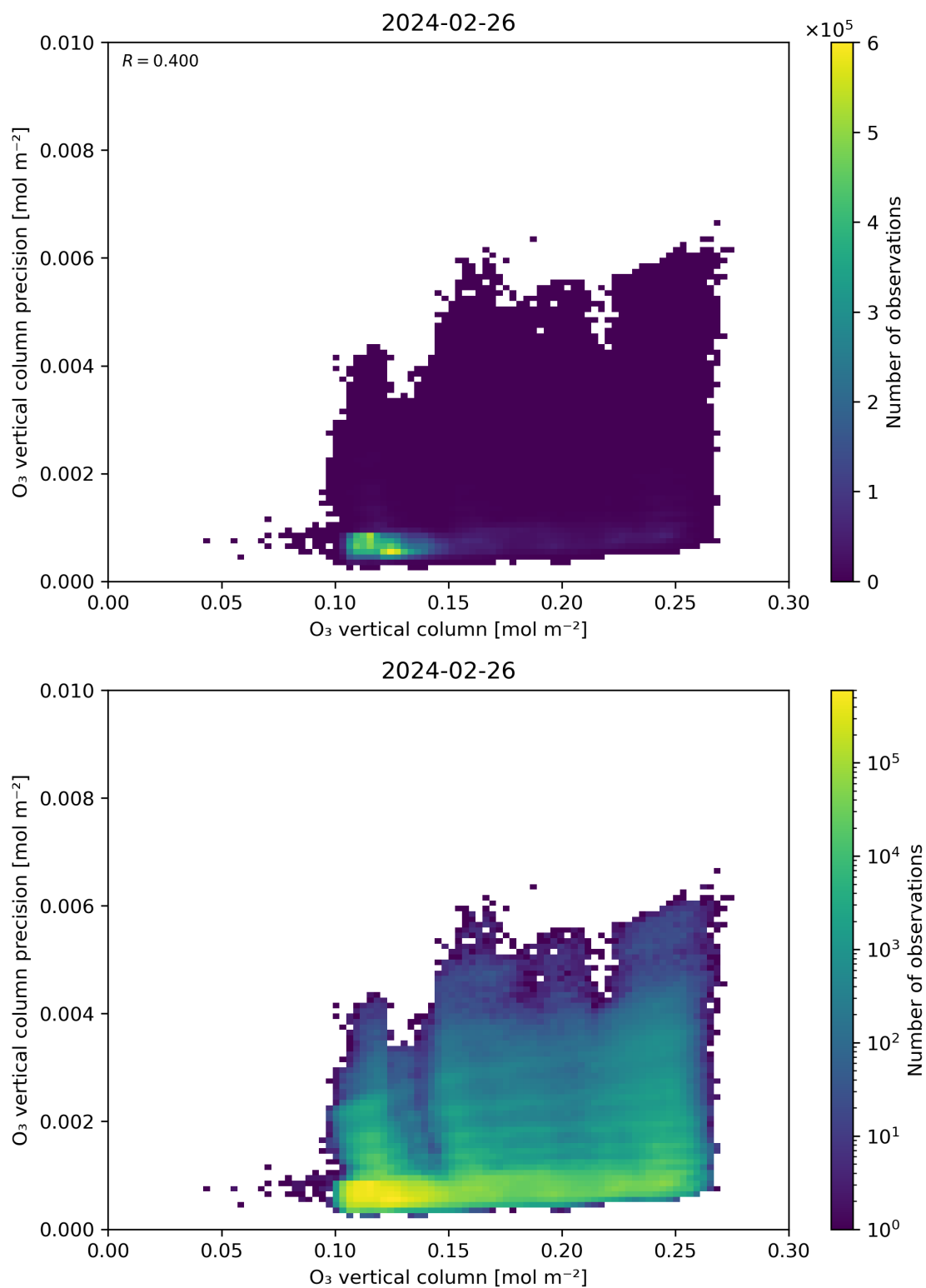
Figure 41: Scatter density plot of “O 3 vertical column” against “O 3 vertical column precision” for 2024-02-25 to 2024-02-27.
