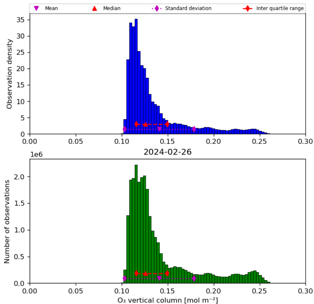
Figure 21: Histogram of “O 3 vertical column” for 2024-02-25 to 2024-02-27
