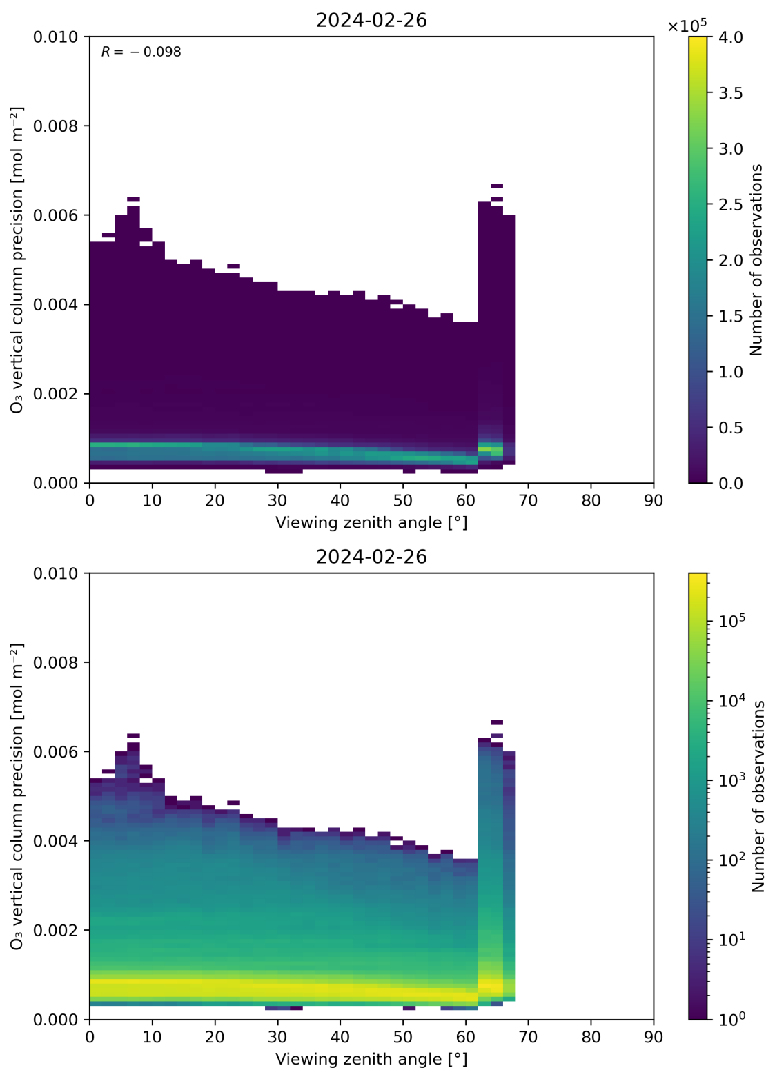
Figure 53: Scatter density plot of “Viewing zenith angle” against “O 3 vertical column precision” for 2024-02-25 to 2024-02-27.
