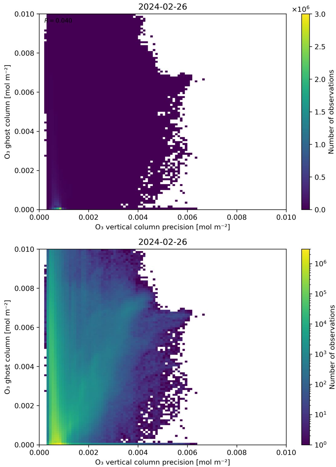
Figure 43: Scatter density plot of “ \text{O}_3 vertical column precision” against “ \text{O}_3 ghost column” for 2024-02-25 to 2024-02-27.
