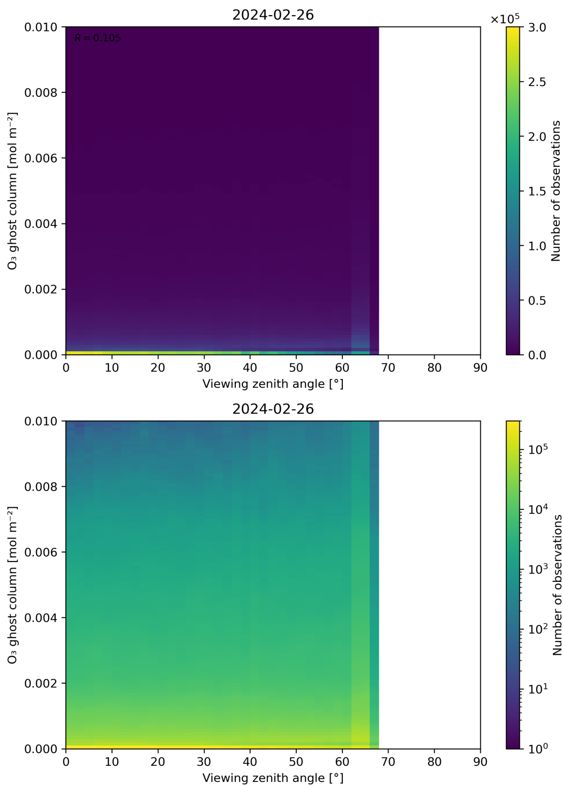
Figure 51: Scatter density plot of “Viewing zenith angle” against “O 3 ghost column” for 2024-02-25 to 2024-02-27.
