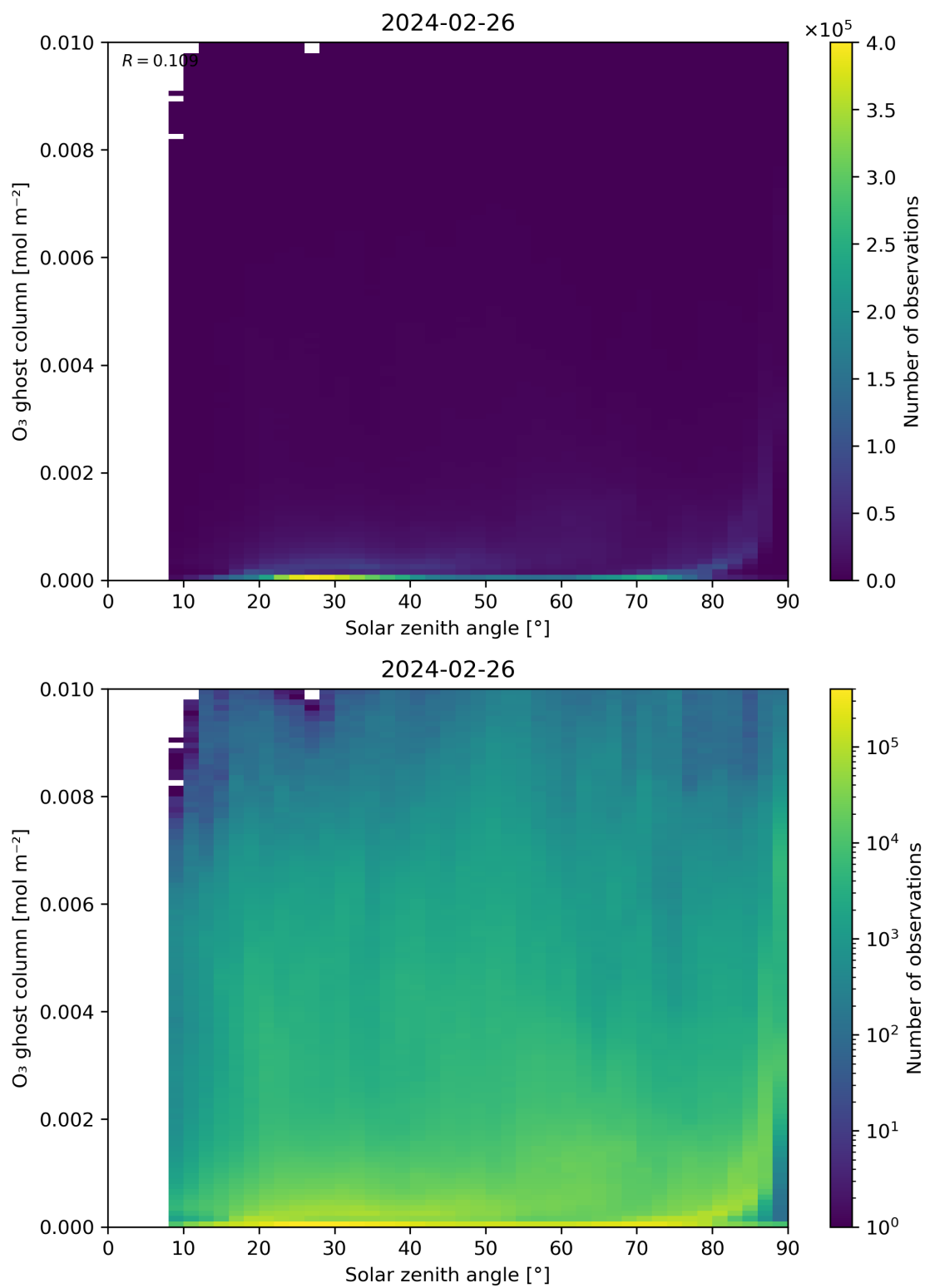
Figure 46: Scatter density plot of “Solar zenith angle” against “O 3 ghost column” for 2024-02-25 to 2024-02-27.
