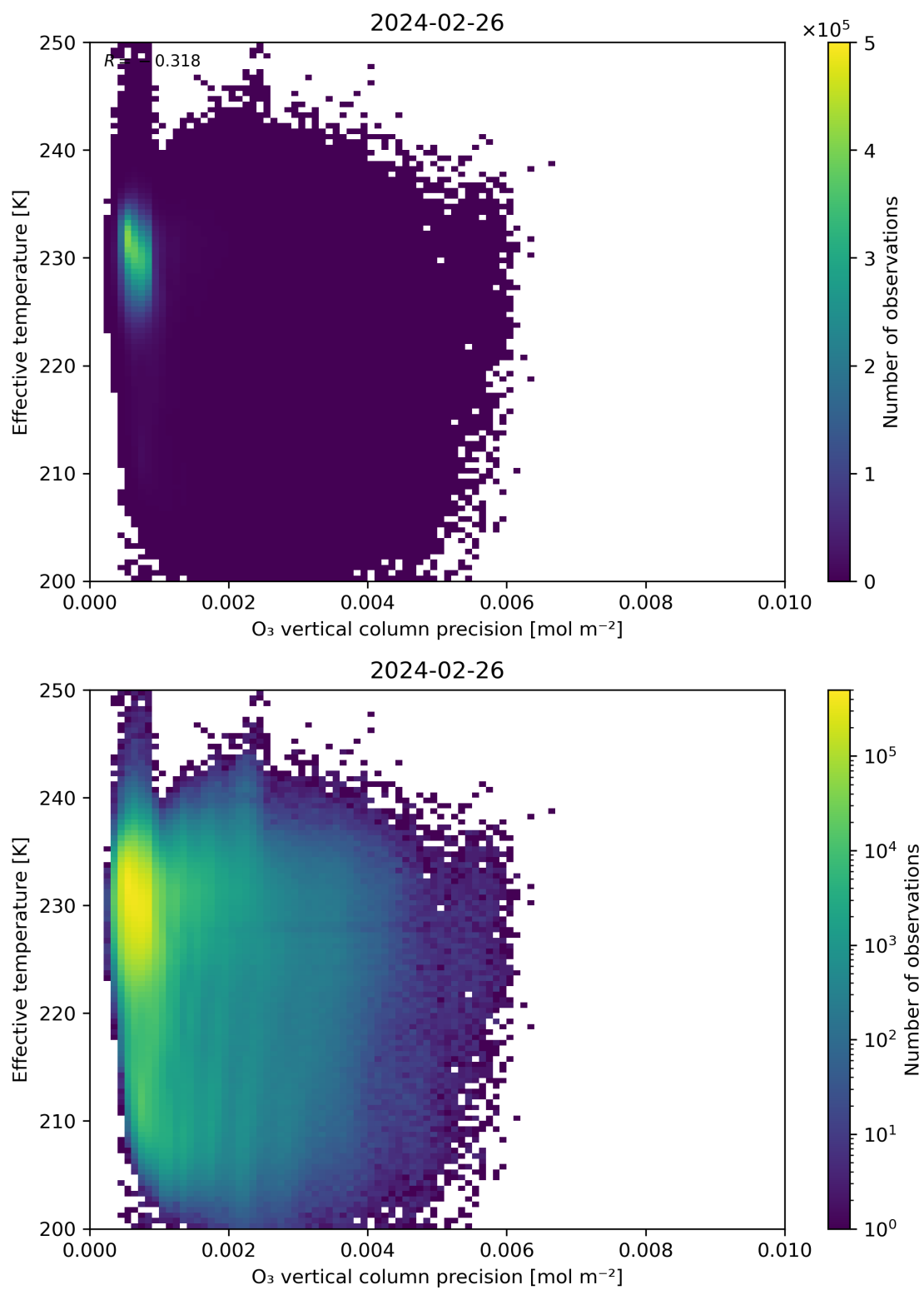
Figure 42: Scatter density plot of “O 3 vertical column precision” against “Effective temperature” for 2024-02-25 to 2024-02-27.
