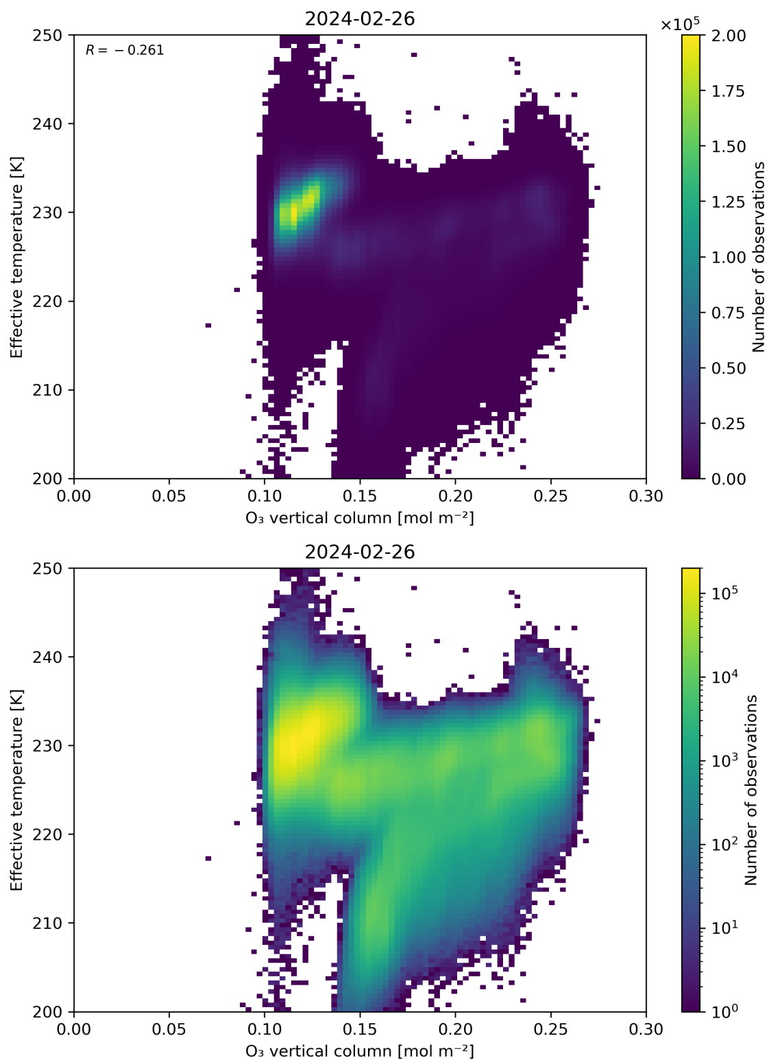
Figure 39: Scatter density plot of “O 3 vertical column” against “Effective temperature” for 2024-02-25 to 2024-02-27.
