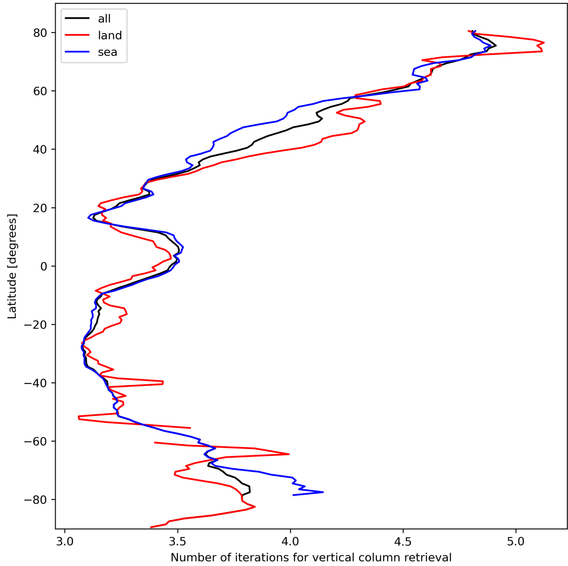
Figure 19: Zonal average of “Number of iterations for vertical column retrieval” for 2024-02-25 to 2024-02-27.
