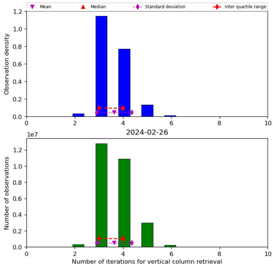
Figure 26: Histogram of “Number of iterations for vertical column retrieval” for 2024-02-25 to 2024-02-27
