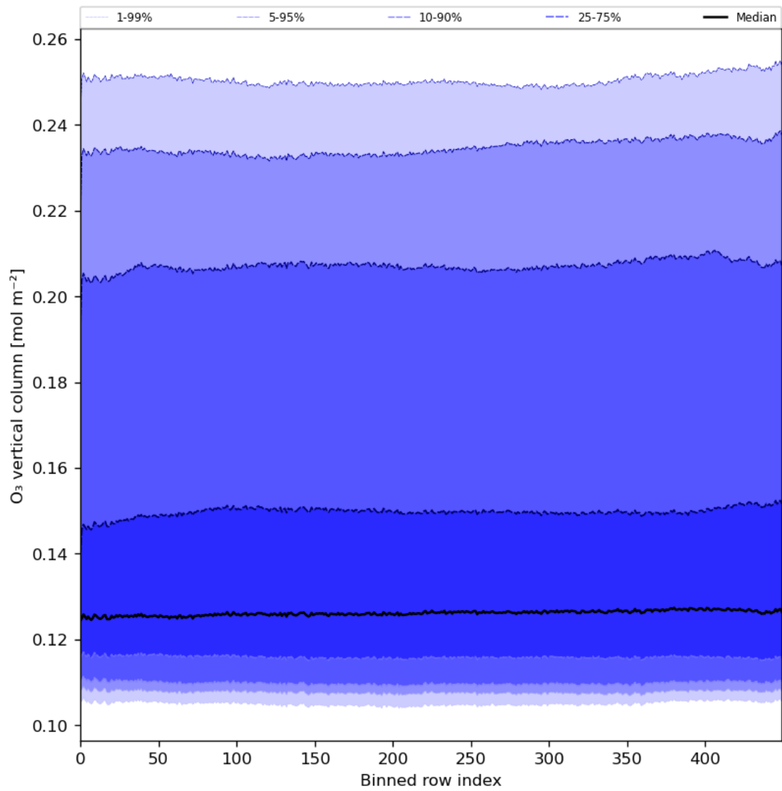
Figure 28: Along track statistics of “O 3 vertical column” for 2024-02-25 to 2024-02-27
