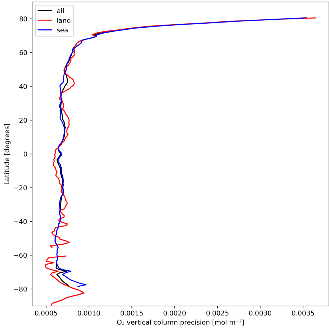
Figure 15: Zonal average of "O 3 vertical column precision" for 2024-02-25 to 2024-02-27.
