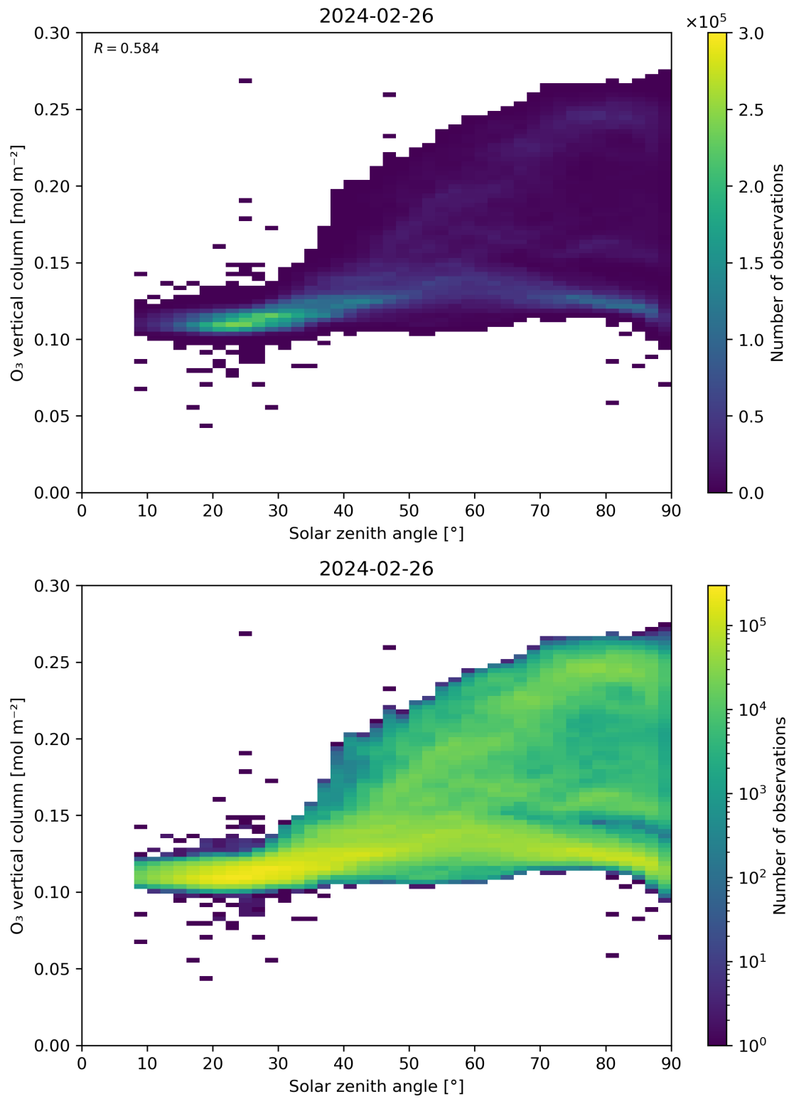
Figure 47: Scatter density plot of “Solar zenith angle” against “O 3 vertical column” for 2024-02-25 to 2024-02-27.
