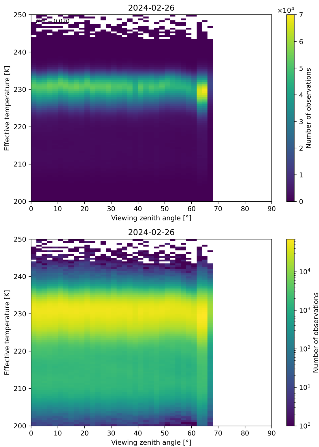
Figure 50: Scatter density plot of “Viewing zenith angle” against “Effective temperature” for 2024-02-25 to 2024-02-27.
