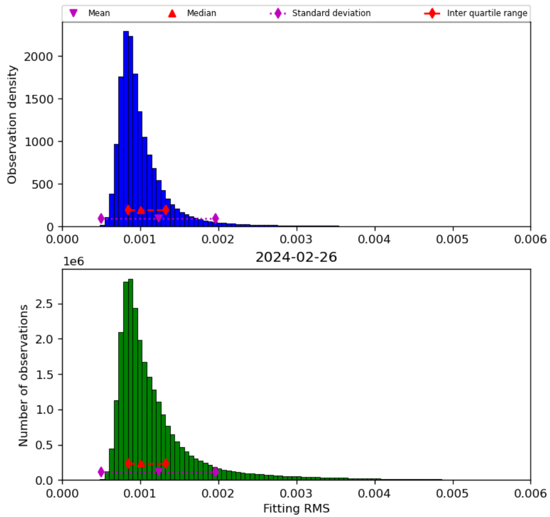
Figure 23: Histogram of “Fitting RMS” for 2024-02-25 to 2024-02-27
