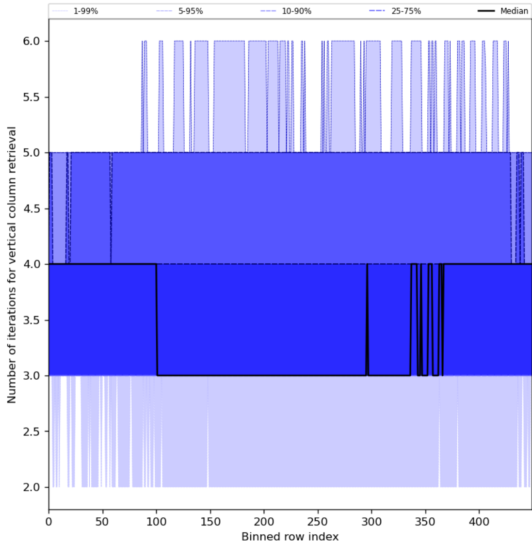
Figure 33: Along track statistics of “Number of iterations for vertical column retrieval” for 2024-02-25 to 2024-02-27
