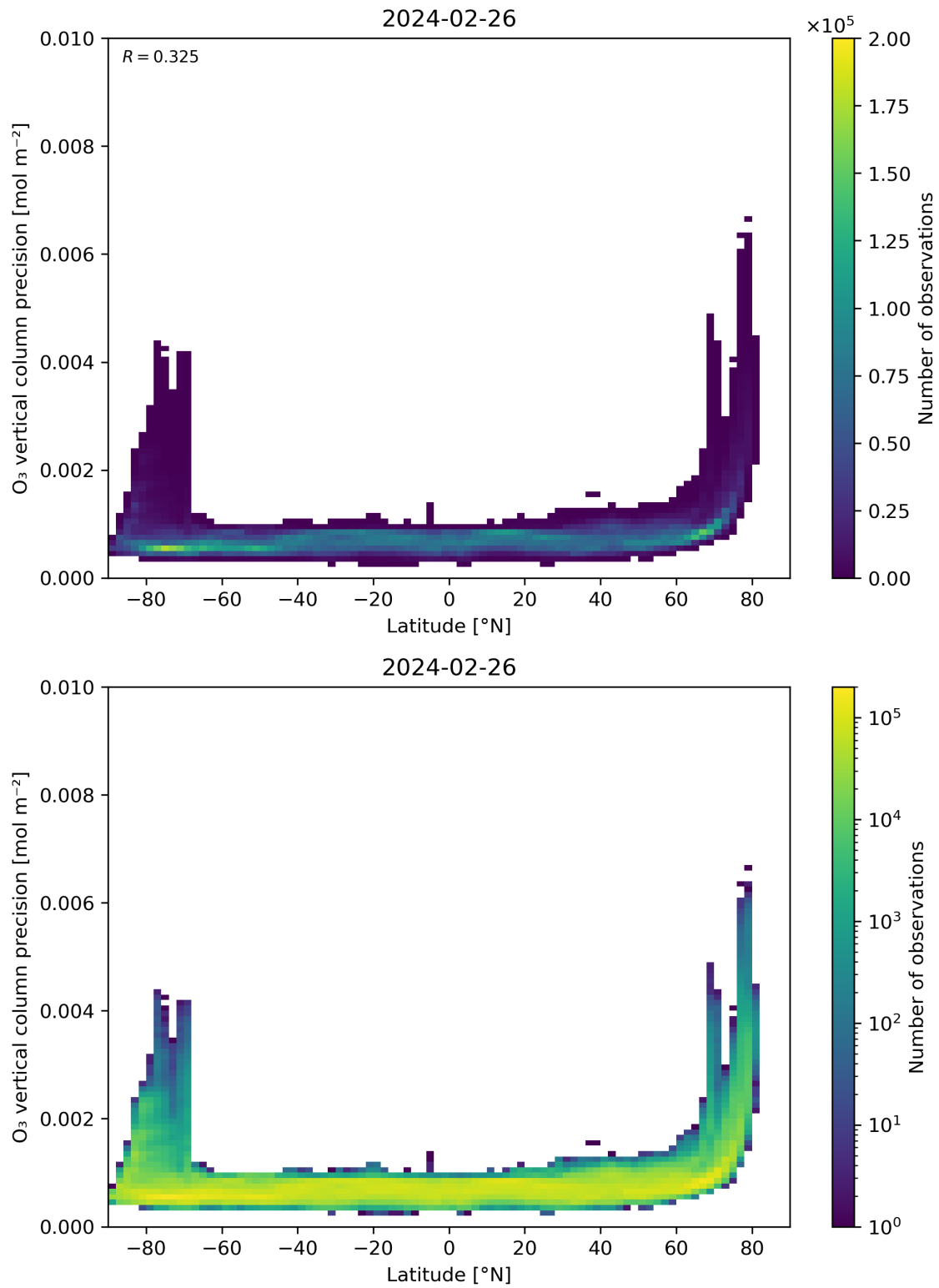
Figure 37: Scatter density plot of “Latitude” against “O 3 vertical column precision” for 2024-02-25 to 2024-02-27.
