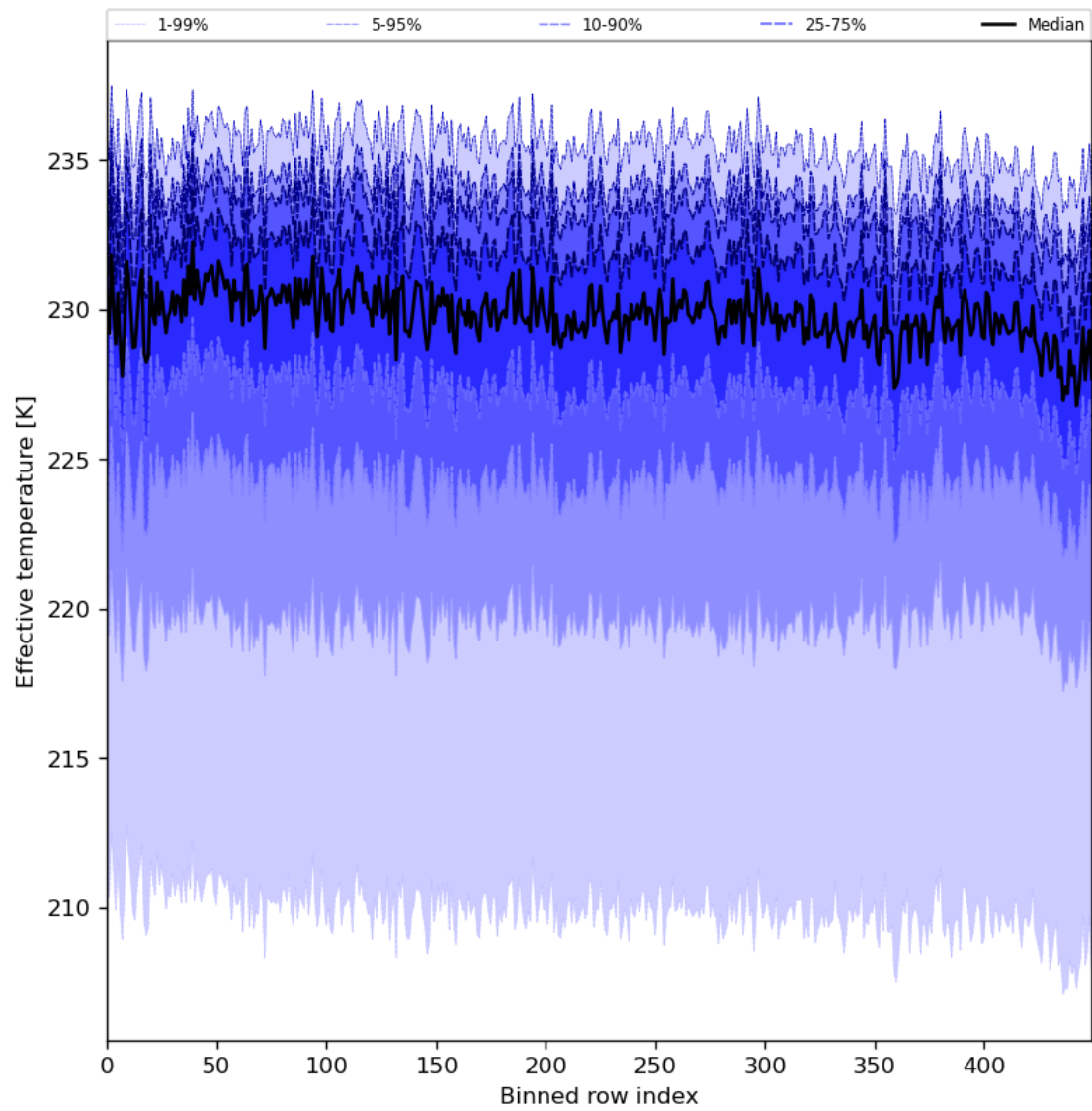
Figure 31: Along track statistics of “Effective temperature” for 2024-02-25 to 2024-02-27
