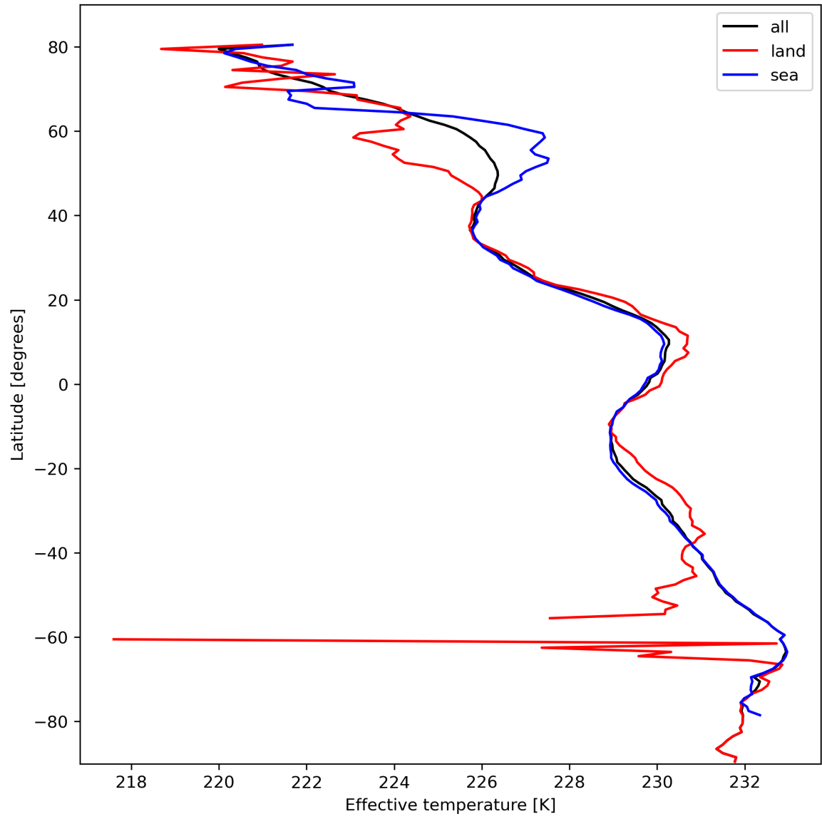
Figure 17: Zonal average of “Effective temperature” for 2024-02-25 to 2024-02-27.
