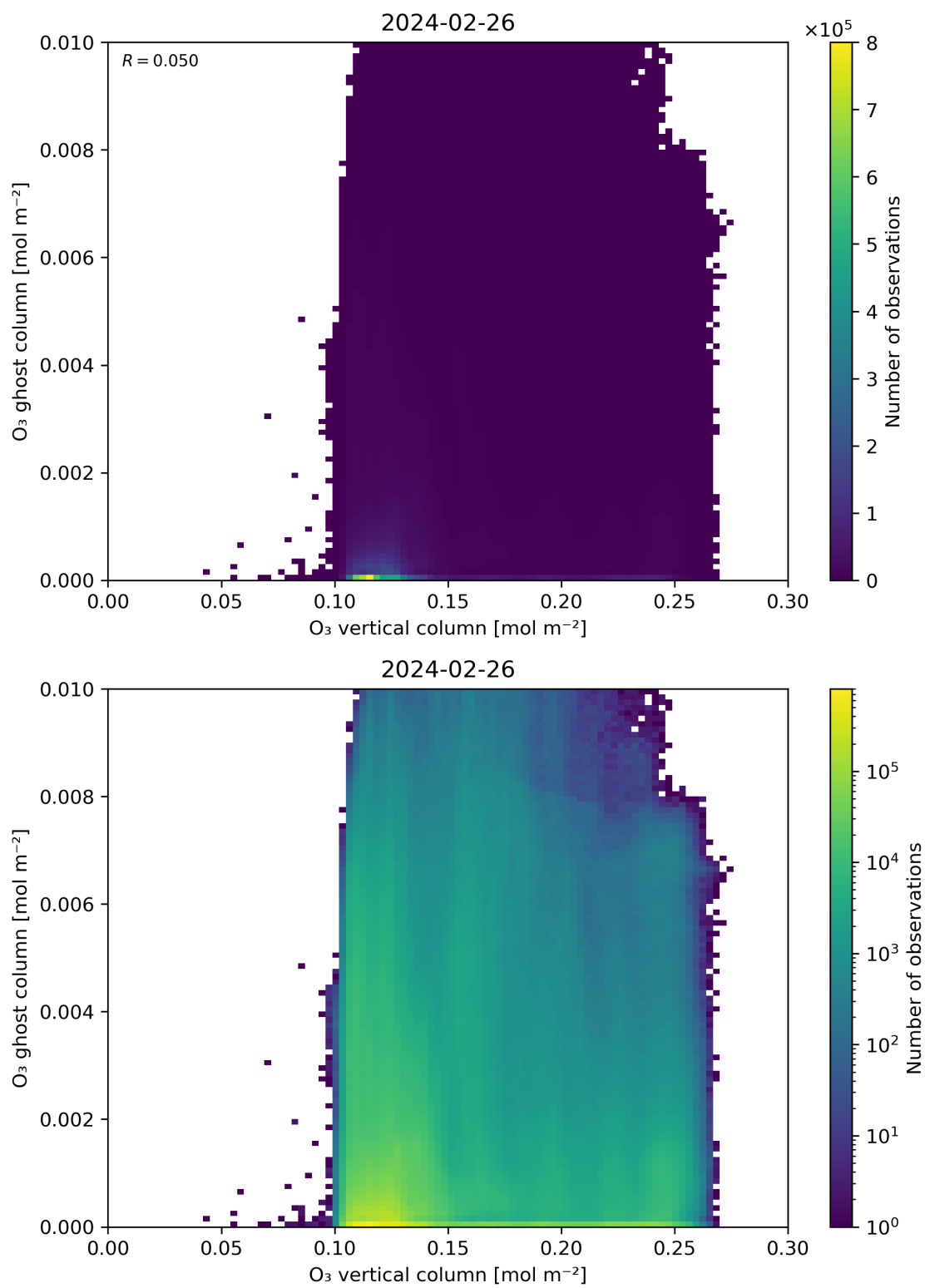
Figure 40: Scatter density plot of “O 3 vertical column” against “O 3 ghost column” for 2024-02-25 to 2024-02-27.
