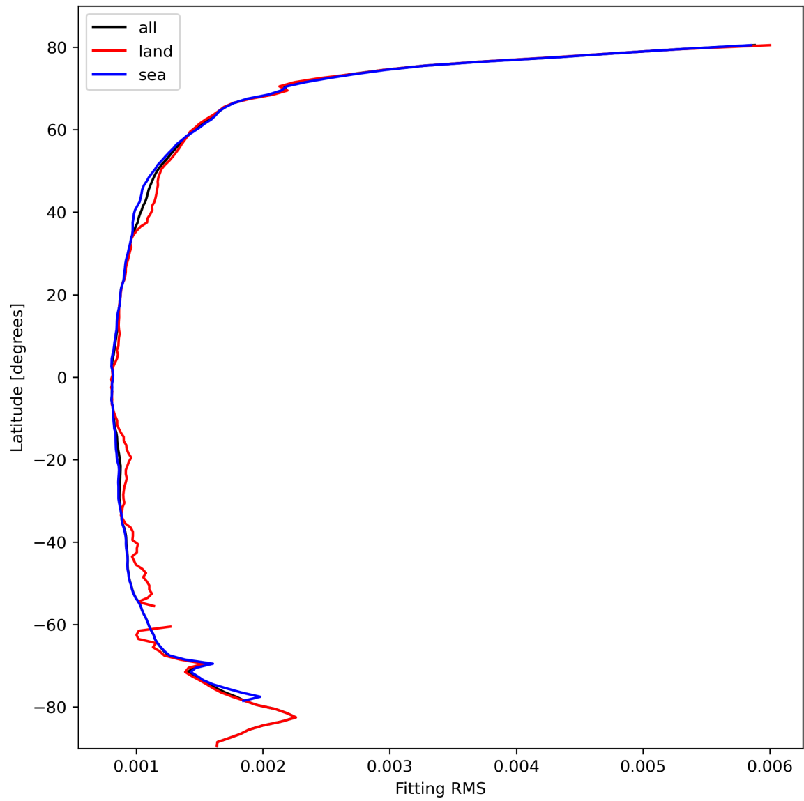
Figure 16: Zonal average of “Fitting RMS” for 2024-02-25 to 2024-02-27.
