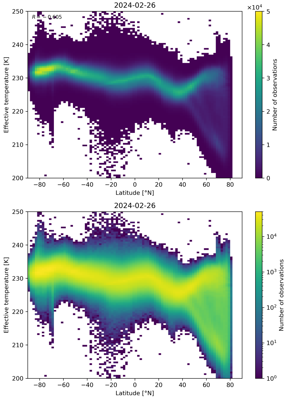
Figure 34: Scatter density plot of “Latitude” against “Effective temperature” for 2024-02-25 to 2024-02-27.
