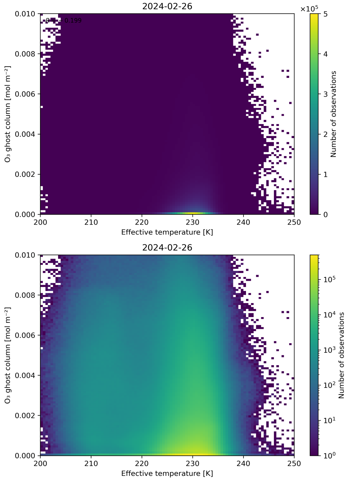
Figure 38: Scatter density plot of “Effective temperature” against “O 3 ghost column” for 2024-02-25 to 2024-02-27.
