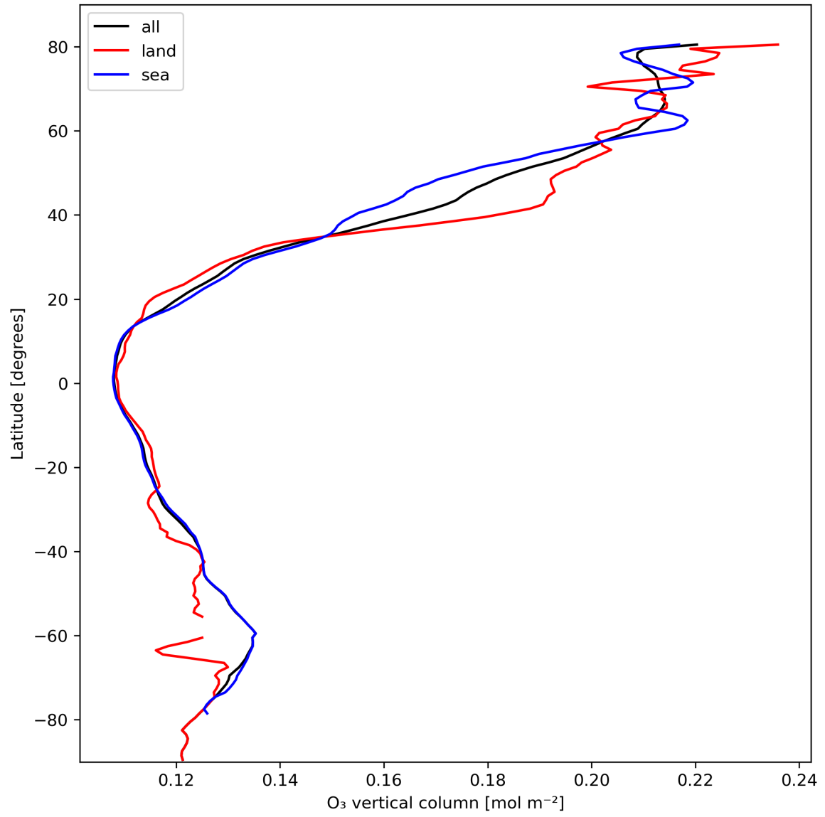
Figure 14: Zonal average of “O 3 vertical column” for 2024-02-25 to 2024-02-27.
