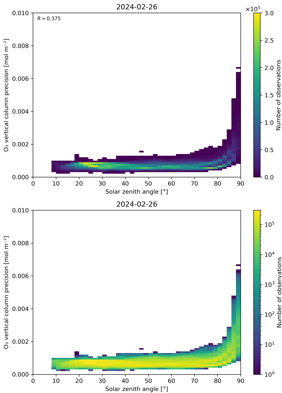
Figure 48: Scatter density plot of “Solar zenith angle” against “O 3 vertical column precision” for 2024-02-25 to 2024-02-27.
