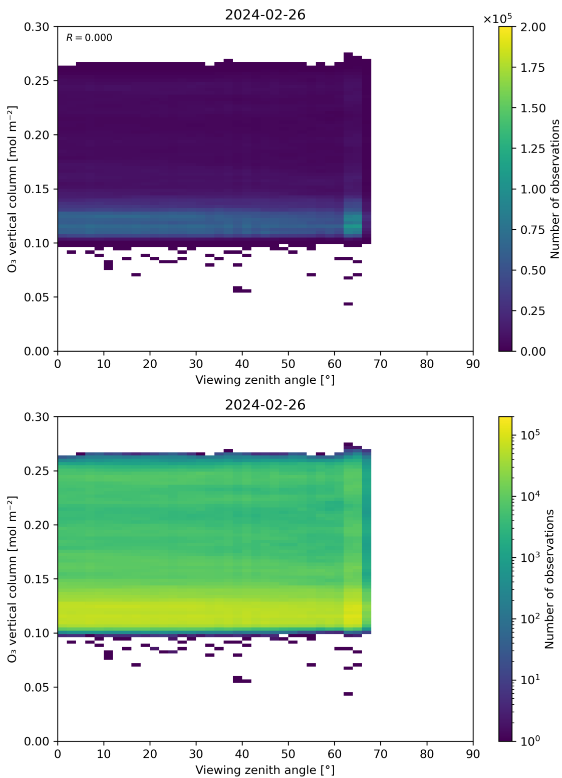
Figure 52: Scatter density plot of “Viewing zenith angle” against “O 3 vertical column” for 2024-02-25 to 2024-02-27.
