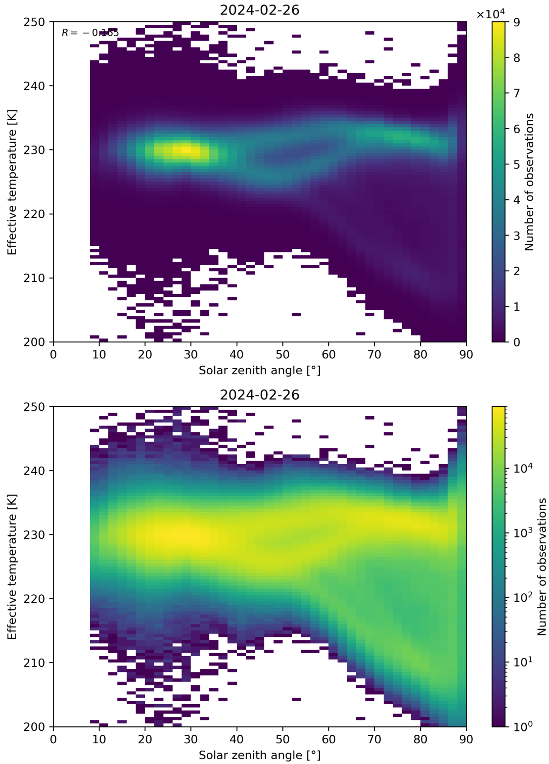
Figure 45: Scatter density plot of “Solar zenith angle” against “Effective temperature” for 2024-02-25 to 2024-02-27.
