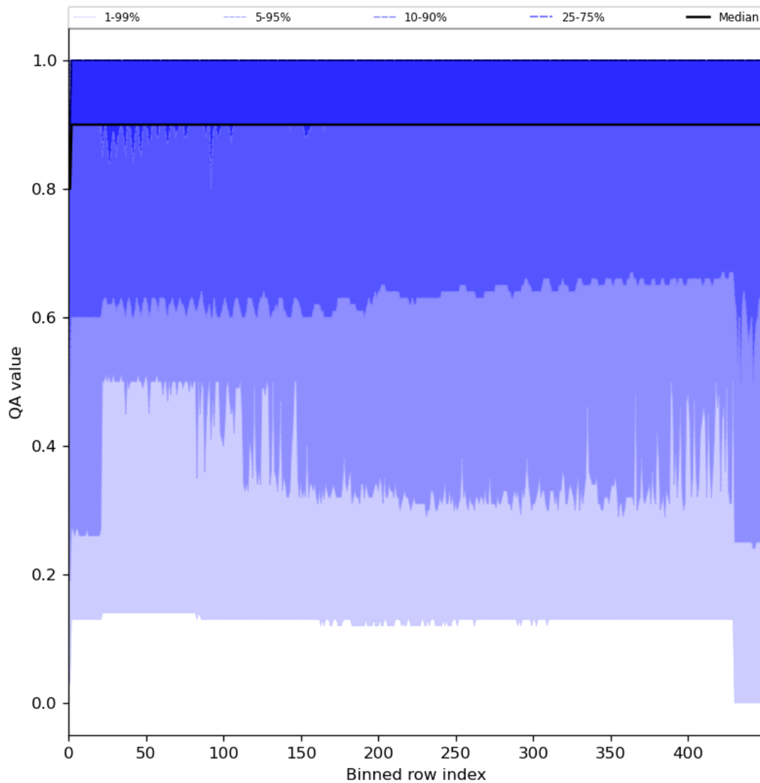
Figure 27: Along track statistics of “QA value” for 2024-02-25 to 2024-02-27
