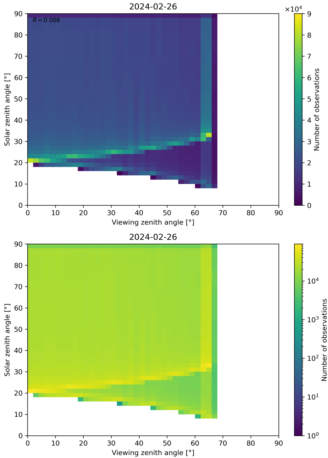
Figure 54: Scatter density plot of “Viewing zenith angle” against “Solar zenith angle” for 2024-02-25 to 2024-02-27.
