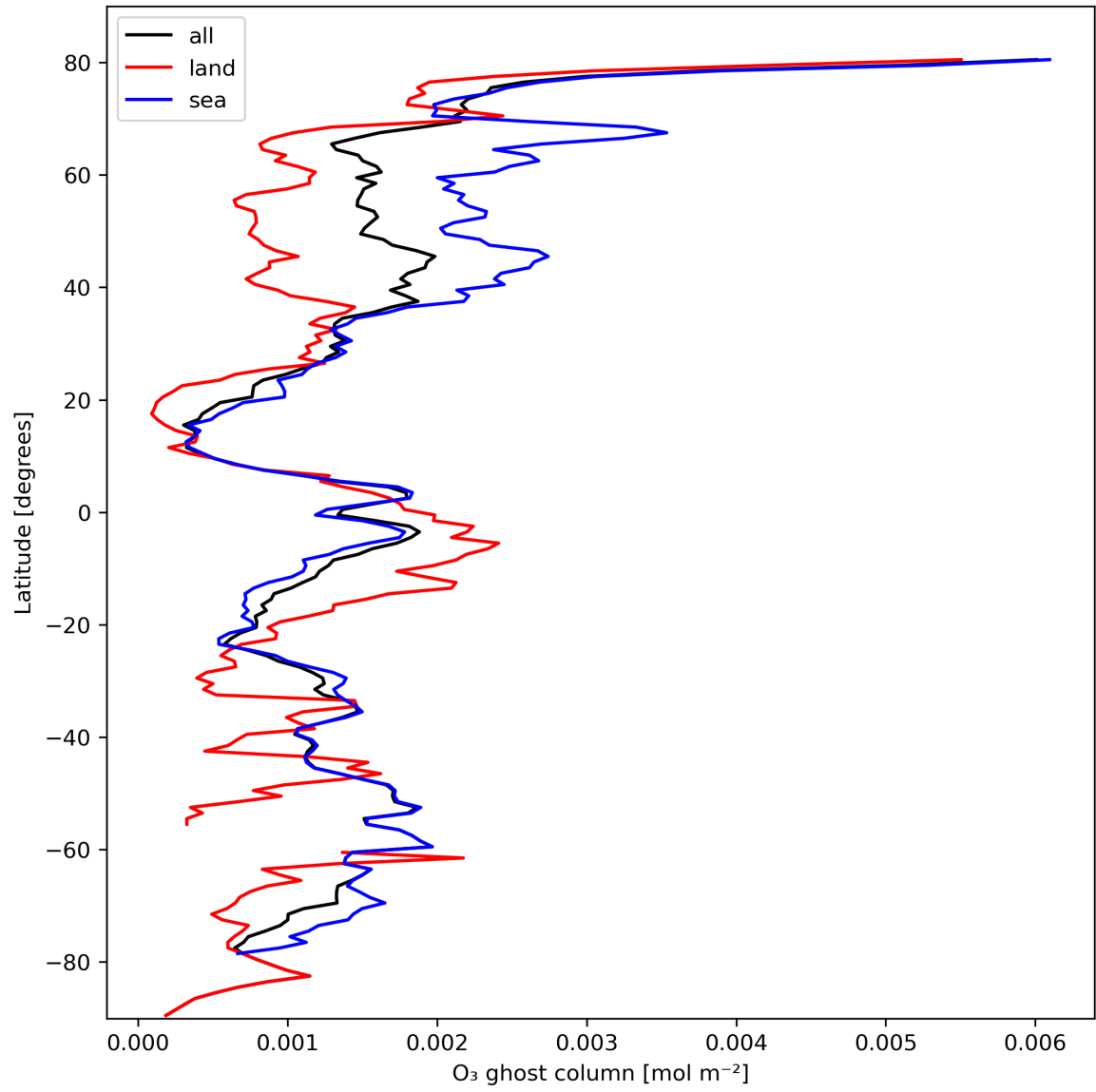
Figure 18: Zonal average of “O 3 ghost column” for 2024-02-25 to 2024-02-27.
