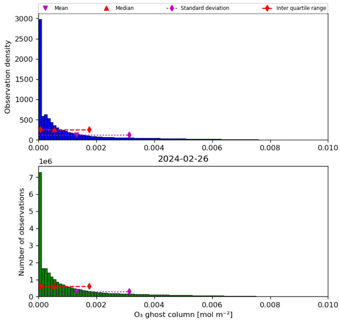
Figure 25: Histogram of “O 3 ghost column” for 2024-02-25 to 2024-02-27
