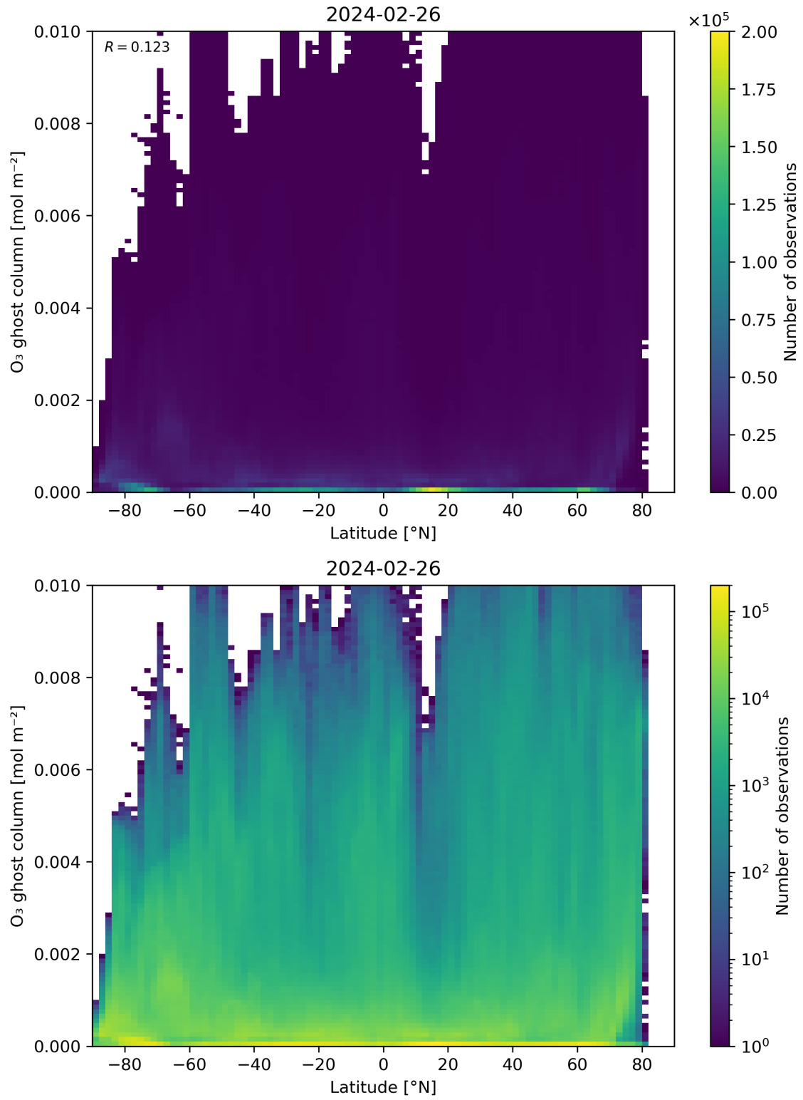
Figure 35: Scatter density plot of “Latitude” against “O 3 ghost column” for 2024-02-25 to 2024-02-27.
