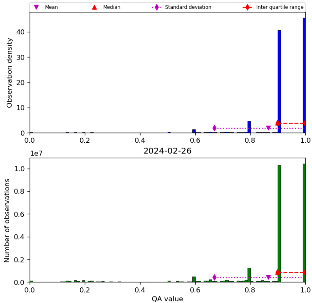
Figure 20: Histogram of “QA value” for 2024-02-25 to 2024-02-27
