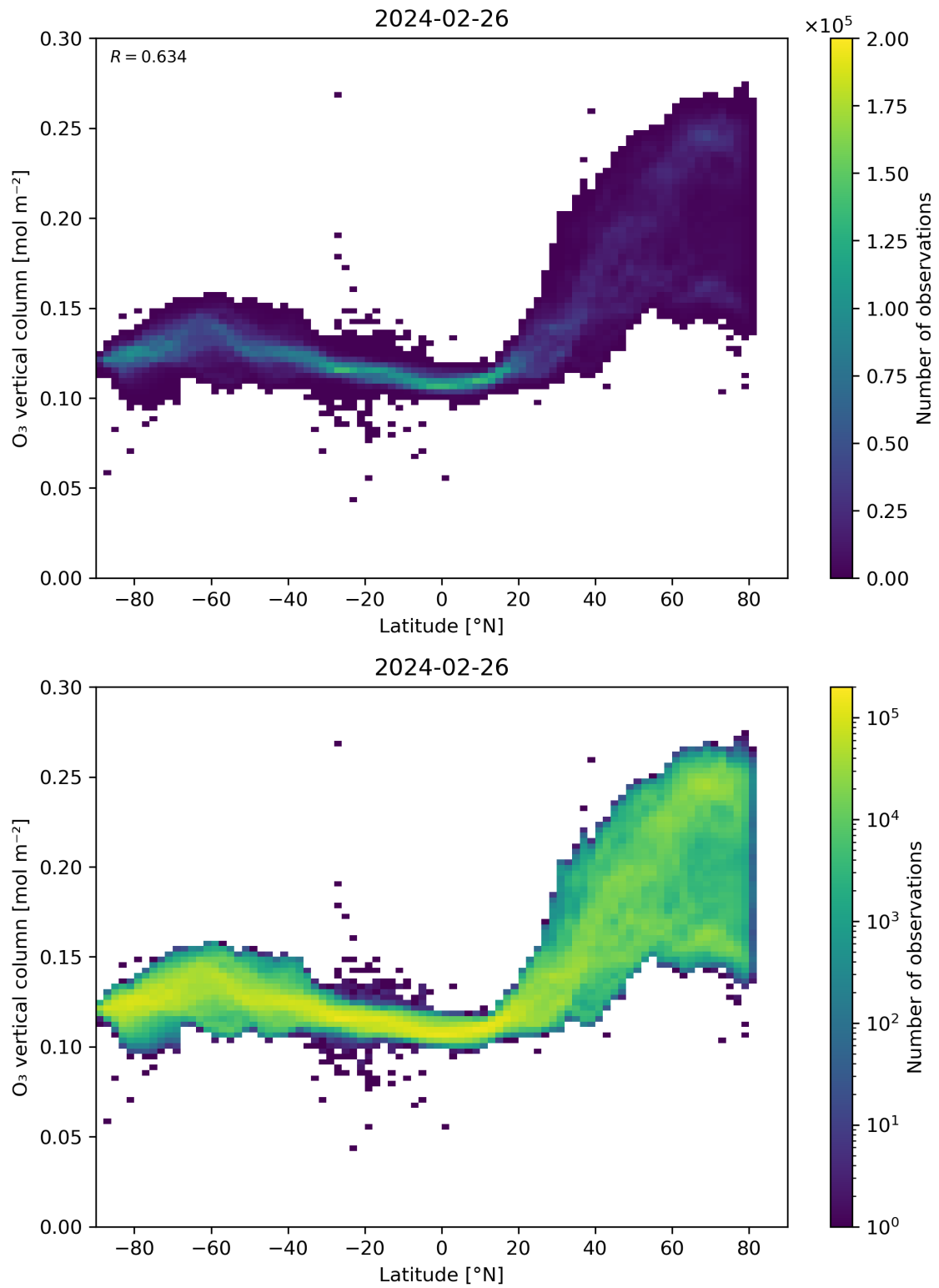
Figure 36: Scatter density plot of “Latitude” against “O 3 vertical column” for 2024-02-25 to 2024-02-27.
