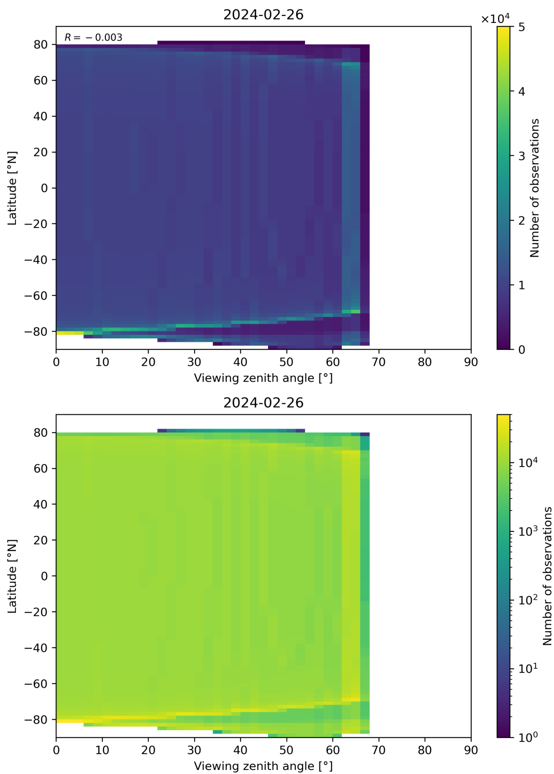
Figure 49: Scatter density plot of “Viewing zenith angle” against “Latitude” for 2024-02-25 to 2024-02-27.
