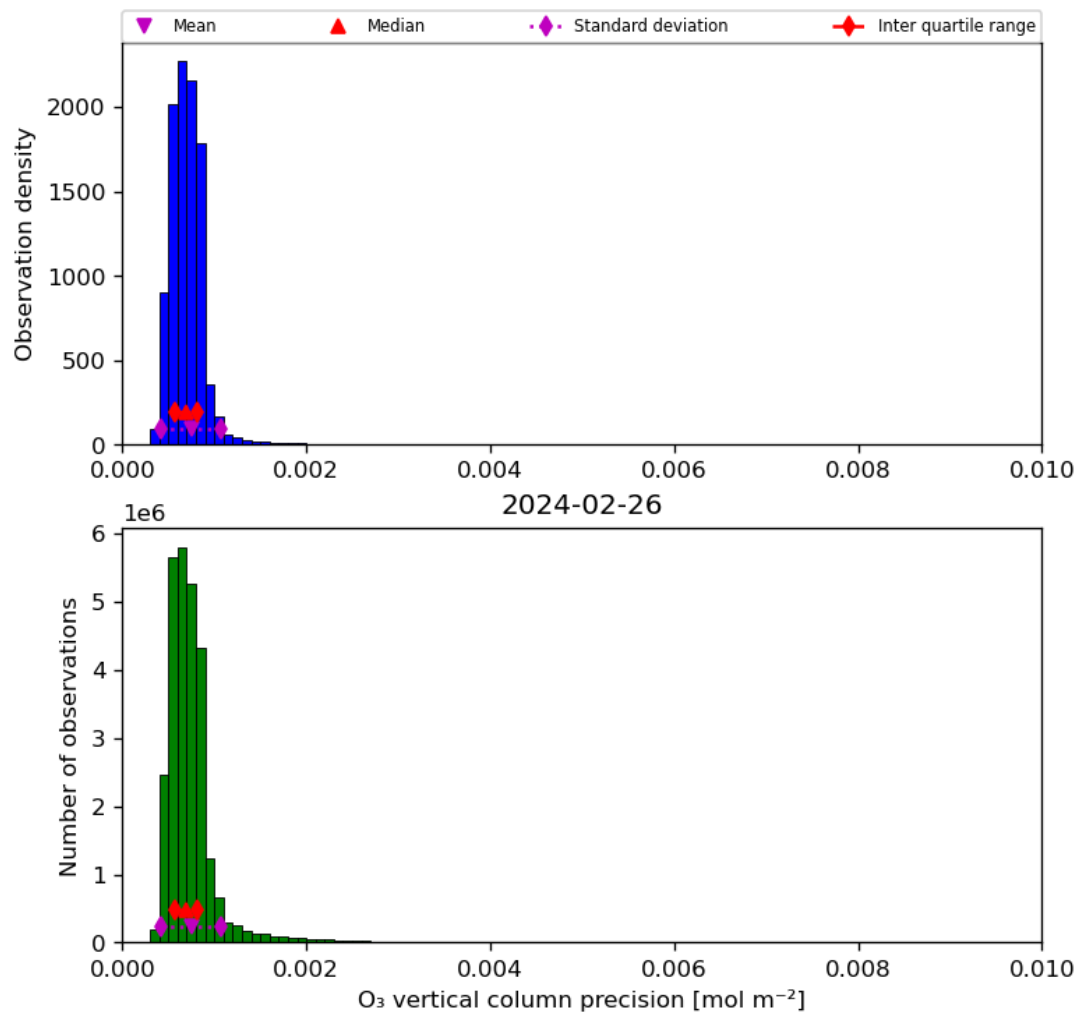
Figure 22: Histogram of “O 3 vertical column precision” for 2024-02-25 to 2024-02-27
