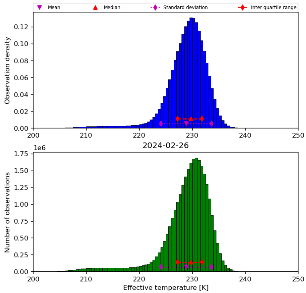
Figure 24: Histogram of “Effective temperature” for 2024-02-25 to 2024-02-27
