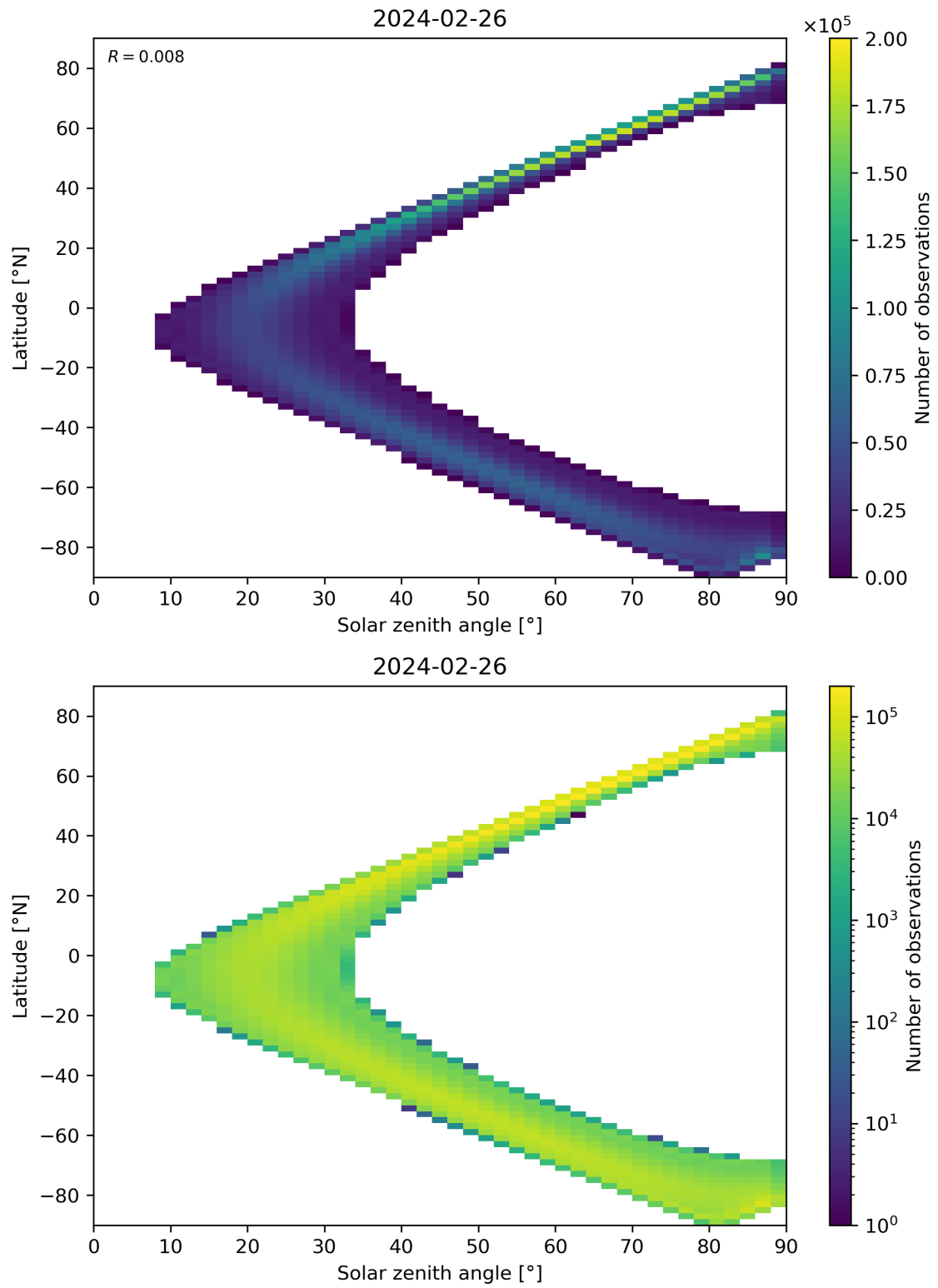
Figure 44: Scatter density plot of “Solar zenith angle” against “Latitude” for 2024-02-25 to 2024-02-27.
