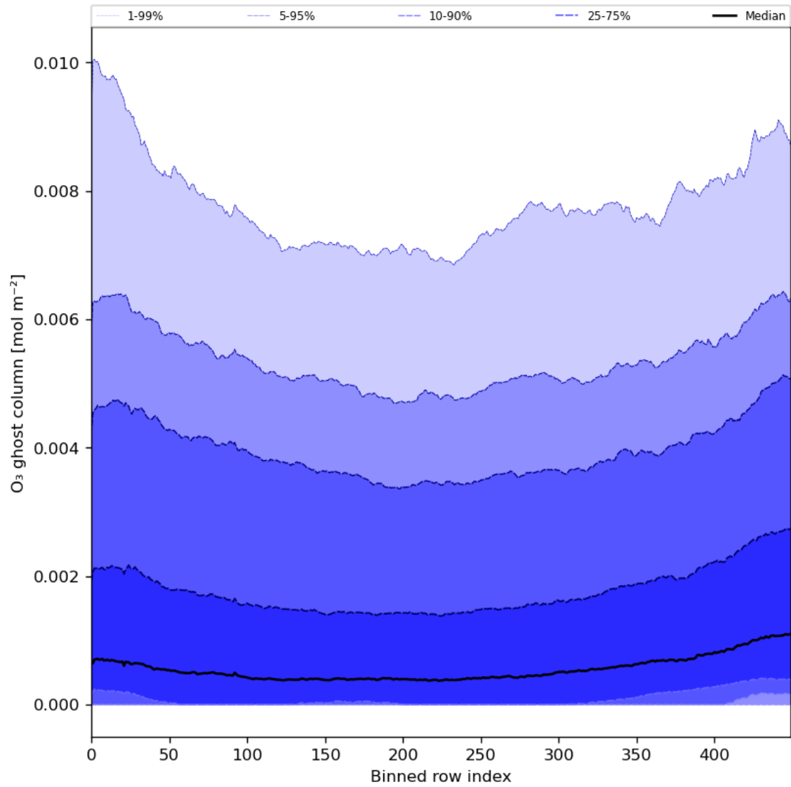
Figure 32: Along track statistics of “O 3 ghost column” for 2024-02-25 to 2024-02-27
