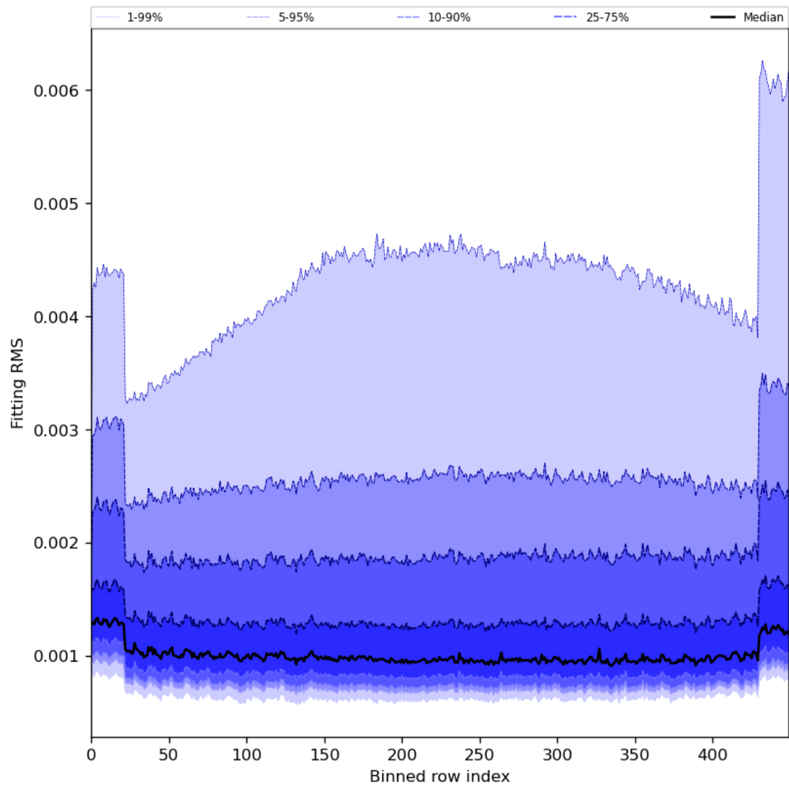
Figure 30: Along track statistics of “Fitting RMS” for 2024-02-25 to 2024-02-27
