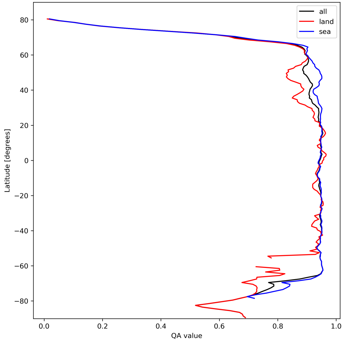
Figure 13: Zonal average of “QA value” for 2024-02-25 to 2024-02-27.
