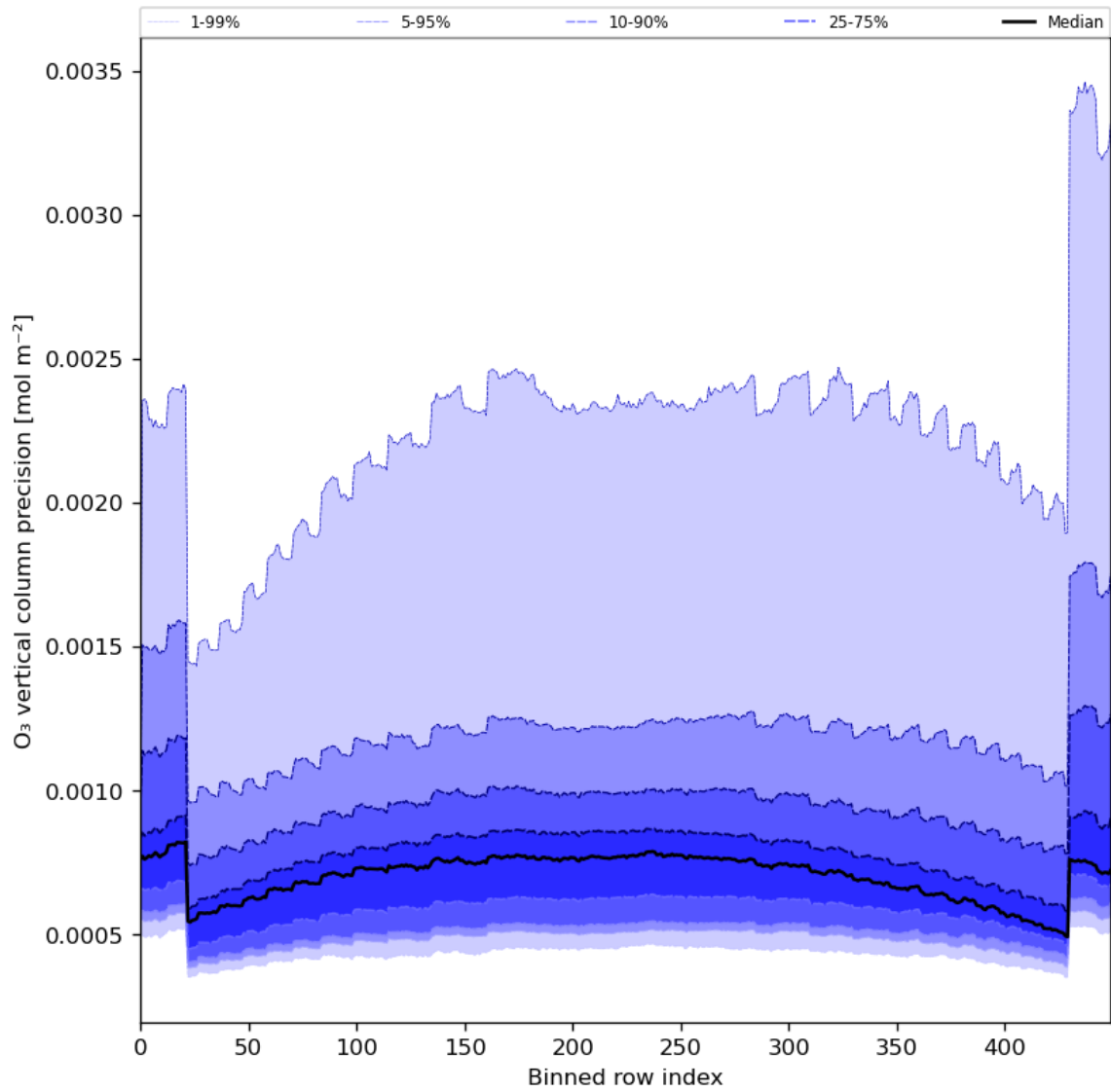
Figure 29: Along track statistics of “O 3 vertical column precision” for 2024-02-25 to 2024-02-27
