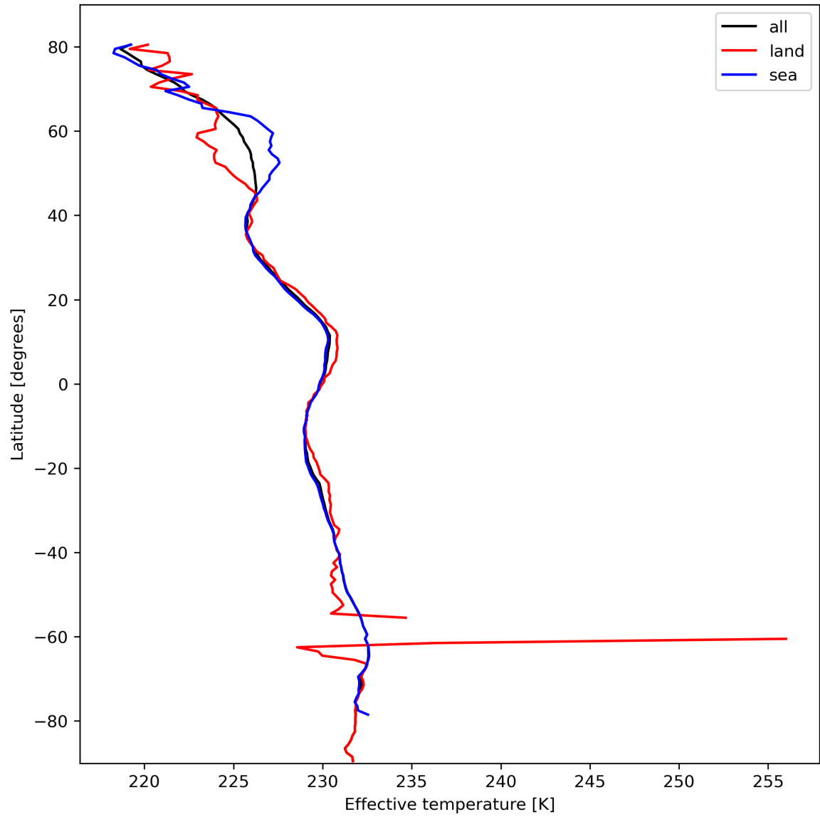
Figure 17: Zonal average of “Effective temperature” for 2024-02-27 to 2024-02-28.
