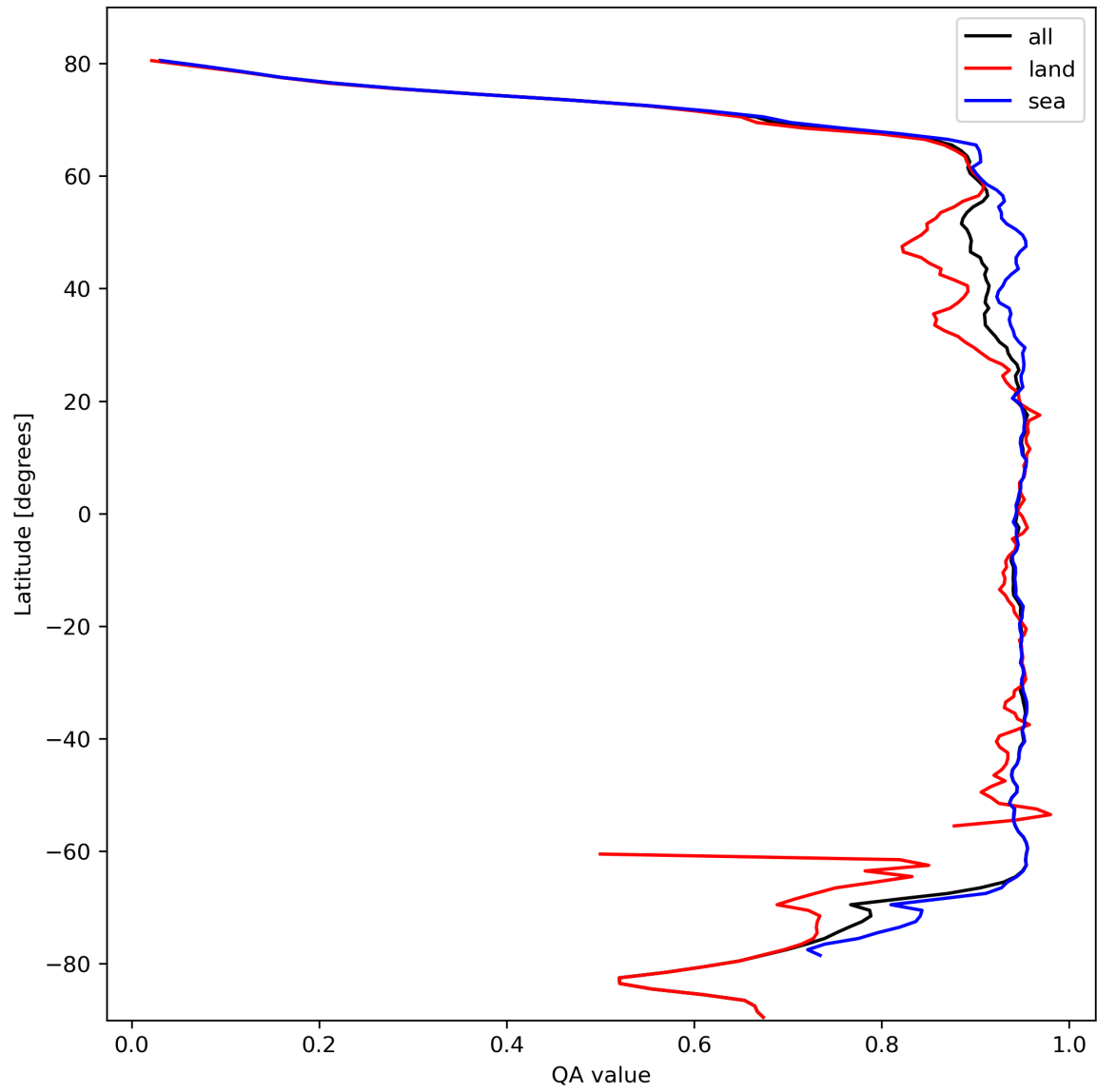
Figure 13: Zonal average of “QA value” for 2024-02-27 to 2024-02-28.
