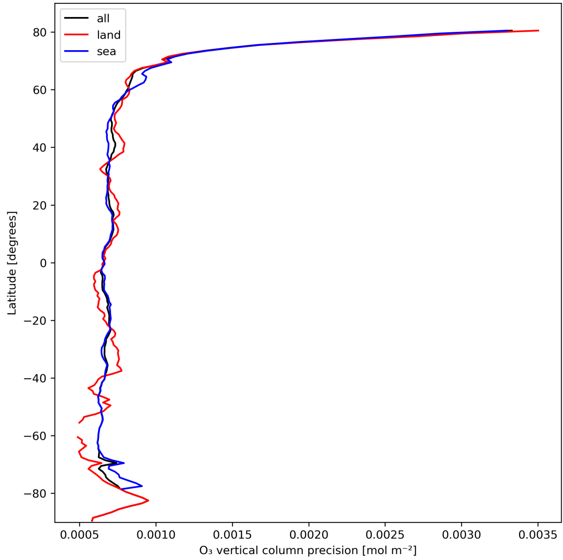
Figure 15: Zonal average of “O 3 vertical column precision” for 2024-02-27 to 2024-02-28.
