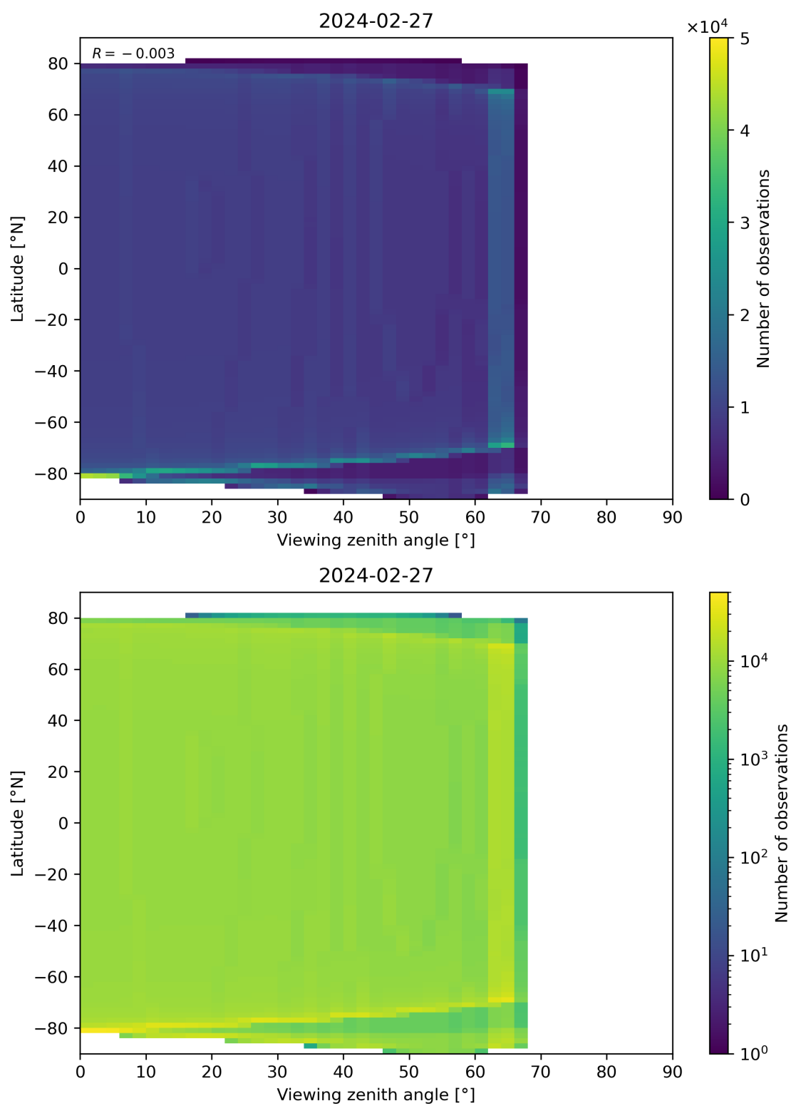
Figure 49: Scatter density plot of “Viewing zenith angle” against “Latitude” for 2024-02-27 to 2024-02-28.
