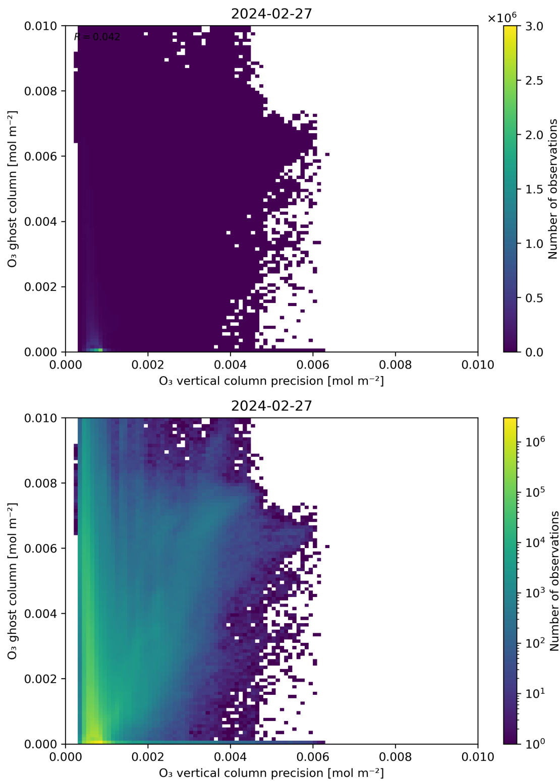
Figure 43: Scatter density plot of “O 3 vertical column precision” against “O 3 ghost column” for 2024-02-27 to 2024-02-28.
