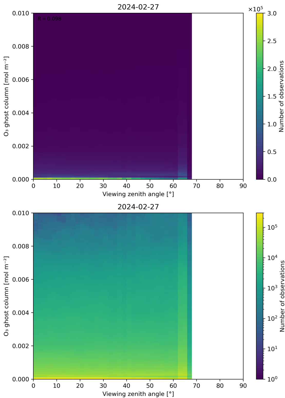
Figure 51: Scatter density plot of “Viewing zenith angle” against “O 3 ghost column” for 2024-02-27 to 2024-02-28.
