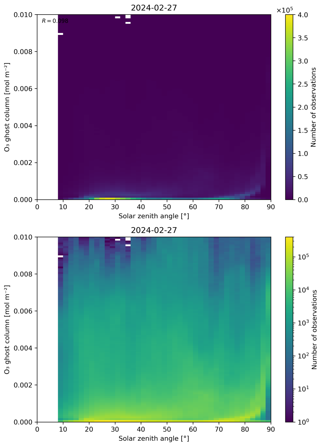
Figure 46: Scatter density plot of “Solar zenith angle” against “O 3 ghost column” for 2024-02-27 to 2024-02-28.
