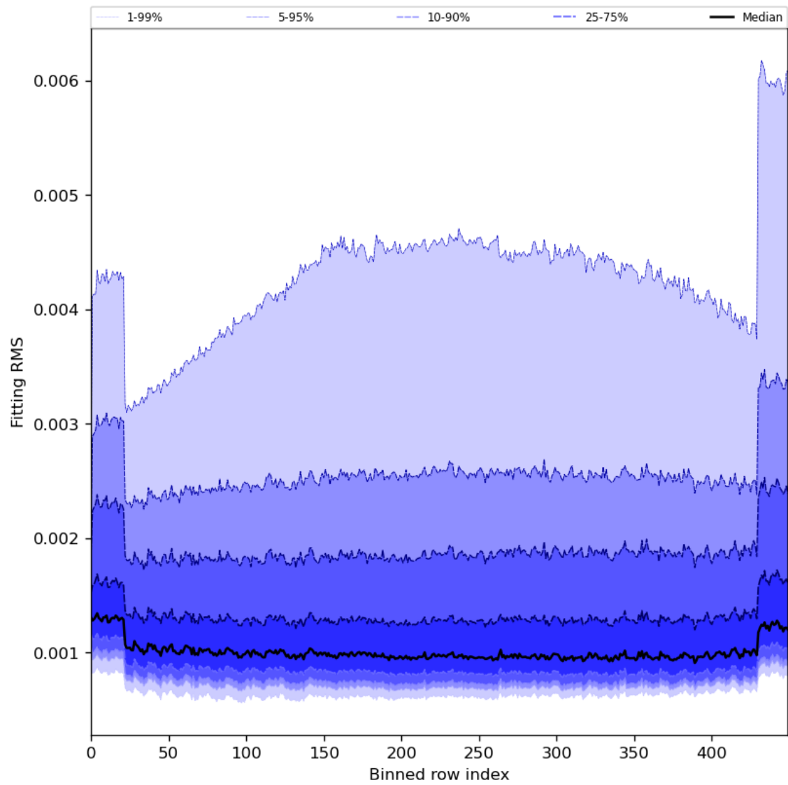
Figure 30: Along track statistics of “Fitting RMS” for 2024-02-27 to 2024-02-28
