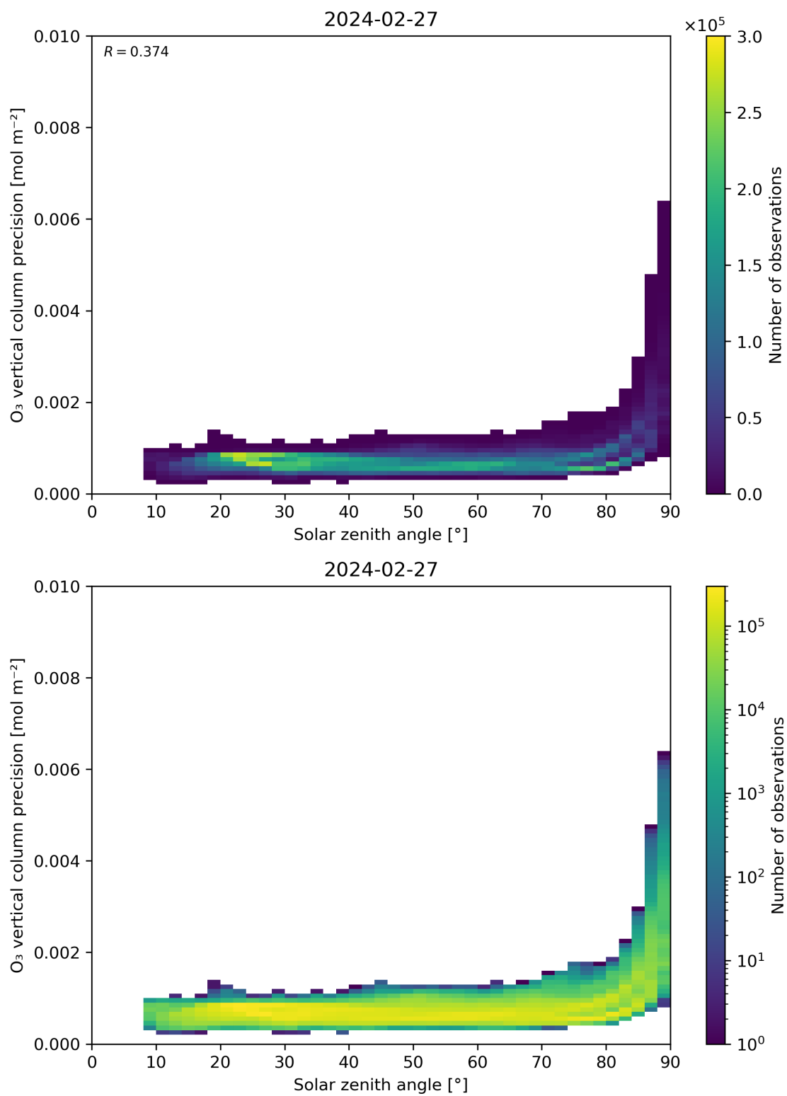
Figure 48: Scatter density plot of “Solar zenith angle” against “O 3 vertical column precision” for 2024-02-27 to 2024-02-28.
