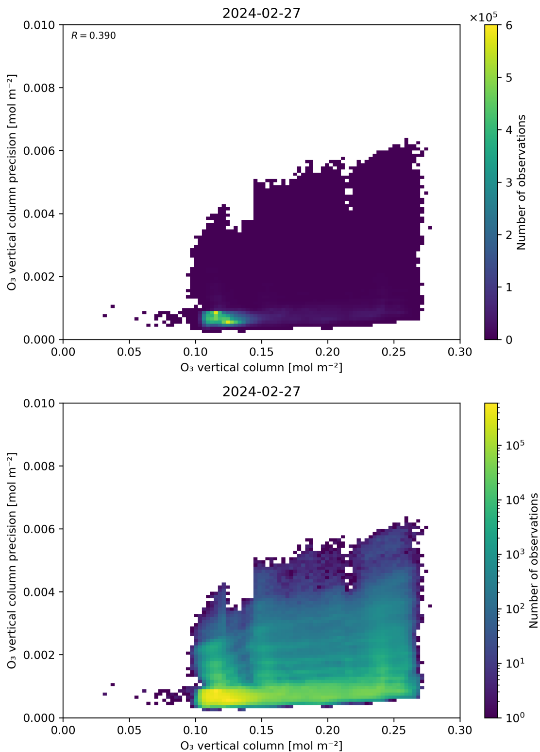
Figure 41: Scatter density plot of “O 3 vertical column” against “O 3 vertical column precision” for 2024-02-27 to 2024-02-28.
