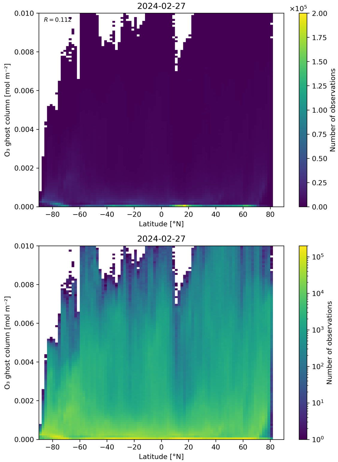
Figure 35: Scatter density plot of “Latitude” against “O 3 ghost column” for 2024-02-27 to 2024-02-28.
