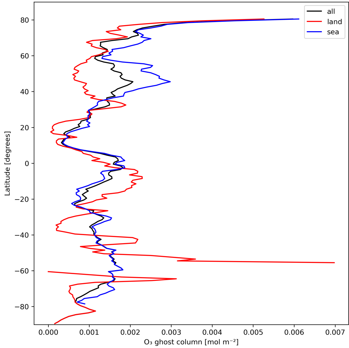
Figure 18: Zonal average of “O 3 ghost column” for 2024-02-27 to 2024-02-28.
