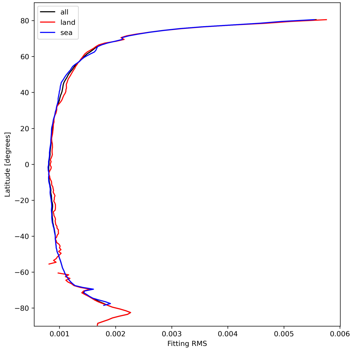
Figure 16: Zonal average of “Fitting RMS” for 2024-02-27 to 2024-02-28.
