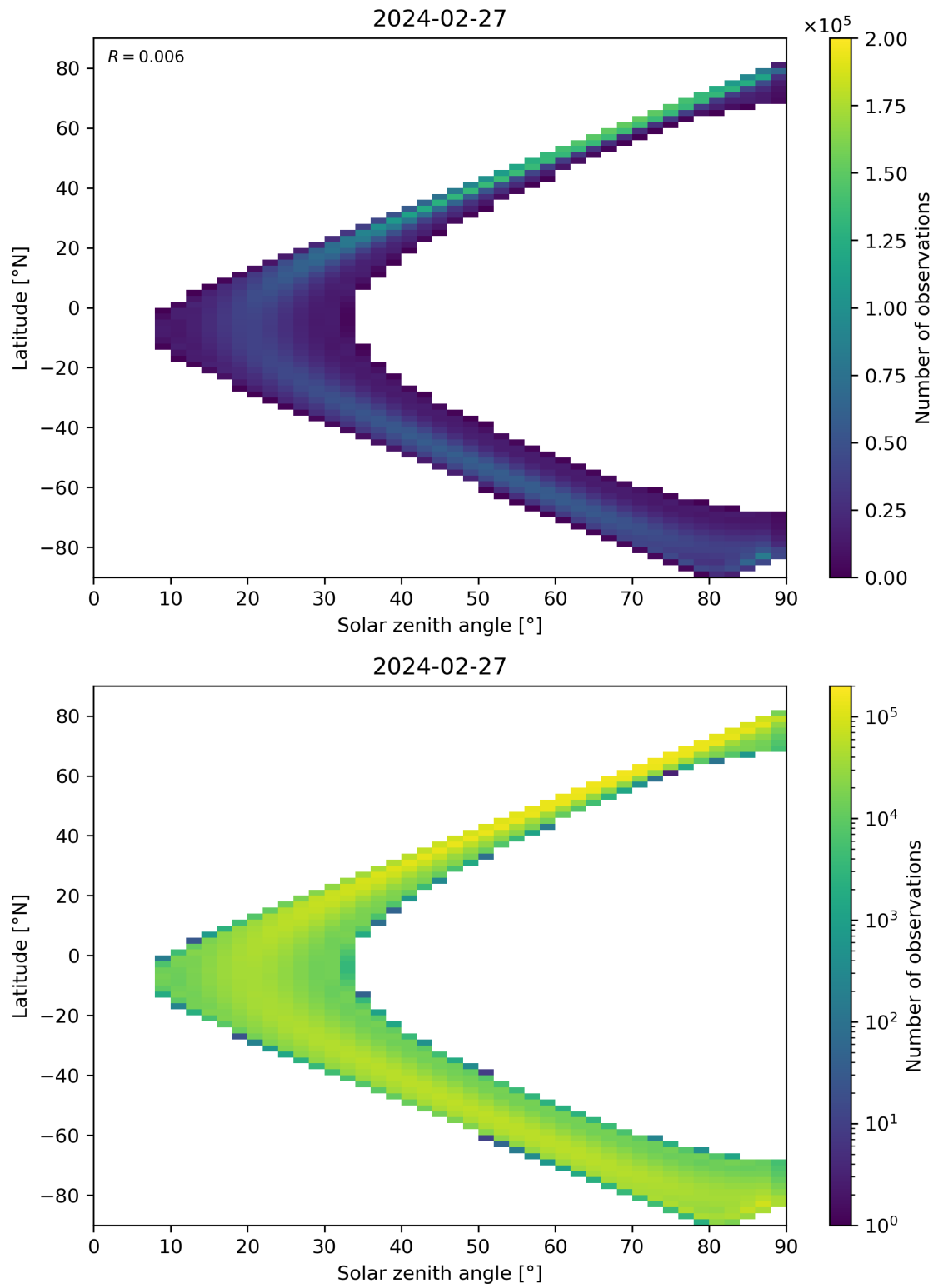
Figure 44: Scatter density plot of “Solar zenith angle” against “Latitude” for 2024-02-27 to 2024-02-28.
