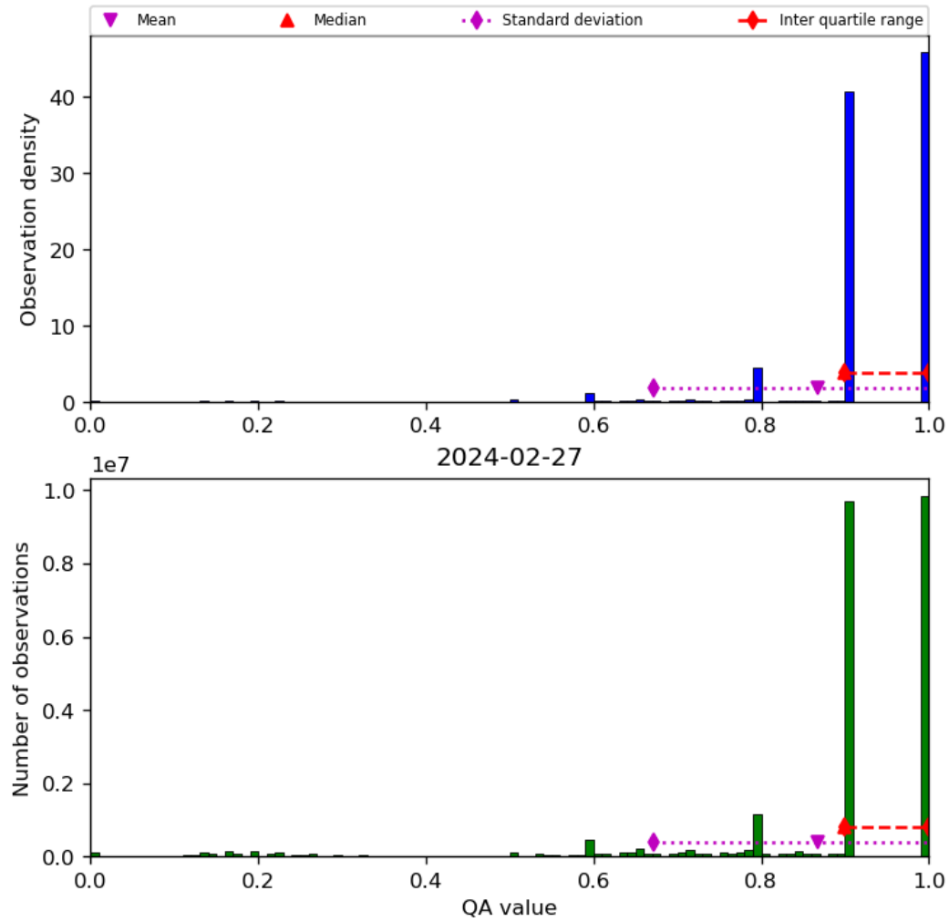
Figure 20: Histogram of “QA value” for 2024-02-27 to 2024-02-28
