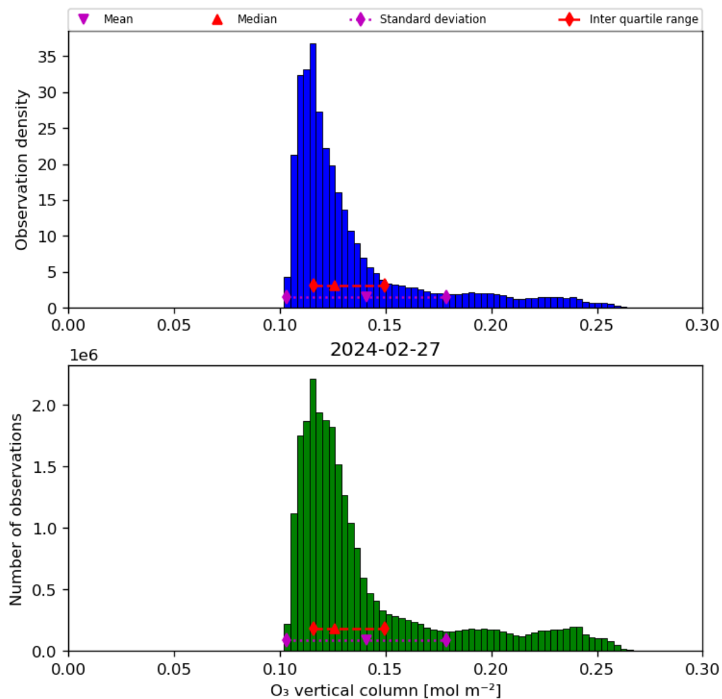
Figure 21: Histogram of “O 3 vertical column” for 2024-02-27 to 2024-02-28
