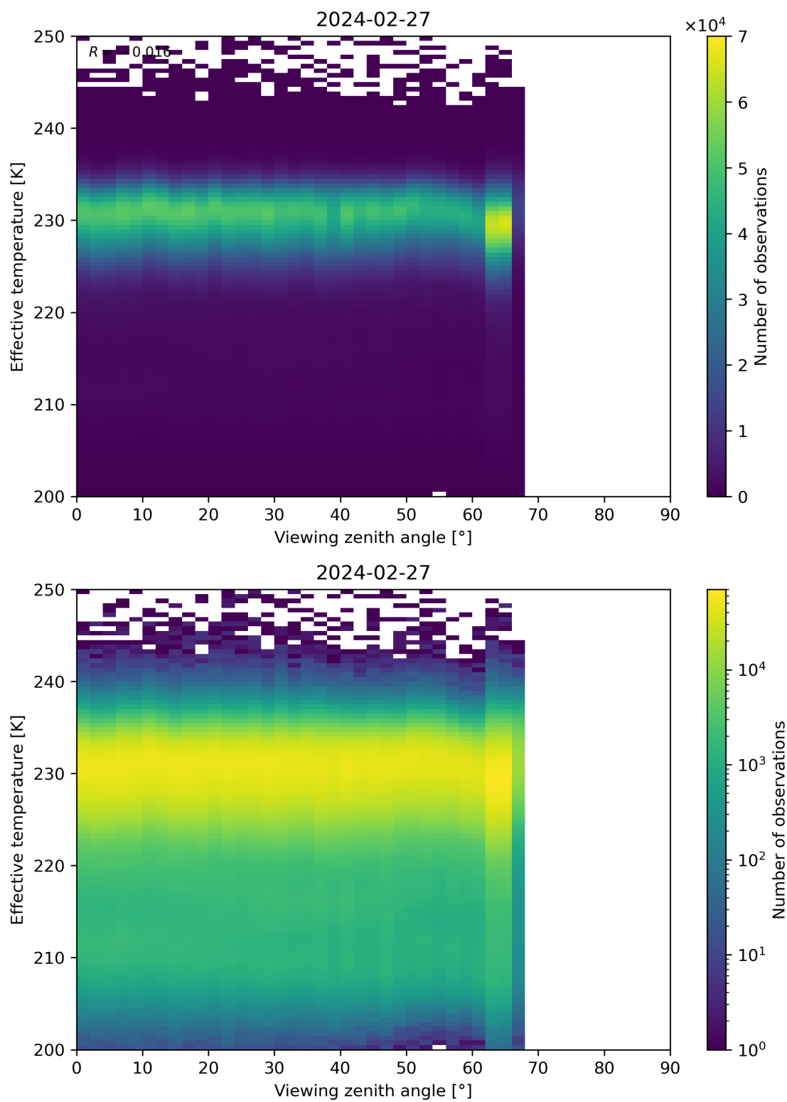
Figure 50: Scatter density plot of “Viewing zenith angle” against “Effective temperature” for 2024-02-27 to 2024-02-28.
