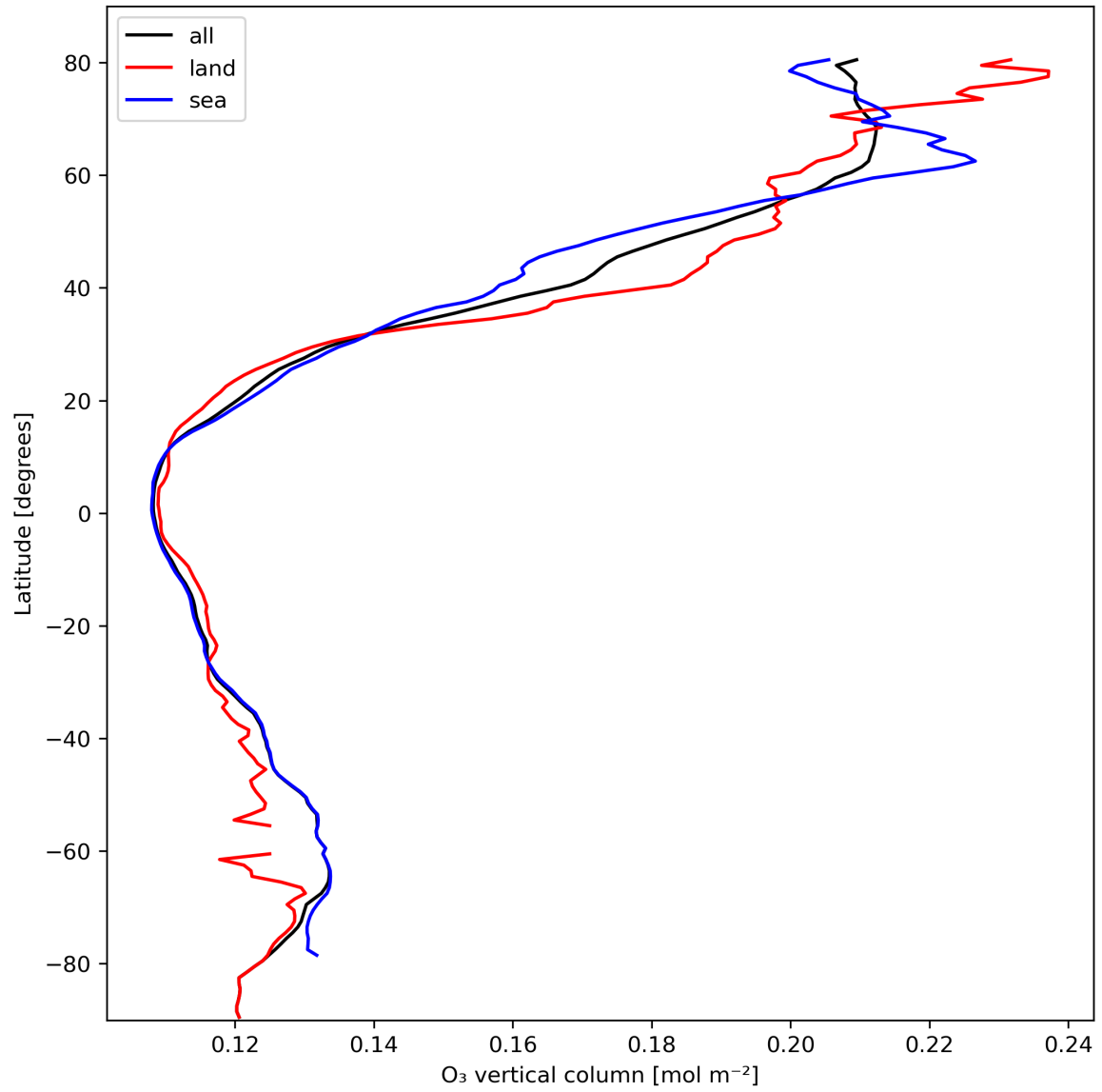
Figure 14: Zonal average of “O 3 vertical column” for 2024-02-27 to 2024-02-28.
