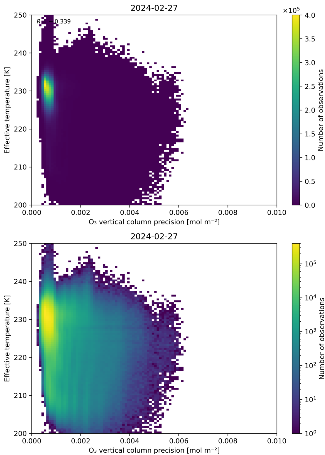
Figure 42: Scatter density plot of “O 3 vertical column precision” against “Effective temperature” for 2024-02-27 to 2024-02-28.
