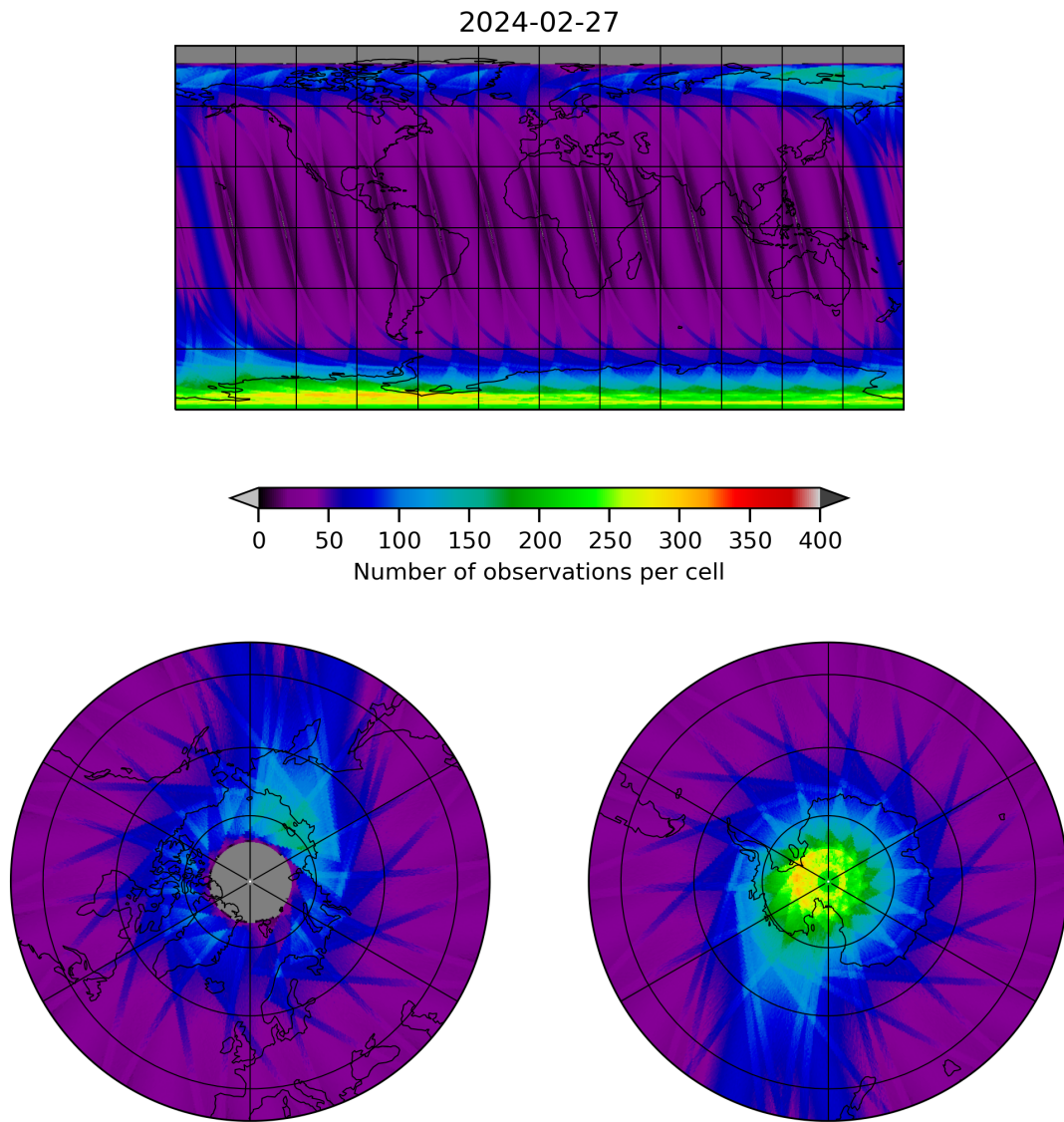
Figure 12: Map of the number of observations for 2024-02-27 to 2024-02-28
