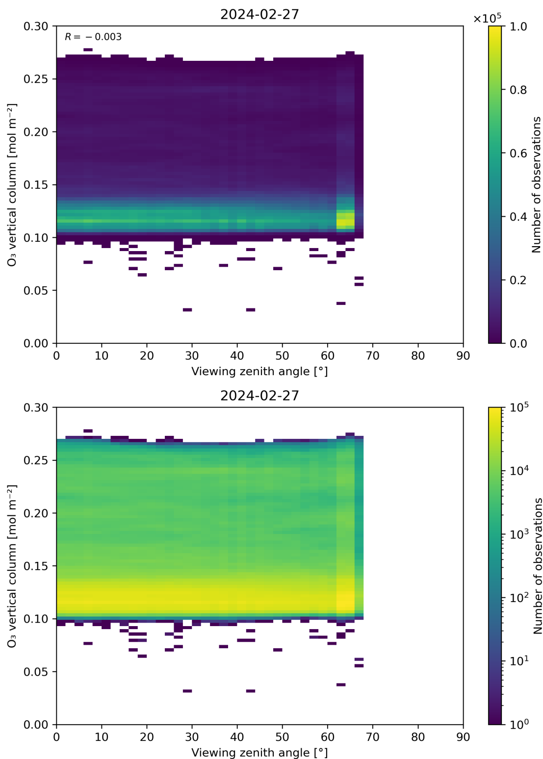
Figure 52: Scatter density plot of “Viewing zenith angle” against “O 3 vertical column” for 2024-02-27 to 2024-02-28.
