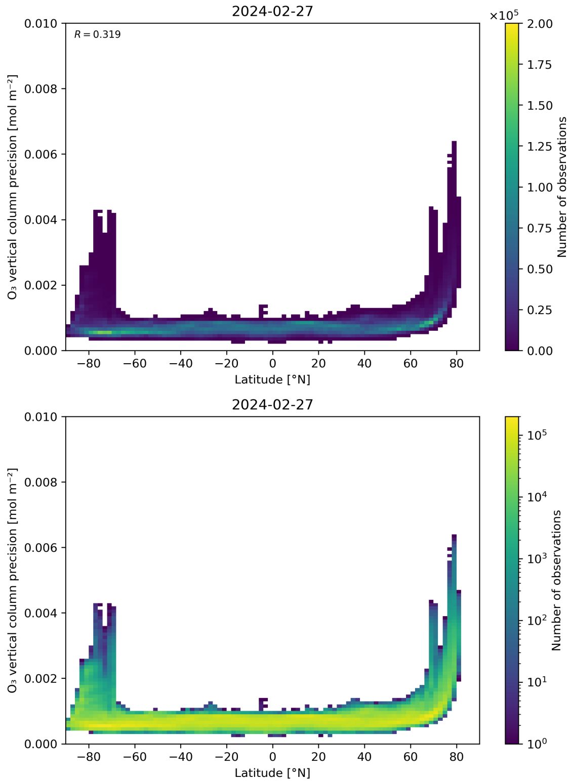
Figure 37: Scatter density plot of “Latitude” against “O 3 vertical column precision” for 2024-02-27 to 2024-02-28.
