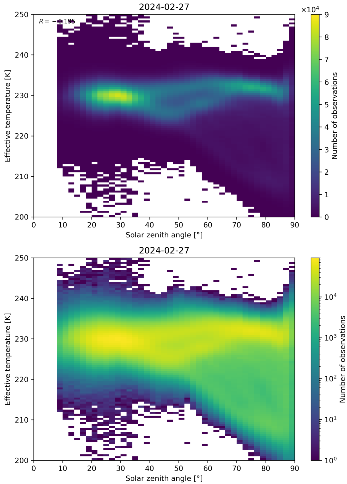
Figure 45: Scatter density plot of “Solar zenith angle” against “Effective temperature” for 2024-02-27 to 2024-02-28.
