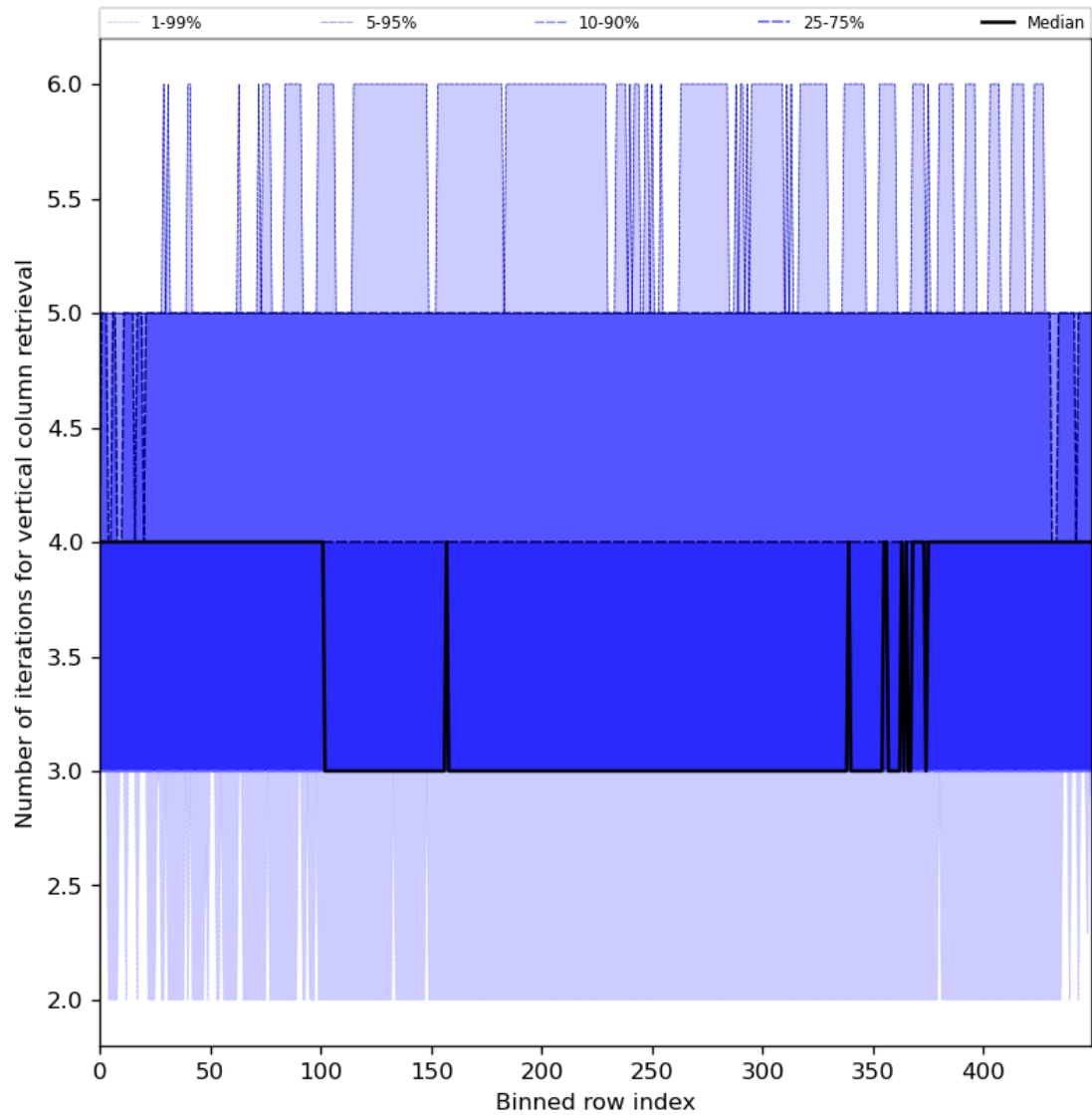
Figure 33: Along track statistics of “Number of iterations for vertical column retrieval” for 2024-02-27 to 2024-02-28
