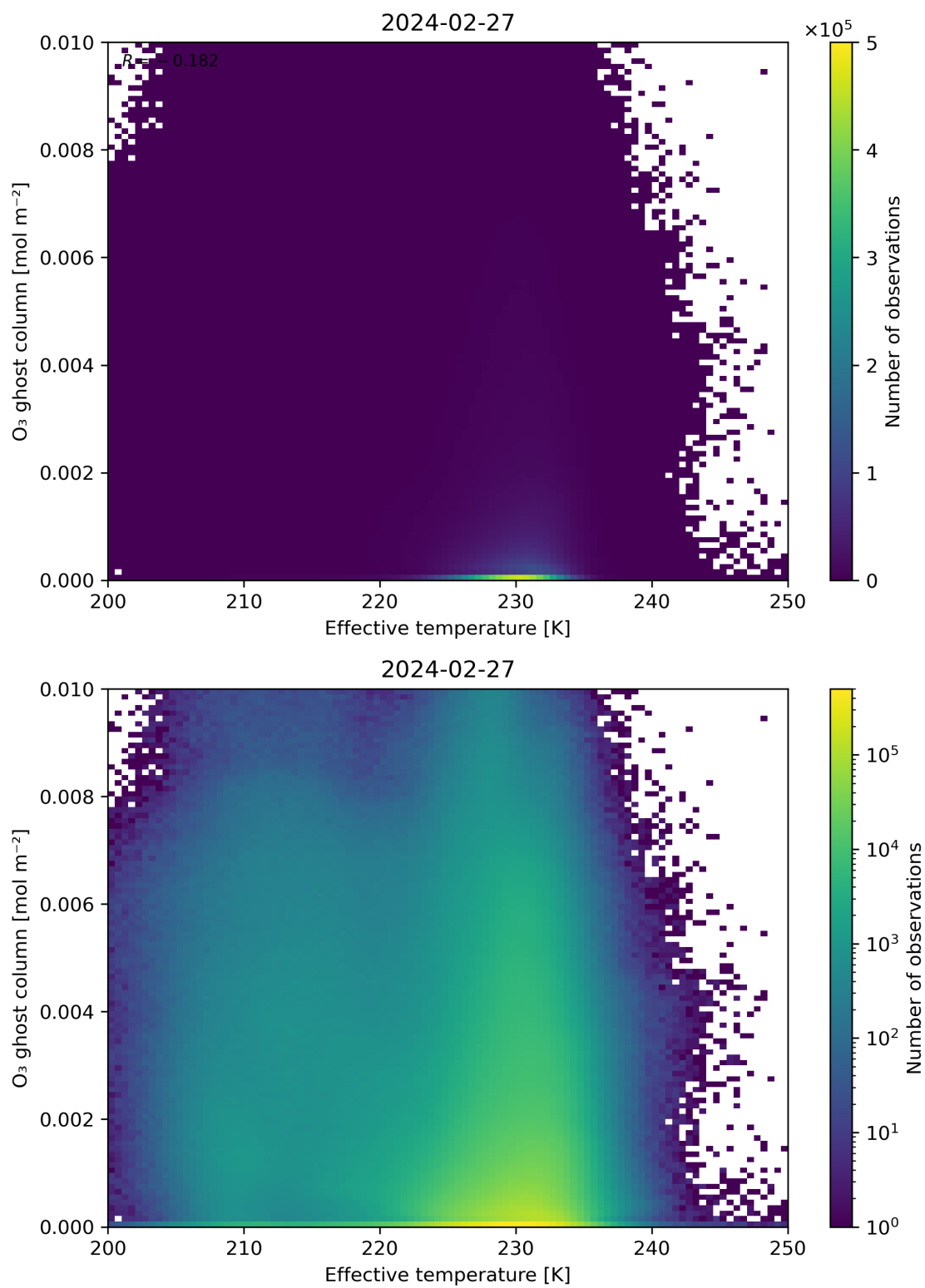
Figure 38: Scatter density plot of “Effective temperature” against “O 3 ghost column” for 2024-02-27 to 2024-02-28.
