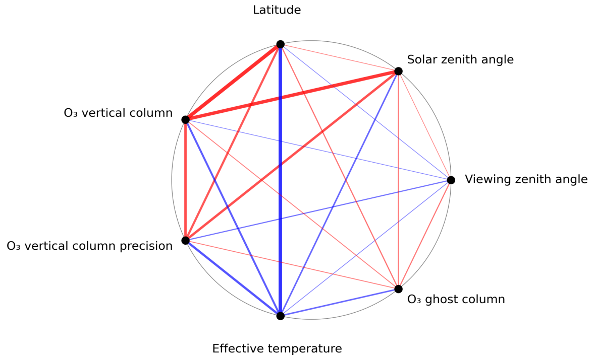
Figure 1: Map of correlation graph for 2024-02-27 to 2024-02-28.
