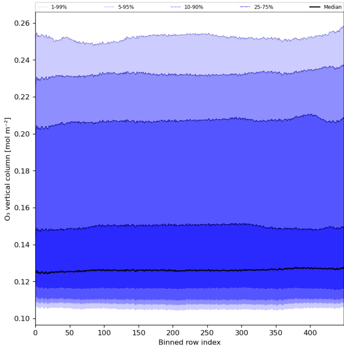
Figure 28: Along track statistics of “O 3 vertical column” for 2024-02-27 to 2024-02-28
