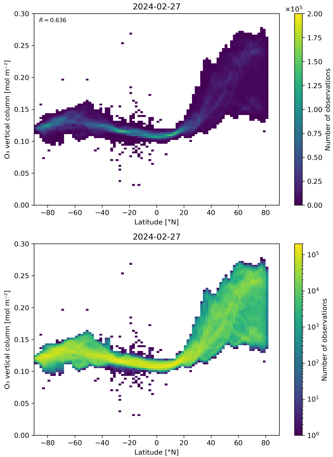
Figure 36: Scatter density plot of “Latitude” against “O 3 vertical column” for 2024-02-27 to 2024-02-28.
