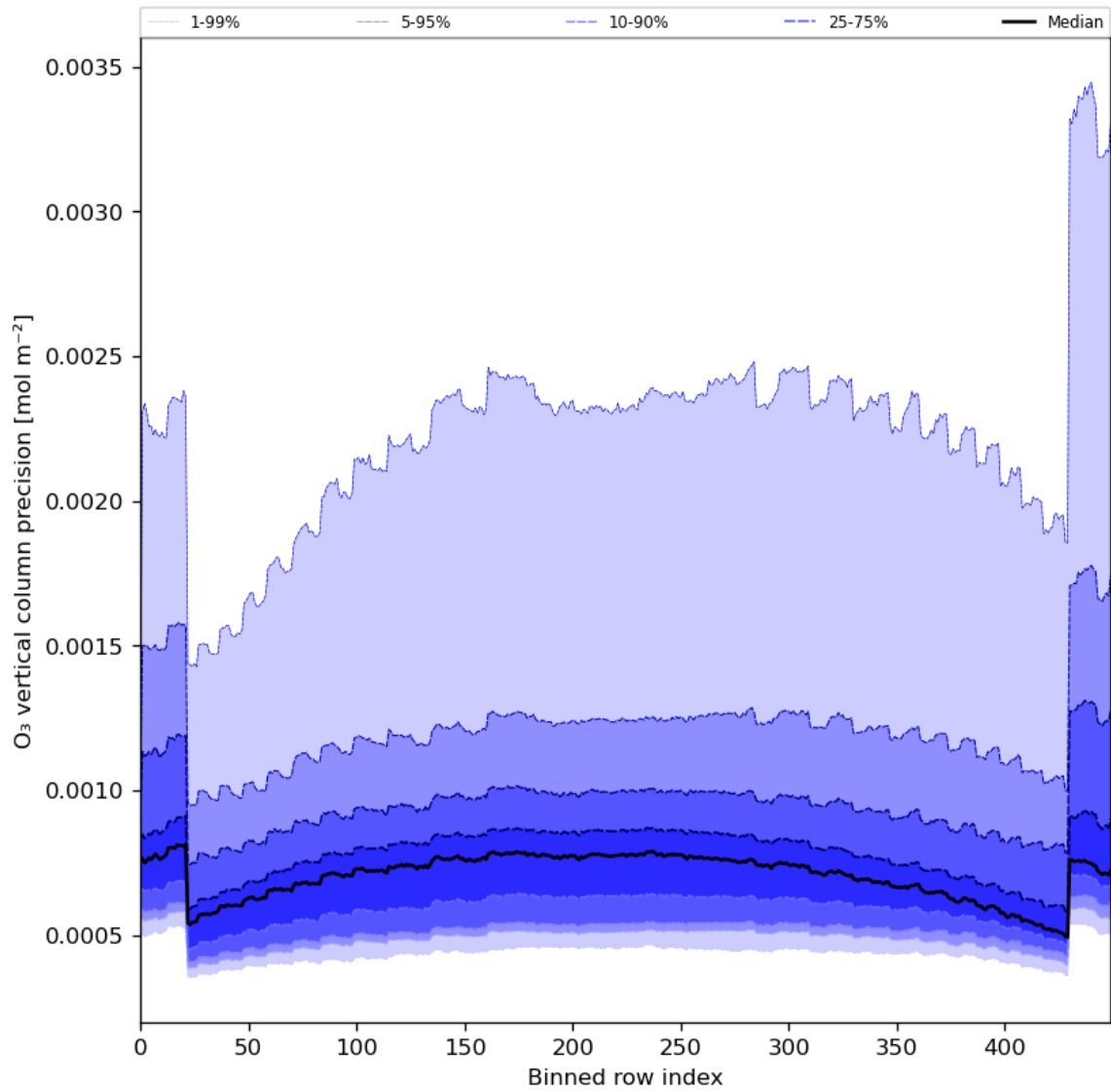
Figure 29: Along track statistics of “O 3 vertical column precision” for 2024-02-27 to 2024-02-28
