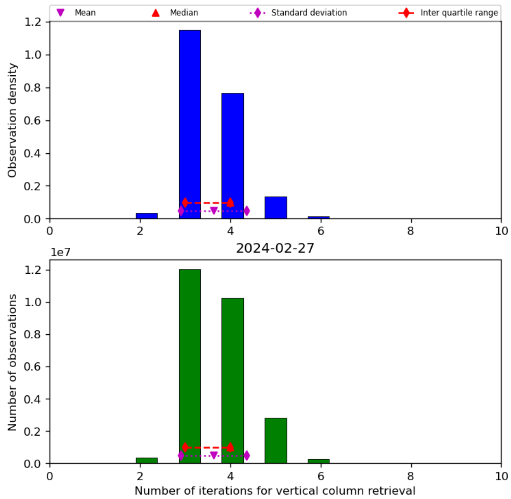
Figure 26: Histogram of “Number of iterations for vertical column retrieval” for 2024-02-27 to 2024-02-28
