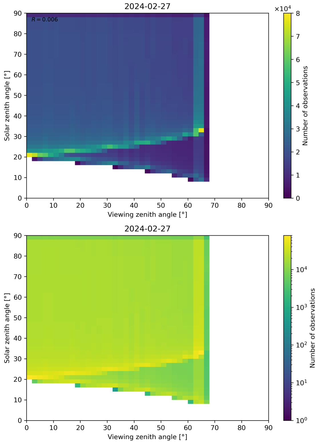
Figure 54: Scatter density plot of “Viewing zenith angle” against “Solar zenith angle” for 2024-02-27 to 2024-02-28.
