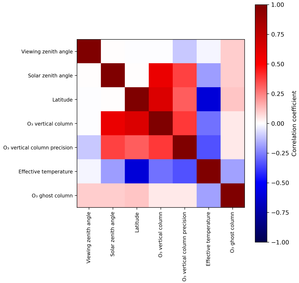
Figure 2: Map of correlation matrix for 2024-02-27 to 2024-02-28.
