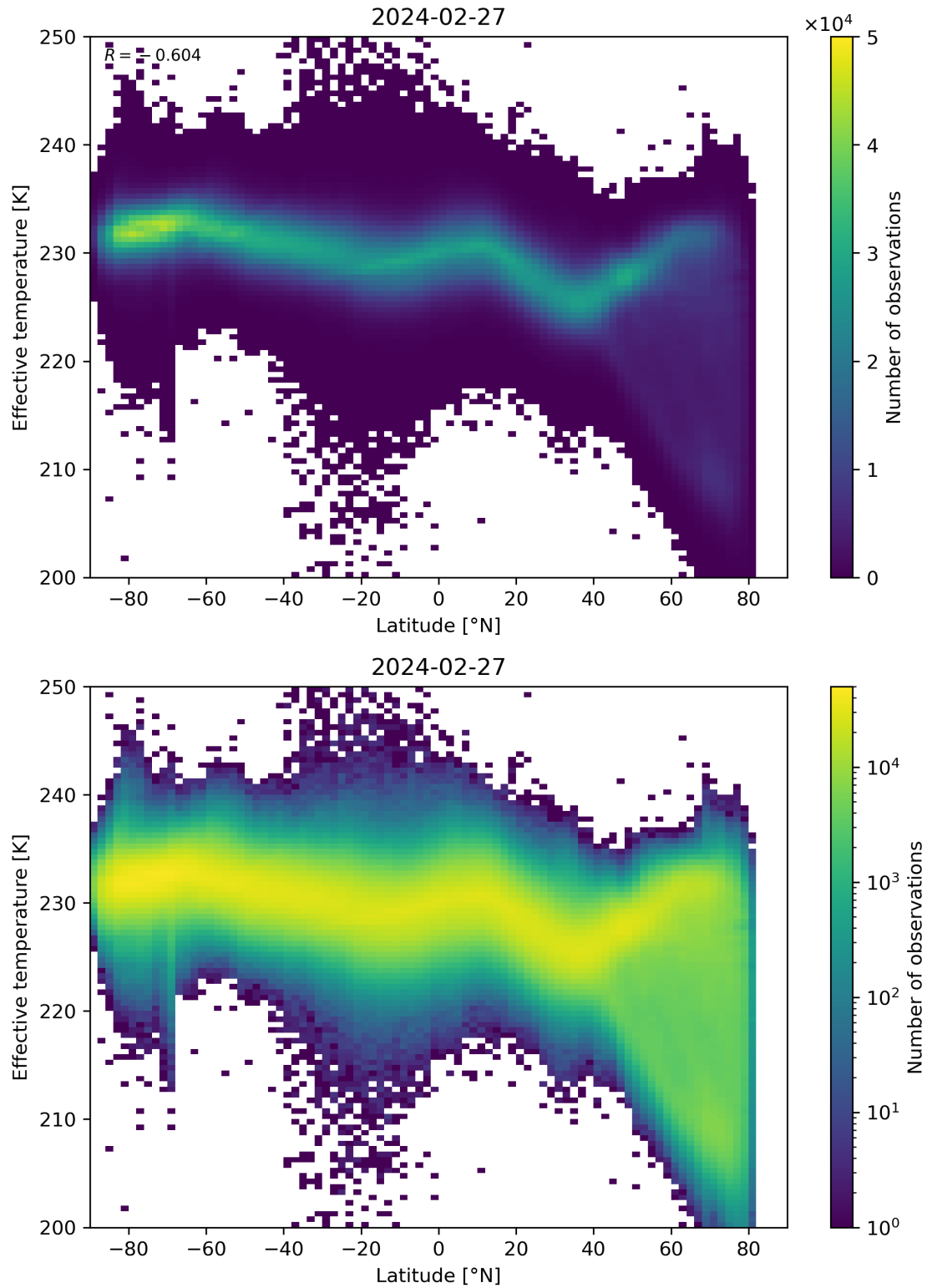
Figure 34: Scatter density plot of “Latitude” against “Effective temperature” for 2024-02-27 to 2024-02-28.
