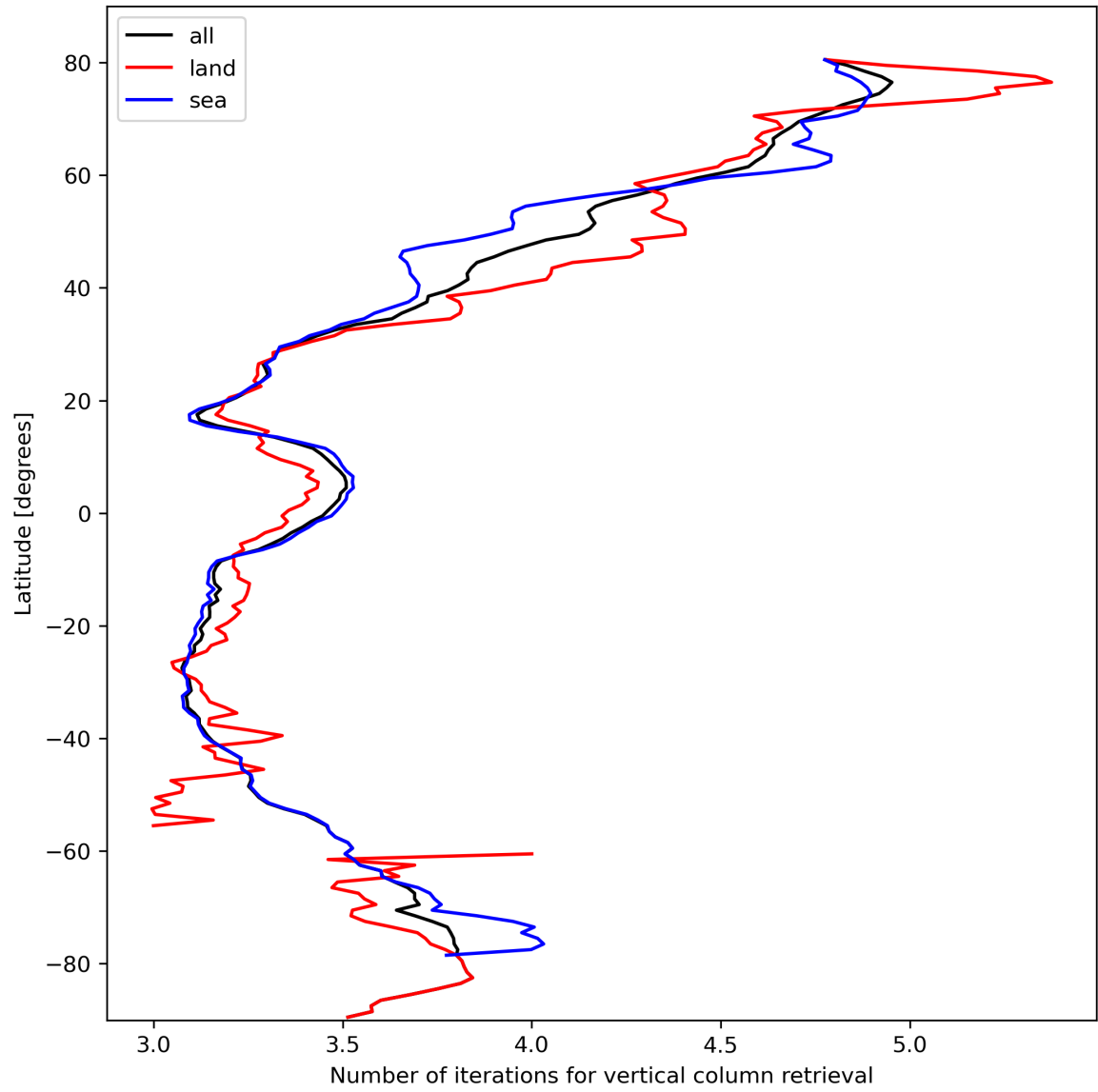
Figure 19: Zonal average of “Number of iterations for vertical column retrieval” for 2024-02-27 to 2024-02-28.
