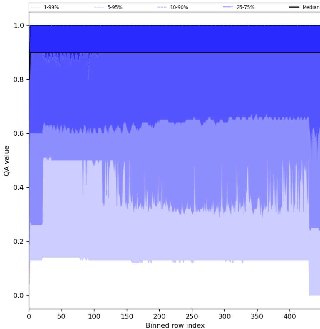
Figure 27: Along track statistics of “QA value” for 2024-02-27 to 2024-02-28
