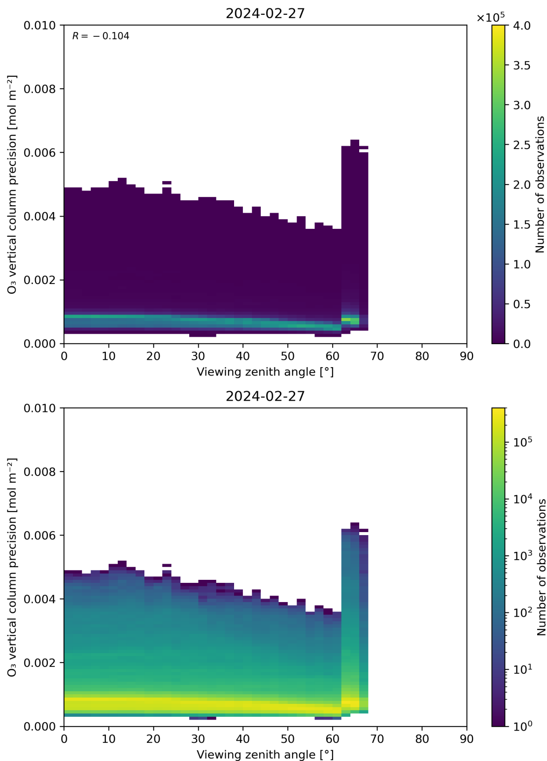
Figure 53: Scatter density plot of “Viewing zenith angle” against “O 3 vertical column precision” for 2024-02-27 to 2024-02-28.
