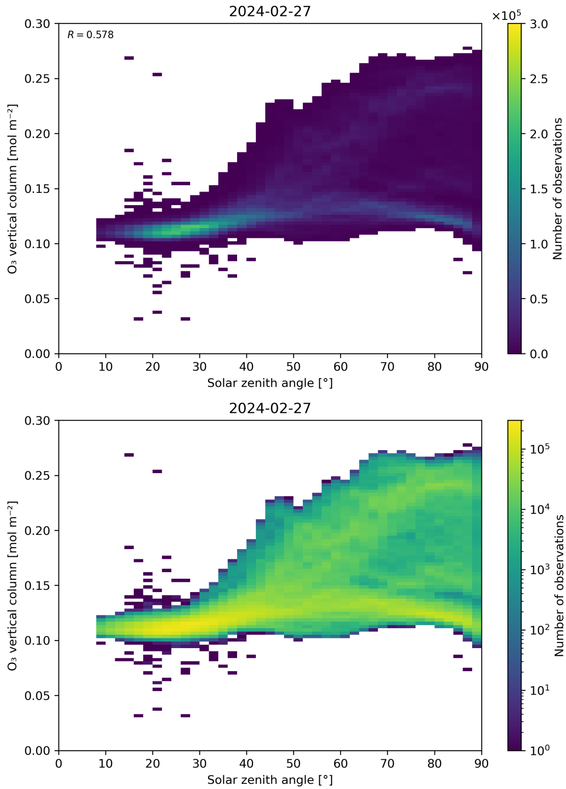
Figure 47: Scatter density plot of “Solar zenith angle” against “O 3 vertical column” for 2024-02-27 to 2024-02-28.
