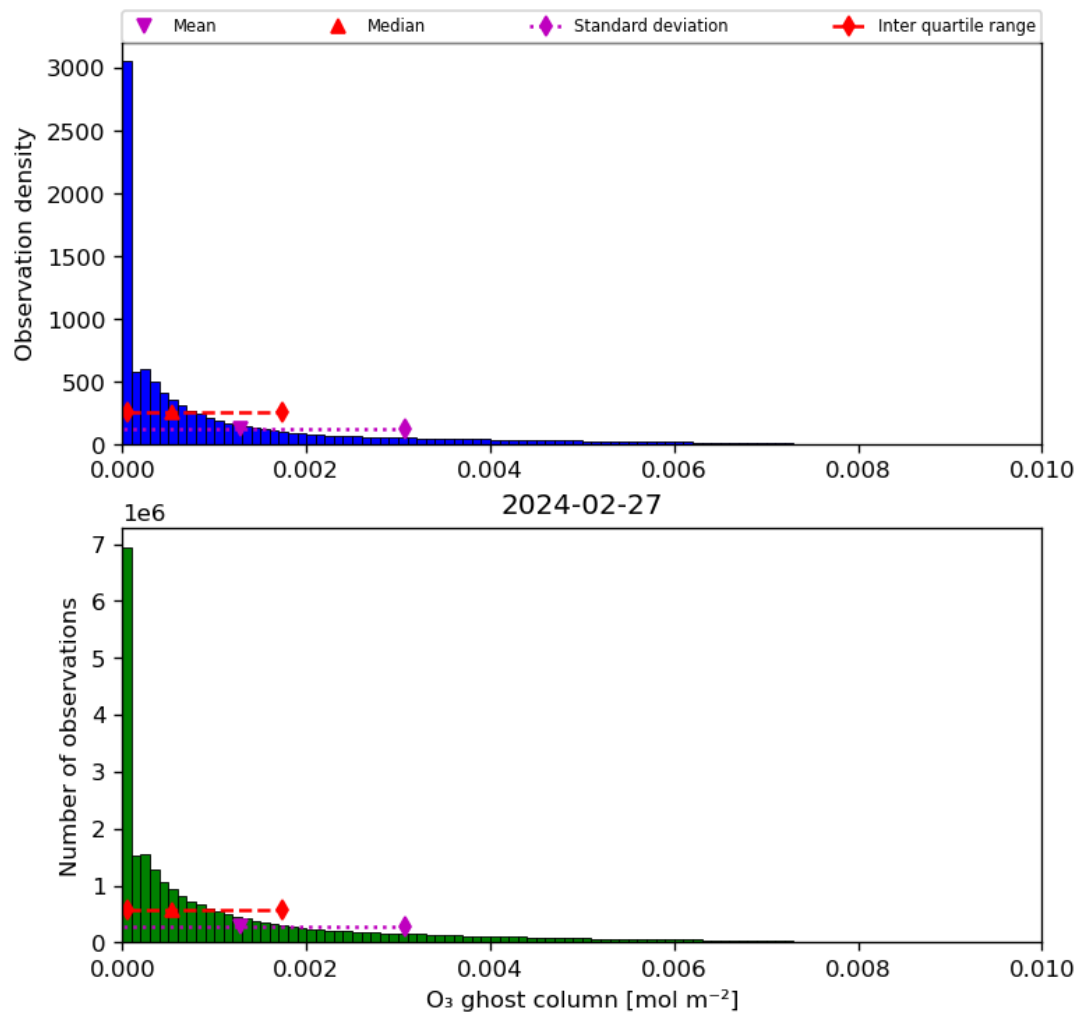
Figure 25: Histogram of “O 3 ghost column” for 2024-02-27 to 2024-02-28
