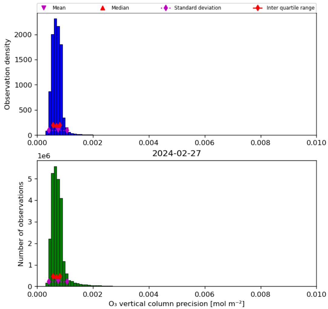
Figure 22: Histogram of “O 3 vertical column precision” for 2024-02-27 to 2024-02-28
