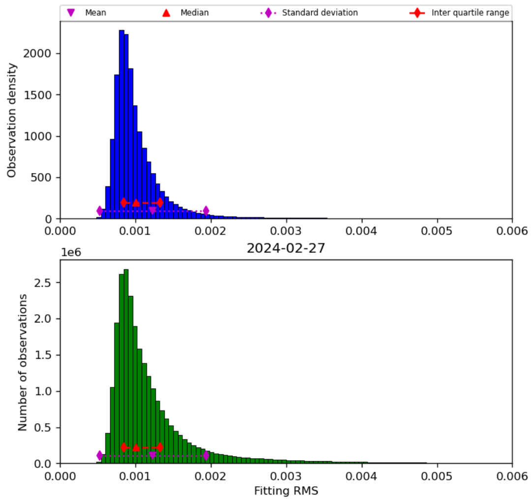
Figure 23: Histogram of “Fitting RMS” for 2024-02-27 to 2024-02-28
