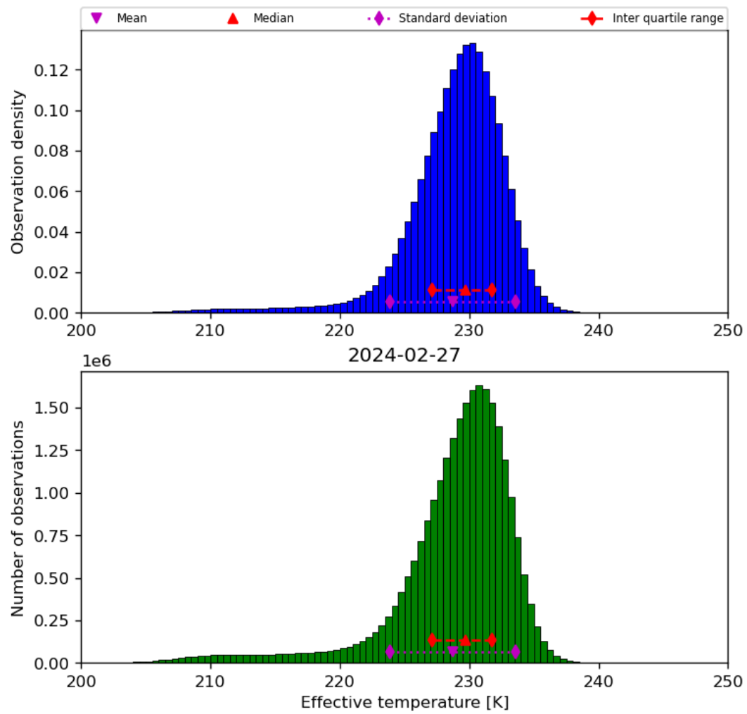
Figure 24: Histogram of “Effective temperature” for 2024-02-27 to 2024-02-28
