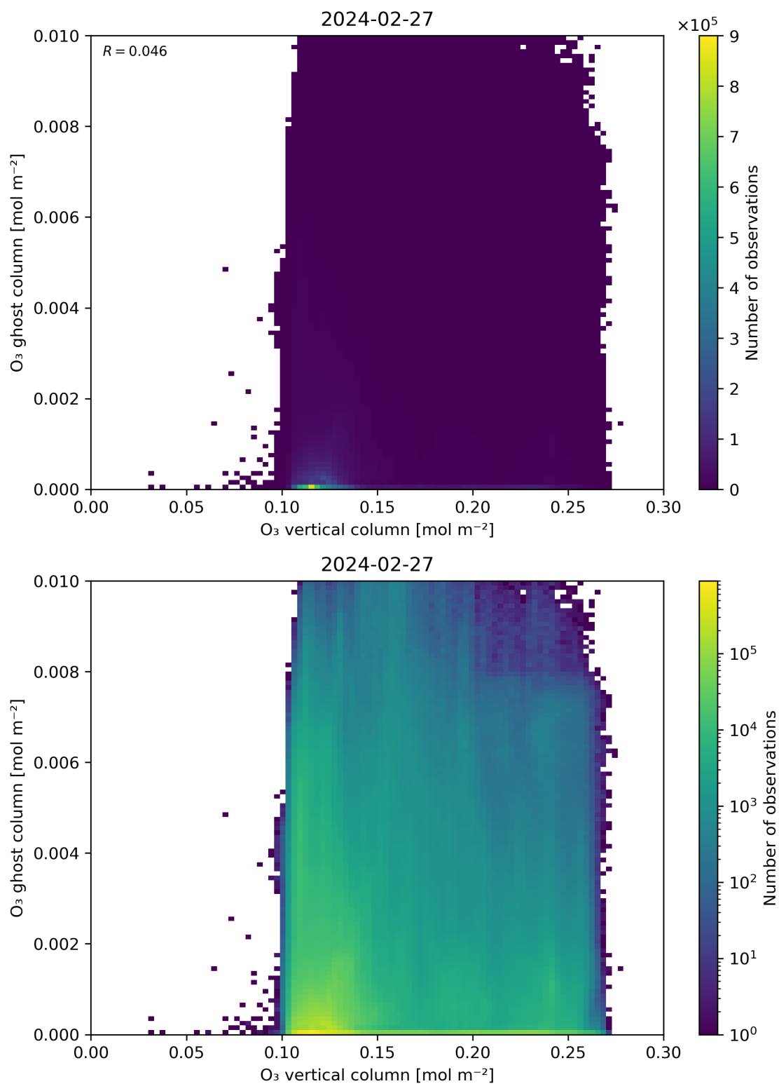
Figure 40: Scatter density plot of “O 3 vertical column” against “O 3 ghost column” for 2024-02-27 to 2024-02-28.
