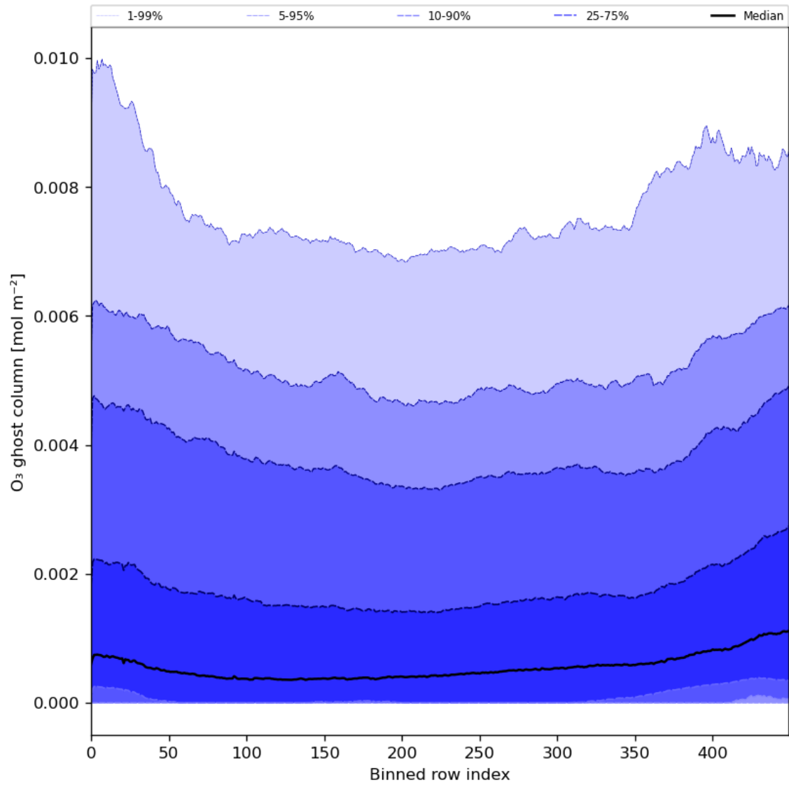
Figure 32: Along track statistics of "O 3 ghost column" for 2024-02-27 to 2024-02-28
