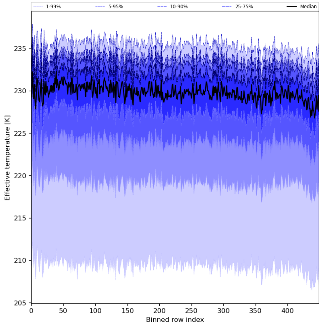
Figure 31: Along track statistics of “Effective temperature” for 2024-02-27 to 2024-02-28
