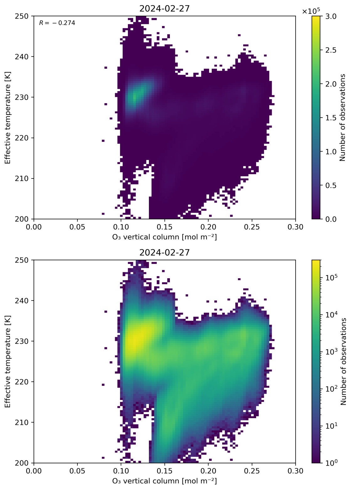
Figure 39: Scatter density plot of “O 3 vertical column” against “Effective temperature” for 2024-02-27 to 2024-02-28.
