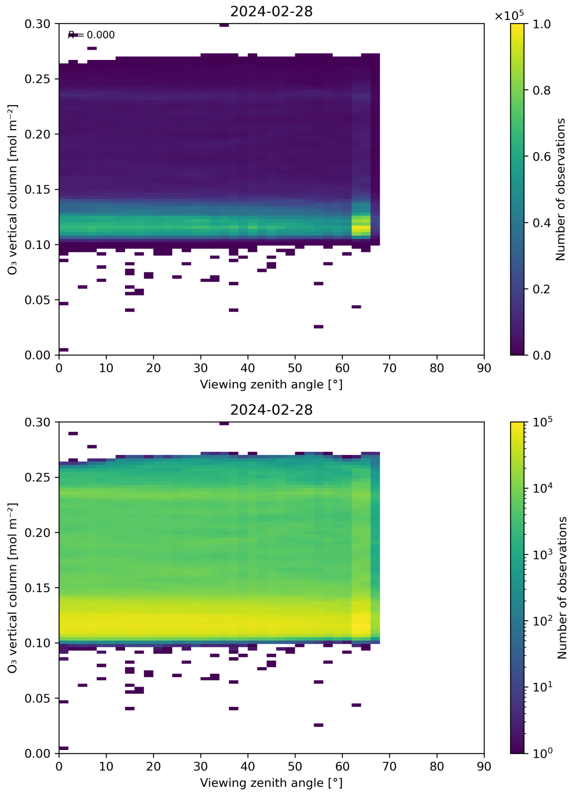
Figure 52: Scatter density plot of “Viewing zenith angle” against “O 3 vertical column” for 2024-02-27 to 2024-02-29.
