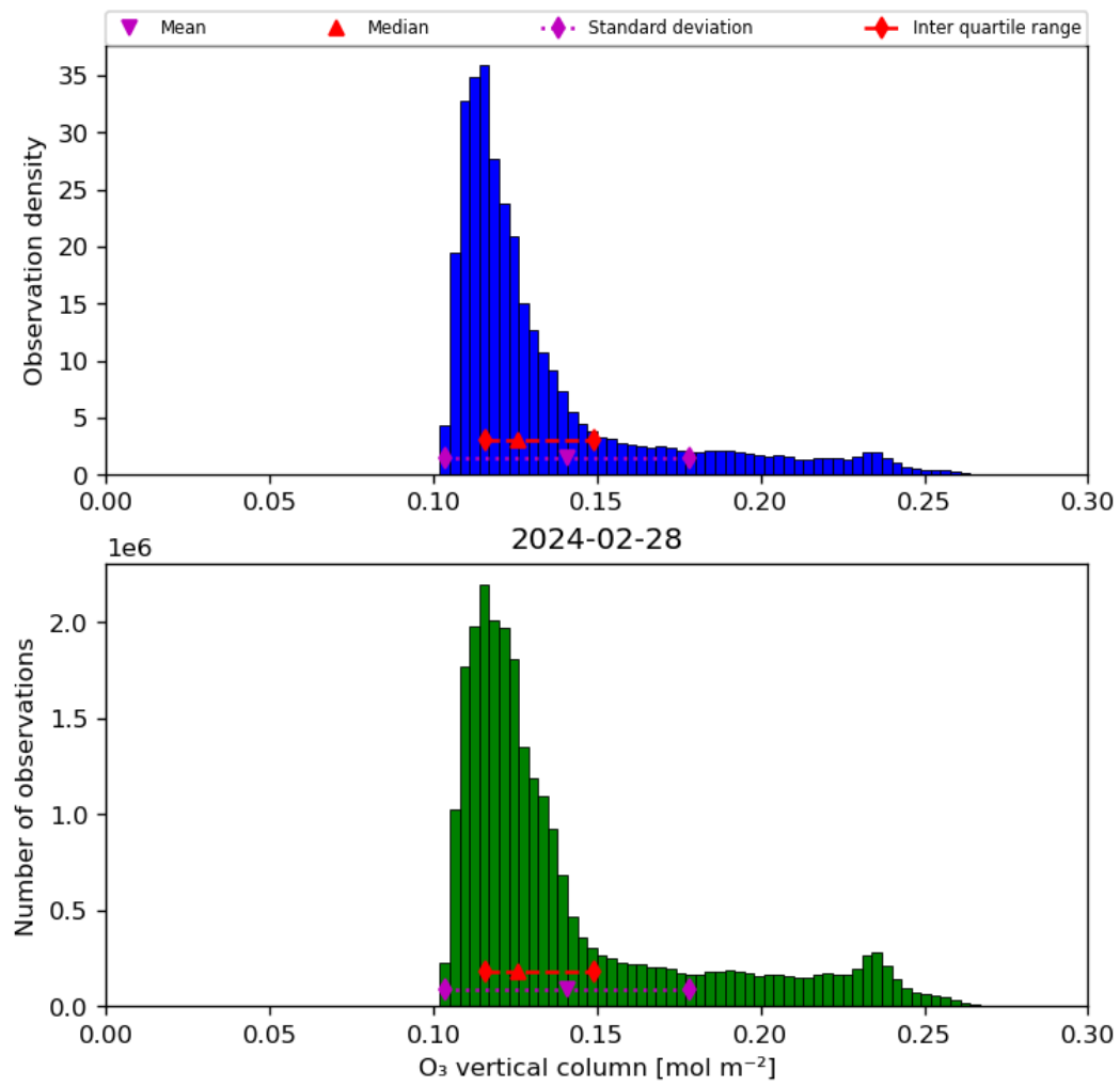
Figure 21: Histogram of “O 3 vertical column” for 2024-02-27 to 2024-02-29
