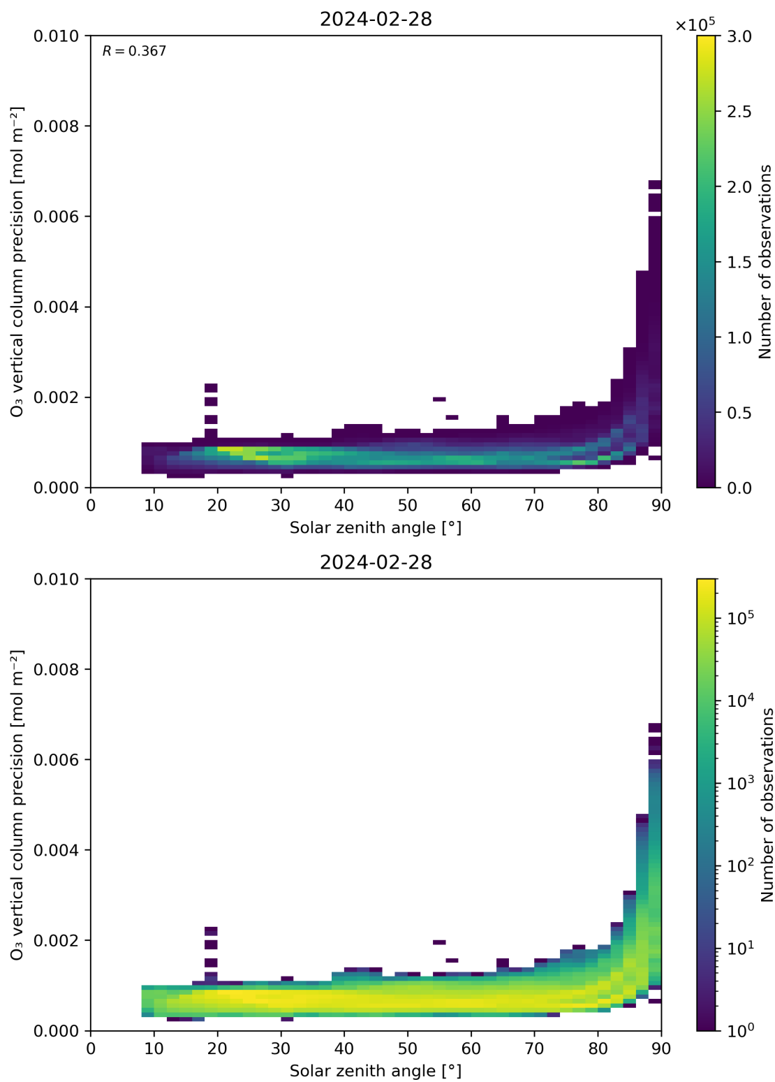
Figure 48: Scatter density plot of “Solar zenith angle” against “O 3 vertical column precision” for 2024-02-27 to 2024-02-29.
