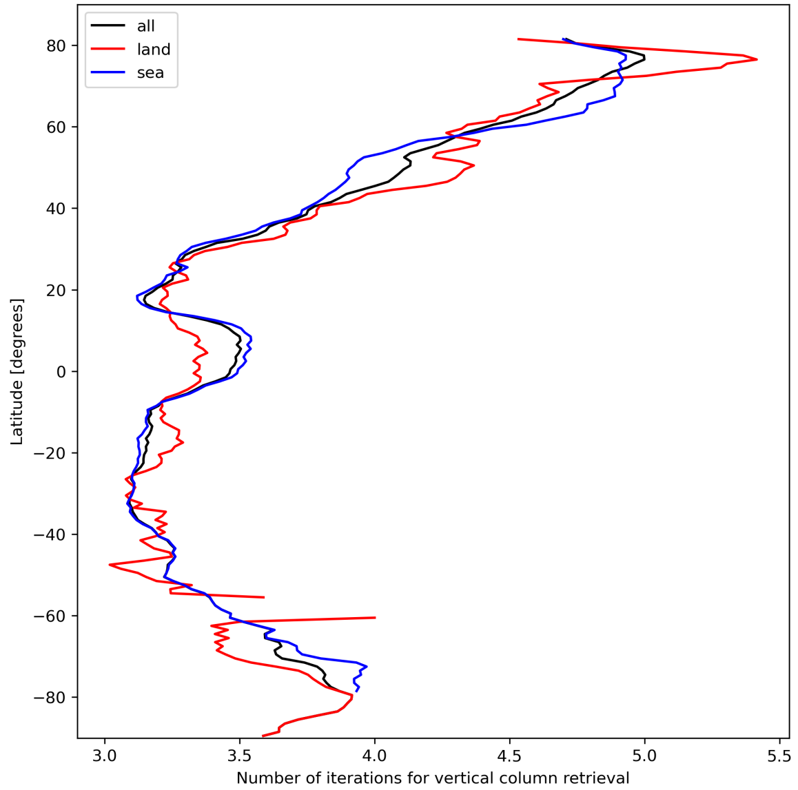
Figure 19: Zonal average of “Number of iterations for vertical column retrieval” for 2024-02-27 to 2024-02-29.
