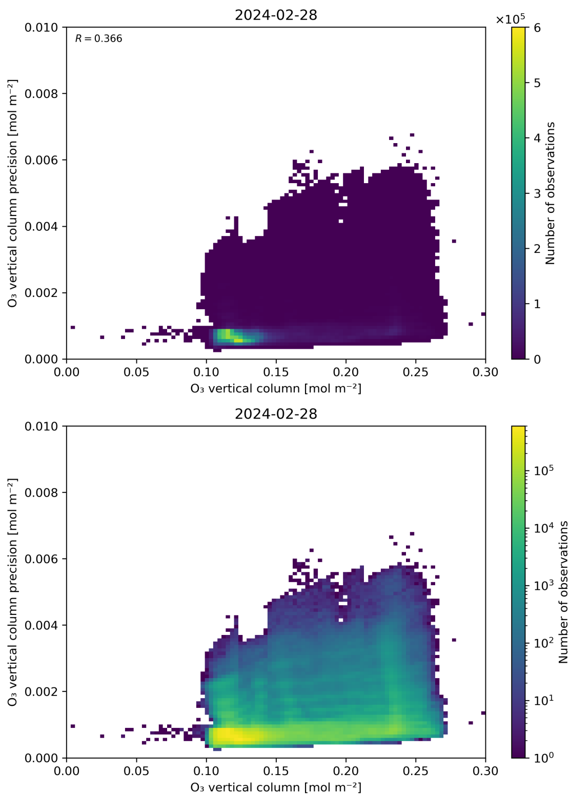
Figure 41: Scatter density plot of “O 3 vertical column” against “O 3 vertical column precision” for 2024-02-27 to 2024-02-29.
