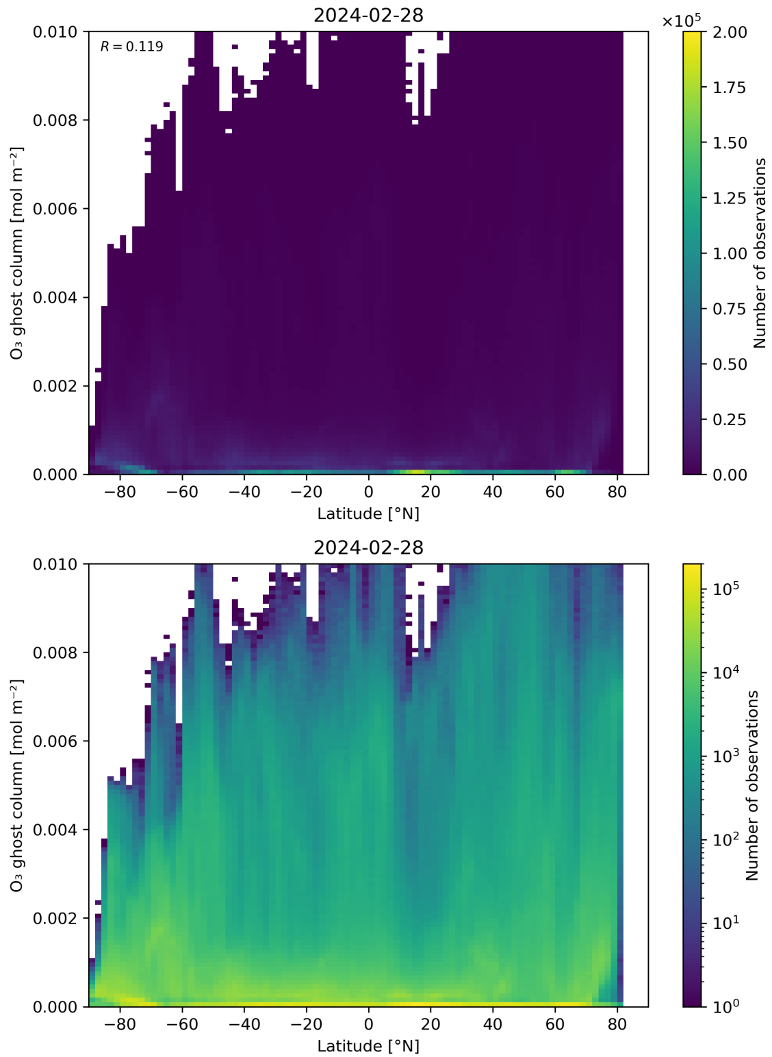
Figure 35: Scatter density plot of “Latitude” against “O 3 ghost column” for 2024-02-27 to 2024-02-29.
