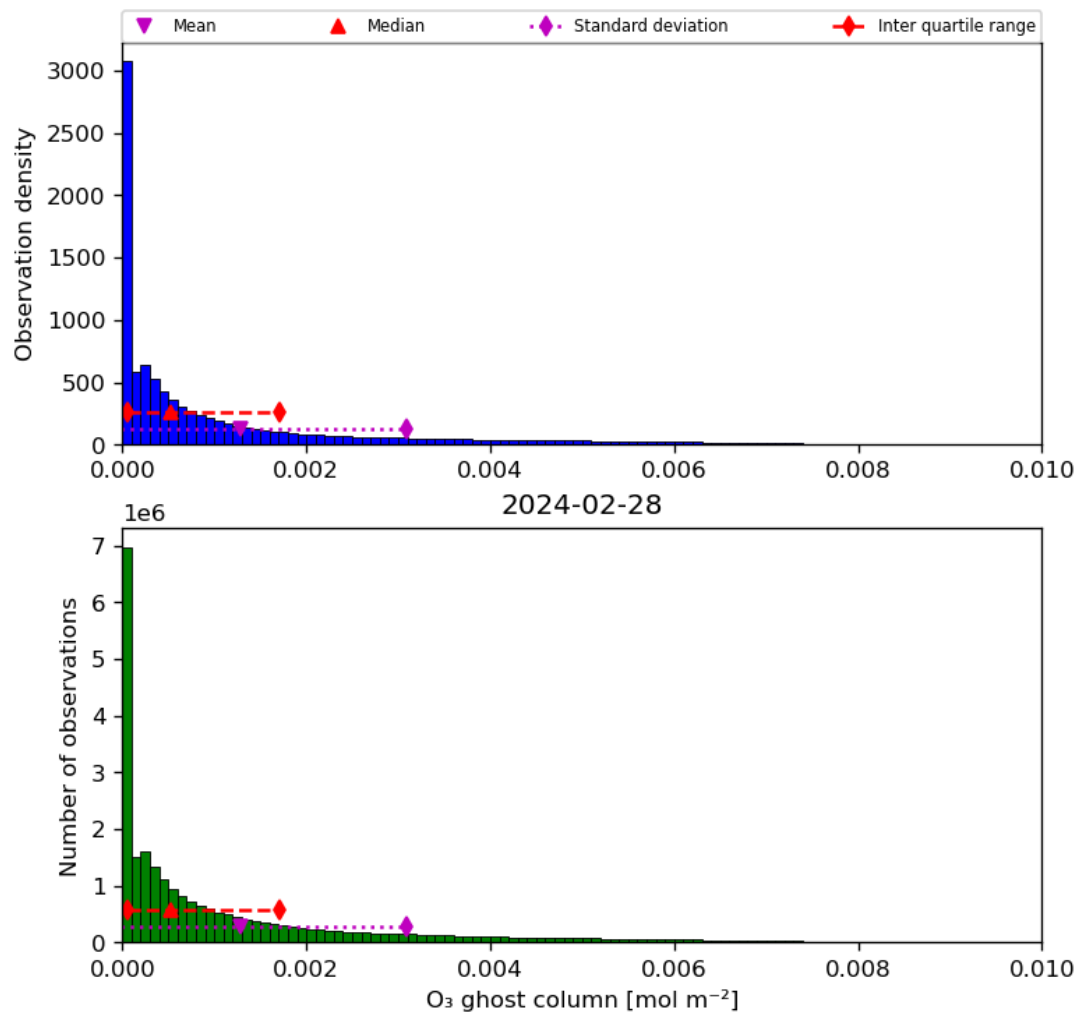
Figure 25: Histogram of “O 3 ghost column” for 2024-02-27 to 2024-02-29
