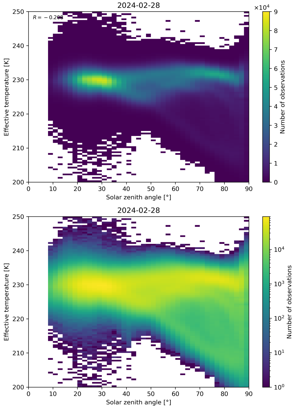
Figure 45: Scatter density plot of “Solar zenith angle” against “Effective temperature” for 2024-02-27 to 2024-02-29.
