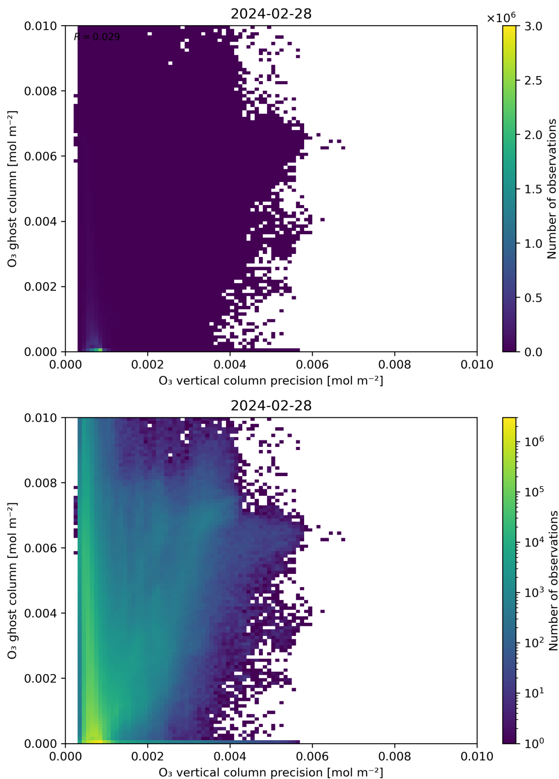
Figure 43: Scatter density plot of “ \text{O}_3 vertical column precision” against “ \text{O}_3 ghost column” for 2024-02-27 to 2024-02-29.
