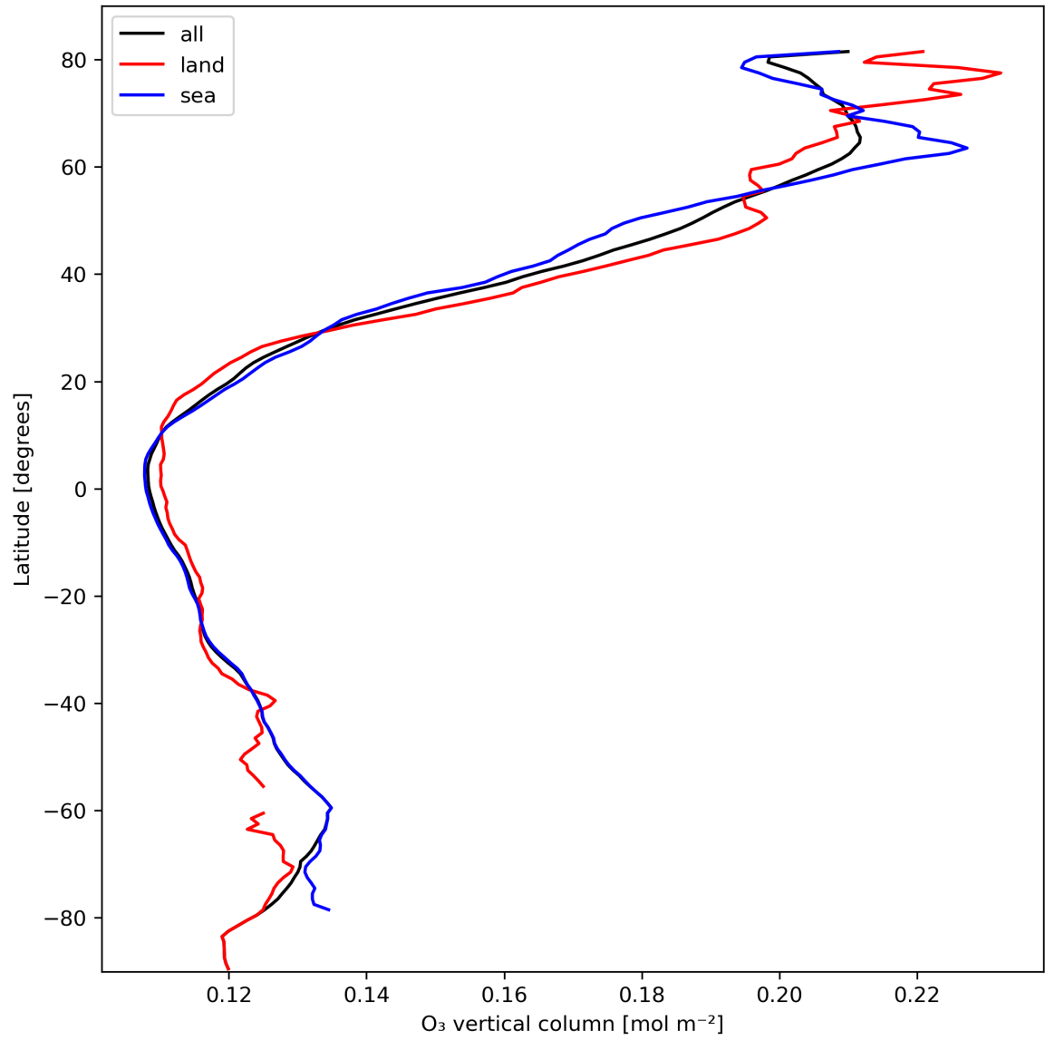
Figure 14: Zonal average of “O 3 vertical column” for 2024-02-27 to 2024-02-29.
