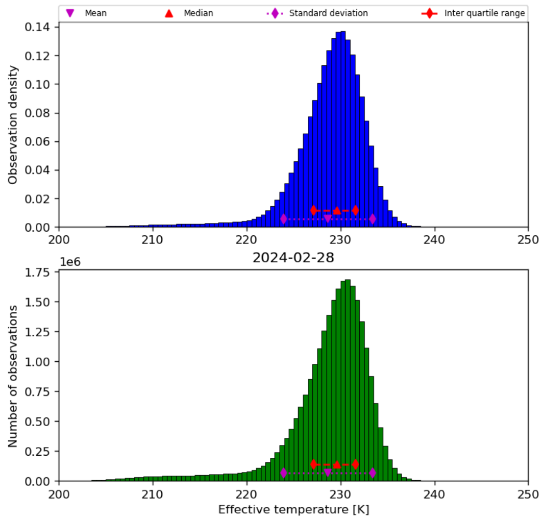
Figure 24: Histogram of “Effective temperature” for 2024-02-27 to 2024-02-29
