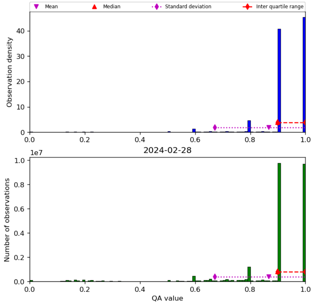
Figure 20: Histogram of “QA value” for 2024-02-27 to 2024-02-29
