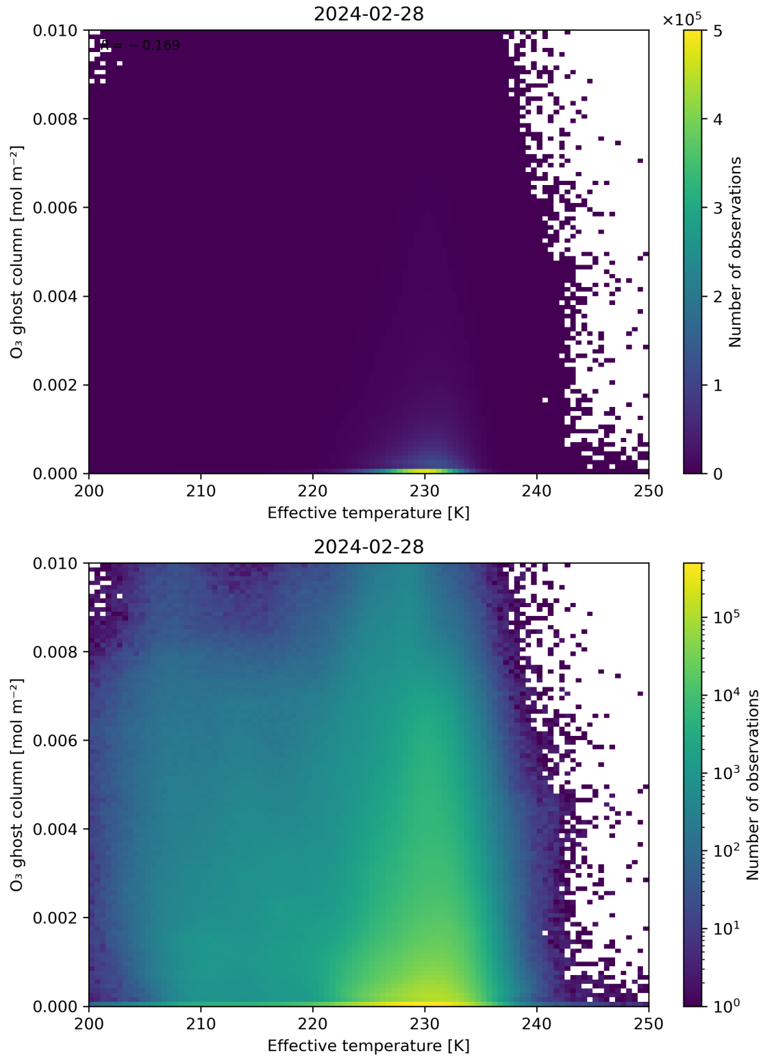
Figure 38: Scatter density plot of “Effective temperature” against “O 3 ghost column” for 2024-02-27 to 2024-02-29.
