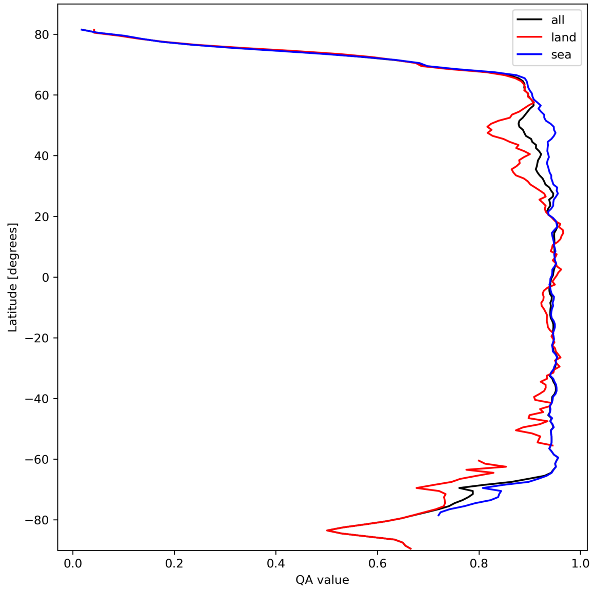
Figure 13: Zonal average of “QA value” for 2024-02-27 to 2024-02-29.
