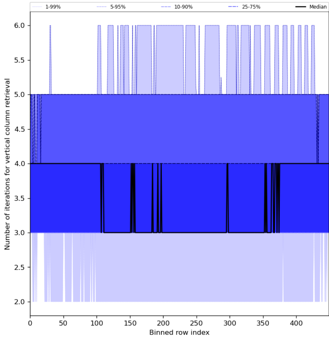
Figure 33: Along track statistics of “Number of iterations for vertical column retrieval” for 2024-02-27 to 2024-02-29
