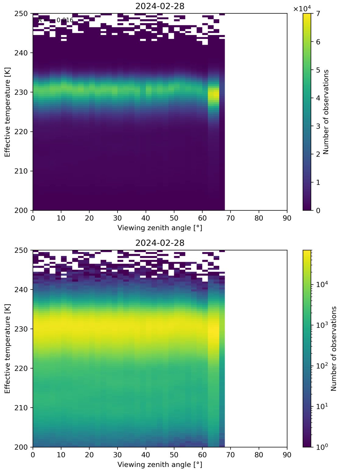
Figure 50: Scatter density plot of “Viewing zenith angle” against “Effective temperature” for 2024-02-27 to 2024-02-29.
