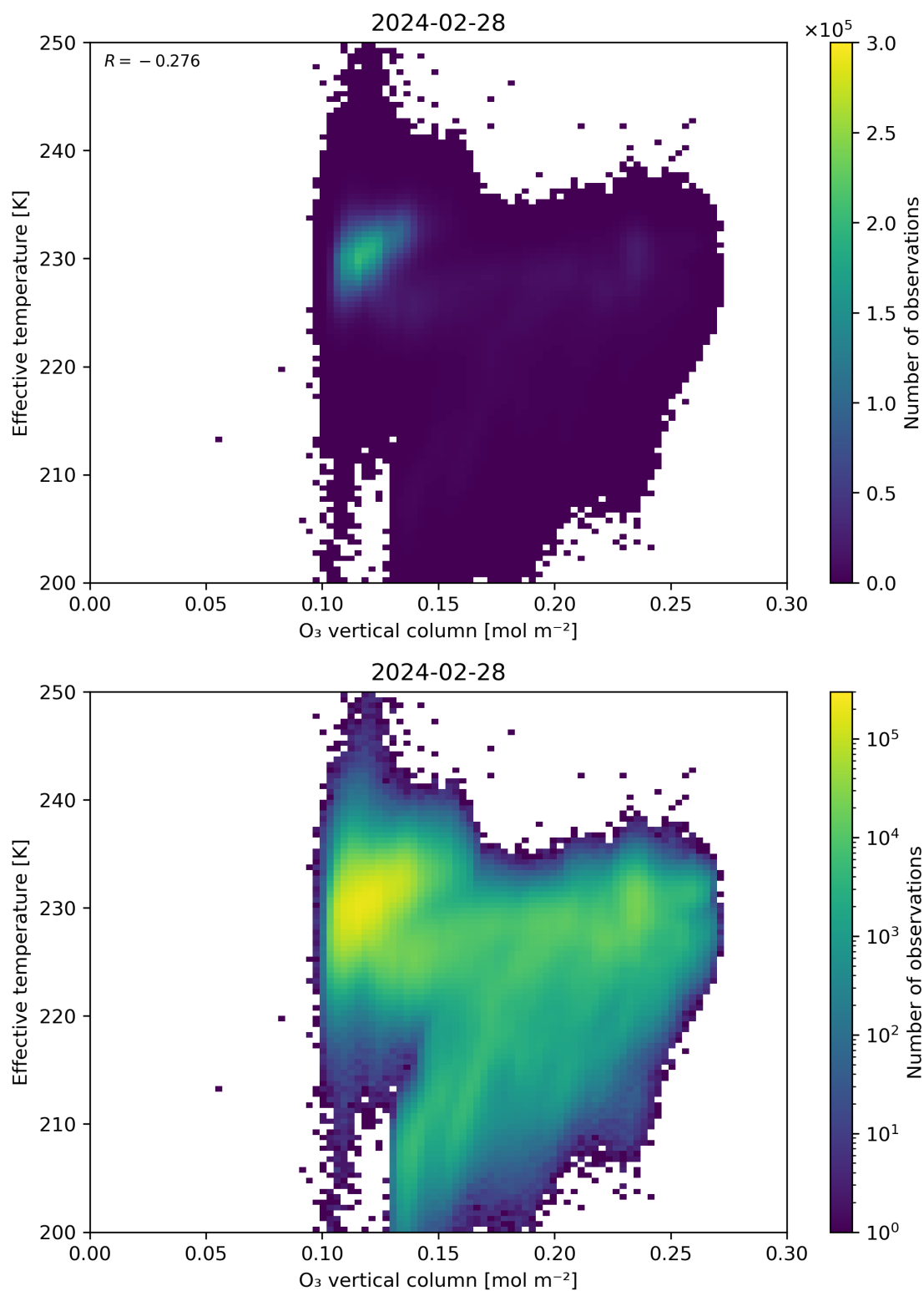
Figure 39: Scatter density plot of “O 3 vertical column” against “Effective temperature” for 2024-02-27 to 2024-02-29.
