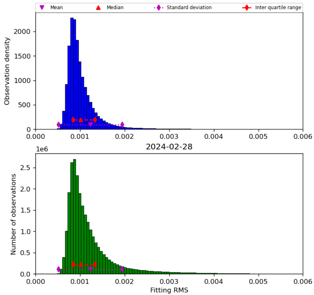
Figure 23: Histogram of “Fitting RMS” for 2024-02-27 to 2024-02-29
