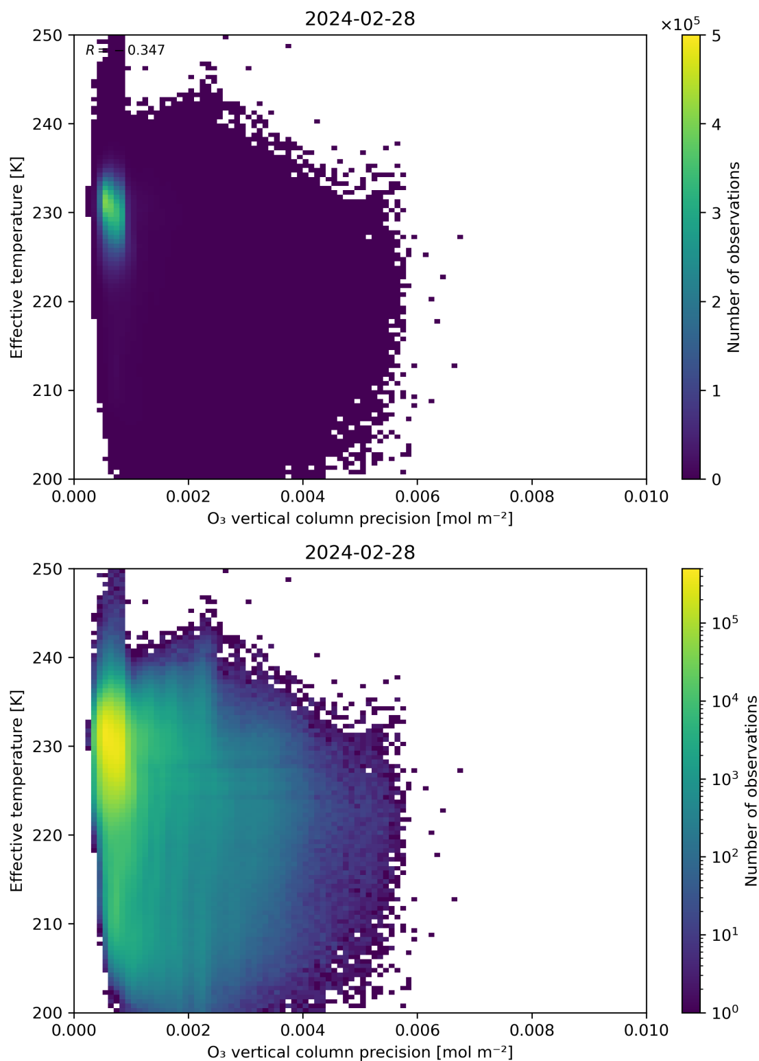
Figure 42: Scatter density plot of “O 3 vertical column precision” against “Effective temperature” for 2024-02-27 to 2024-02-29.
