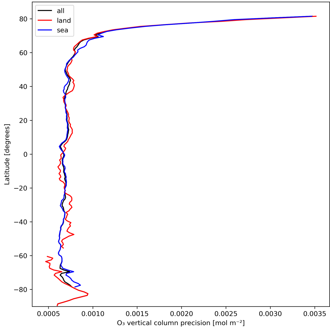
Figure 15: Zonal average of “O 3 vertical column precision” for 2024-02-27 to 2024-02-29.
