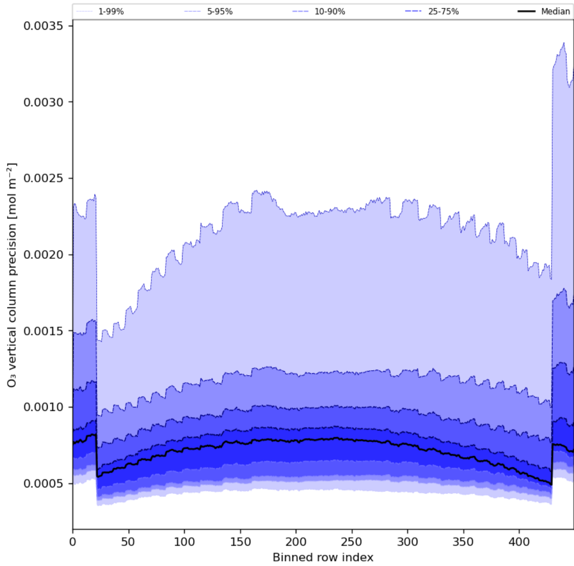
Figure 29: Along track statistics of “O 3 vertical column precision” for 2024-02-27 to 2024-02-29
