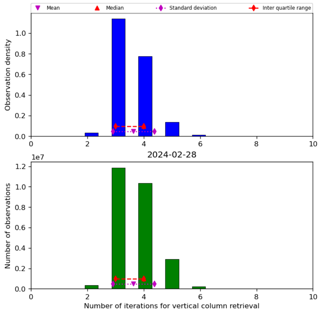
Figure 26: Histogram of “Number of iterations for vertical column retrieval” for 2024-02-27 to 2024-02-29
