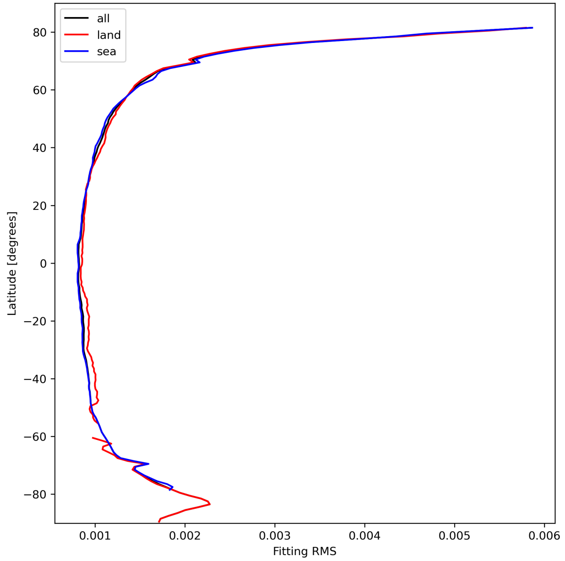
Figure 16: Zonal average of “Fitting RMS” for 2024-02-27 to 2024-02-29.
