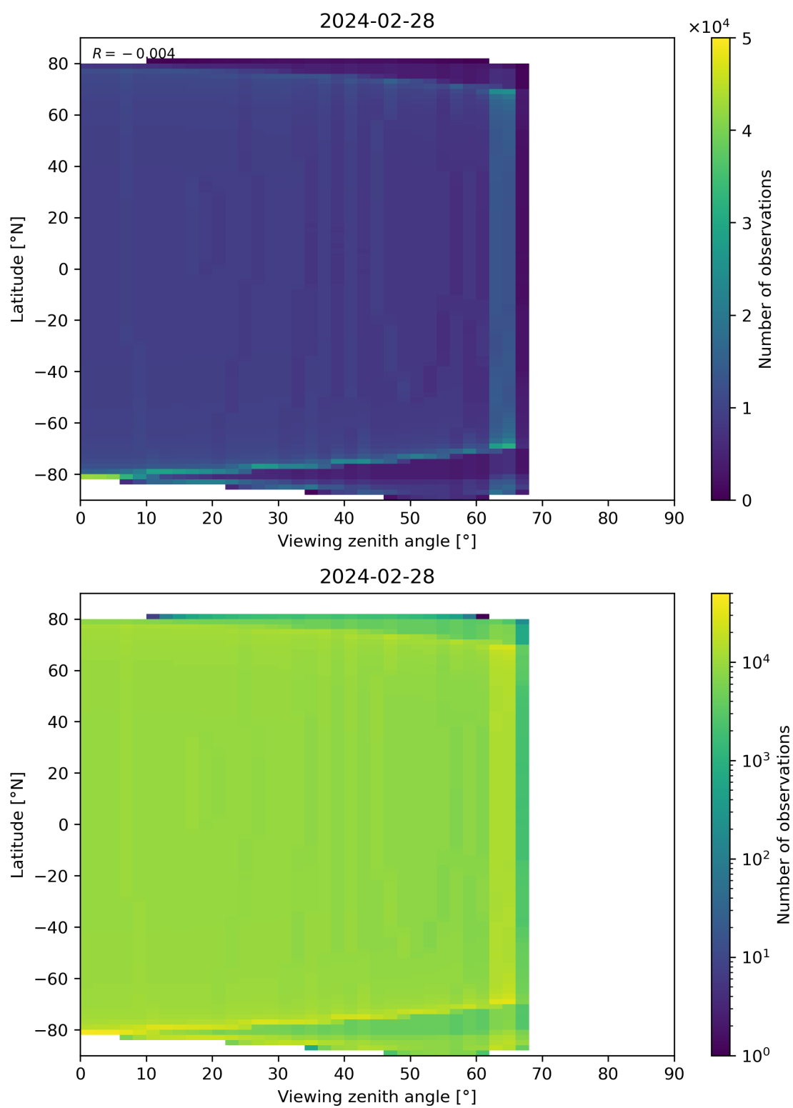
Figure 49: Scatter density plot of “Viewing zenith angle” against “Latitude” for 2024-02-27 to 2024-02-29.
