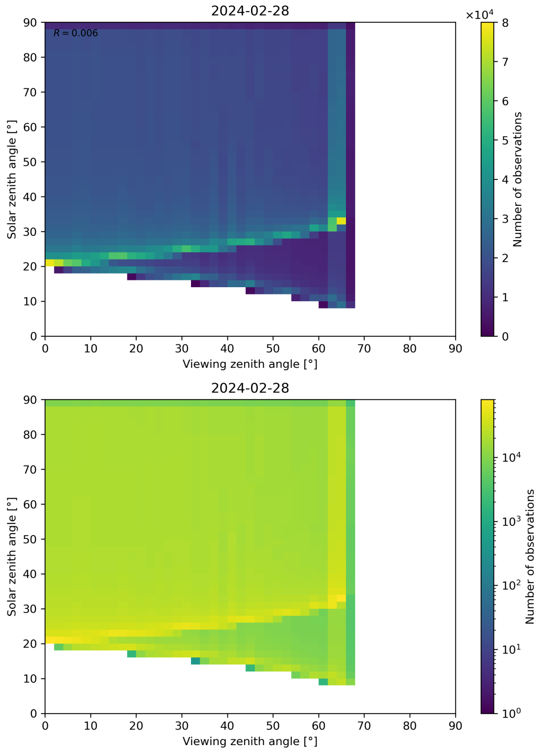
Figure 54: Scatter density plot of “Viewing zenith angle” against “Solar zenith angle” for 2024-02-27 to 2024-02-29.
