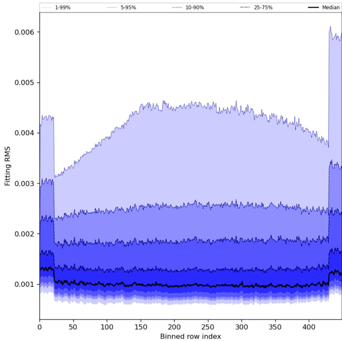
Figure 30: Along track statistics of “Fitting RMS” for 2024-02-27 to 2024-02-29
