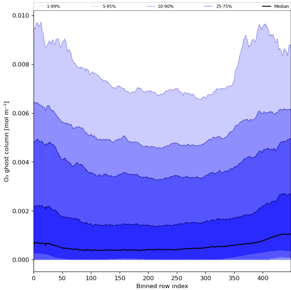
Figure 32: Along track statistics of “O 3 ghost column” for 2024-02-27 to 2024-02-29
