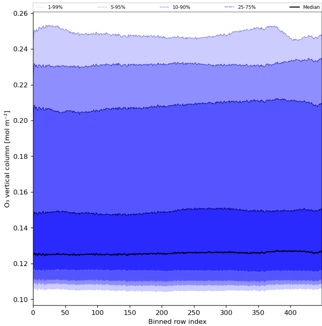
Figure 28: Along track statistics of “O 3 vertical column” for 2024-02-27 to 2024-02-29
