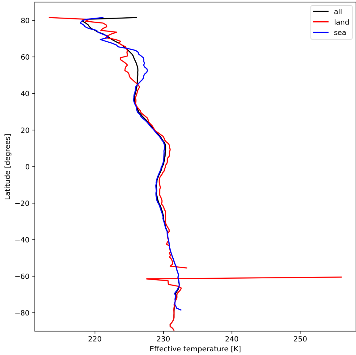
Figure 17: Zonal average of “Effective temperature” for 2024-02-27 to 2024-02-29.
