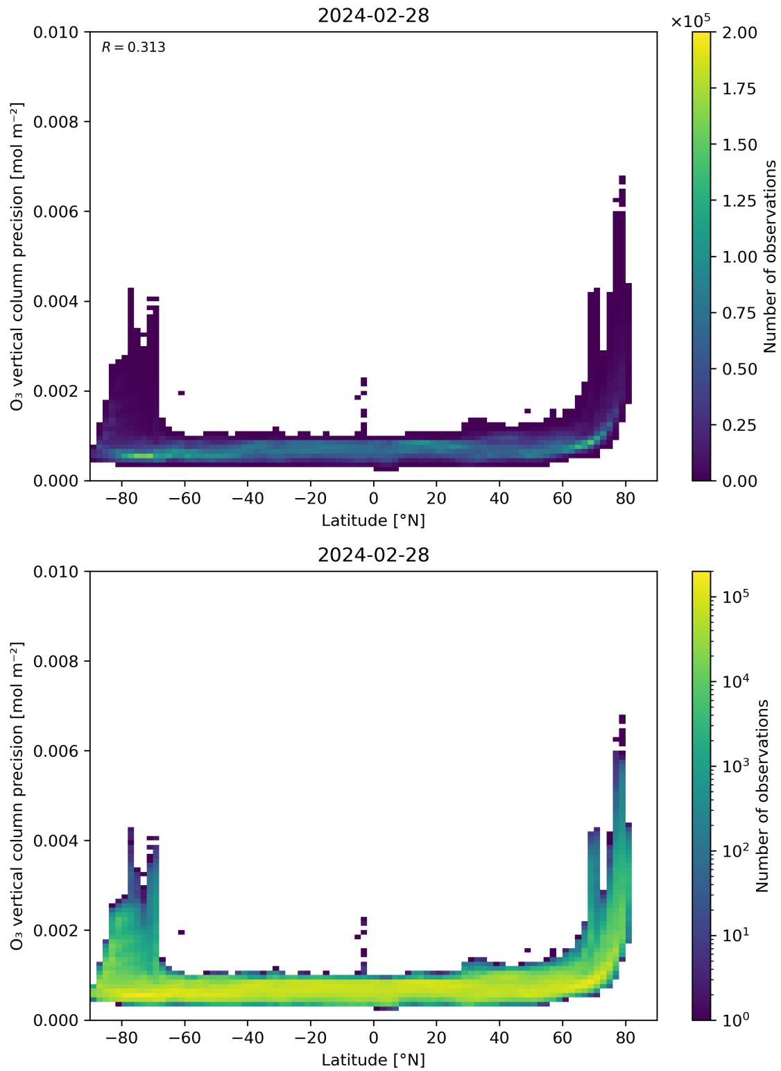
Figure 37: Scatter density plot of “Latitude” against “O 3 vertical column precision” for 2024-02-27 to 2024-02-29.
