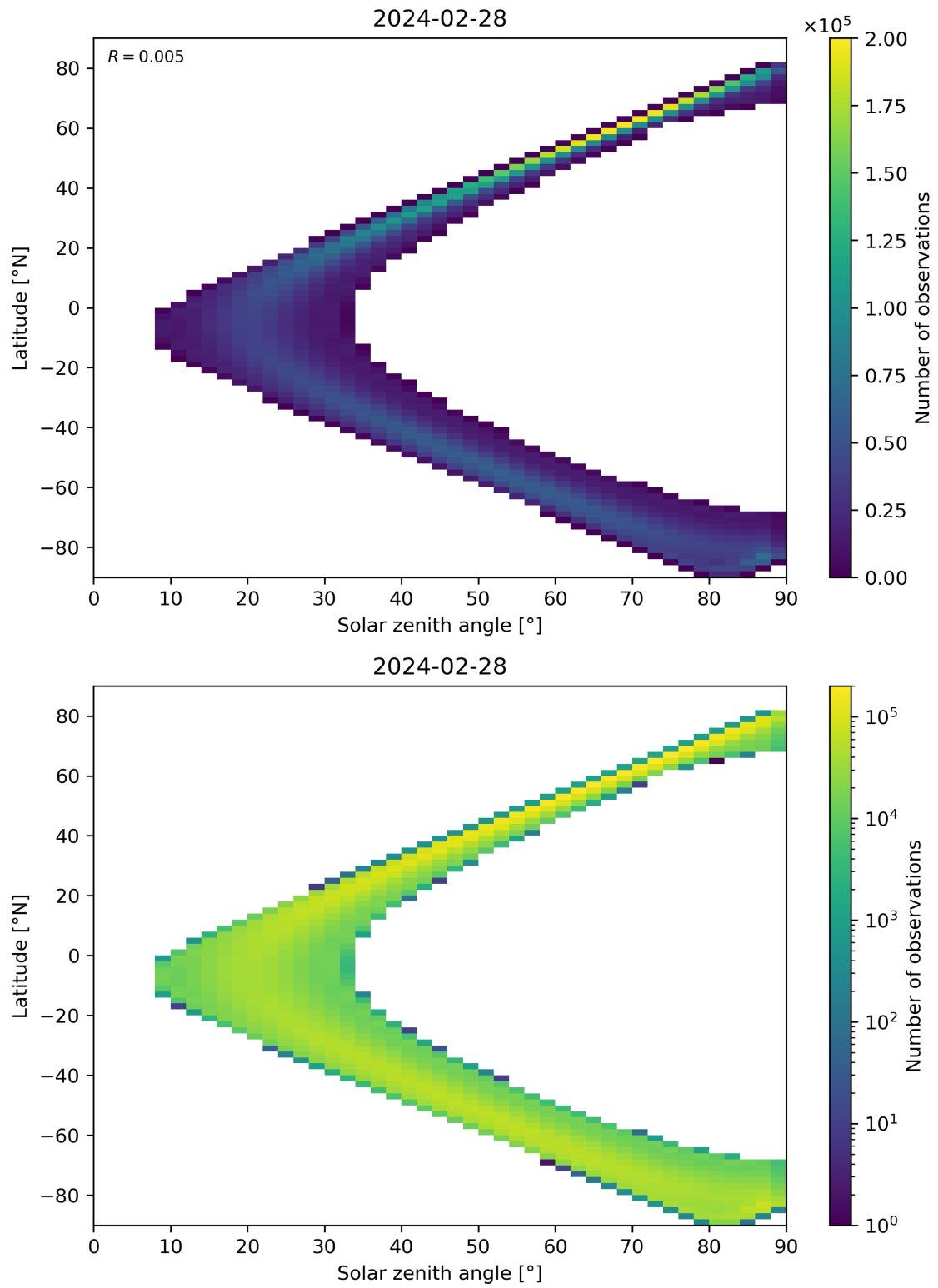
Figure 44: Scatter density plot of “Solar zenith angle” against “Latitude” for 2024-02-27 to 2024-02-29.
