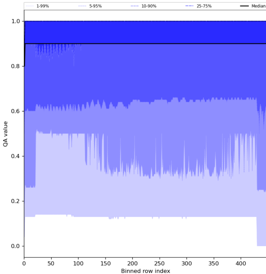
Figure 27: Along track statistics of “QA value” for 2024-02-27 to 2024-02-29
