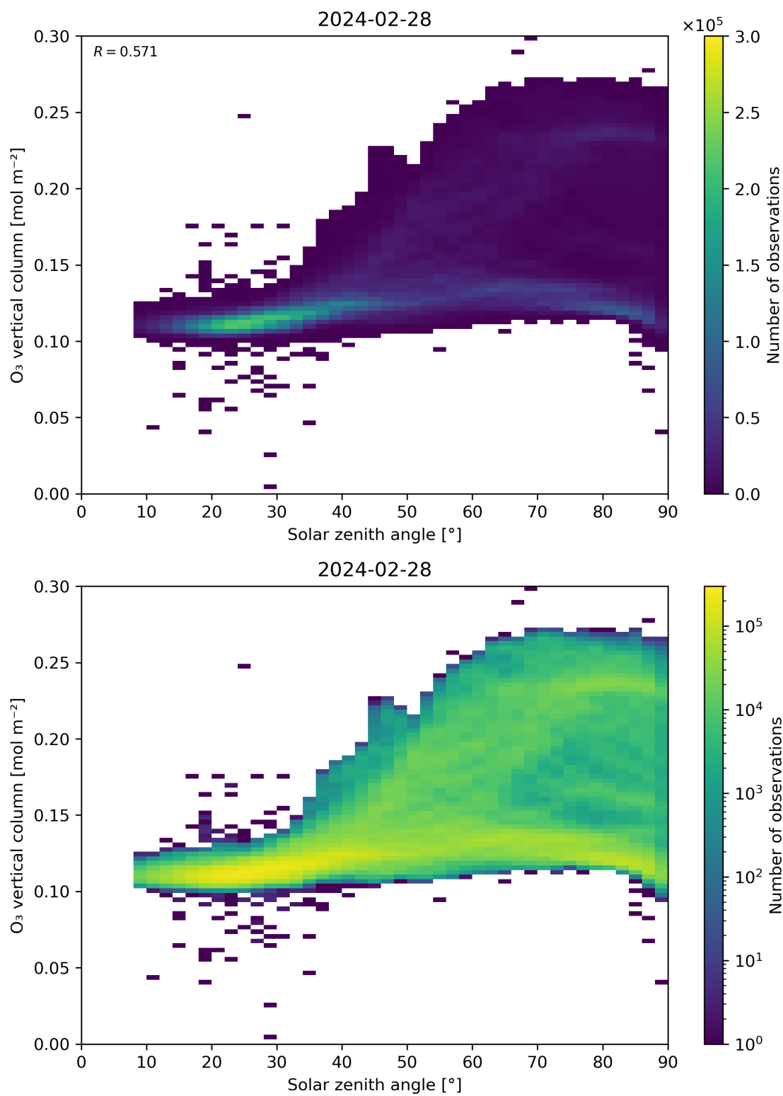
Figure 47: Scatter density plot of “Solar zenith angle” against “O 3 vertical column” for 2024-02-27 to 2024-02-29.
