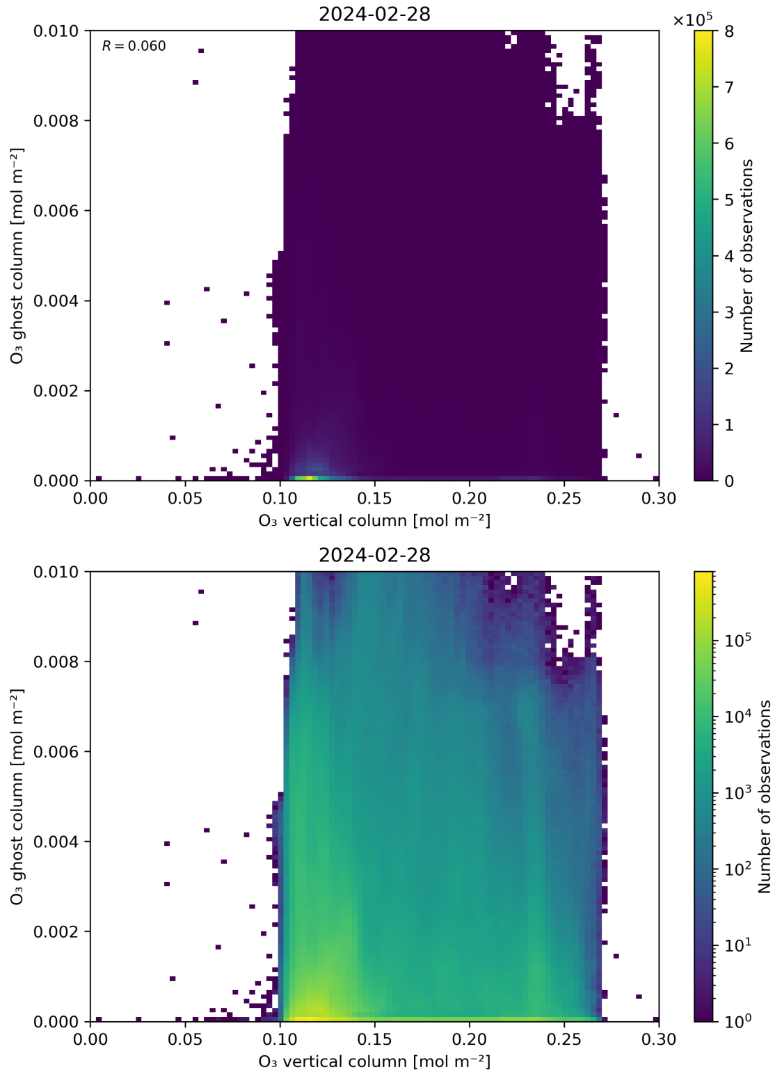
Figure 40: Scatter density plot of “O 3 vertical column” against “O 3 ghost column” for 2024-02-27 to 2024-02-29.
