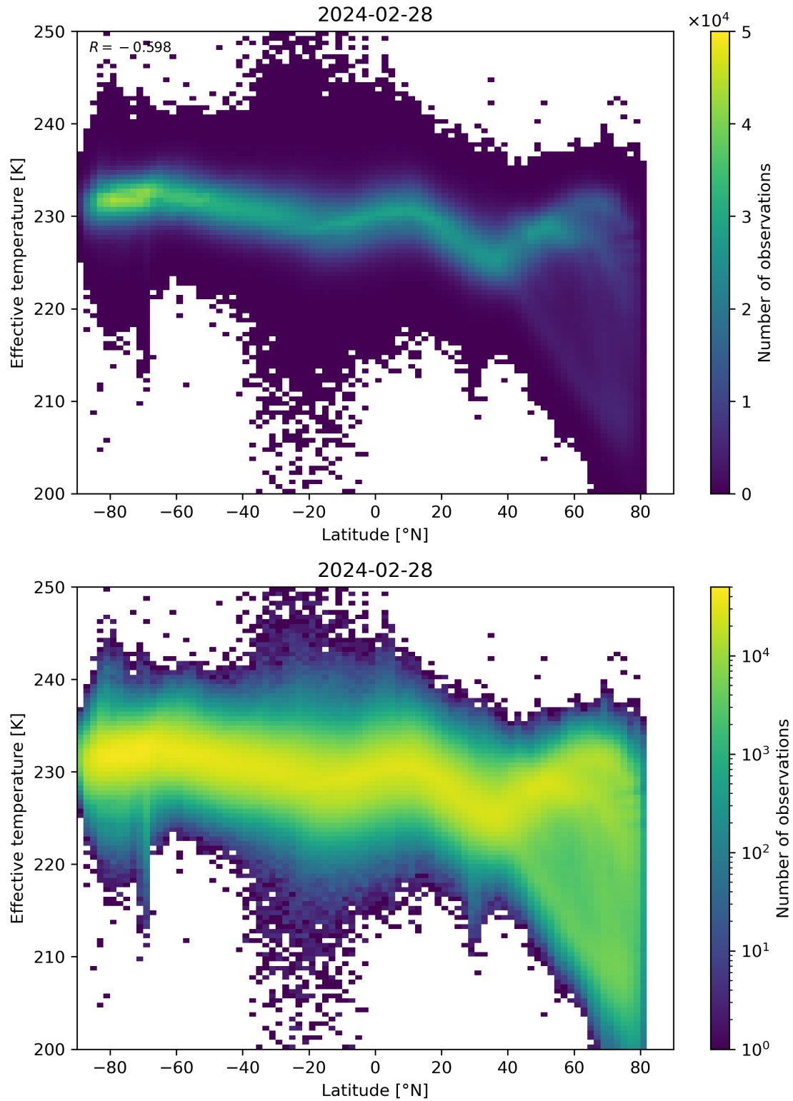
Figure 34: Scatter density plot of “Latitude” against “Effective temperature” for 2024-02-27 to 2024-02-29.
