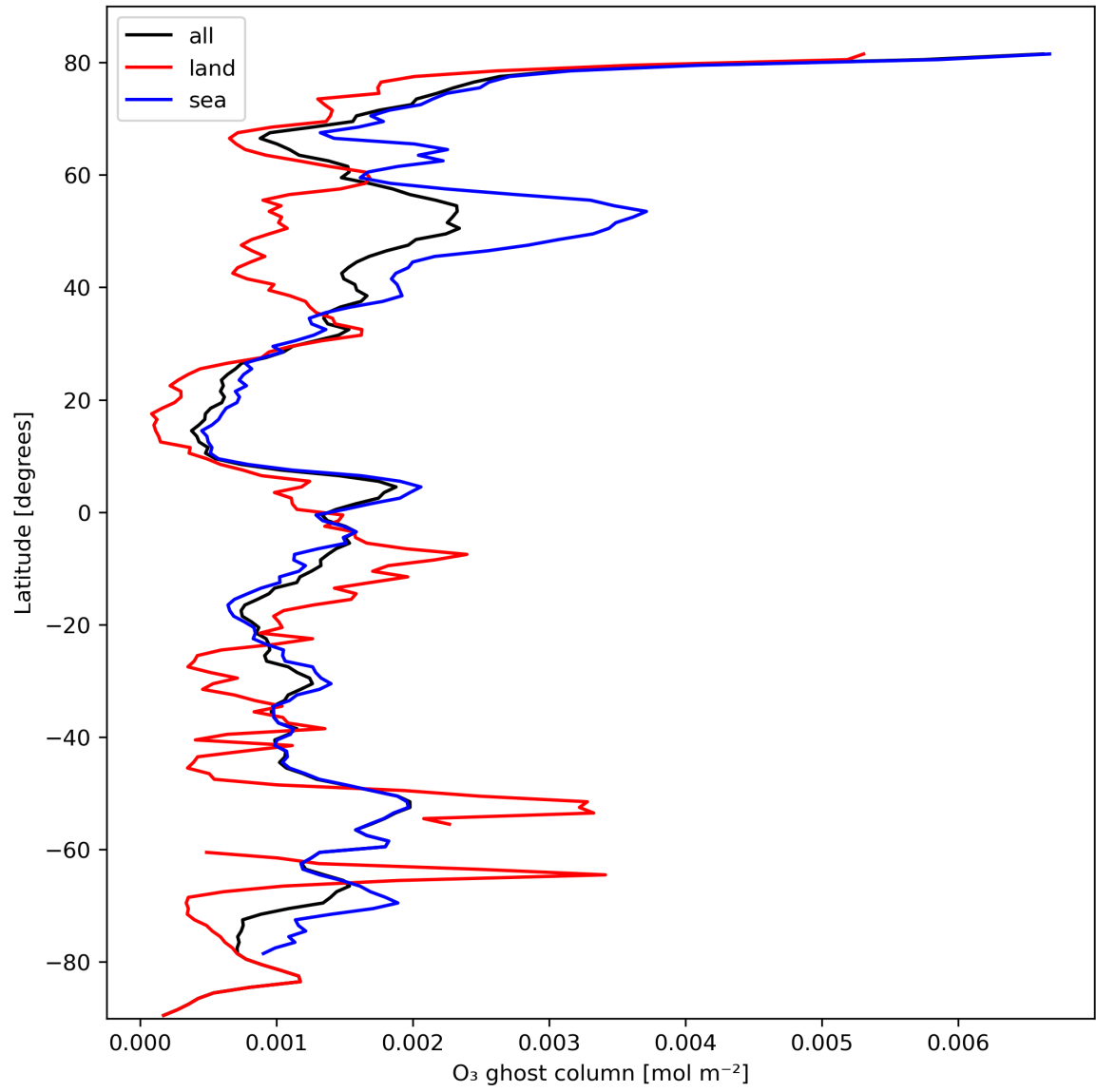
Figure 18: Zonal average of "O 3 ghost column" for 2024-02-27 to 2024-02-29.
