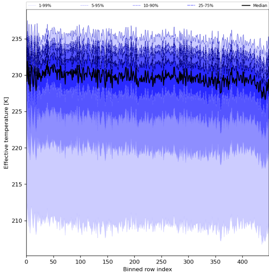
Figure 31: Along track statistics of “Effective temperature” for 2024-02-27 to 2024-02-29
