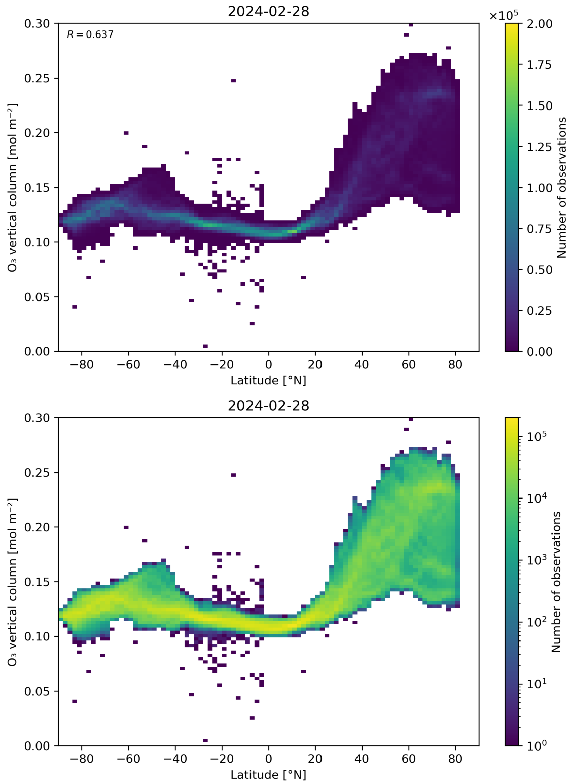
Figure 36: Scatter density plot of “Latitude” against “O 3 vertical column” for 2024-02-27 to 2024-02-29.
