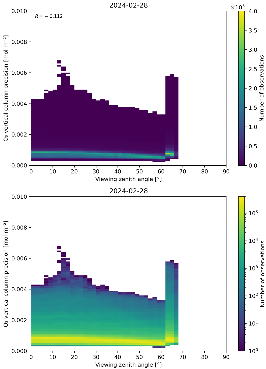
Figure 53: Scatter density plot of “Viewing zenith angle” against “O 3 vertical column precision” for 2024-02-27 to 2024-02-29.
