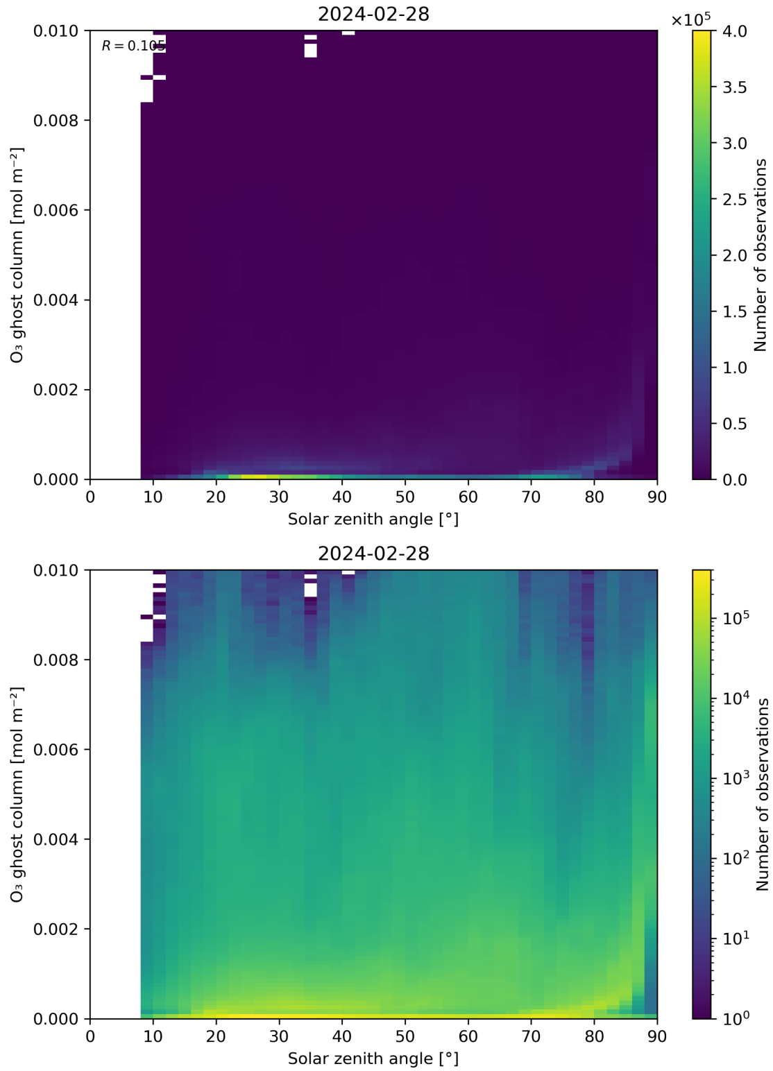
Figure 46: Scatter density plot of “Solar zenith angle” against “O 3 ghost column” for 2024-02-27 to 2024-02-29.
