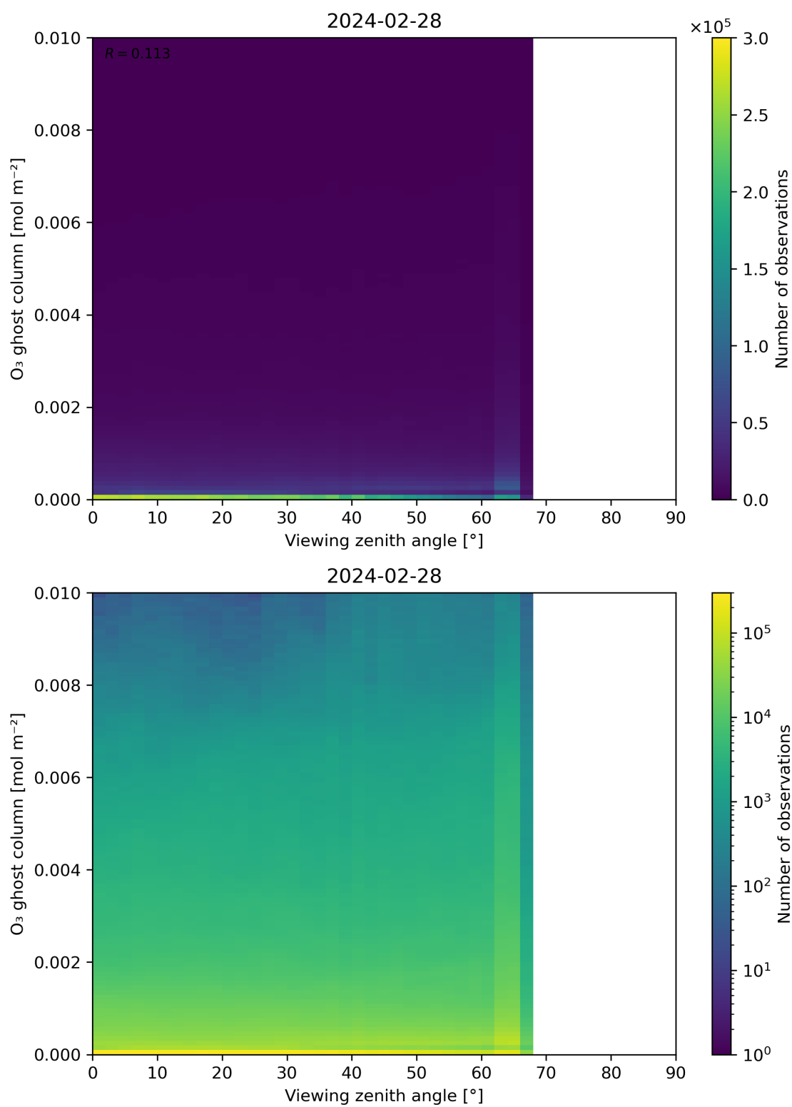
Figure 51: Scatter density plot of “Viewing zenith angle” against “O 3 ghost column” for 2024-02-27 to 2024-02-29.
