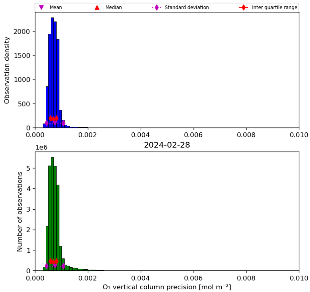
Figure 22: Histogram of “O 3 vertical column precision” for 2024-02-27 to 2024-02-29
