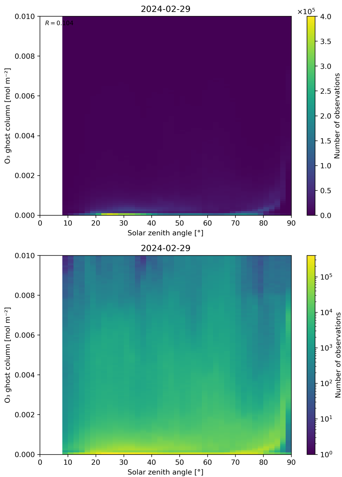
Figure 46: Scatter density plot of “Solar zenith angle” against “O 3 ghost column” for 2024-02-28 to 2024-03-01.
