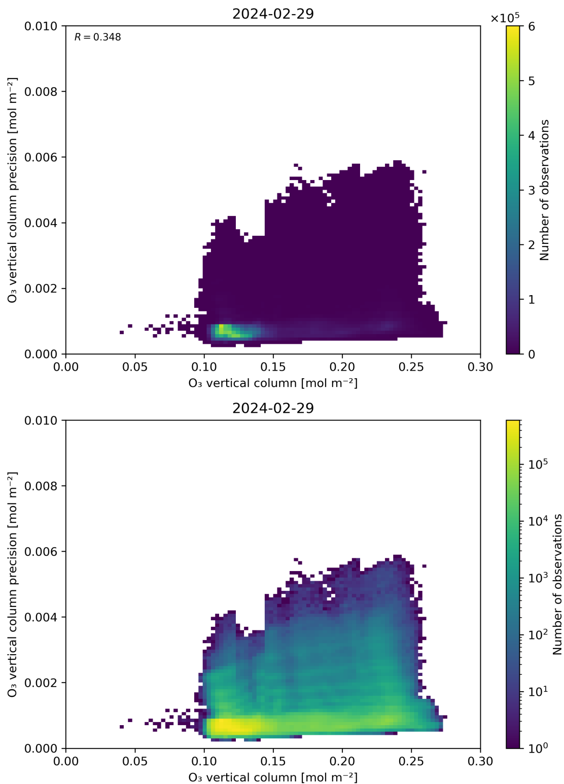
Figure 41: Scatter density plot of “O 3 vertical column” against “O 3 vertical column precision” for 2024-02-28 to 2024-03-01.
