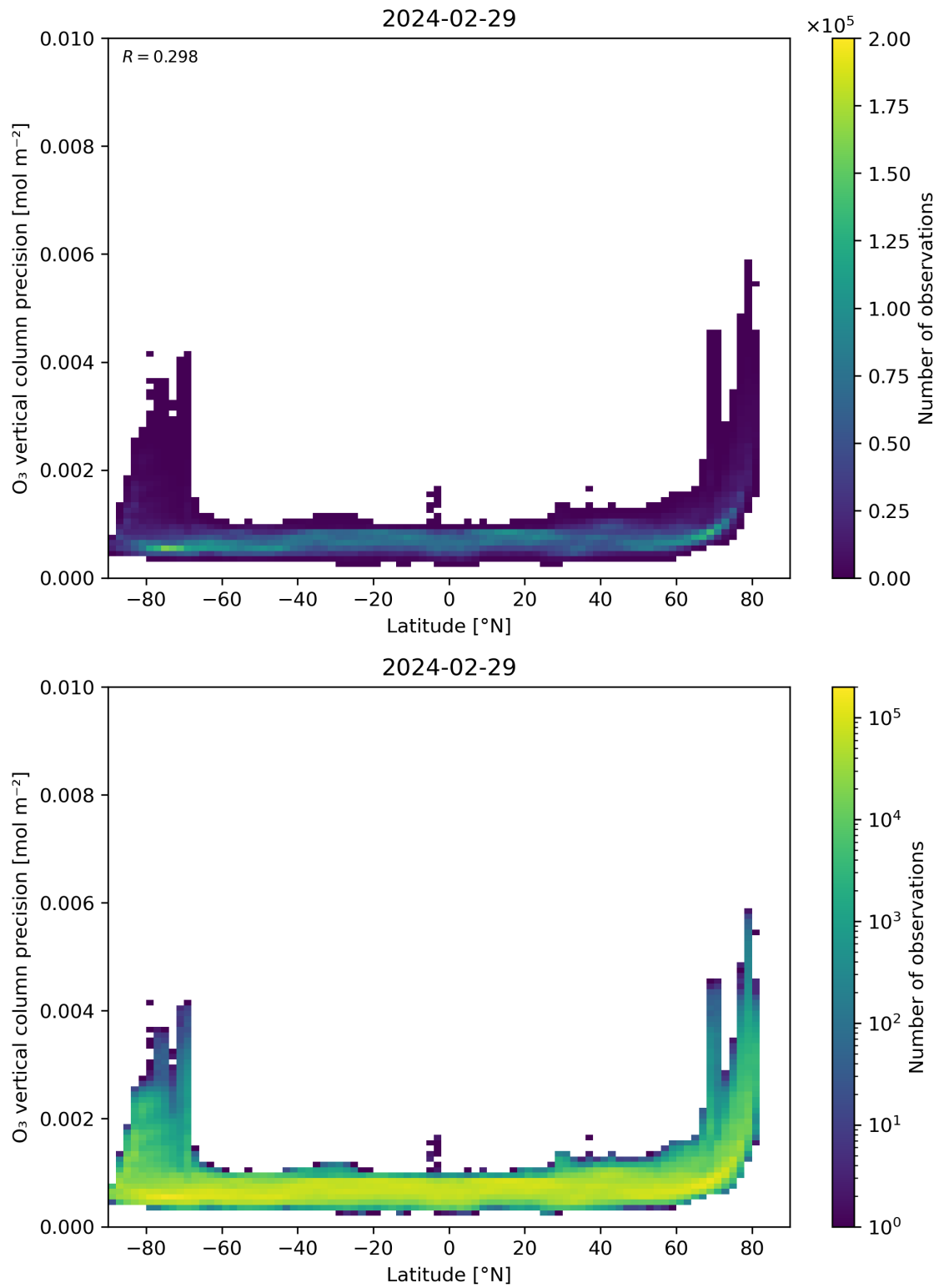
Figure 37: Scatter density plot of “Latitude” against “O 3 vertical column precision” for 2024-02-28 to 2024-03-01.
