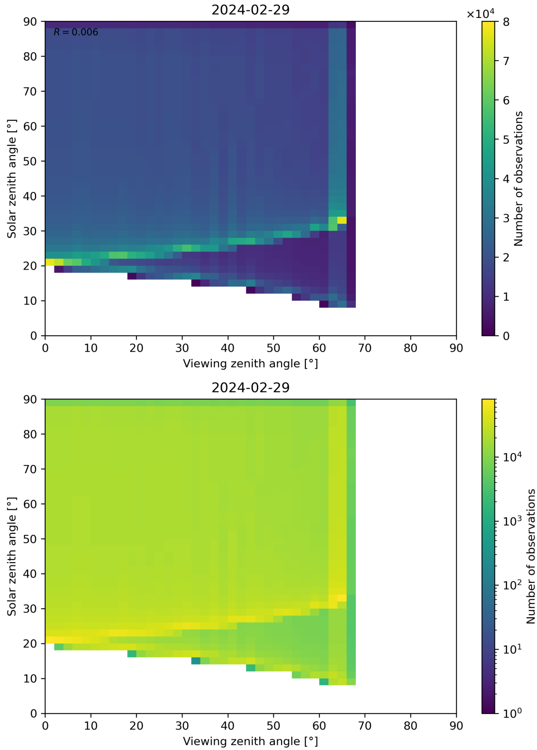
Figure 54: Scatter density plot of “Viewing zenith angle” against “Solar zenith angle” for 2024-02-28 to 2024-03-01.
