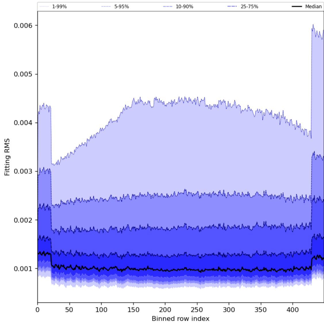
Figure 30: Along track statistics of “Fitting RMS” for 2024-02-28 to 2024-03-01
