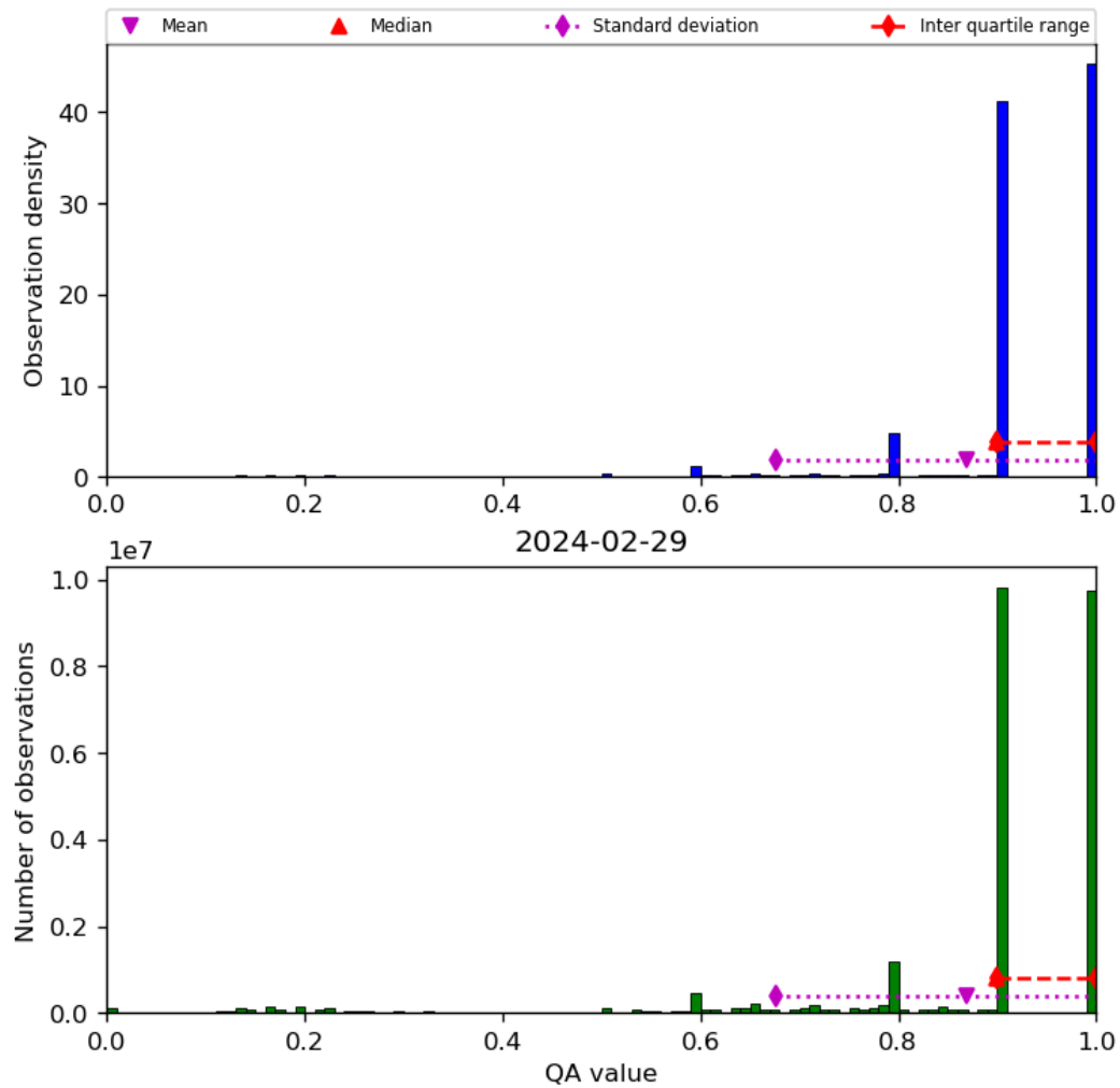
Figure 20: Histogram of “QA value” for 2024-02-28 to 2024-03-01
