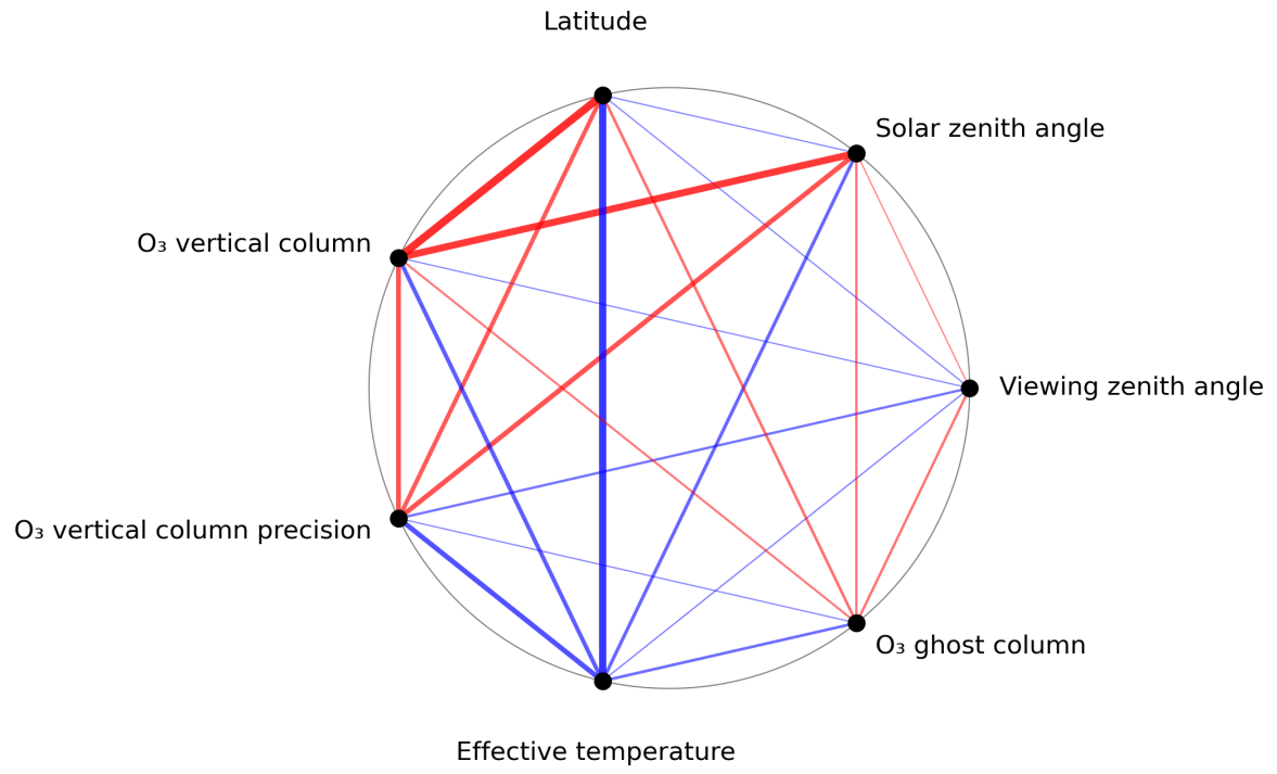
Figure 1: Map of correlation graph for 2024-02-28 to 2024-03-01.
