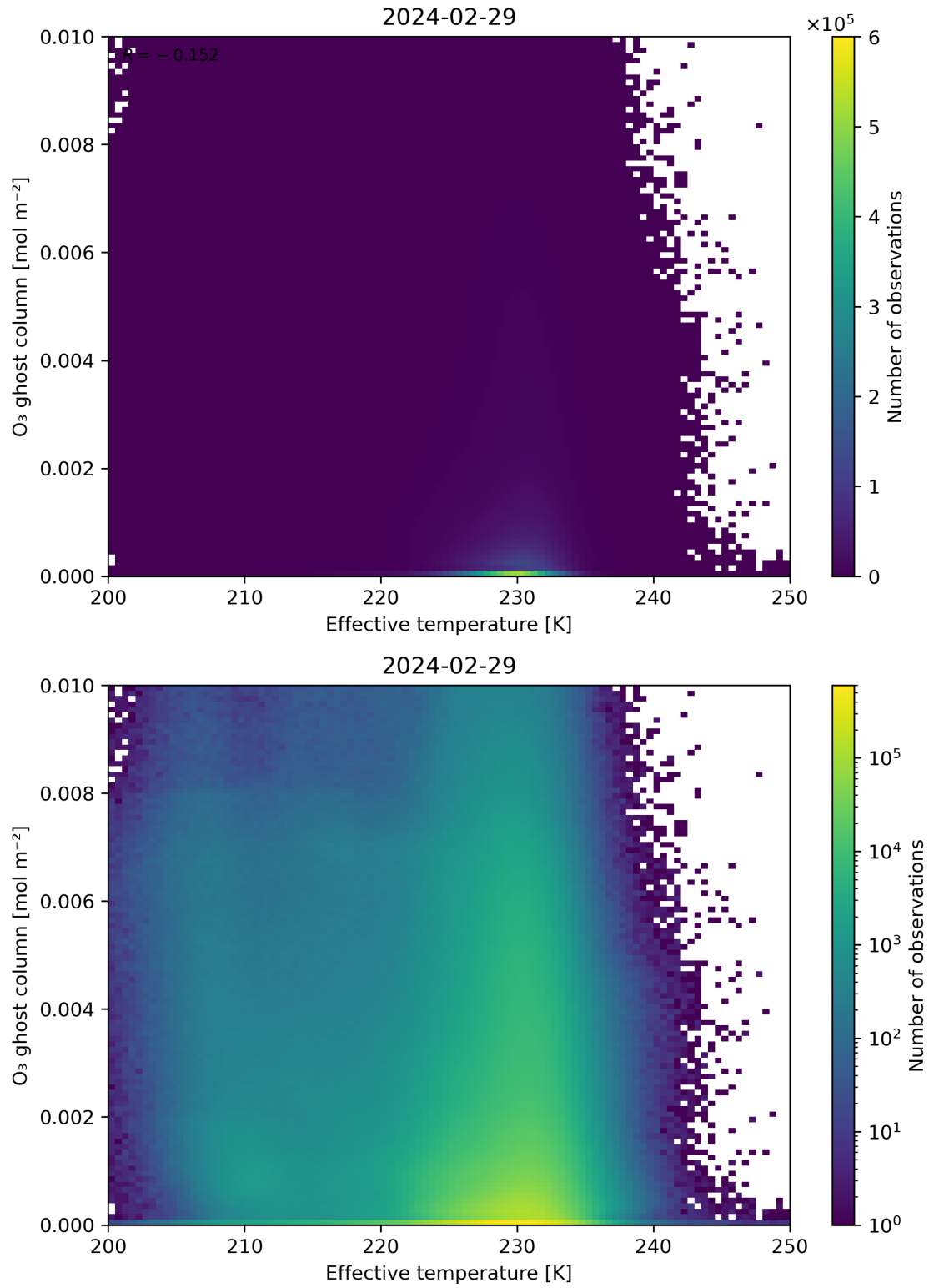
Figure 38: Scatter density plot of “Effective temperature” against “O 3 ghost column” for 2024-02-28 to 2024-03-01.
