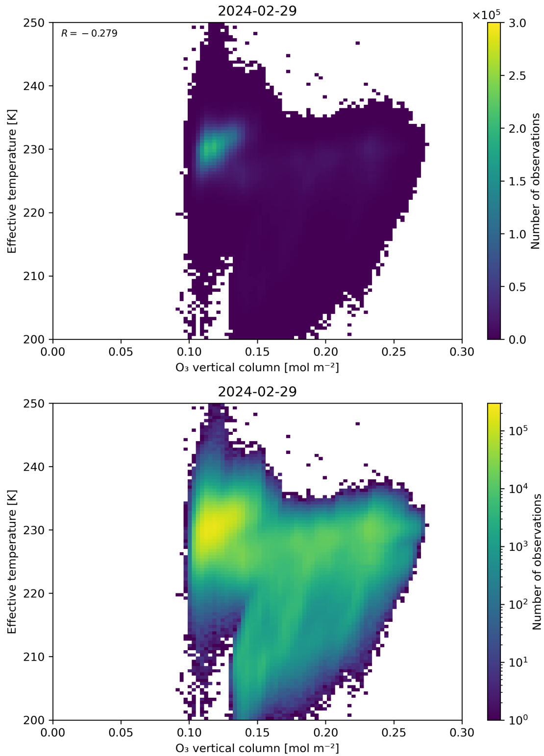
Figure 39: Scatter density plot of “O 3 vertical column” against “Effective temperature” for 2024-02-28 to 2024-03-01.
