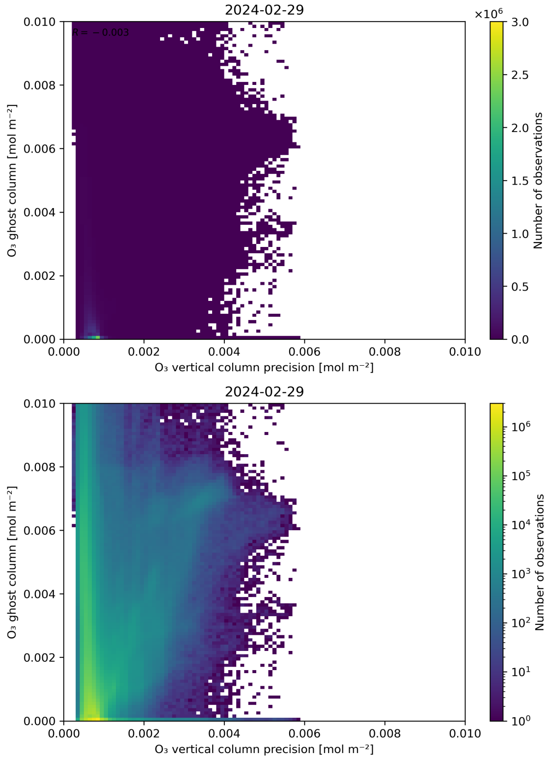
Figure 43: Scatter density plot of “ \text{O}_3 vertical column precision” against “ \text{O}_3 ghost column” for 2024-02-28 to 2024-03-01.
