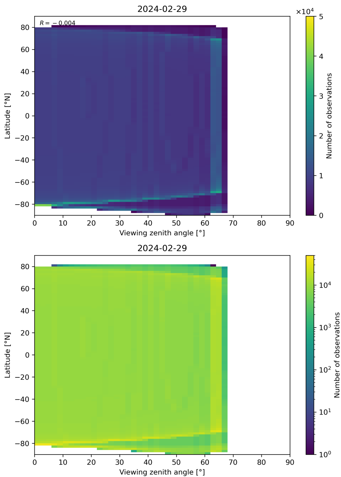
Figure 49: Scatter density plot of “Viewing zenith angle” against “Latitude” for 2024-02-28 to 2024-03-01.
