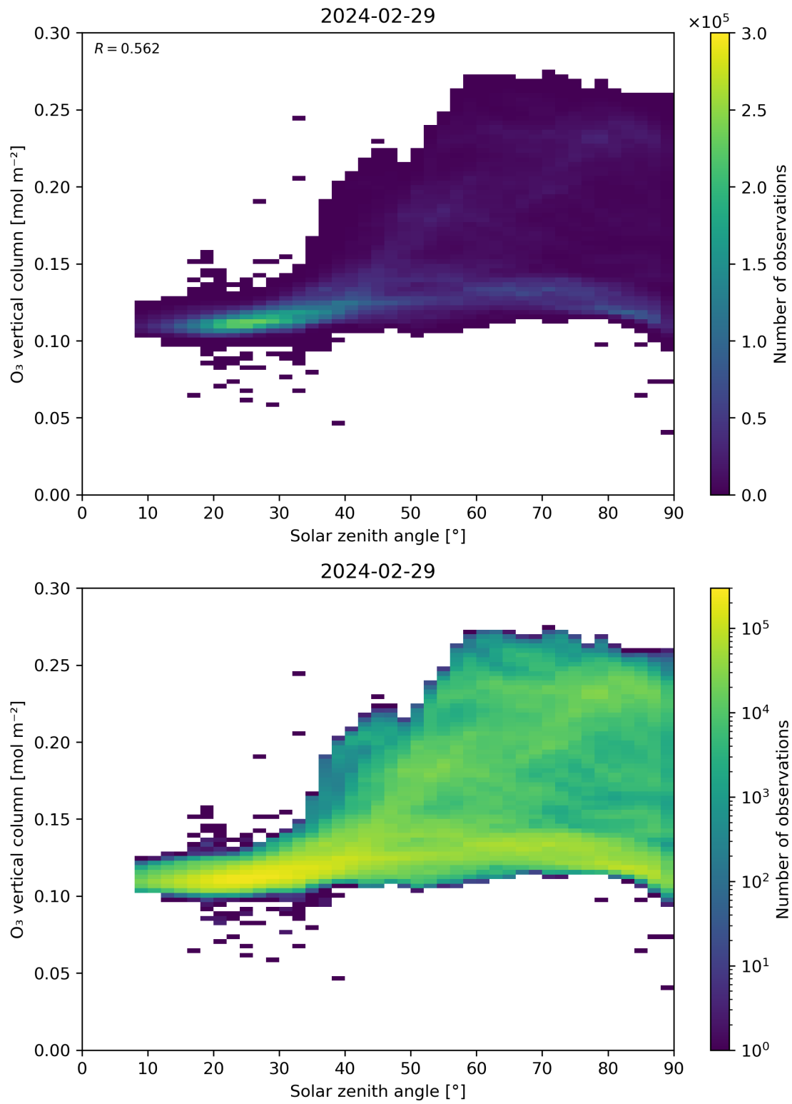
Figure 47: Scatter density plot of “Solar zenith angle” against “O 3 vertical column” for 2024-02-28 to 2024-03-01.
