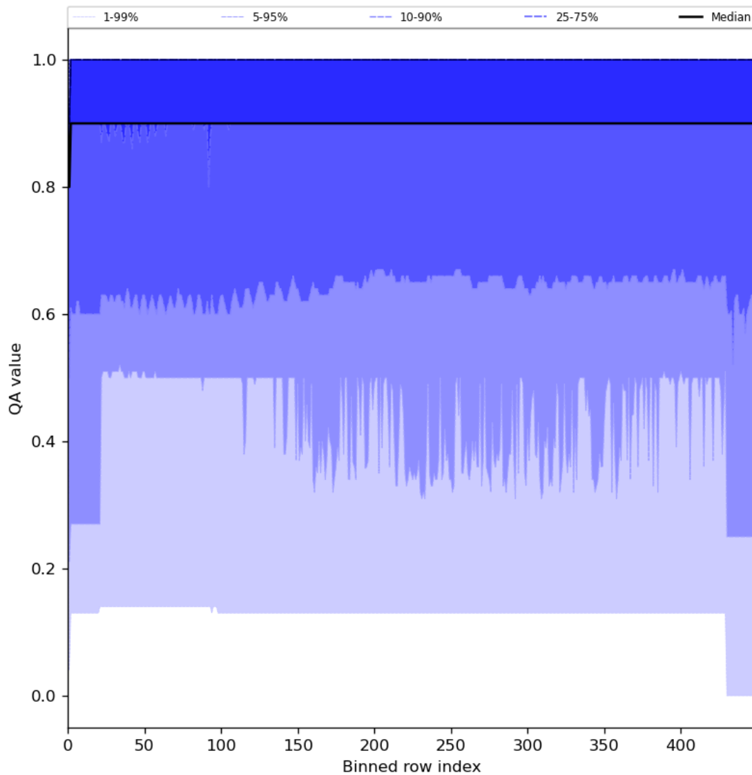
Figure 27: Along track statistics of “QA value” for 2024-02-28 to 2024-03-01
