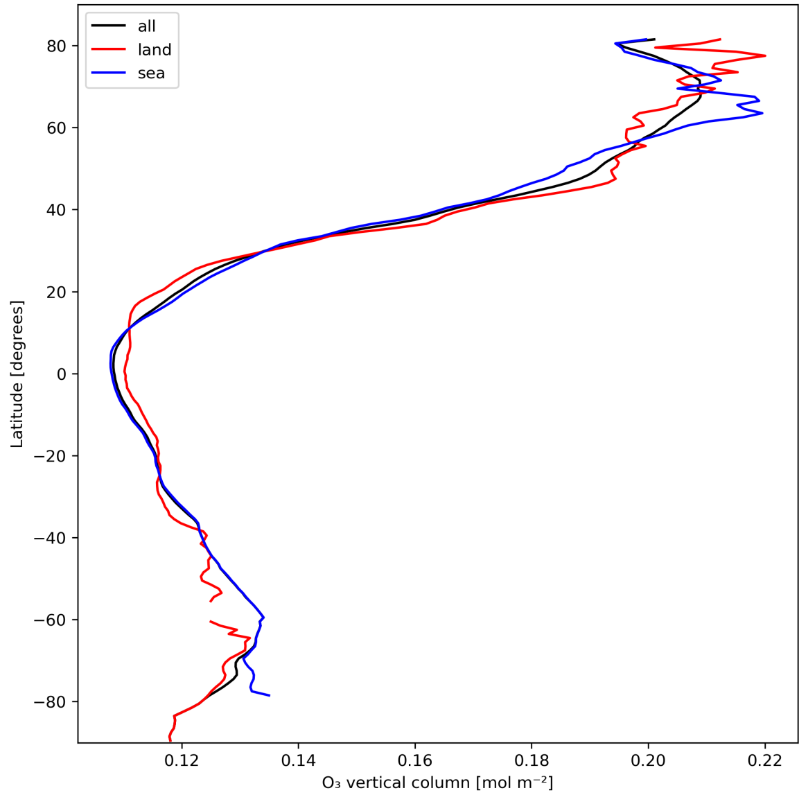
Figure 14: Zonal average of “O 3 vertical column” for 2024-02-28 to 2024-03-01.
