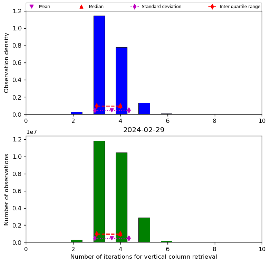
Figure 26: Histogram of “Number of iterations for vertical column retrieval” for 2024-02-28 to 2024-03-01
