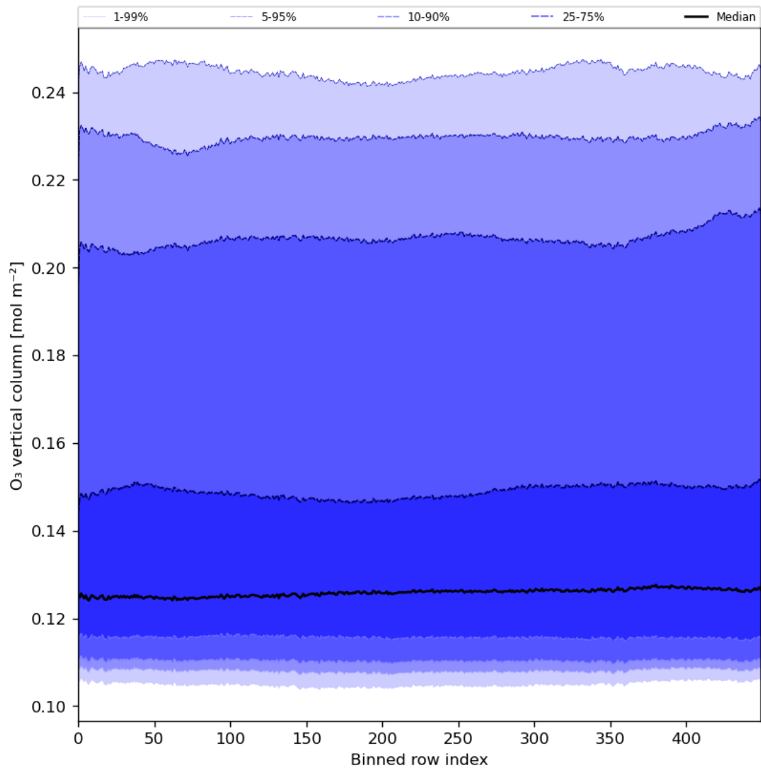
Figure 28: Along track statistics of “O 3 vertical column” for 2024-02-28 to 2024-03-01
