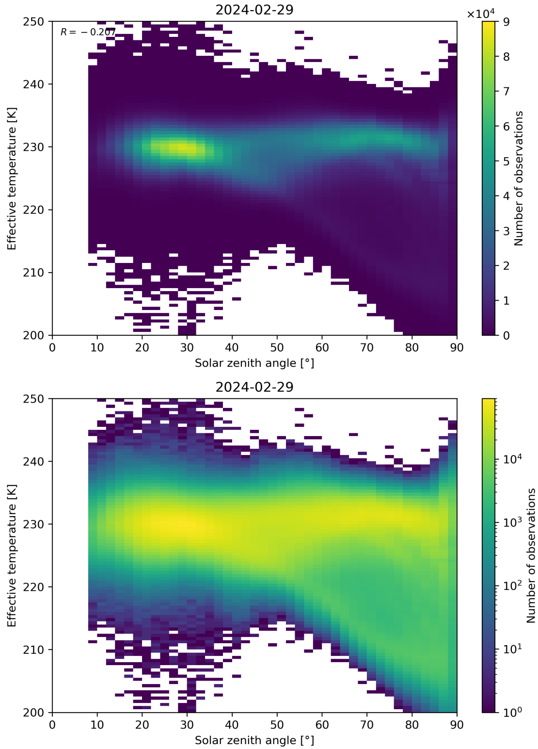
Figure 45: Scatter density plot of “Solar zenith angle” against “Effective temperature” for 2024-02-28 to 2024-03-01.
