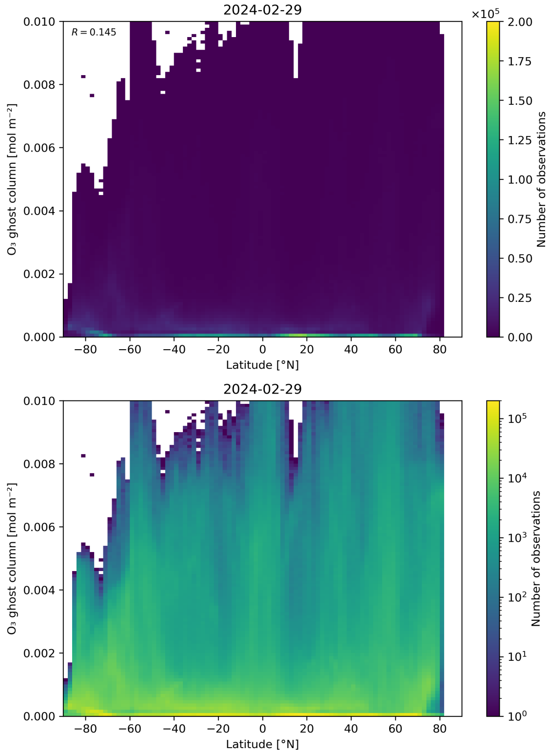
Figure 35: Scatter density plot of “Latitude” against “O 3 ghost column” for 2024-02-28 to 2024-03-01.
