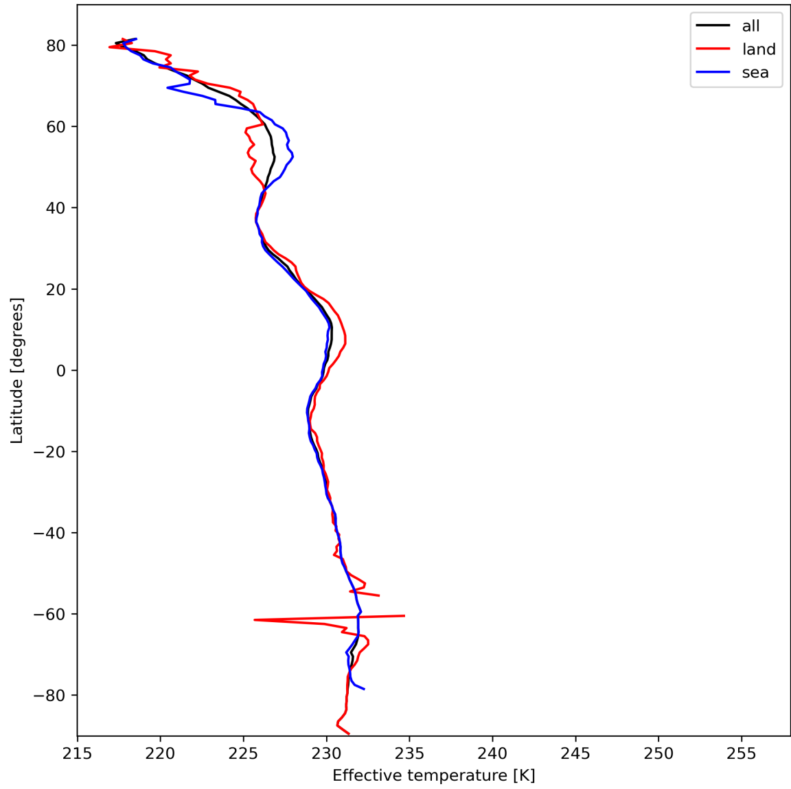
Figure 17: Zonal average of “Effective temperature” for 2024-02-28 to 2024-03-01.
