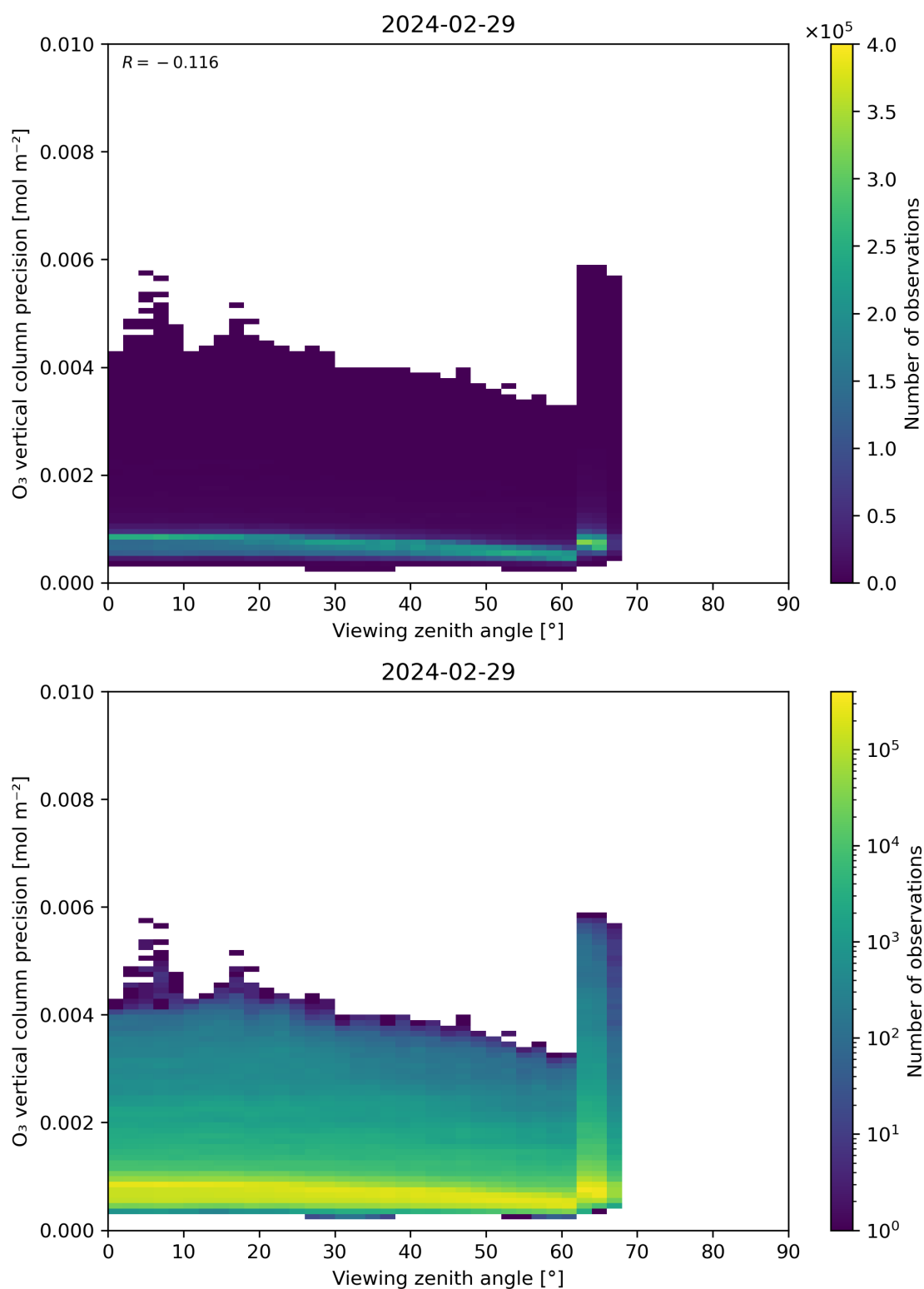
Figure 53: Scatter density plot of “Viewing zenith angle” against “O 3 vertical column precision” for 2024-02-28 to 2024-03-01.
