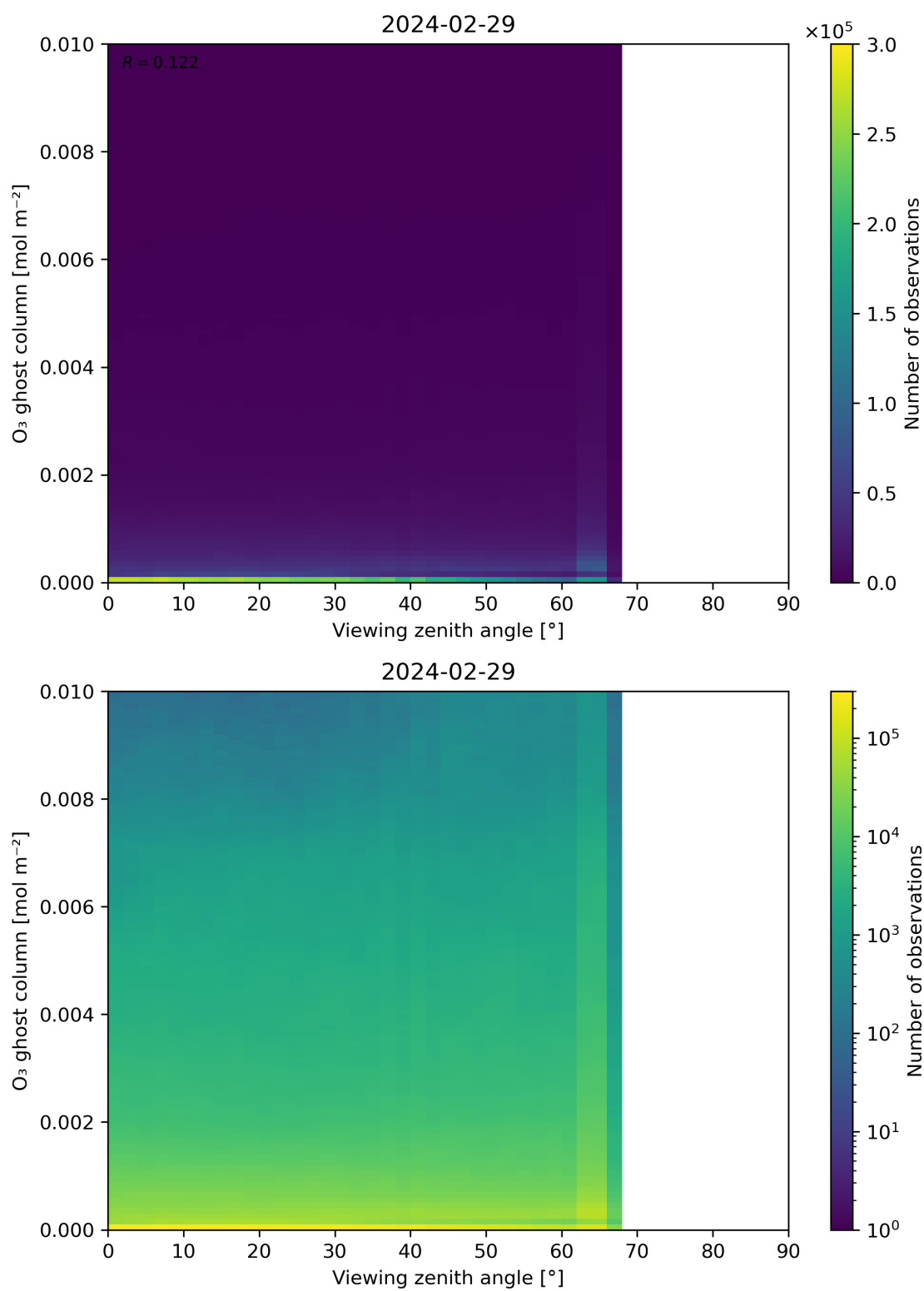
Figure 51: Scatter density plot of “Viewing zenith angle” against “O 3 ghost column” for 2024-02-28 to 2024-03-01.
