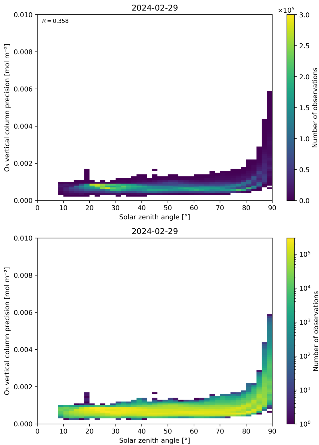
Figure 48: Scatter density plot of “Solar zenith angle” against “O 3 vertical column precision” for 2024-02-28 to 2024-03-01.
