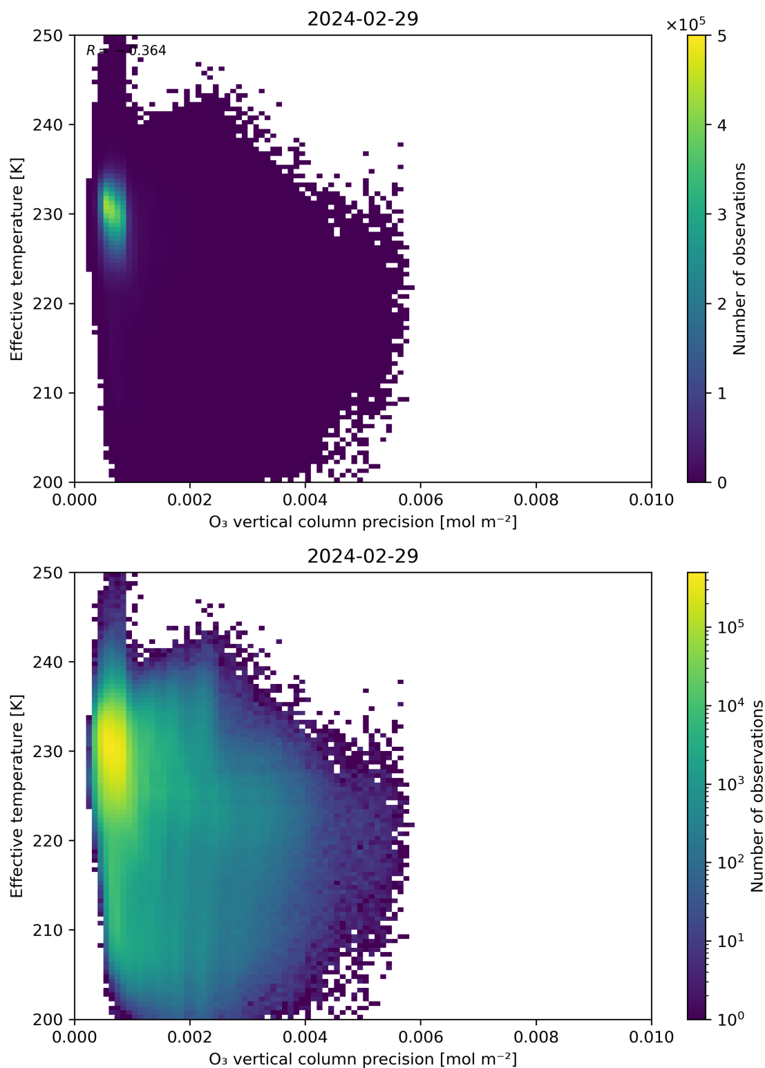
Figure 42: Scatter density plot of “O 3 vertical column precision” against “Effective temperature” for 2024-02-28 to 2024-03-01.
