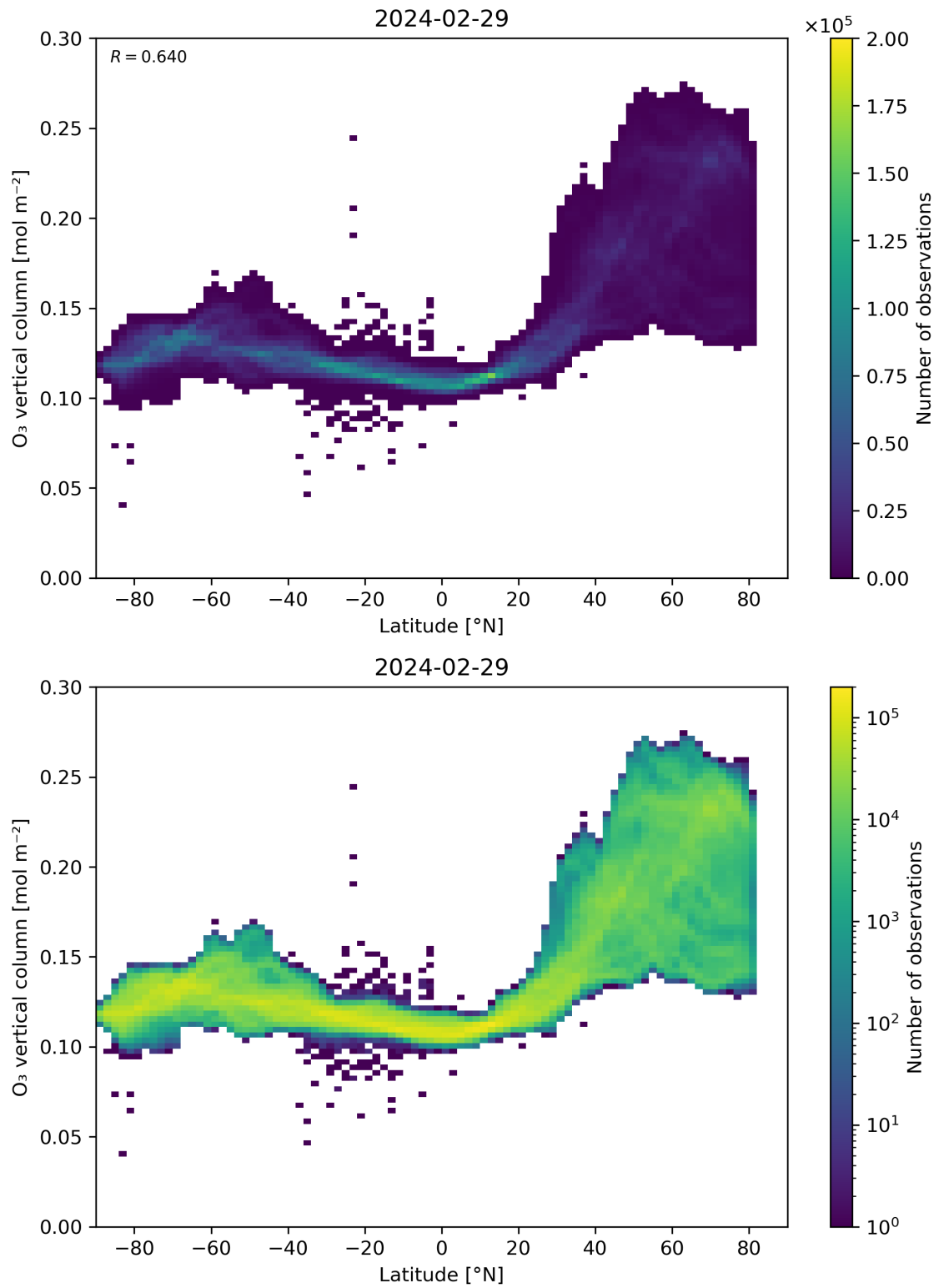
Figure 36: Scatter density plot of “Latitude” against “O 3 vertical column” for 2024-02-28 to 2024-03-01.
