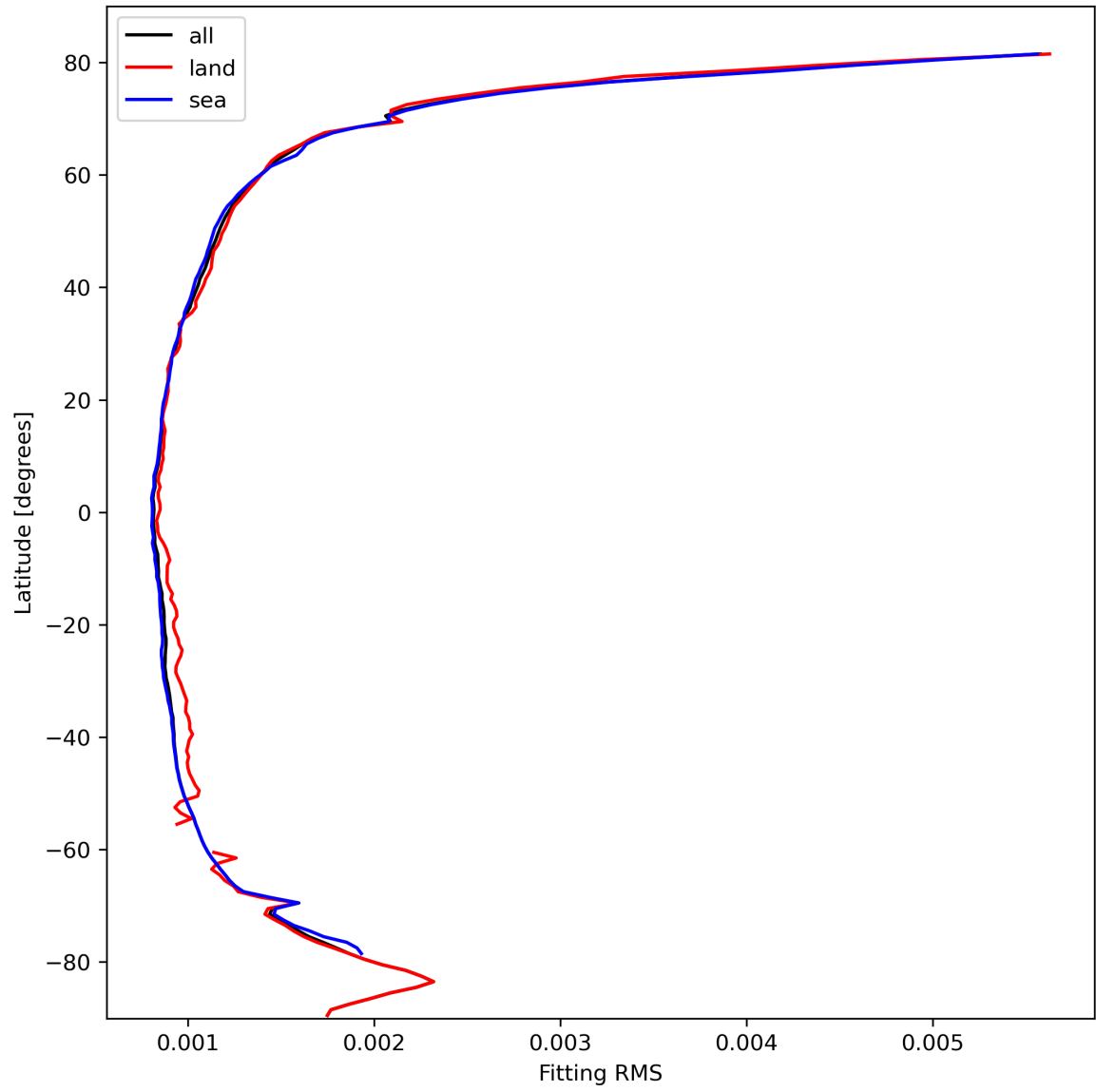
Figure 16: Zonal average of “Fitting RMS” for 2024-02-28 to 2024-03-01.
