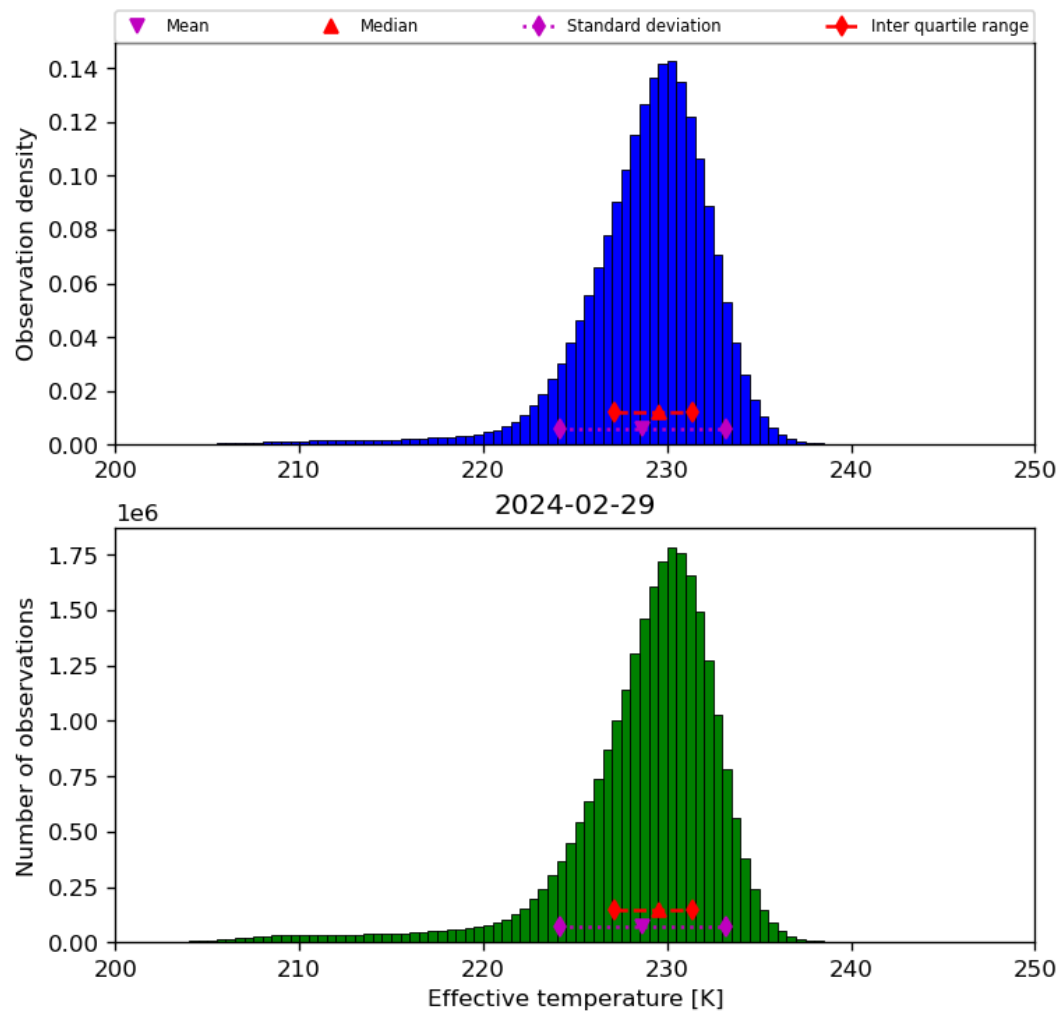
Figure 24: Histogram of “Effective temperature” for 2024-02-28 to 2024-03-01
