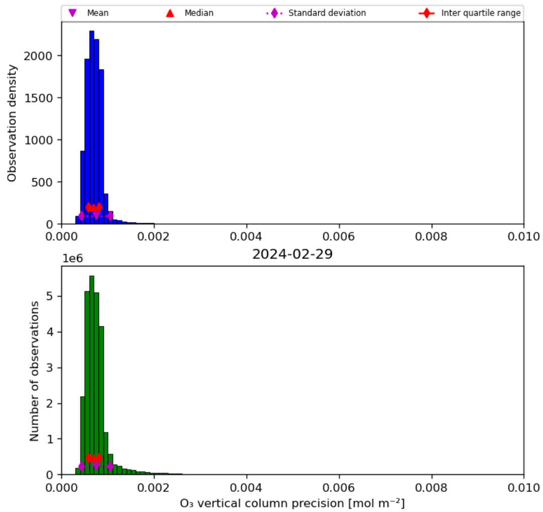
Figure 22: Histogram of “O 3 vertical column precision” for 2024-02-28 to 2024-03-01
