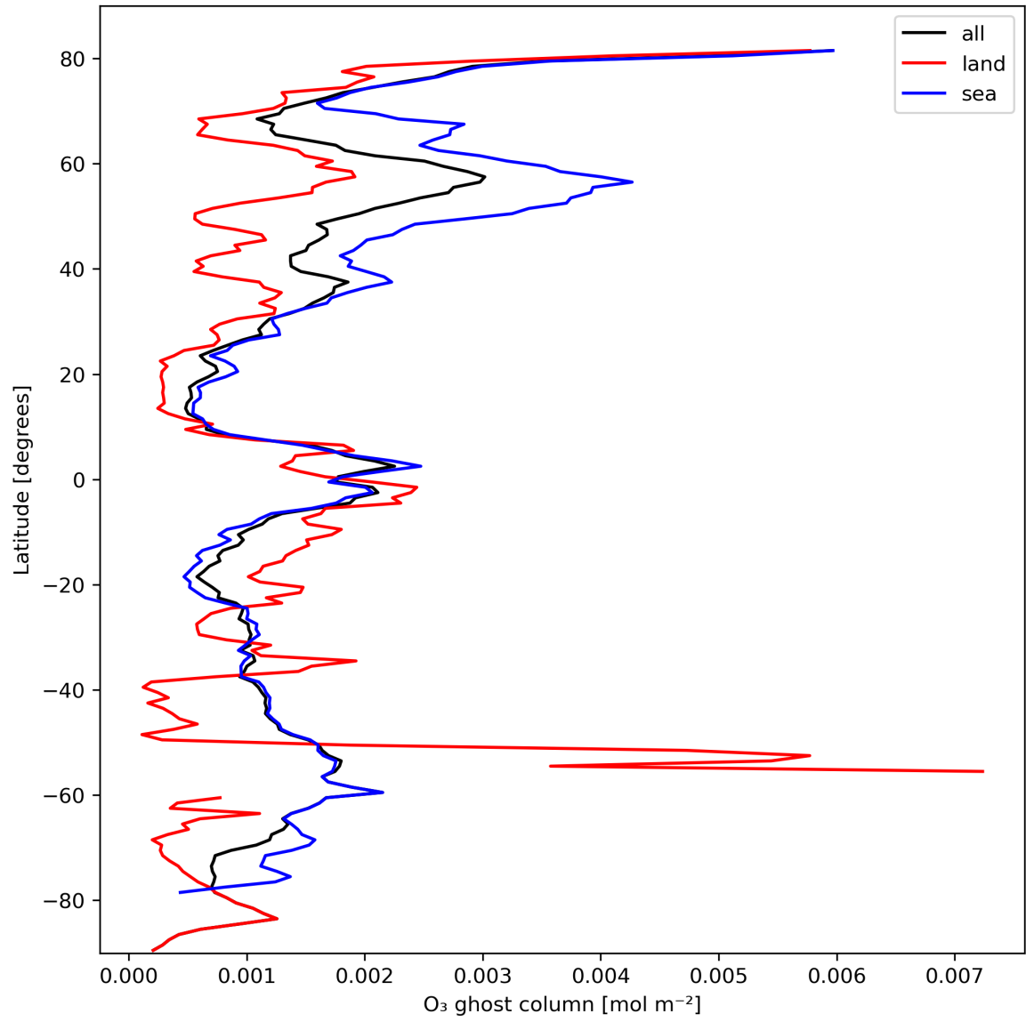
Figure 18: Zonal average of “O 3 ghost column” for 2024-02-28 to 2024-03-01.
