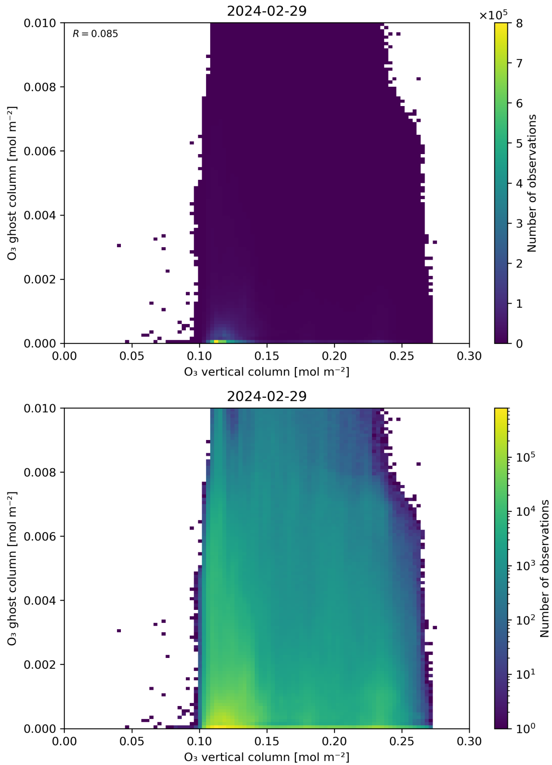
Figure 40: Scatter density plot of “O 3 vertical column” against “O 3 ghost column” for 2024-02-28 to 2024-03-01.
