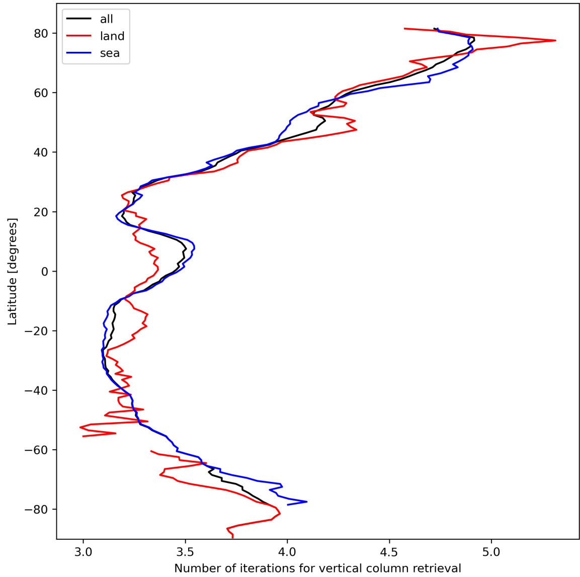
Figure 19: Zonal average of “Number of iterations for vertical column retrieval” for 2024-02-28 to 2024-03-01.
