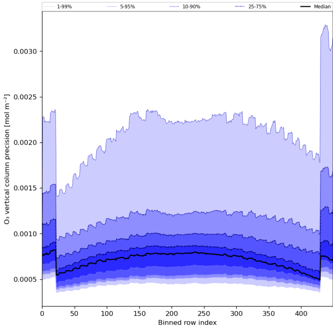
Figure 29: Along track statistics of “O 3 vertical column precision” for 2024-02-28 to 2024-03-01
