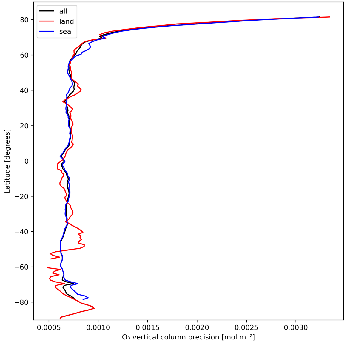
Figure 15: Zonal average of “O 3 vertical column precision” for 2024-02-28 to 2024-03-01.
