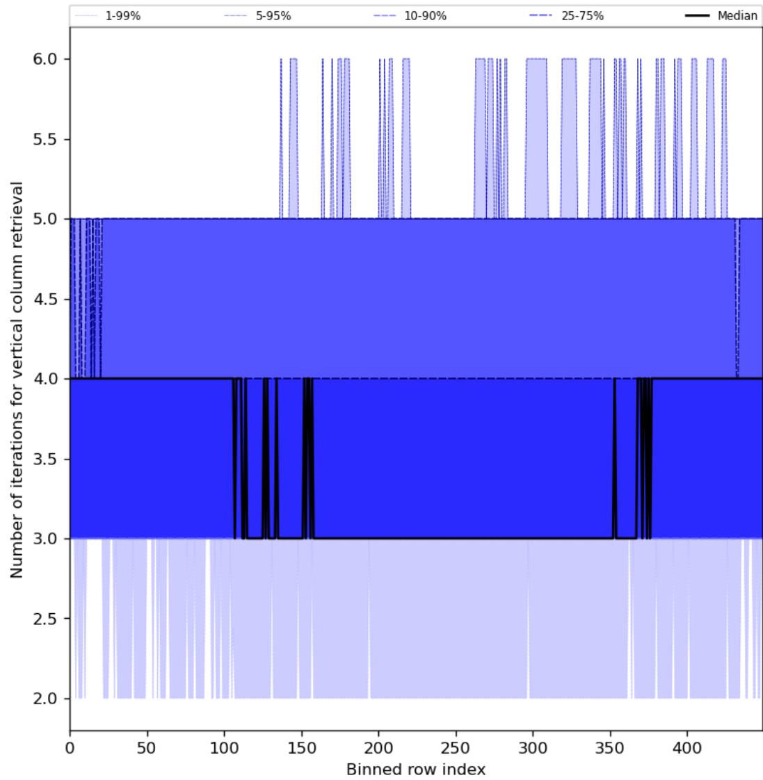
Figure 33: Along track statistics of “Number of iterations for vertical column retrieval” for 2024-02-28 to 2024-03-01
