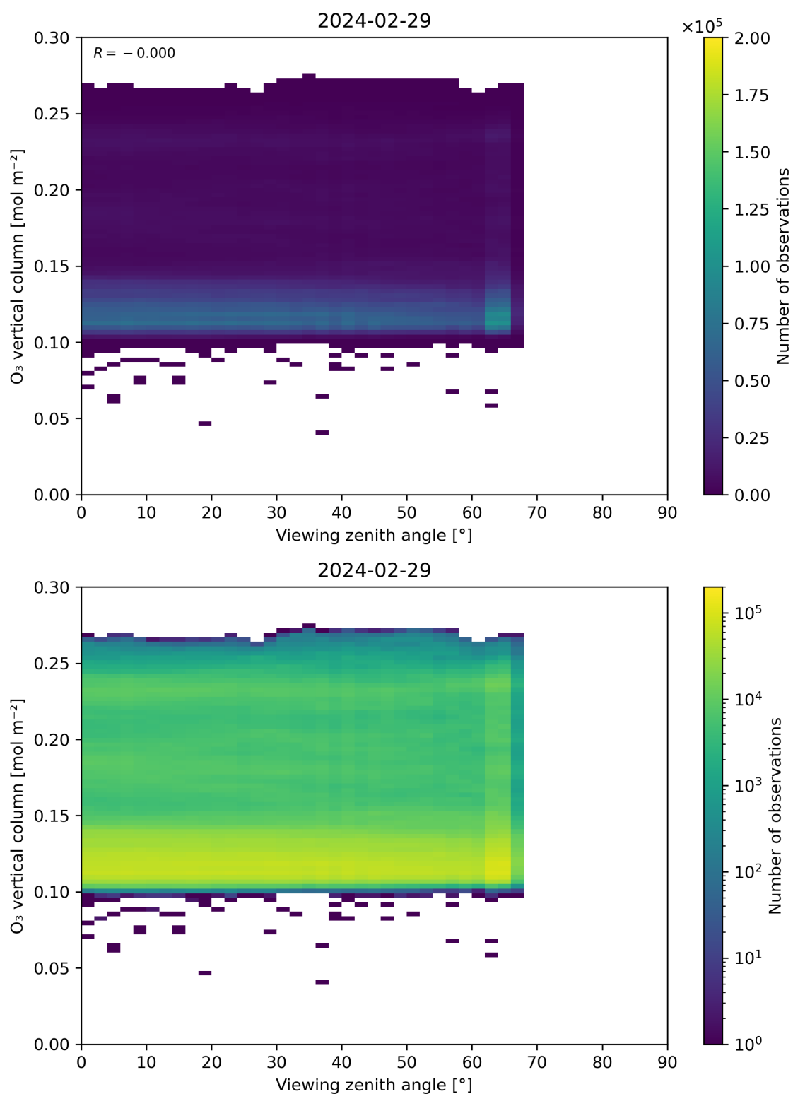
Figure 52: Scatter density plot of “Viewing zenith angle” against “O 3 vertical column” for 2024-02-28 to 2024-03-01.
