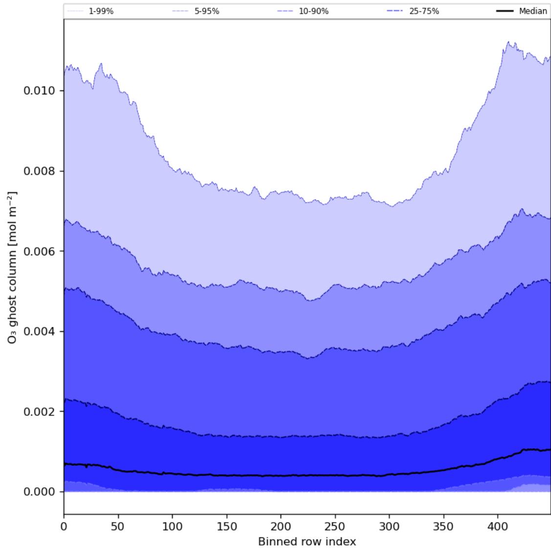
Figure 32: Along track statistics of “O 3 ghost column” for 2024-02-28 to 2024-03-01
