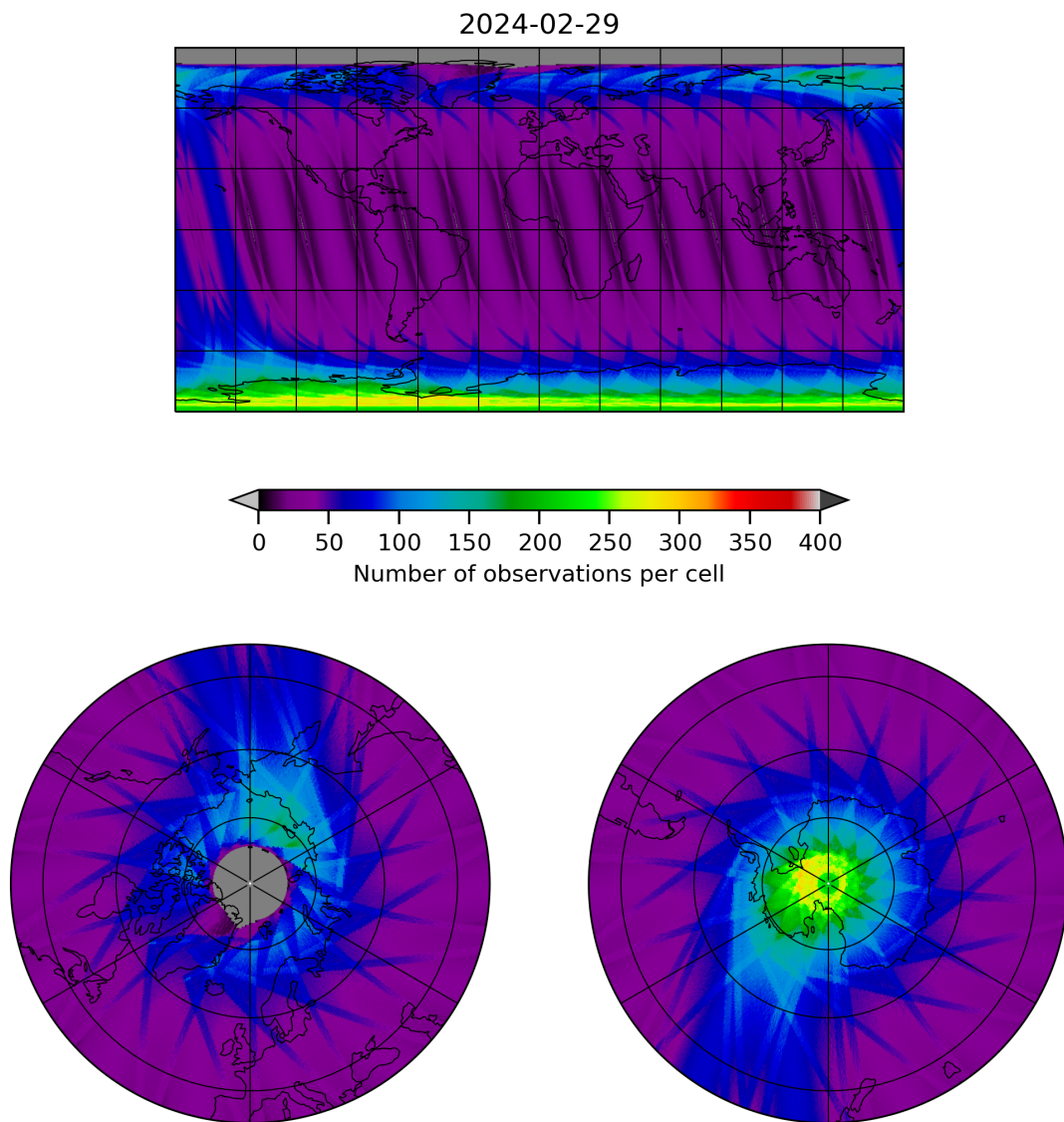
Figure 12: Map of the number of observations for 2024-02-28 to 2024-03-01
