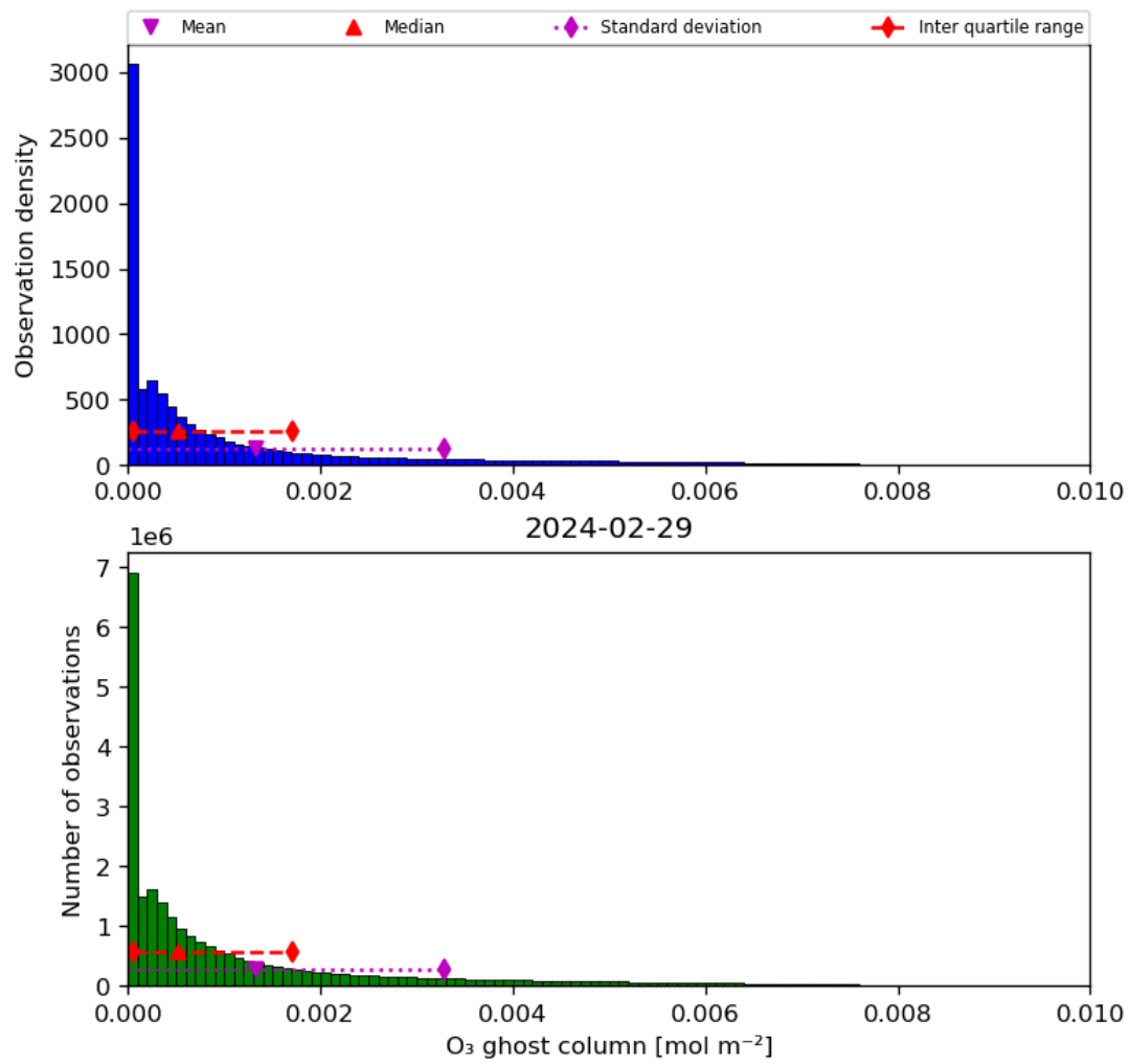
Figure 25: Histogram of "O 3 ghost column" for 2024-02-28 to 2024-03-01
