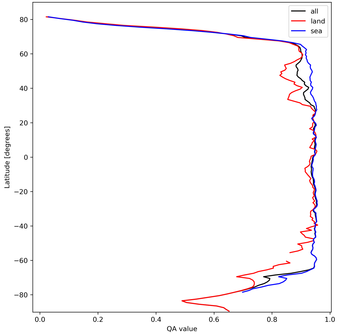
Figure 13: Zonal average of “QA value” for 2024-02-28 to 2024-03-01.
