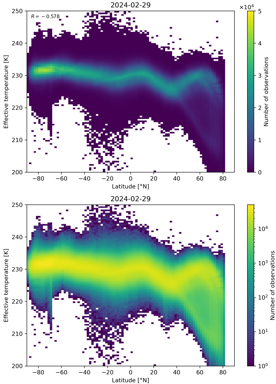
Figure 34: Scatter density plot of “Latitude” against “Effective temperature” for 2024-02-28 to 2024-03-01.
