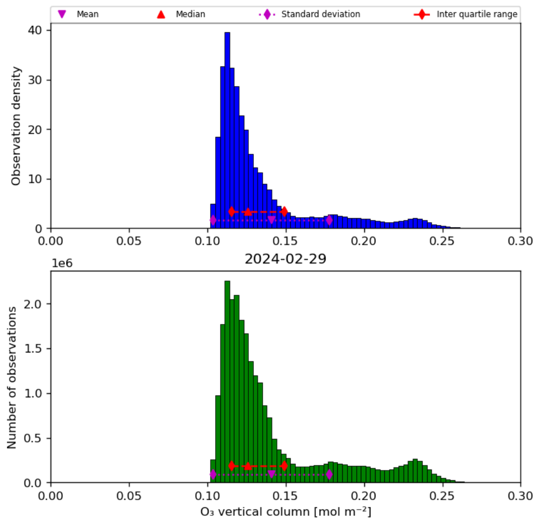
Figure 21: Histogram of “O 3 vertical column” for 2024-02-28 to 2024-03-01
