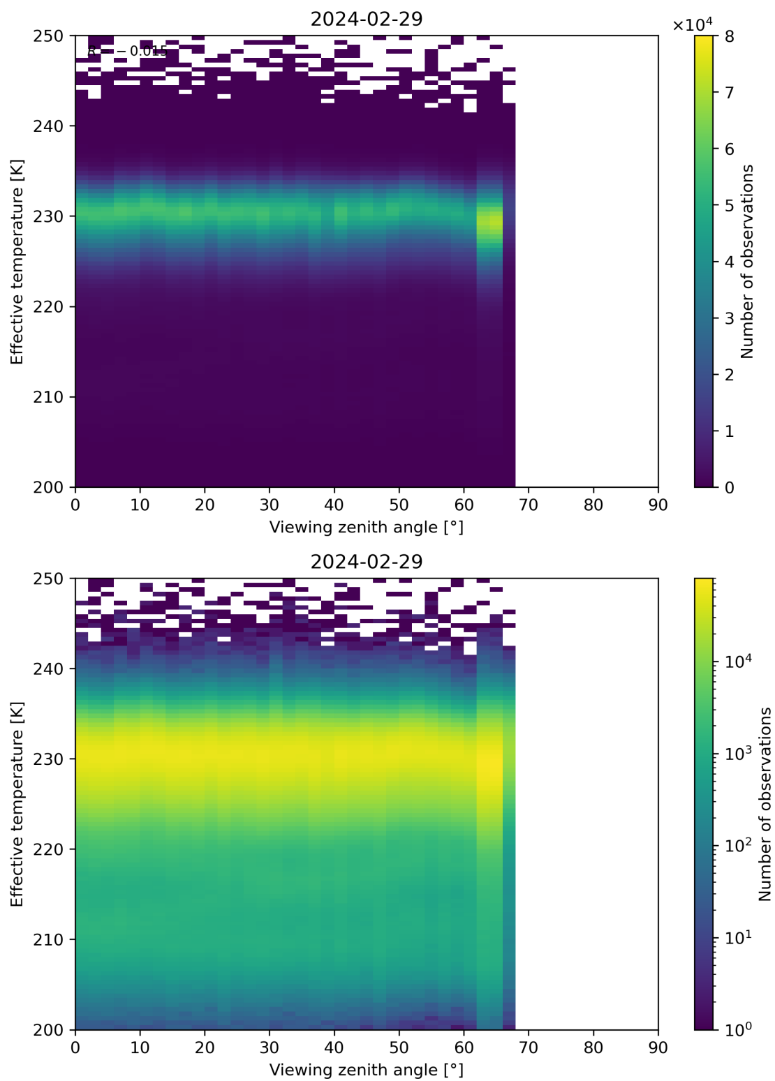
Figure 50: Scatter density plot of “Viewing zenith angle” against “Effective temperature” for 2024-02-28 to 2024-03-01.
