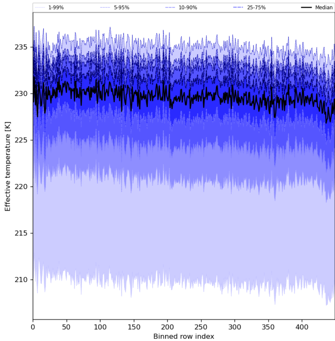
Figure 31: Along track statistics of “Effective temperature” for 2024-02-28 to 2024-03-01
