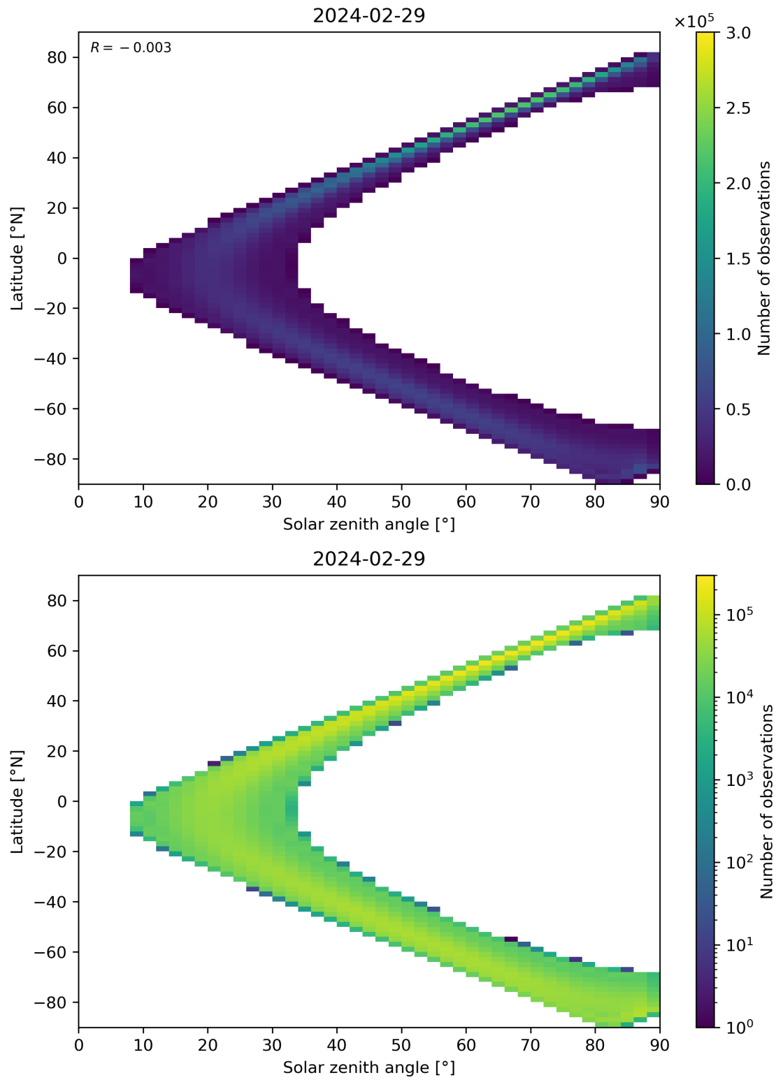
Figure 44: Scatter density plot of “Solar zenith angle” against “Latitude” for 2024-02-28 to 2024-03-01.
