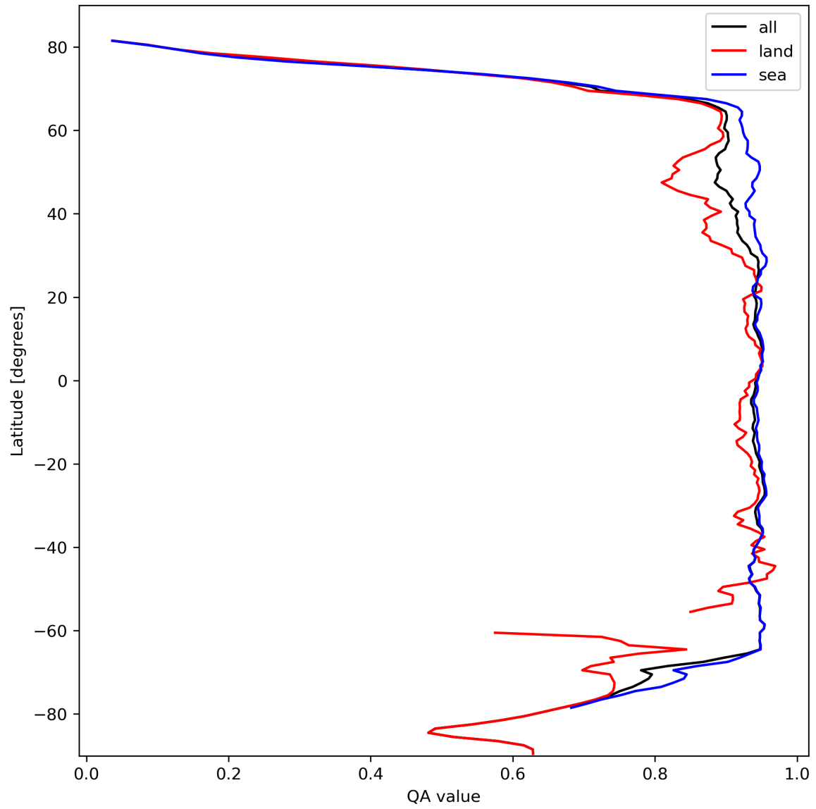
Figure 13: Zonal average of “QA value” for 2024-02-29 to 2024-03-02.
