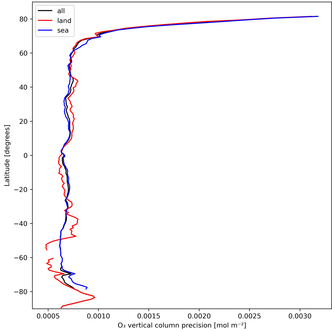
Figure 15: Zonal average of “O 3 vertical column precision” for 2024-02-29 to 2024-03-02.
