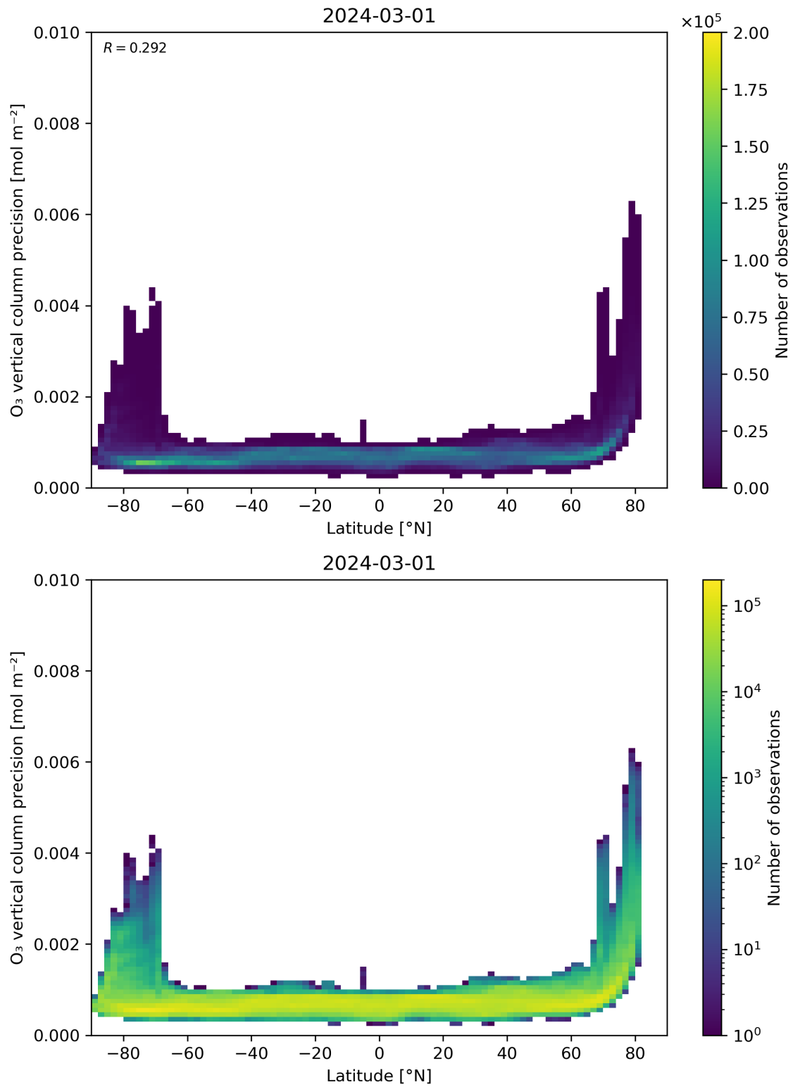
Figure 37: Scatter density plot of “Latitude” against “O 3 vertical column precision” for 2024-02-29 to 2024-03-02.
