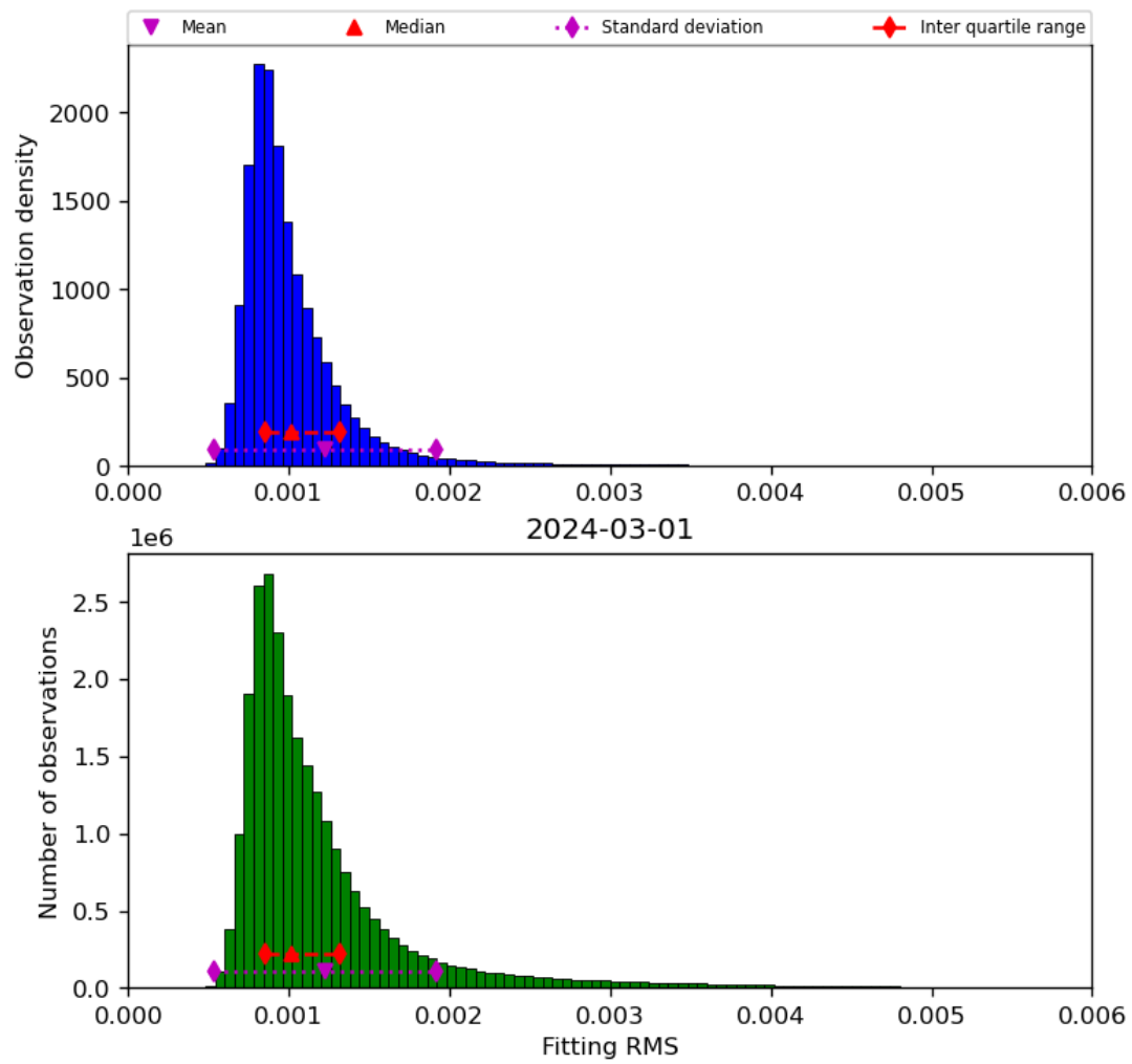
Figure 23: Histogram of “Fitting RMS” for 2024-02-29 to 2024-03-02
