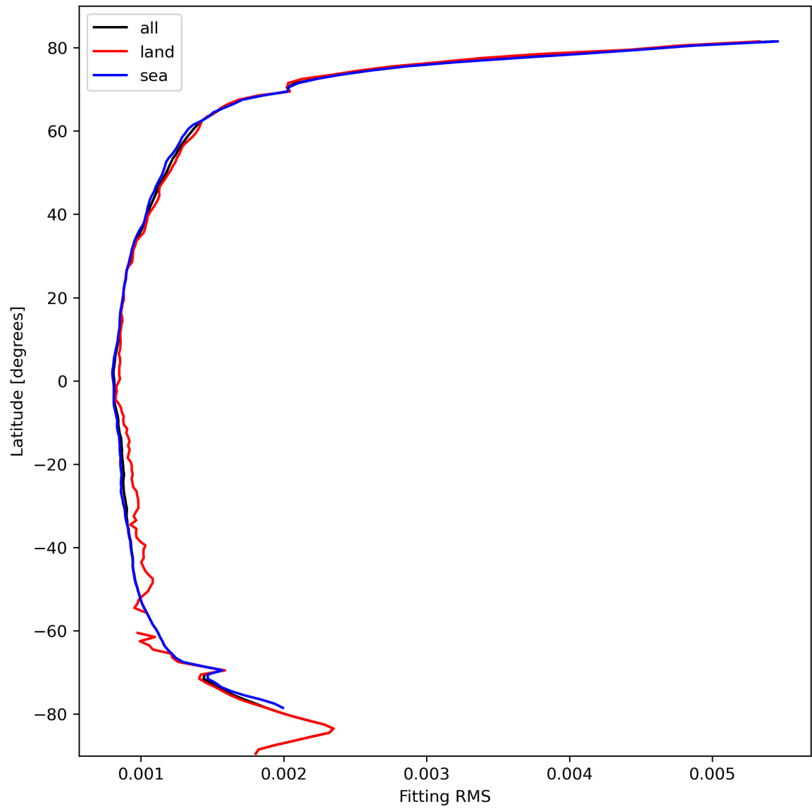
Figure 16: Zonal average of “Fitting RMS” for 2024-02-29 to 2024-03-02.
