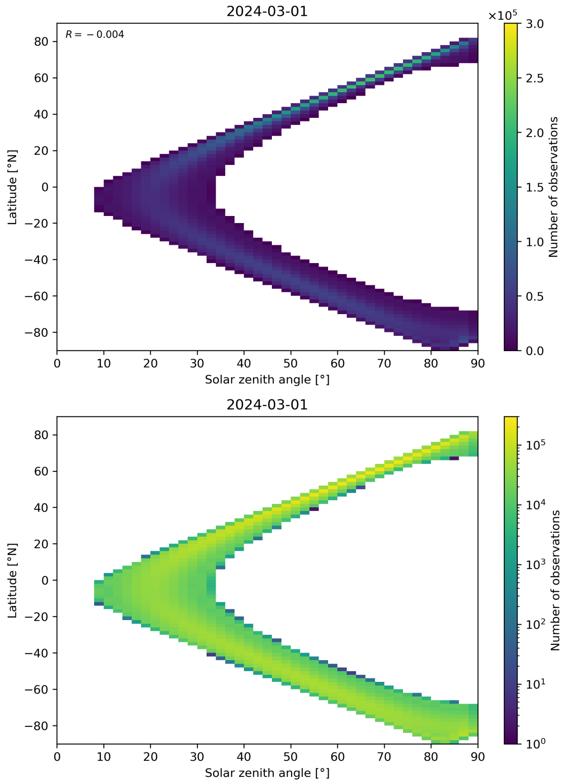
Figure 44: Scatter density plot of “Solar zenith angle” against “Latitude” for 2024-02-29 to 2024-03-02.
