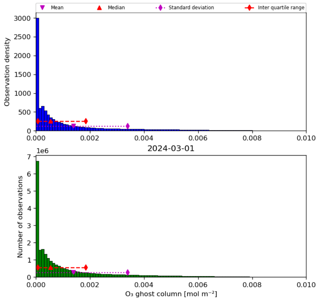
Figure 25: Histogram of “O 3 ghost column” for 2024-02-29 to 2024-03-02
