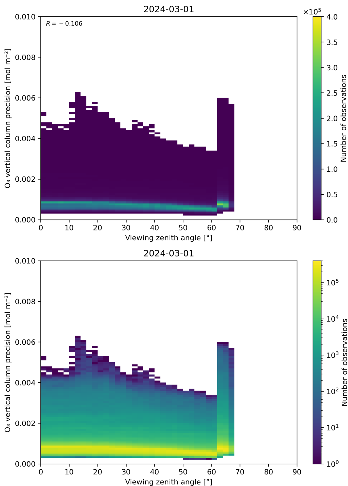
Figure 53: Scatter density plot of “Viewing zenith angle” against “O 3 vertical column precision” for 2024-02-29 to 2024-03-02.
