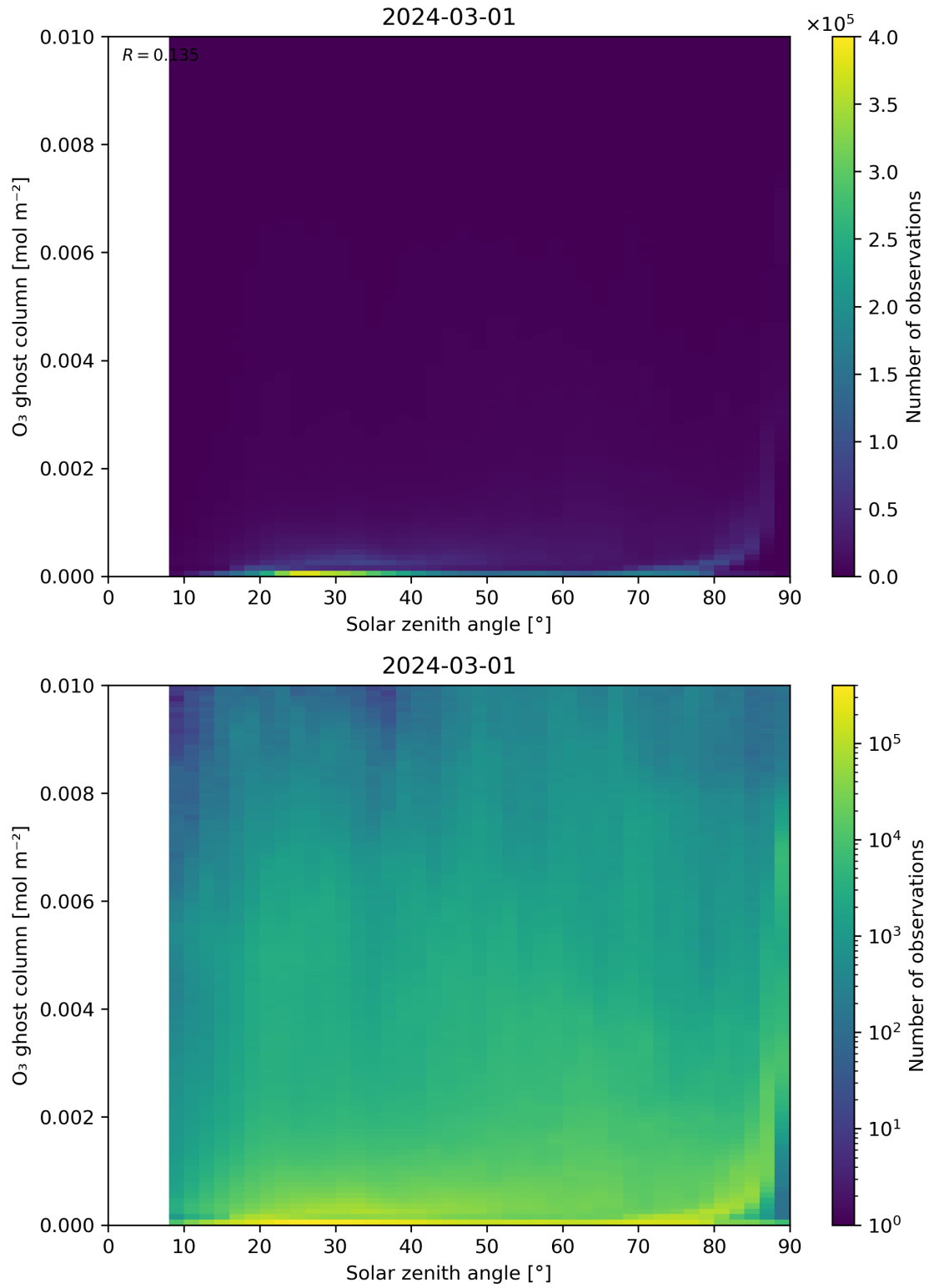
Figure 46: Scatter density plot of “Solar zenith angle” against “O 3 ghost column” for 2024-02-29 to 2024-03-02.
