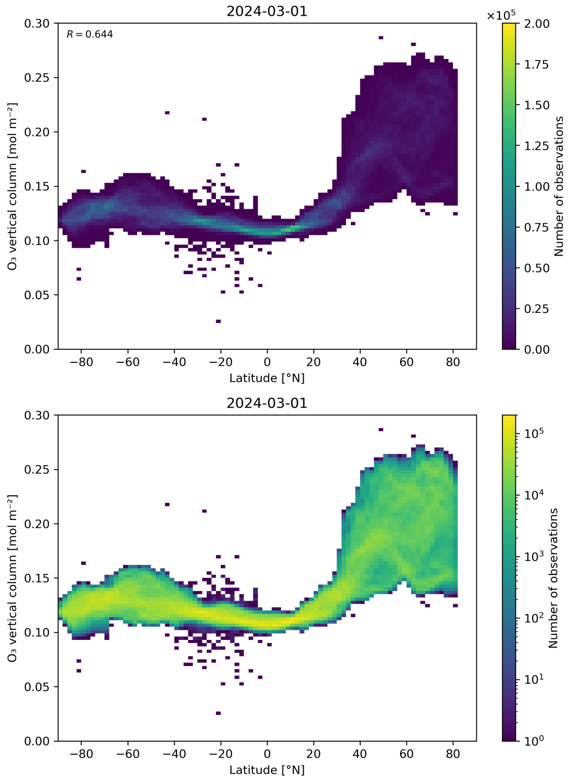
Figure 36: Scatter density plot of “Latitude” against “O 3 vertical column” for 2024-02-29 to 2024-03-02.
