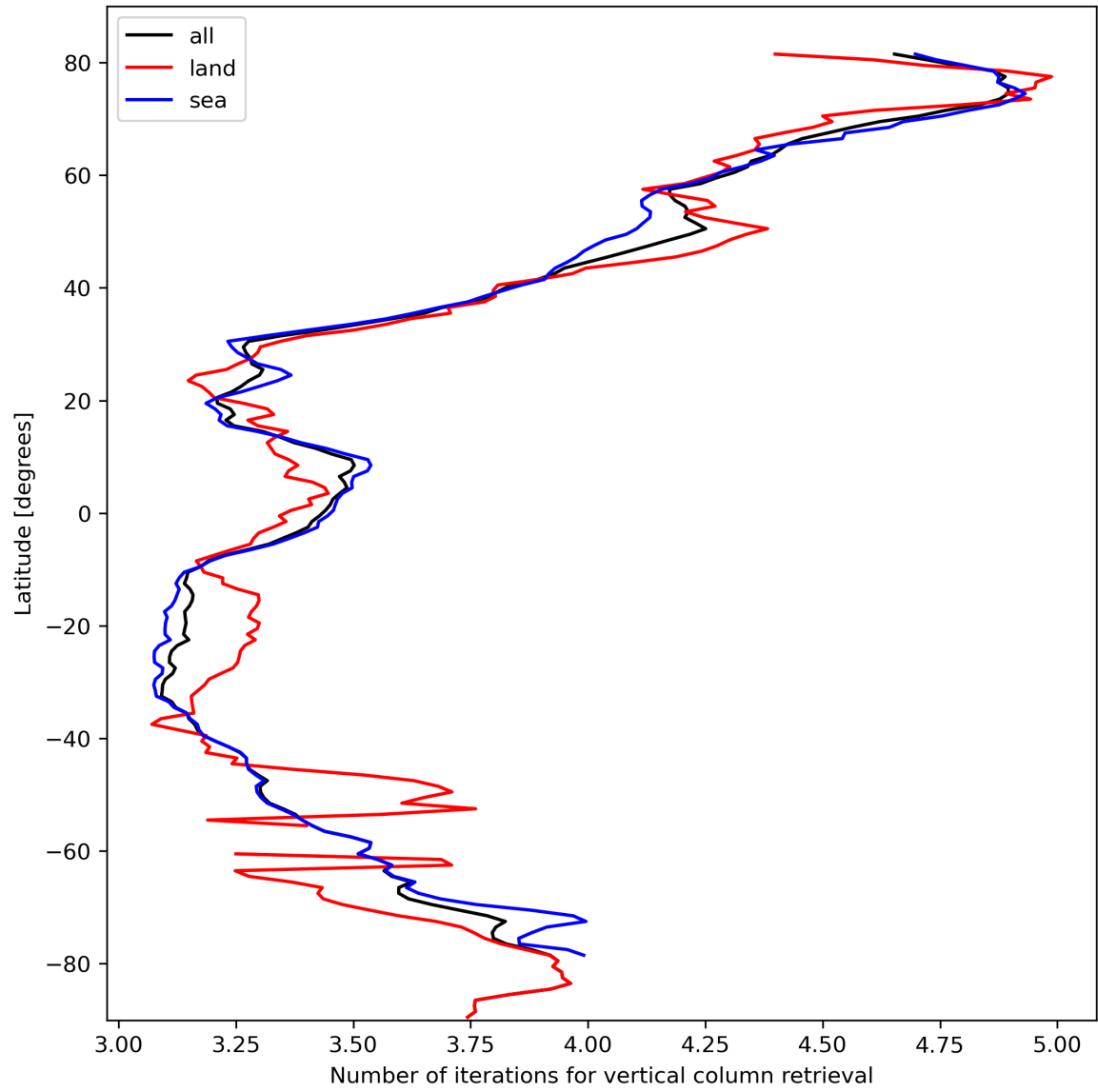
Figure 19: Zonal average of “Number of iterations for vertical column retrieval” for 2024-02-29 to 2024-03-02.
