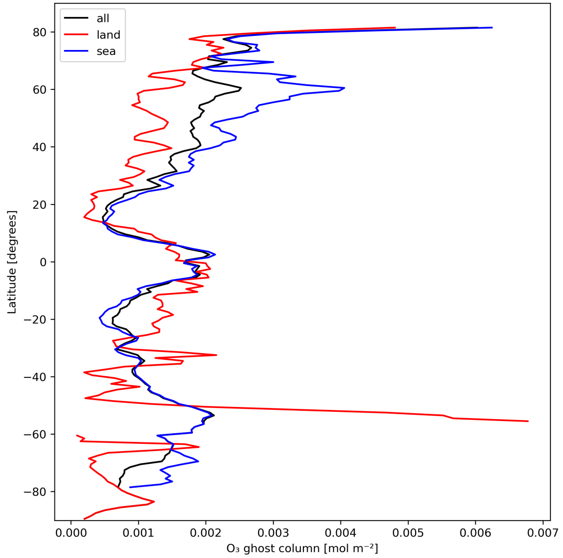
Figure 18: Zonal average of "O 3 ghost column" for 2024-02-29 to 2024-03-02.
