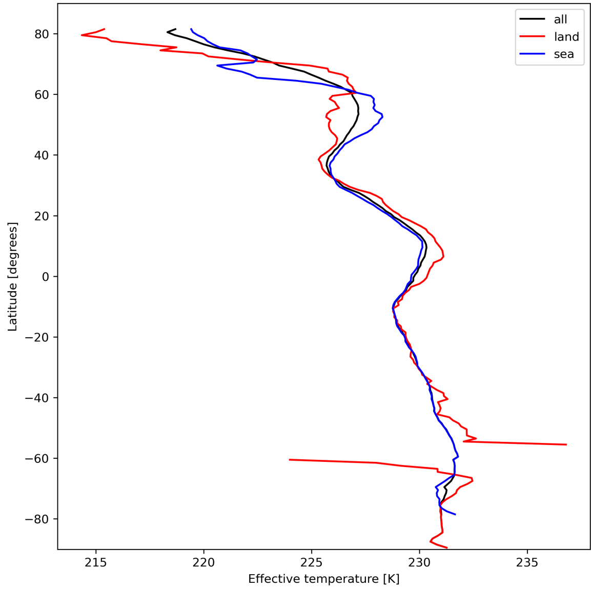
Figure 17: Zonal average of "Effective temperature" for 2024-02-29 to 2024-03-02.
