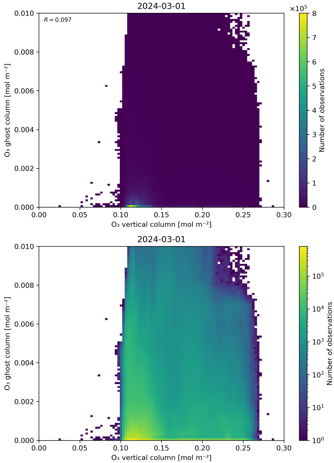
Figure 40: Scatter density plot of “O 3 vertical column” against “O 3 ghost column” for 2024-02-29 to 2024-03-02.
