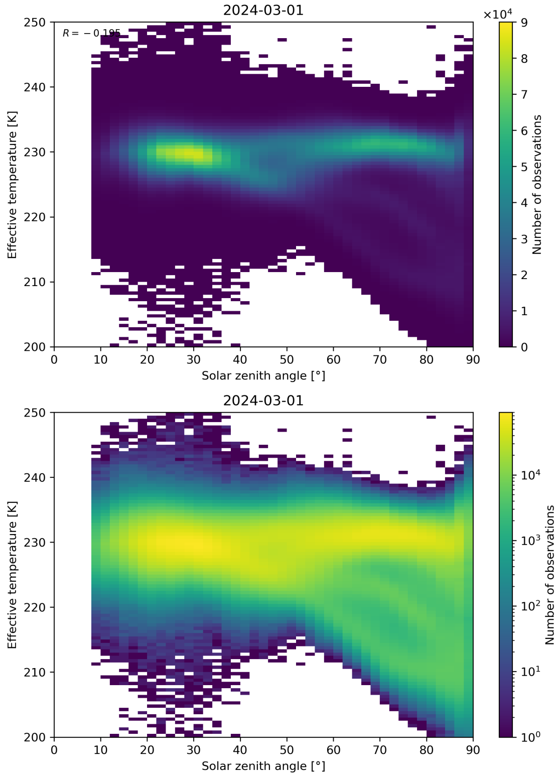
Figure 45: Scatter density plot of “Solar zenith angle” against “Effective temperature” for 2024-02-29 to 2024-03-02.
