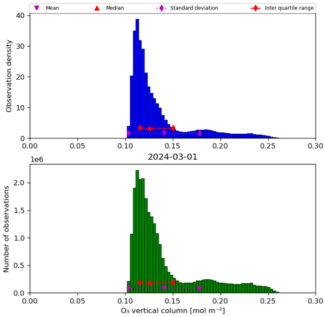
Figure 21: Histogram of “O 3 vertical column” for 2024-02-29 to 2024-03-02
