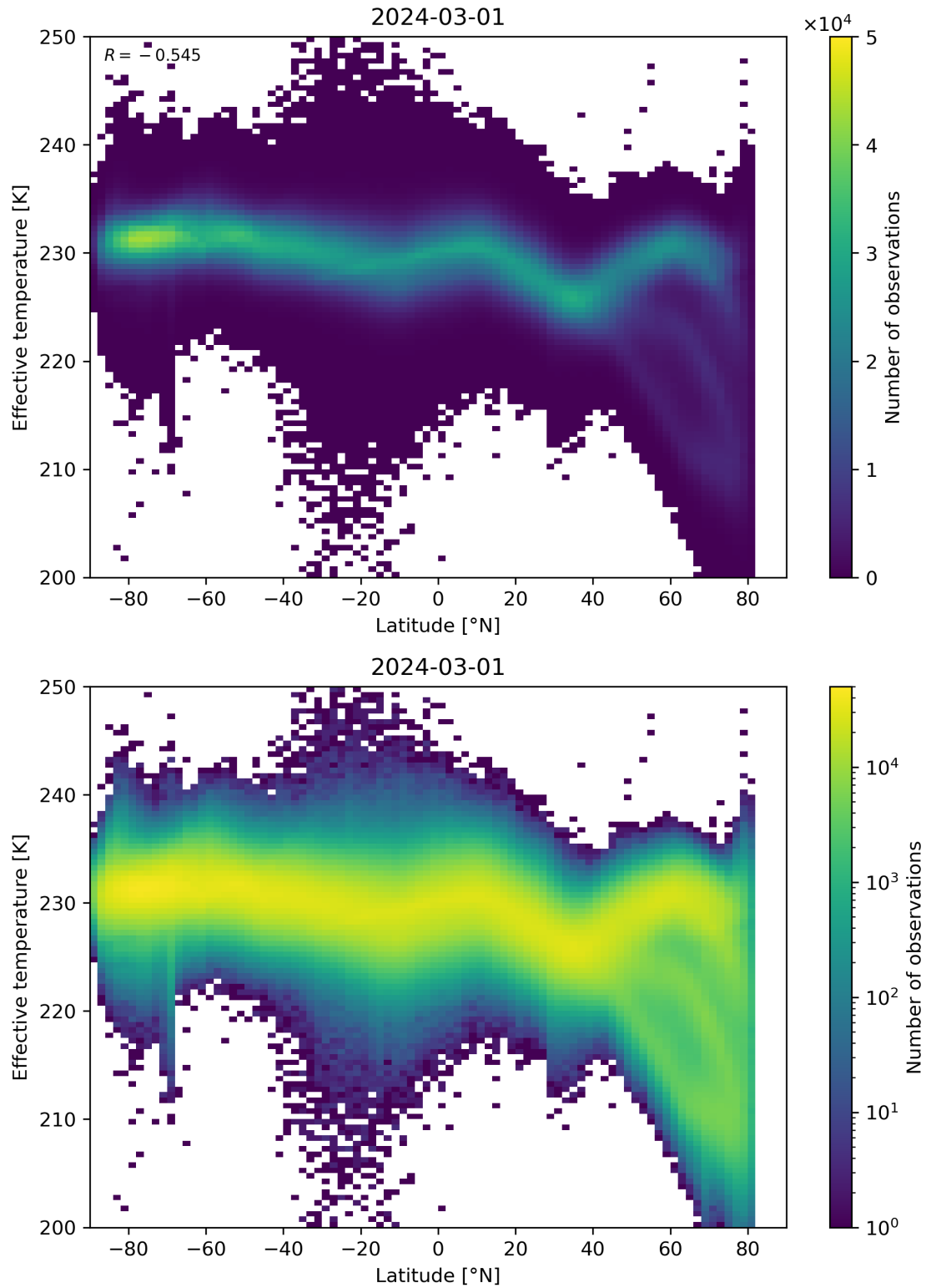
Figure 34: Scatter density plot of “Latitude” against “Effective temperature” for 2024-02-29 to 2024-03-02.
