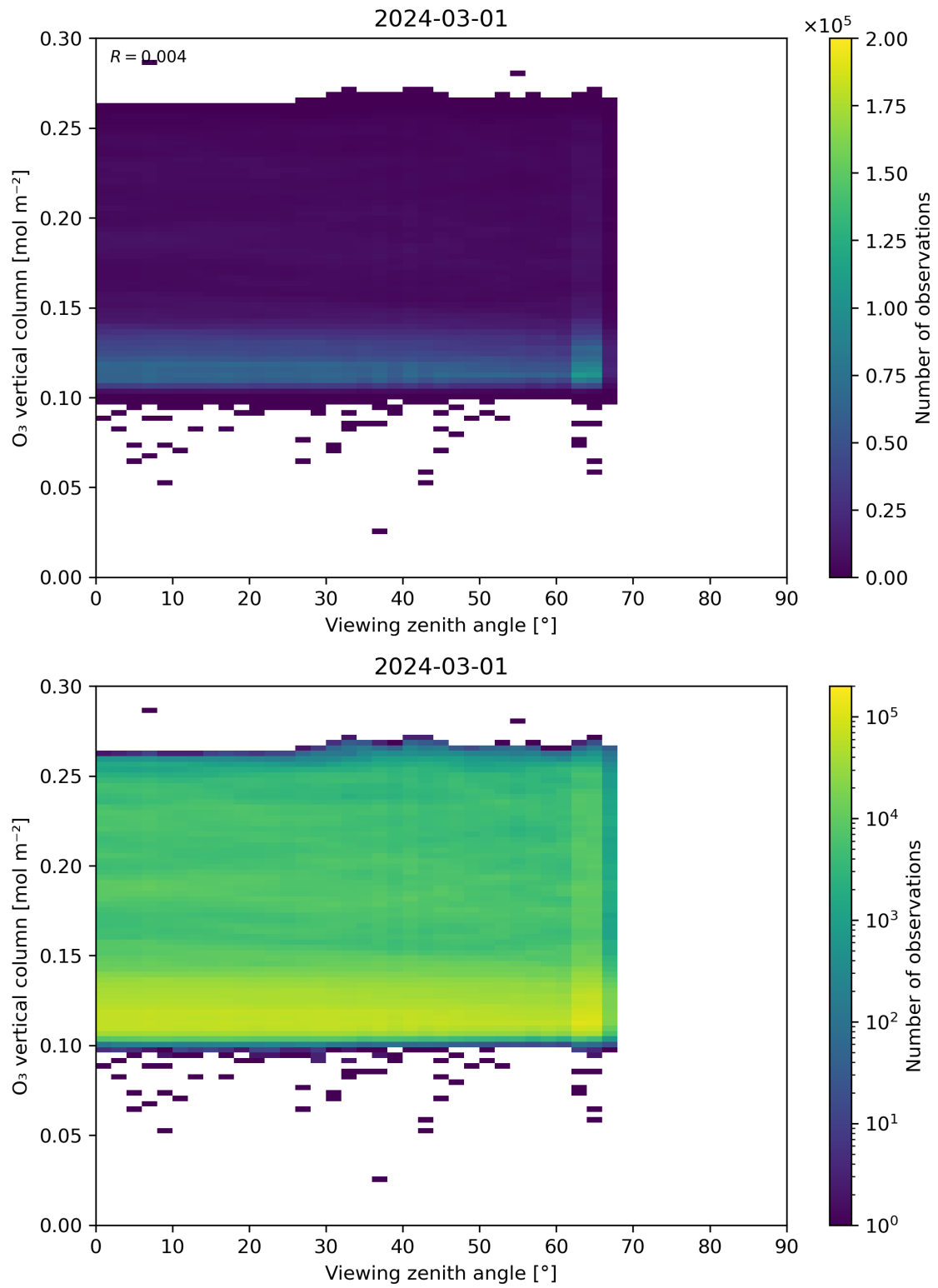
Figure 52: Scatter density plot of “Viewing zenith angle” against “O 3 vertical column” for 2024-02-29 to 2024-03-02.
