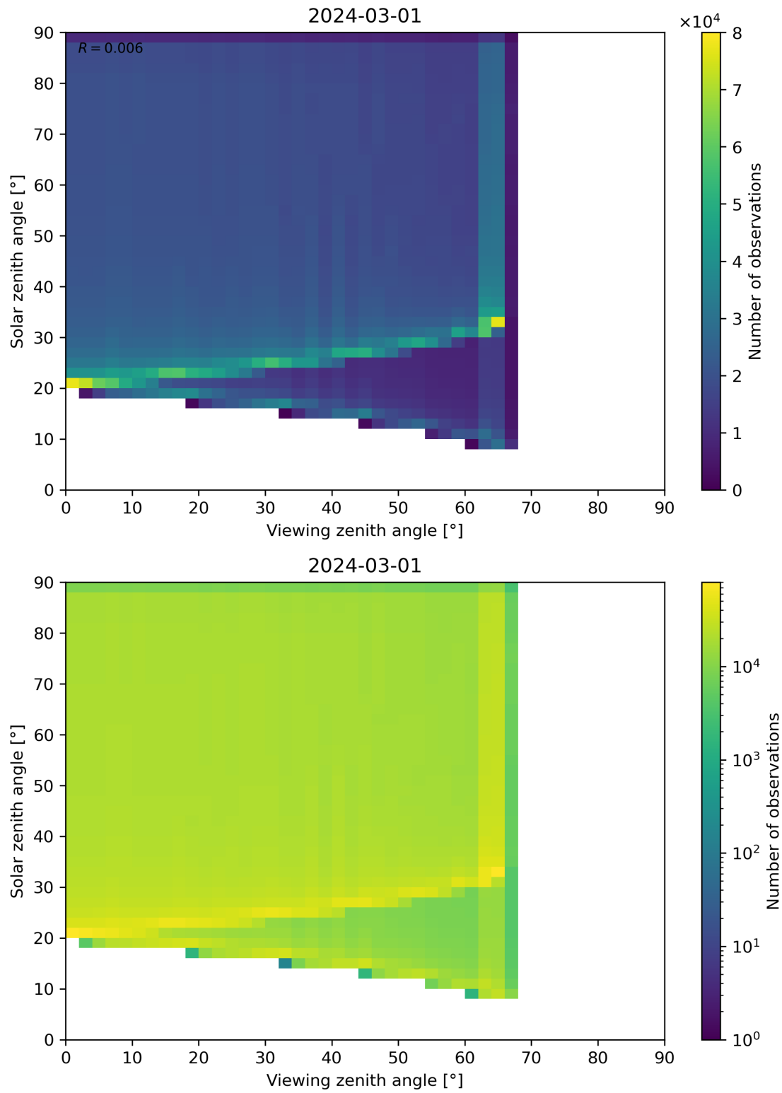
Figure 54: Scatter density plot of “Viewing zenith angle” against “Solar zenith angle” for 2024-02-29 to 2024-03-02.
