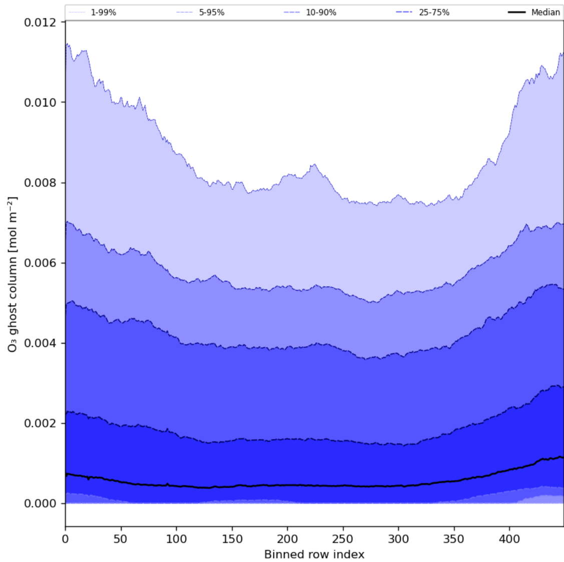
Figure 32: Along track statistics of "O 3 ghost column" for 2024-02-29 to 2024-03-02
