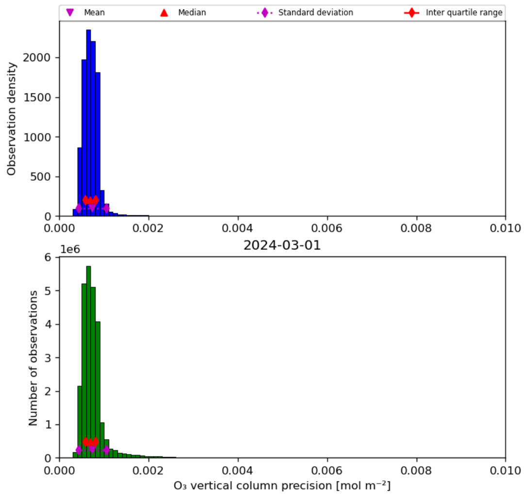
Figure 22: Histogram of “O 3 vertical column precision” for 2024-02-29 to 2024-03-02
