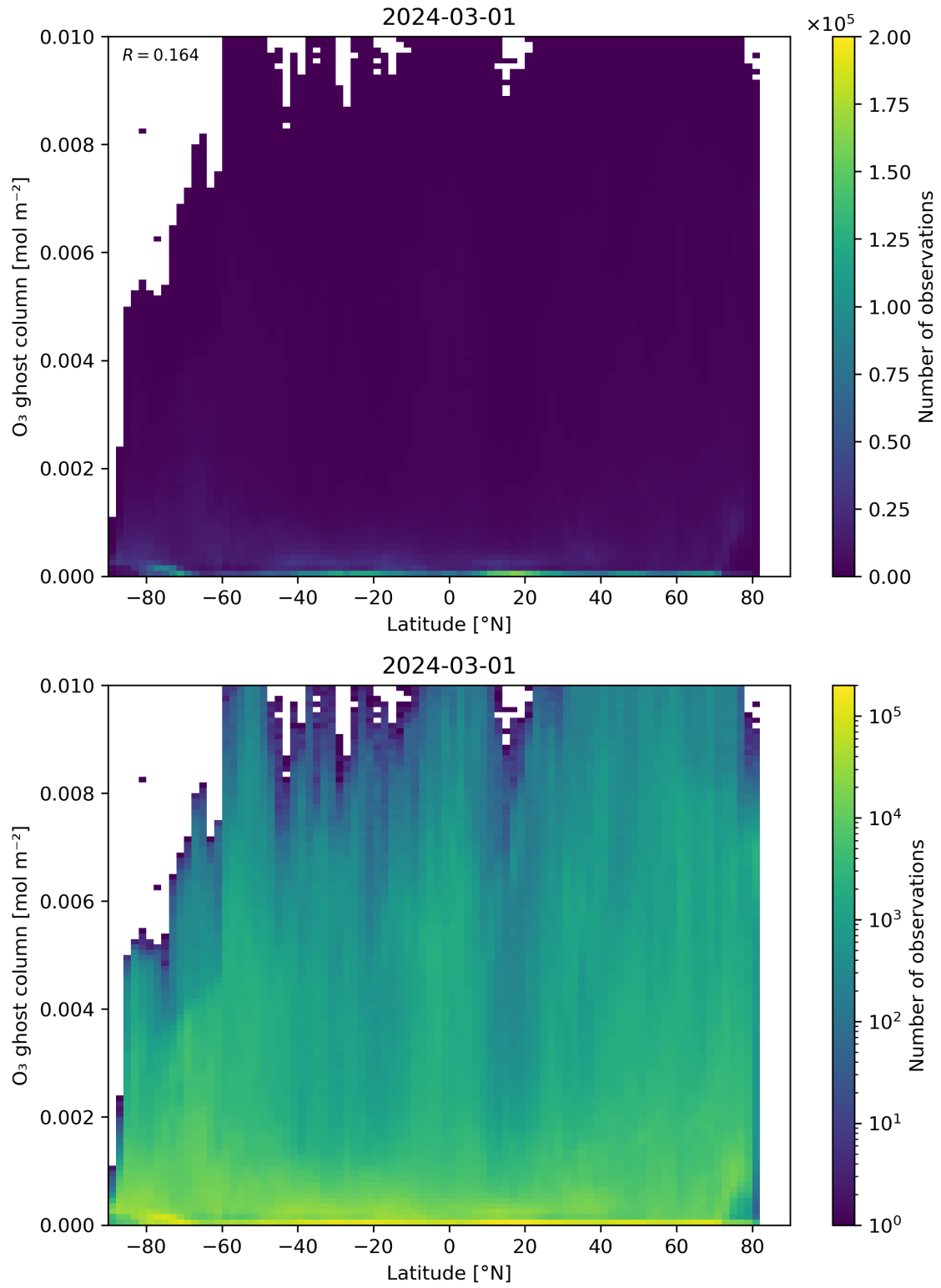
Figure 35: Scatter density plot of “Latitude” against “O 3 ghost column” for 2024-02-29 to 2024-03-02.
