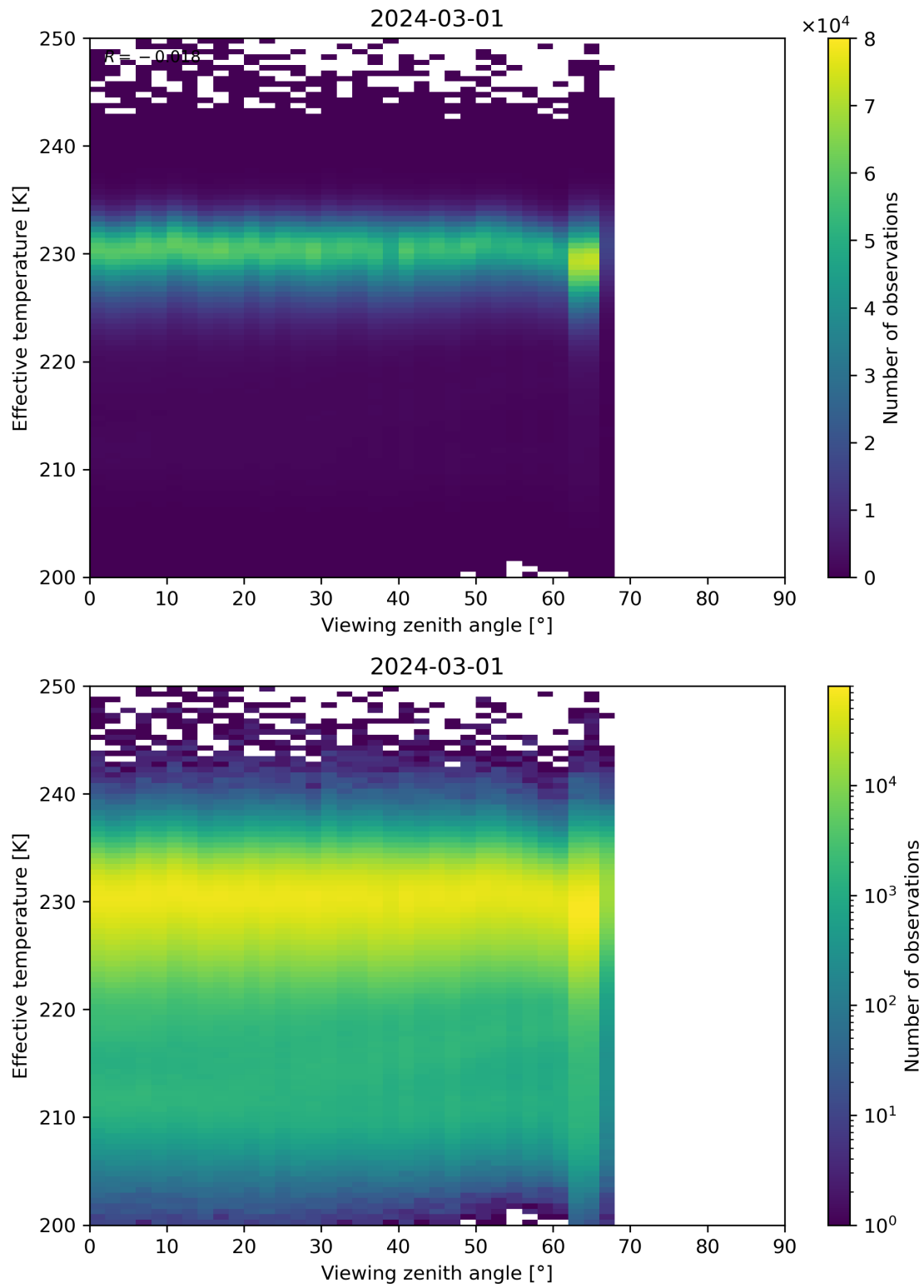
Figure 50: Scatter density plot of “Viewing zenith angle” against “Effective temperature” for 2024-02-29 to 2024-03-02.
