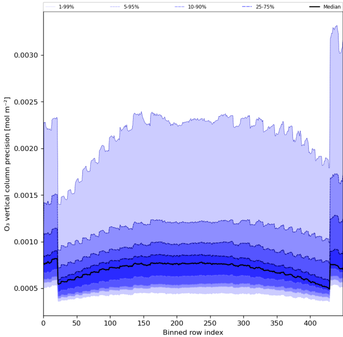
Figure 29: Along track statistics of “O 3 vertical column precision” for 2024-02-29 to 2024-03-02
