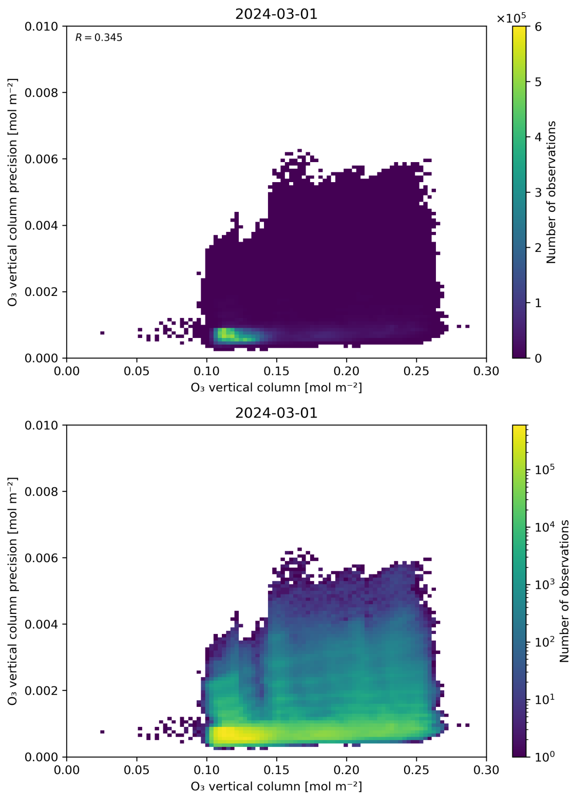
Figure 41: Scatter density plot of “O 3 vertical column” against “O 3 vertical column precision” for 2024-02-29 to 2024-03-02.
