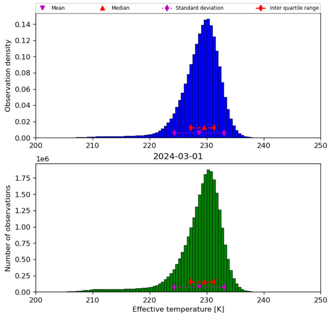
Figure 24: Histogram of “Effective temperature” for 2024-02-29 to 2024-03-02
