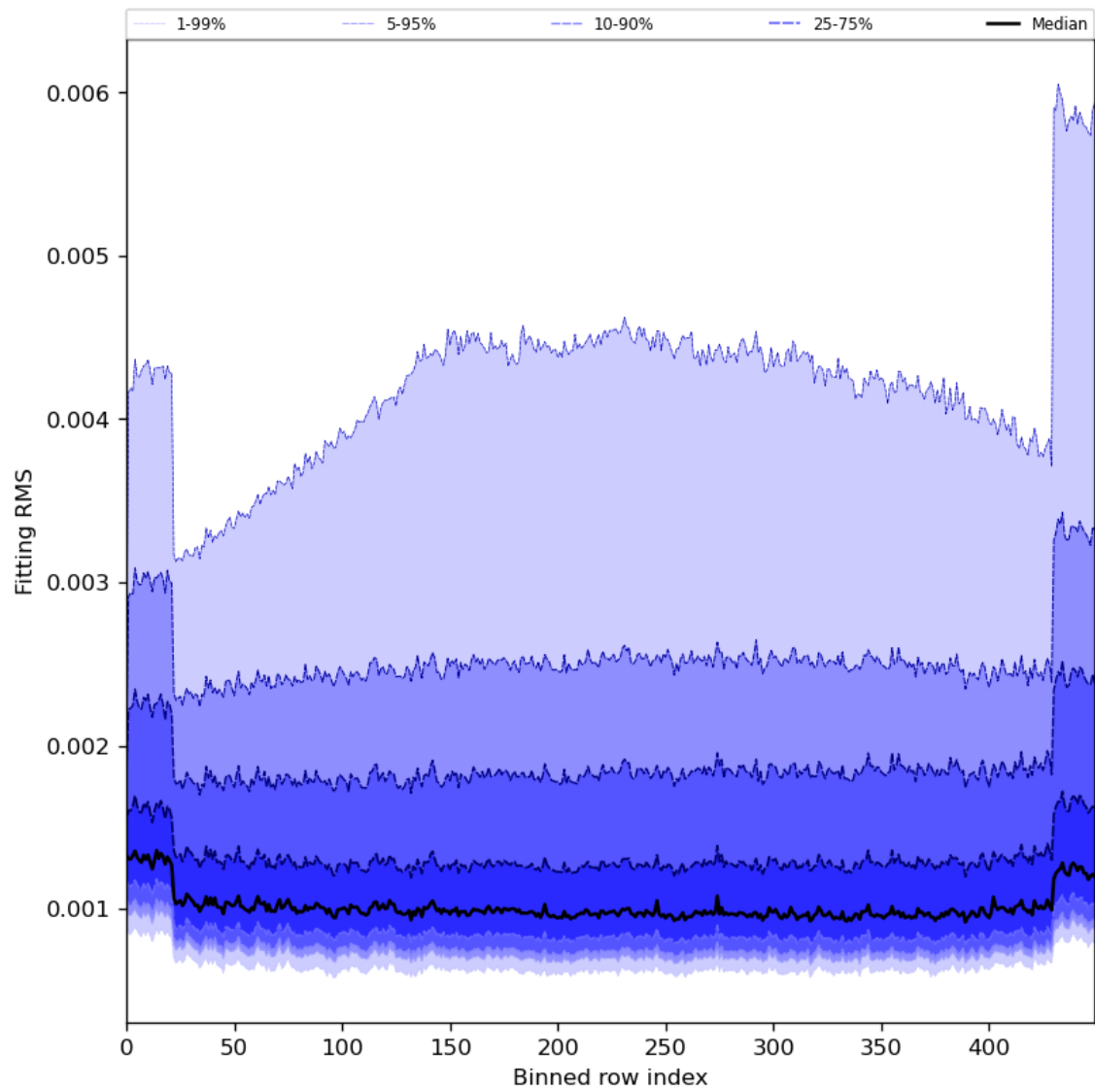
Figure 30: Along track statistics of “Fitting RMS” for 2024-02-29 to 2024-03-02
