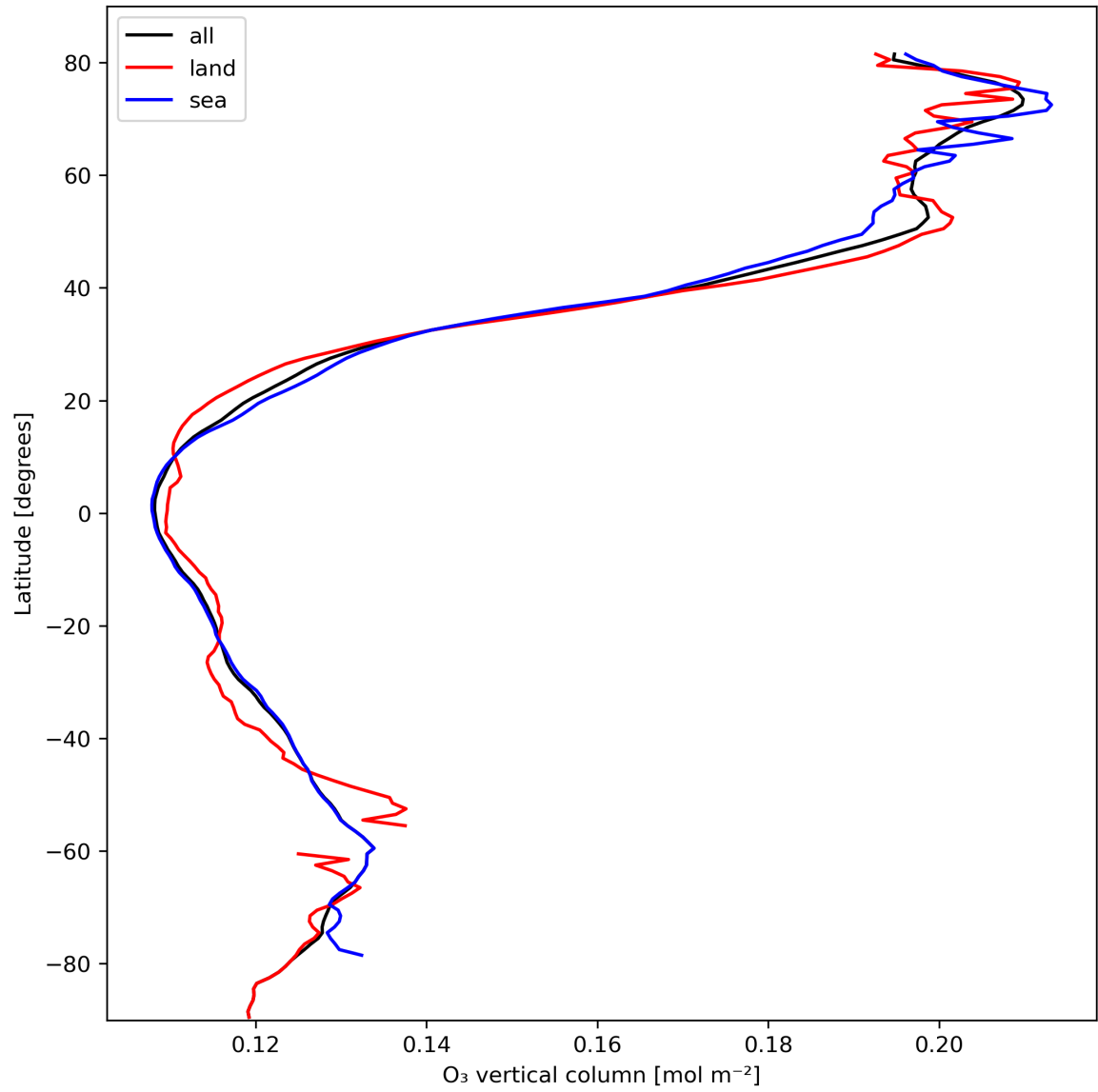
Figure 14: Zonal average of “O 3 vertical column” for 2024-02-29 to 2024-03-02.
