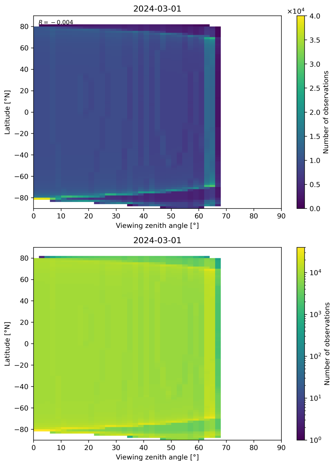
Figure 49: Scatter density plot of “Viewing zenith angle” against “Latitude” for 2024-02-29 to 2024-03-02.
