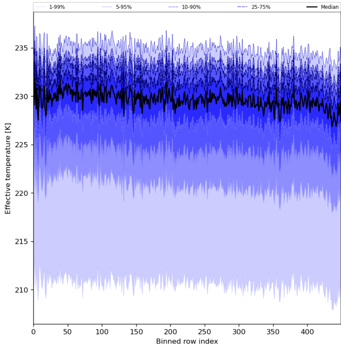
Figure 31: Along track statistics of “Effective temperature” for 2024-02-29 to 2024-03-02
