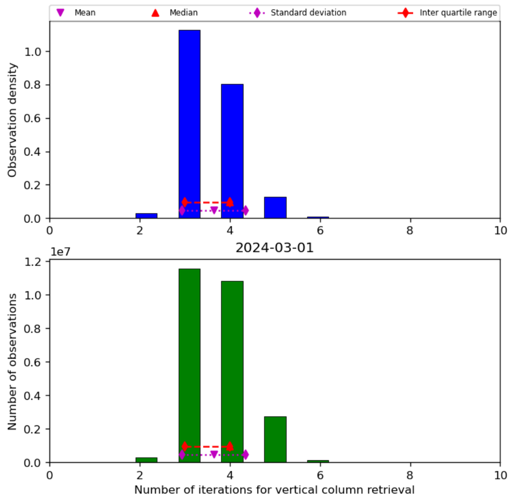
Figure 26: Histogram of “Number of iterations for vertical column retrieval” for 2024-02-29 to 2024-03-02
