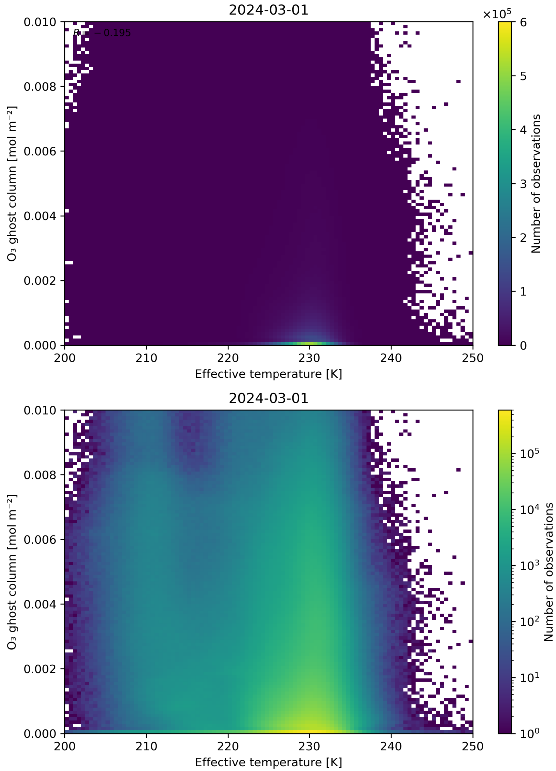
Figure 38: Scatter density plot of “Effective temperature” against “O 3 ghost column” for 2024-02-29 to 2024-03-02.
