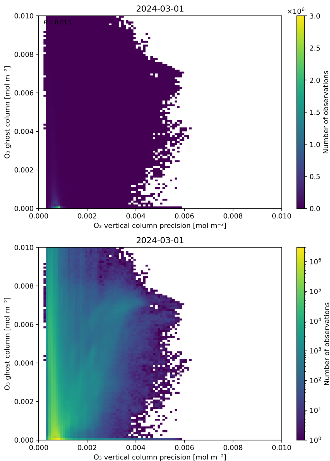
Figure 43: Scatter density plot of “O 3 vertical column precision” against “O 3 ghost column” for 2024-02-29 to 2024-03-02.
