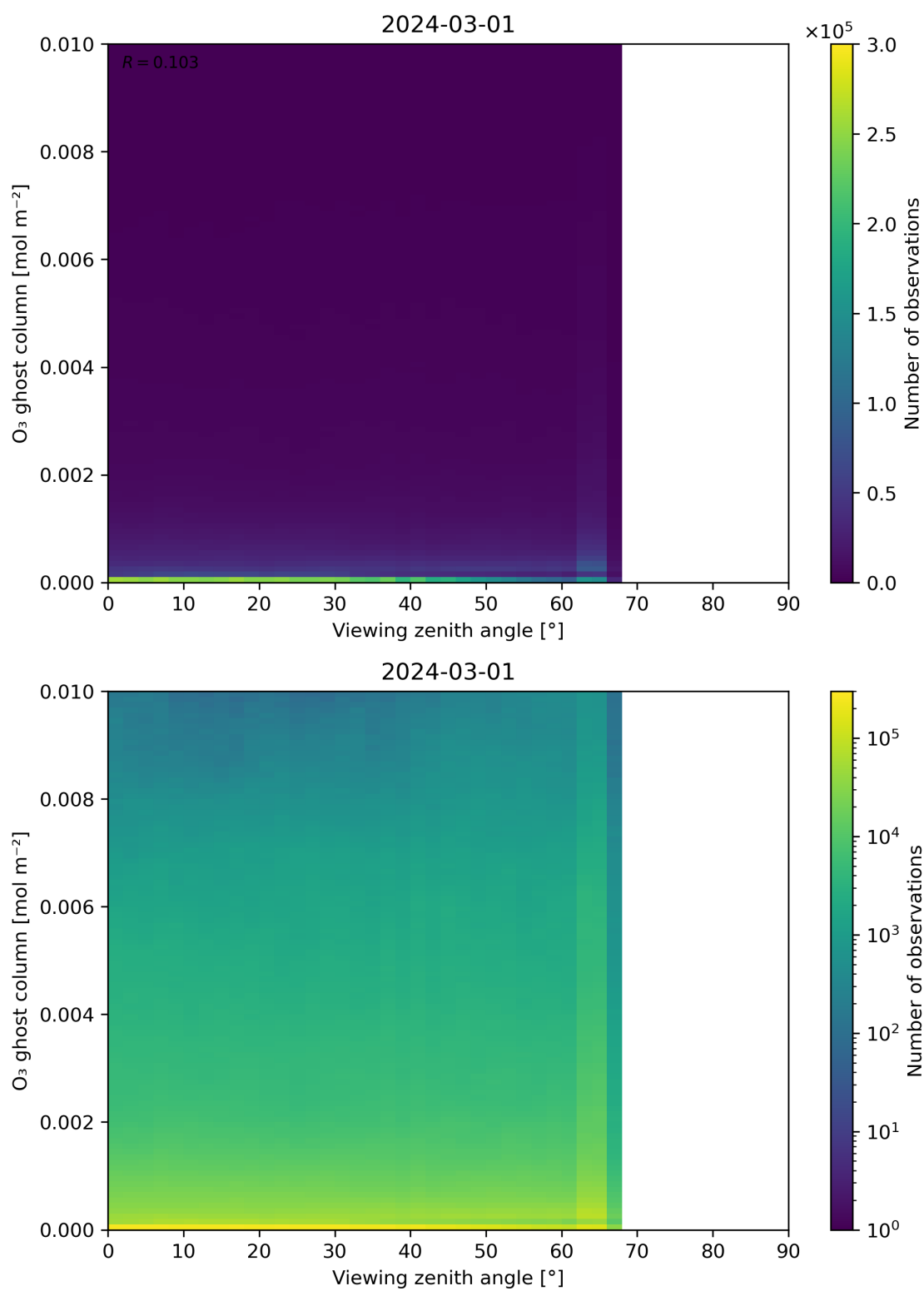
Figure 51: Scatter density plot of “Viewing zenith angle” against “O 3 ghost column” for 2024-02-29 to 2024-03-02.
