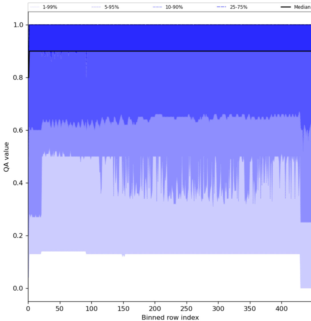
Figure 27: Along track statistics of “QA value” for 2024-02-29 to 2024-03-02
