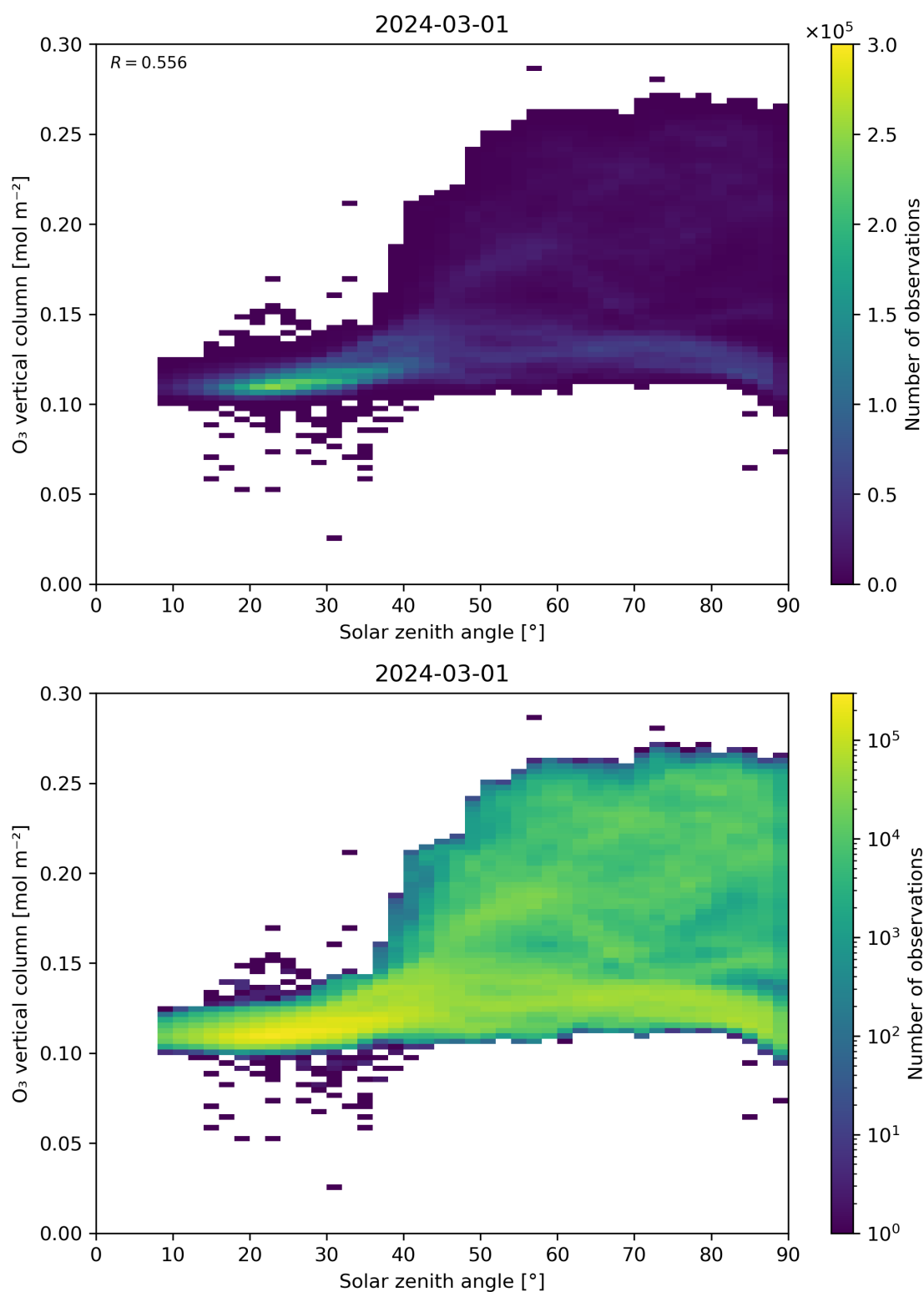
Figure 47: Scatter density plot of “Solar zenith angle” against “O 3 vertical column” for 2024-02-29 to 2024-03-02.
