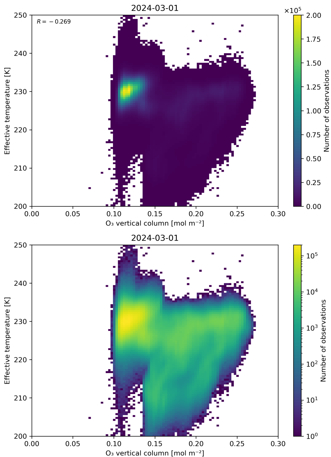
Figure 39: Scatter density plot of “O 3 vertical column” against “Effective temperature” for 2024-02-29 to 2024-03-02.
