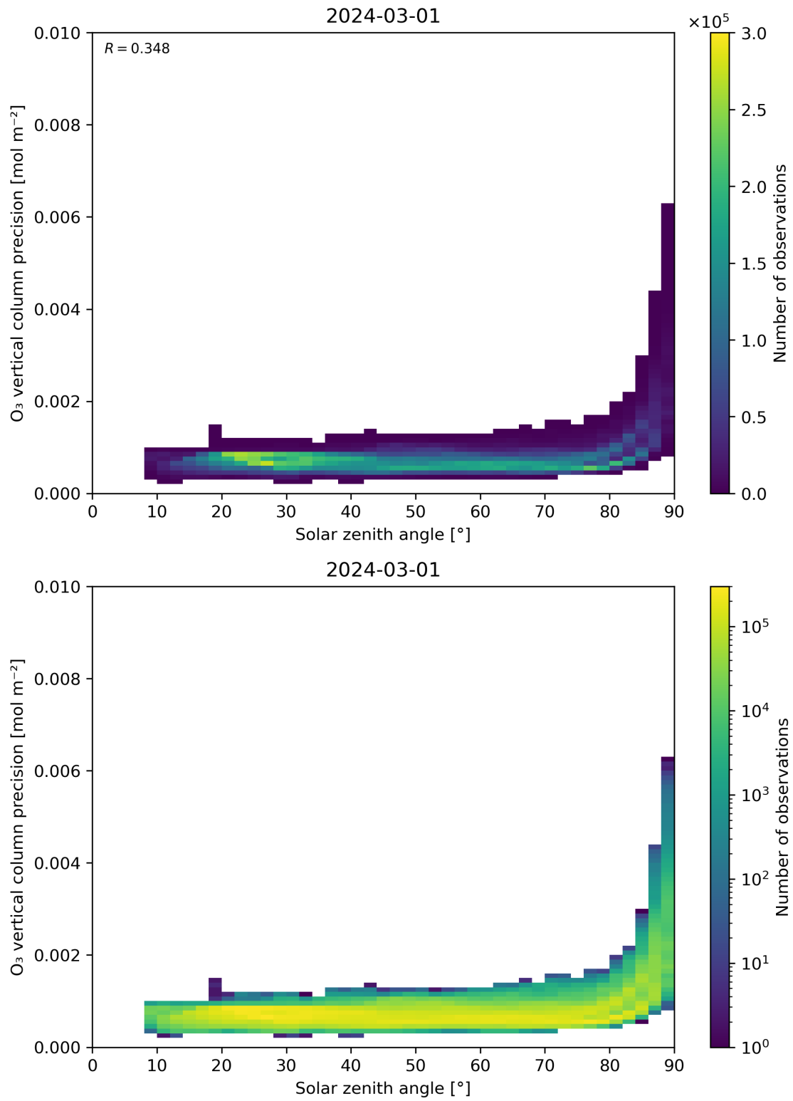
Figure 48: Scatter density plot of “Solar zenith angle” against “O 3 vertical column precision” for 2024-02-29 to 2024-03-02.
