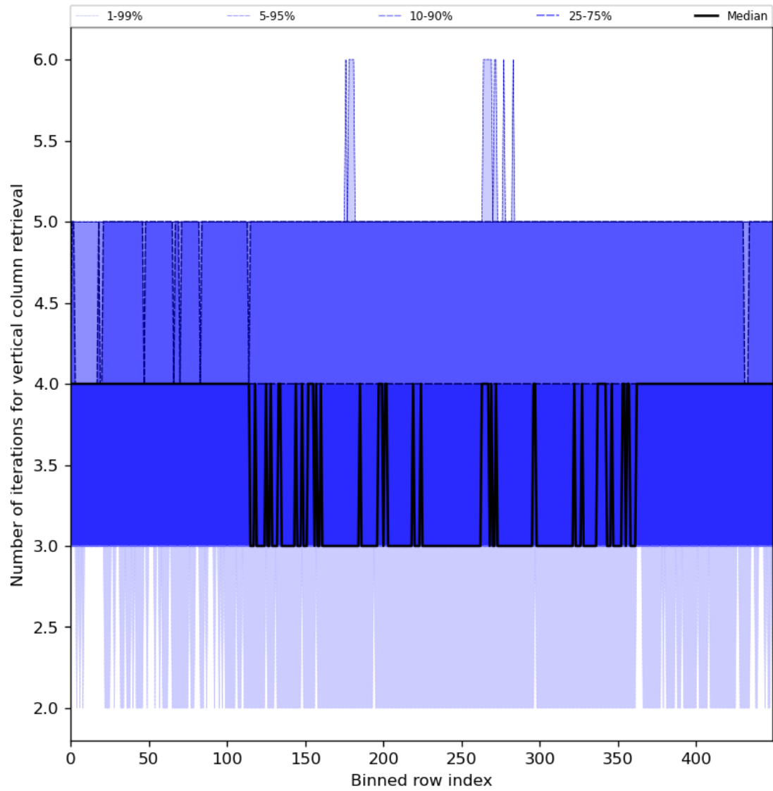
Figure 33: Along track statistics of “Number of iterations for vertical column retrieval” for 2024-02-29 to 2024-03-02
