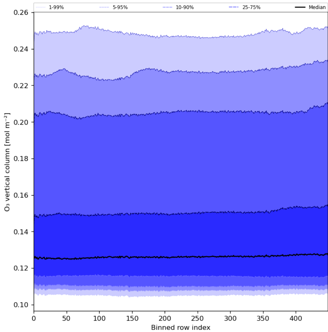
Figure 28: Along track statistics of “O 3 vertical column” for 2024-02-29 to 2024-03-02
