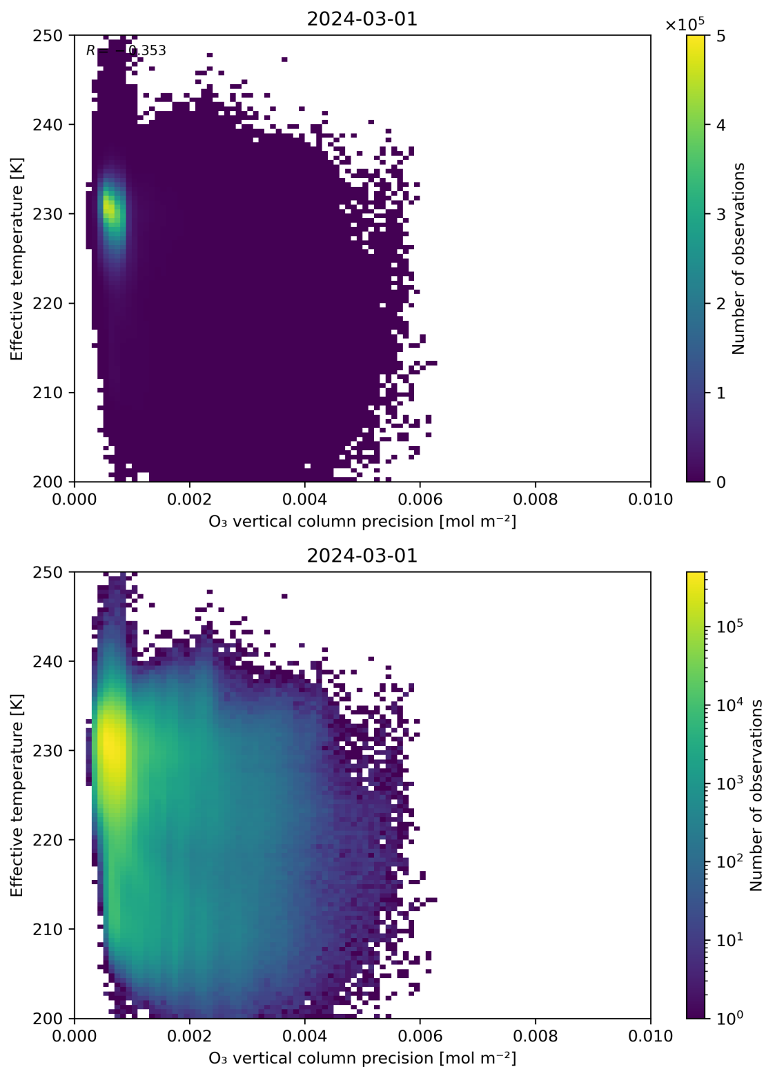
Figure 42: Scatter density plot of “O 3 vertical column precision” against “Effective temperature” for 2024-02-29 to 2024-03-02.
