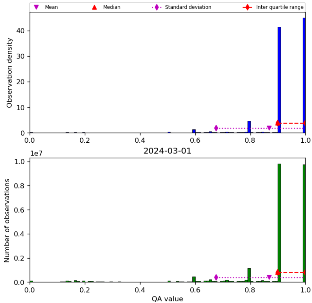
Figure 20: Histogram of “QA value” for 2024-02-29 to 2024-03-02
