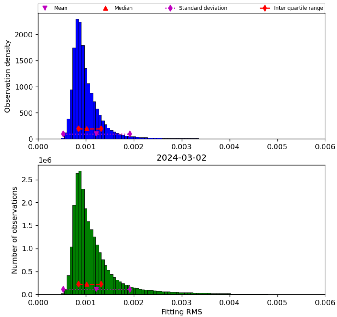
Figure 23: Histogram of “Fitting RMS” for 2024-03-01 to 2024-03-03
