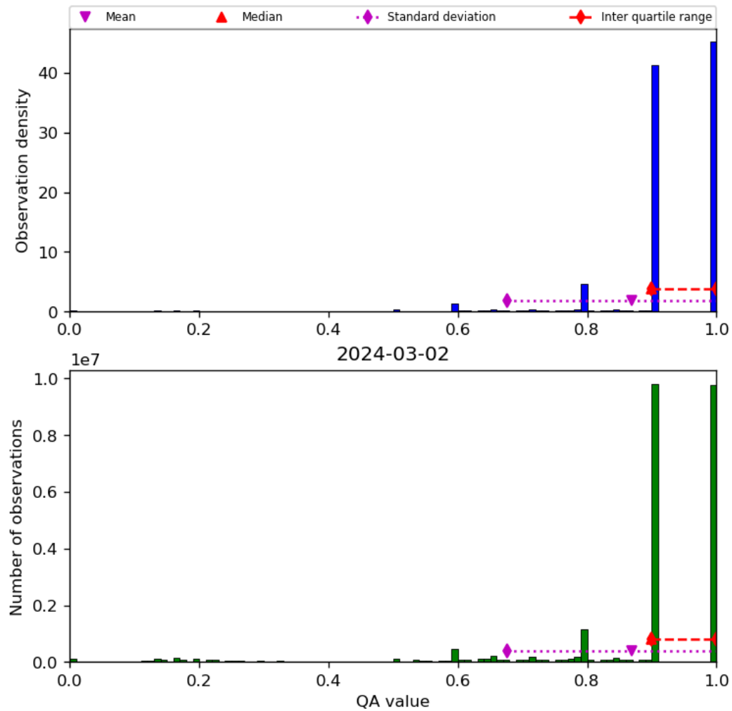
Figure 20: Histogram of “QA value” for 2024-03-01 to 2024-03-03
