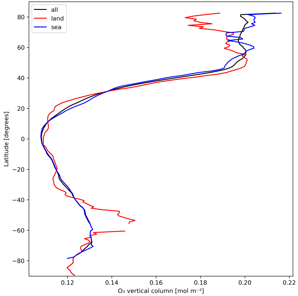
Figure 14: Zonal average of “O 3 vertical column” for 2024-03-01 to 2024-03-03.
