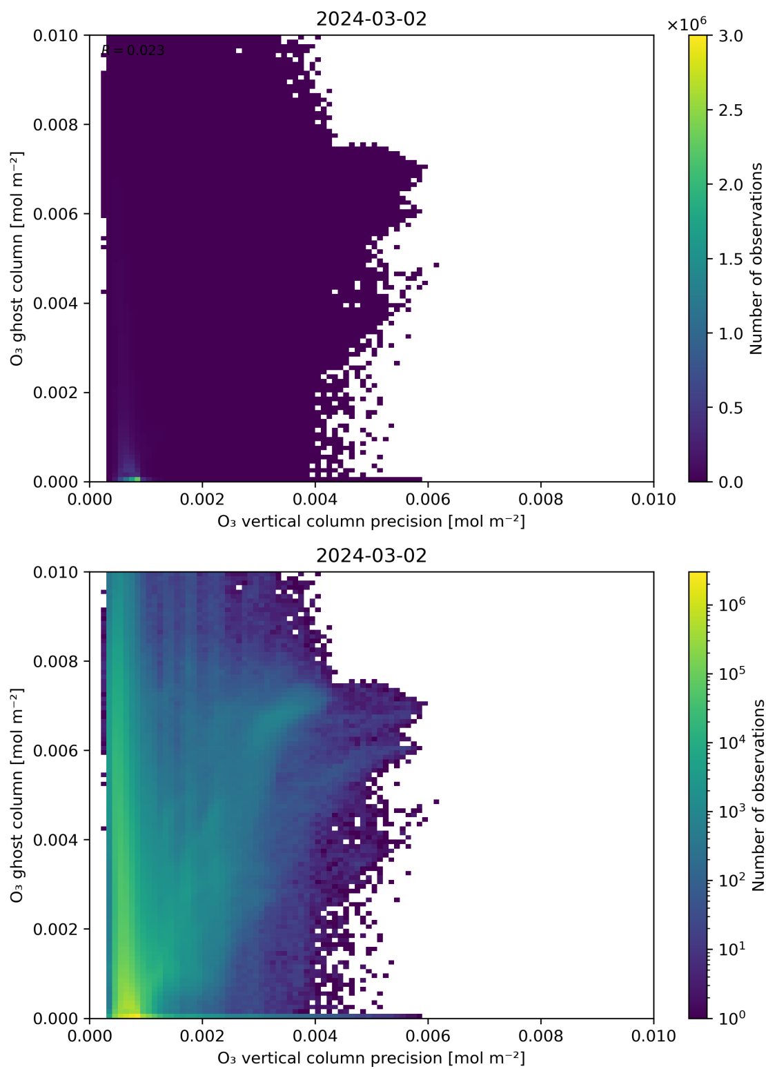
Figure 43: Scatter density plot of “ O_3 vertical column precision” against “ O_3 ghost column” for 2024-03-01 to 2024-03-03.
