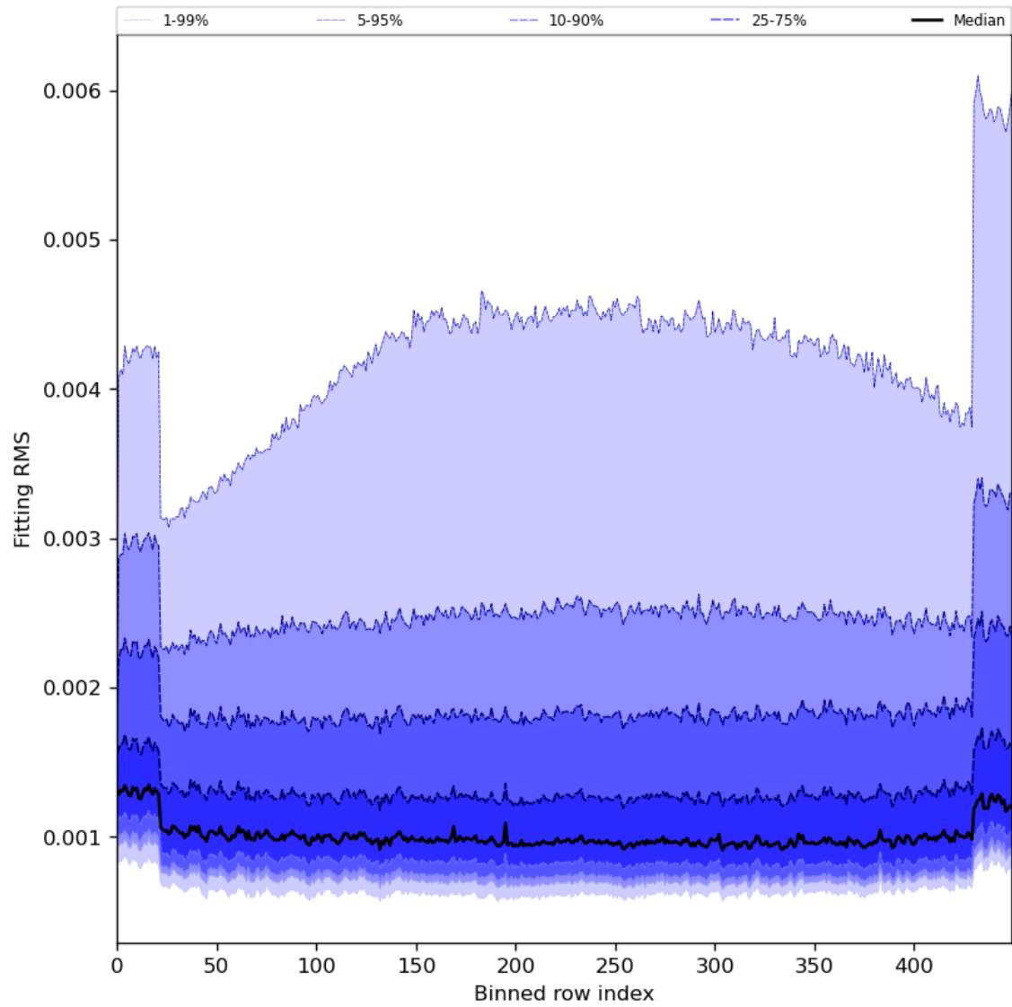
Figure 30: Along track statistics of “Fitting RMS” for 2024-03-01 to 2024-03-03
