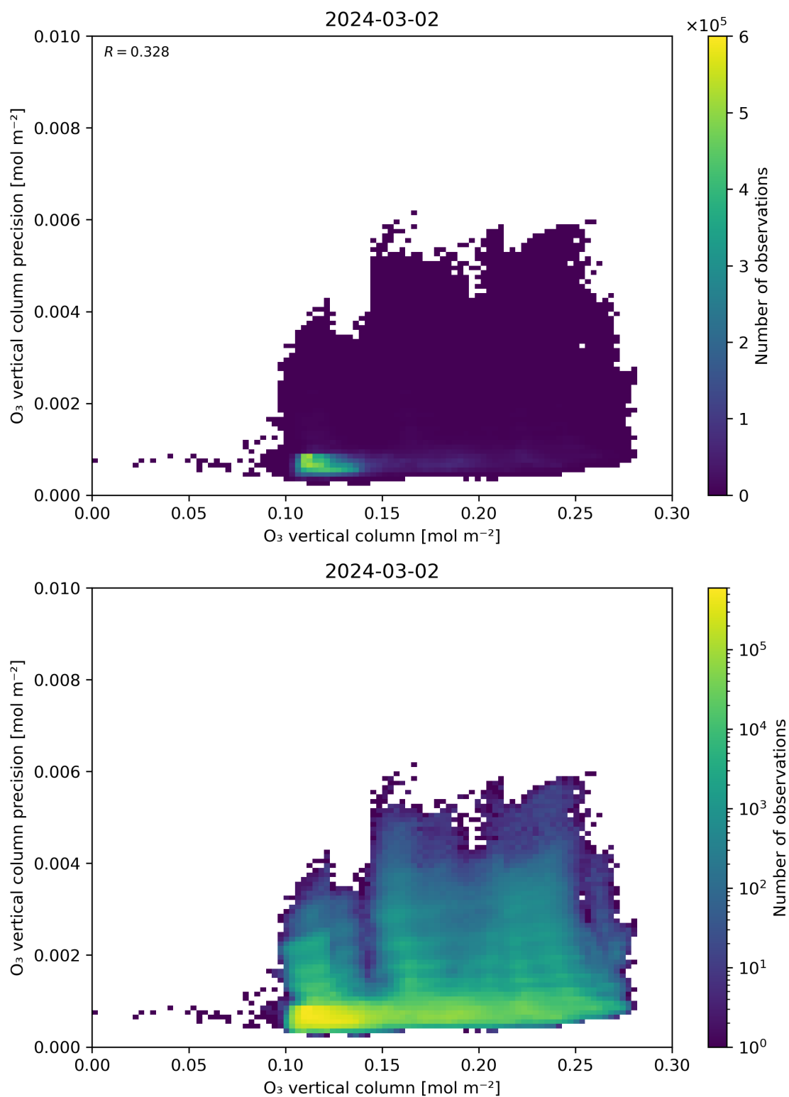
Figure 41: Scatter density plot of “O 3 vertical column” against “O 3 vertical column precision” for 2024-03-01 to 2024-03-03.
