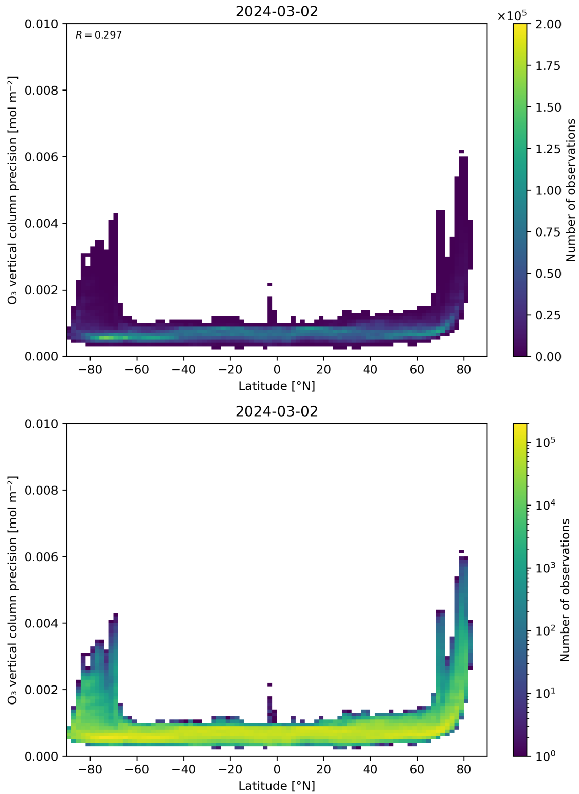
Figure 37: Scatter density plot of “Latitude” against “O 3 vertical column precision” for 2024-03-01 to 2024-03-03.
