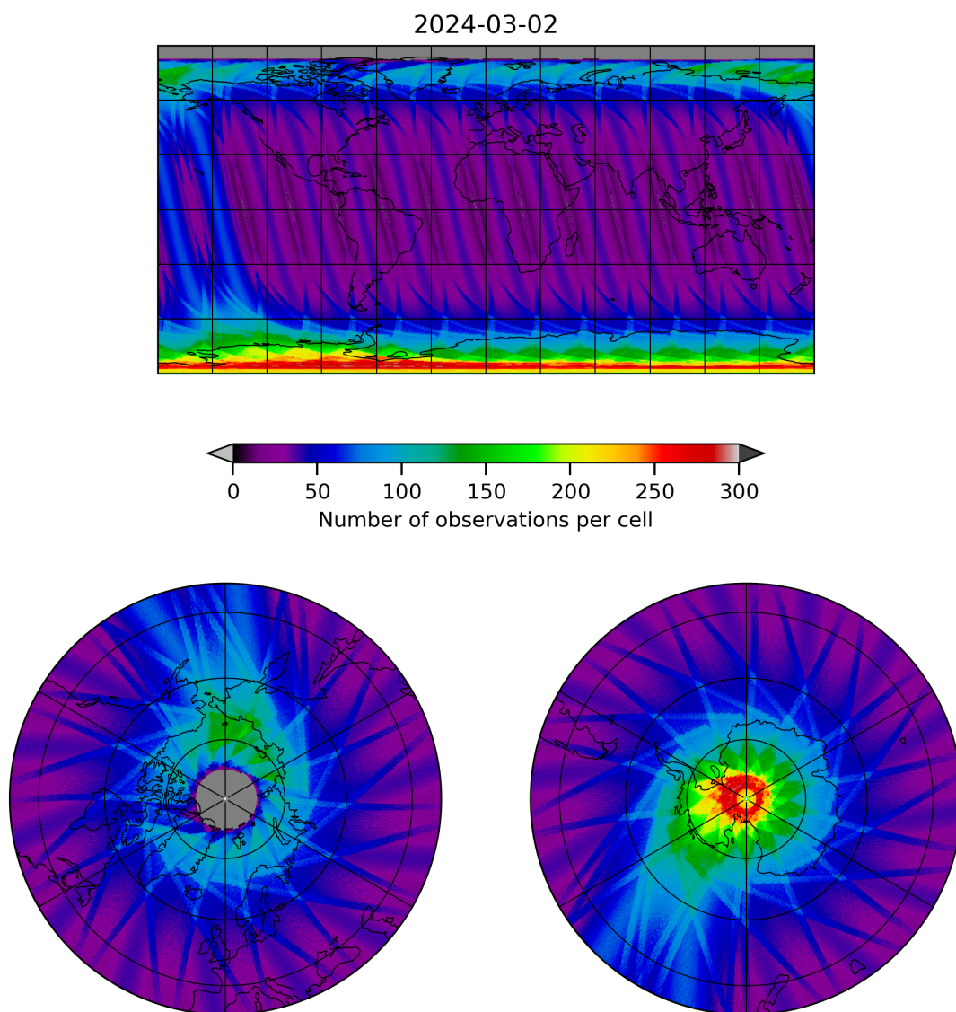
Figure 12: Map of the number of observations for 2024-03-01 to 2024-03-03
