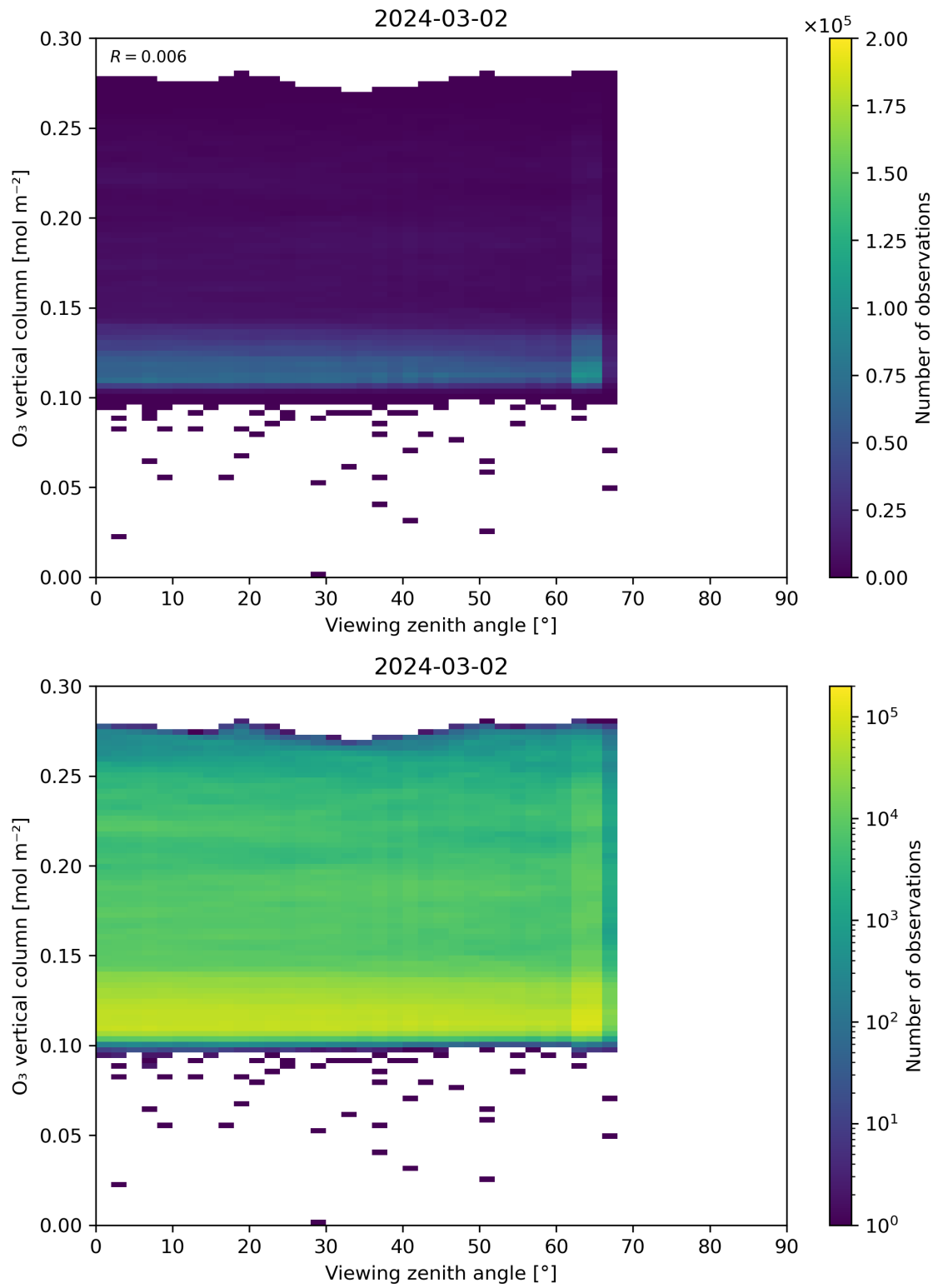
Figure 52: Scatter density plot of “Viewing zenith angle” against “O 3 vertical column” for 2024-03-01 to 2024-03-03.
