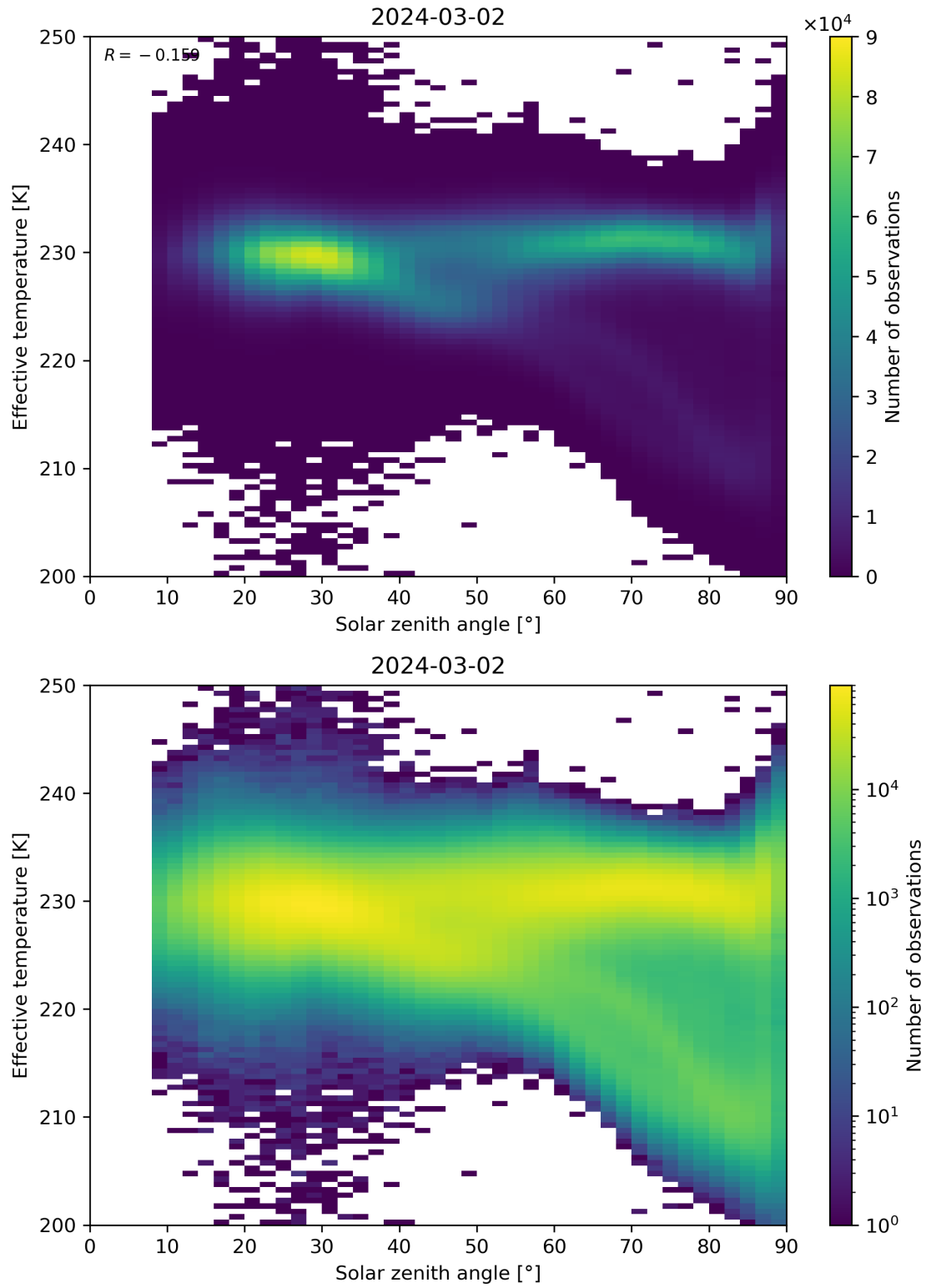
Figure 45: Scatter density plot of “Solar zenith angle” against “Effective temperature” for 2024-03-01 to 2024-03-03.
