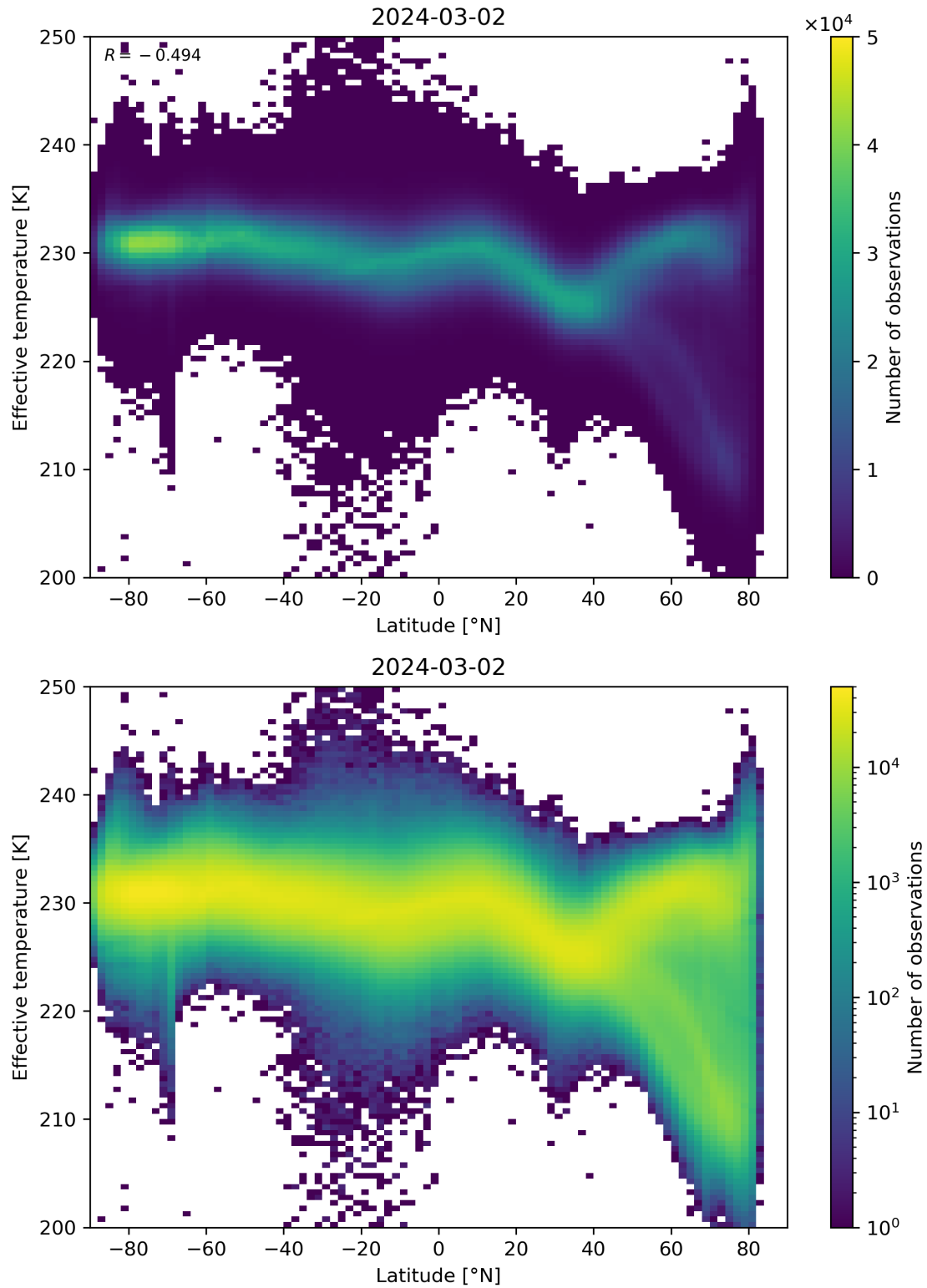
Figure 34: Scatter density plot of “Latitude” against “Effective temperature” for 2024-03-01 to 2024-03-03.
