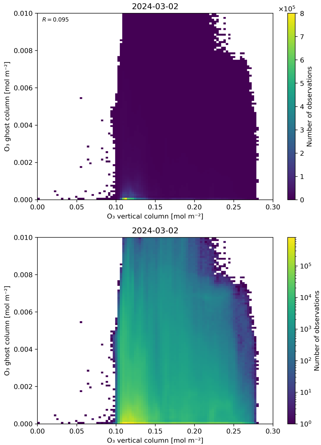
Figure 40: Scatter density plot of “O 3 vertical column” against “O 3 ghost column” for 2024-03-01 to 2024-03-03.
