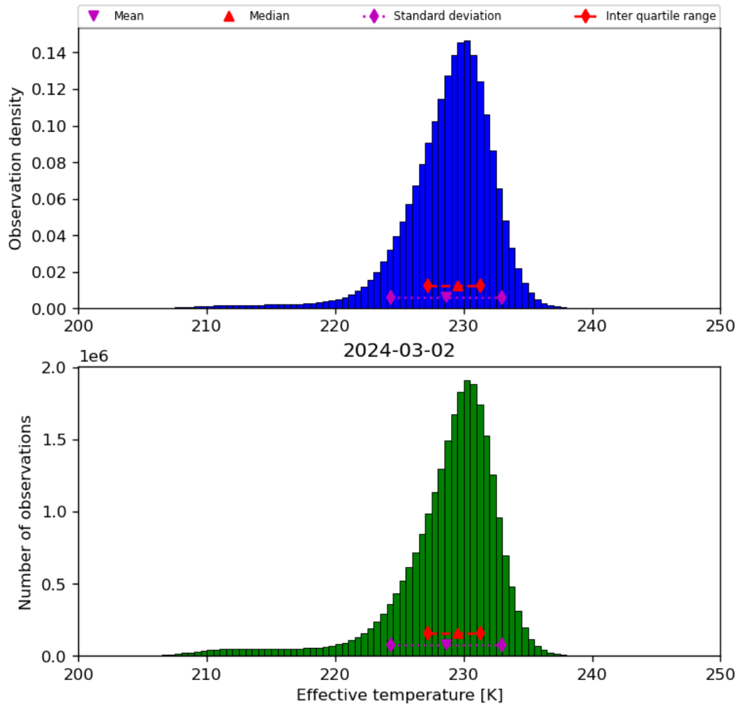
Figure 24: Histogram of “Effective temperature” for 2024-03-01 to 2024-03-03
