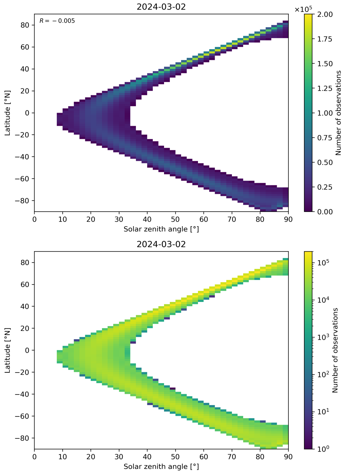
Figure 44: Scatter density plot of “Solar zenith angle” against “Latitude” for 2024-03-01 to 2024-03-03.
