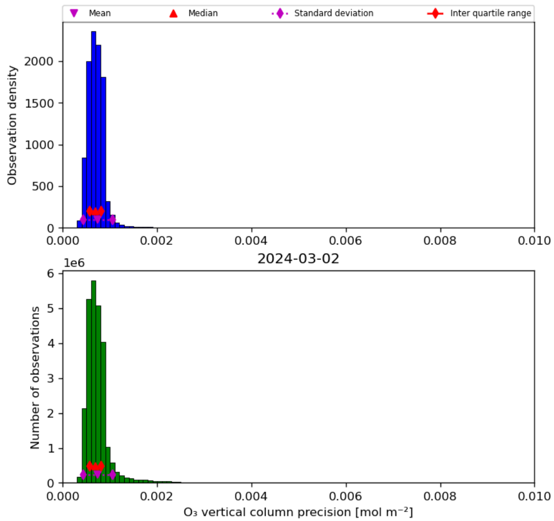
Figure 22: Histogram of “O 3 vertical column precision” for 2024-03-01 to 2024-03-03
