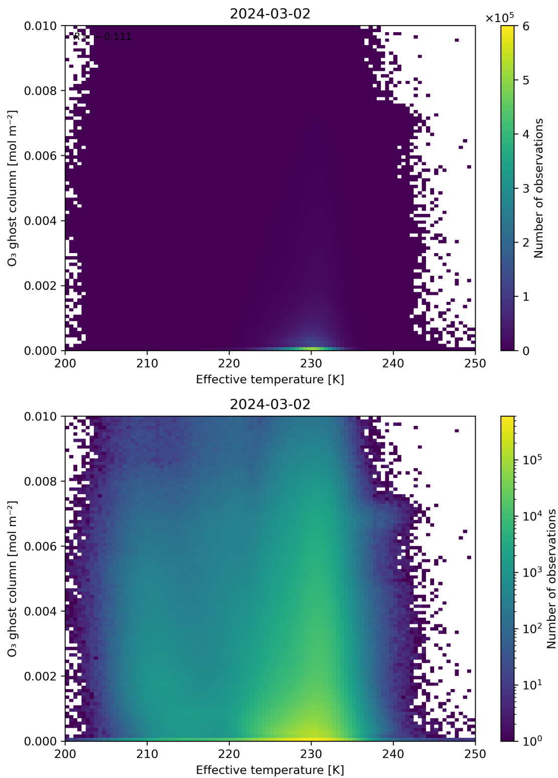
Figure 38: Scatter density plot of “Effective temperature” against “O 3 ghost column” for 2024-03-01 to 2024-03-03.
