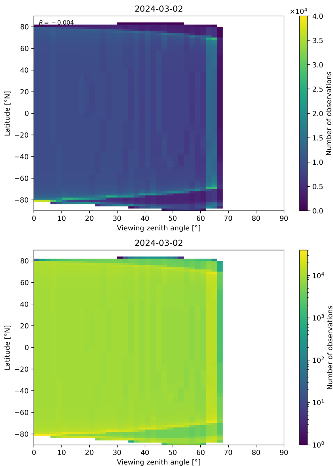
Figure 49: Scatter density plot of “Viewing zenith angle” against “Latitude” for 2024-03-01 to 2024-03-03.
