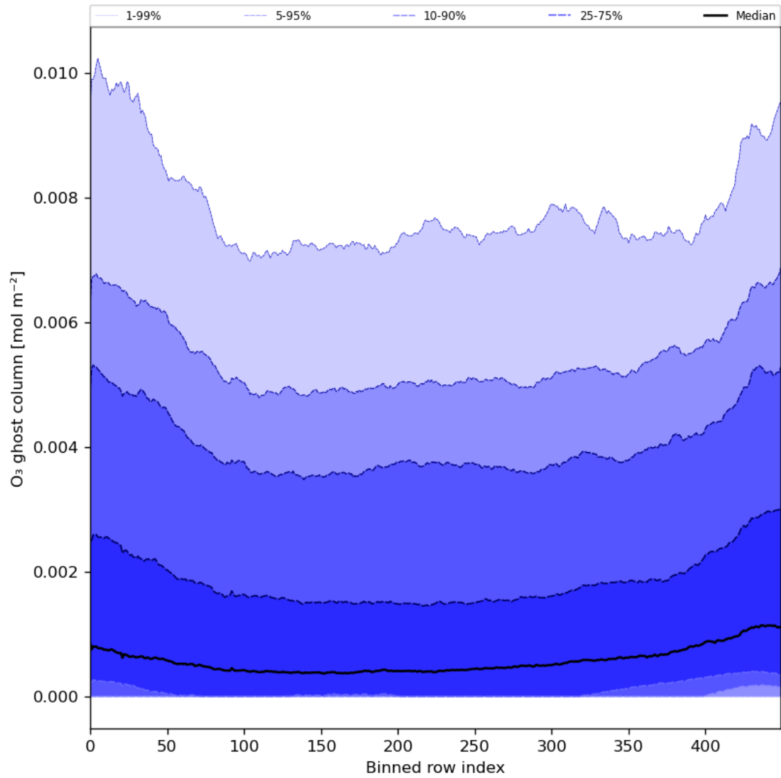
Figure 32: Along track statistics of “O 3 ghost column” for 2024-03-01 to 2024-03-03
