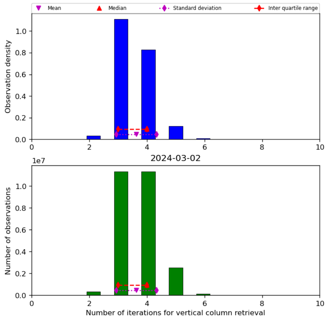
Figure 26: Histogram of “Number of iterations for vertical column retrieval” for 2024-03-01 to 2024-03-03
