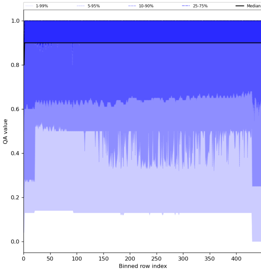
Figure 27: Along track statistics of “QA value” for 2024-03-01 to 2024-03-03
