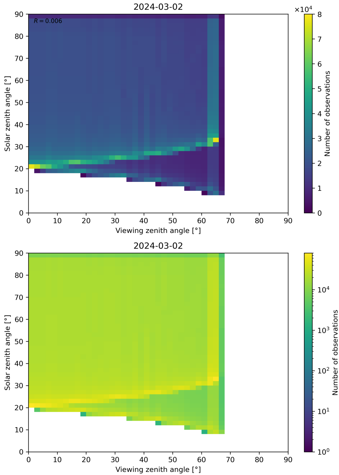
Figure 54: Scatter density plot of “Viewing zenith angle” against “Solar zenith angle” for 2024-03-01 to 2024-03-03.
