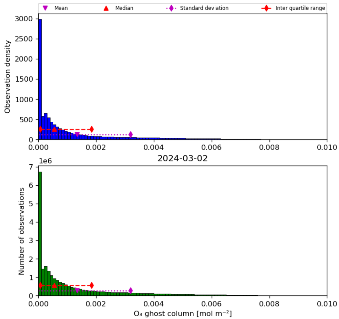
Figure 25: Histogram of “O 3 ghost column” for 2024-03-01 to 2024-03-03
