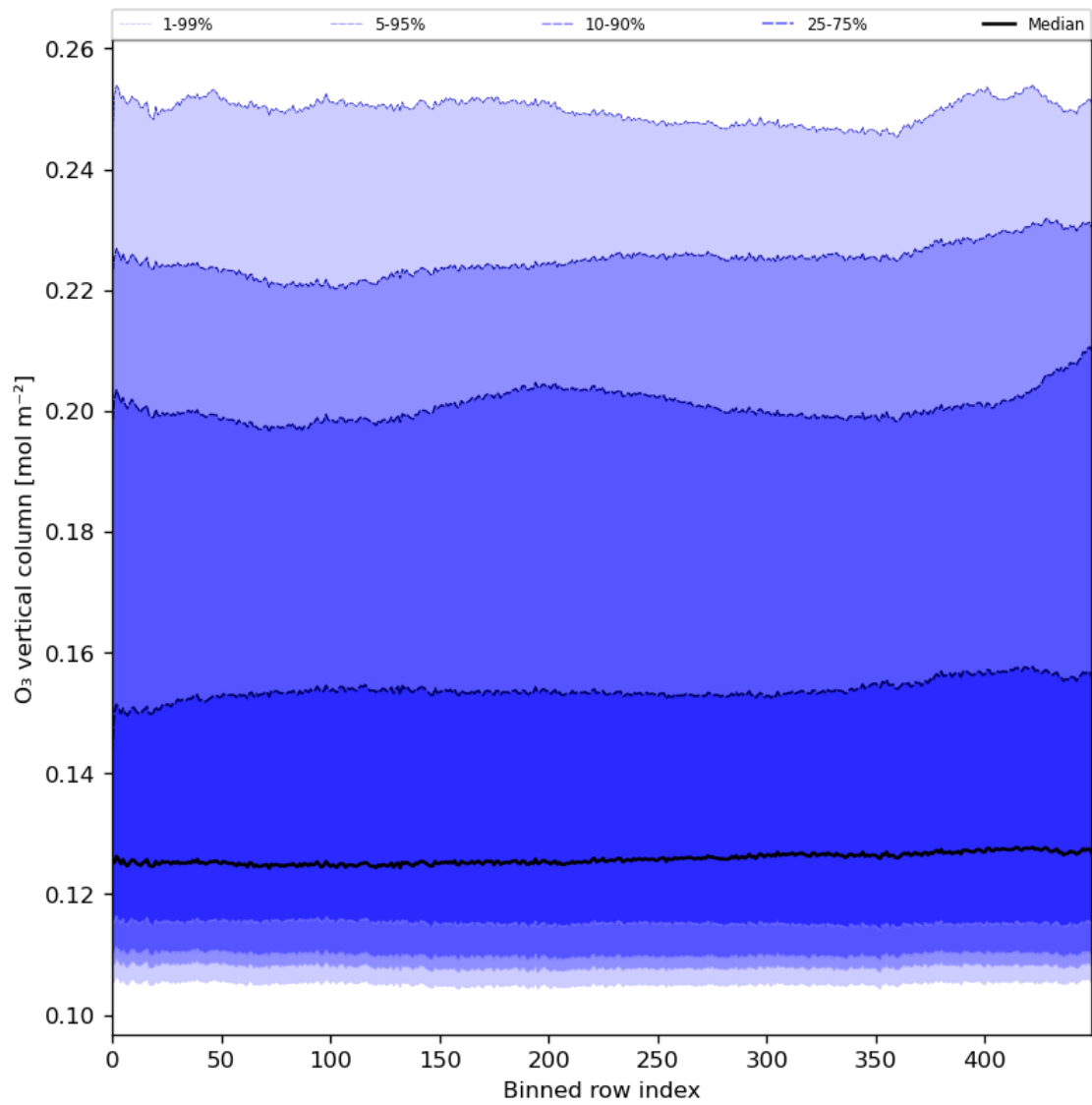
Figure 28: Along track statistics of “O 3 vertical column” for 2024-03-01 to 2024-03-03
