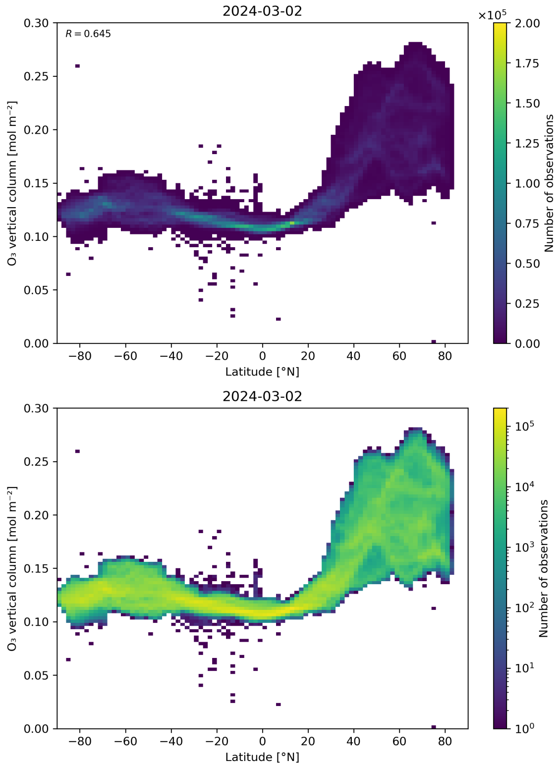
Figure 36: Scatter density plot of “Latitude” against “O 3 vertical column” for 2024-03-01 to 2024-03-03.
