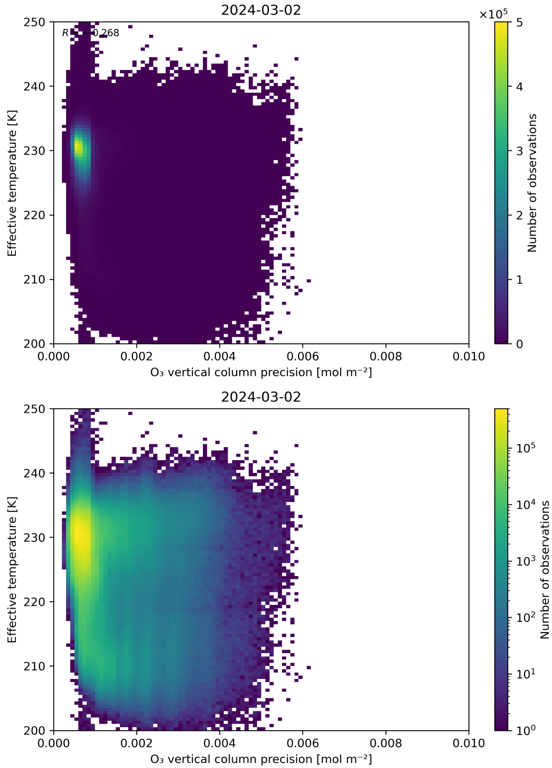
Figure 42: Scatter density plot of “O 3 vertical column precision” against “Effective temperature” for 2024-03-01 to 2024-03-03.
