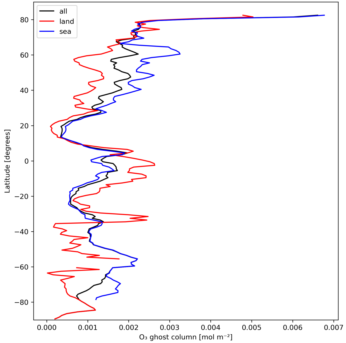
Figure 18: Zonal average of "O 3 ghost column" for 2024-03-01 to 2024-03-03.
