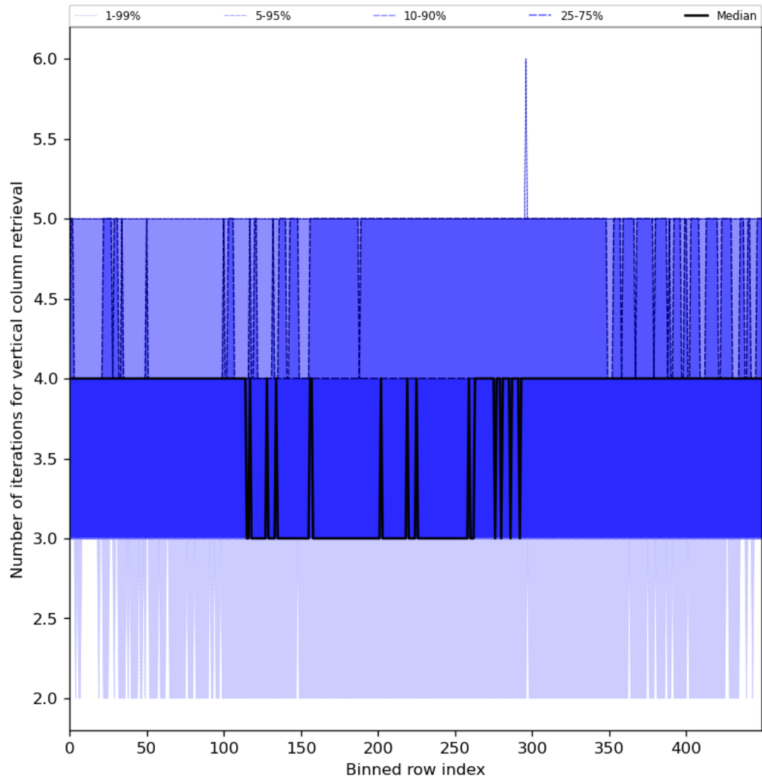
Figure 33: Along track statistics of “Number of iterations for vertical column retrieval” for 2024-03-01 to 2024-03-03
