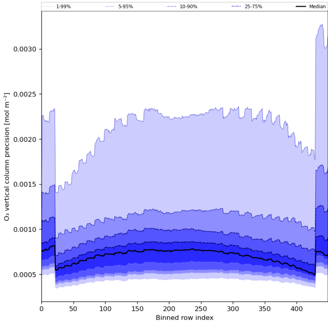
Figure 29: Along track statistics of “O 3 vertical column precision” for 2024-03-01 to 2024-03-03
