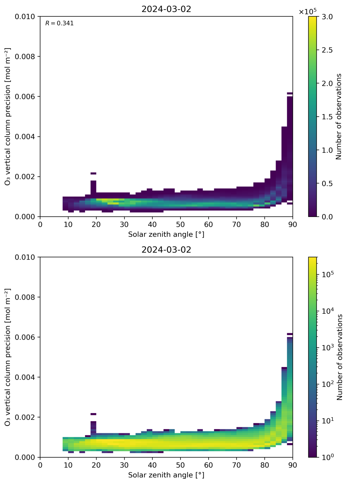
Figure 48: Scatter density plot of “Solar zenith angle” against “O 3 vertical column precision” for 2024-03-01 to 2024-03-03.
