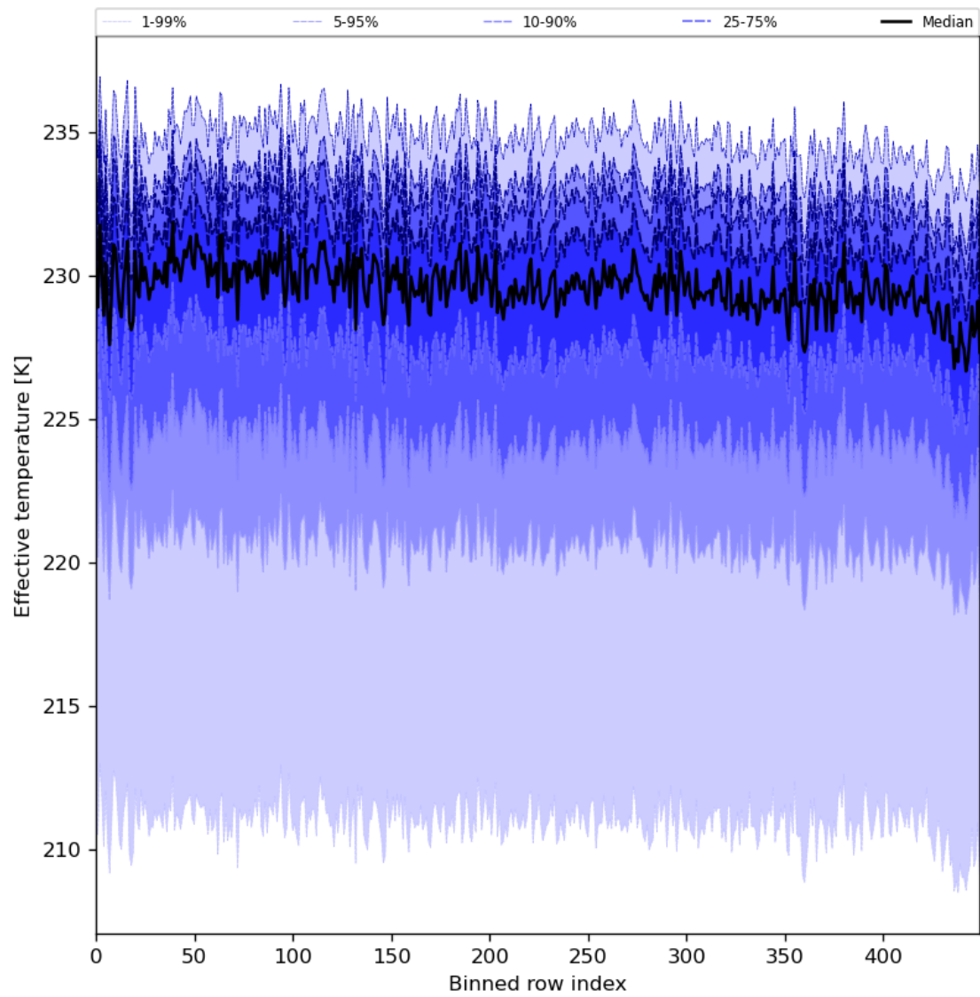
Figure 31: Along track statistics of “Effective temperature” for 2024-03-01 to 2024-03-03
