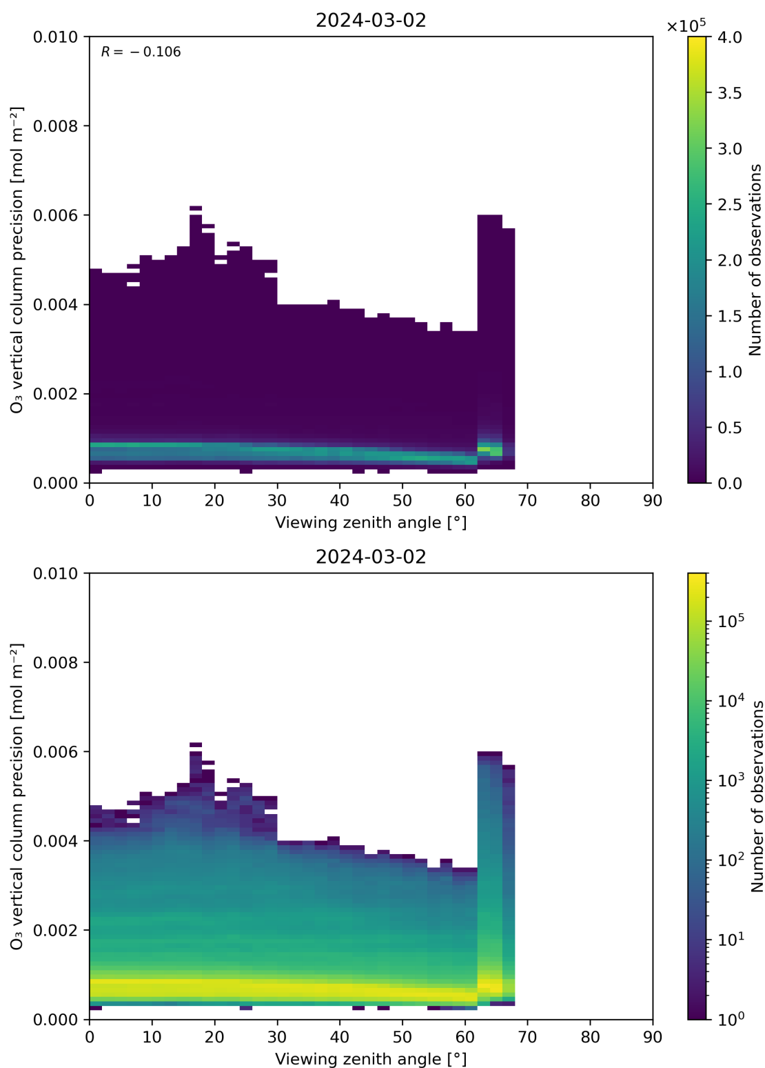
Figure 53: Scatter density plot of “Viewing zenith angle” against “O 3 vertical column precision” for 2024-03-01 to 2024-03-03.
