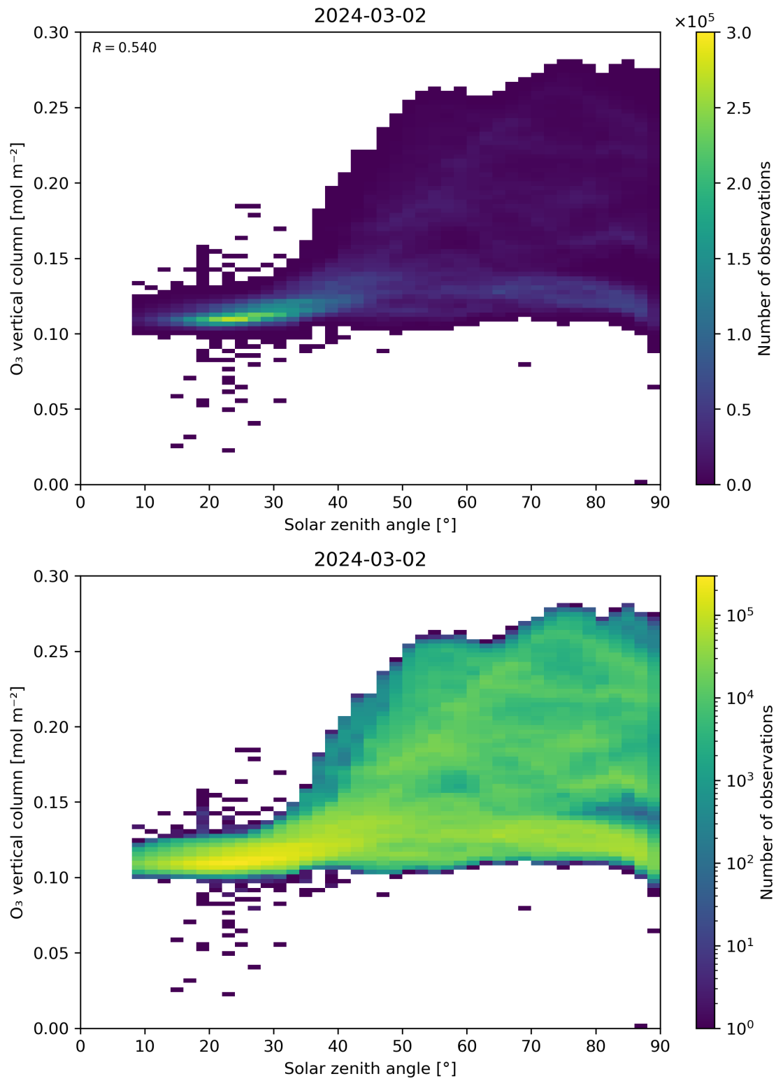
Figure 47: Scatter density plot of “Solar zenith angle” against “O 3 vertical column” for 2024-03-01 to 2024-03-03.
