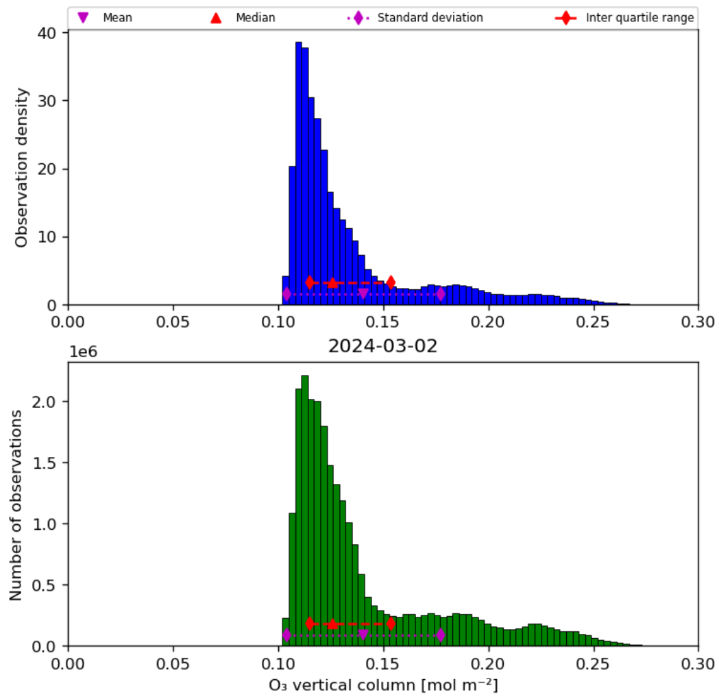
Figure 21: Histogram of “O 3 vertical column” for 2024-03-01 to 2024-03-03
