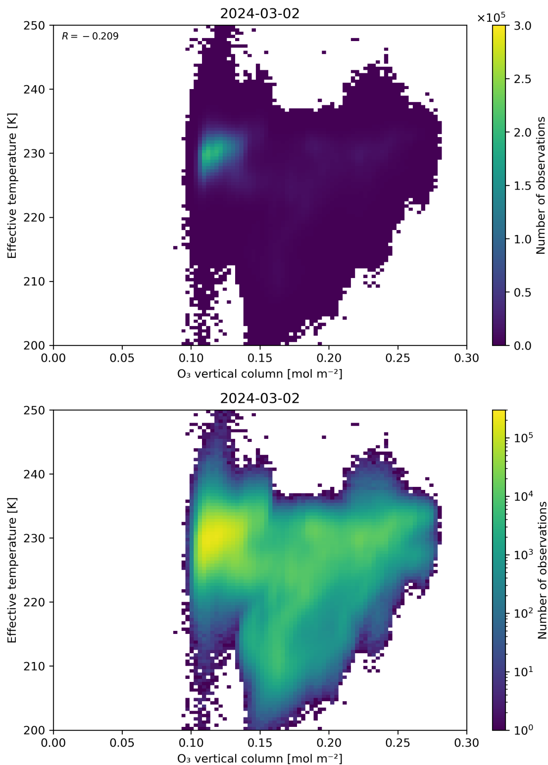
Figure 39: Scatter density plot of “O 3 vertical column” against “Effective temperature” for 2024-03-01 to 2024-03-03.
