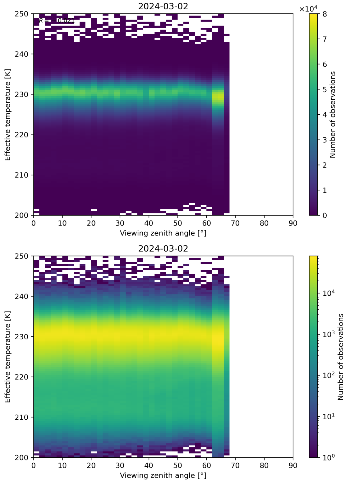
Figure 50: Scatter density plot of “Viewing zenith angle” against “Effective temperature” for 2024-03-01 to 2024-03-03.
