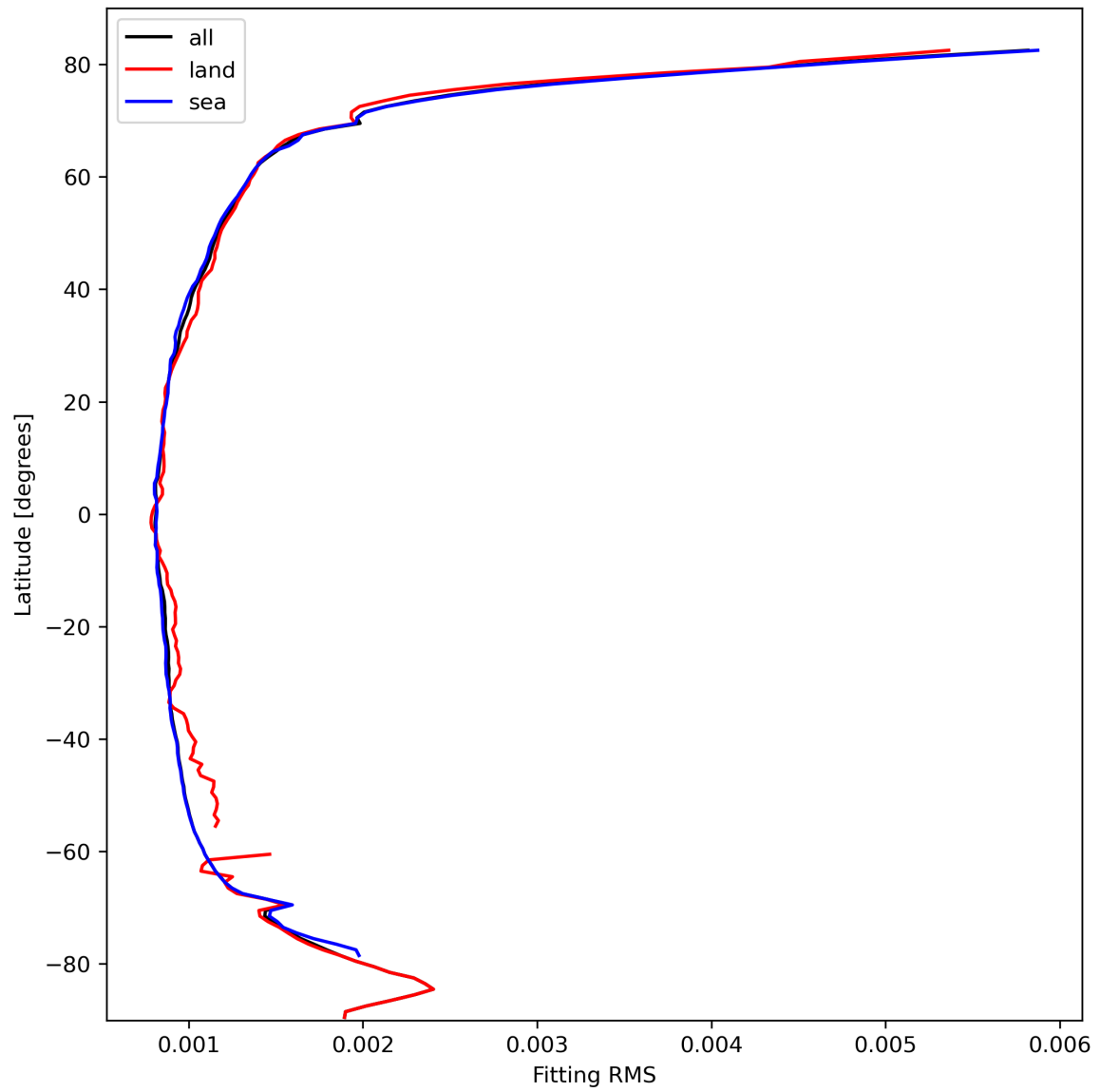
Figure 16: Zonal average of “Fitting RMS” for 2024-03-01 to 2024-03-03.
