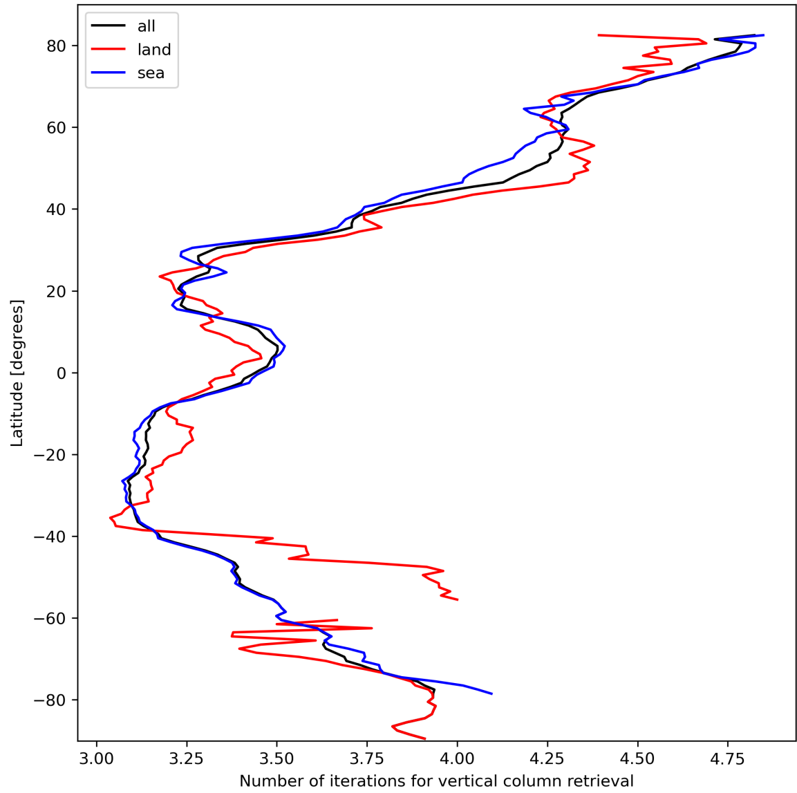
Figure 19: Zonal average of “Number of iterations for vertical column retrieval” for 2024-03-01 to 2024-03-03.
