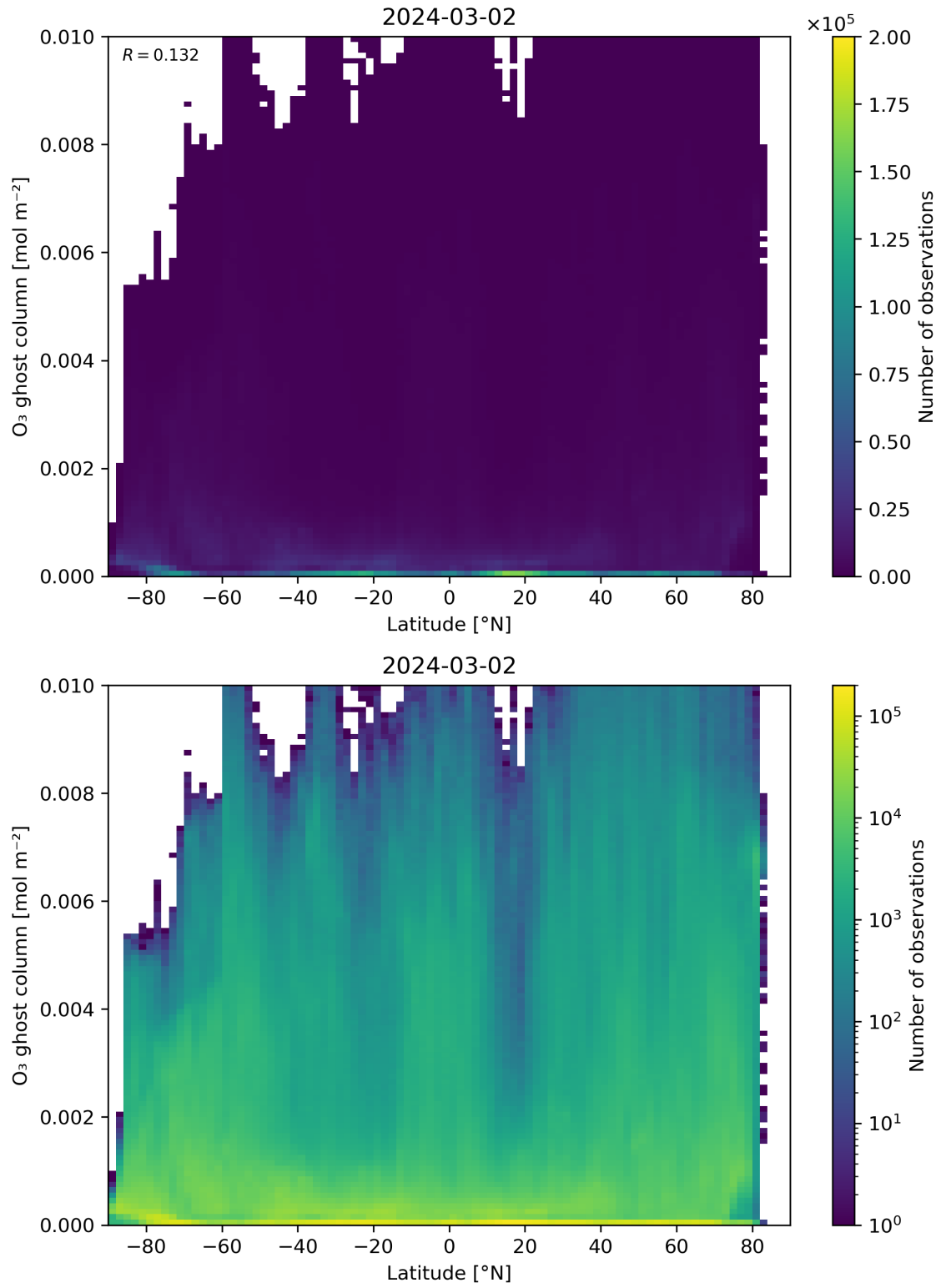
Figure 35: Scatter density plot of “Latitude” against “O 3 ghost column” for 2024-03-01 to 2024-03-03.
