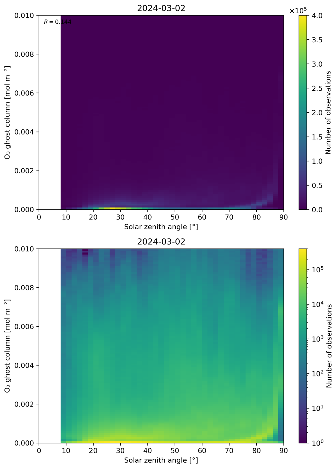
Figure 46: Scatter density plot of “Solar zenith angle” against “O 3 ghost column” for 2024-03-01 to 2024-03-03.
