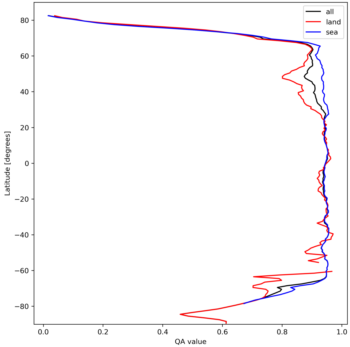
Figure 13: Zonal average of “QA value” for 2024-03-01 to 2024-03-03.
