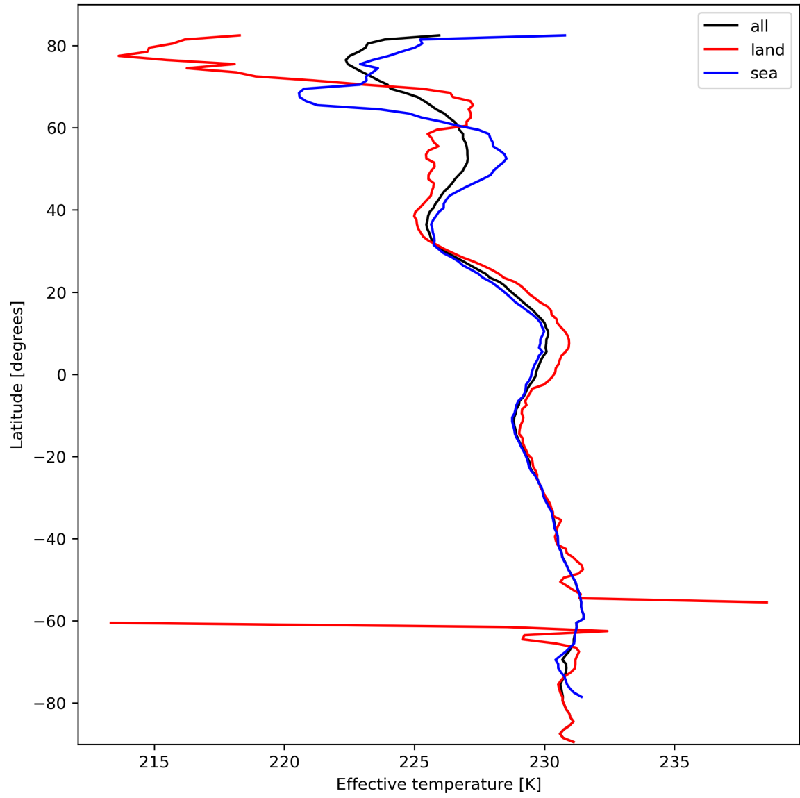
Figure 17: Zonal average of “Effective temperature” for 2024-03-01 to 2024-03-03.
