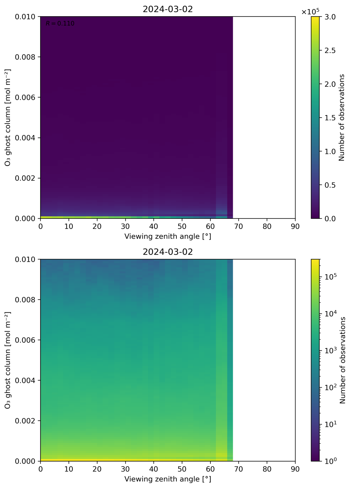
Figure 51: Scatter density plot of “Viewing zenith angle” against “O 3 ghost column” for 2024-03-01 to 2024-03-03.
