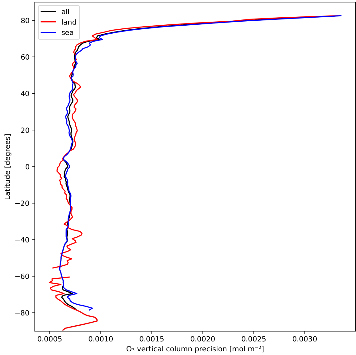
Figure 15: Zonal average of “O 3 vertical column precision” for 2024-03-01 to 2024-03-03.
