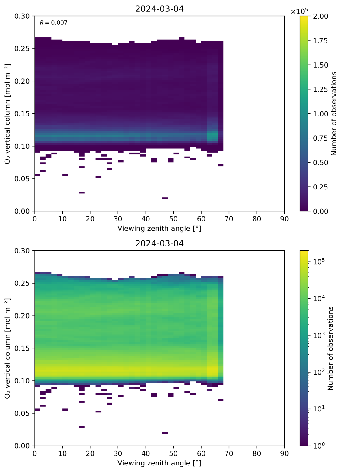
Figure 52: Scatter density plot of “Viewing zenith angle” against “O 3 vertical column” for 2024-03-04 to 2024-03-05.
