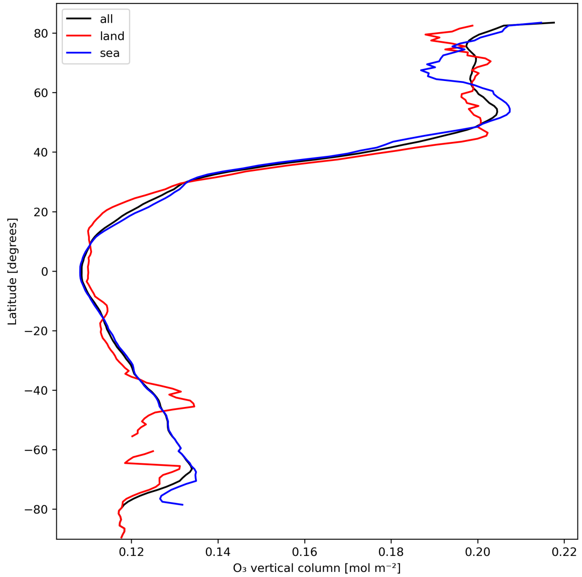
Figure 14: Zonal average of “O 3 vertical column” for 2024-03-04 to 2024-03-05.
