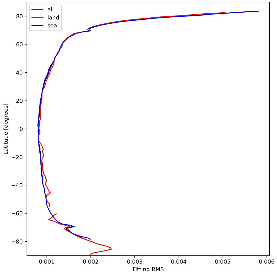
Figure 16: Zonal average of “Fitting RMS” for 2024-03-04 to 2024-03-05.
