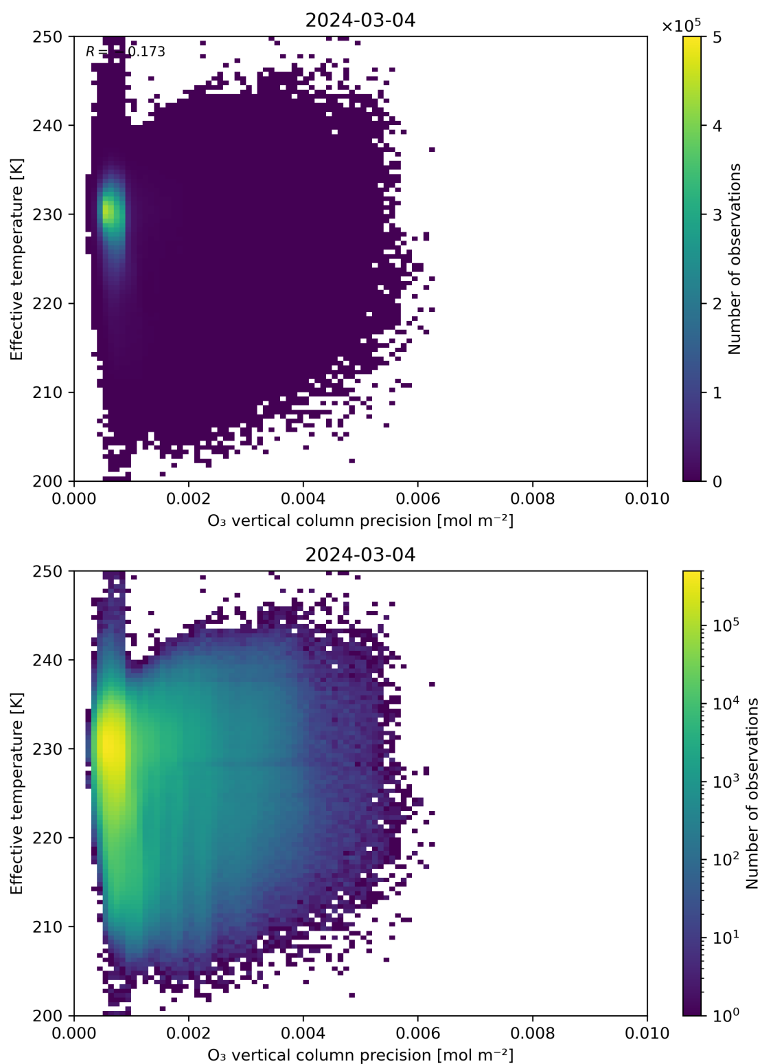
Figure 42: Scatter density plot of “O 3 vertical column precision” against “Effective temperature” for 2024-03-04 to 2024-03-05.
