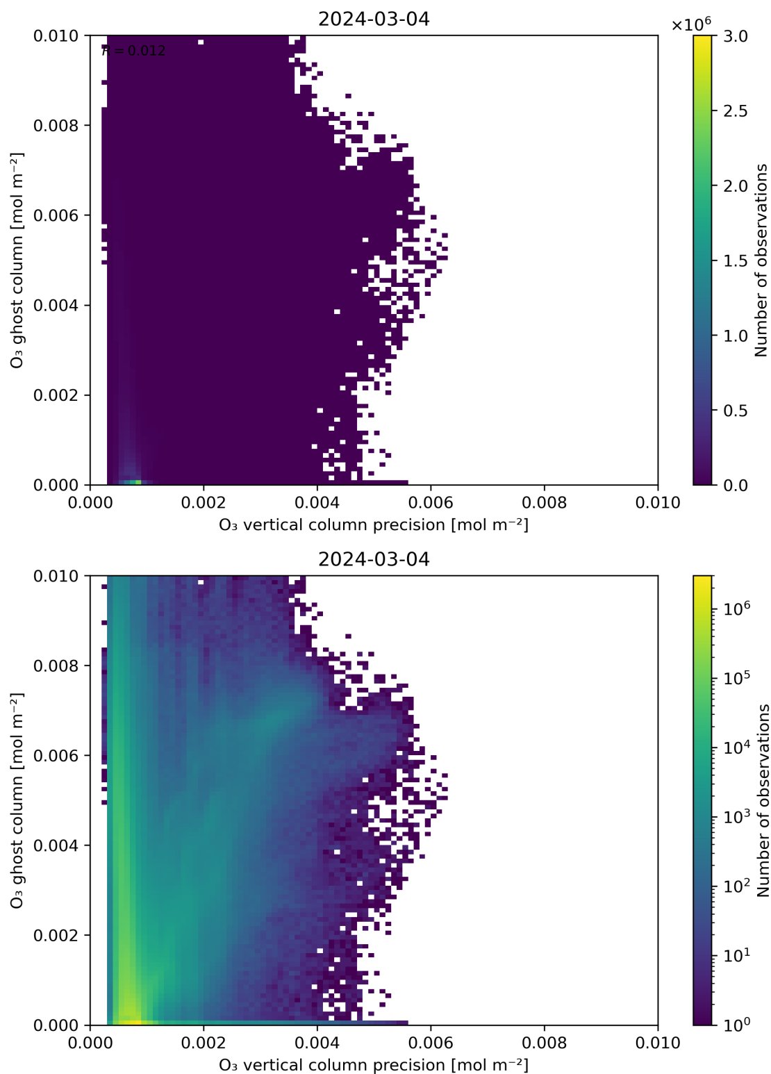
Figure 43: Scatter density plot of “O 3 vertical column precision” against “O 3 ghost column” for 2024-03-04 to 2024-03-05.
