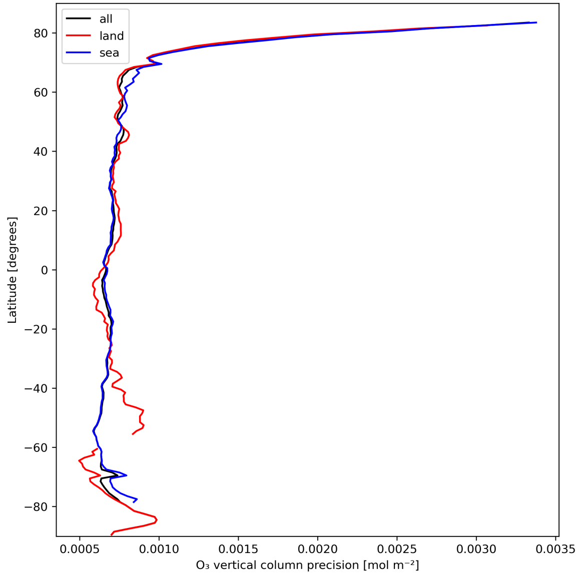
Figure 15: Zonal average of “O 3 vertical column precision” for 2024-03-04 to 2024-03-05.
