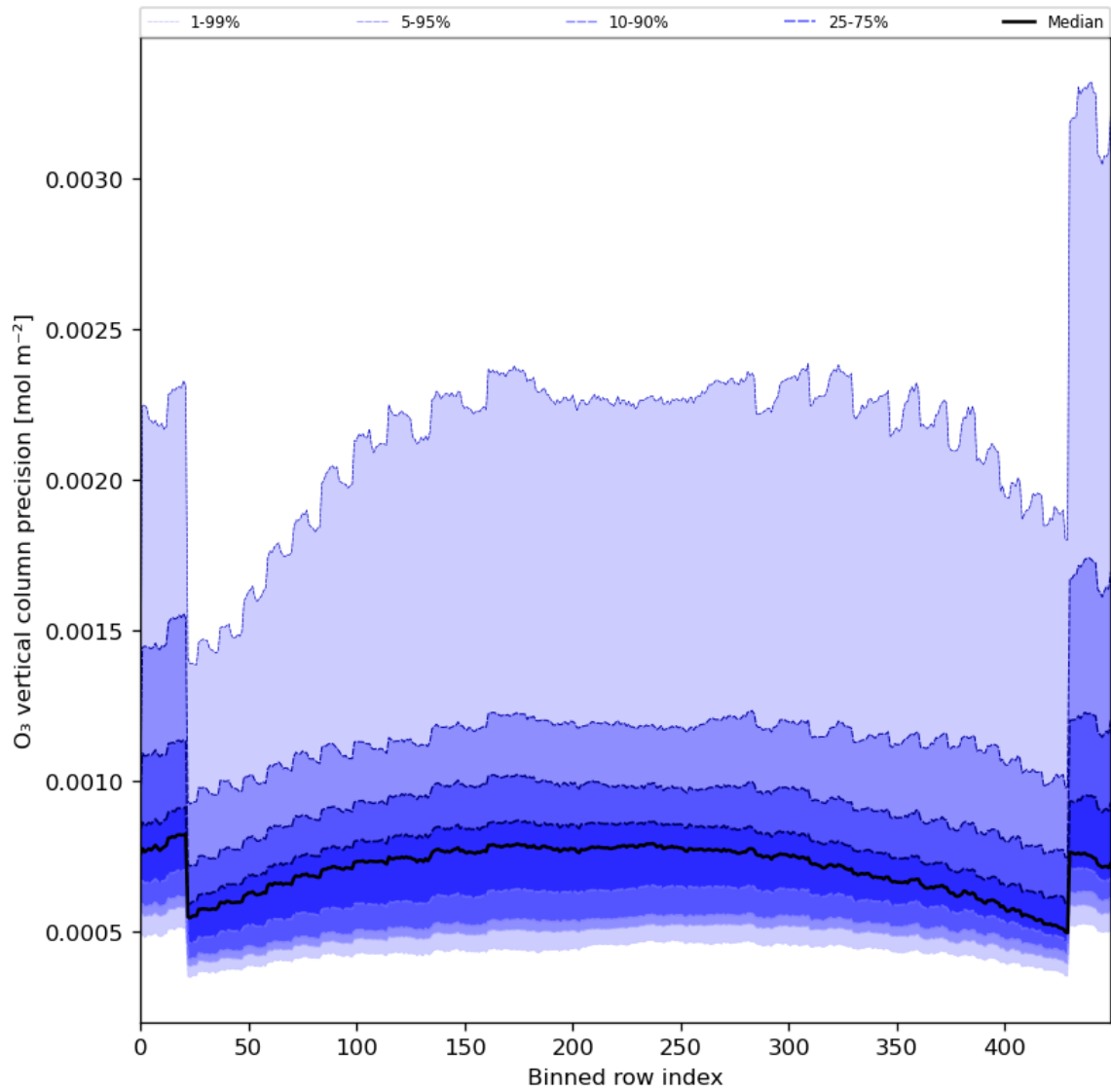
Figure 29: Along track statistics of “O 3 vertical column precision” for 2024-03-04 to 2024-03-05
