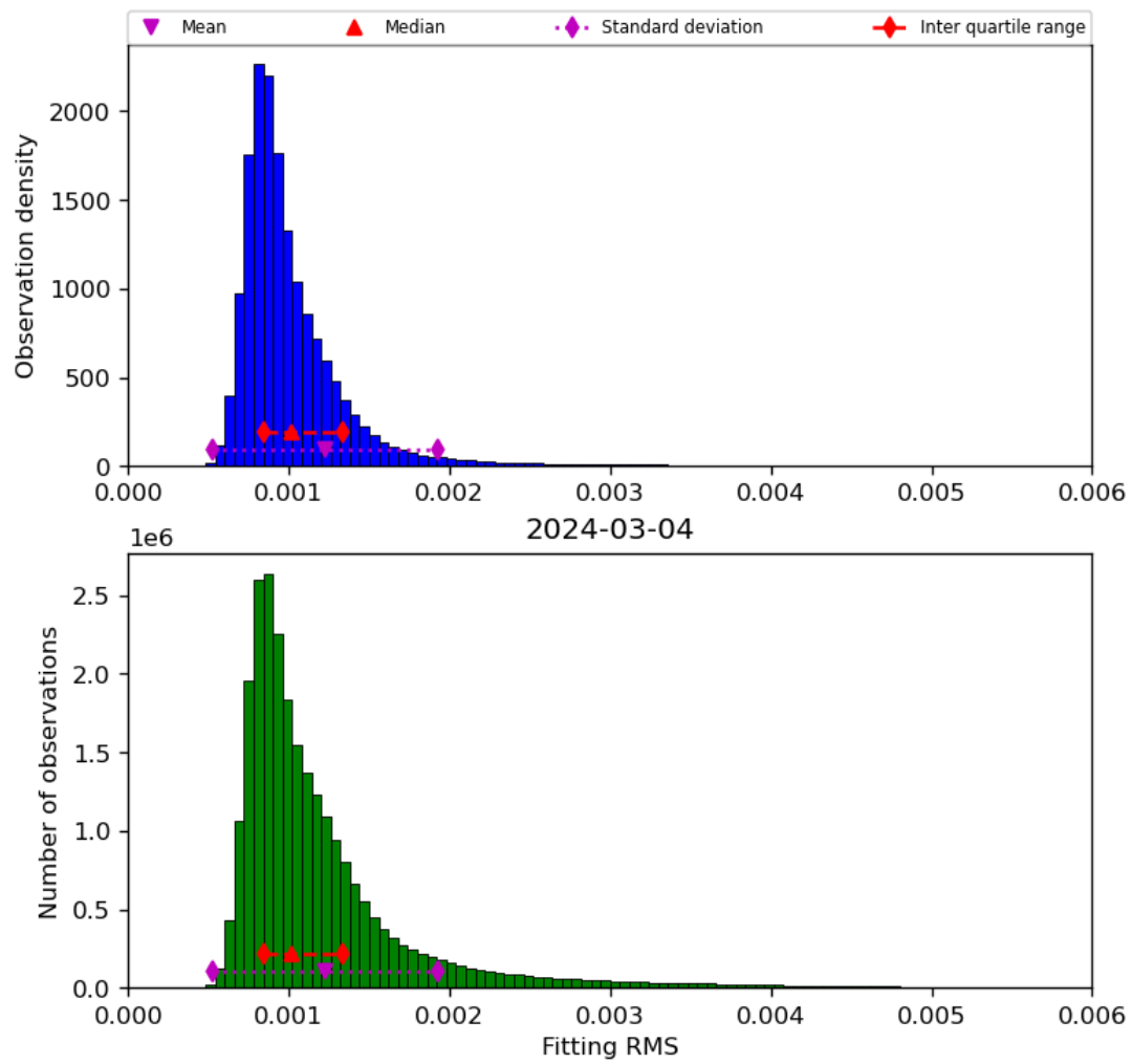
Figure 23: Histogram of “Fitting RMS” for 2024-03-04 to 2024-03-05
