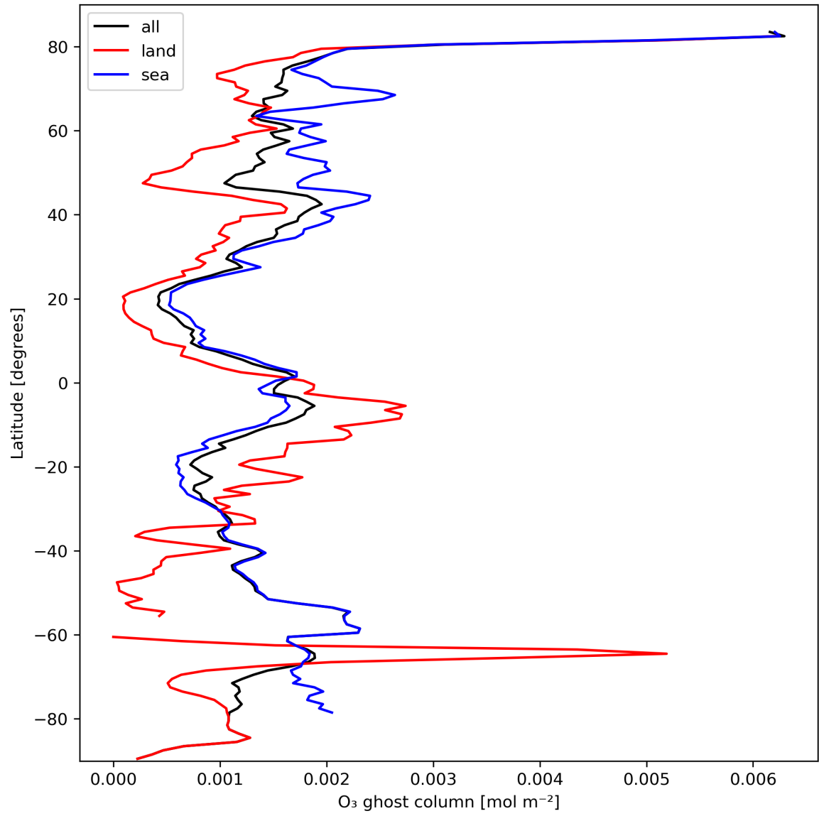
Figure 18: Zonal average of "O 3 ghost column" for 2024-03-04 to 2024-03-05.
