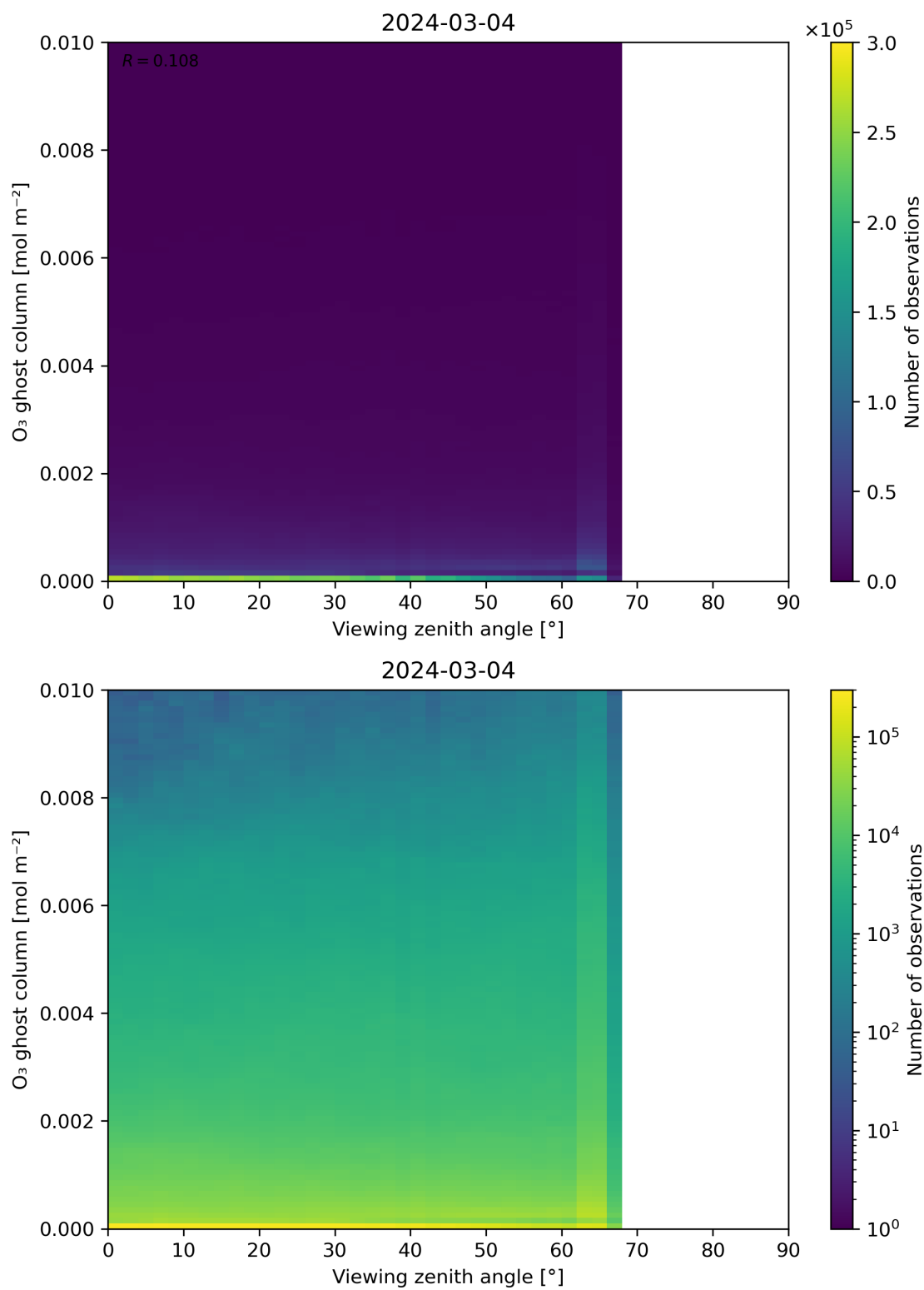
Figure 51: Scatter density plot of “Viewing zenith angle” against “O 3 ghost column” for 2024-03-04 to 2024-03-05.
