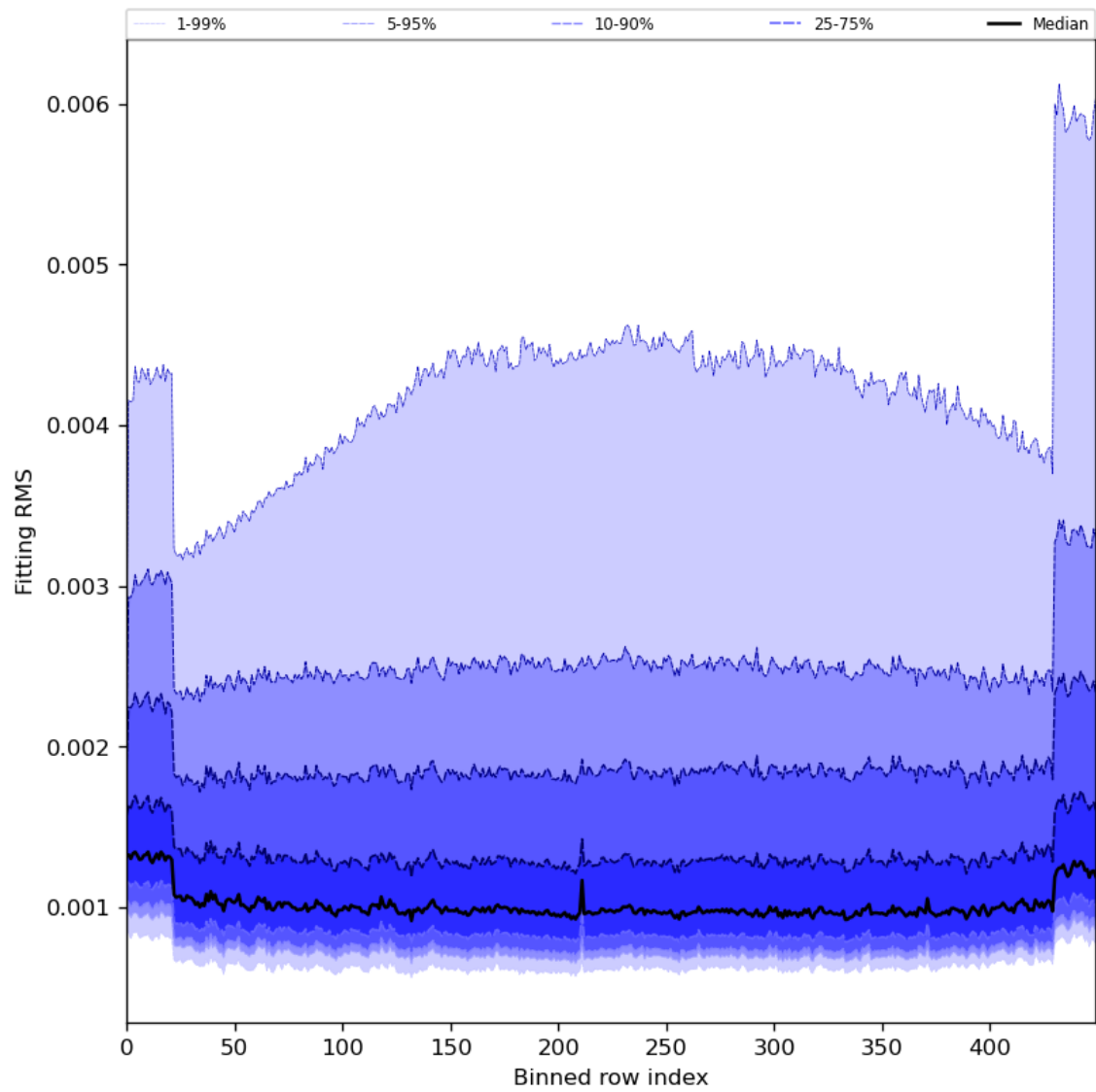
Figure 30: Along track statistics of “Fitting RMS” for 2024-03-04 to 2024-03-05
