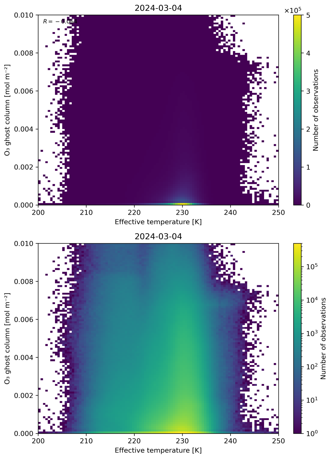
Figure 38: Scatter density plot of “Effective temperature” against “O 3 ghost column” for 2024-03-04 to 2024-03-05.
