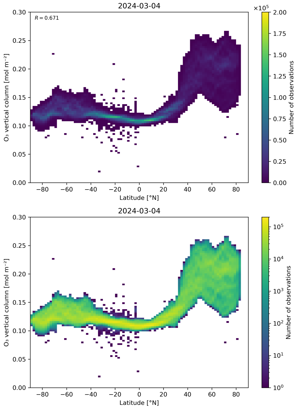
Figure 36: Scatter density plot of “Latitude” against “O 3 vertical column” for 2024-03-04 to 2024-03-05.
