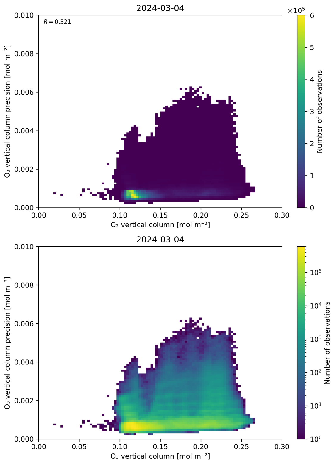
Figure 41: Scatter density plot of “O 3 vertical column” against “O 3 vertical column precision” for 2024-03-04 to 2024-03-05.
