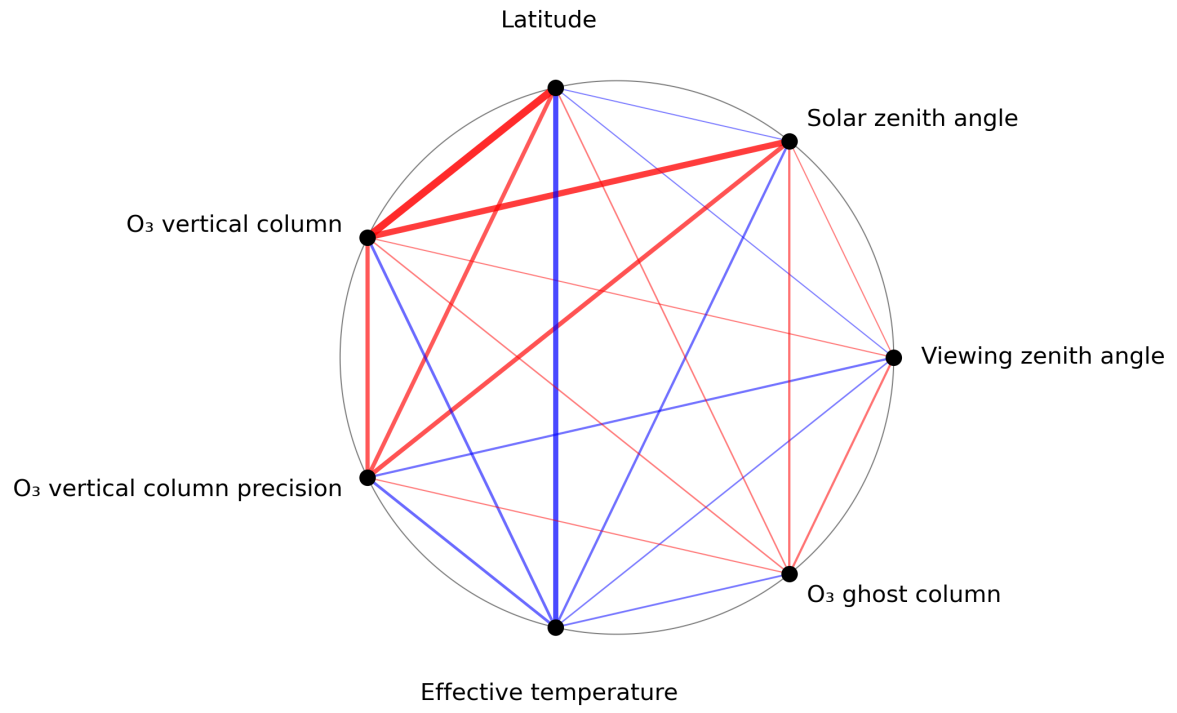
Figure 1: Map of correlation graph for 2024-03-04 to 2024-03-05.
