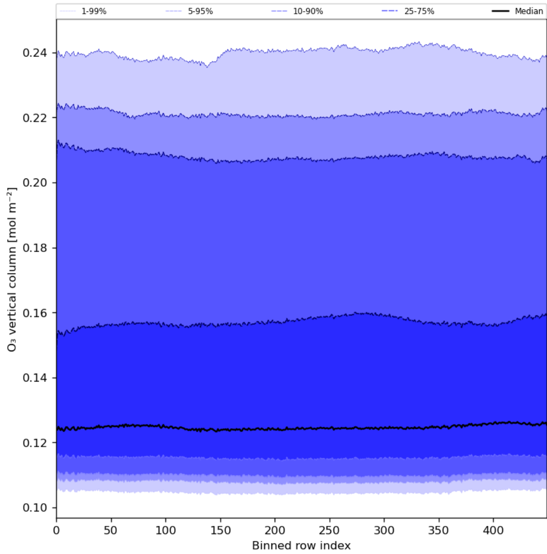
Figure 28: Along track statistics of “O 3 vertical column” for 2024-03-04 to 2024-03-05
