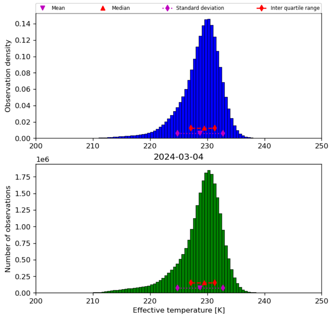
Figure 24: Histogram of “Effective temperature” for 2024-03-04 to 2024-03-05
