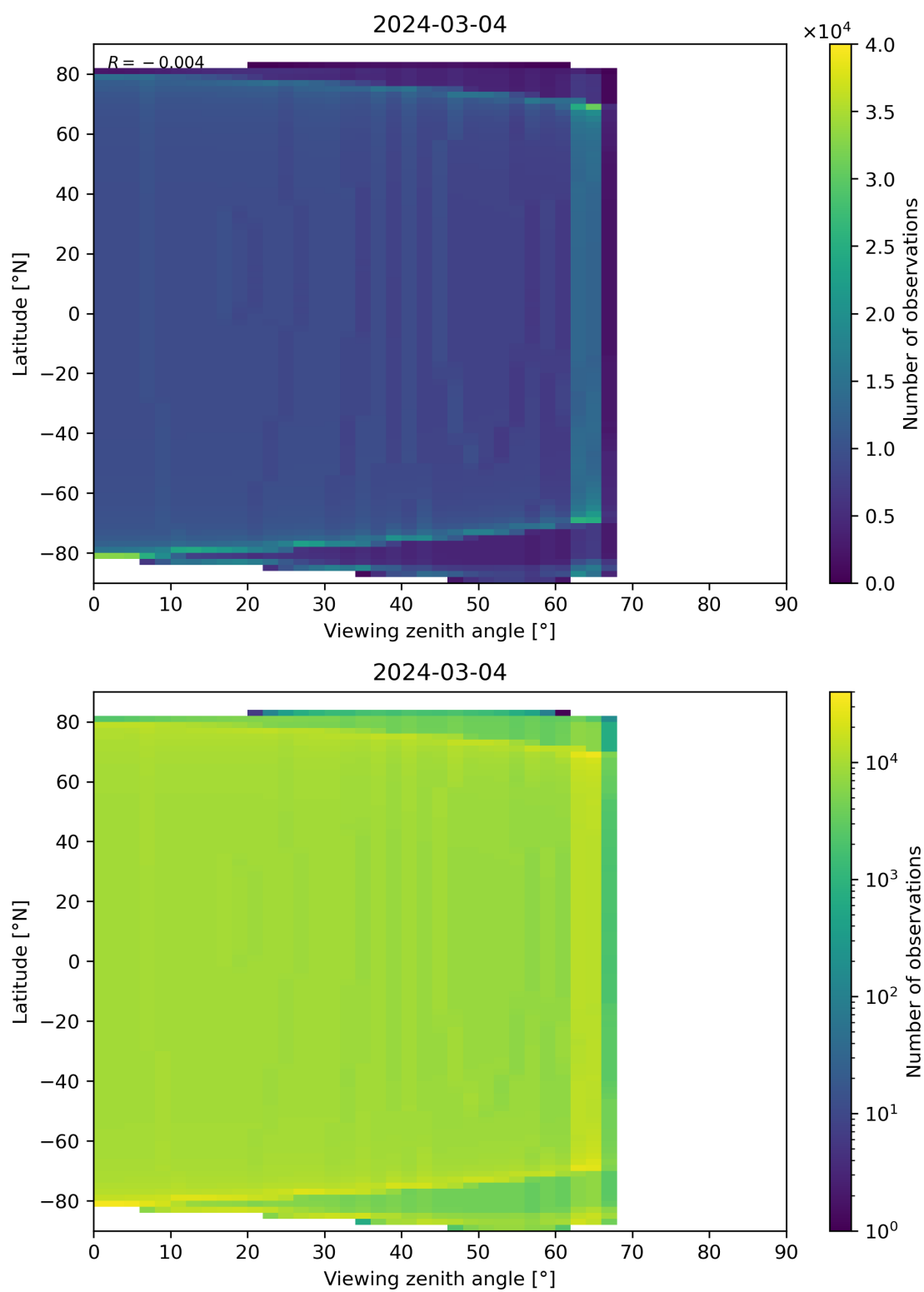
Figure 49: Scatter density plot of “Viewing zenith angle” against “Latitude” for 2024-03-04 to 2024-03-05.
