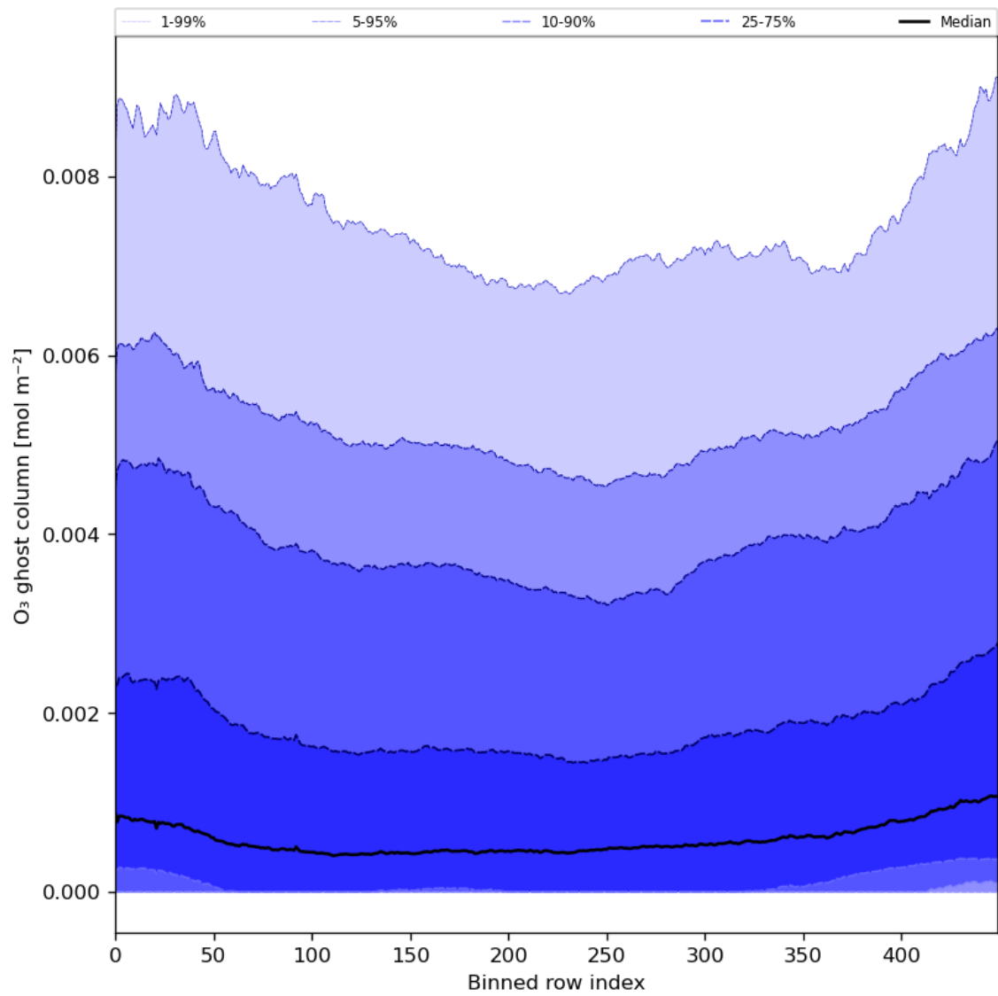
Figure 32: Along track statistics of “O 3 ghost column” for 2024-03-04 to 2024-03-05
