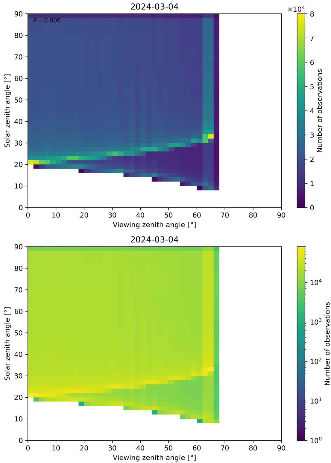
Figure 54: Scatter density plot of “Viewing zenith angle” against “Solar zenith angle” for 2024-03-04 to 2024-03-05.
