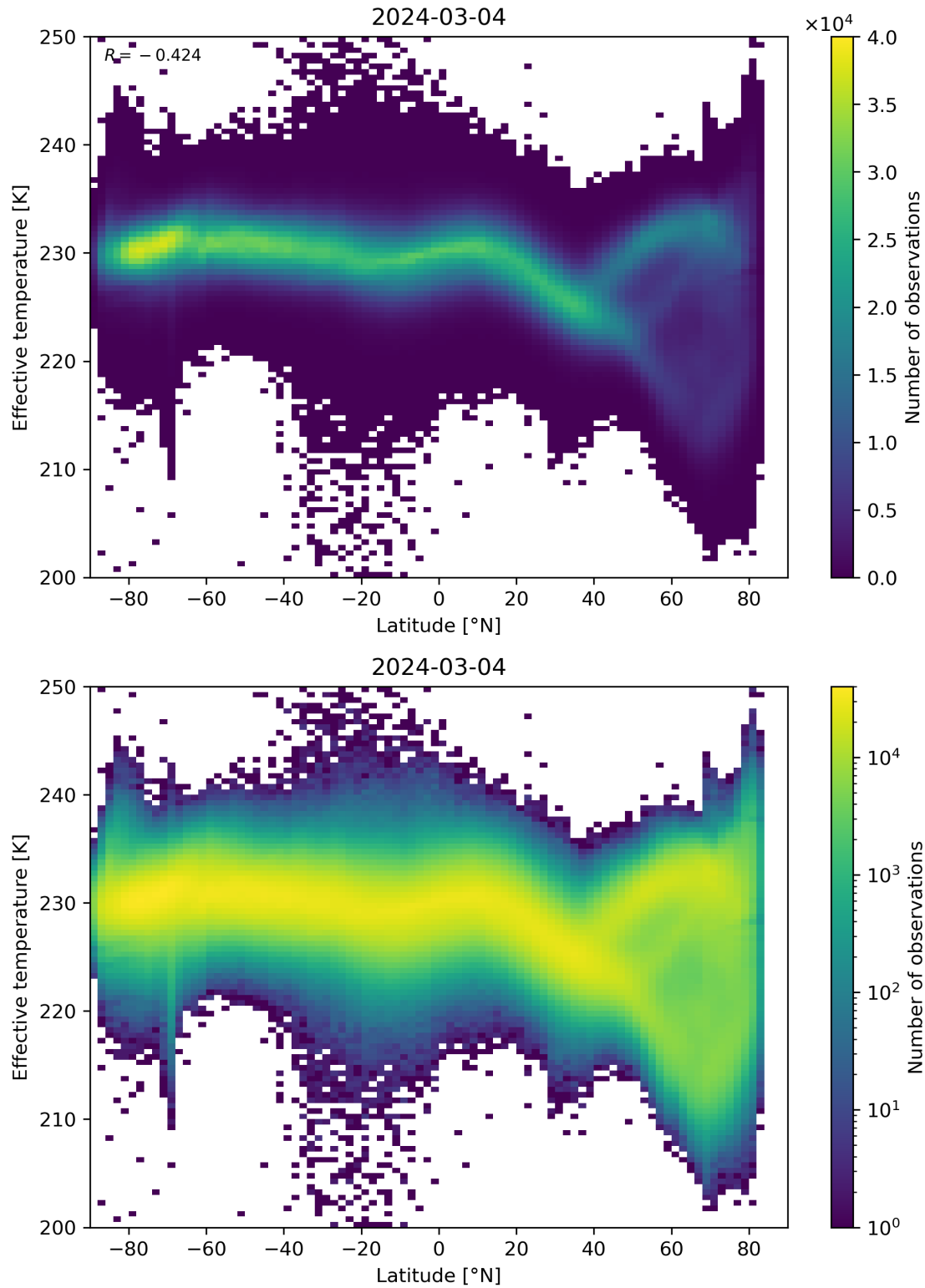
Figure 34: Scatter density plot of “Latitude” against “Effective temperature” for 2024-03-04 to 2024-03-05.
