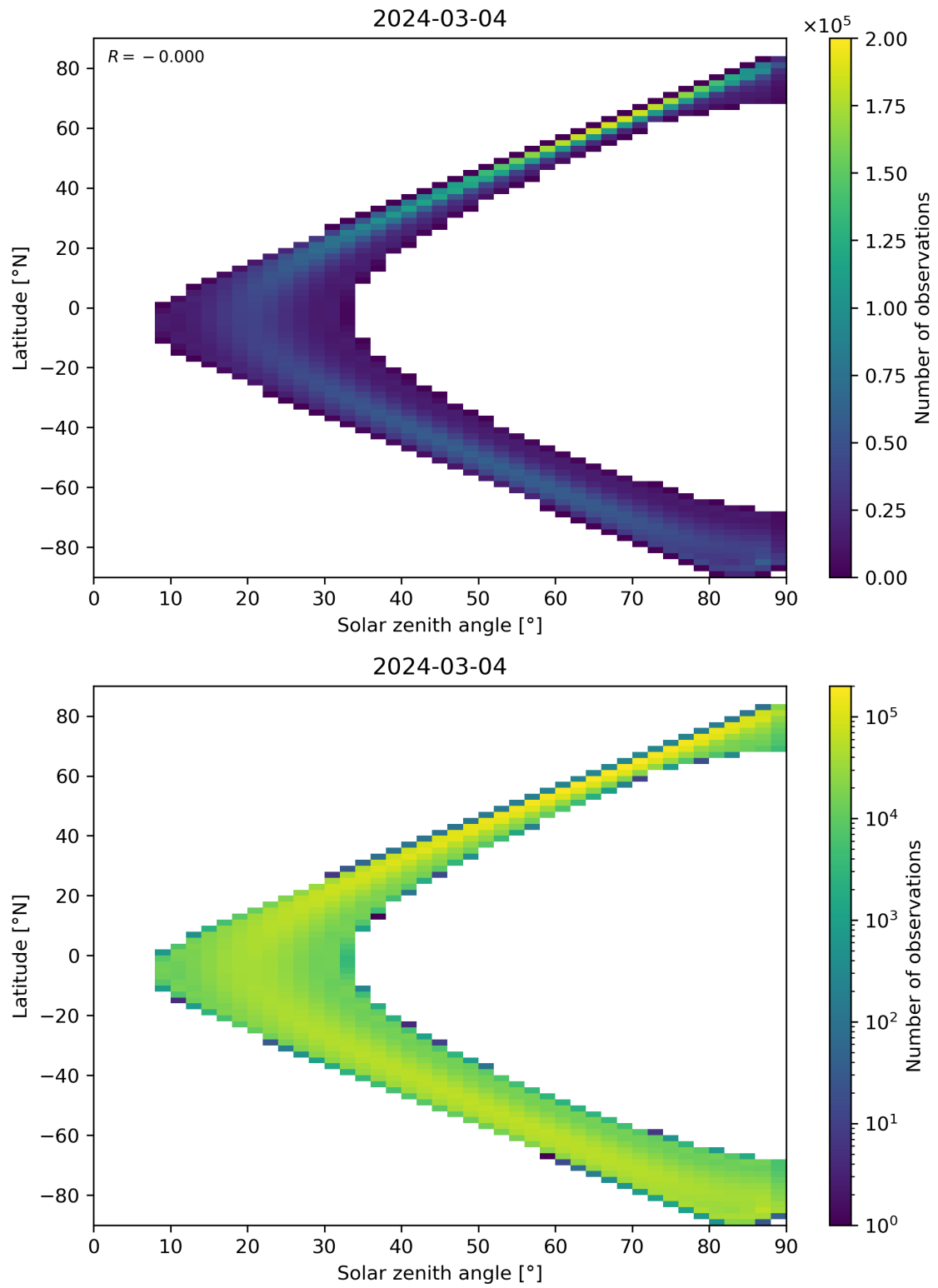
Figure 44: Scatter density plot of “Solar zenith angle” against “Latitude” for 2024-03-04 to 2024-03-05.
