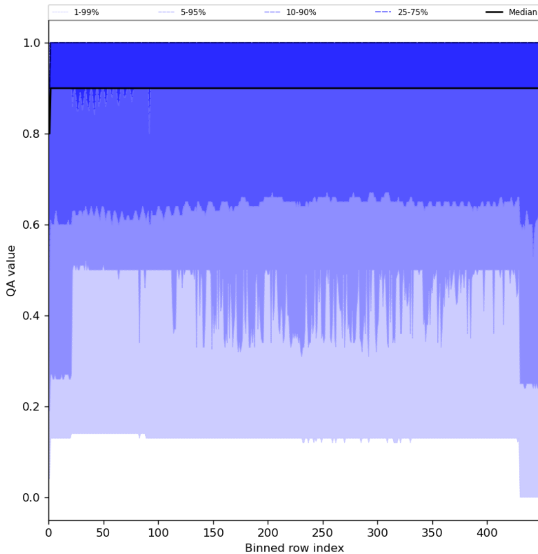
Figure 27: Along track statistics of “QA value” for 2024-03-04 to 2024-03-05
