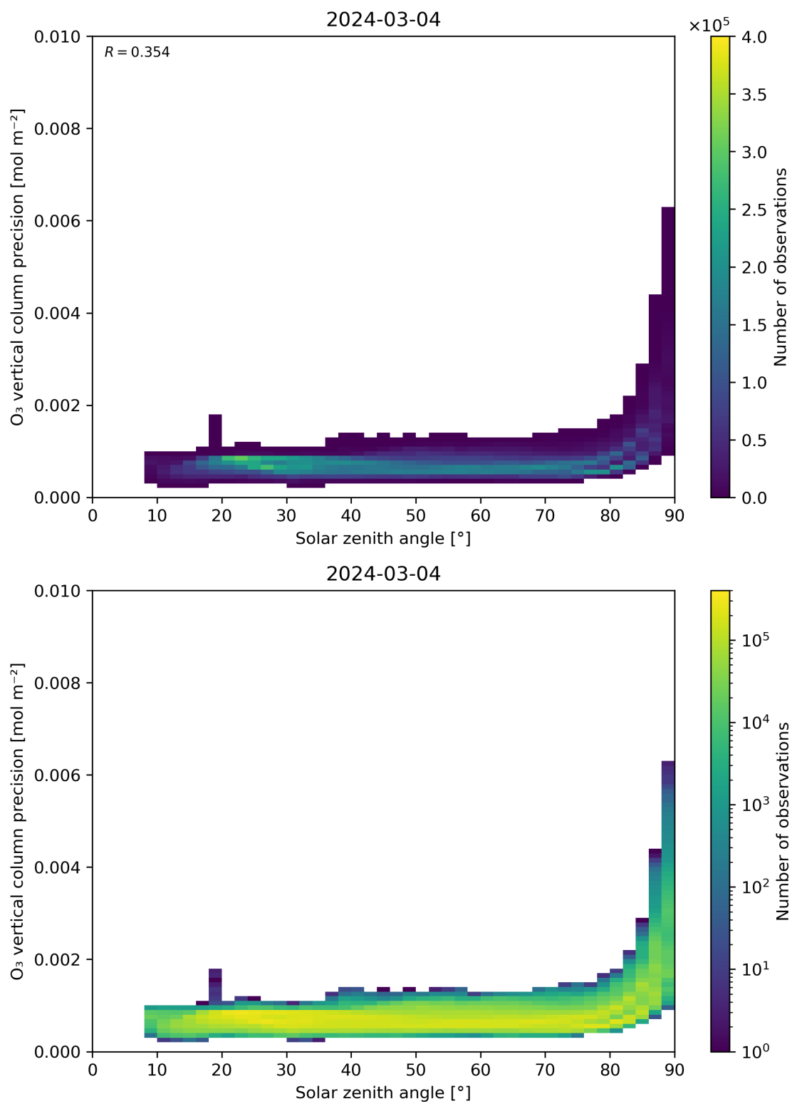
Figure 48: Scatter density plot of “Solar zenith angle” against “O 3 vertical column precision” for 2024-03-04 to 2024-03-05.
