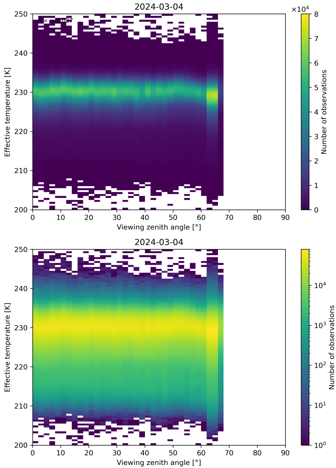
Figure 50: Scatter density plot of “Viewing zenith angle” against “Effective temperature” for 2024-03-04 to 2024-03-05.
