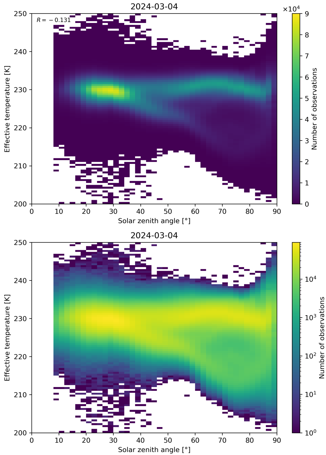
Figure 45: Scatter density plot of “Solar zenith angle” against “Effective temperature” for 2024-03-04 to 2024-03-05.
