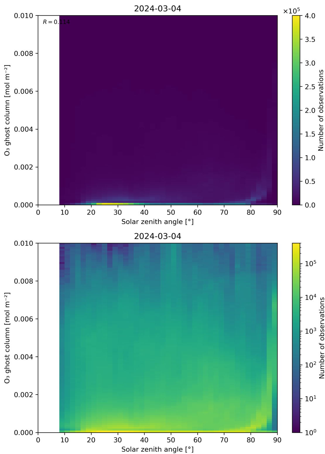
Figure 46: Scatter density plot of “Solar zenith angle” against “O 3 ghost column” for 2024-03-04 to 2024-03-05.
