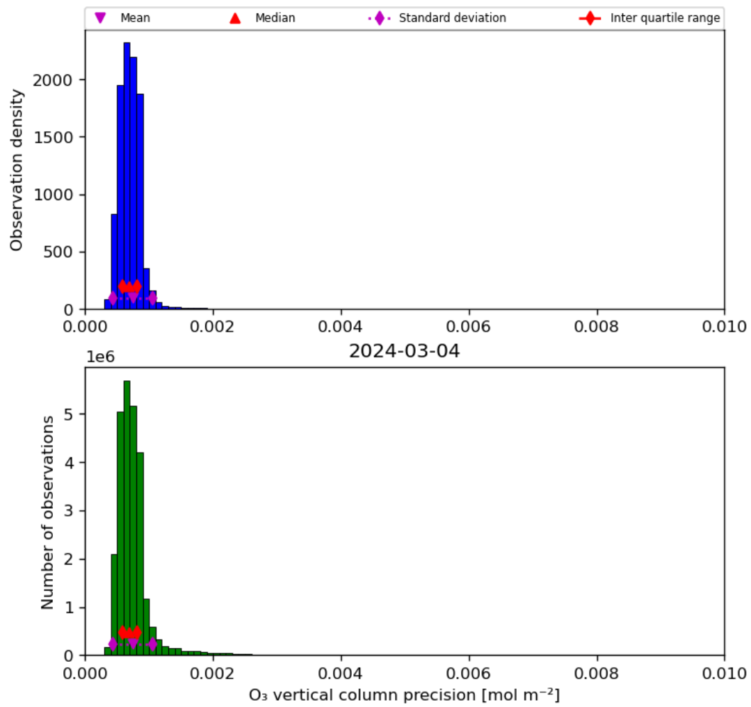
Figure 22: Histogram of “O 3 vertical column precision” for 2024-03-04 to 2024-03-05
