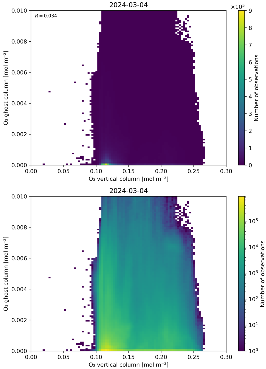
Figure 40: Scatter density plot of “O 3 vertical column” against “O 3 ghost column” for 2024-03-04 to 2024-03-05.
