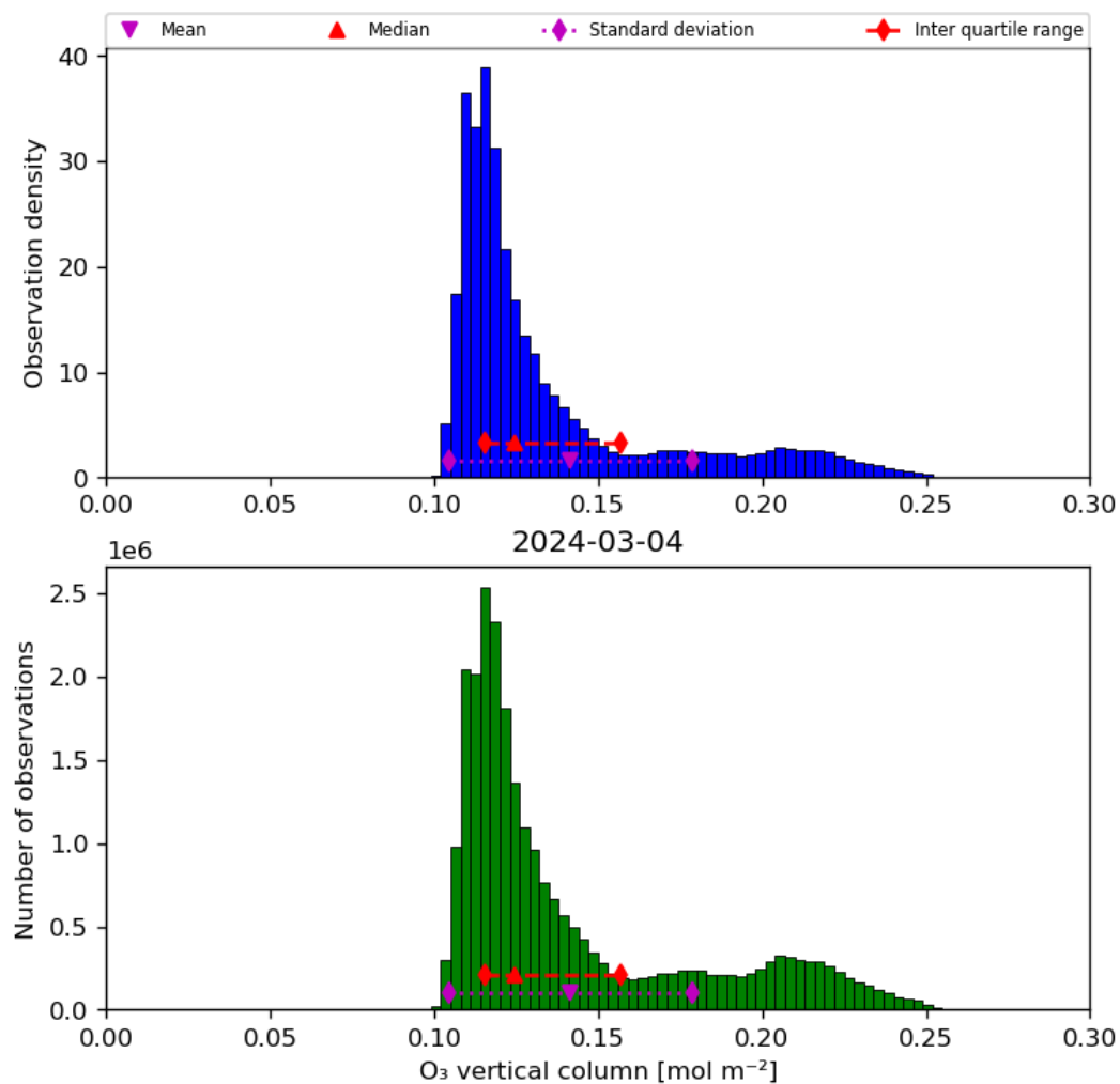
Figure 21: Histogram of “O 3 vertical column” for 2024-03-04 to 2024-03-05
