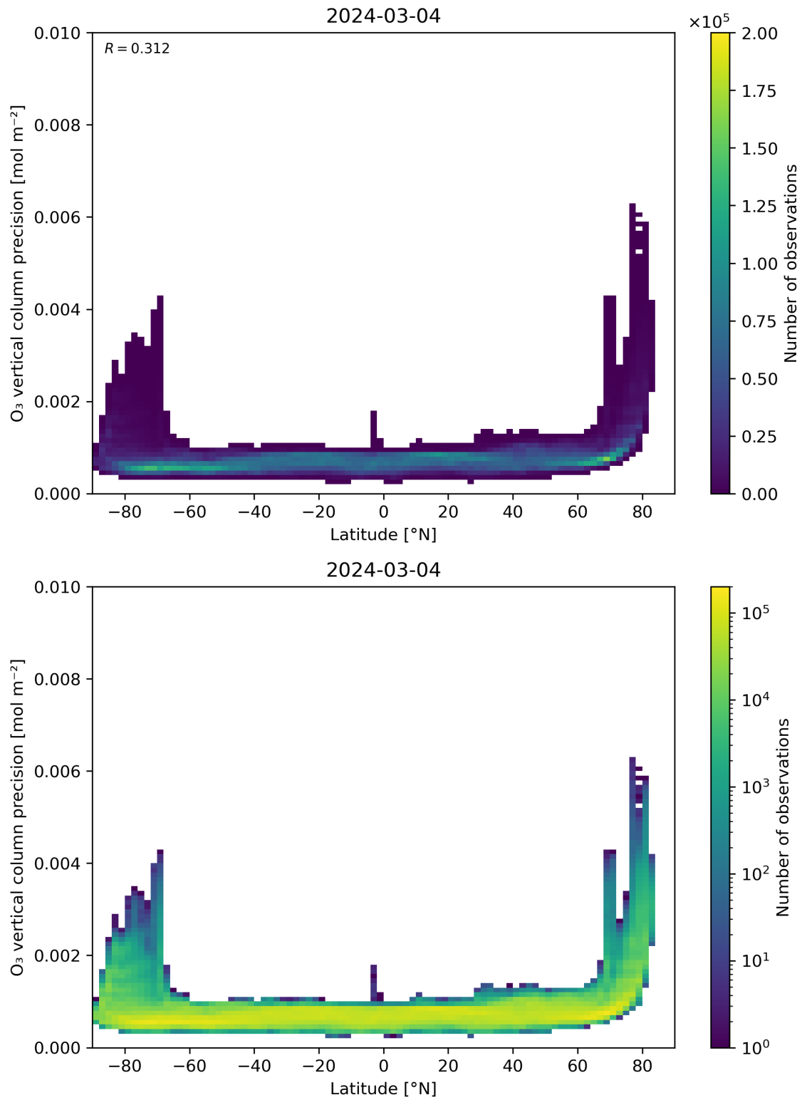
Figure 37: Scatter density plot of “Latitude” against “O 3 vertical column precision” for 2024-03-04 to 2024-03-05.
