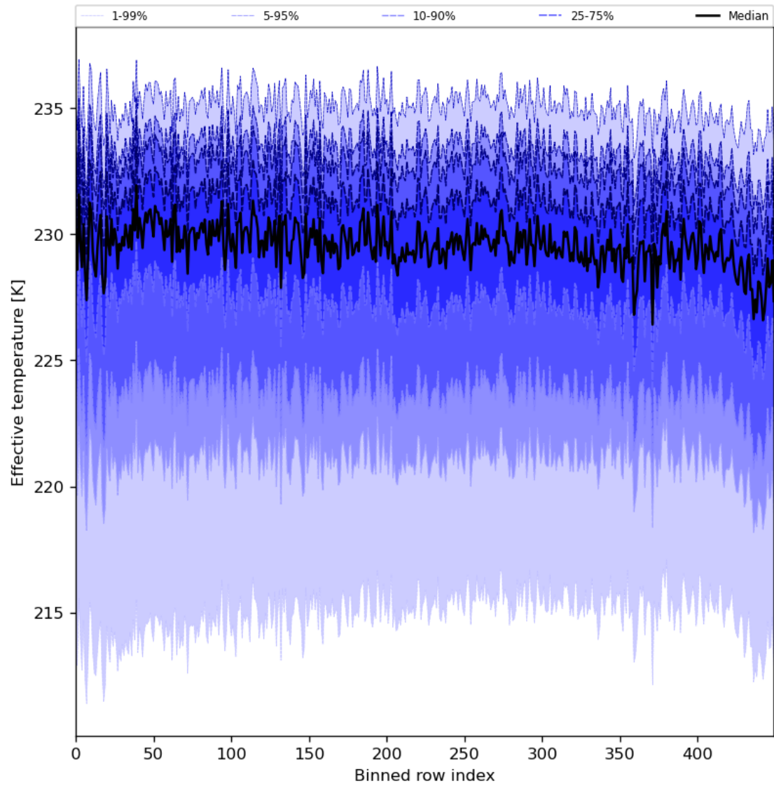
Figure 31: Along track statistics of “Effective temperature” for 2024-03-04 to 2024-03-05
