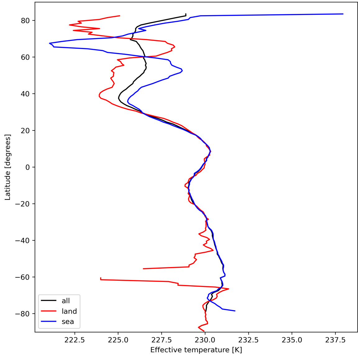
Figure 17: Zonal average of “Effective temperature” for 2024-03-04 to 2024-03-05.
