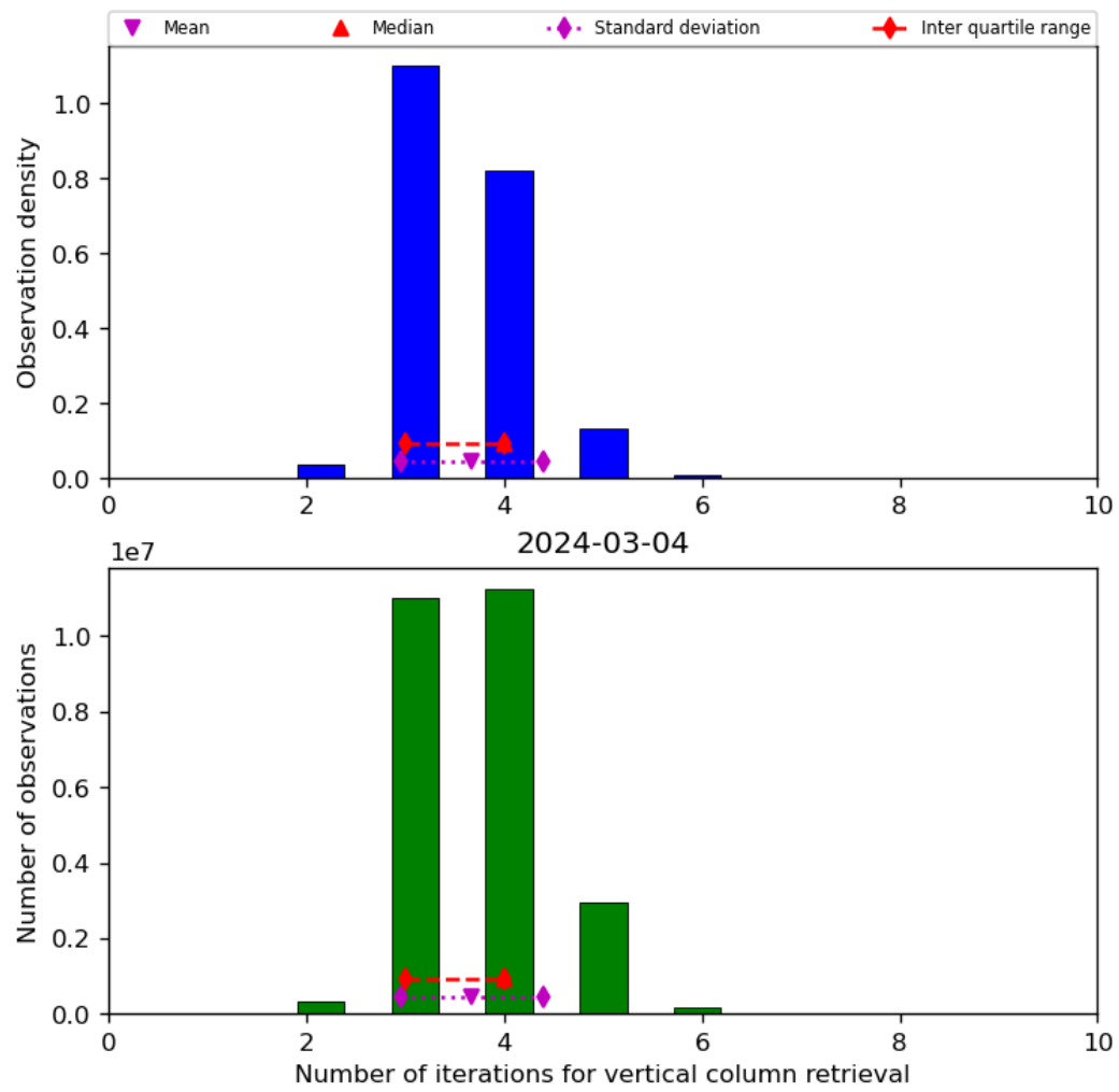
Figure 26: Histogram of “Number of iterations for vertical column retrieval” for 2024-03-04 to 2024-03-05
