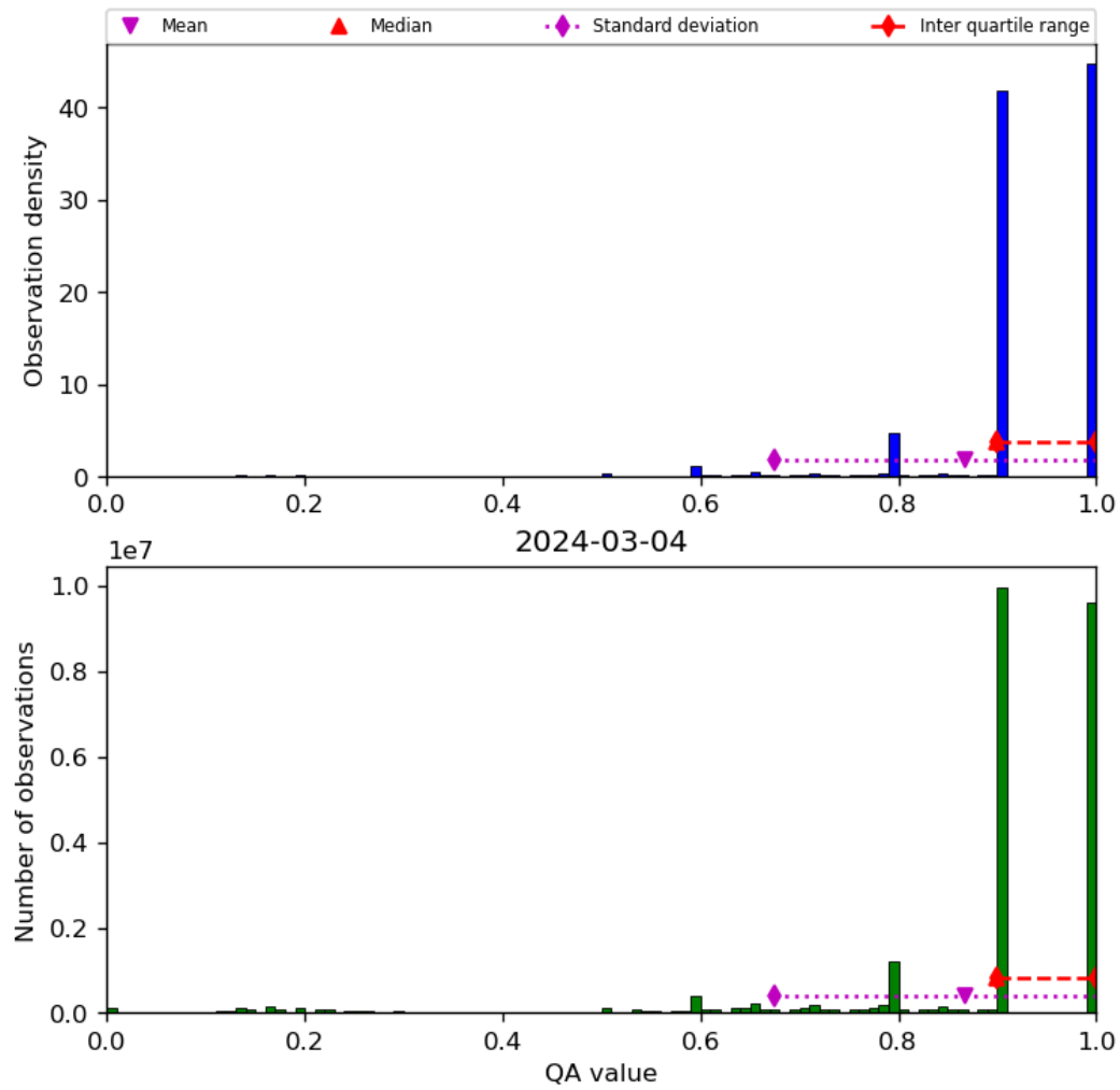
Figure 20: Histogram of “QA value” for 2024-03-04 to 2024-03-05
