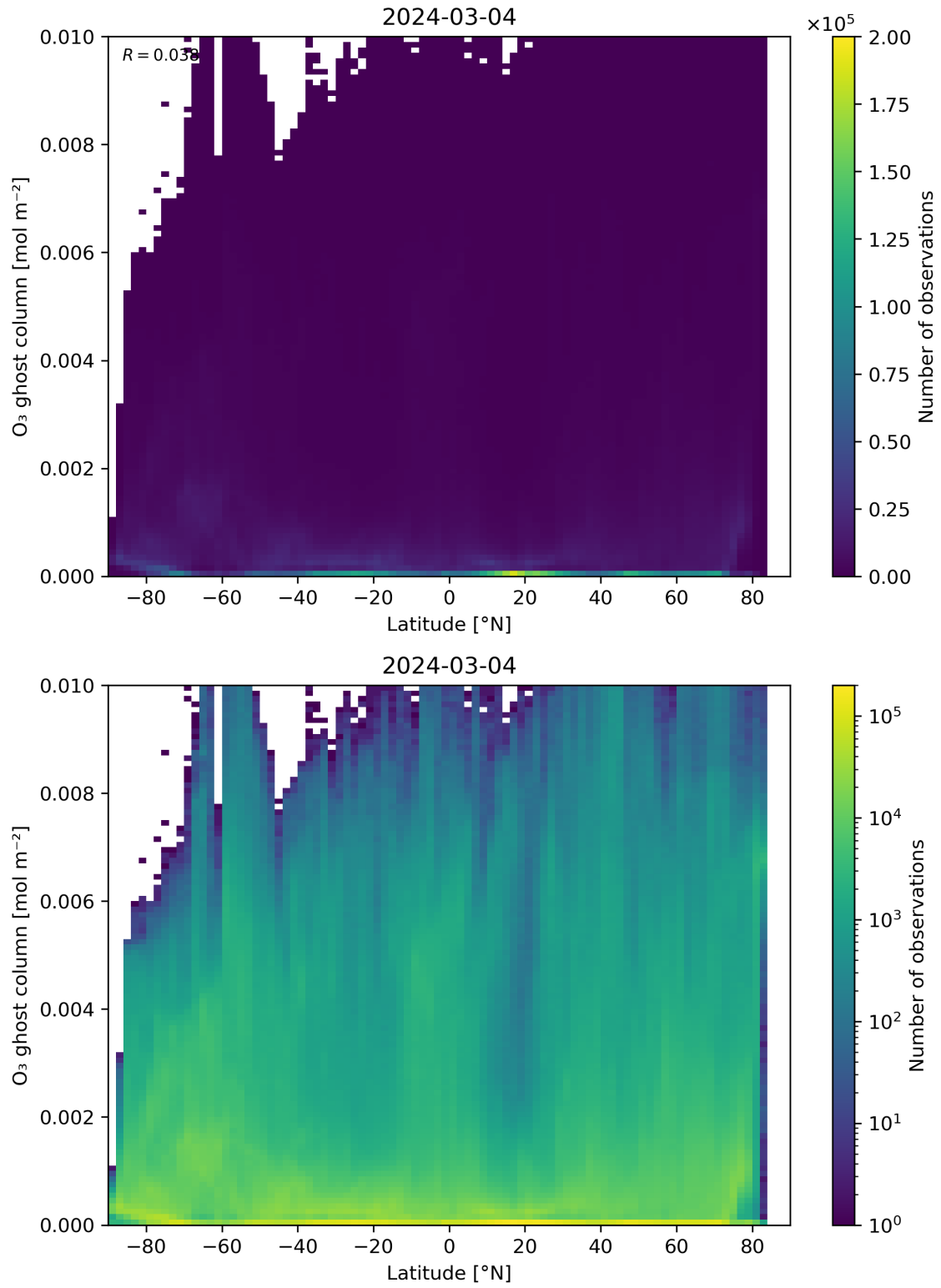
Figure 35: Scatter density plot of “Latitude” against “O 3 ghost column” for 2024-03-04 to 2024-03-05.
