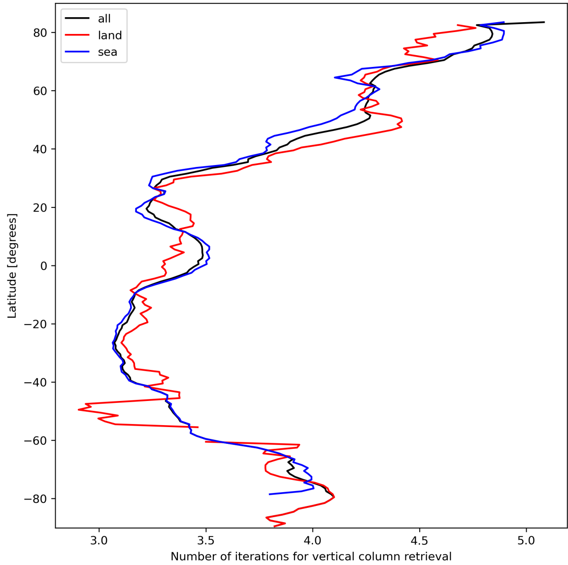
Figure 19: Zonal average of “Number of iterations for vertical column retrieval” for 2024-03-04 to 2024-03-05.
