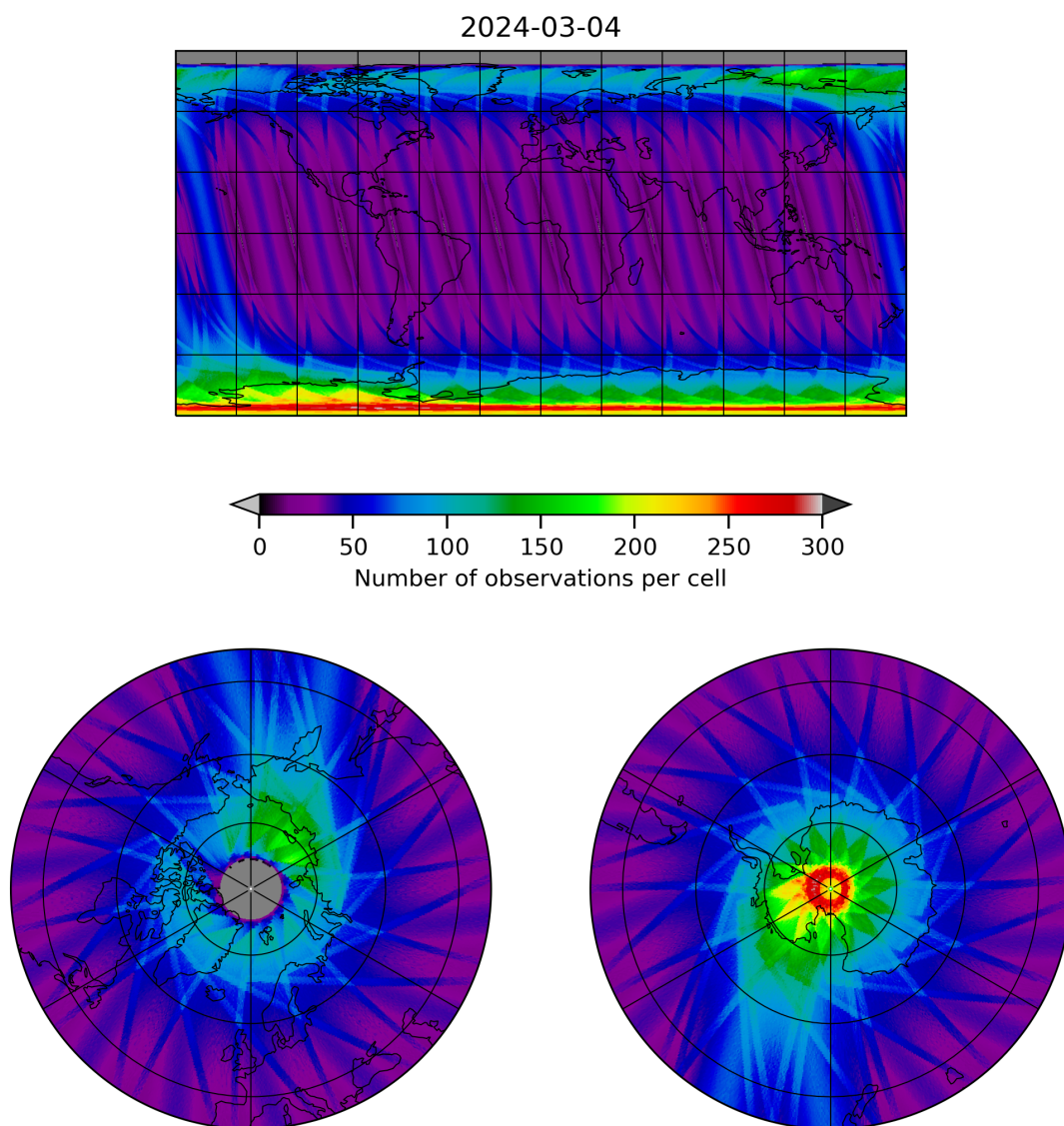
Figure 12: Map of the number of observations for 2024-03-04 to 2024-03-05
