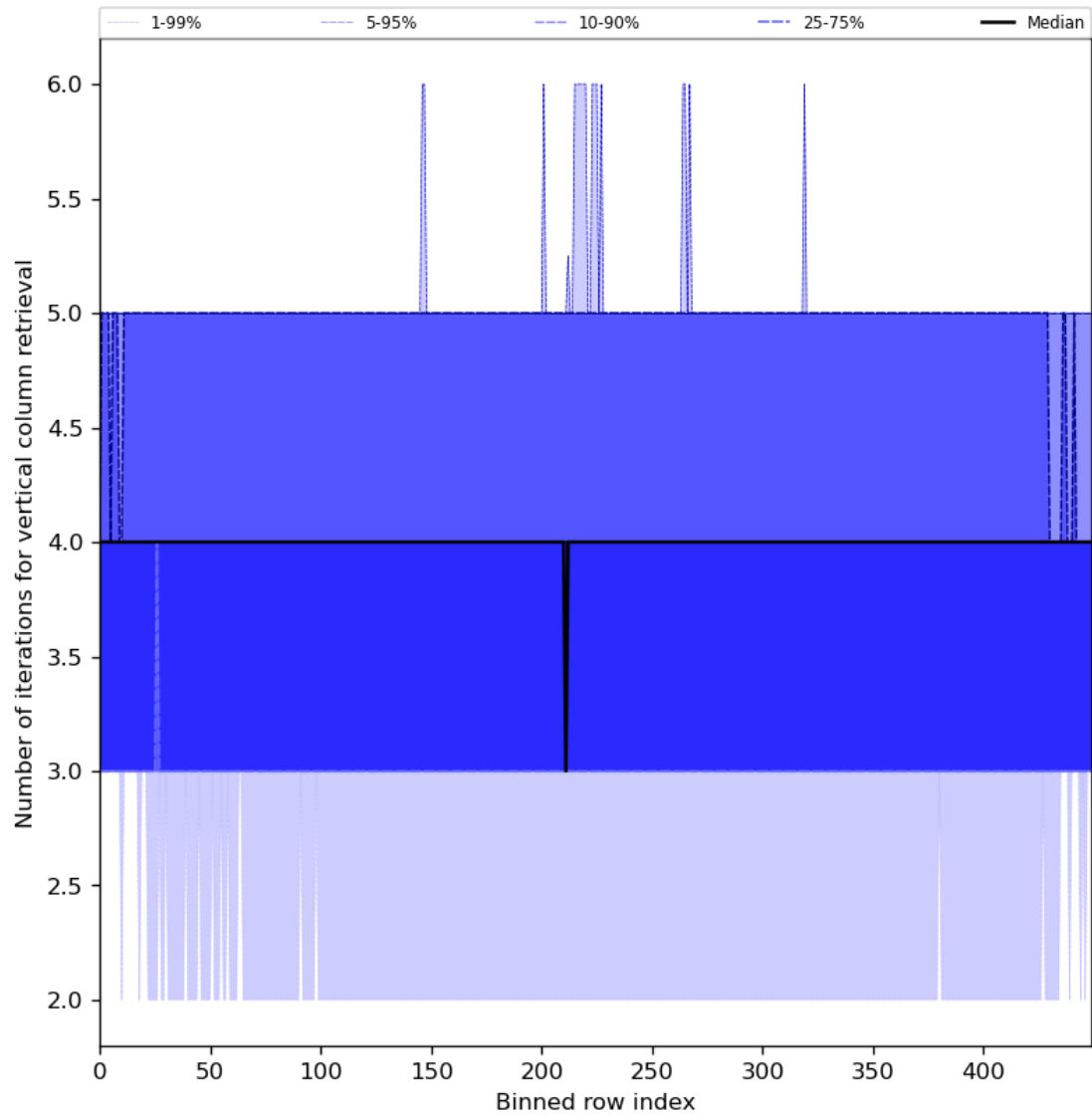
Figure 33: Along track statistics of “Number of iterations for vertical column retrieval” for 2024-03-04 to 2024-03-05
