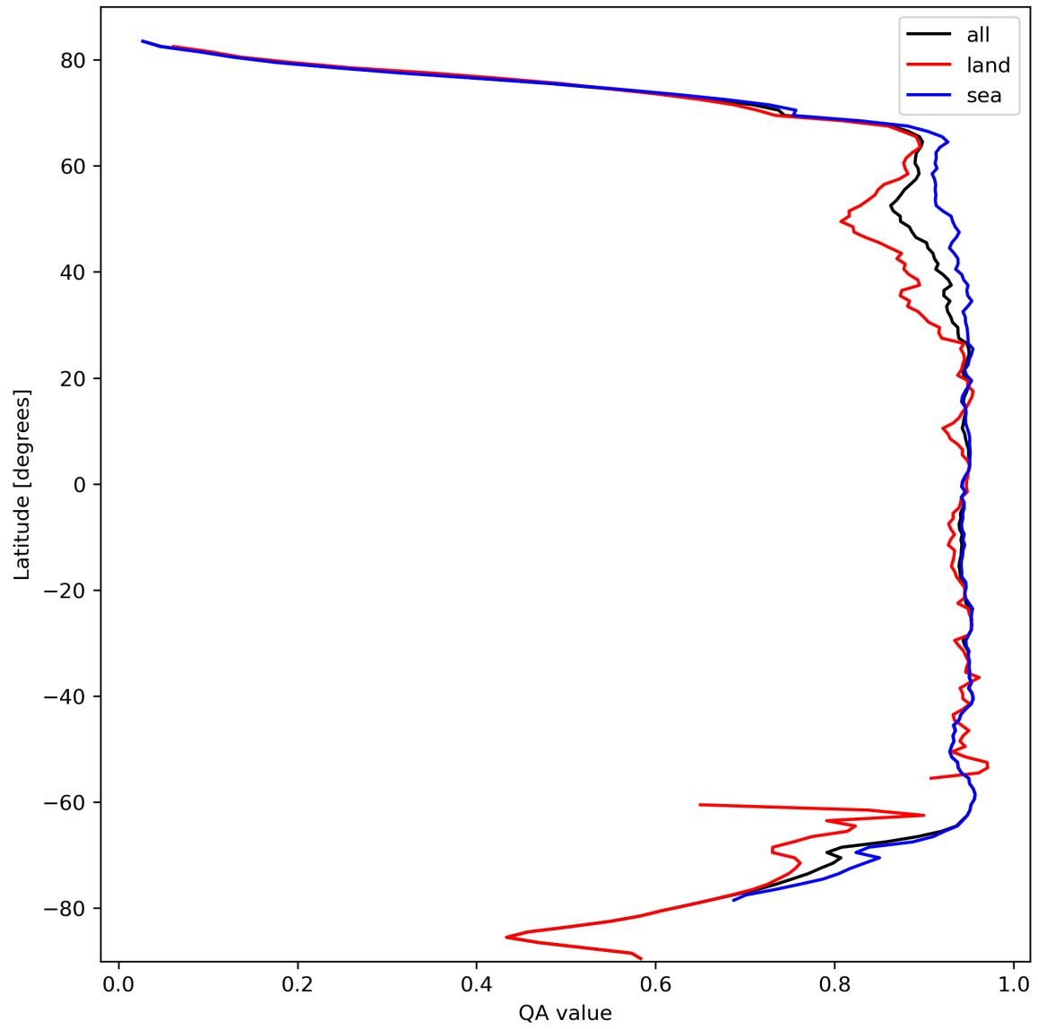
Figure 13: Zonal average of “QA value” for 2024-03-04 to 2024-03-05.
