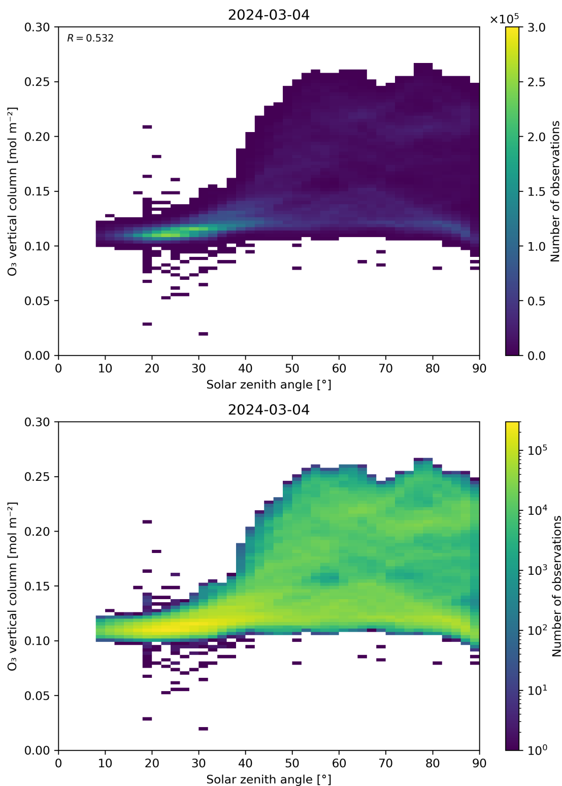
Figure 47: Scatter density plot of “Solar zenith angle” against “O 3 vertical column” for 2024-03-04 to 2024-03-05.
