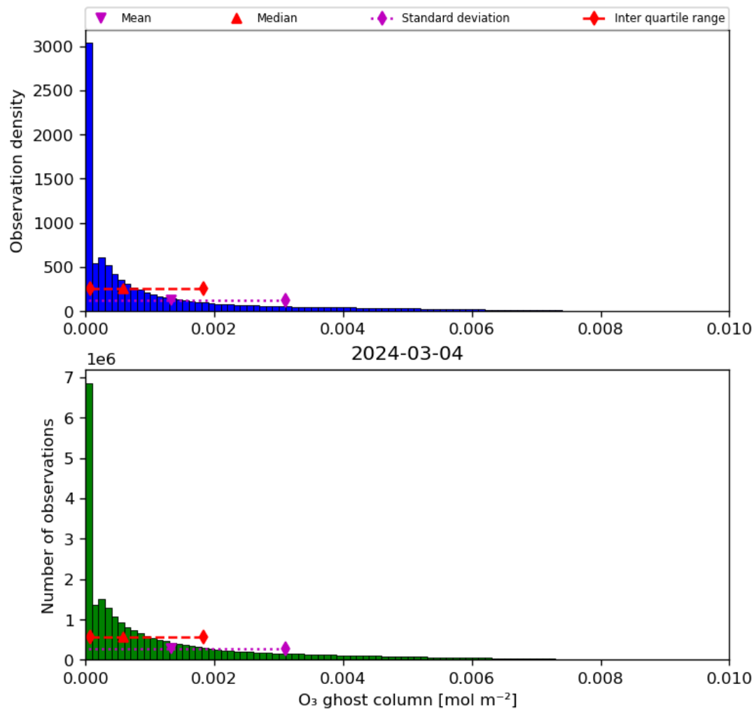
Figure 25: Histogram of “O 3 ghost column” for 2024-03-04 to 2024-03-05
