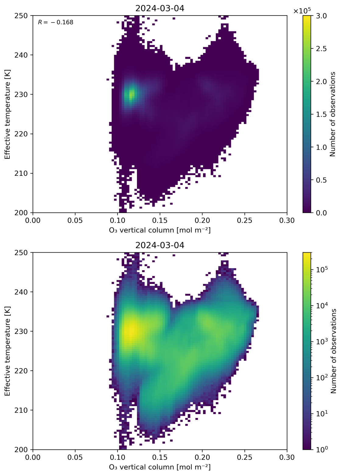
Figure 39: Scatter density plot of “O 3 vertical column” against “Effective temperature” for 2024-03-04 to 2024-03-05.
