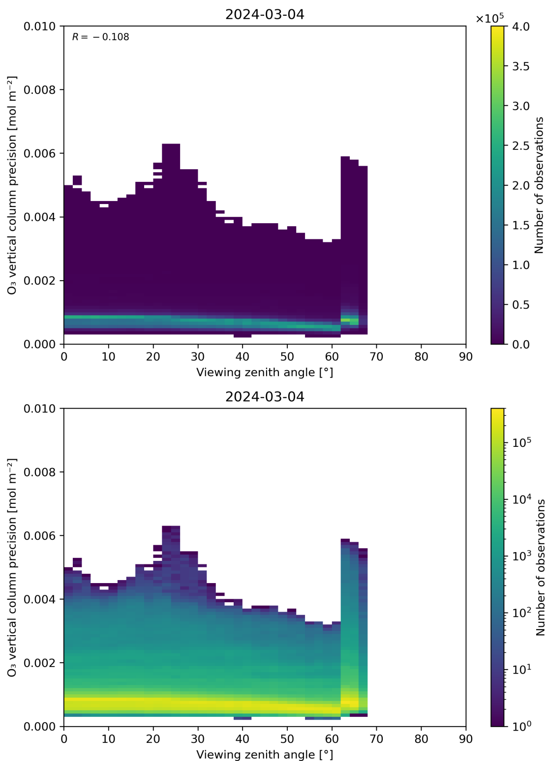
Figure 53: Scatter density plot of “Viewing zenith angle” against “O 3 vertical column precision” for 2024-03-04 to 2024-03-05.
