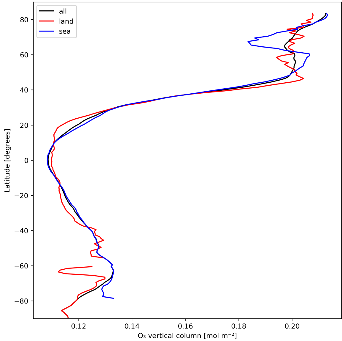
Figure 14: Zonal average of “O 3 vertical column” for 2024-03-04 to 2024-03-06.
