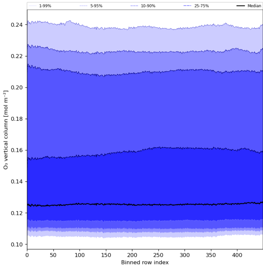
Figure 28: Along track statistics of “O 3 vertical column” for 2024-03-04 to 2024-03-06
