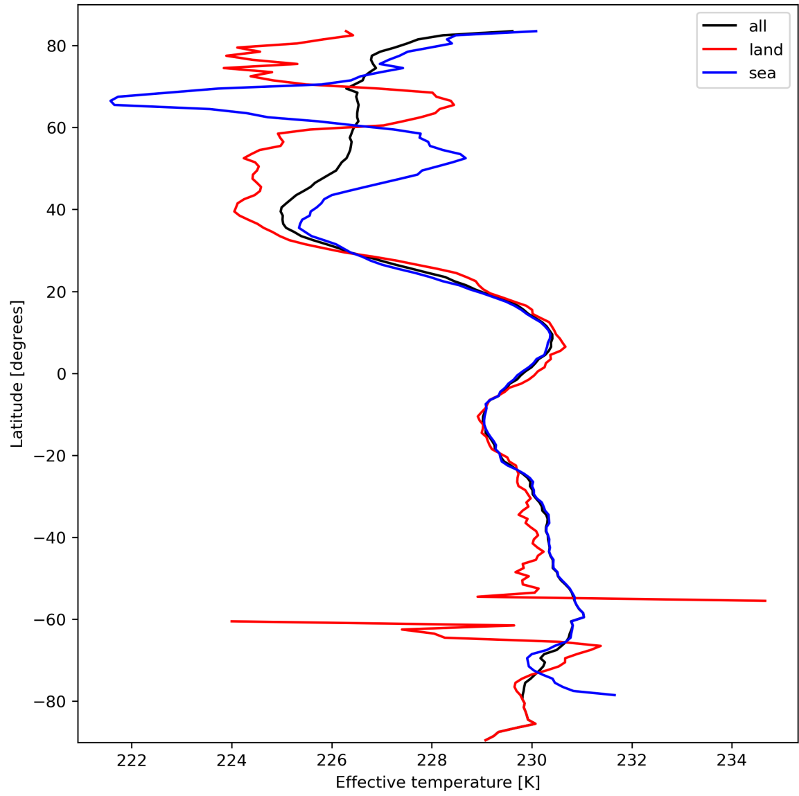
Figure 17: Zonal average of “Effective temperature” for 2024-03-04 to 2024-03-06.
