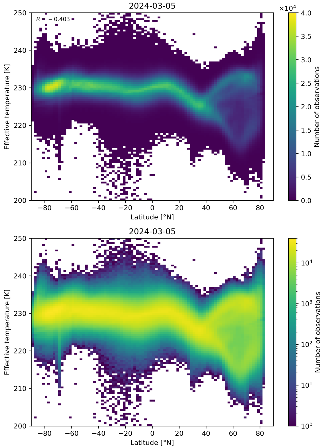
Figure 34: Scatter density plot of “Latitude” against “Effective temperature” for 2024-03-04 to 2024-03-06.
