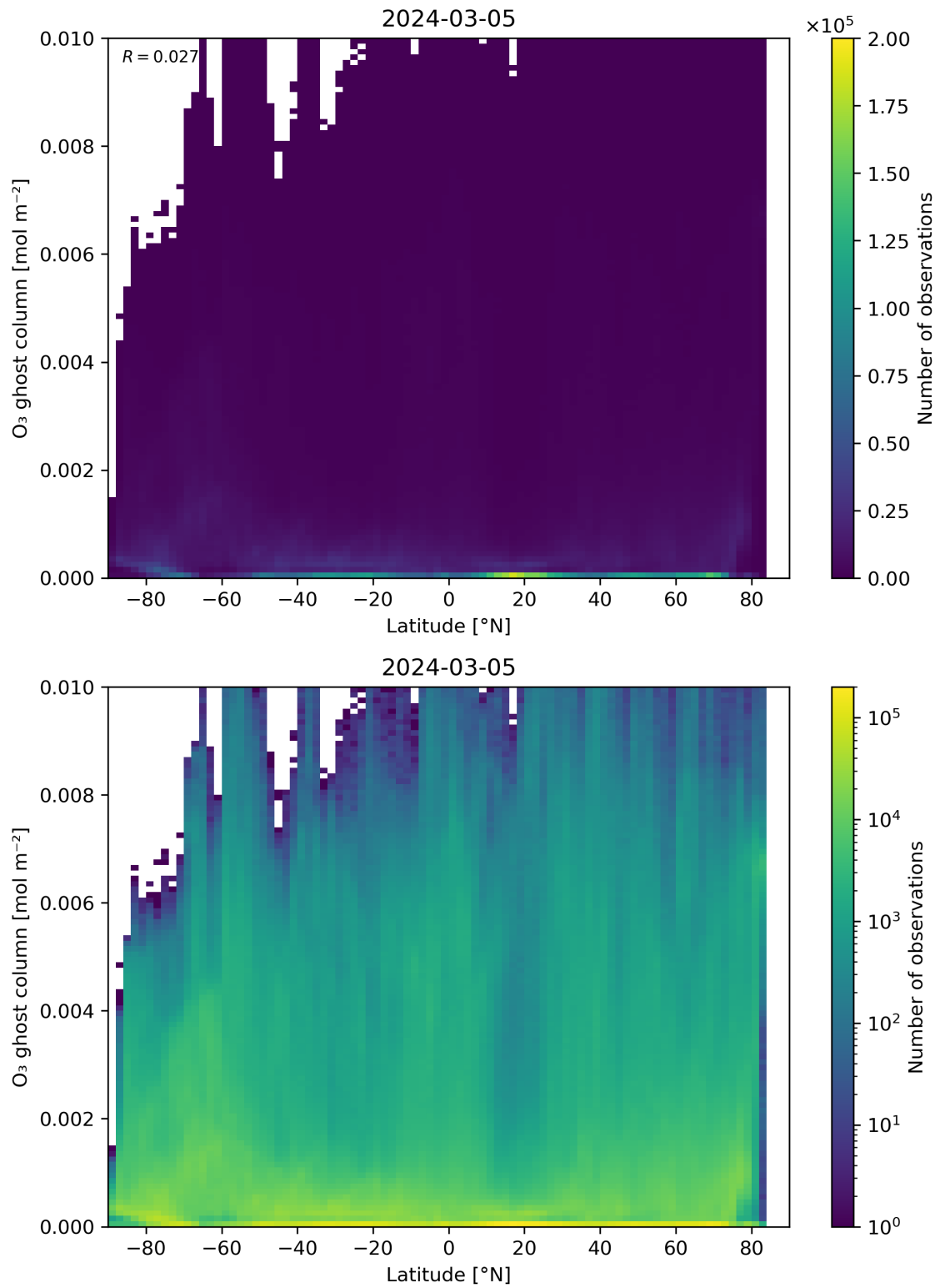
Figure 35: Scatter density plot of “Latitude” against “O 3 ghost column” for 2024-03-04 to 2024-03-06.
