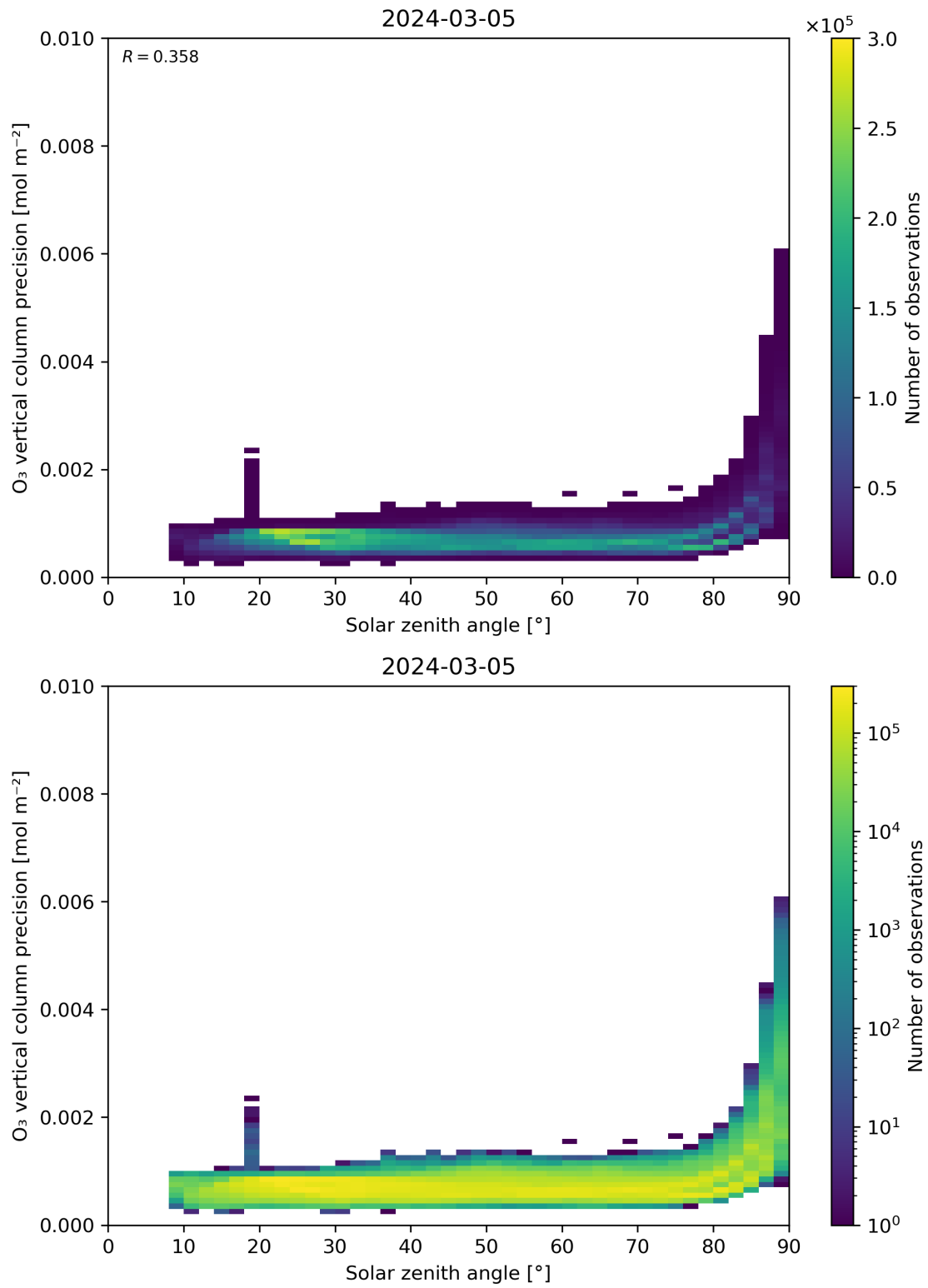
Figure 48: Scatter density plot of “Solar zenith angle” against “O 3 vertical column precision” for 2024-03-04 to 2024-03-06.
