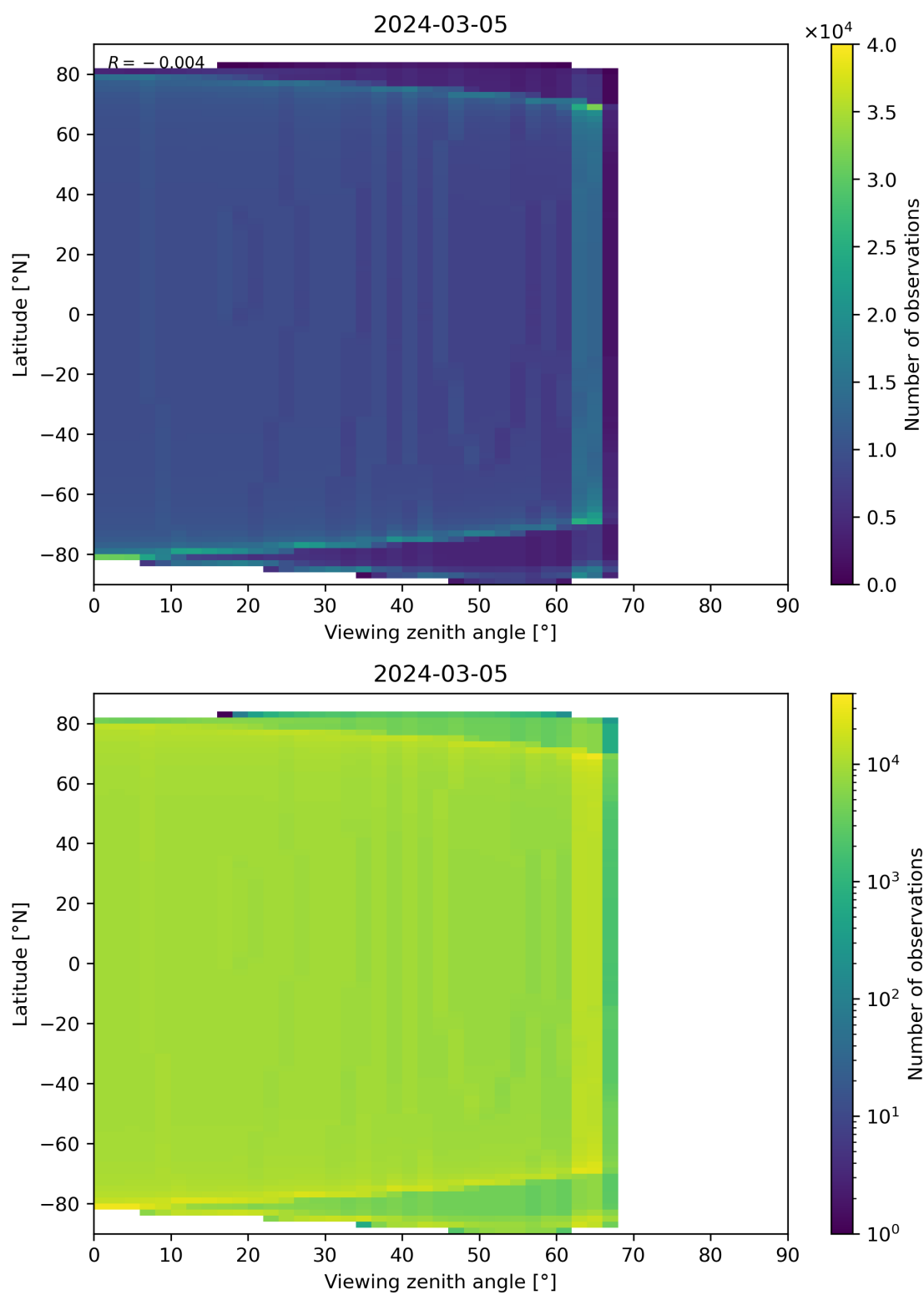
Figure 49: Scatter density plot of “Viewing zenith angle” against “Latitude” for 2024-03-04 to 2024-03-06.
