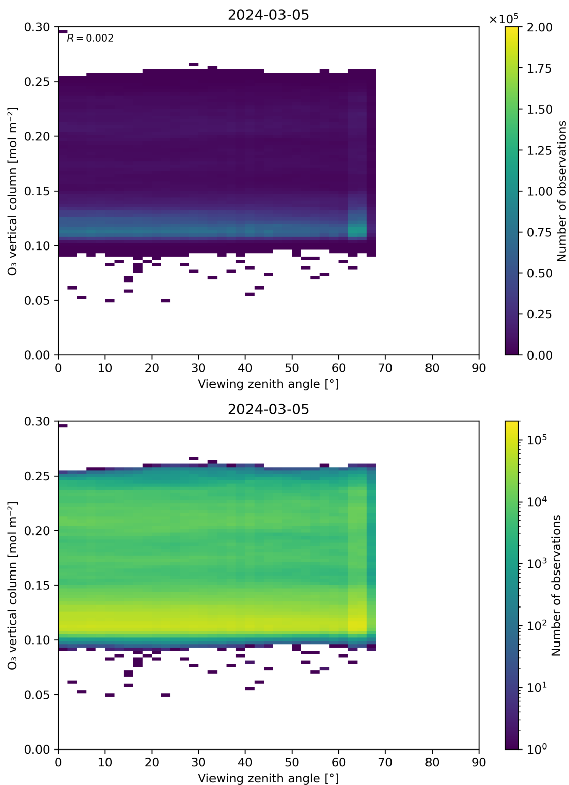
Figure 52: Scatter density plot of “Viewing zenith angle” against “O 3 vertical column” for 2024-03-04 to 2024-03-06.
