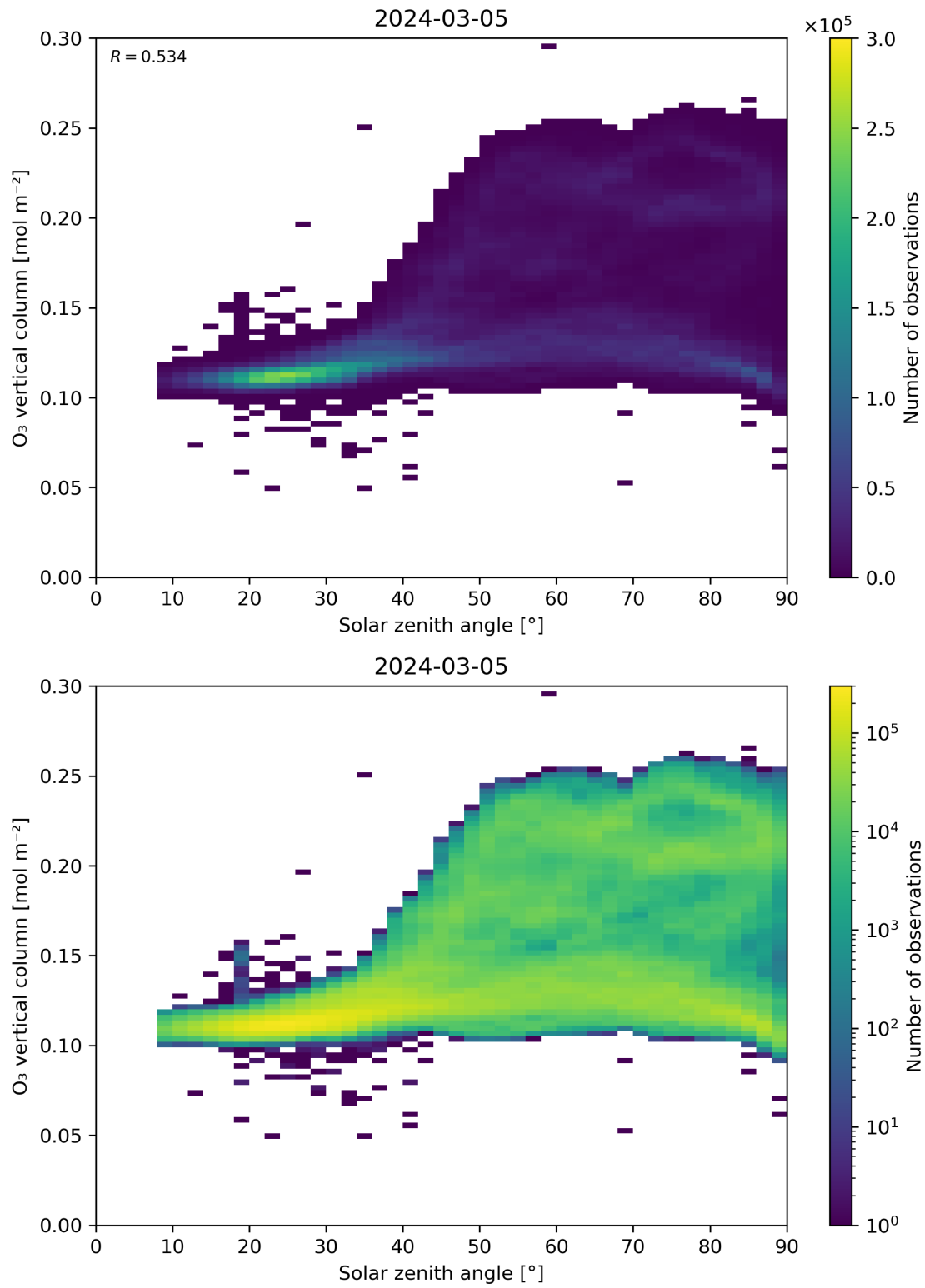
Figure 47: Scatter density plot of “Solar zenith angle” against “O 3 vertical column” for 2024-03-04 to 2024-03-06.
