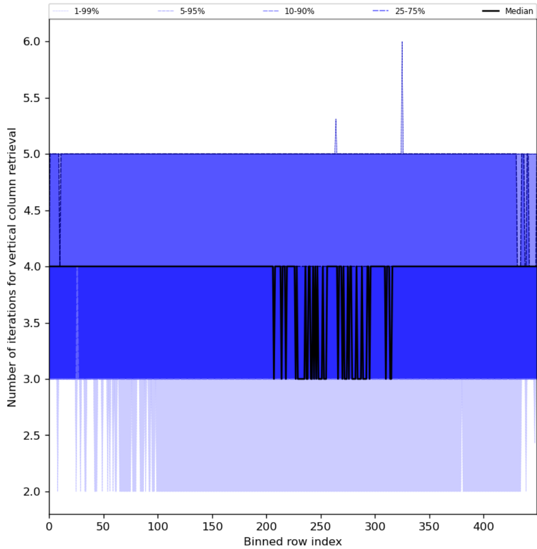
Figure 33: Along track statistics of “Number of iterations for vertical column retrieval” for 2024-03-04 to 2024-03-06
