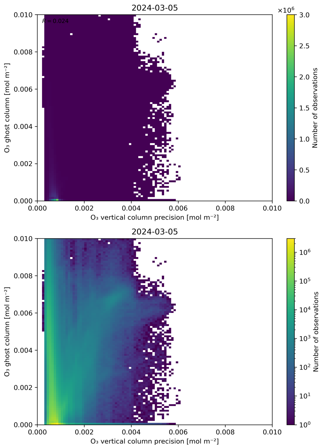
Figure 43: Scatter density plot of “ \text{O}_3 vertical column precision” against “ \text{O}_3 ghost column” for 2024-03-04 to 2024-03-06.
