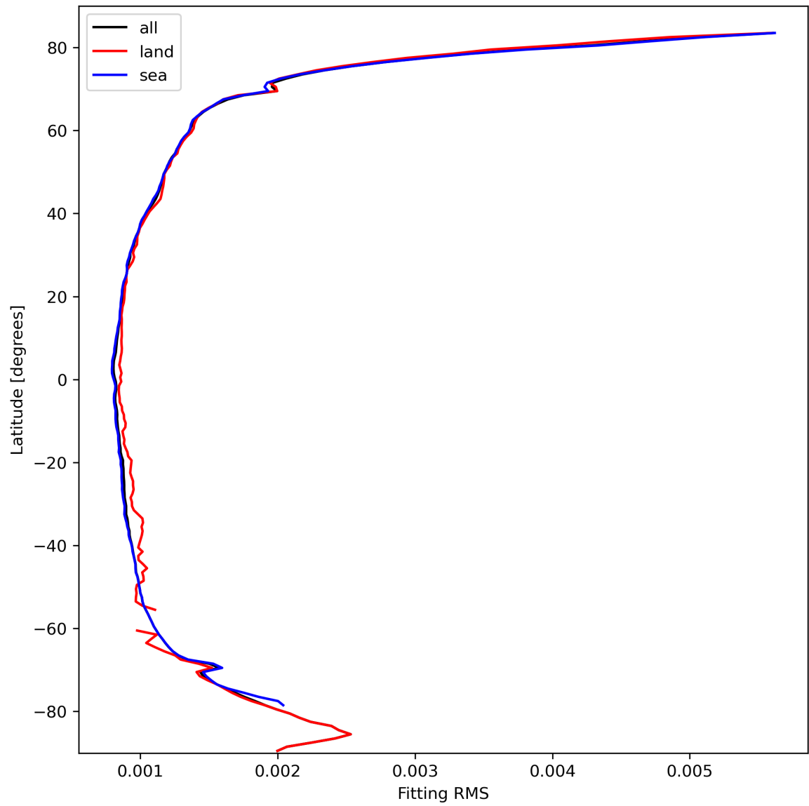
Figure 16: Zonal average of “Fitting RMS” for 2024-03-04 to 2024-03-06.
