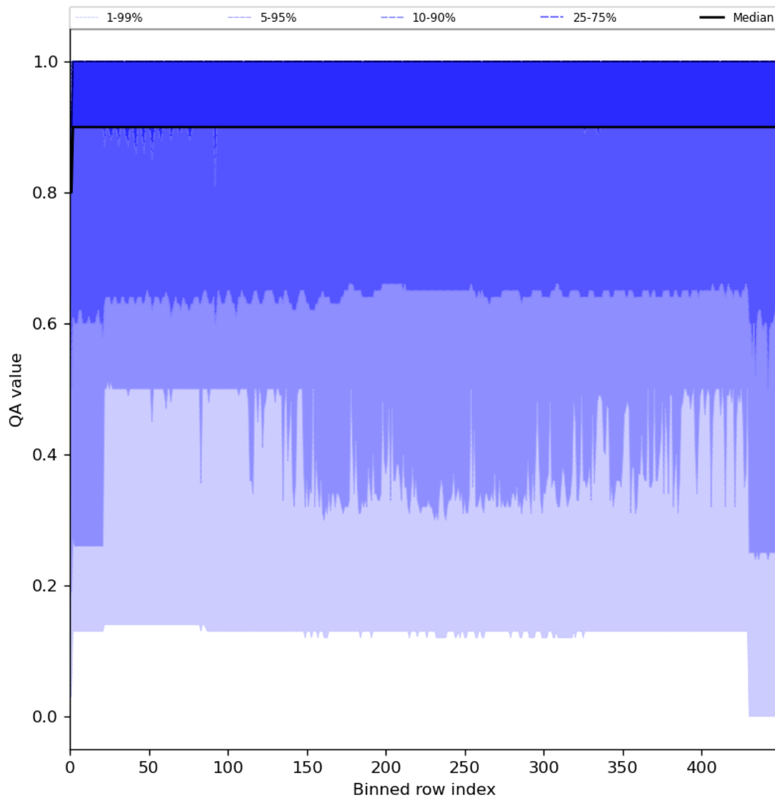
Figure 27: Along track statistics of “QA value” for 2024-03-04 to 2024-03-06
