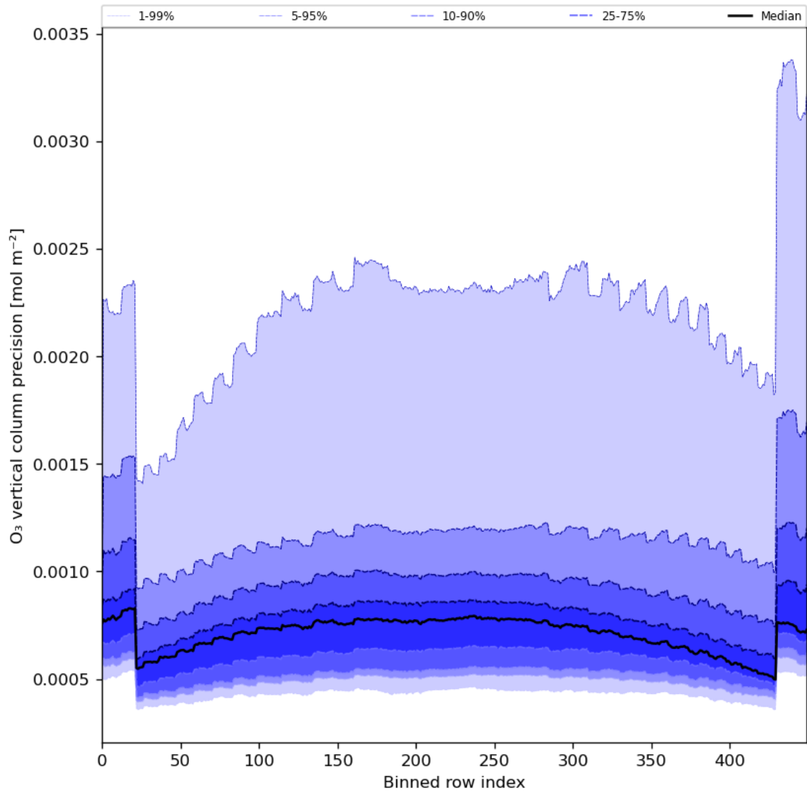
Figure 29: Along track statistics of “O 3 vertical column precision” for 2024-03-04 to 2024-03-06
