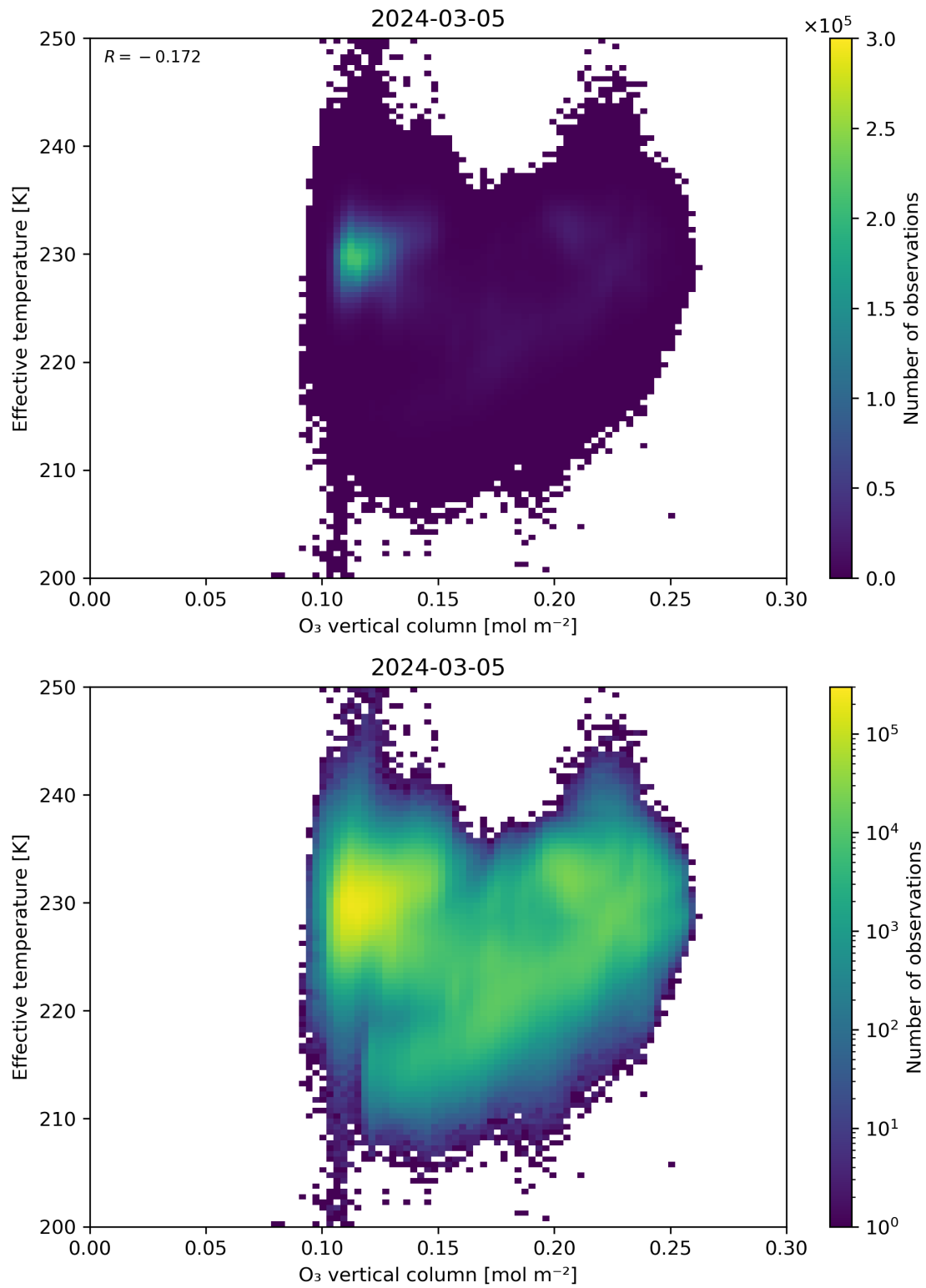
Figure 39: Scatter density plot of “O 3 vertical column” against “Effective temperature” for 2024-03-04 to 2024-03-06.
