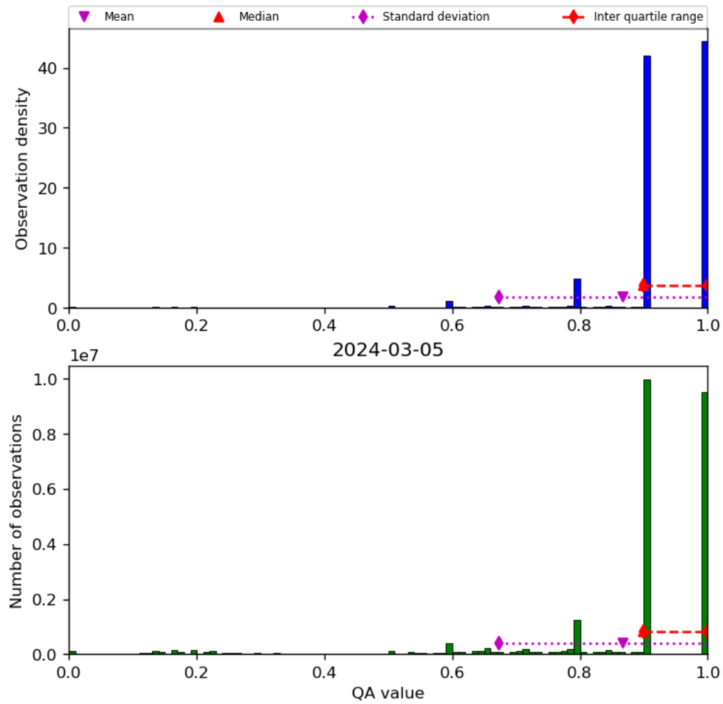
Figure 20: Histogram of “QA value” for 2024-03-04 to 2024-03-06
