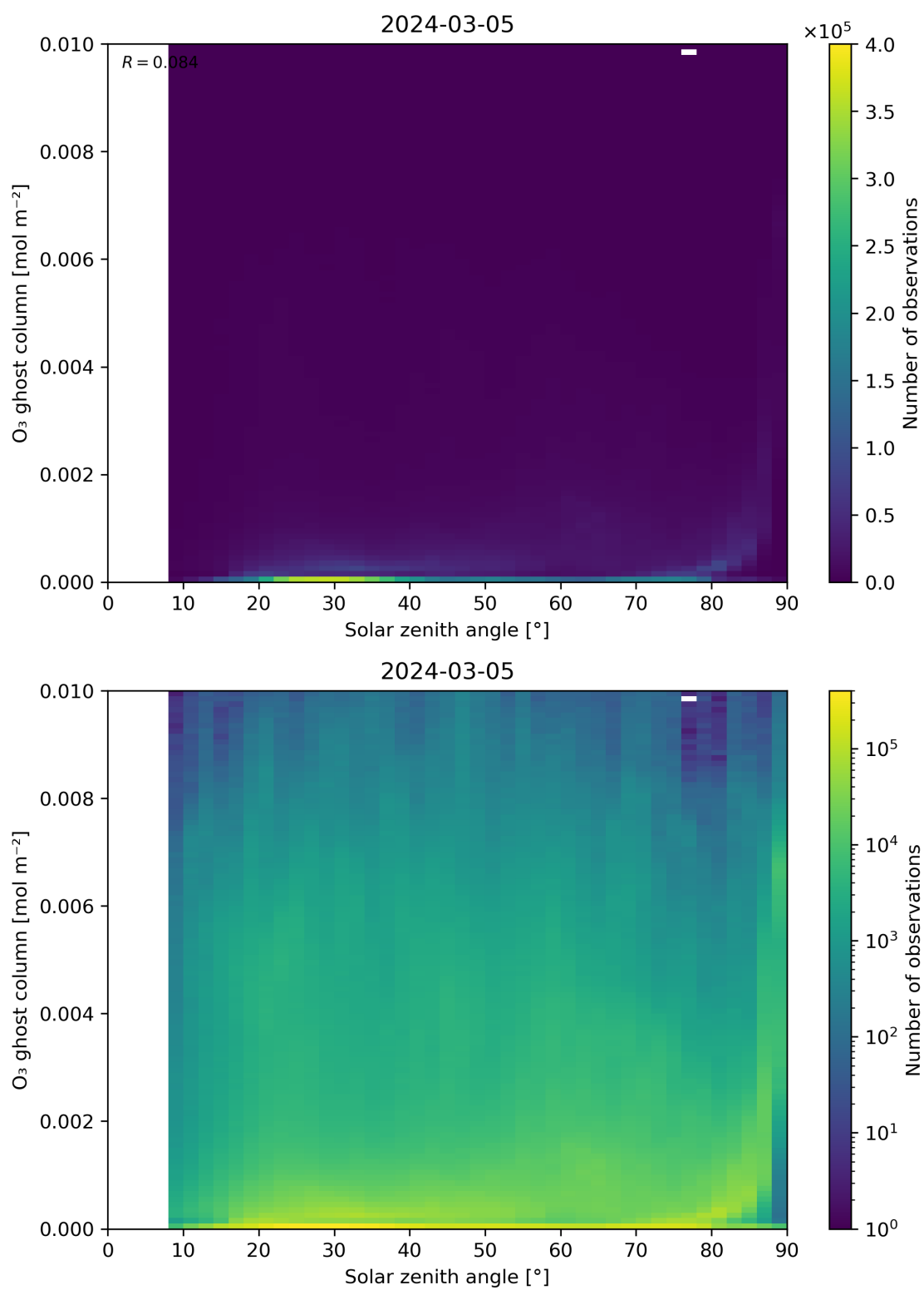
Figure 46: Scatter density plot of “Solar zenith angle” against “O 3 ghost column” for 2024-03-04 to 2024-03-06.
