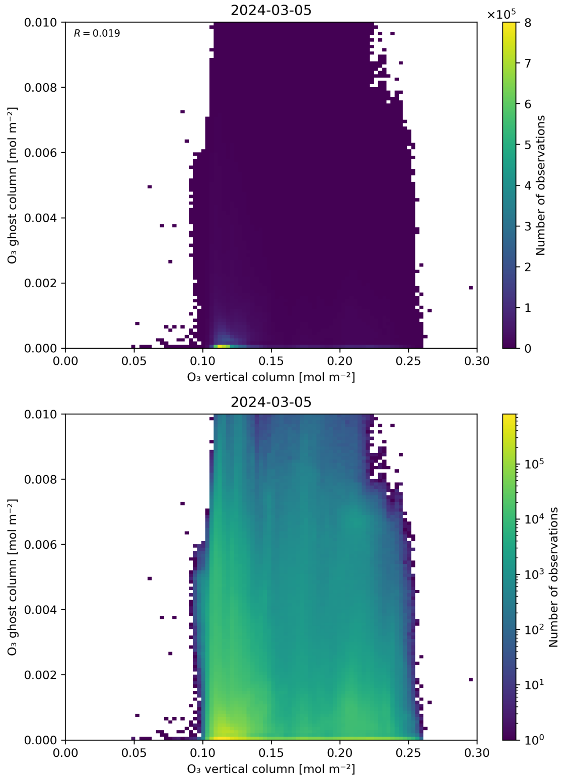
Figure 40: Scatter density plot of “O 3 vertical column” against “O 3 ghost column” for 2024-03-04 to 2024-03-06.
