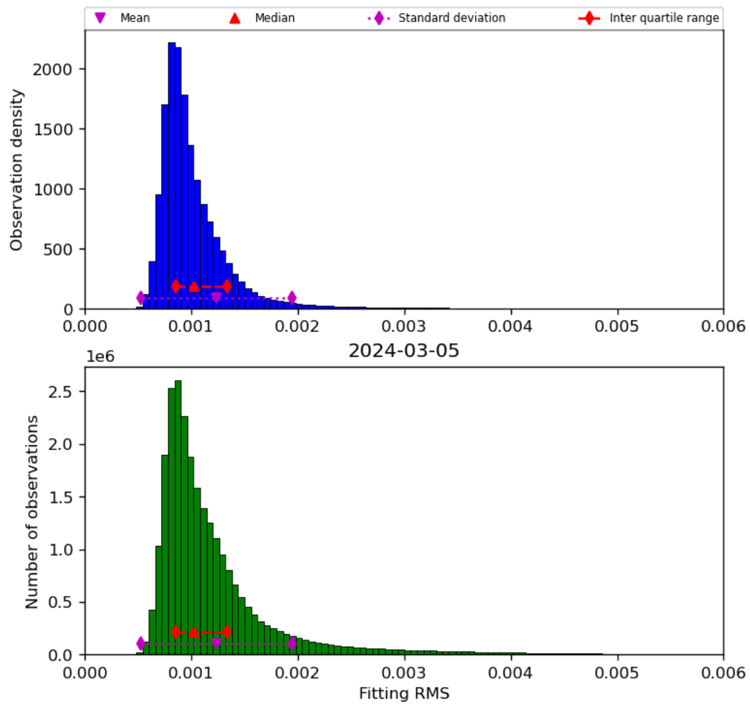
Figure 23: Histogram of “Fitting RMS” for 2024-03-04 to 2024-03-06
