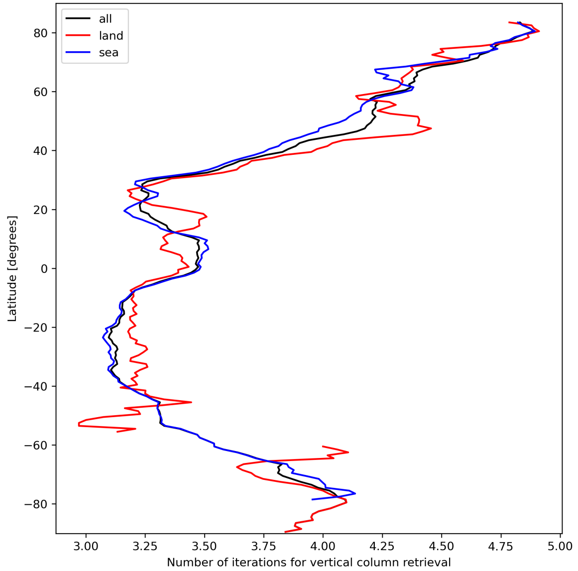
Figure 19: Zonal average of “Number of iterations for vertical column retrieval” for 2024-03-04 to 2024-03-06.
