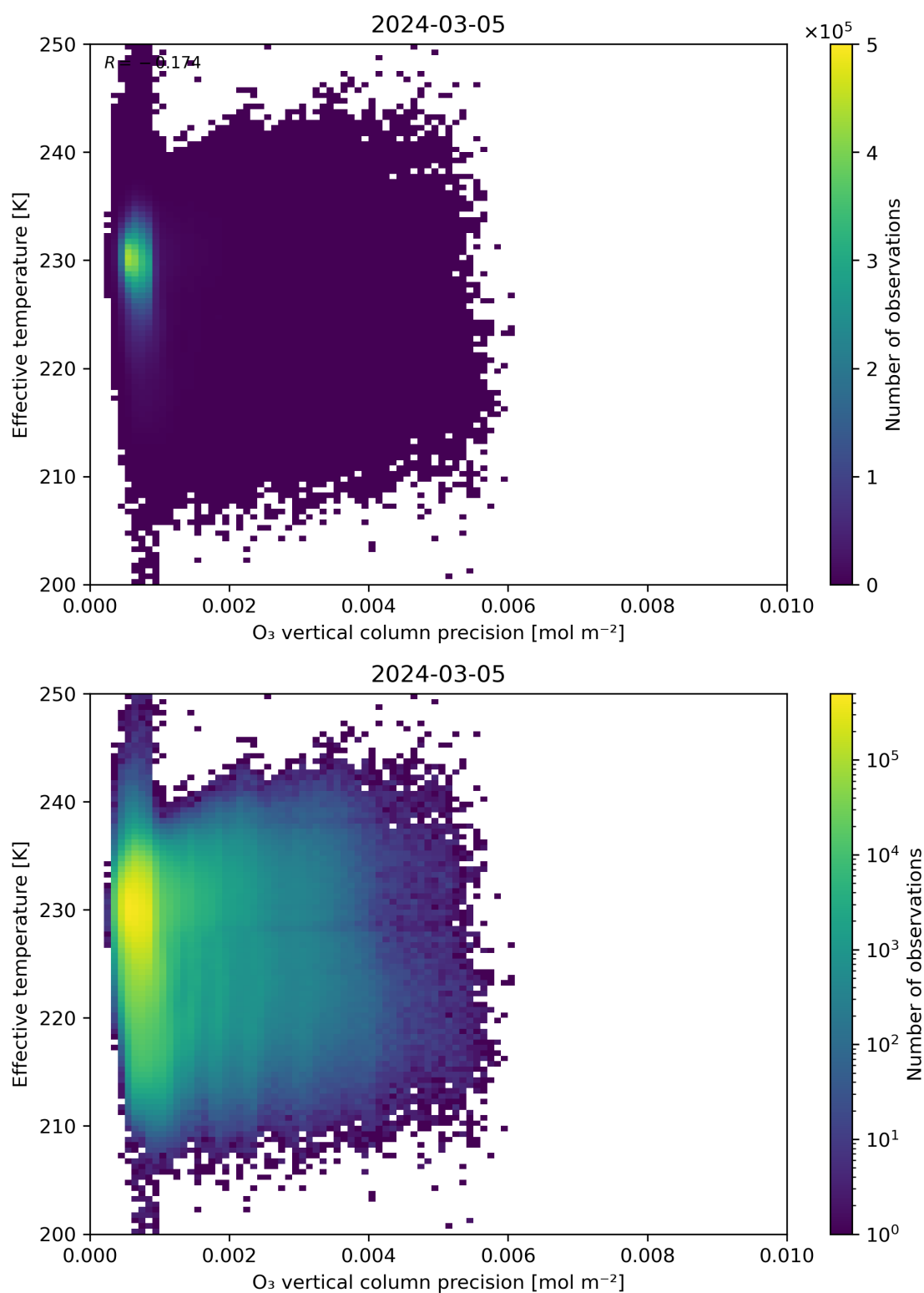
Figure 42: Scatter density plot of “O 3 vertical column precision” against “Effective temperature” for 2024-03-04 to 2024-03-06.
