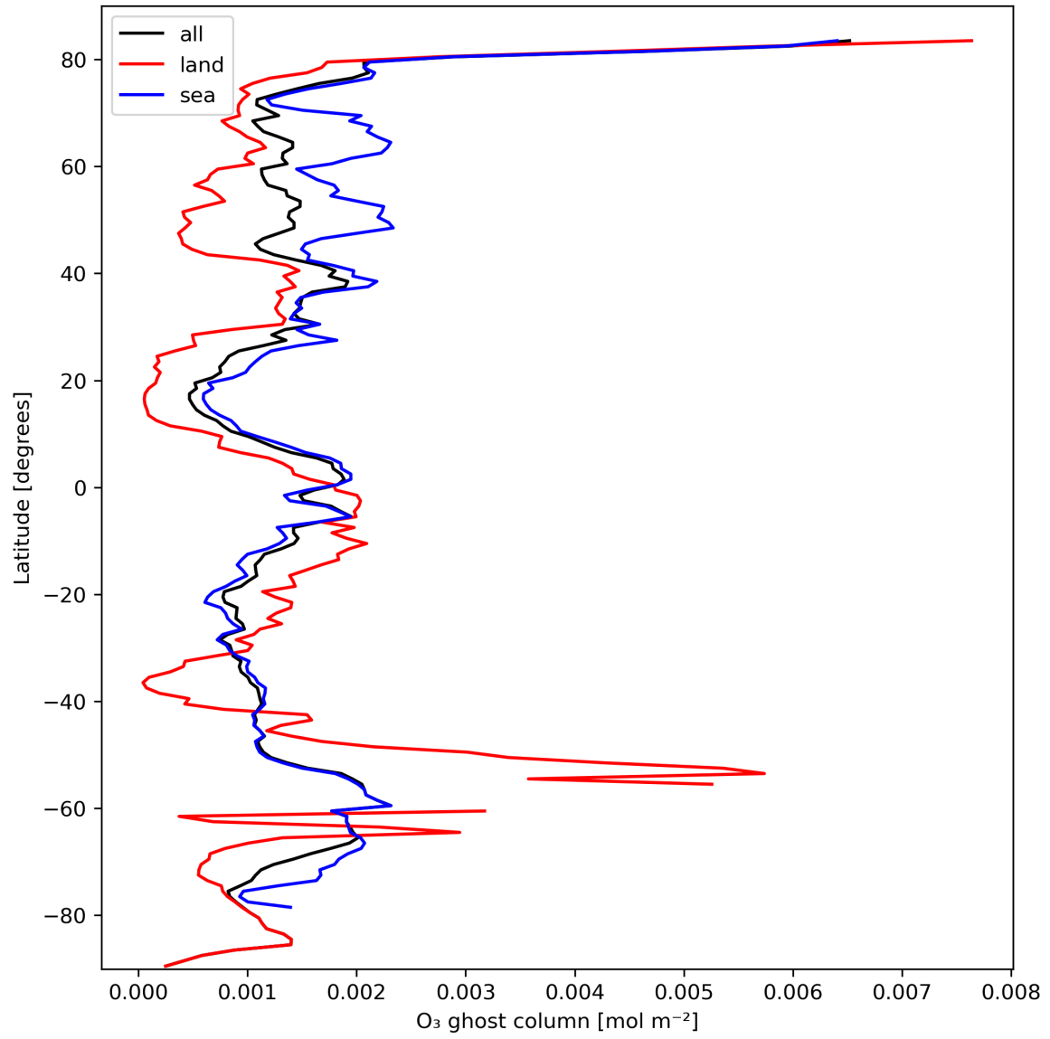
Figure 18: Zonal average of "O 3 ghost column" for 2024-03-04 to 2024-03-06.
