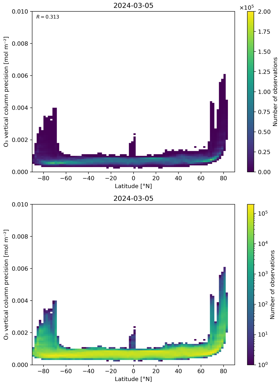
Figure 37: Scatter density plot of “Latitude” against “O 3 vertical column precision” for 2024-03-04 to 2024-03-06.
