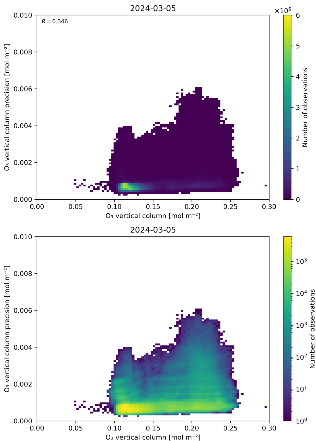
Figure 41: Scatter density plot of “O 3 vertical column” against “O 3 vertical column precision” for 2024-03-04 to 2024-03-06.
