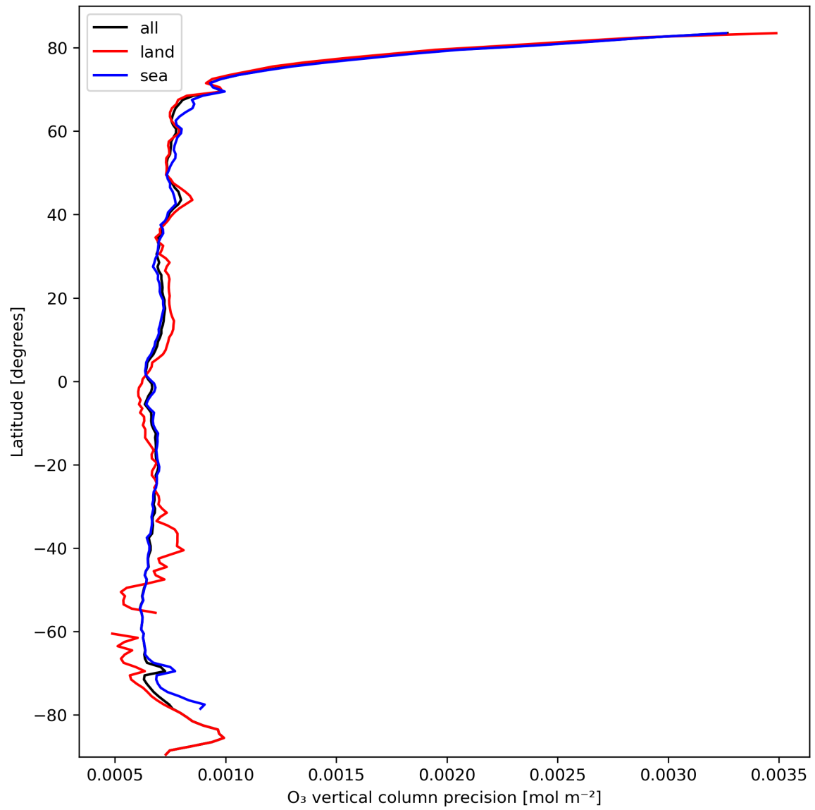
Figure 15: Zonal average of “O 3 vertical column precision” for 2024-03-04 to 2024-03-06.
