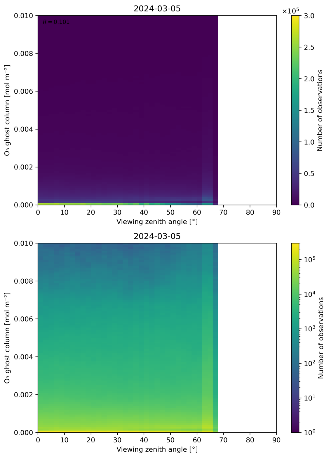
Figure 51: Scatter density plot of “Viewing zenith angle” against “O 3 ghost column” for 2024-03-04 to 2024-03-06.
