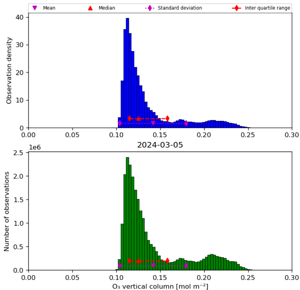
Figure 21: Histogram of “O 3 vertical column” for 2024-03-04 to 2024-03-06
