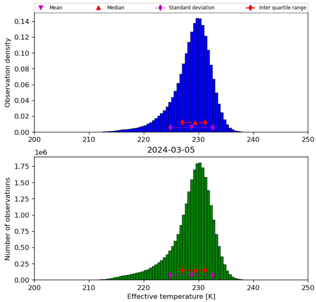
Figure 24: Histogram of “Effective temperature” for 2024-03-04 to 2024-03-06
