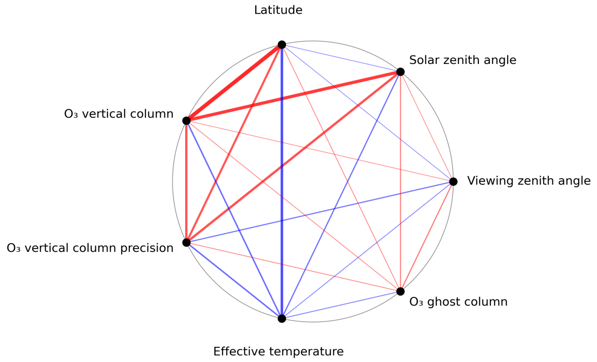
Figure 1: Map of correlation graph for 2024-03-04 to 2024-03-06.
