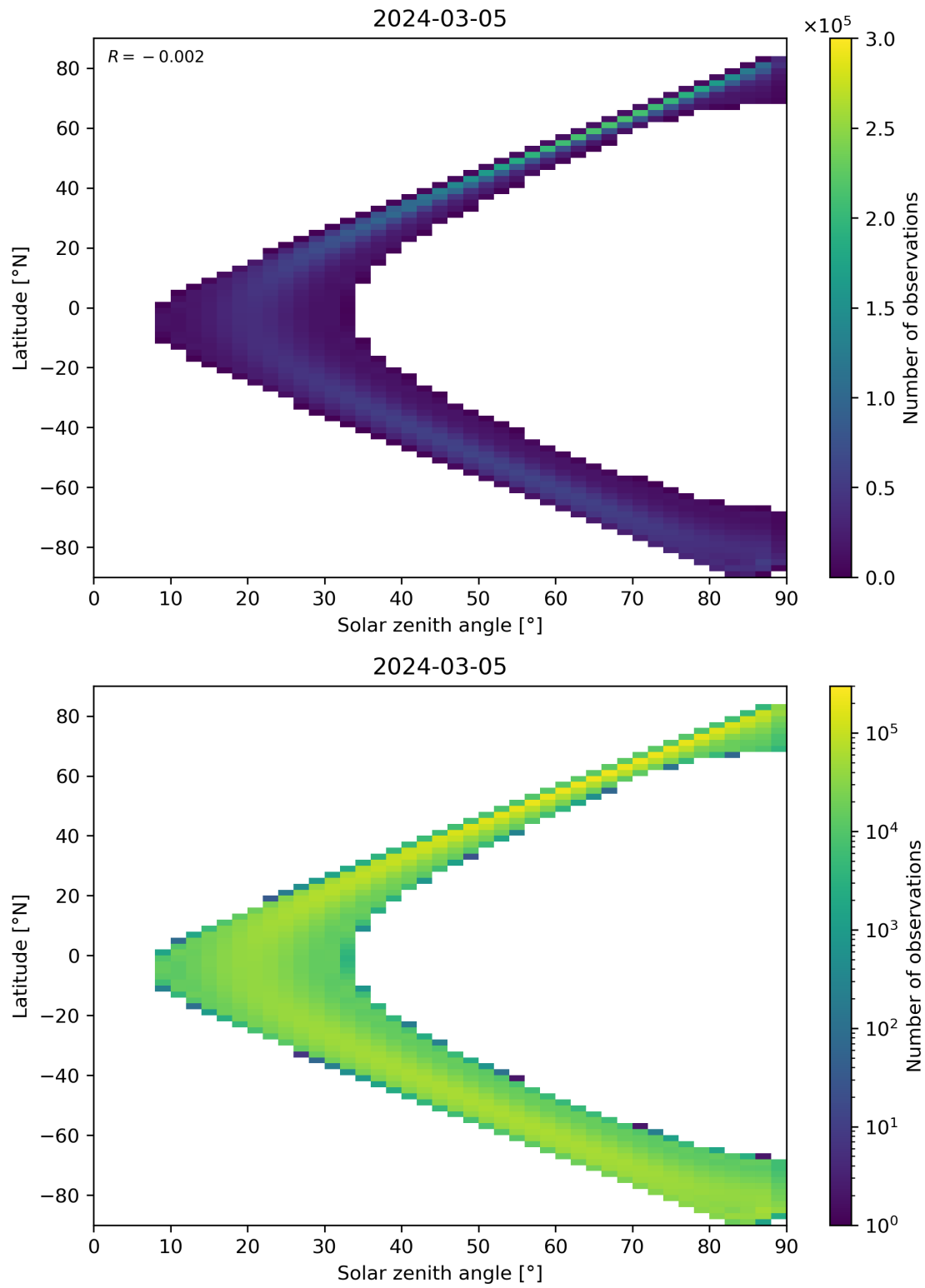
Figure 44: Scatter density plot of “Solar zenith angle” against “Latitude” for 2024-03-04 to 2024-03-06.
