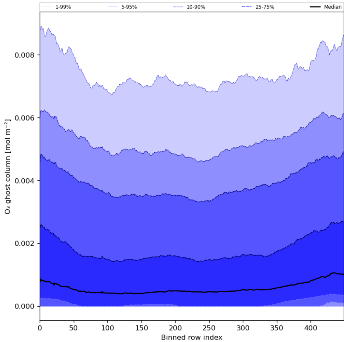
Figure 32: Along track statistics of “O 3 ghost column” for 2024-03-04 to 2024-03-06
