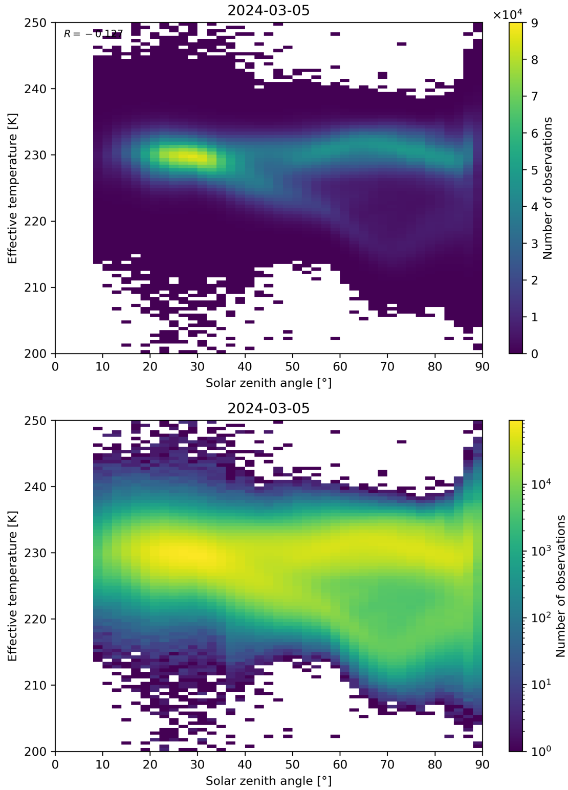
Figure 45: Scatter density plot of “Solar zenith angle” against “Effective temperature” for 2024-03-04 to 2024-03-06.
