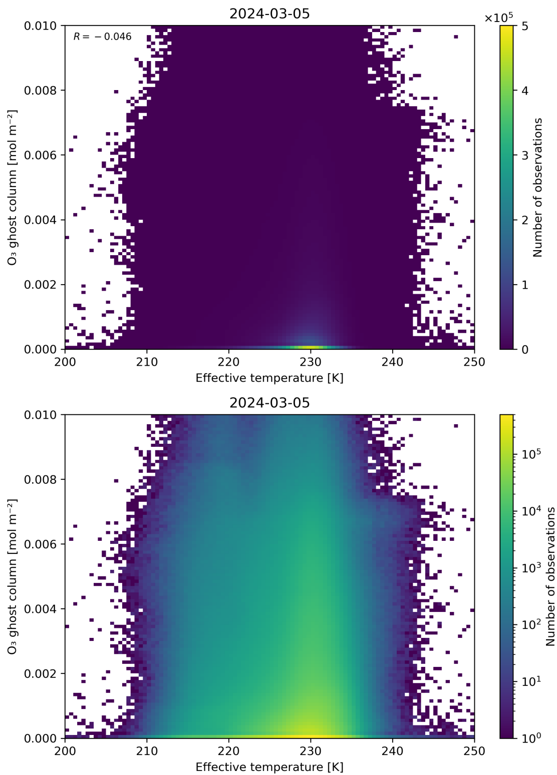
Figure 38: Scatter density plot of “Effective temperature” against “O 3 ghost column” for 2024-03-04 to 2024-03-06.
