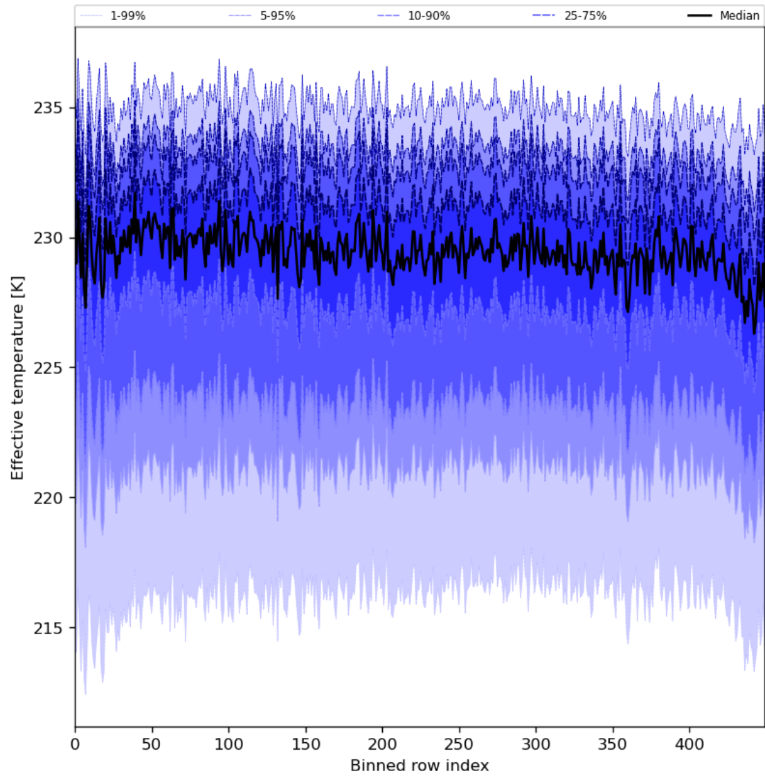
Figure 31: Along track statistics of “Effective temperature” for 2024-03-04 to 2024-03-06
