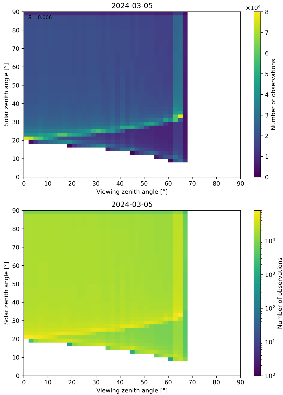
Figure 54: Scatter density plot of “Viewing zenith angle” against “Solar zenith angle” for 2024-03-04 to 2024-03-06.
