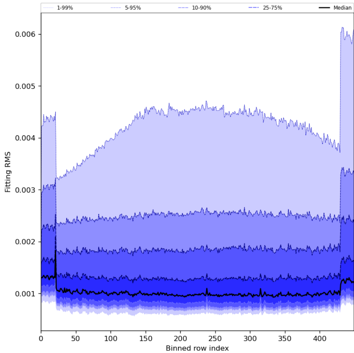
Figure 30: Along track statistics of “Fitting RMS” for 2024-03-04 to 2024-03-06
