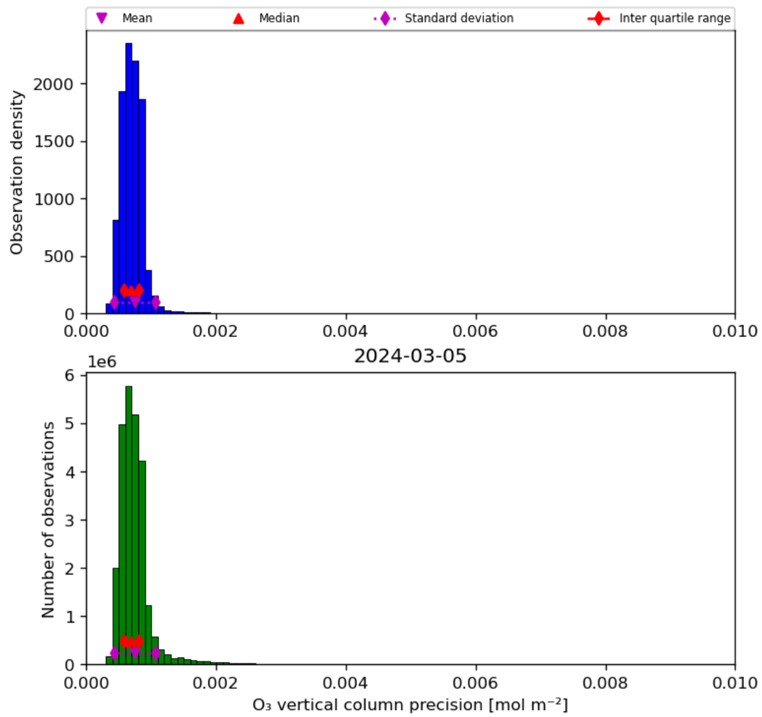
Figure 22: Histogram of “O 3 vertical column precision” for 2024-03-04 to 2024-03-06
