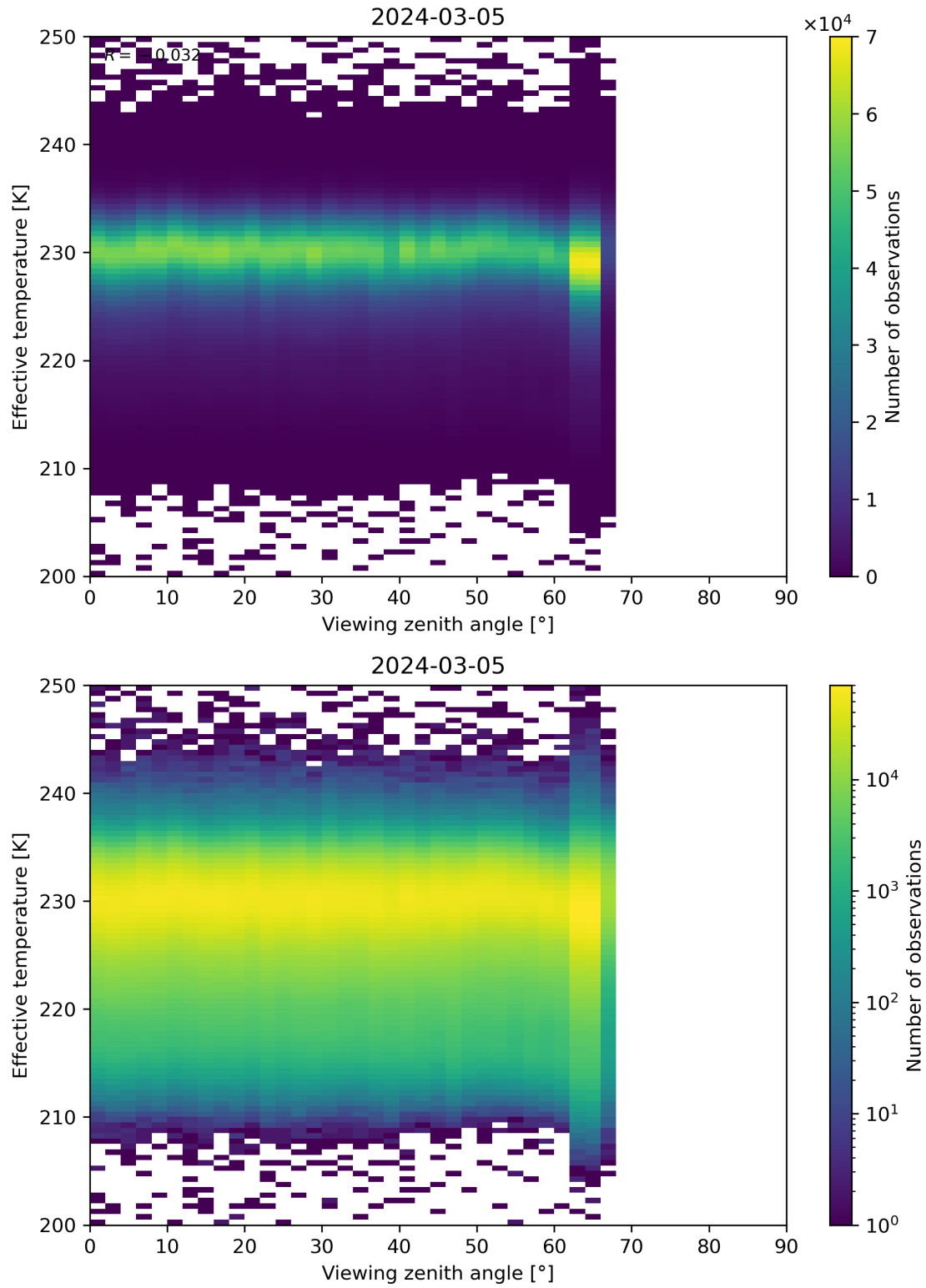
Figure 50: Scatter density plot of “Viewing zenith angle” against “Effective temperature” for 2024-03-04 to 2024-03-06.
