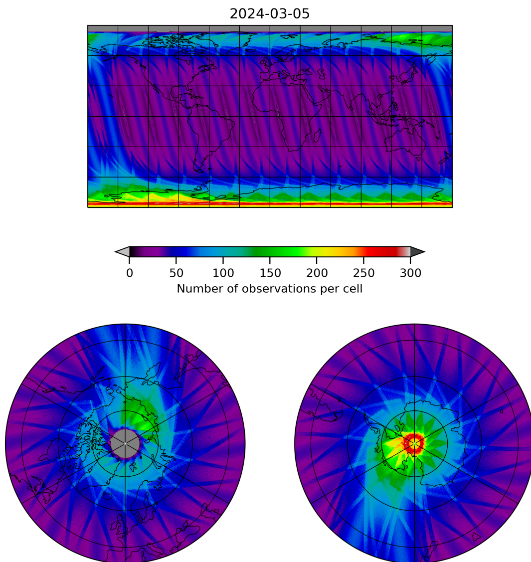
Figure 12: Map of the number of observations for 2024-03-04 to 2024-03-06
