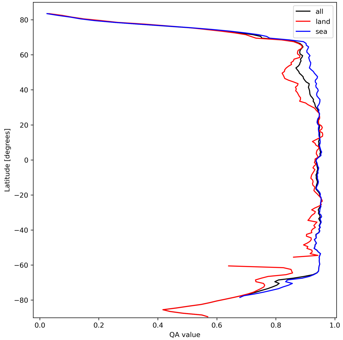
Figure 13: Zonal average of “QA value” for 2024-03-04 to 2024-03-06.
