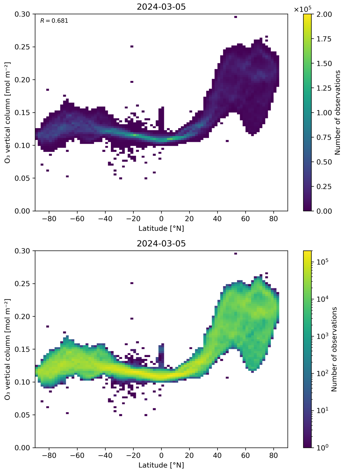
Figure 36: Scatter density plot of “Latitude” against “O 3 vertical column” for 2024-03-04 to 2024-03-06.
