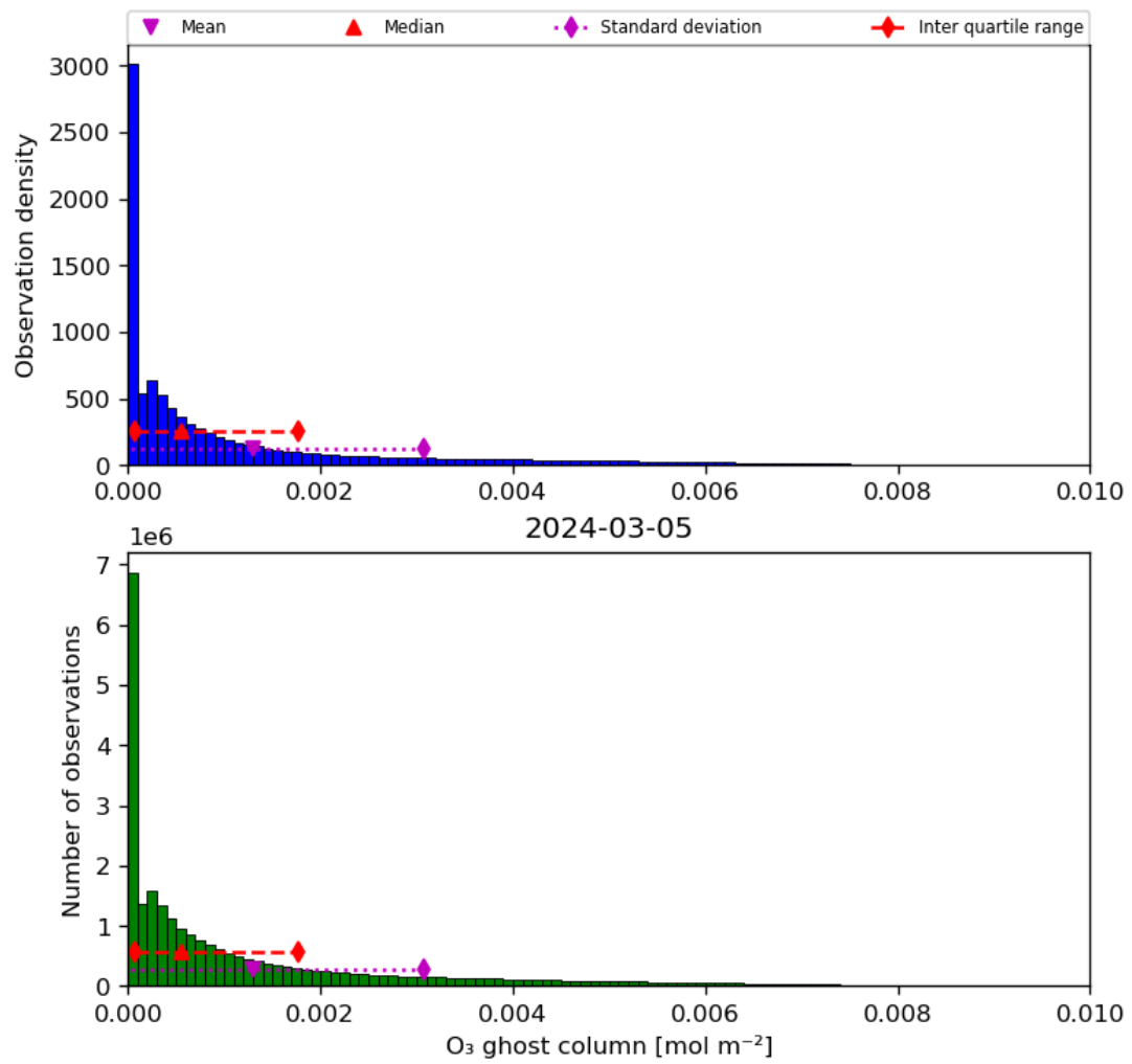
Figure 25: Histogram of “O 3 ghost column” for 2024-03-04 to 2024-03-06
