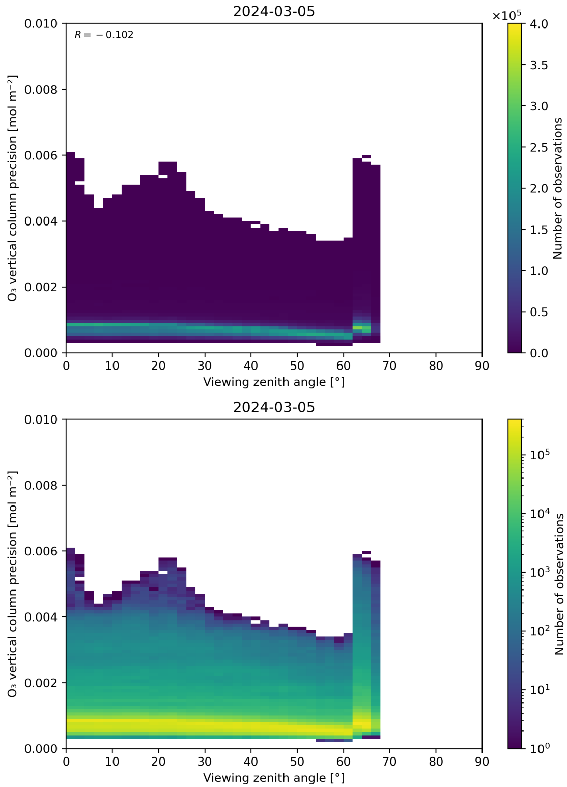
Figure 53: Scatter density plot of “Viewing zenith angle” against “O 3 vertical column precision” for 2024-03-04 to 2024-03-06.
