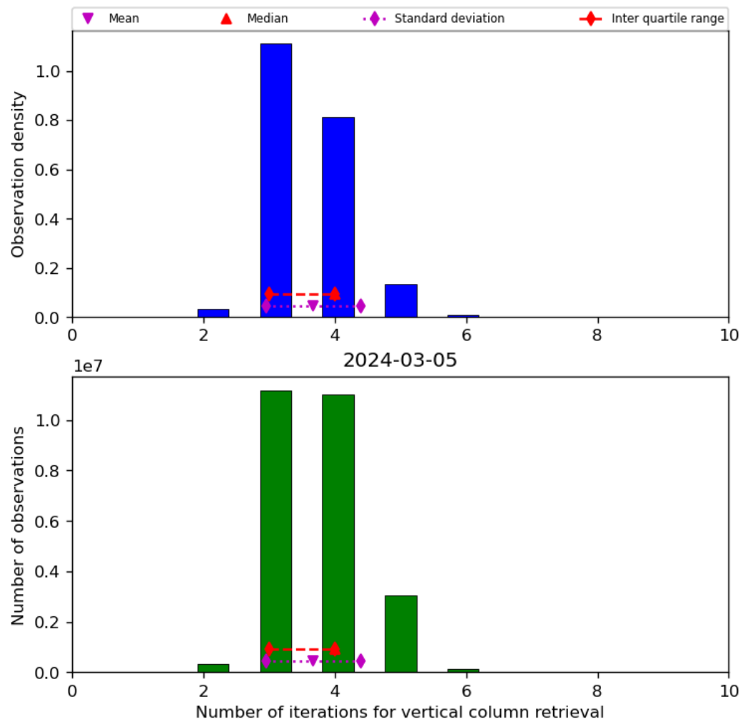
Figure 26: Histogram of “Number of iterations for vertical column retrieval” for 2024-03-04 to 2024-03-06
