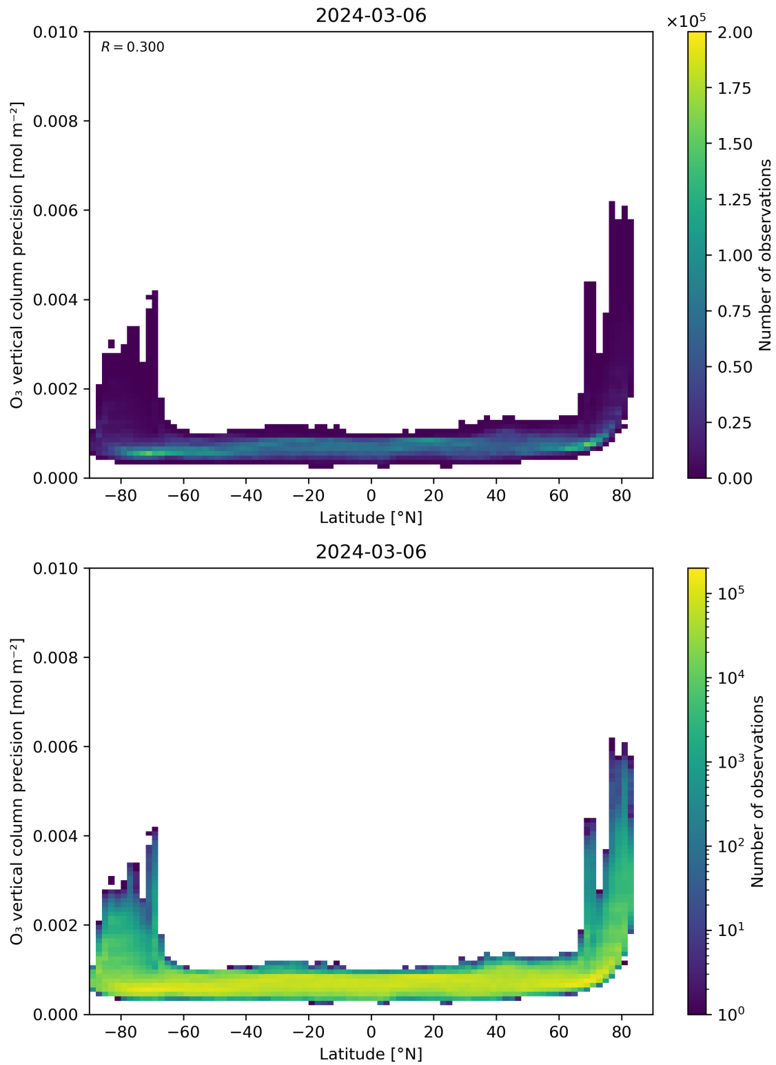
Figure 37: Scatter density plot of “Latitude” against “O 3 vertical column precision” for 2024-03-05 to 2024-03-07.
