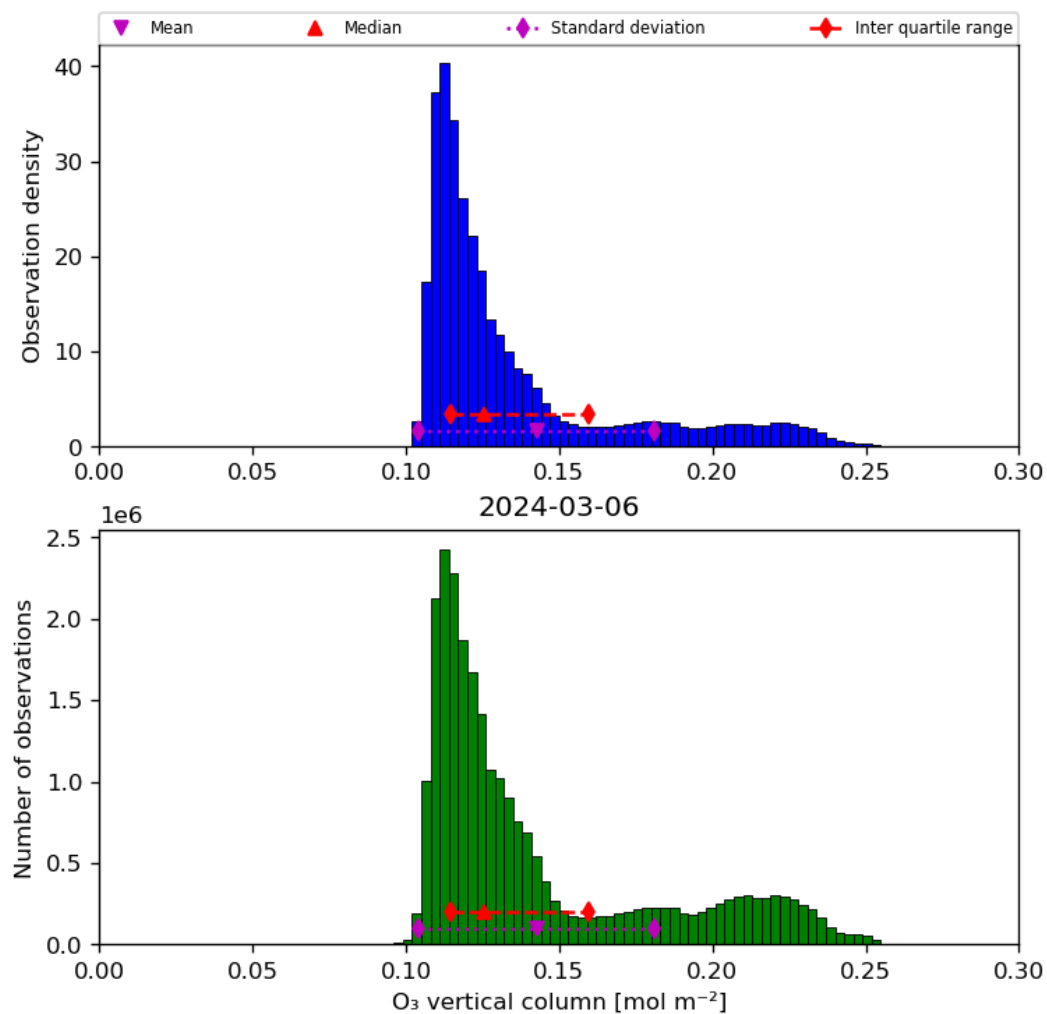
Figure 21: Histogram of “O 3 vertical column” for 2024-03-05 to 2024-03-07
