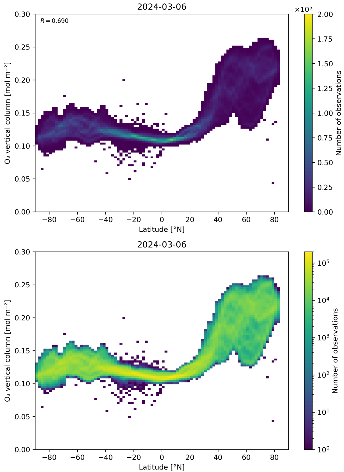
Figure 36: Scatter density plot of “Latitude” against “O 3 vertical column” for 2024-03-05 to 2024-03-07.
