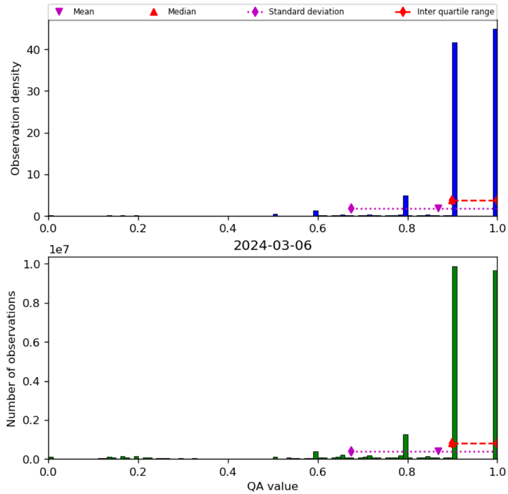
Figure 20: Histogram of “QA value” for 2024-03-05 to 2024-03-07
