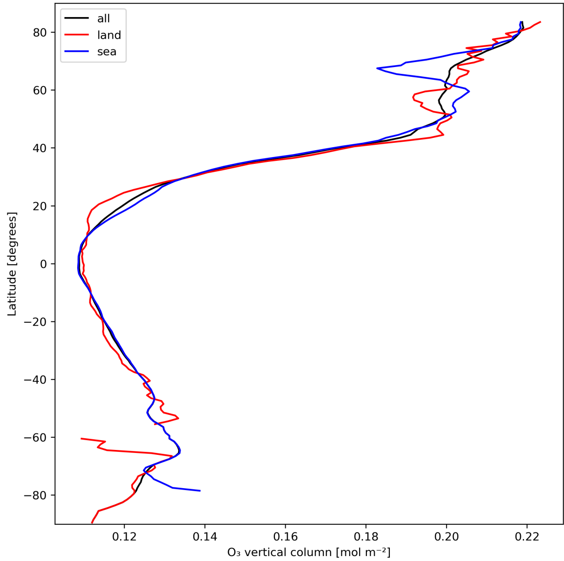
Figure 14: Zonal average of “O 3 vertical column” for 2024-03-05 to 2024-03-07.
