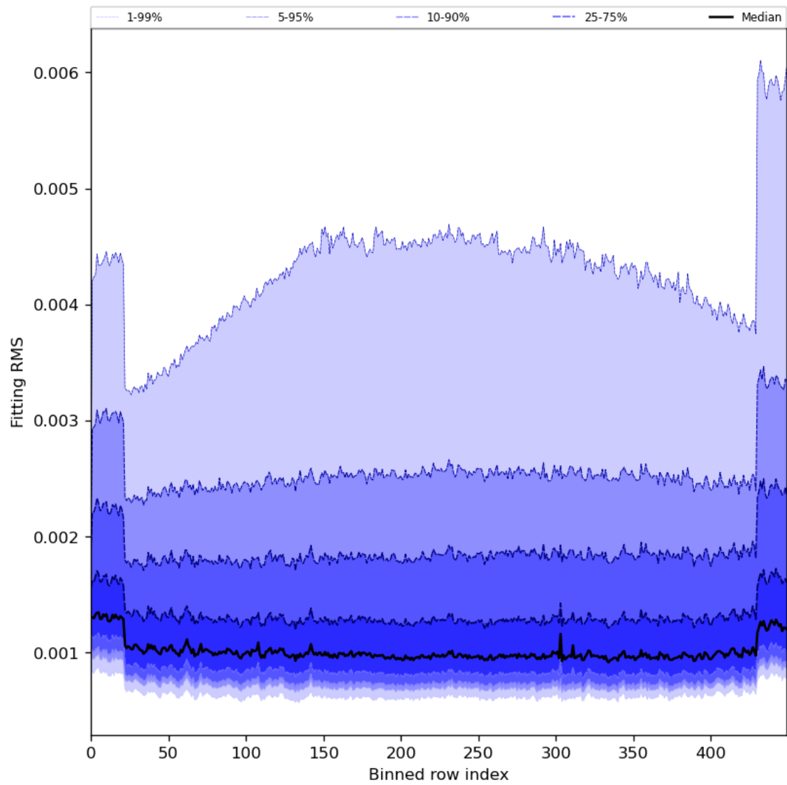
Figure 30: Along track statistics of “Fitting RMS” for 2024-03-05 to 2024-03-07
