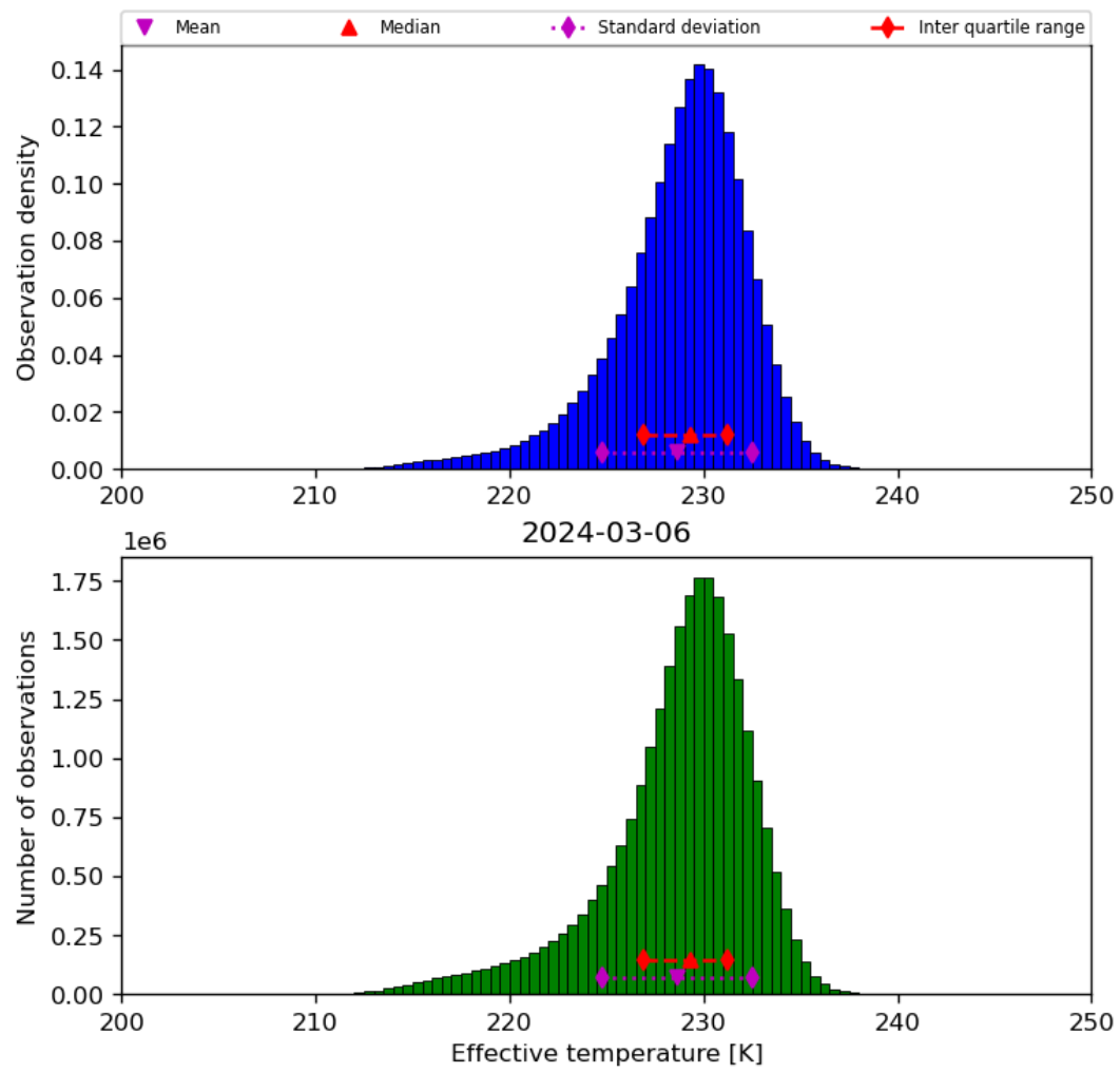
Figure 24: Histogram of “Effective temperature” for 2024-03-05 to 2024-03-07
