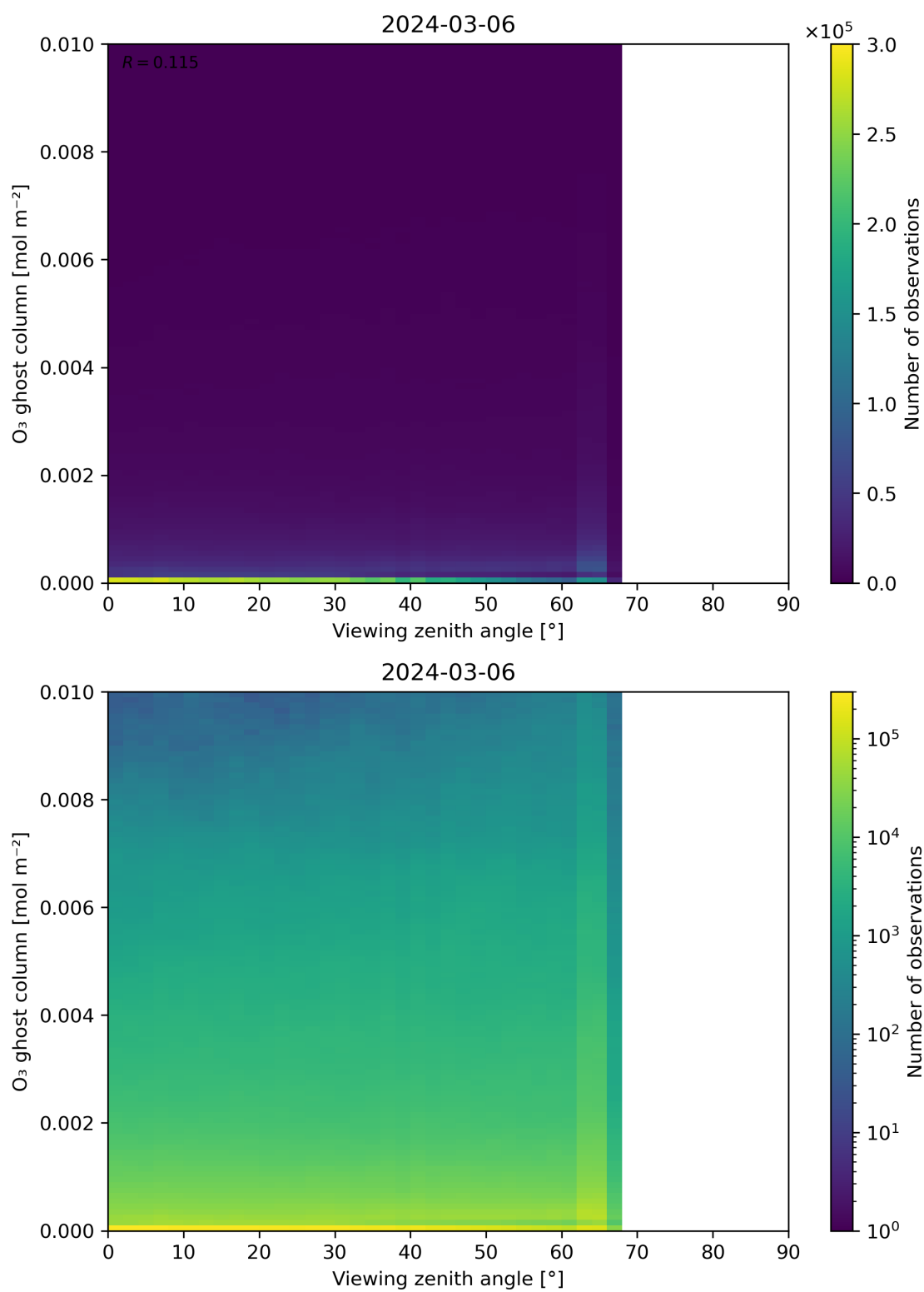
Figure 51: Scatter density plot of “Viewing zenith angle” against “O 3 ghost column” for 2024-03-05 to 2024-03-07.
