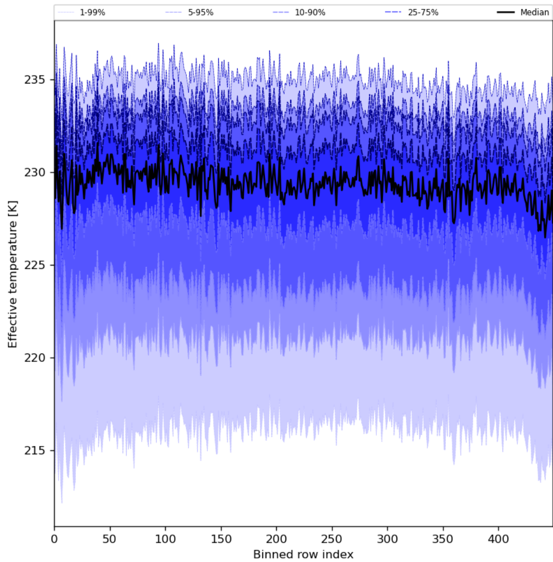
Figure 31: Along track statistics of “Effective temperature” for 2024-03-05 to 2024-03-07
