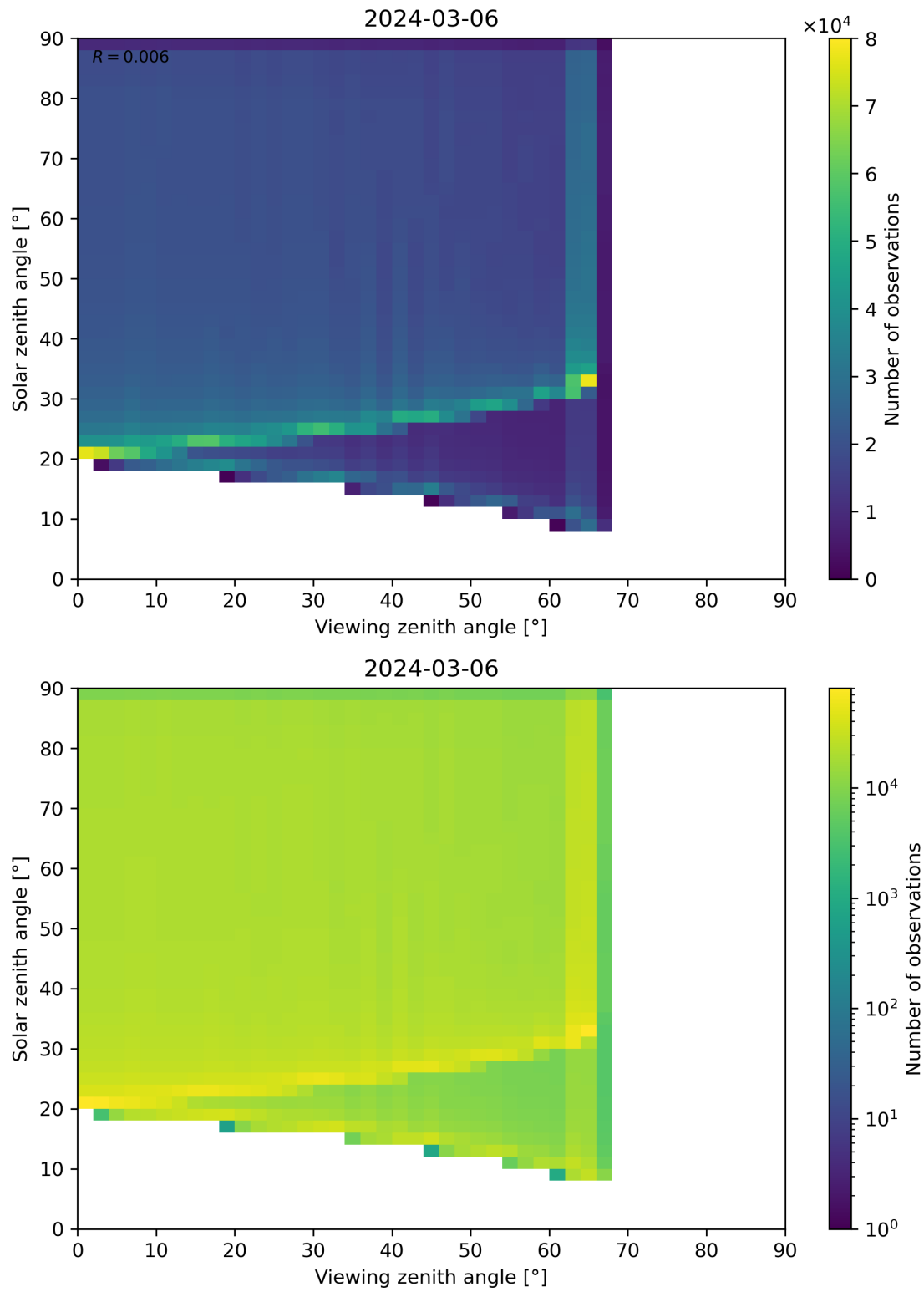
Figure 54: Scatter density plot of “Viewing zenith angle” against “Solar zenith angle” for 2024-03-05 to 2024-03-07.
