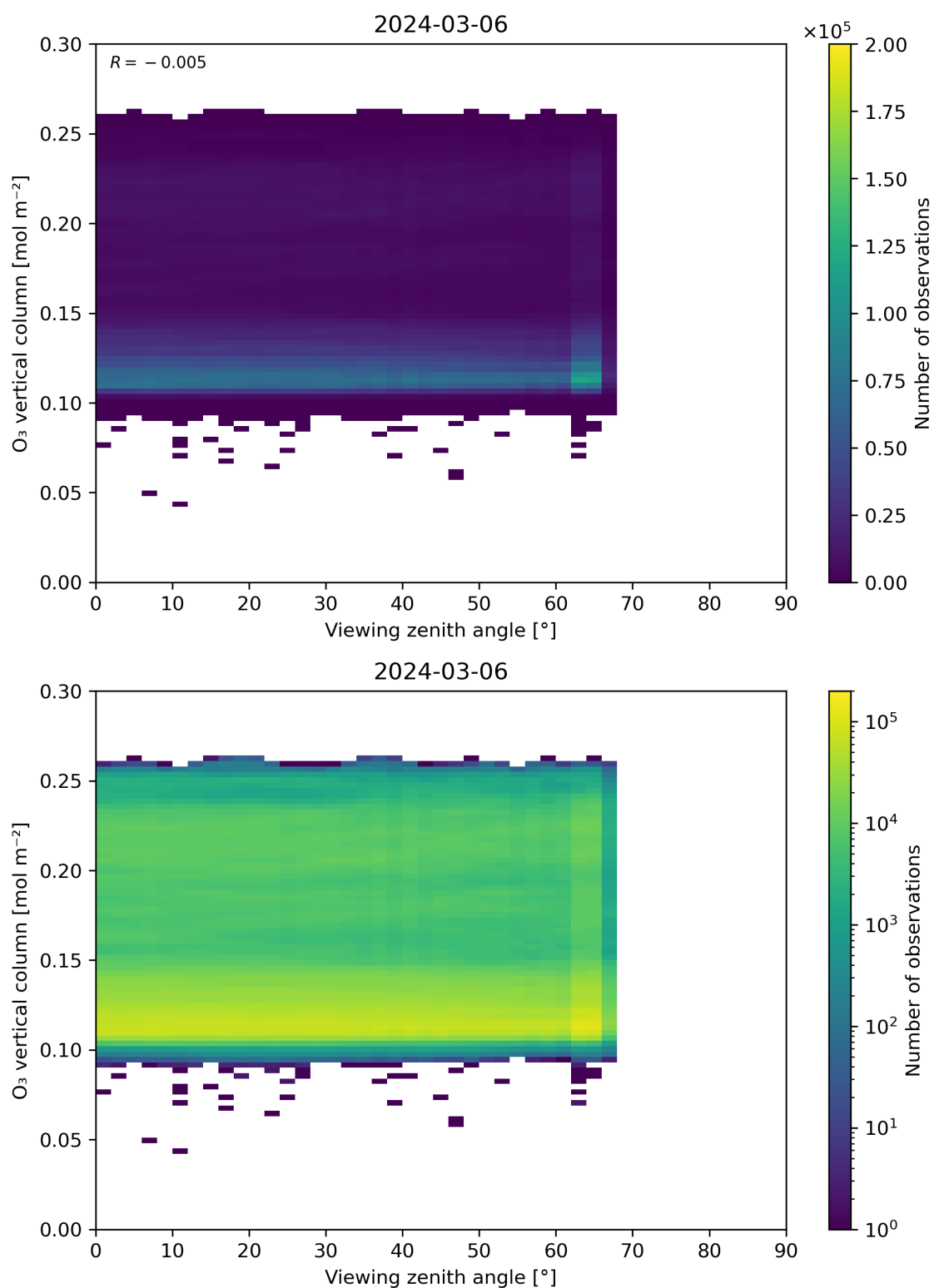
Figure 52: Scatter density plot of “Viewing zenith angle” against “O 3 vertical column” for 2024-03-05 to 2024-03-07.
