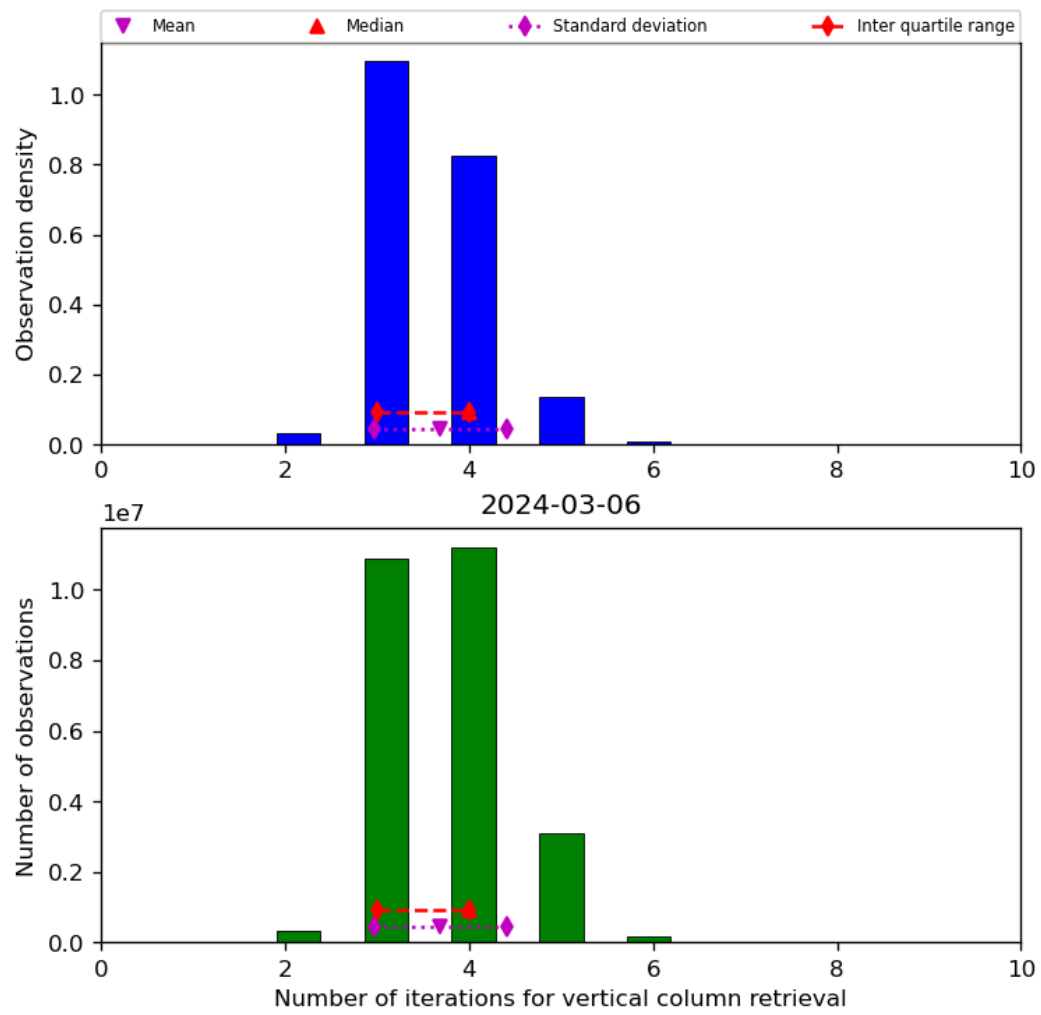
Figure 26: Histogram of “Number of iterations for vertical column retrieval” for 2024-03-05 to 2024-03-07
