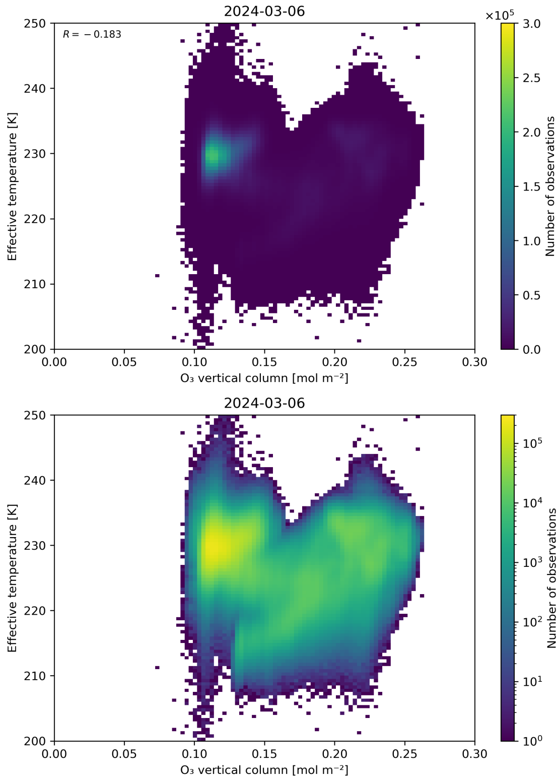
Figure 39: Scatter density plot of “O 3 vertical column” against “Effective temperature” for 2024-03-05 to 2024-03-07.
