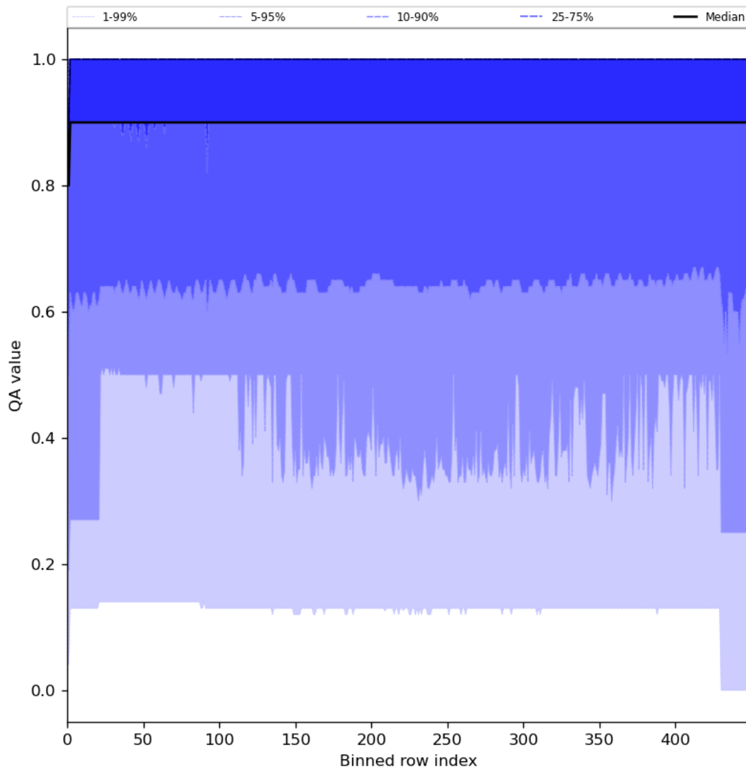
Figure 27: Along track statistics of “QA value” for 2024-03-05 to 2024-03-07
