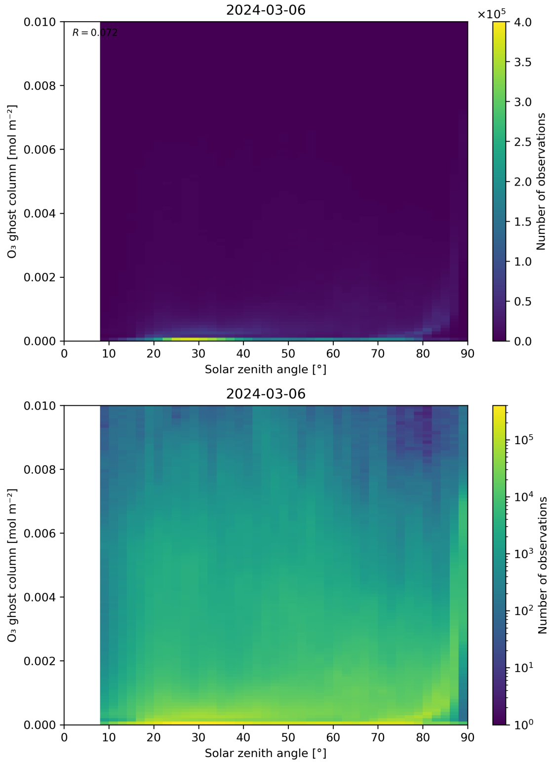
Figure 46: Scatter density plot of “Solar zenith angle” against “O 3 ghost column” for 2024-03-05 to 2024-03-07.
