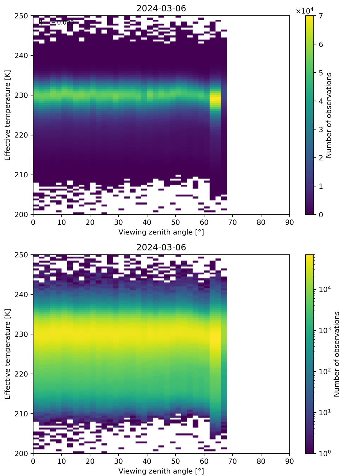
Figure 50: Scatter density plot of “Viewing zenith angle” against “Effective temperature” for 2024-03-05 to 2024-03-07.
