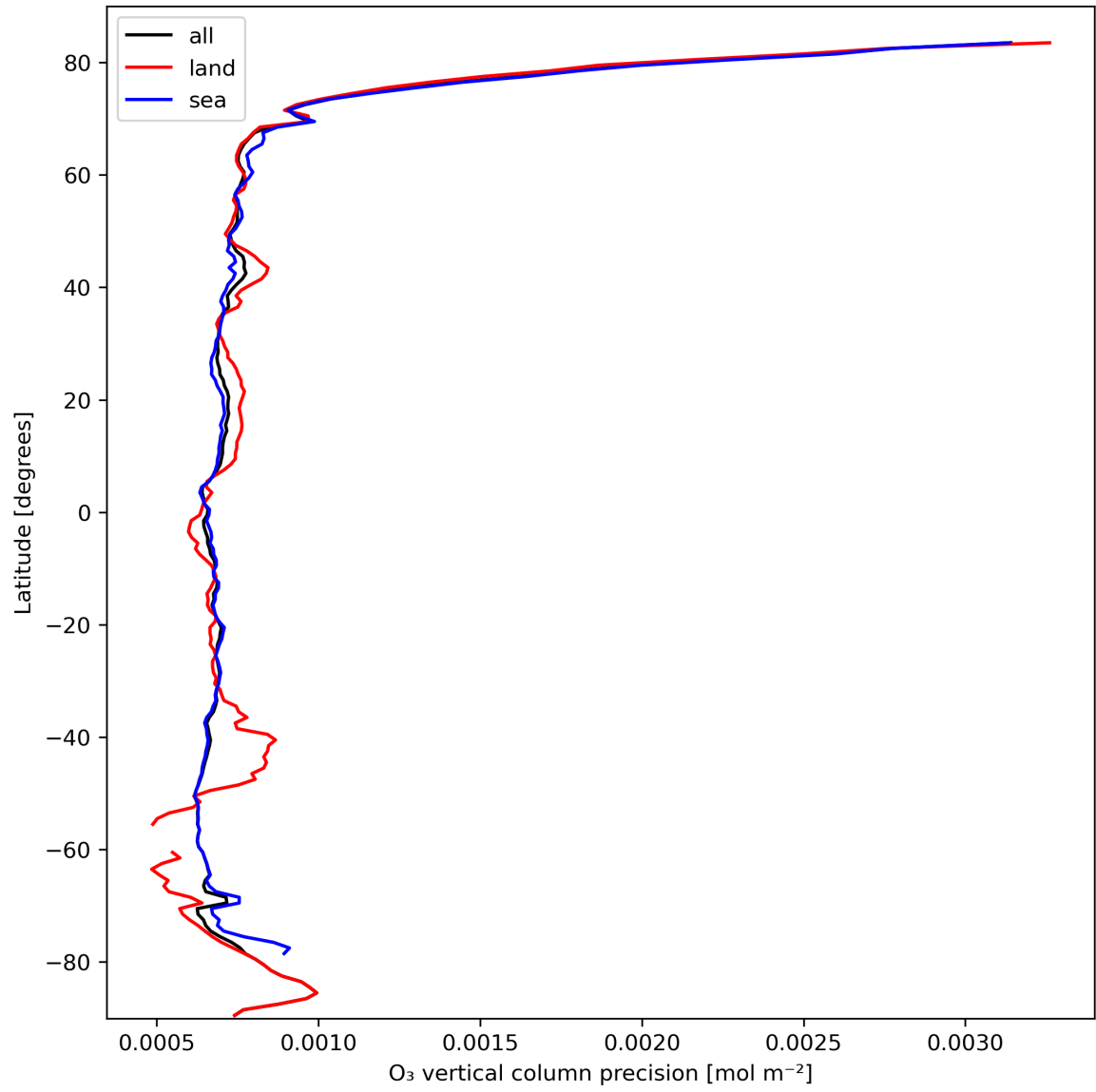
Figure 15: Zonal average of “O 3 vertical column precision” for 2024-03-05 to 2024-03-07.
