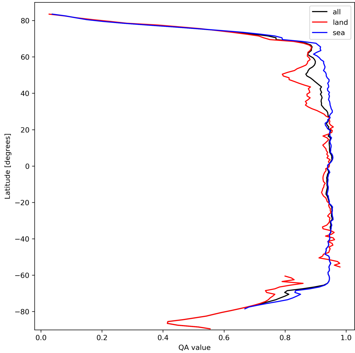
Figure 13: Zonal average of “QA value” for 2024-03-05 to 2024-03-07.
