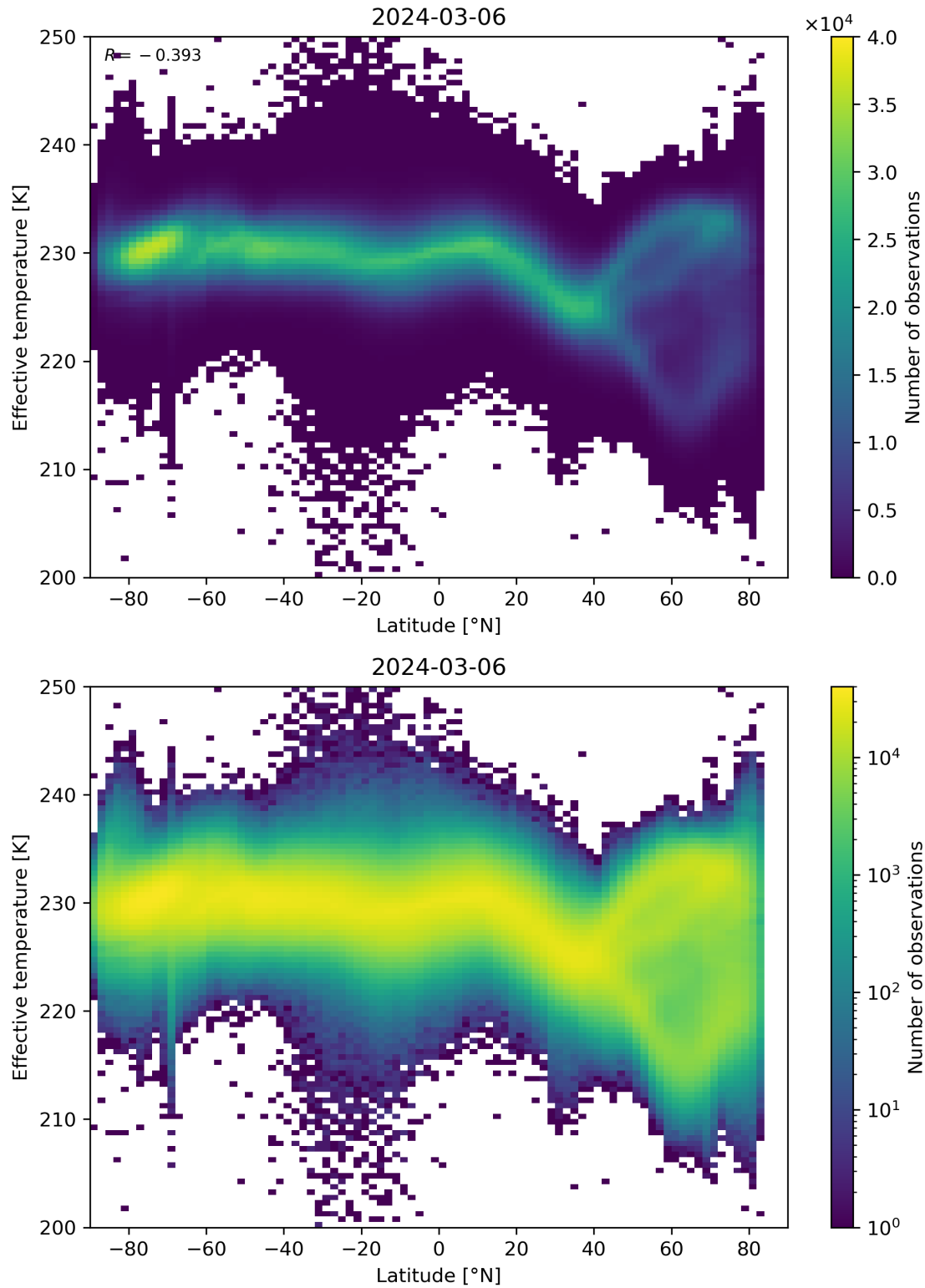
Figure 34: Scatter density plot of “Latitude” against “Effective temperature” for 2024-03-05 to 2024-03-07.
