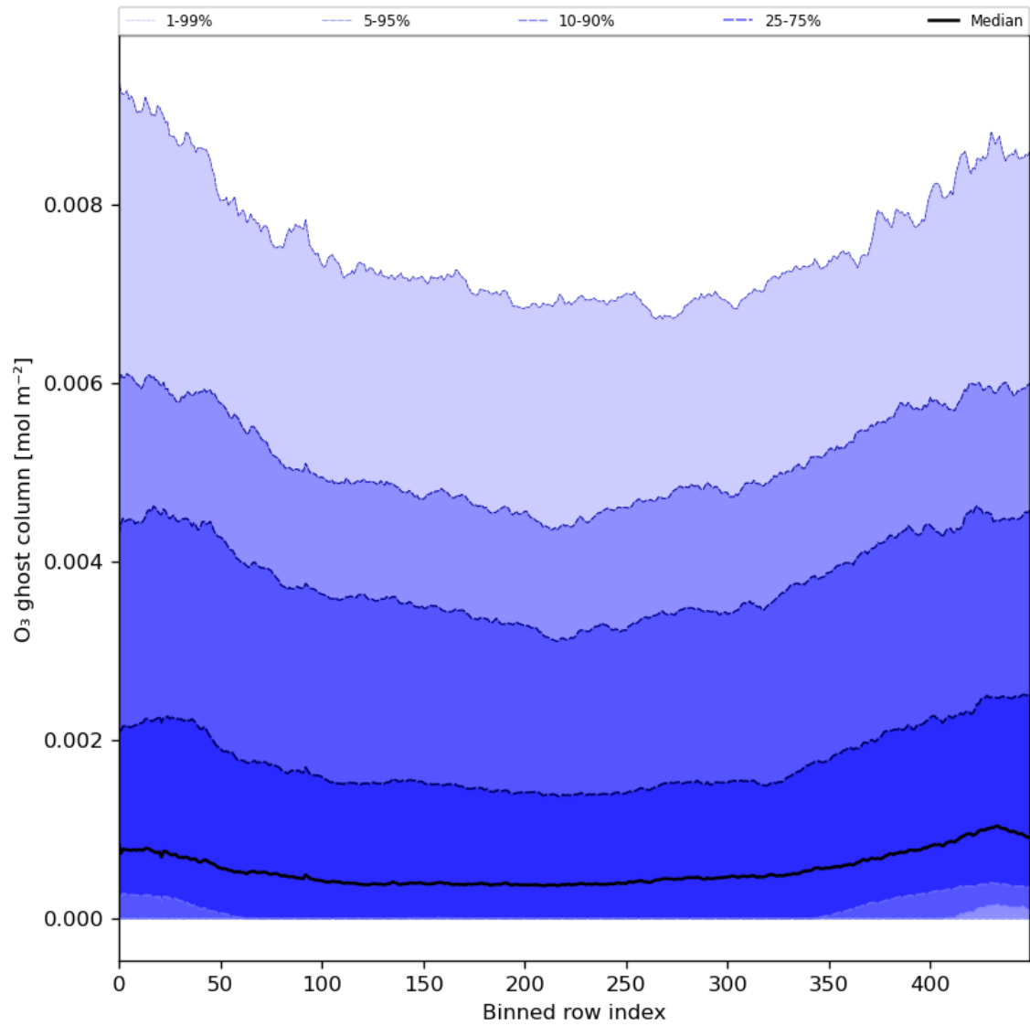
Figure 32: Along track statistics of “O 3 ghost column” for 2024-03-05 to 2024-03-07
