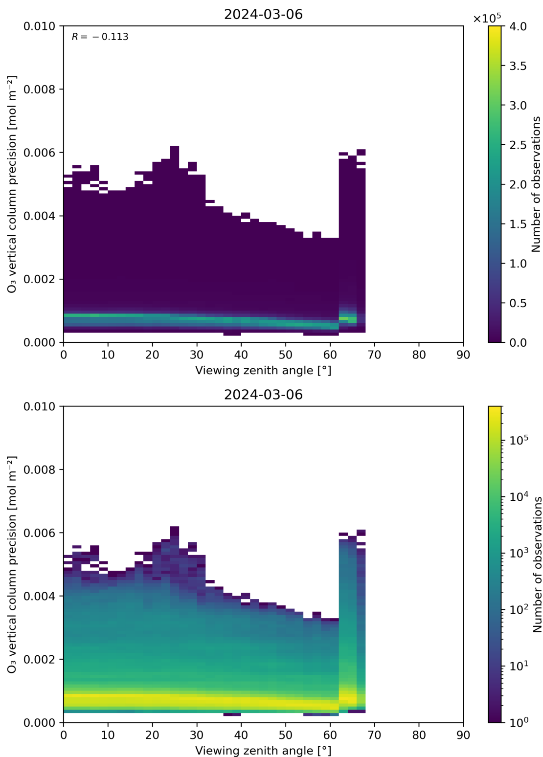
Figure 53: Scatter density plot of “Viewing zenith angle” against “O 3 vertical column precision” for 2024-03-05 to 2024-03-07.
