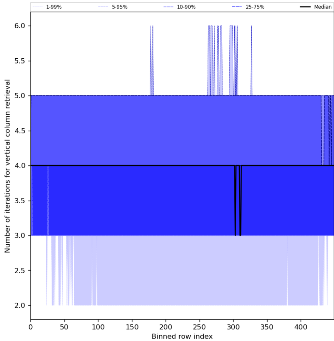
Figure 33: Along track statistics of “Number of iterations for vertical column retrieval” for 2024-03-05 to 2024-03-07
