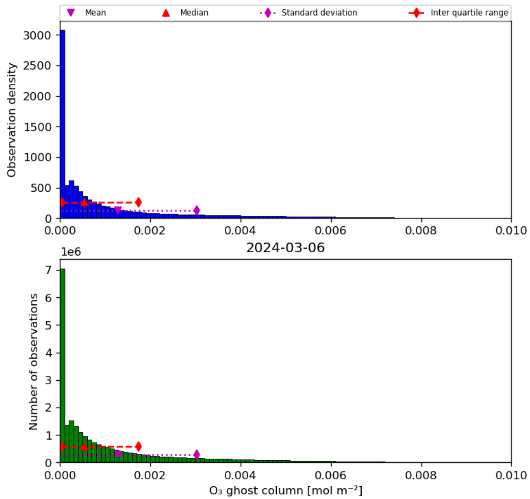
Figure 25: Histogram of “O 3 ghost column” for 2024-03-05 to 2024-03-07
