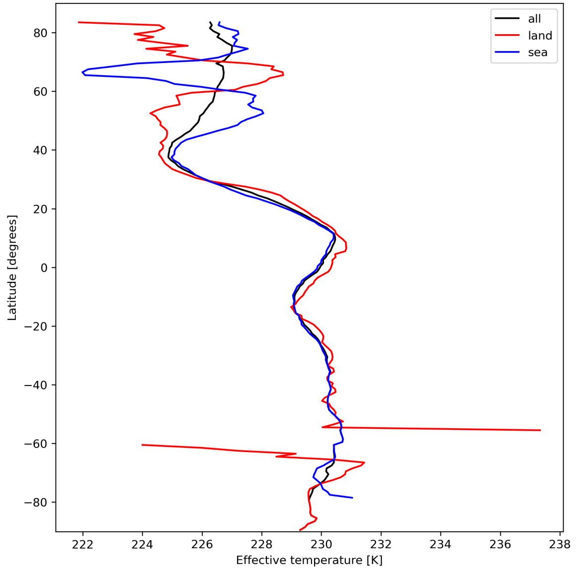
Figure 17: Zonal average of “Effective temperature” for 2024-03-05 to 2024-03-07.
