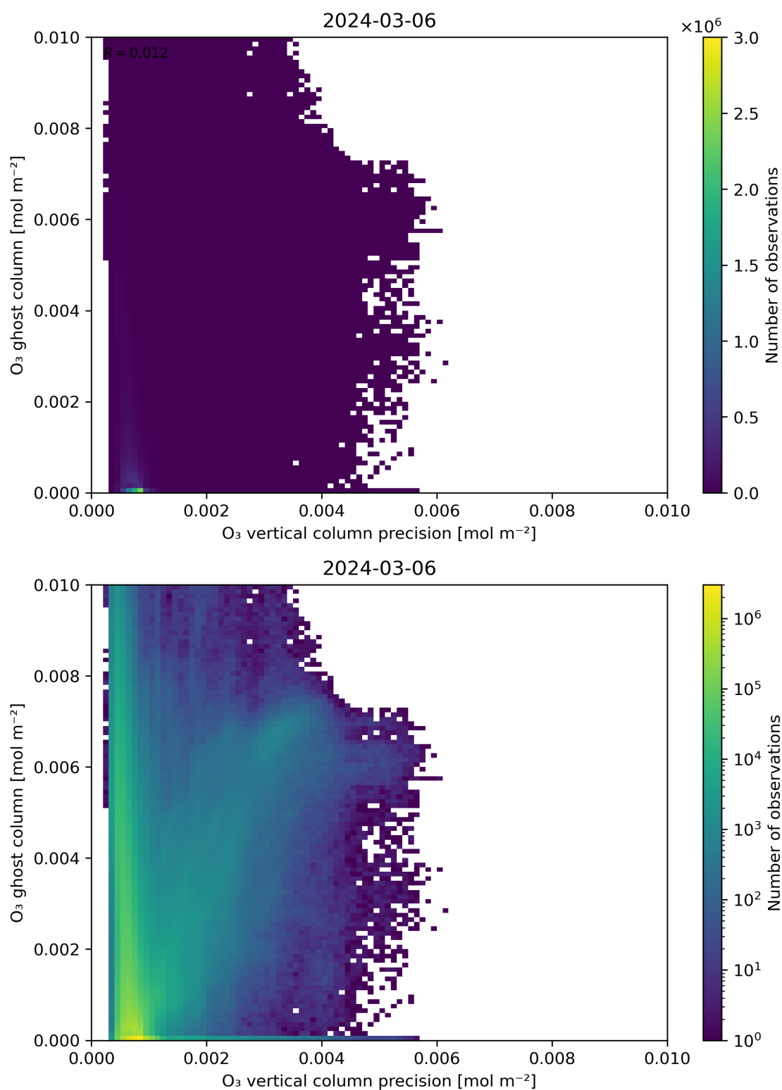
Figure 43: Scatter density plot of “O 3 vertical column precision” against “O 3 ghost column” for 2024-03-05 to 2024-03-07.
