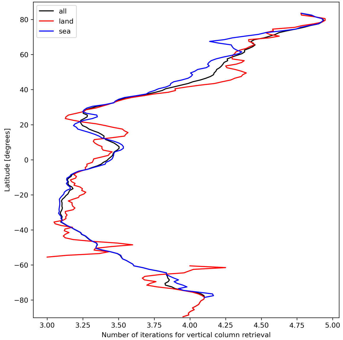
Figure 19: Zonal average of “Number of iterations for vertical column retrieval” for 2024-03-05 to 2024-03-07.
