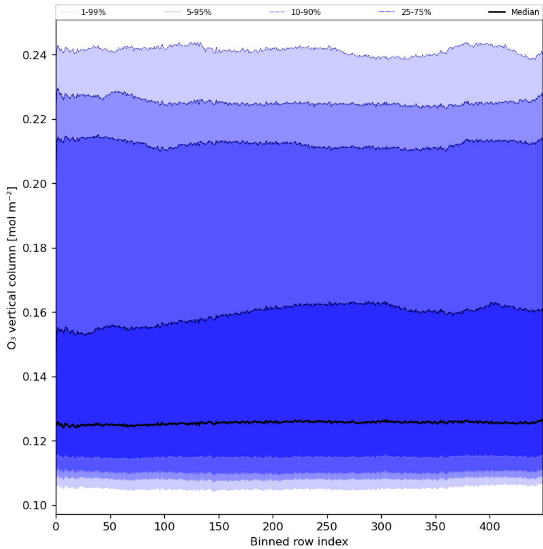
Figure 28: Along track statistics of “O 3 vertical column” for 2024-03-05 to 2024-03-07
