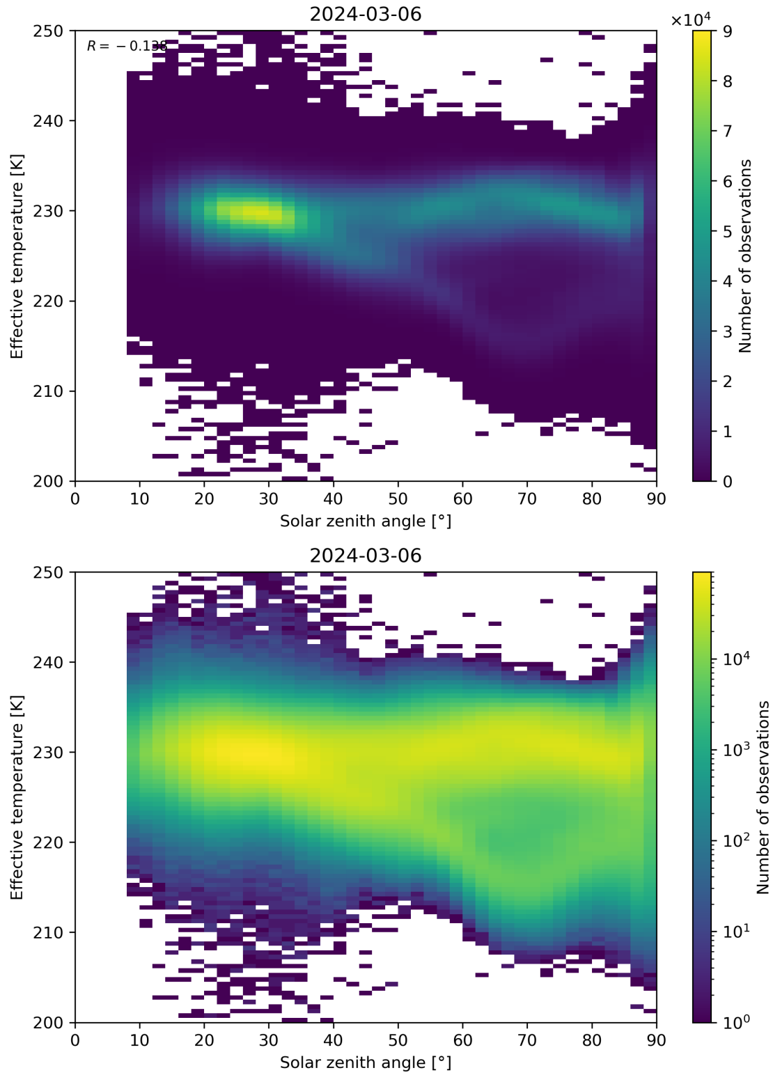
Figure 45: Scatter density plot of “Solar zenith angle” against “Effective temperature” for 2024-03-05 to 2024-03-07.
