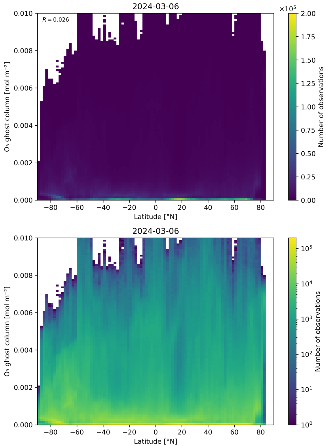
Figure 35: Scatter density plot of “Latitude” against “O 3 ghost column” for 2024-03-05 to 2024-03-07.
