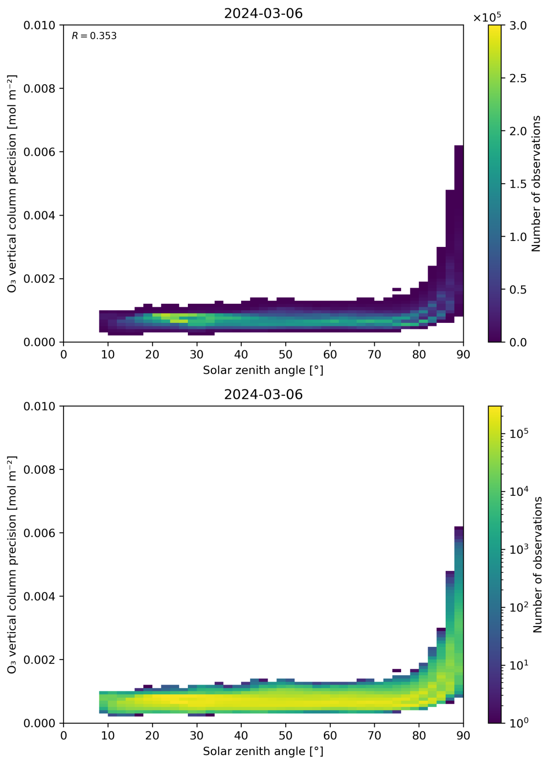
Figure 48: Scatter density plot of “Solar zenith angle” against “O 3 vertical column precision” for 2024-03-05 to 2024-03-07.
