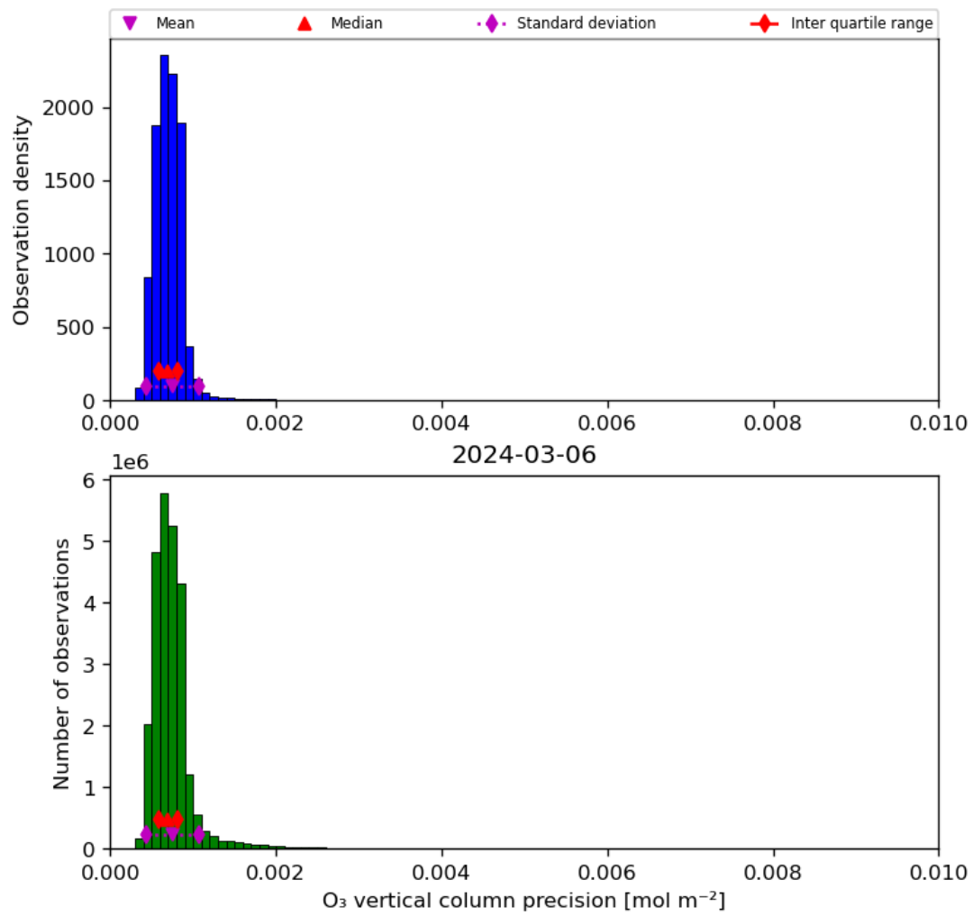
Figure 22: Histogram of “O 3 vertical column precision” for 2024-03-05 to 2024-03-07
