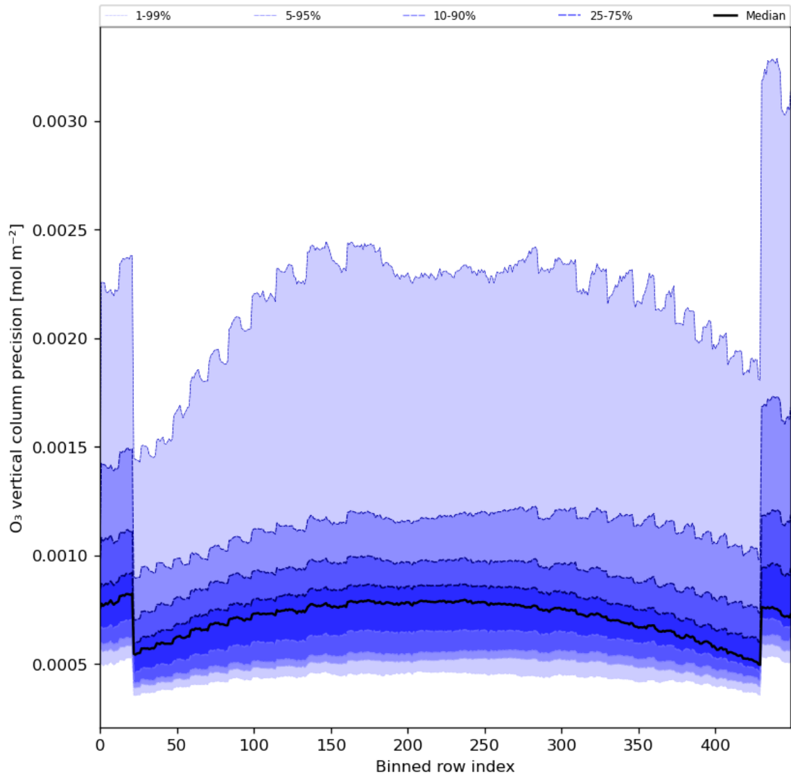
Figure 29: Along track statistics of “O 3 vertical column precision” for 2024-03-05 to 2024-03-07
