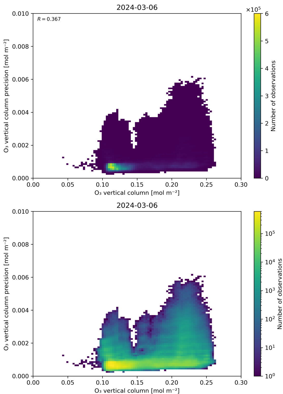
Figure 41: Scatter density plot of “O 3 vertical column” against “O 3 vertical column precision” for 2024-03-05 to 2024-03-07.
