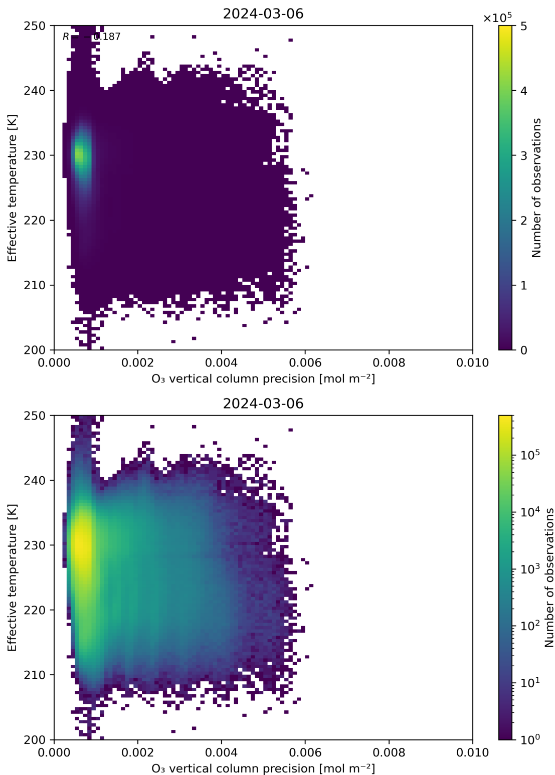
Figure 42: Scatter density plot of “O 3 vertical column precision” against “Effective temperature” for 2024-03-05 to 2024-03-07.
