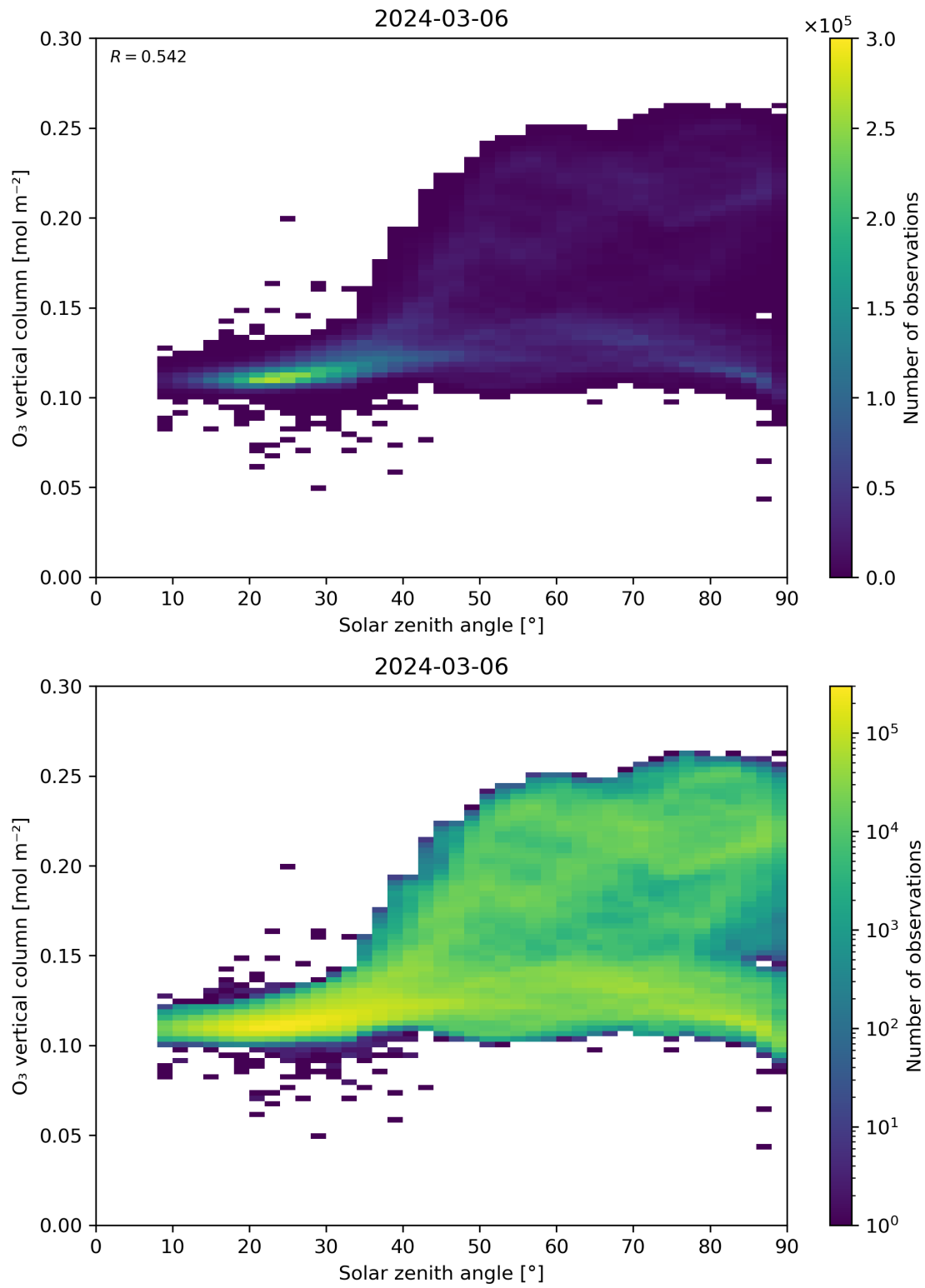
Figure 47: Scatter density plot of “Solar zenith angle” against “O 3 vertical column” for 2024-03-05 to 2024-03-07.
