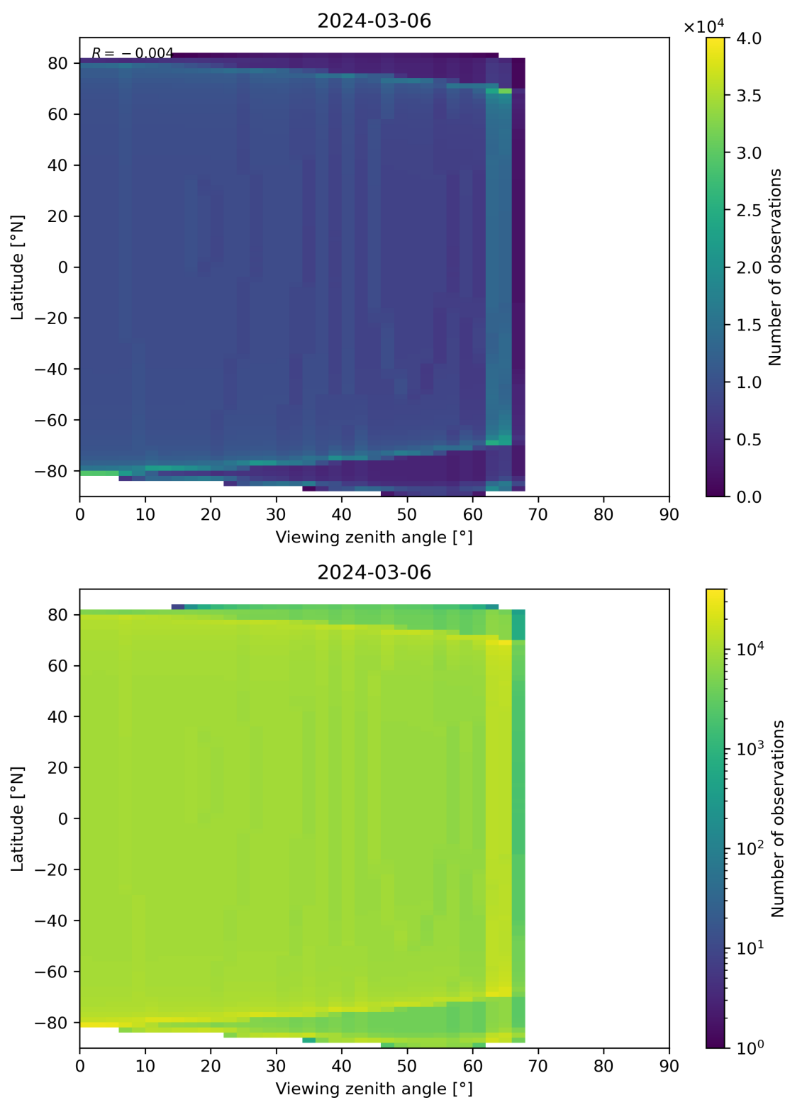
Figure 49: Scatter density plot of “Viewing zenith angle” against “Latitude” for 2024-03-05 to 2024-03-07.
