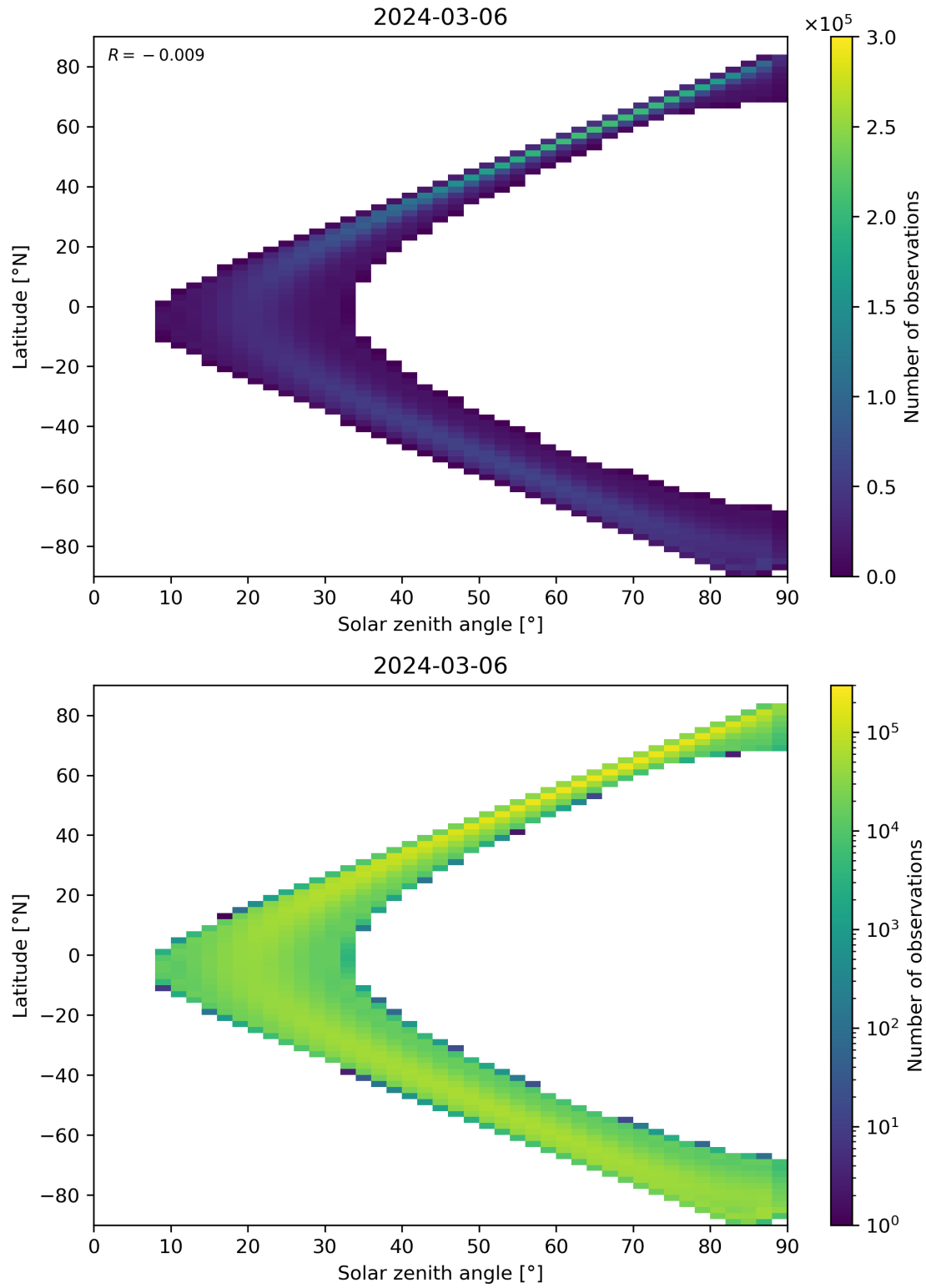
Figure 44: Scatter density plot of “Solar zenith angle” against “Latitude” for 2024-03-05 to 2024-03-07.
