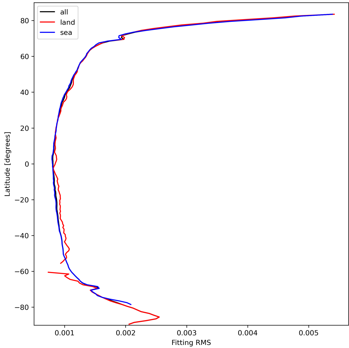
Figure 16: Zonal average of “Fitting RMS” for 2024-03-05 to 2024-03-07.
