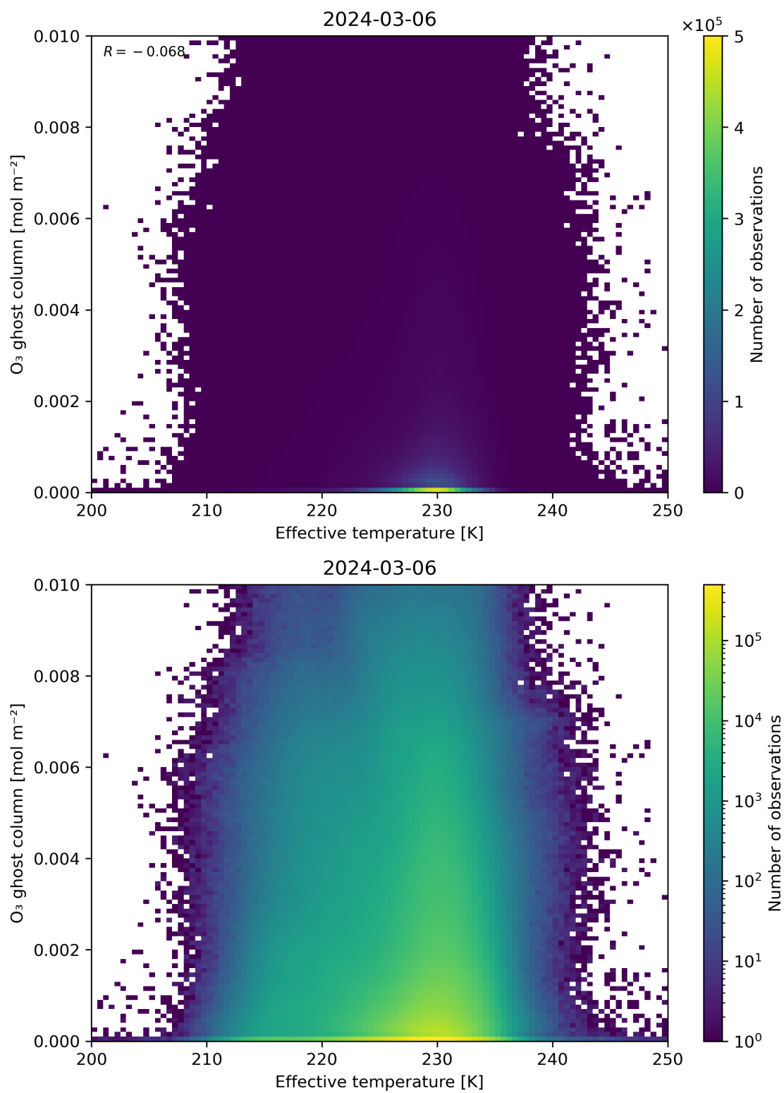
Figure 38: Scatter density plot of “Effective temperature” against “O 3 ghost column” for 2024-03-05 to 2024-03-07.
