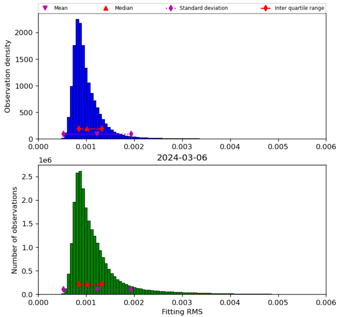
Figure 23: Histogram of “Fitting RMS” for 2024-03-05 to 2024-03-07
