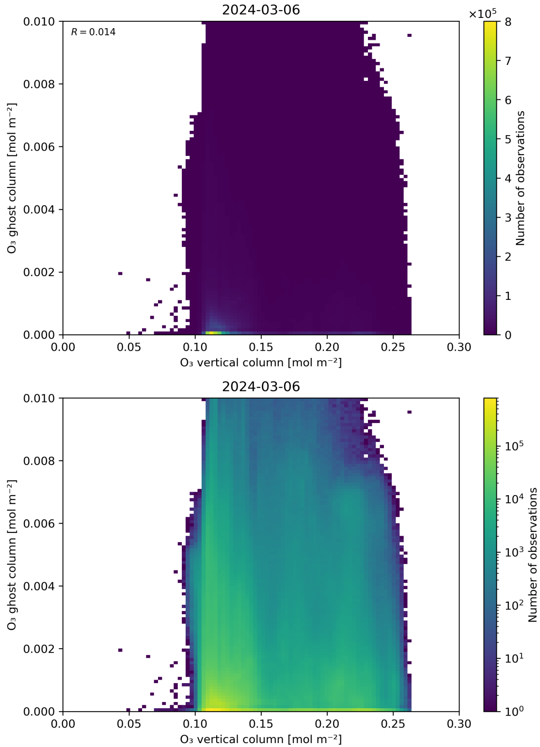
Figure 40: Scatter density plot of “O 3 vertical column” against “O 3 ghost column” for 2024-03-05 to 2024-03-07.
