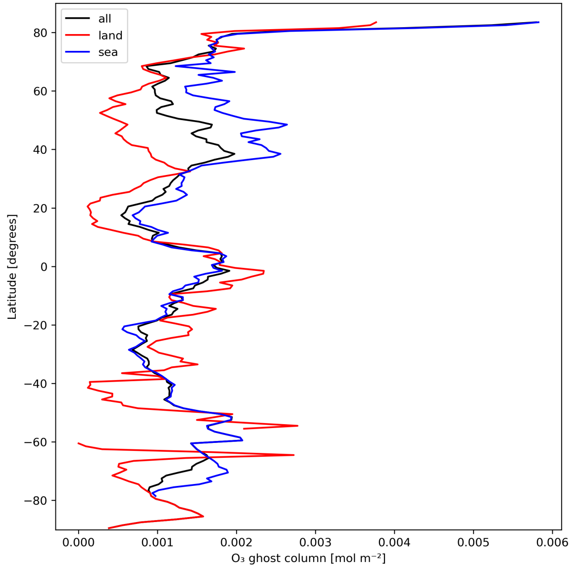
Figure 18: Zonal average of “O 3 ghost column” for 2024-03-05 to 2024-03-07.
