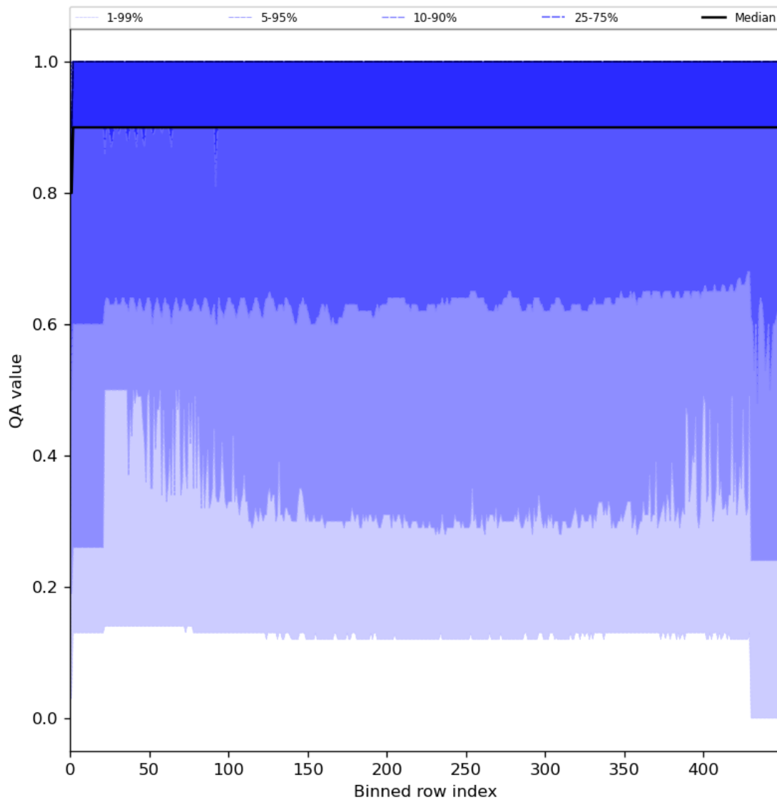
Figure 27: Along track statistics of “QA value” for 2024-03-06 to 2024-03-08
