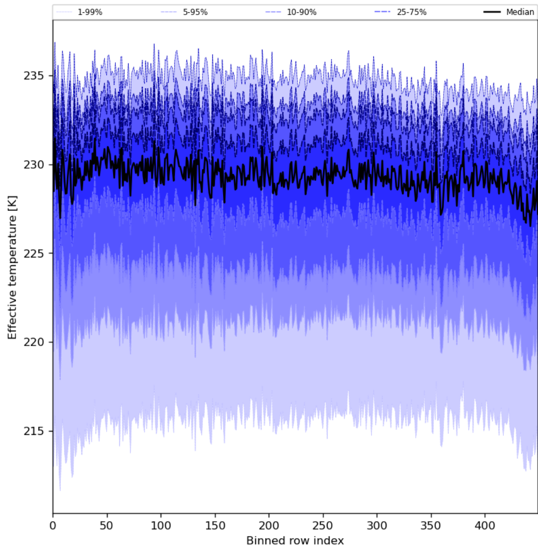
Figure 31: Along track statistics of “Effective temperature” for 2024-03-06 to 2024-03-08
