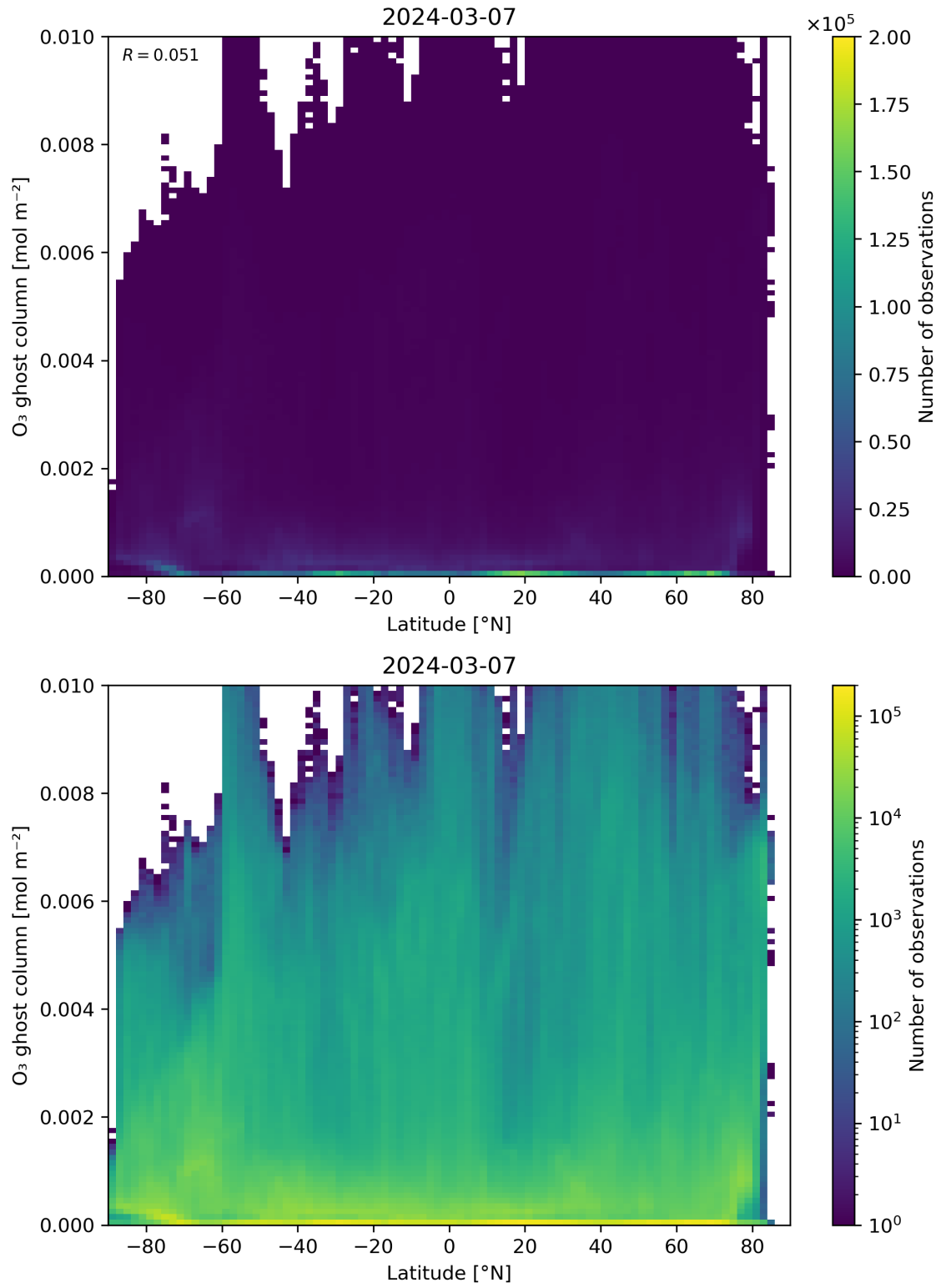
Figure 35: Scatter density plot of “Latitude” against “O 3 ghost column” for 2024-03-06 to 2024-03-08.
