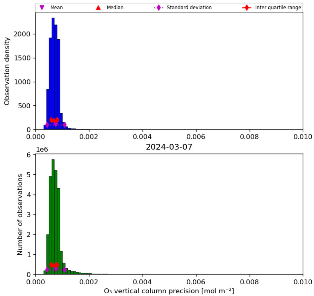
Figure 22: Histogram of “O 3 vertical column precision” for 2024-03-06 to 2024-03-08
