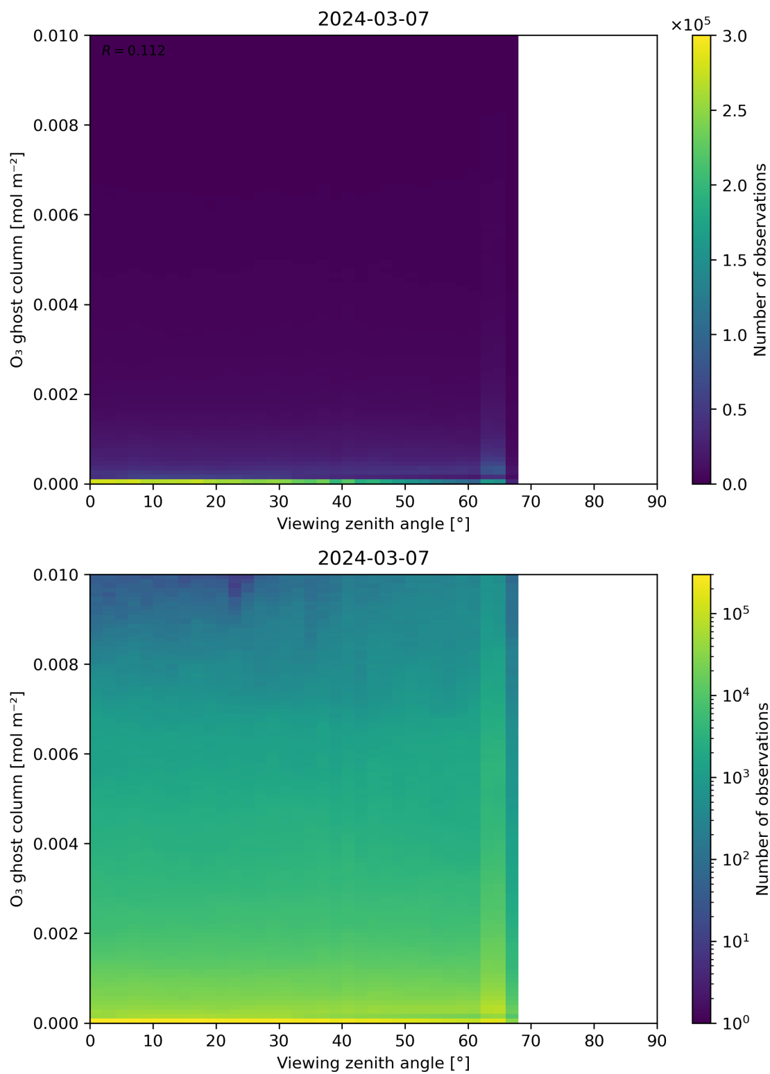
Figure 51: Scatter density plot of “Viewing zenith angle” against “O 3 ghost column” for 2024-03-06 to 2024-03-08.
