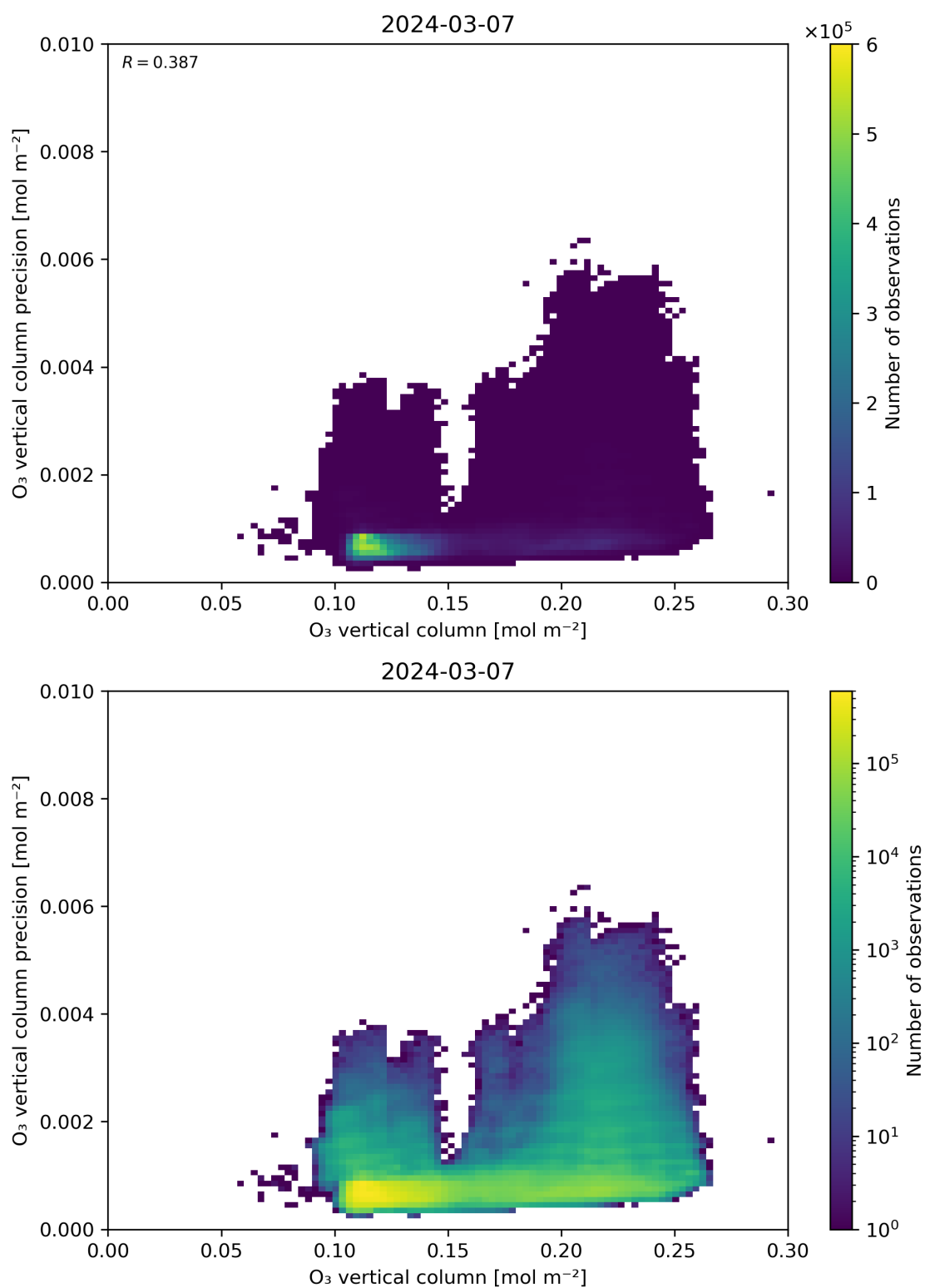
Figure 41: Scatter density plot of “O 3 vertical column” against “O 3 vertical column precision” for 2024-03-06 to 2024-03-08.
