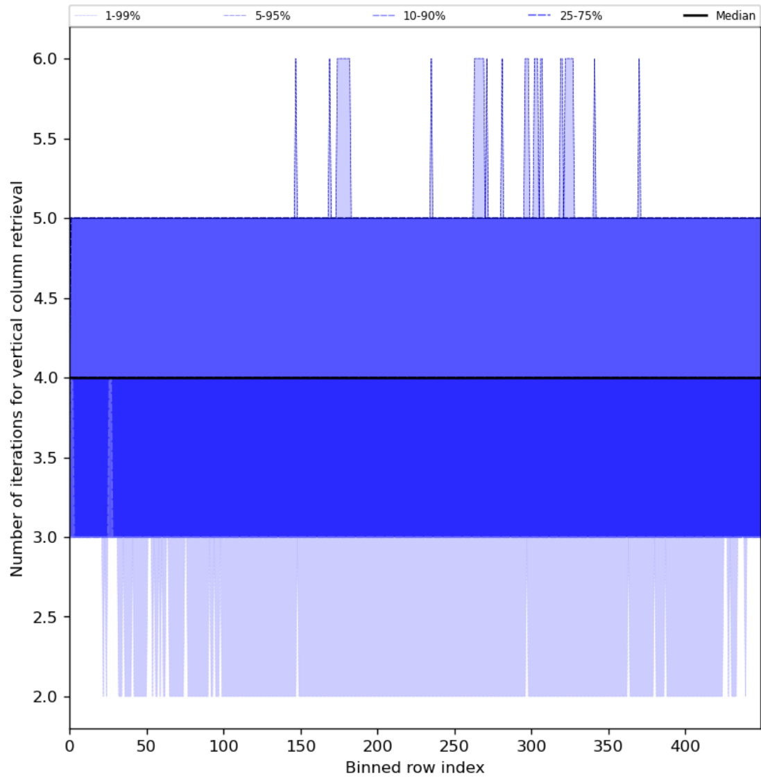
Figure 33: Along track statistics of “Number of iterations for vertical column retrieval” for 2024-03-06 to 2024-03-08
