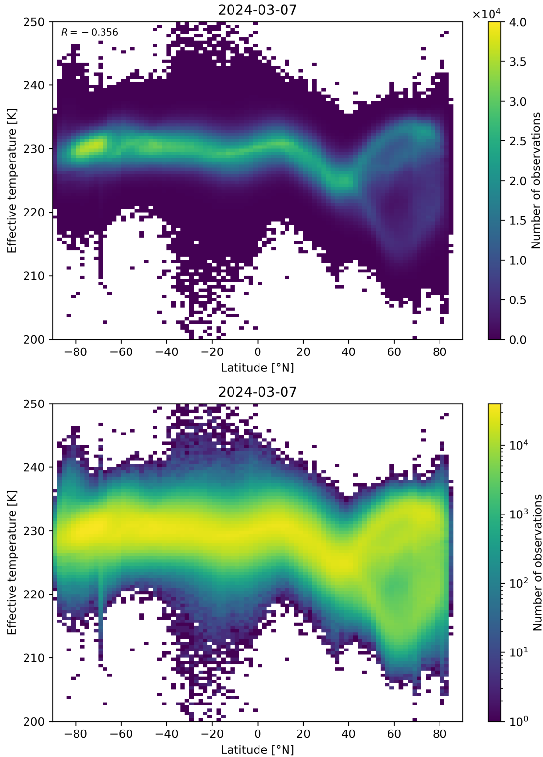
Figure 34: Scatter density plot of “Latitude” against “Effective temperature” for 2024-03-06 to 2024-03-08.
