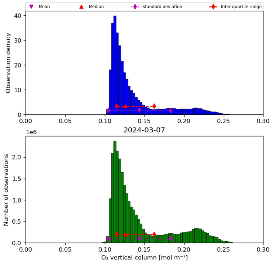
Figure 21: Histogram of “O 3 vertical column” for 2024-03-06 to 2024-03-08
