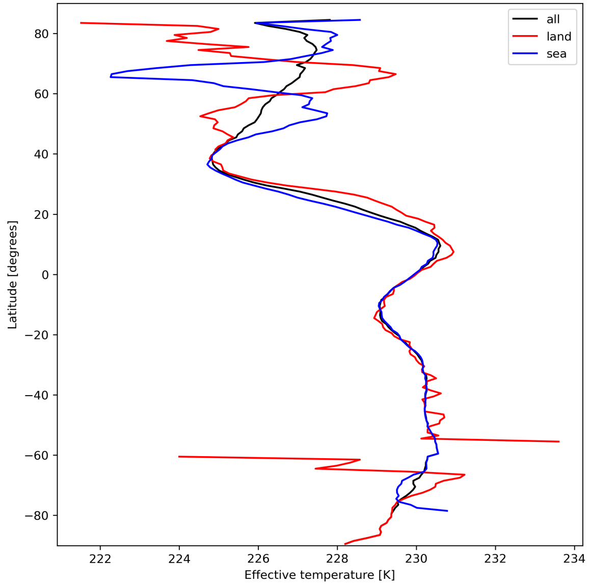
Figure 17: Zonal average of “Effective temperature” for 2024-03-06 to 2024-03-08.
