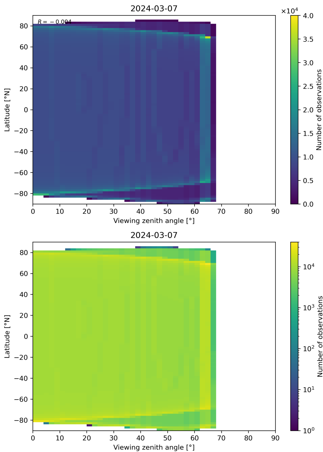
Figure 49: Scatter density plot of “Viewing zenith angle” against “Latitude” for 2024-03-06 to 2024-03-08.
