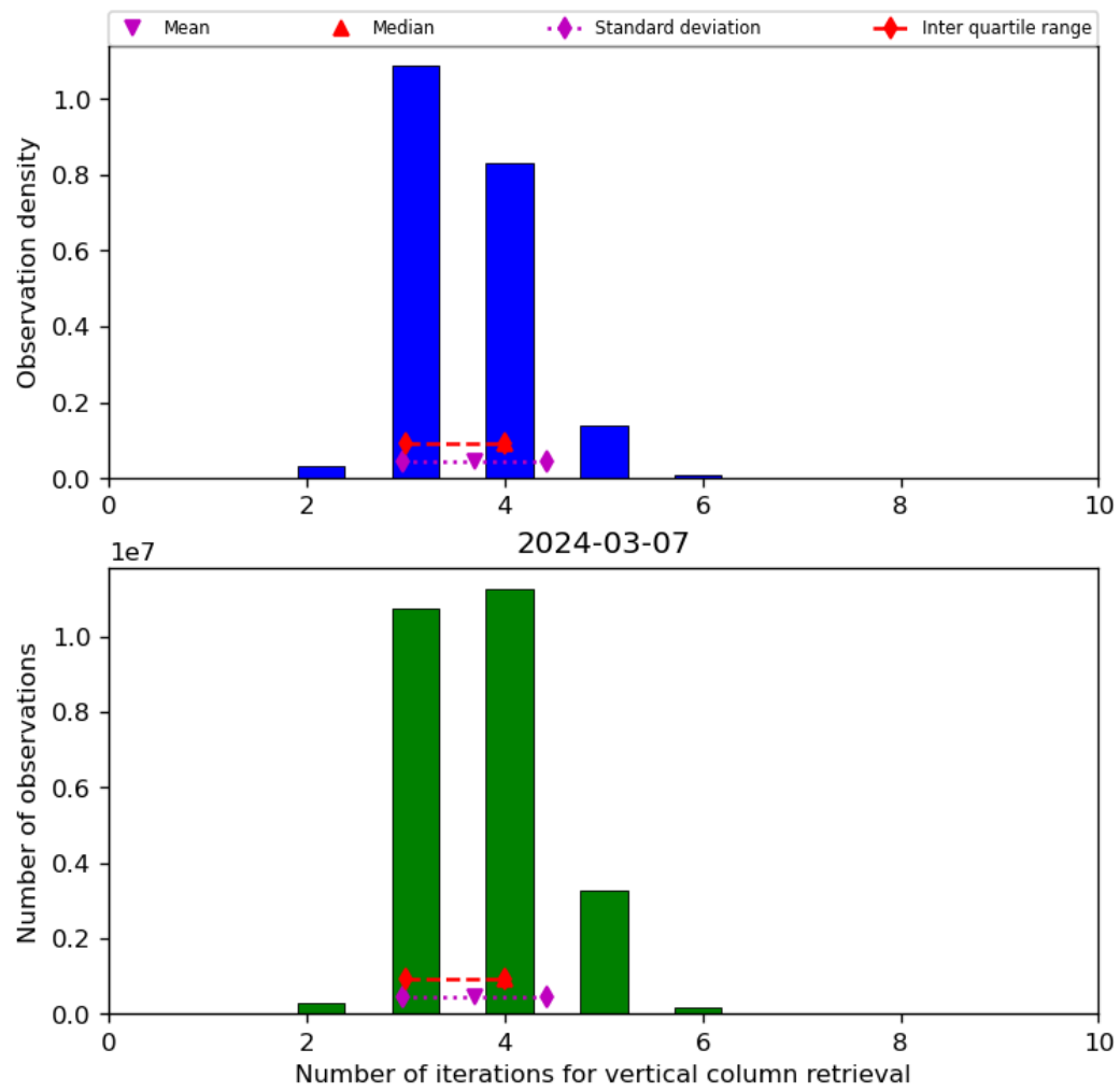
Figure 26: Histogram of “Number of iterations for vertical column retrieval” for 2024-03-06 to 2024-03-08
