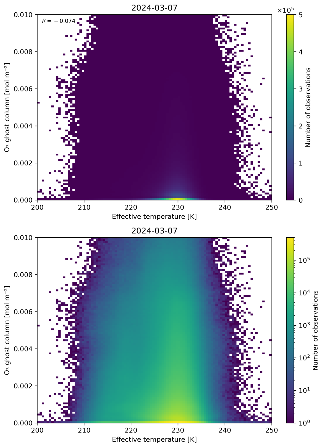
Figure 38: Scatter density plot of “Effective temperature” against “O 3 ghost column” for 2024-03-06 to 2024-03-08.
