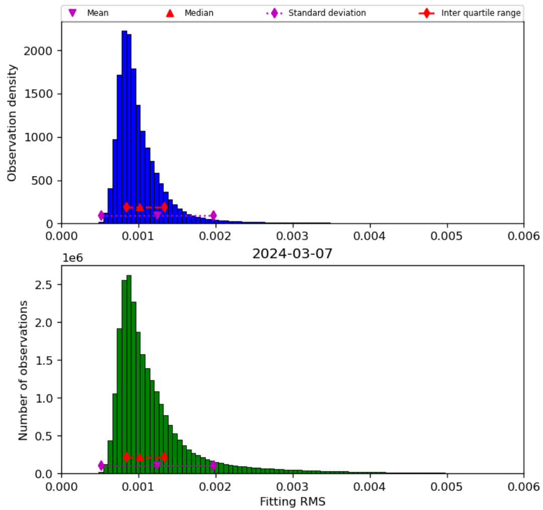
Figure 23: Histogram of “Fitting RMS” for 2024-03-06 to 2024-03-08
