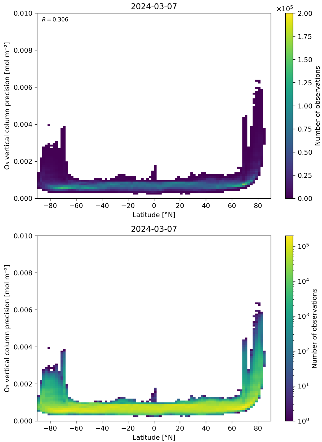
Figure 37: Scatter density plot of “Latitude” against “O 3 vertical column precision” for 2024-03-06 to 2024-03-08.
