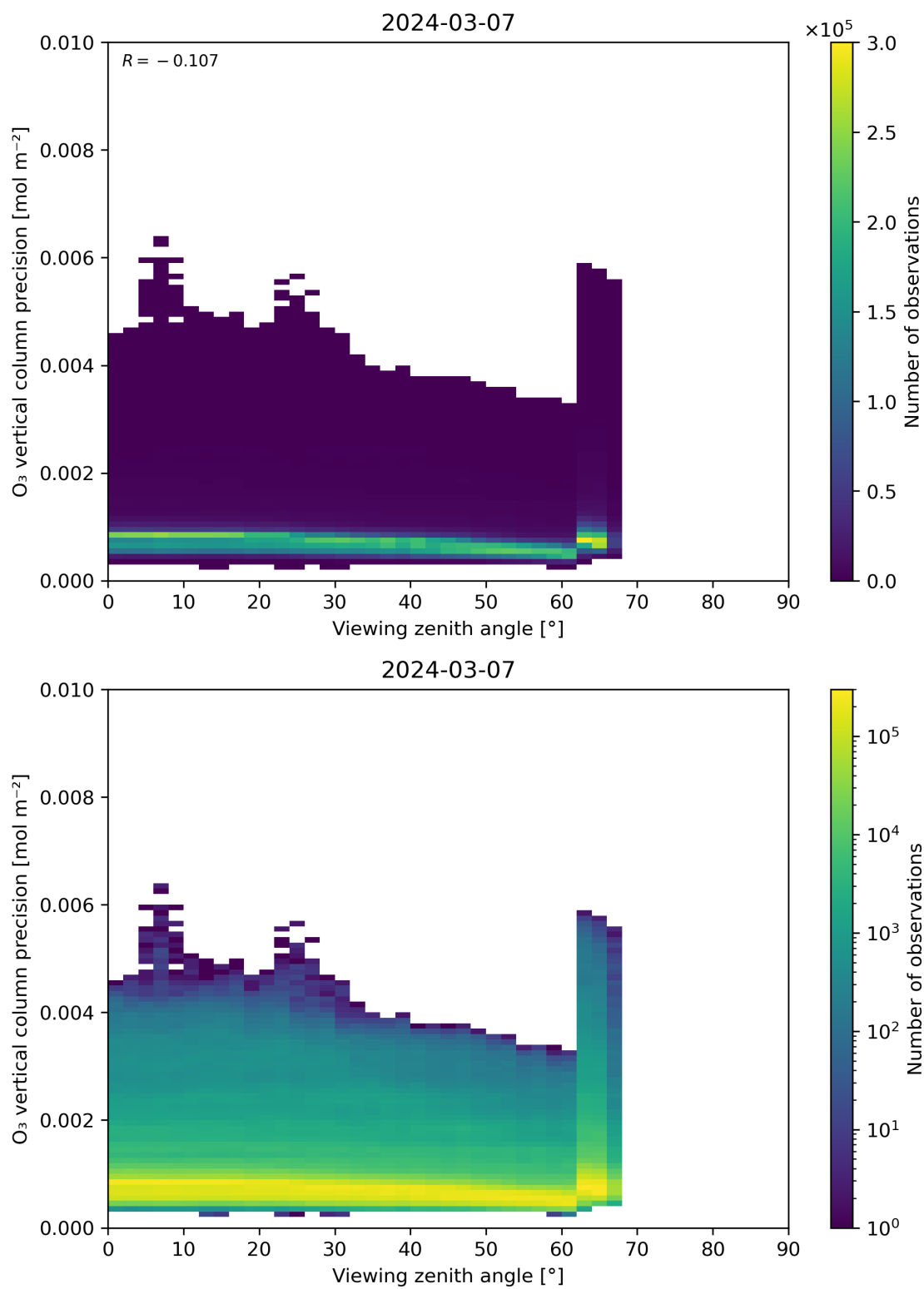
Figure 53: Scatter density plot of “Viewing zenith angle” against “O 3 vertical column precision” for 2024-03-06 to 2024-03-08.
