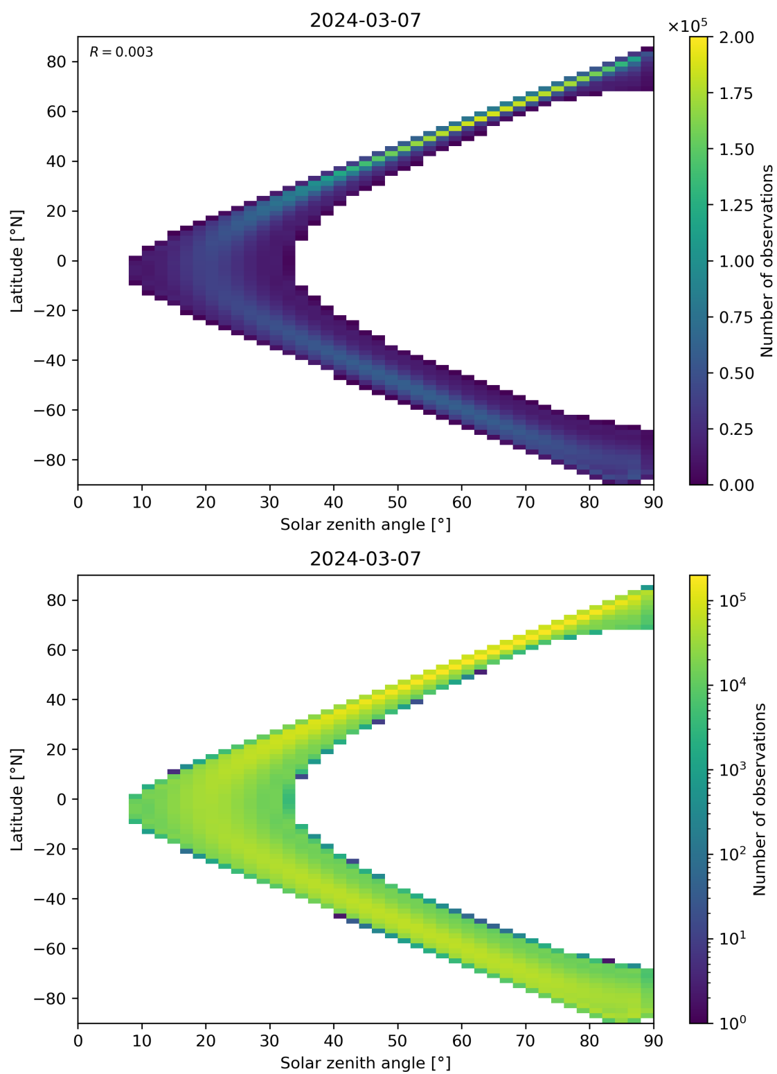
Figure 44: Scatter density plot of “Solar zenith angle” against “Latitude” for 2024-03-06 to 2024-03-08.
