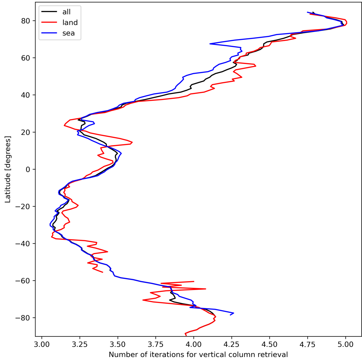
Figure 19: Zonal average of “Number of iterations for vertical column retrieval” for 2024-03-06 to 2024-03-08.
