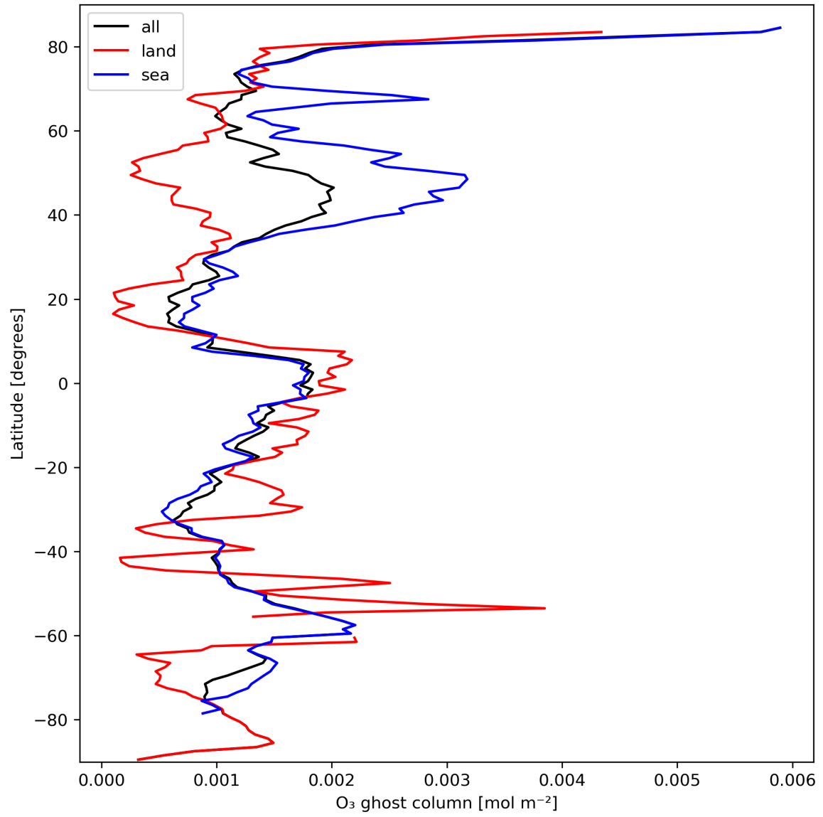
Figure 18: Zonal average of “O 3 ghost column” for 2024-03-06 to 2024-03-08.
