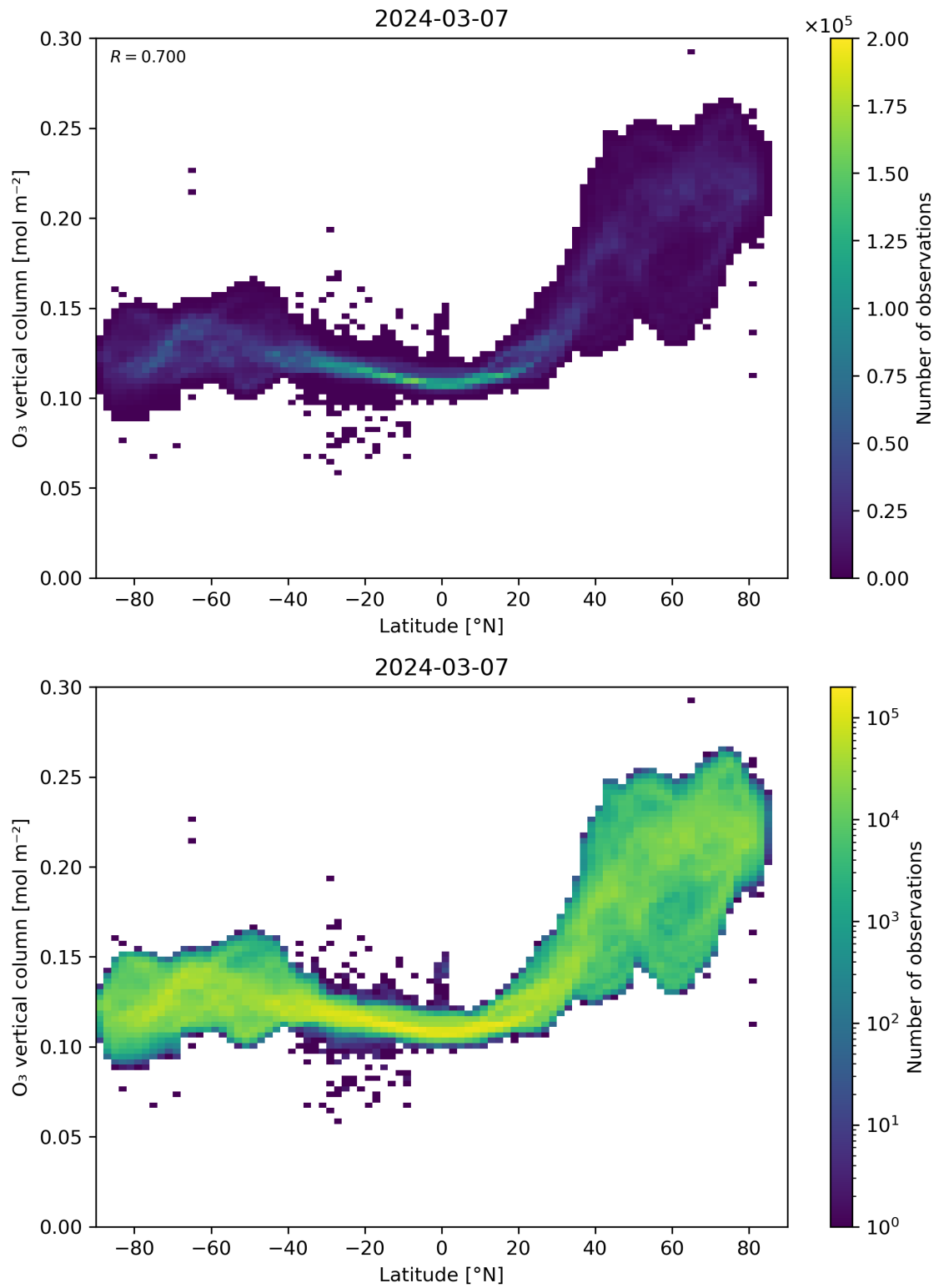
Figure 36: Scatter density plot of “Latitude” against “O 3 vertical column” for 2024-03-06 to 2024-03-08.
