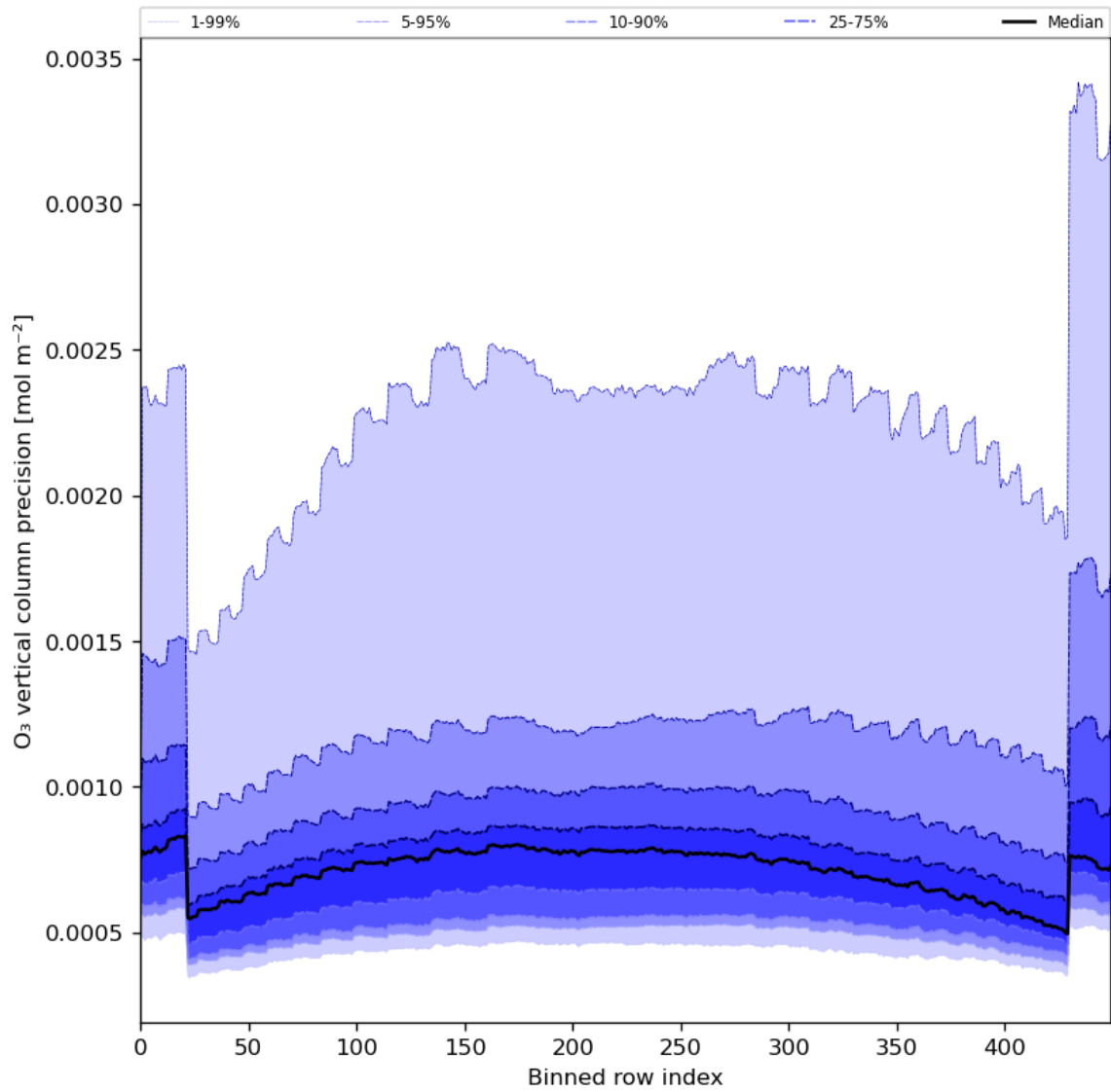
Figure 29: Along track statistics of “O 3 vertical column precision” for 2024-03-06 to 2024-03-08
