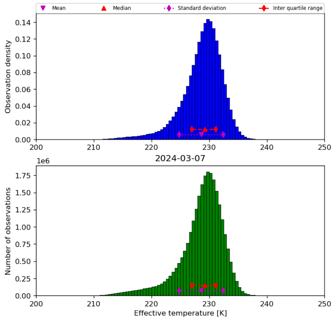
Figure 24: Histogram of “Effective temperature” for 2024-03-06 to 2024-03-08
