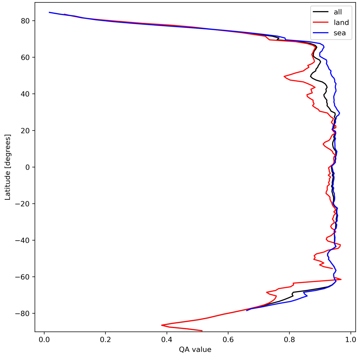
Figure 13: Zonal average of “QA value” for 2024-03-06 to 2024-03-08.
