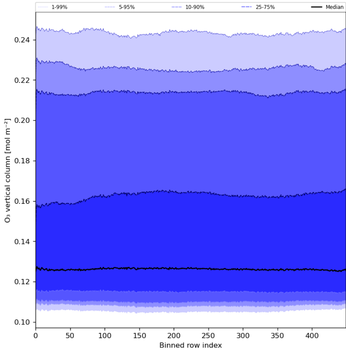
Figure 28: Along track statistics of "O 3 vertical column" for 2024-03-06 to 2024-03-08
