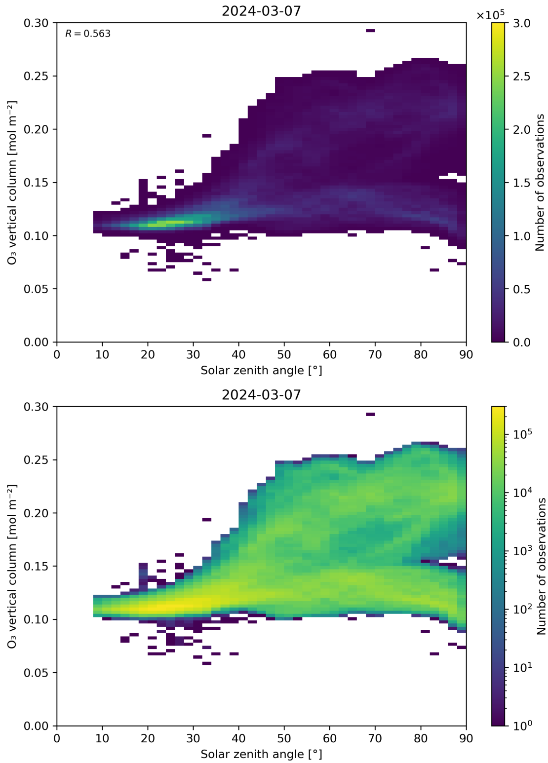
Figure 47: Scatter density plot of “Solar zenith angle” against “O 3 vertical column” for 2024-03-06 to 2024-03-08.
