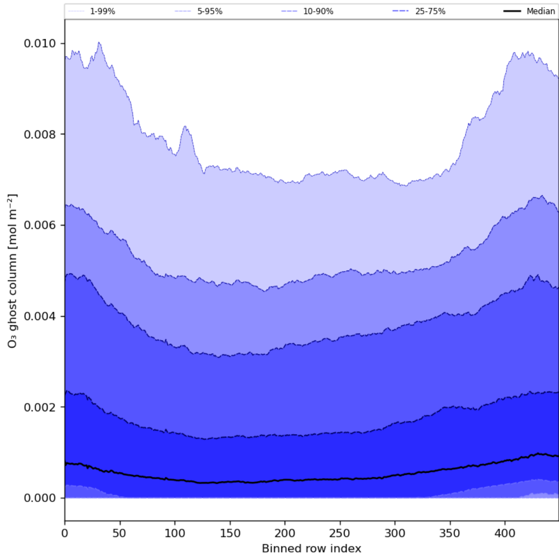
Figure 32: Along track statistics of “O 3 ghost column” for 2024-03-06 to 2024-03-08
