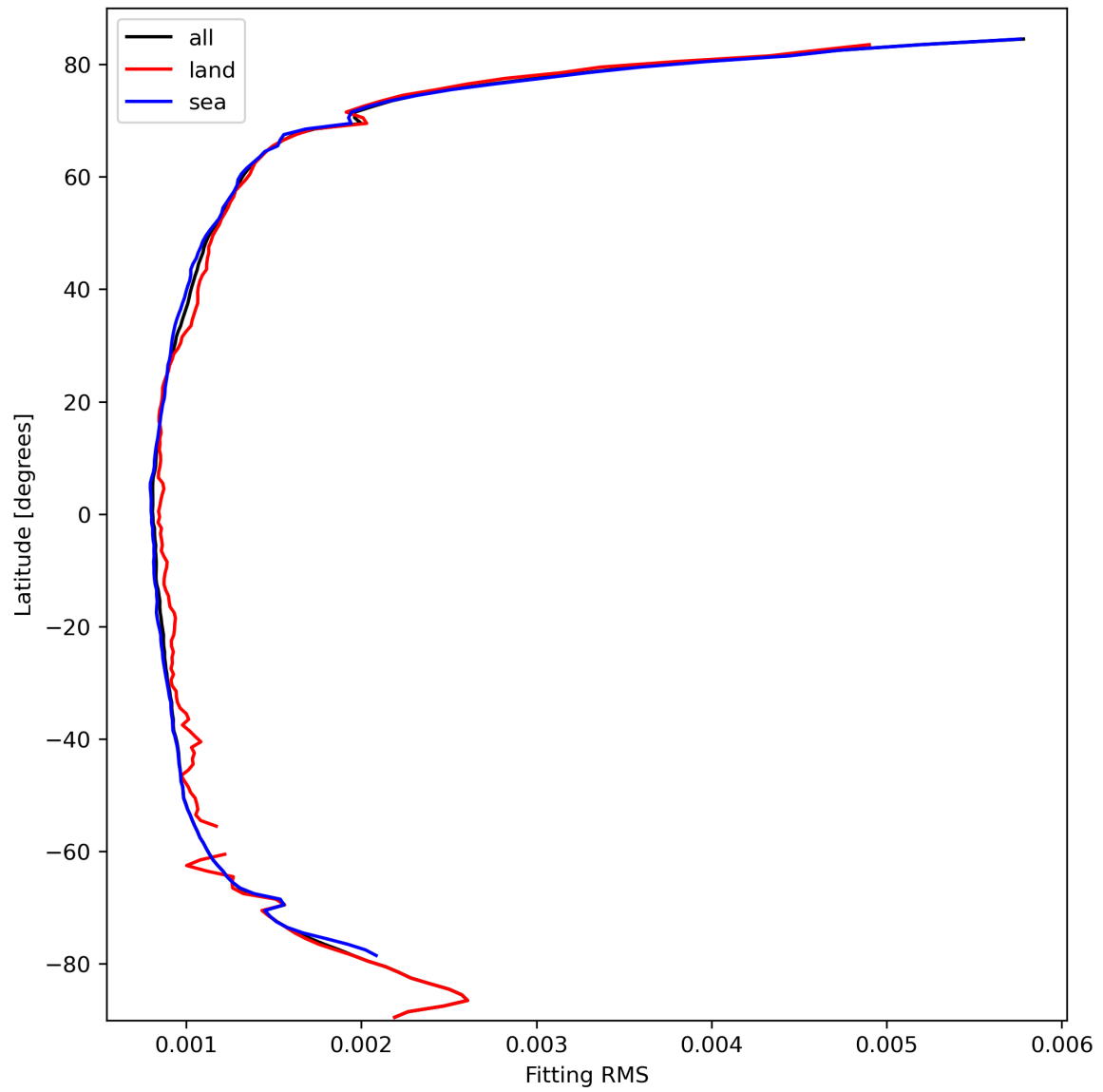
Figure 16: Zonal average of “Fitting RMS” for 2024-03-06 to 2024-03-08.
