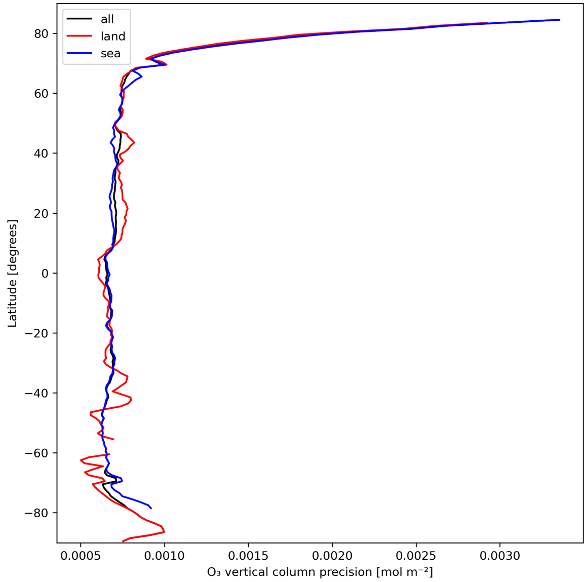
Figure 15: Zonal average of "O 3 vertical column precision" for 2024-03-06 to 2024-03-08.
