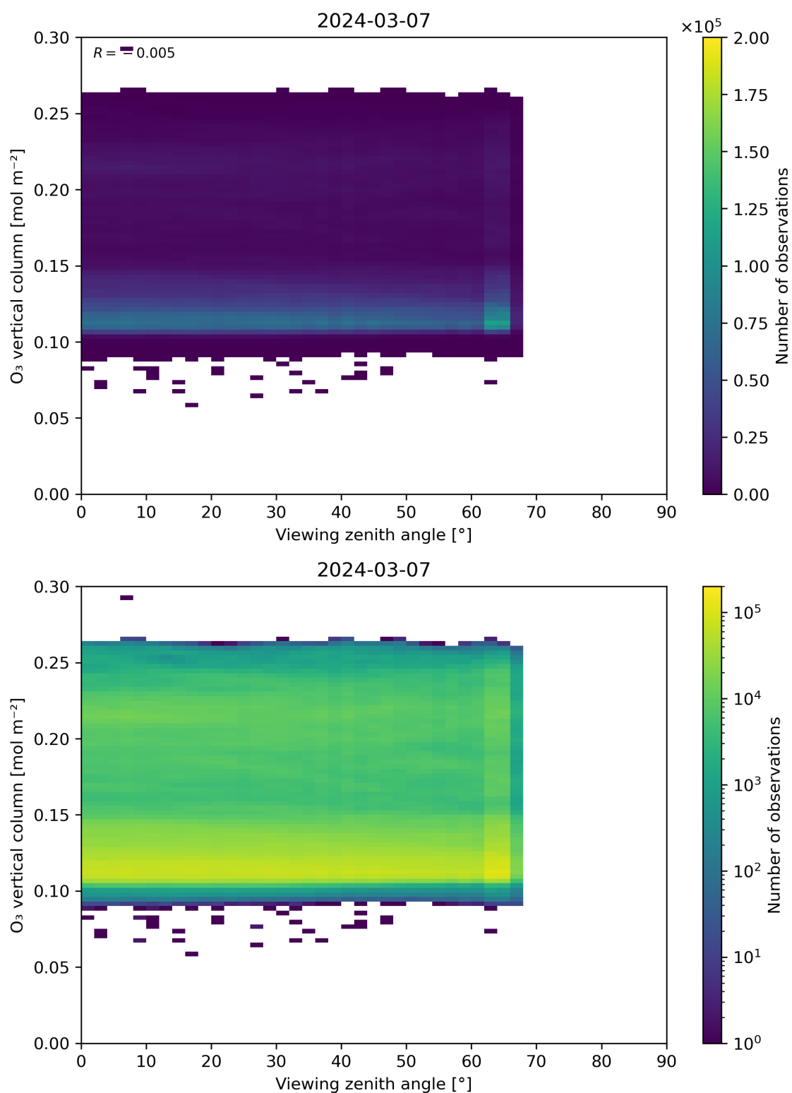
Figure 52: Scatter density plot of “Viewing zenith angle” against “O 3 vertical column” for 2024-03-06 to 2024-03-08.
