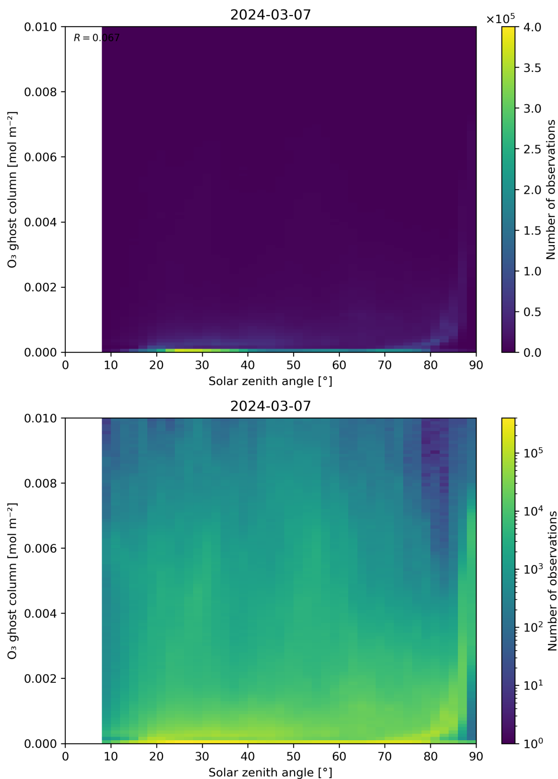
Figure 46: Scatter density plot of “Solar zenith angle” against “O 3 ghost column” for 2024-03-06 to 2024-03-08.
