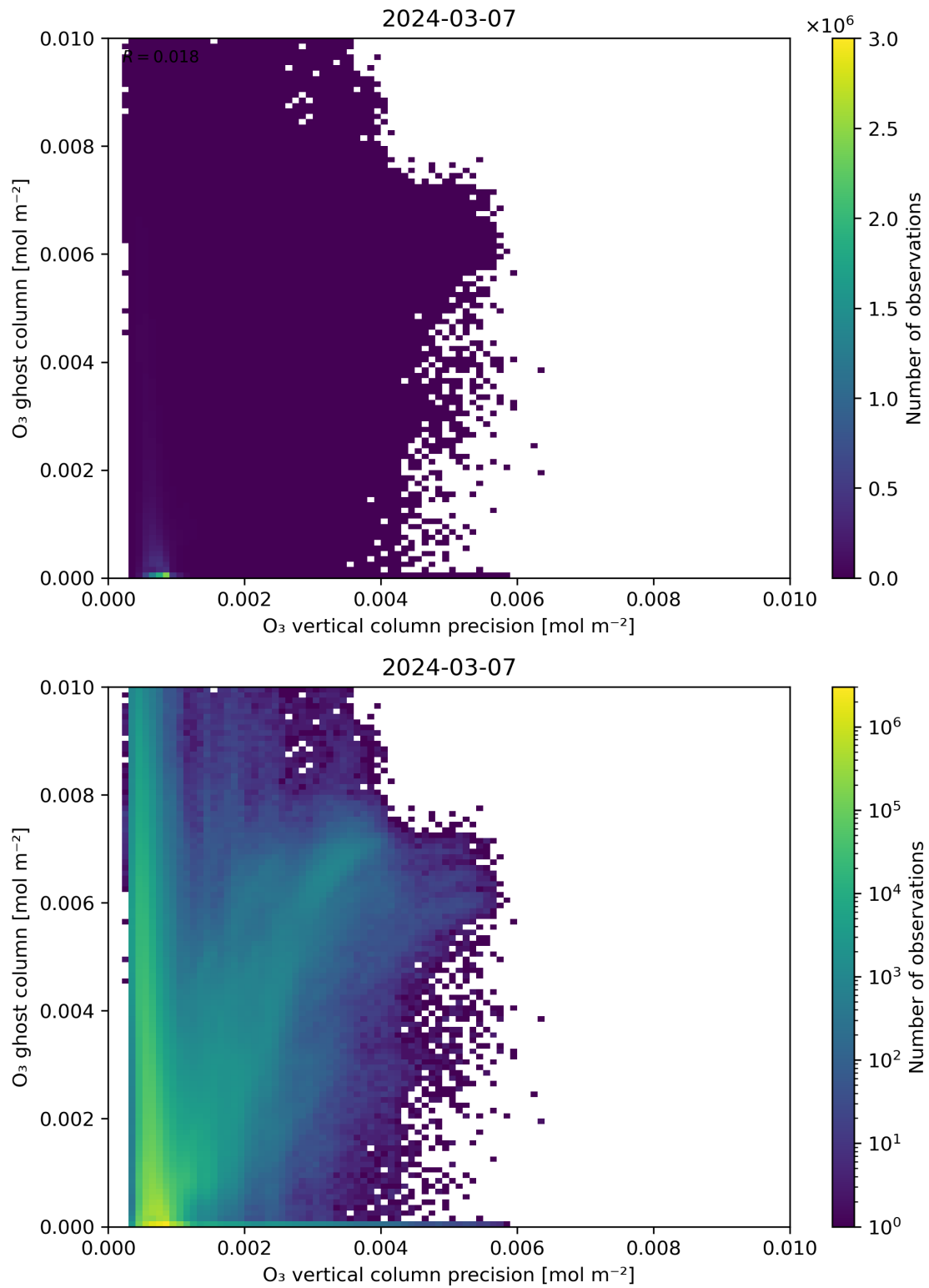
Figure 43: Scatter density plot of “ \text{O}_3 vertical column precision” against “ \text{O}_3 ghost column” for 2024-03-06 to 2024-03-08.
