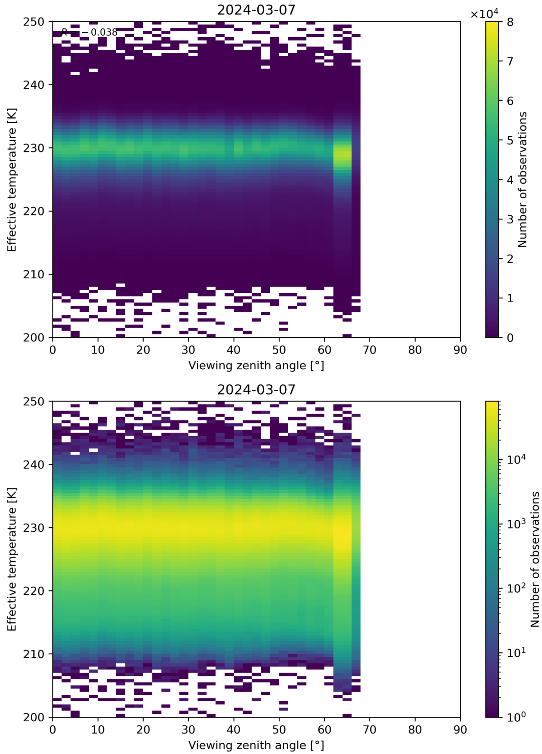
Figure 50: Scatter density plot of “Viewing zenith angle” against “Effective temperature” for 2024-03-06 to 2024-03-08.
