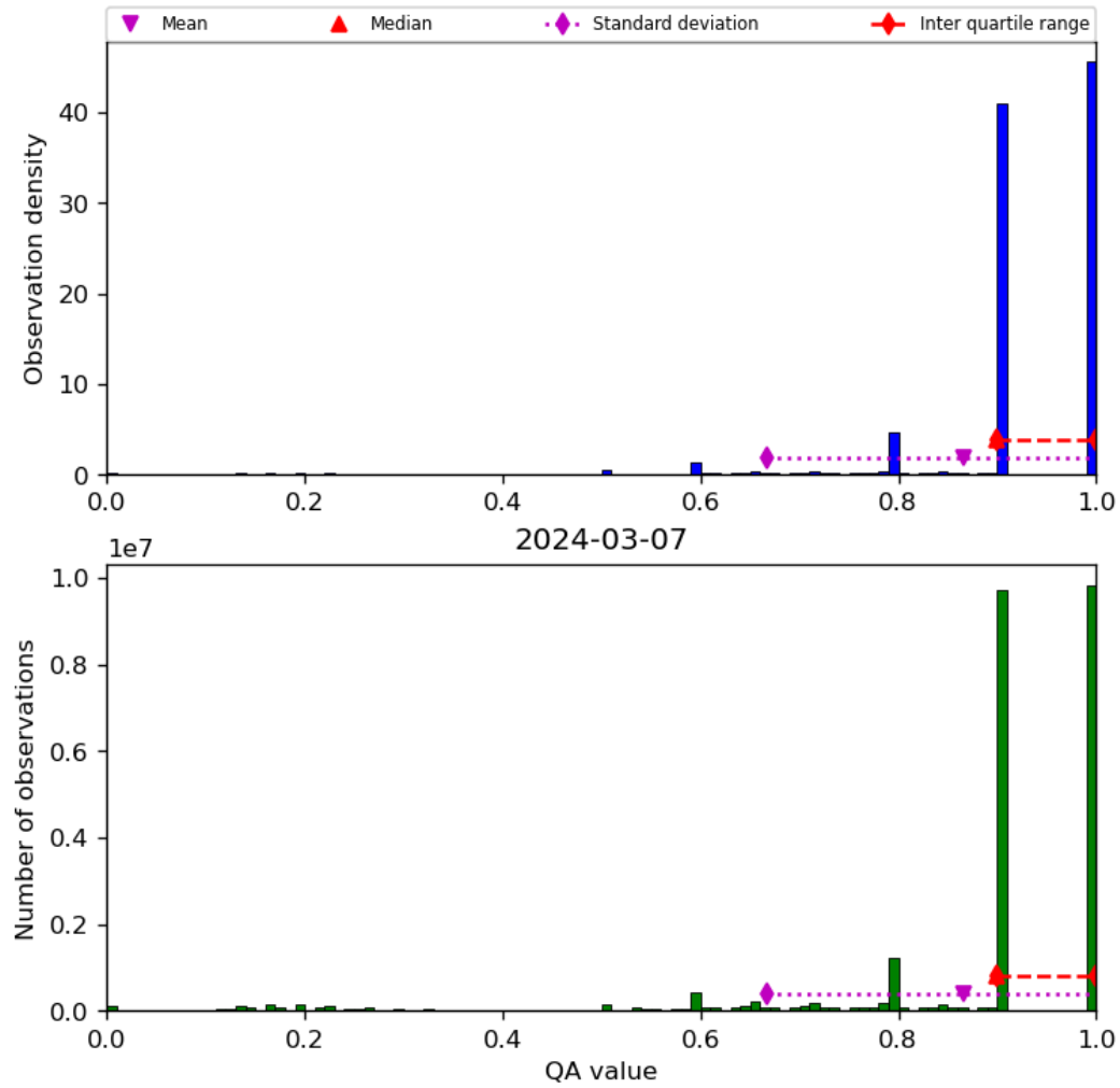
Figure 20: Histogram of “QA value” for 2024-03-06 to 2024-03-08
