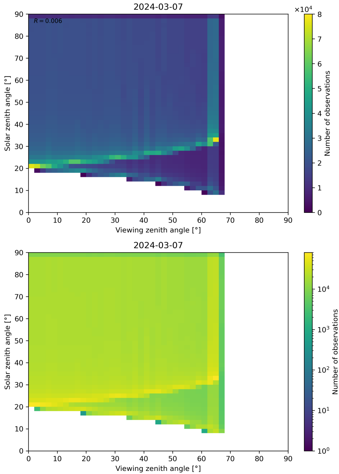
Figure 54: Scatter density plot of “Viewing zenith angle” against “Solar zenith angle” for 2024-03-06 to 2024-03-08.
