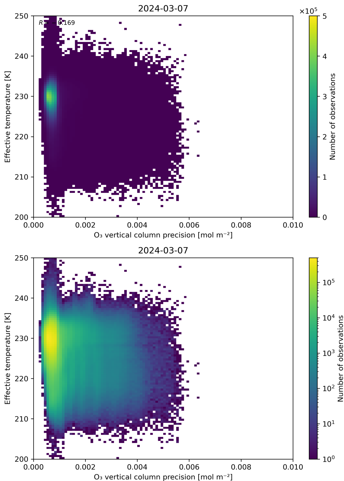
Figure 42: Scatter density plot of “O 3 vertical column precision” against “Effective temperature” for 2024-03-06 to 2024-03-08.
