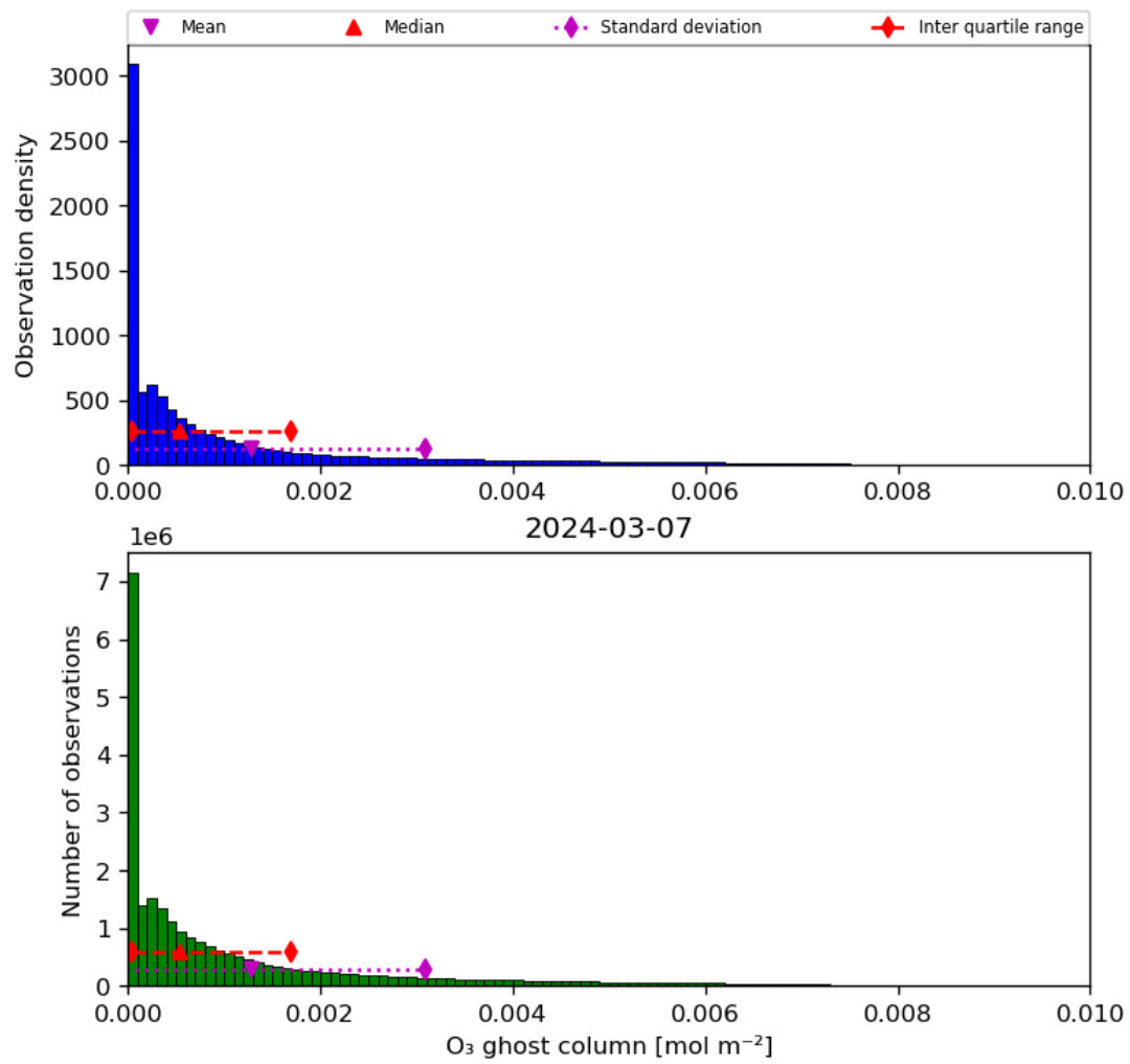
Figure 25: Histogram of “O 3 ghost column” for 2024-03-06 to 2024-03-08
