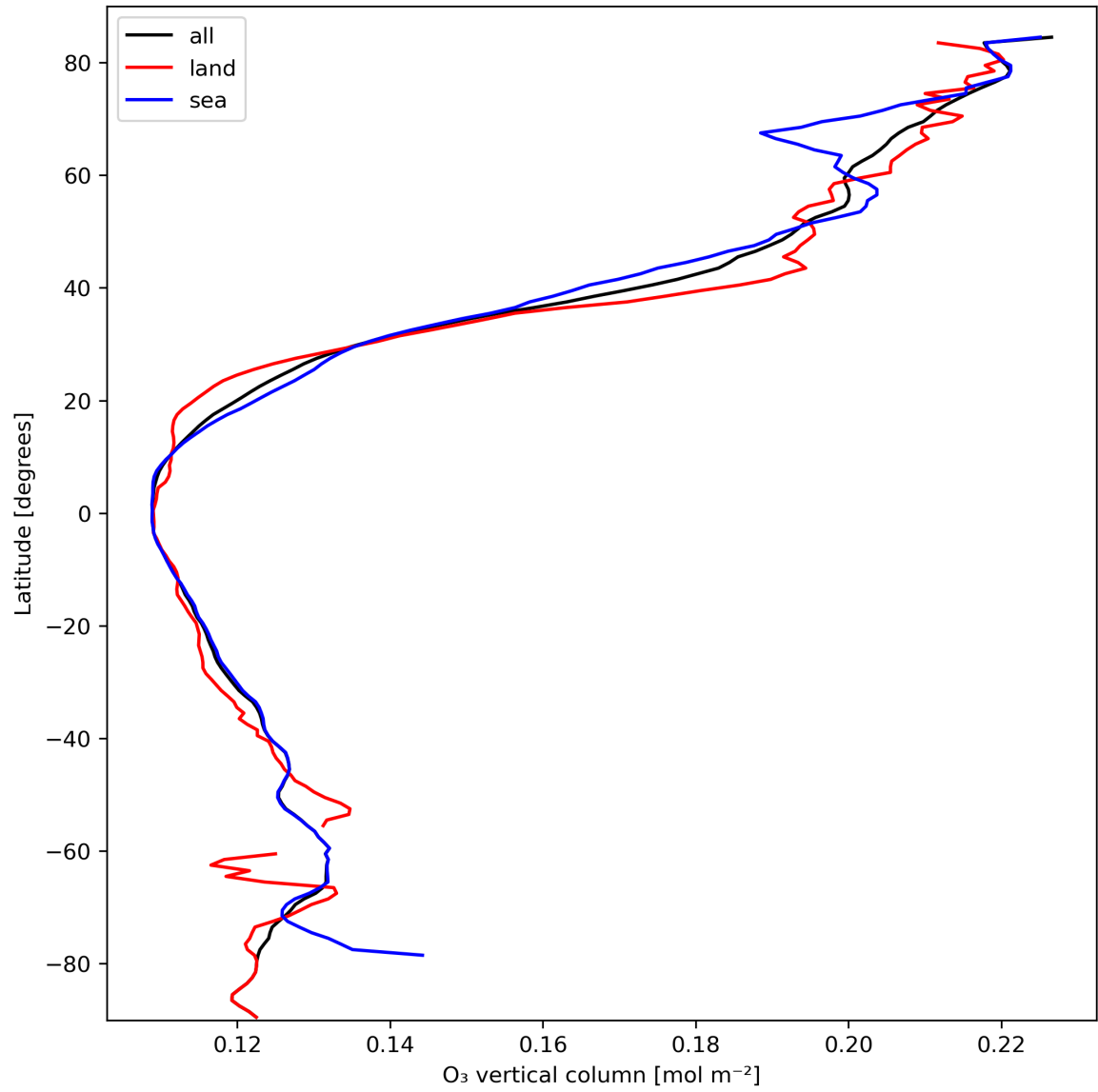
Figure 14: Zonal average of “O 3 vertical column” for 2024-03-06 to 2024-03-08.
