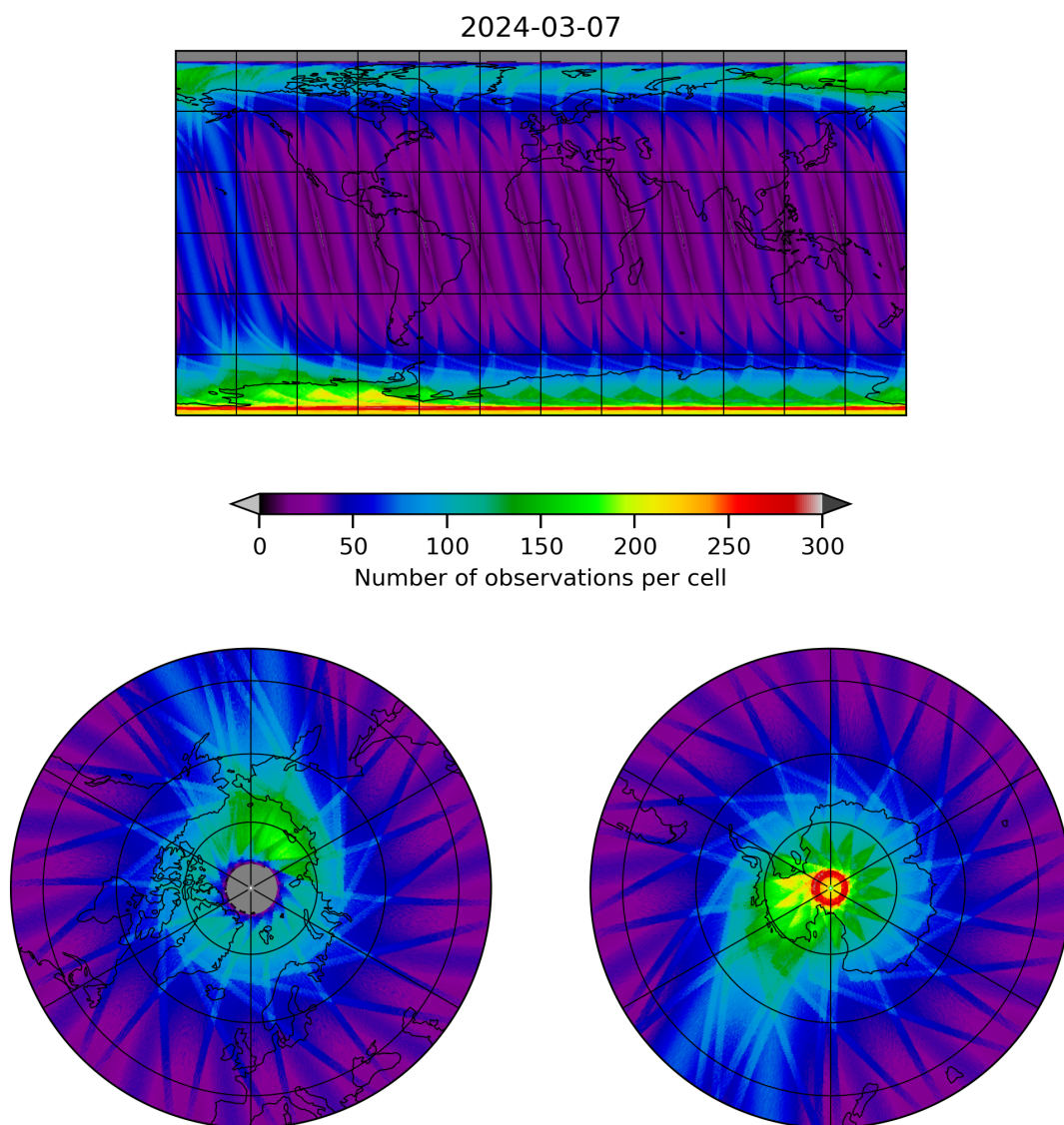
Figure 12: Map of the number of observations for 2024-03-06 to 2024-03-08
