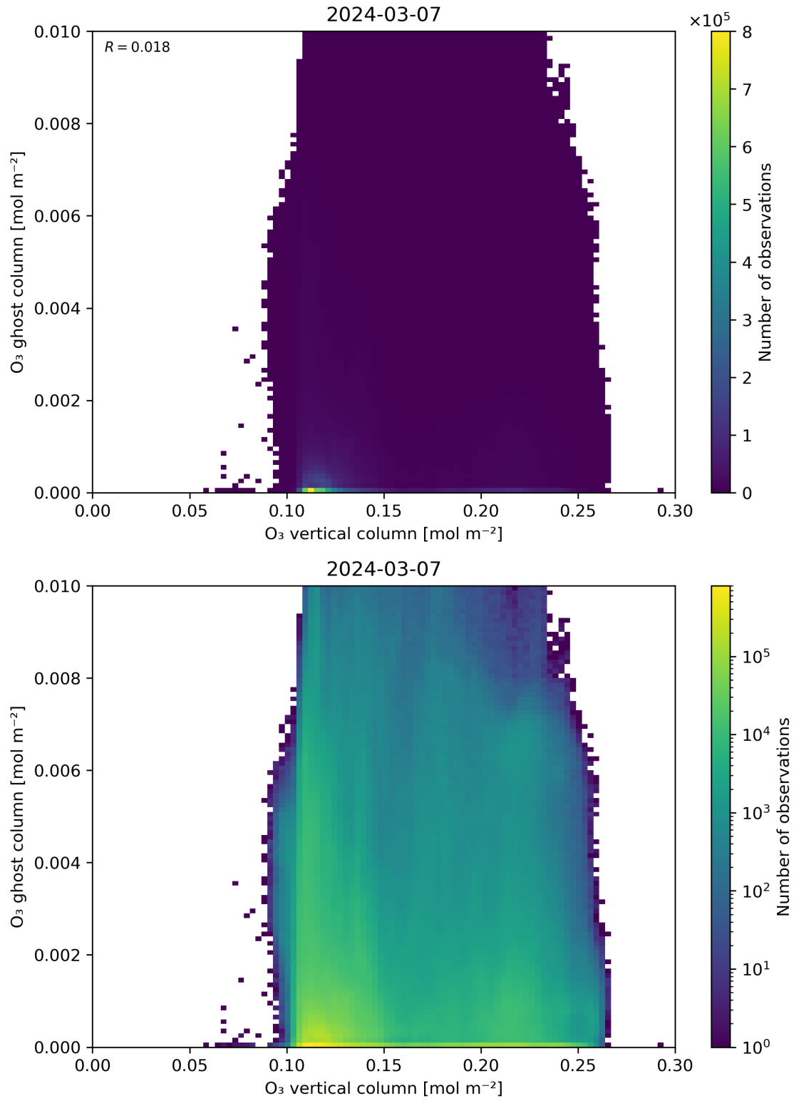
Figure 40: Scatter density plot of “O 3 vertical column” against “O 3 ghost column” for 2024-03-06 to 2024-03-08.
