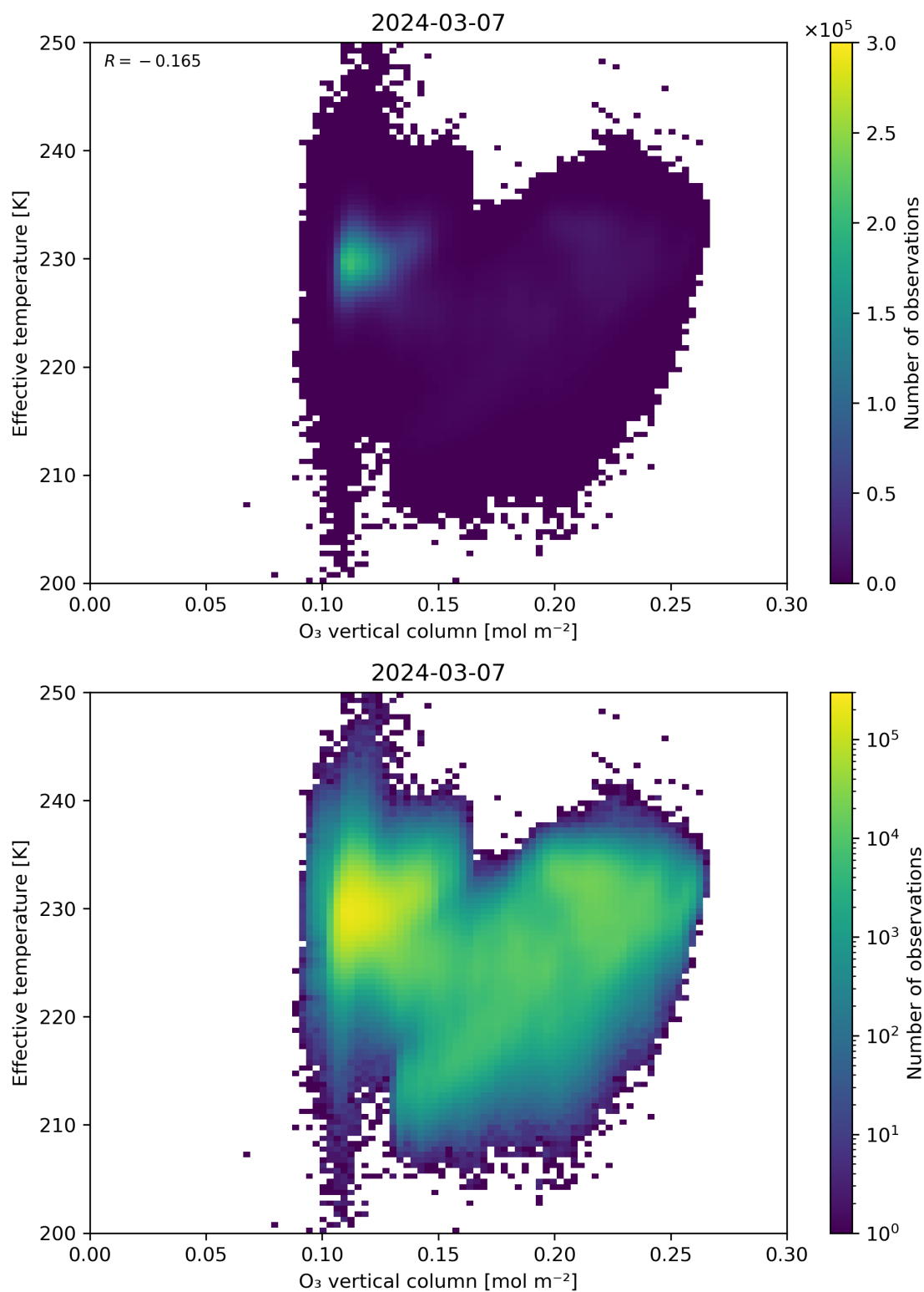
Figure 39: Scatter density plot of “O 3 vertical column” against “Effective temperature” for 2024-03-06 to 2024-03-08.
