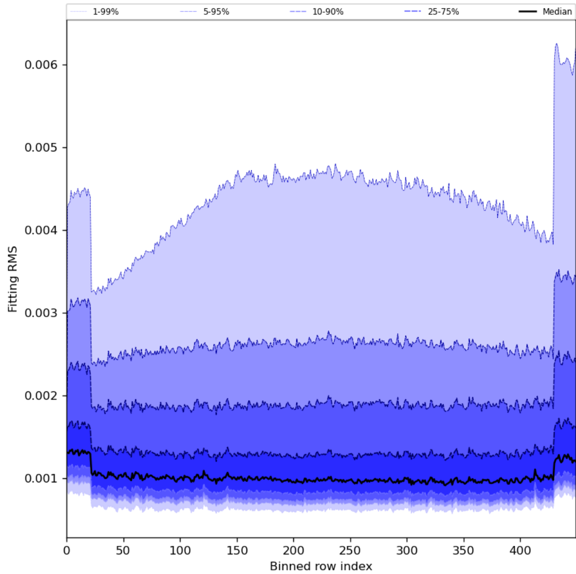
Figure 30: Along track statistics of “Fitting RMS” for 2024-03-06 to 2024-03-08
