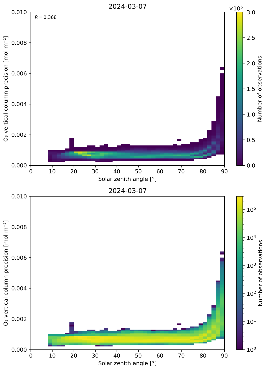
Figure 48: Scatter density plot of “Solar zenith angle” against “O 3 vertical column precision” for 2024-03-06 to 2024-03-08.
