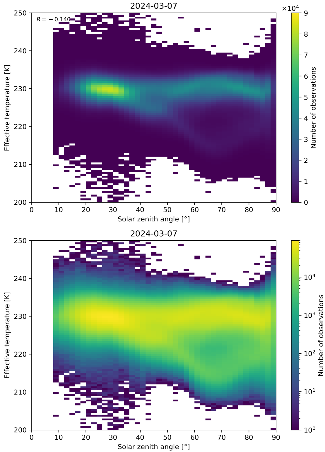
Figure 45: Scatter density plot of “Solar zenith angle” against “Effective temperature” for 2024-03-06 to 2024-03-08.
