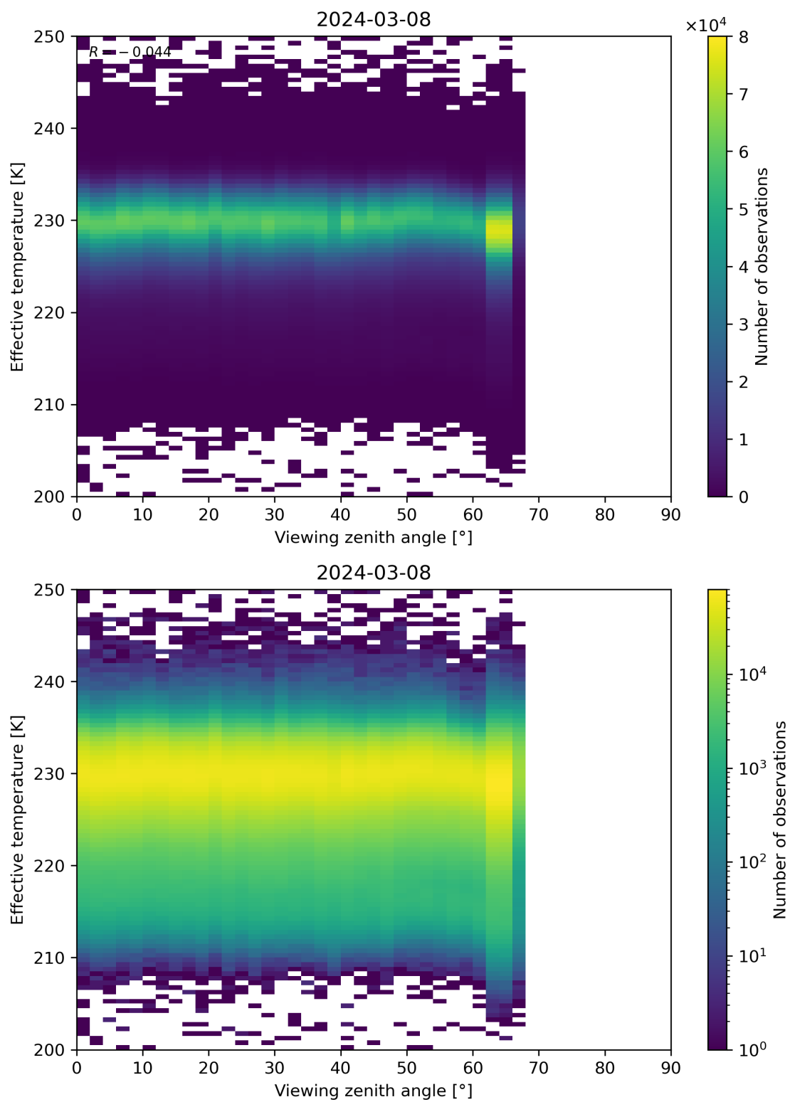
Figure 50: Scatter density plot of “Viewing zenith angle” against “Effective temperature” for 2024-03-07 to 2024-03-09.
