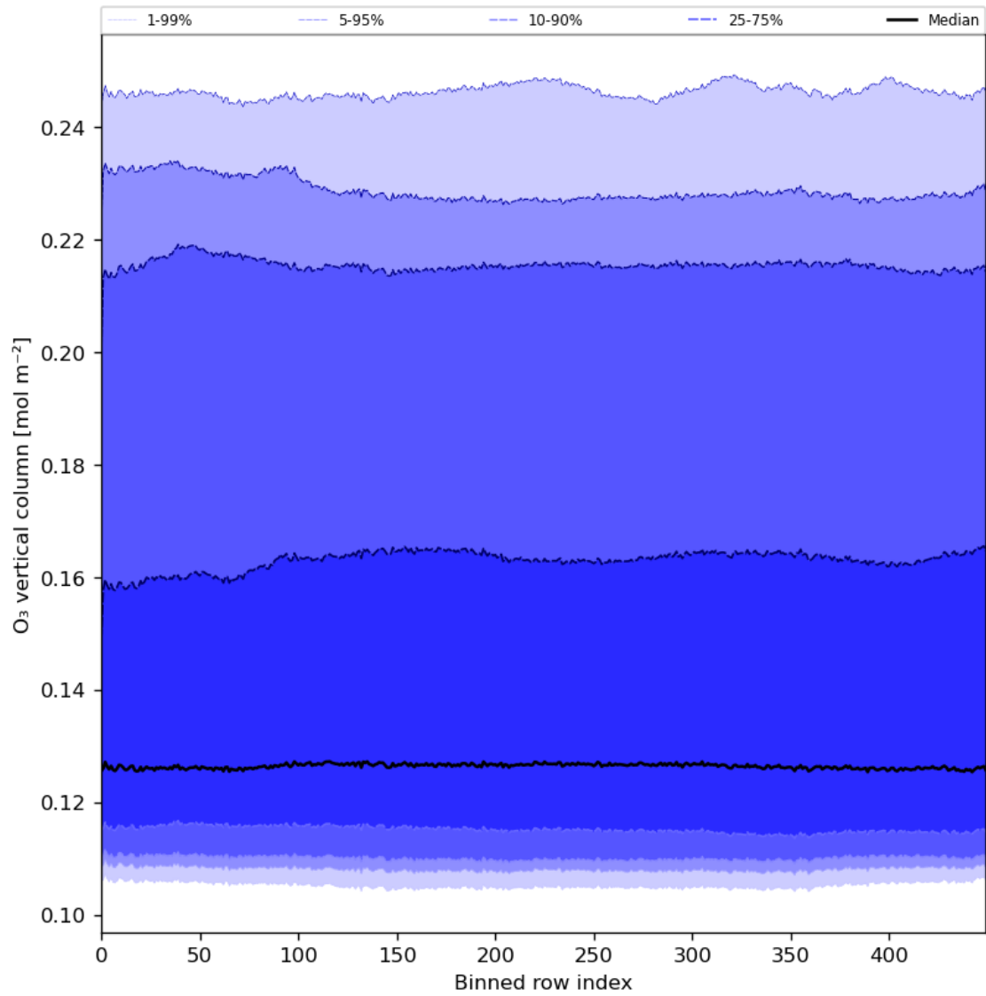
Figure 28: Along track statistics of “O 3 vertical column” for 2024-03-07 to 2024-03-09
