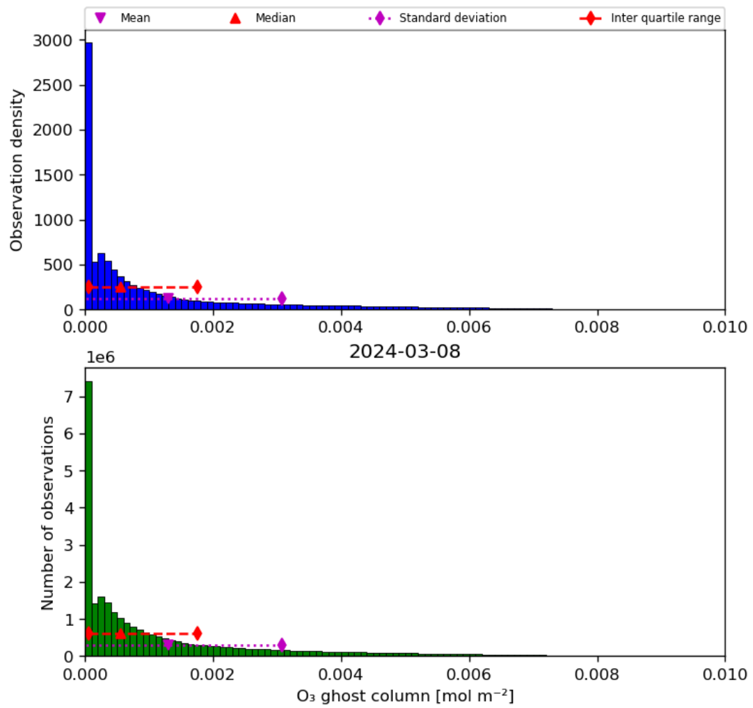
Figure 25: Histogram of “O 3 ghost column” for 2024-03-07 to 2024-03-09
