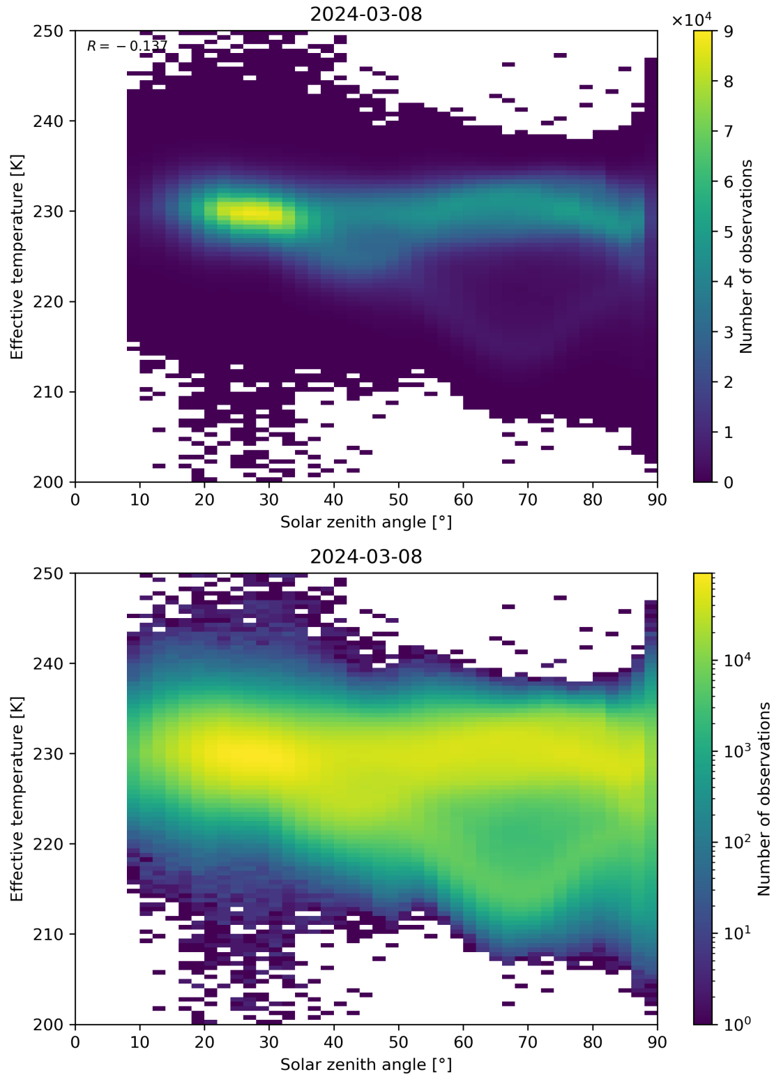
Figure 45: Scatter density plot of “Solar zenith angle” against “Effective temperature” for 2024-03-07 to 2024-03-09.
