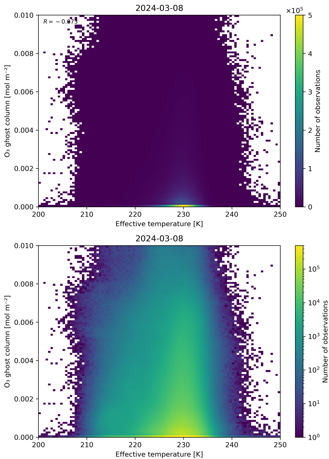
Figure 38: Scatter density plot of “Effective temperature” against “O 3 ghost column” for 2024-03-07 to 2024-03-09.
