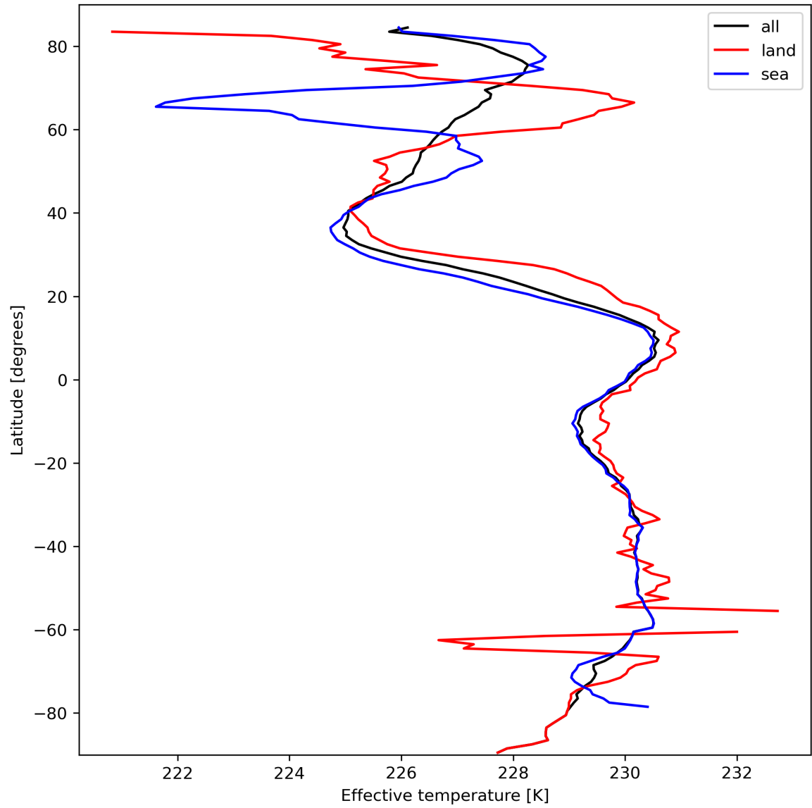
Figure 17: Zonal average of "Effective temperature" for 2024-03-07 to 2024-03-09.
