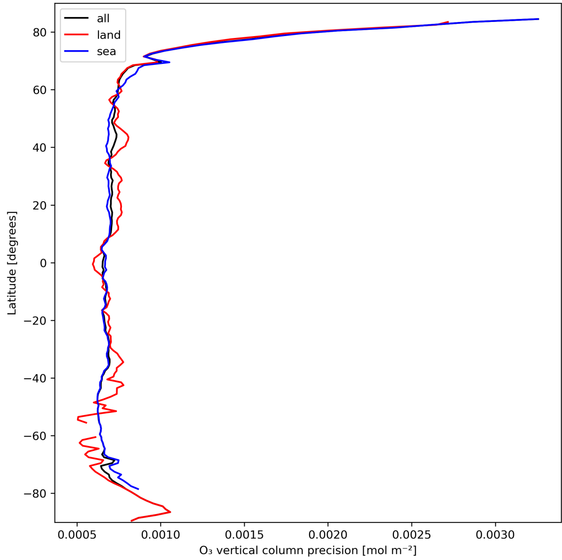
Figure 15: Zonal average of “O 3 vertical column precision” for 2024-03-07 to 2024-03-09.
