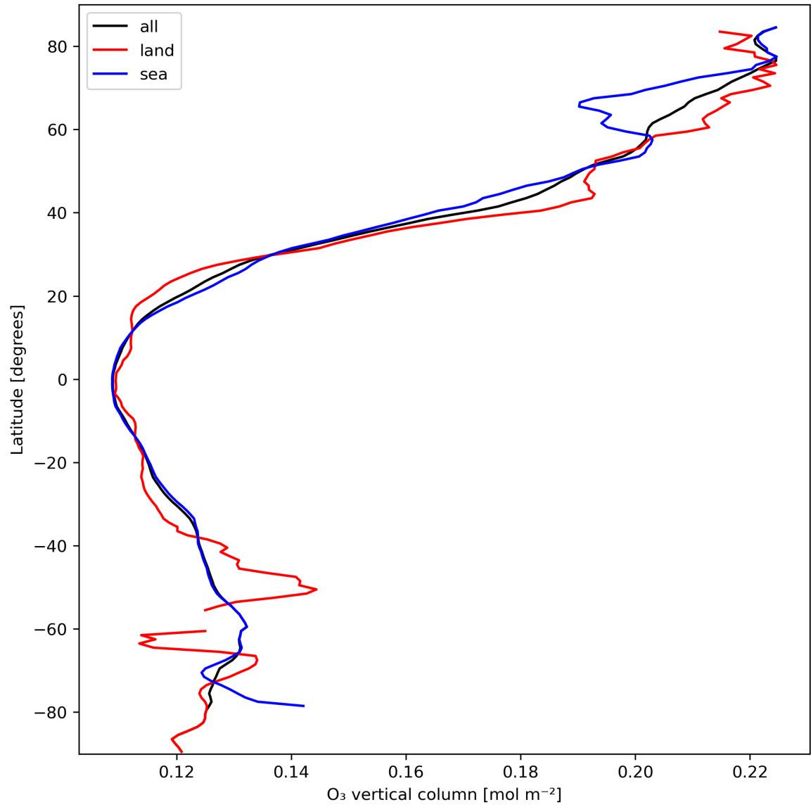
Figure 14: Zonal average of “O 3 vertical column” for 2024-03-07 to 2024-03-09.
