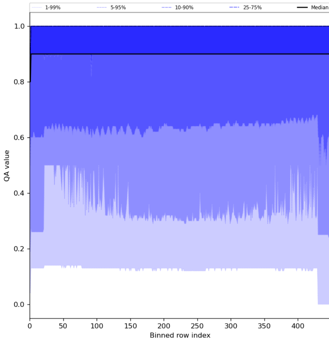
Figure 27: Along track statistics of “QA value” for 2024-03-07 to 2024-03-09
