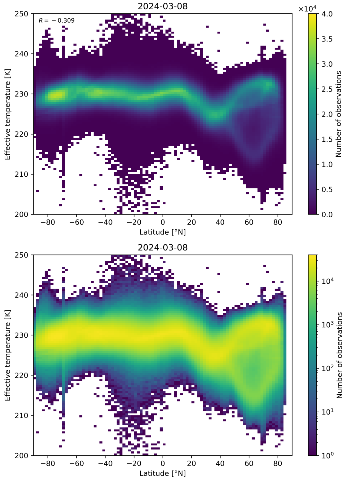
Figure 34: Scatter density plot of “Latitude” against “Effective temperature” for 2024-03-07 to 2024-03-09.
