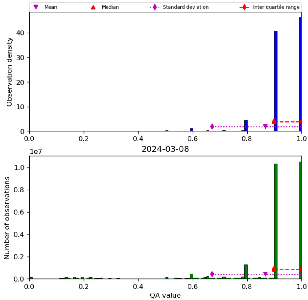
Figure 20: Histogram of “QA value” for 2024-03-07 to 2024-03-09
