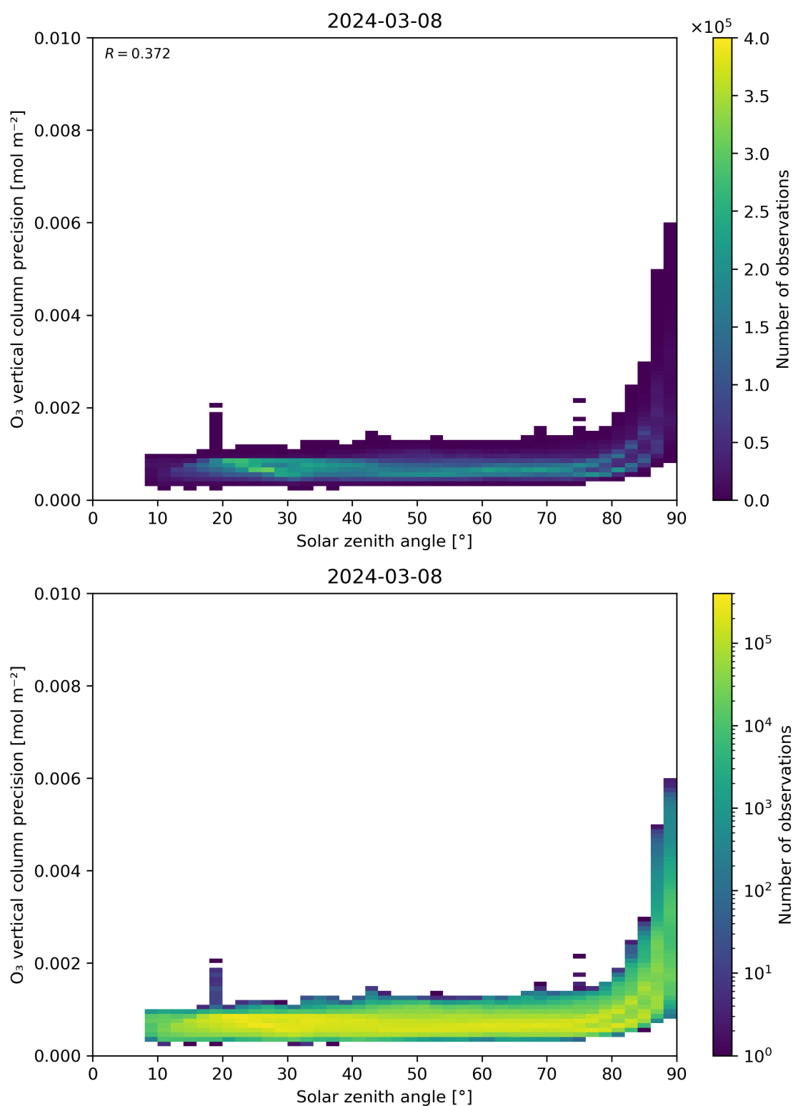
Figure 48: Scatter density plot of “Solar zenith angle” against “O 3 vertical column precision” for 2024-03-07 to 2024-03-09.
