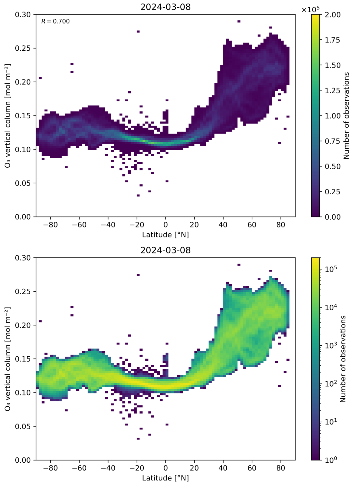
Figure 36: Scatter density plot of “Latitude” against “O 3 vertical column” for 2024-03-07 to 2024-03-09.
