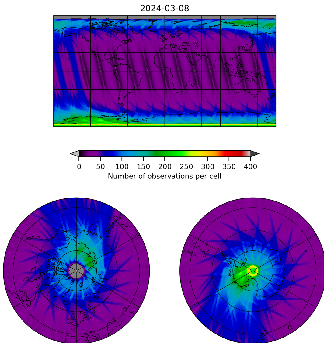
Figure 12: Map of the number of observations for 2024-03-07 to 2024-03-09
