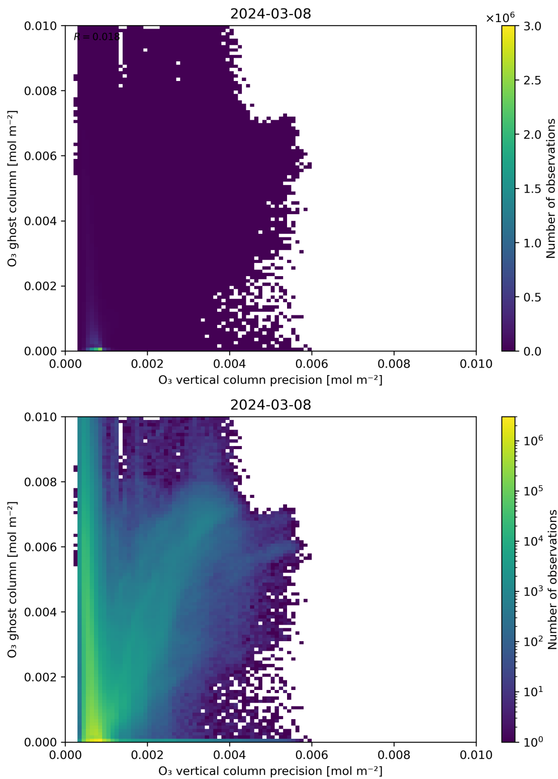
Figure 43: Scatter density plot of “O 3 vertical column precision” against “O 3 ghost column” for 2024-03-07 to 2024-03-09.
