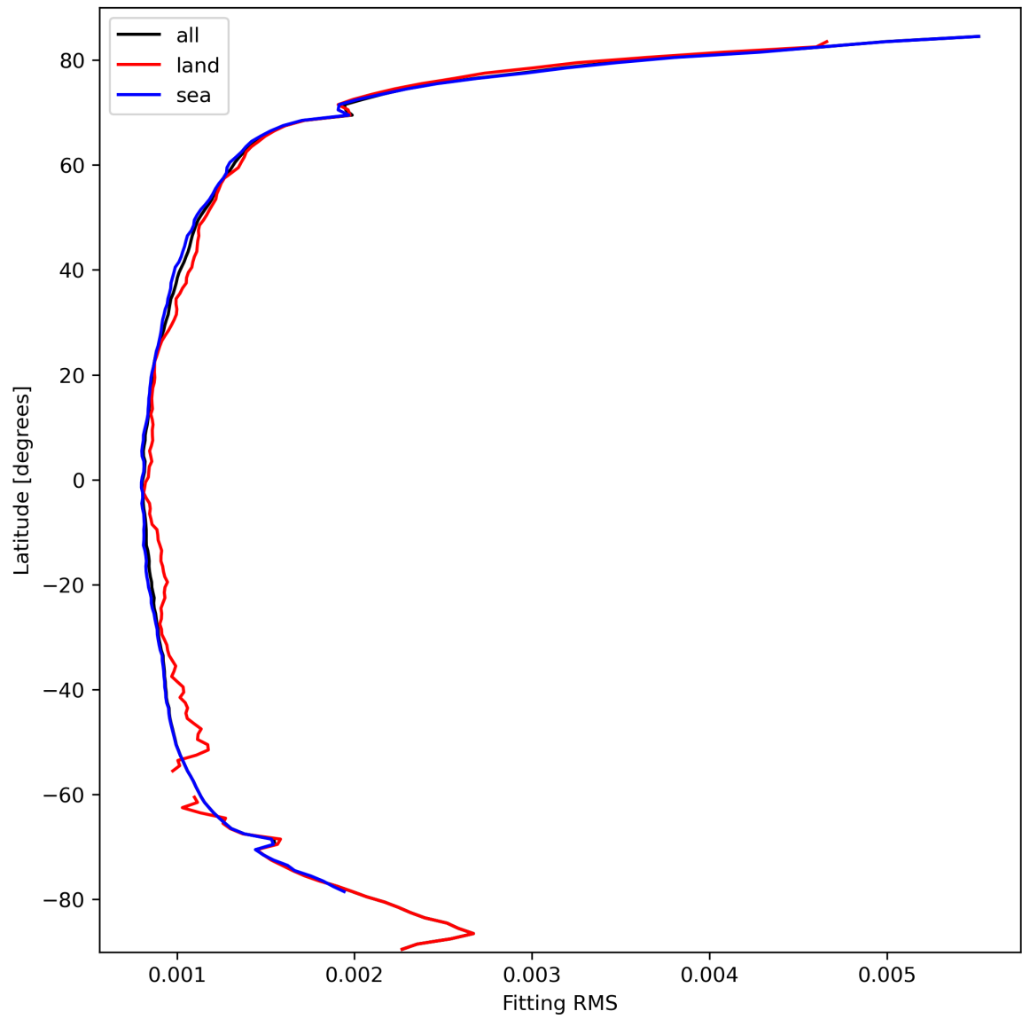
Figure 16: Zonal average of “Fitting RMS” for 2024-03-07 to 2024-03-09.
