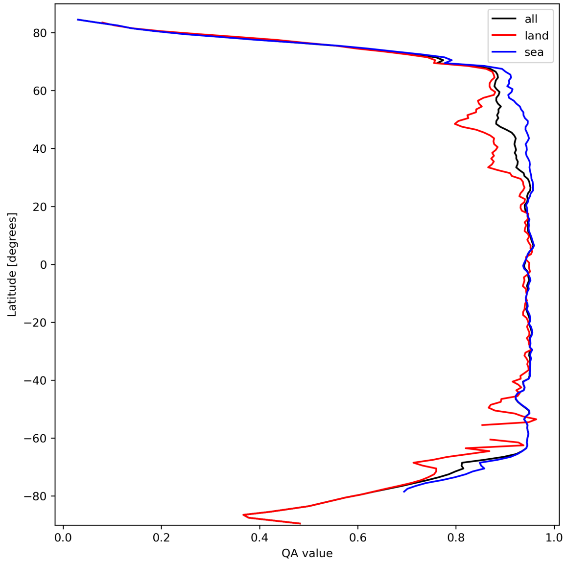
Figure 13: Zonal average of “QA value” for 2024-03-07 to 2024-03-09.
