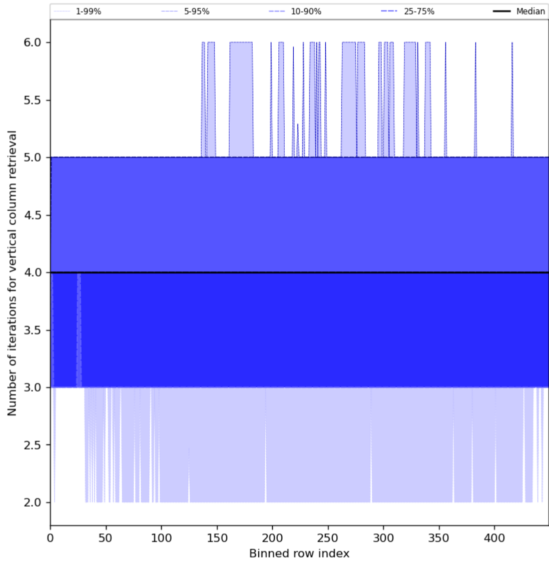
Figure 33: Along track statistics of “Number of iterations for vertical column retrieval” for 2024-03-07 to 2024-03-09
