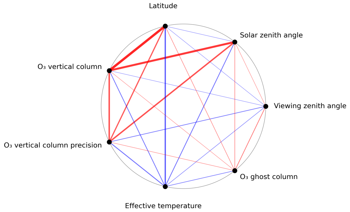
Figure 1: Map of correlation graph for 2024-03-07 to 2024-03-09.
