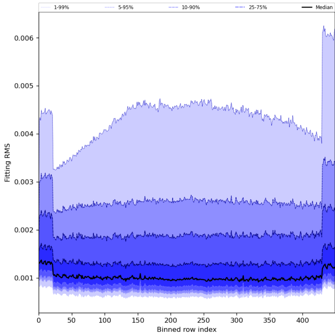
Figure 30: Along track statistics of “Fitting RMS” for 2024-03-07 to 2024-03-09
