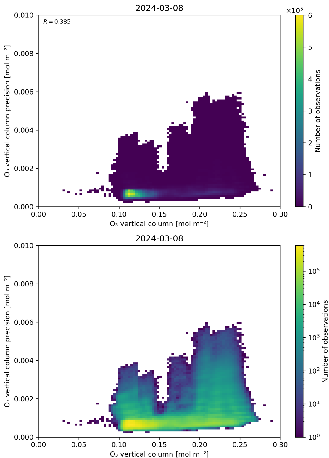
Figure 41: Scatter density plot of “O 3 vertical column” against “O 3 vertical column precision” for 2024-03-07 to 2024-03-09.
