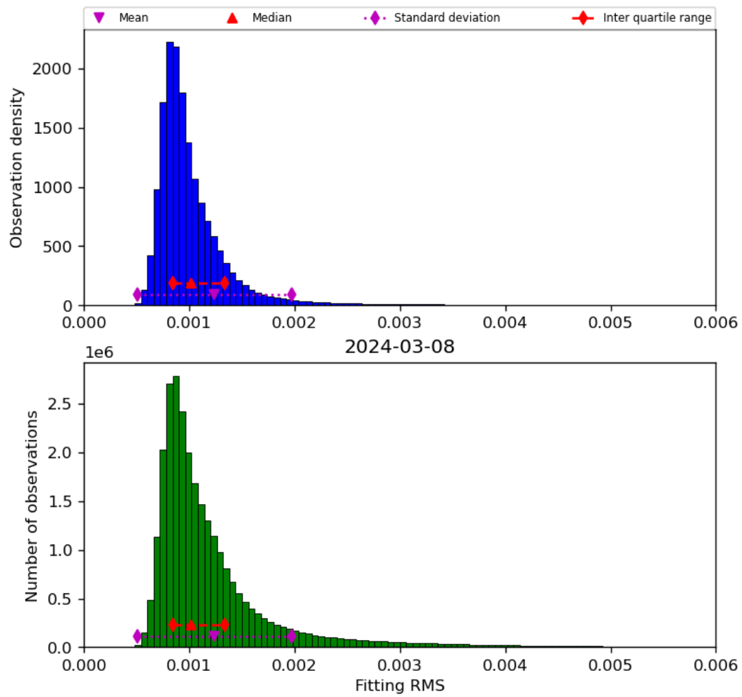
Figure 23: Histogram of “Fitting RMS” for 2024-03-07 to 2024-03-09
