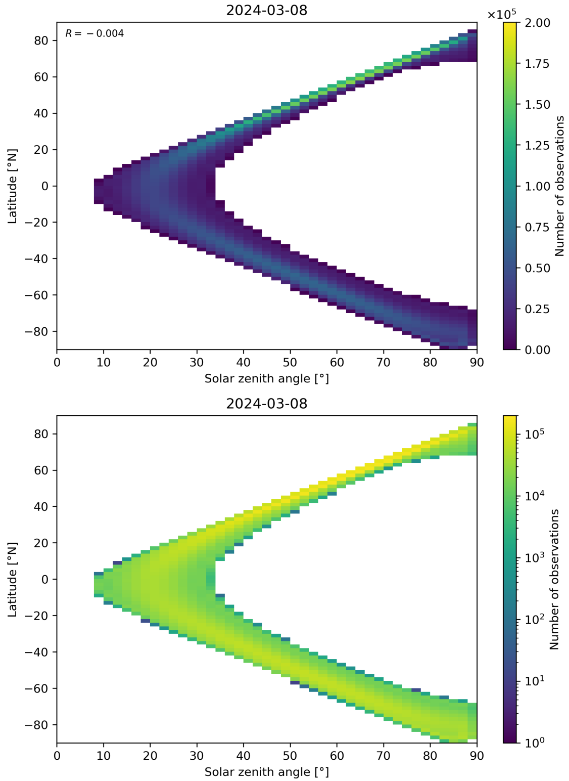
Figure 44: Scatter density plot of “Solar zenith angle” against “Latitude” for 2024-03-07 to 2024-03-09.
