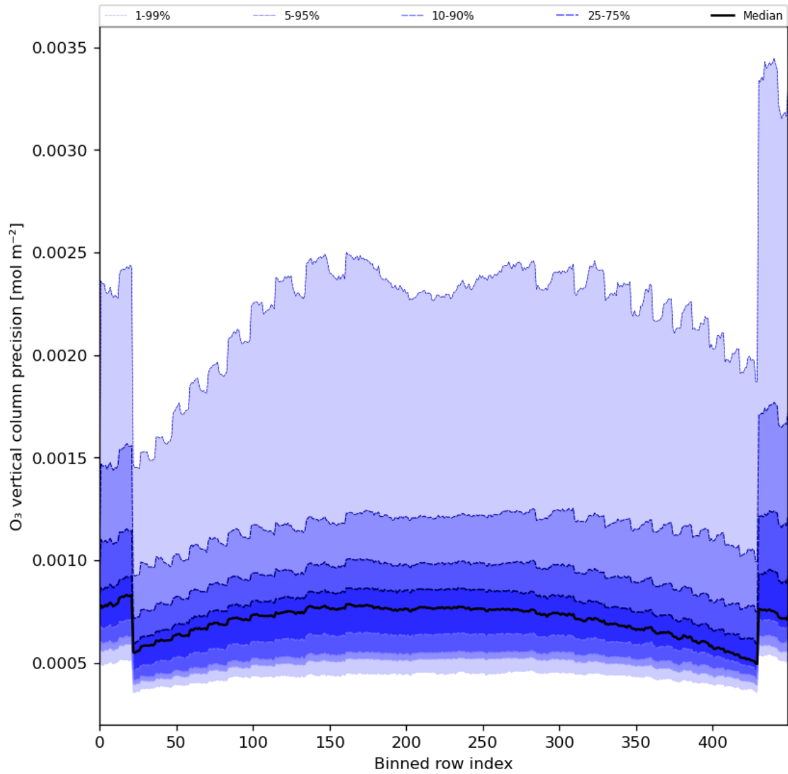
Figure 29: Along track statistics of “O 3 vertical column precision” for 2024-03-07 to 2024-03-09
