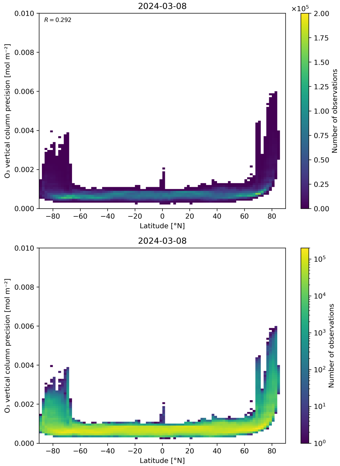
Figure 37: Scatter density plot of “Latitude” against “O 3 vertical column precision” for 2024-03-07 to 2024-03-09.
