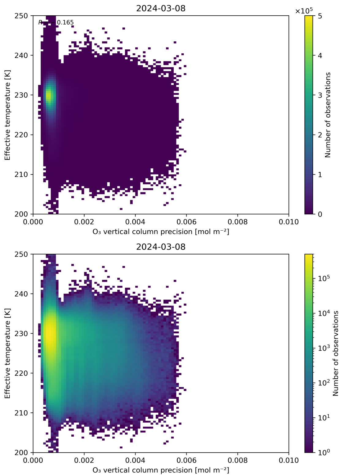
Figure 42: Scatter density plot of “O 3 vertical column precision” against “Effective temperature” for 2024-03-07 to 2024-03-09.
