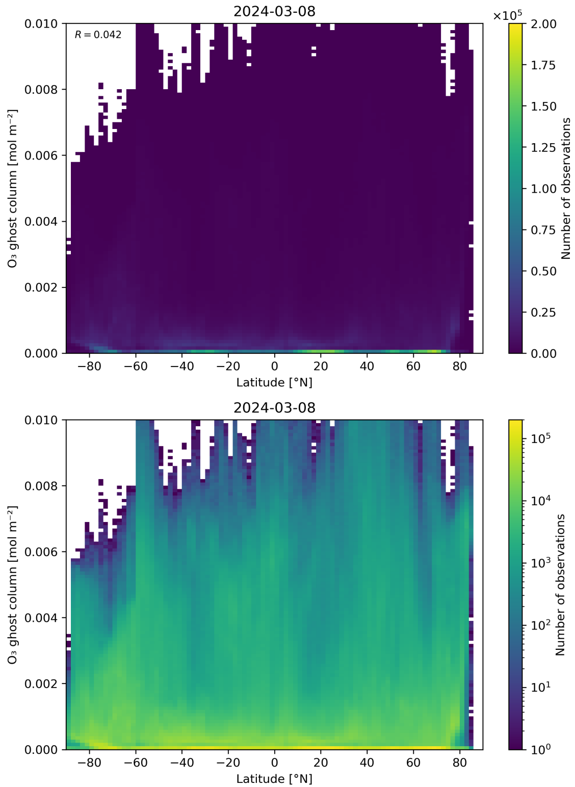
Figure 35: Scatter density plot of “Latitude” against “O 3 ghost column” for 2024-03-07 to 2024-03-09.
