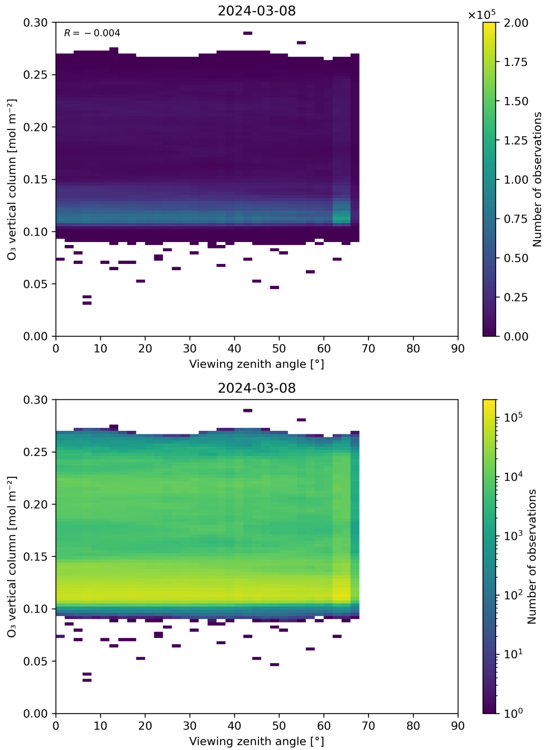
Figure 52: Scatter density plot of “Viewing zenith angle” against “O 3 vertical column” for 2024-03-07 to 2024-03-09.
