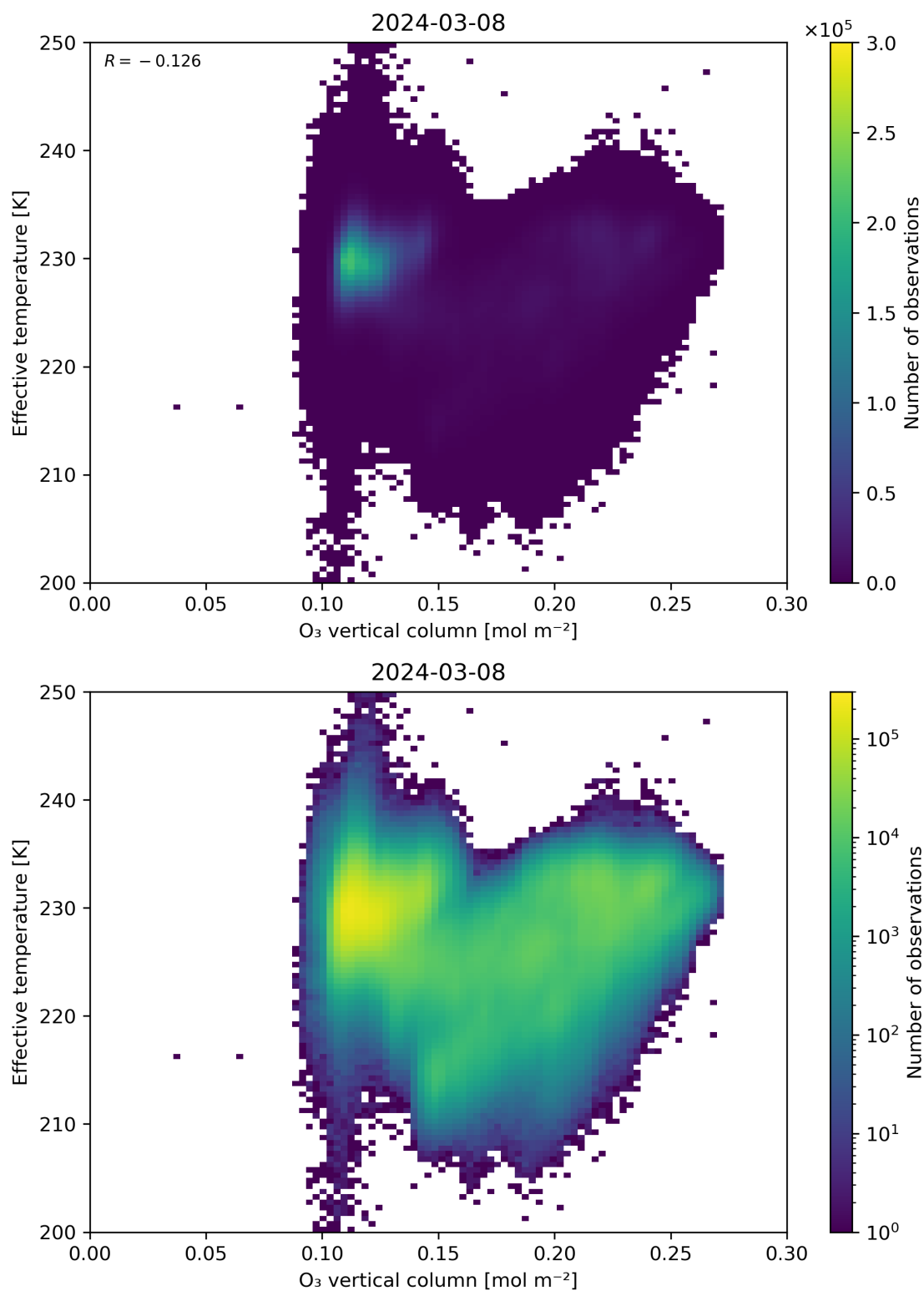
Figure 39: Scatter density plot of “O 3 vertical column” against “Effective temperature” for 2024-03-07 to 2024-03-09.
