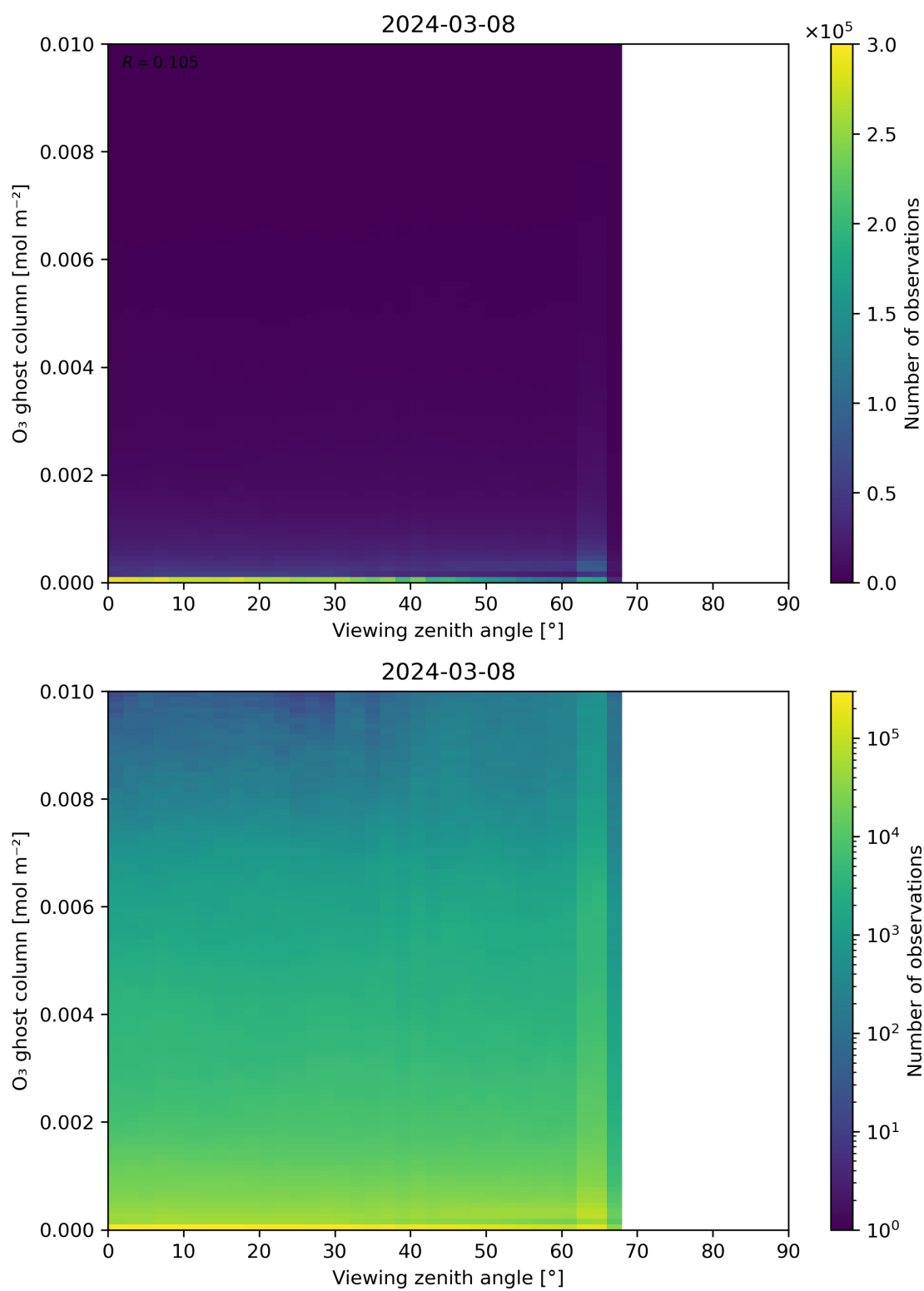
Figure 51: Scatter density plot of “Viewing zenith angle” against “O 3 ghost column” for 2024-03-07 to 2024-03-09.
