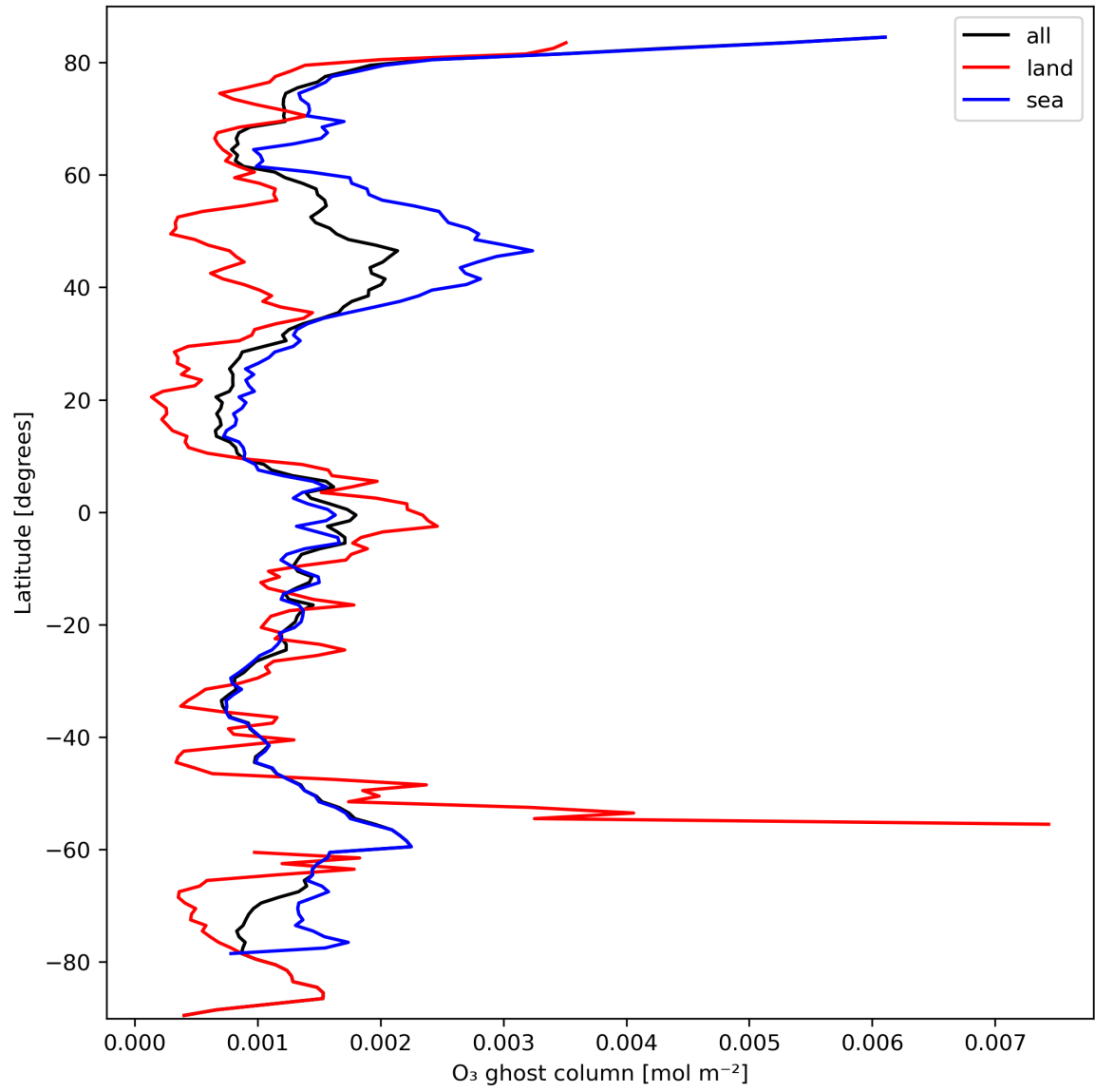
Figure 18: Zonal average of “O 3 ghost column” for 2024-03-07 to 2024-03-09.
