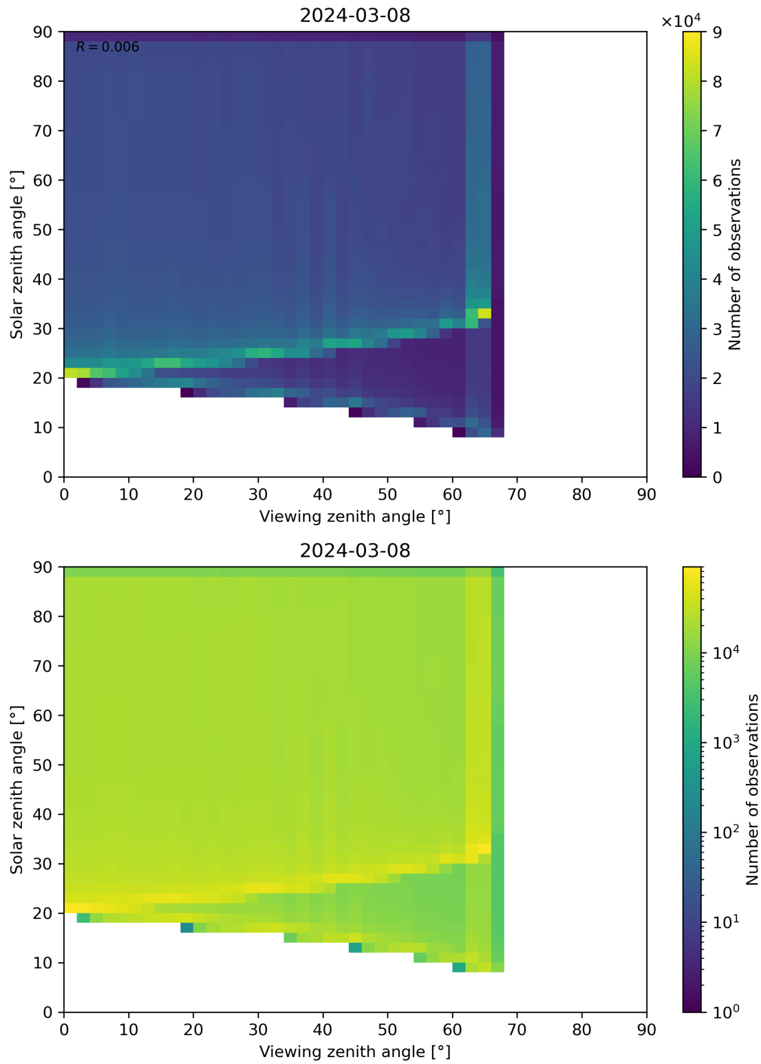
Figure 54: Scatter density plot of “Viewing zenith angle” against “Solar zenith angle” for 2024-03-07 to 2024-03-09.
