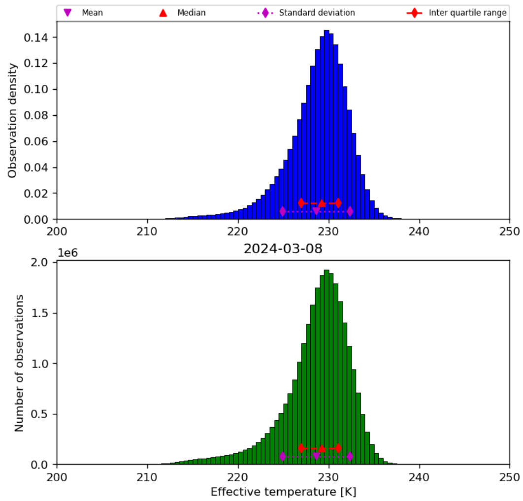
Figure 24: Histogram of “Effective temperature” for 2024-03-07 to 2024-03-09
