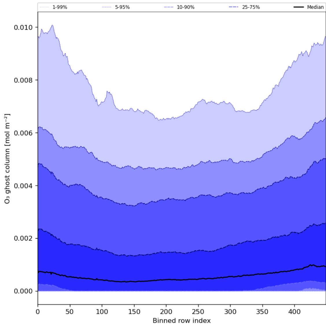
Figure 32: Along track statistics of “O 3 ghost column” for 2024-03-07 to 2024-03-09
