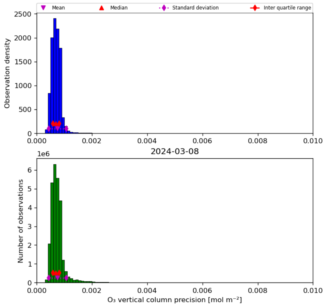
Figure 22: Histogram of “O 3 vertical column precision” for 2024-03-07 to 2024-03-09
