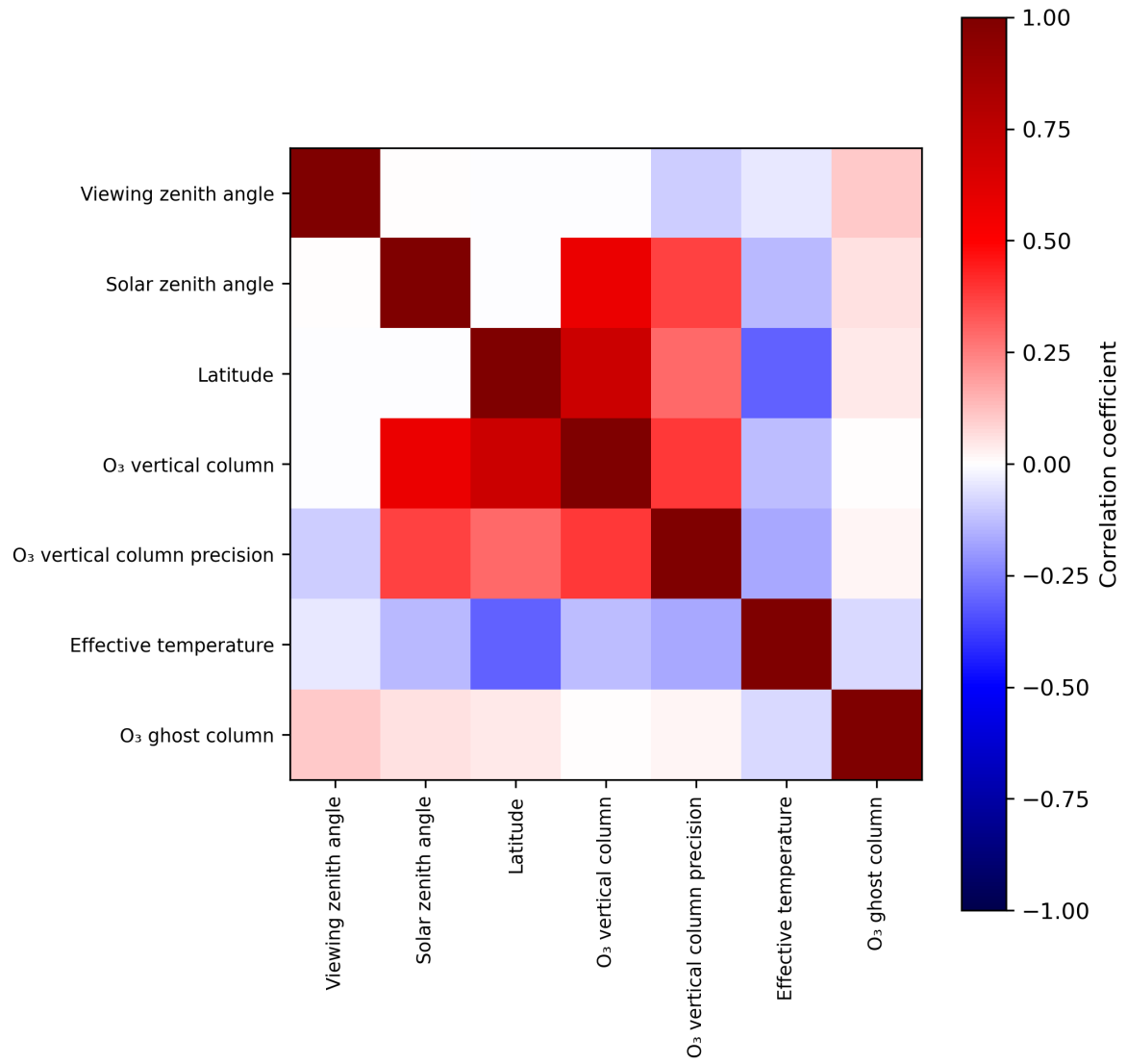
Figure 2: Map of correlation matrix for 2024-03-07 to 2024-03-09.
