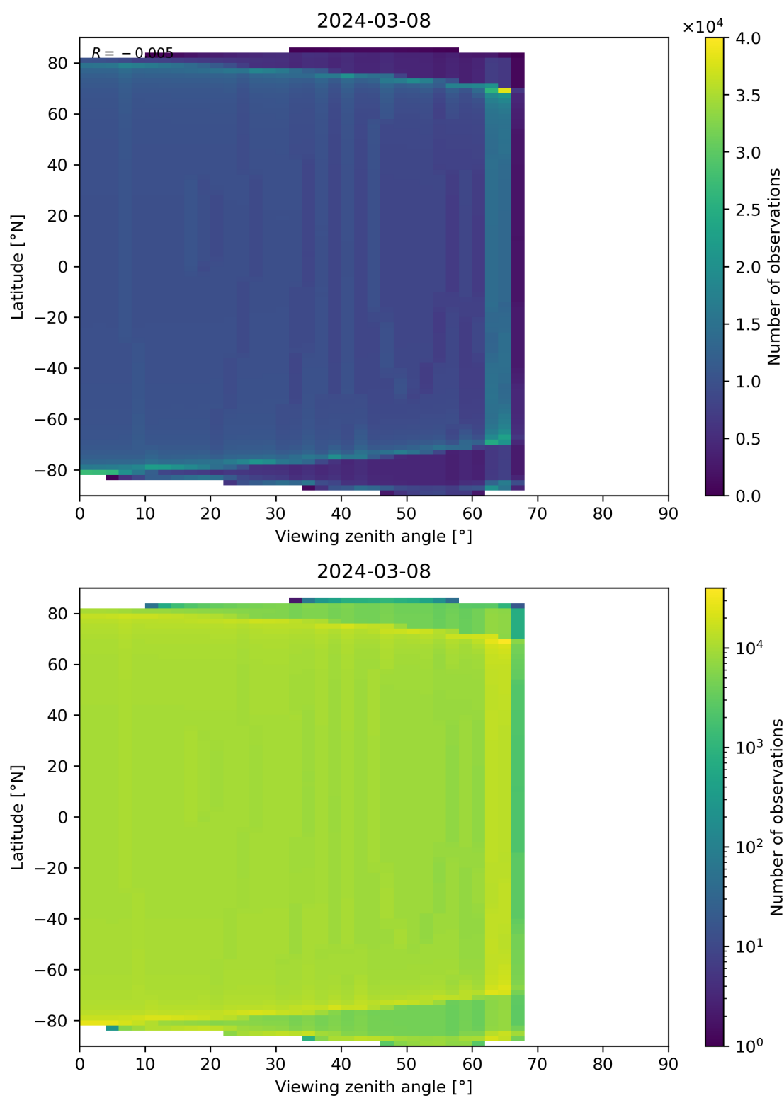
Figure 49: Scatter density plot of “Viewing zenith angle” against “Latitude” for 2024-03-07 to 2024-03-09.
