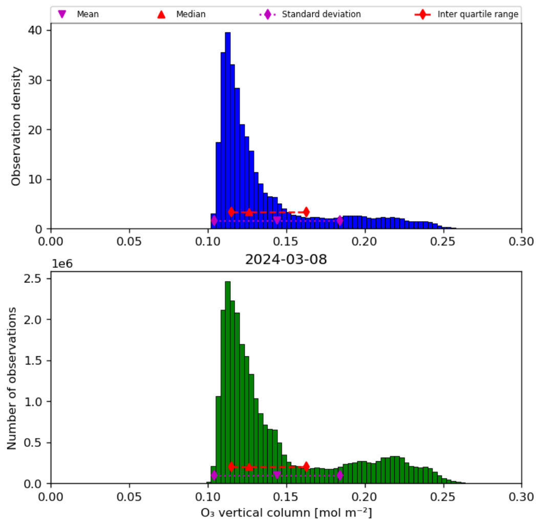
Figure 21: Histogram of “O 3 vertical column” for 2024-03-07 to 2024-03-09
