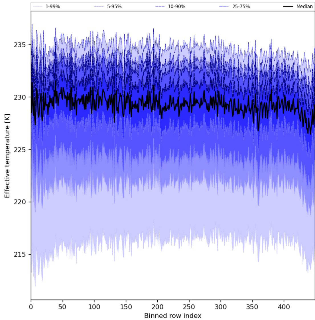
Figure 31: Along track statistics of “Effective temperature” for 2024-03-07 to 2024-03-09
