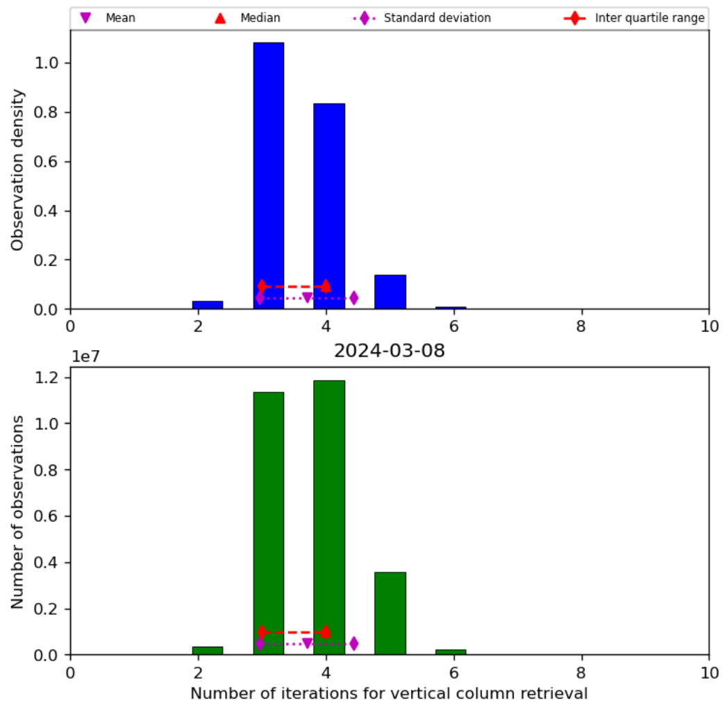
Figure 26: Histogram of “Number of iterations for vertical column retrieval” for 2024-03-07 to 2024-03-09
