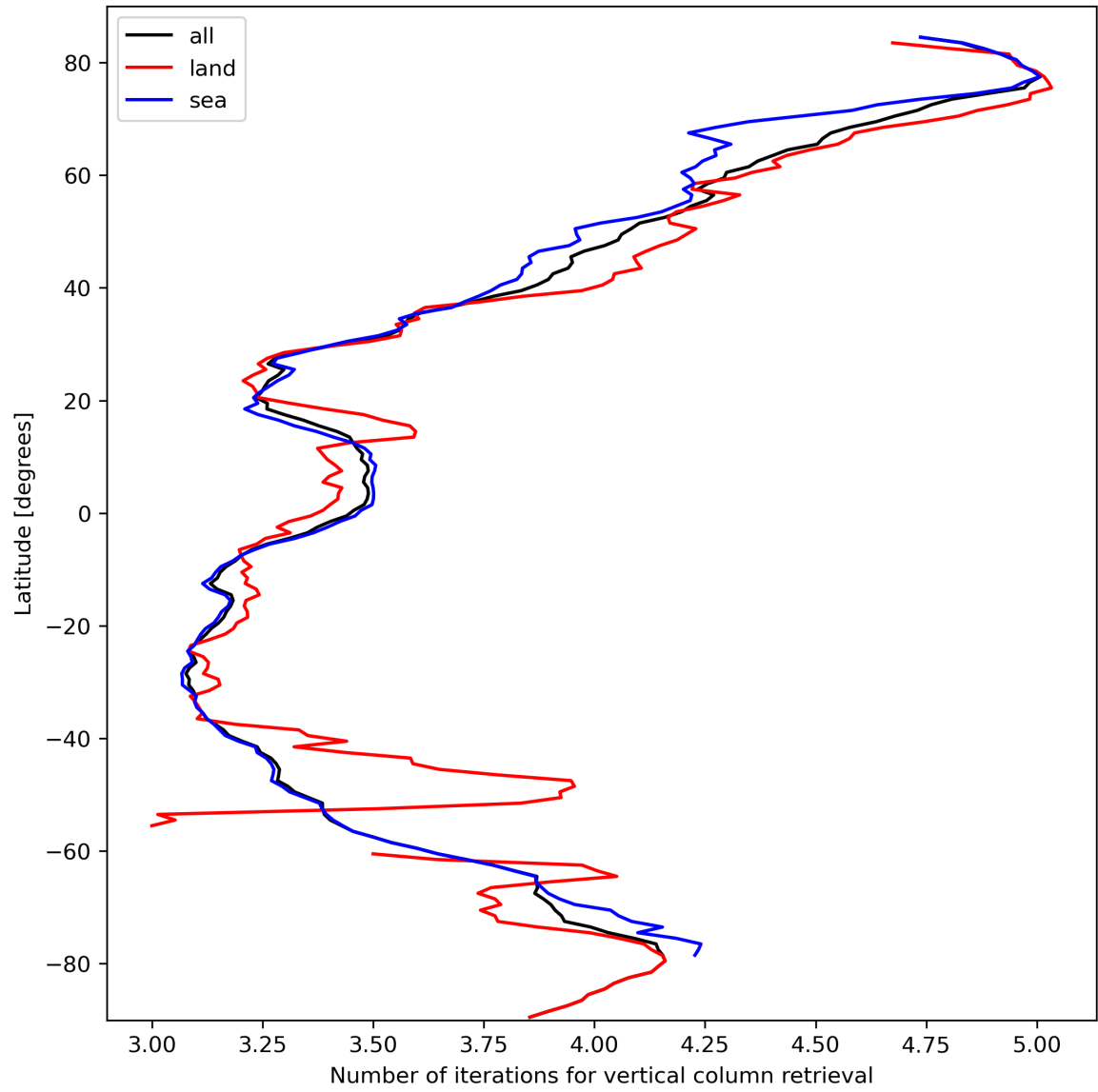
Figure 19: Zonal average of “Number of iterations for vertical column retrieval” for 2024-03-07 to 2024-03-09.
