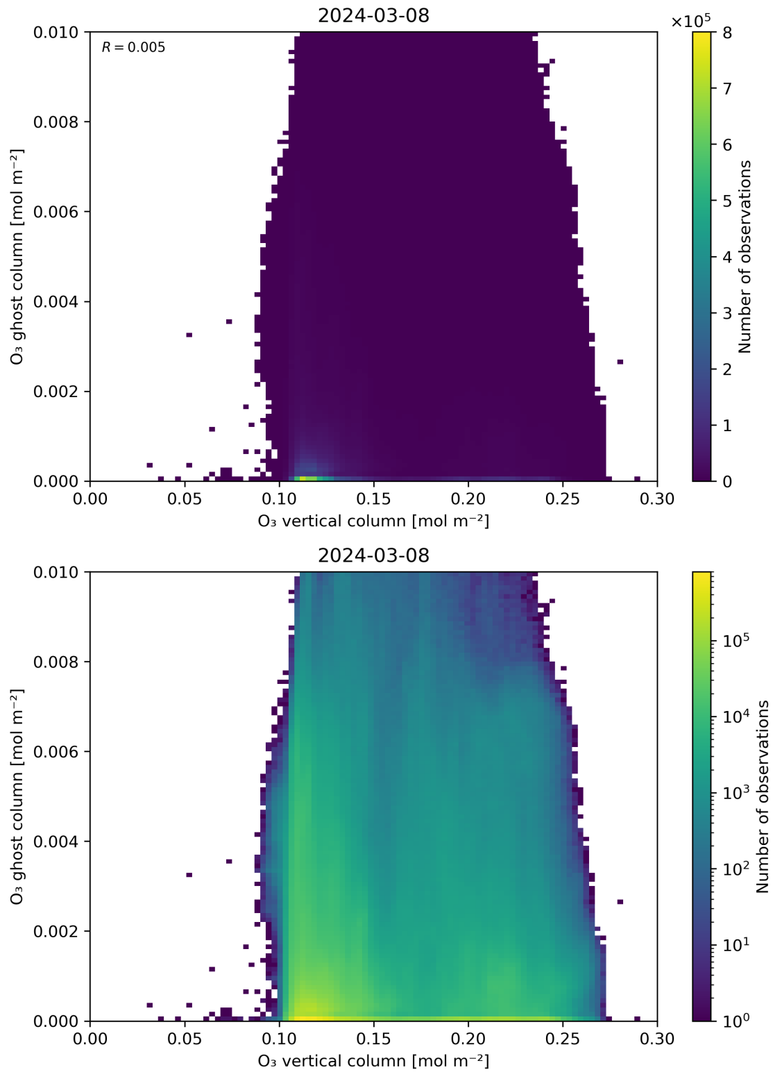
Figure 40: Scatter density plot of “O 3 vertical column” against “O 3 ghost column” for 2024-03-07 to 2024-03-09.
