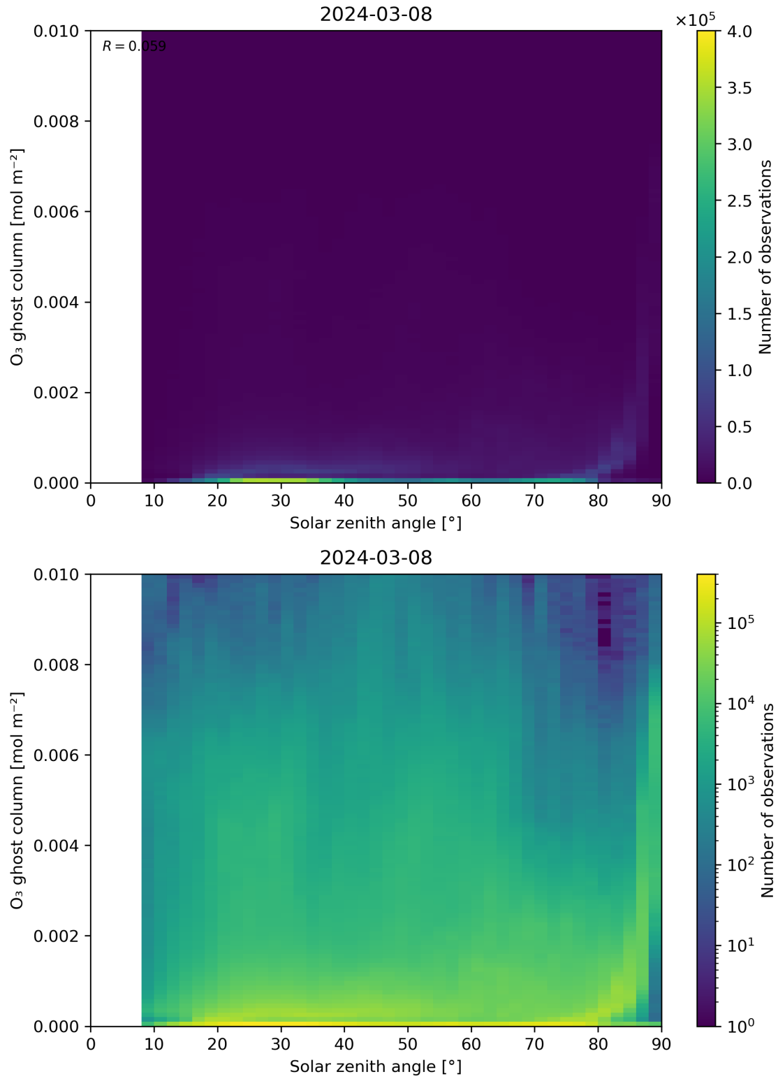
Figure 46: Scatter density plot of “Solar zenith angle” against “O 3 ghost column” for 2024-03-07 to 2024-03-09.
