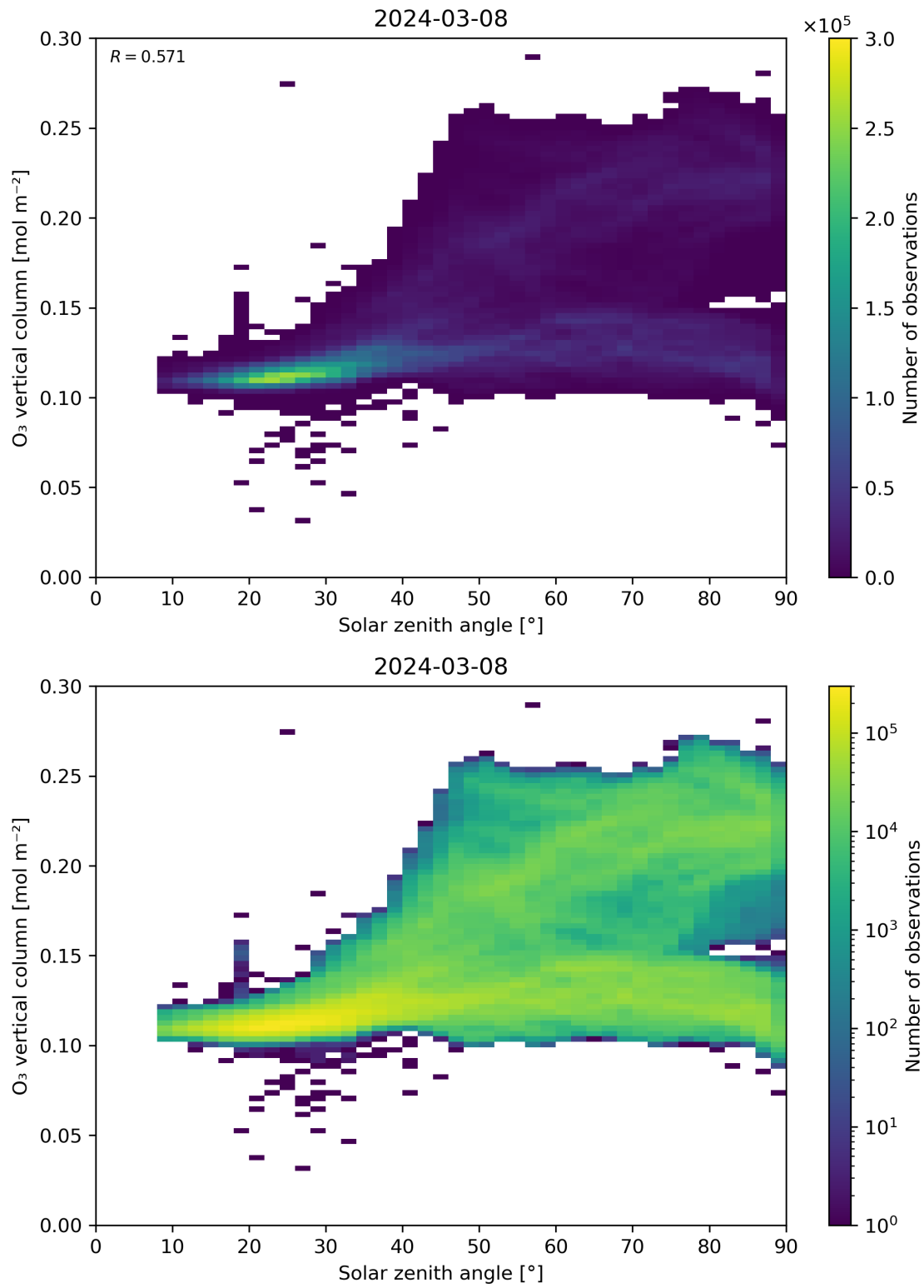
Figure 47: Scatter density plot of “Solar zenith angle” against “O 3 vertical column” for 2024-03-07 to 2024-03-09.
