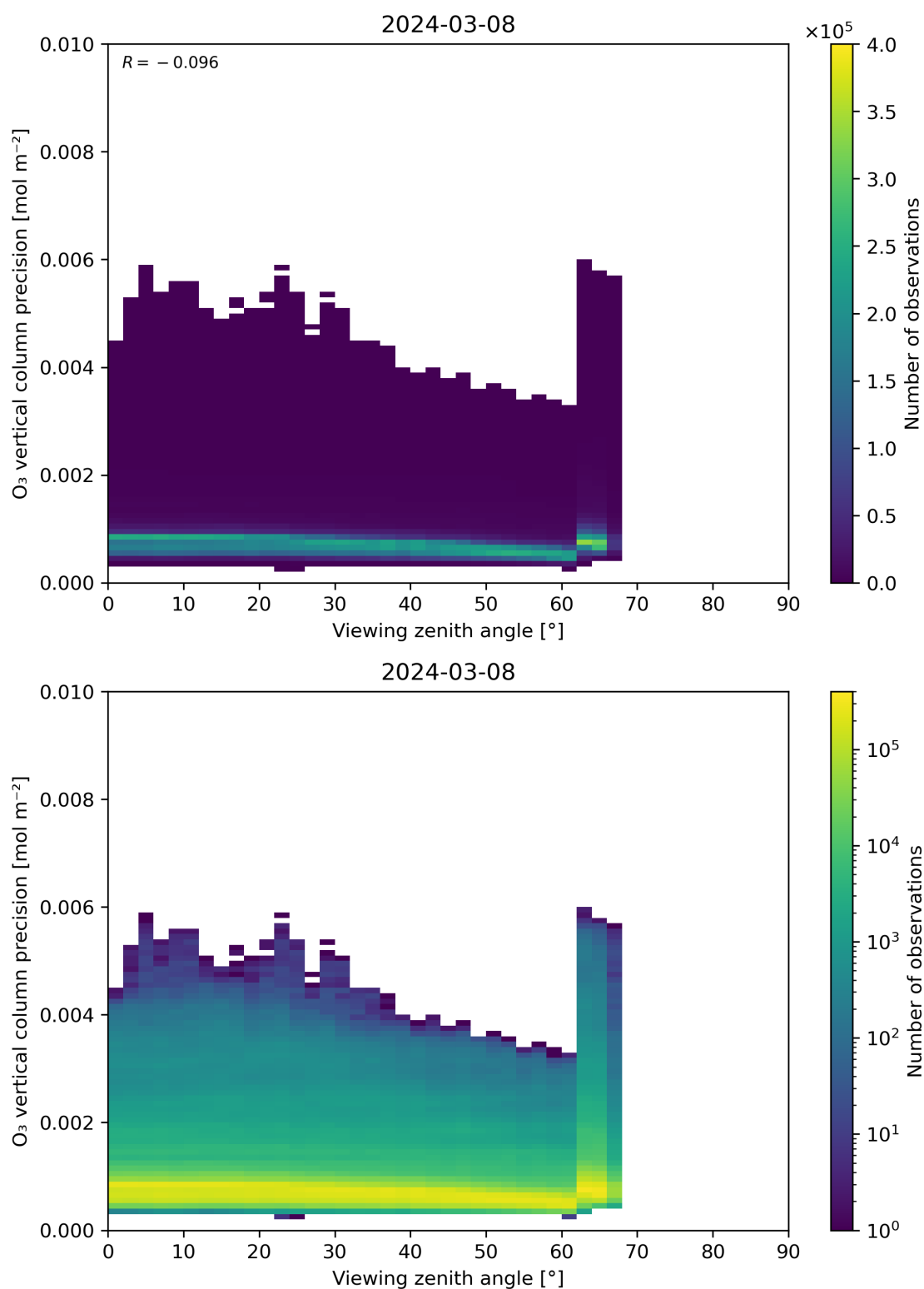
Figure 53: Scatter density plot of “Viewing zenith angle” against “O 3 vertical column precision” for 2024-03-07 to 2024-03-09.
