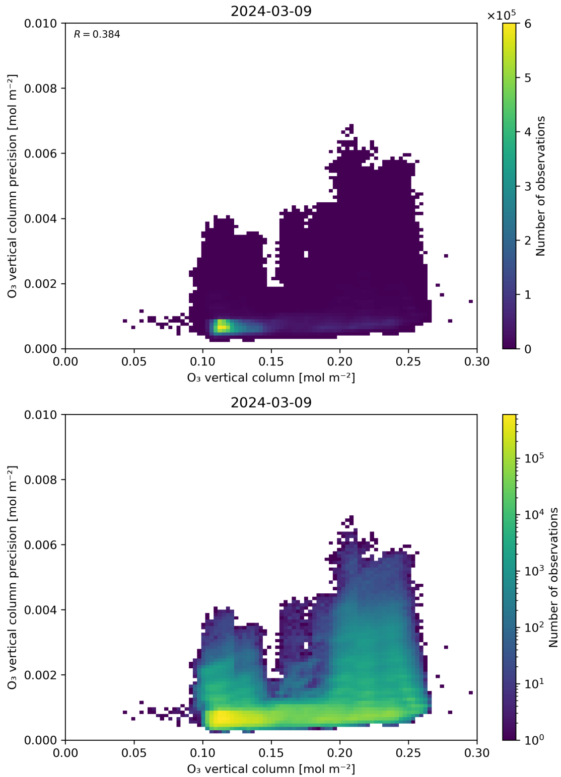
Figure 41: Scatter density plot of “O 3 vertical column” against “O 3 vertical column precision” for 2024-03-09 to 2024-03-10.
