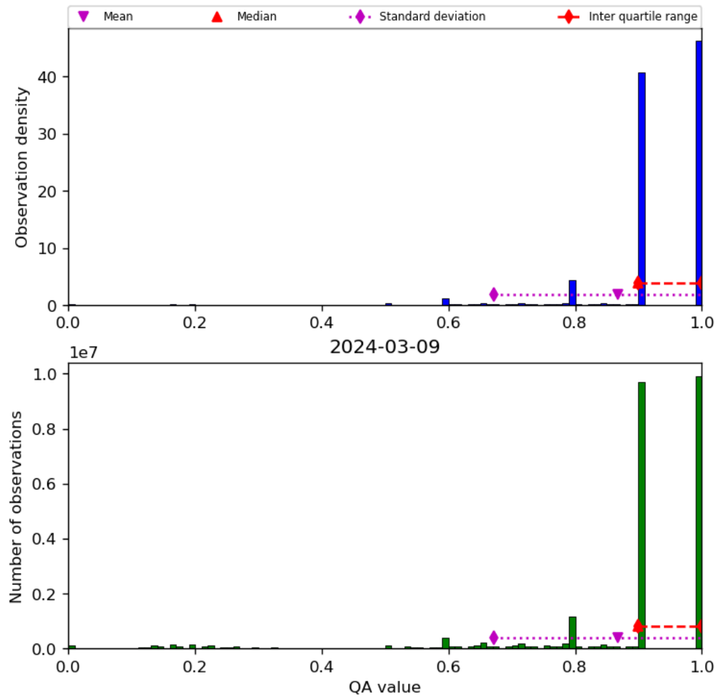
Figure 20: Histogram of “QA value” for 2024-03-09 to 2024-03-10
