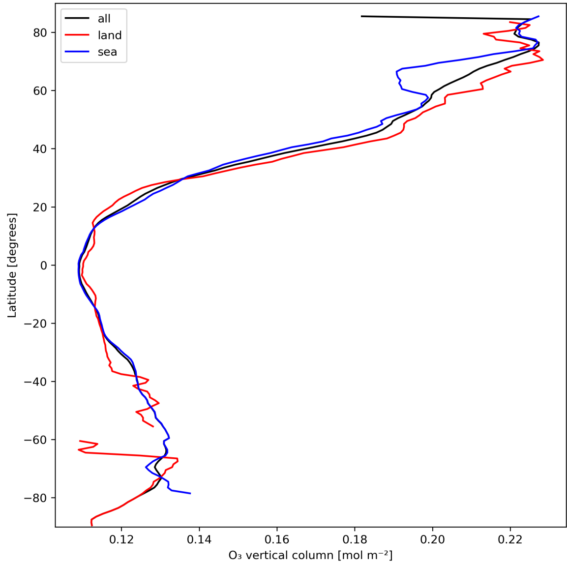
Figure 14: Zonal average of “O 3 vertical column” for 2024-03-09 to 2024-03-10.
