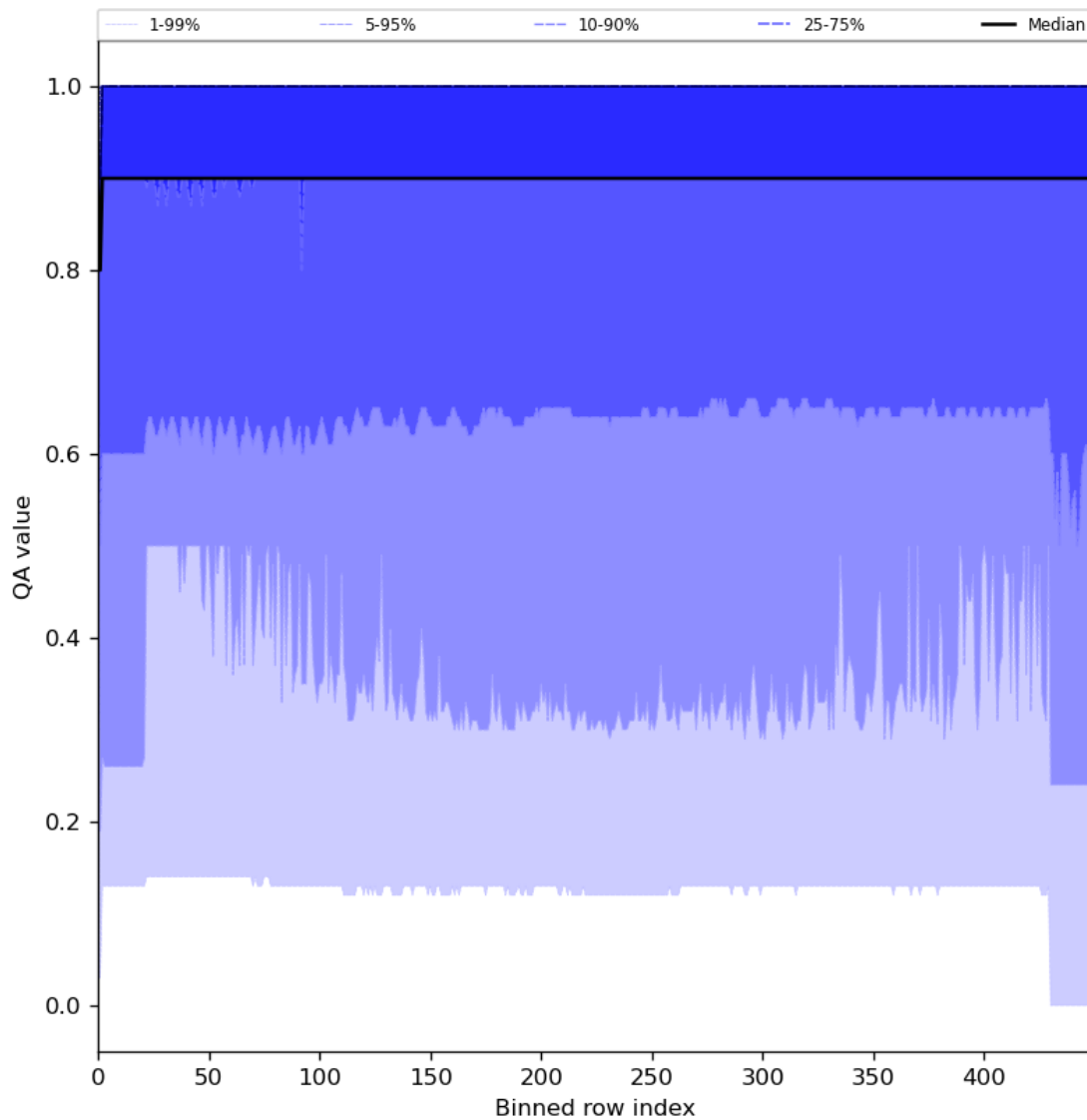
Figure 27: Along track statistics of “QA value” for 2024-03-09 to 2024-03-10
