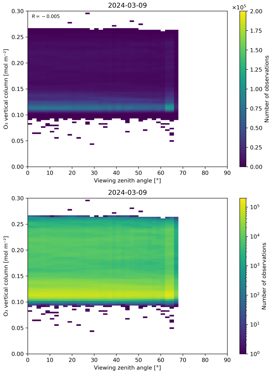
Figure 52: Scatter density plot of “Viewing zenith angle” against “O 3 vertical column” for 2024-03-09 to 2024-03-10.
