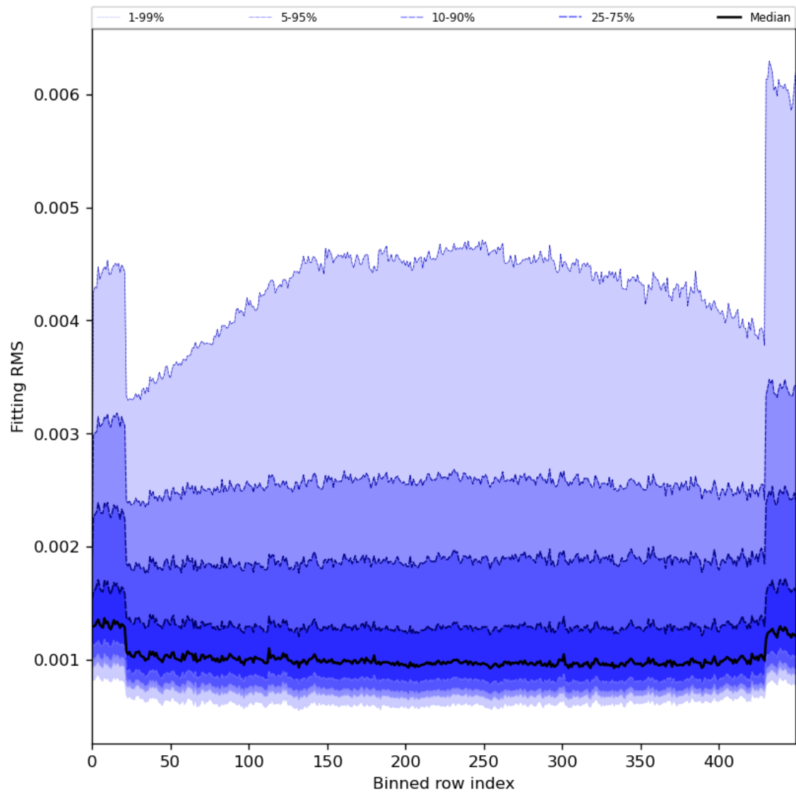
Figure 30: Along track statistics of “Fitting RMS” for 2024-03-09 to 2024-03-10
