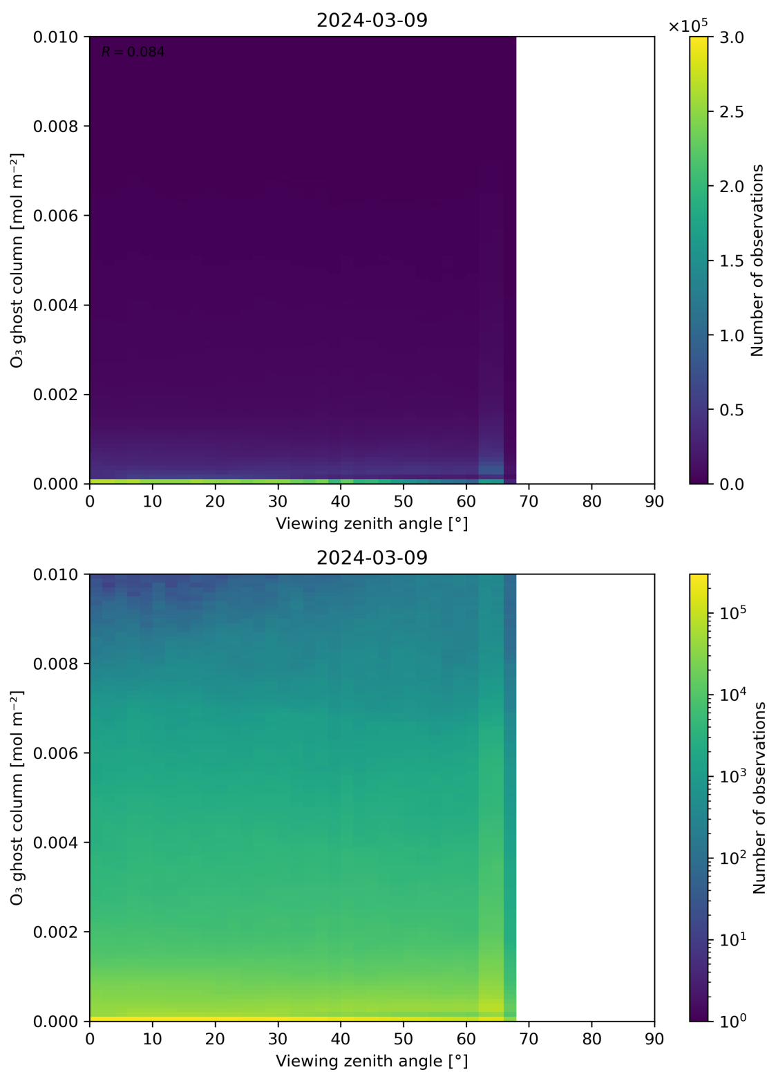
Figure 51: Scatter density plot of “Viewing zenith angle” against “O 3 ghost column” for 2024-03-09 to 2024-03-10.
