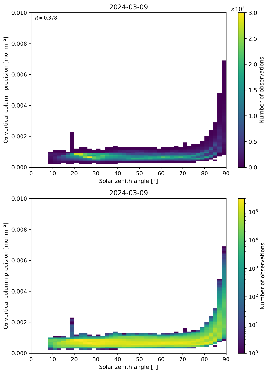
Figure 48: Scatter density plot of “Solar zenith angle” against “O 3 vertical column precision” for 2024-03-09 to 2024-03-10.
