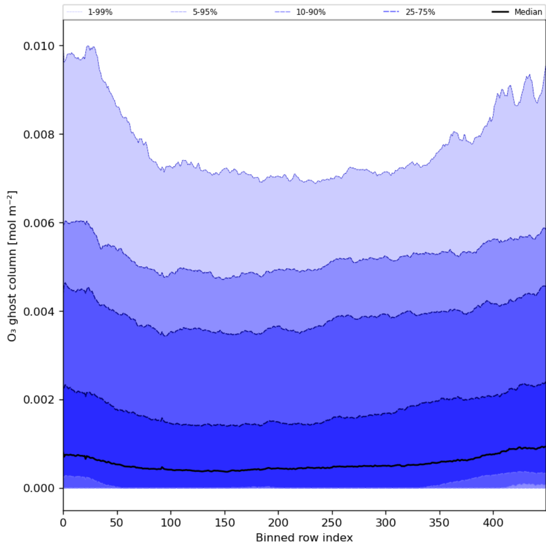
Figure 32: Along track statistics of “O 3 ghost column” for 2024-03-09 to 2024-03-10
