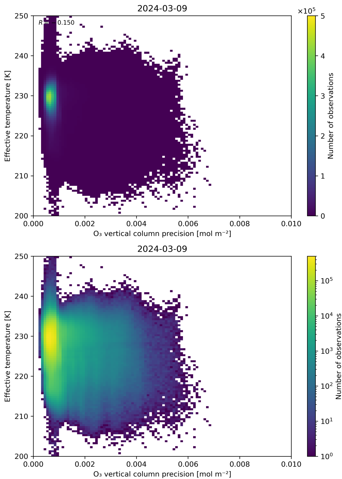
Figure 42: Scatter density plot of "O 3 vertical column precision" against "Effective temperature" for 2024-03-09 to 2024-03-10.
