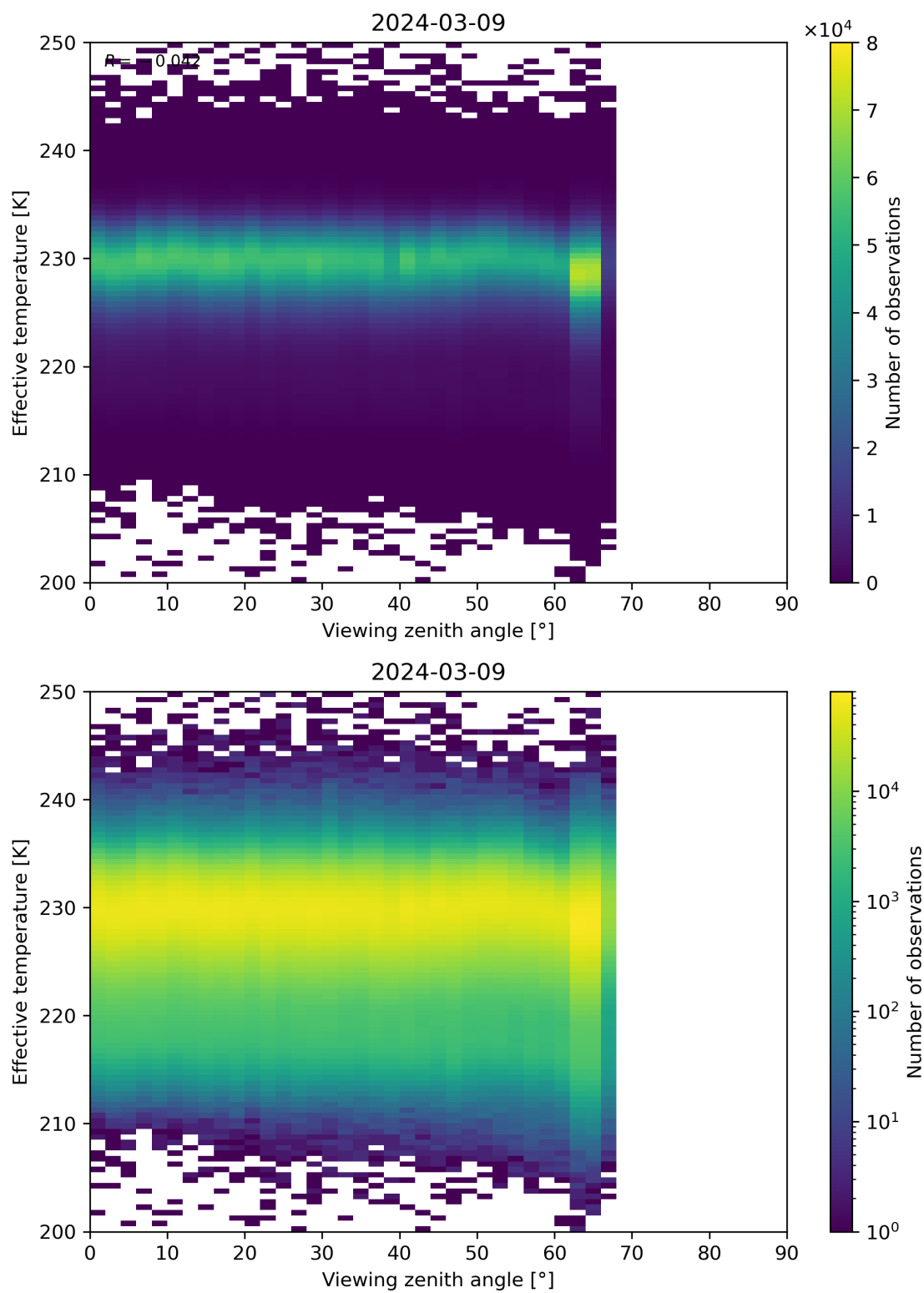
Figure 50: Scatter density plot of “Viewing zenith angle” against “Effective temperature” for 2024-03-09 to 2024-03-10.
