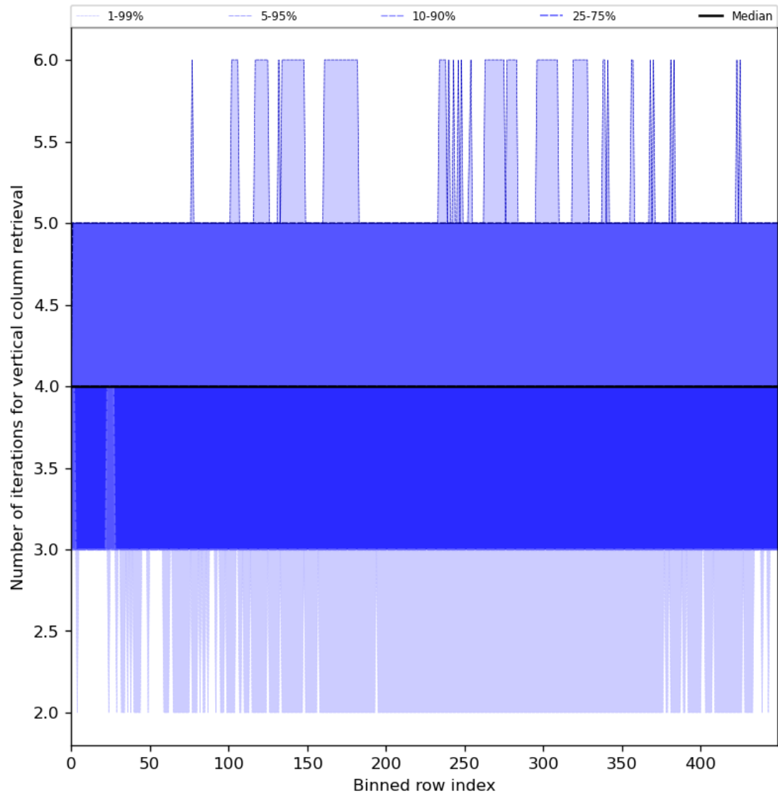
Figure 33: Along track statistics of “Number of iterations for vertical column retrieval” for 2024-03-09 to 2024-03-10
