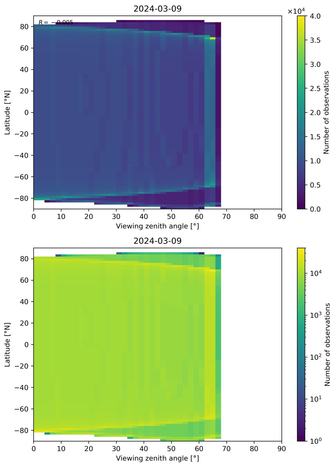
Figure 49: Scatter density plot of “Viewing zenith angle” against “Latitude” for 2024-03-09 to 2024-03-10.
