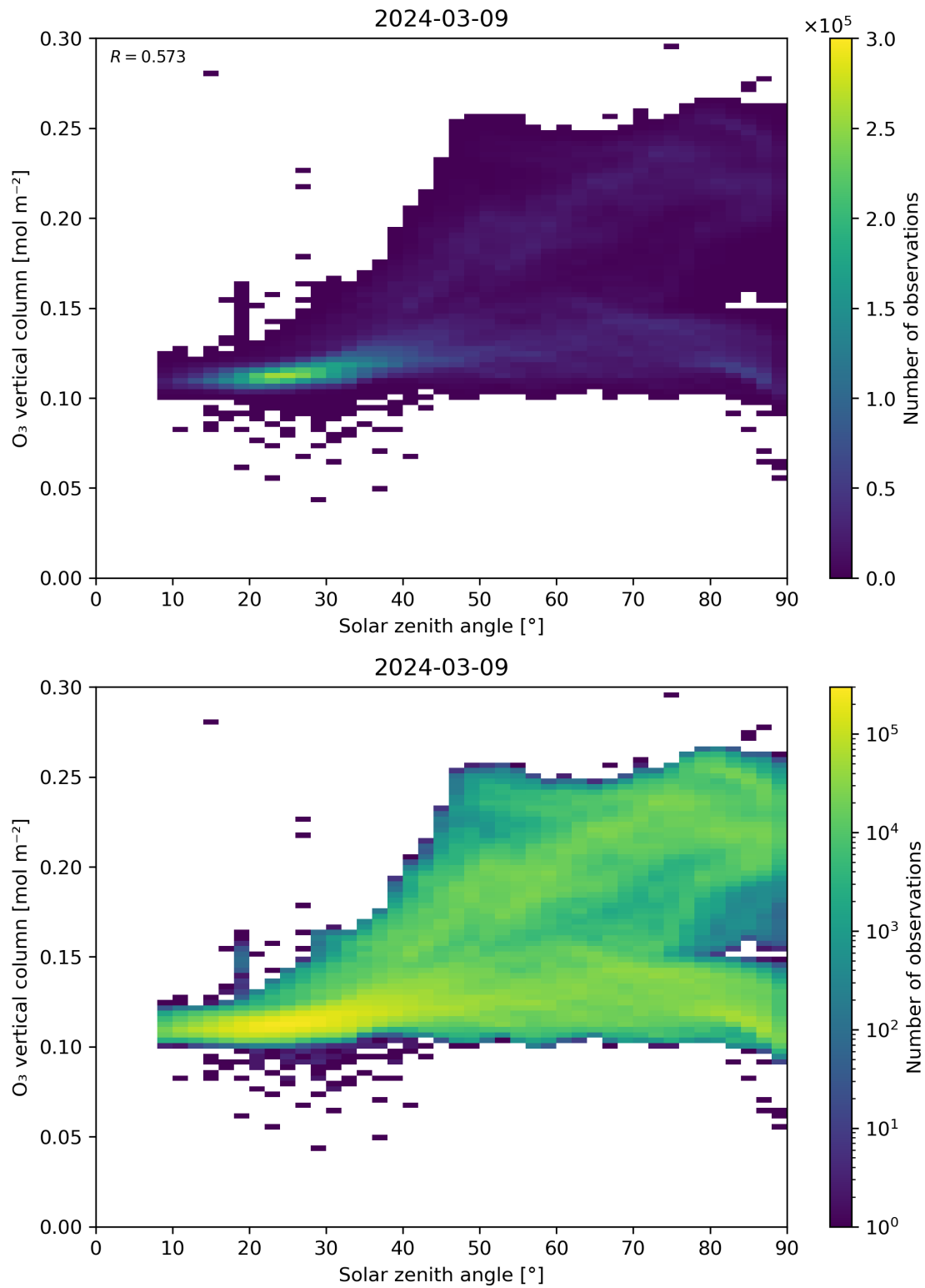
Figure 47: Scatter density plot of “Solar zenith angle” against “O 3 vertical column” for 2024-03-09 to 2024-03-10.
