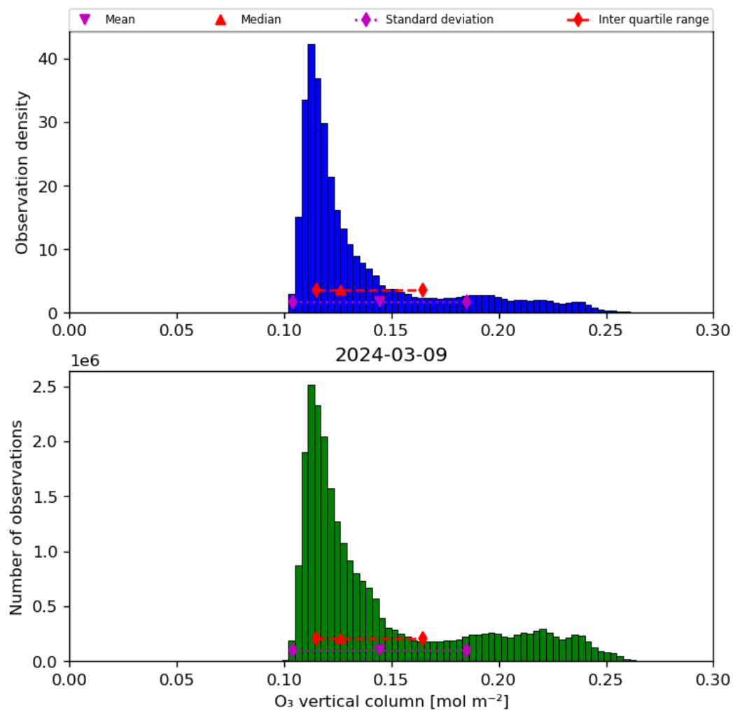
Figure 21: Histogram of “O 3 vertical column” for 2024-03-09 to 2024-03-10
