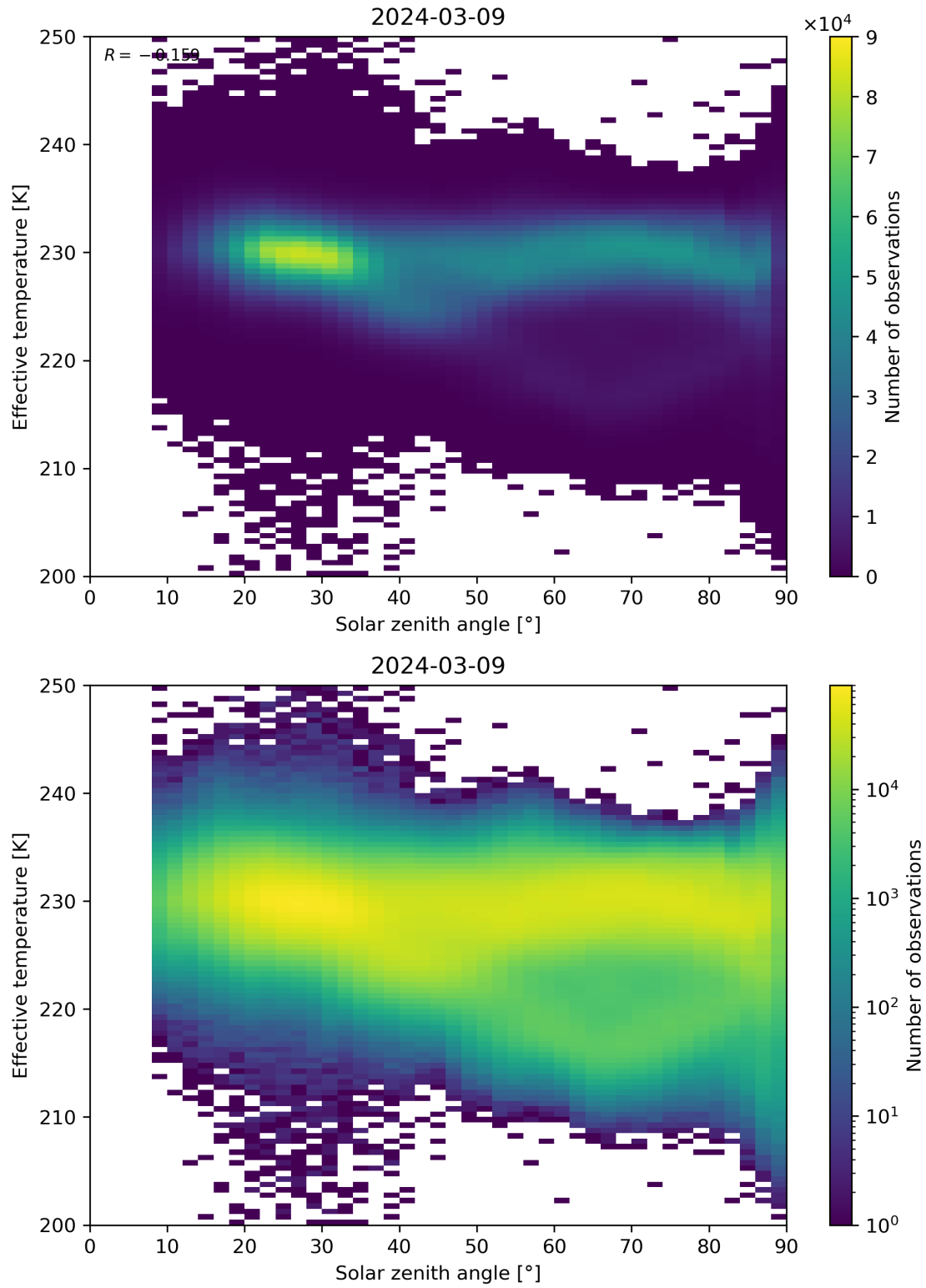
Figure 45: Scatter density plot of “Solar zenith angle” against “Effective temperature” for 2024-03-09 to 2024-03-10.
