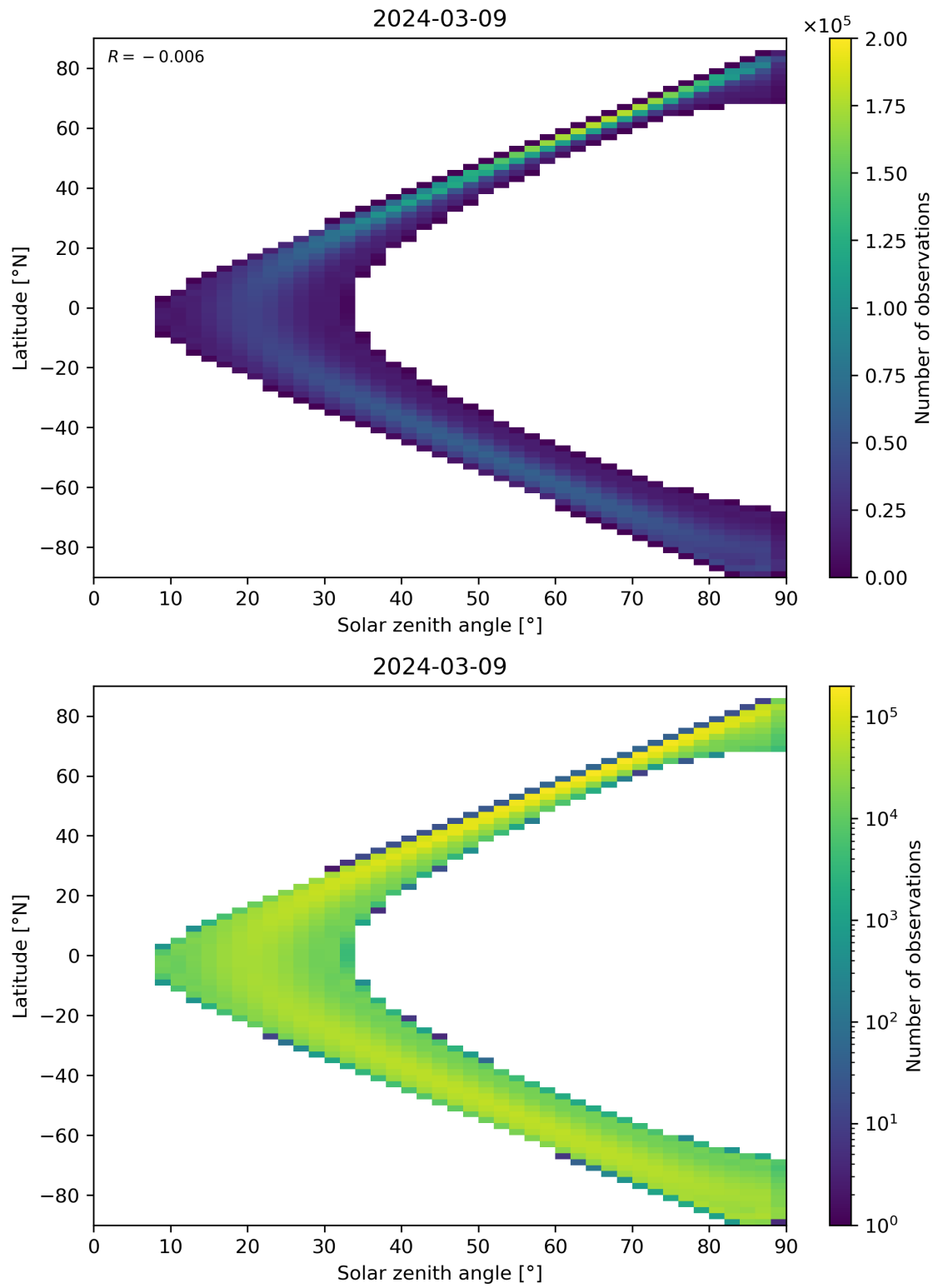
Figure 44: Scatter density plot of “Solar zenith angle” against “Latitude” for 2024-03-09 to 2024-03-10.
