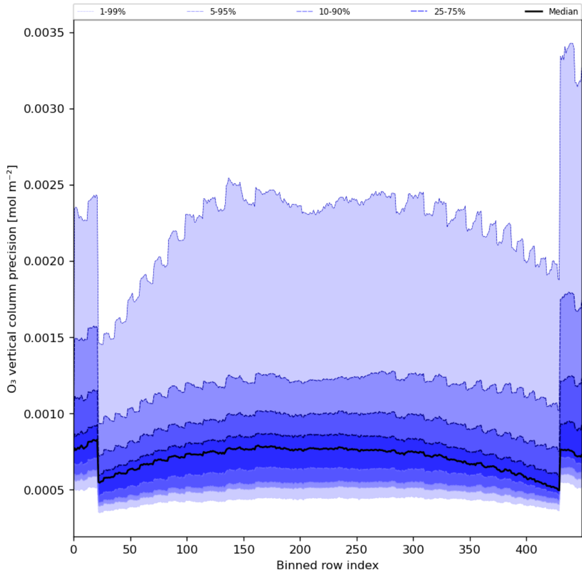
Figure 29: Along track statistics of “O 3 vertical column precision” for 2024-03-09 to 2024-03-10
