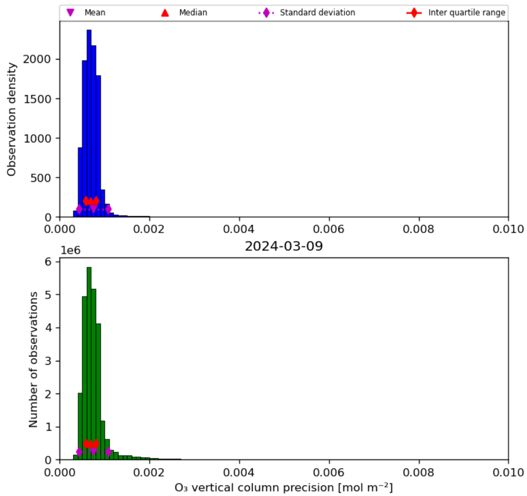
Figure 22: Histogram of “O 3 vertical column precision” for 2024-03-09 to 2024-03-10
