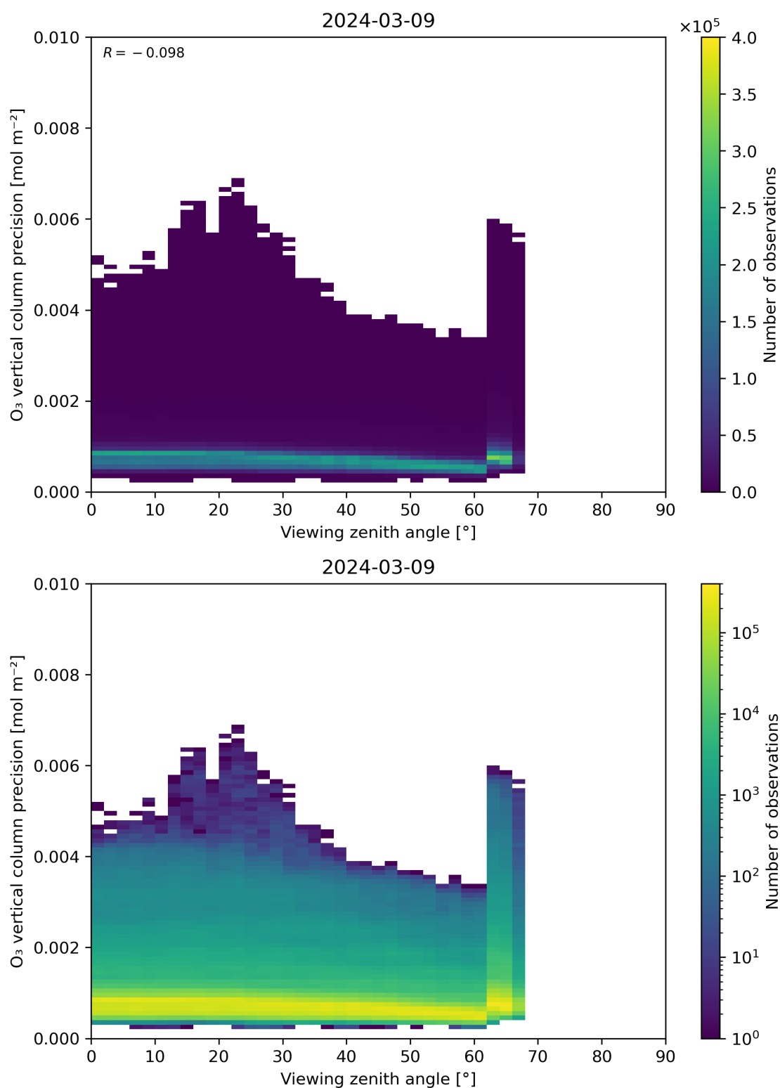
Figure 53: Scatter density plot of “Viewing zenith angle” against “O 3 vertical column precision” for 2024-03-09 to 2024-03-10.
