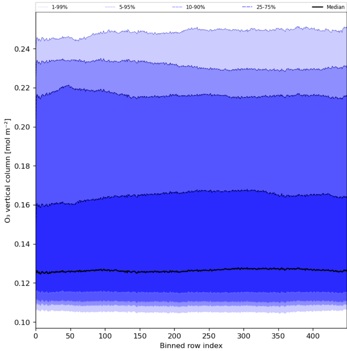
Figure 28: Along track statistics of “O 3 vertical column” for 2024-03-09 to 2024-03-10
