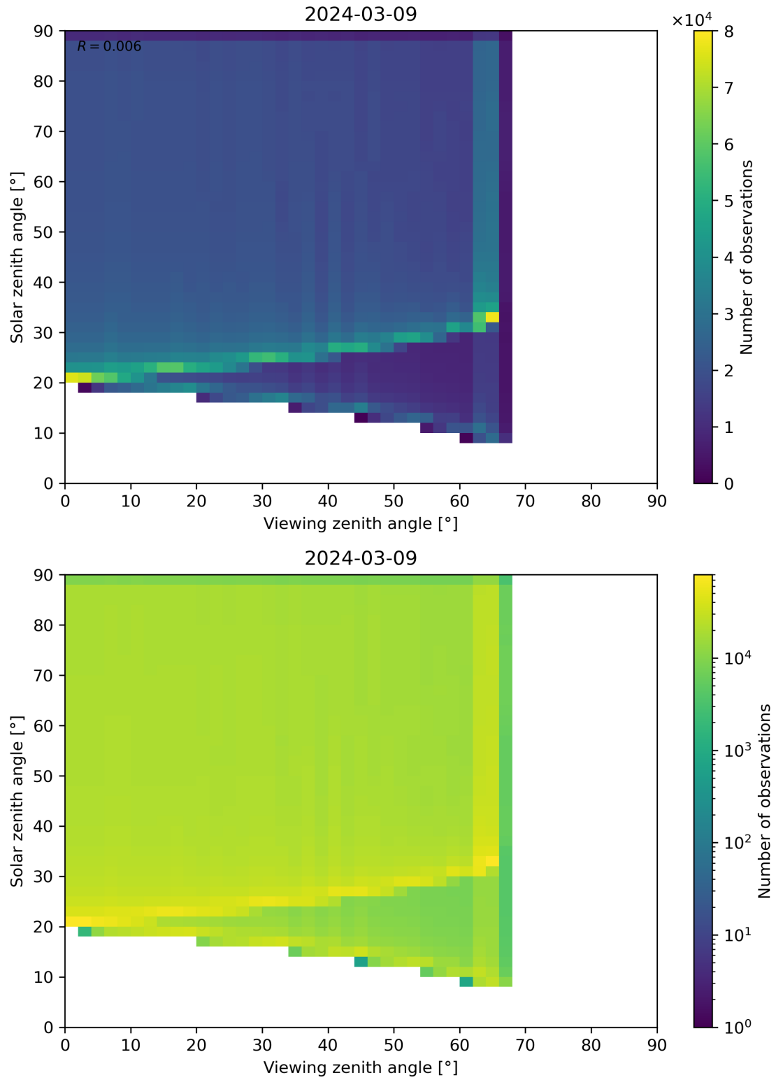
Figure 54: Scatter density plot of “Viewing zenith angle” against “Solar zenith angle” for 2024-03-09 to 2024-03-10.
