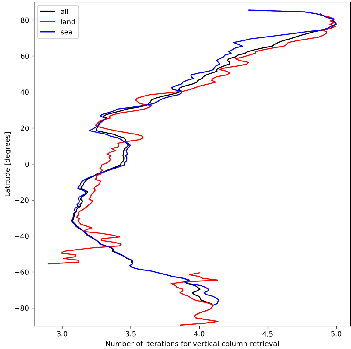
Figure 19: Zonal average of “Number of iterations for vertical column retrieval” for 2024-03-09 to 2024-03-10.
