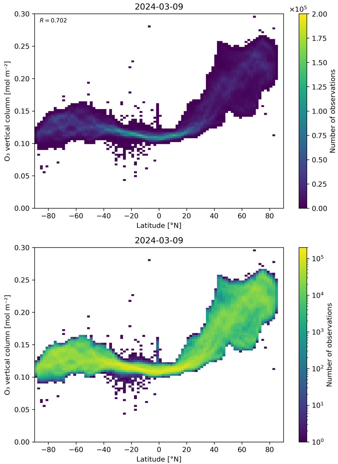
Figure 36: Scatter density plot of “Latitude” against “O 3 vertical column” for 2024-03-09 to 2024-03-10.
