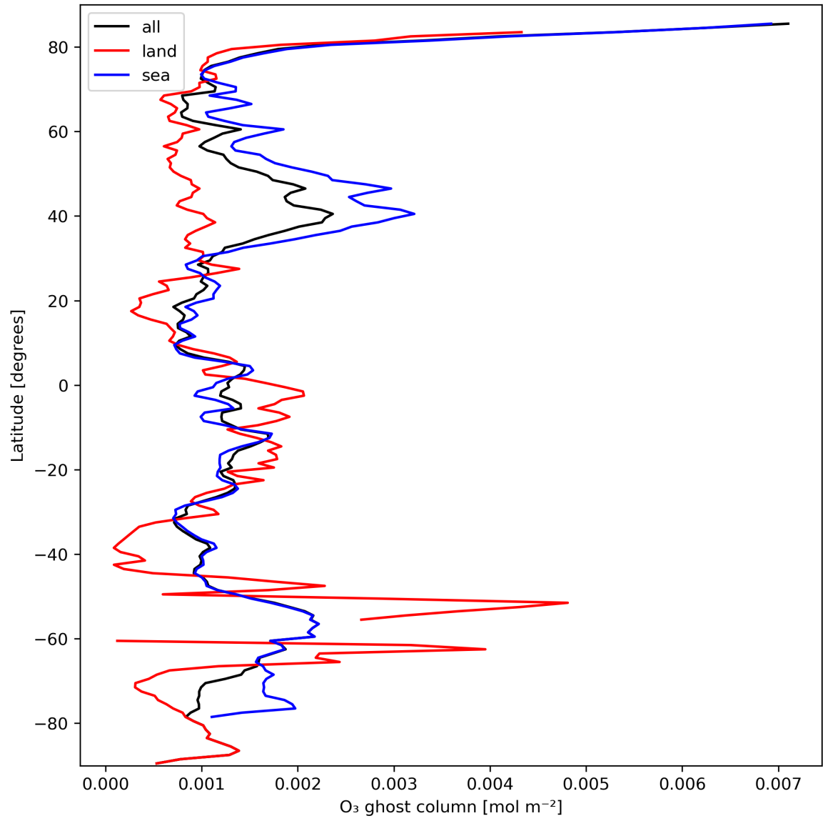
Figure 18: Zonal average of “O 3 ghost column” for 2024-03-09 to 2024-03-10.
