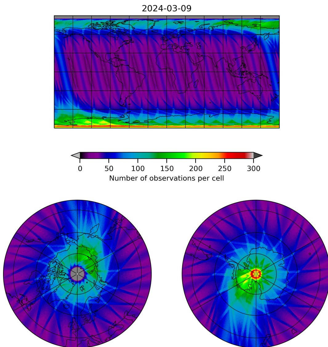
Figure 12: Map of the number of observations for 2024-03-09 to 2024-03-10
