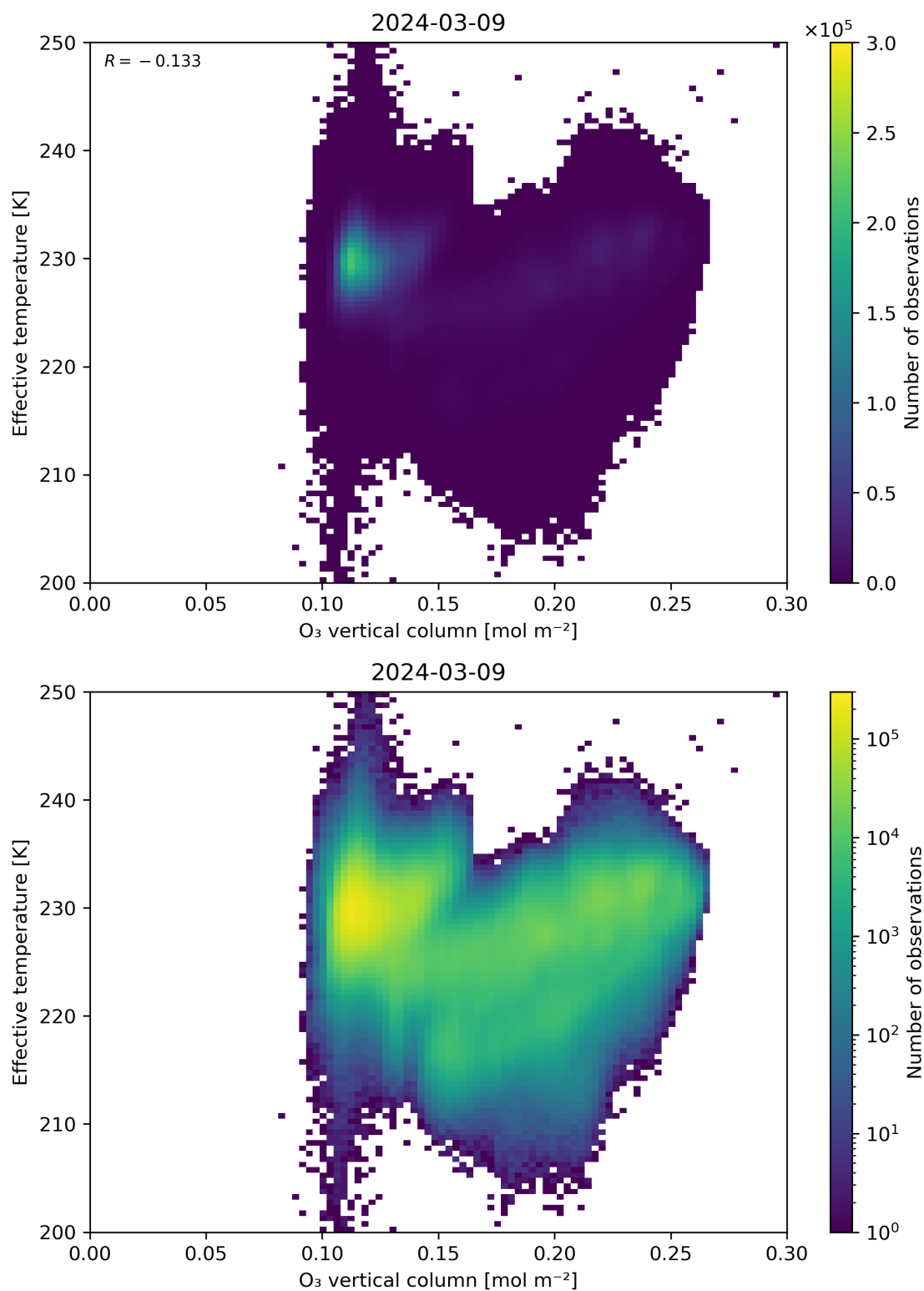
Figure 39: Scatter density plot of “O 3 vertical column” against “Effective temperature” for 2024-03-09 to 2024-03-10.
