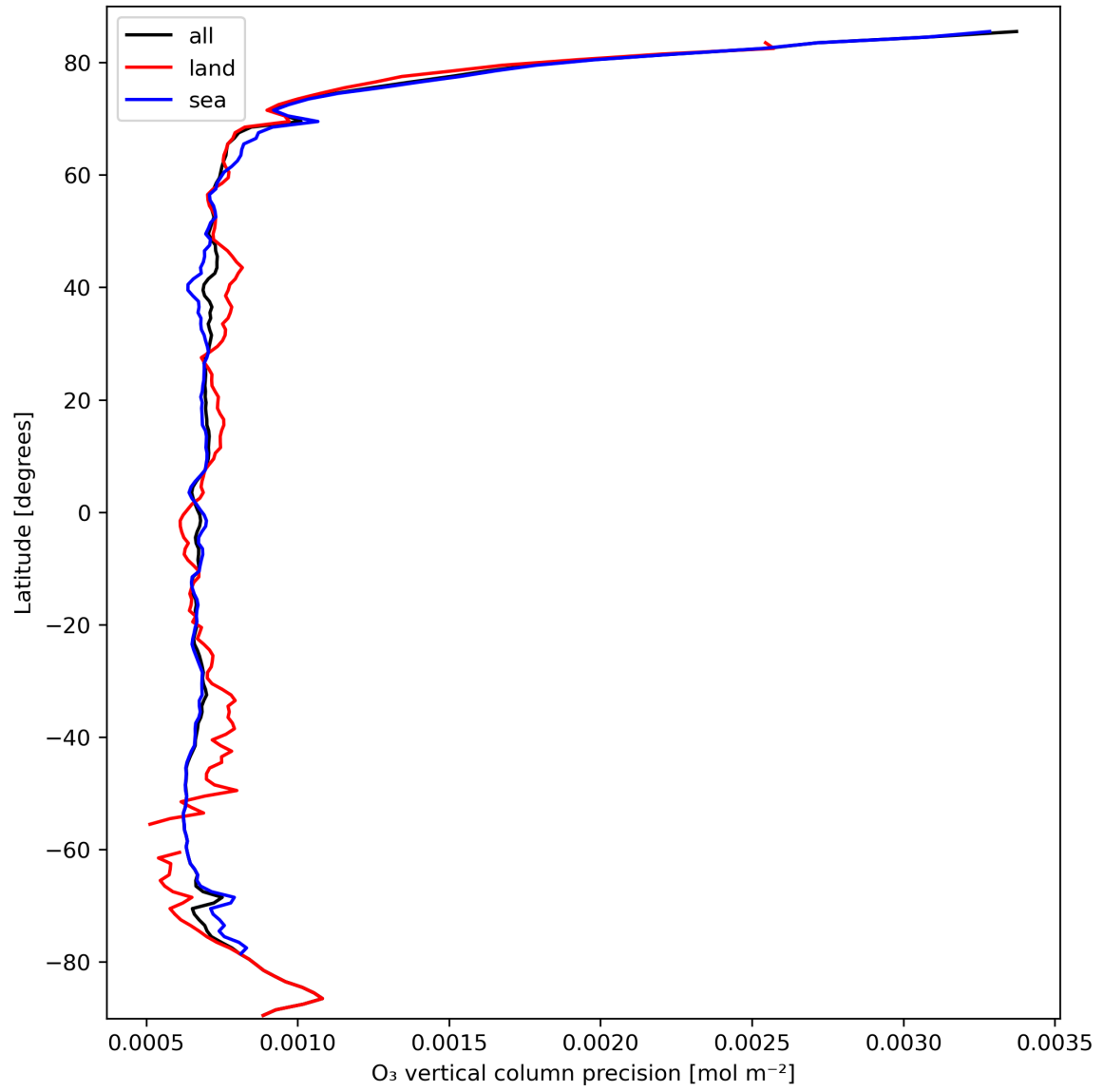
Figure 15: Zonal average of "O 3 vertical column precision" for 2024-03-09 to 2024-03-10.
