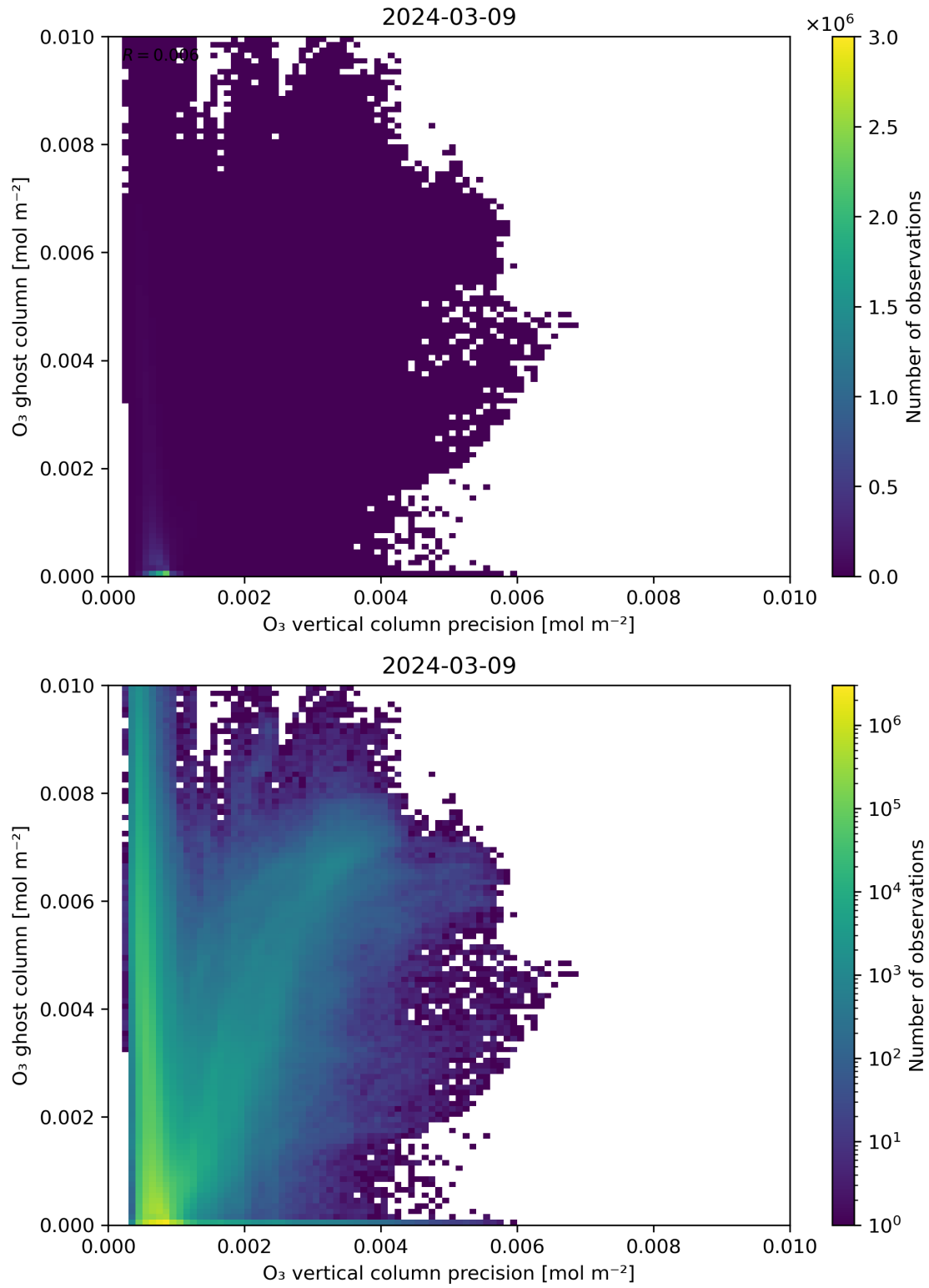
Figure 43: Scatter density plot of “ \text{O}_3 vertical column precision” against “ \text{O}_3 ghost column” for 2024-03-09 to 2024-03-10.
