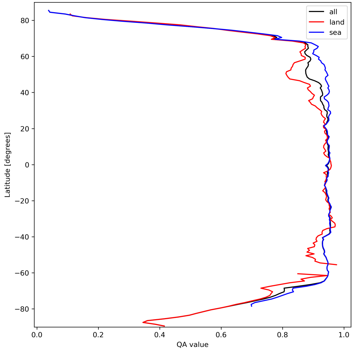
Figure 13: Zonal average of “QA value” for 2024-03-09 to 2024-03-10.
