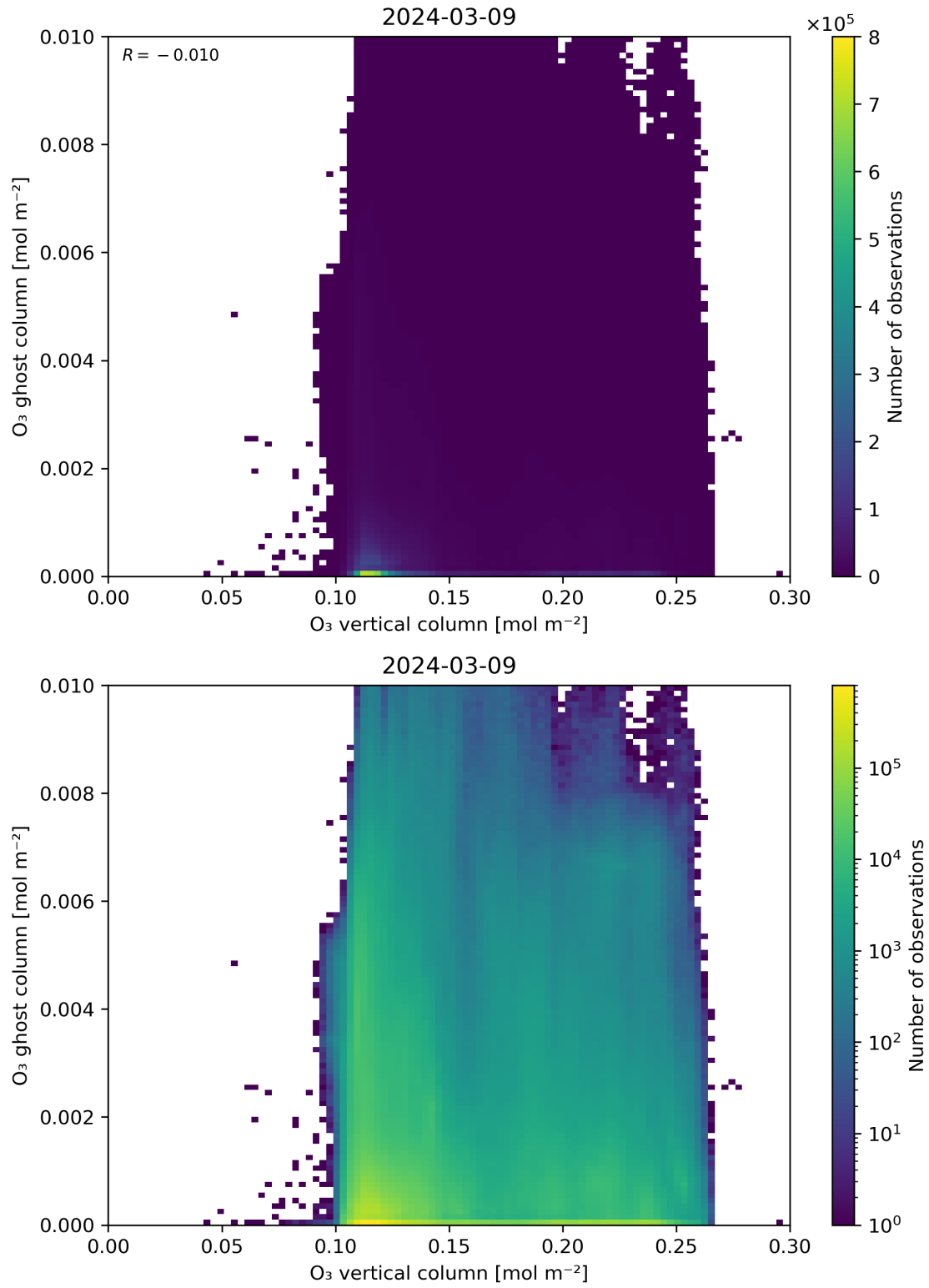
Figure 40: Scatter density plot of “O 3 vertical column” against “O 3 ghost column” for 2024-03-09 to 2024-03-10.
