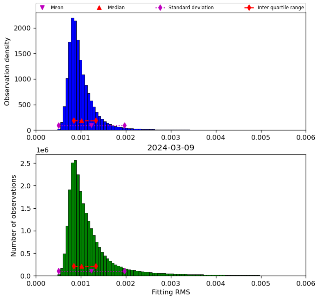
Figure 23: Histogram of “Fitting RMS” for 2024-03-09 to 2024-03-10
