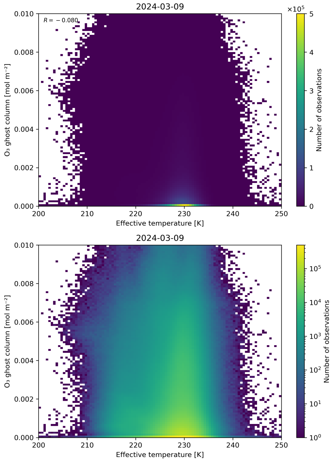
Figure 38: Scatter density plot of “Effective temperature” against “O 3 ghost column” for 2024-03-09 to 2024-03-10.
