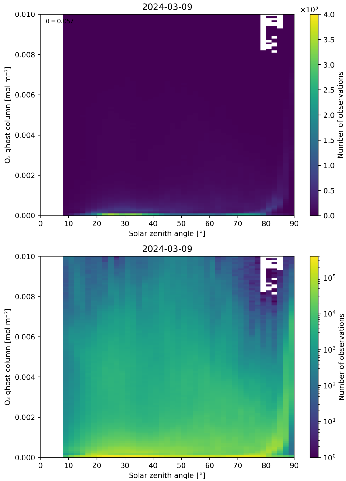
Figure 46: Scatter density plot of “Solar zenith angle” against “O 3 ghost column” for 2024-03-09 to 2024-03-10.
