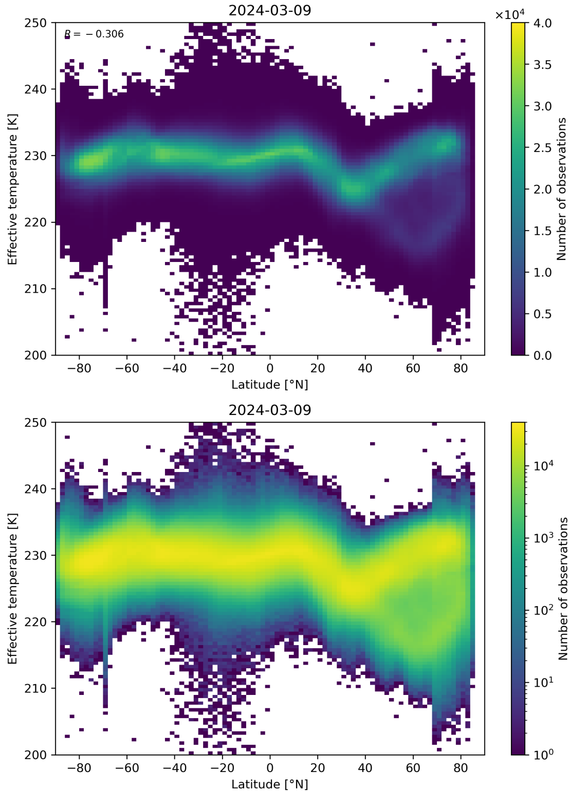
Figure 34: Scatter density plot of “Latitude” against “Effective temperature” for 2024-03-09 to 2024-03-10.
