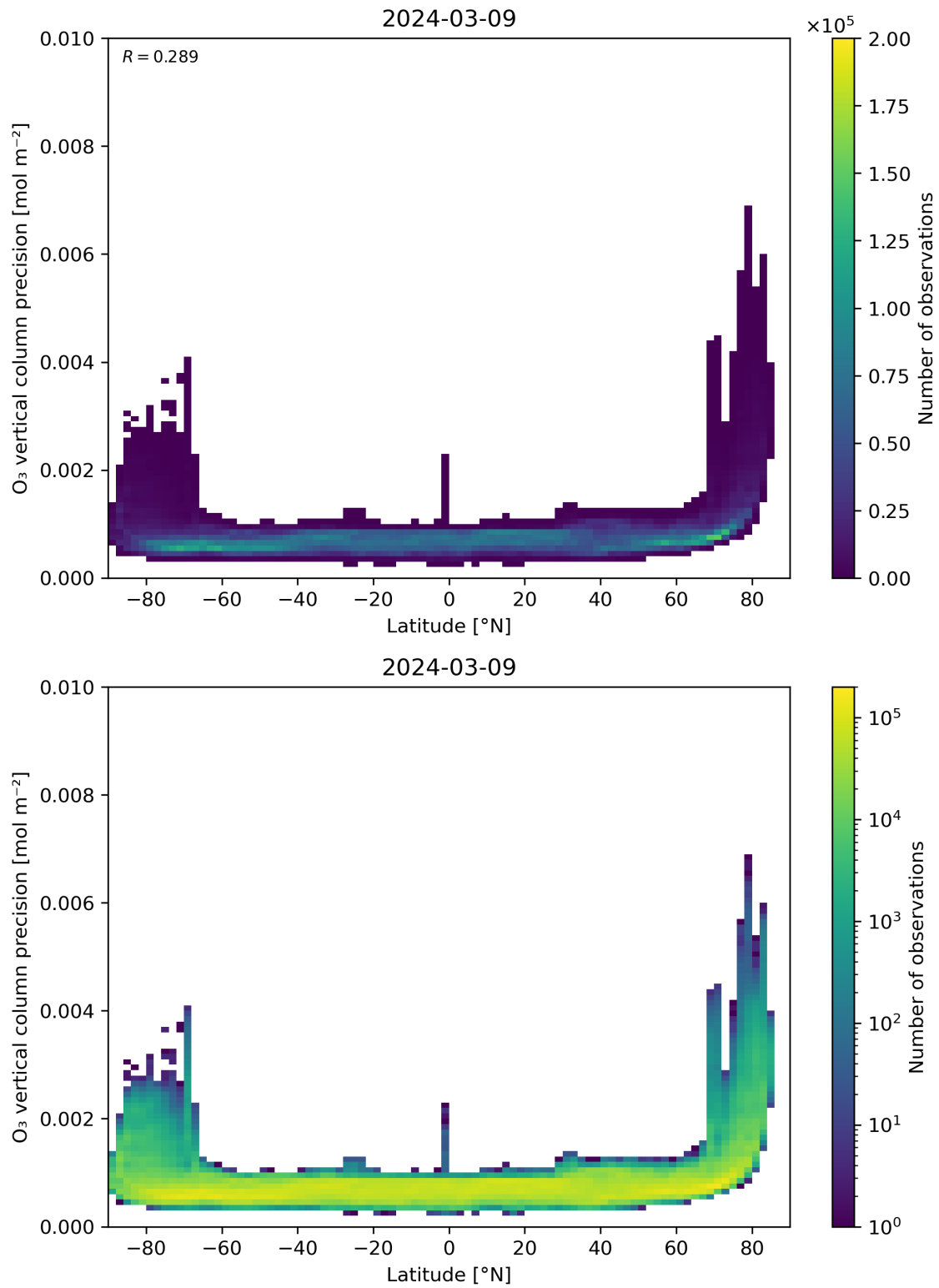
Figure 37: Scatter density plot of “Latitude” against “O 3 vertical column precision” for 2024-03-09 to 2024-03-10.
