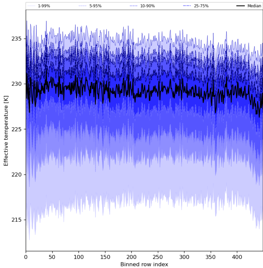
Figure 31: Along track statistics of “Effective temperature” for 2024-03-09 to 2024-03-10
