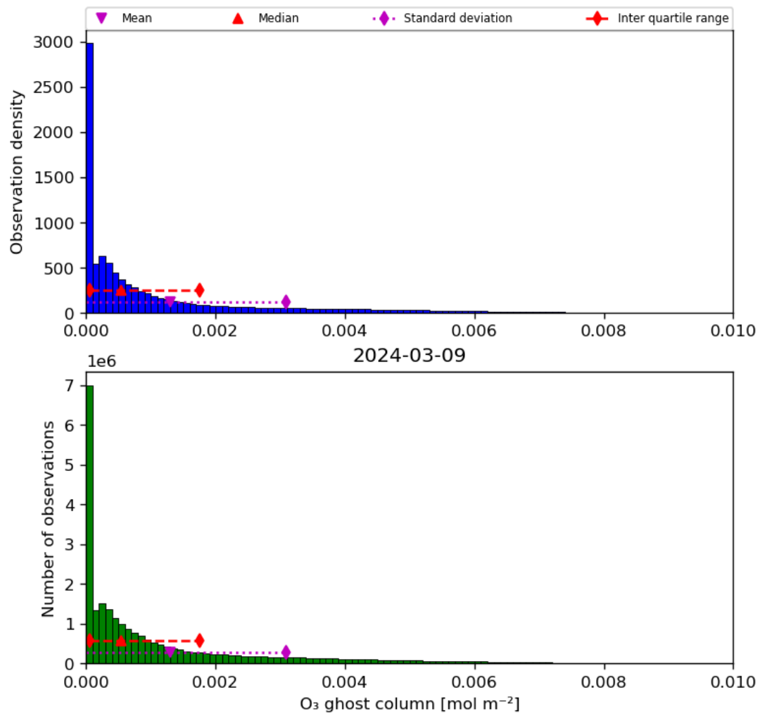
Figure 25: Histogram of “O 3 ghost column” for 2024-03-09 to 2024-03-10
