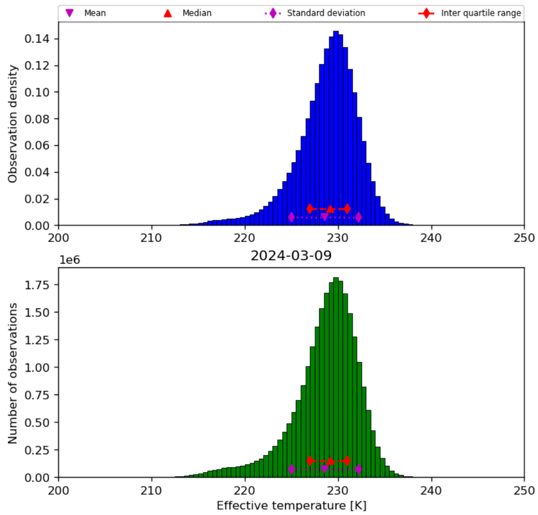
Figure 24: Histogram of “Effective temperature” for 2024-03-09 to 2024-03-10
