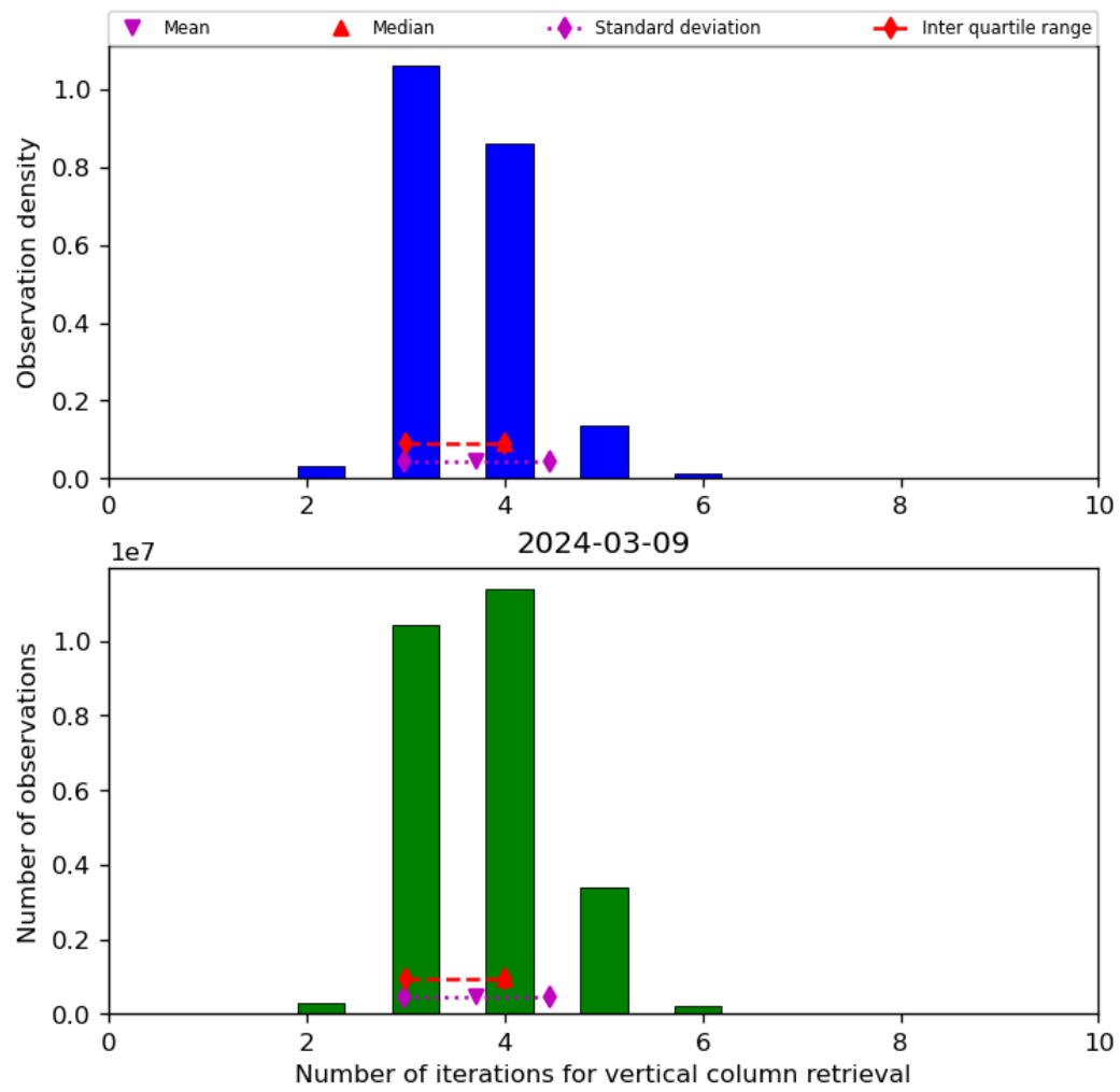
Figure 26: Histogram of “Number of iterations for vertical column retrieval” for 2024-03-09 to 2024-03-10
