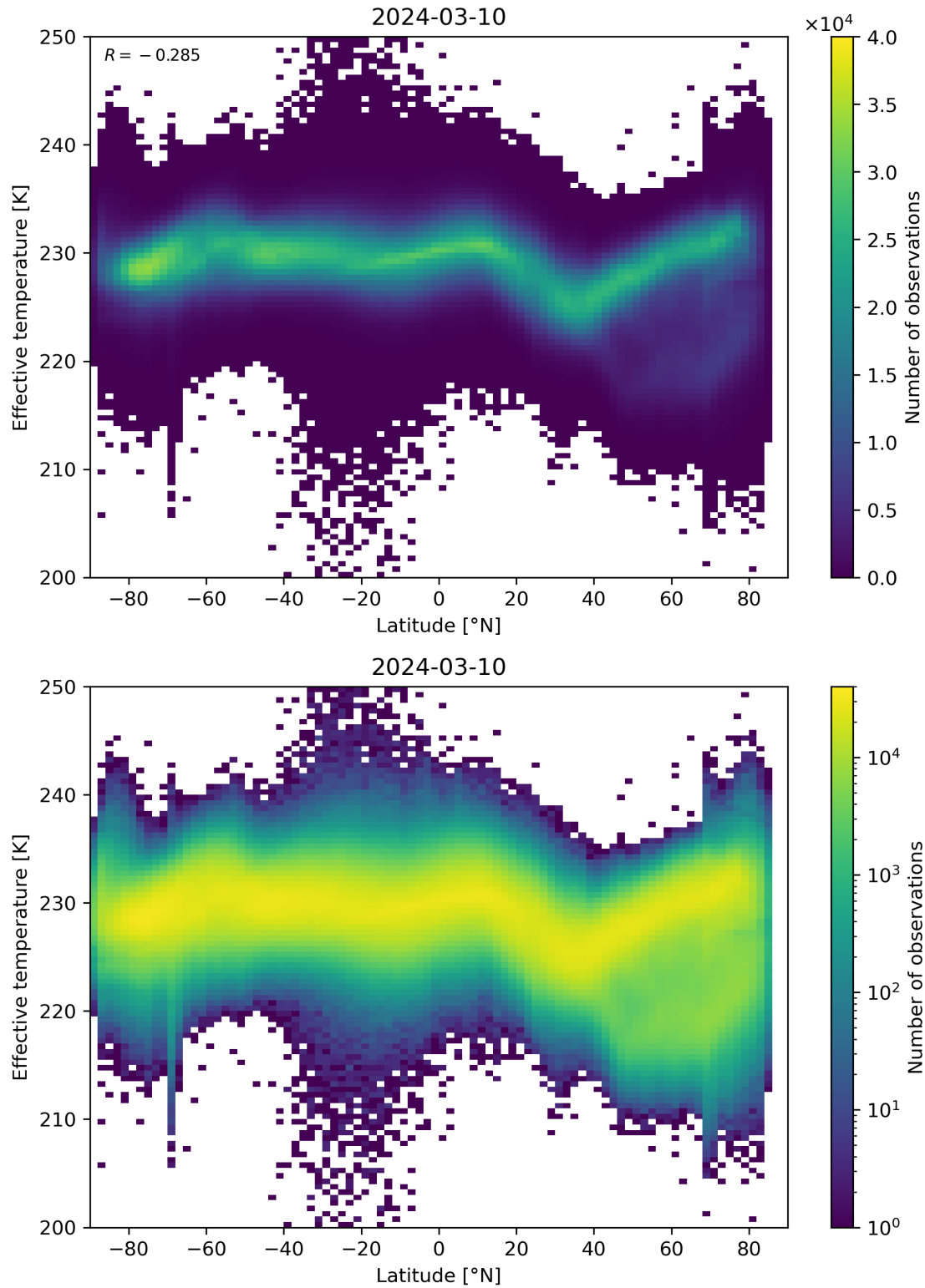
Figure 34: Scatter density plot of “Latitude” against “Effective temperature” for 2024-03-09 to 2024-03-11.
