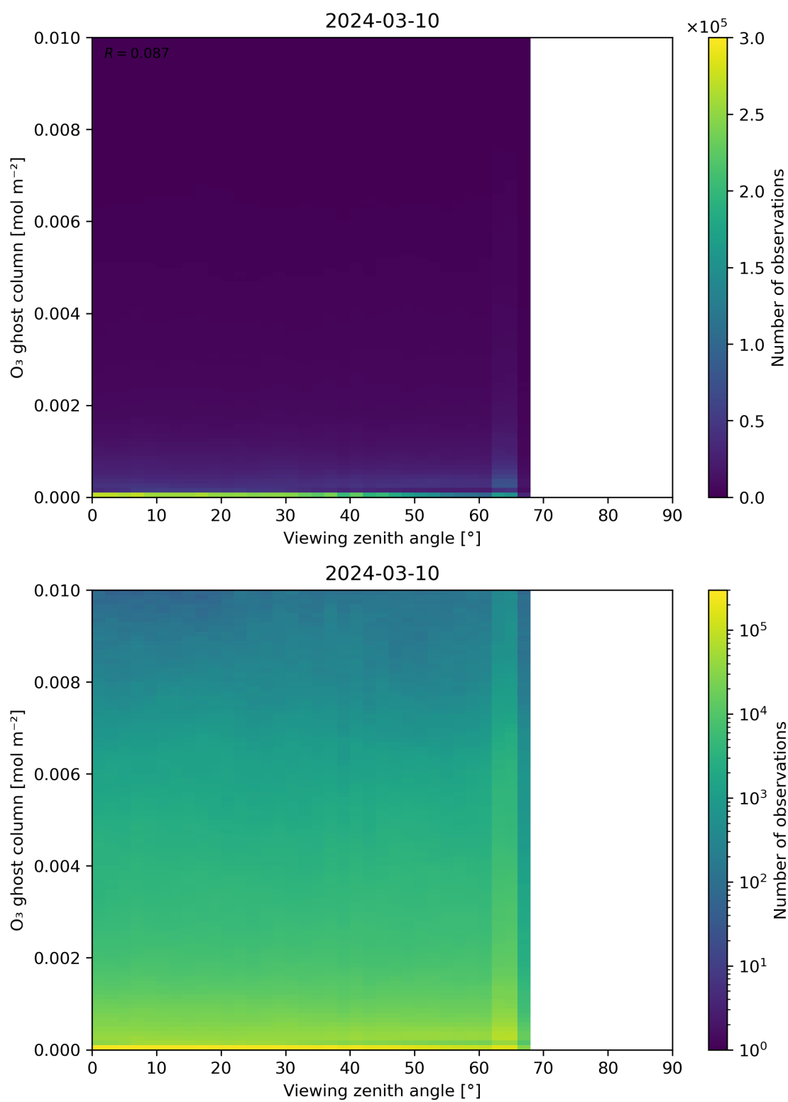
Figure 51: Scatter density plot of “Viewing zenith angle” against “O 3 ghost column” for 2024-03-09 to 2024-03-11.
