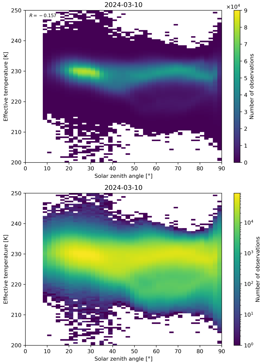
Figure 45: Scatter density plot of “Solar zenith angle” against “Effective temperature” for 2024-03-09 to 2024-03-11.
