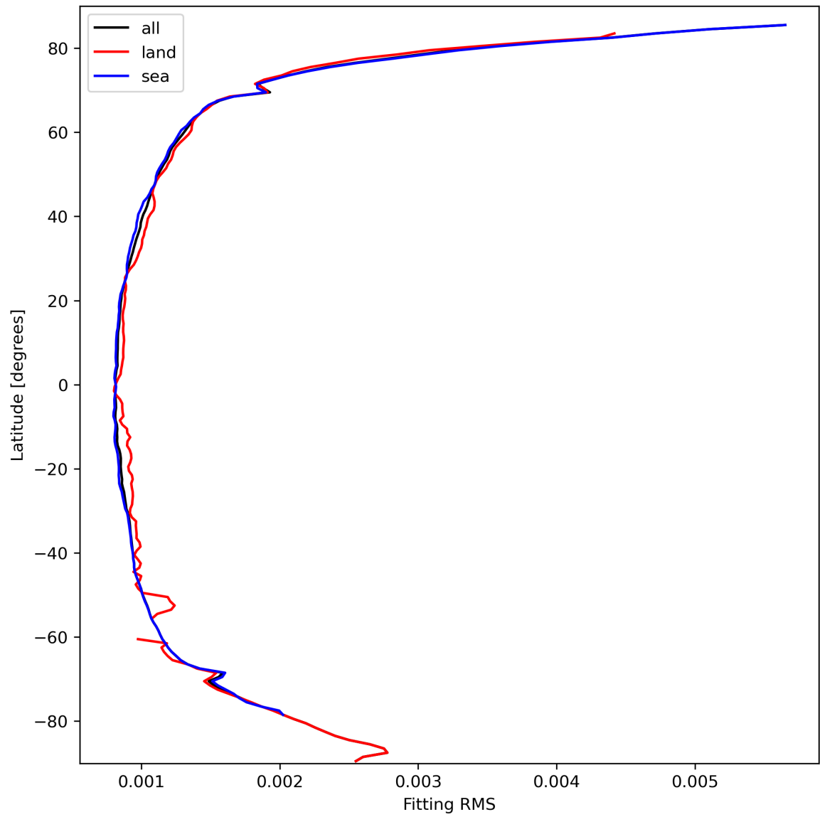
Figure 16: Zonal average of “Fitting RMS” for 2024-03-09 to 2024-03-11.
