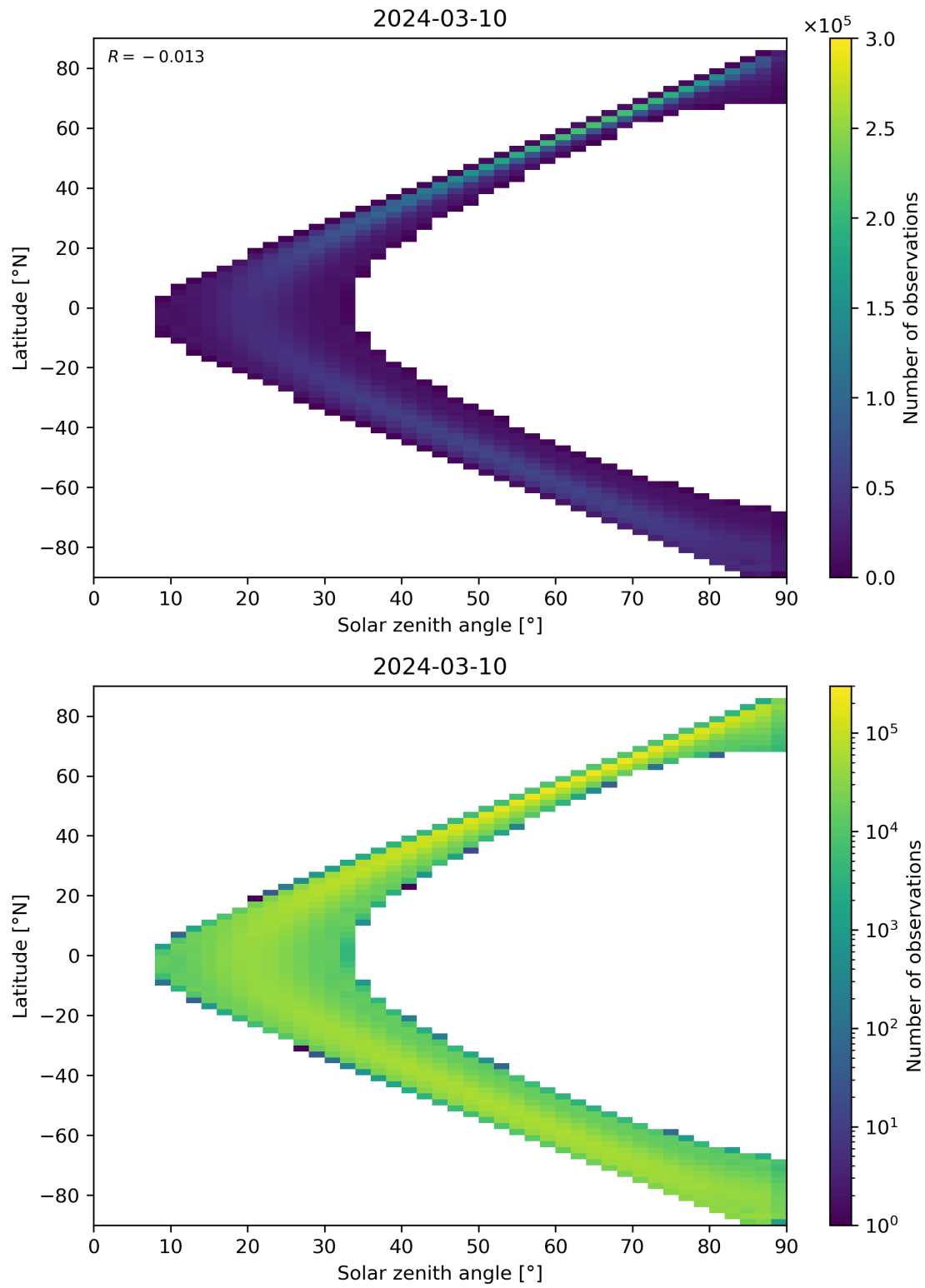
Figure 44: Scatter density plot of “Solar zenith angle” against “Latitude” for 2024-03-09 to 2024-03-11.
