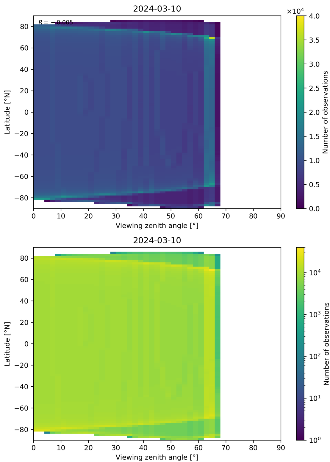
Figure 49: Scatter density plot of “Viewing zenith angle” against “Latitude” for 2024-03-09 to 2024-03-11.
