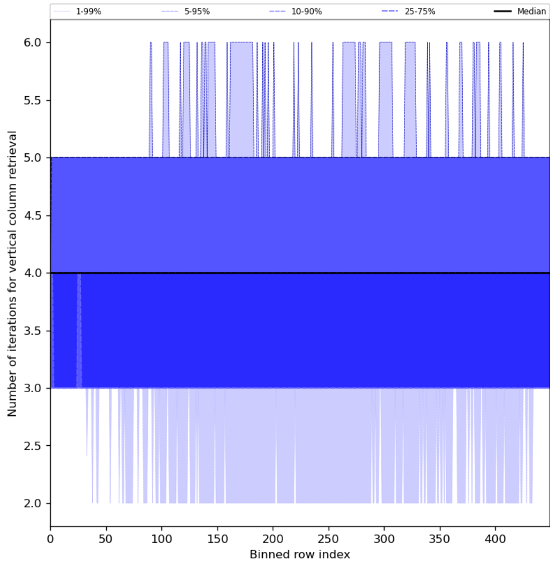
Figure 33: Along track statistics of “Number of iterations for vertical column retrieval” for 2024-03-09 to 2024-03-11
