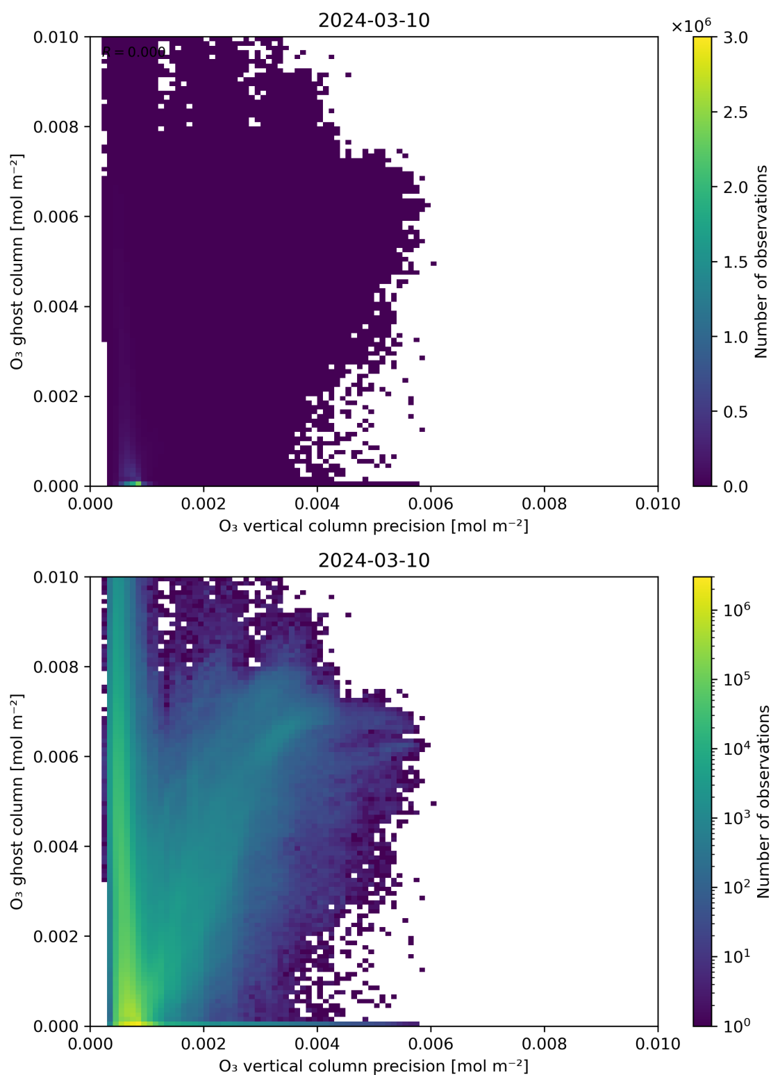
Figure 43: Scatter density plot of “O 3 vertical column precision” against “O 3 ghost column” for 2024-03-09 to 2024-03-11.
