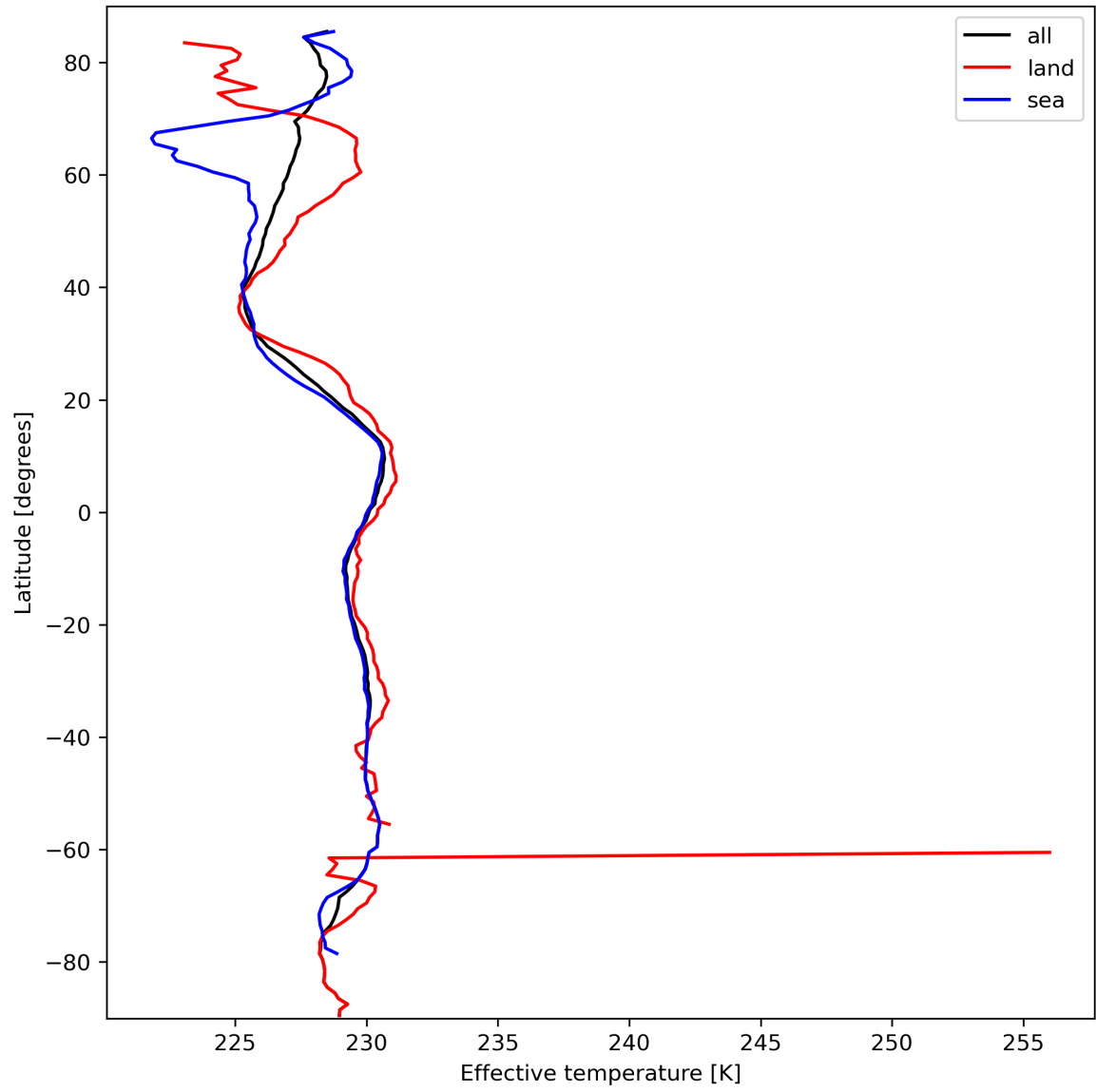
Figure 17: Zonal average of "Effective temperature" for 2024-03-09 to 2024-03-11.
