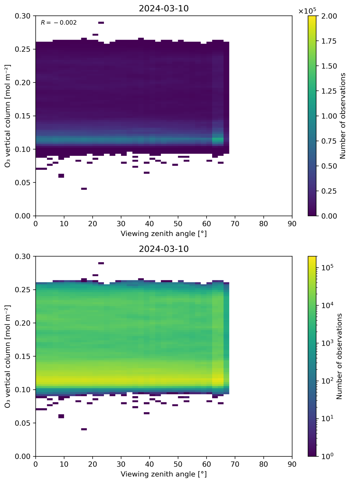
Figure 52: Scatter density plot of “Viewing zenith angle” against “O 3 vertical column” for 2024-03-09 to 2024-03-11.
