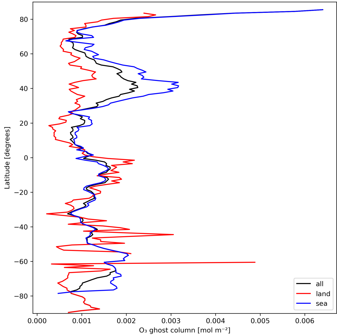
Figure 18: Zonal average of "O 3 ghost column" for 2024-03-09 to 2024-03-11.
