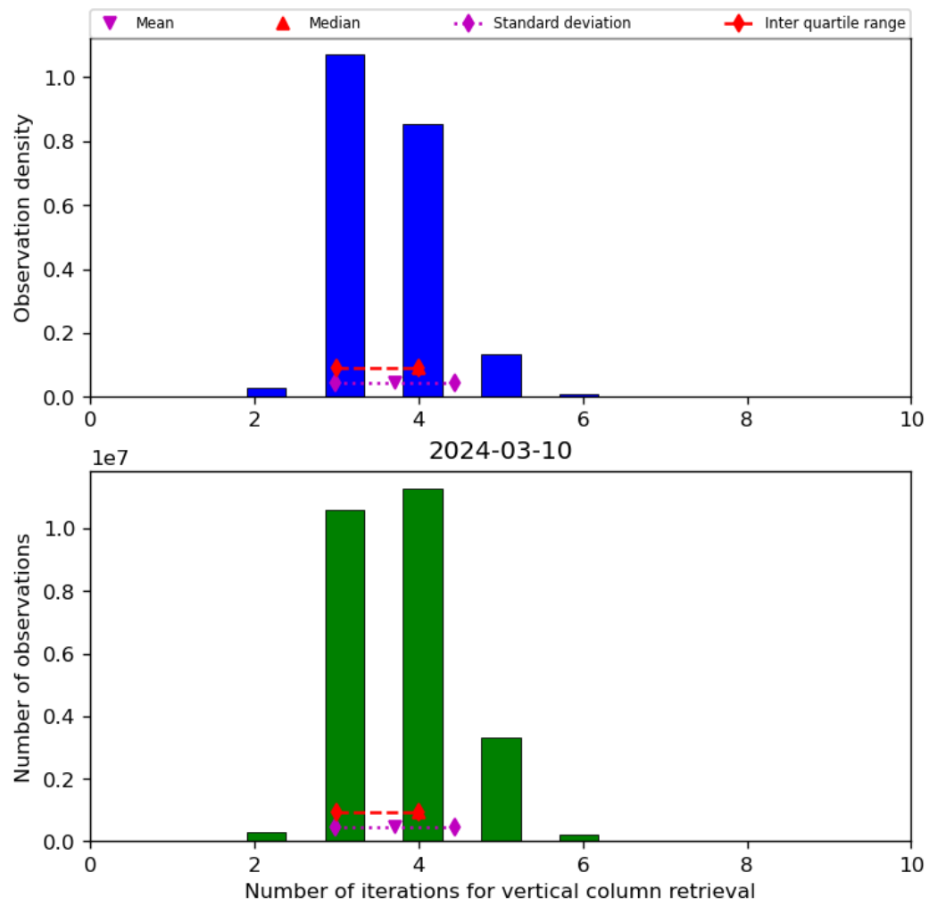
Figure 26: Histogram of “Number of iterations for vertical column retrieval” for 2024-03-09 to 2024-03-11
