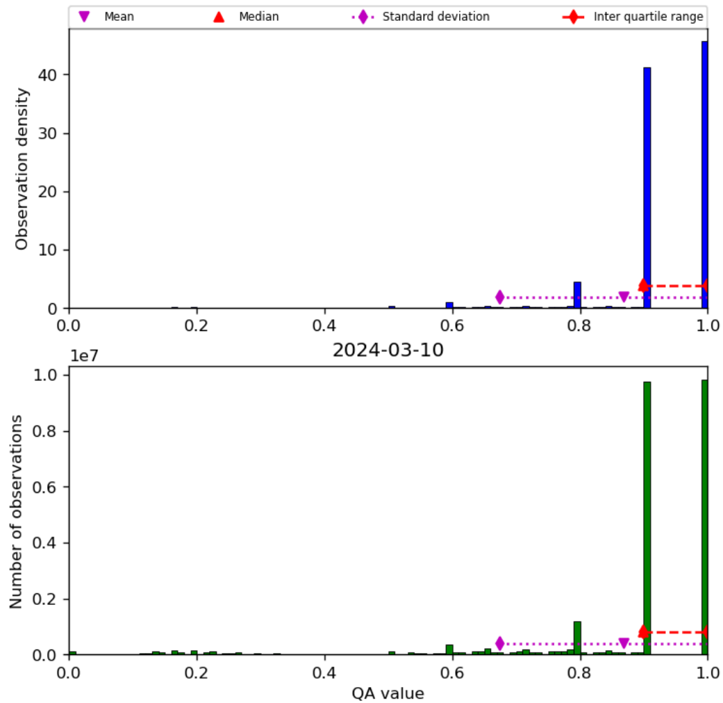
Figure 20: Histogram of “QA value” for 2024-03-09 to 2024-03-11
