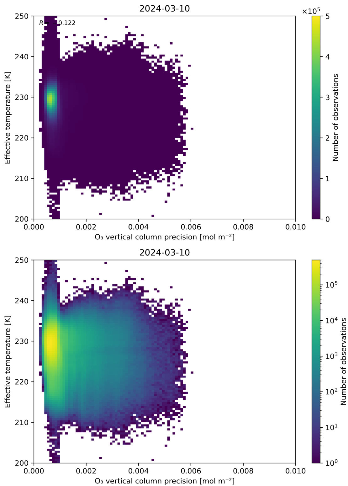
Figure 42: Scatter density plot of “O 3 vertical column precision” against “Effective temperature” for 2024-03-09 to 2024-03-11.
