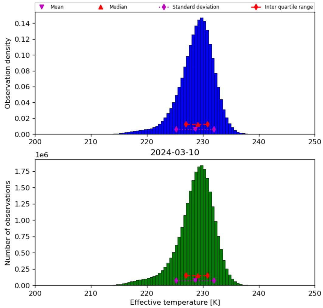
Figure 24: Histogram of “Effective temperature” for 2024-03-09 to 2024-03-11
