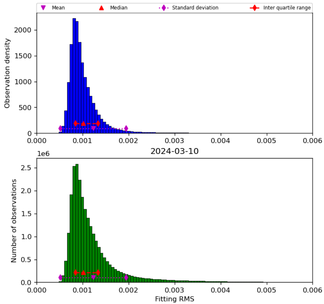
Figure 23: Histogram of “Fitting RMS” for 2024-03-09 to 2024-03-11
