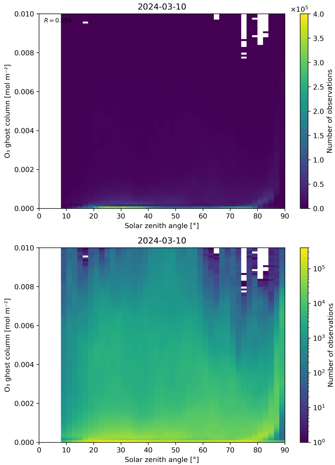
Figure 46: Scatter density plot of “Solar zenith angle” against “O 3 ghost column” for 2024-03-09 to 2024-03-11.
