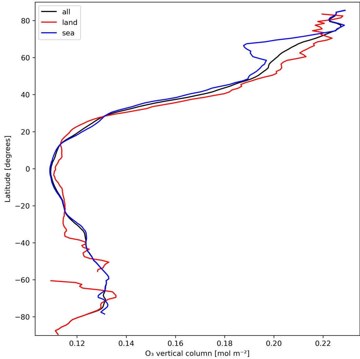
Figure 14: Zonal average of “O 3 vertical column” for 2024-03-09 to 2024-03-11.
