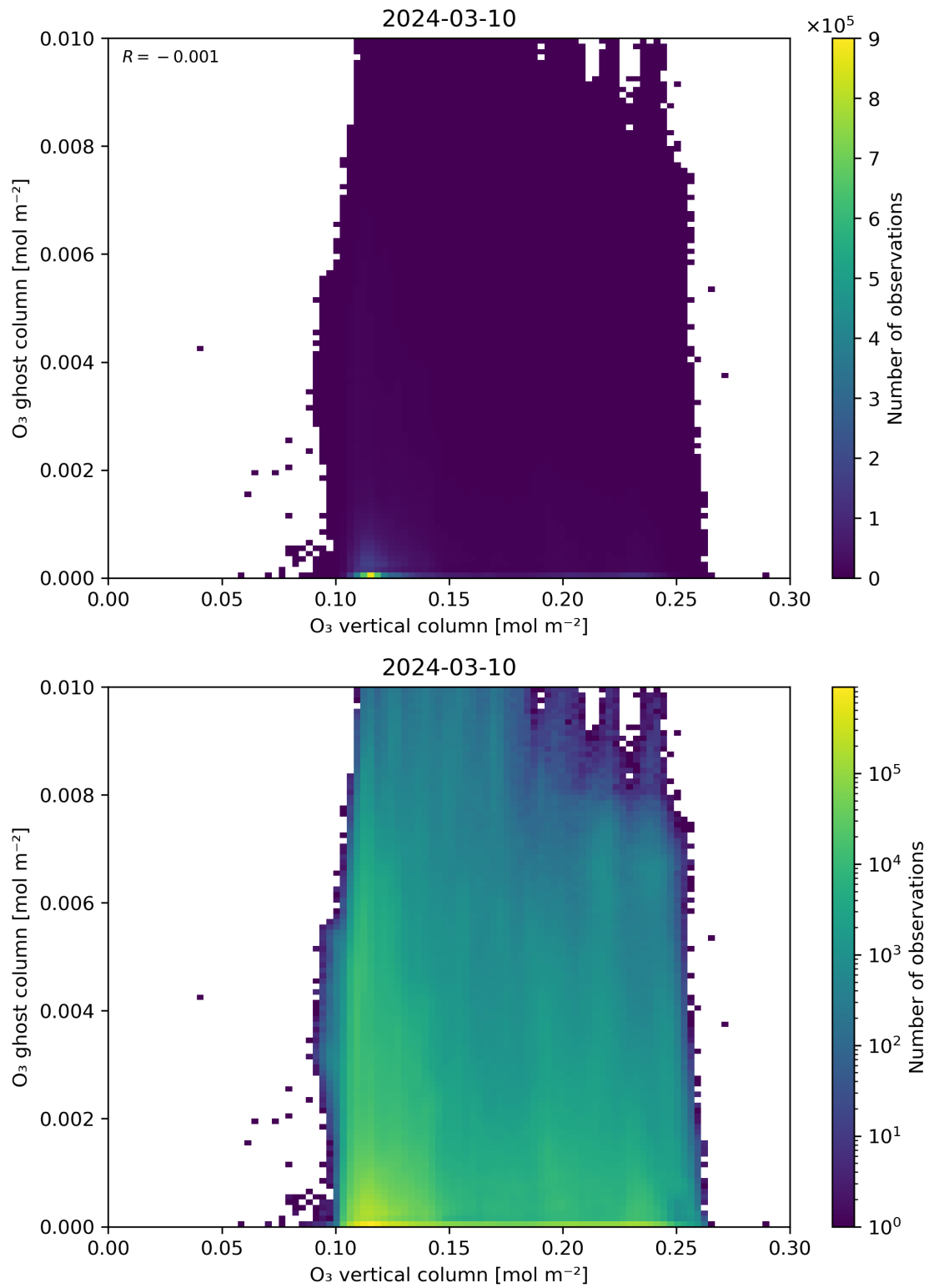
Figure 40: Scatter density plot of “O 3 vertical column” against “O 3 ghost column” for 2024-03-09 to 2024-03-11.
