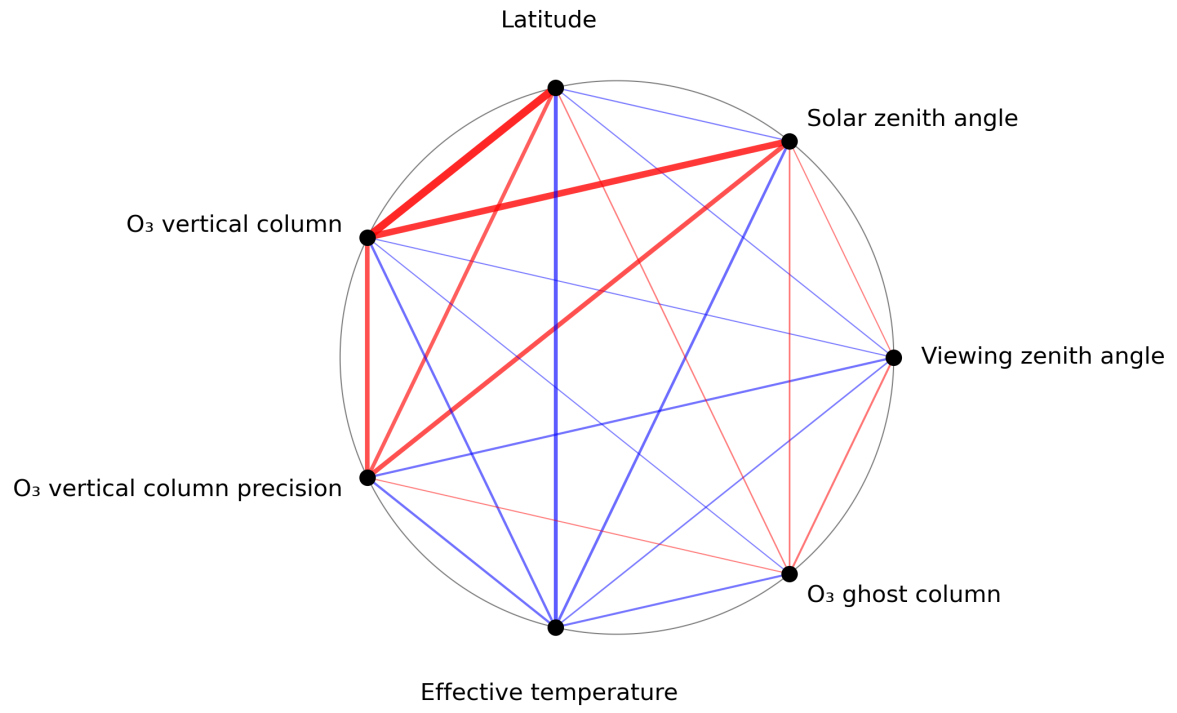
Figure 1: Map of correlation graph for 2024-03-09 to 2024-03-11.
