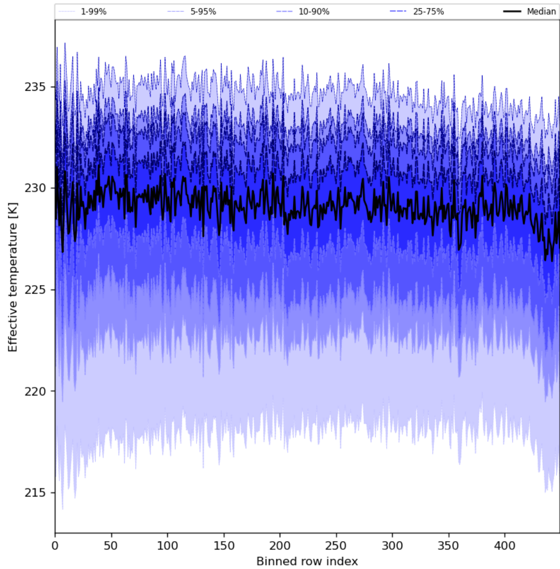
Figure 31: Along track statistics of “Effective temperature” for 2024-03-09 to 2024-03-11
