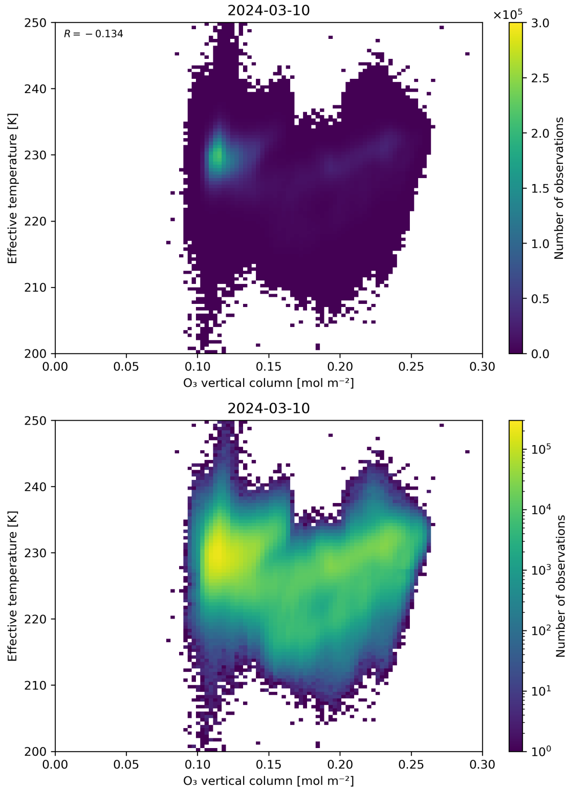
Figure 39: Scatter density plot of “O 3 vertical column” against “Effective temperature” for 2024-03-09 to 2024-03-11.
