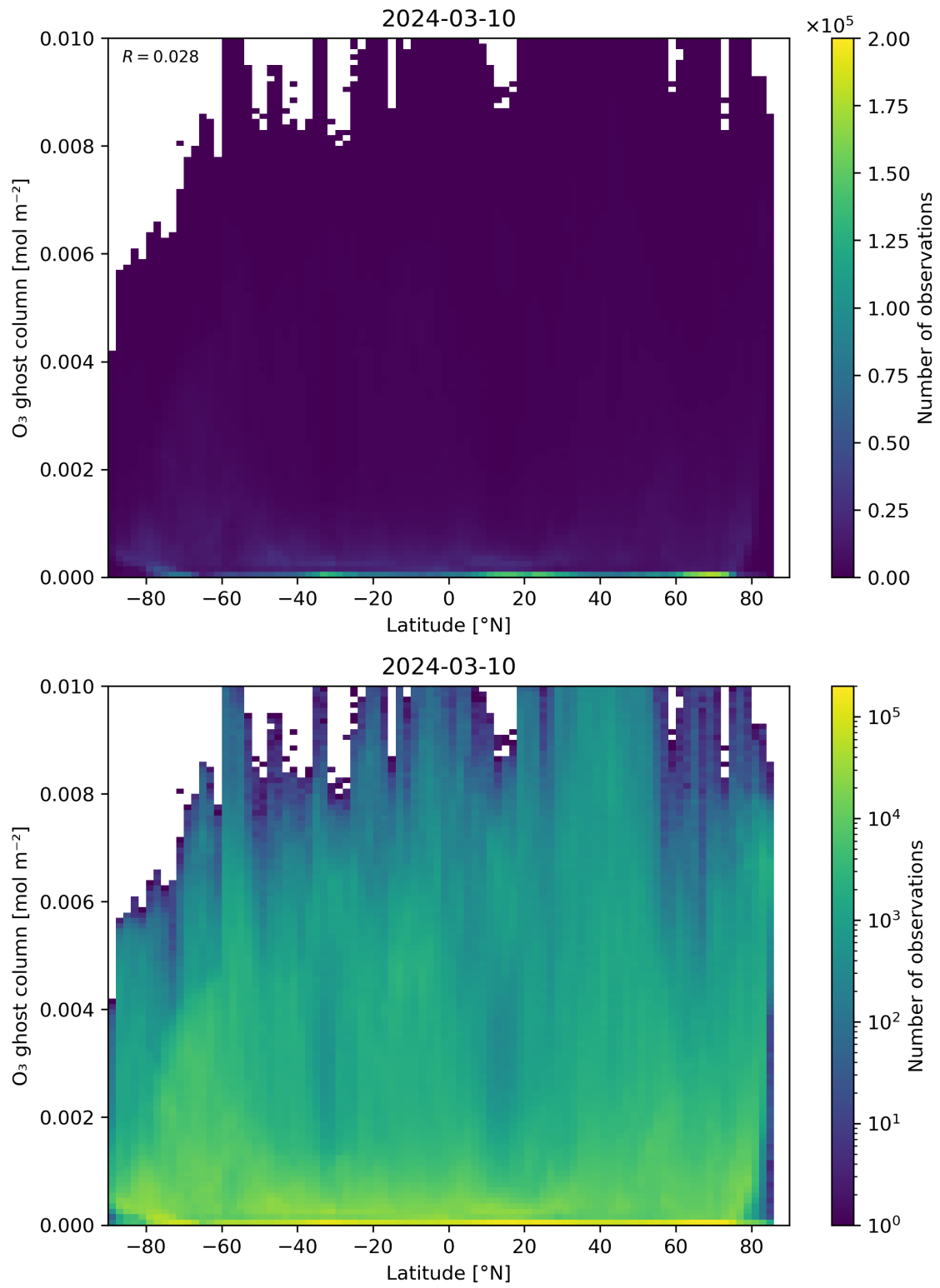
Figure 35: Scatter density plot of “Latitude” against “O 3 ghost column” for 2024-03-09 to 2024-03-11.
