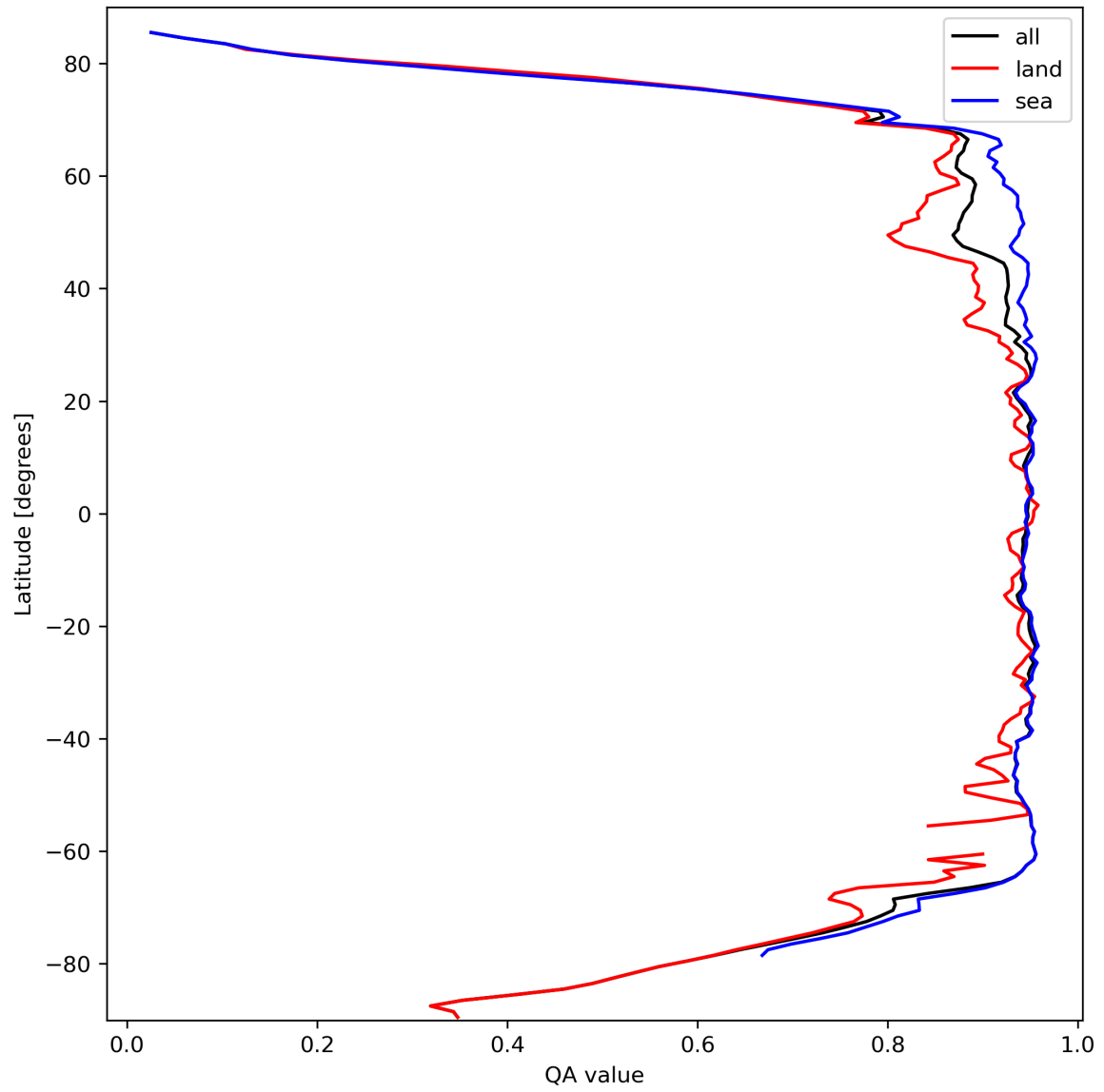
Figure 13: Zonal average of “QA value” for 2024-03-09 to 2024-03-11.
