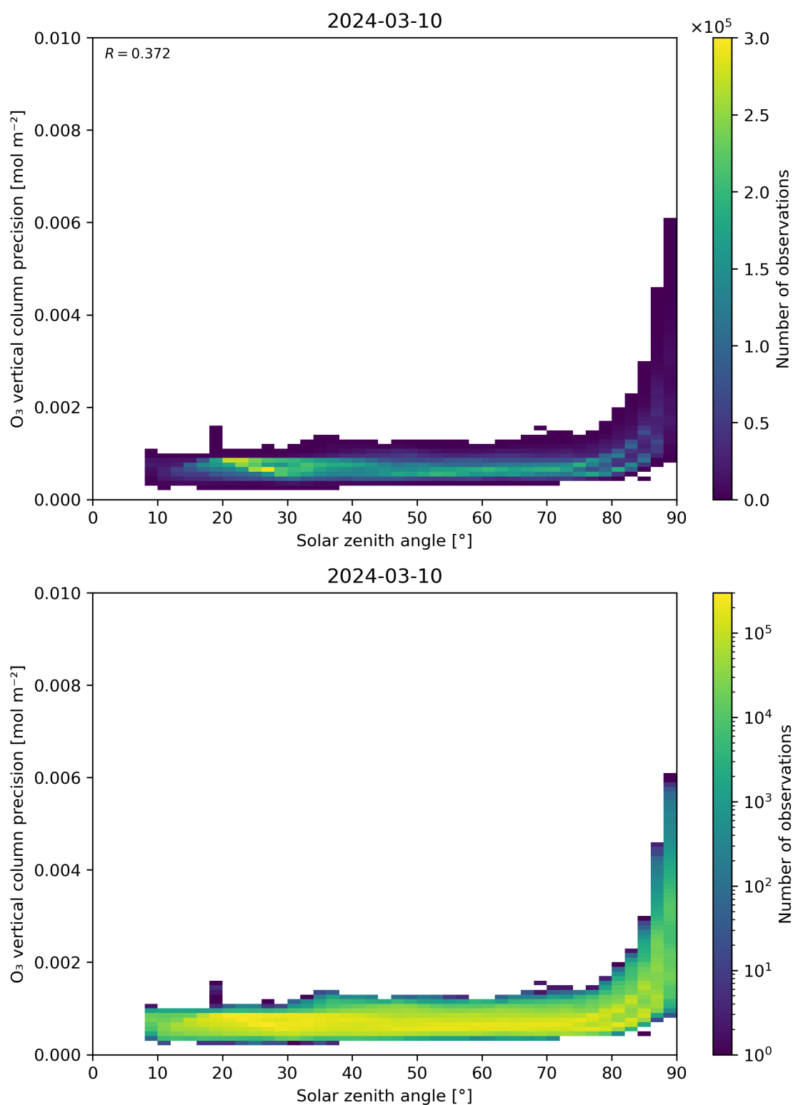
Figure 48: Scatter density plot of “Solar zenith angle” against “O 3 vertical column precision” for 2024-03-09 to 2024-03-11.
