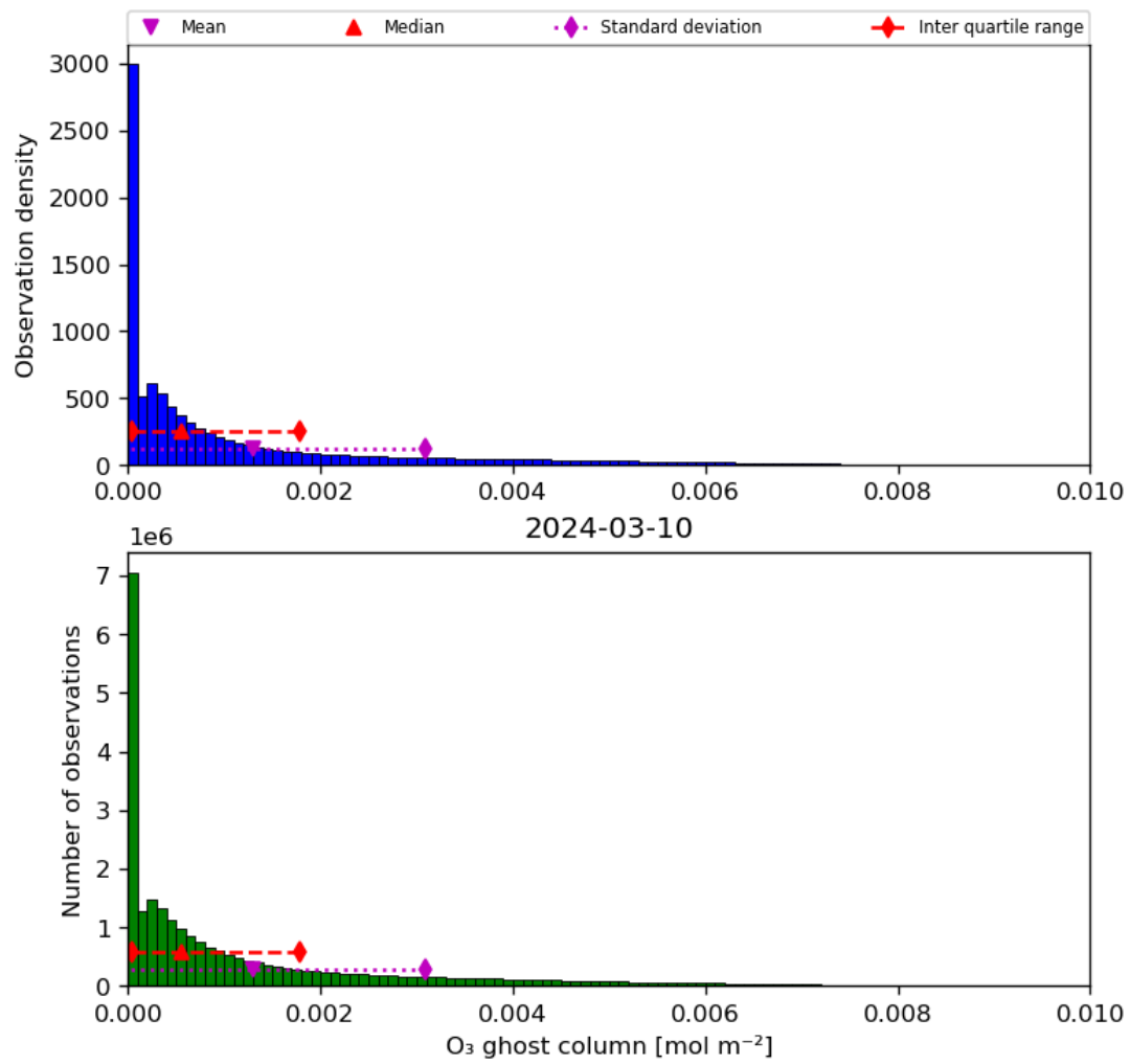
Figure 25: Histogram of “O 3 ghost column” for 2024-03-09 to 2024-03-11
