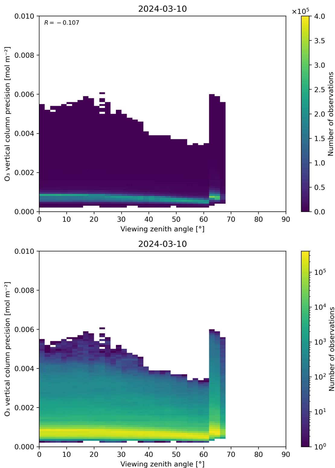
Figure 53: Scatter density plot of “Viewing zenith angle” against “O 3 vertical column precision” for 2024-03-09 to 2024-03-11.
