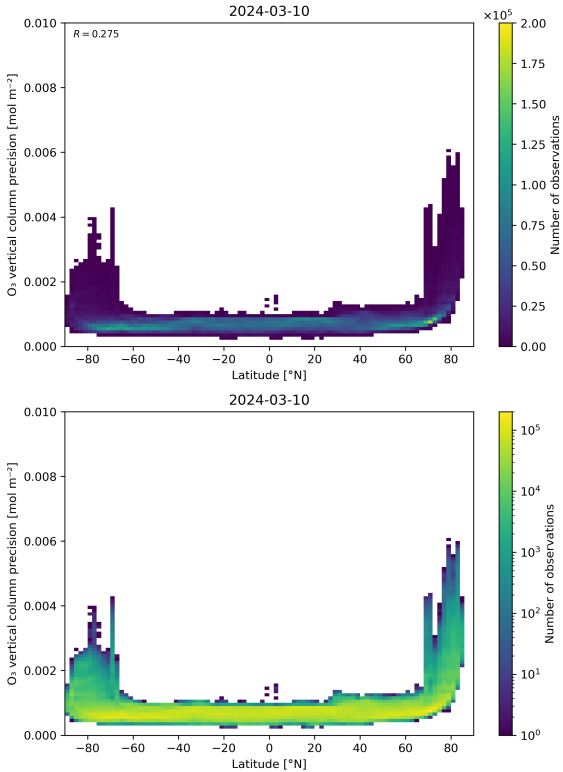
Figure 37: Scatter density plot of “Latitude” against “O 3 vertical column precision” for 2024-03-09 to 2024-03-11.
