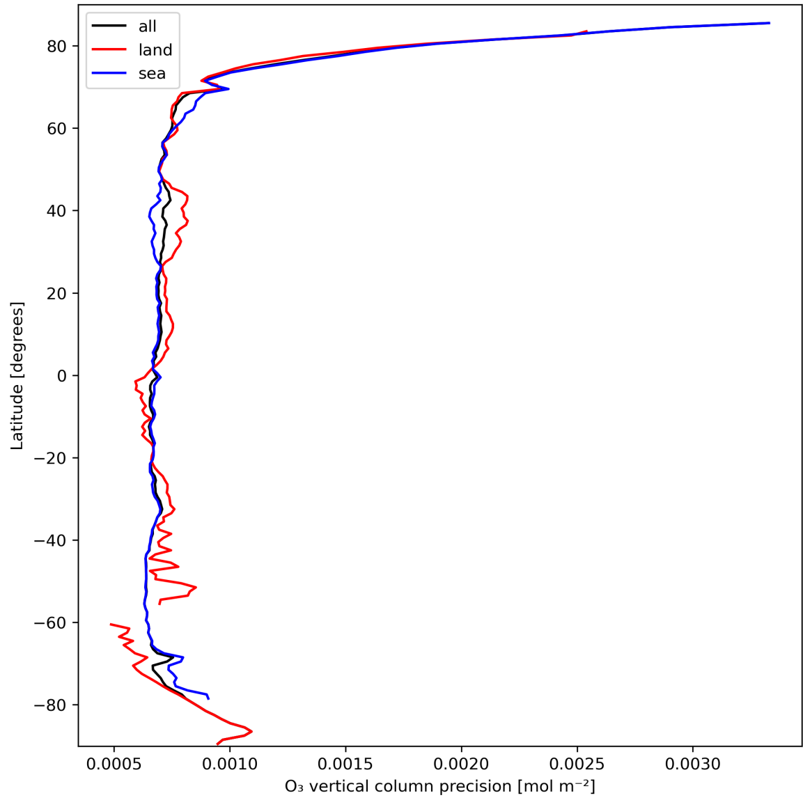
Figure 15: Zonal average of “O 3 vertical column precision” for 2024-03-09 to 2024-03-11.
