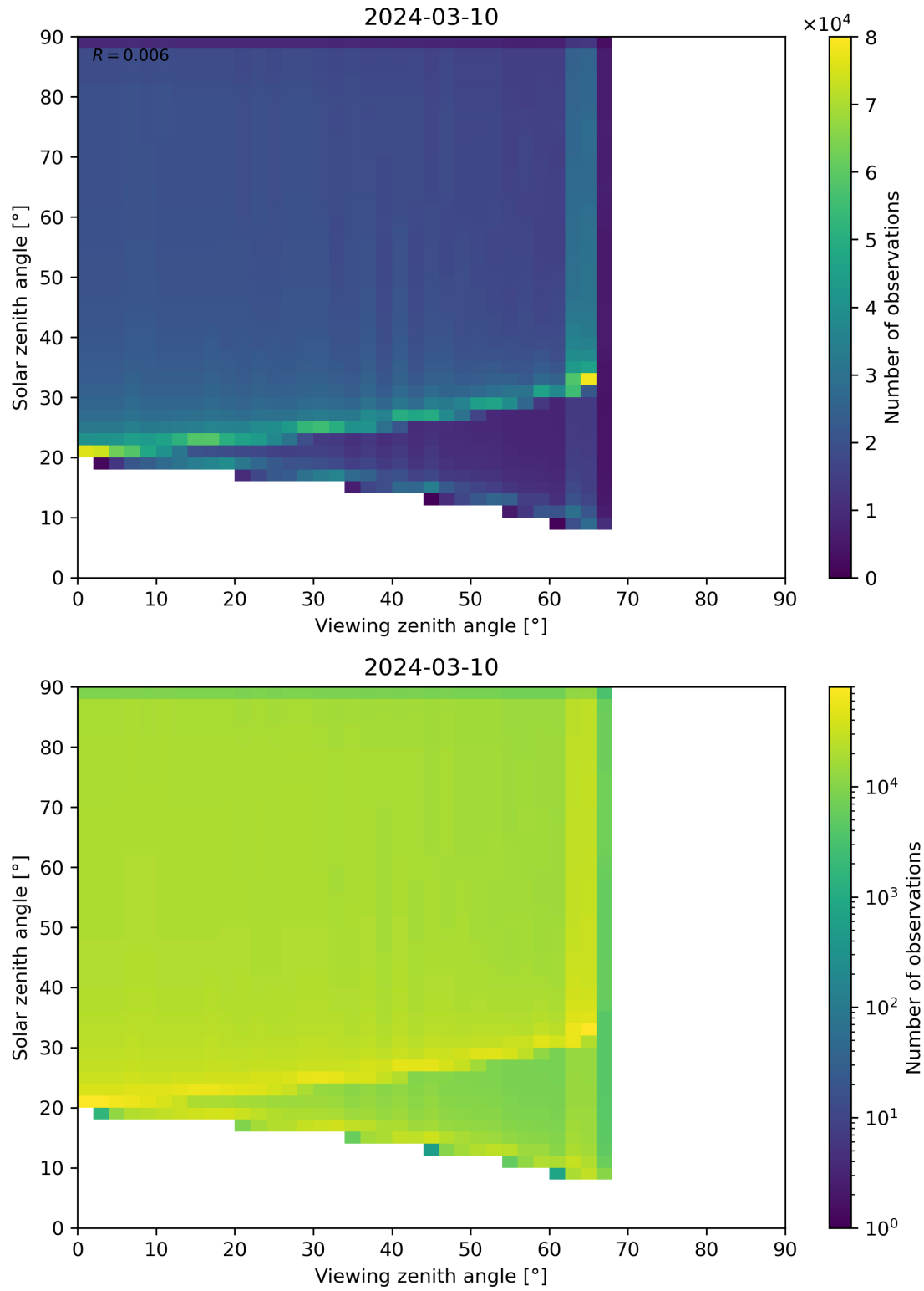
Figure 54: Scatter density plot of “Viewing zenith angle” against “Solar zenith angle” for 2024-03-09 to 2024-03-11.
