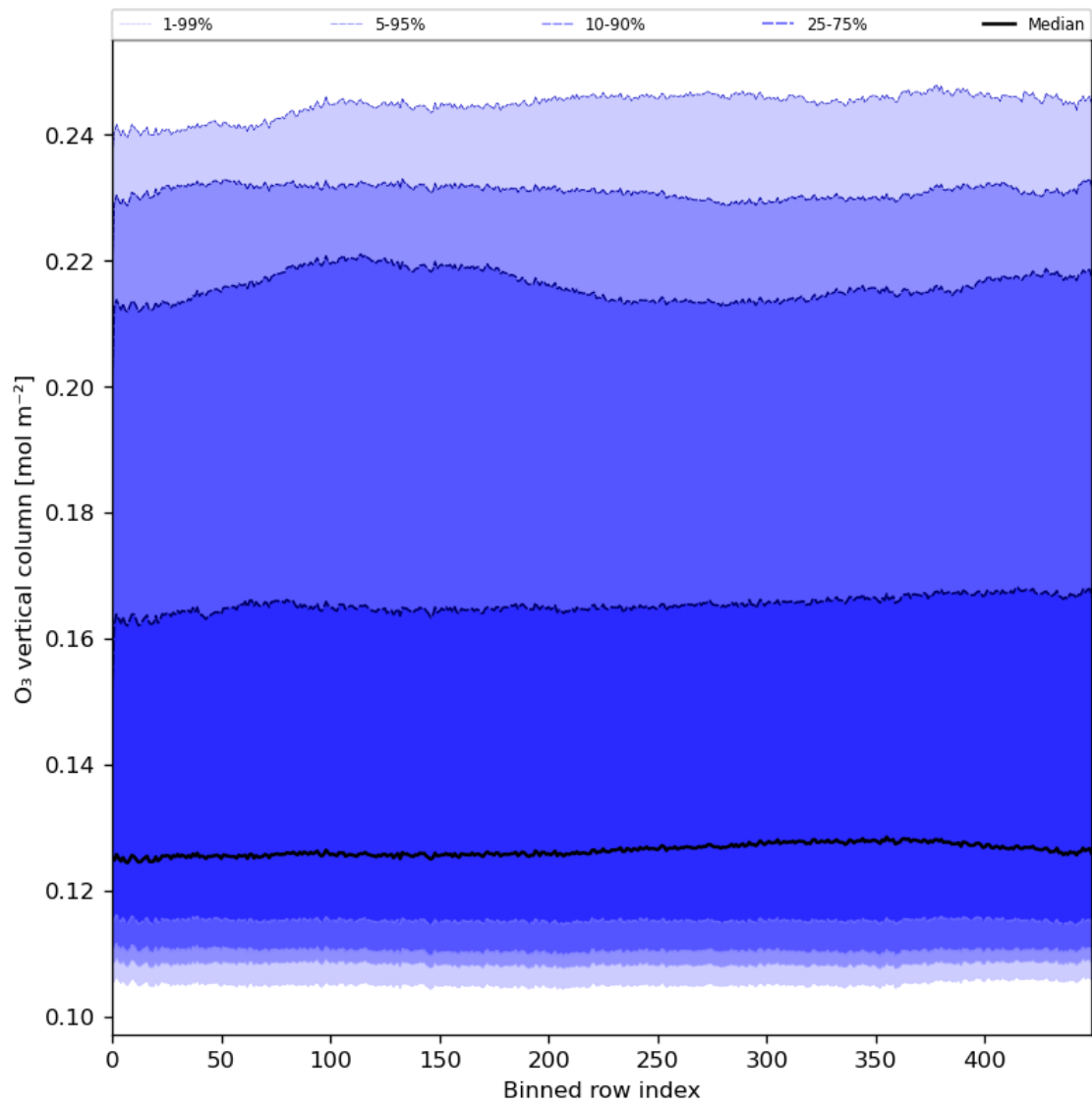
Figure 28: Along track statistics of “O 3 vertical column” for 2024-03-09 to 2024-03-11
