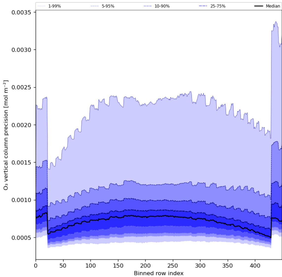
Figure 29: Along track statistics of “O 3 vertical column precision” for 2024-03-09 to 2024-03-11
