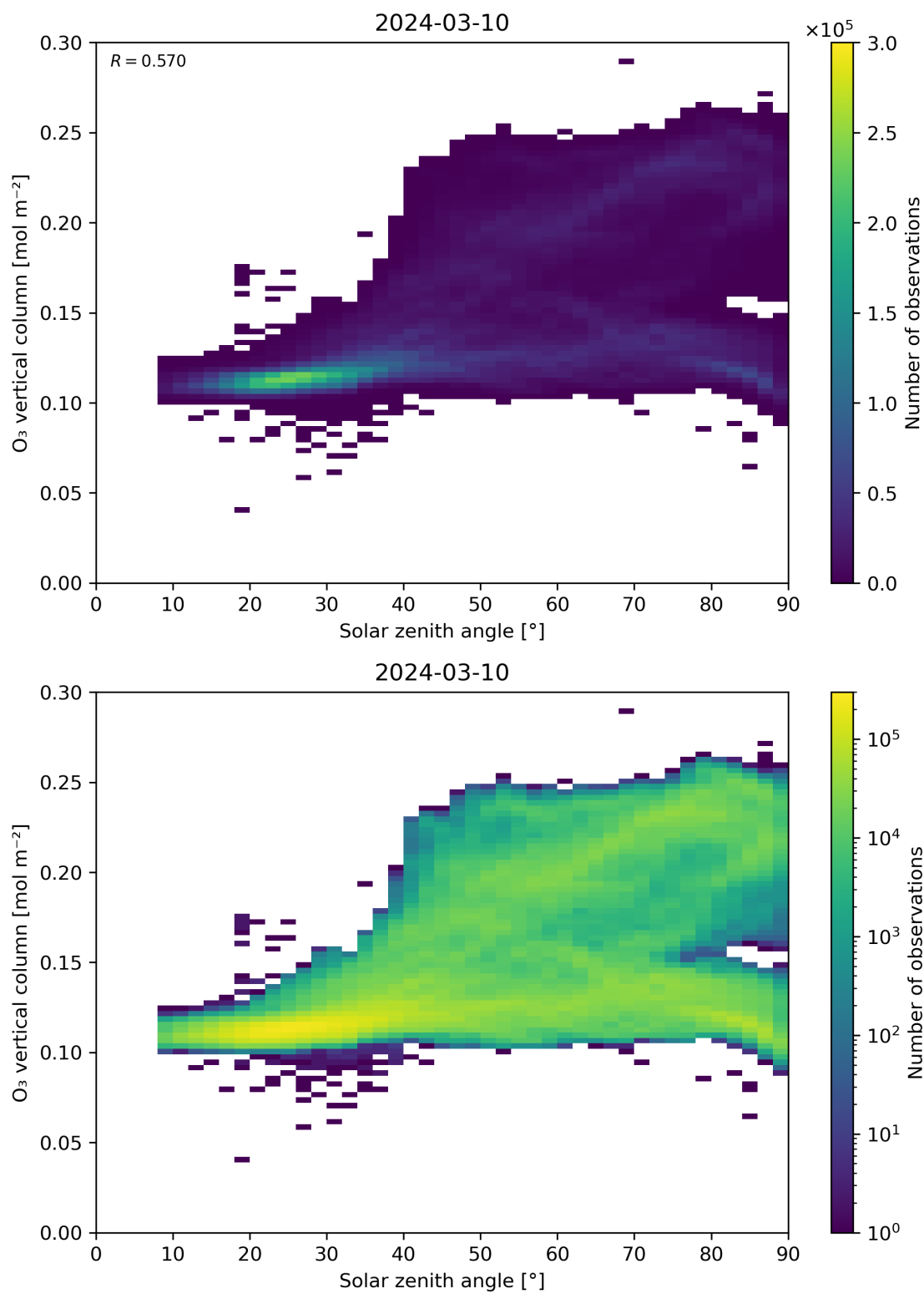
Figure 47: Scatter density plot of “Solar zenith angle” against “O 3 vertical column” for 2024-03-09 to 2024-03-11.
