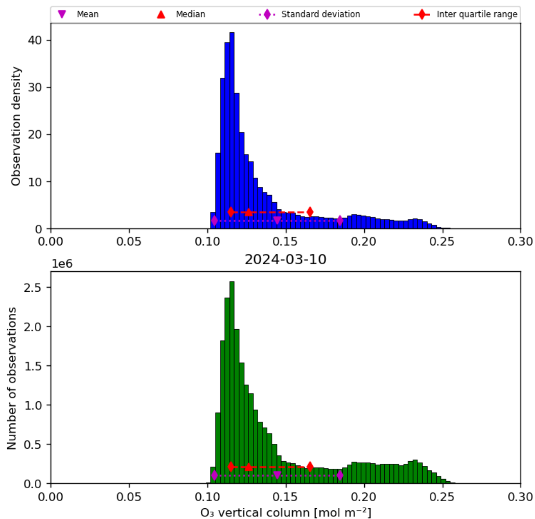
Figure 21: Histogram of “O 3 vertical column” for 2024-03-09 to 2024-03-11
