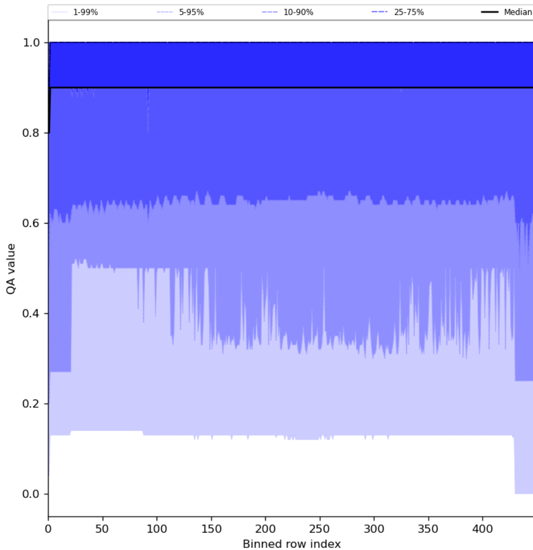
Figure 27: Along track statistics of “QA value” for 2024-03-09 to 2024-03-11
