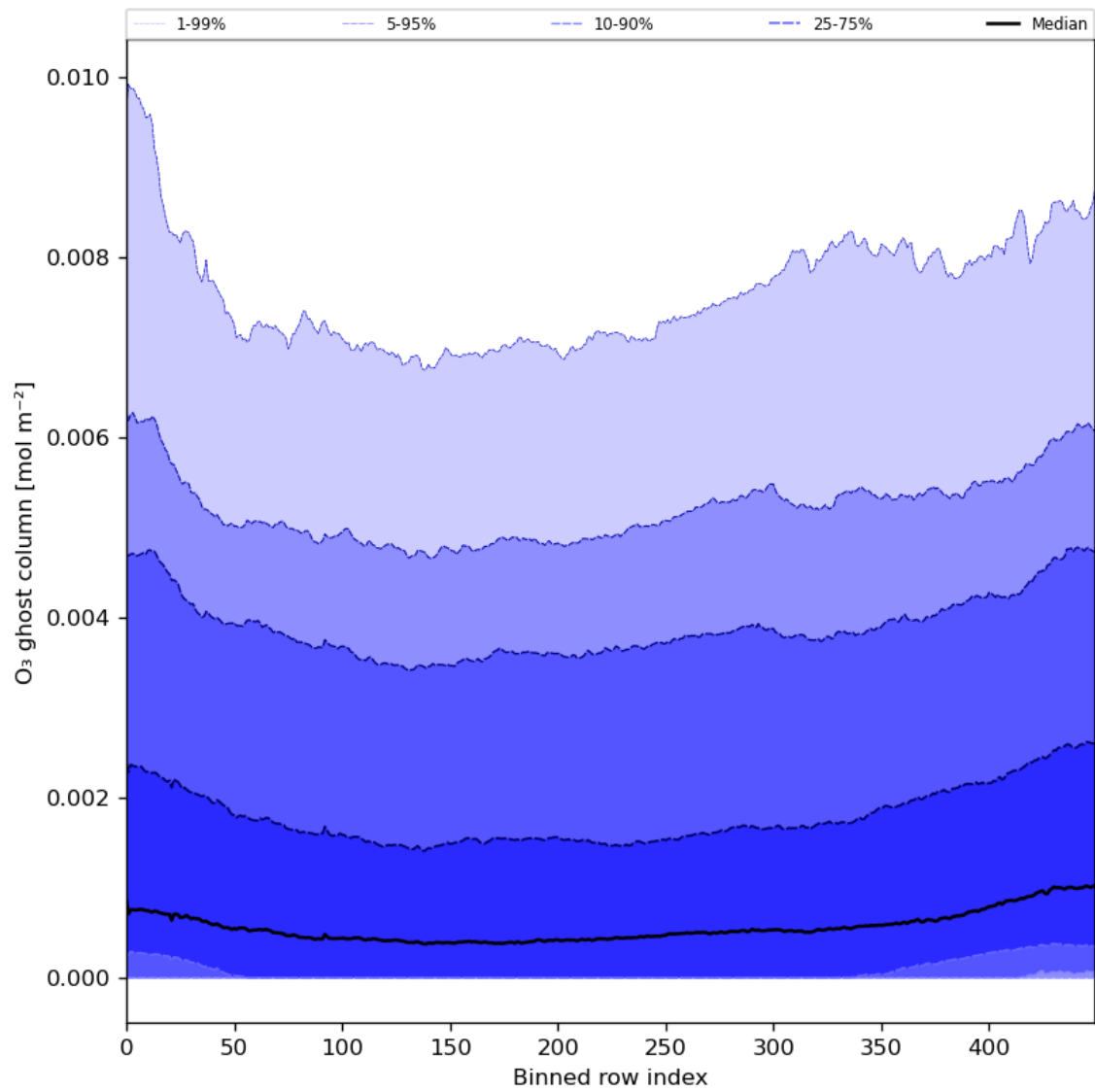
Figure 32: Along track statistics of “O 3 ghost column” for 2024-03-09 to 2024-03-11
