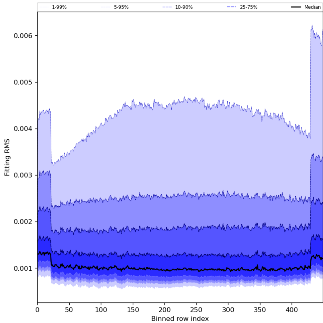
Figure 30: Along track statistics of “Fitting RMS” for 2024-03-09 to 2024-03-11
