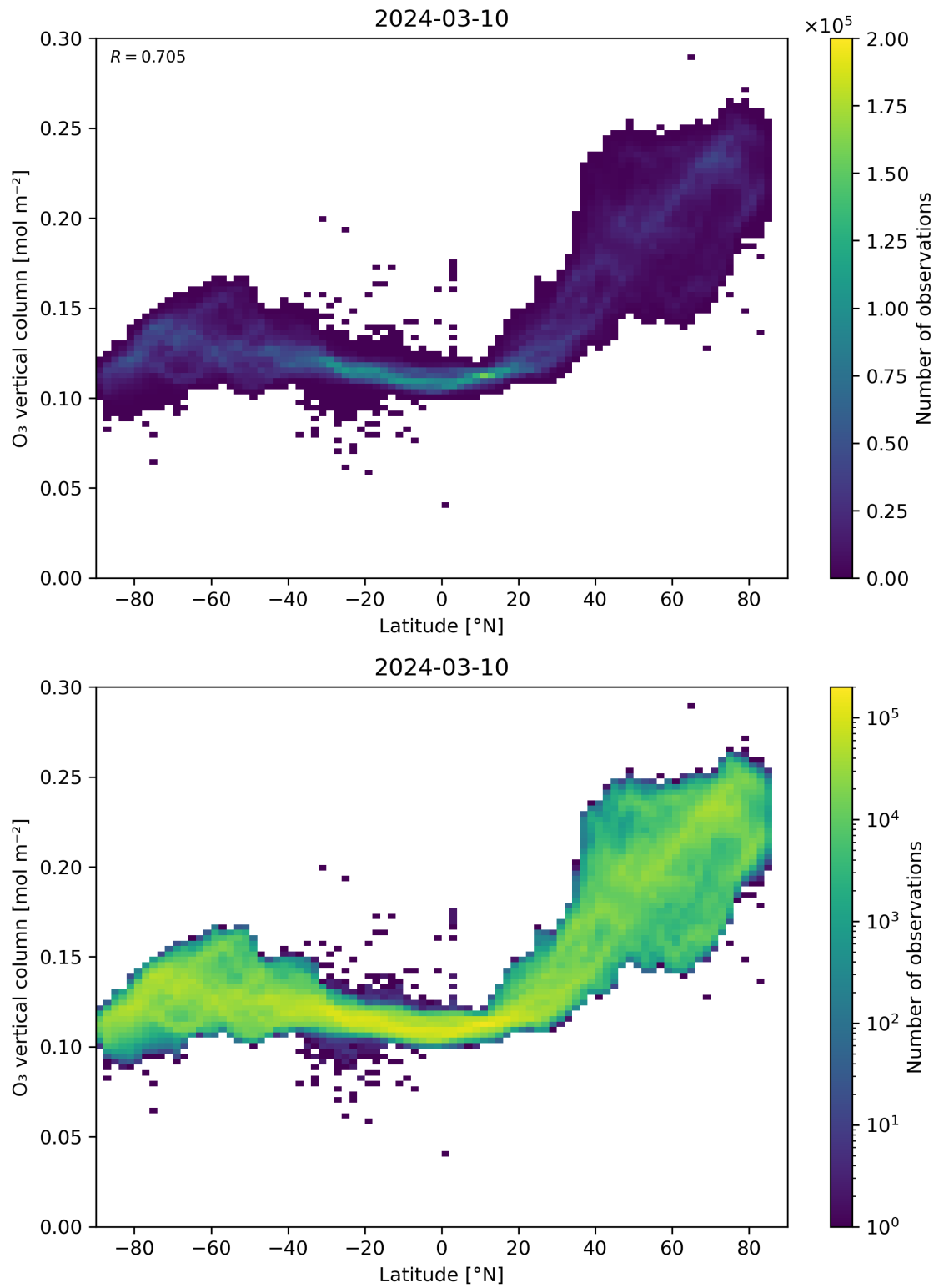
Figure 36: Scatter density plot of “Latitude” against “O 3 vertical column” for 2024-03-09 to 2024-03-11.
