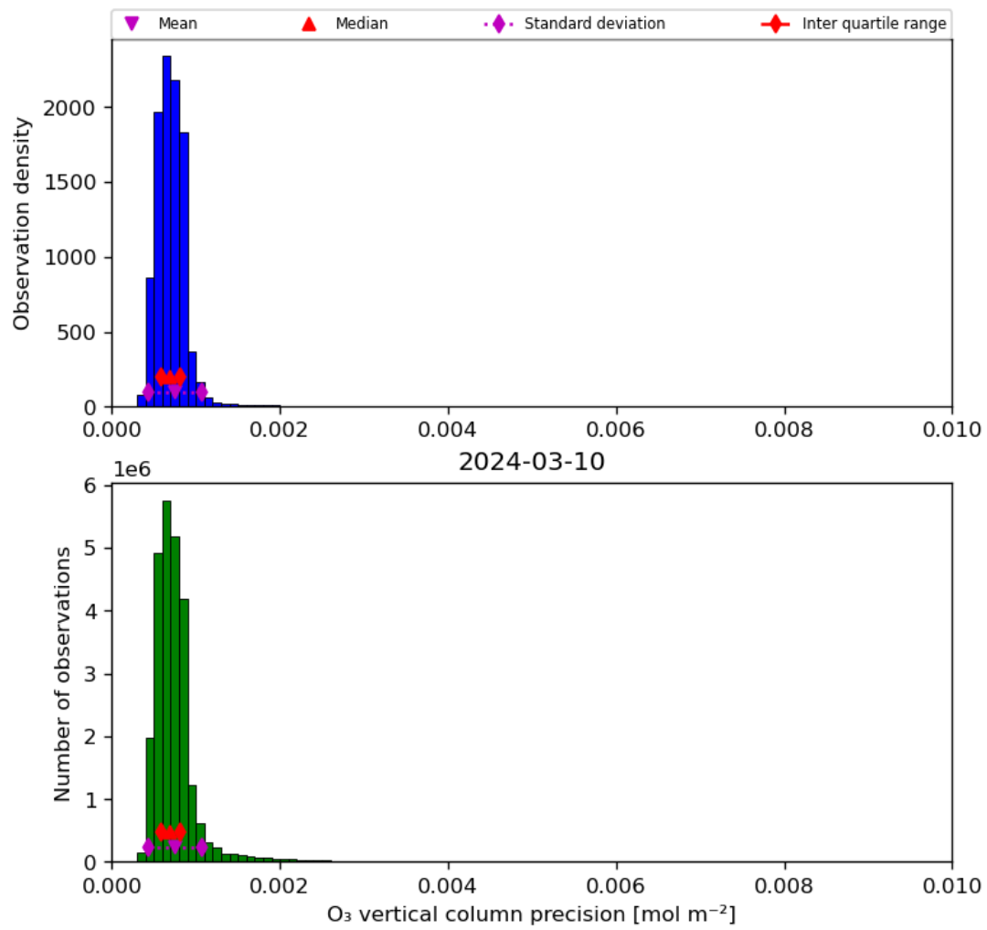
Figure 22: Histogram of “O 3 vertical column precision” for 2024-03-09 to 2024-03-11
