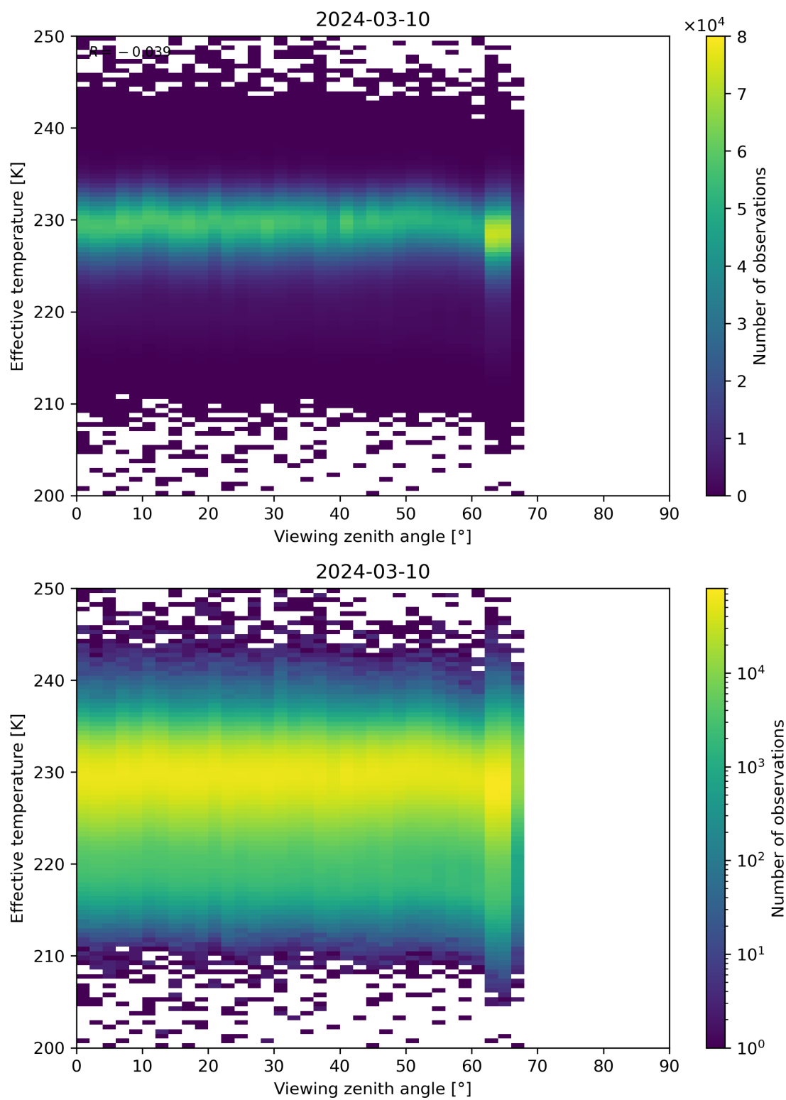
Figure 50: Scatter density plot of “Viewing zenith angle” against “Effective temperature” for 2024-03-09 to 2024-03-11.
