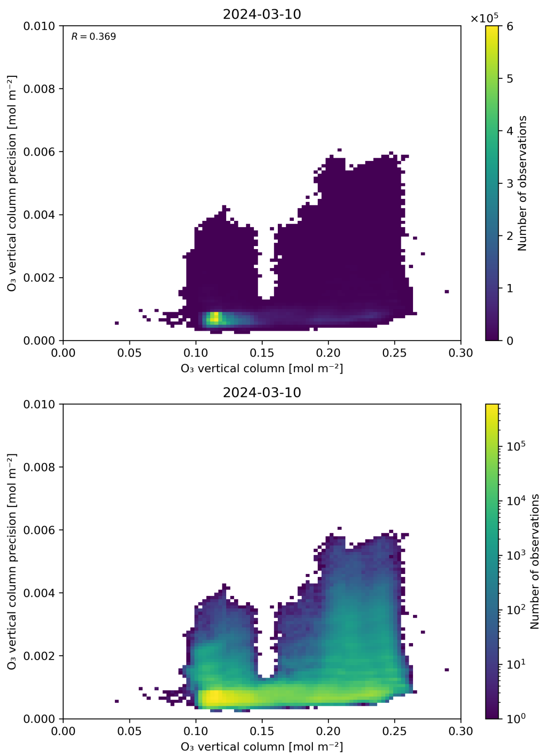
Figure 41: Scatter density plot of “O 3 vertical column” against “O 3 vertical column precision” for 2024-03-09 to 2024-03-11.
