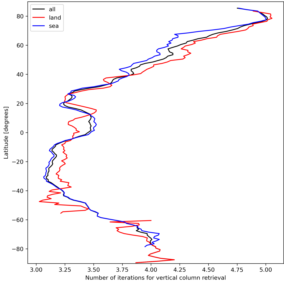
Figure 19: Zonal average of “Number of iterations for vertical column retrieval” for 2024-03-09 to 2024-03-11.
