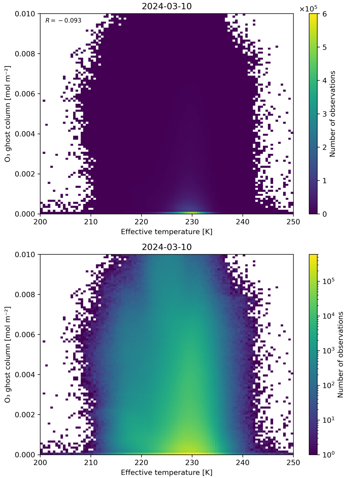
Figure 38: Scatter density plot of “Effective temperature” against “O 3 ghost column” for 2024-03-09 to 2024-03-11.
