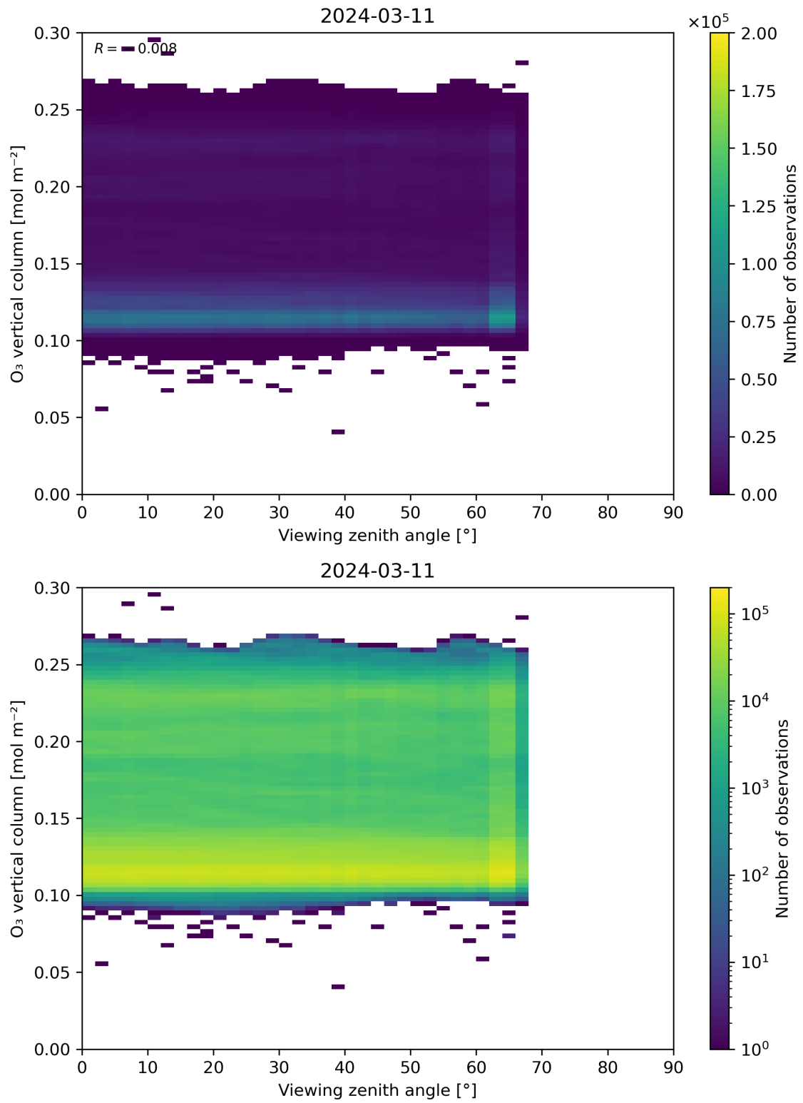
Figure 52: Scatter density plot of “Viewing zenith angle” against “O 3 vertical column” for 2024-03-10 to 2024-03-12.
