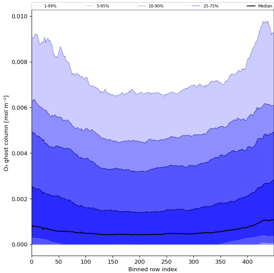
Figure 32: Along track statistics of “O 3 ghost column” for 2024-03-10 to 2024-03-12
