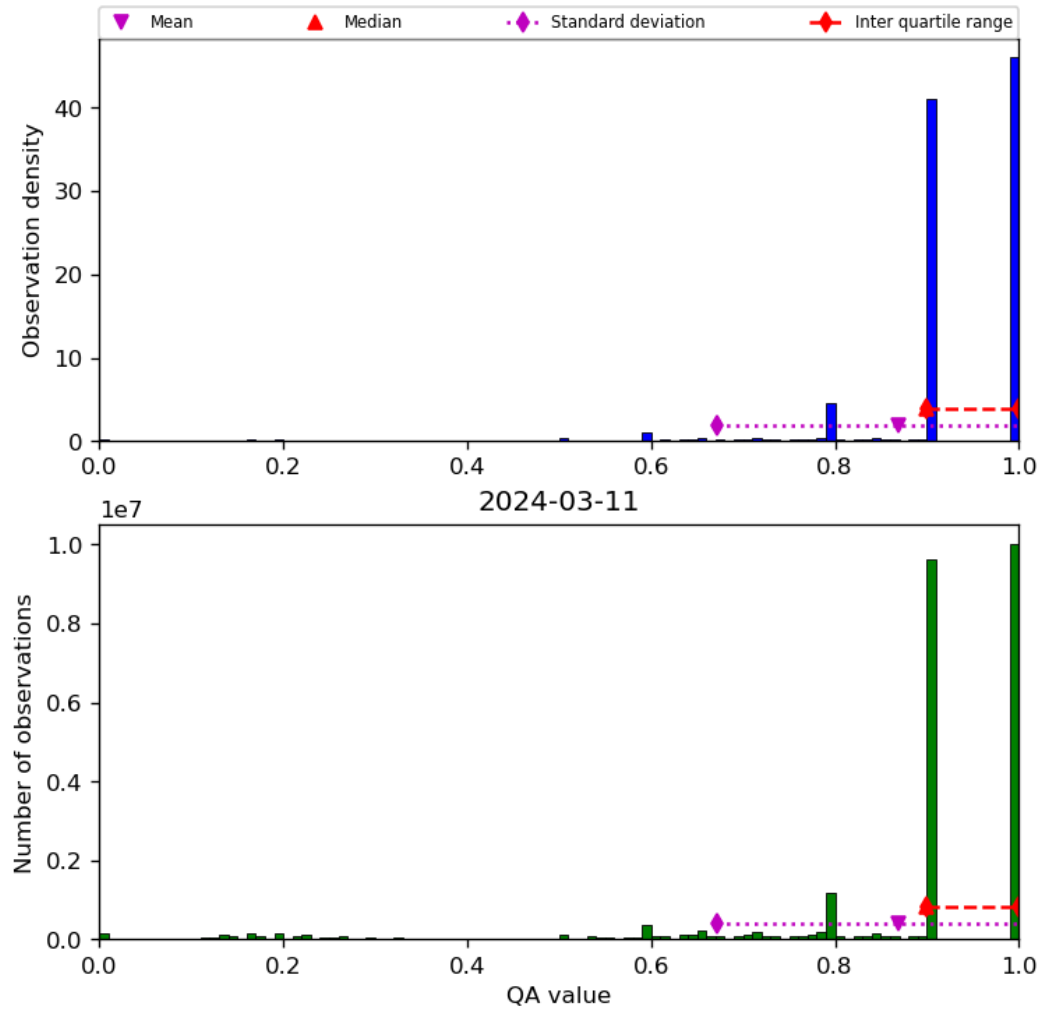
Figure 20: Histogram of “QA value” for 2024-03-10 to 2024-03-12
