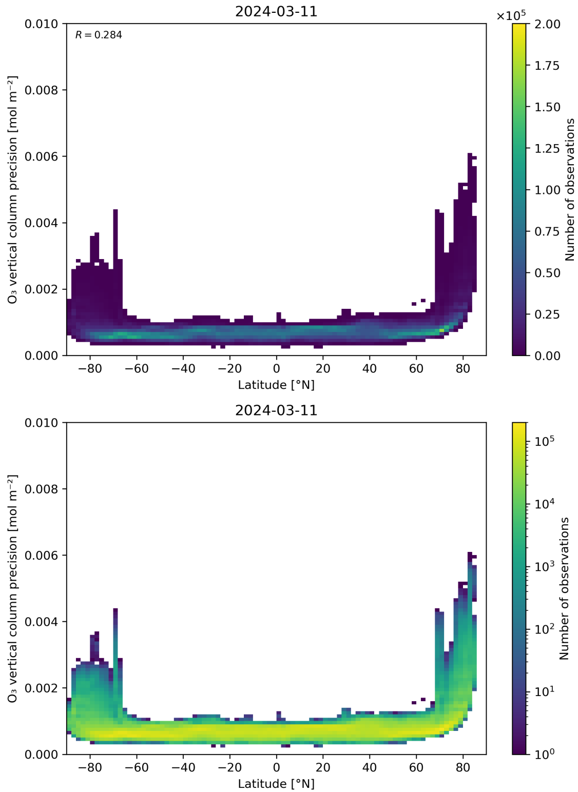
Figure 37: Scatter density plot of “Latitude” against “O 3 vertical column precision” for 2024-03-10 to 2024-03-12.
