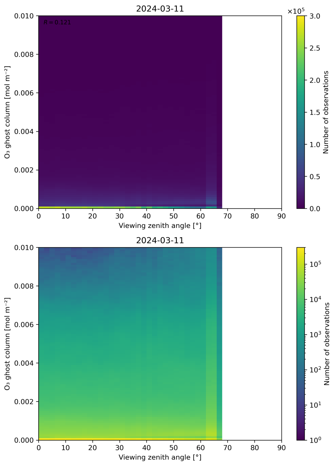
Figure 51: Scatter density plot of “Viewing zenith angle” against “O 3 ghost column” for 2024-03-10 to 2024-03-12.
