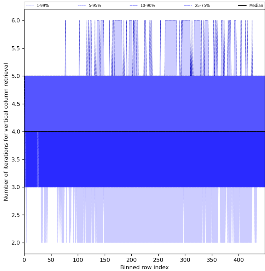
Figure 33: Along track statistics of “Number of iterations for vertical column retrieval” for 2024-03-10 to 2024-03-12
