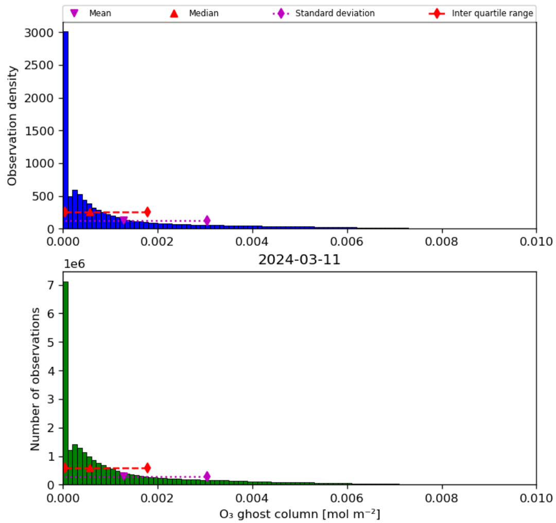
Figure 25: Histogram of “O 3 ghost column” for 2024-03-10 to 2024-03-12
