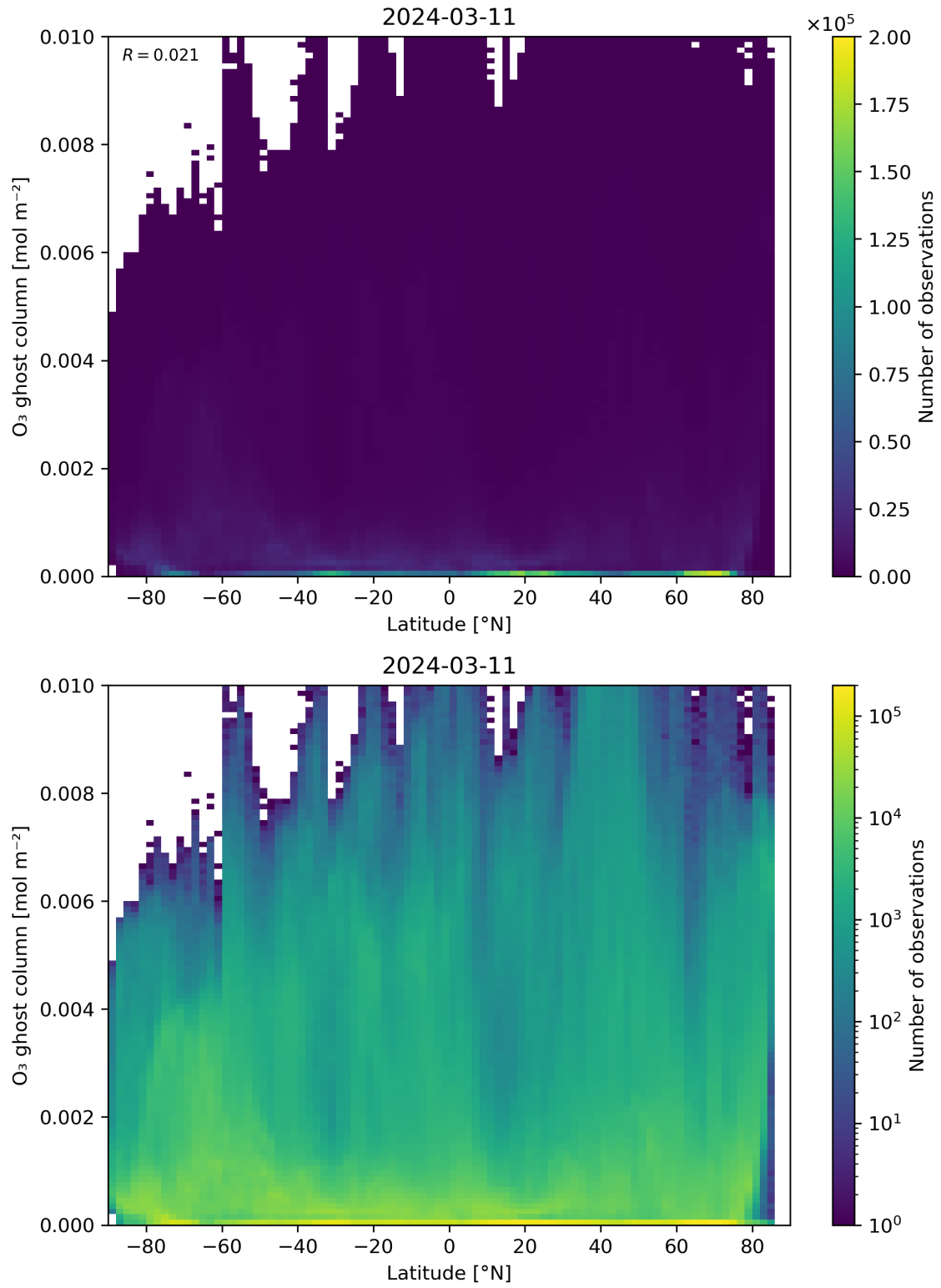
Figure 35: Scatter density plot of “Latitude” against “O 3 ghost column” for 2024-03-10 to 2024-03-12.
