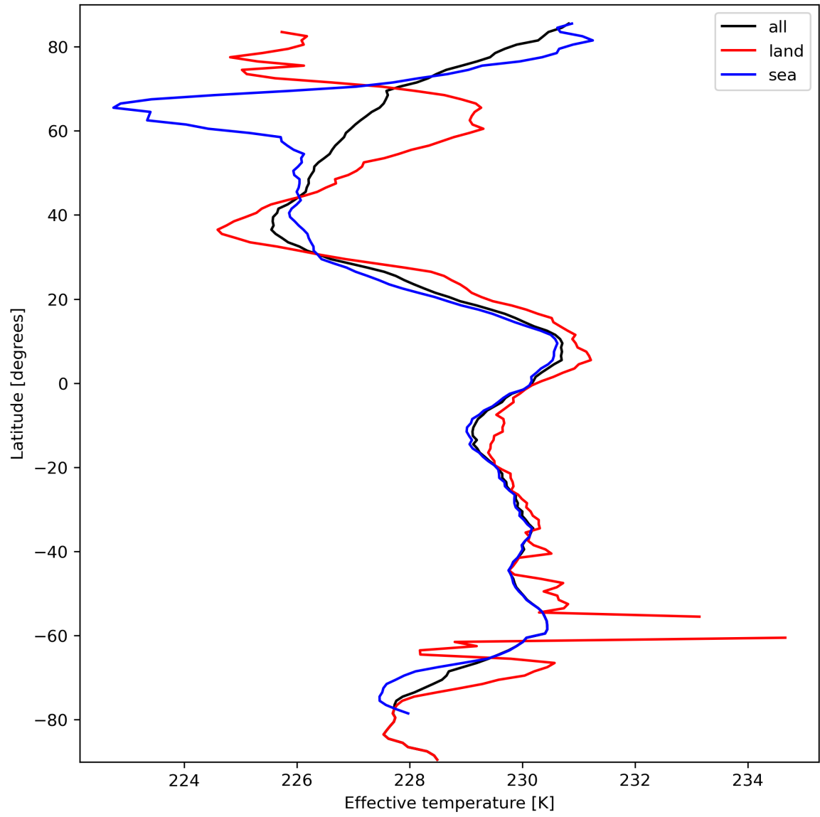
Figure 17: Zonal average of “Effective temperature” for 2024-03-10 to 2024-03-12.
