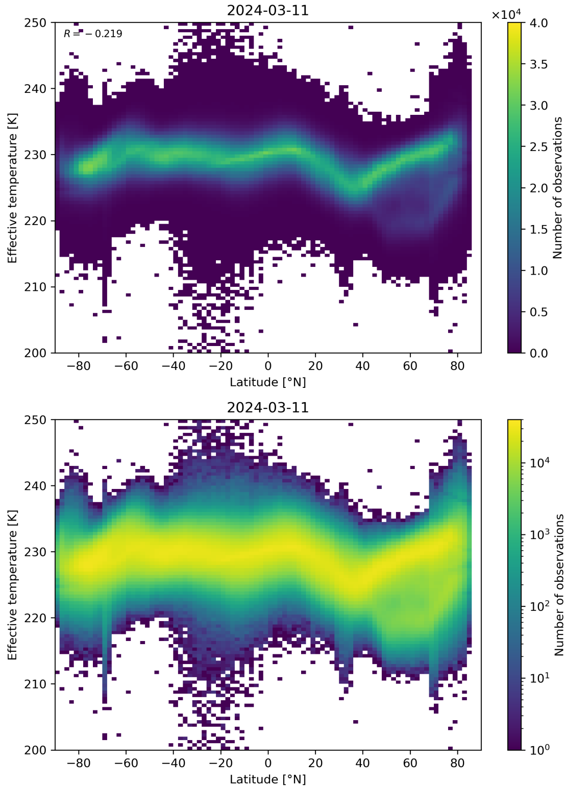
Figure 34: Scatter density plot of “Latitude” against “Effective temperature” for 2024-03-10 to 2024-03-12.
