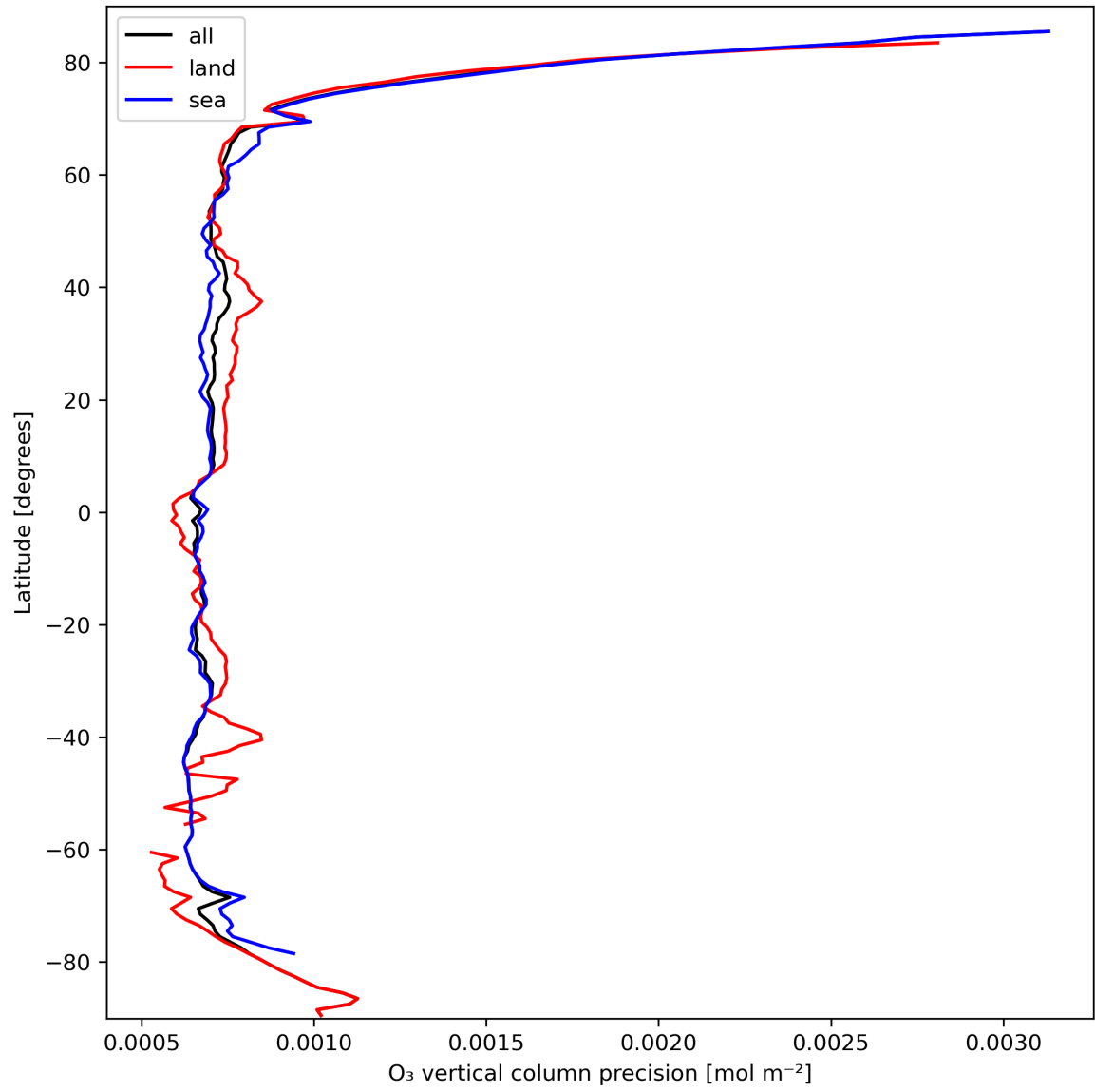
Figure 15: Zonal average of “O 3 vertical column precision” for 2024-03-10 to 2024-03-12.
