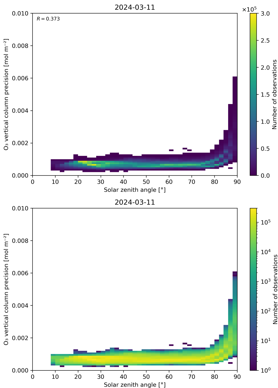
Figure 48: Scatter density plot of “Solar zenith angle” against “O 3 vertical column precision” for 2024-03-10 to 2024-03-12.
