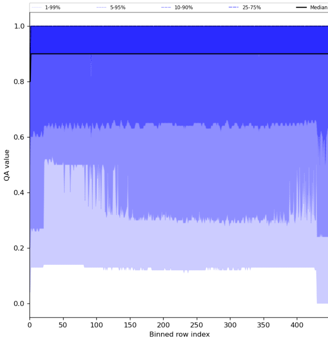
Figure 27: Along track statistics of “QA value” for 2024-03-10 to 2024-03-12
