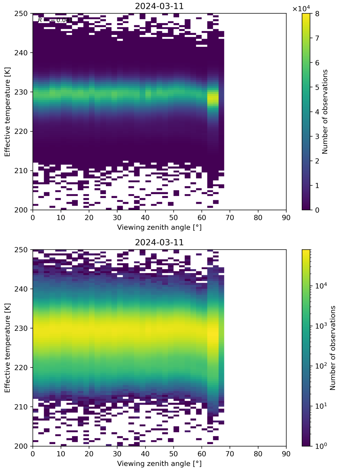
Figure 50: Scatter density plot of “Viewing zenith angle” against “Effective temperature” for 2024-03-10 to 2024-03-12.
