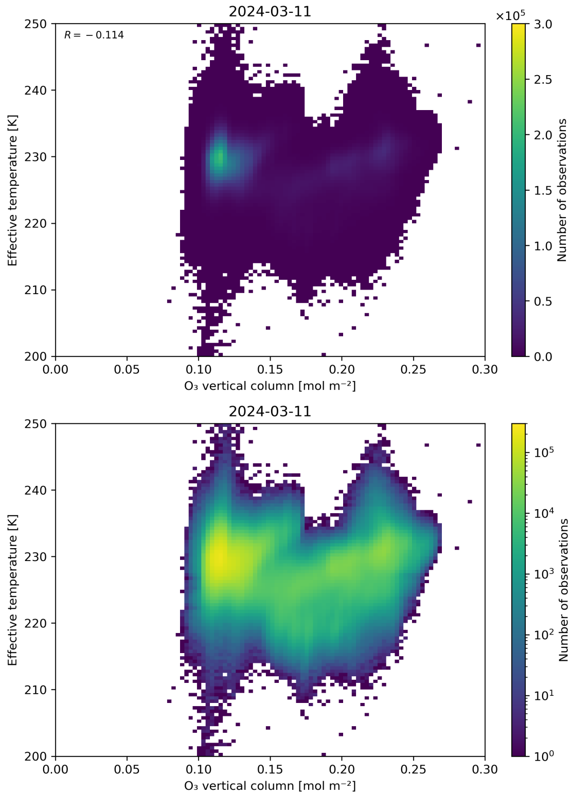
Figure 39: Scatter density plot of “O 3 vertical column” against “Effective temperature” for 2024-03-10 to 2024-03-12.
