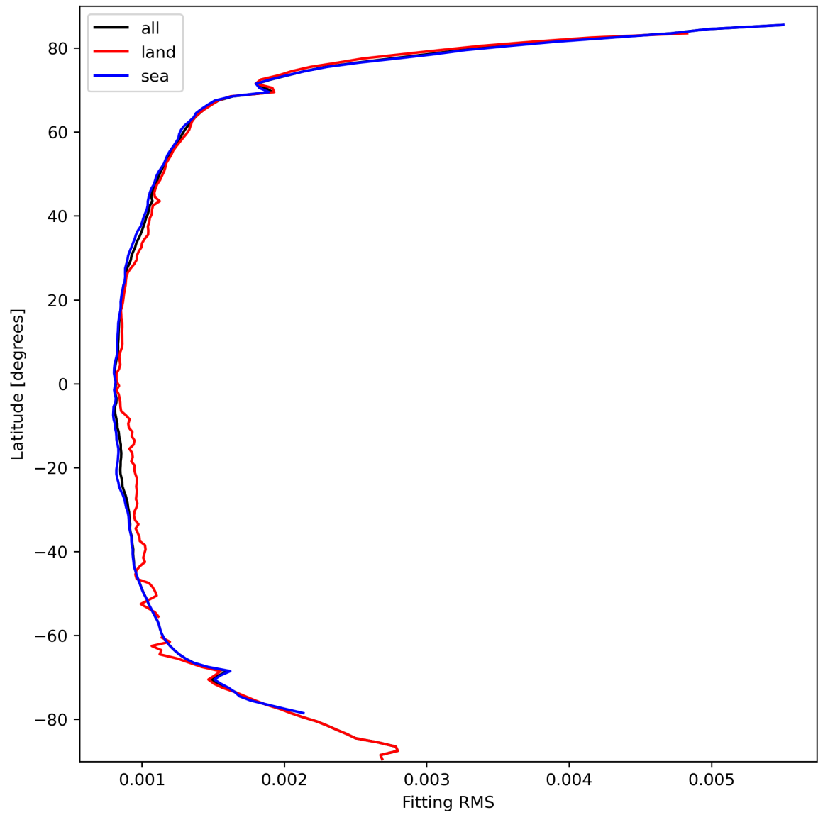
Figure 16: Zonal average of “Fitting RMS” for 2024-03-10 to 2024-03-12.
