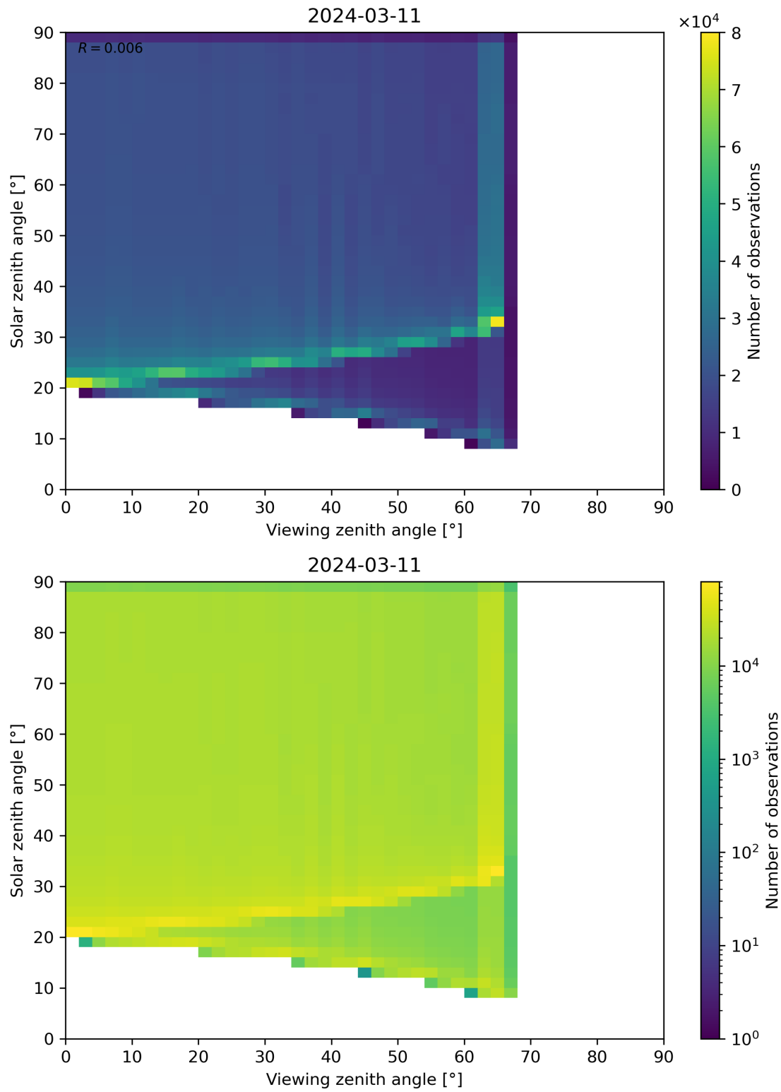
Figure 54: Scatter density plot of “Viewing zenith angle” against “Solar zenith angle” for 2024-03-10 to 2024-03-12.
