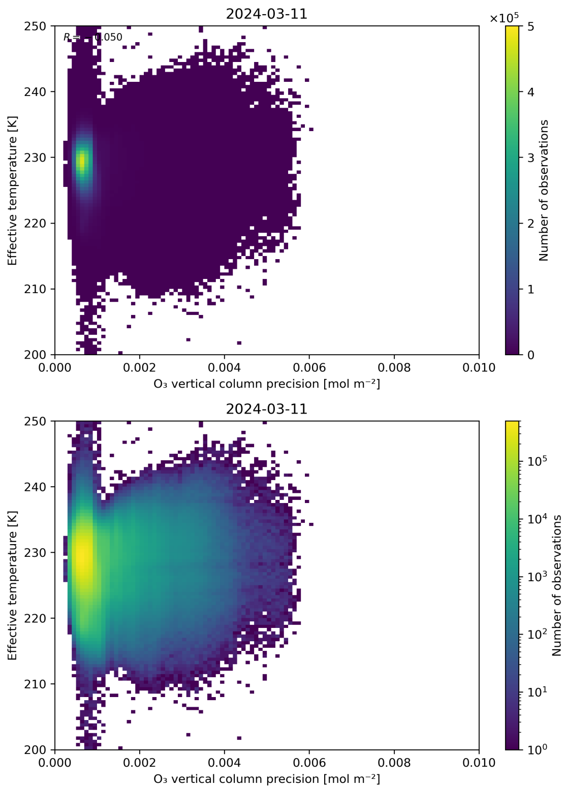
Figure 42: Scatter density plot of “O 3 vertical column precision” against “Effective temperature” for 2024-03-10 to 2024-03-12.
