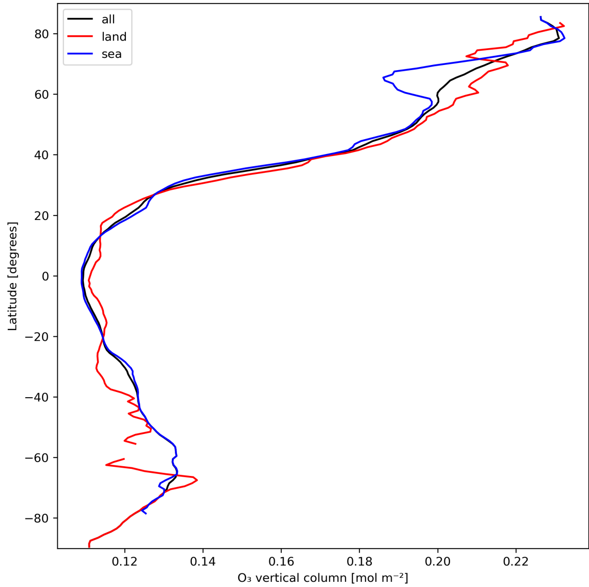
Figure 14: Zonal average of “O 3 vertical column” for 2024-03-10 to 2024-03-12.
