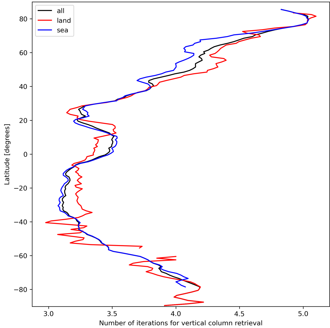
Figure 19: Zonal average of “Number of iterations for vertical column retrieval” for 2024-03-10 to 2024-03-12.
