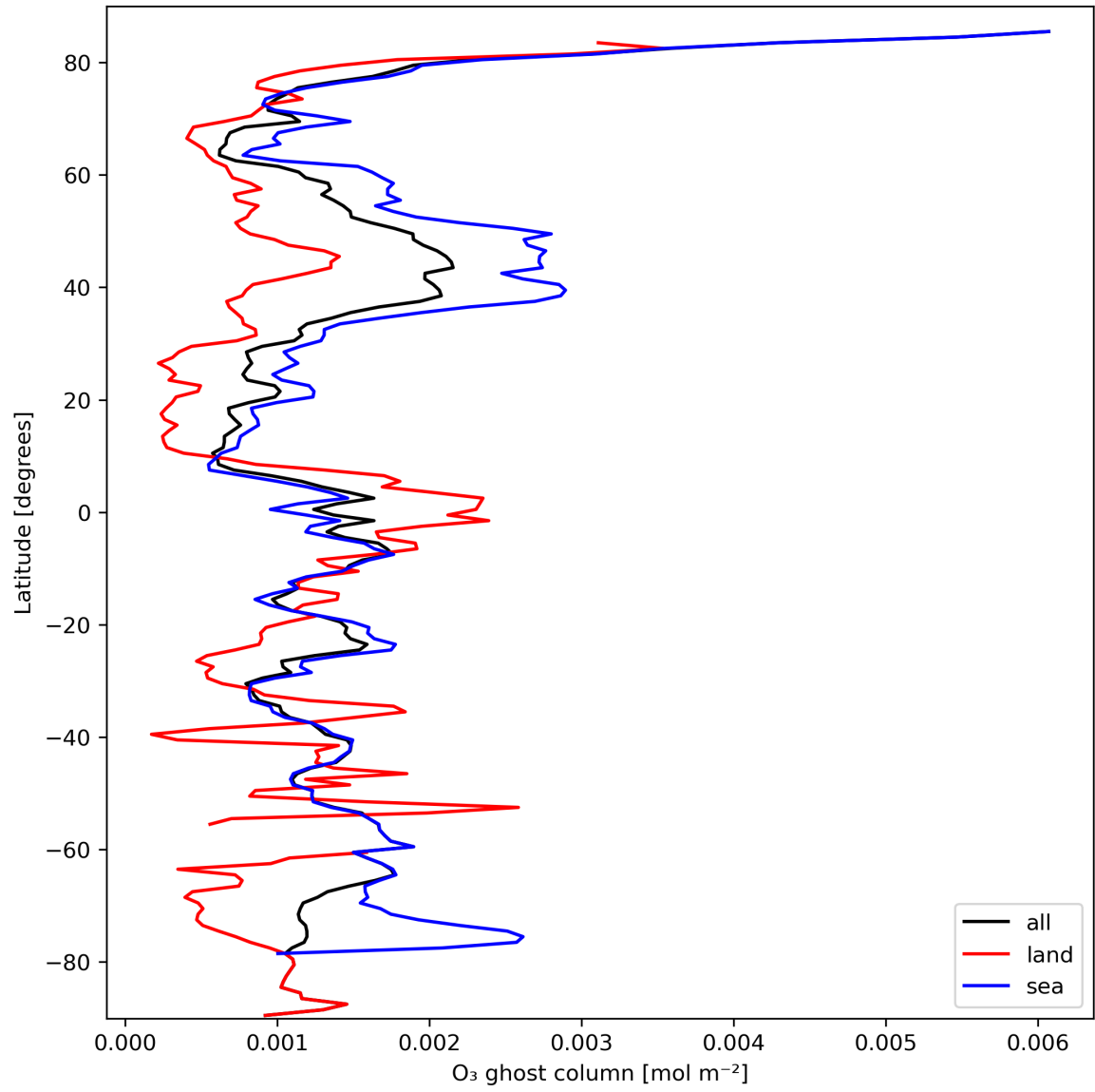
Figure 18: Zonal average of “O 3 ghost column” for 2024-03-10 to 2024-03-12.
