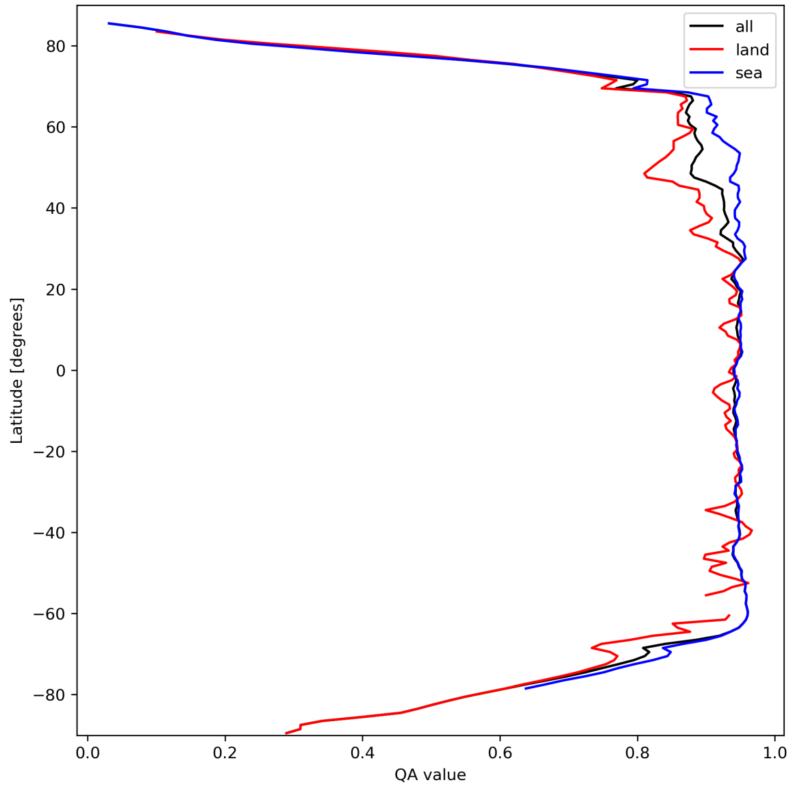
Figure 13: Zonal average of “QA value” for 2024-03-10 to 2024-03-12.
