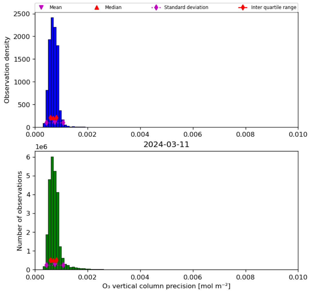
Figure 22: Histogram of “O 3 vertical column precision” for 2024-03-10 to 2024-03-12
