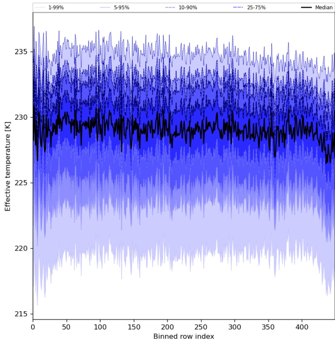
Figure 31: Along track statistics of “Effective temperature” for 2024-03-10 to 2024-03-12
