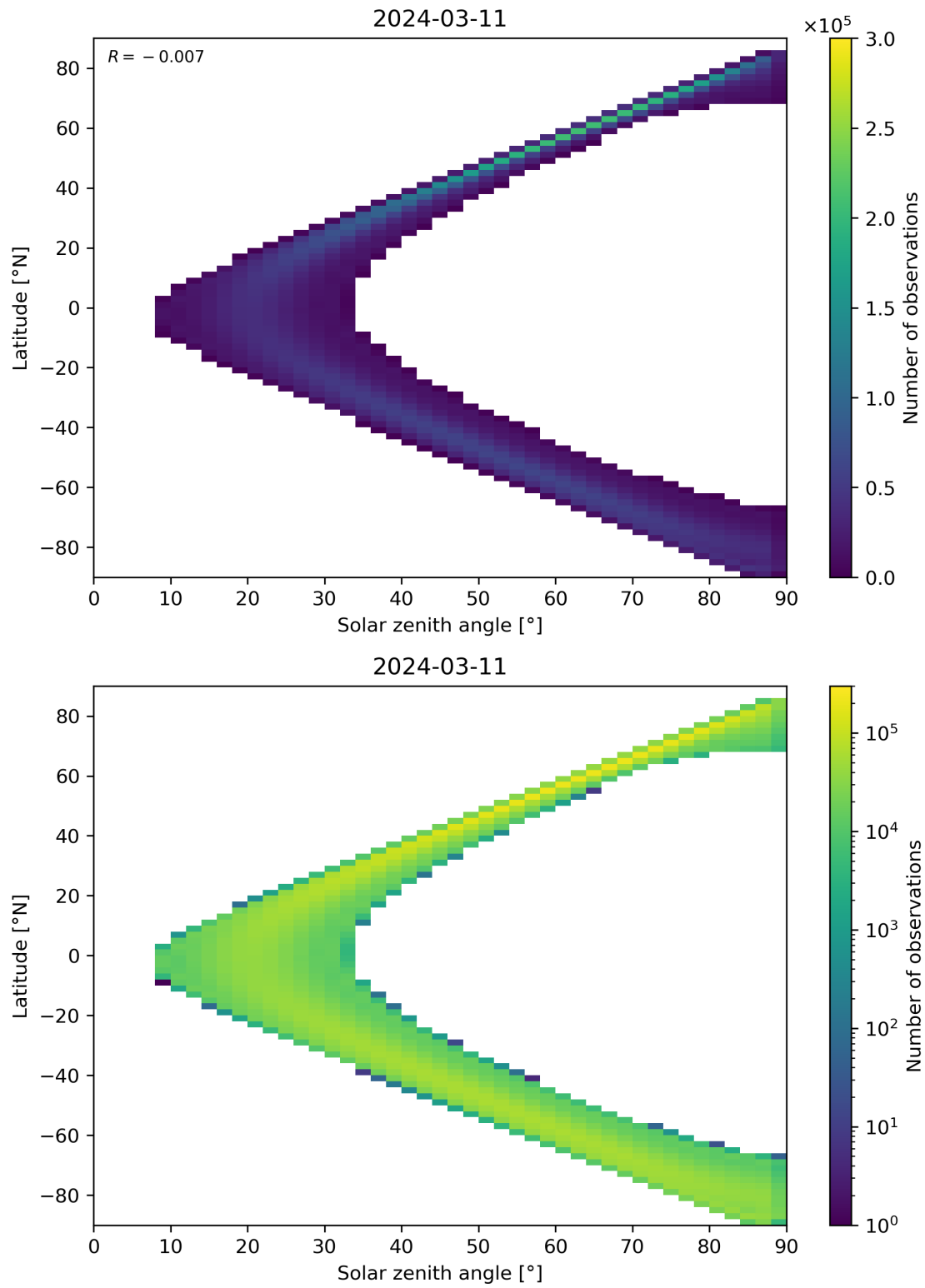
Figure 44: Scatter density plot of “Solar zenith angle” against “Latitude” for 2024-03-10 to 2024-03-12.
