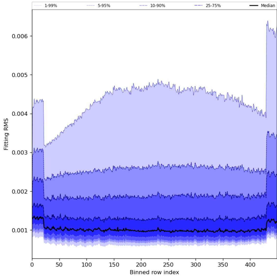
Figure 30: Along track statistics of “Fitting RMS” for 2024-03-10 to 2024-03-12
