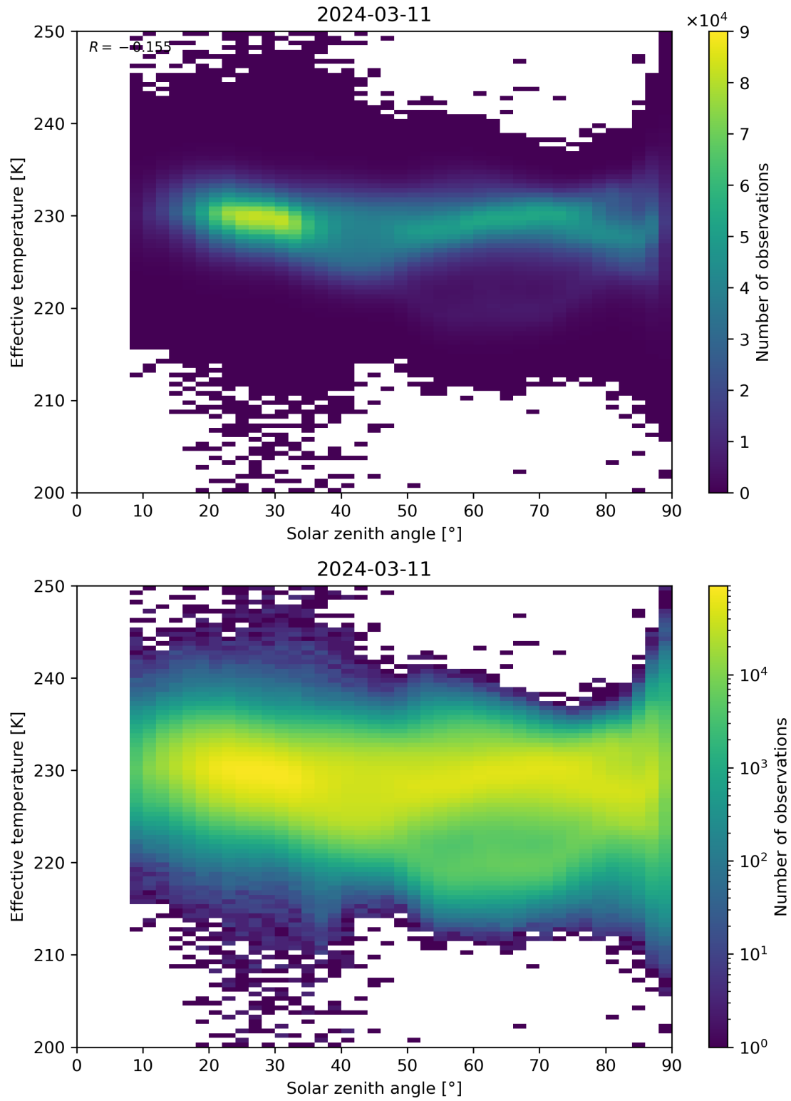
Figure 45: Scatter density plot of “Solar zenith angle” against “Effective temperature” for 2024-03-10 to 2024-03-12.
