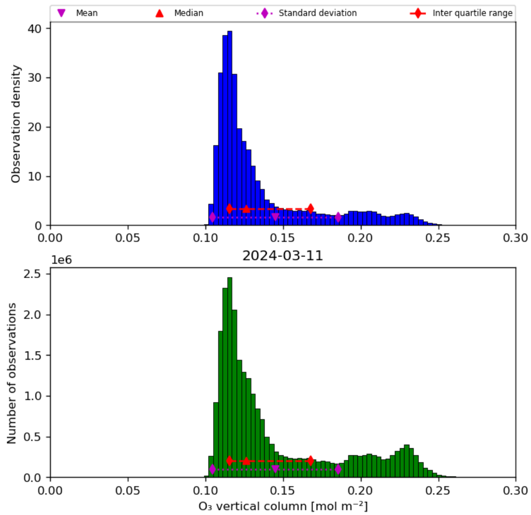
Figure 21: Histogram of “O 3 vertical column” for 2024-03-10 to 2024-03-12
