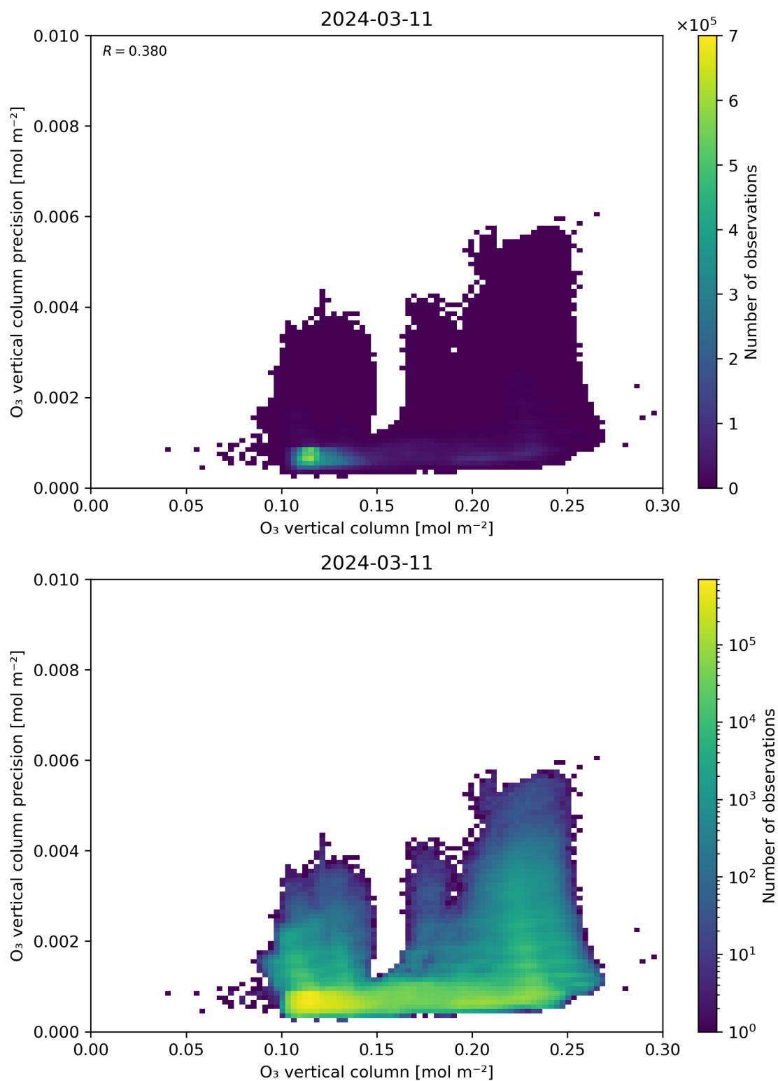
Figure 41: Scatter density plot of “O 3 vertical column” against “O 3 vertical column precision” for 2024-03-10 to 2024-03-12.
