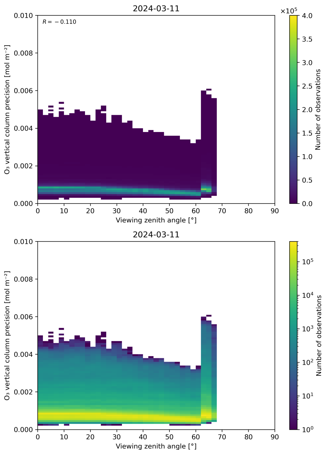
Figure 53: Scatter density plot of “Viewing zenith angle” against “O 3 vertical column precision” for 2024-03-10 to 2024-03-12.
