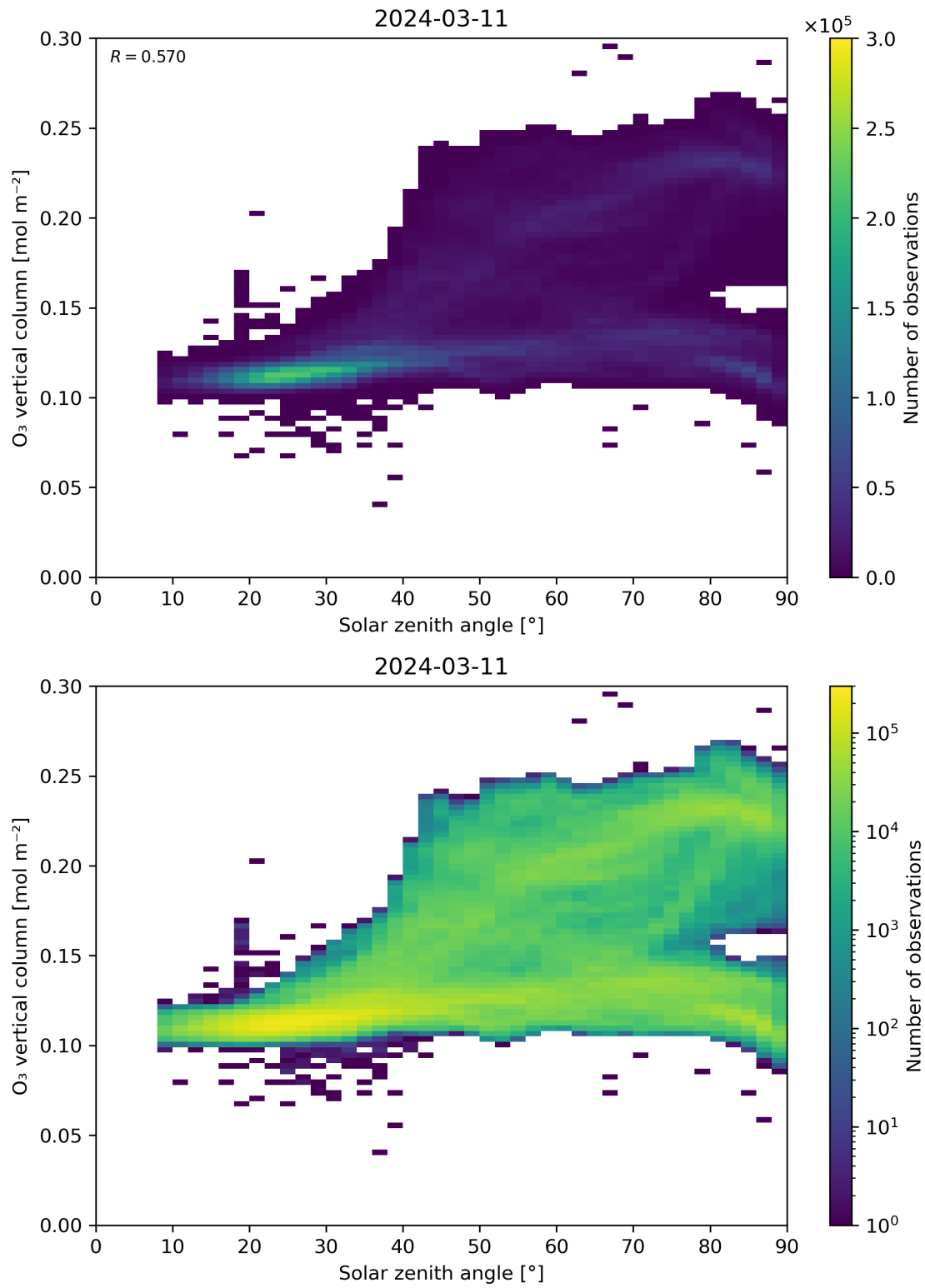
Figure 47: Scatter density plot of “Solar zenith angle” against “O 3 vertical column” for 2024-03-10 to 2024-03-12.
