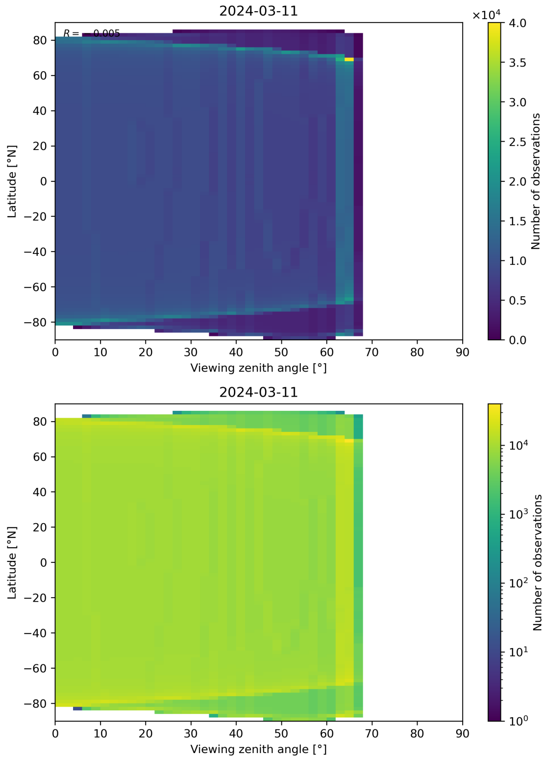
Figure 49: Scatter density plot of “Viewing zenith angle” against “Latitude” for 2024-03-10 to 2024-03-12.
