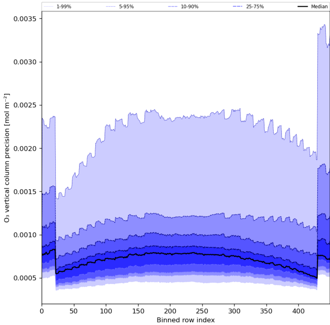
Figure 29: Along track statistics of “O 3 vertical column precision” for 2024-03-10 to 2024-03-12
