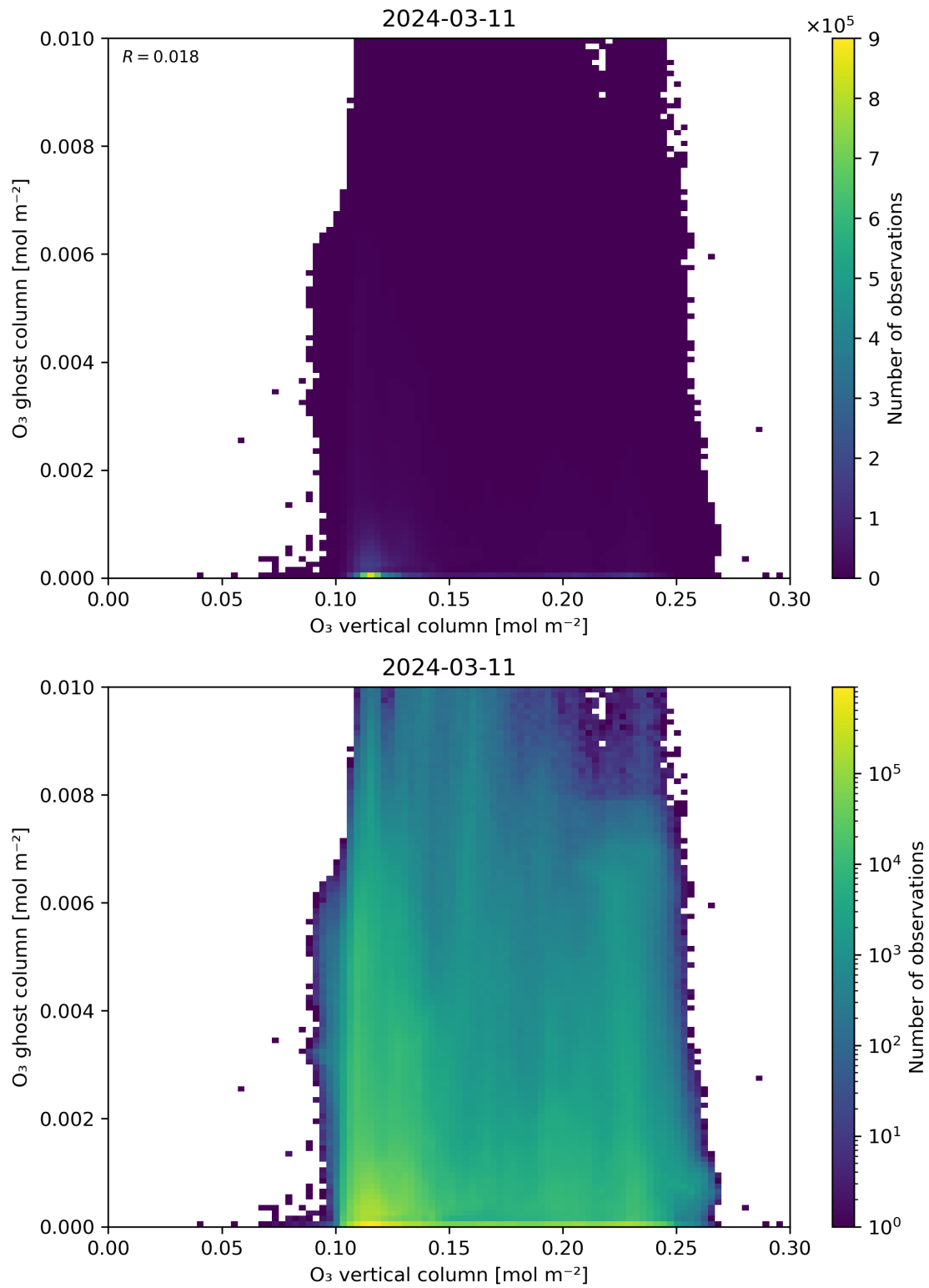
Figure 40: Scatter density plot of “O 3 vertical column” against “O 3 ghost column” for 2024-03-10 to 2024-03-12.
