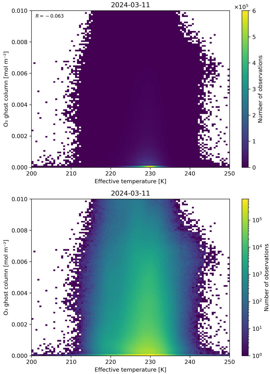
Figure 38: Scatter density plot of “Effective temperature” against “O 3 ghost column” for 2024-03-10 to 2024-03-12.
