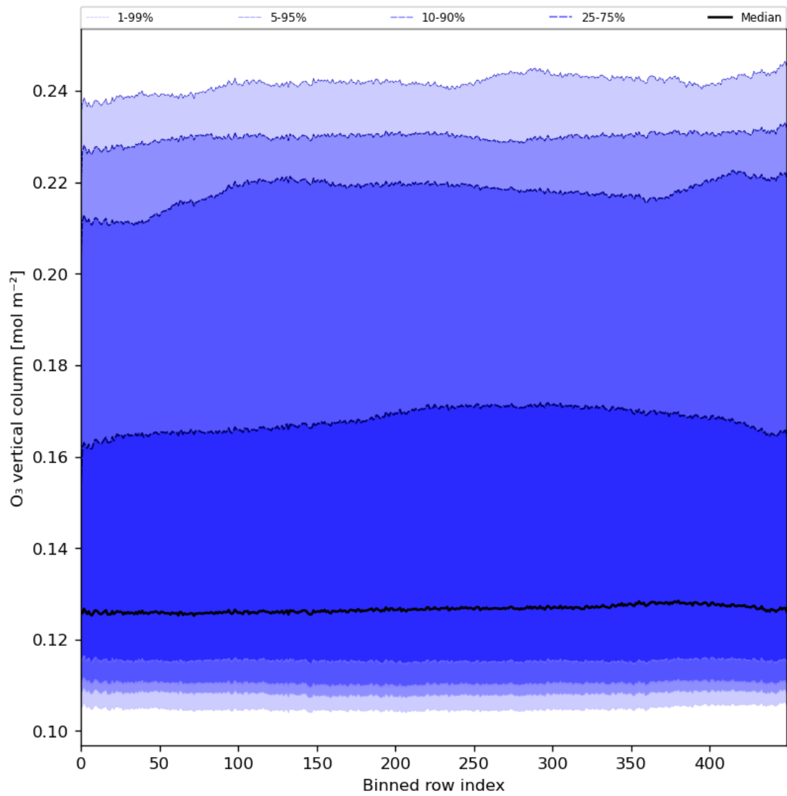
Figure 28: Along track statistics of “O 3 vertical column” for 2024-03-10 to 2024-03-12
