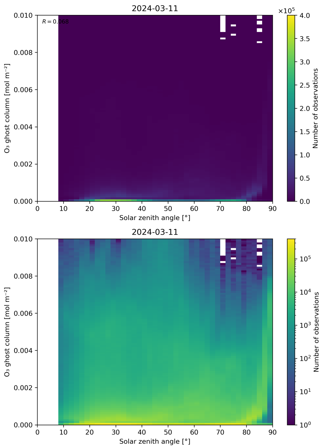
Figure 46: Scatter density plot of “Solar zenith angle” against “O 3 ghost column” for 2024-03-10 to 2024-03-12.
