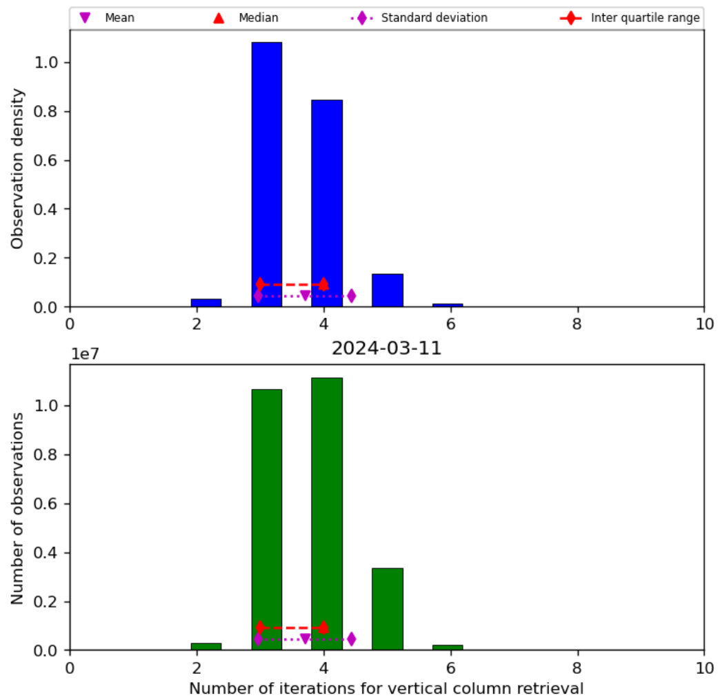
Figure 26: Histogram of “Number of iterations for vertical column retrieval” for 2024-03-10 to 2024-03-12
