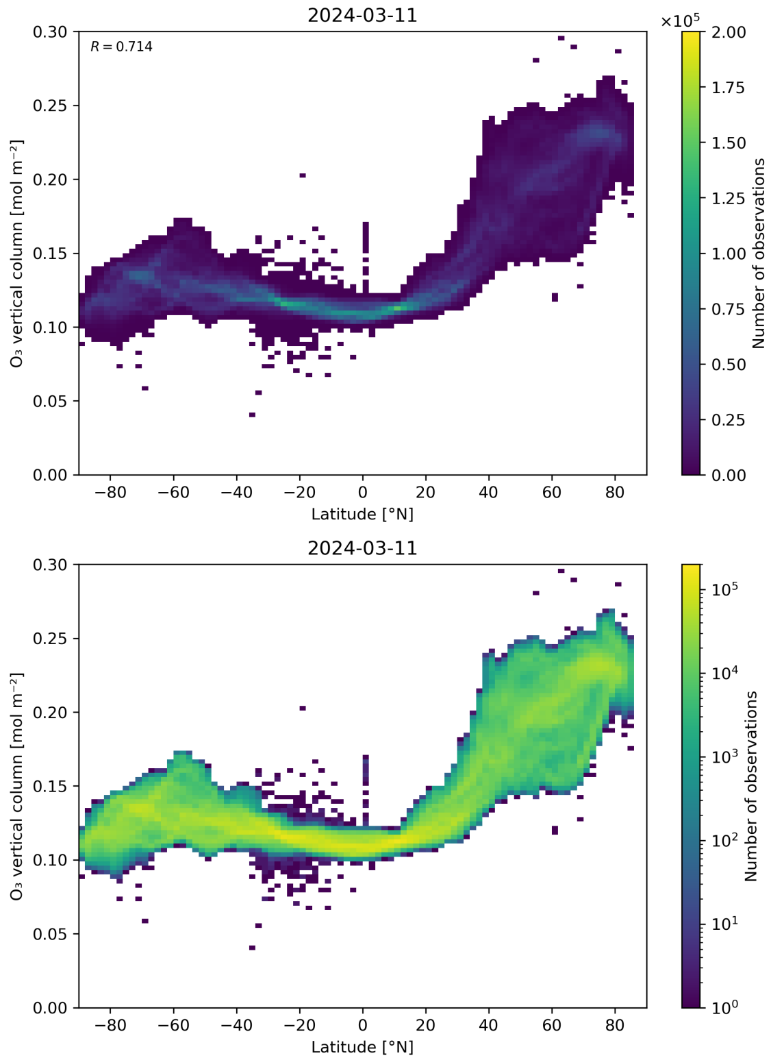
Figure 36: Scatter density plot of “Latitude” against “O 3 vertical column” for 2024-03-10 to 2024-03-12.
