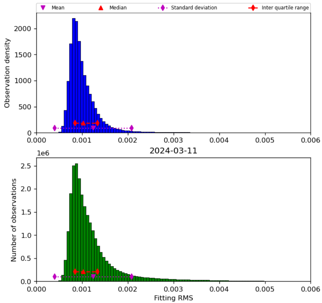
Figure 23: Histogram of “Fitting RMS” for 2024-03-10 to 2024-03-12
