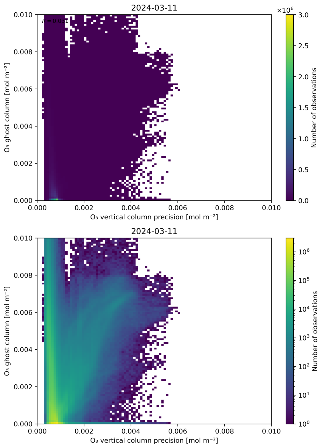
Figure 43: Scatter density plot of “O 3 vertical column precision” against “O 3 ghost column” for 2024-03-10 to 2024-03-12.
