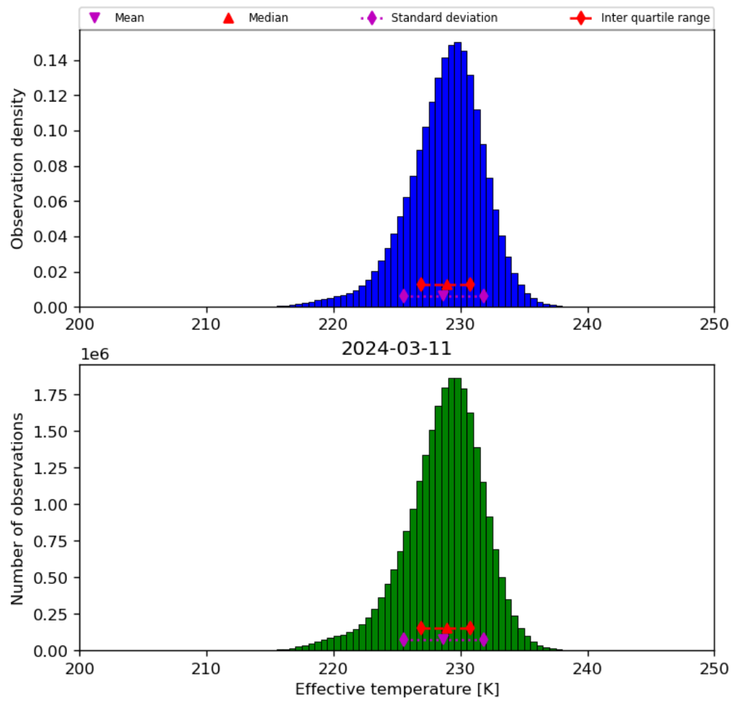
Figure 24: Histogram of “Effective temperature” for 2024-03-10 to 2024-03-12
