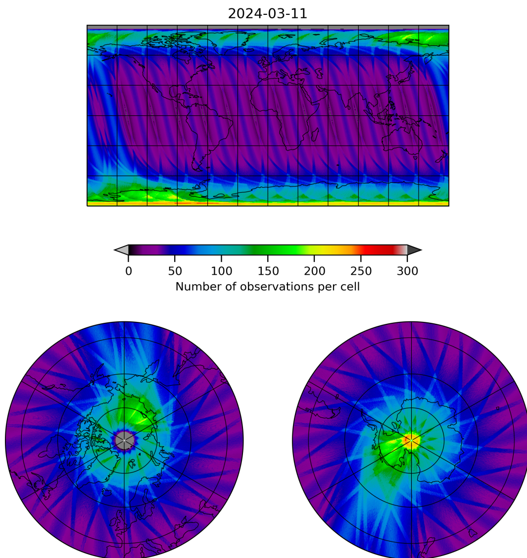
Figure 12: Map of the number of observations for 2024-03-10 to 2024-03-12
