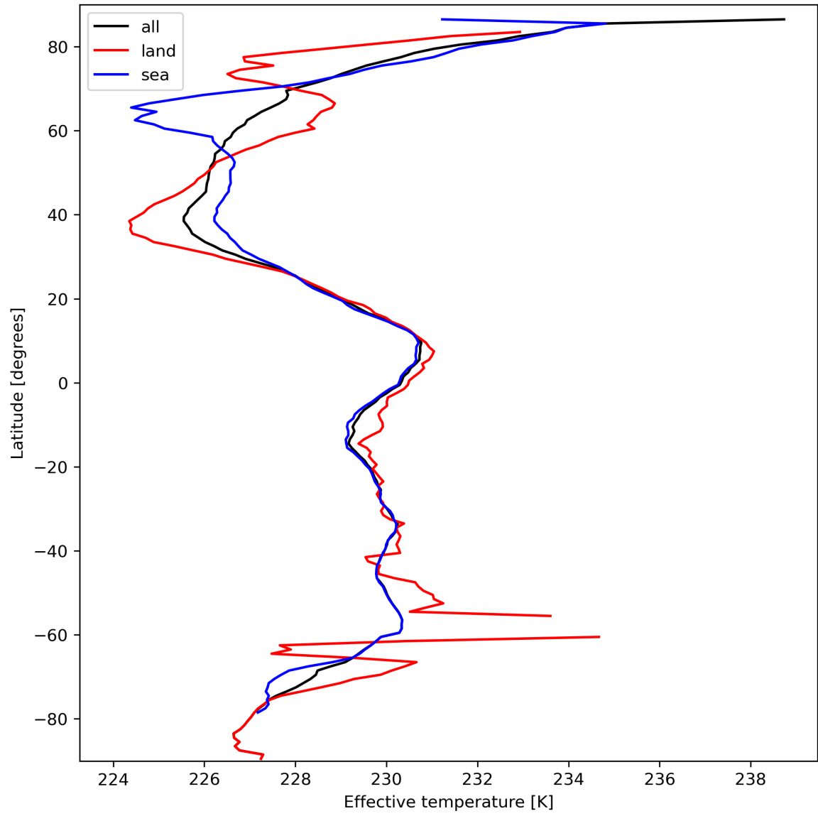
Figure 17: Zonal average of “Effective temperature” for 2024-03-11 to 2024-03-13.
