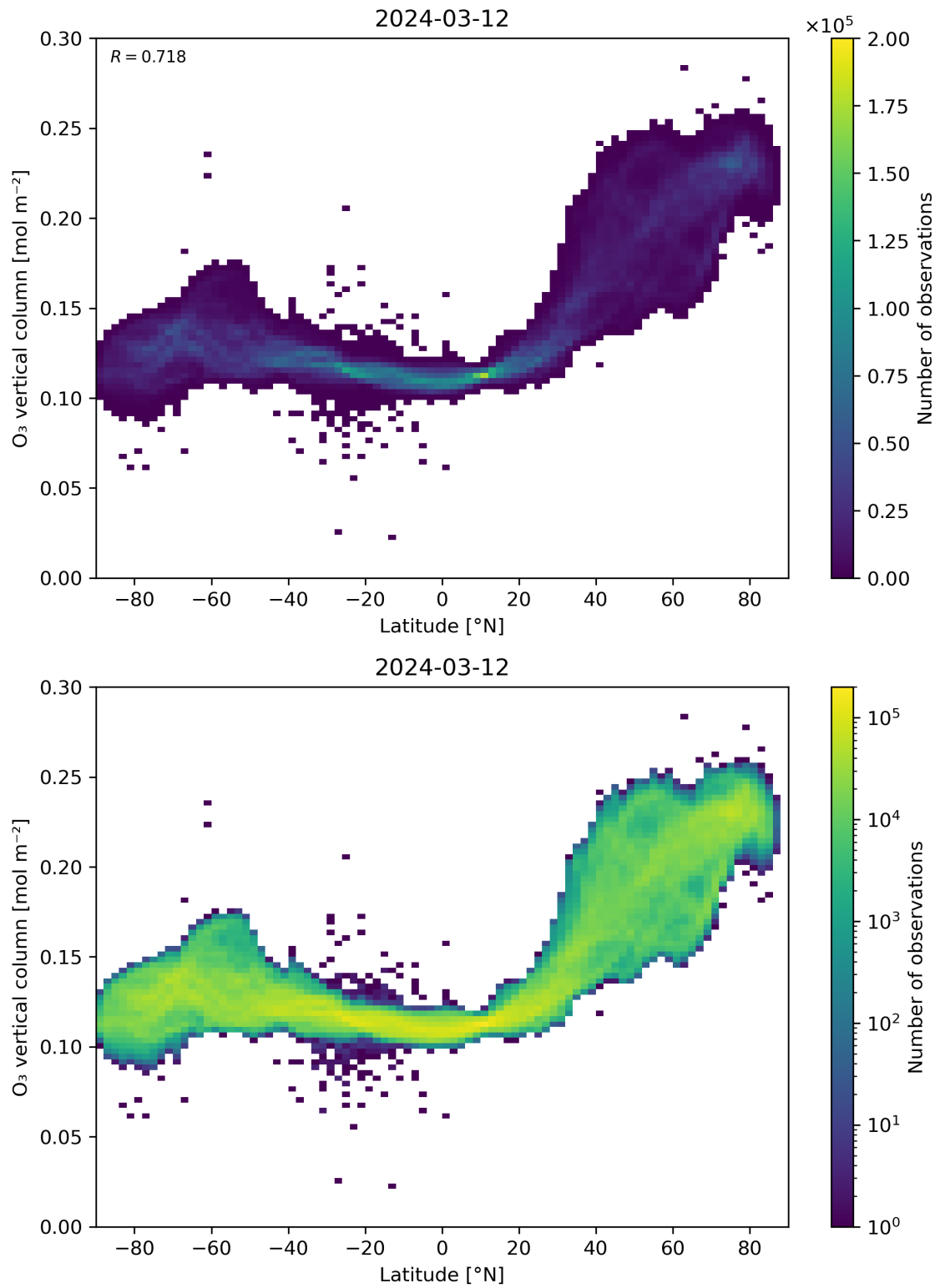
Figure 36: Scatter density plot of “Latitude” against “O 3 vertical column” for 2024-03-11 to 2024-03-13.
