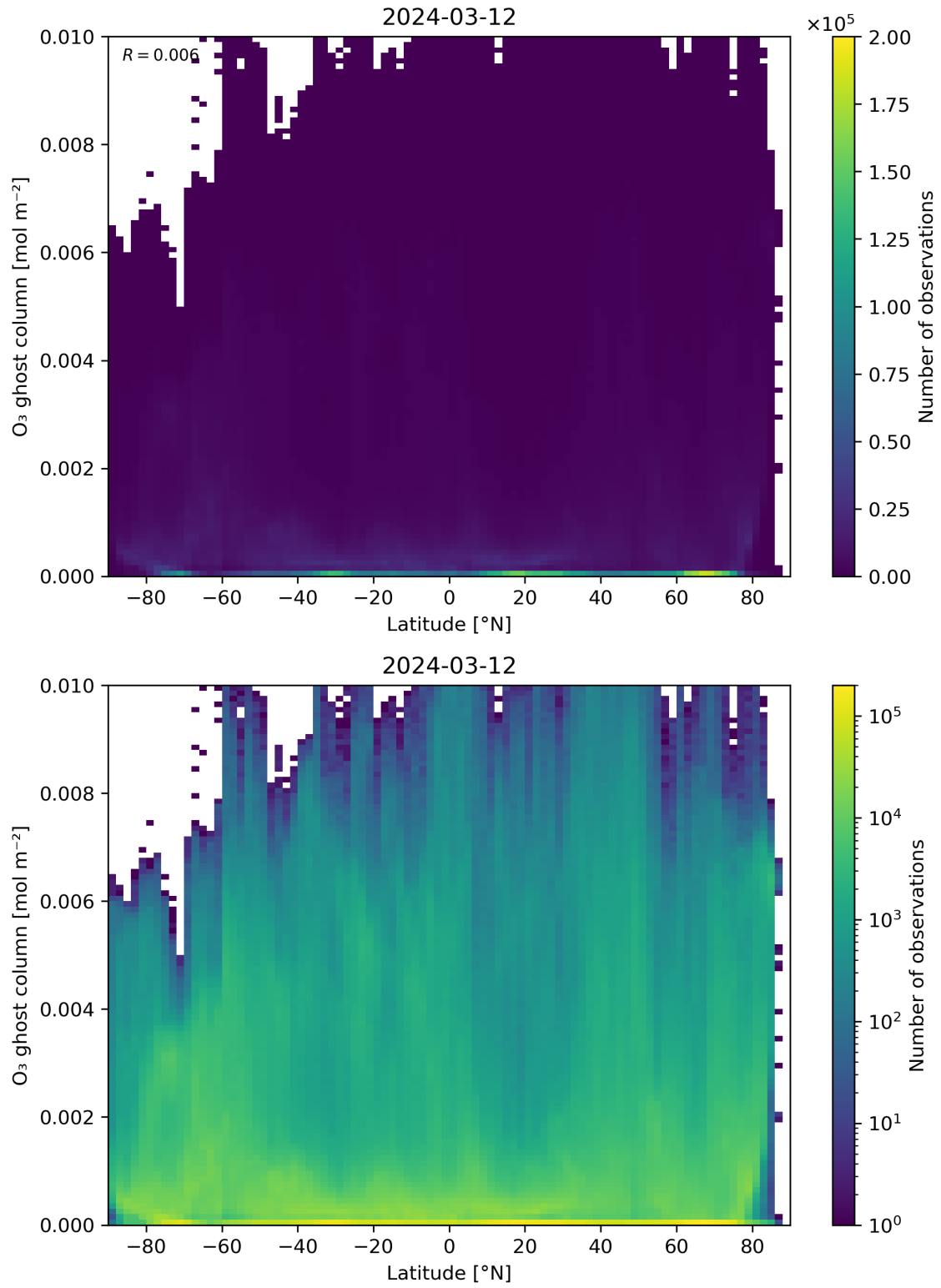
Figure 35: Scatter density plot of “Latitude” against “O 3 ghost column” for 2024-03-11 to 2024-03-13.
