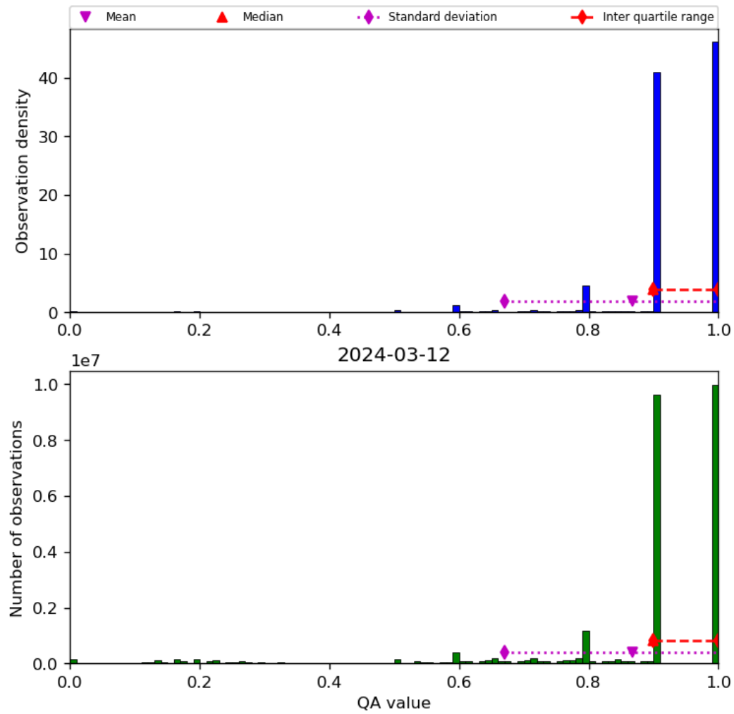
Figure 20: Histogram of “QA value” for 2024-03-11 to 2024-03-13
