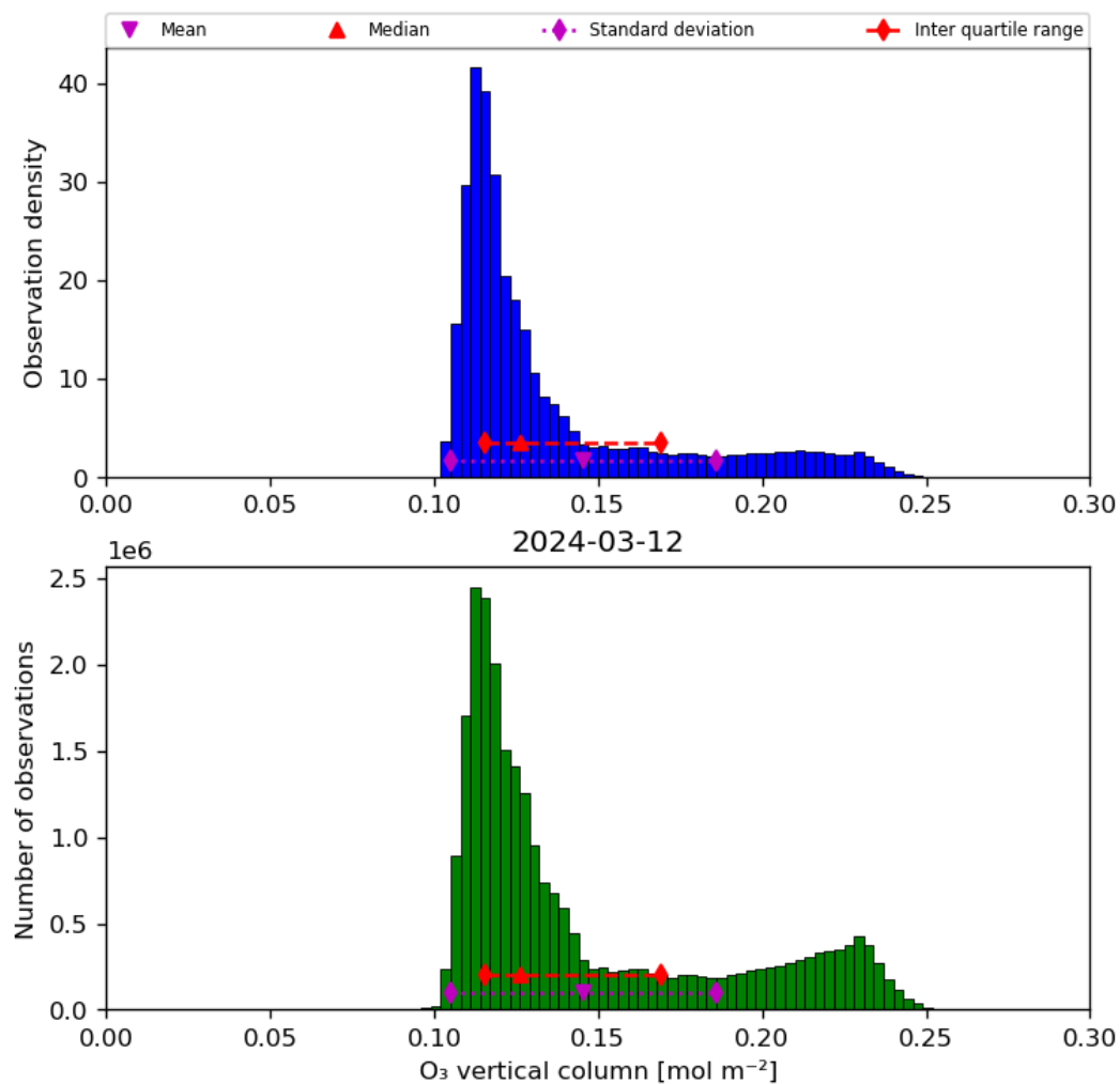
Figure 21: Histogram of “O 3 vertical column” for 2024-03-11 to 2024-03-13
