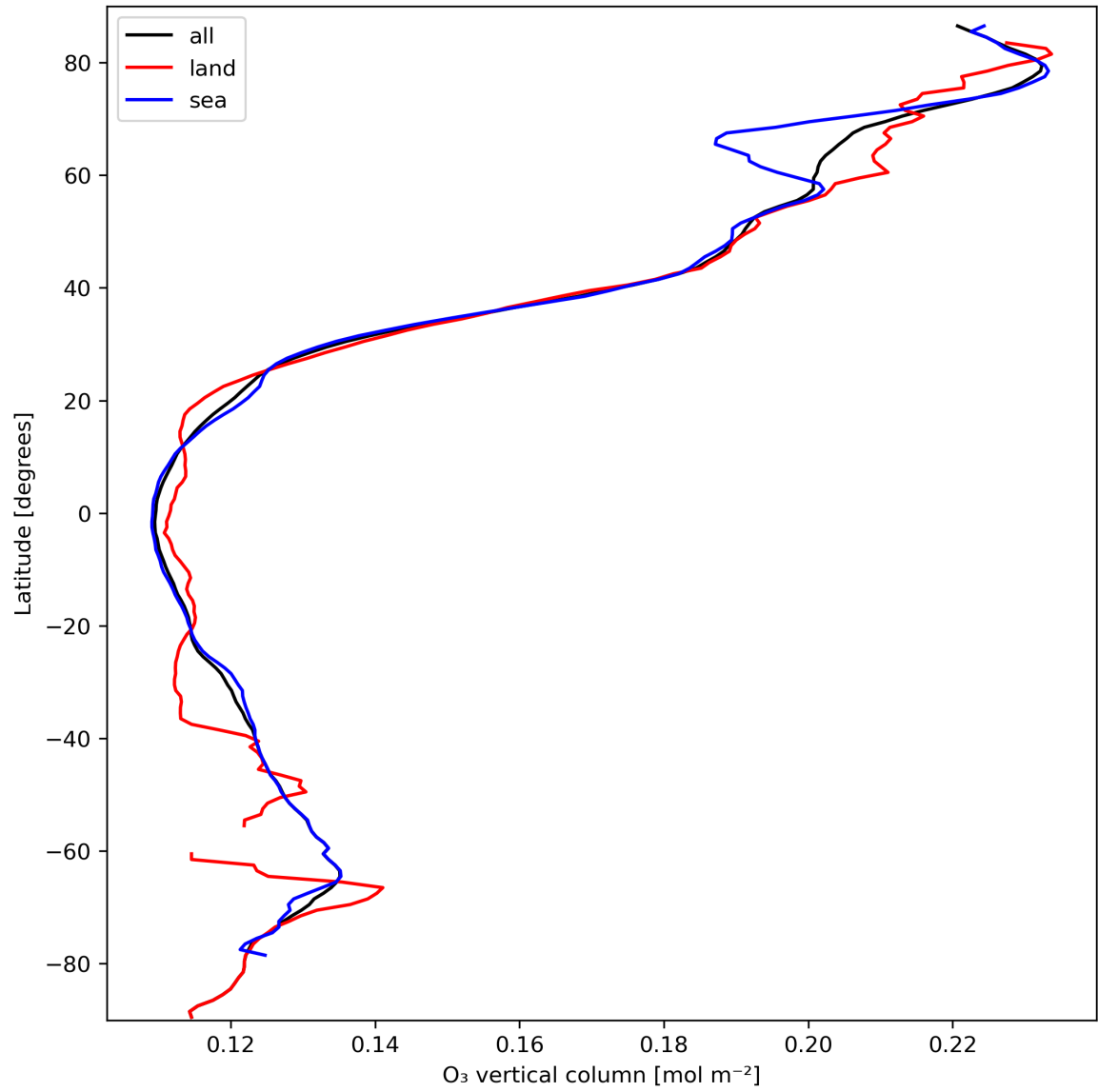
Figure 14: Zonal average of “O 3 vertical column” for 2024-03-11 to 2024-03-13.
