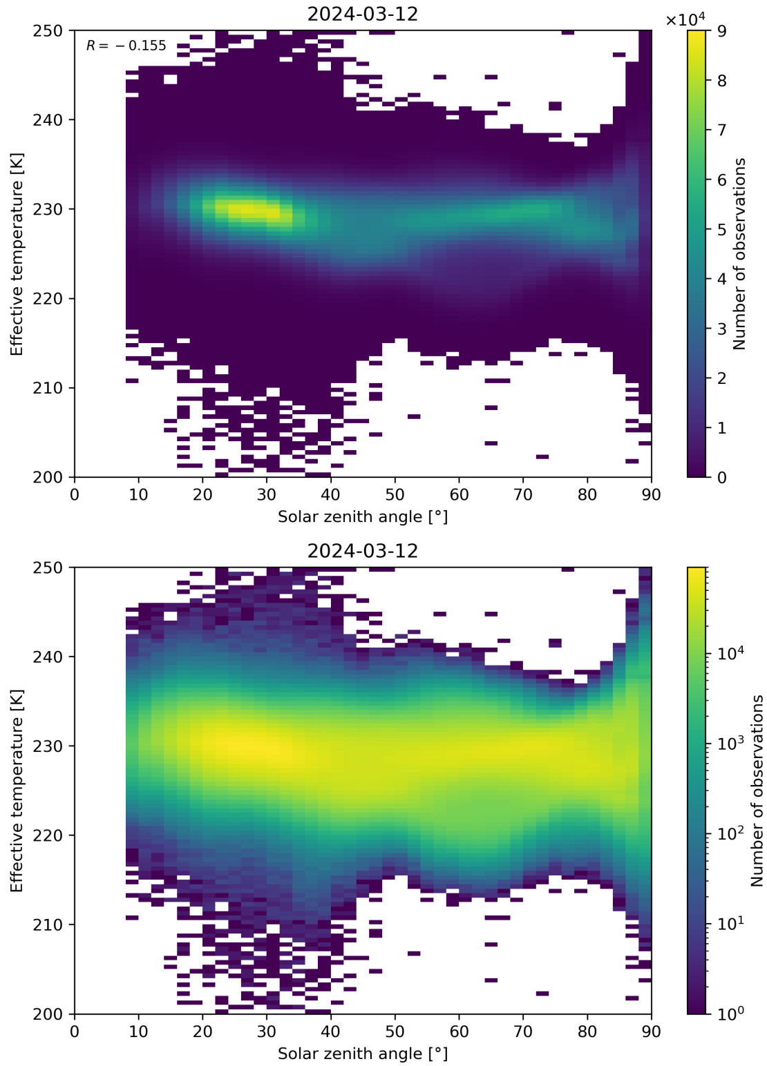
Figure 45: Scatter density plot of “Solar zenith angle” against “Effective temperature” for 2024-03-11 to 2024-03-13.
