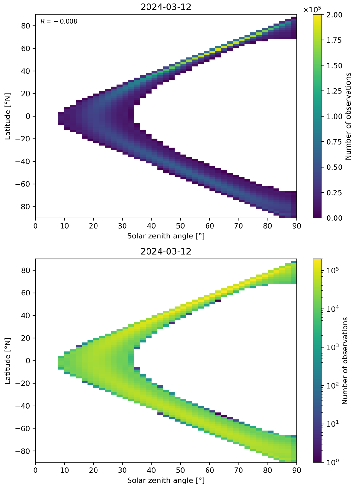
Figure 44: Scatter density plot of “Solar zenith angle” against “Latitude” for 2024-03-11 to 2024-03-13.
