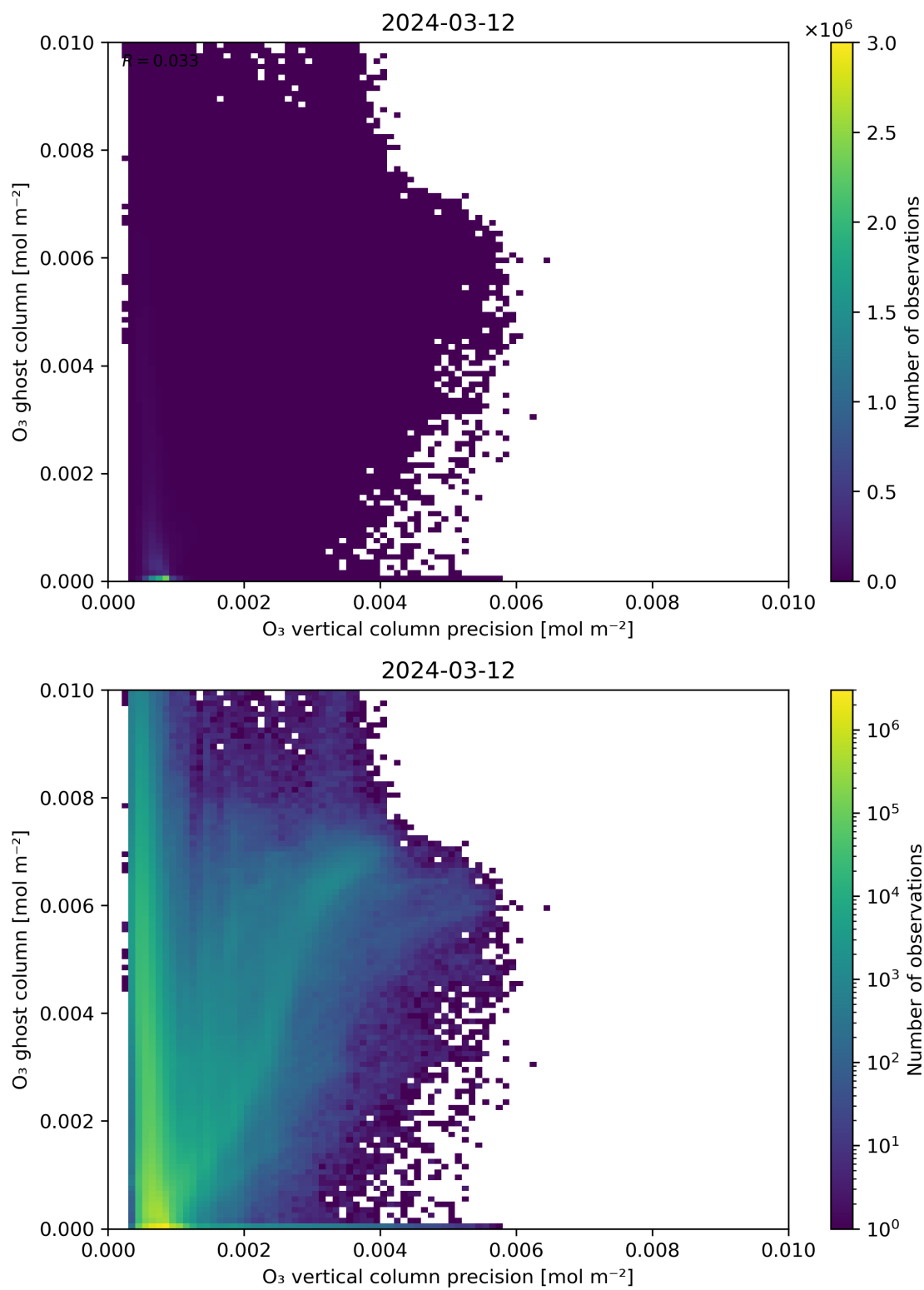
Figure 43: Scatter density plot of “O 3 vertical column precision” against “O 3 ghost column” for 2024-03-11 to 2024-03-13.
