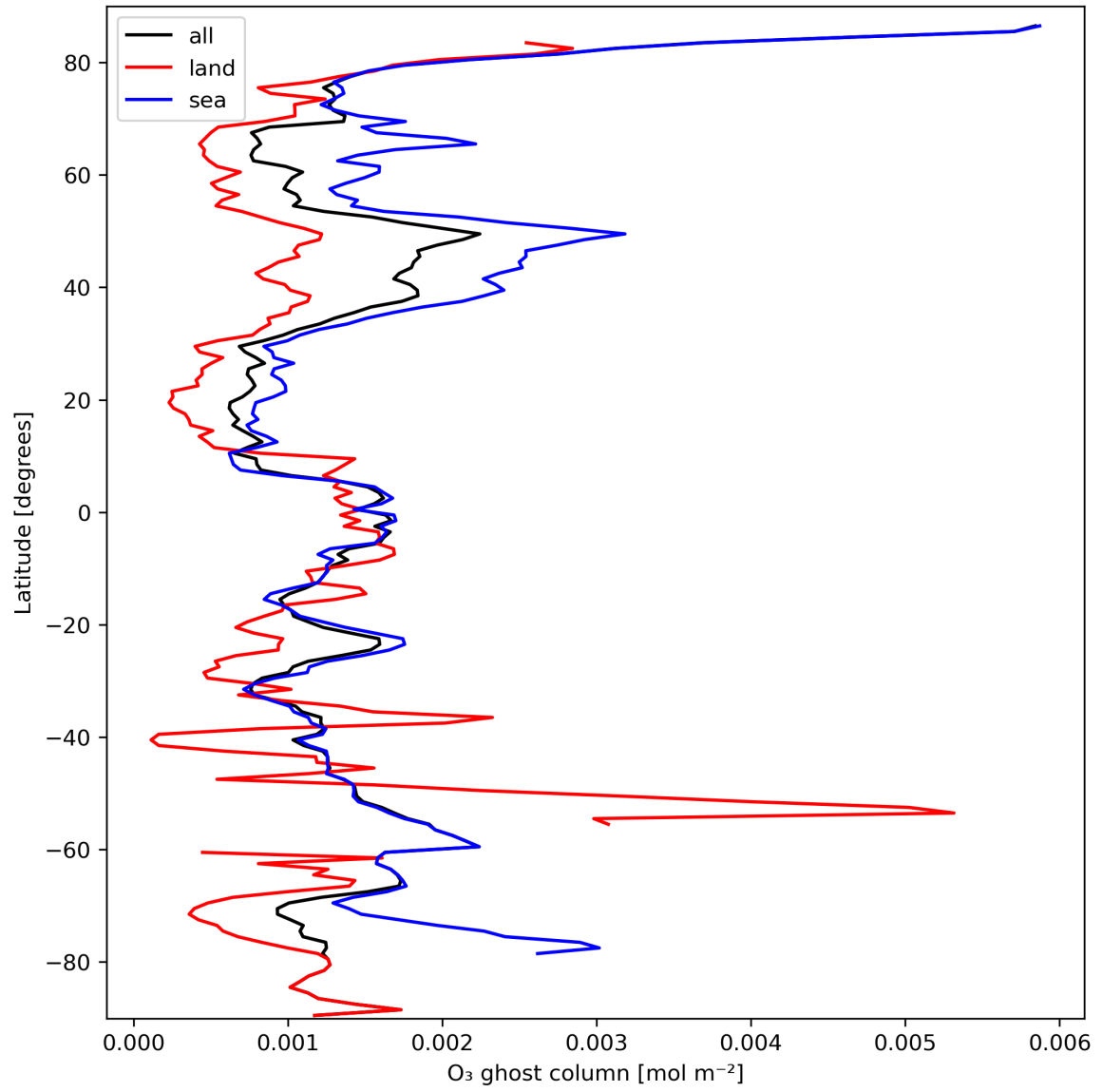
Figure 18: Zonal average of "O 3 ghost column" for 2024-03-11 to 2024-03-13.
