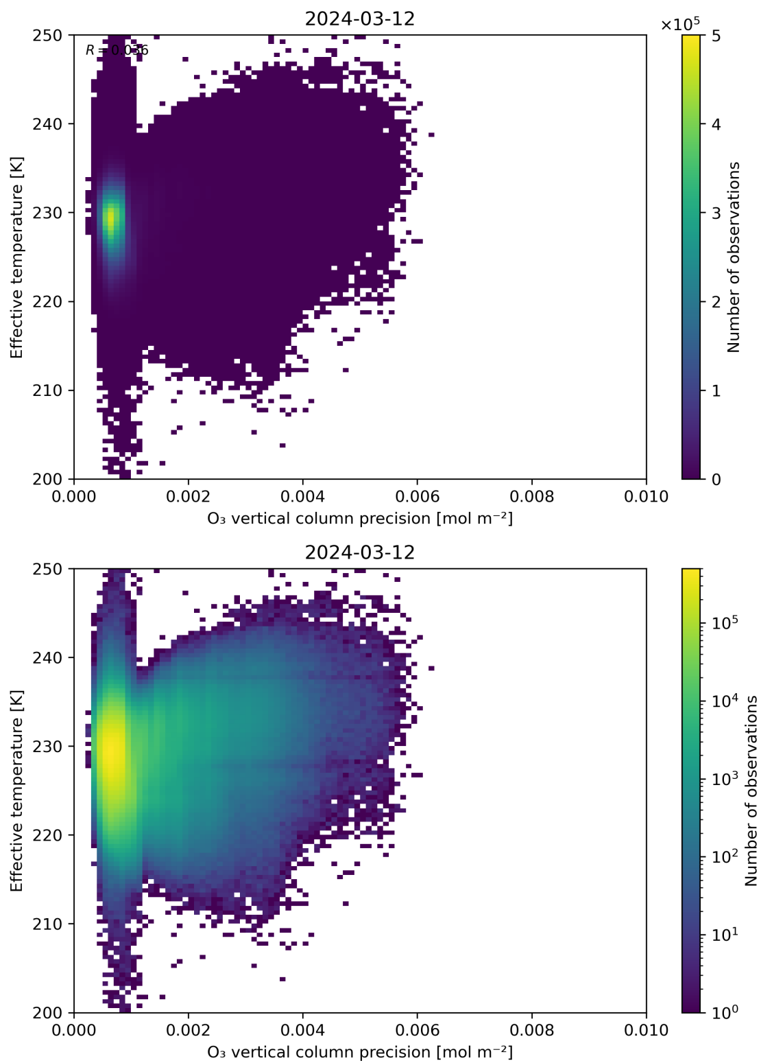
Figure 42: Scatter density plot of “O 3 vertical column precision” against “Effective temperature” for 2024-03-11 to 2024-03-13.
