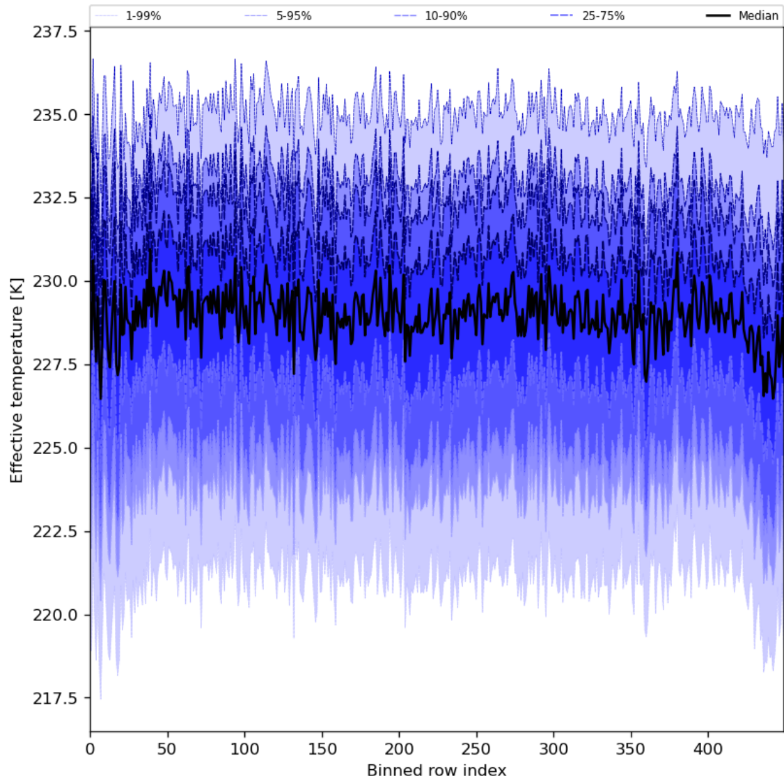
Figure 31: Along track statistics of “Effective temperature” for 2024-03-11 to 2024-03-13
