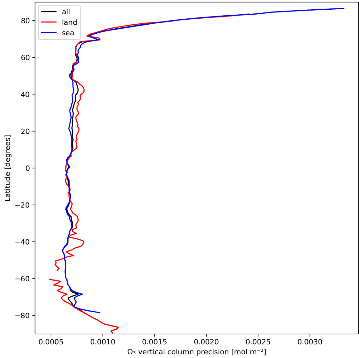
Figure 15: Zonal average of "O 3 vertical column precision" for 2024-03-11 to 2024-03-13.
