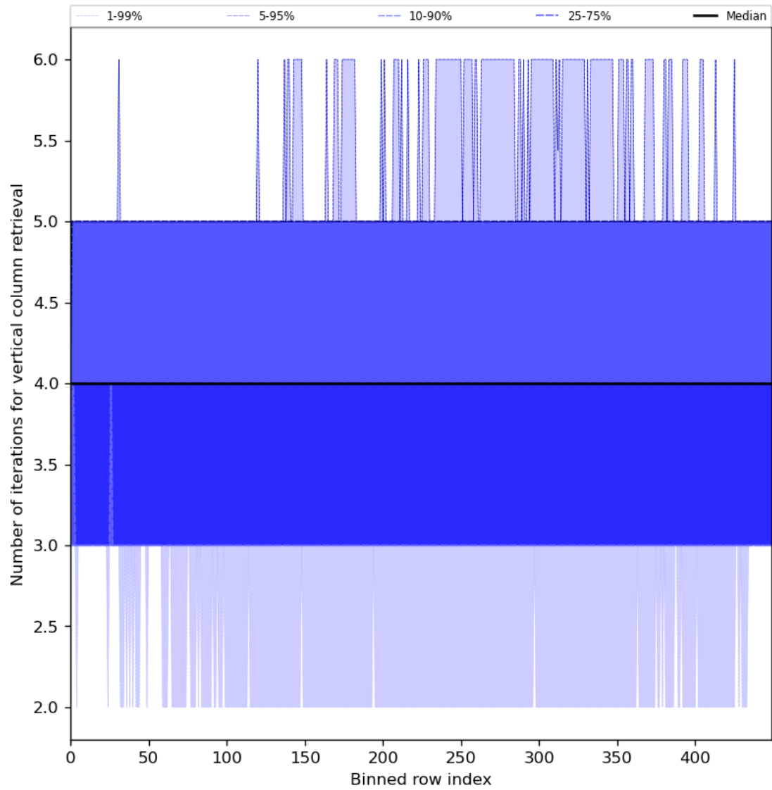
Figure 33: Along track statistics of “Number of iterations for vertical column retrieval” for 2024-03-11 to 2024-03-13
