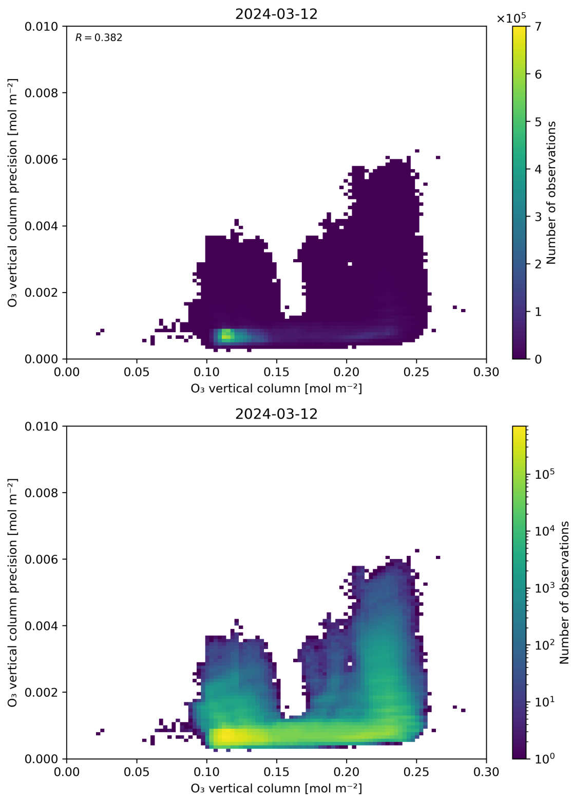
Figure 41: Scatter density plot of “O 3 vertical column” against “O 3 vertical column precision” for 2024-03-11 to 2024-03-13.
