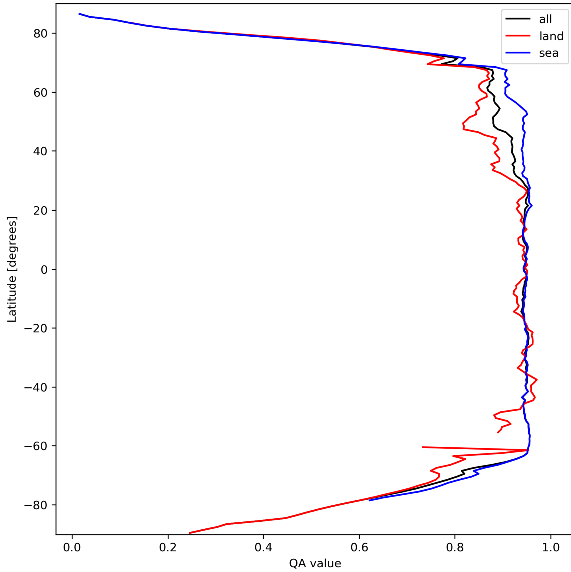
Figure 13: Zonal average of “QA value” for 2024-03-11 to 2024-03-13.
