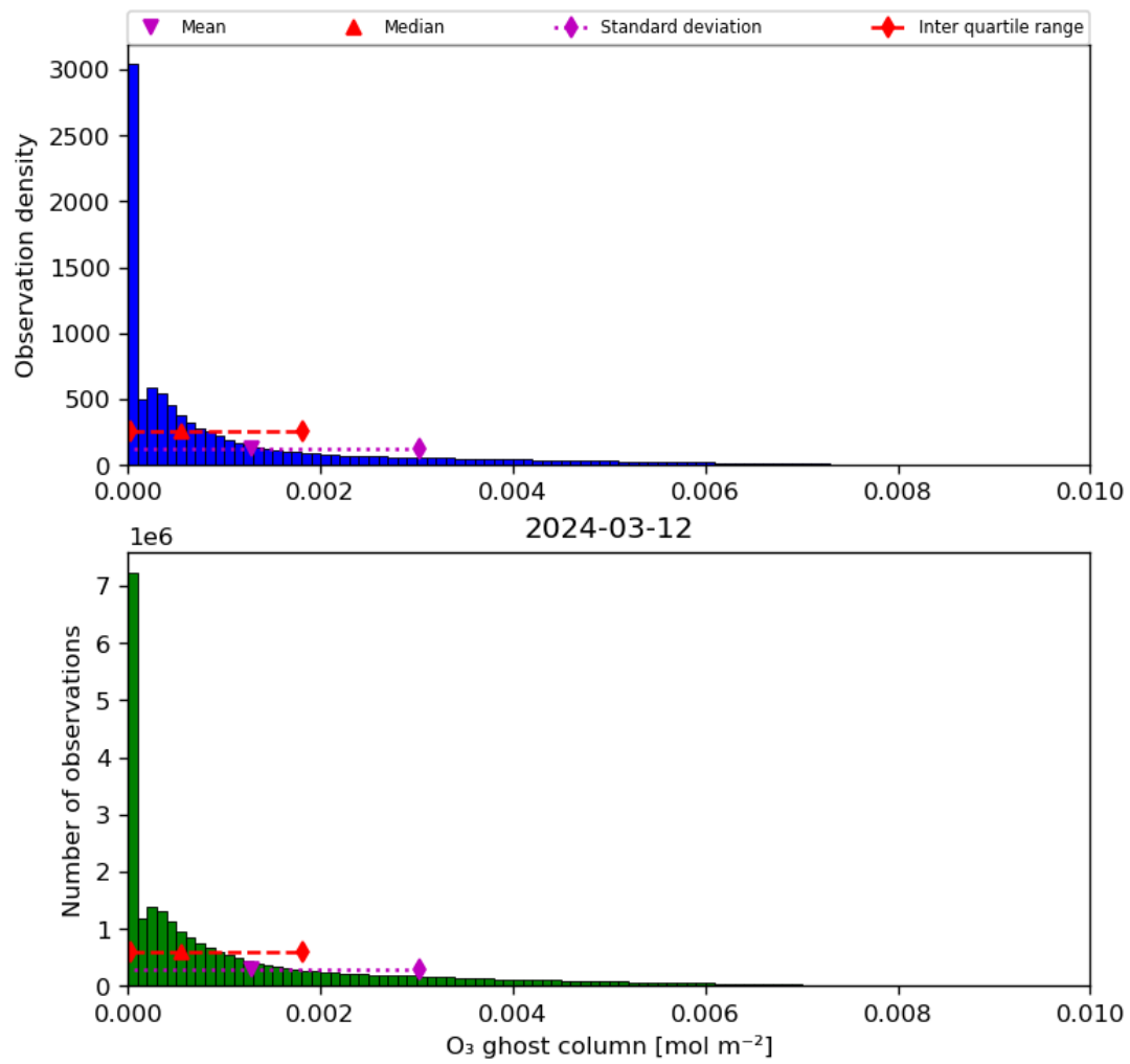
Figure 25: Histogram of “O 3 ghost column” for 2024-03-11 to 2024-03-13
