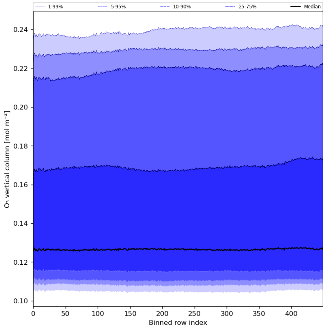
Figure 28: Along track statistics of “O 3 vertical column” for 2024-03-11 to 2024-03-13
