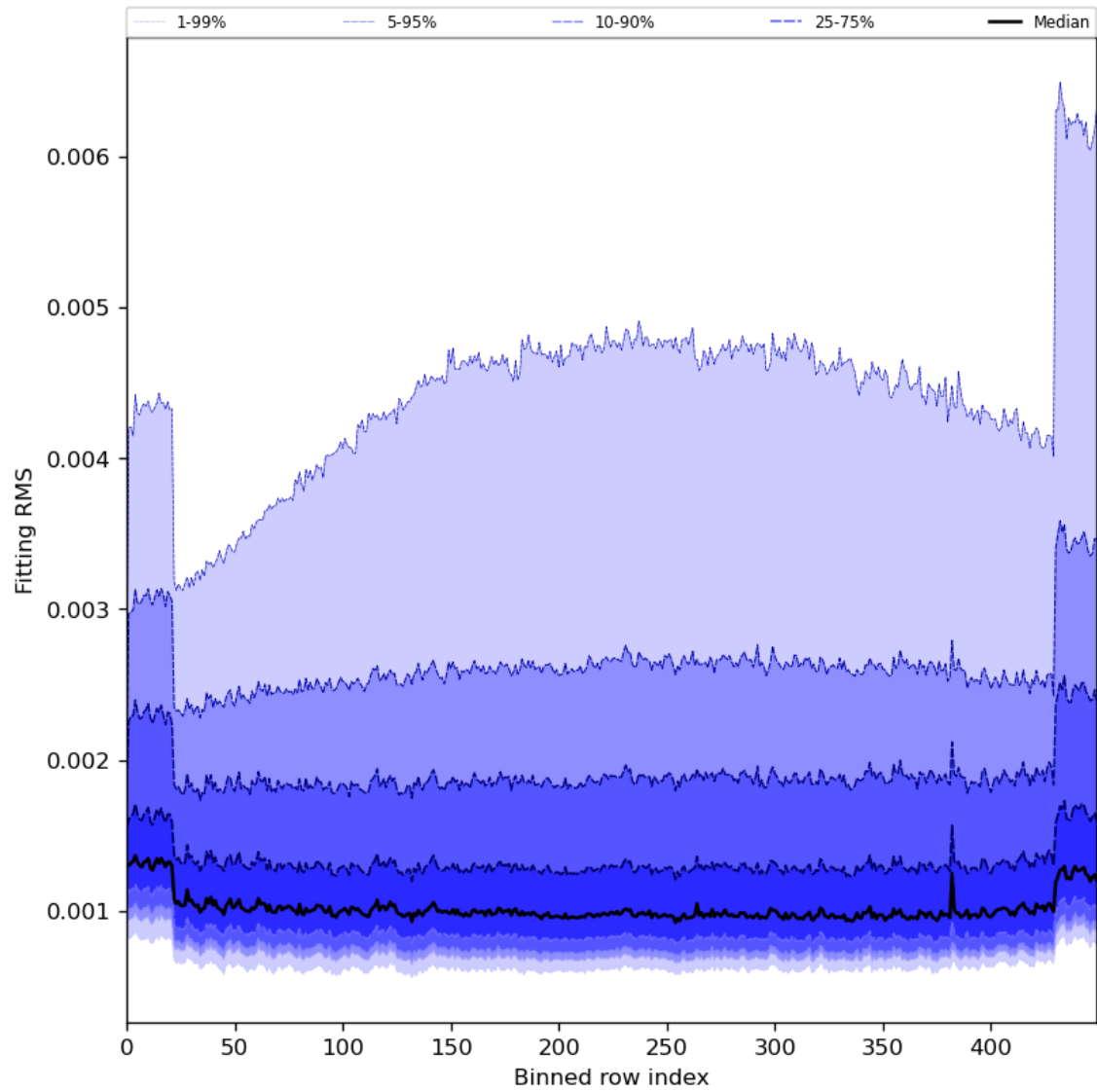
Figure 30: Along track statistics of “Fitting RMS” for 2024-03-11 to 2024-03-13
