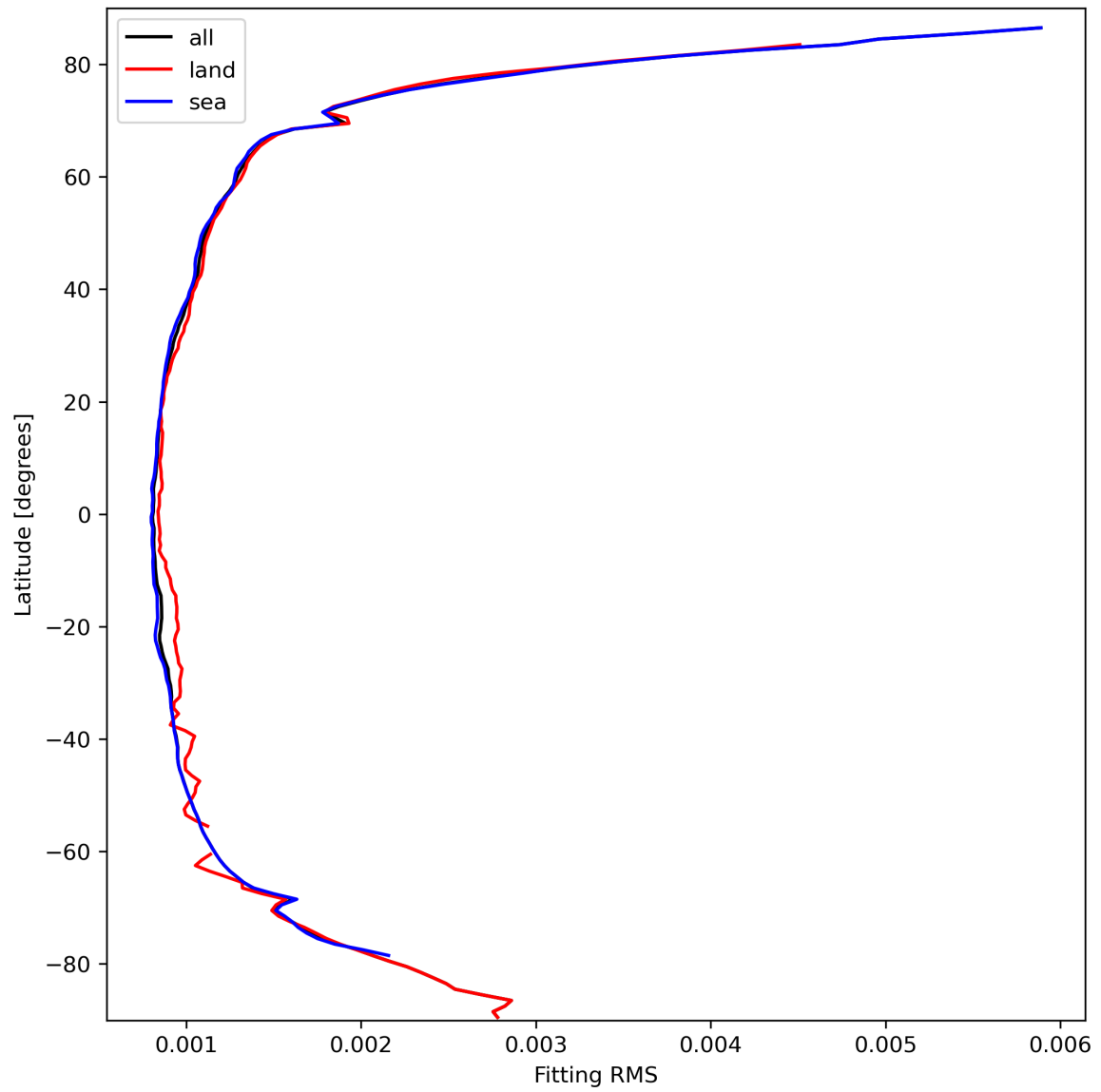
Figure 16: Zonal average of “Fitting RMS” for 2024-03-11 to 2024-03-13.
