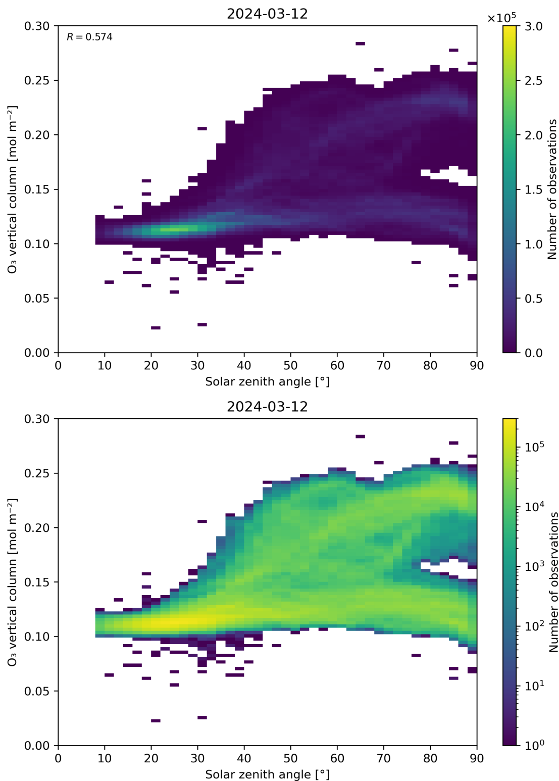
Figure 47: Scatter density plot of “Solar zenith angle” against “O 3 vertical column” for 2024-03-11 to 2024-03-13.
