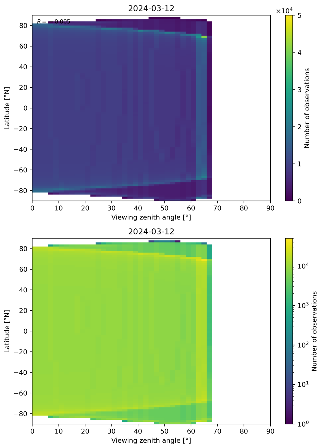
Figure 49: Scatter density plot of “Viewing zenith angle” against “Latitude” for 2024-03-11 to 2024-03-13.
