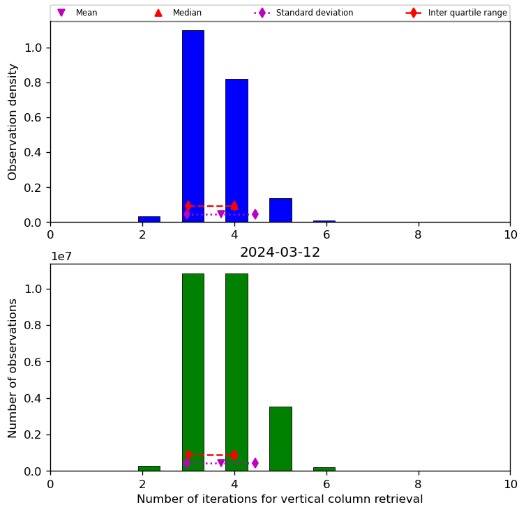
Figure 26: Histogram of “Number of iterations for vertical column retrieval” for 2024-03-11 to 2024-03-13
