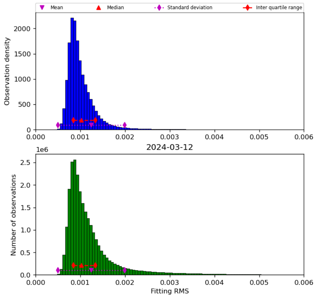
Figure 23: Histogram of “Fitting RMS” for 2024-03-11 to 2024-03-13
