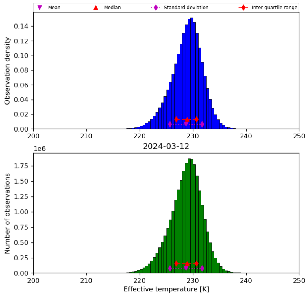
Figure 24: Histogram of “Effective temperature” for 2024-03-11 to 2024-03-13
