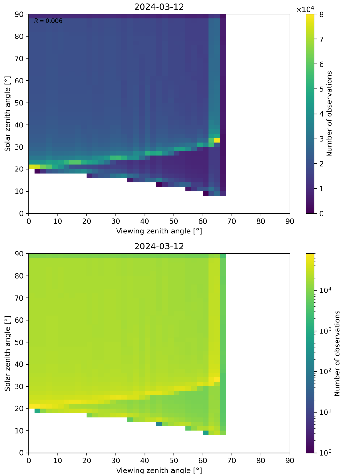
Figure 54: Scatter density plot of “Viewing zenith angle” against “Solar zenith angle” for 2024-03-11 to 2024-03-13.
