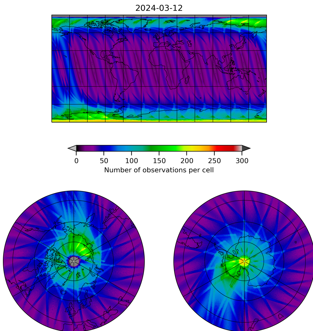
Figure 12: Map of the number of observations for 2024-03-11 to 2024-03-13
