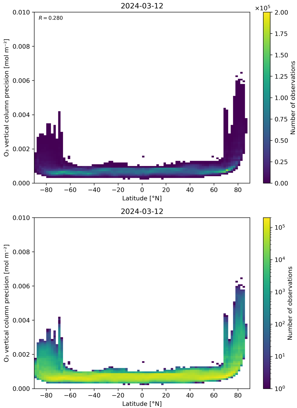
Figure 37: Scatter density plot of “Latitude” against “O 3 vertical column precision” for 2024-03-11 to 2024-03-13.
