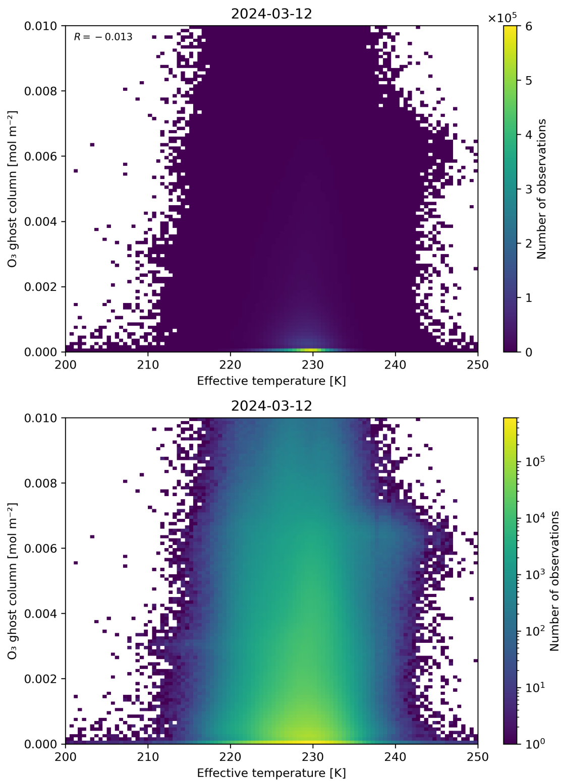
Figure 38: Scatter density plot of “Effective temperature” against “O 3 ghost column” for 2024-03-11 to 2024-03-13.
