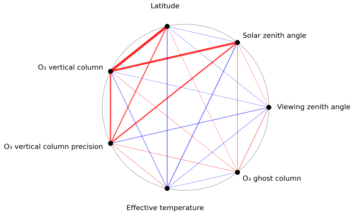
Figure 1: Map of correlation graph for 2024-03-11 to 2024-03-13.
