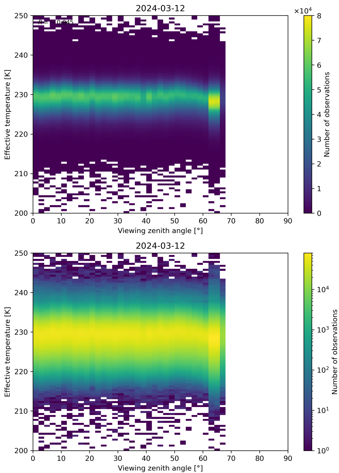
Figure 50: Scatter density plot of “Viewing zenith angle” against “Effective temperature” for 2024-03-11 to 2024-03-13.
