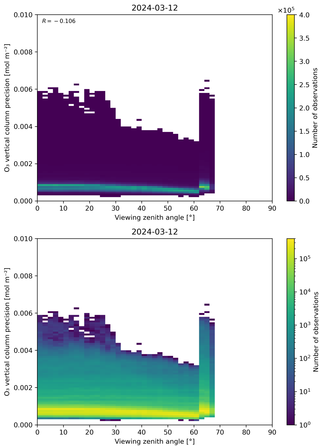
Figure 53: Scatter density plot of “Viewing zenith angle” against “O 3 vertical column precision” for 2024-03-11 to 2024-03-13.
