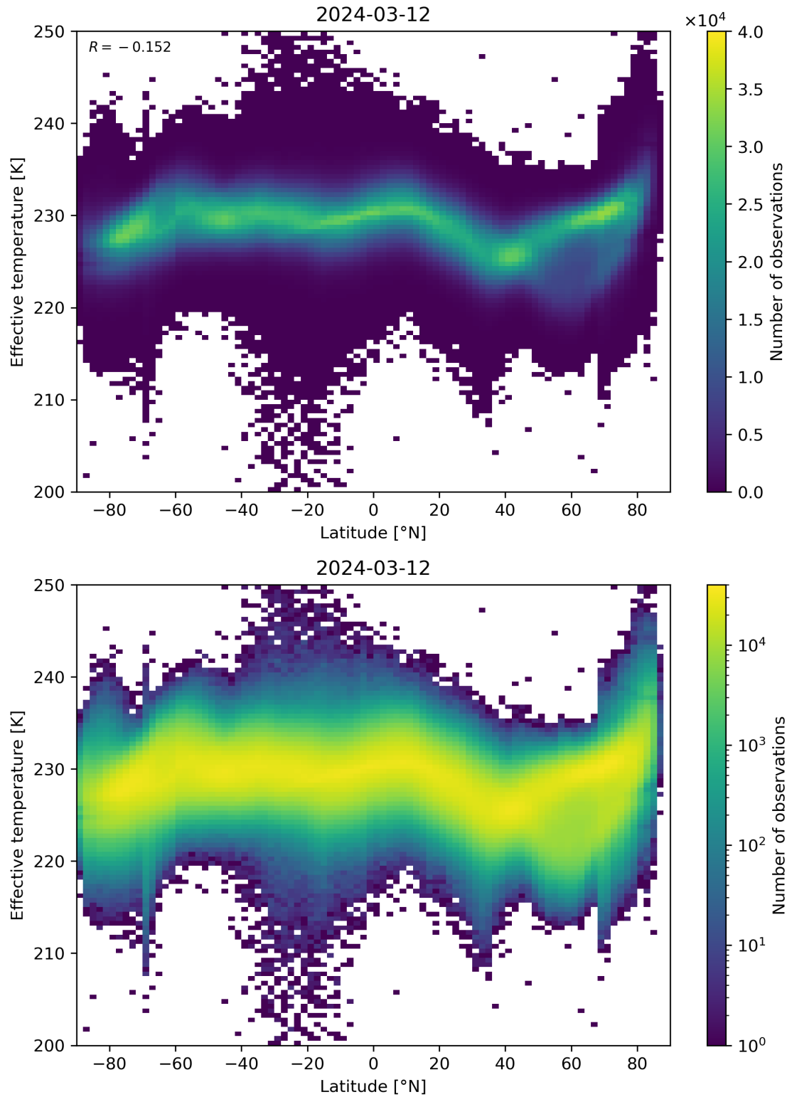
Figure 34: Scatter density plot of “Latitude” against “Effective temperature” for 2024-03-11 to 2024-03-13.
