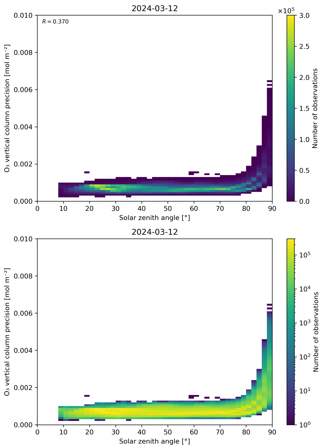
Figure 48: Scatter density plot of “Solar zenith angle” against “O 3 vertical column precision” for 2024-03-11 to 2024-03-13.
