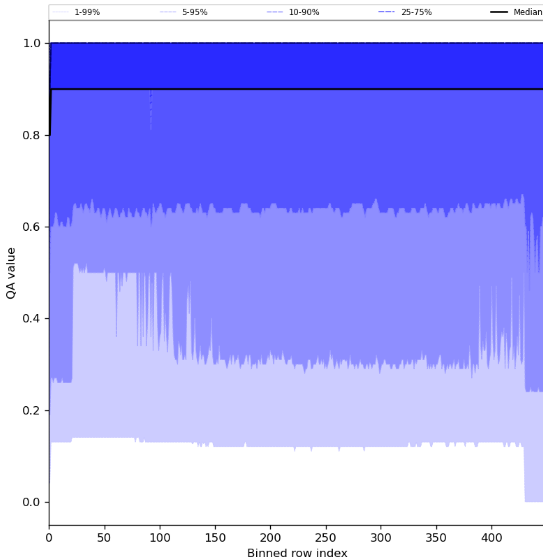
Figure 27: Along track statistics of “QA value” for 2024-03-11 to 2024-03-13
