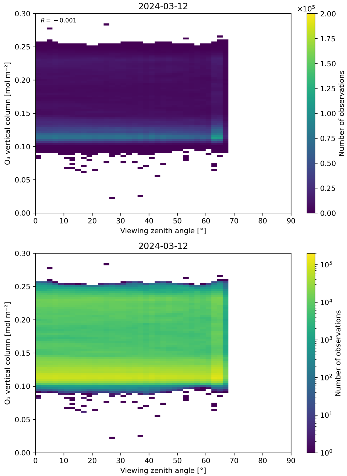
Figure 52: Scatter density plot of “Viewing zenith angle” against “O 3 vertical column” for 2024-03-11 to 2024-03-13.
