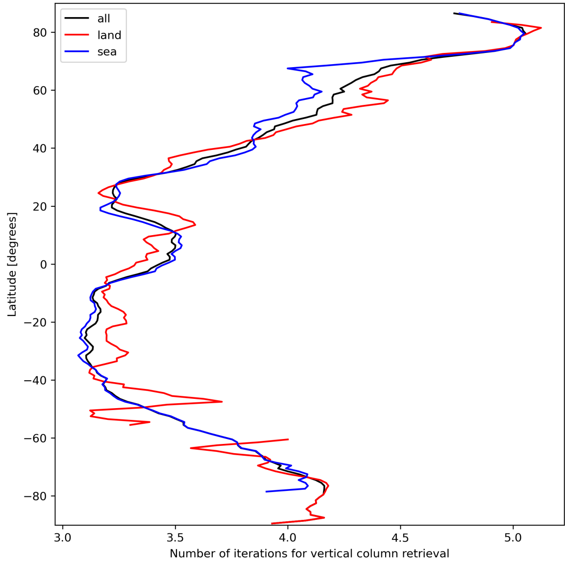
Figure 19: Zonal average of “Number of iterations for vertical column retrieval” for 2024-03-11 to 2024-03-13.
