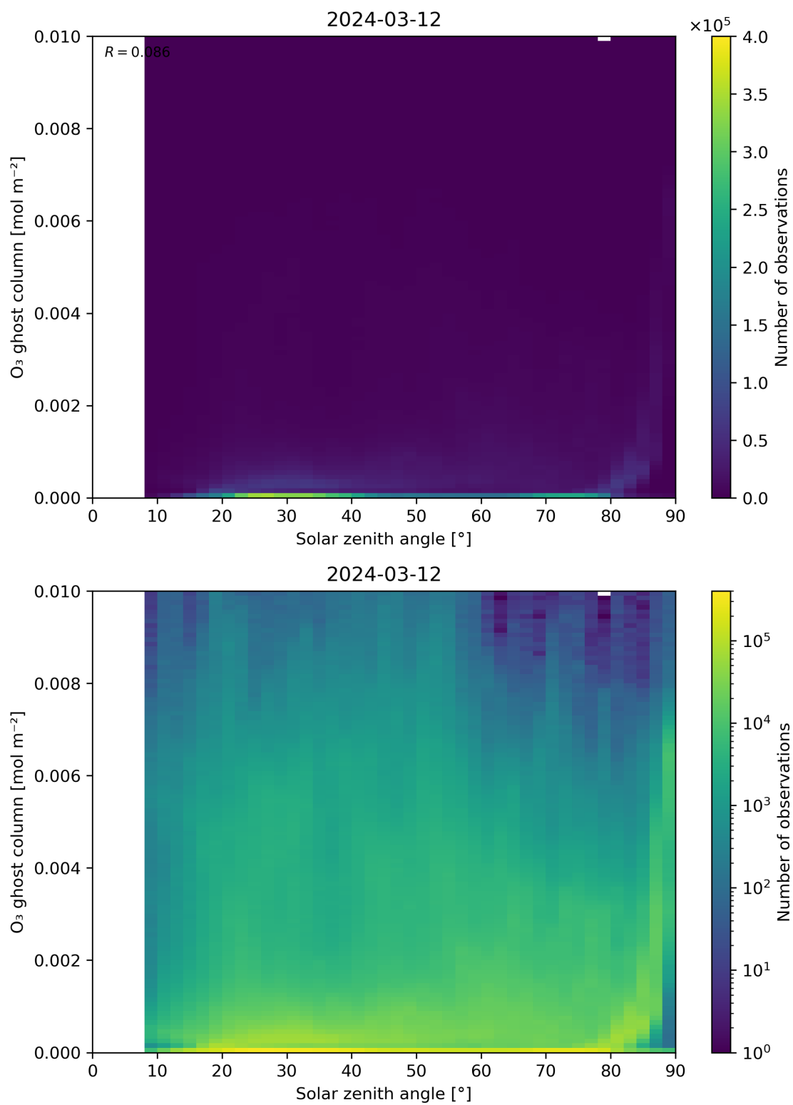
Figure 46: Scatter density plot of “Solar zenith angle” against “O 3 ghost column” for 2024-03-11 to 2024-03-13.
