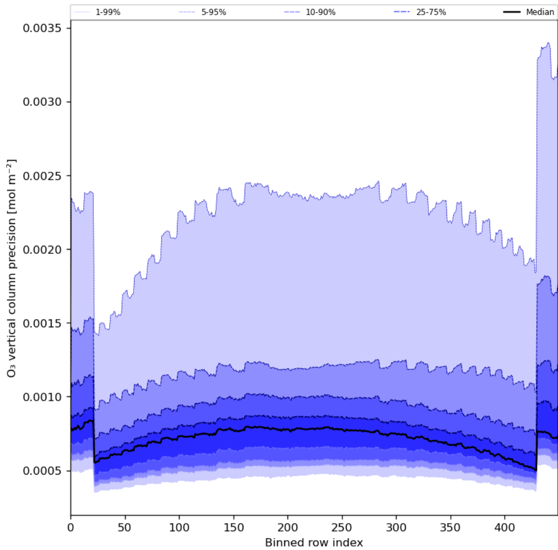
Figure 29: Along track statistics of “O 3 vertical column precision” for 2024-03-11 to 2024-03-13
