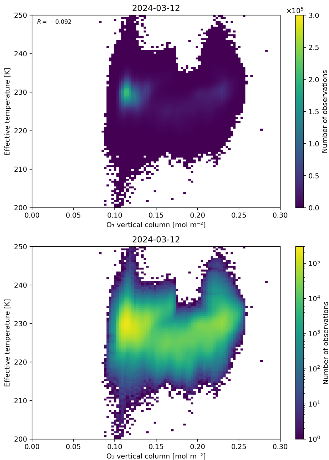
Figure 39: Scatter density plot of “O 3 vertical column” against “Effective temperature” for 2024-03-11 to 2024-03-13.
