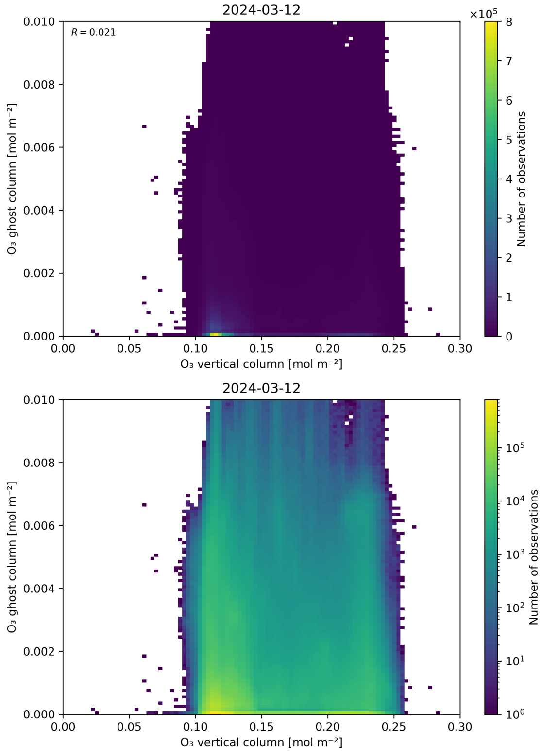
Figure 40: Scatter density plot of “O 3 vertical column” against “O 3 ghost column” for 2024-03-11 to 2024-03-13.
