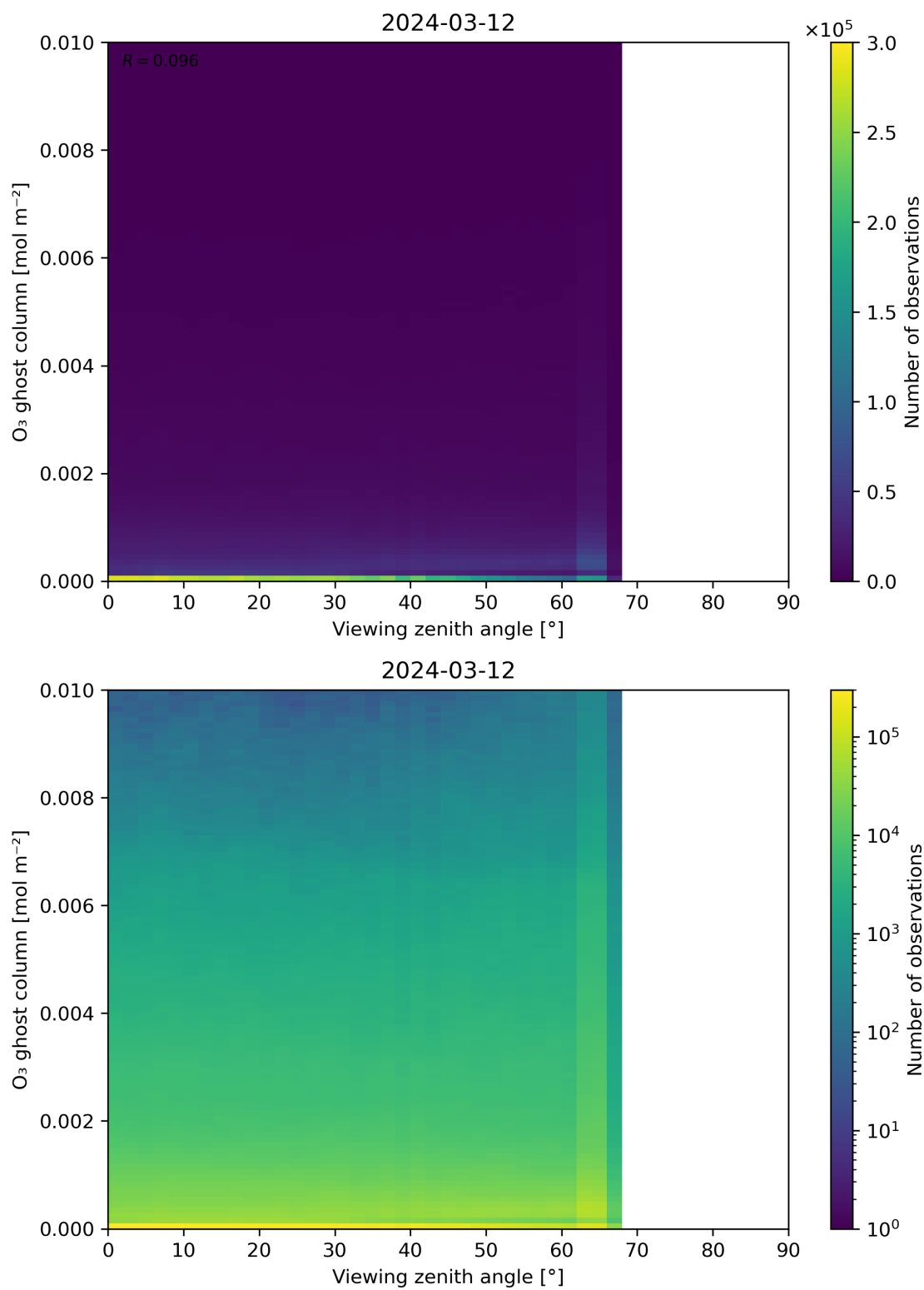
Figure 51: Scatter density plot of “Viewing zenith angle” against “O 3 ghost column” for 2024-03-11 to 2024-03-13.
