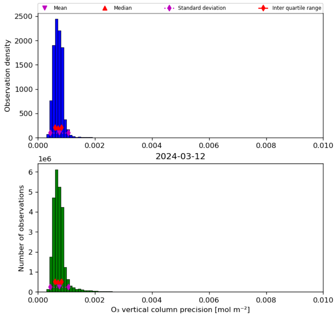
Figure 22: Histogram of “O 3 vertical column precision” for 2024-03-11 to 2024-03-13
