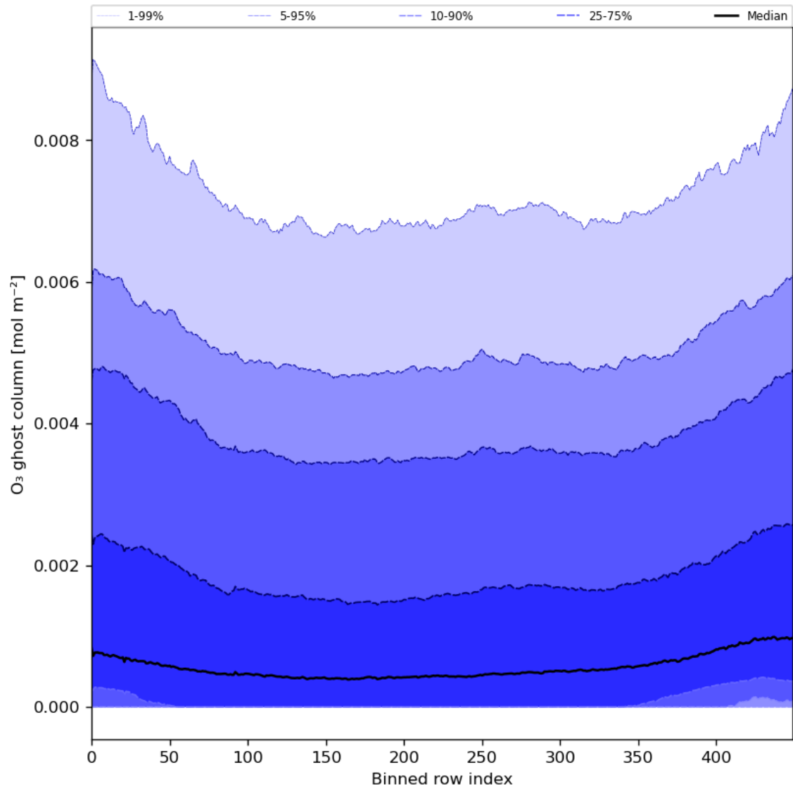
Figure 32: Along track statistics of "O 3 ghost column" for 2024-03-11 to 2024-03-13
