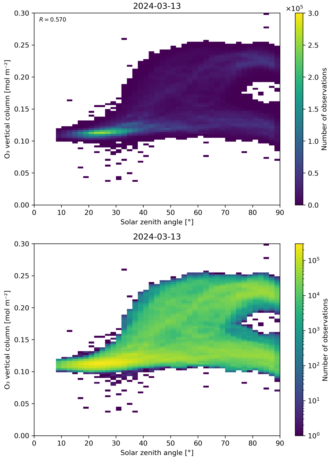
Figure 47: Scatter density plot of “Solar zenith angle” against “O 3 vertical column” for 2024-03-12 to 2024-03-14.
