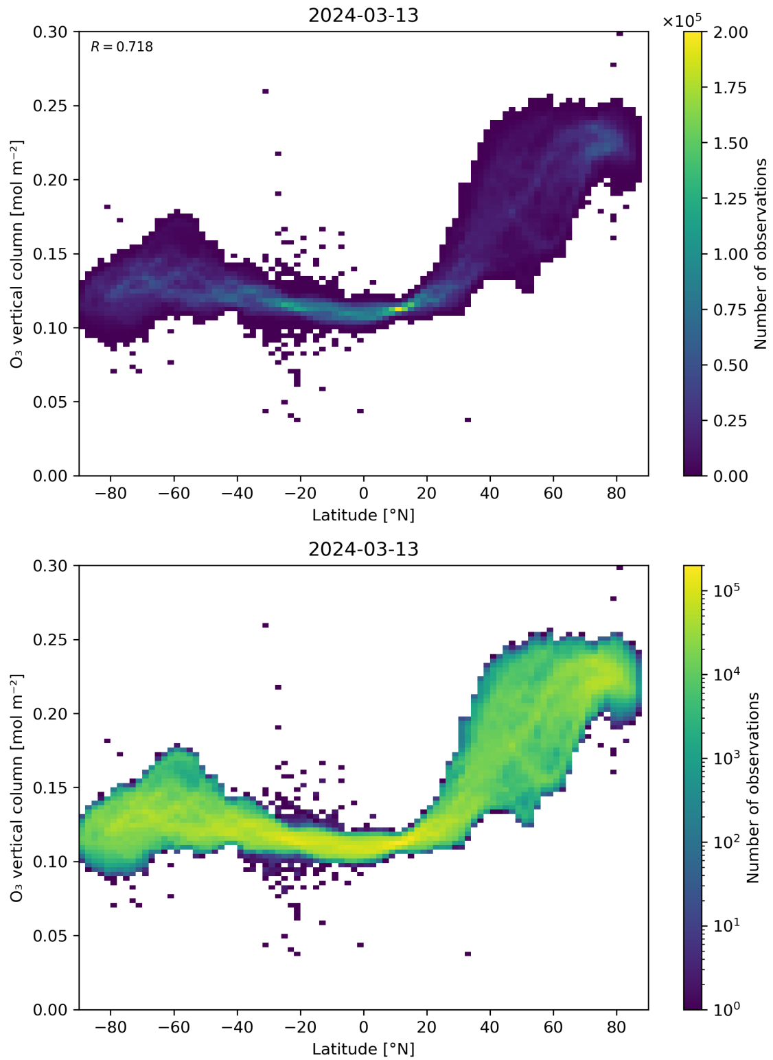
Figure 36: Scatter density plot of “Latitude” against “O 3 vertical column” for 2024-03-12 to 2024-03-14.
