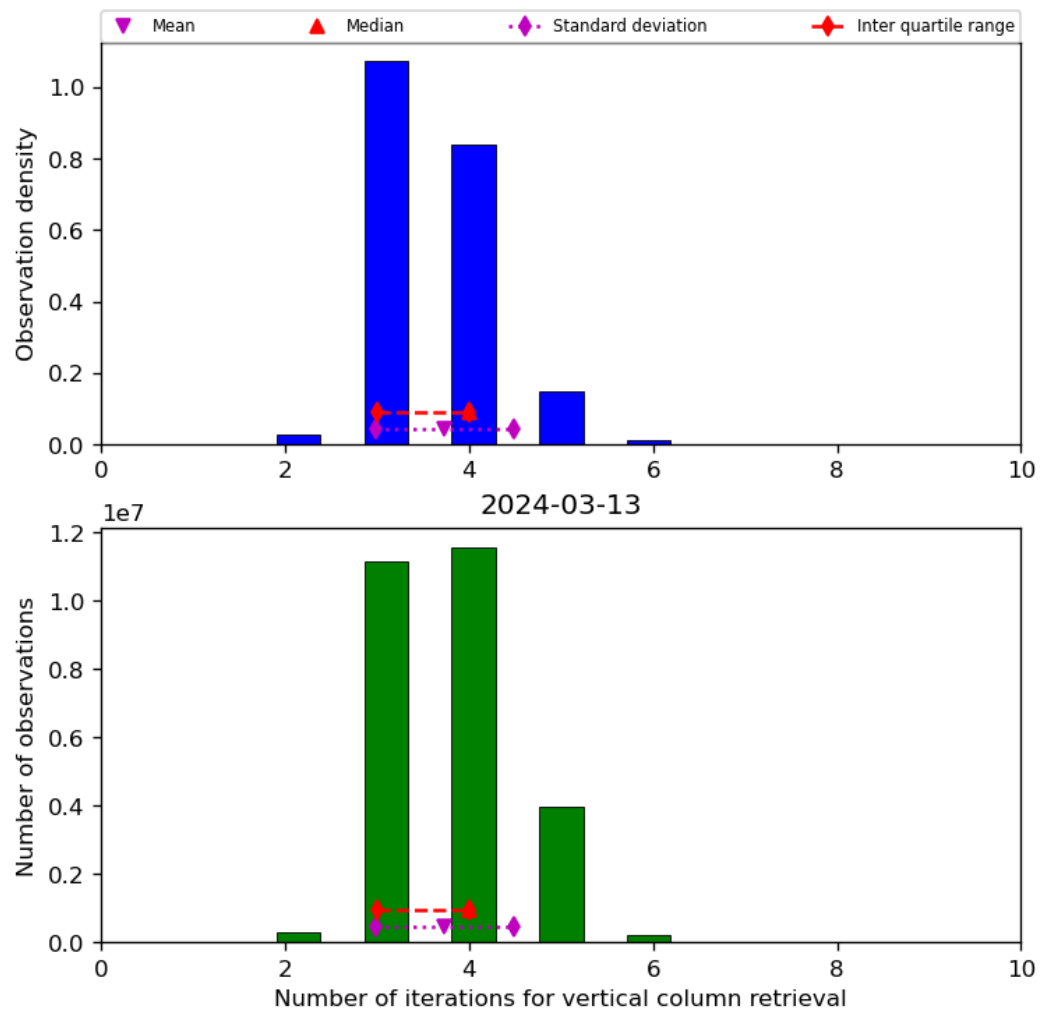
Figure 26: Histogram of “Number of iterations for vertical column retrieval” for 2024-03-12 to 2024-03-14
