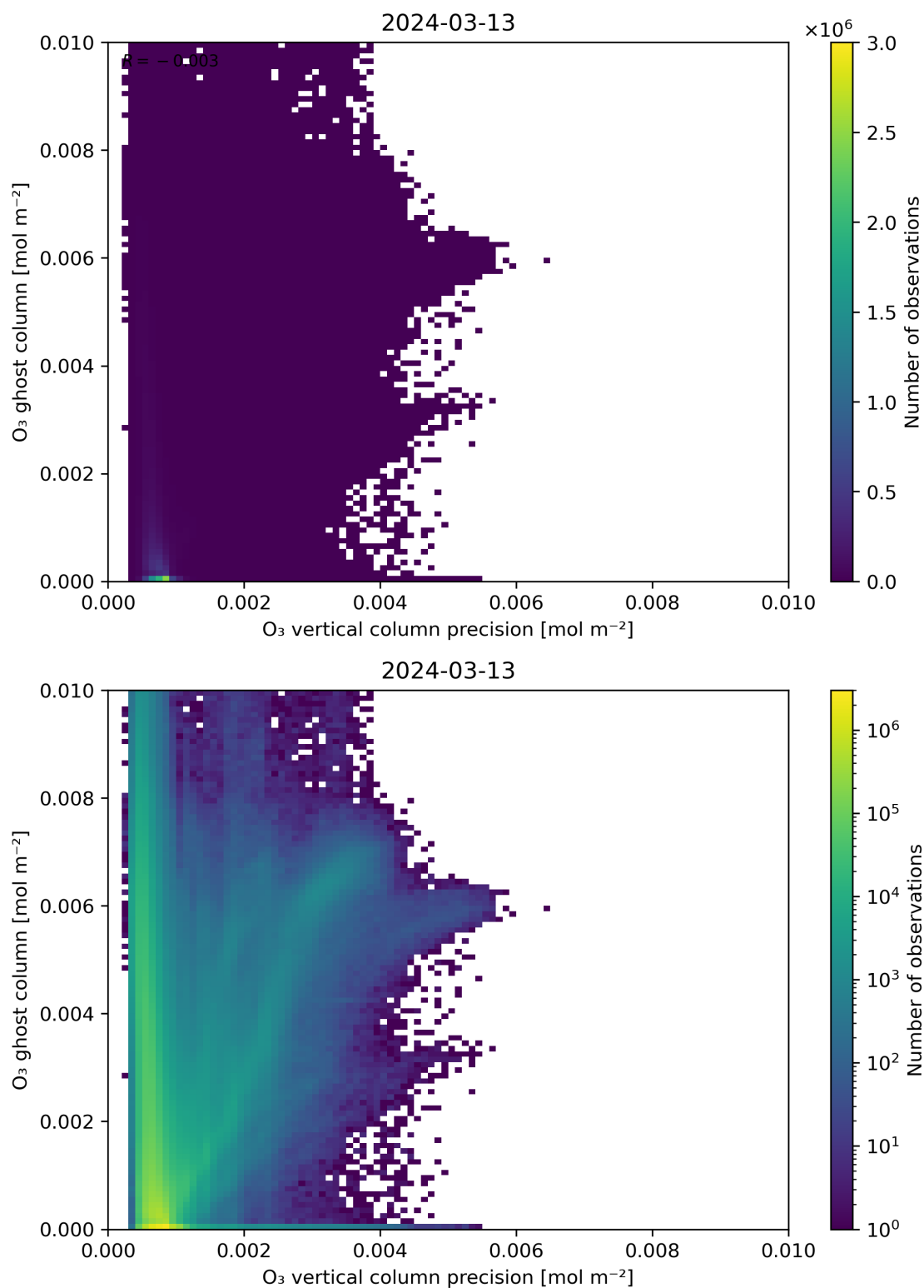
Figure 43: Scatter density plot of “ \text{O}_3 vertical column precision” against “ \text{O}_3 ghost column” for 2024-03-12 to 2024-03-14.
