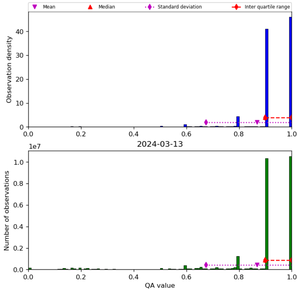
Figure 20: Histogram of “QA value” for 2024-03-12 to 2024-03-14
