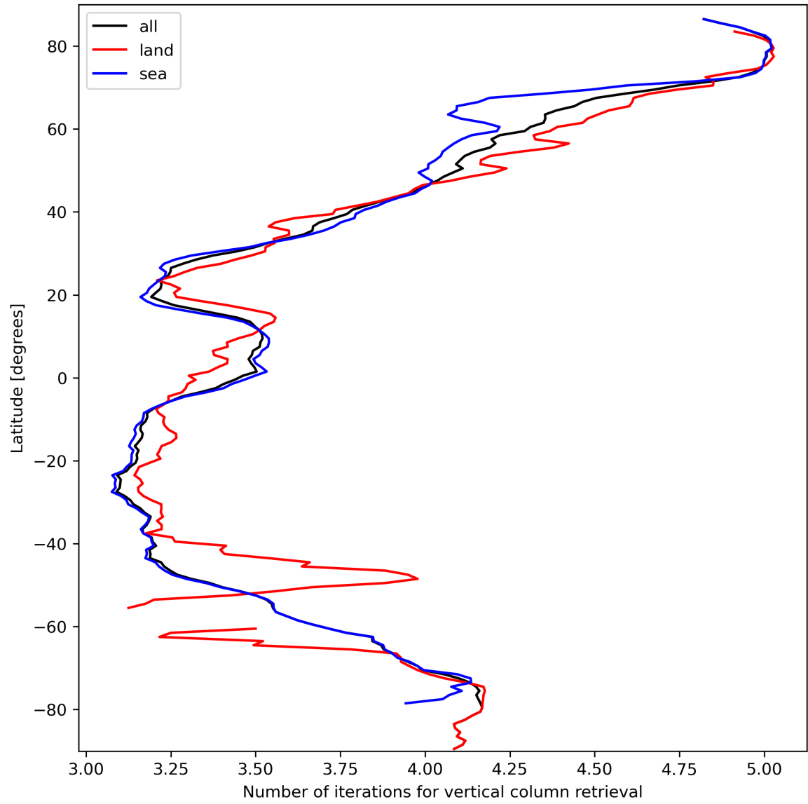
Figure 19: Zonal average of “Number of iterations for vertical column retrieval” for 2024-03-12 to 2024-03-14.
