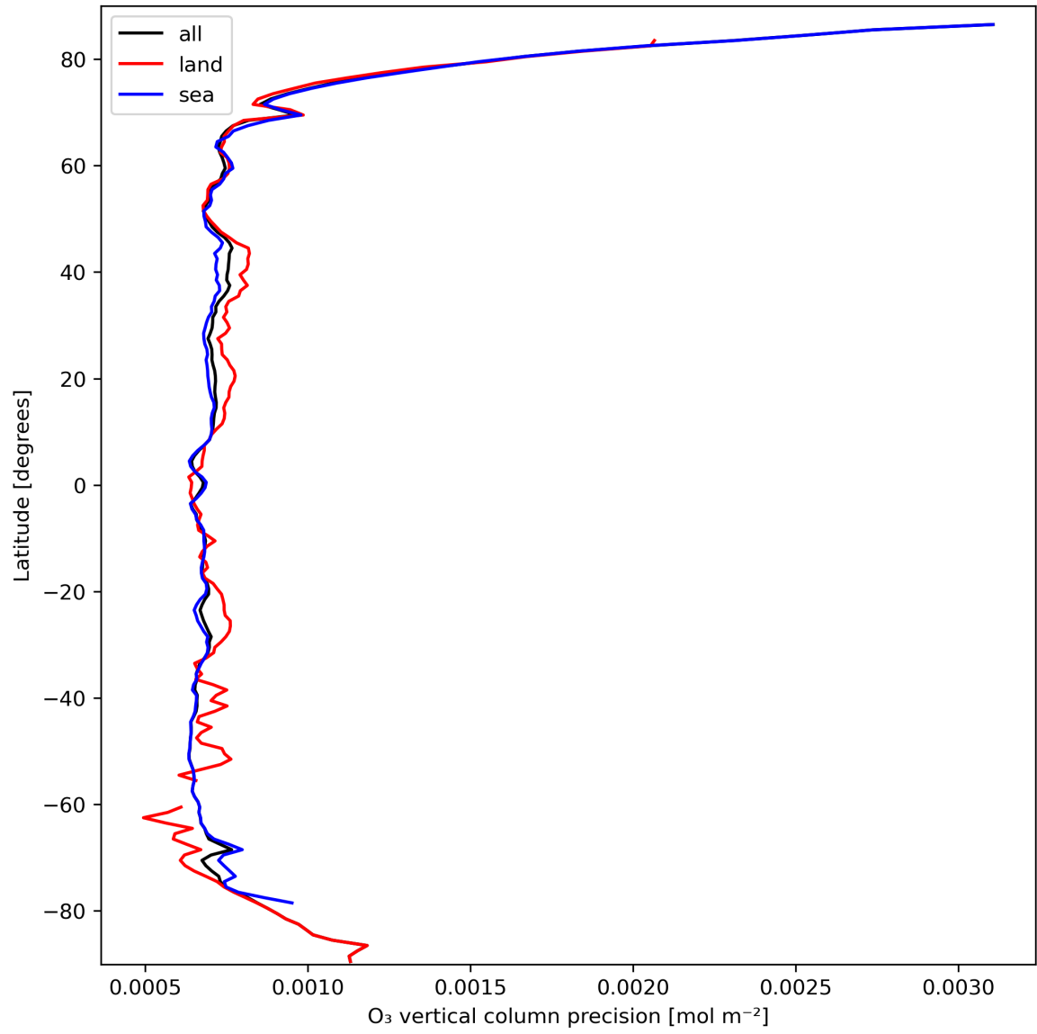
Figure 15: Zonal average of "O 3 vertical column precision" for 2024-03-12 to 2024-03-14.
