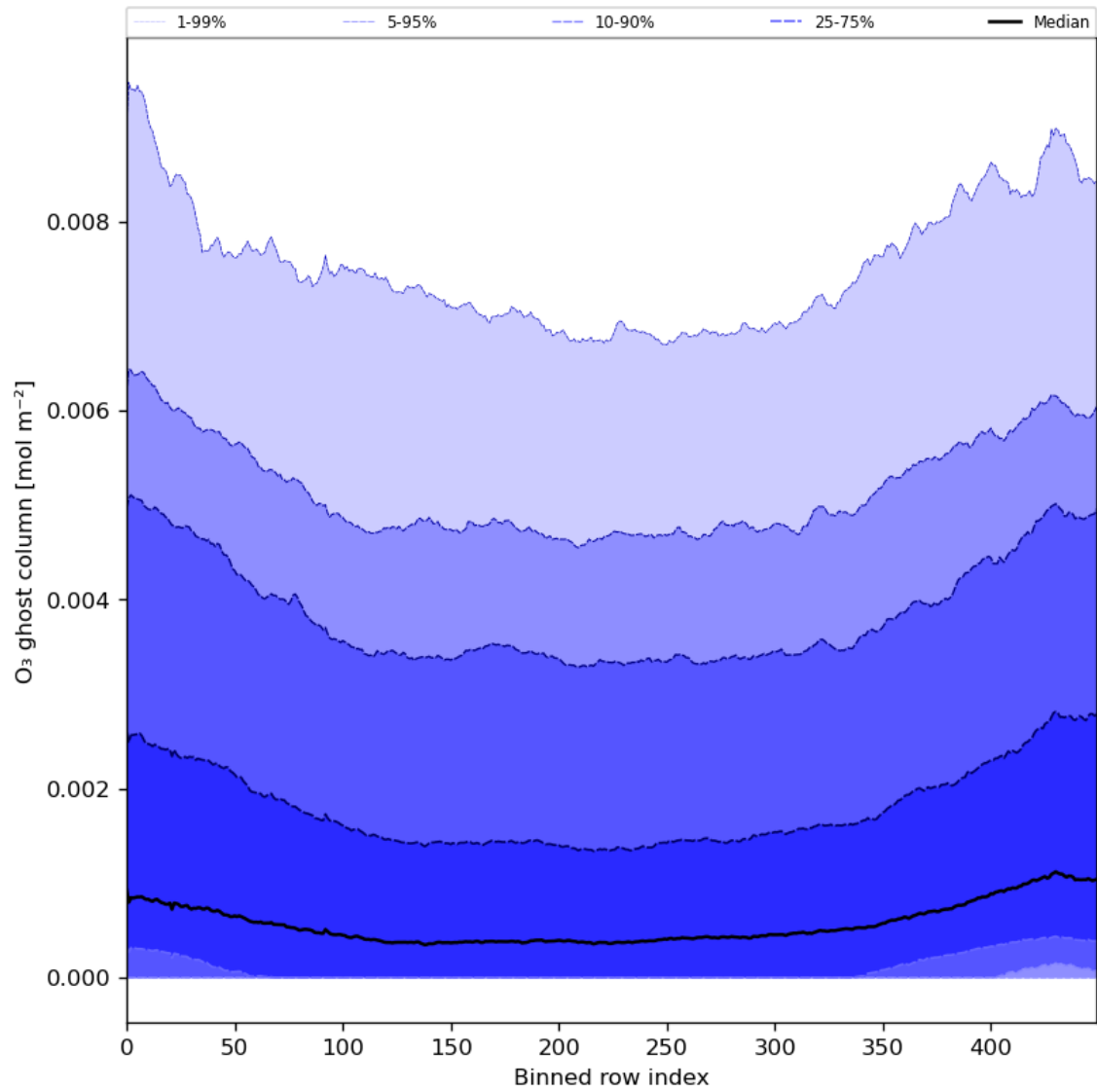
Figure 32: Along track statistics of “O 3 ghost column” for 2024-03-12 to 2024-03-14
