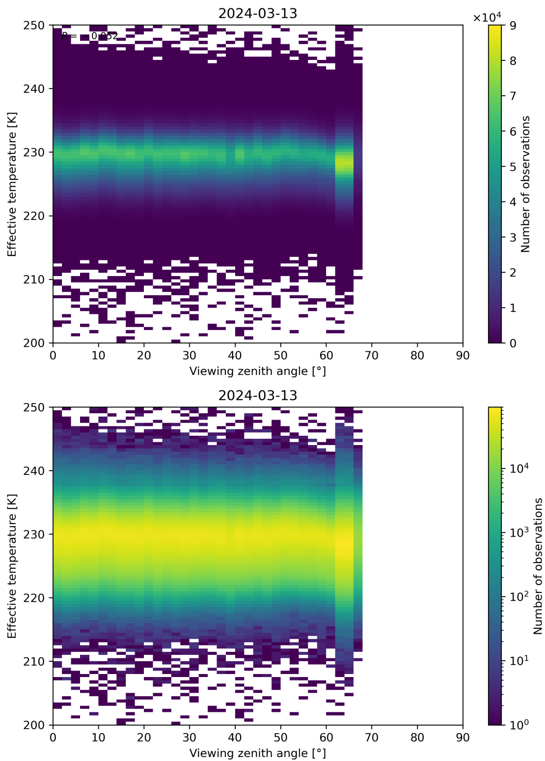
Figure 50: Scatter density plot of “Viewing zenith angle” against “Effective temperature” for 2024-03-12 to 2024-03-14.
