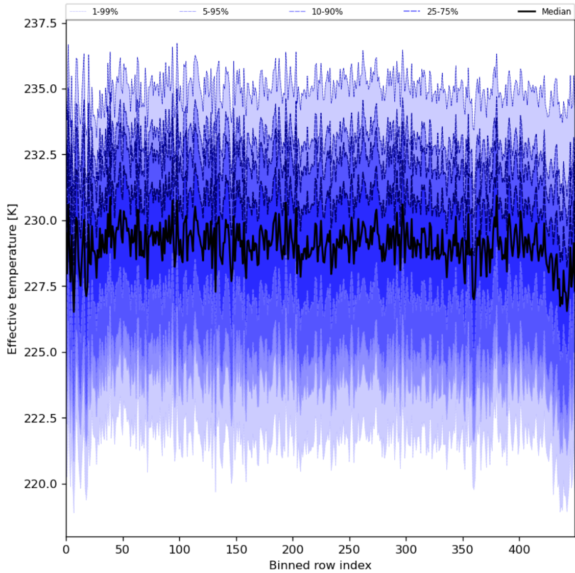
Figure 31: Along track statistics of “Effective temperature” for 2024-03-12 to 2024-03-14
