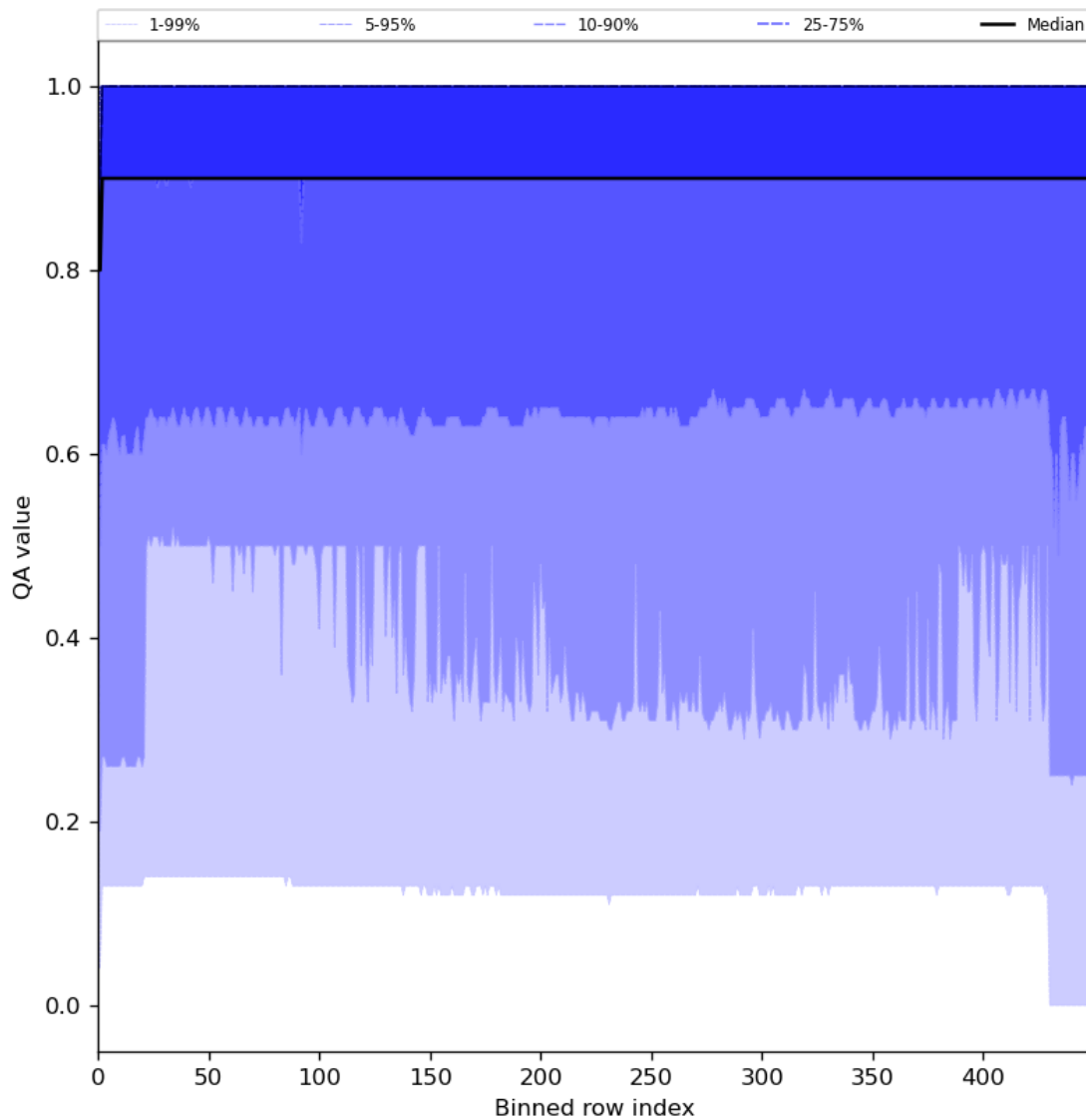
Figure 27: Along track statistics of “QA value” for 2024-03-12 to 2024-03-14
