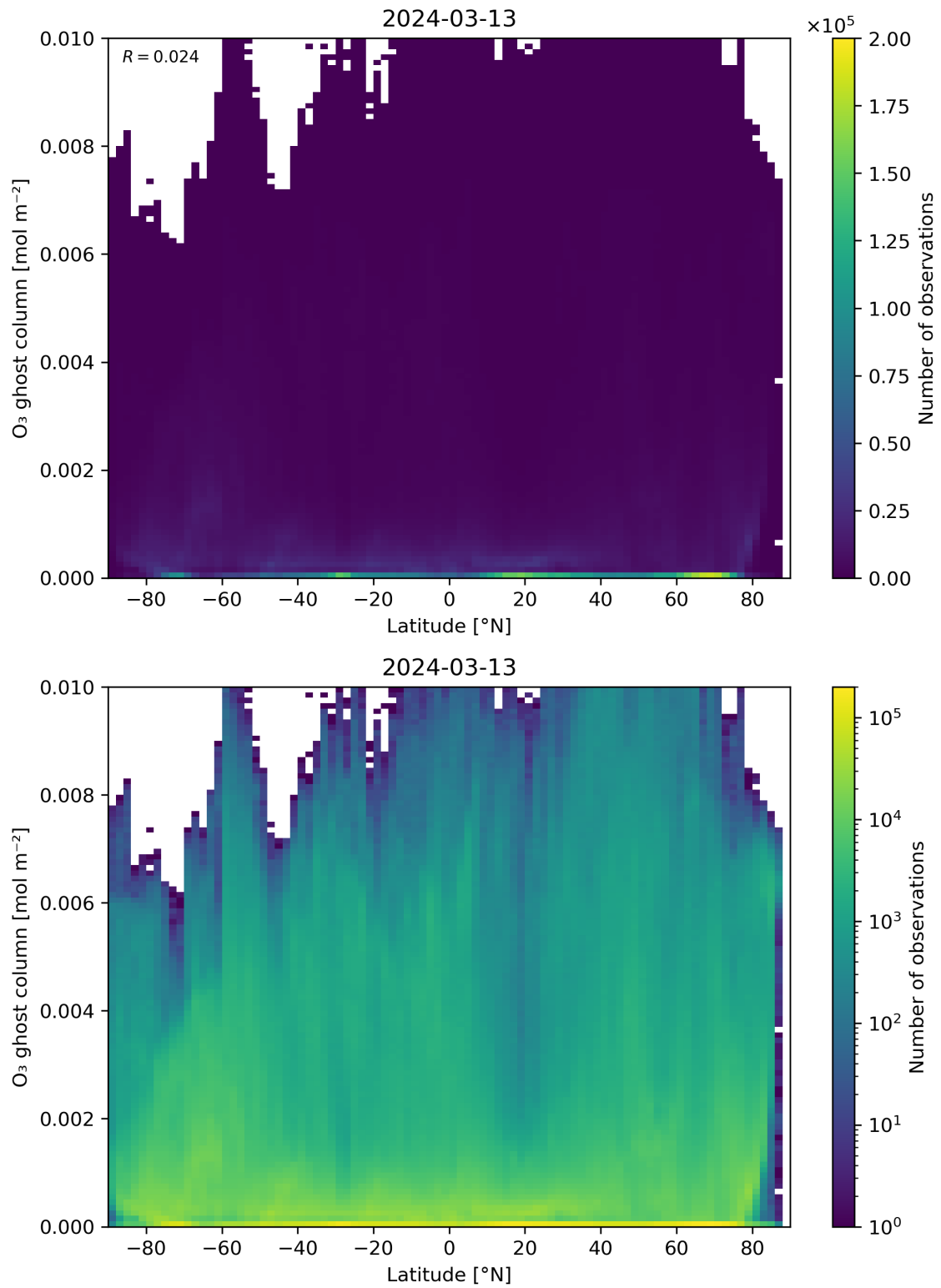
Figure 35: Scatter density plot of “Latitude” against “O 3 ghost column” for 2024-03-12 to 2024-03-14.
