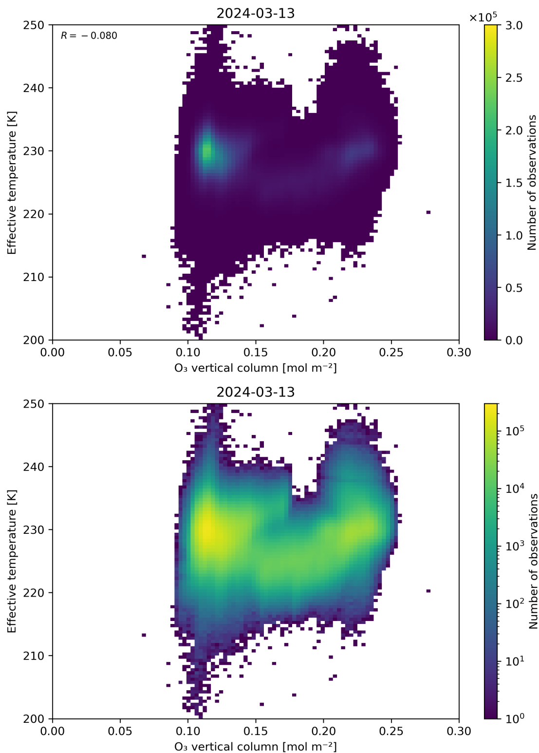
Figure 39: Scatter density plot of “O 3 vertical column” against “Effective temperature” for 2024-03-12 to 2024-03-14.
