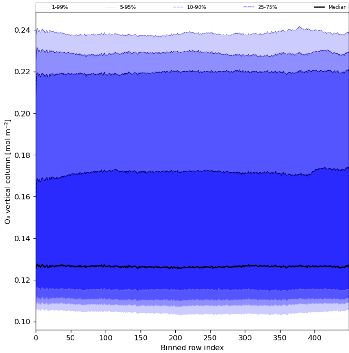
Figure 28: Along track statistics of “O 3 vertical column” for 2024-03-12 to 2024-03-14
