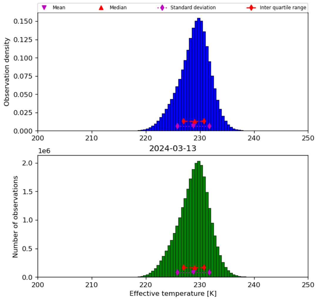
Figure 24: Histogram of “Effective temperature” for 2024-03-12 to 2024-03-14
