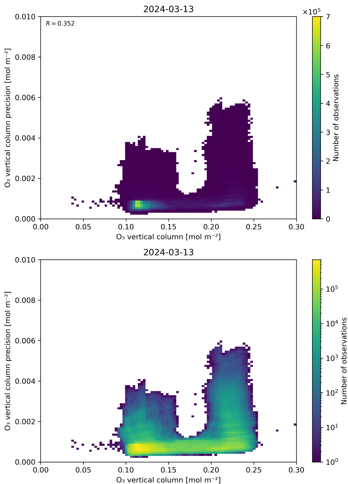
Figure 41: Scatter density plot of “O 3 vertical column” against “O 3 vertical column precision” for 2024-03-12 to 2024-03-14.
