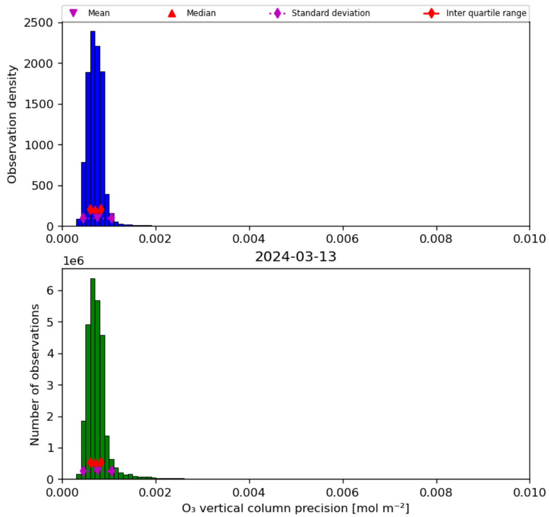
Figure 22: Histogram of “O 3 vertical column precision” for 2024-03-12 to 2024-03-14
