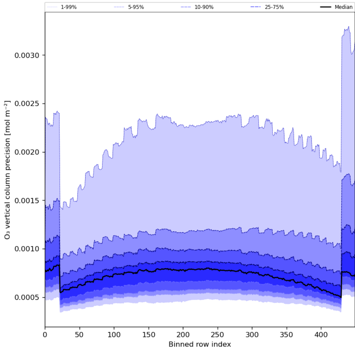
Figure 29: Along track statistics of “O 3 vertical column precision” for 2024-03-12 to 2024-03-14
