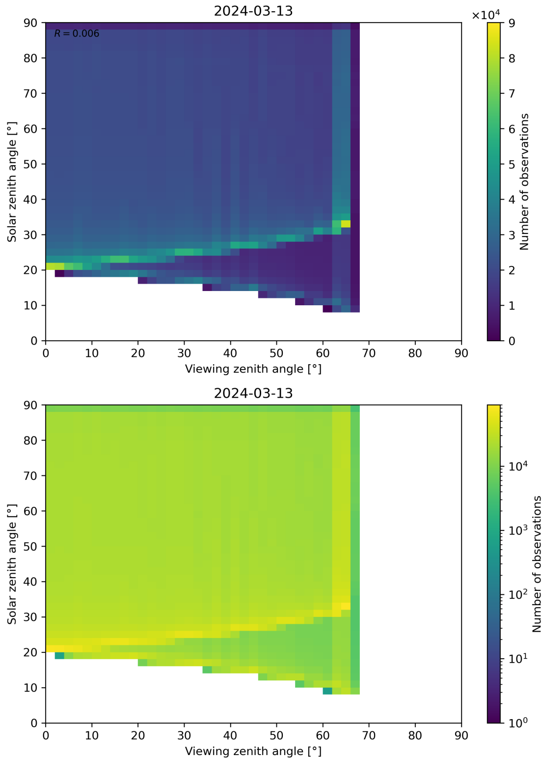
Figure 54: Scatter density plot of “Viewing zenith angle” against “Solar zenith angle” for 2024-03-12 to 2024-03-14.
