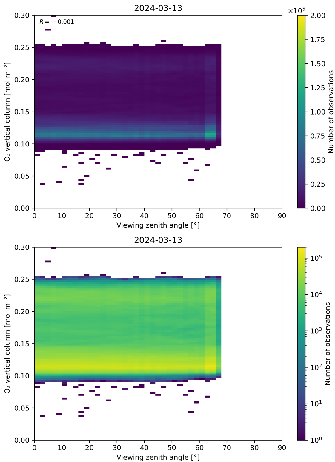
Figure 52: Scatter density plot of “Viewing zenith angle” against “O 3 vertical column” for 2024-03-12 to 2024-03-14.
