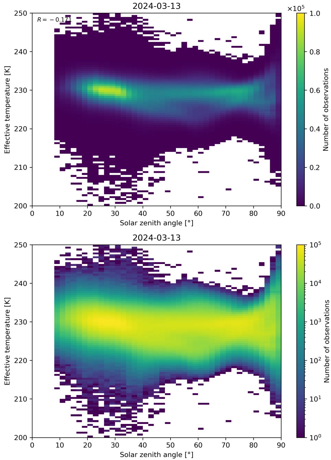
Figure 45: Scatter density plot of “Solar zenith angle” against “Effective temperature” for 2024-03-12 to 2024-03-14.
