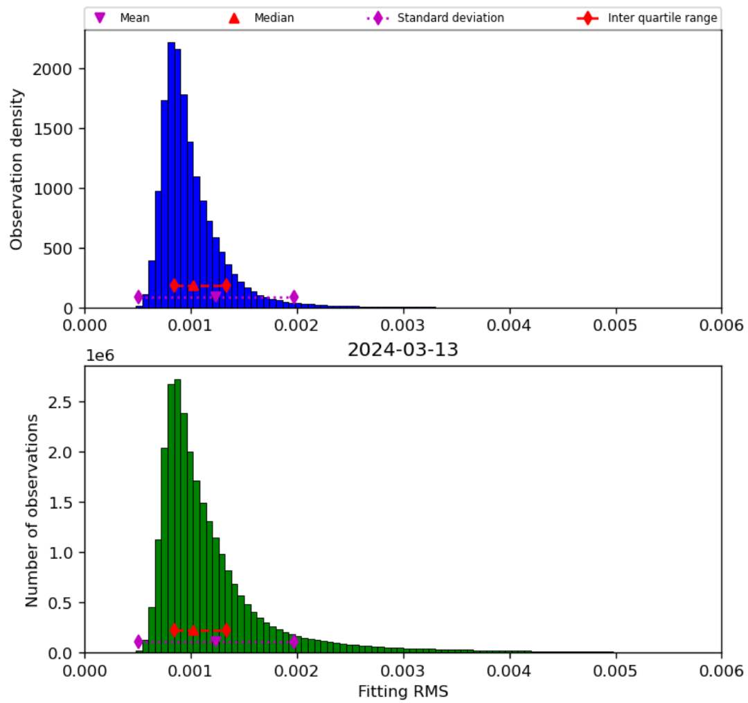
Figure 23: Histogram of “Fitting RMS” for 2024-03-12 to 2024-03-14
