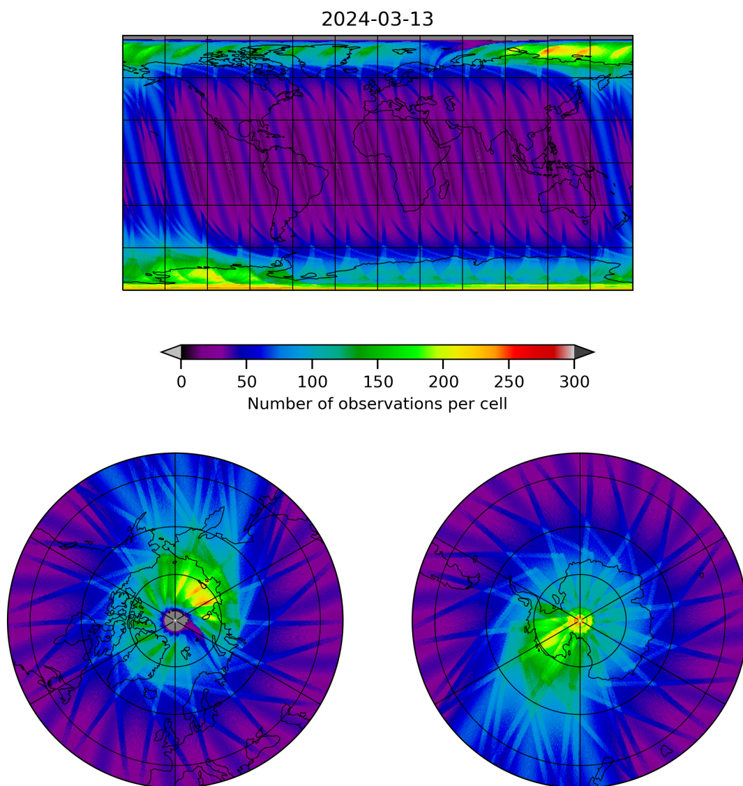
Figure 12: Map of the number of observations for 2024-03-12 to 2024-03-14
