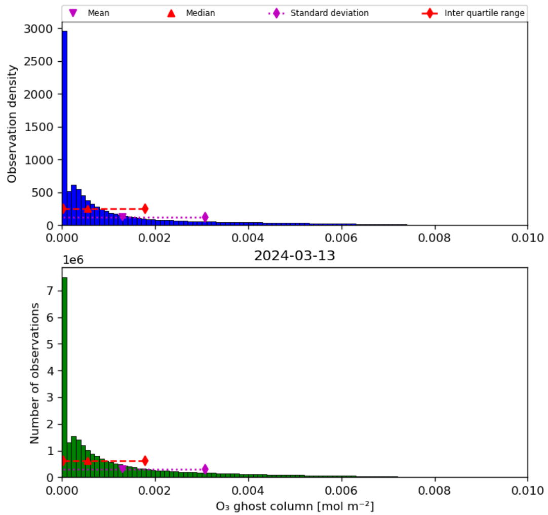
Figure 25: Histogram of “O 3 ghost column” for 2024-03-12 to 2024-03-14
