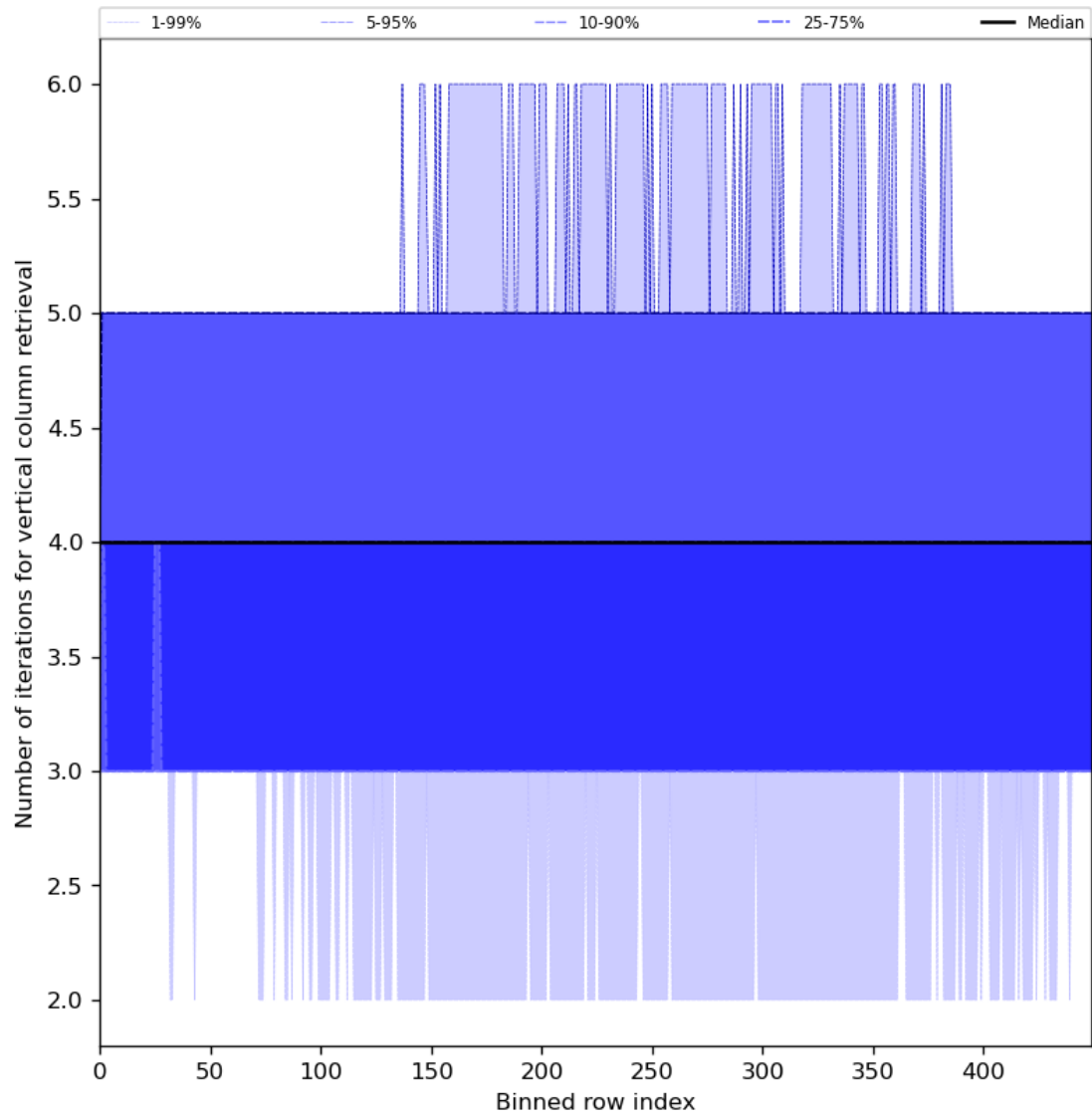
Figure 33: Along track statistics of “Number of iterations for vertical column retrieval” for 2024-03-12 to 2024-03-14
