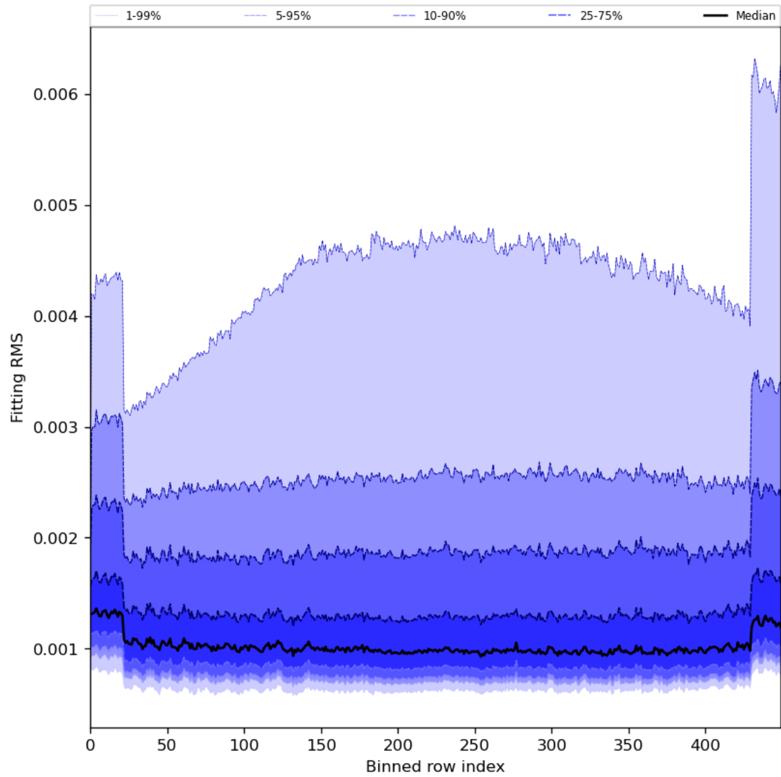
Figure 30: Along track statistics of “Fitting RMS” for 2024-03-12 to 2024-03-14
