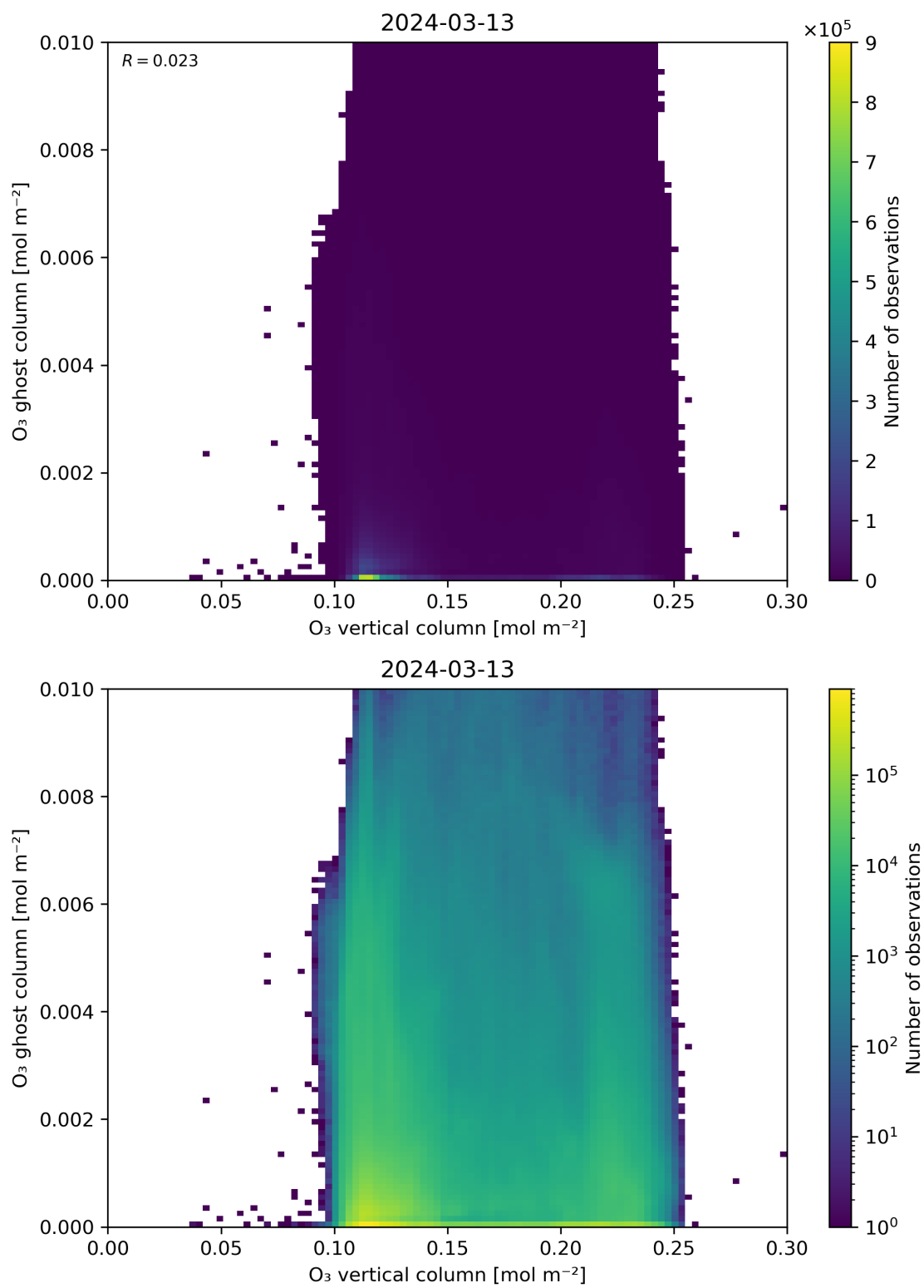
Figure 40: Scatter density plot of “O 3 vertical column” against “O 3 ghost column” for 2024-03-12 to 2024-03-14.
