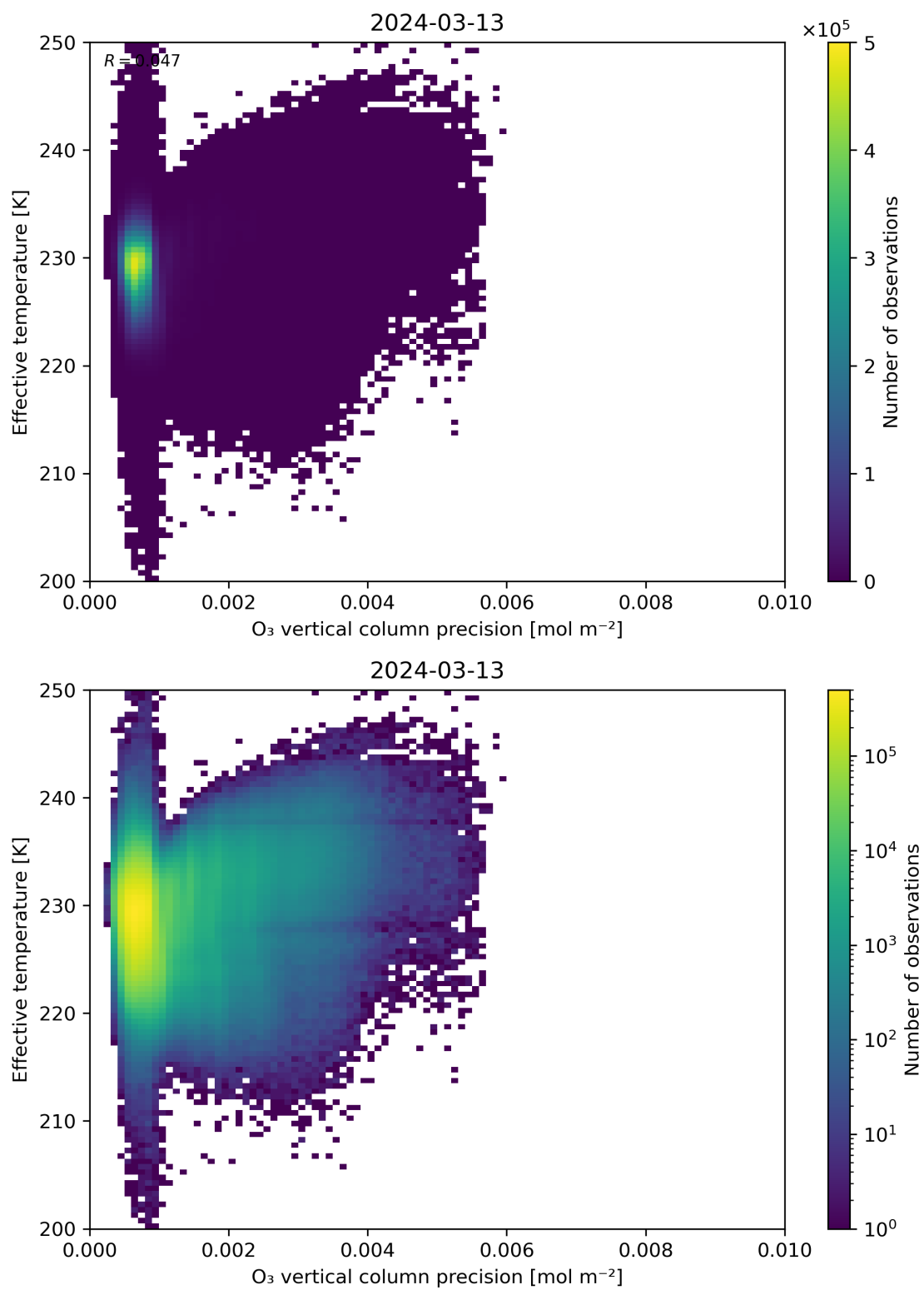
Figure 42: Scatter density plot of “O 3 vertical column precision” against “Effective temperature” for 2024-03-12 to 2024-03-14.
