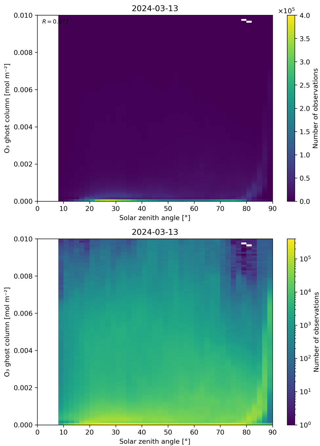
Figure 46: Scatter density plot of “Solar zenith angle” against “O 3 ghost column” for 2024-03-12 to 2024-03-14.
