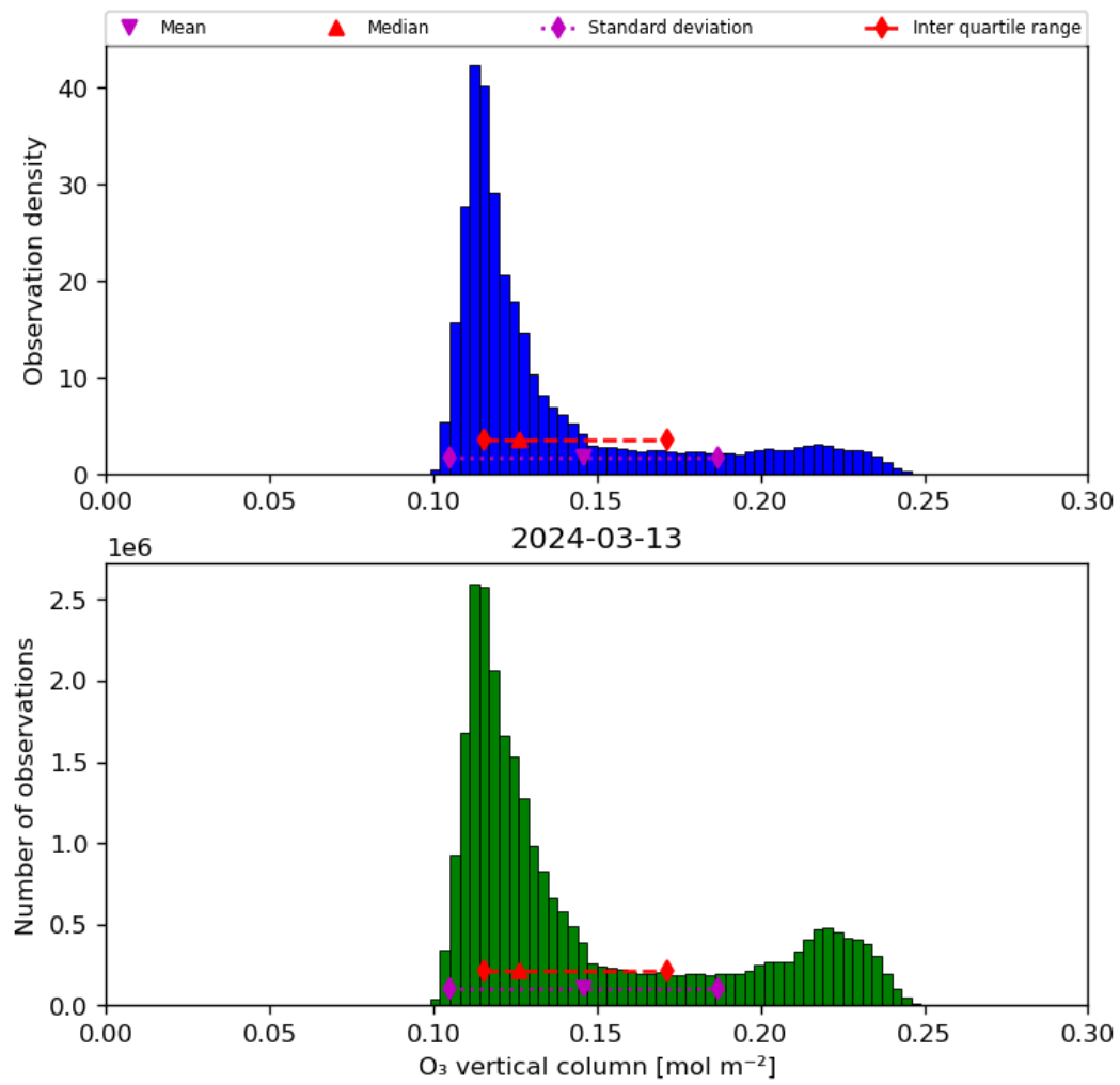
Figure 21: Histogram of “O 3 vertical column” for 2024-03-12 to 2024-03-14
