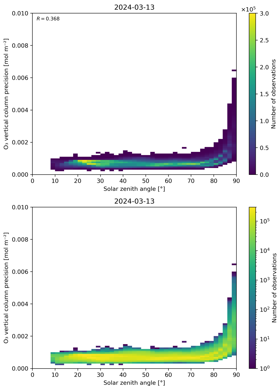
Figure 48: Scatter density plot of “Solar zenith angle” against “O 3 vertical column precision” for 2024-03-12 to 2024-03-14.
