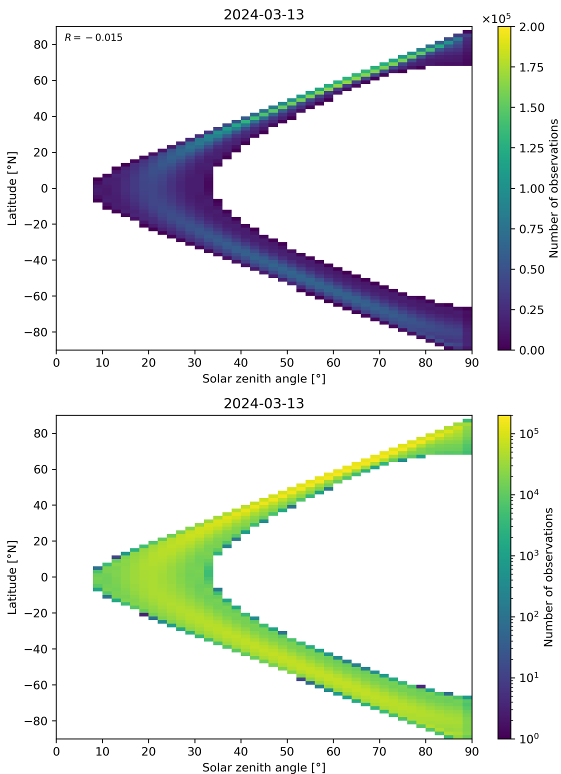
Figure 44: Scatter density plot of “Solar zenith angle” against “Latitude” for 2024-03-12 to 2024-03-14.
