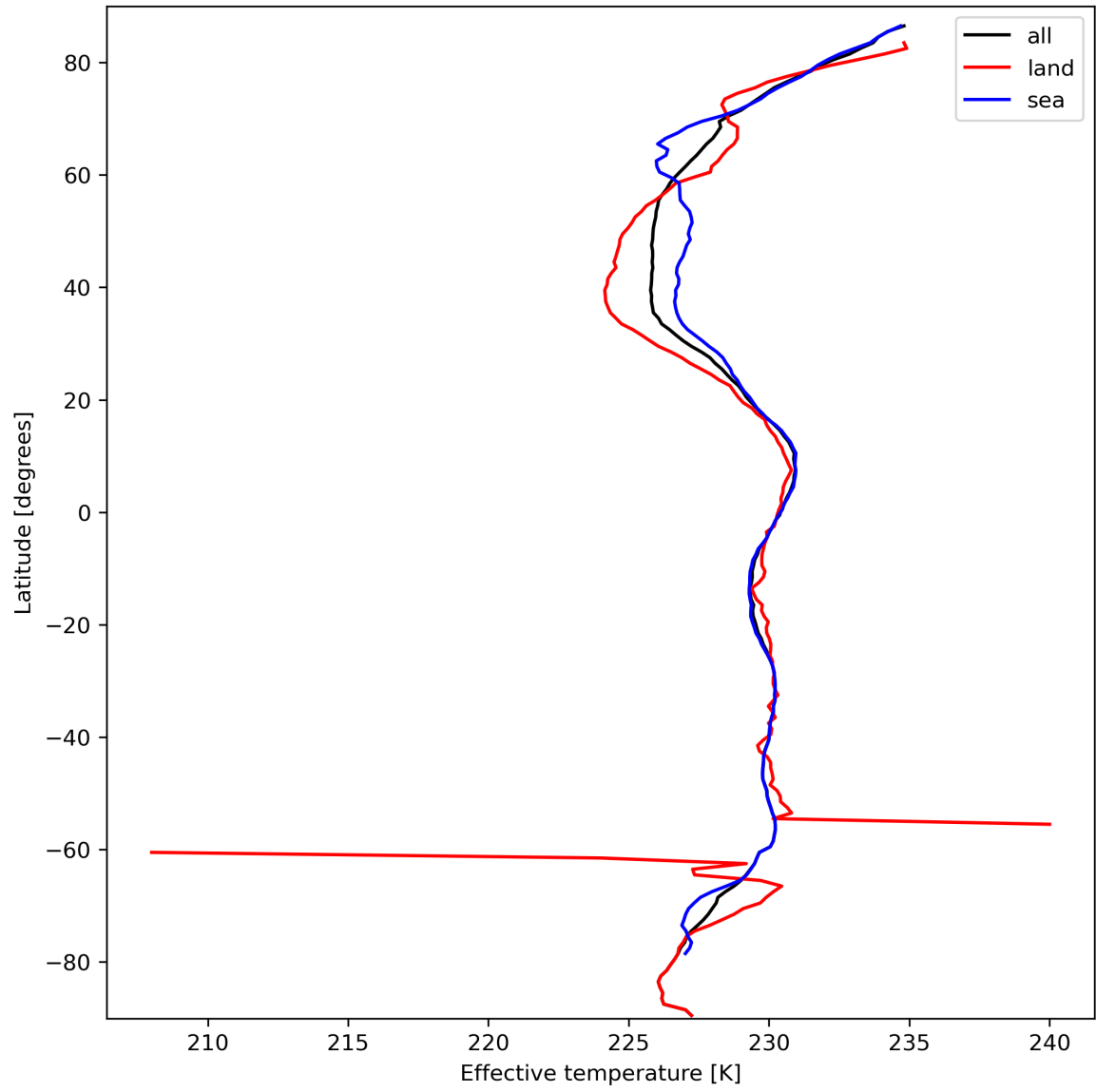
Figure 17: Zonal average of "Effective temperature" for 2024-03-12 to 2024-03-14.
