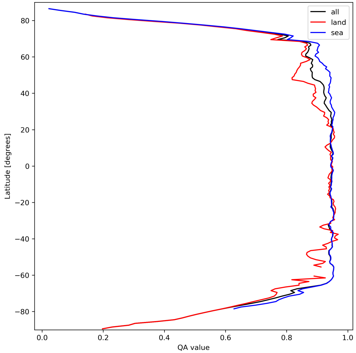
Figure 13: Zonal average of “QA value” for 2024-03-12 to 2024-03-14.
