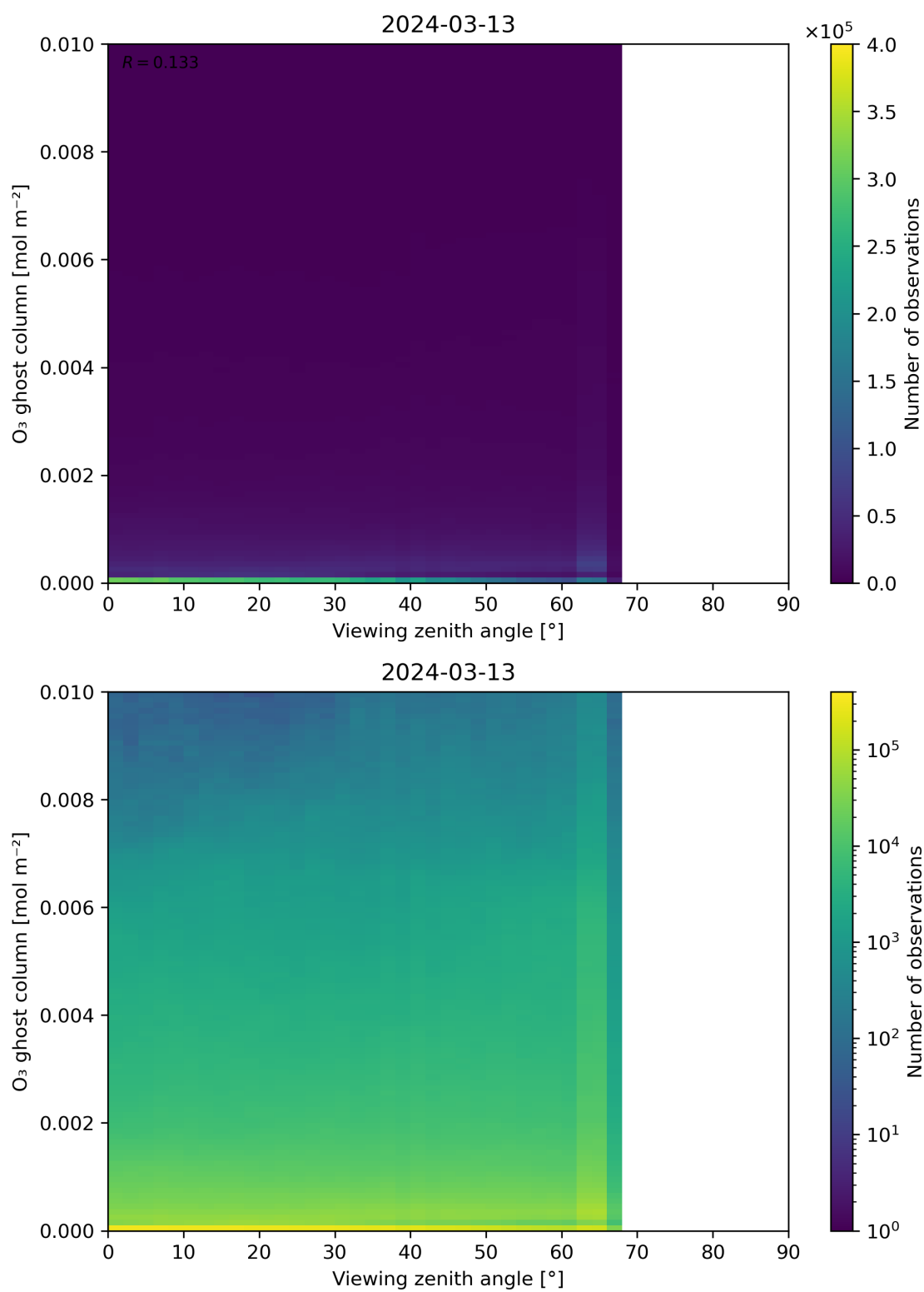
Figure 51: Scatter density plot of “Viewing zenith angle” against “O 3 ghost column” for 2024-03-12 to 2024-03-14.
