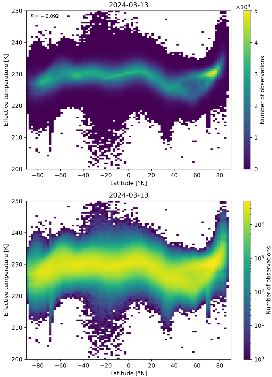
Figure 34: Scatter density plot of “Latitude” against “Effective temperature” for 2024-03-12 to 2024-03-14.
