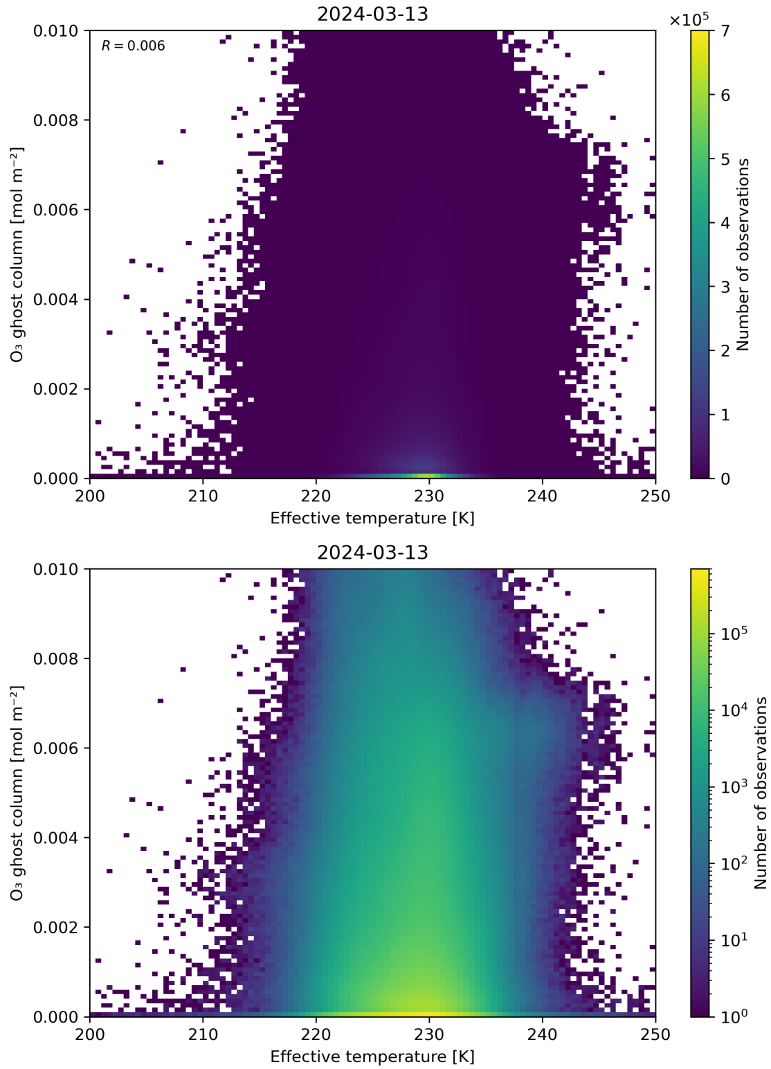
Figure 38: Scatter density plot of “Effective temperature” against “O 3 ghost column” for 2024-03-12 to 2024-03-14.
