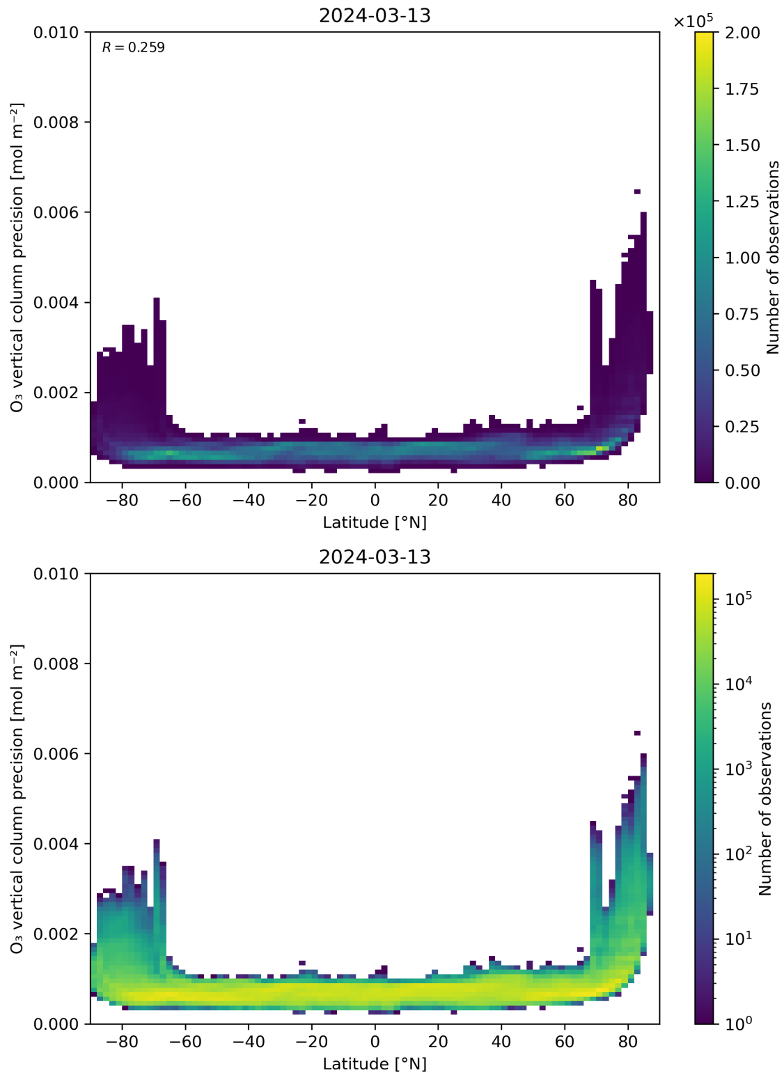
Figure 37: Scatter density plot of “Latitude” against “O 3 vertical column precision” for 2024-03-12 to 2024-03-14.
