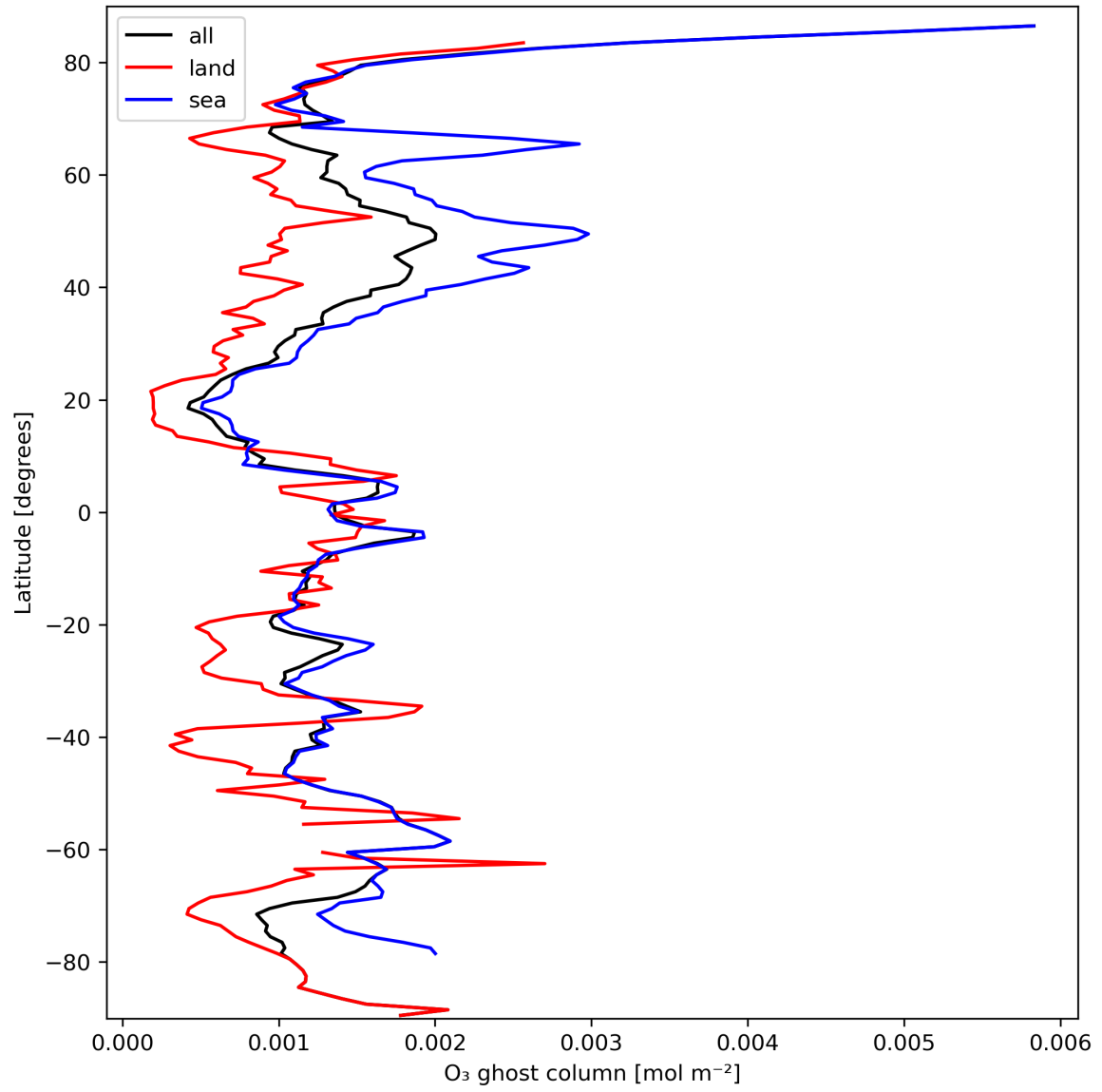
Figure 18: Zonal average of “O 3 ghost column” for 2024-03-12 to 2024-03-14.
