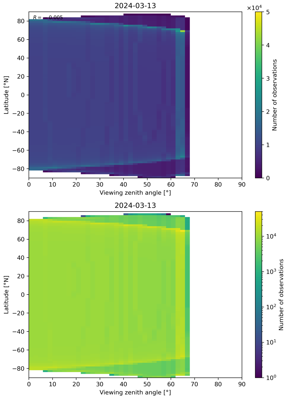
Figure 49: Scatter density plot of “Viewing zenith angle” against “Latitude” for 2024-03-12 to 2024-03-14.
