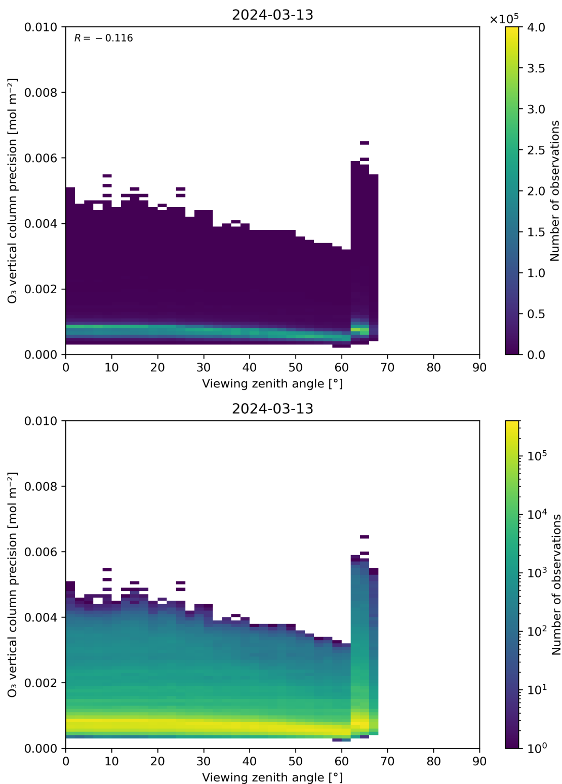
Figure 53: Scatter density plot of “Viewing zenith angle” against “O 3 vertical column precision” for 2024-03-12 to 2024-03-14.
