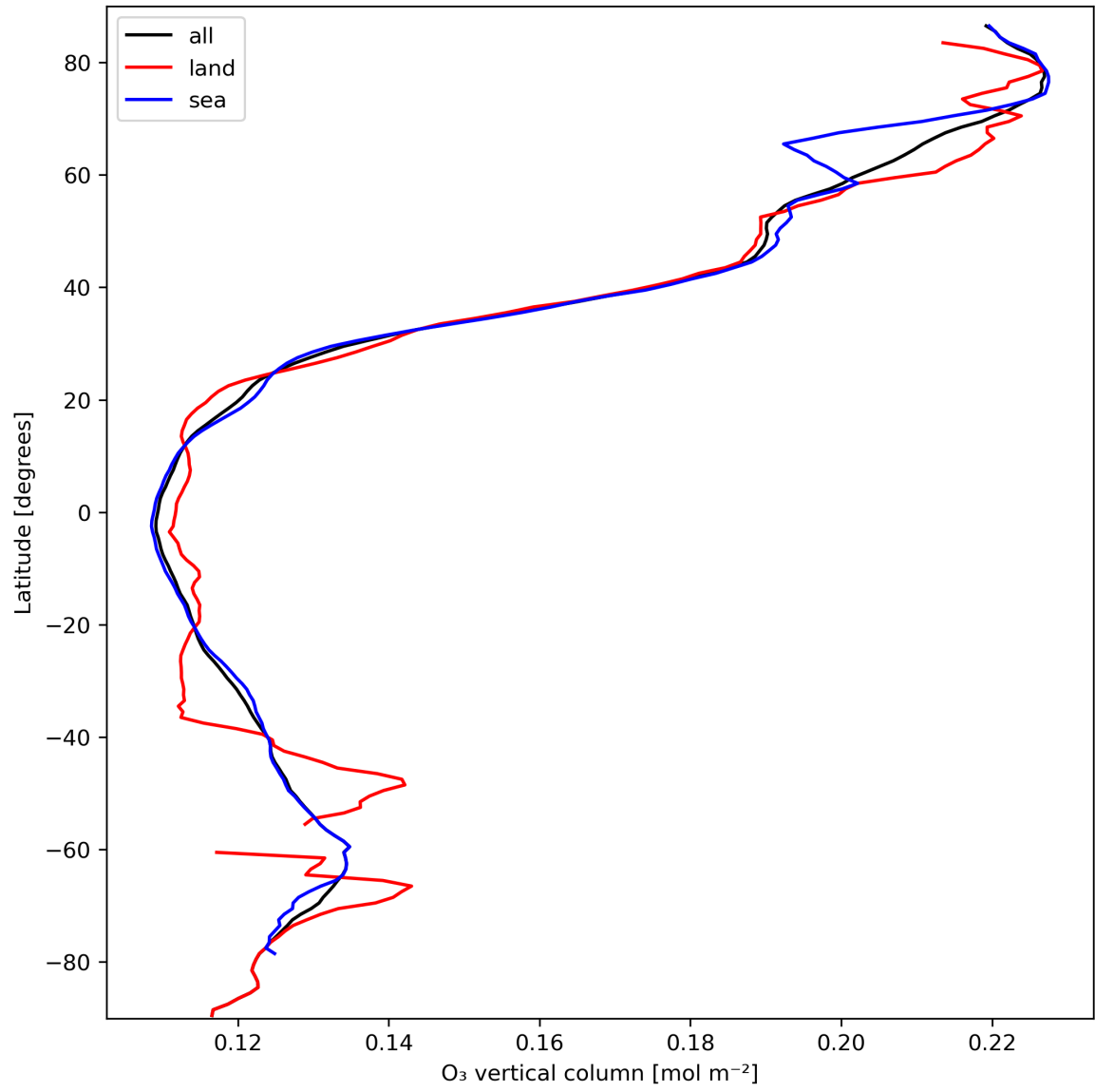
Figure 14: Zonal average of “O 3 vertical column” for 2024-03-12 to 2024-03-14.
