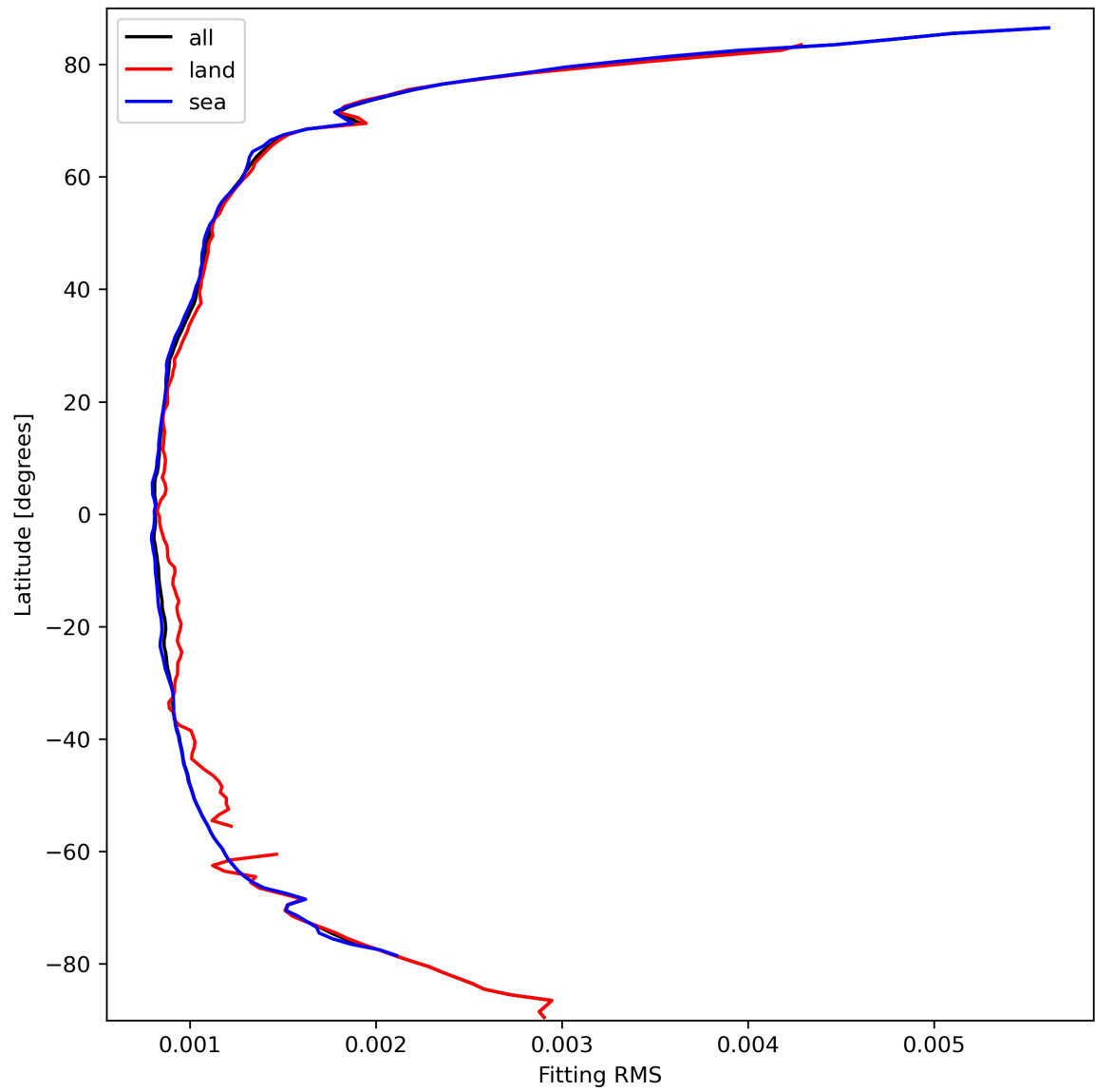
Figure 16: Zonal average of “Fitting RMS” for 2024-03-12 to 2024-03-14.
