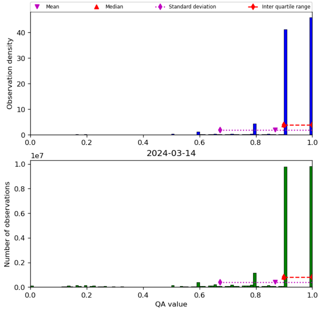
Figure 20: Histogram of “QA value” for 2024-03-14 to 2024-03-15
