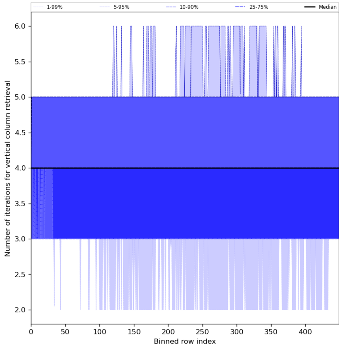
Figure 33: Along track statistics of “Number of iterations for vertical column retrieval” for 2024-03-14 to 2024-03-15
