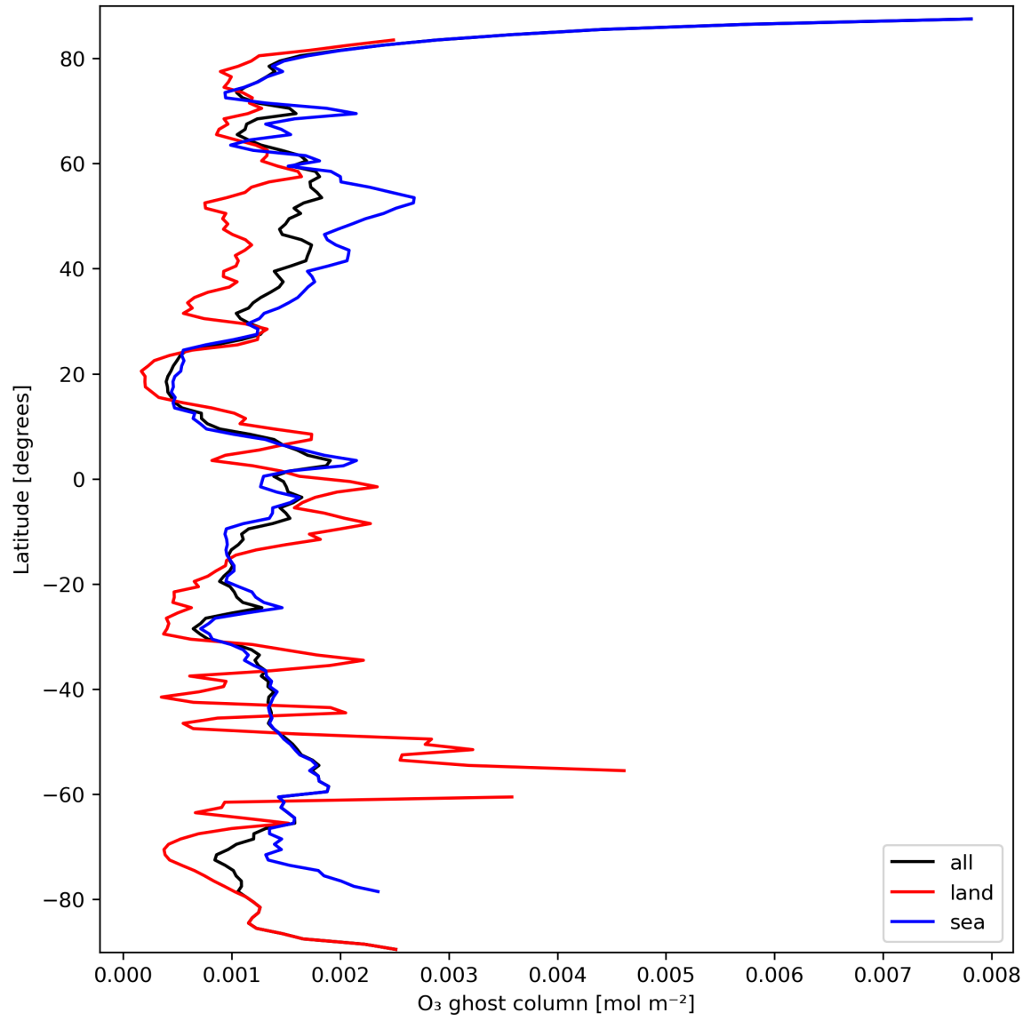
Figure 18: Zonal average of “O 3 ghost column” for 2024-03-14 to 2024-03-15.
