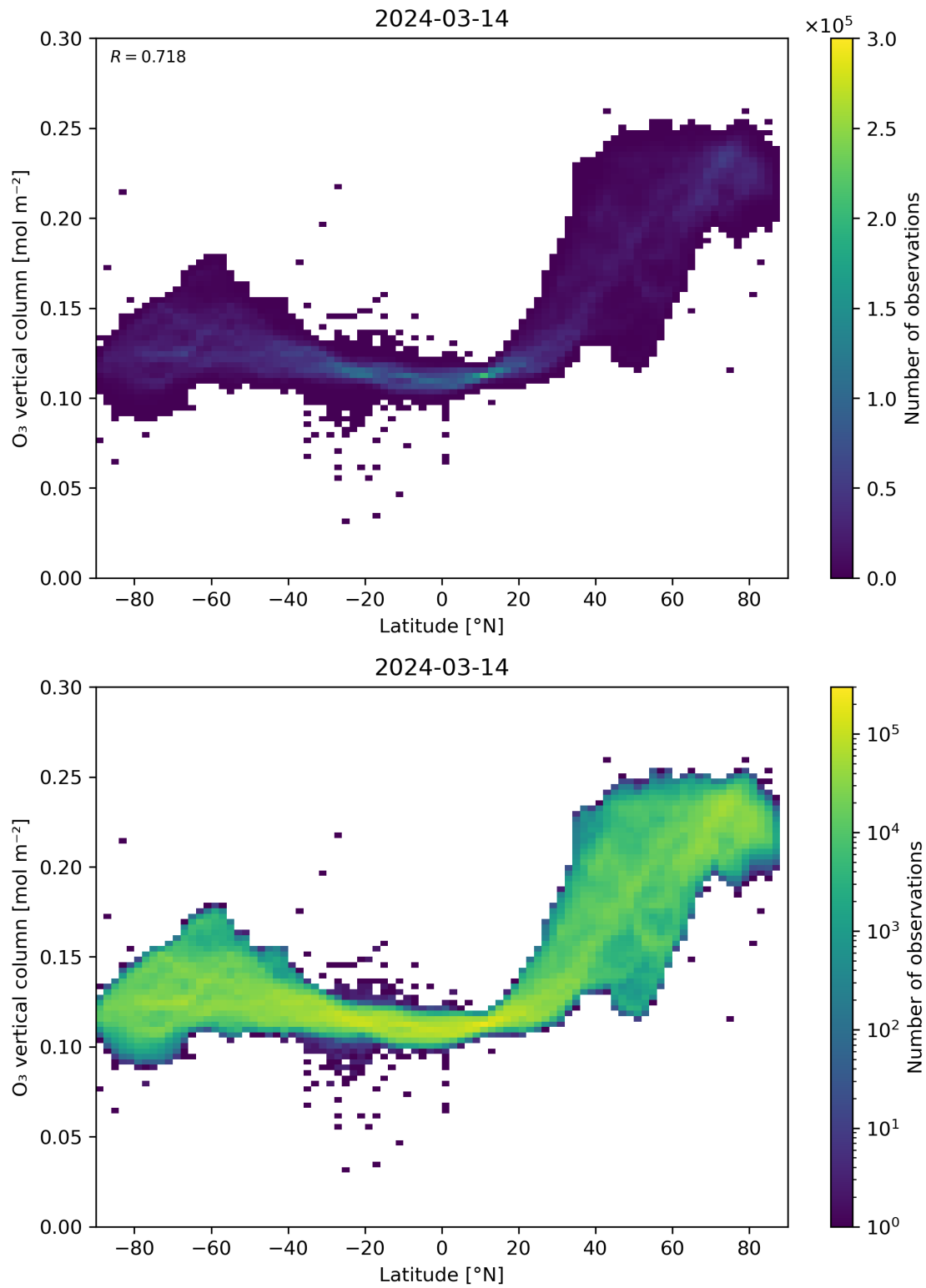
Figure 36: Scatter density plot of “Latitude” against “O 3 vertical column” for 2024-03-14 to 2024-03-15.
