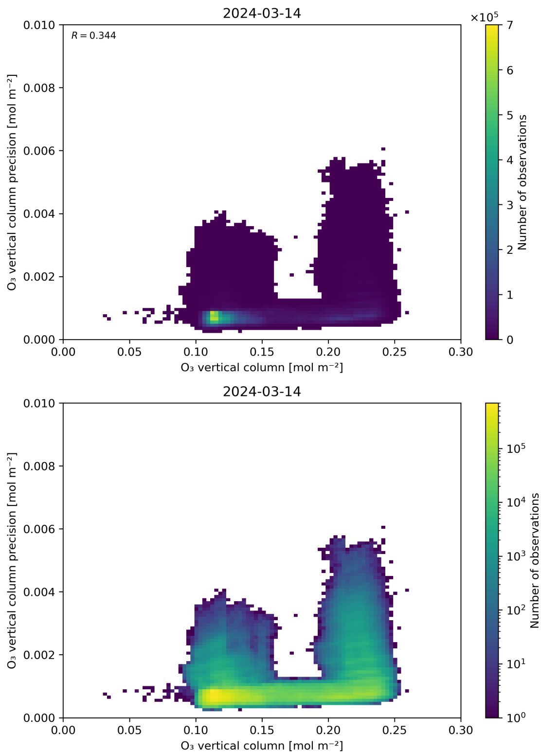
Figure 41: Scatter density plot of “O 3 vertical column” against “O 3 vertical column precision” for 2024-03-14 to 2024-03-15.
