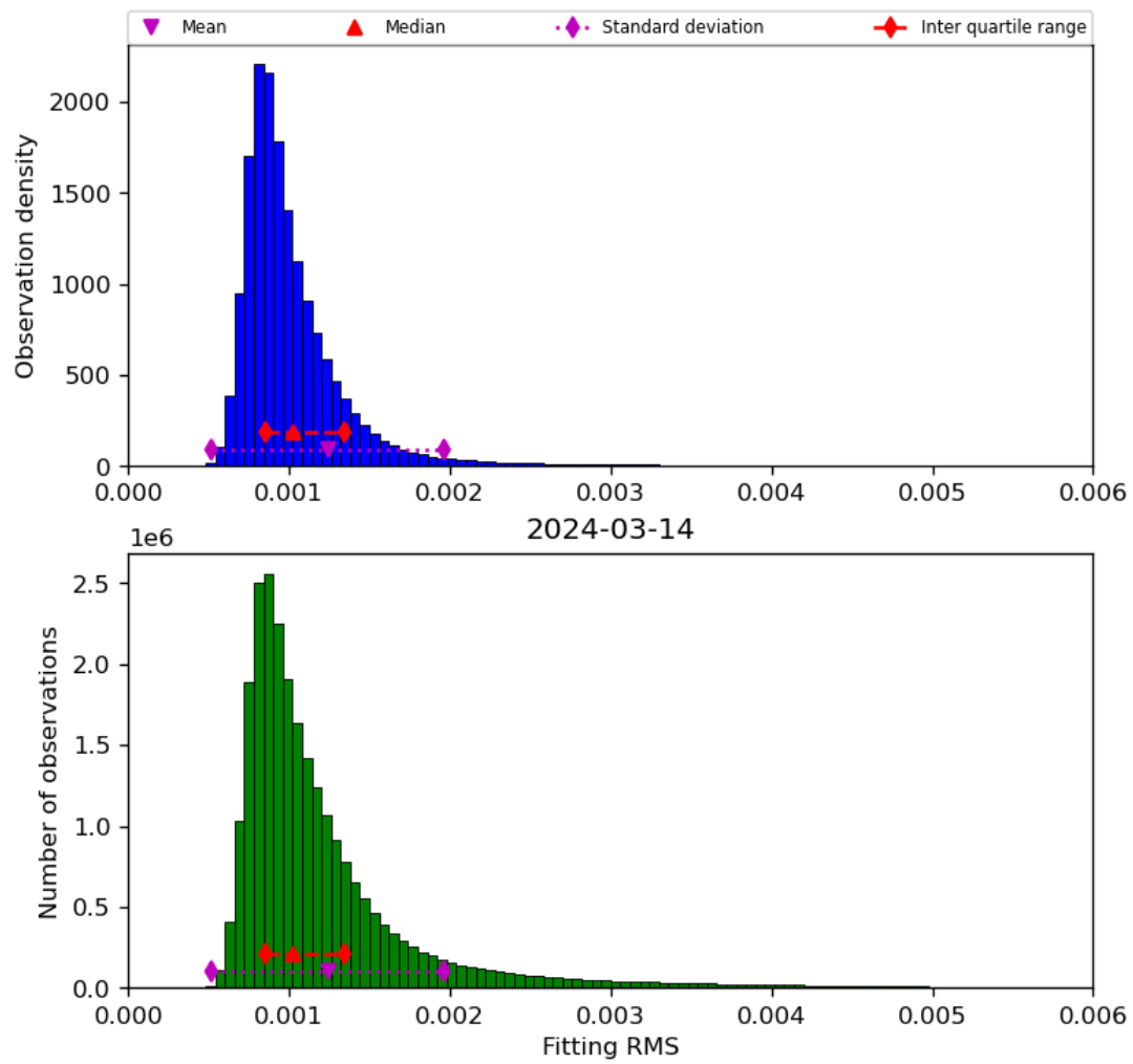
Figure 23: Histogram of “Fitting RMS” for 2024-03-14 to 2024-03-15
