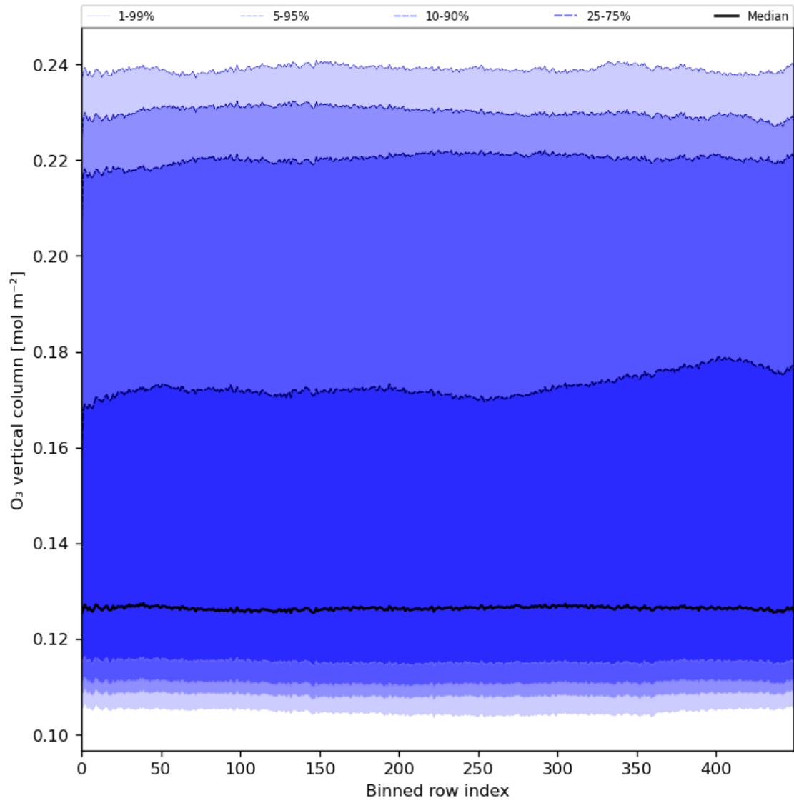
Figure 28: Along track statistics of “O 3 vertical column” for 2024-03-14 to 2024-03-15
