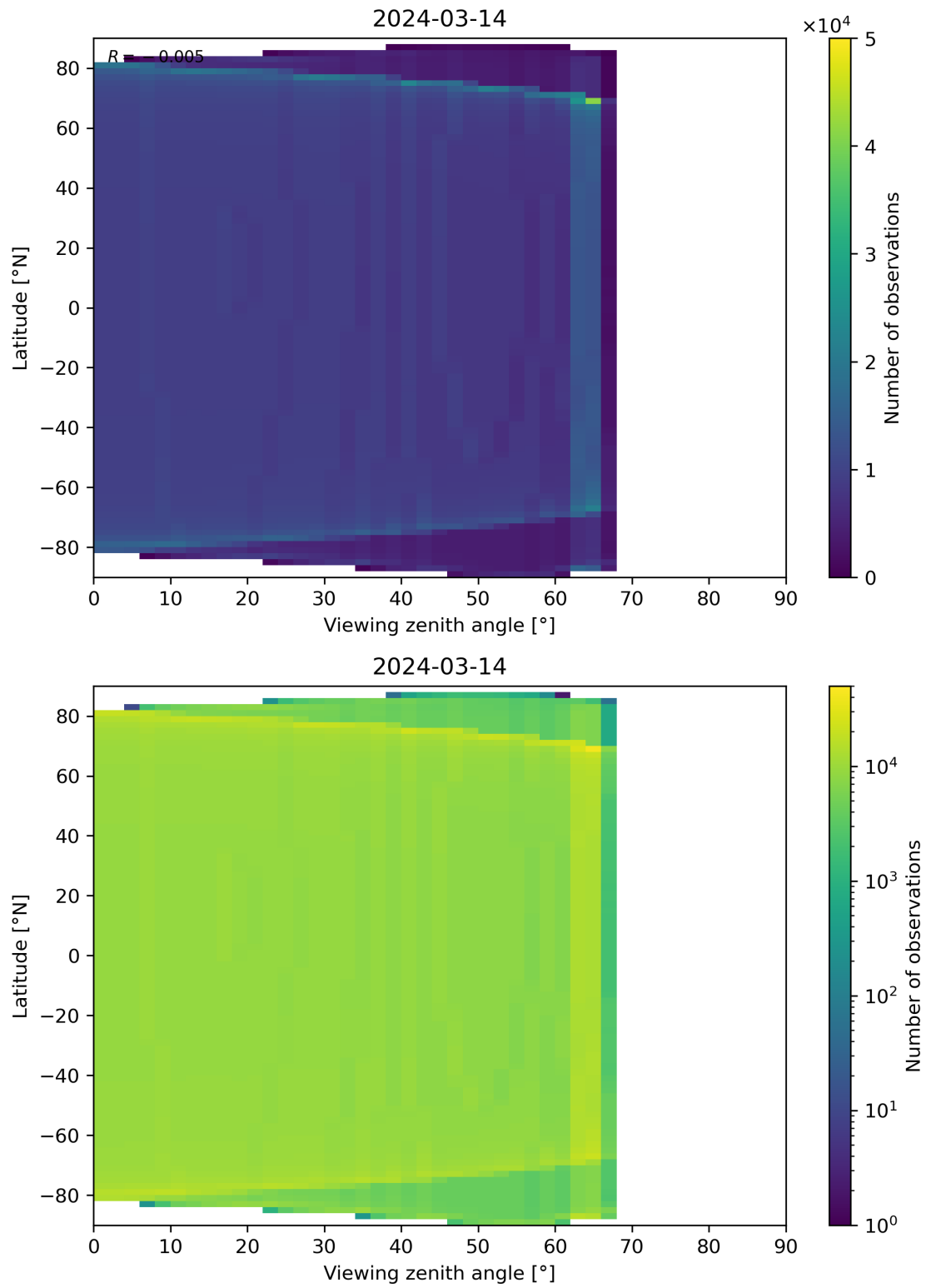
Figure 49: Scatter density plot of “Viewing zenith angle” against “Latitude” for 2024-03-14 to 2024-03-15.
