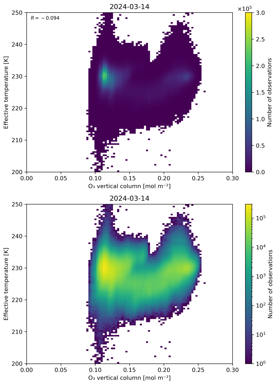
Figure 39: Scatter density plot of “O 3 vertical column” against “Effective temperature” for 2024-03-14 to 2024-03-15.
