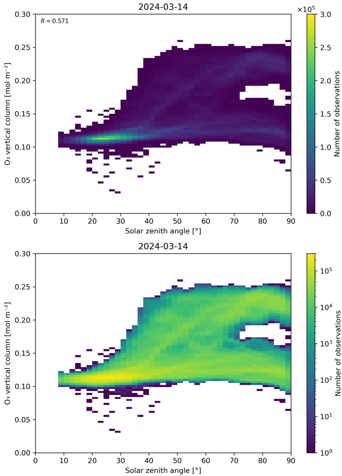
Figure 47: Scatter density plot of “Solar zenith angle” against “O 3 vertical column” for 2024-03-14 to 2024-03-15.
