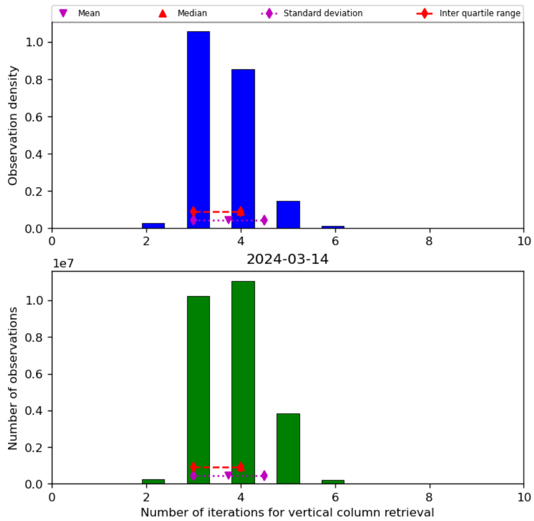
Figure 26: Histogram of “Number of iterations for vertical column retrieval” for 2024-03-14 to 2024-03-15
