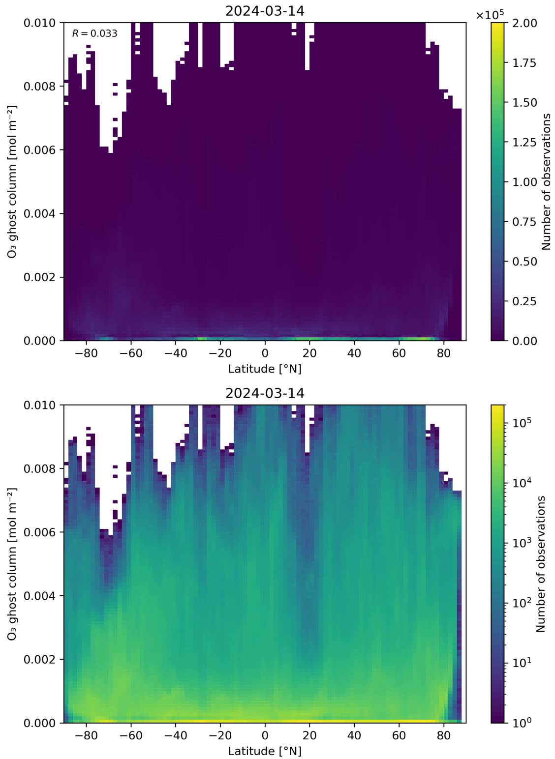
Figure 35: Scatter density plot of “Latitude” against “O 3 ghost column” for 2024-03-14 to 2024-03-15.
