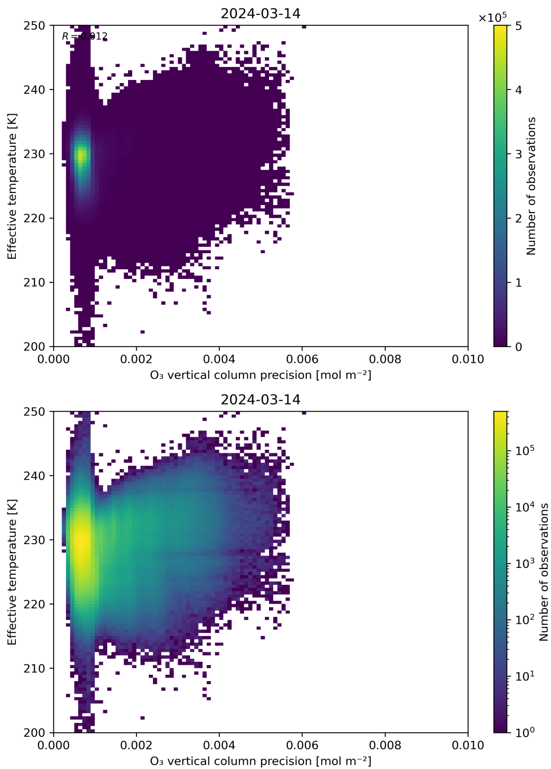
Figure 42: Scatter density plot of “O 3 vertical column precision” against “Effective temperature” for 2024-03-14 to 2024-03-15.
