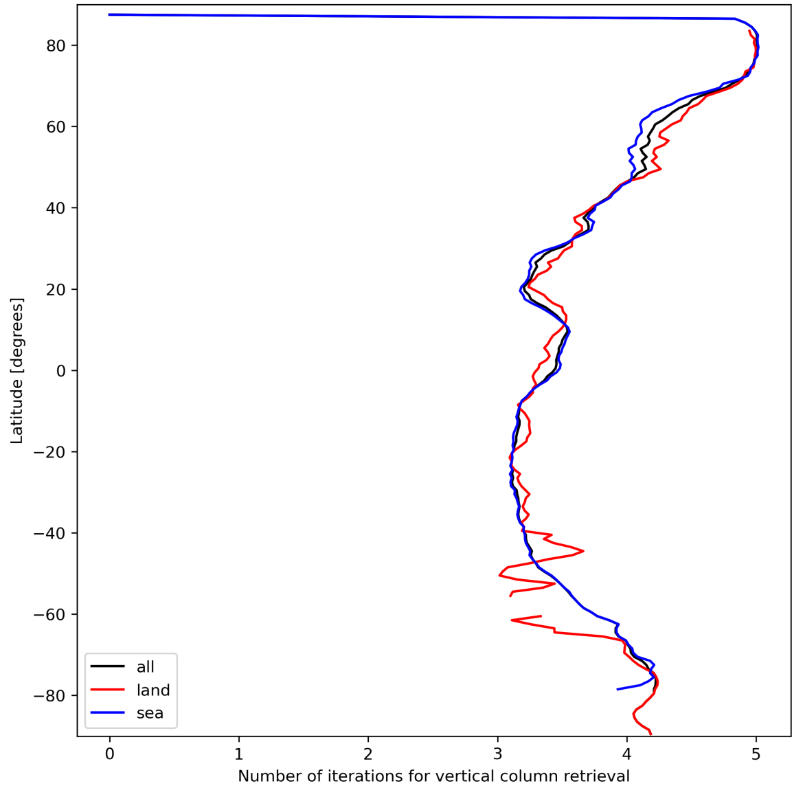
Figure 19: Zonal average of “Number of iterations for vertical column retrieval” for 2024-03-14 to 2024-03-15.
