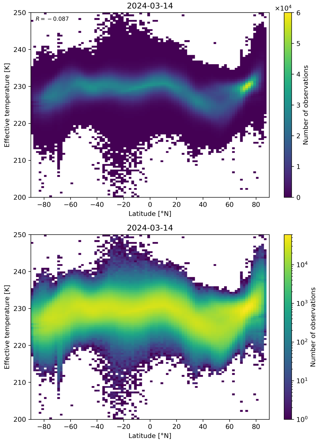
Figure 34: Scatter density plot of “Latitude” against “Effective temperature” for 2024-03-14 to 2024-03-15.
