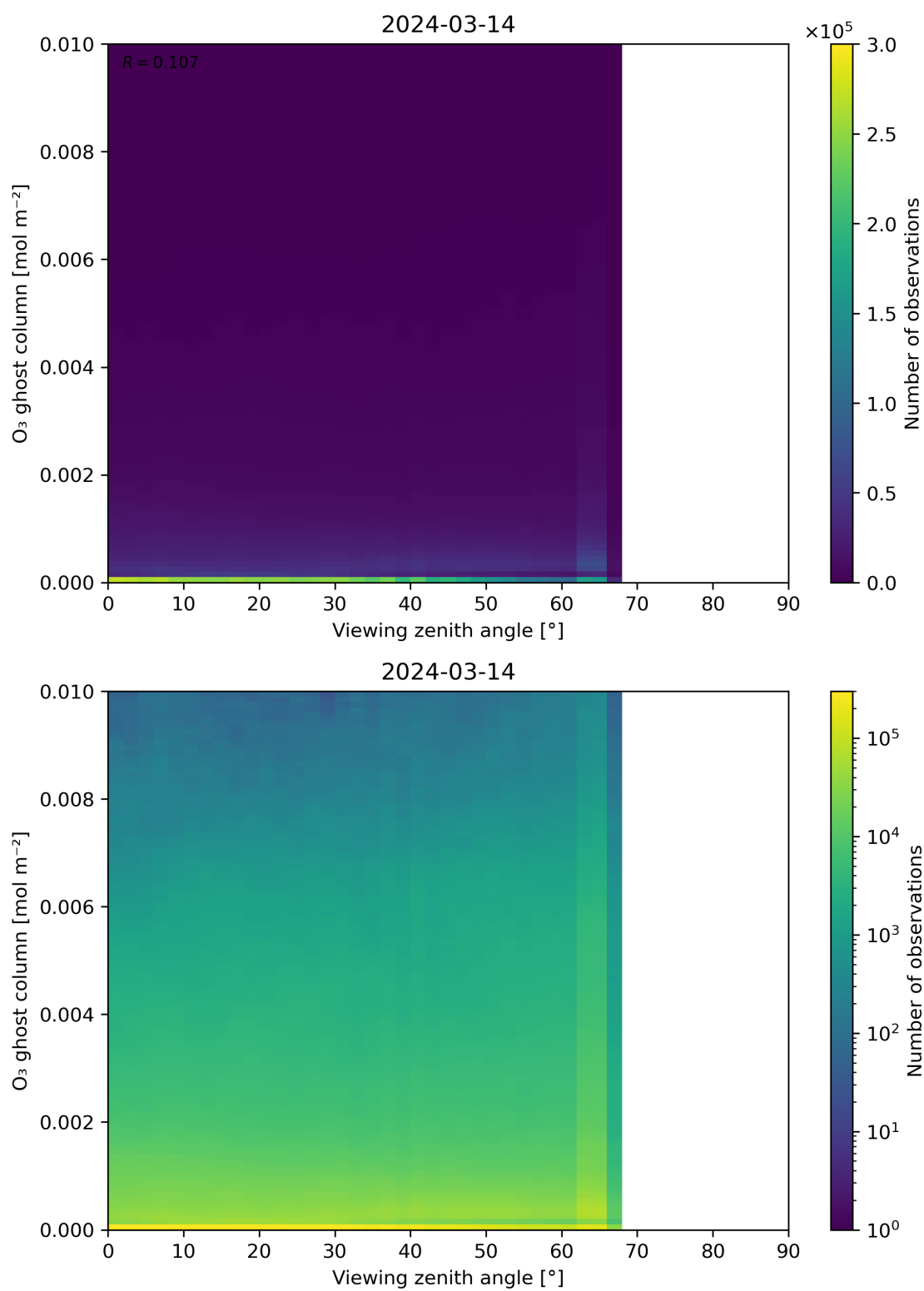
Figure 51: Scatter density plot of “Viewing zenith angle” against “O 3 ghost column” for 2024-03-14 to 2024-03-15.
