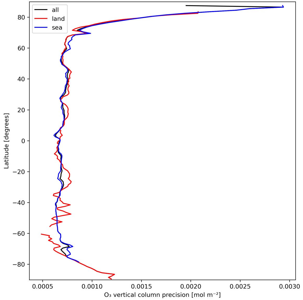
Figure 15: Zonal average of “O 3 vertical column precision” for 2024-03-14 to 2024-03-15.
