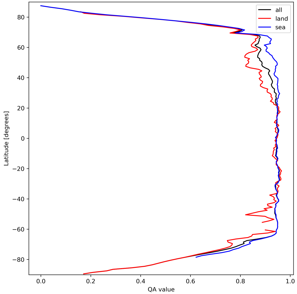
Figure 13: Zonal average of “QA value” for 2024-03-14 to 2024-03-15.
