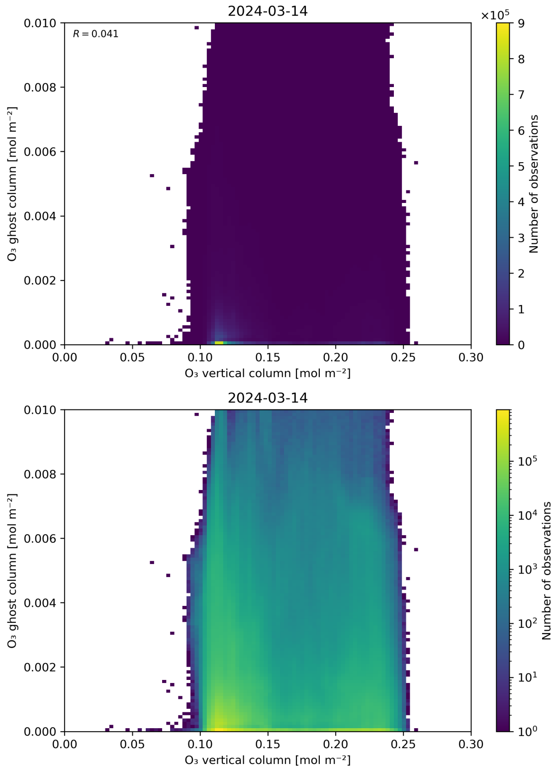
Figure 40: Scatter density plot of “O 3 vertical column” against “O 3 ghost column” for 2024-03-14 to 2024-03-15.
