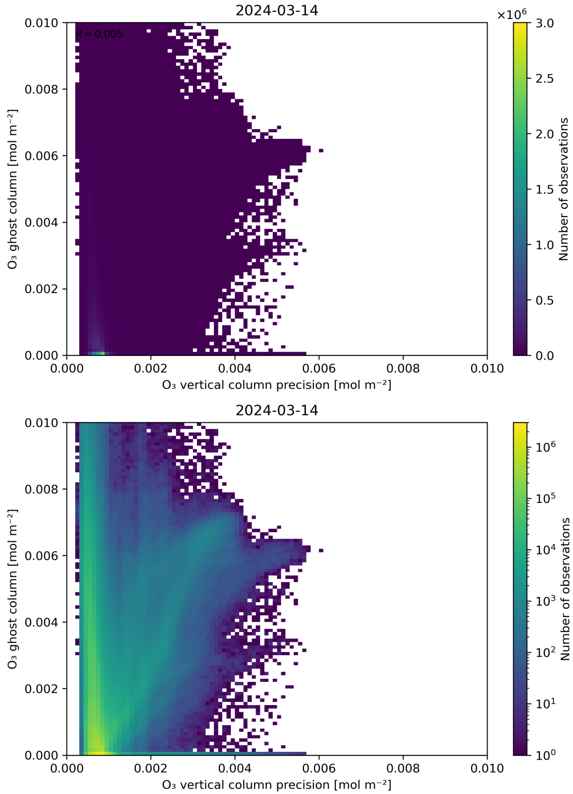
Figure 43: Scatter density plot of “ \text{O}_3 vertical column precision” against “ \text{O}_3 ghost column” for 2024-03-14 to 2024-03-15.
