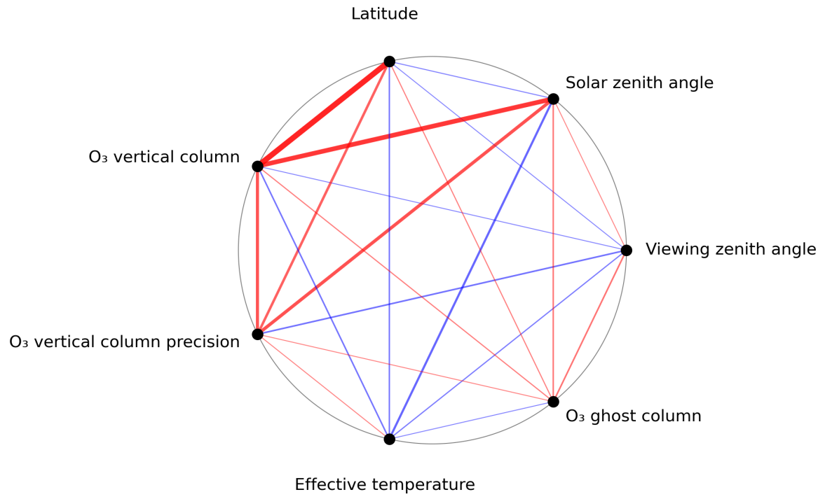
Figure 1: Map of correlation graph for 2024-03-14 to 2024-03-15.
