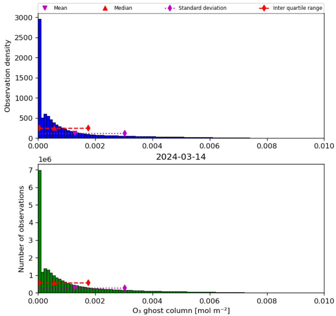
Figure 25: Histogram of “O 3 ghost column” for 2024-03-14 to 2024-03-15
