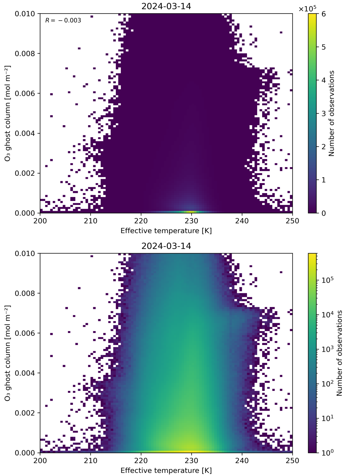
Figure 38: Scatter density plot of “Effective temperature” against “O 3 ghost column” for 2024-03-14 to 2024-03-15.
