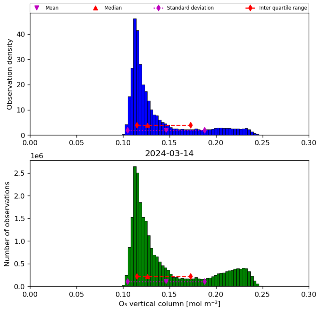
Figure 21: Histogram of “O 3 vertical column” for 2024-03-14 to 2024-03-15
