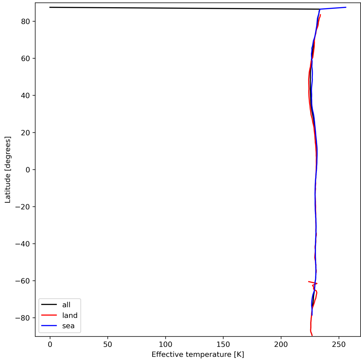
Figure 17: Zonal average of "Effective temperature" for 2024-03-14 to 2024-03-15.
