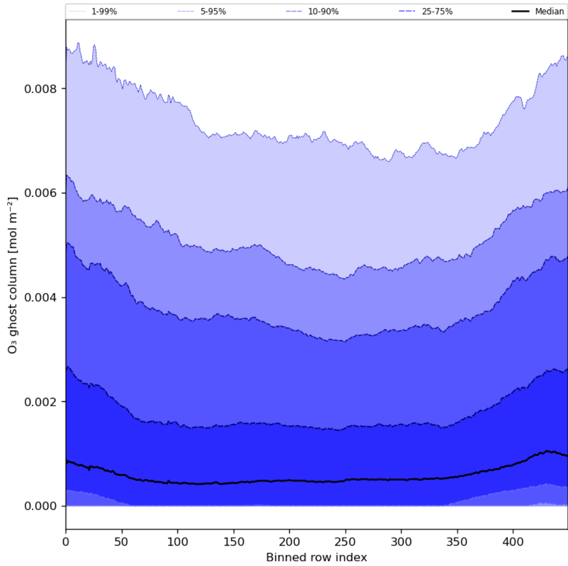
Figure 32: Along track statistics of “O 3 ghost column” for 2024-03-14 to 2024-03-15
