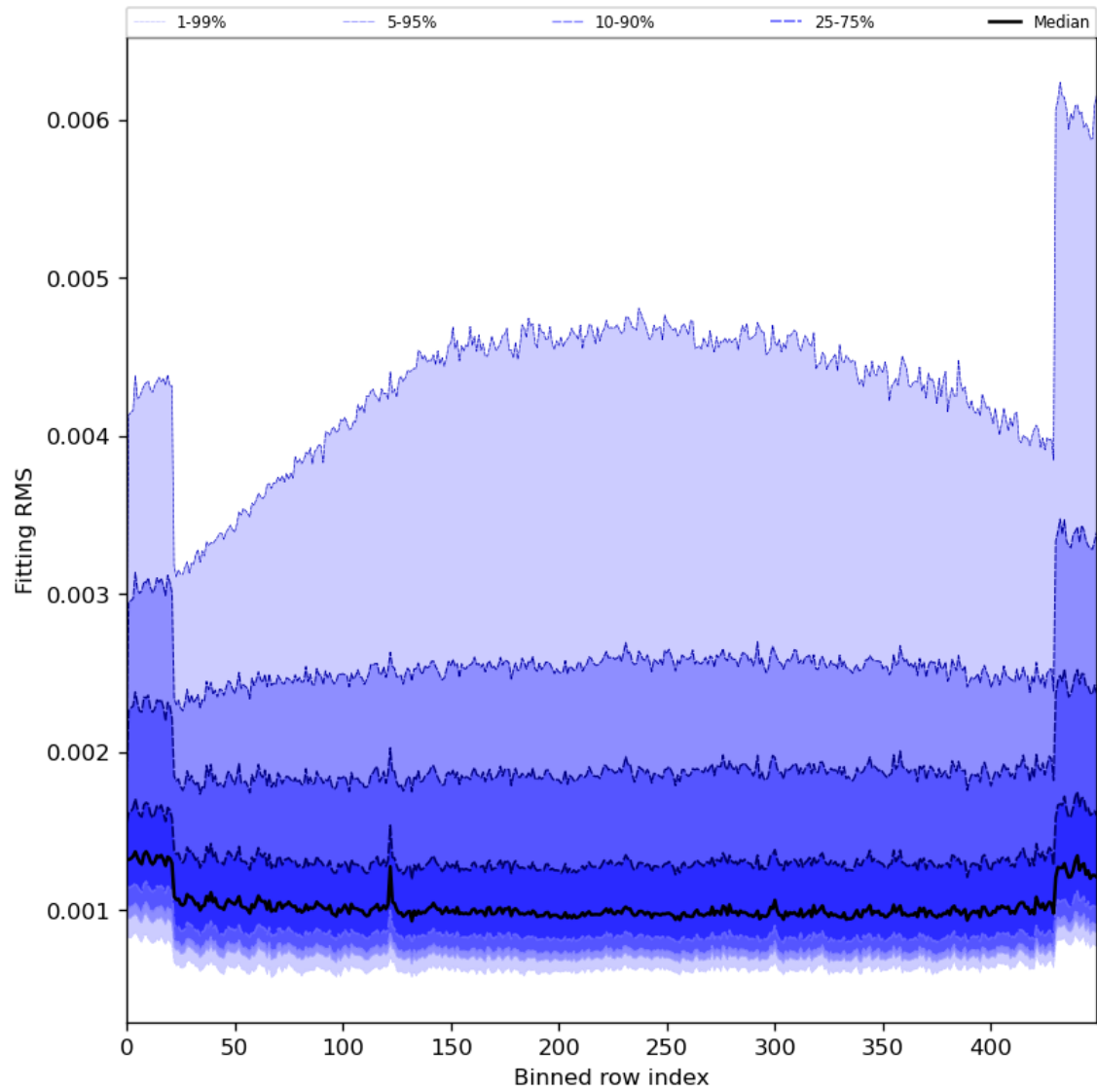
Figure 30: Along track statistics of “Fitting RMS” for 2024-03-14 to 2024-03-15
