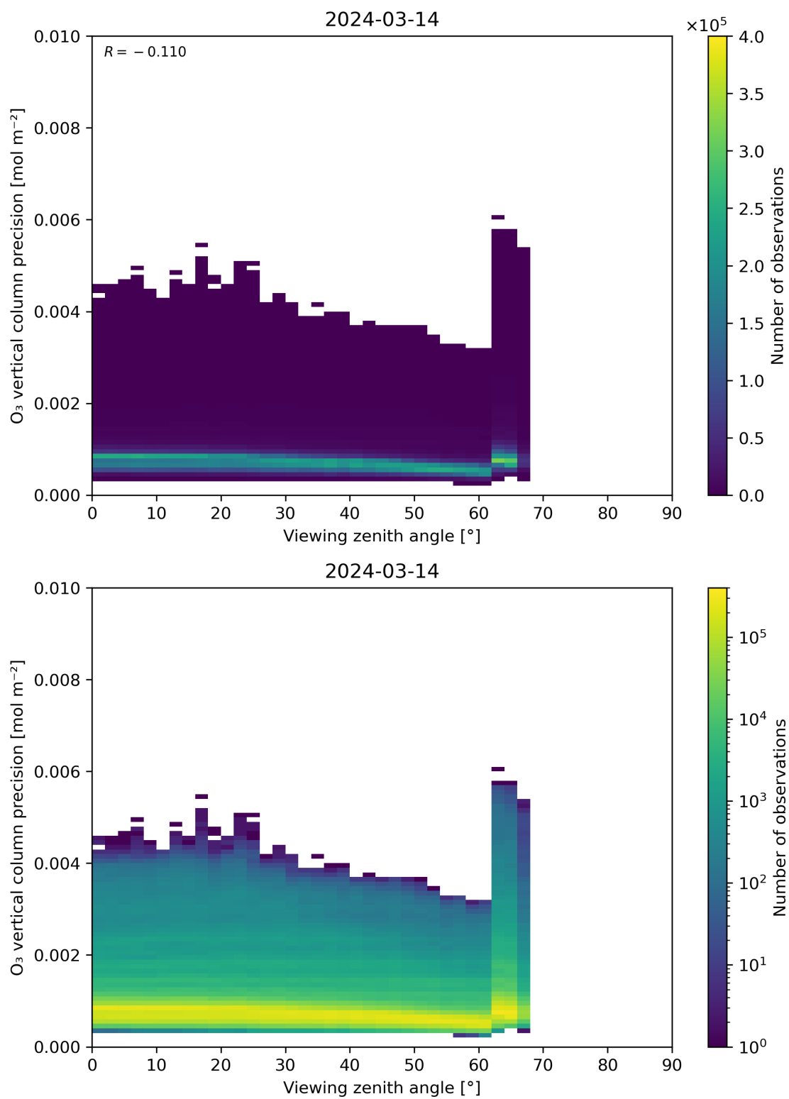
Figure 53: Scatter density plot of “Viewing zenith angle” against “O 3 vertical column precision” for 2024-03-14 to 2024-03-15.
