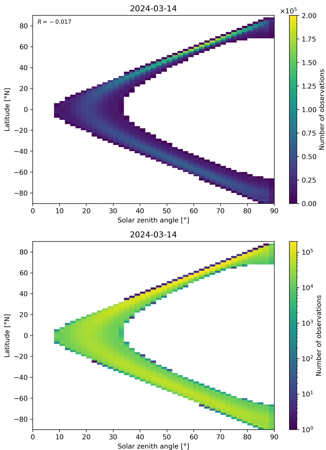
Figure 44: Scatter density plot of “Solar zenith angle” against “Latitude” for 2024-03-14 to 2024-03-15.
