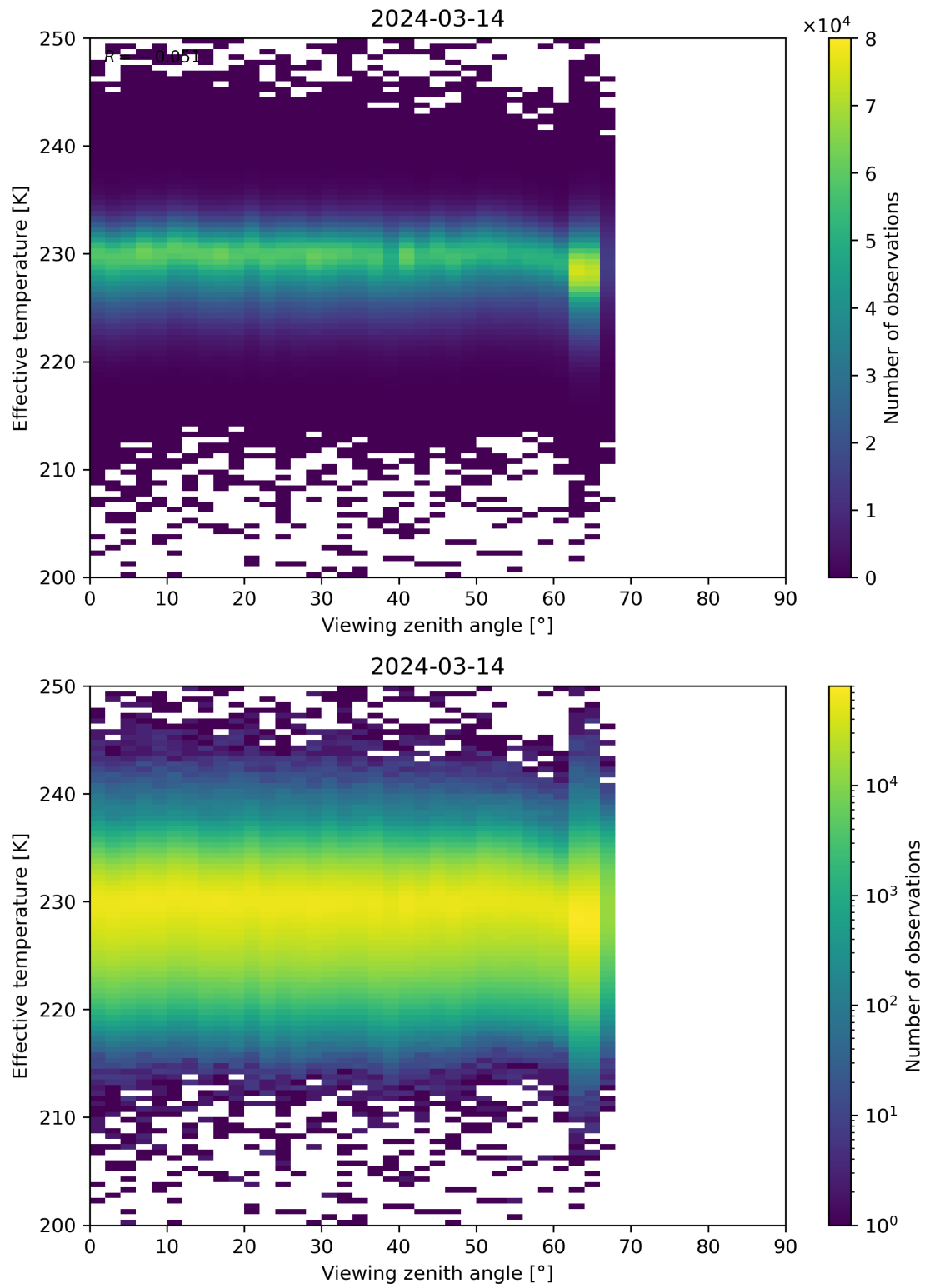
Figure 50: Scatter density plot of “Viewing zenith angle” against “Effective temperature” for 2024-03-14 to 2024-03-15.
