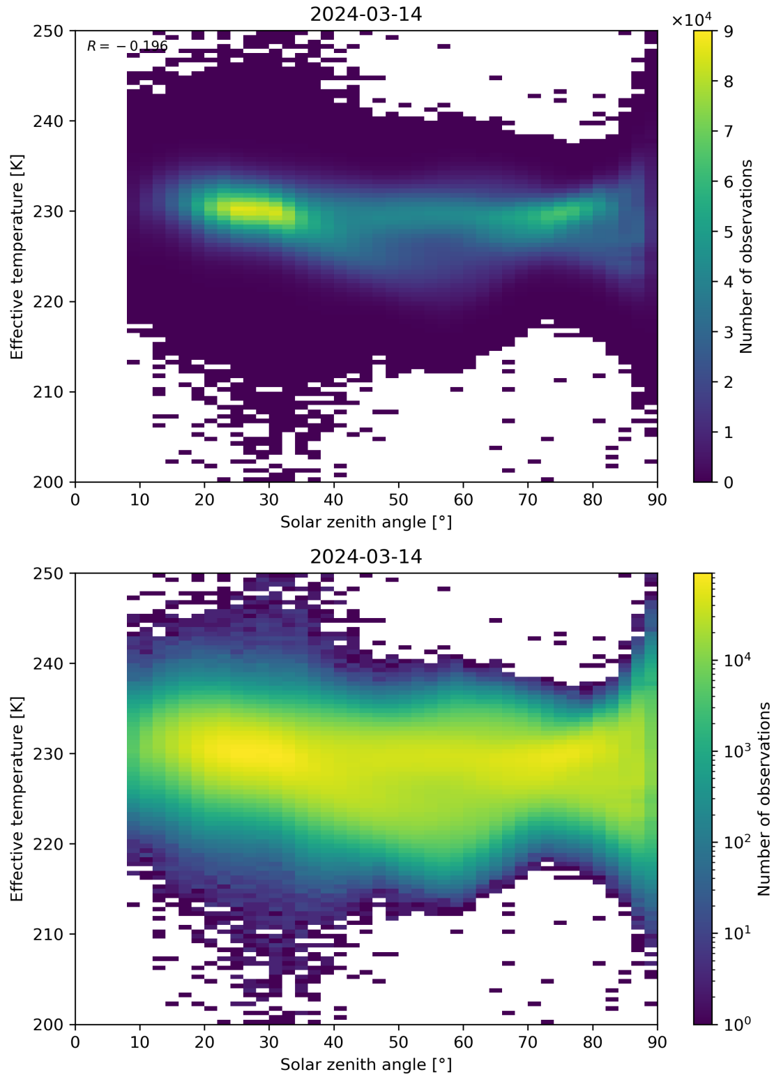
Figure 45: Scatter density plot of “Solar zenith angle” against “Effective temperature” for 2024-03-14 to 2024-03-15.
