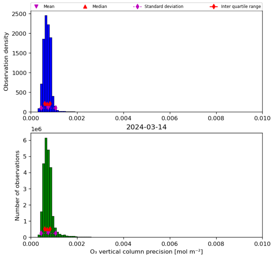
Figure 22: Histogram of “O 3 vertical column precision” for 2024-03-14 to 2024-03-15
