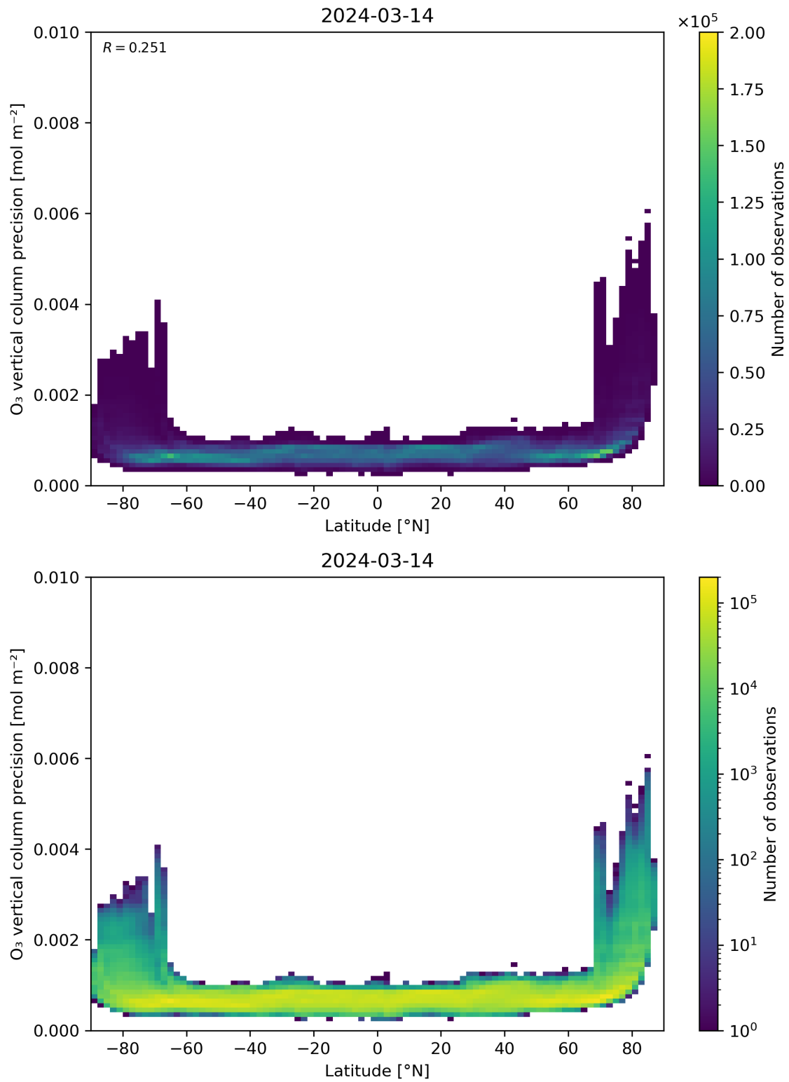
Figure 37: Scatter density plot of “Latitude” against “O 3 vertical column precision” for 2024-03-14 to 2024-03-15.
