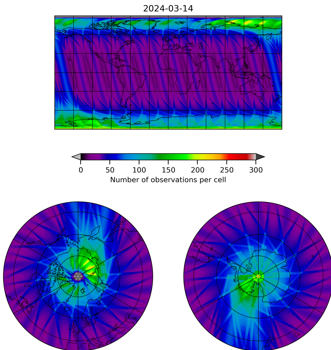
Figure 12: Map of the number of observations for 2024-03-14 to 2024-03-15
