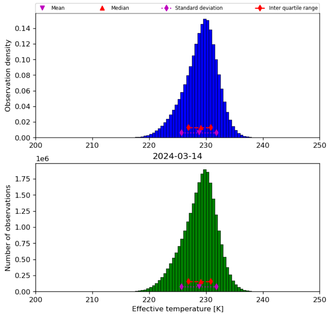
Figure 24: Histogram of “Effective temperature” for 2024-03-14 to 2024-03-15
