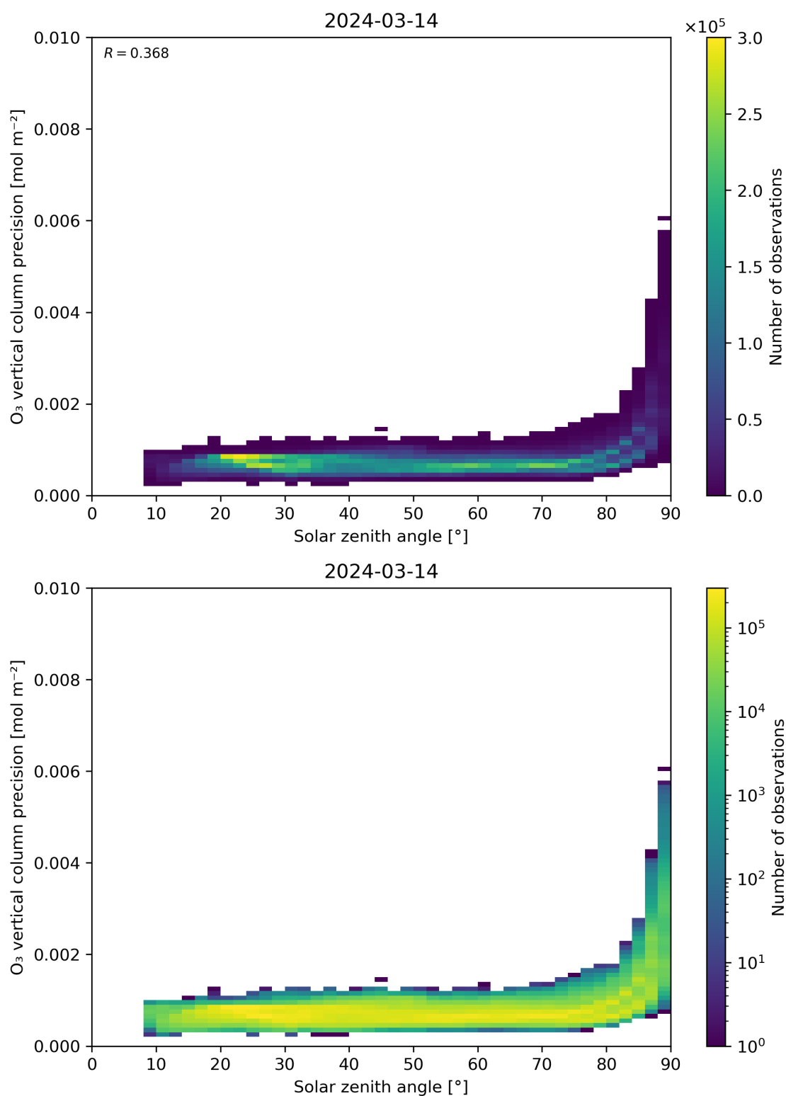
Figure 48: Scatter density plot of “Solar zenith angle” against “O 3 vertical column precision” for 2024-03-14 to 2024-03-15.
