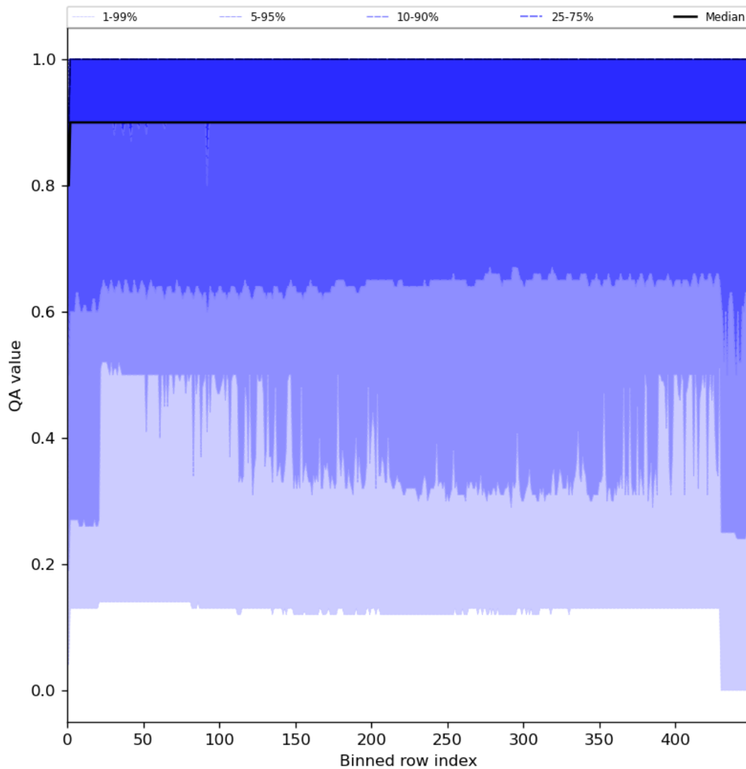
Figure 27: Along track statistics of “QA value” for 2024-03-14 to 2024-03-15
