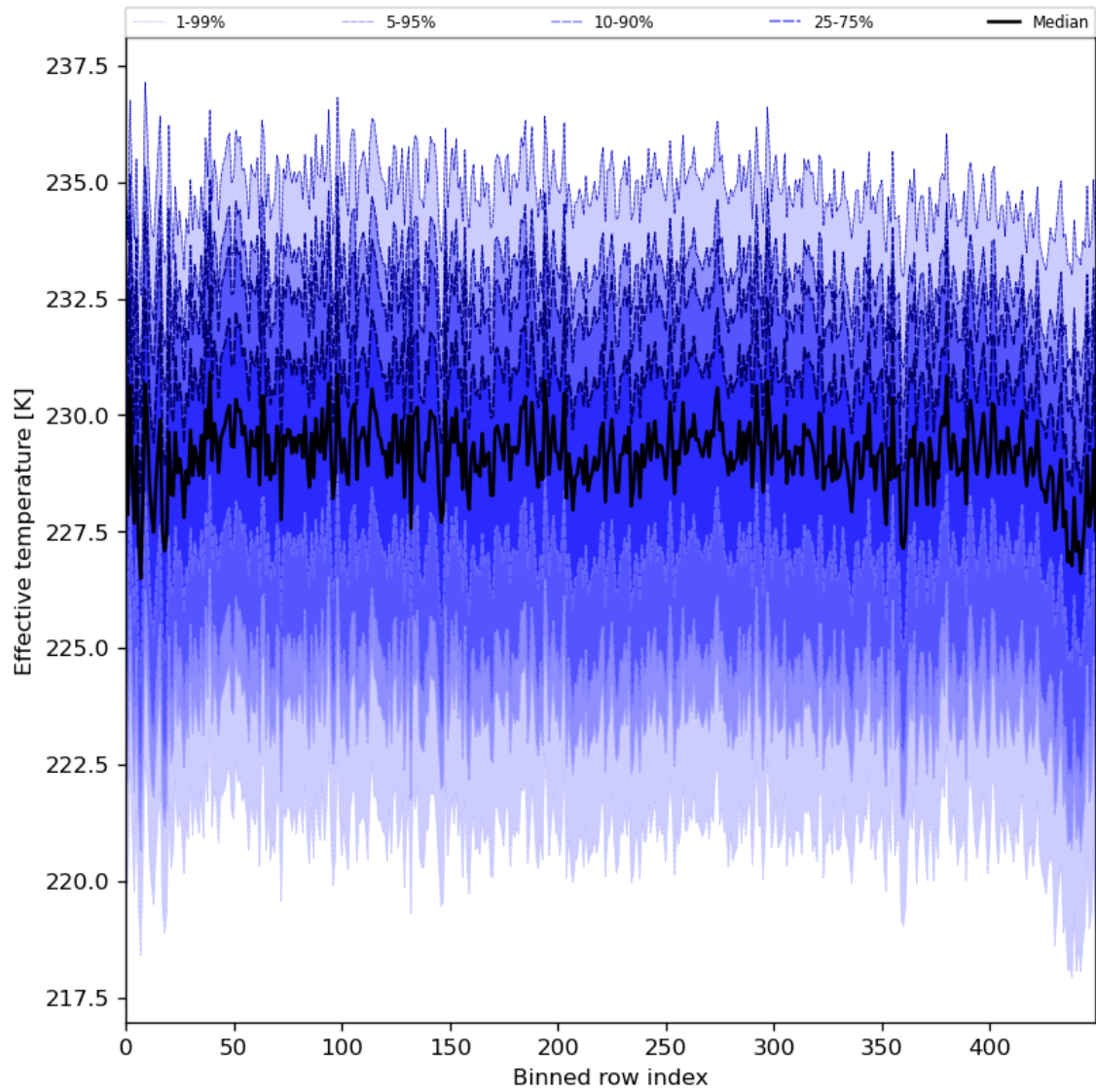
Figure 31: Along track statistics of “Effective temperature” for 2024-03-14 to 2024-03-15
