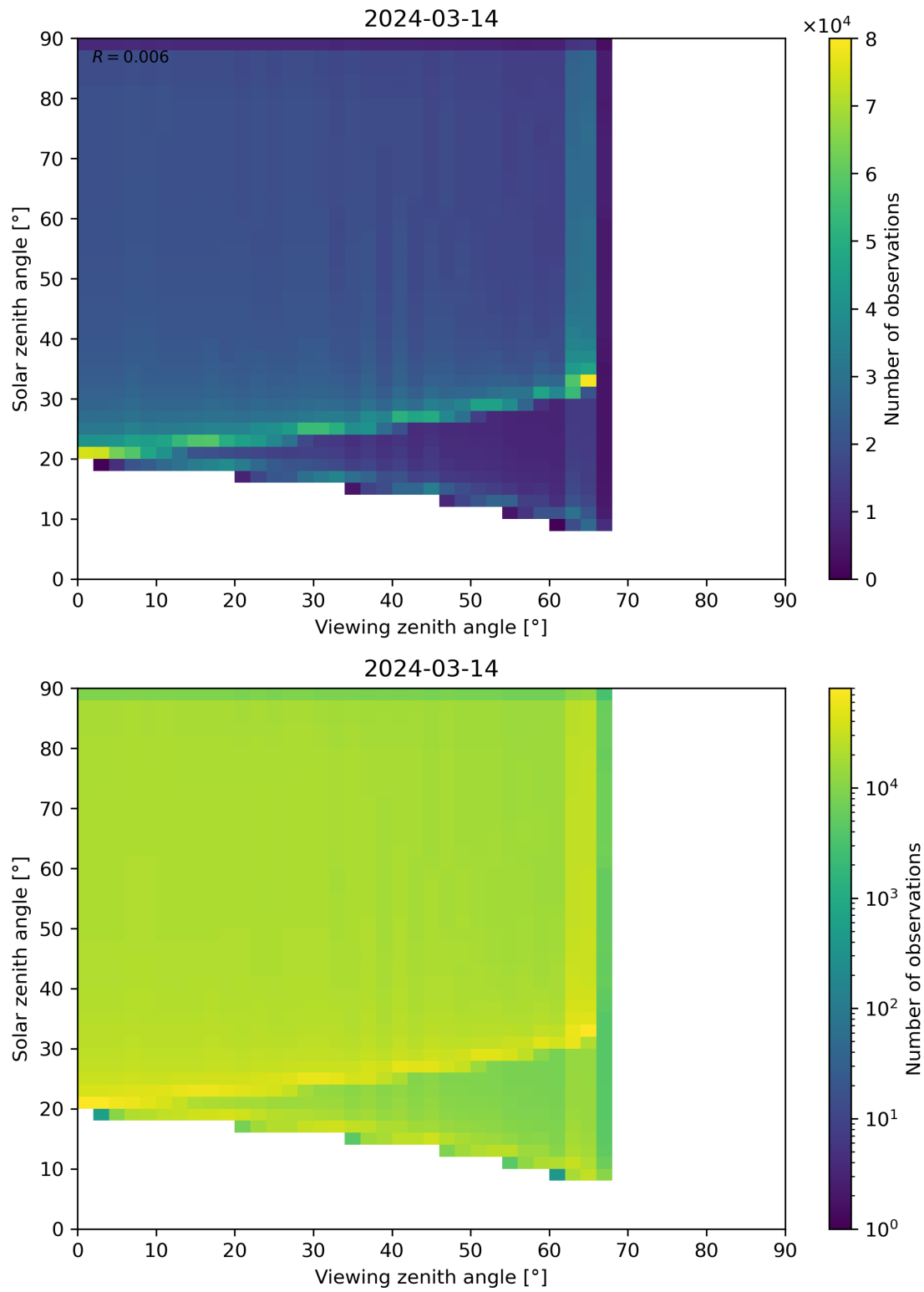
Figure 54: Scatter density plot of “Viewing zenith angle” against “Solar zenith angle” for 2024-03-14 to 2024-03-15.
