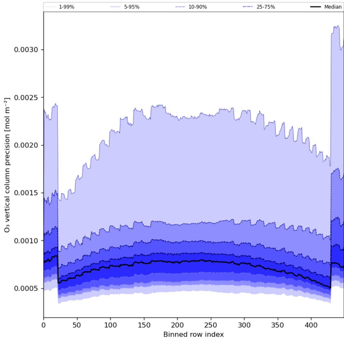
Figure 29: Along track statistics of “O 3 vertical column precision” for 2024-03-14 to 2024-03-15
