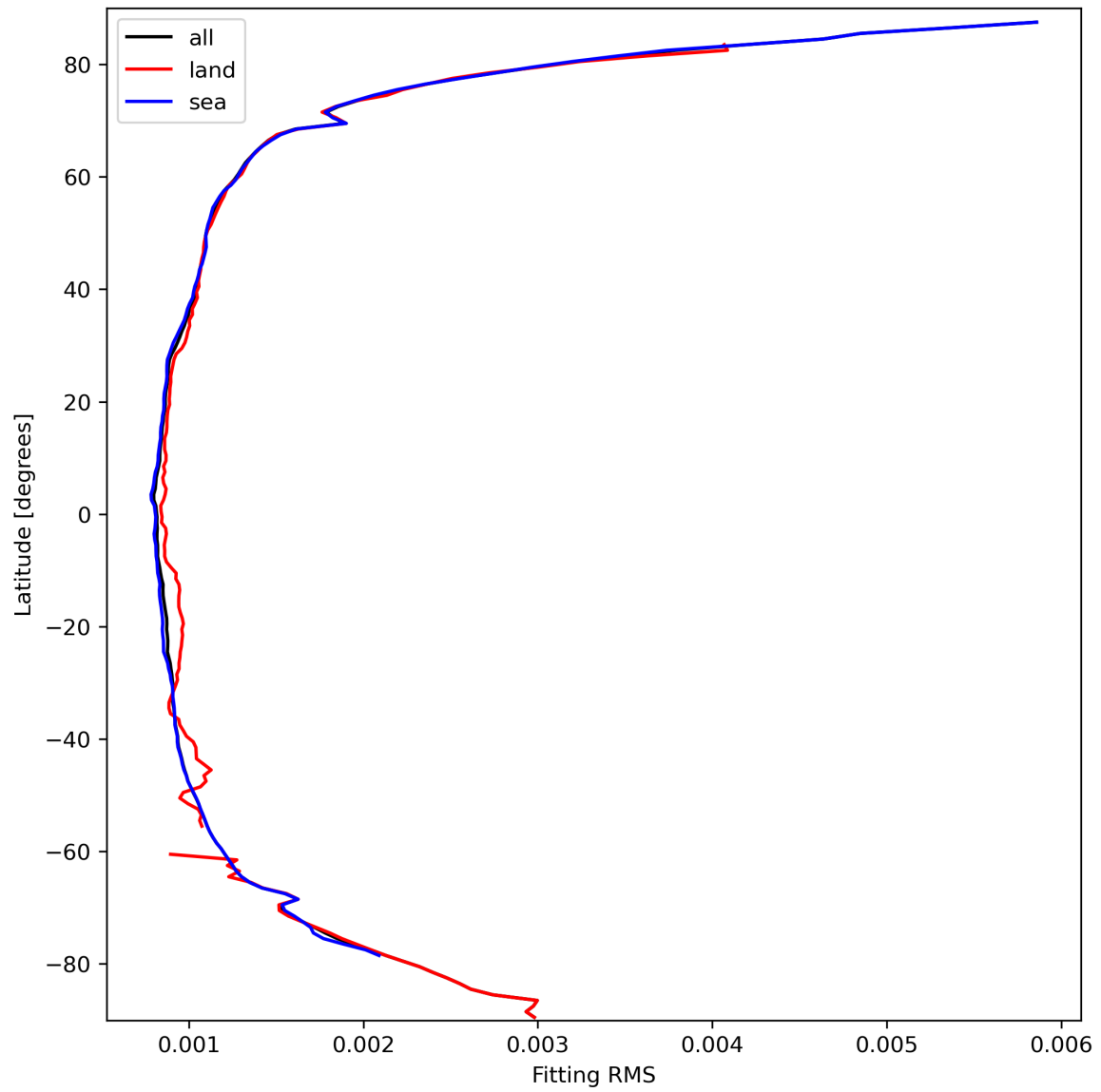
Figure 16: Zonal average of “Fitting RMS” for 2024-03-14 to 2024-03-15.
