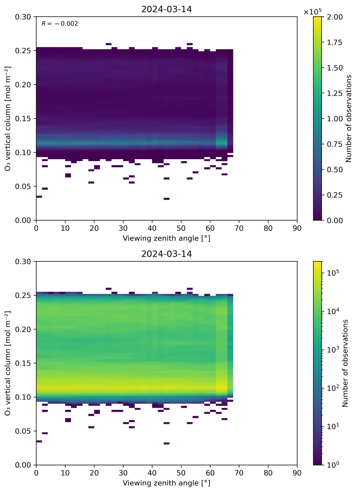
Figure 52: Scatter density plot of “Viewing zenith angle” against “O 3 vertical column” for 2024-03-14 to 2024-03-15.
