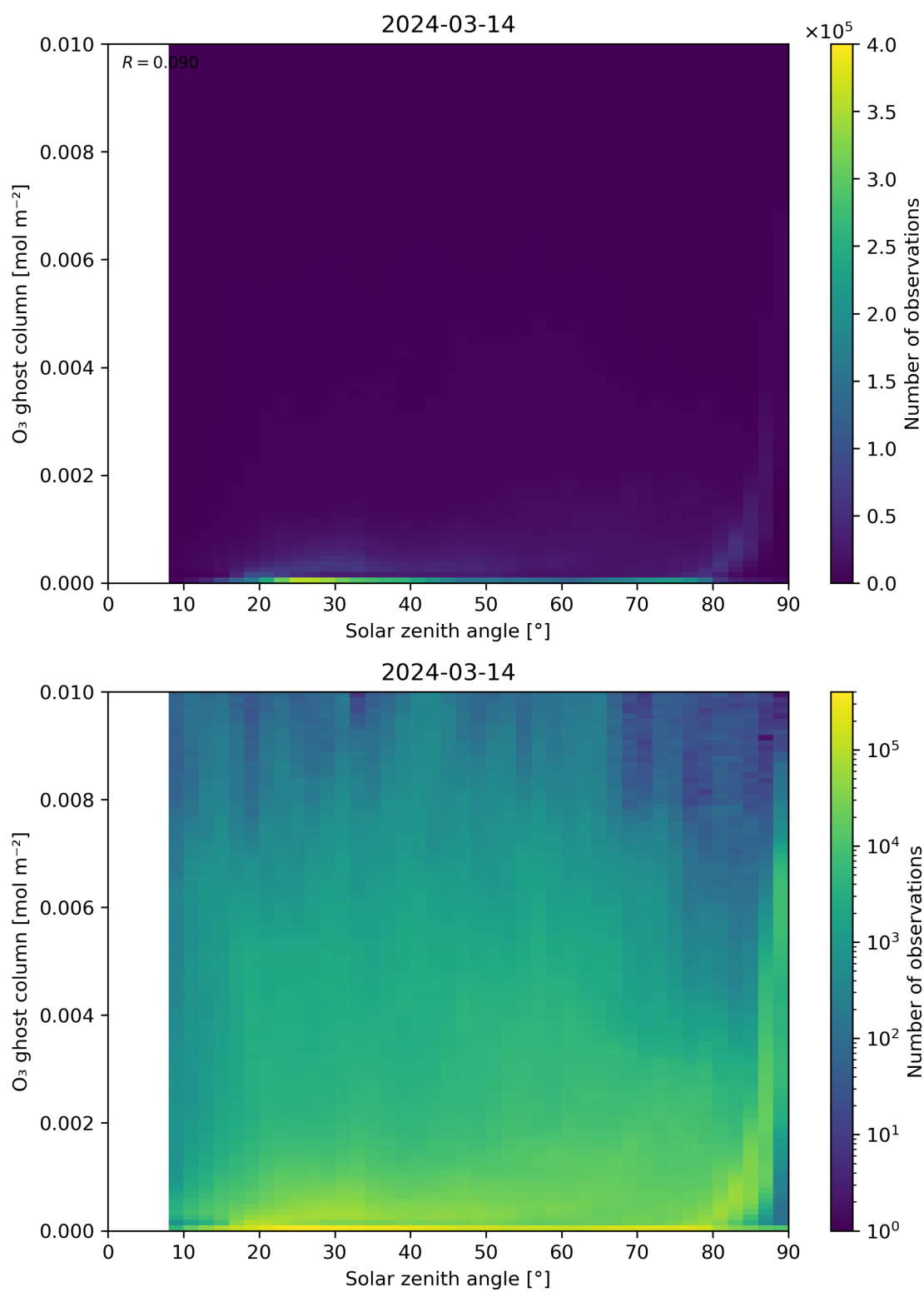
Figure 46: Scatter density plot of “Solar zenith angle” against “O 3 ghost column” for 2024-03-14 to 2024-03-15.
