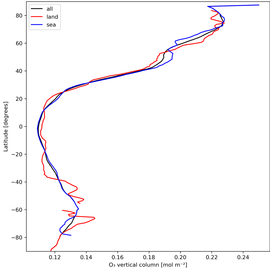
Figure 14: Zonal average of “O 3 vertical column” for 2024-03-14 to 2024-03-15.
