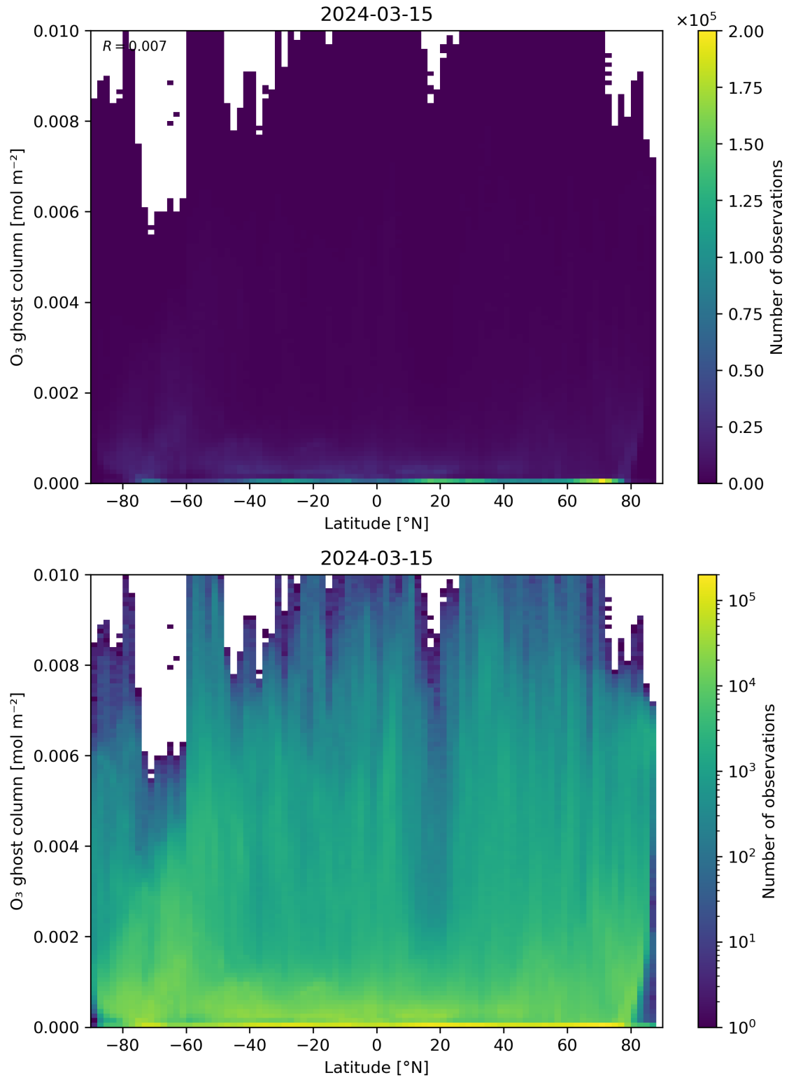
Figure 35: Scatter density plot of “Latitude” against “O 3 ghost column” for 2024-03-14 to 2024-03-16.
