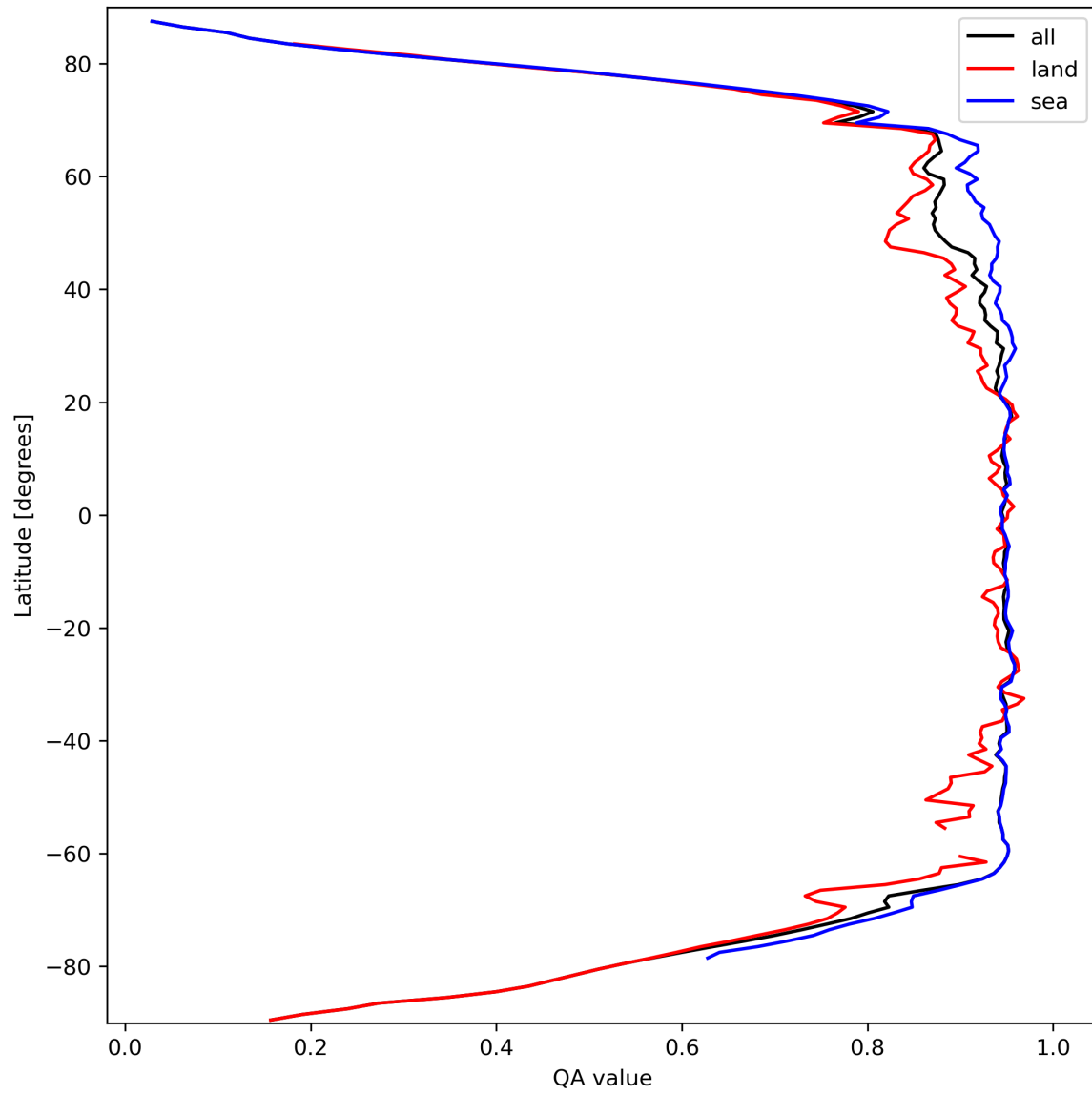
Figure 13: Zonal average of “QA value” for 2024-03-14 to 2024-03-16.
