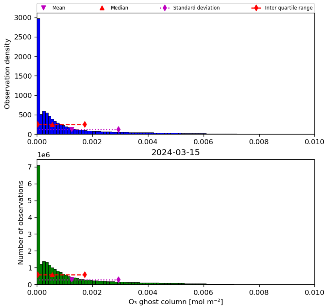
Figure 25: Histogram of “O 3 ghost column” for 2024-03-14 to 2024-03-16
