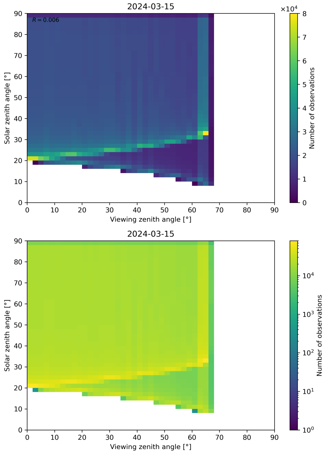
Figure 54: Scatter density plot of “Viewing zenith angle” against “Solar zenith angle” for 2024-03-14 to 2024-03-16.
