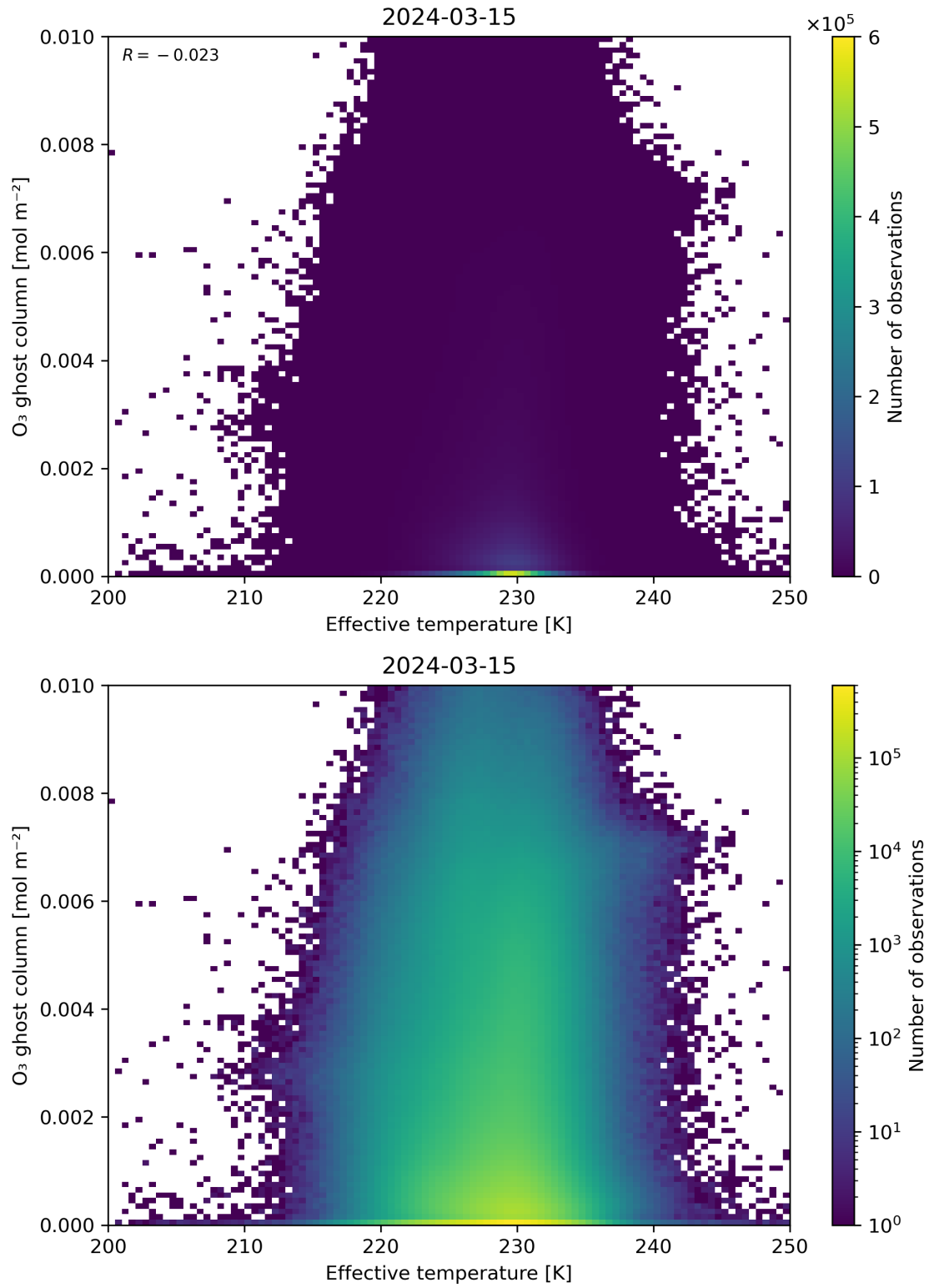
Figure 38: Scatter density plot of “Effective temperature” against “O 3 ghost column” for 2024-03-14 to 2024-03-16.
