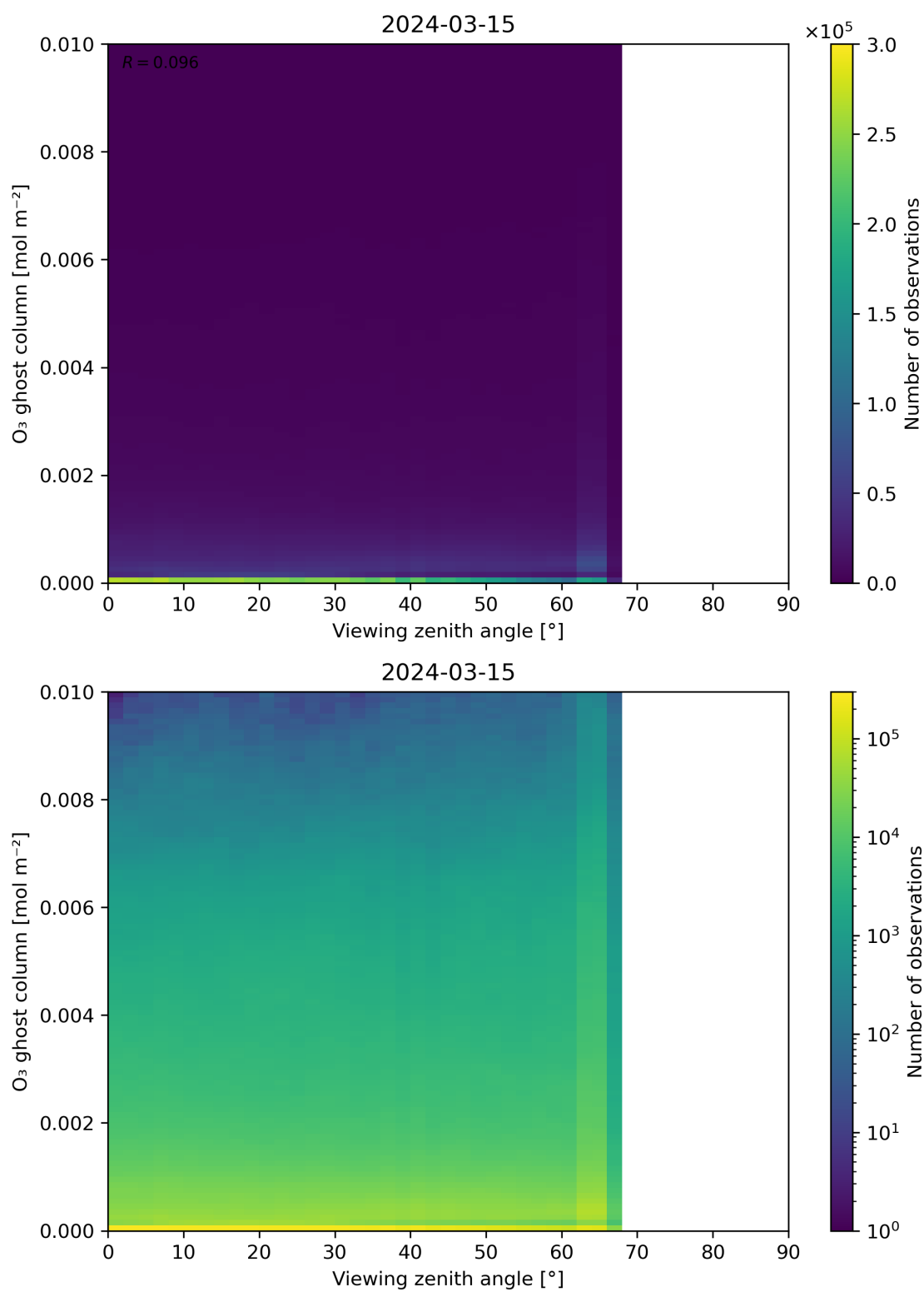
Figure 51: Scatter density plot of “Viewing zenith angle” against “O 3 ghost column” for 2024-03-14 to 2024-03-16.
