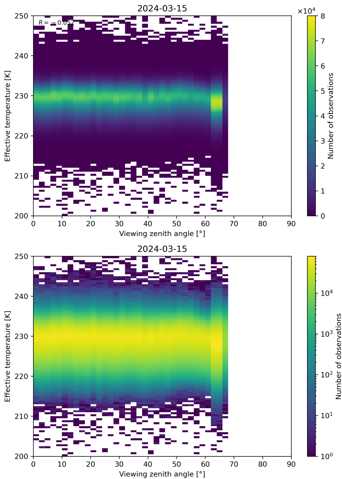
Figure 50: Scatter density plot of “Viewing zenith angle” against “Effective temperature” for 2024-03-14 to 2024-03-16.
