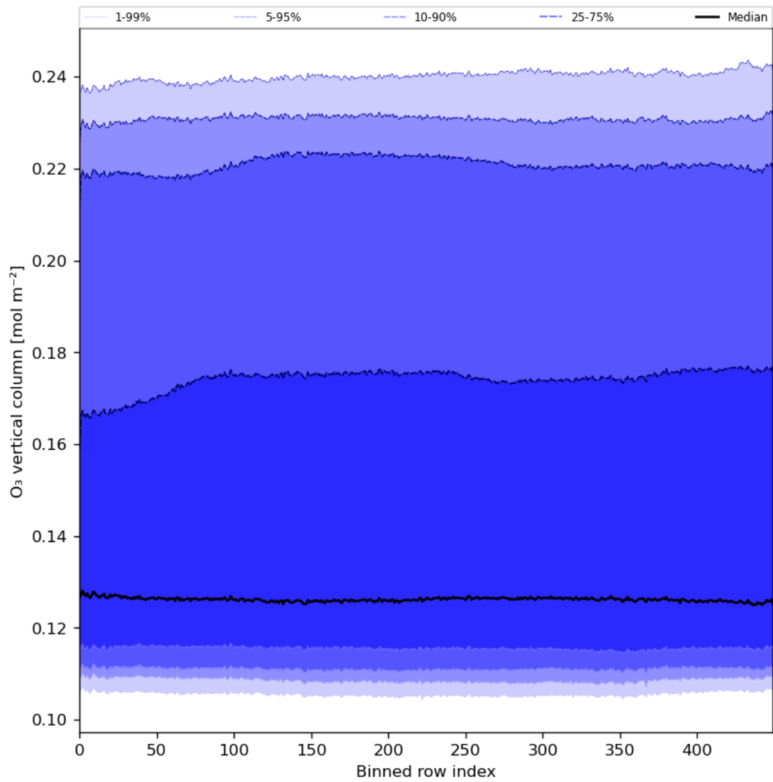
Figure 28: Along track statistics of “O 3 vertical column” for 2024-03-14 to 2024-03-16
