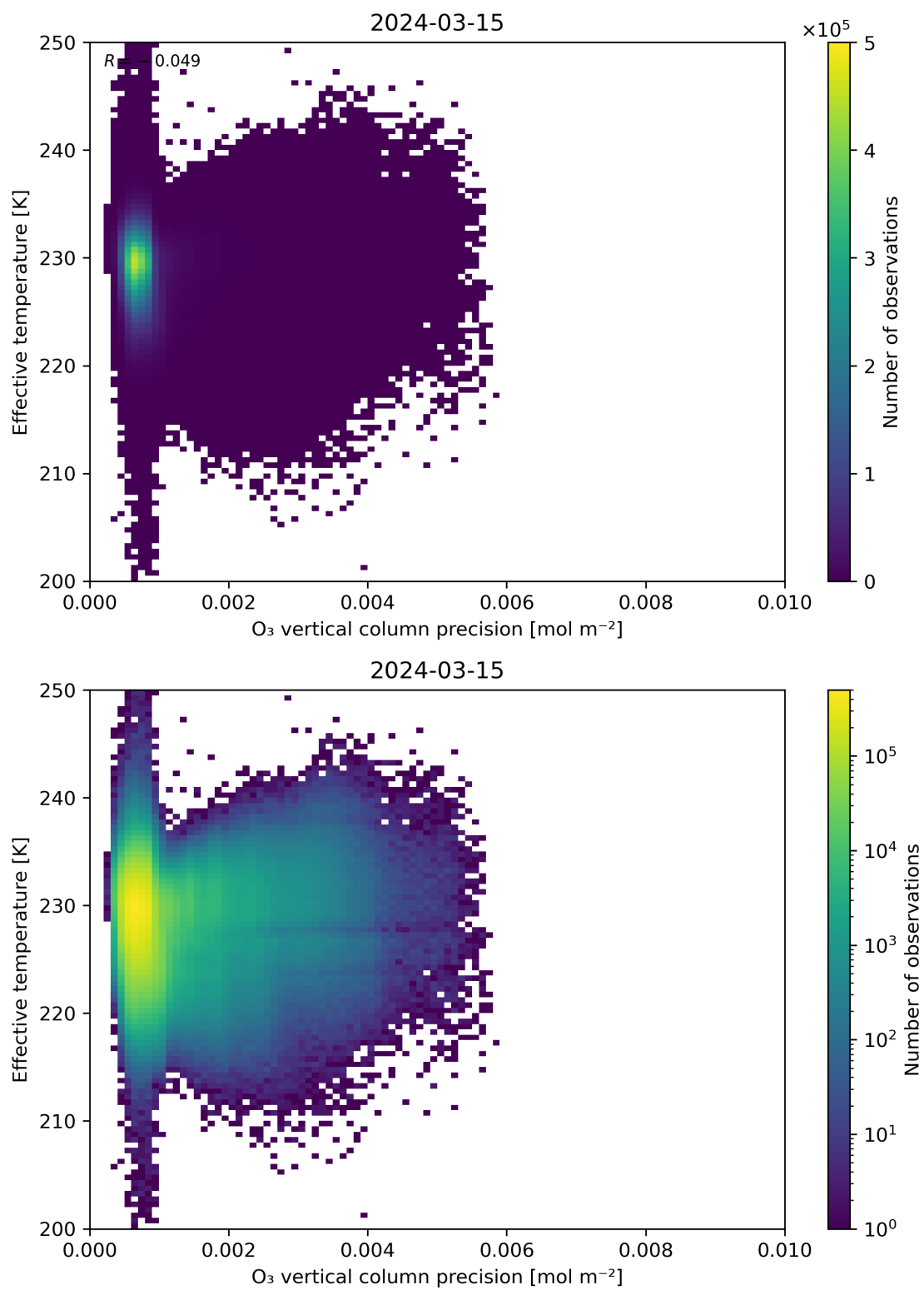
Figure 42: Scatter density plot of “O 3 vertical column precision” against “Effective temperature” for 2024-03-14 to 2024-03-16.
