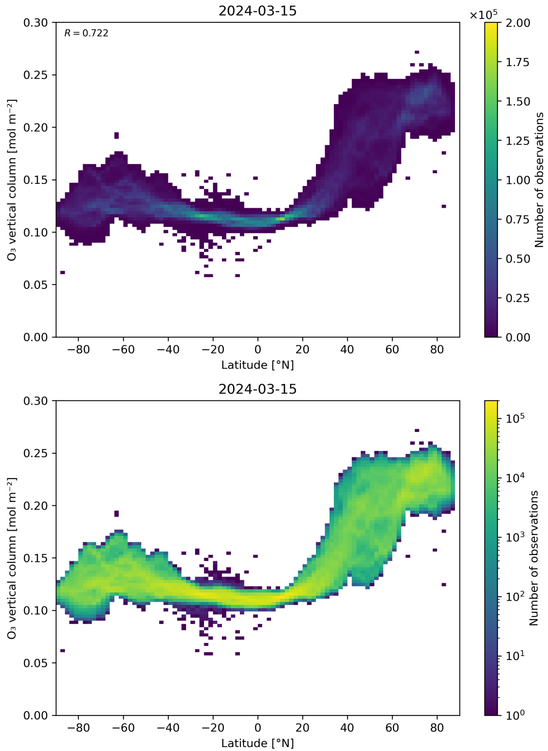
Figure 36: Scatter density plot of “Latitude” against “O 3 vertical column” for 2024-03-14 to 2024-03-16.
