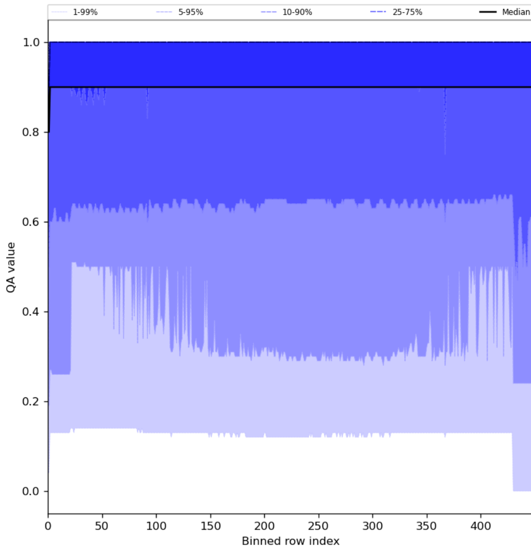
Figure 27: Along track statistics of “QA value” for 2024-03-14 to 2024-03-16
