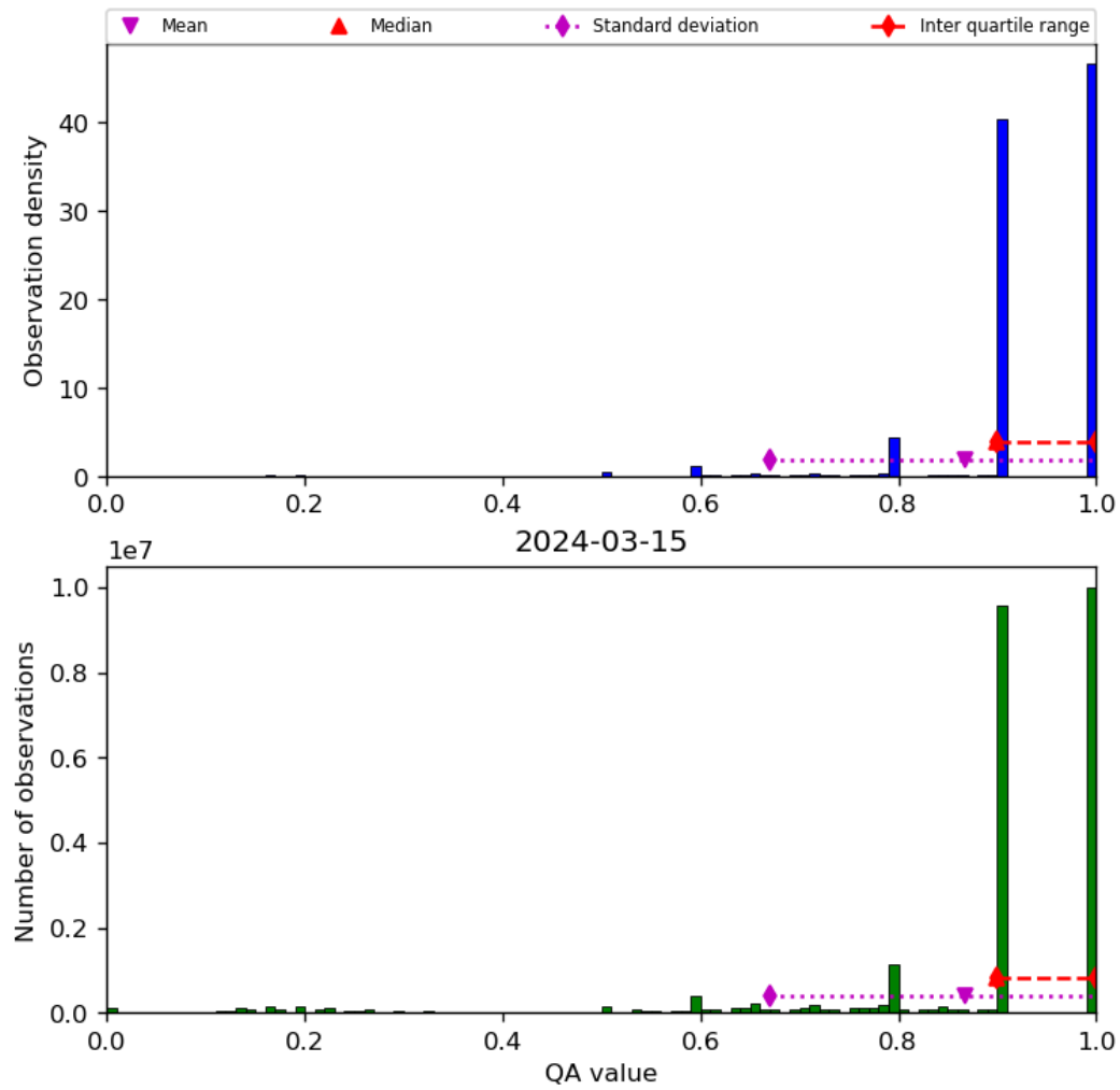
Figure 20: Histogram of “QA value” for 2024-03-14 to 2024-03-16
