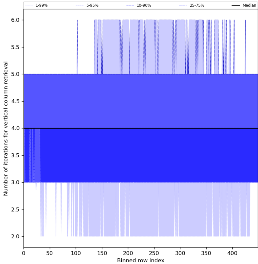
Figure 33: Along track statistics of “Number of iterations for vertical column retrieval” for 2024-03-14 to 2024-03-16
