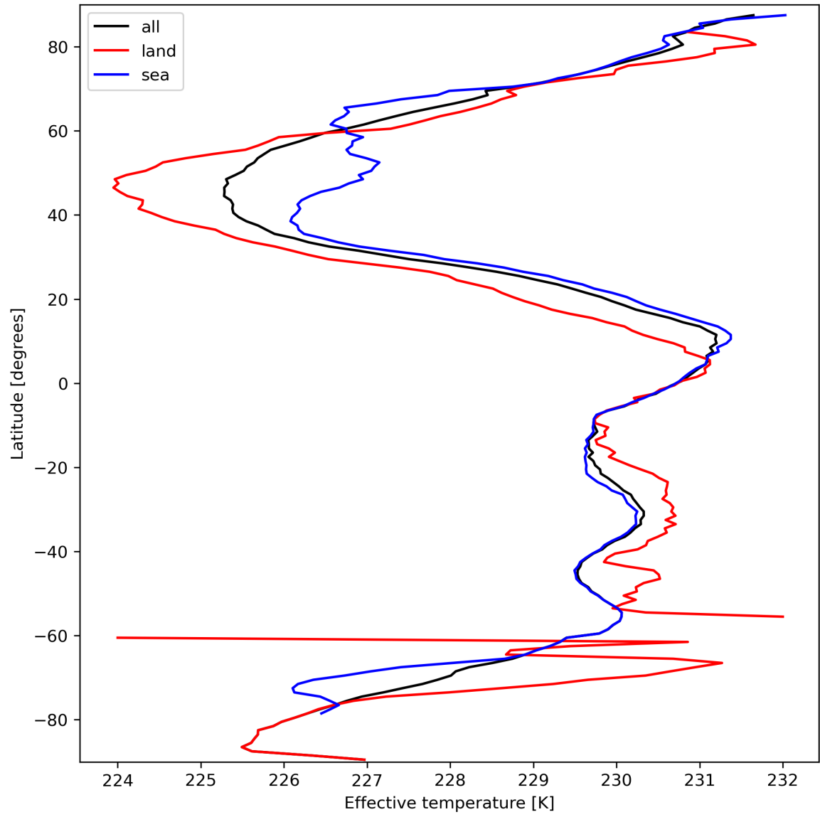
Figure 17: Zonal average of “Effective temperature” for 2024-03-14 to 2024-03-16.
