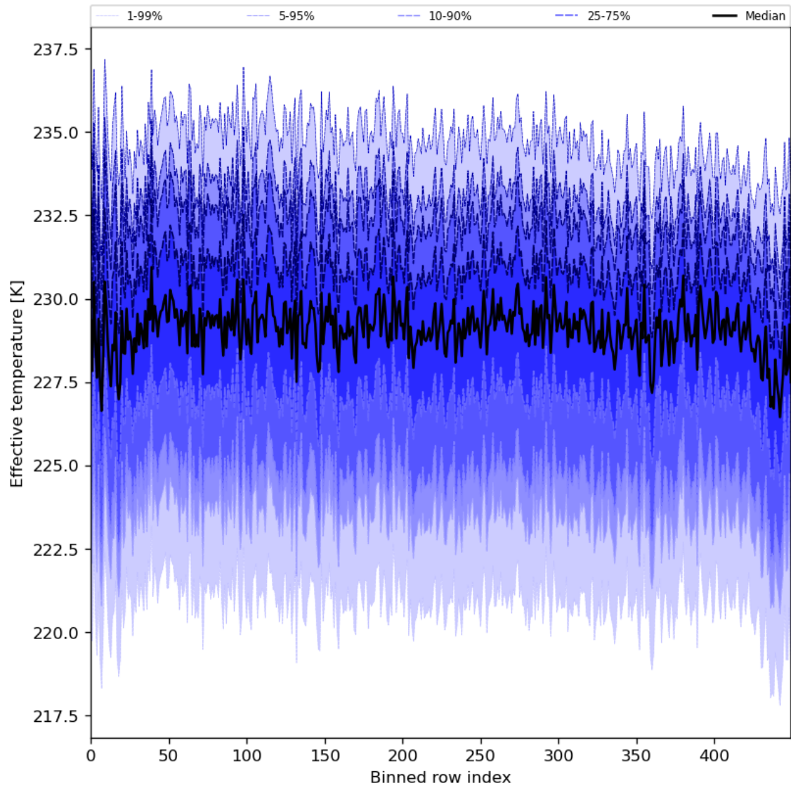
Figure 31: Along track statistics of “Effective temperature” for 2024-03-14 to 2024-03-16
