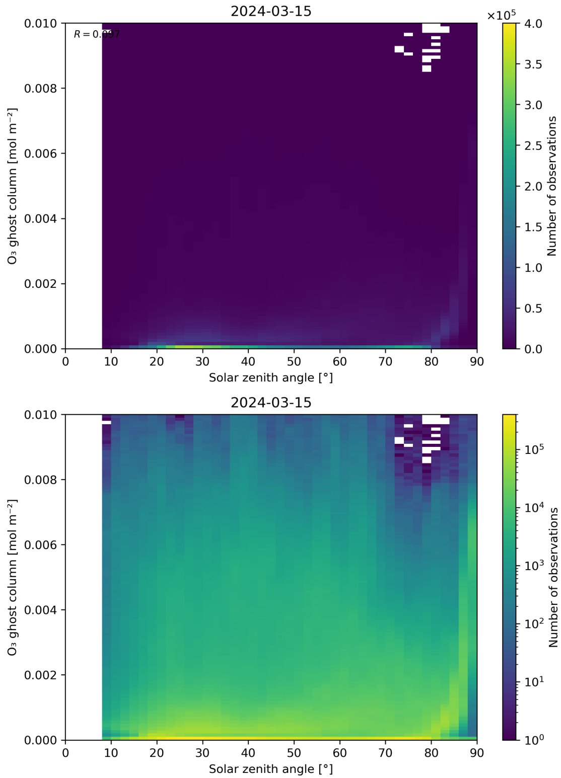
Figure 46: Scatter density plot of “Solar zenith angle” against “O 3 ghost column” for 2024-03-14 to 2024-03-16.
