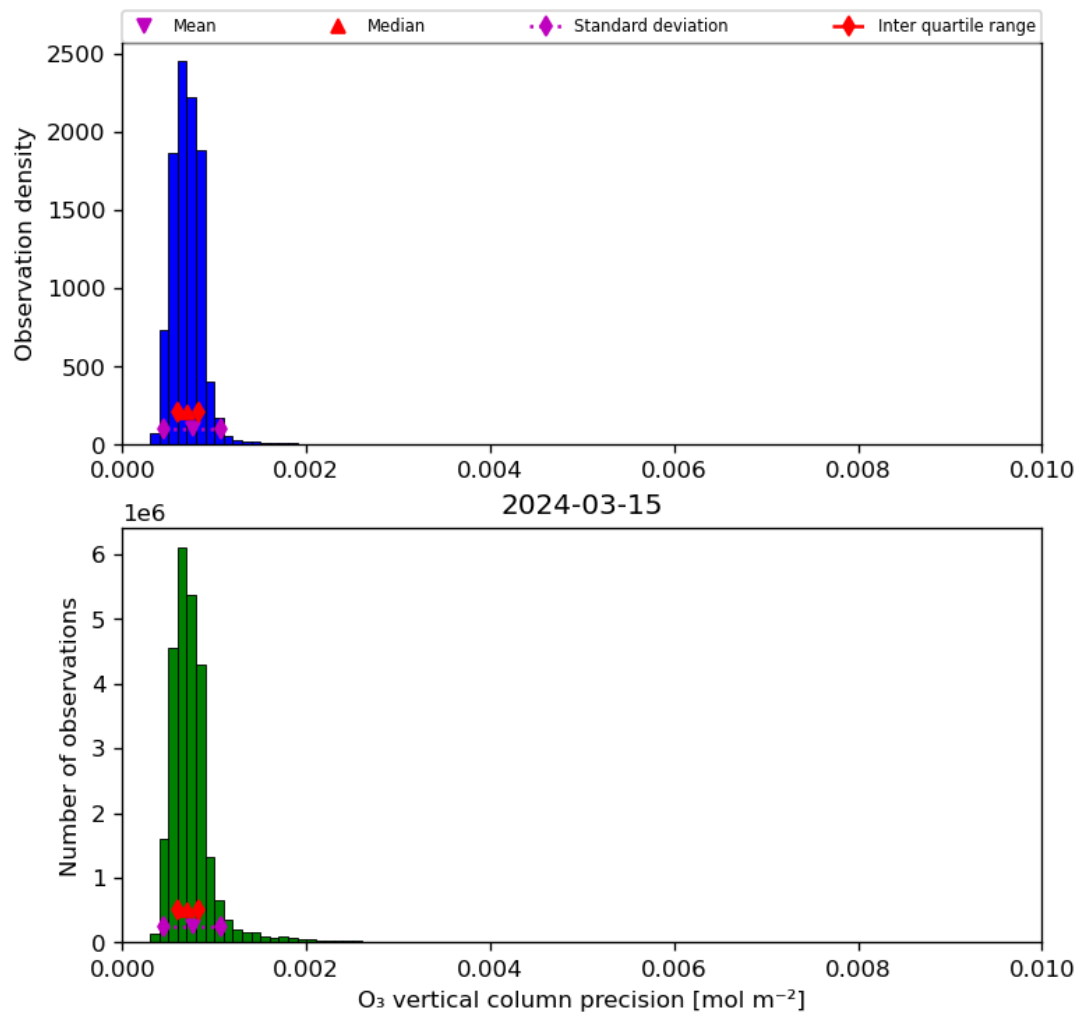
Figure 22: Histogram of “O 3 vertical column precision” for 2024-03-14 to 2024-03-16
