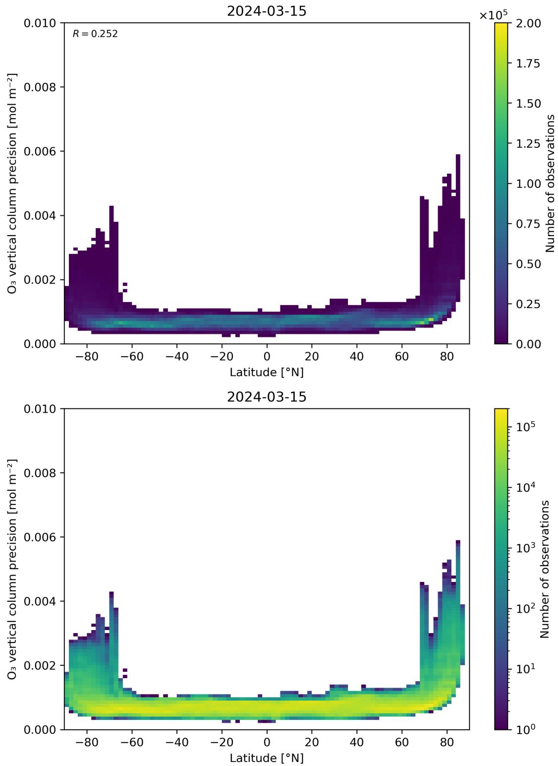
Figure 37: Scatter density plot of “Latitude” against “O 3 vertical column precision” for 2024-03-14 to 2024-03-16.
