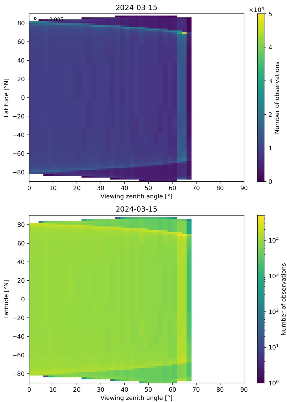
Figure 49: Scatter density plot of “Viewing zenith angle” against “Latitude” for 2024-03-14 to 2024-03-16.
