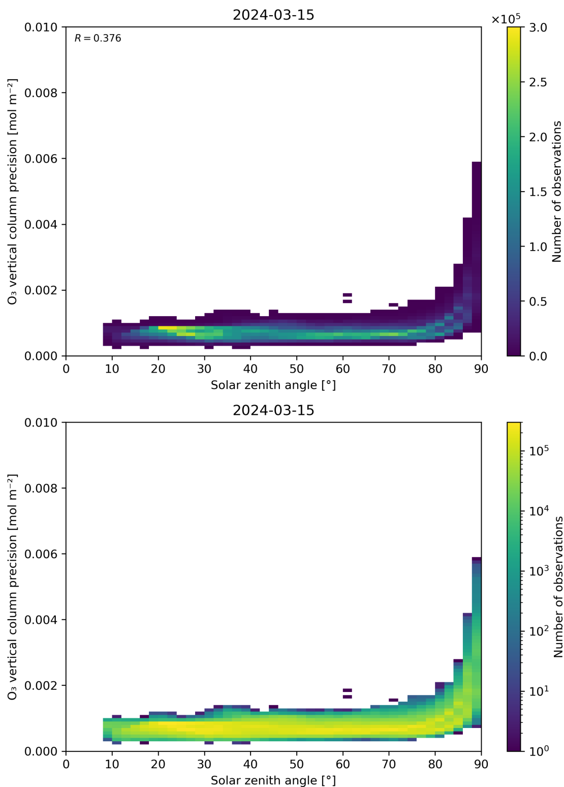
Figure 48: Scatter density plot of “Solar zenith angle” against “O 3 vertical column precision” for 2024-03-14 to 2024-03-16.
