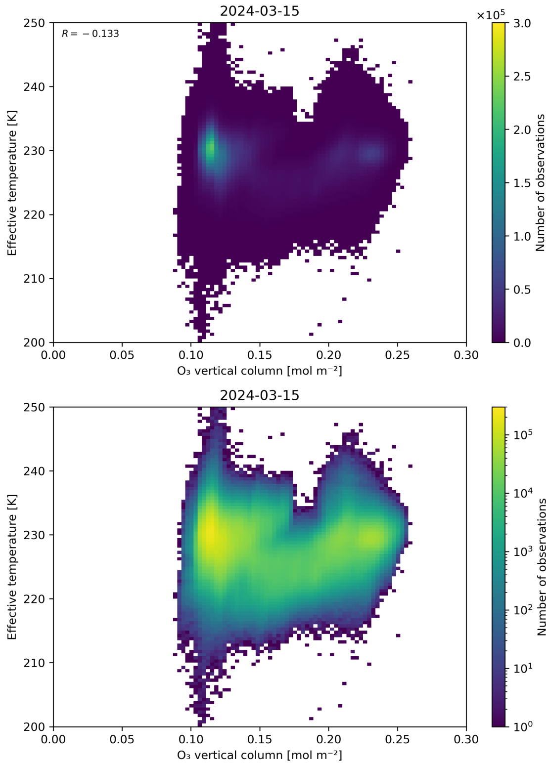
Figure 39: Scatter density plot of “O 3 vertical column” against “Effective temperature” for 2024-03-14 to 2024-03-16.
