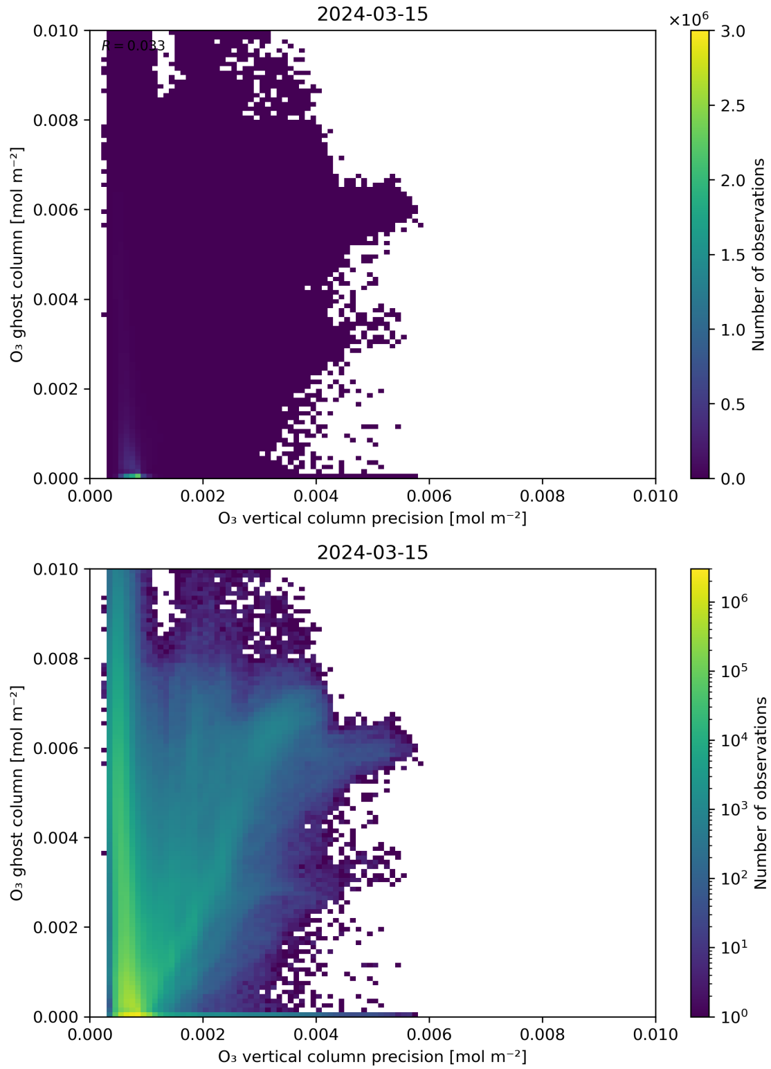
Figure 43: Scatter density plot of “O 3 vertical column precision” against “O 3 ghost column” for 2024-03-14 to 2024-03-16.
