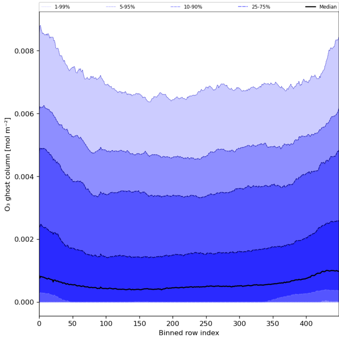
Figure 32: Along track statistics of “O 3 ghost column” for 2024-03-14 to 2024-03-16
