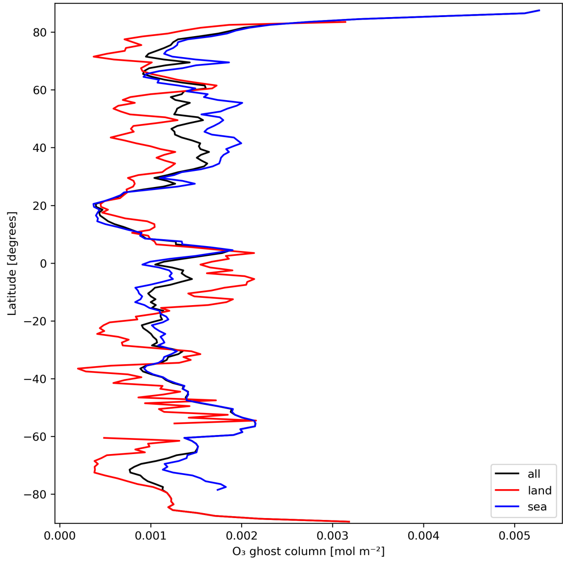
Figure 18: Zonal average of "O 3 ghost column" for 2024-03-14 to 2024-03-16.
