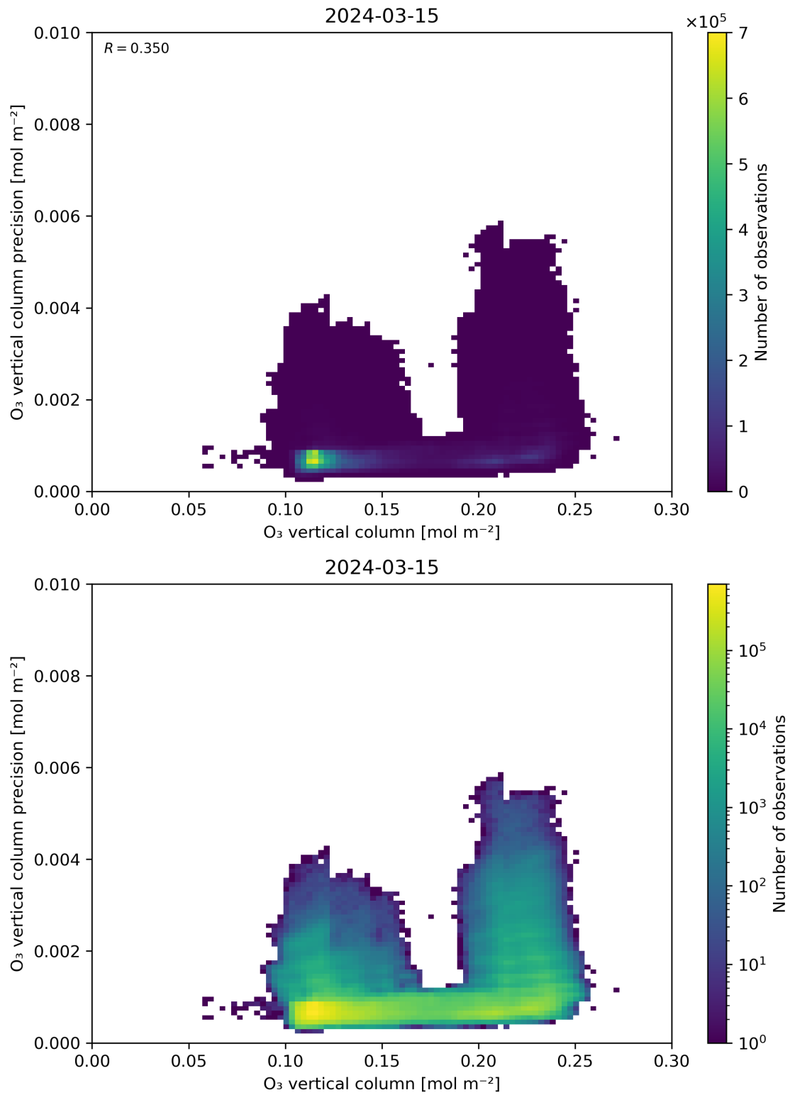
Figure 41: Scatter density plot of “O 3 vertical column” against “O 3 vertical column precision” for 2024-03-14 to 2024-03-16.
