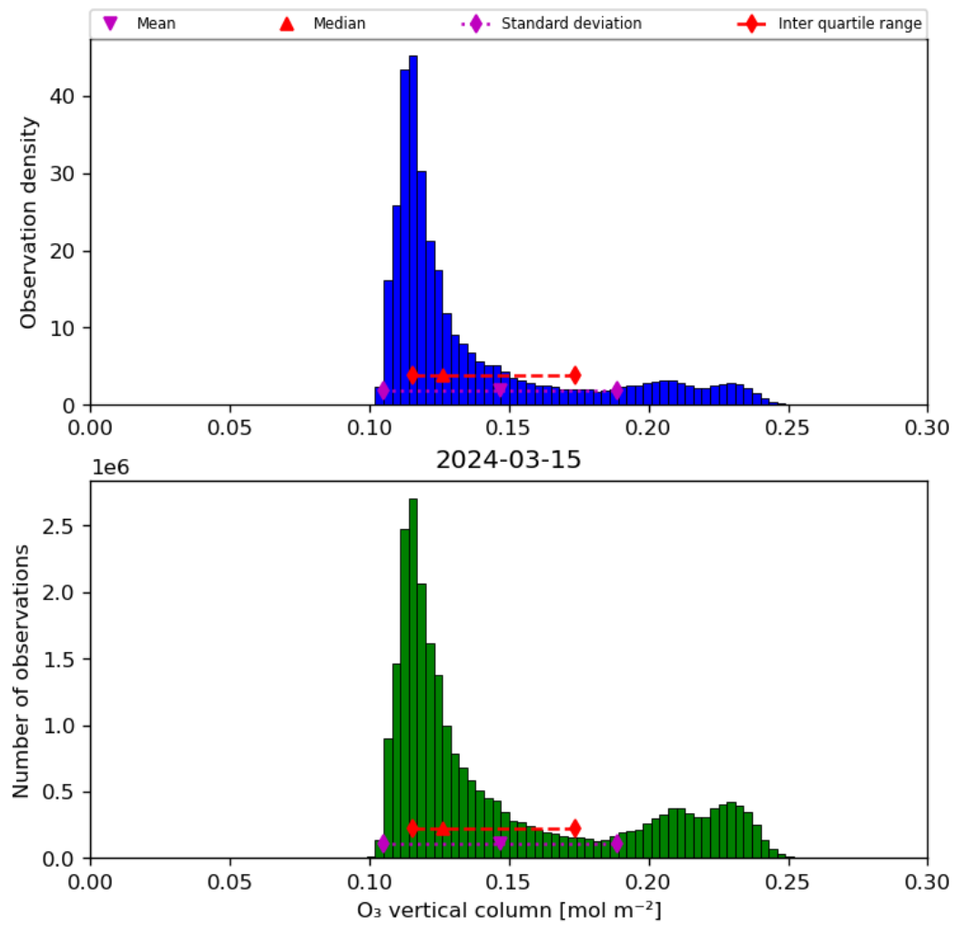
Figure 21: Histogram of “O 3 vertical column” for 2024-03-14 to 2024-03-16
