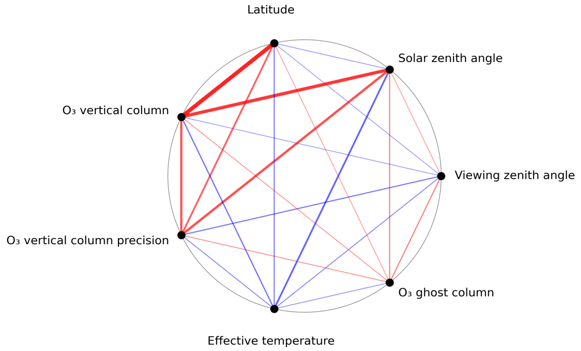
Figure 1: Map of correlation graph for 2024-03-14 to 2024-03-16.
