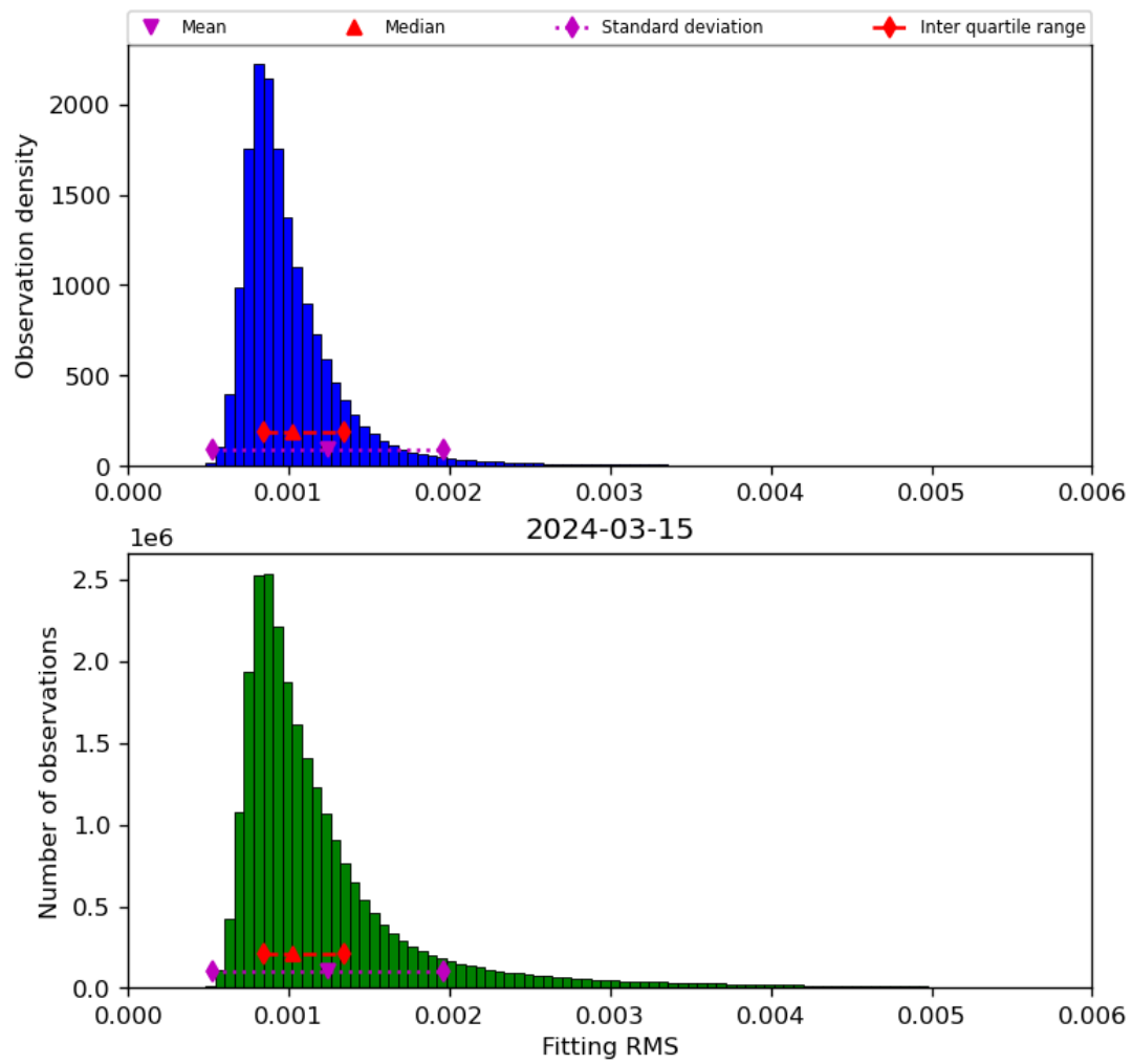
Figure 23: Histogram of “Fitting RMS” for 2024-03-14 to 2024-03-16
