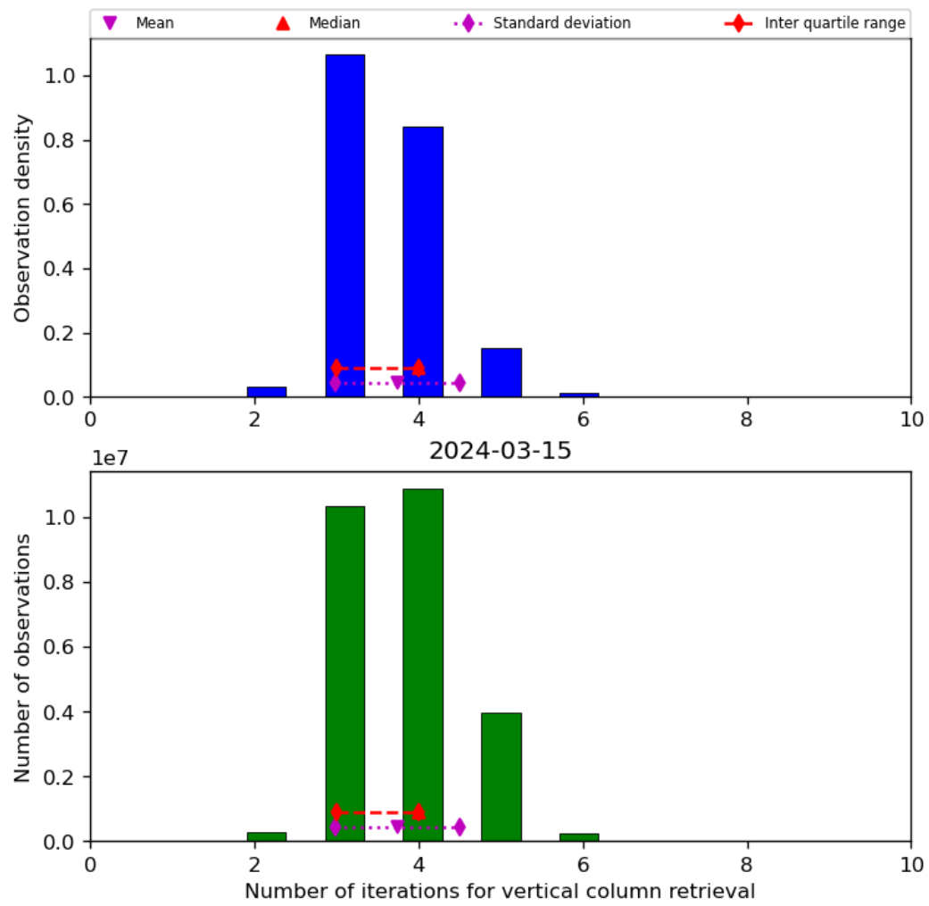
Figure 26: Histogram of “Number of iterations for vertical column retrieval” for 2024-03-14 to 2024-03-16
