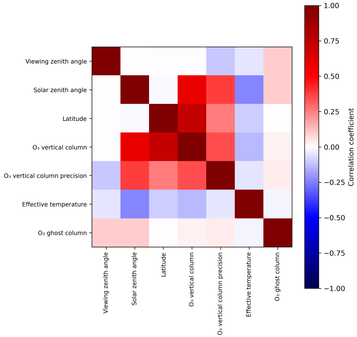
Figure 2: Map of correlation matrix for 2024-03-14 to 2024-03-16.
