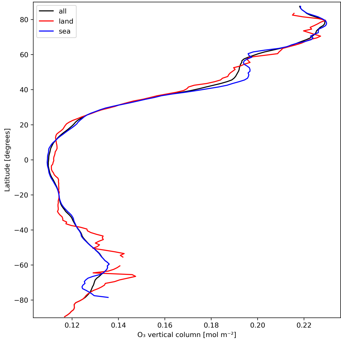
Figure 14: Zonal average of “O 3 vertical column” for 2024-03-14 to 2024-03-16.
