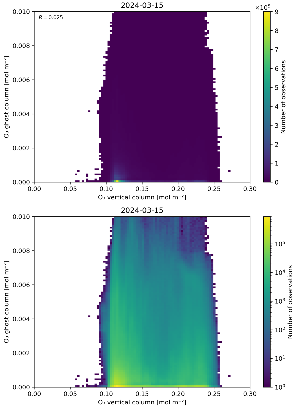
Figure 40: Scatter density plot of “O 3 vertical column” against “O 3 ghost column” for 2024-03-14 to 2024-03-16.
