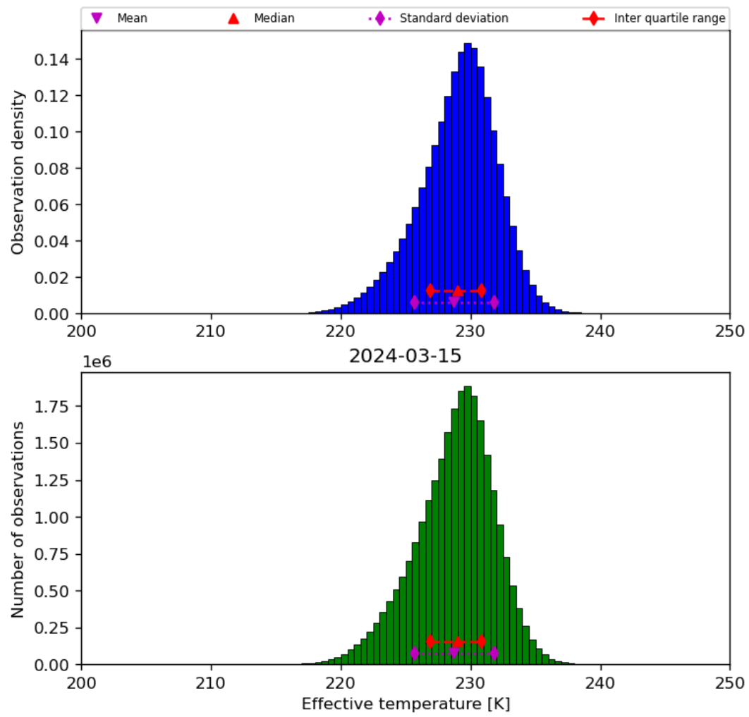
Figure 24: Histogram of “Effective temperature” for 2024-03-14 to 2024-03-16
