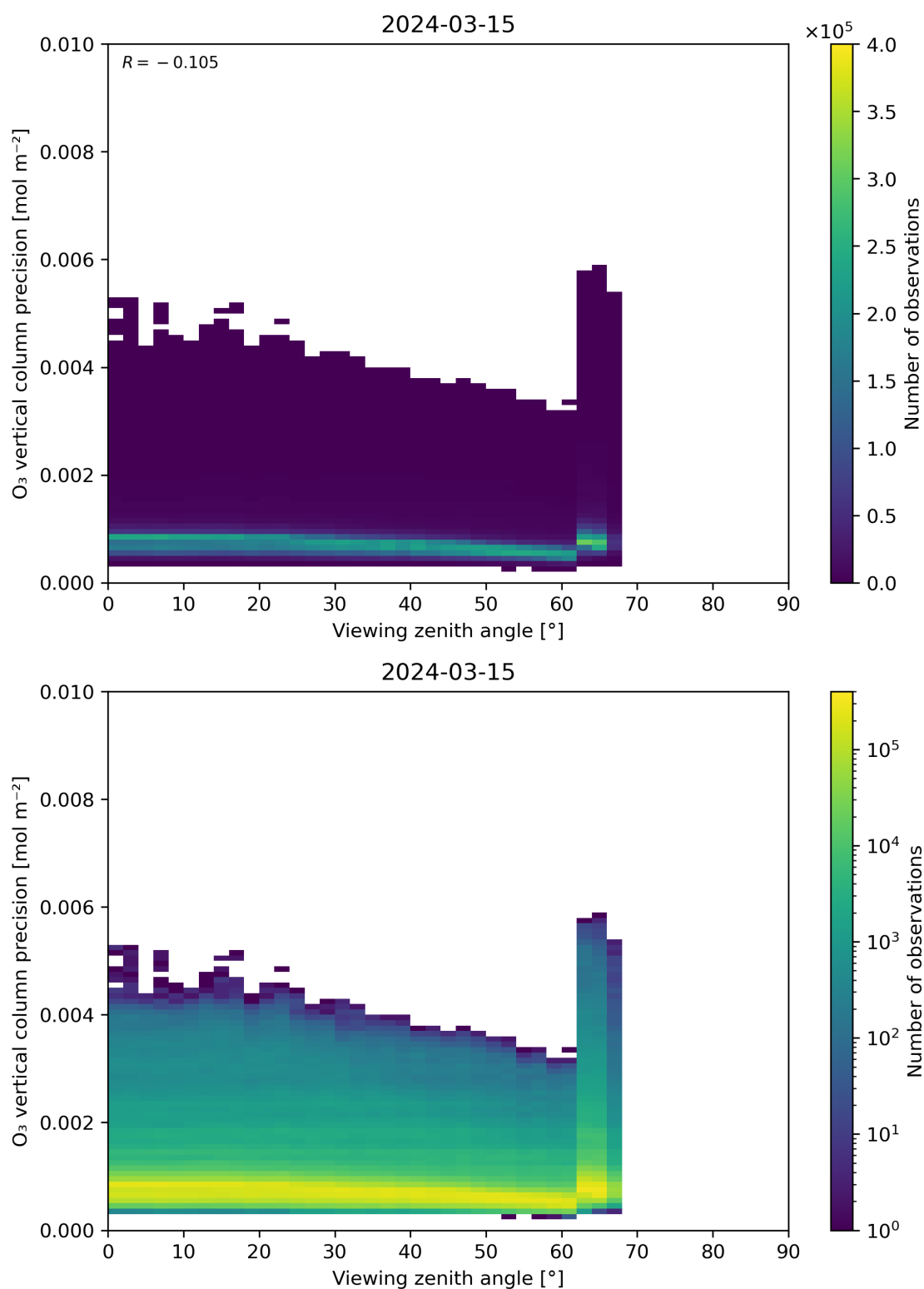
Figure 53: Scatter density plot of “Viewing zenith angle” against “O 3 vertical column precision” for 2024-03-14 to 2024-03-16.
