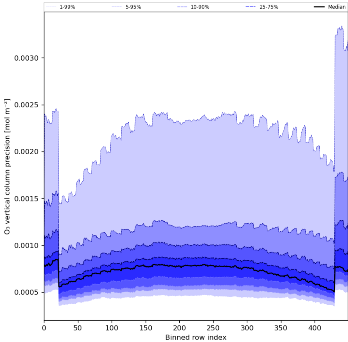
Figure 29: Along track statistics of “O 3 vertical column precision” for 2024-03-14 to 2024-03-16
