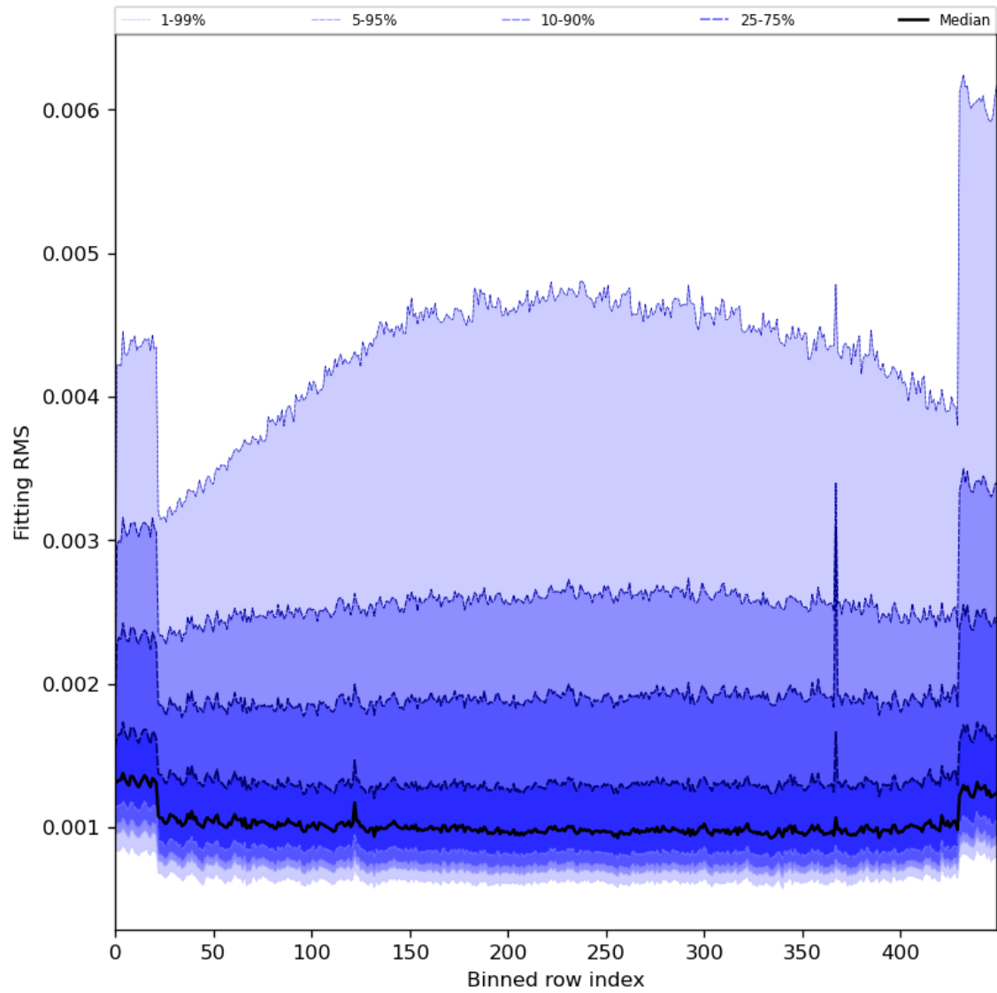
Figure 30: Along track statistics of “Fitting RMS” for 2024-03-14 to 2024-03-16
