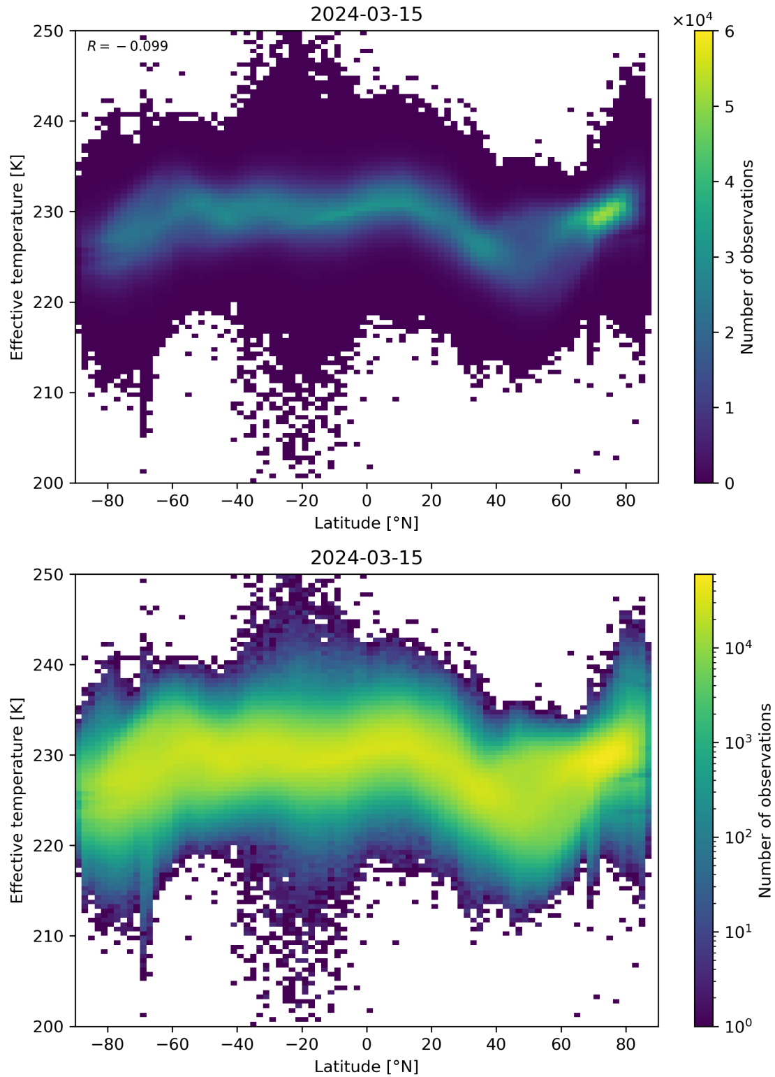
Figure 34: Scatter density plot of “Latitude” against “Effective temperature” for 2024-03-14 to 2024-03-16.
