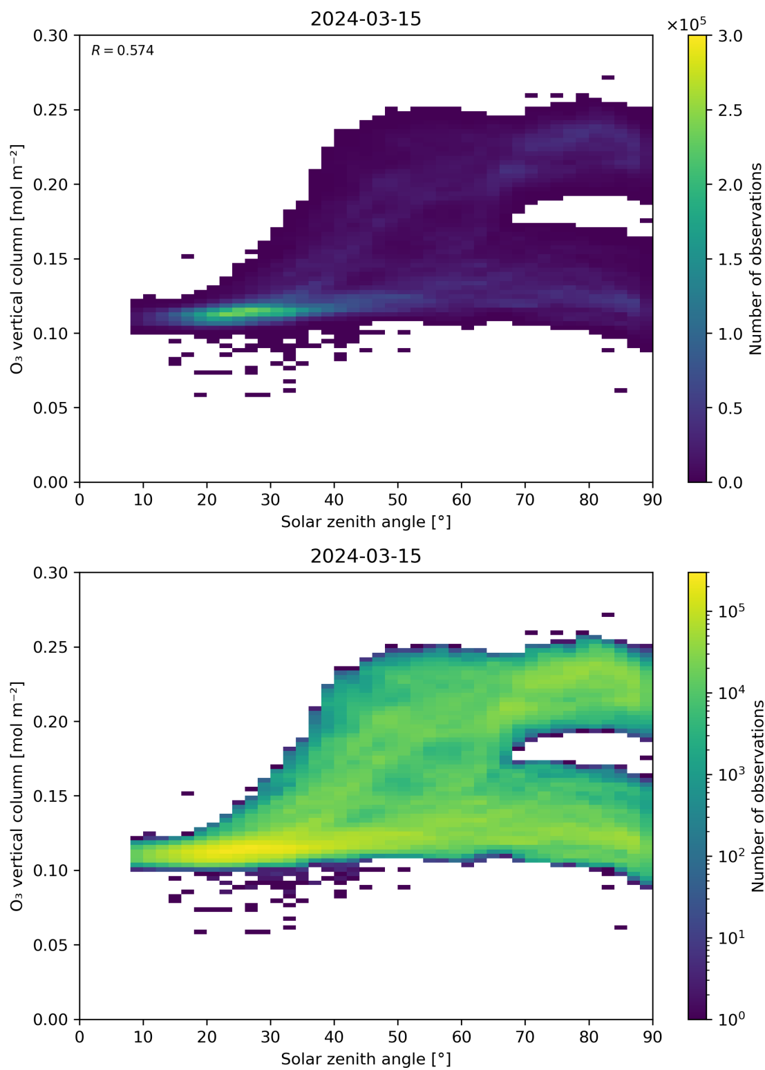
Figure 47: Scatter density plot of “Solar zenith angle” against “O 3 vertical column” for 2024-03-14 to 2024-03-16.
