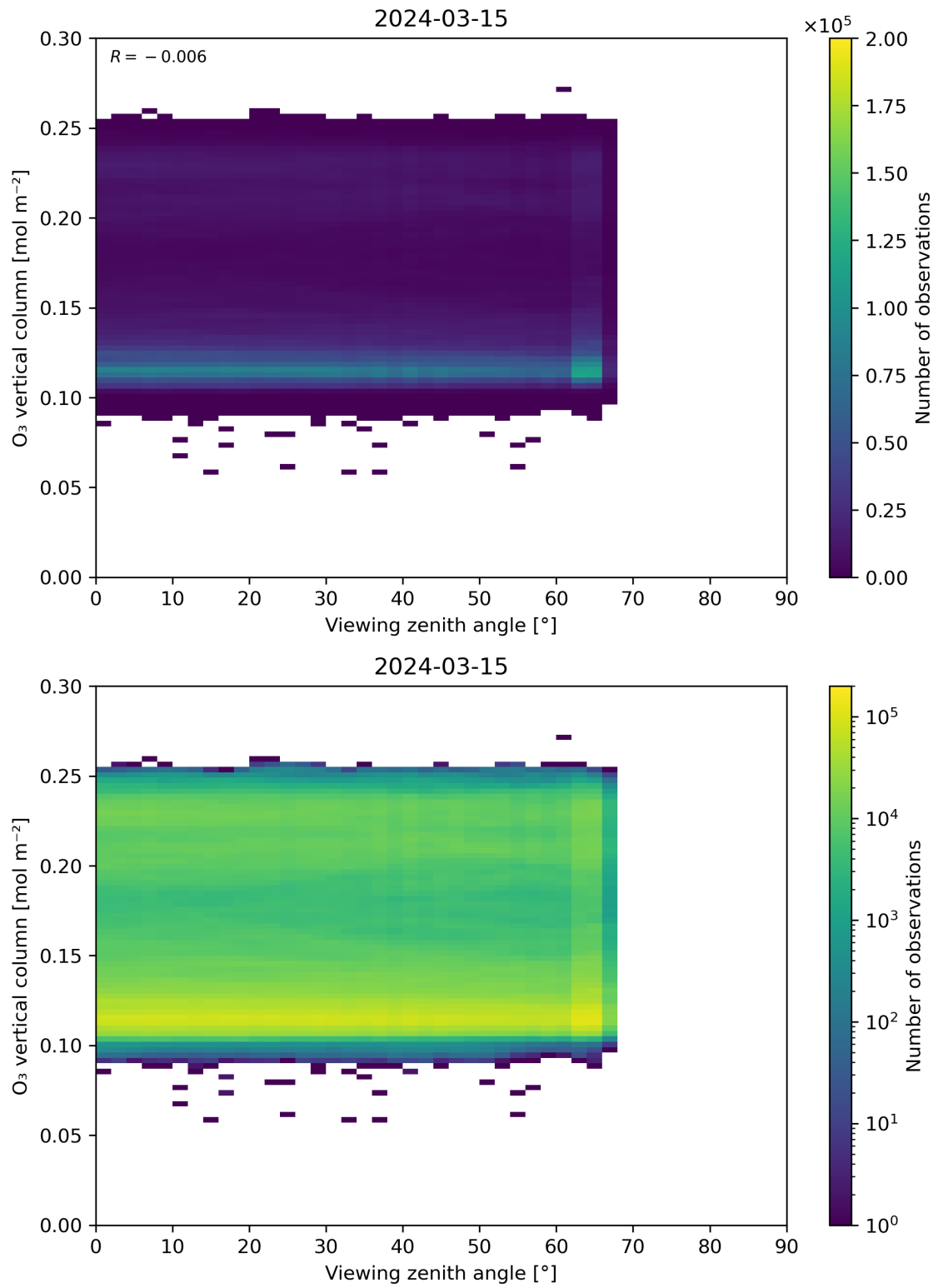
Figure 52: Scatter density plot of “Viewing zenith angle” against “O 3 vertical column” for 2024-03-14 to 2024-03-16.
