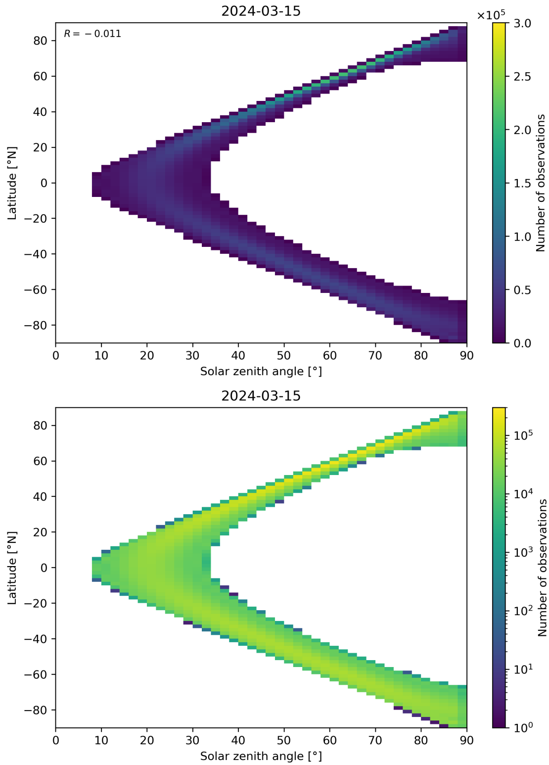
Figure 44: Scatter density plot of “Solar zenith angle” against “Latitude” for 2024-03-14 to 2024-03-16.
