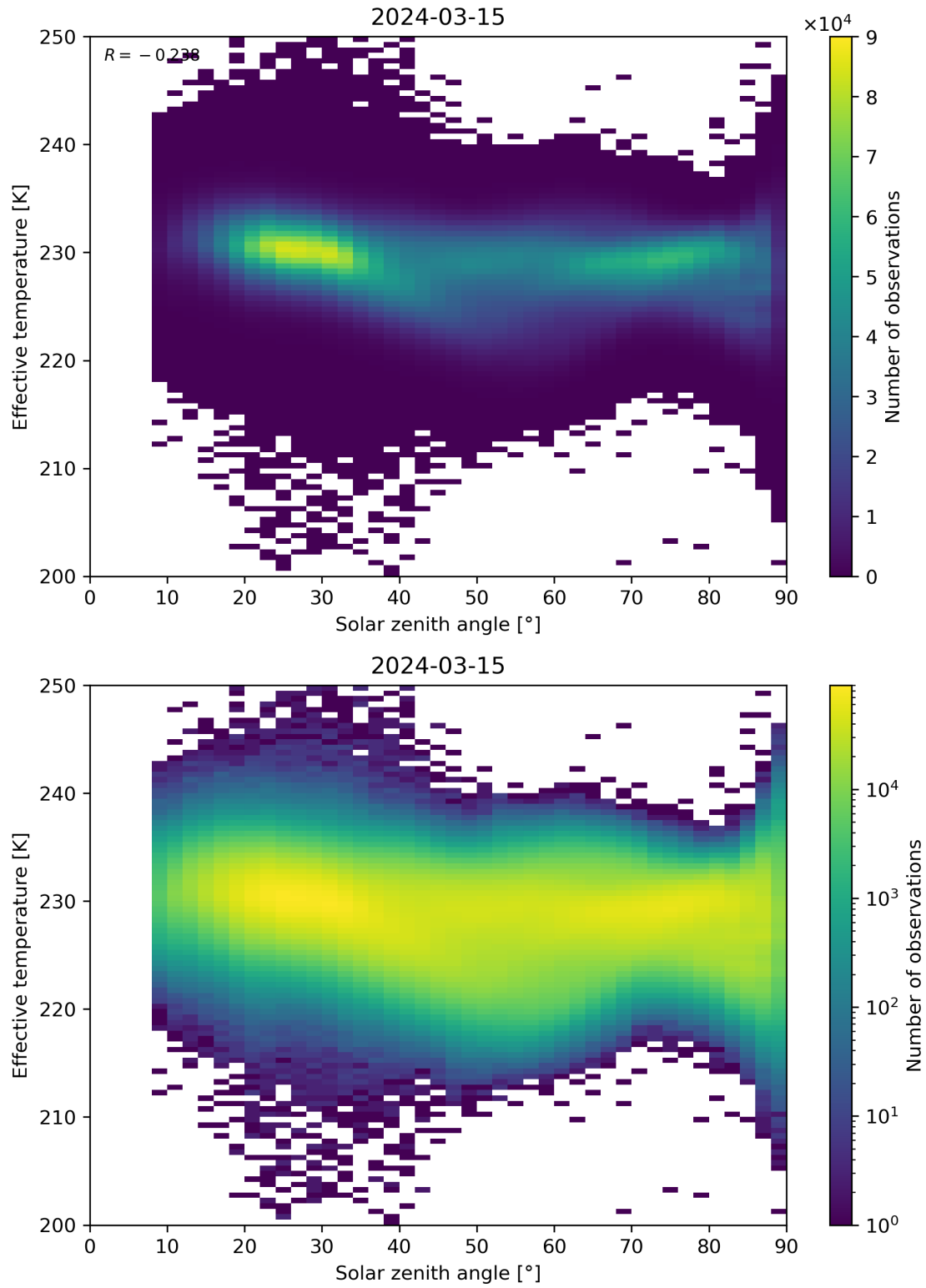
Figure 45: Scatter density plot of “Solar zenith angle” against “Effective temperature” for 2024-03-14 to 2024-03-16.
