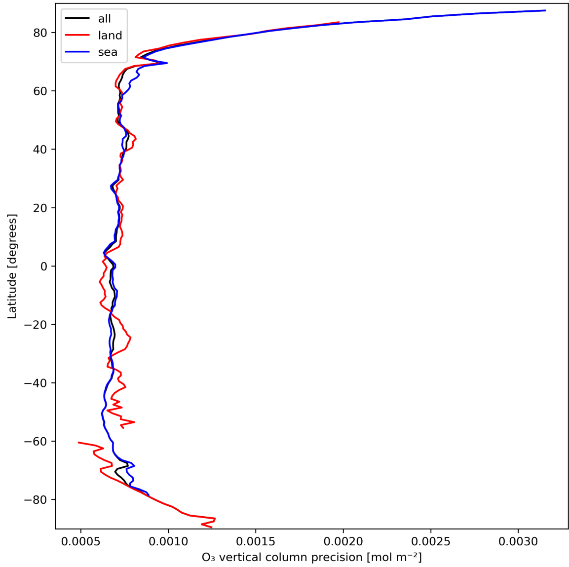
Figure 15: Zonal average of “O 3 vertical column precision” for 2024-03-14 to 2024-03-16.
