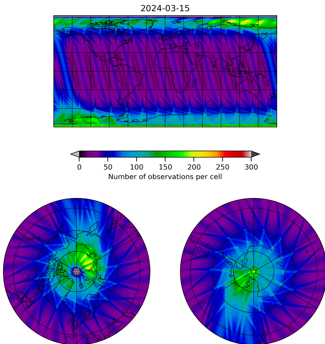
Figure 12: Map of the number of observations for 2024-03-14 to 2024-03-16
