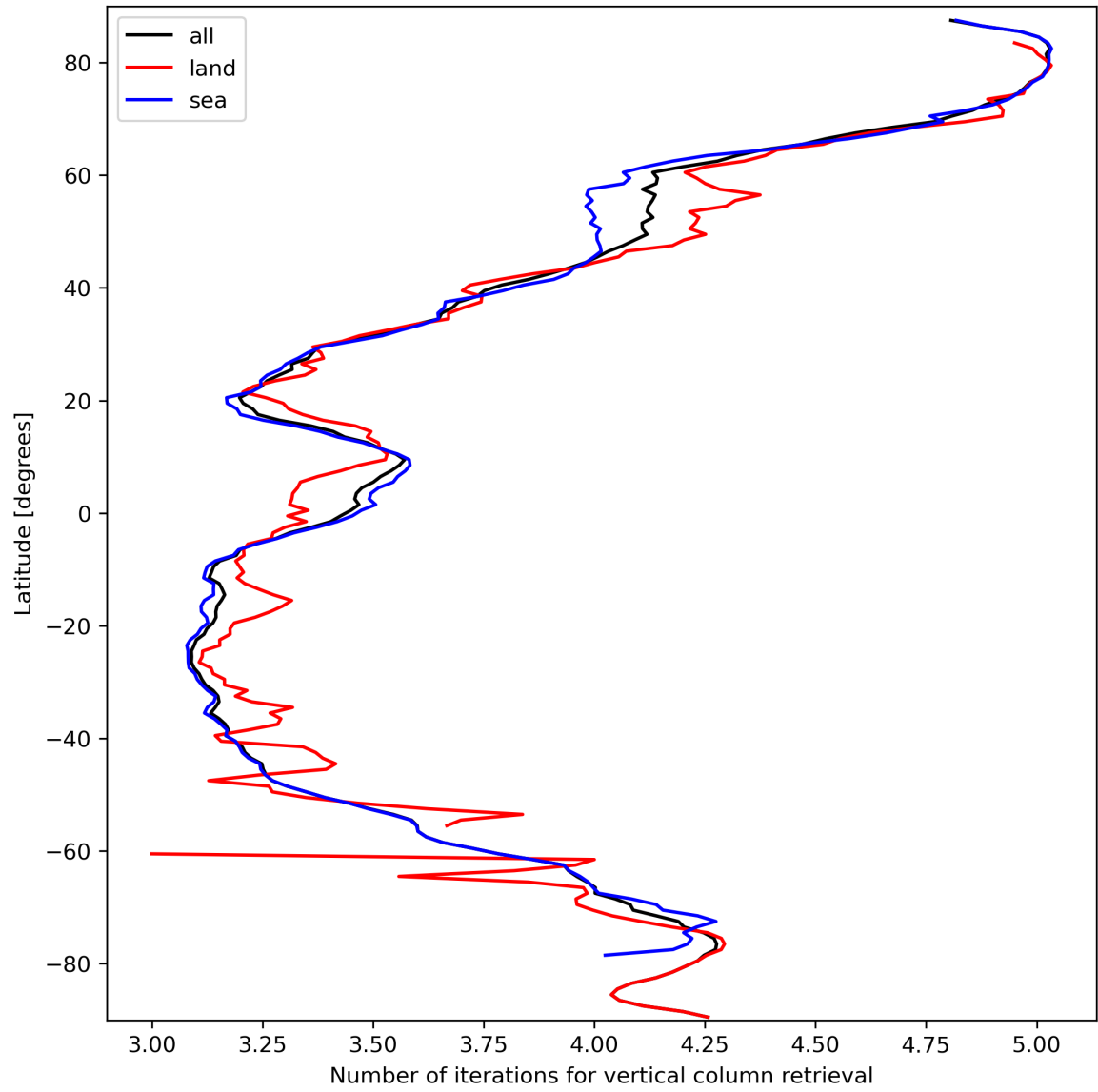
Figure 19: Zonal average of “Number of iterations for vertical column retrieval” for 2024-03-14 to 2024-03-16.
