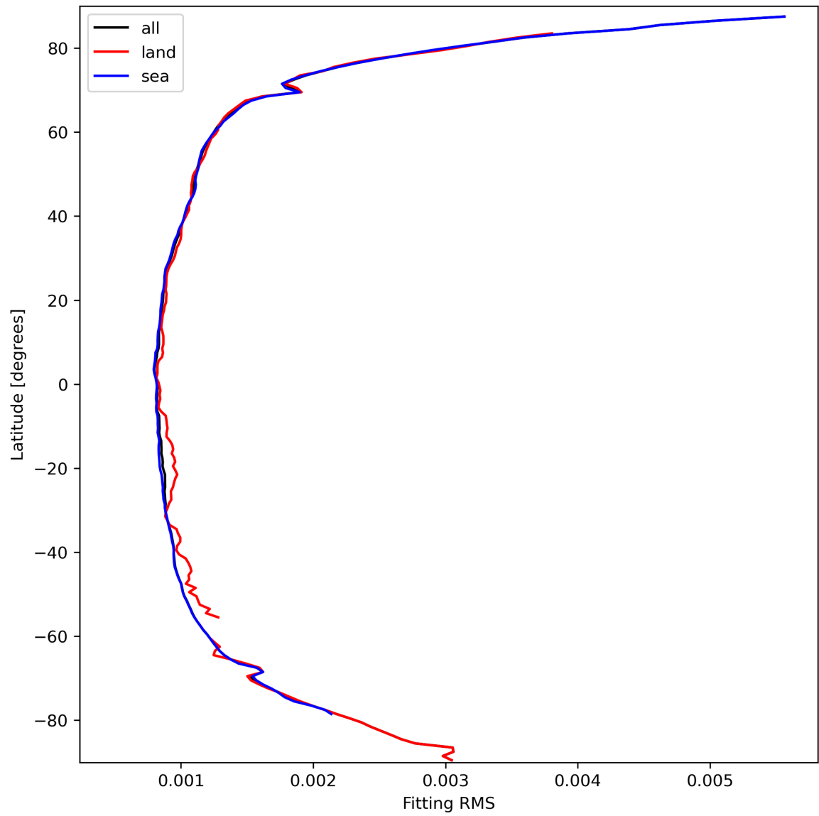
Figure 16: Zonal average of “Fitting RMS” for 2024-03-14 to 2024-03-16.
