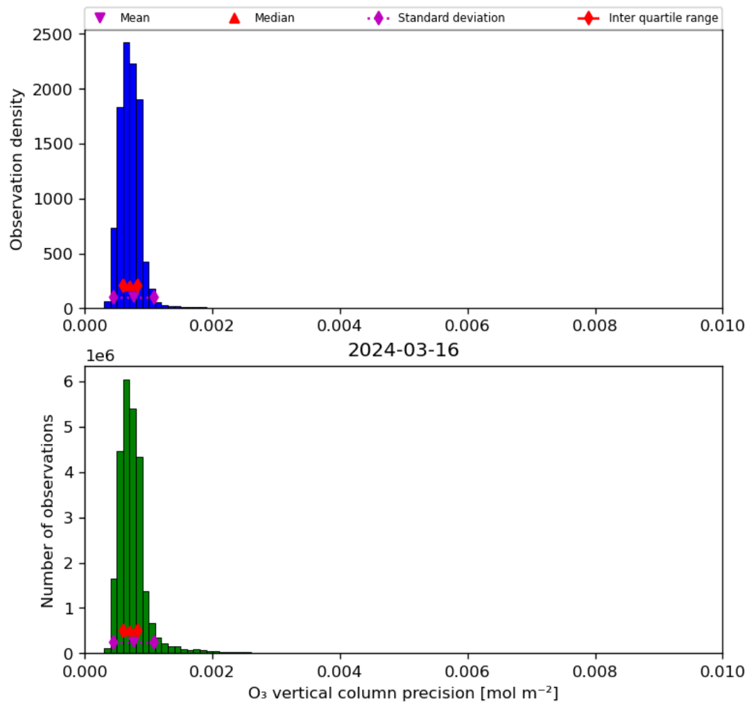
Figure 22: Histogram of “O 3 vertical column precision” for 2024-03-15 to 2024-03-17
