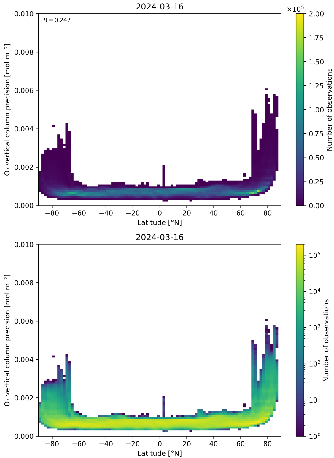
Figure 37: Scatter density plot of “Latitude” against “O 3 vertical column precision” for 2024-03-15 to 2024-03-17.
