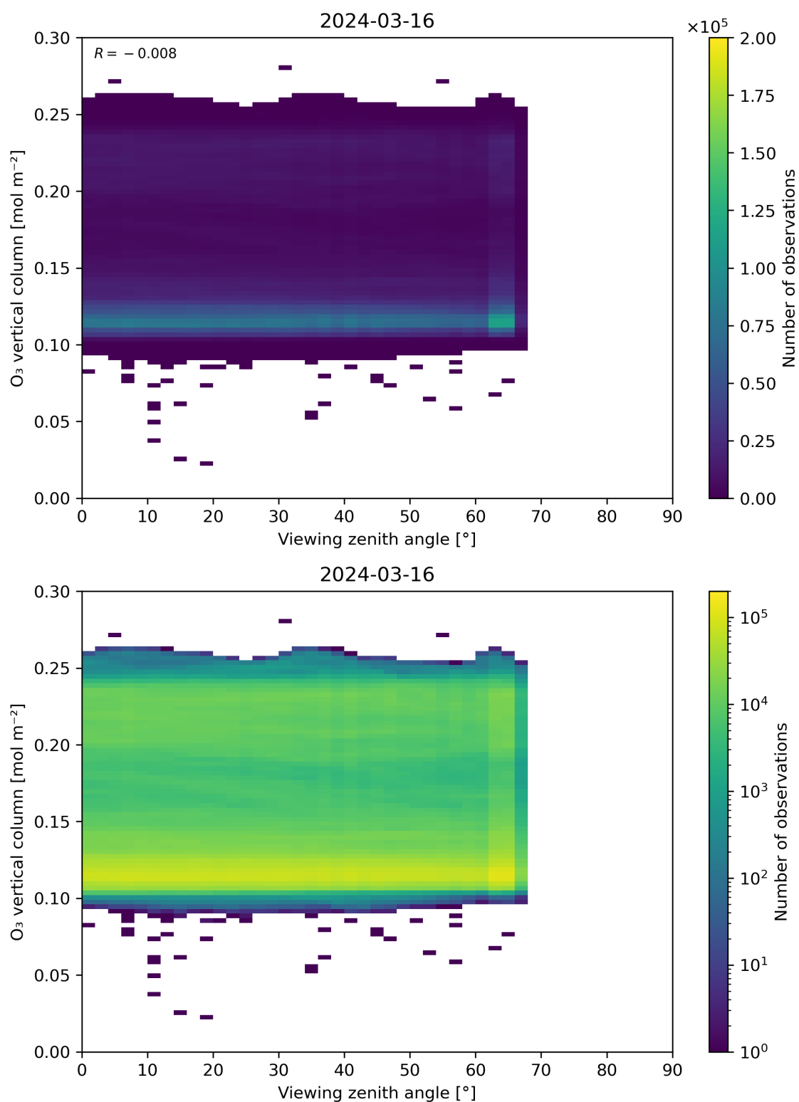
Figure 52: Scatter density plot of “Viewing zenith angle” against “O 3 vertical column” for 2024-03-15 to 2024-03-17.
