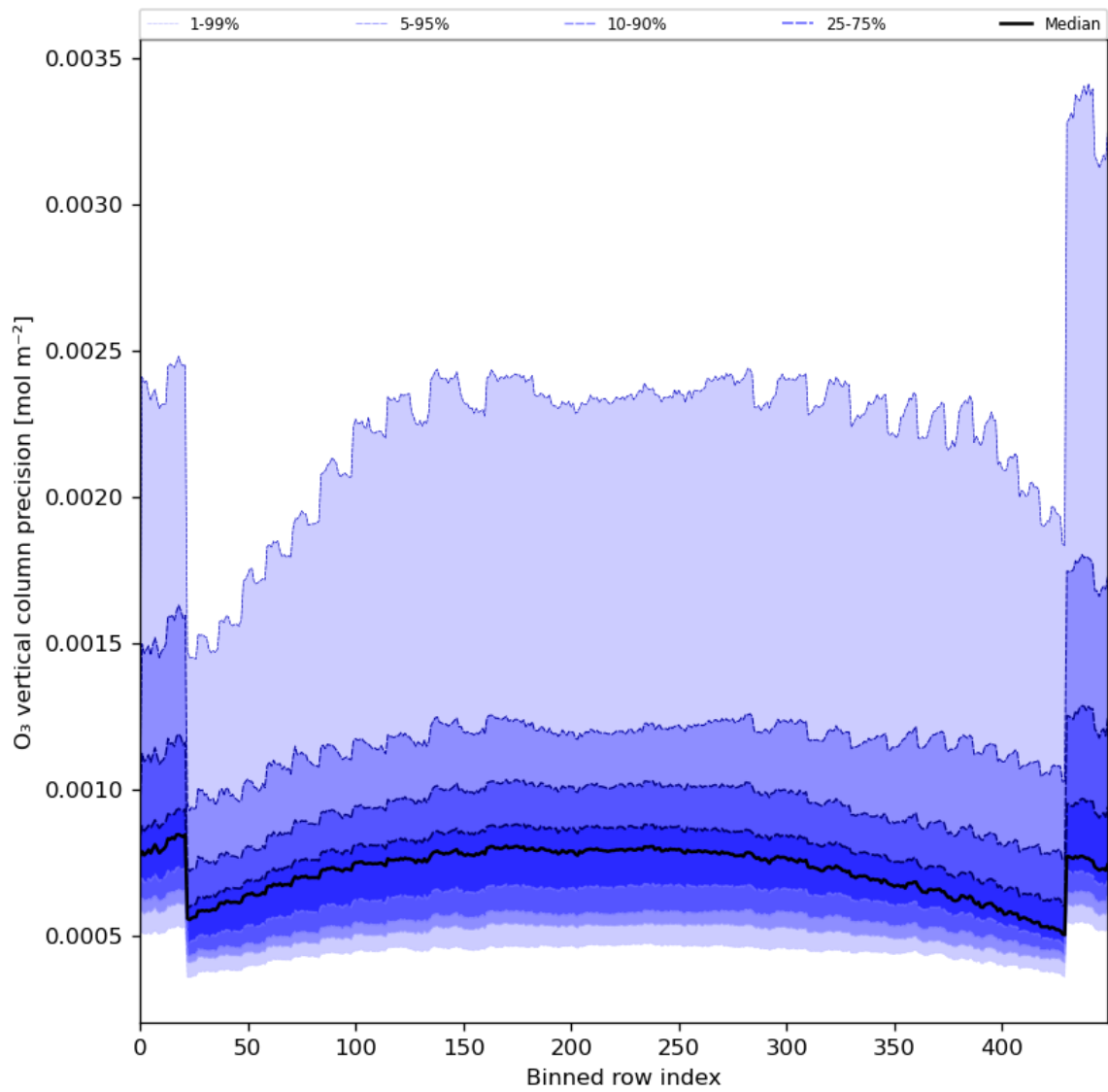
Figure 29: Along track statistics of “O 3 vertical column precision” for 2024-03-15 to 2024-03-17
