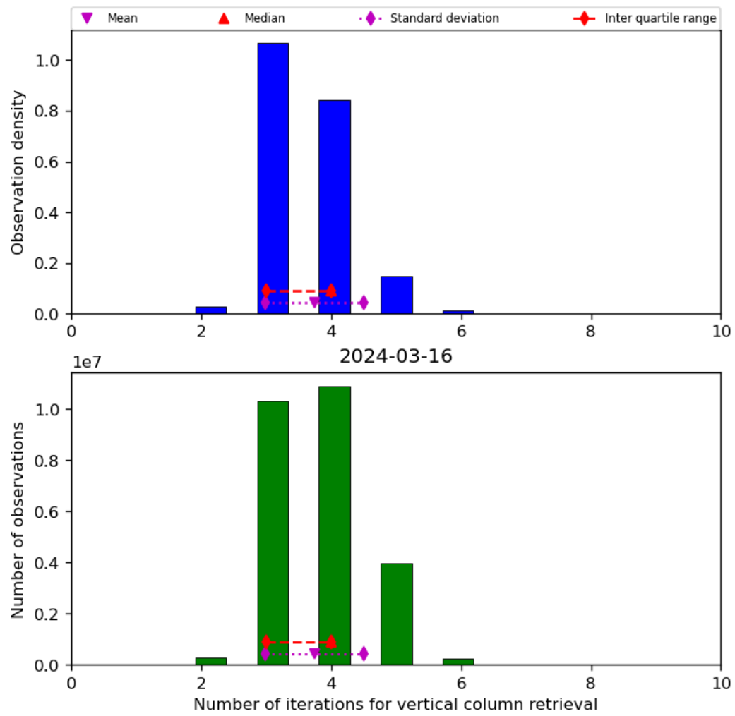
Figure 26: Histogram of “Number of iterations for vertical column retrieval” for 2024-03-15 to 2024-03-17
