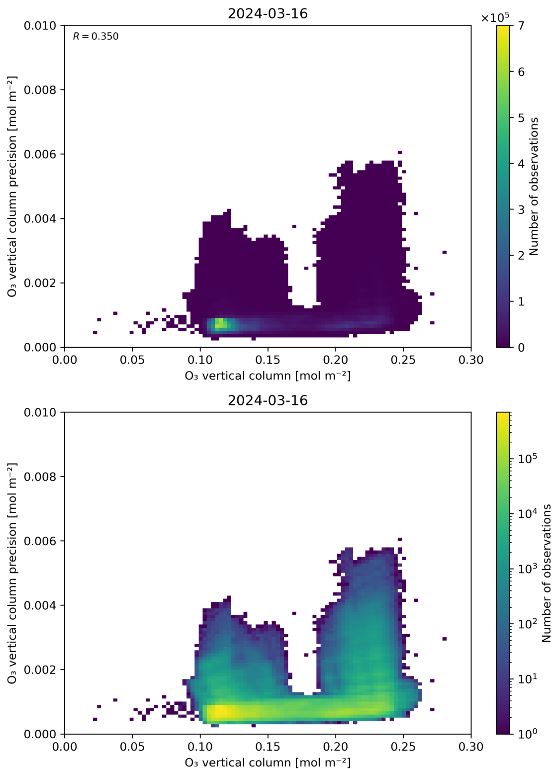
Figure 41: Scatter density plot of “O 3 vertical column” against “O 3 vertical column precision” for 2024-03-15 to 2024-03-17.
