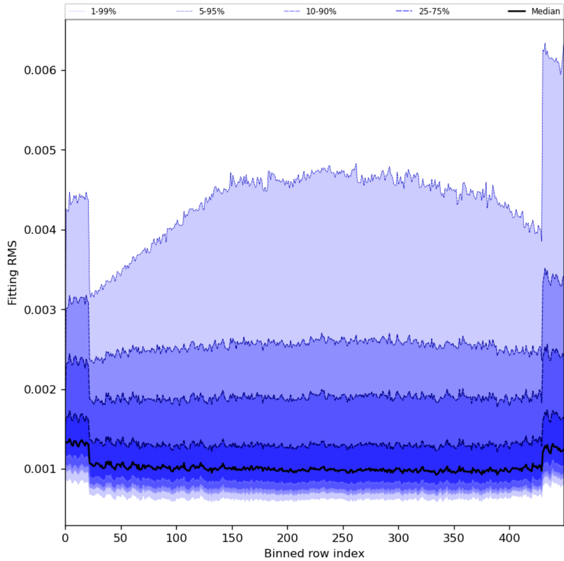
Figure 30: Along track statistics of “Fitting RMS” for 2024-03-15 to 2024-03-17
