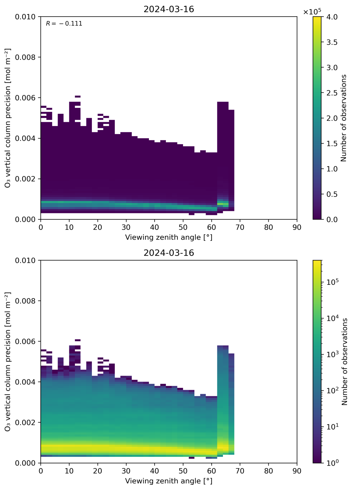
Figure 53: Scatter density plot of “Viewing zenith angle” against “O 3 vertical column precision” for 2024-03-15 to 2024-03-17.
