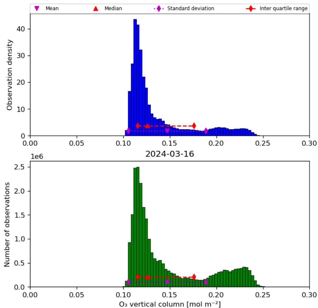
Figure 21: Histogram of “O 3 vertical column” for 2024-03-15 to 2024-03-17
