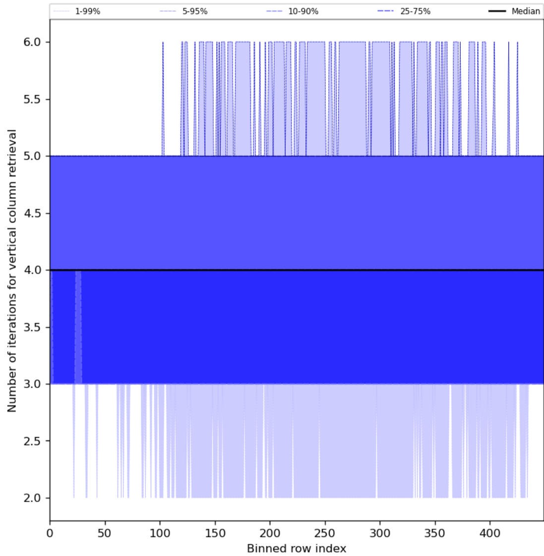
Figure 33: Along track statistics of “Number of iterations for vertical column retrieval” for 2024-03-15 to 2024-03-17
