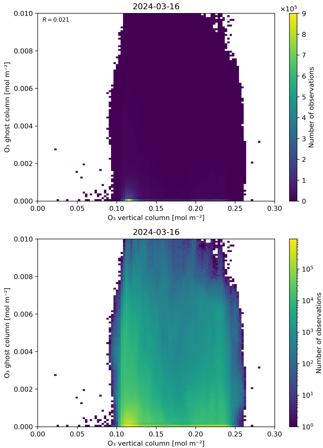
Figure 40: Scatter density plot of “O 3 vertical column” against “O 3 ghost column” for 2024-03-15 to 2024-03-17.
