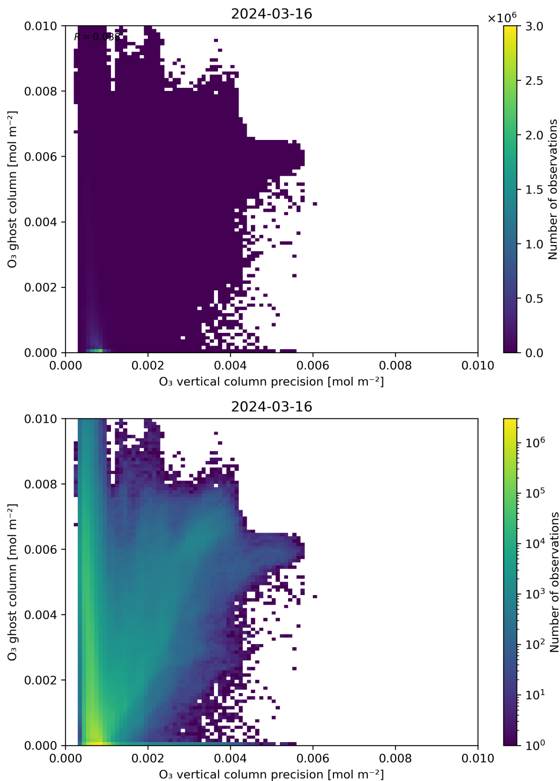
Figure 43: Scatter density plot of “O 3 vertical column precision” against “O 3 ghost column” for 2024-03-15 to 2024-03-17.
