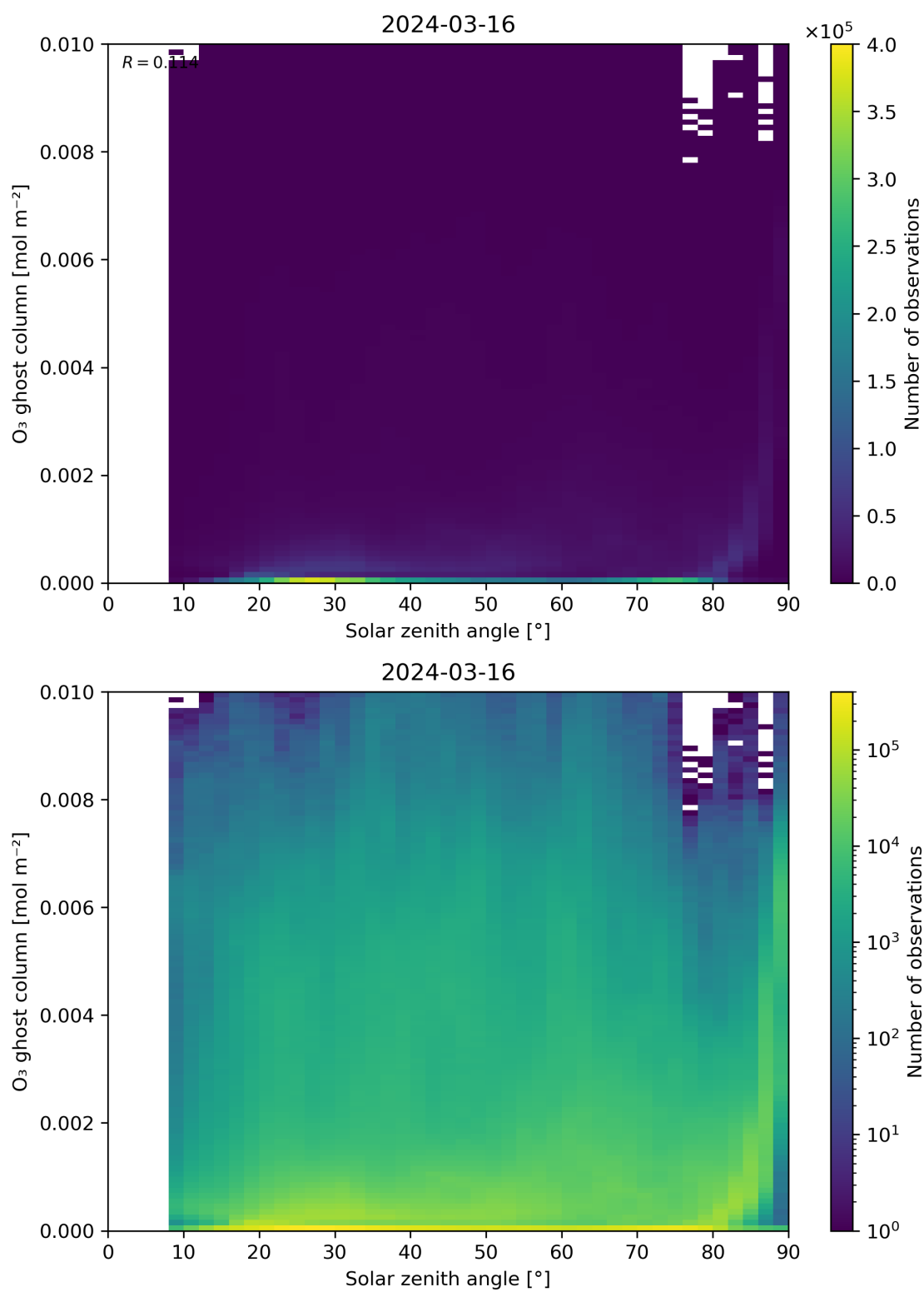
Figure 46: Scatter density plot of “Solar zenith angle” against “O 3 ghost column” for 2024-03-15 to 2024-03-17.
