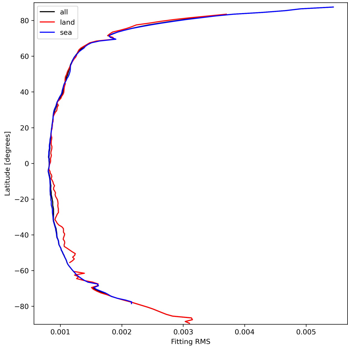
Figure 16: Zonal average of “Fitting RMS” for 2024-03-15 to 2024-03-17.
