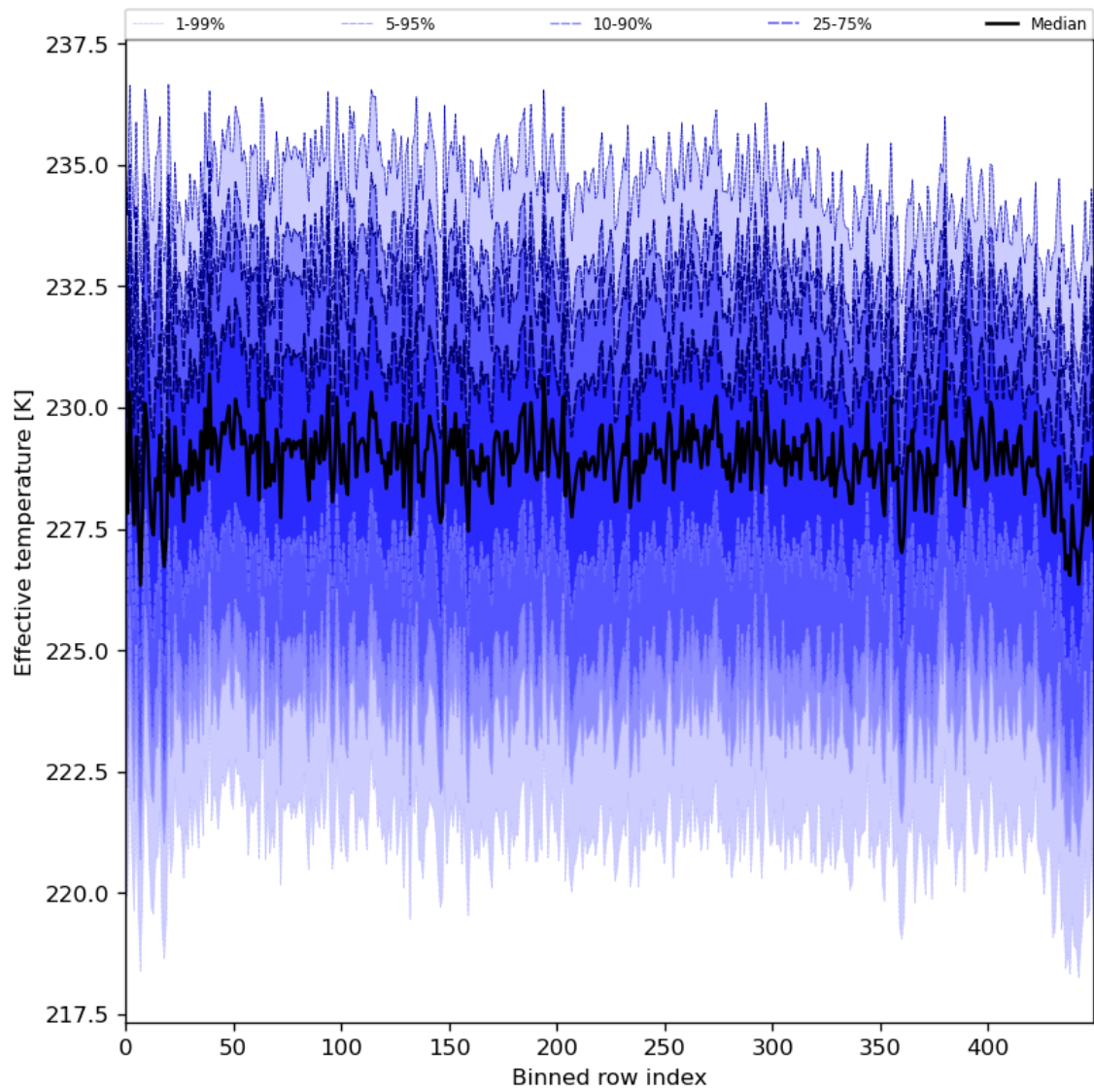
Figure 31: Along track statistics of “Effective temperature” for 2024-03-15 to 2024-03-17
