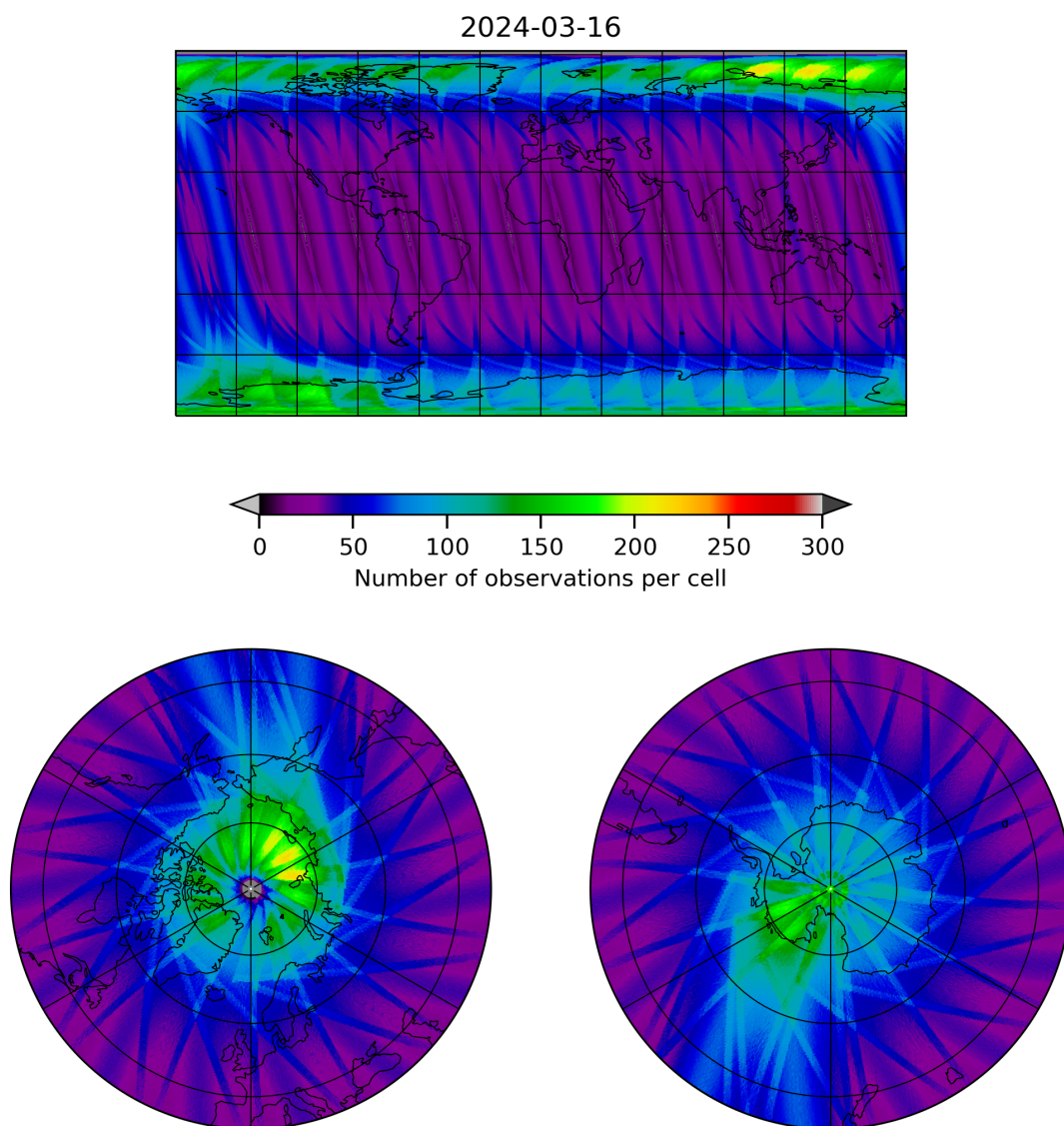
Figure 12: Map of the number of observations for 2024-03-15 to 2024-03-17
