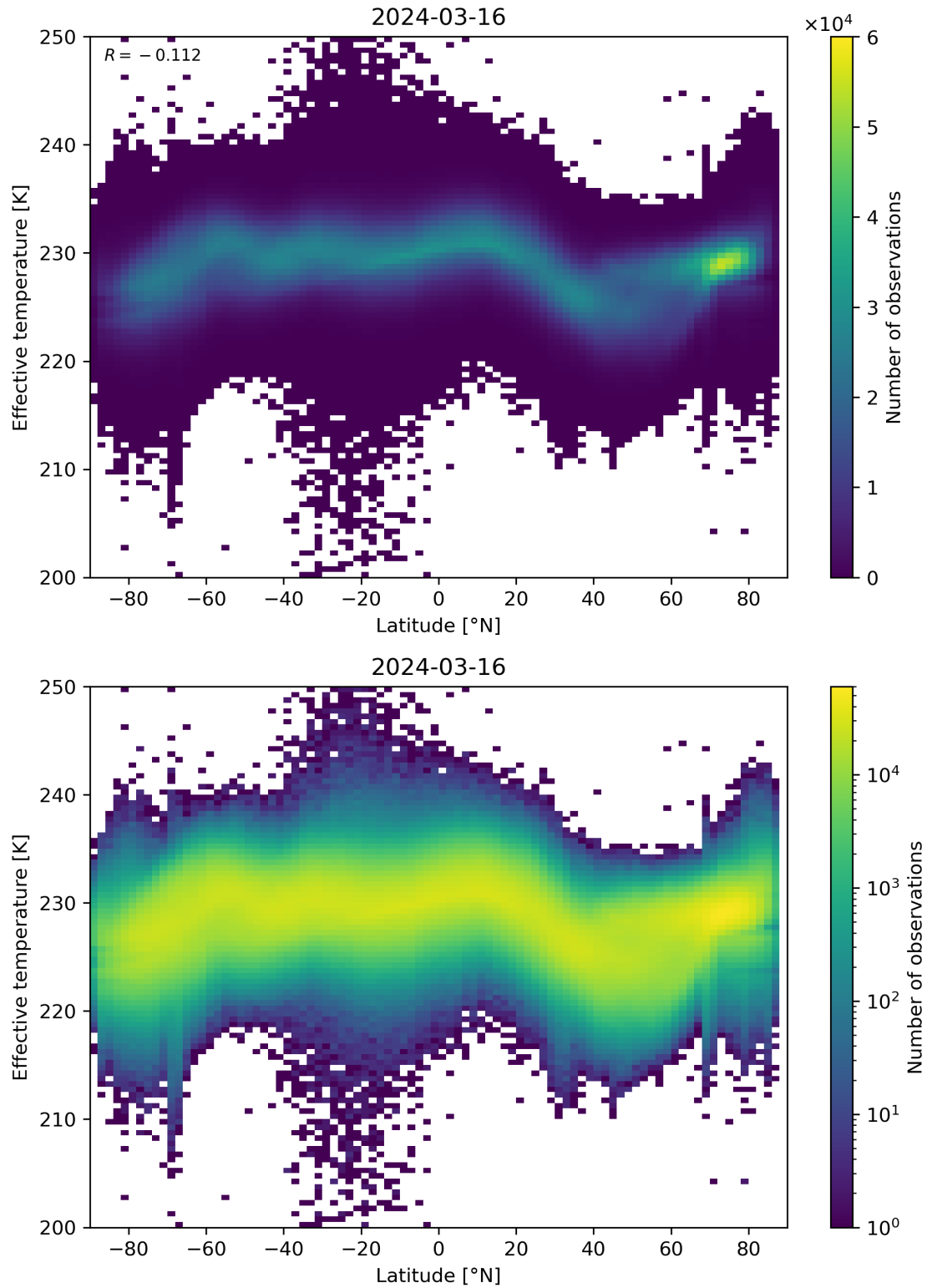
Figure 34: Scatter density plot of “Latitude” against “Effective temperature” for 2024-03-15 to 2024-03-17.
