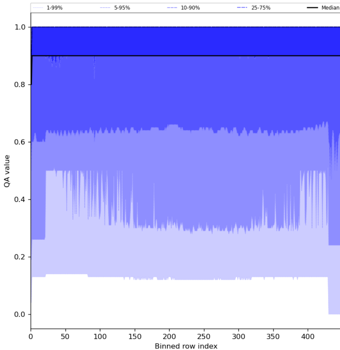
Figure 27: Along track statistics of “QA value” for 2024-03-15 to 2024-03-17
