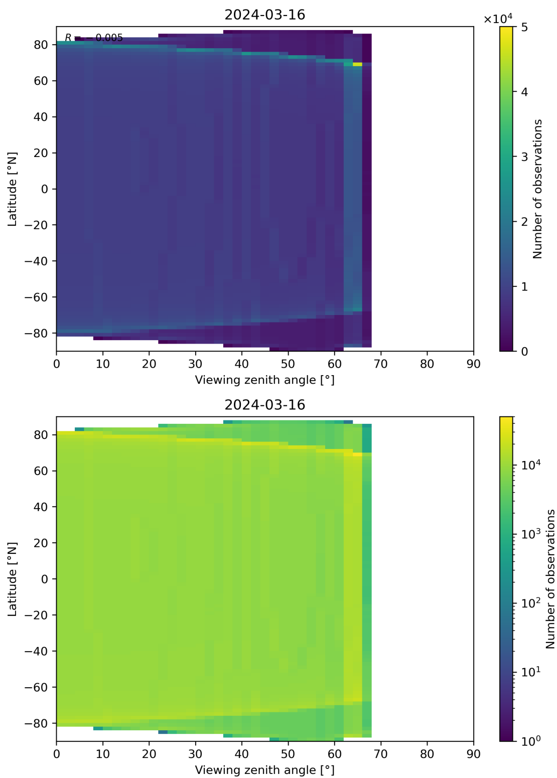
Figure 49: Scatter density plot of “Viewing zenith angle” against “Latitude” for 2024-03-15 to 2024-03-17.
