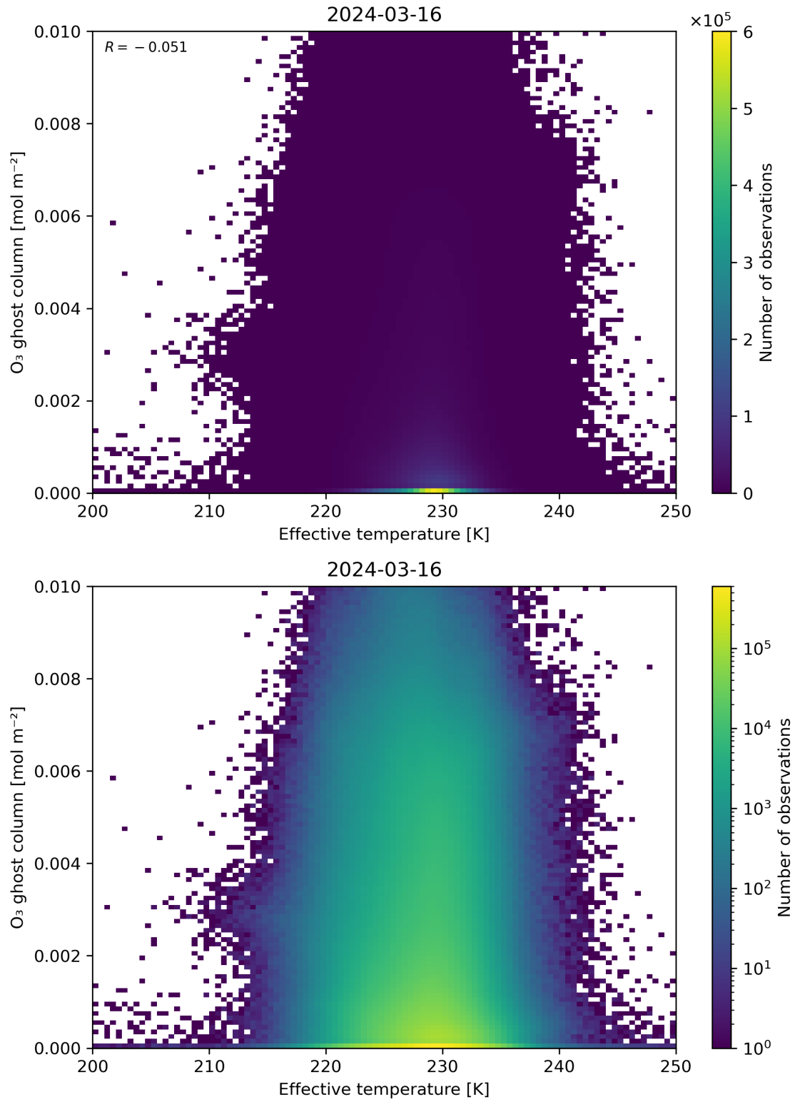
Figure 38: Scatter density plot of “Effective temperature” against “O 3 ghost column” for 2024-03-15 to 2024-03-17.
