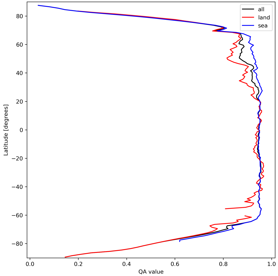
Figure 13: Zonal average of “QA value” for 2024-03-15 to 2024-03-17.
