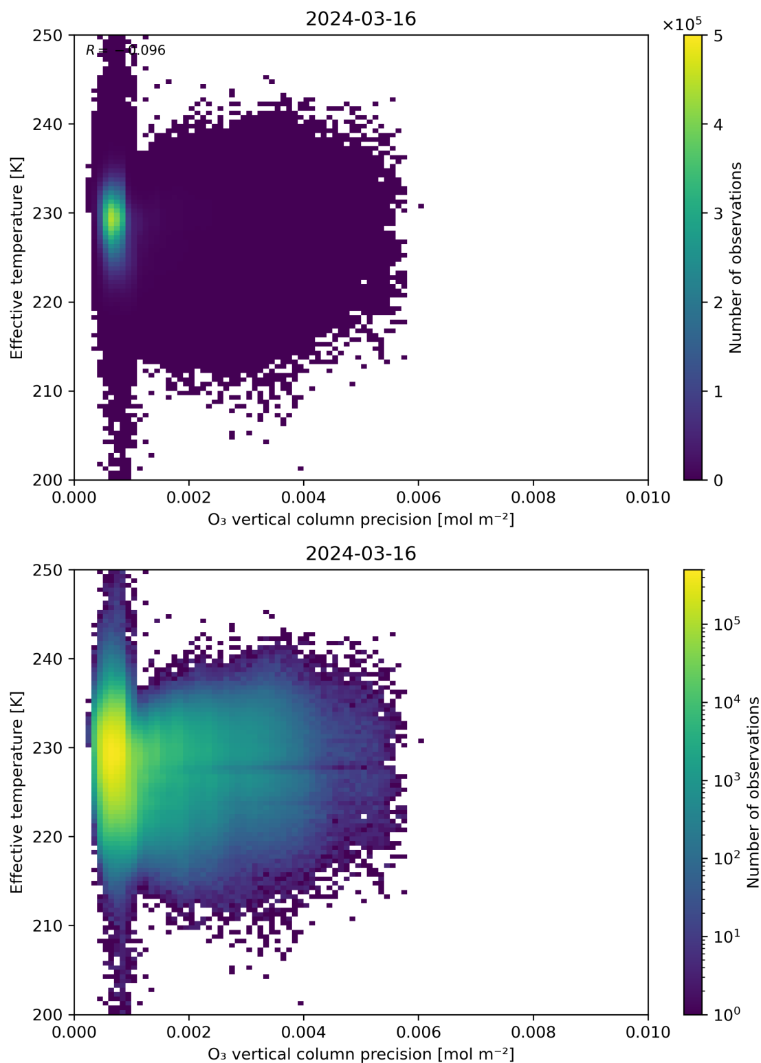
Figure 42: Scatter density plot of “O 3 vertical column precision” against “Effective temperature” for 2024-03-15 to 2024-03-17.
