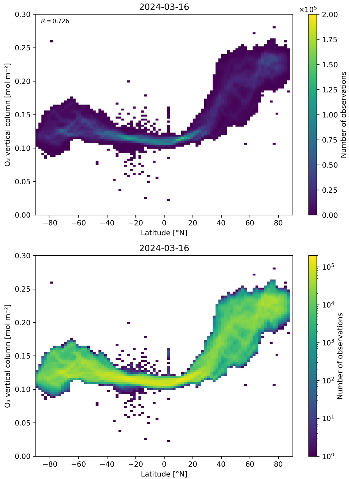
Figure 36: Scatter density plot of “Latitude” against “O 3 vertical column” for 2024-03-15 to 2024-03-17.
