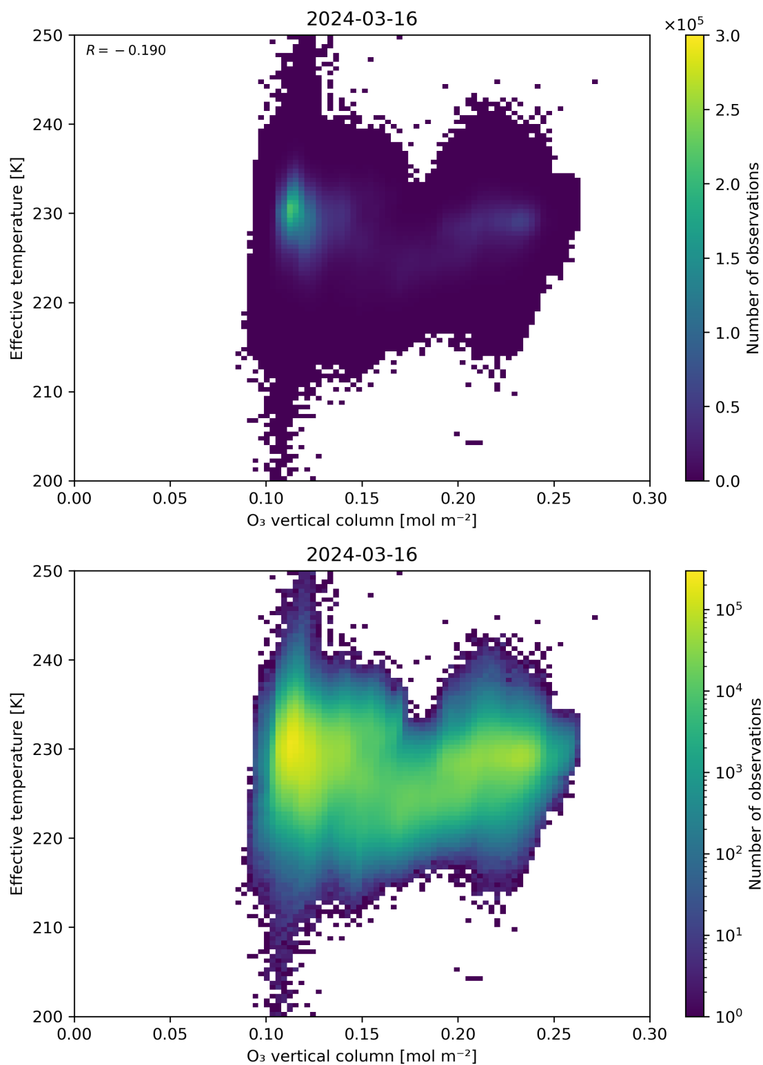
Figure 39: Scatter density plot of “O 3 vertical column” against “Effective temperature” for 2024-03-15 to 2024-03-17.
