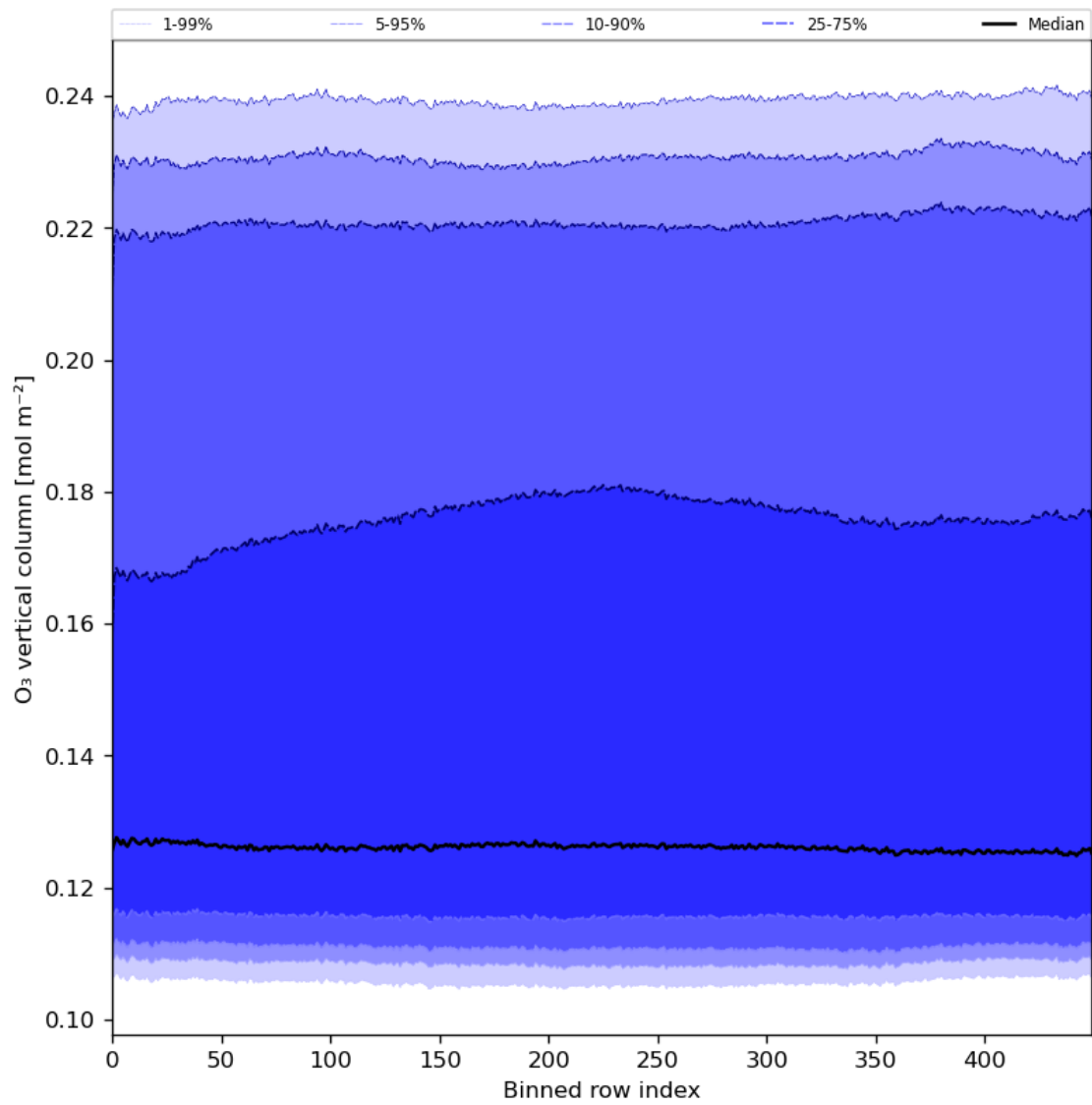
Figure 28: Along track statistics of “O 3 vertical column” for 2024-03-15 to 2024-03-17
