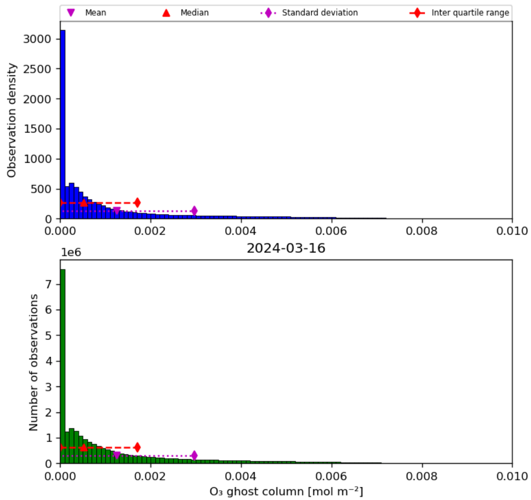
Figure 25: Histogram of “O 3 ghost column” for 2024-03-15 to 2024-03-17
