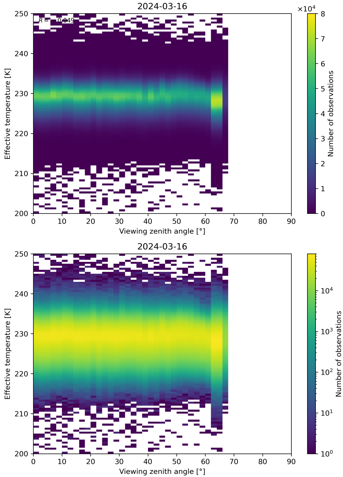
Figure 50: Scatter density plot of “Viewing zenith angle” against “Effective temperature” for 2024-03-15 to 2024-03-17.
