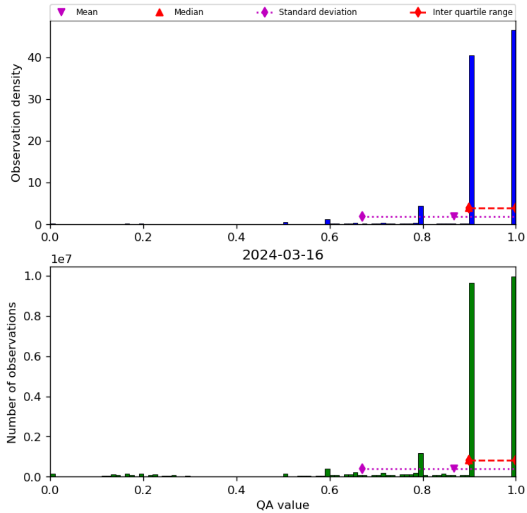
Figure 20: Histogram of “QA value” for 2024-03-15 to 2024-03-17
