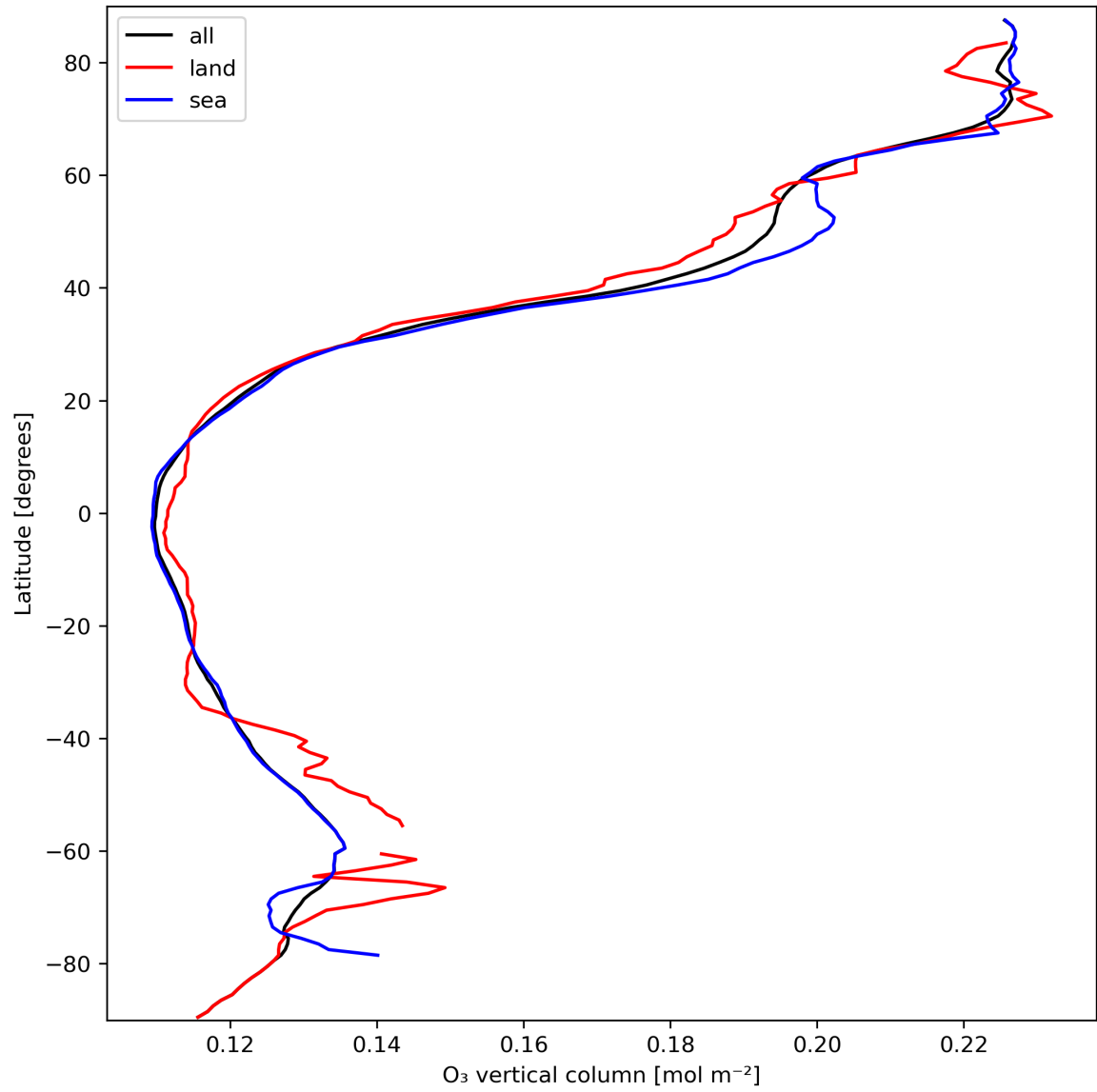
Figure 14: Zonal average of “O 3 vertical column” for 2024-03-15 to 2024-03-17.
