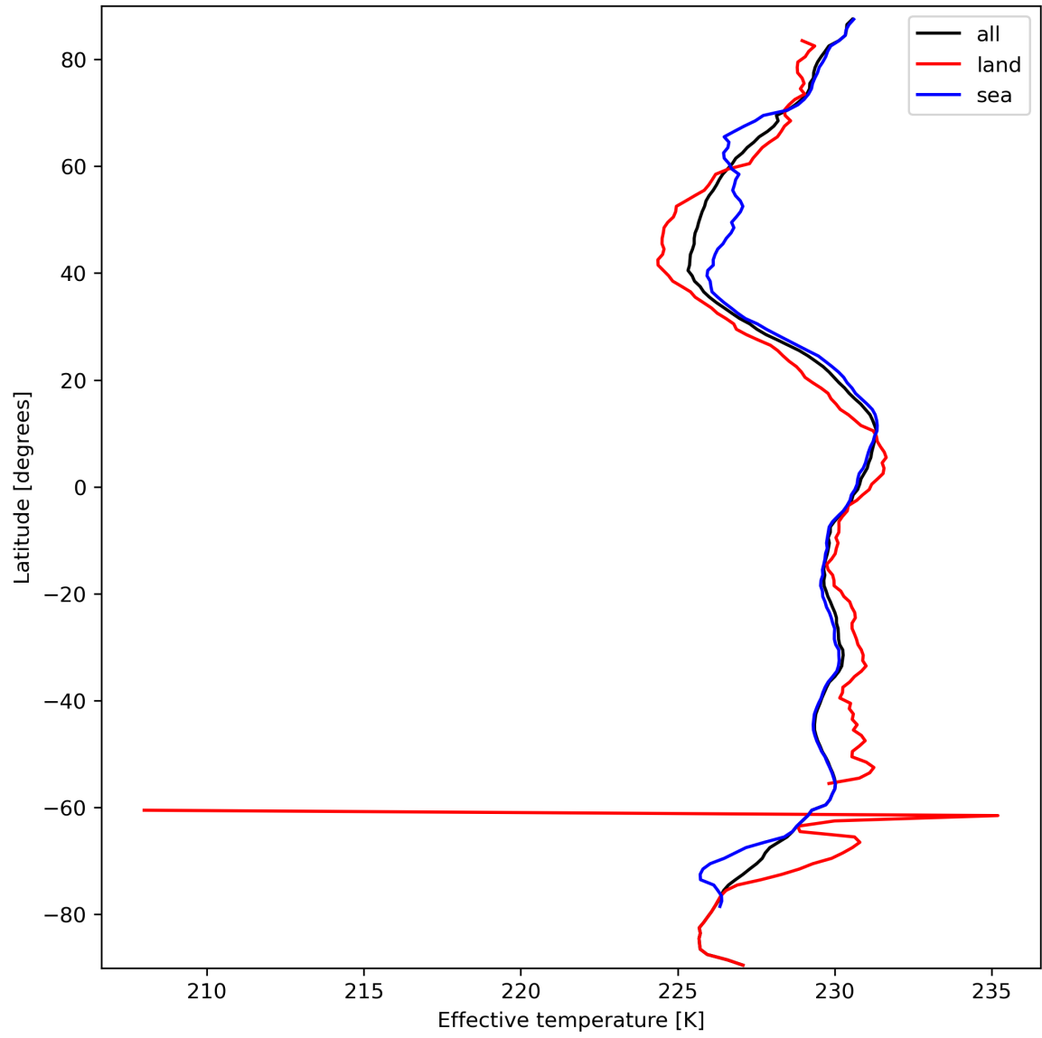
Figure 17: Zonal average of “Effective temperature” for 2024-03-15 to 2024-03-17.
