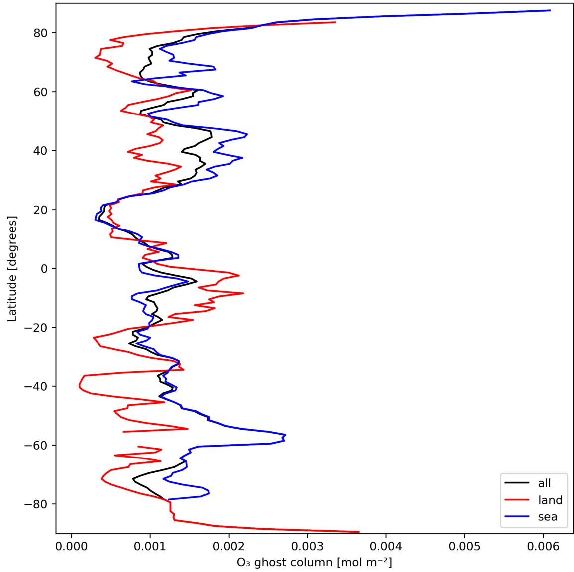
Figure 18: Zonal average of “O 3 ghost column” for 2024-03-15 to 2024-03-17.
