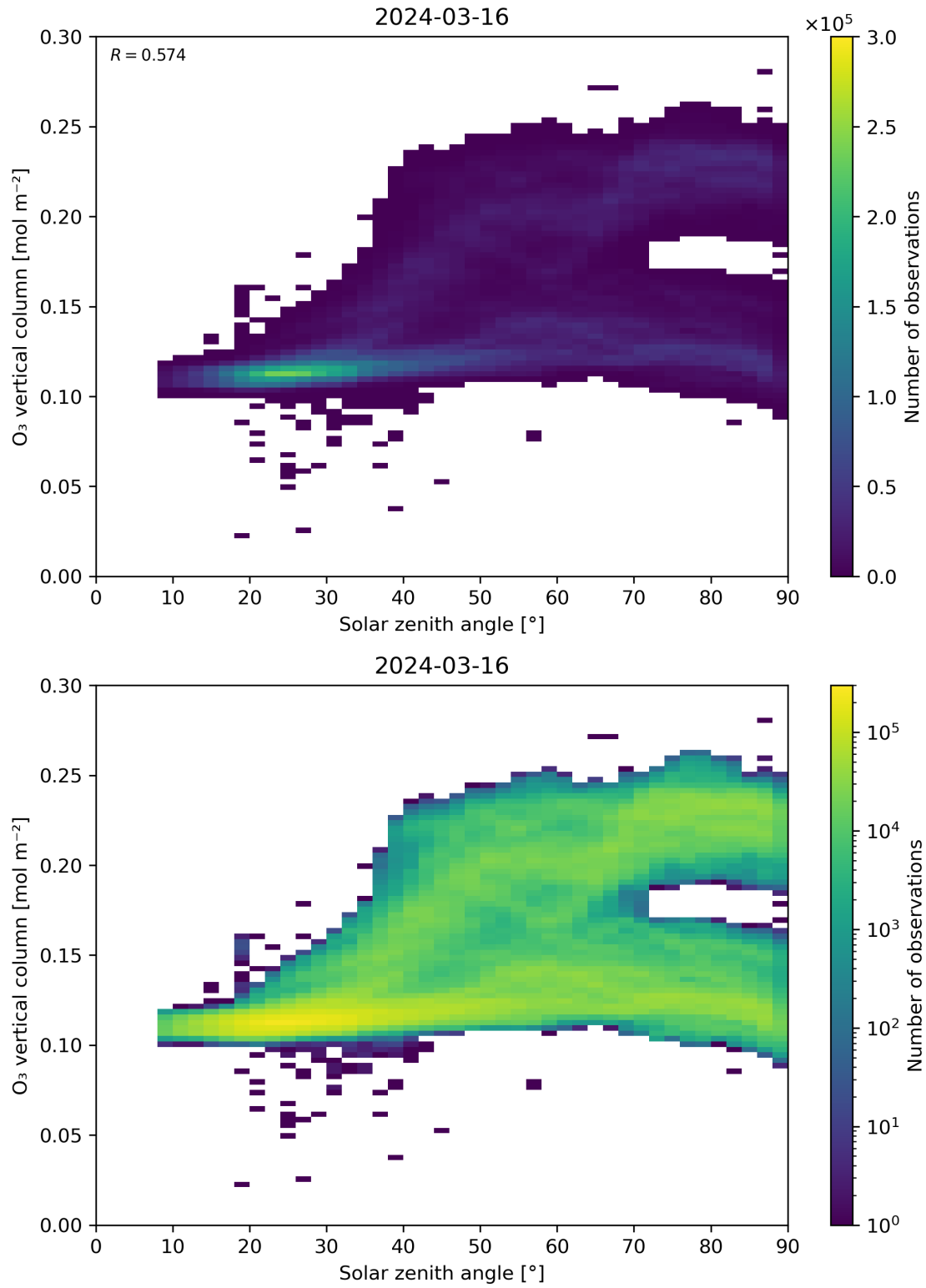
Figure 47: Scatter density plot of “Solar zenith angle” against “O 3 vertical column” for 2024-03-15 to 2024-03-17.
