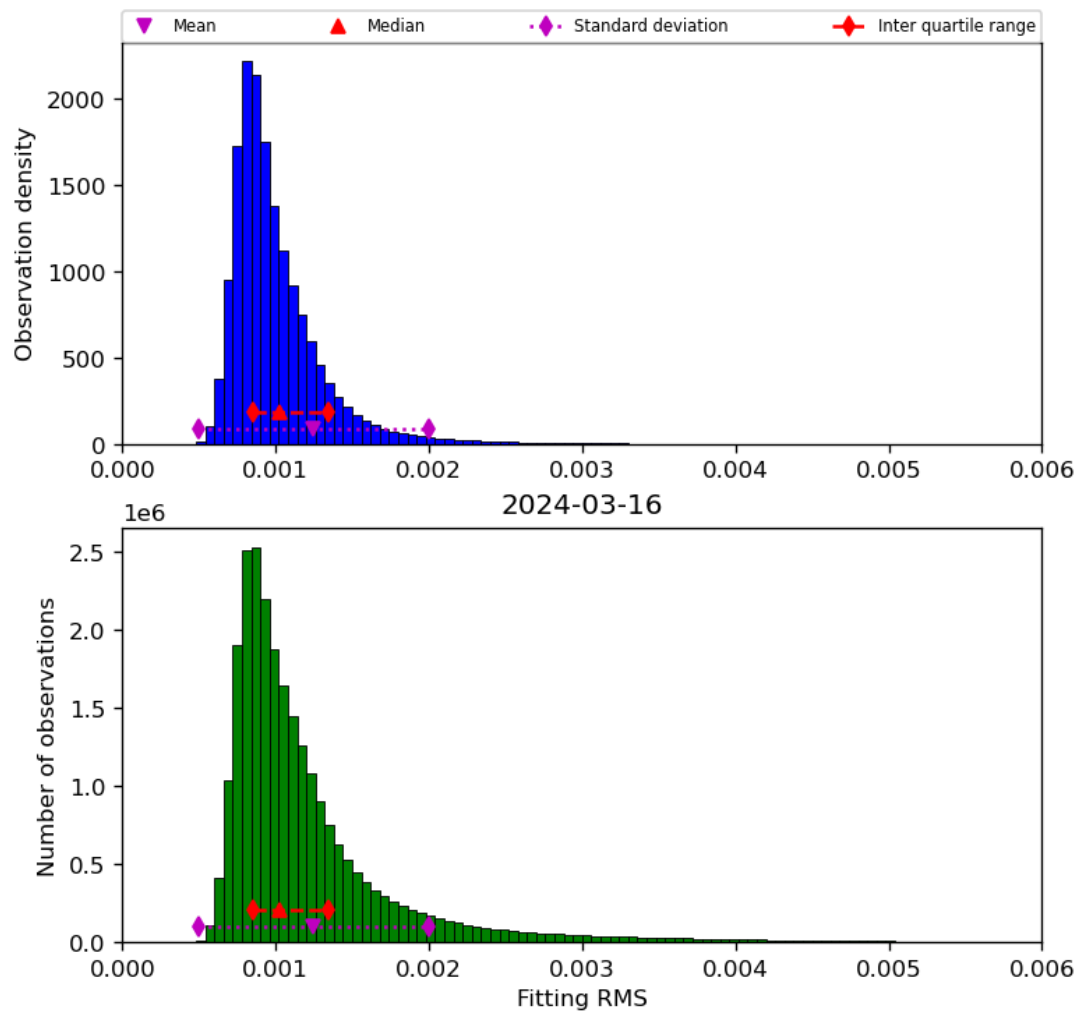
Figure 23: Histogram of “Fitting RMS” for 2024-03-15 to 2024-03-17
