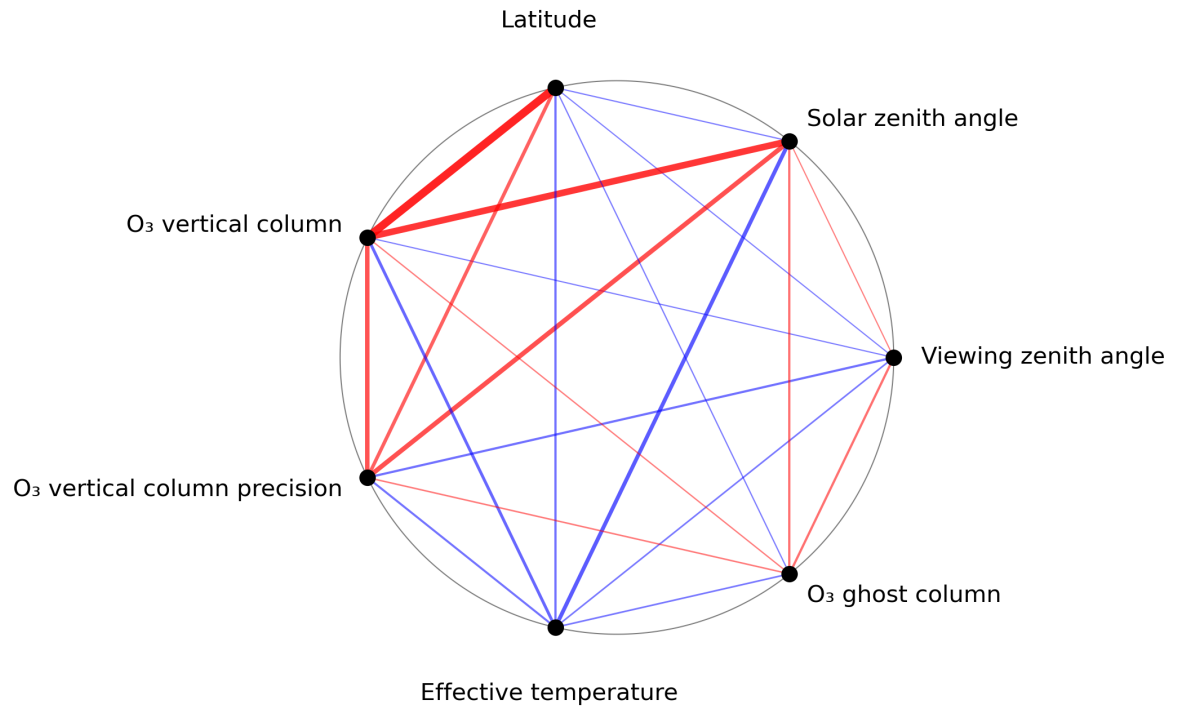
Figure 1: Map of correlation graph for 2024-03-15 to 2024-03-17.
