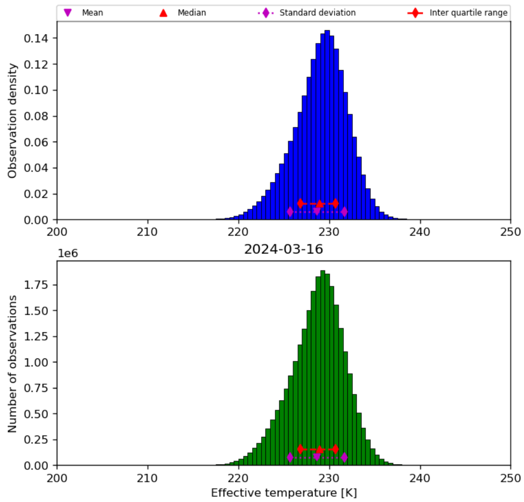
Figure 24: Histogram of “Effective temperature” for 2024-03-15 to 2024-03-17
