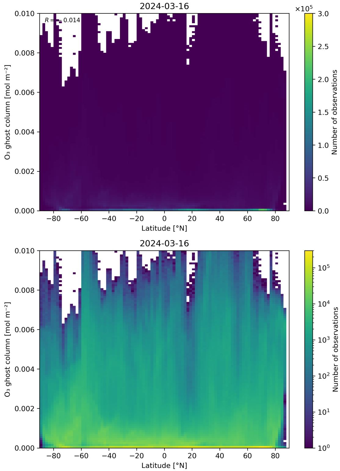
Figure 35: Scatter density plot of “Latitude” against “O 3 ghost column” for 2024-03-15 to 2024-03-17.
