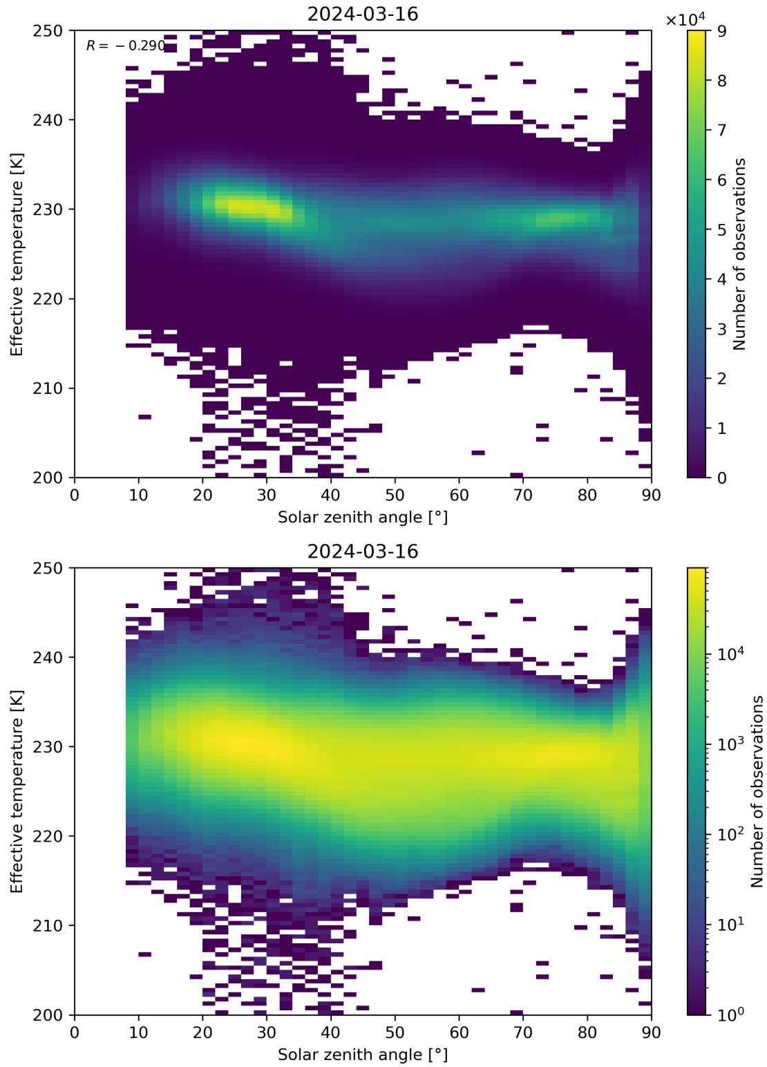
Figure 45: Scatter density plot of “Solar zenith angle” against “Effective temperature” for 2024-03-15 to 2024-03-17.
