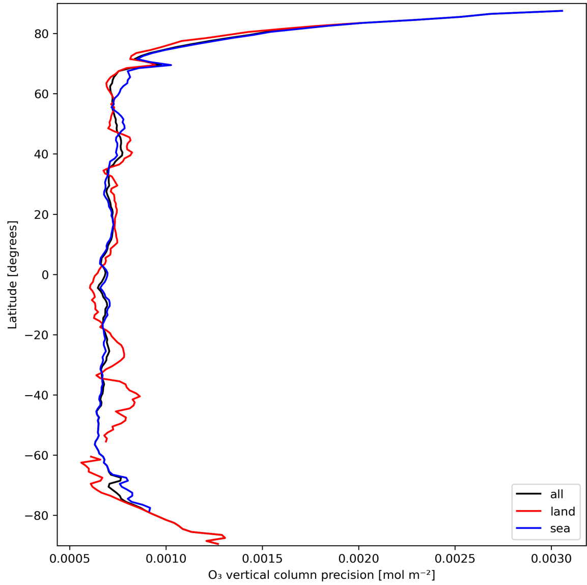
Figure 15: Zonal average of “O 3 vertical column precision” for 2024-03-15 to 2024-03-17.
