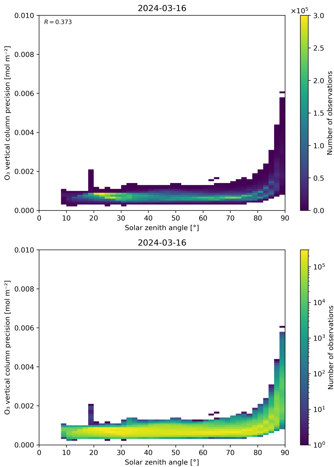
Figure 48: Scatter density plot of “Solar zenith angle” against “O 3 vertical column precision” for 2024-03-15 to 2024-03-17.
