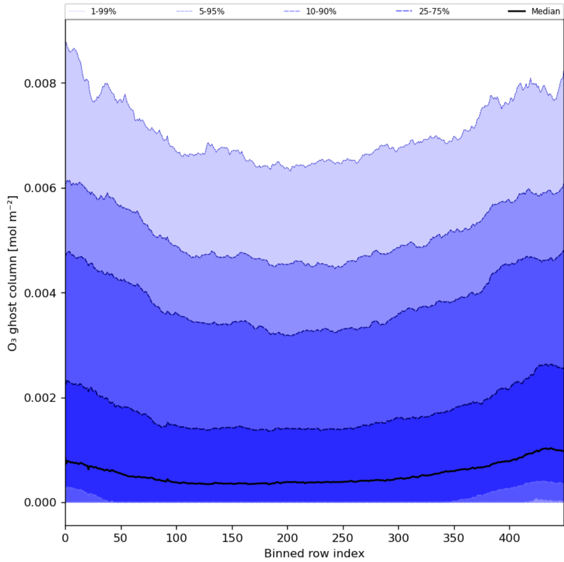
Figure 32: Along track statistics of “O 3 ghost column” for 2024-03-15 to 2024-03-17
