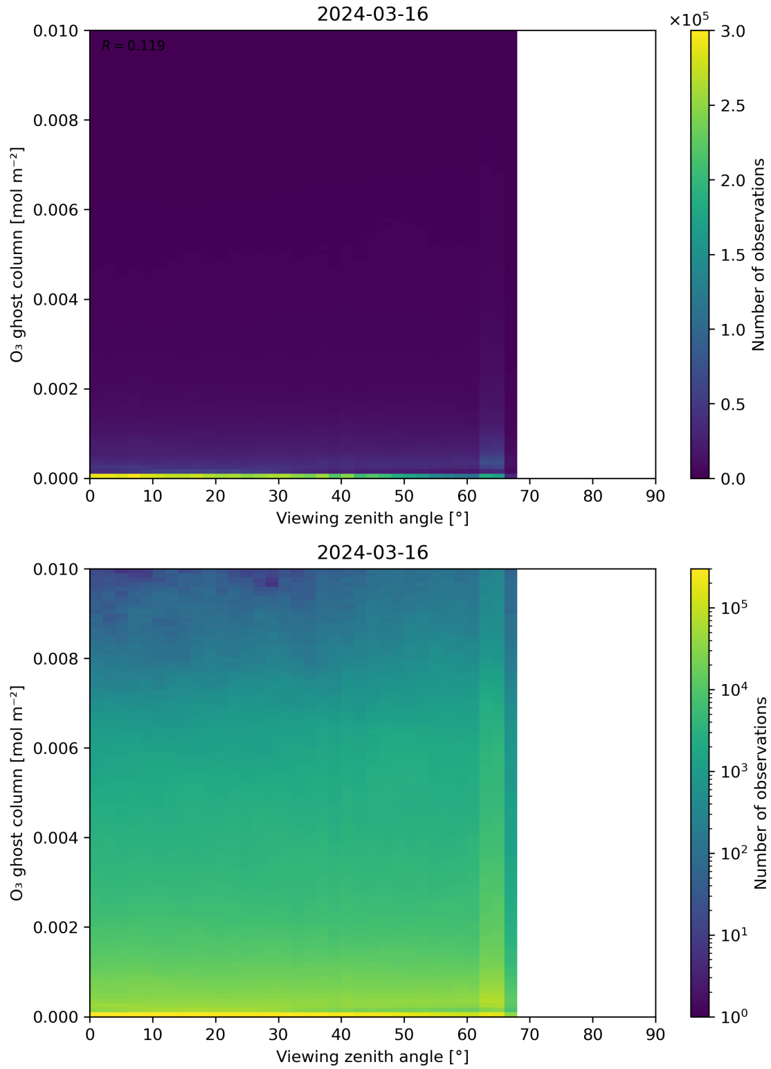
Figure 51: Scatter density plot of “Viewing zenith angle” against “O 3 ghost column” for 2024-03-15 to 2024-03-17.
