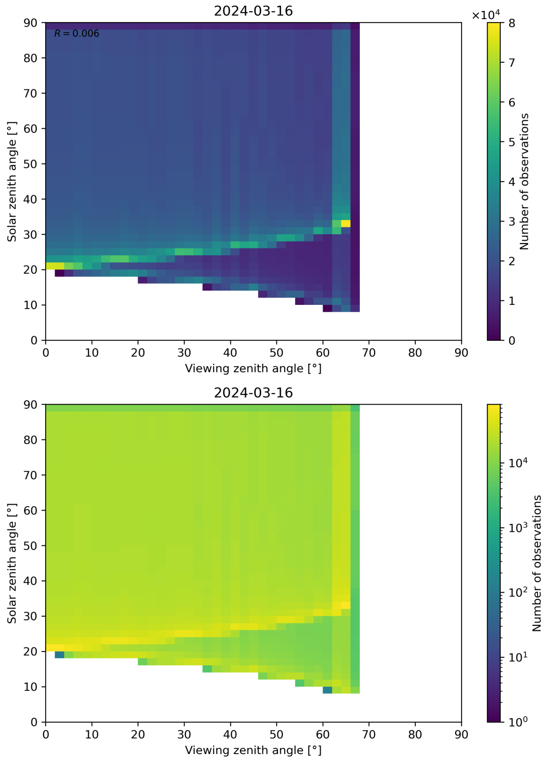
Figure 54: Scatter density plot of “Viewing zenith angle” against “Solar zenith angle” for 2024-03-15 to 2024-03-17.
