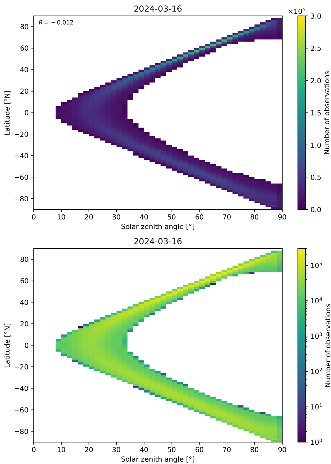
Figure 44: Scatter density plot of “Solar zenith angle” against “Latitude” for 2024-03-15 to 2024-03-17.
