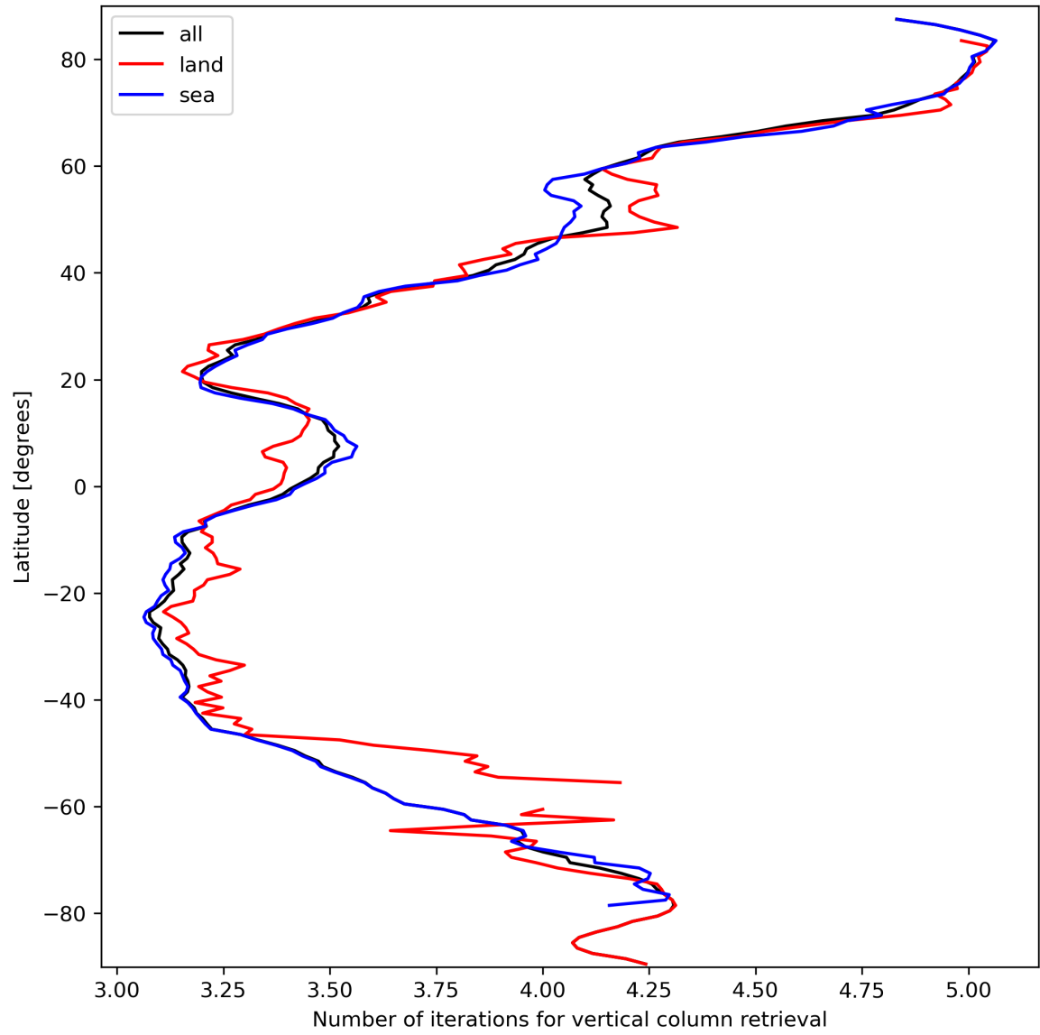
Figure 19: Zonal average of “Number of iterations for vertical column retrieval” for 2024-03-15 to 2024-03-17.
