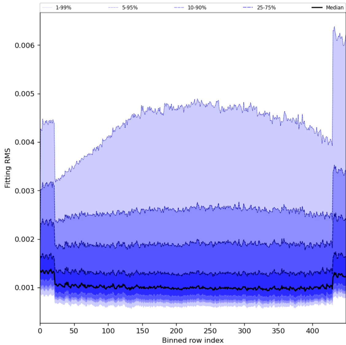
Figure 30: Along track statistics of “Fitting RMS” for 2024-03-16 to 2024-03-18
