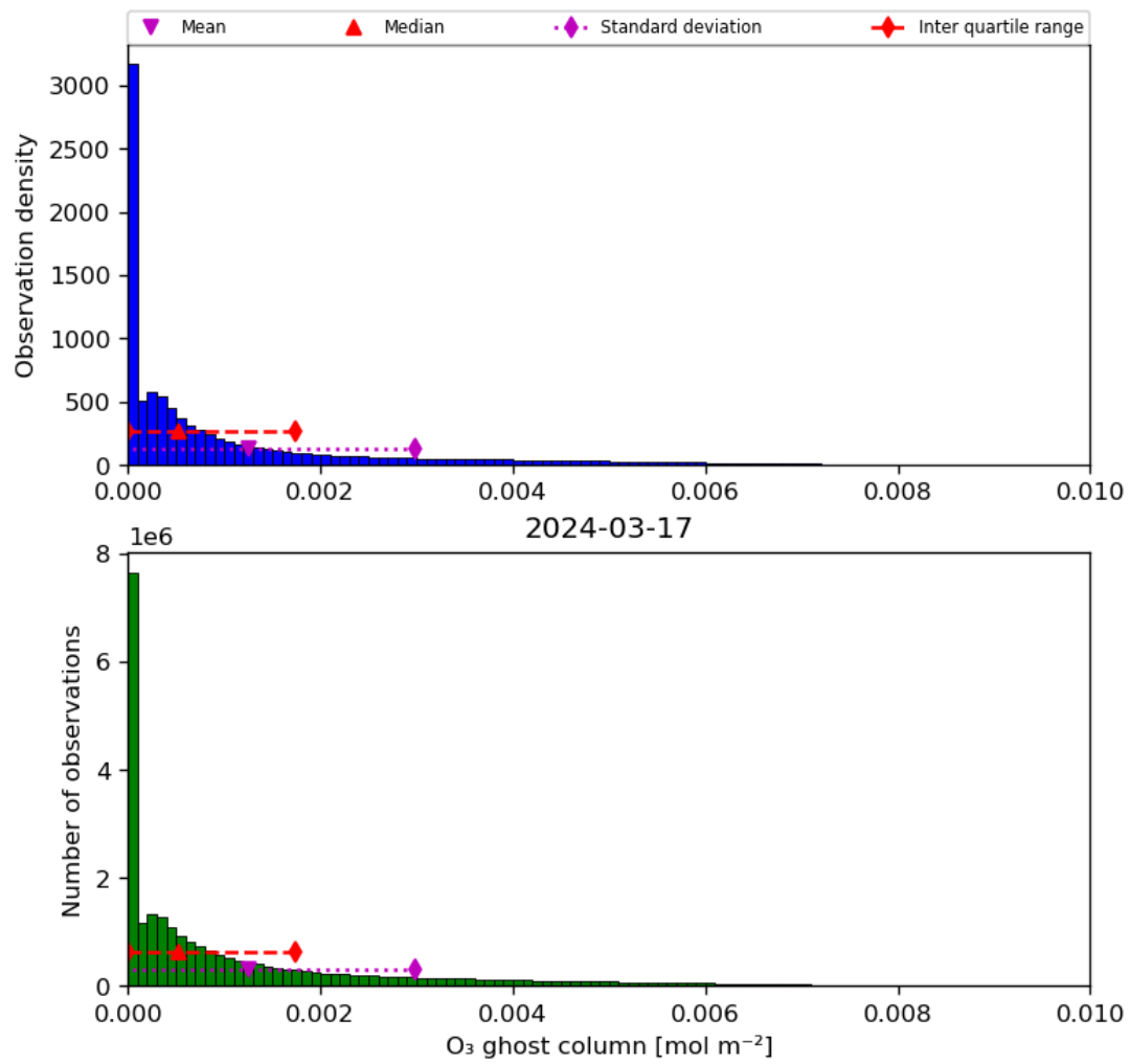
Figure 25: Histogram of “O 3 ghost column” for 2024-03-16 to 2024-03-18
