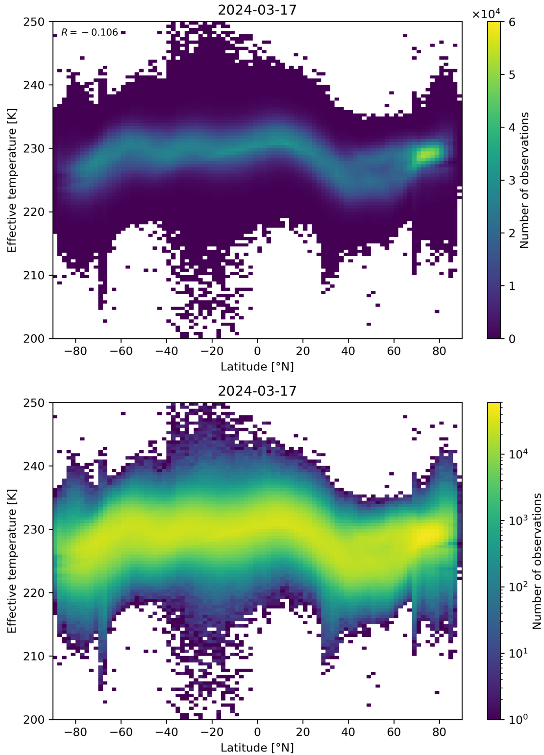
Figure 34: Scatter density plot of “Latitude” against “Effective temperature” for 2024-03-16 to 2024-03-18.
