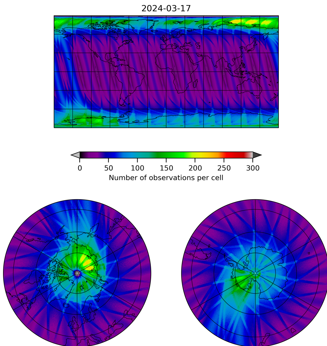
Figure 12: Map of the number of observations for 2024-03-16 to 2024-03-18
