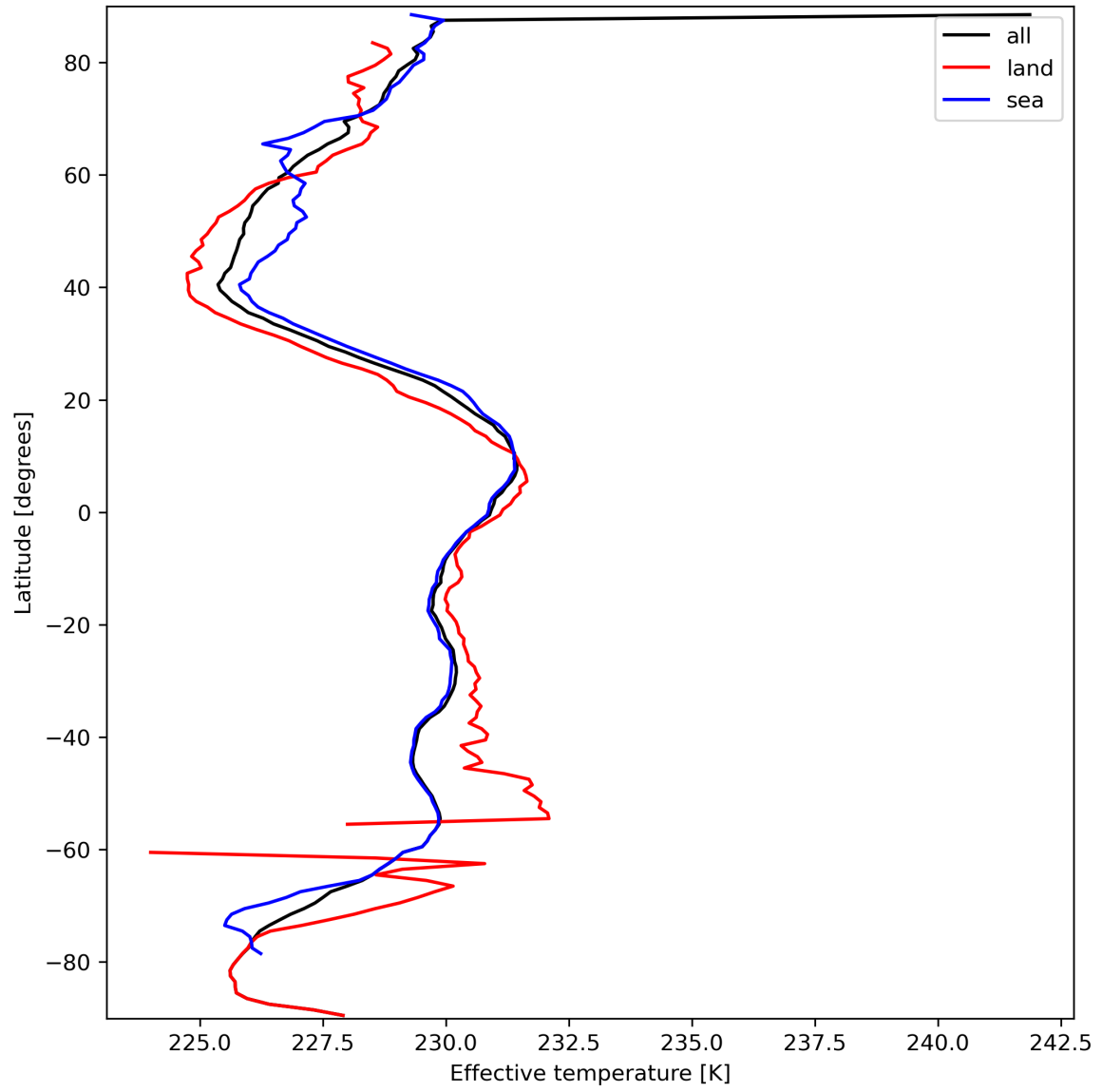
Figure 17: Zonal average of “Effective temperature” for 2024-03-16 to 2024-03-18.
