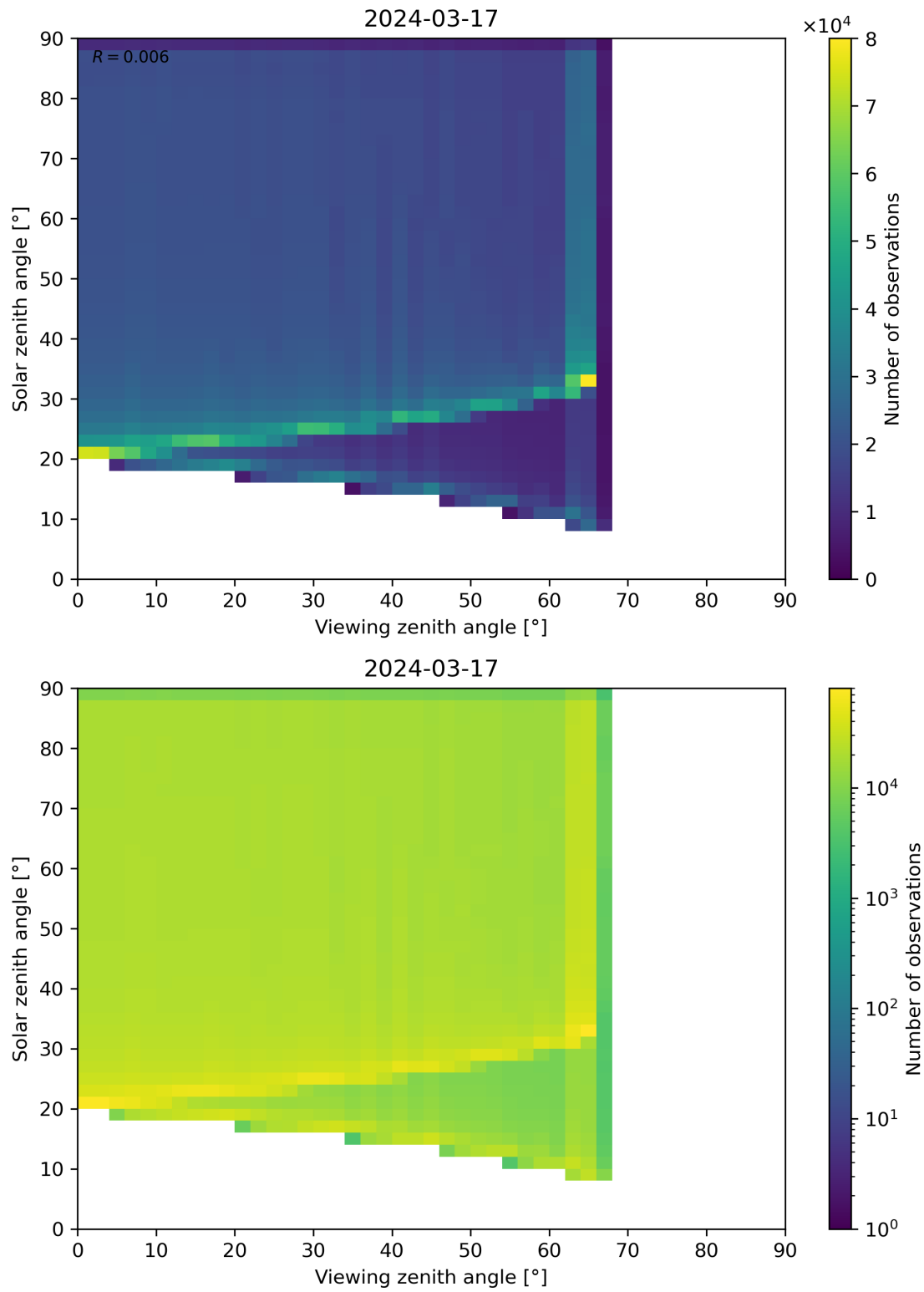
Figure 54: Scatter density plot of “Viewing zenith angle” against “Solar zenith angle” for 2024-03-16 to 2024-03-18.
