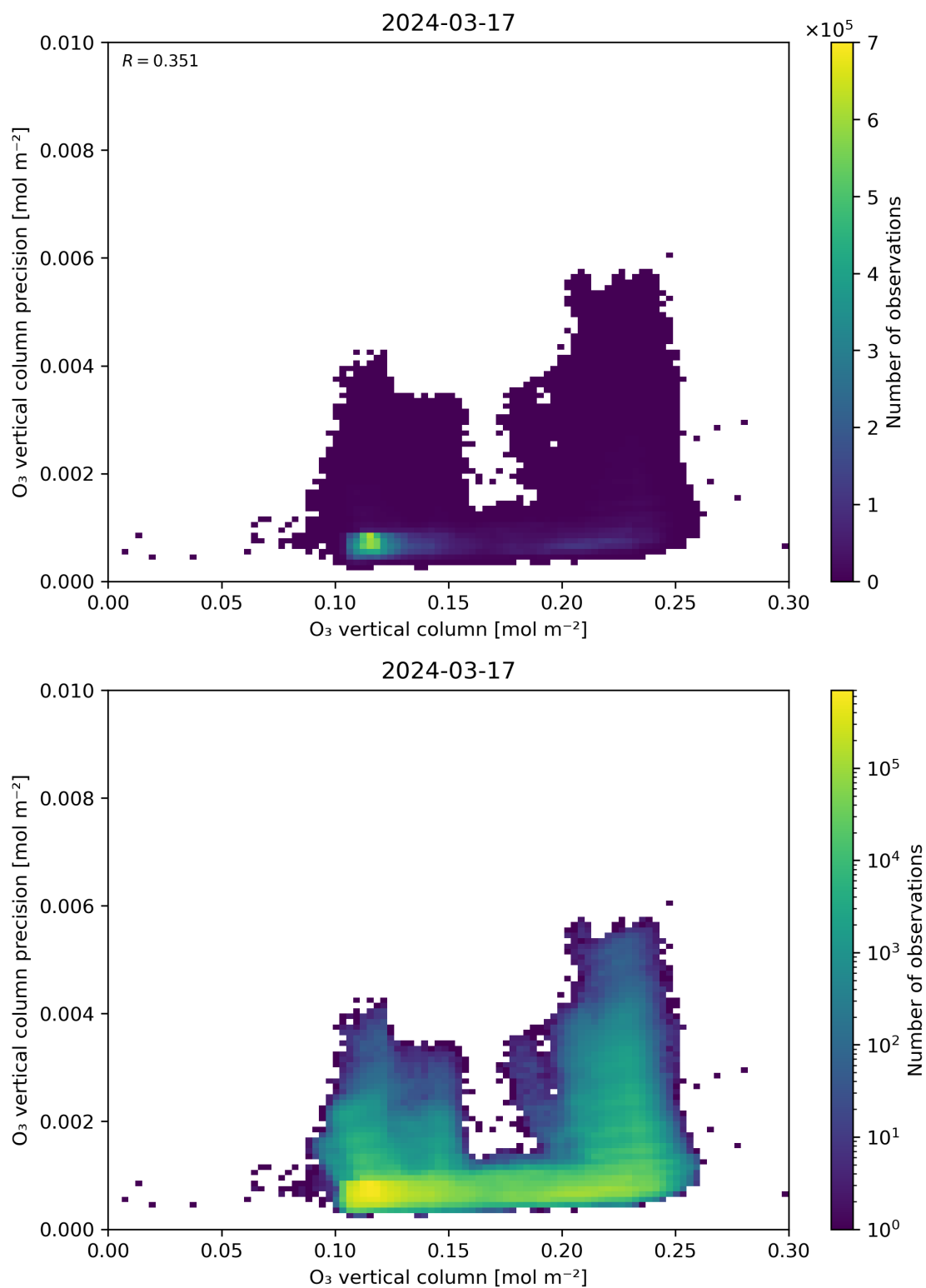
Figure 41: Scatter density plot of “O 3 vertical column” against “O 3 vertical column precision” for 2024-03-16 to 2024-03-18.
