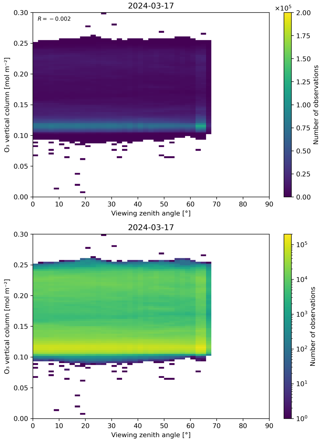
Figure 52: Scatter density plot of “Viewing zenith angle” against “O 3 vertical column” for 2024-03-16 to 2024-03-18.
