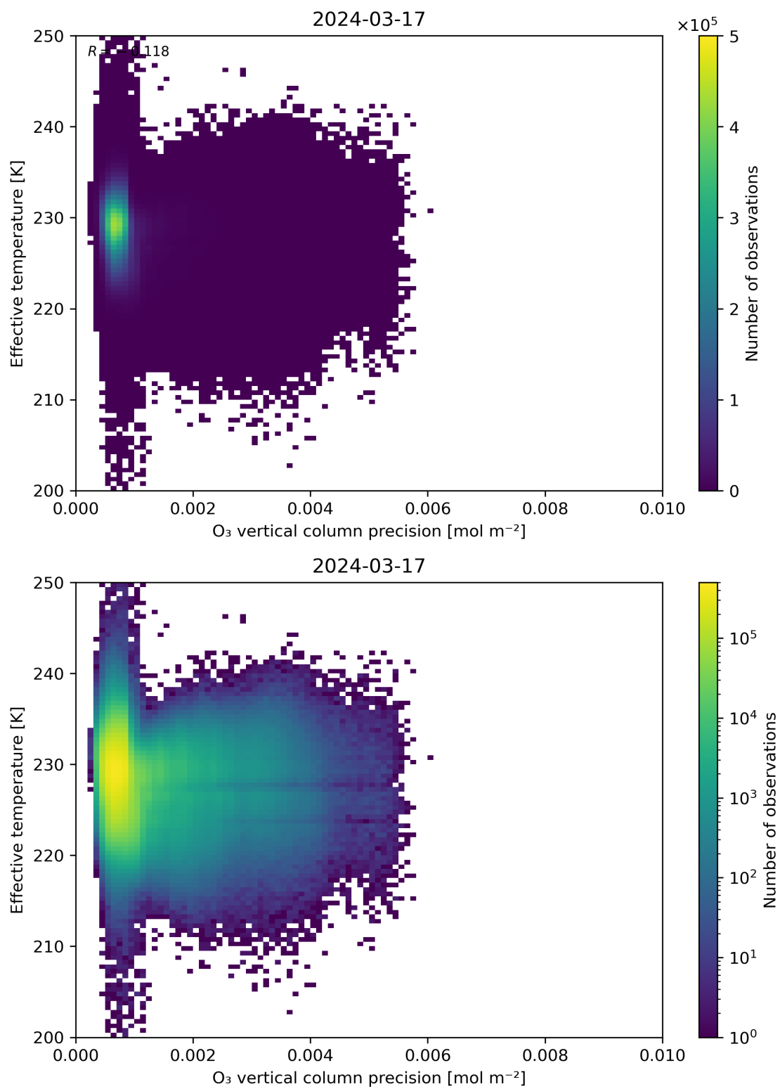
Figure 42: Scatter density plot of “O 3 vertical column precision” against “Effective temperature” for 2024-03-16 to 2024-03-18.
