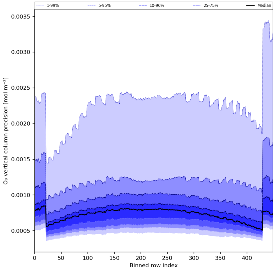
Figure 29: Along track statistics of “O 3 vertical column precision” for 2024-03-16 to 2024-03-18
