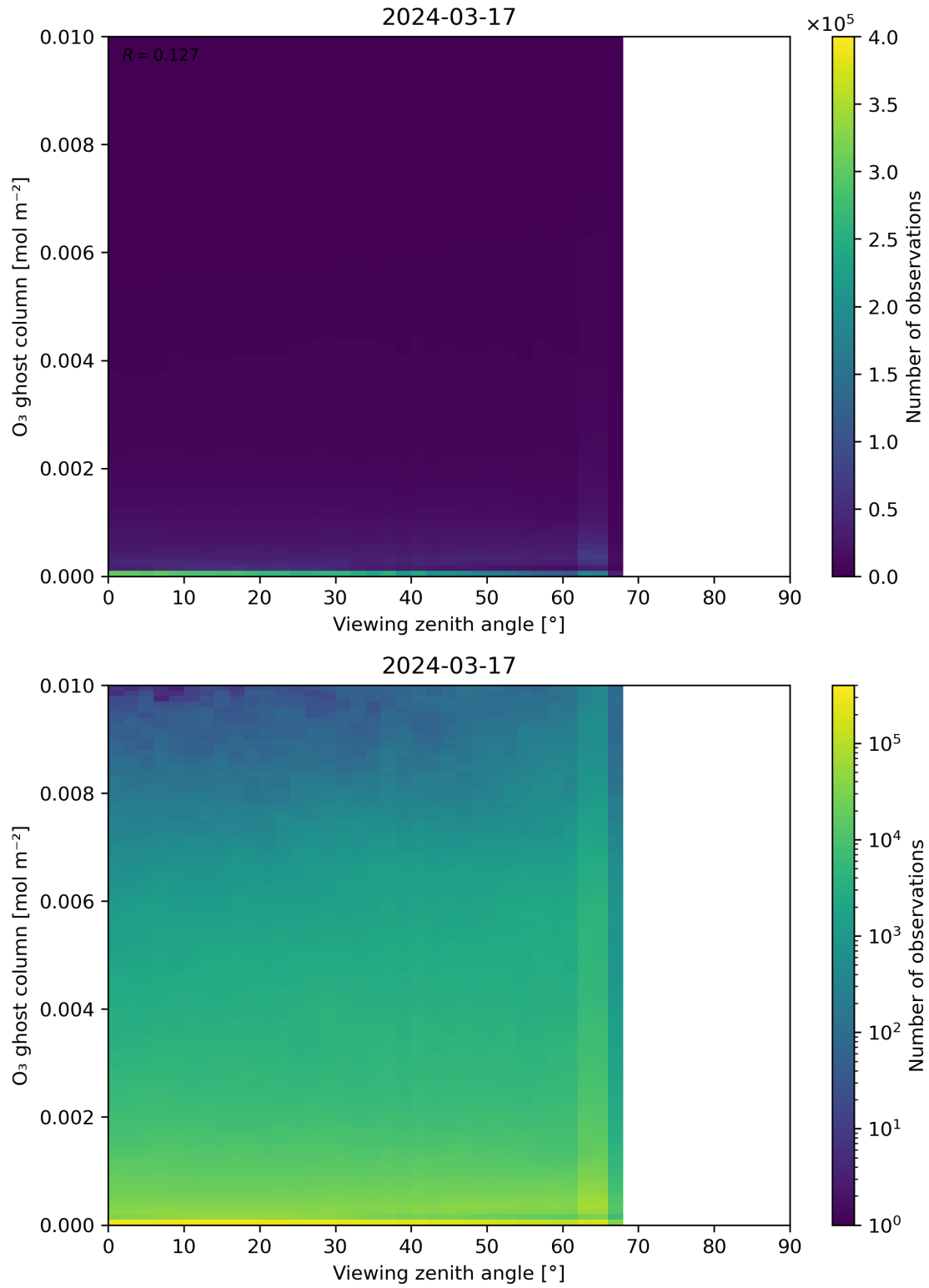
Figure 51: Scatter density plot of “Viewing zenith angle” against “O 3 ghost column” for 2024-03-16 to 2024-03-18.
