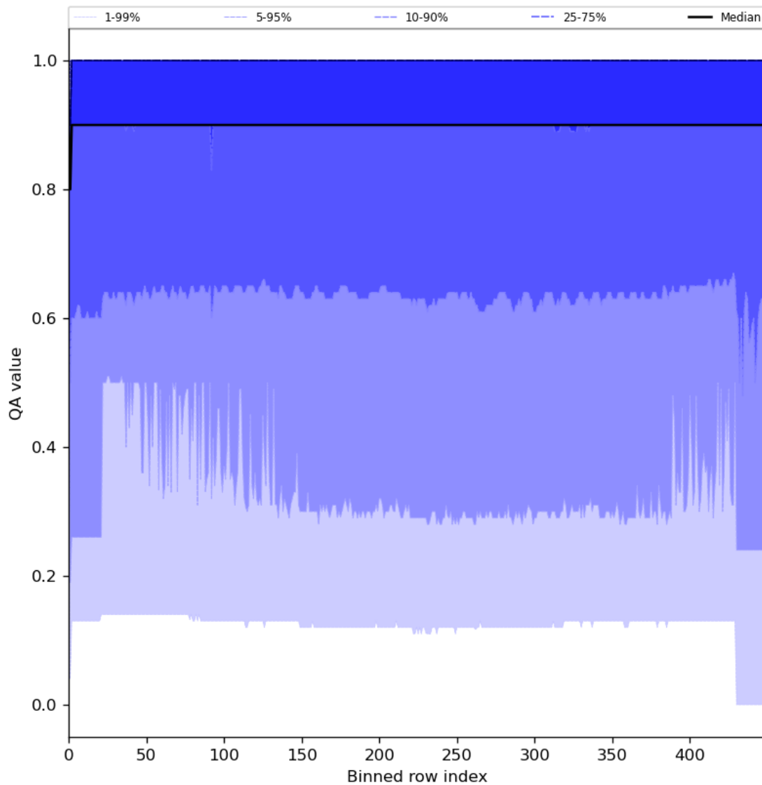
Figure 27: Along track statistics of “QA value” for 2024-03-16 to 2024-03-18
