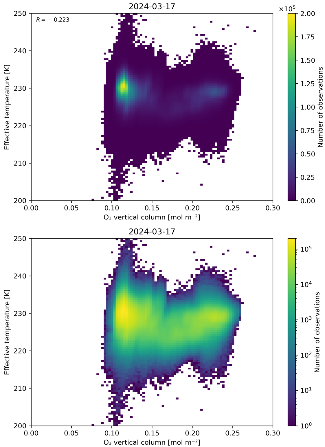
Figure 39: Scatter density plot of “O 3 vertical column” against “Effective temperature” for 2024-03-16 to 2024-03-18.
