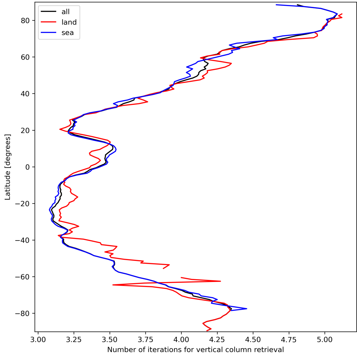
Figure 19: Zonal average of “Number of iterations for vertical column retrieval” for 2024-03-16 to 2024-03-18.
