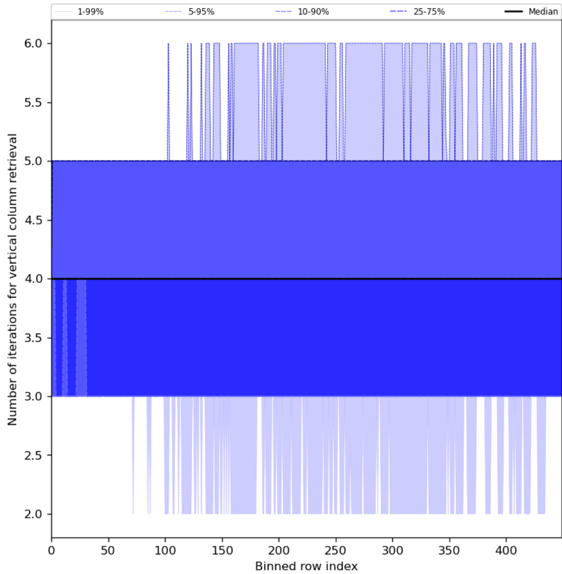
Figure 33: Along track statistics of “Number of iterations for vertical column retrieval” for 2024-03-16 to 2024-03-18
