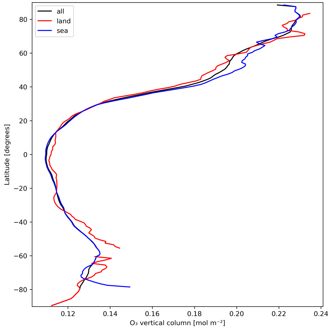
Figure 14: Zonal average of “O 3 vertical column” for 2024-03-16 to 2024-03-18.
