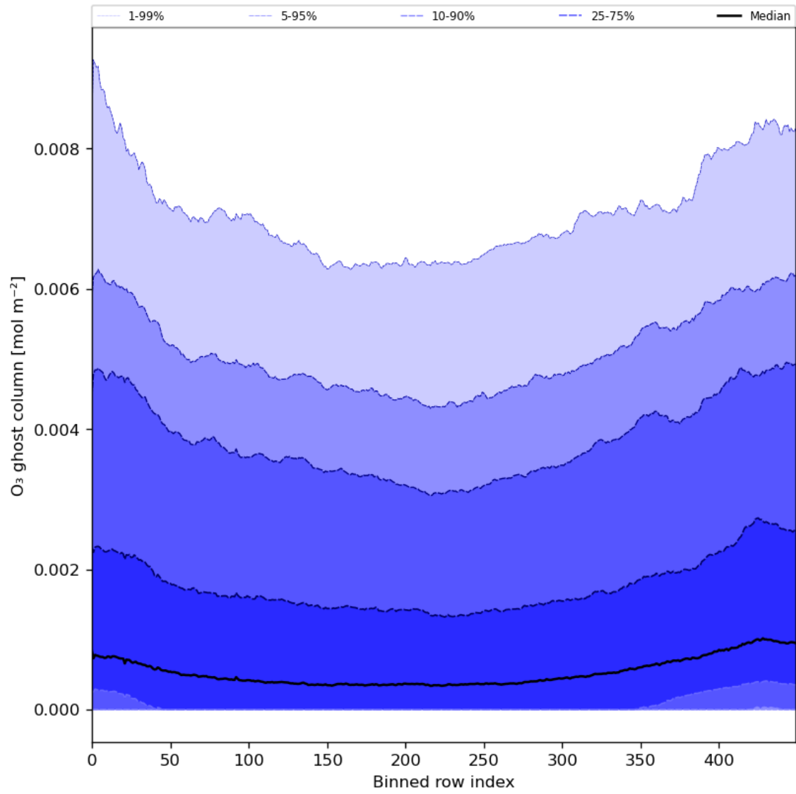
Figure 32: Along track statistics of “O 3 ghost column” for 2024-03-16 to 2024-03-18
