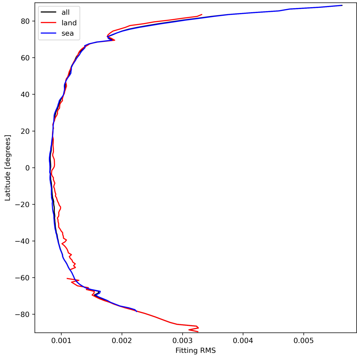
Figure 16: Zonal average of “Fitting RMS” for 2024-03-16 to 2024-03-18.
