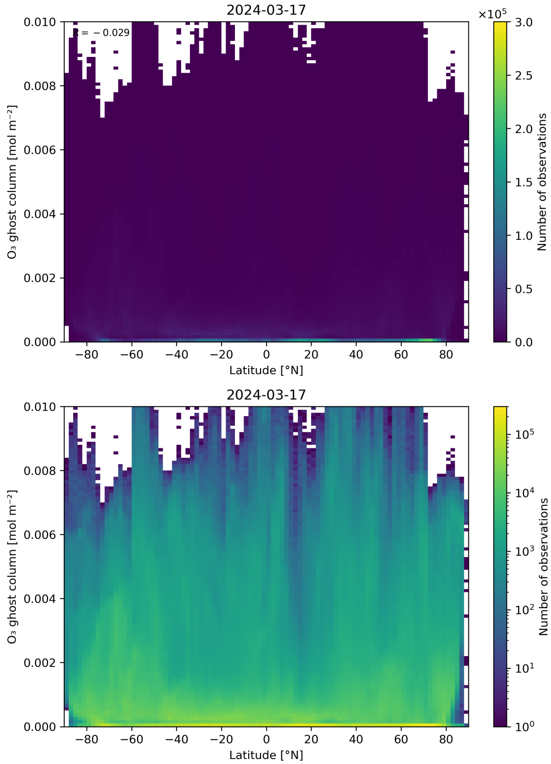
Figure 35: Scatter density plot of “Latitude” against “O 3 ghost column” for 2024-03-16 to 2024-03-18.
