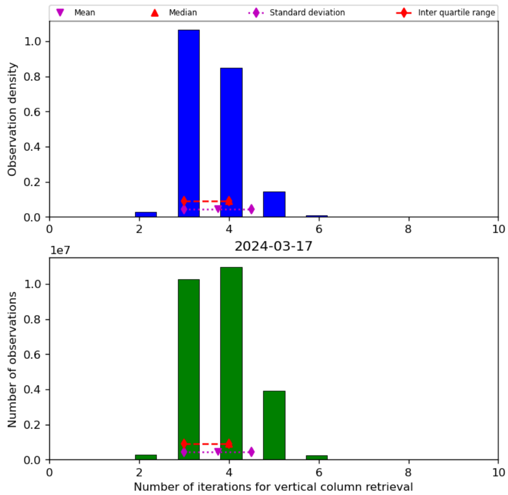
Figure 26: Histogram of “Number of iterations for vertical column retrieval” for 2024-03-16 to 2024-03-18
