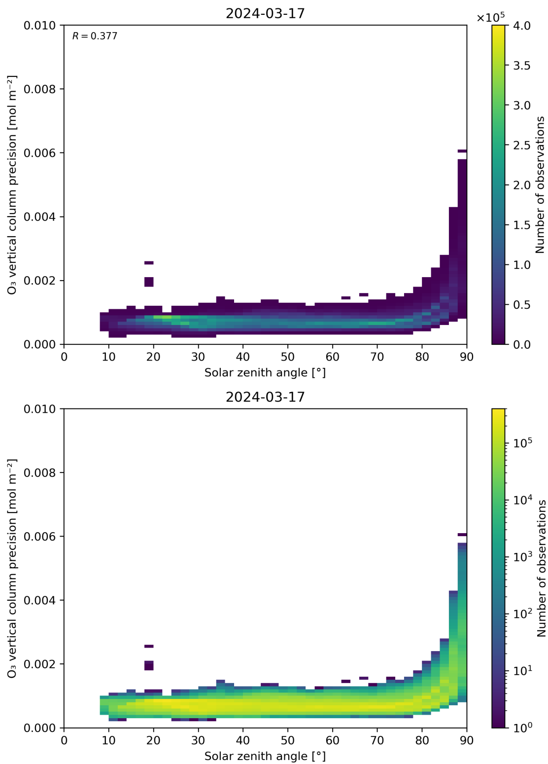
Figure 48: Scatter density plot of “Solar zenith angle” against “O 3 vertical column precision” for 2024-03-16 to 2024-03-18.
