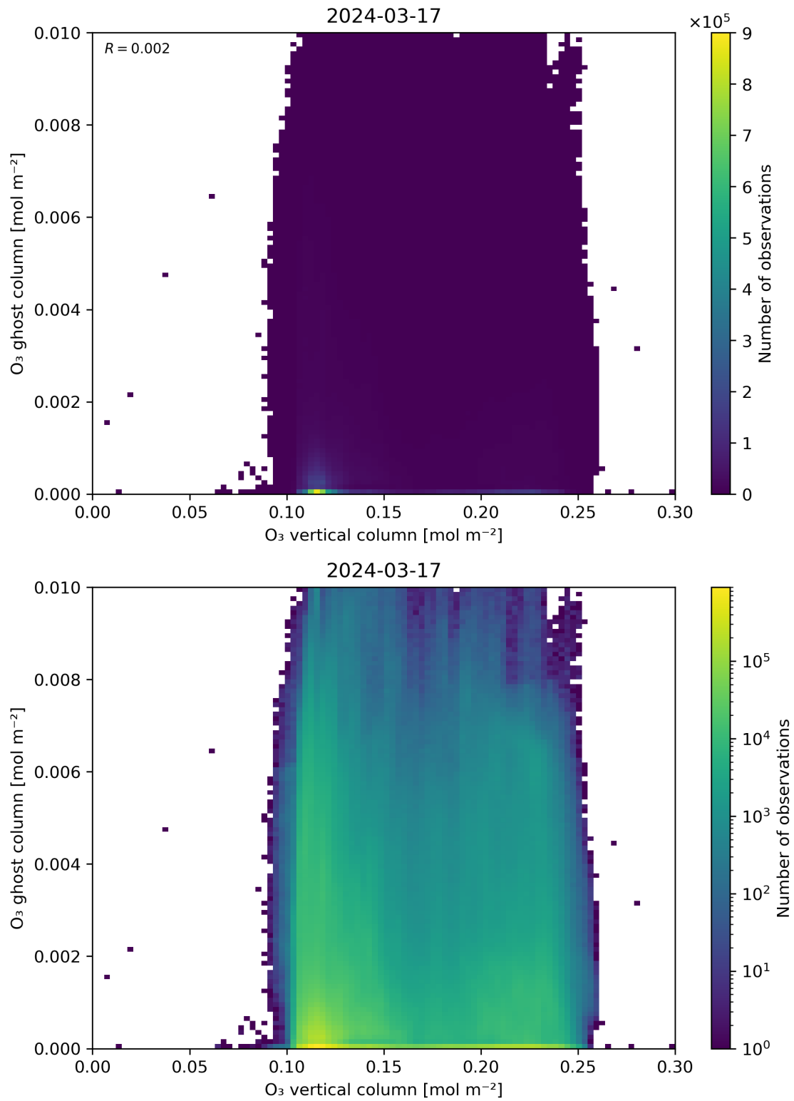
Figure 40: Scatter density plot of “O 3 vertical column” against “O 3 ghost column” for 2024-03-16 to 2024-03-18.
