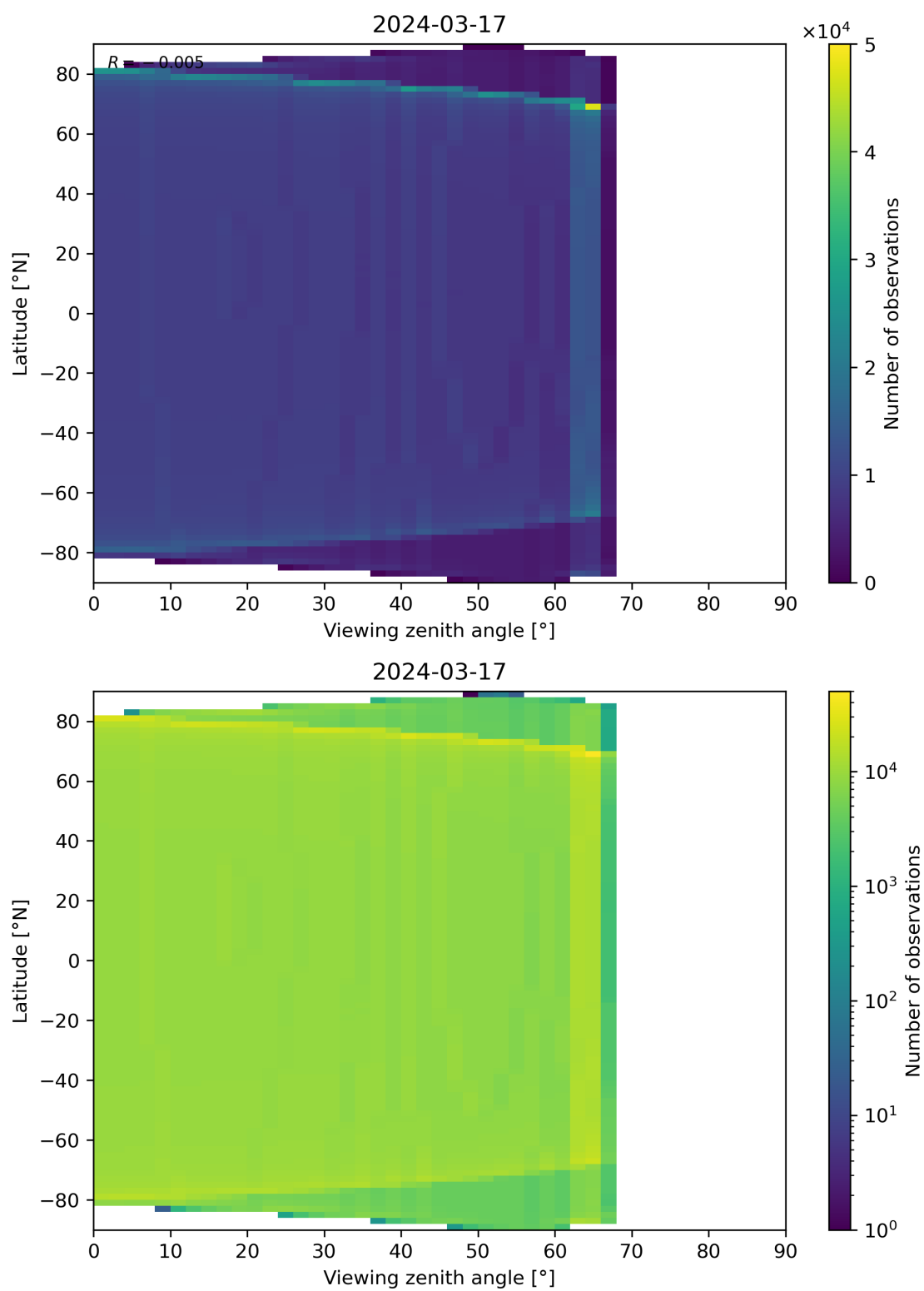
Figure 49: Scatter density plot of “Viewing zenith angle” against “Latitude” for 2024-03-16 to 2024-03-18.
