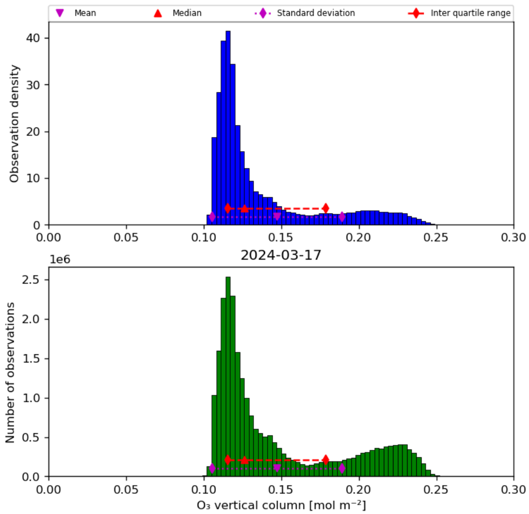
Figure 21: Histogram of “O 3 vertical column” for 2024-03-16 to 2024-03-18
