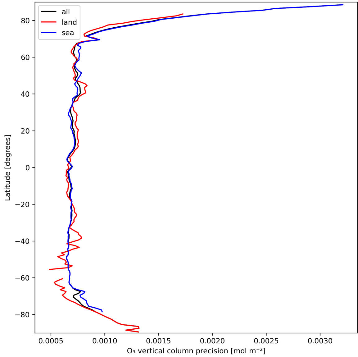
Figure 15: Zonal average of “O 3 vertical column precision” for 2024-03-16 to 2024-03-18.
