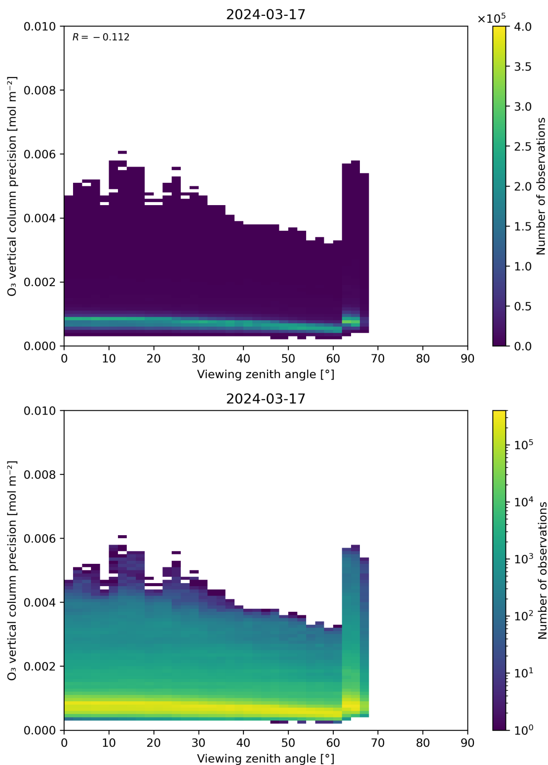
Figure 53: Scatter density plot of “Viewing zenith angle” against “O 3 vertical column precision” for 2024-03-16 to 2024-03-18.
