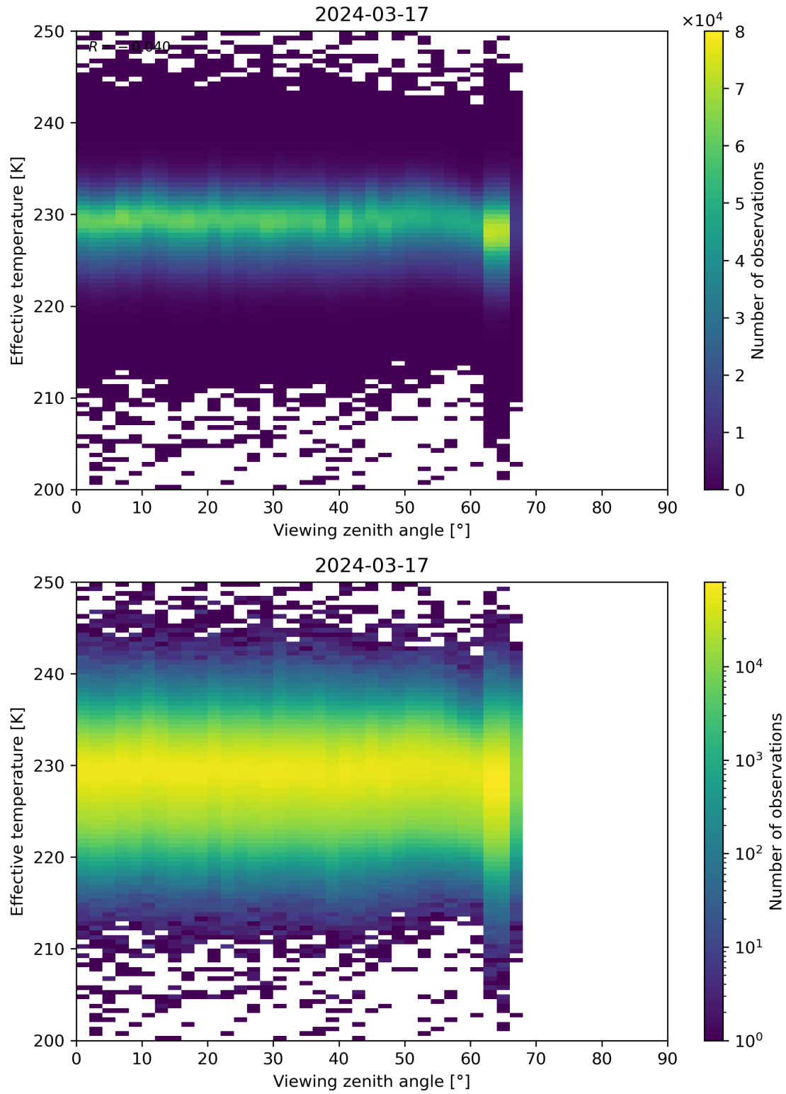
Figure 50: Scatter density plot of “Viewing zenith angle” against “Effective temperature” for 2024-03-16 to 2024-03-18.
