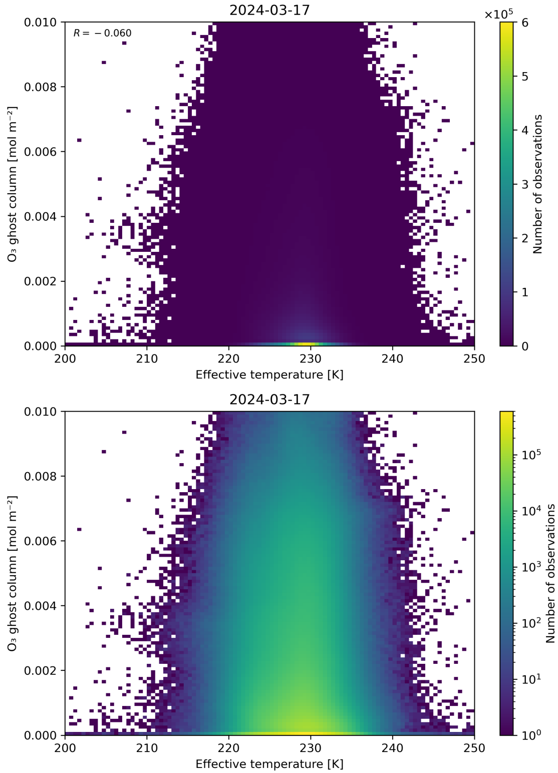
Figure 38: Scatter density plot of “Effective temperature” against “O 3 ghost column” for 2024-03-16 to 2024-03-18.
