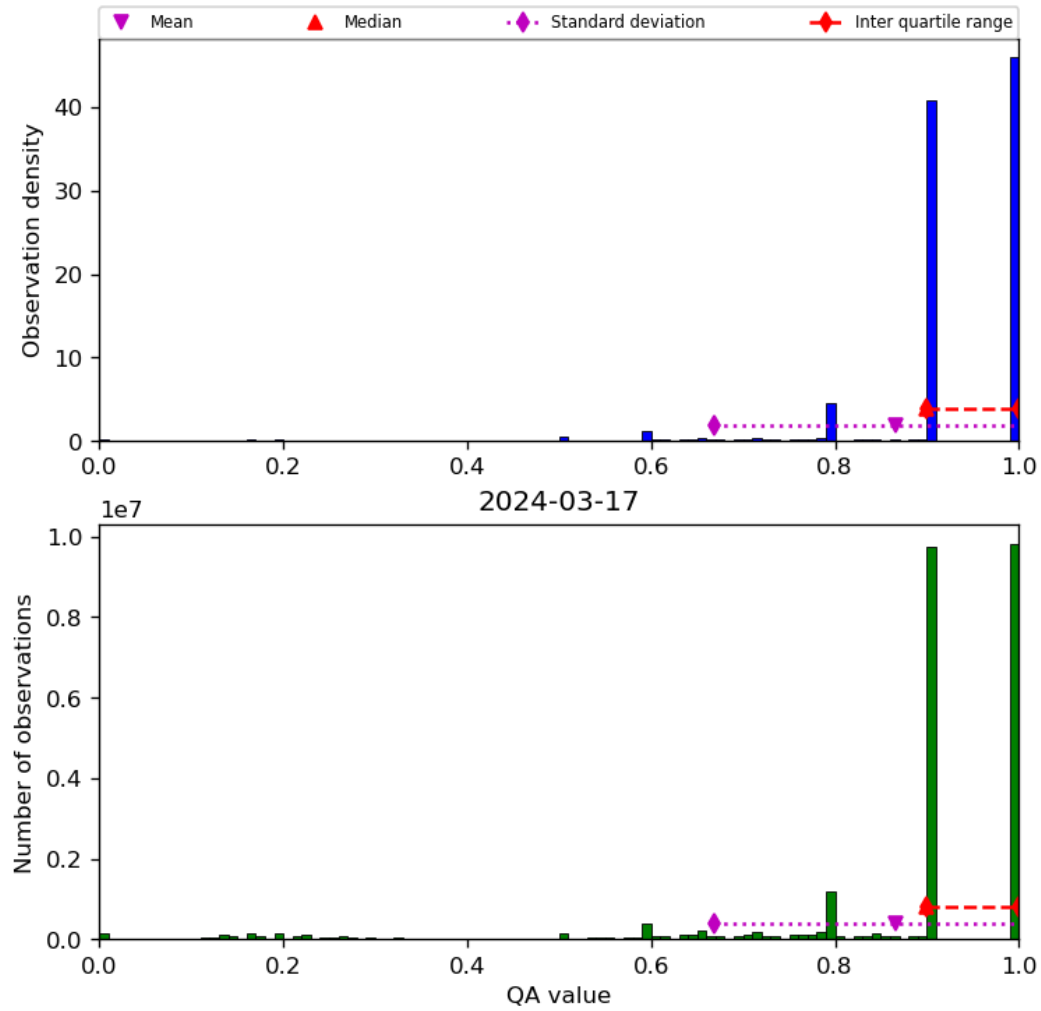
Figure 20: Histogram of “QA value” for 2024-03-16 to 2024-03-18
