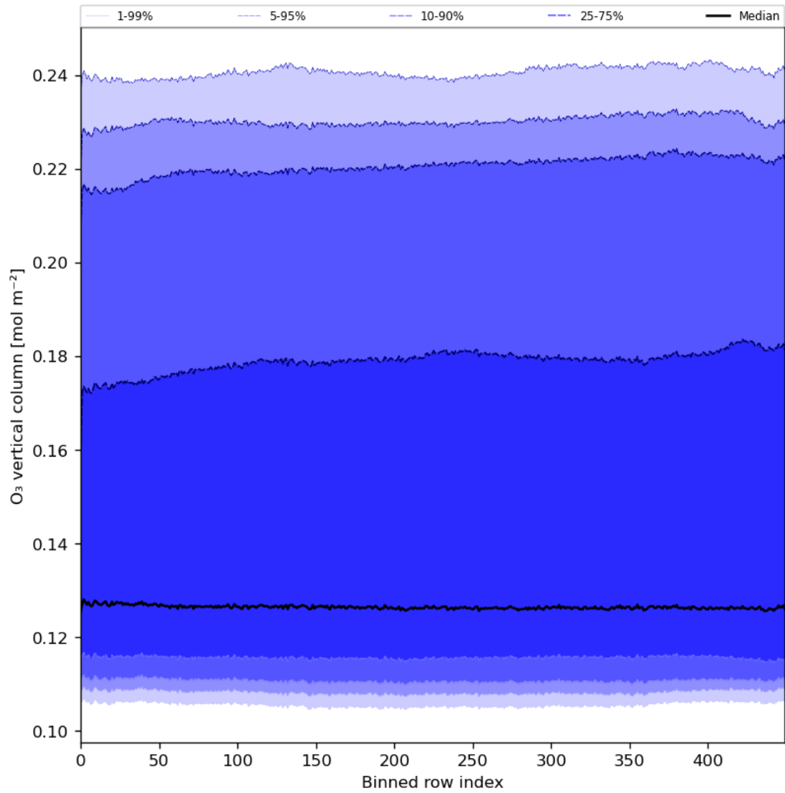
Figure 28: Along track statistics of “O 3 vertical column” for 2024-03-16 to 2024-03-18
