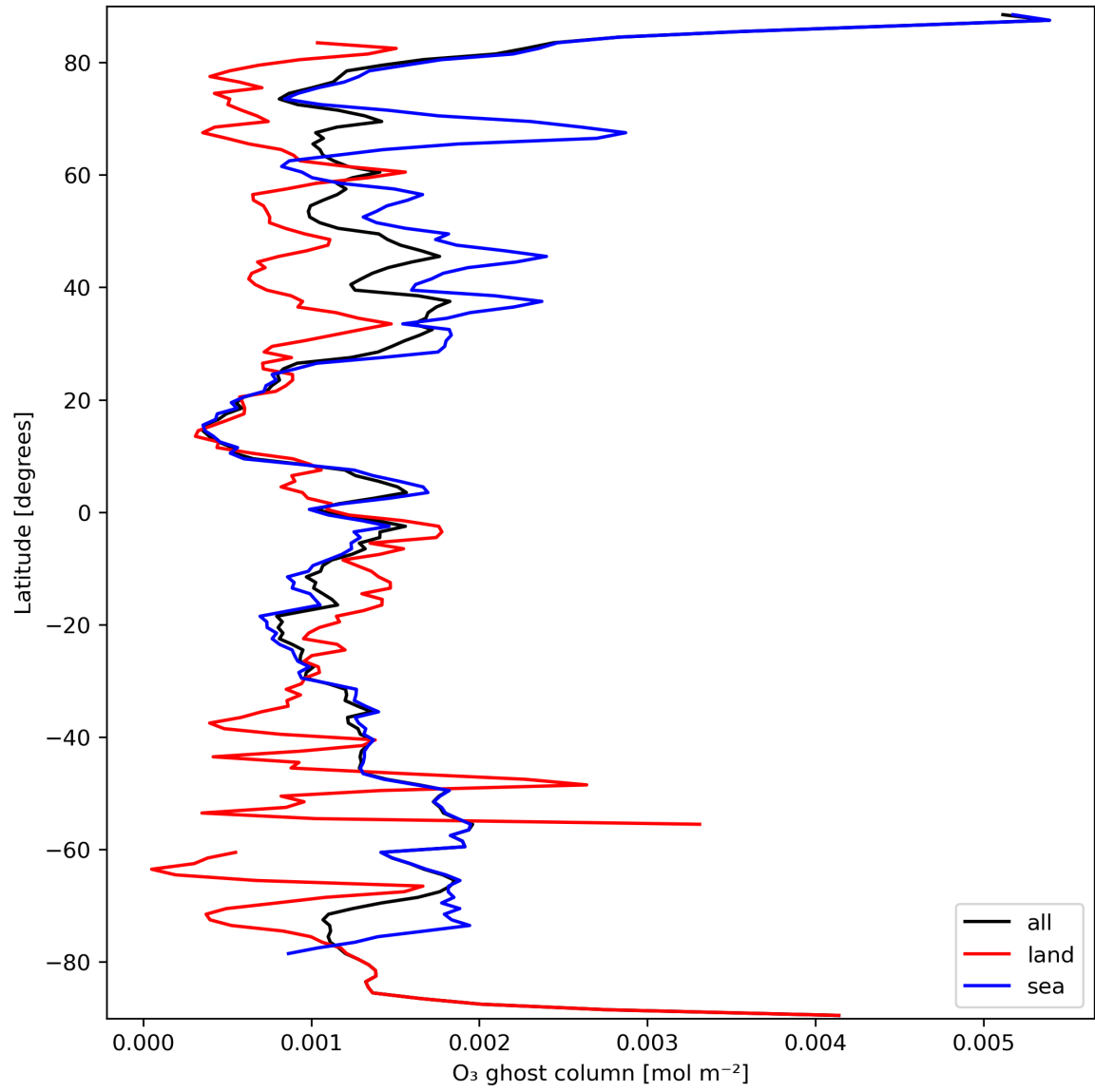
Figure 18: Zonal average of “O 3 ghost column” for 2024-03-16 to 2024-03-18.
