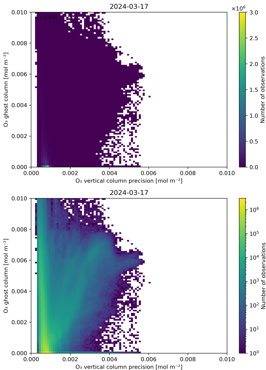
Figure 43: Scatter density plot of “O 3 vertical column precision” against “O 3 ghost column” for 2024-03-16 to 2024-03-18.
