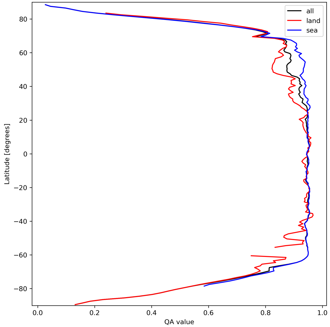
Figure 13: Zonal average of “QA value” for 2024-03-16 to 2024-03-18.
