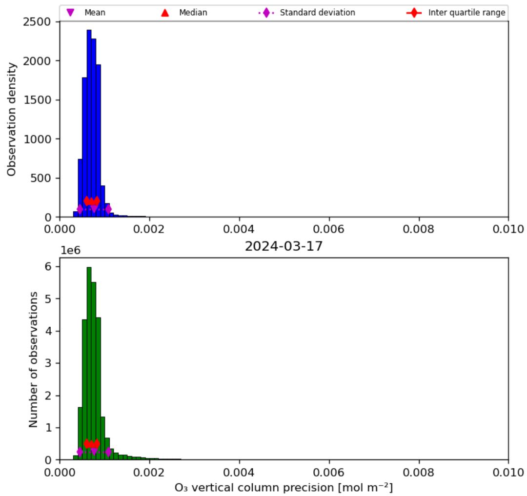
Figure 22: Histogram of “O 3 vertical column precision” for 2024-03-16 to 2024-03-18
