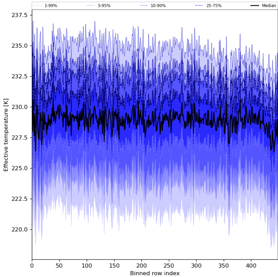
Figure 31: Along track statistics of “Effective temperature” for 2024-03-16 to 2024-03-18
