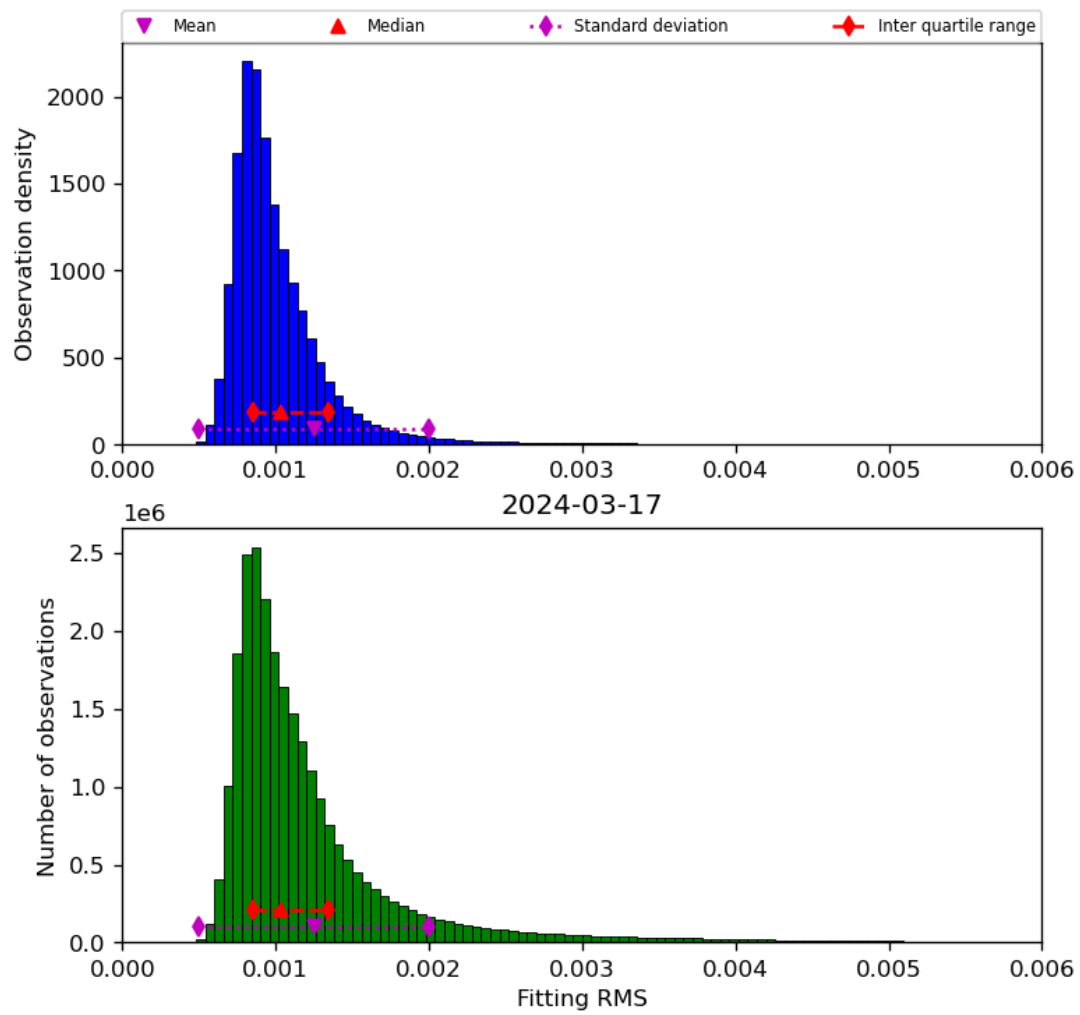
Figure 23: Histogram of “Fitting RMS” for 2024-03-16 to 2024-03-18
