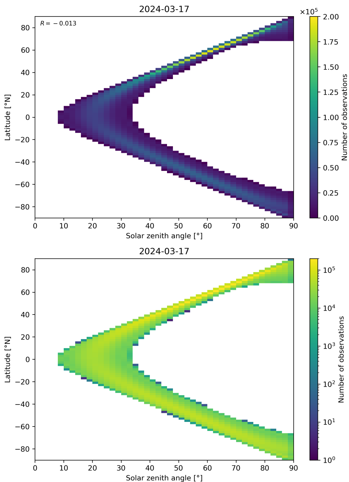
Figure 44: Scatter density plot of “Solar zenith angle” against “Latitude” for 2024-03-16 to 2024-03-18.
