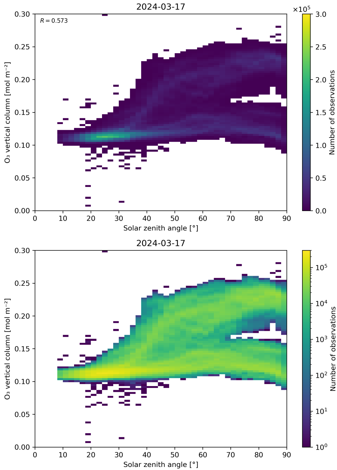
Figure 47: Scatter density plot of “Solar zenith angle” against “O 3 vertical column” for 2024-03-16 to 2024-03-18.
