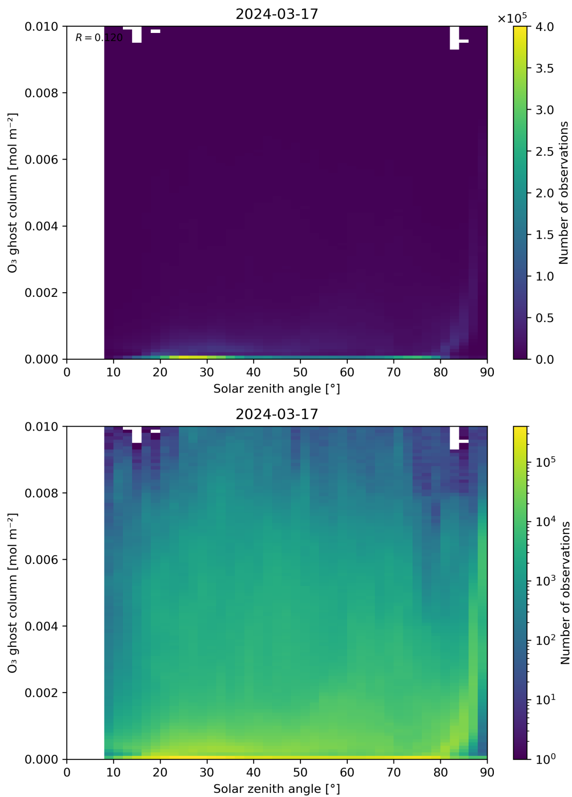
Figure 46: Scatter density plot of “Solar zenith angle” against “O 3 ghost column” for 2024-03-16 to 2024-03-18.
