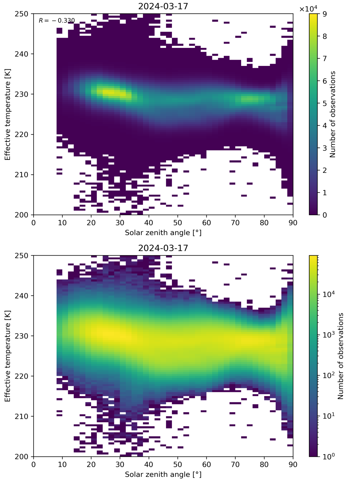
Figure 45: Scatter density plot of “Solar zenith angle” against “Effective temperature” for 2024-03-16 to 2024-03-18.
