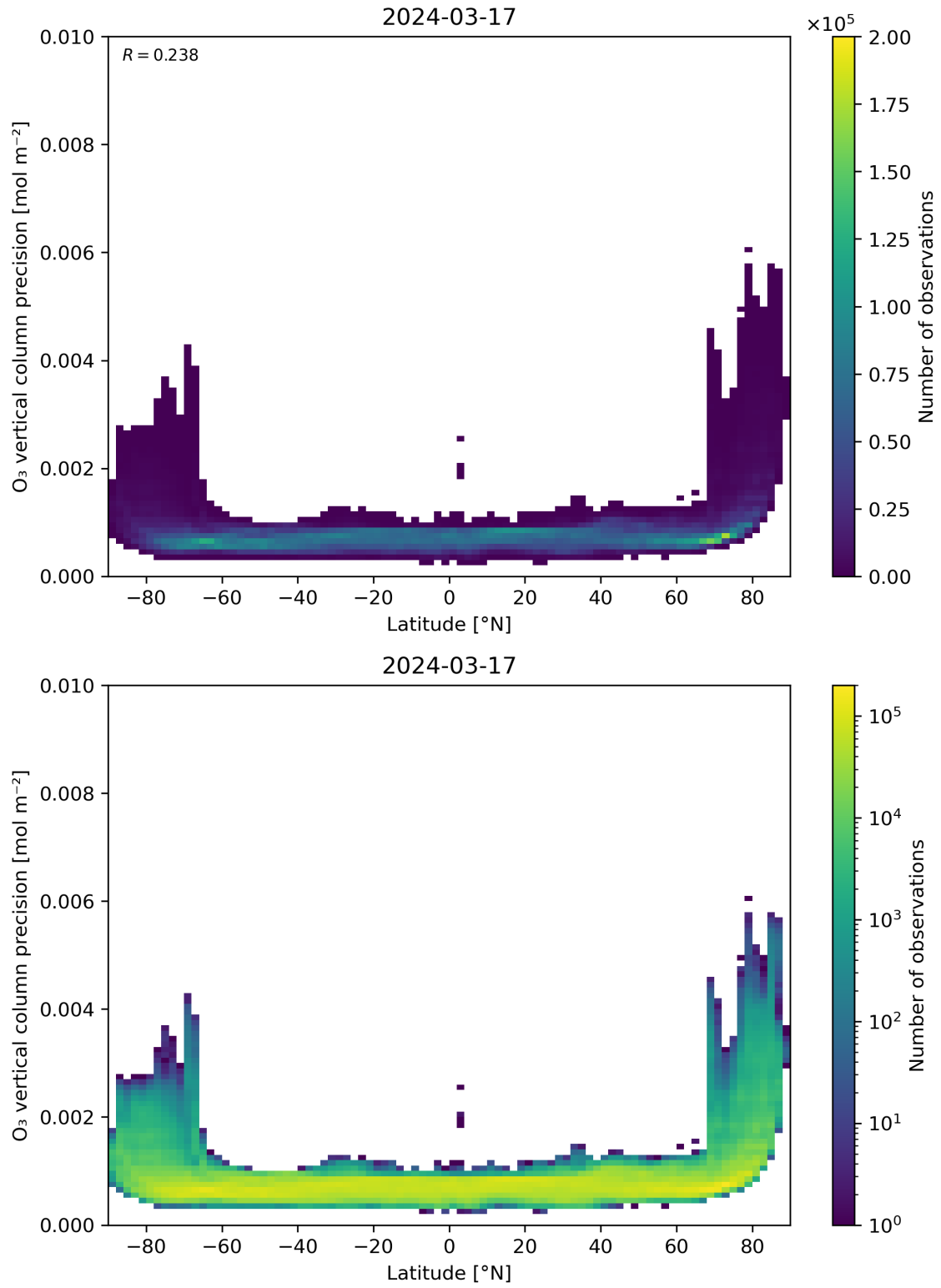
Figure 37: Scatter density plot of “Latitude” against “O 3 vertical column precision” for 2024-03-16 to 2024-03-18.
