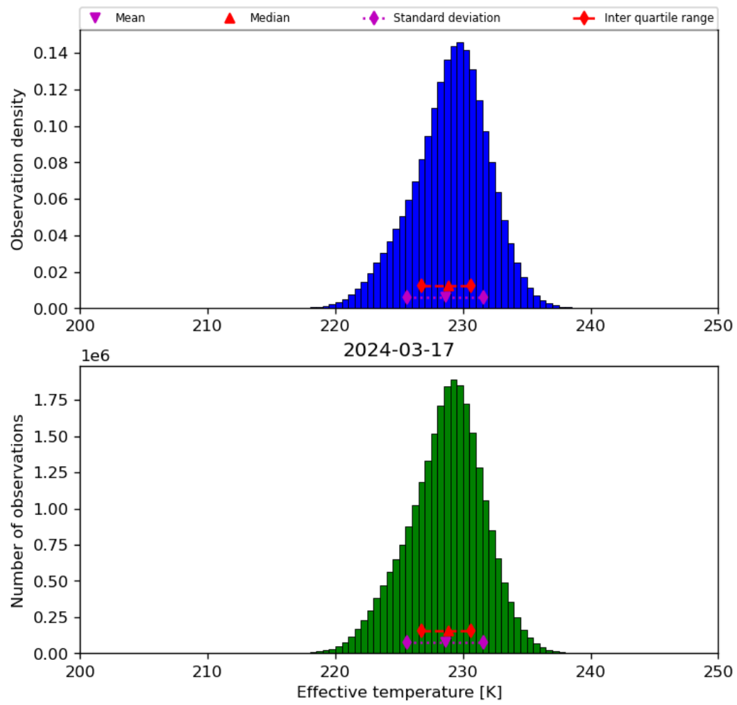
Figure 24: Histogram of “Effective temperature” for 2024-03-16 to 2024-03-18
