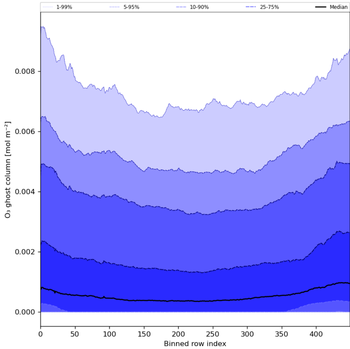
Figure 32: Along track statistics of “O 3 ghost column” for 2024-03-17 to 2024-03-19
