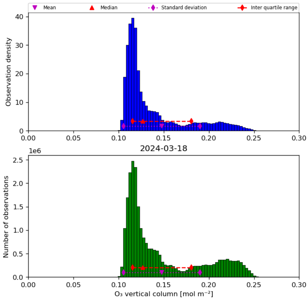
Figure 21: Histogram of “O 3 vertical column” for 2024-03-17 to 2024-03-19
