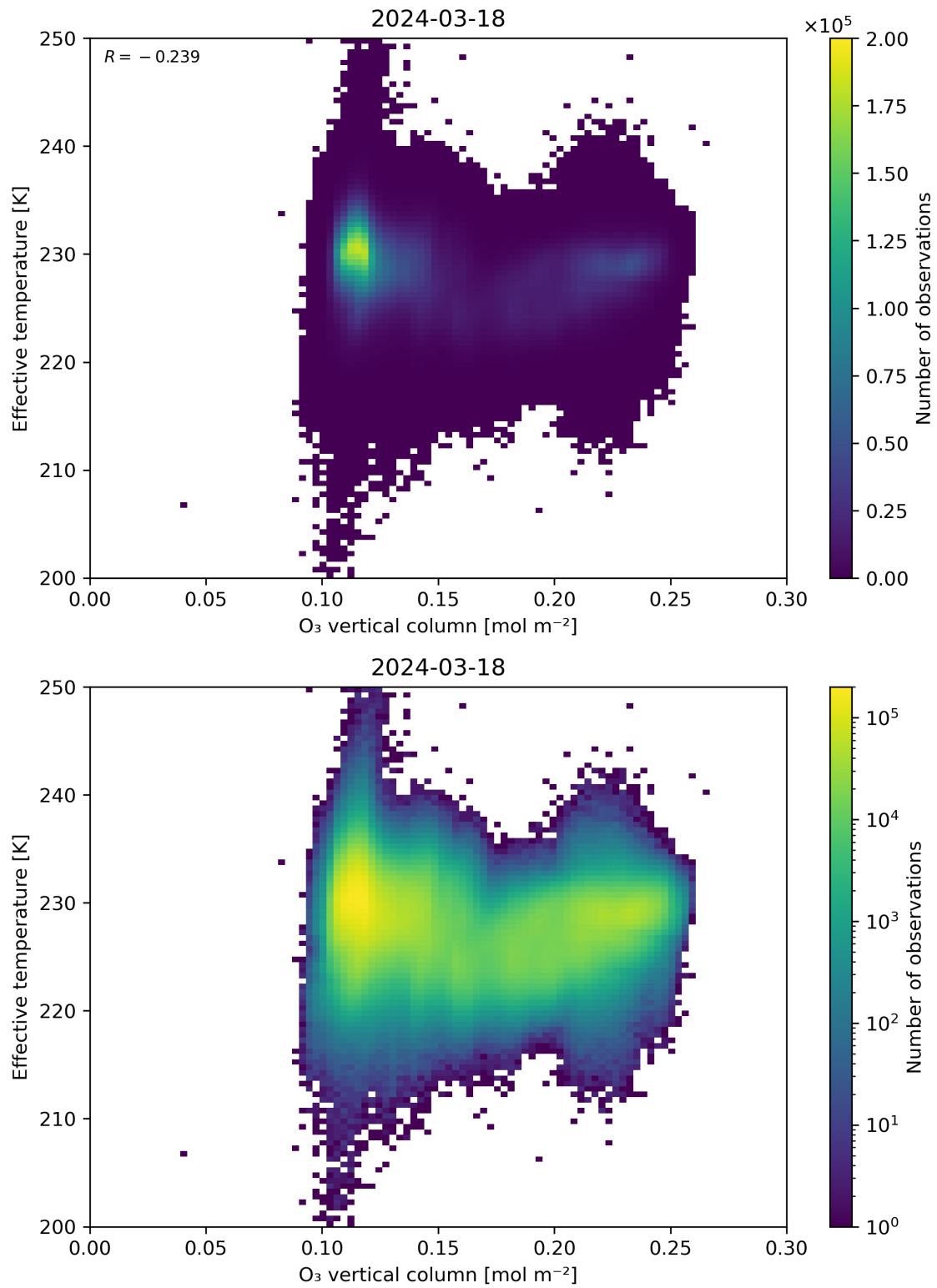
Figure 39: Scatter density plot of “O 3 vertical column” against “Effective temperature” for 2024-03-17 to 2024-03-19.
