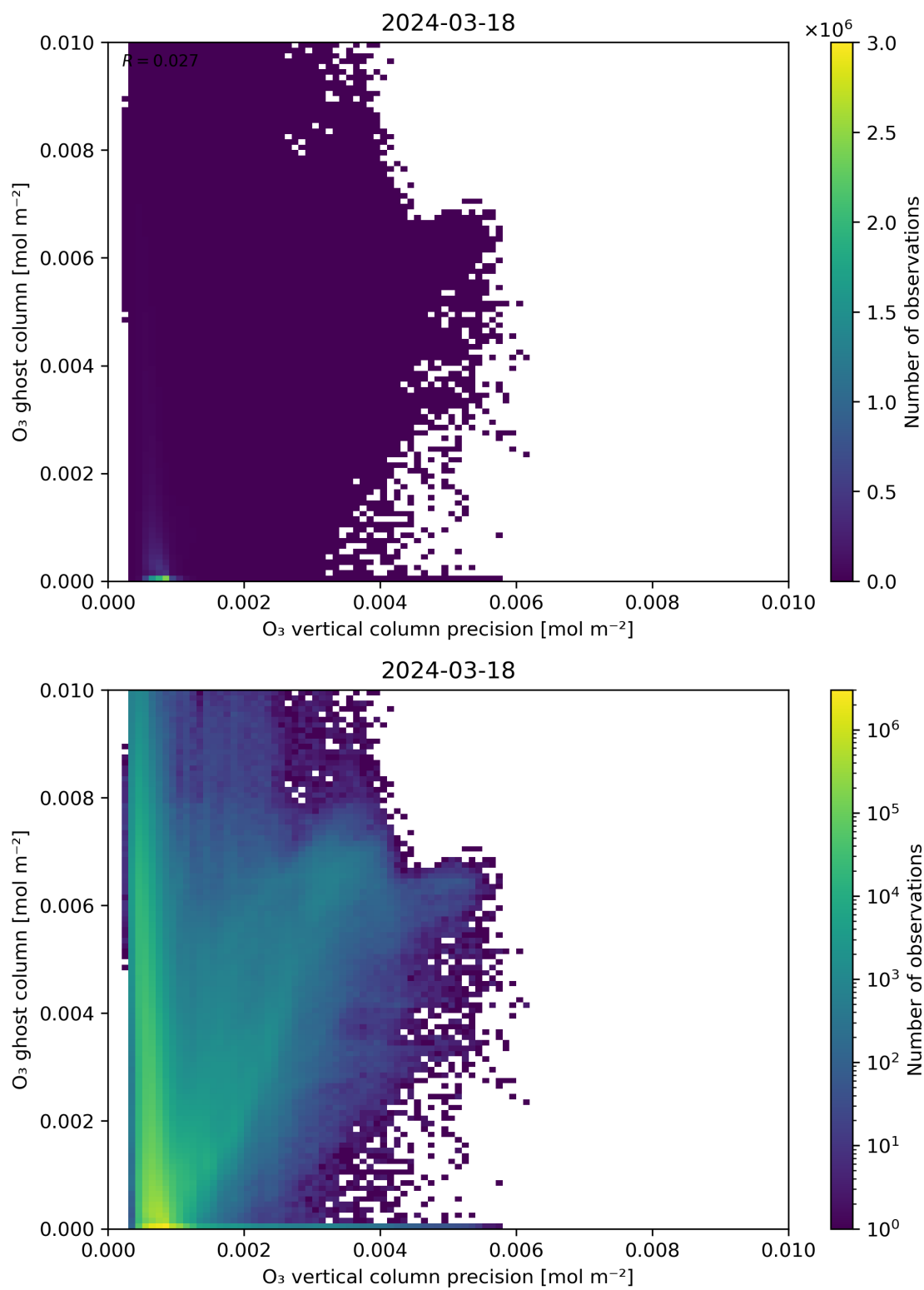
Figure 43: Scatter density plot of “O 3 vertical column precision” against “O 3 ghost column” for 2024-03-17 to 2024-03-19.
