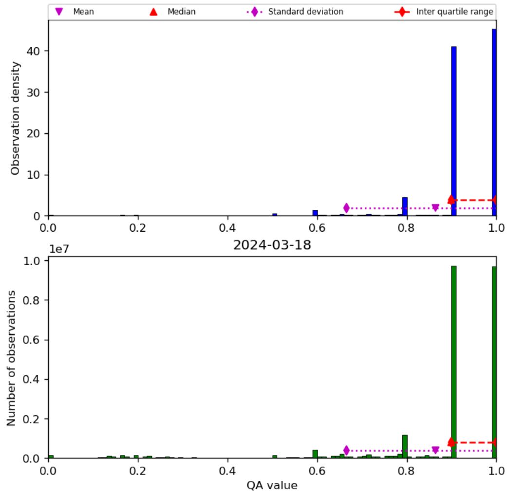
Figure 20: Histogram of “QA value” for 2024-03-17 to 2024-03-19
