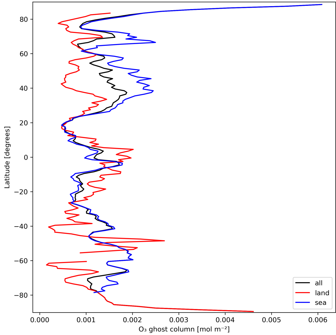
Figure 18: Zonal average of “O 3 ghost column” for 2024-03-17 to 2024-03-19.
