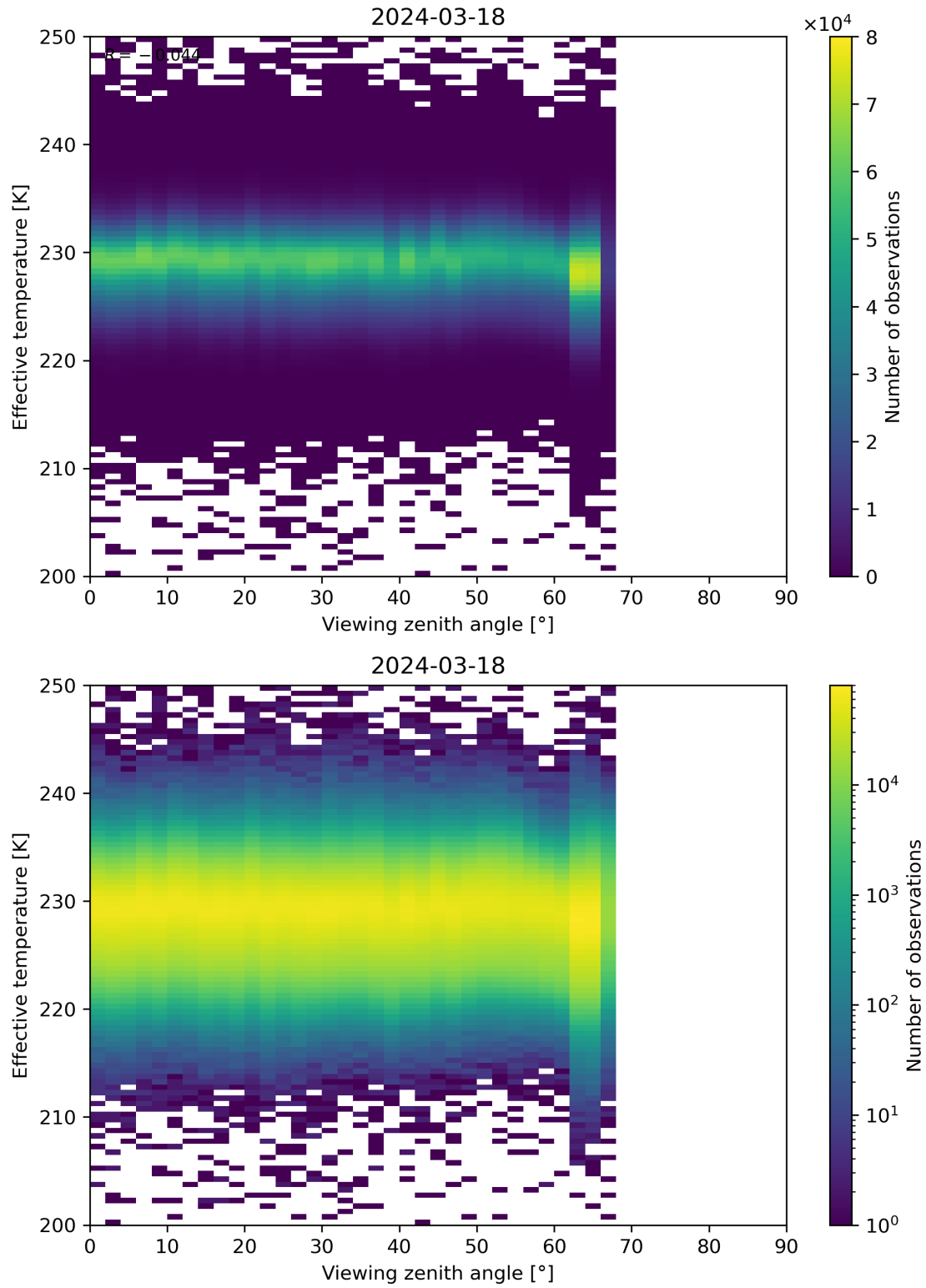
Figure 50: Scatter density plot of “Viewing zenith angle” against “Effective temperature” for 2024-03-17 to 2024-03-19.
