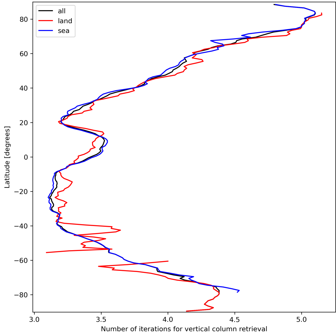
Figure 19: Zonal average of “Number of iterations for vertical column retrieval” for 2024-03-17 to 2024-03-19.
