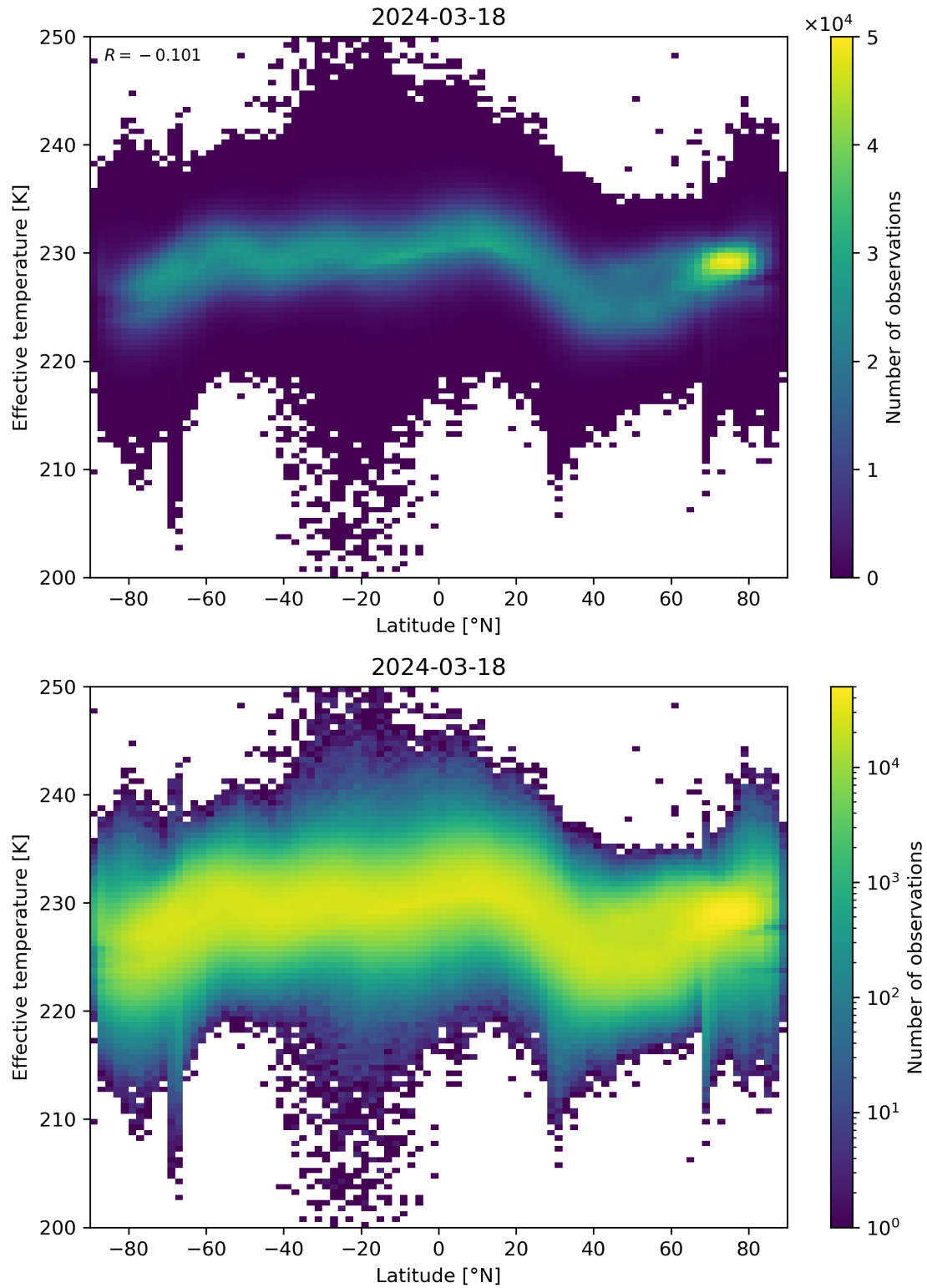
Figure 34: Scatter density plot of “Latitude” against “Effective temperature” for 2024-03-17 to 2024-03-19.
