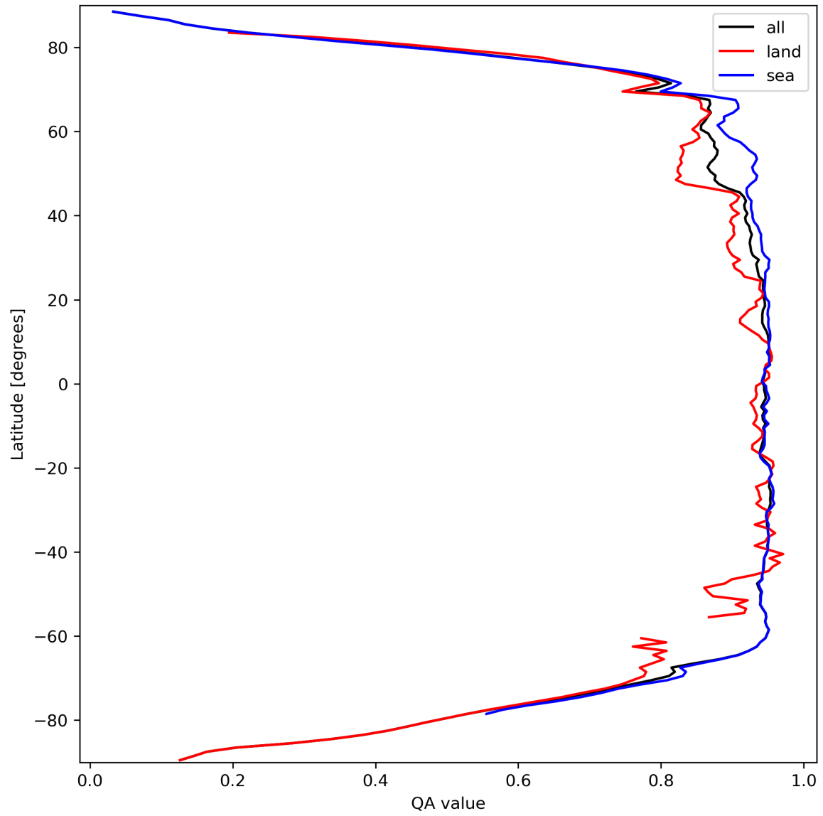
Figure 13: Zonal average of “QA value” for 2024-03-17 to 2024-03-19.
