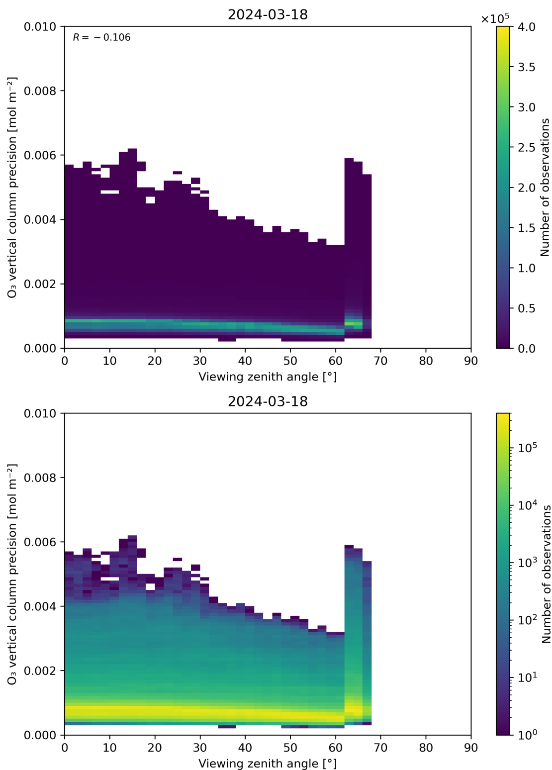
Figure 53: Scatter density plot of “Viewing zenith angle” against “O 3 vertical column precision” for 2024-03-17 to 2024-03-19.
