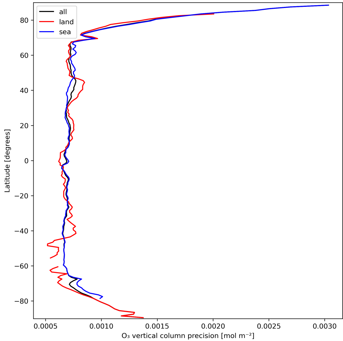
Figure 15: Zonal average of “O 3 vertical column precision” for 2024-03-17 to 2024-03-19.
