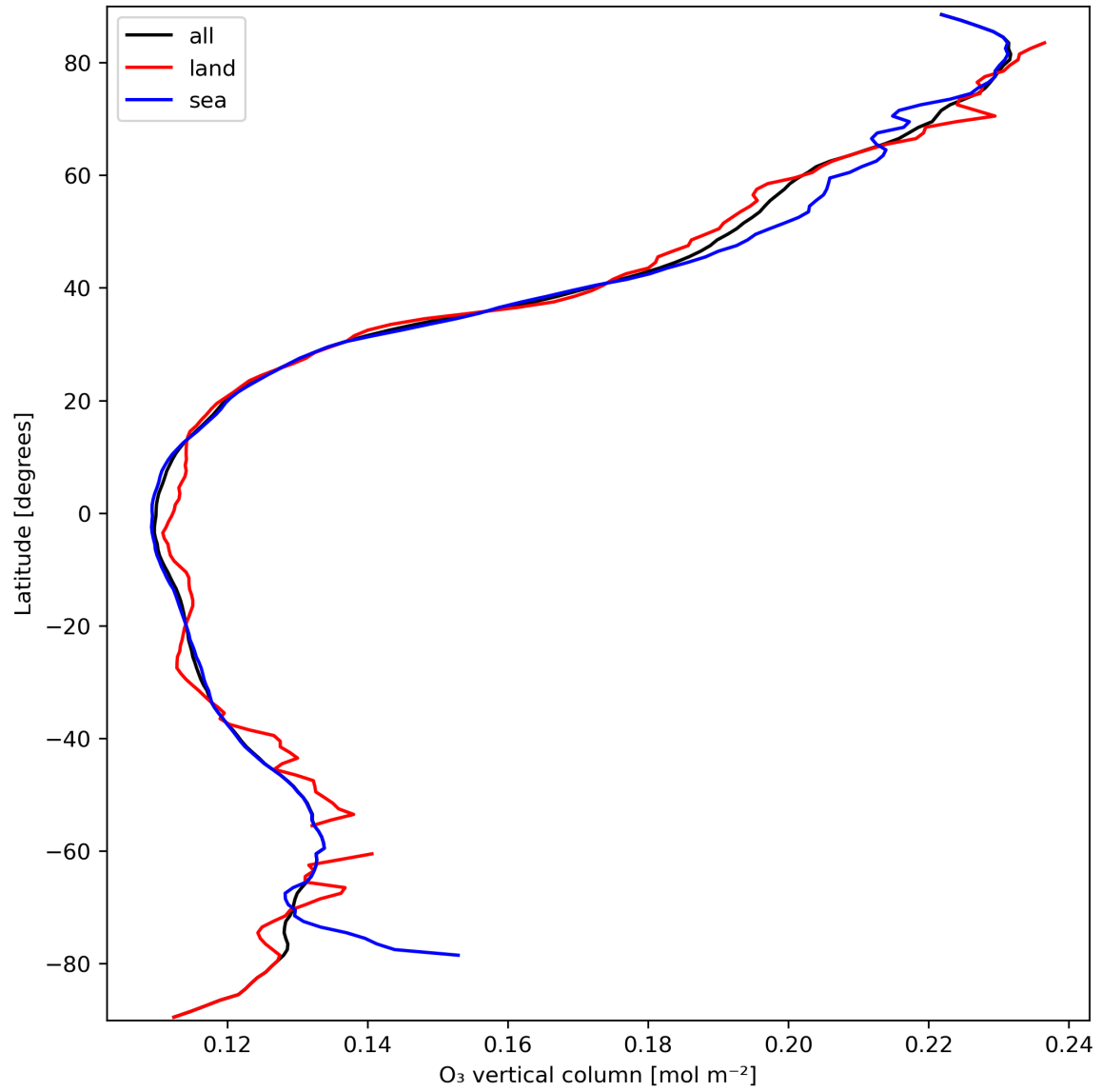
Figure 14: Zonal average of “O 3 vertical column” for 2024-03-17 to 2024-03-19.
