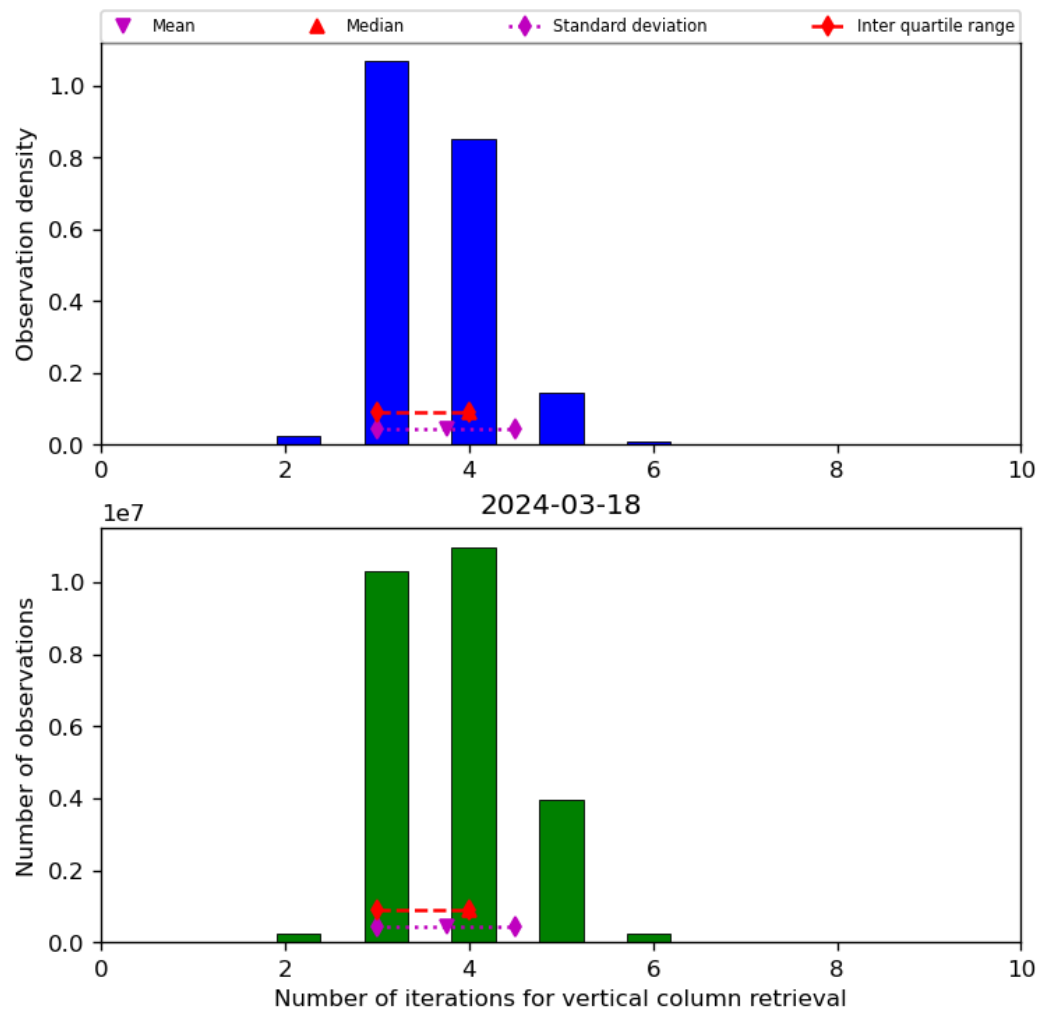
Figure 26: Histogram of “Number of iterations for vertical column retrieval” for 2024-03-17 to 2024-03-19
