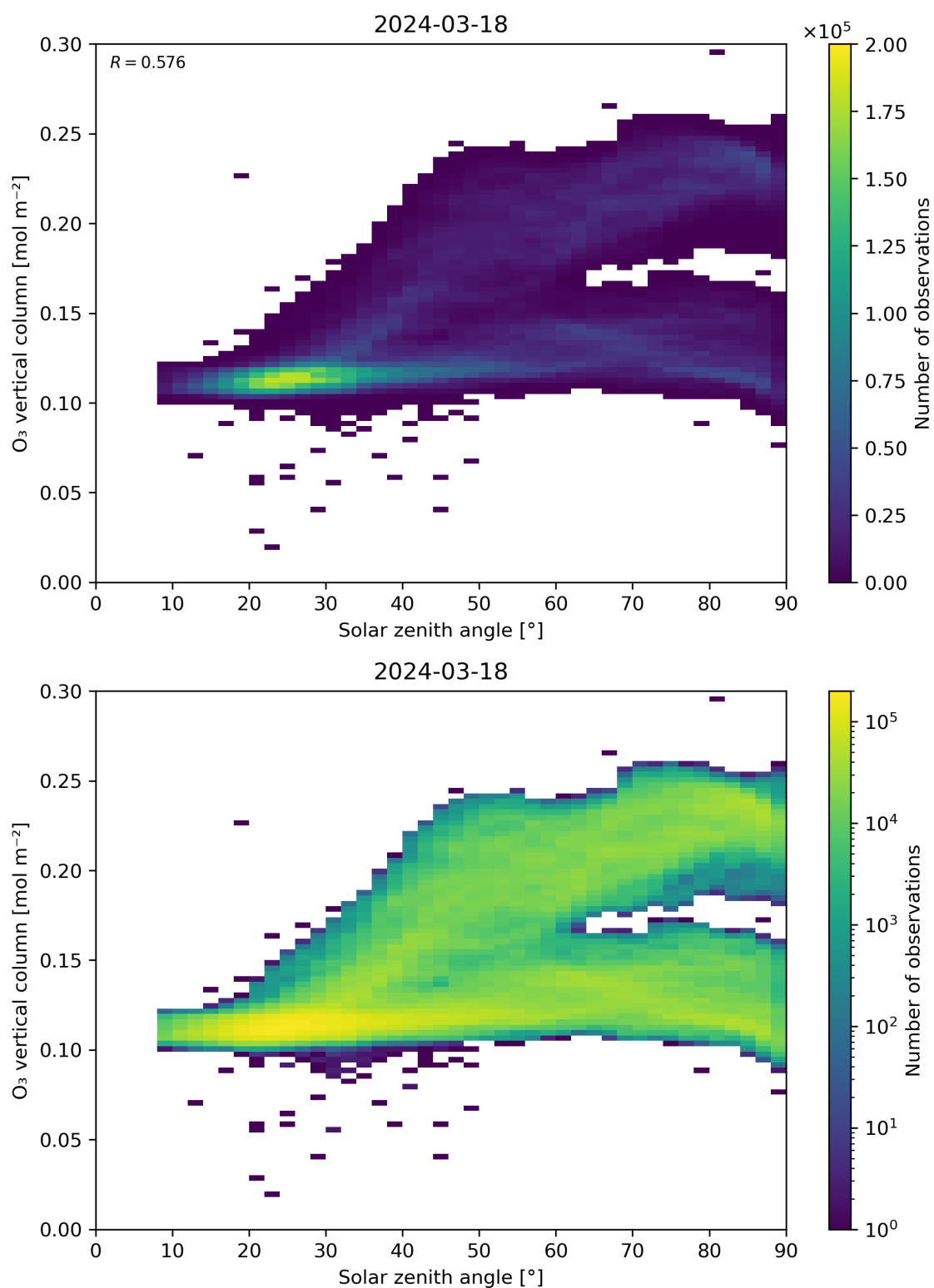
Figure 47: Scatter density plot of “Solar zenith angle” against “O 3 vertical column” for 2024-03-17 to 2024-03-19.
