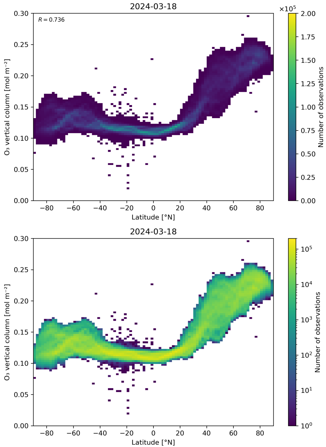
Figure 36: Scatter density plot of “Latitude” against “O 3 vertical column” for 2024-03-17 to 2024-03-19.
