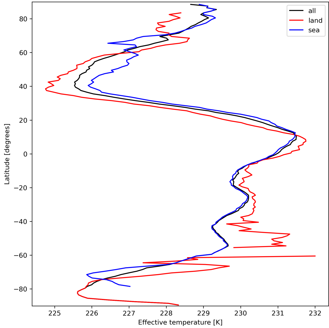
Figure 17: Zonal average of “Effective temperature” for 2024-03-17 to 2024-03-19.
