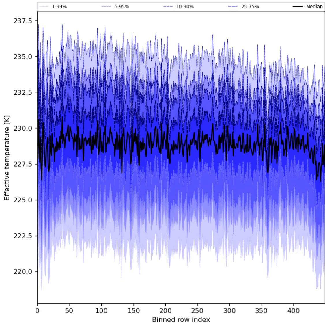
Figure 31: Along track statistics of “Effective temperature” for 2024-03-17 to 2024-03-19
