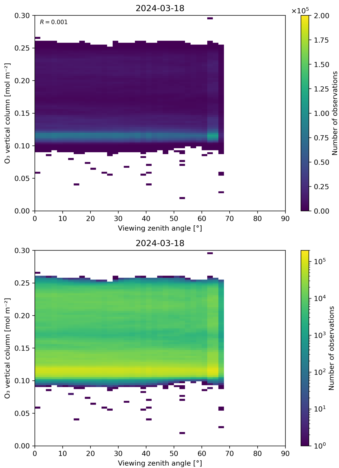
Figure 52: Scatter density plot of “Viewing zenith angle” against “O 3 vertical column” for 2024-03-17 to 2024-03-19.
