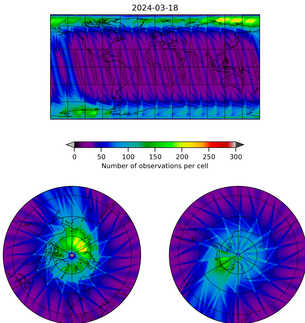
Figure 12: Map of the number of observations for 2024-03-17 to 2024-03-19
