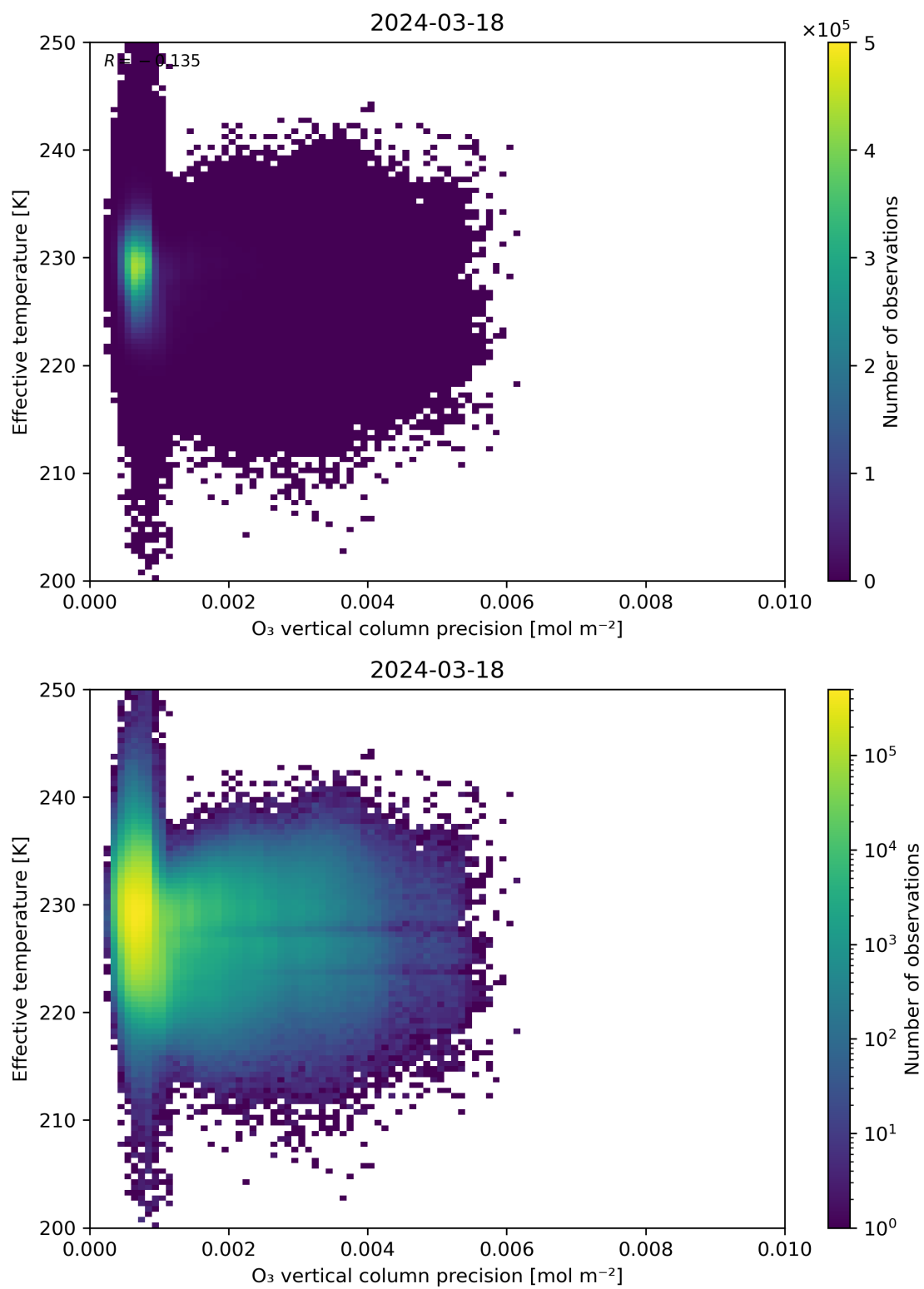
Figure 42: Scatter density plot of “O 3 vertical column precision” against “Effective temperature” for 2024-03-17 to 2024-03-19.
