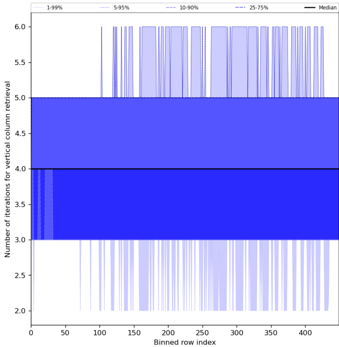
Figure 33: Along track statistics of “Number of iterations for vertical column retrieval” for 2024-03-17 to 2024-03-19
