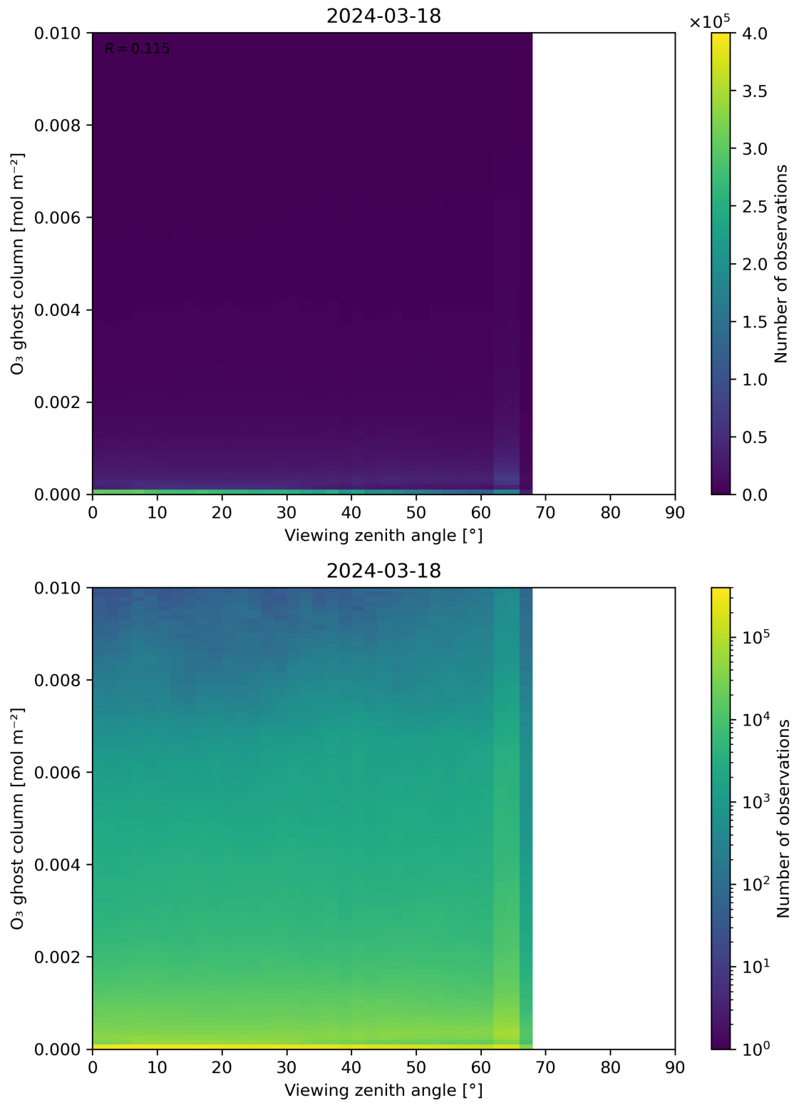
Figure 51: Scatter density plot of “Viewing zenith angle” against “O 3 ghost column” for 2024-03-17 to 2024-03-19.
