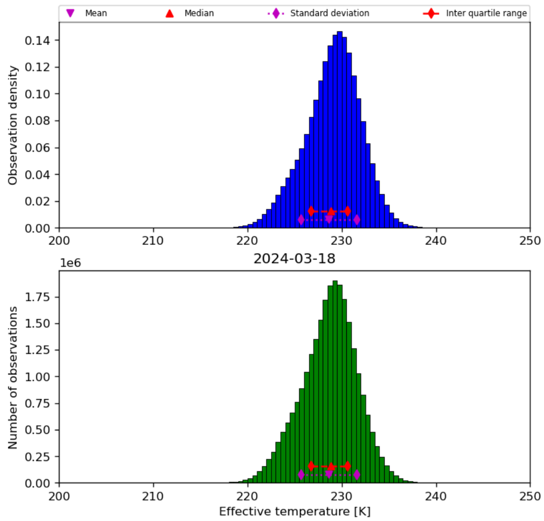
Figure 24: Histogram of “Effective temperature” for 2024-03-17 to 2024-03-19
