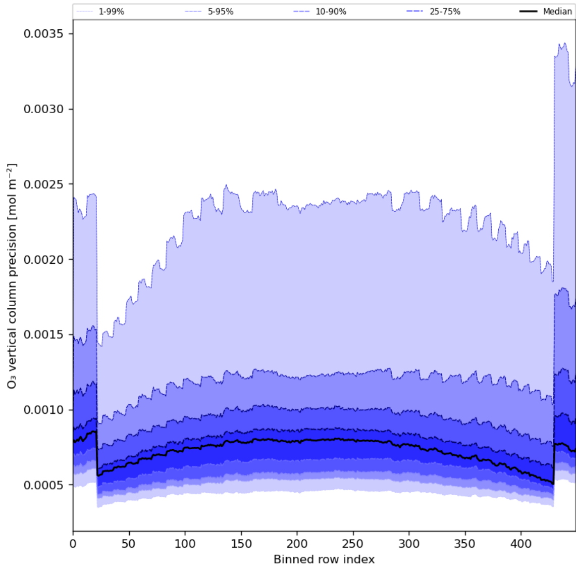
Figure 29: Along track statistics of “O 3 vertical column precision” for 2024-03-17 to 2024-03-19
