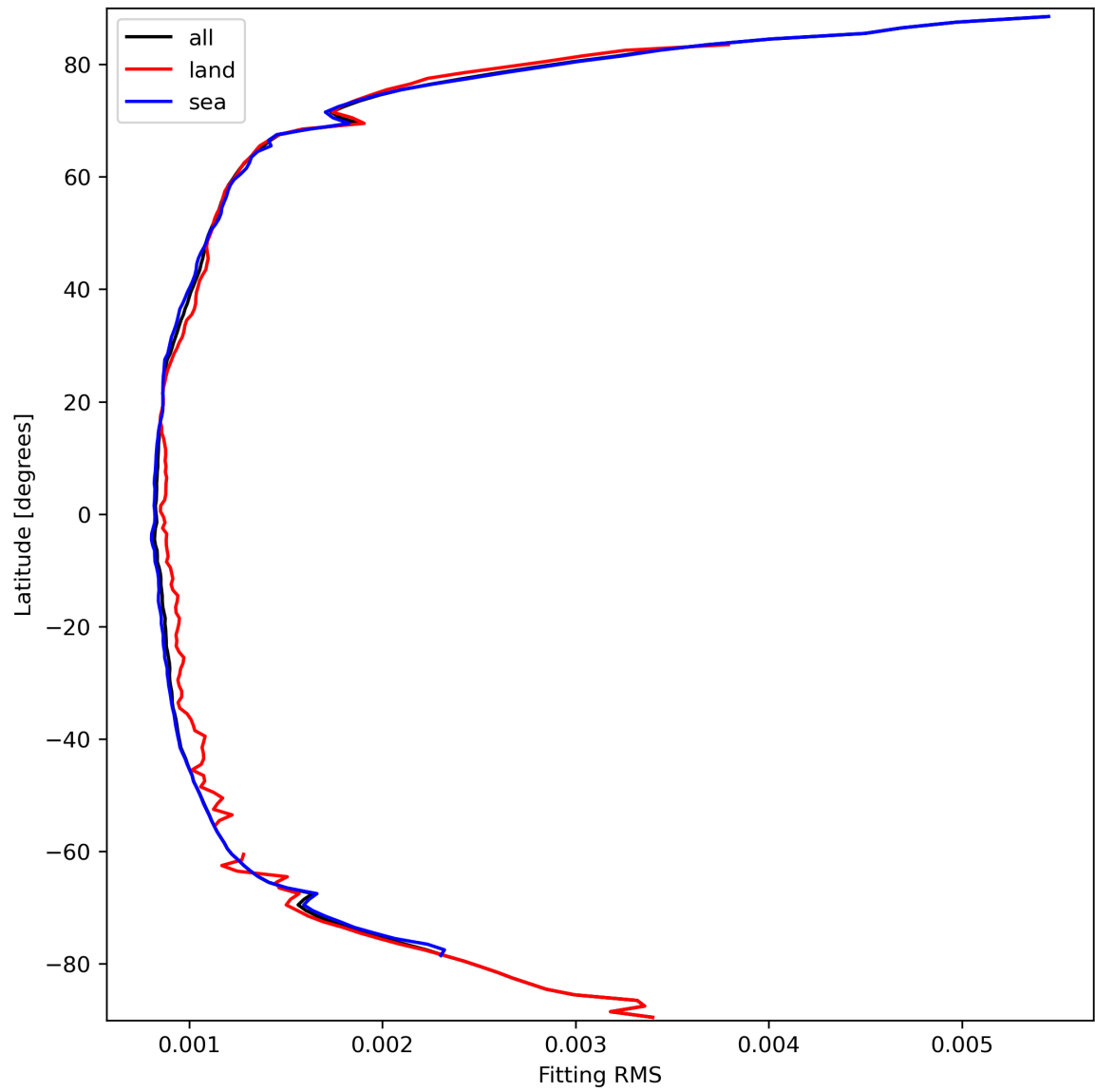
Figure 16: Zonal average of “Fitting RMS” for 2024-03-17 to 2024-03-19.
