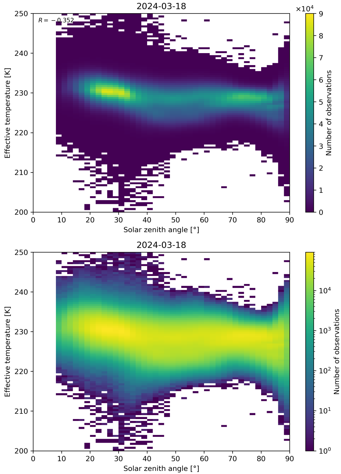
Figure 45: Scatter density plot of “Solar zenith angle” against “Effective temperature” for 2024-03-17 to 2024-03-19.
