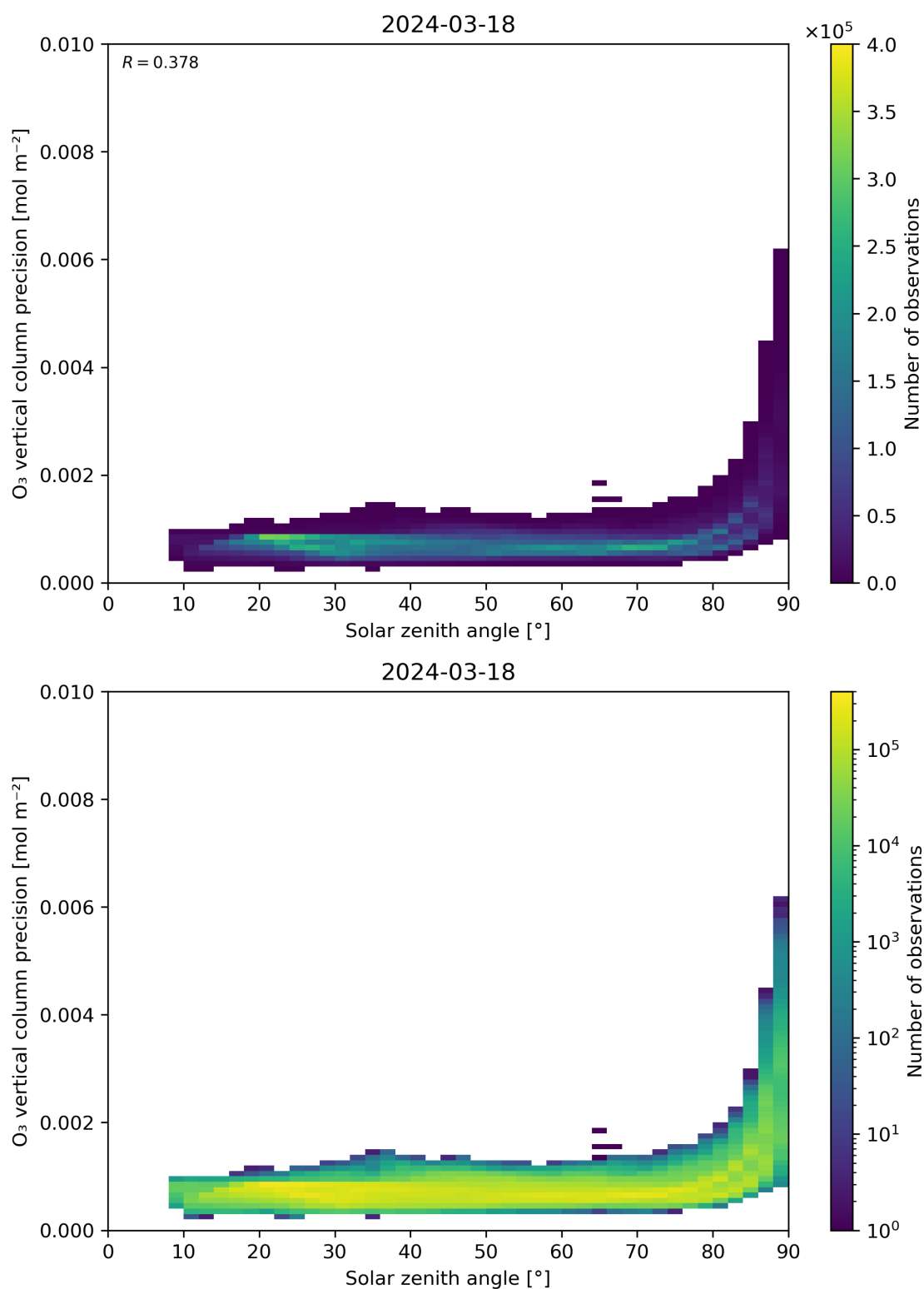
Figure 48: Scatter density plot of “Solar zenith angle” against “O 3 vertical column precision” for 2024-03-17 to 2024-03-19.
