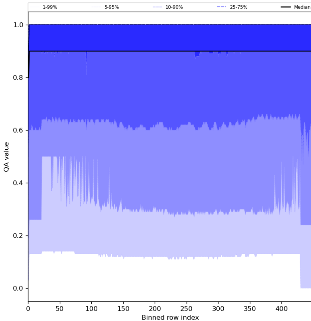
Figure 27: Along track statistics of “QA value” for 2024-03-17 to 2024-03-19
