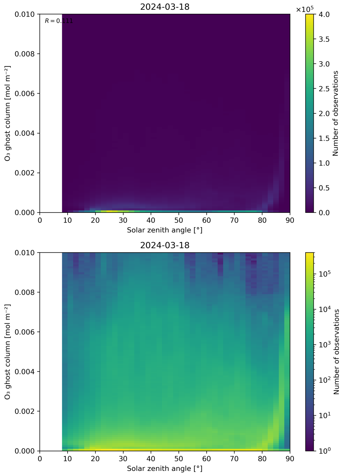
Figure 46: Scatter density plot of “Solar zenith angle” against “O 3 ghost column” for 2024-03-17 to 2024-03-19.
