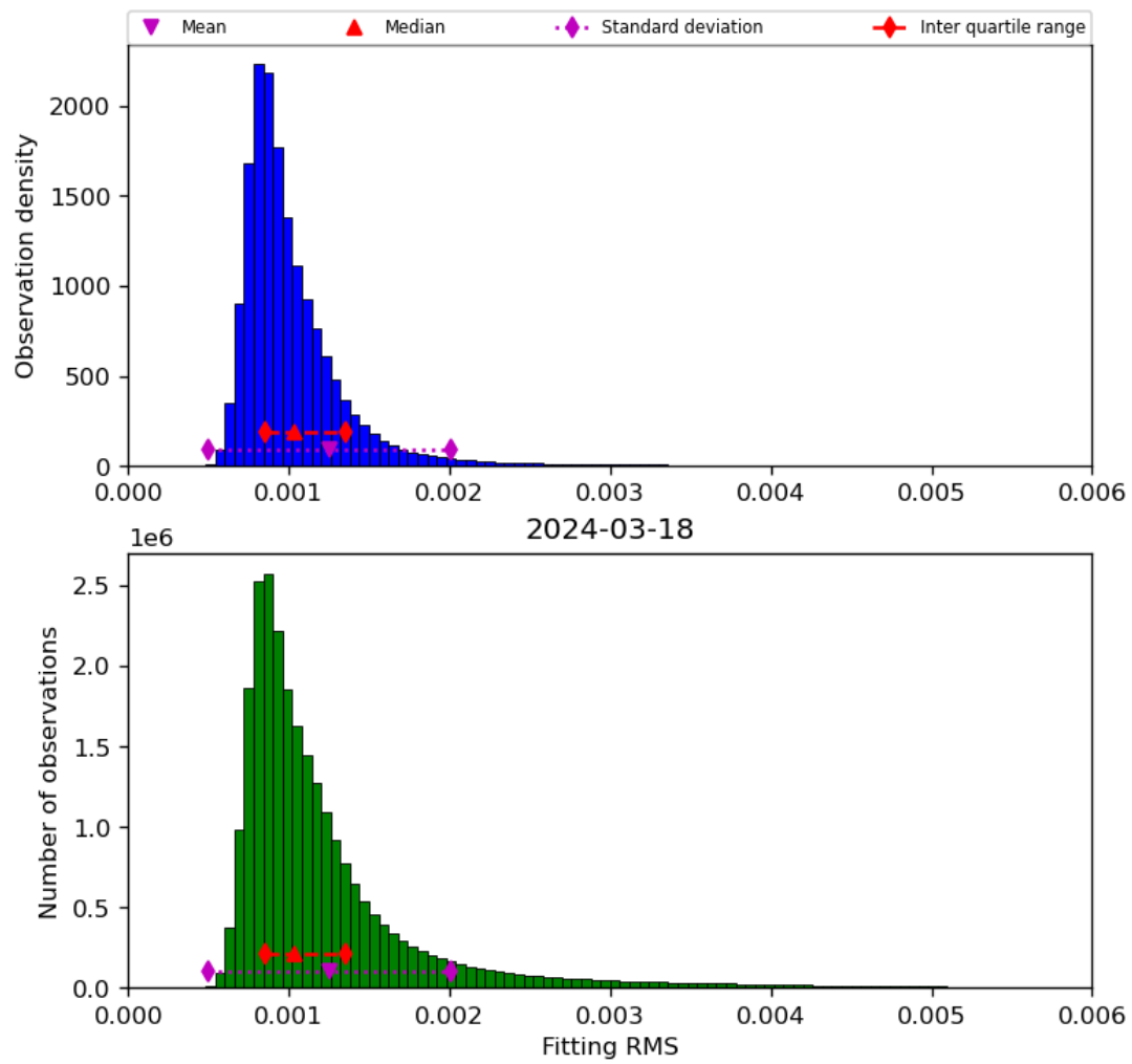
Figure 23: Histogram of “Fitting RMS” for 2024-03-17 to 2024-03-19
