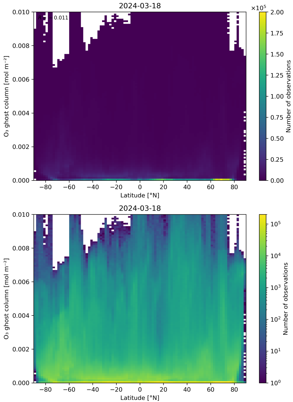
Figure 35: Scatter density plot of “Latitude” against “O 3 ghost column” for 2024-03-17 to 2024-03-19.
