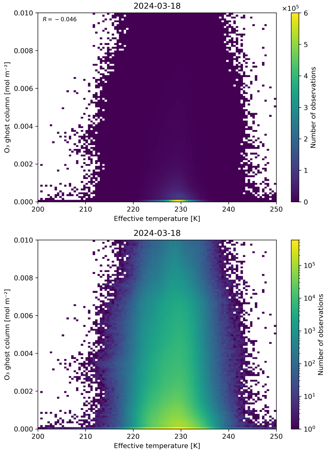
Figure 38: Scatter density plot of “Effective temperature” against “O 3 ghost column” for 2024-03-17 to 2024-03-19.
