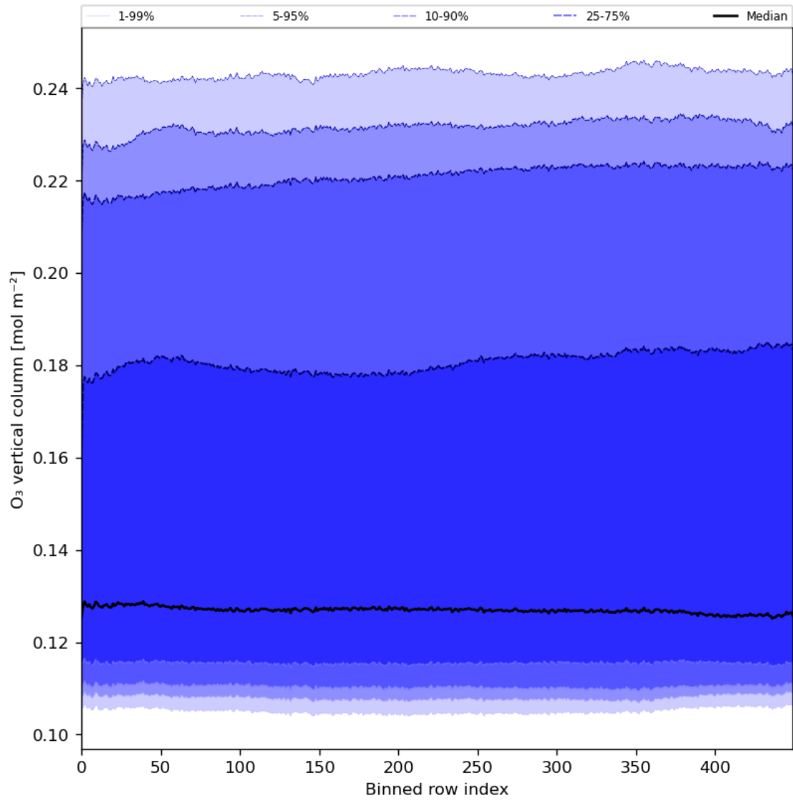
Figure 28: Along track statistics of “ O_3 vertical column” for 2024-03-17 to 2024-03-19
