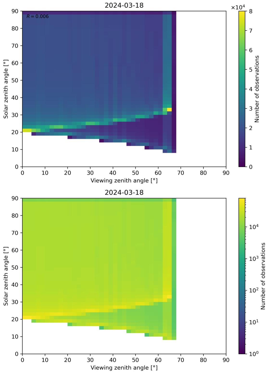
Figure 54: Scatter density plot of “Viewing zenith angle” against “Solar zenith angle” for 2024-03-17 to 2024-03-19.
