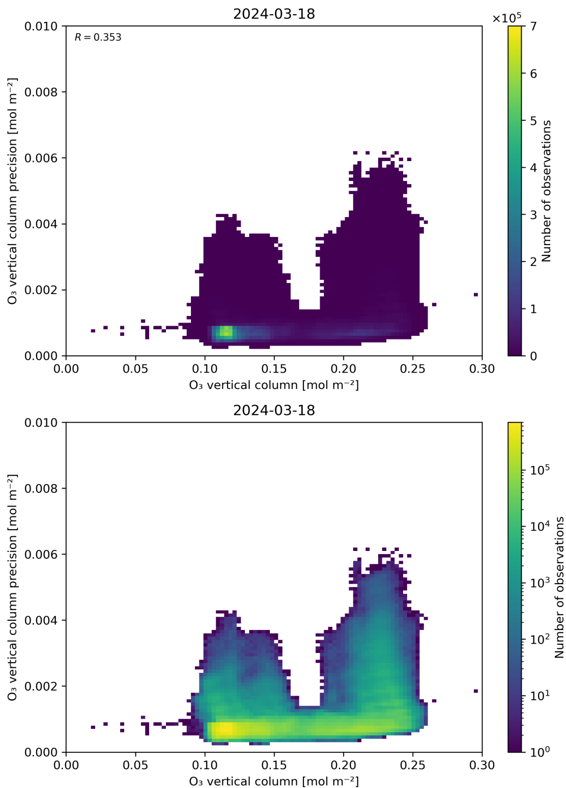
Figure 41: Scatter density plot of “O 3 vertical column” against “O 3 vertical column precision” for 2024-03-17 to 2024-03-19.
