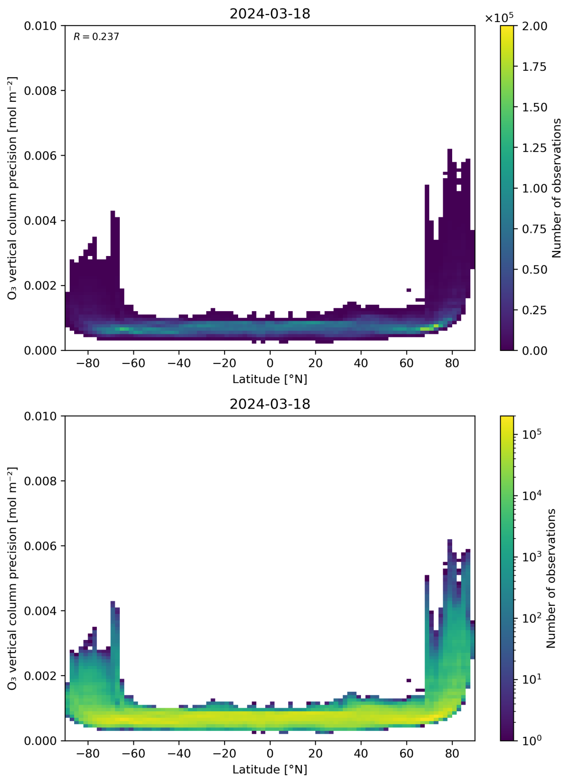
Figure 37: Scatter density plot of “Latitude” against “O 3 vertical column precision” for 2024-03-17 to 2024-03-19.
