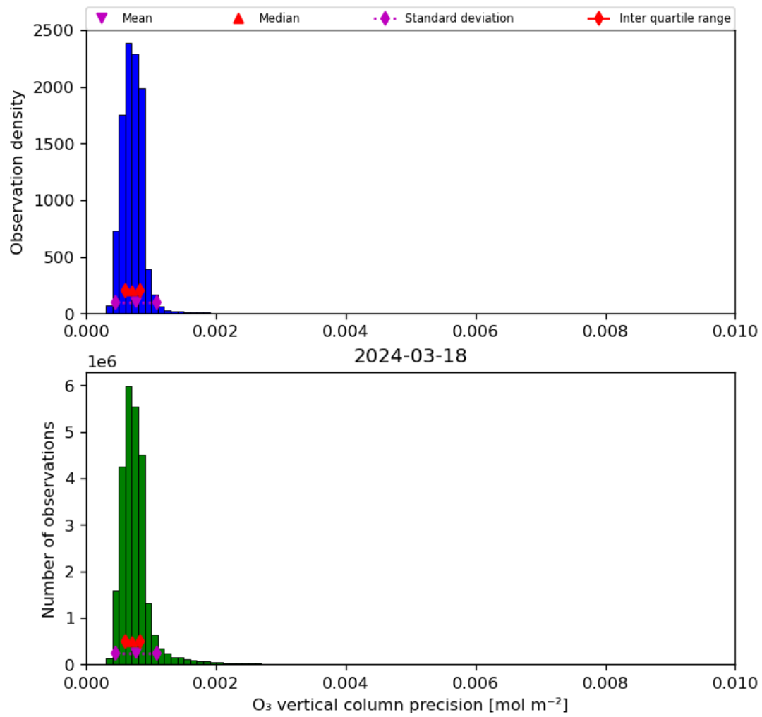
Figure 22: Histogram of “O 3 vertical column precision” for 2024-03-17 to 2024-03-19
