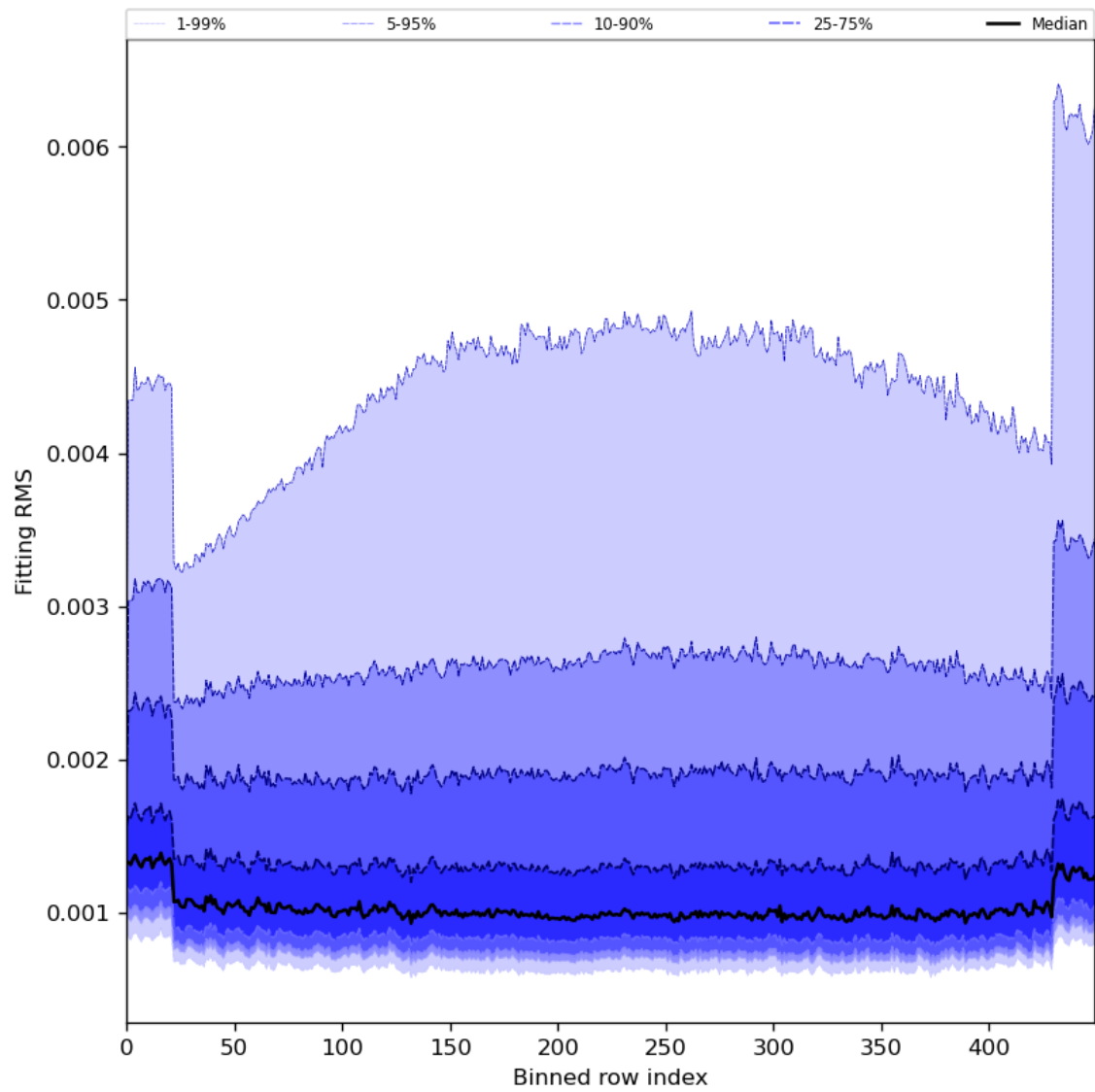
Figure 30: Along track statistics of “Fitting RMS” for 2024-03-17 to 2024-03-19
