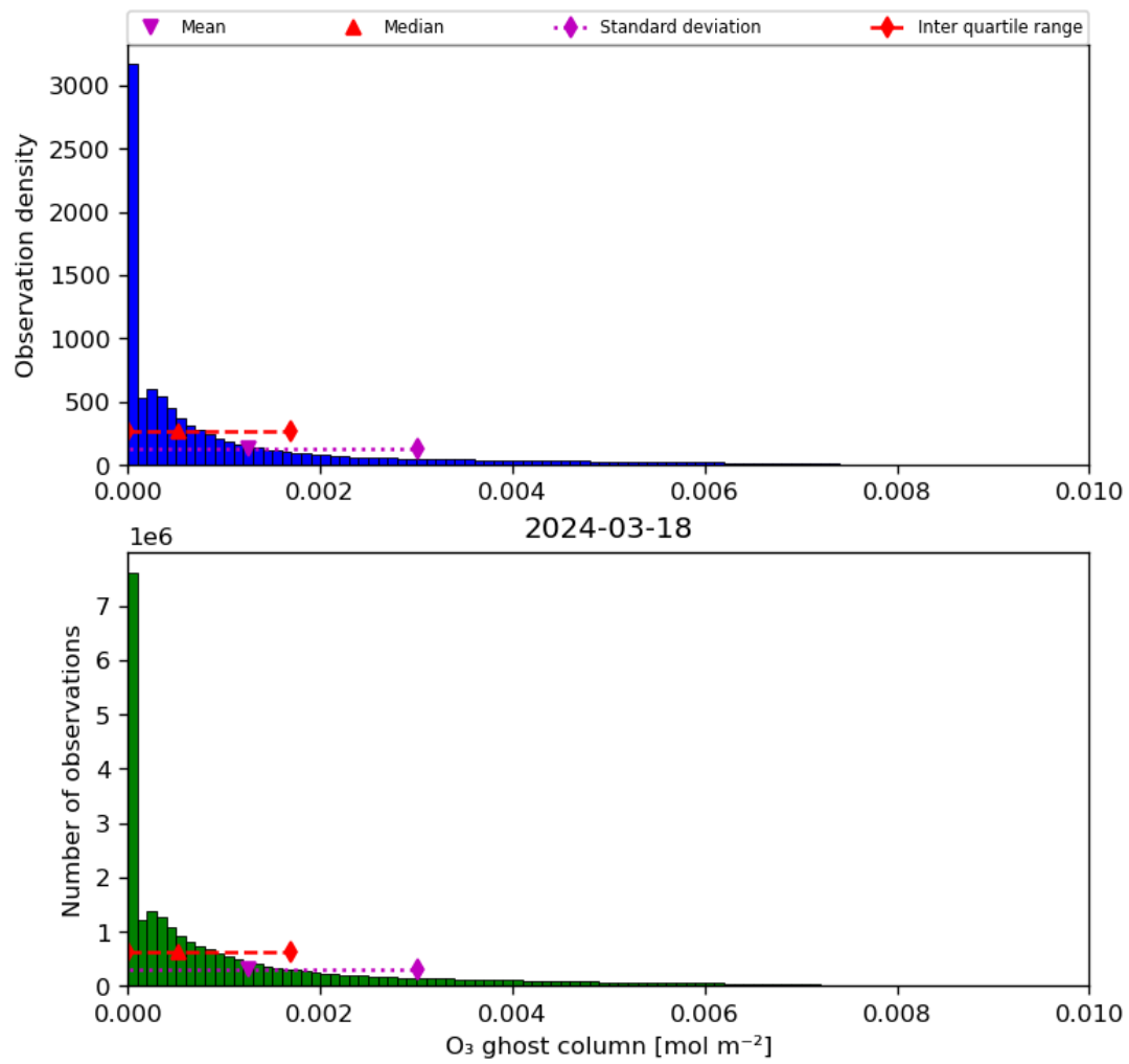
Figure 25: Histogram of "O 3 ghost column" for 2024-03-17 to 2024-03-19
