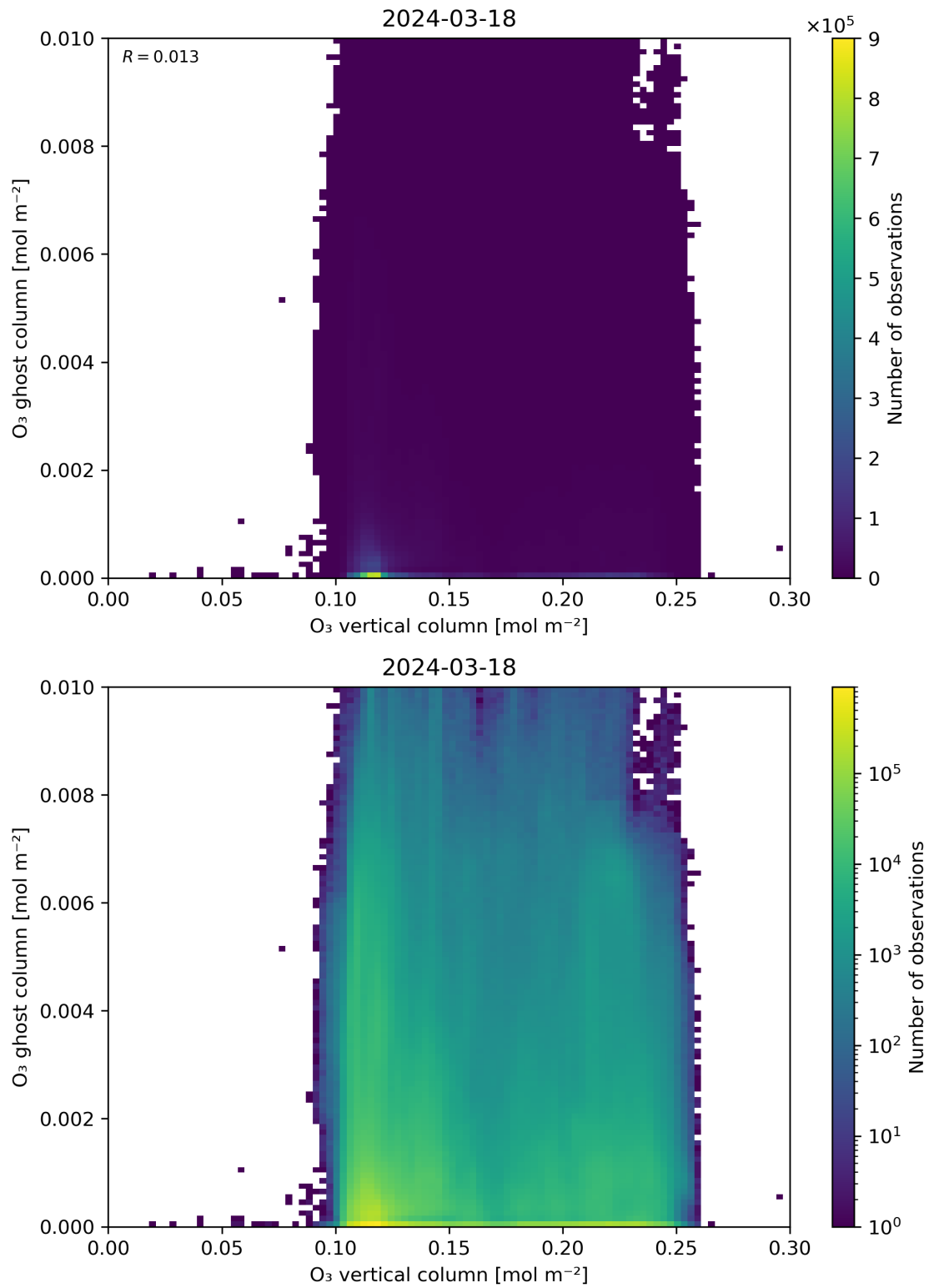
Figure 40: Scatter density plot of “O 3 vertical column” against “O 3 ghost column” for 2024-03-17 to 2024-03-19.
