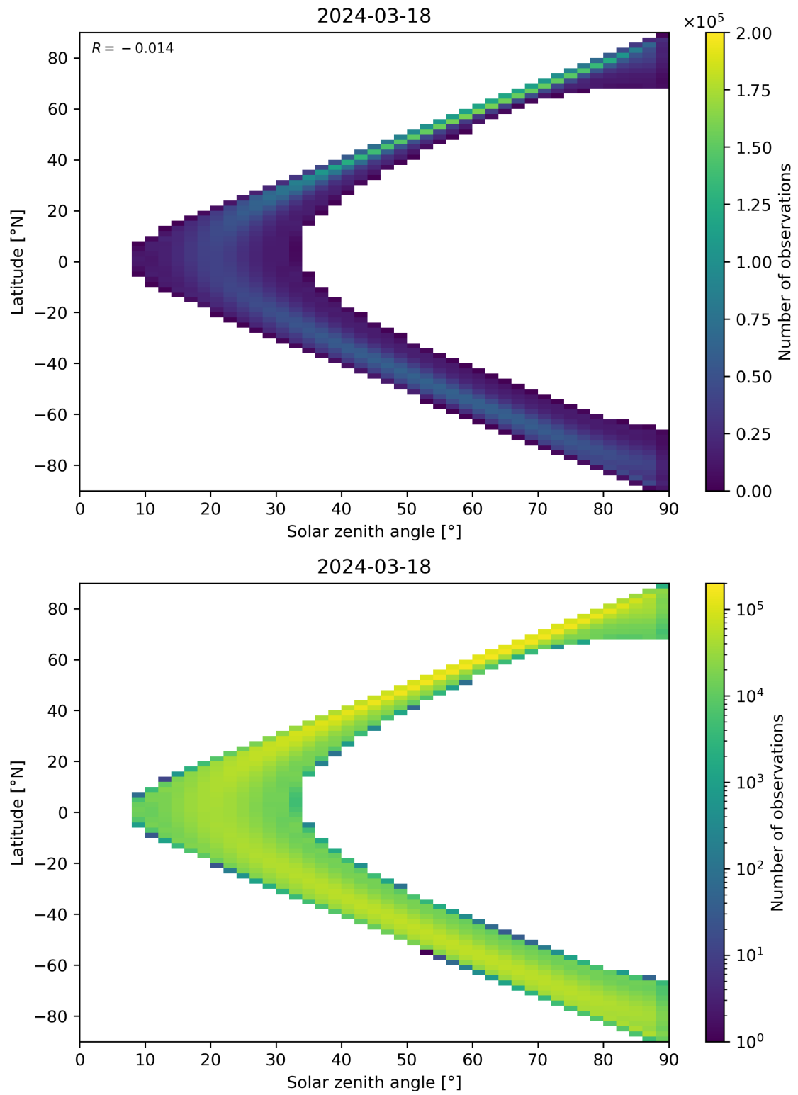
Figure 44: Scatter density plot of “Solar zenith angle” against “Latitude” for 2024-03-17 to 2024-03-19.
