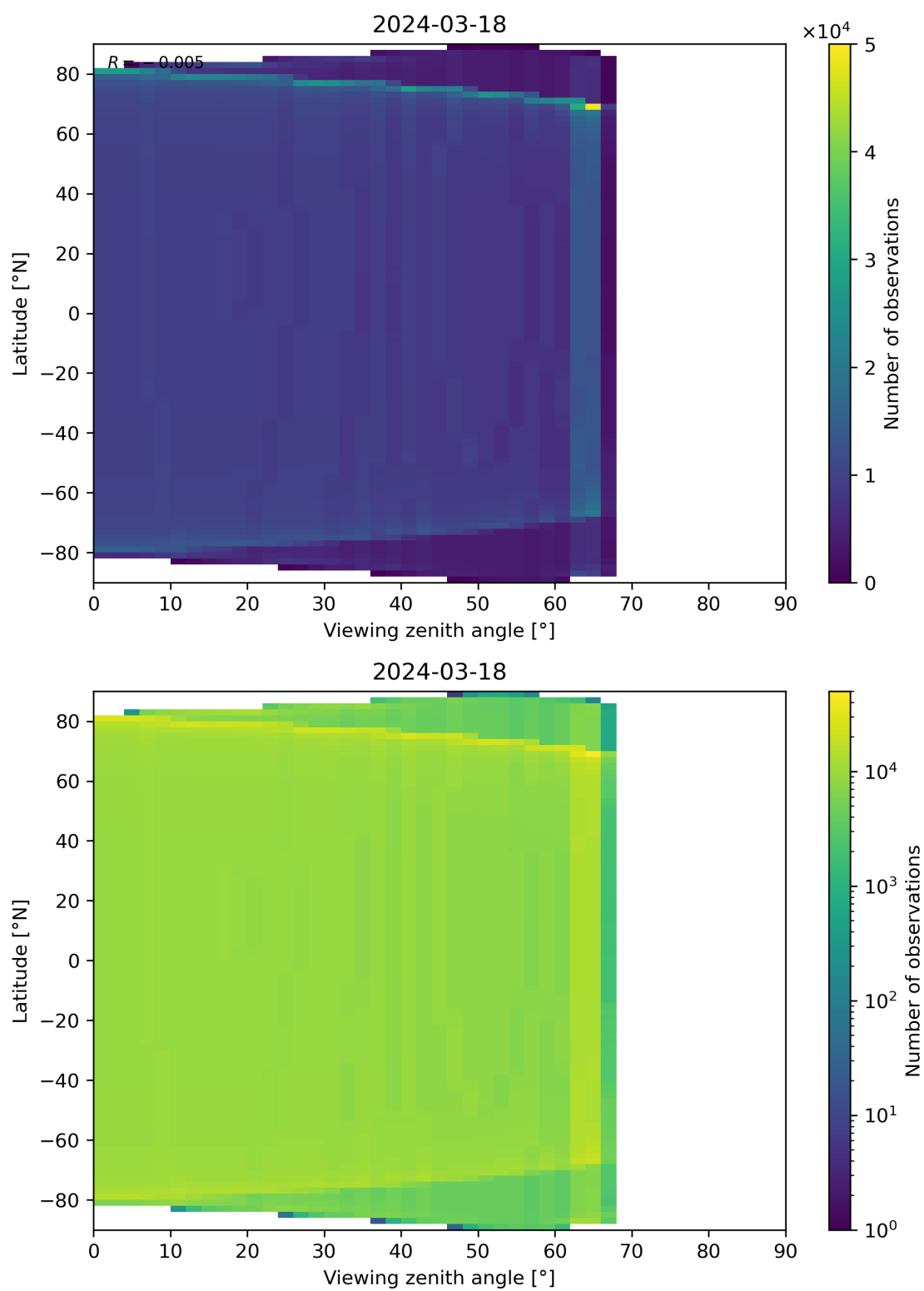
Figure 49: Scatter density plot of “Viewing zenith angle” against “Latitude” for 2024-03-17 to 2024-03-19.
