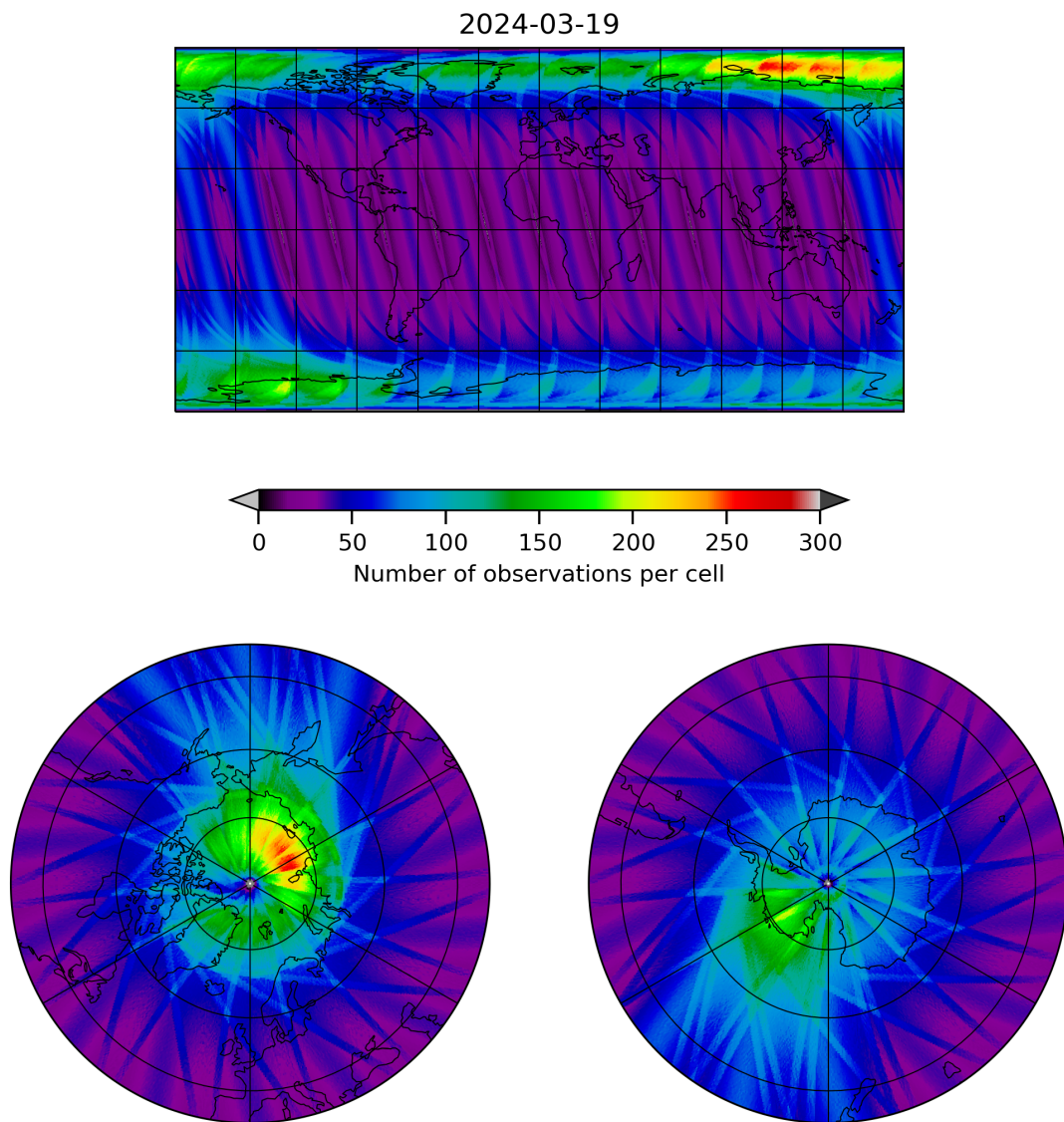
Figure 12: Map of the number of observations for 2024-03-18 to 2024-03-20
