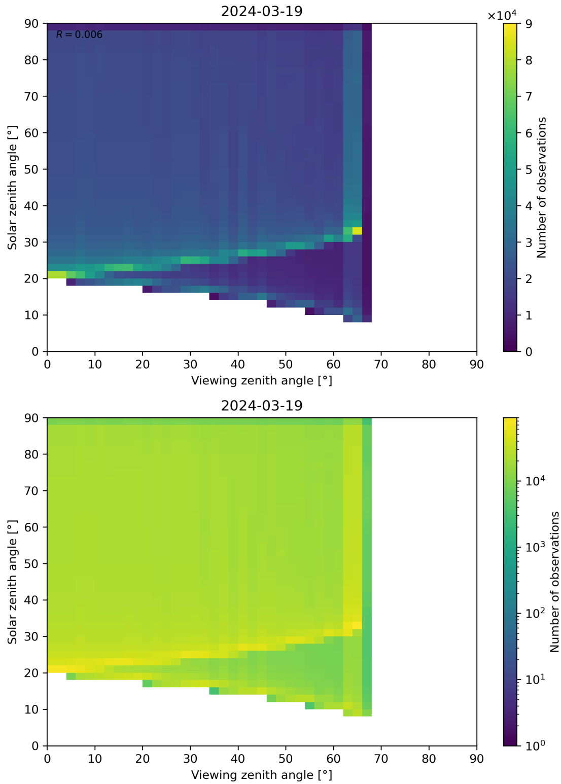
Figure 54: Scatter density plot of “Viewing zenith angle” against “Solar zenith angle” for 2024-03-18 to 2024-03-20.
