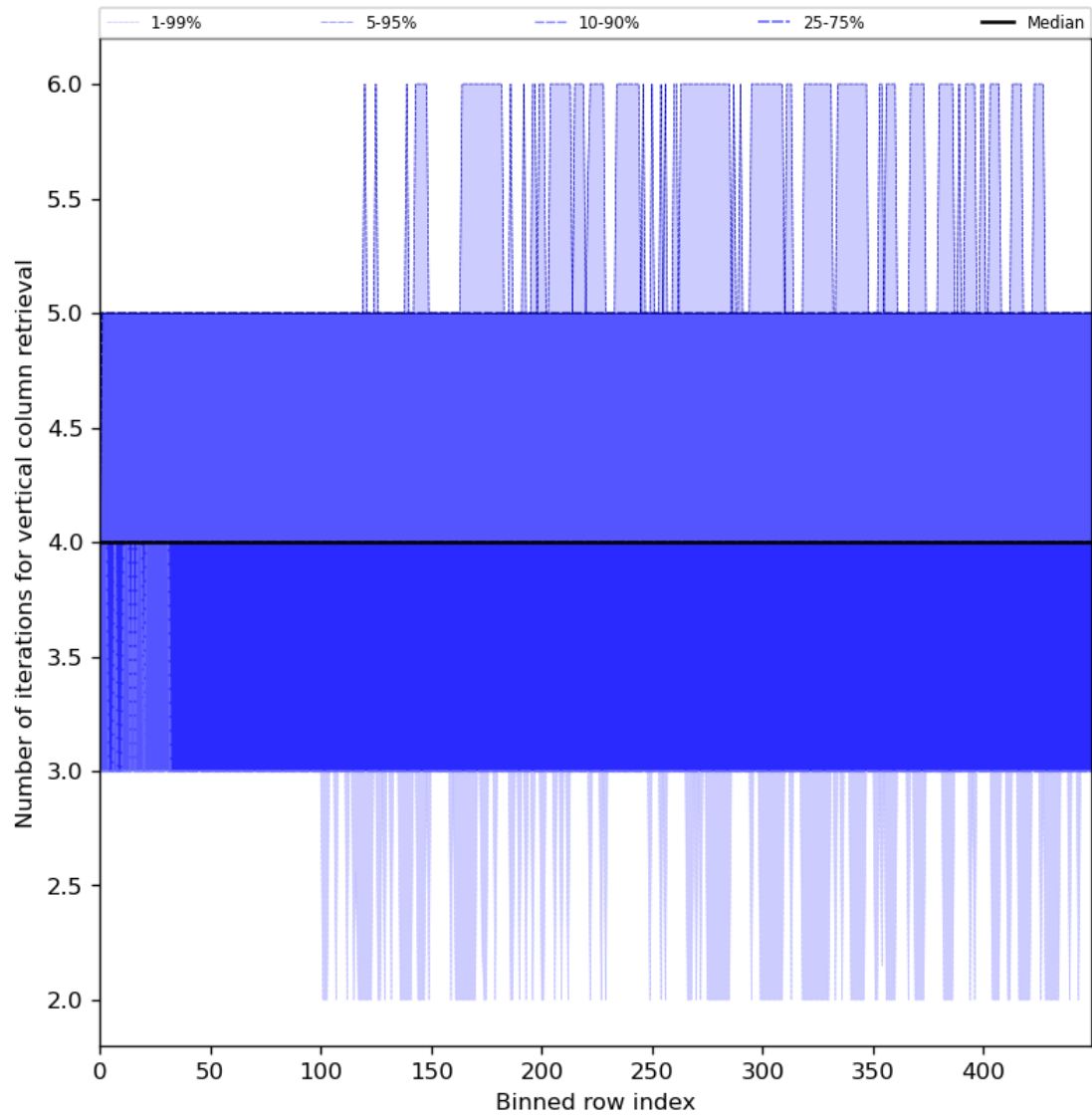
Figure 33: Along track statistics of “Number of iterations for vertical column retrieval” for 2024-03-18 to 2024-03-20
