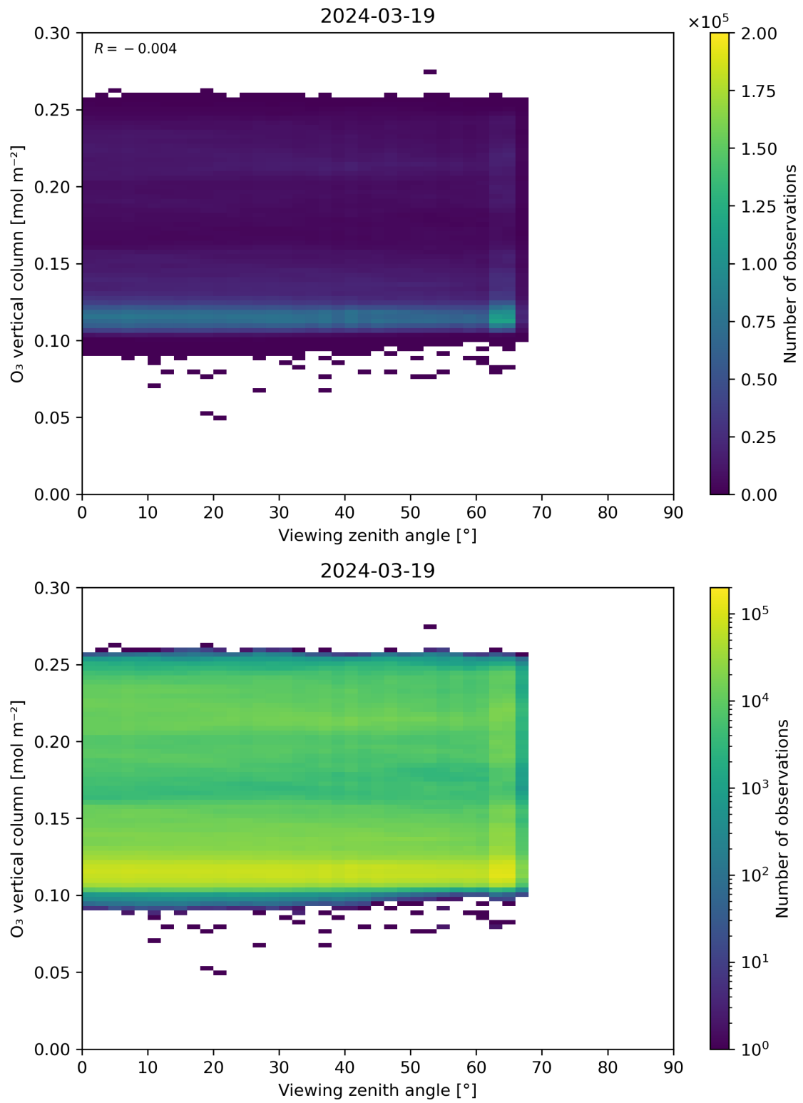
Figure 52: Scatter density plot of “Viewing zenith angle” against “O 3 vertical column” for 2024-03-18 to 2024-03-20.
