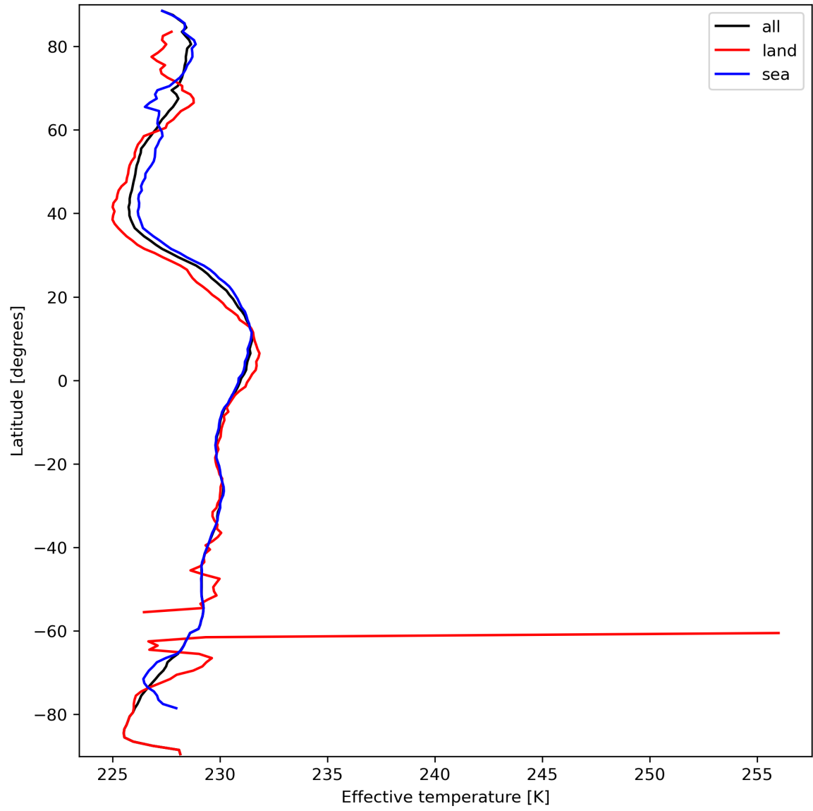
Figure 17: Zonal average of “Effective temperature” for 2024-03-18 to 2024-03-20.
