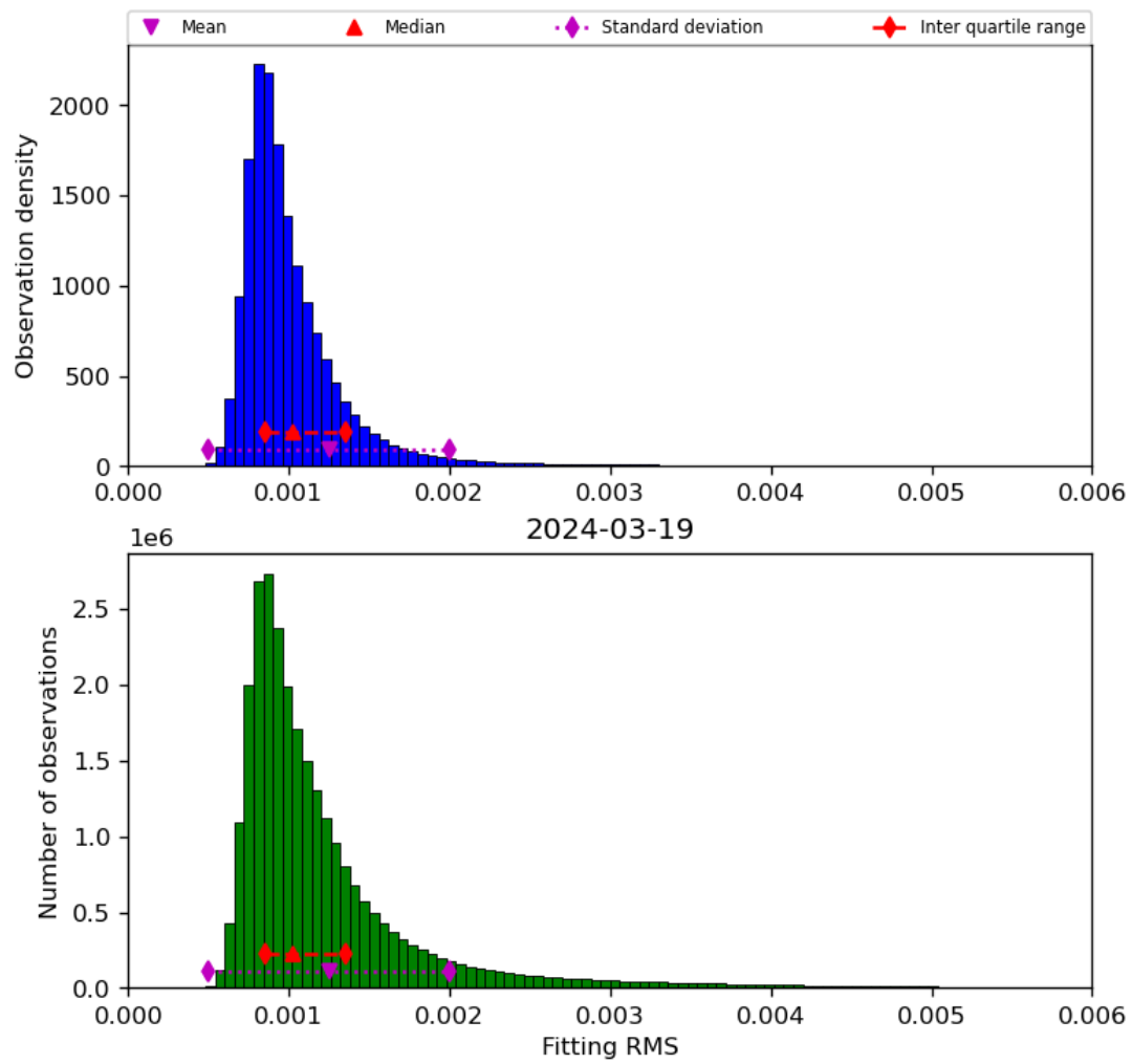
Figure 23: Histogram of “Fitting RMS” for 2024-03-18 to 2024-03-20
