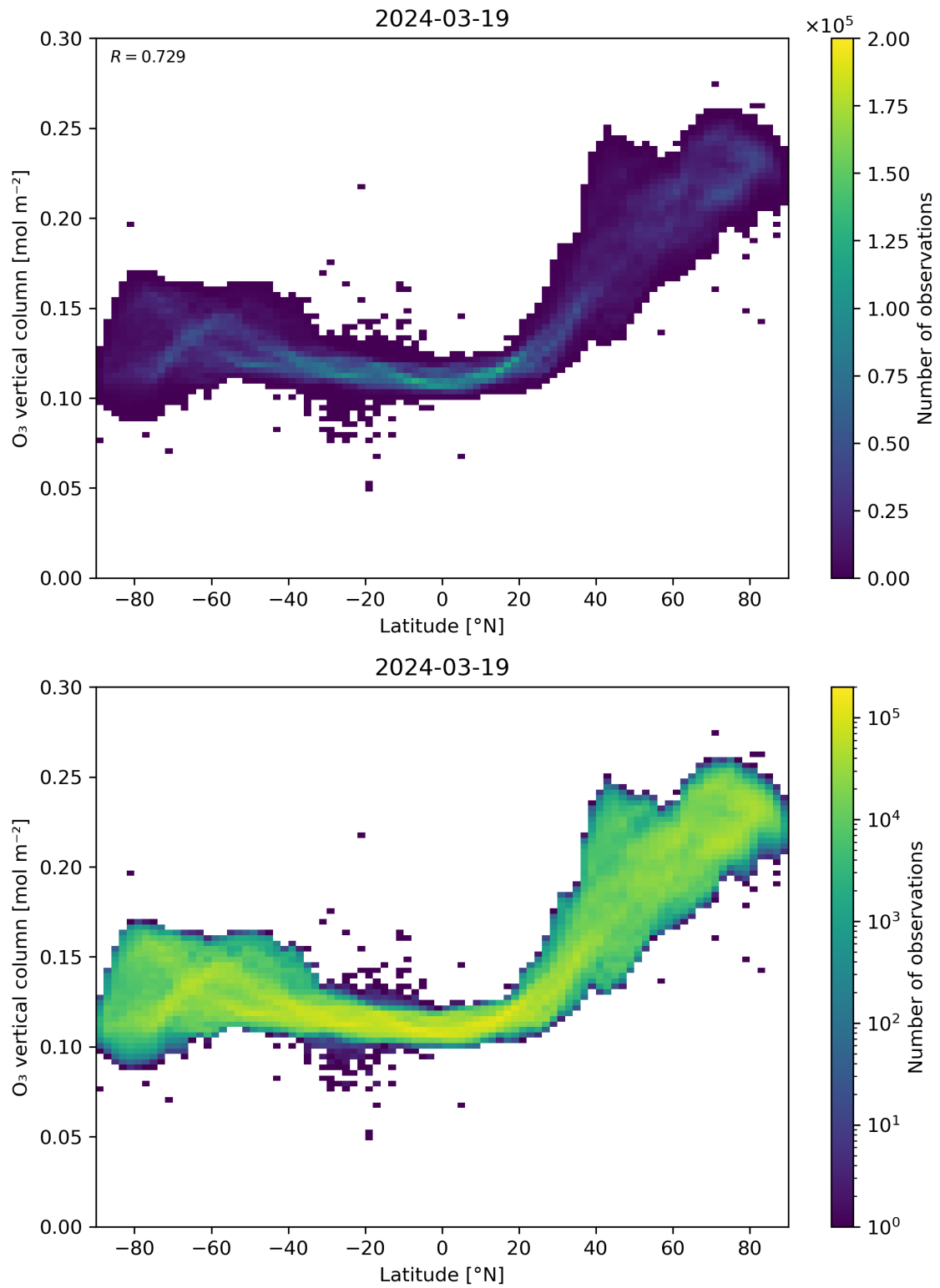
Figure 36: Scatter density plot of “Latitude” against “O 3 vertical column” for 2024-03-18 to 2024-03-20.
