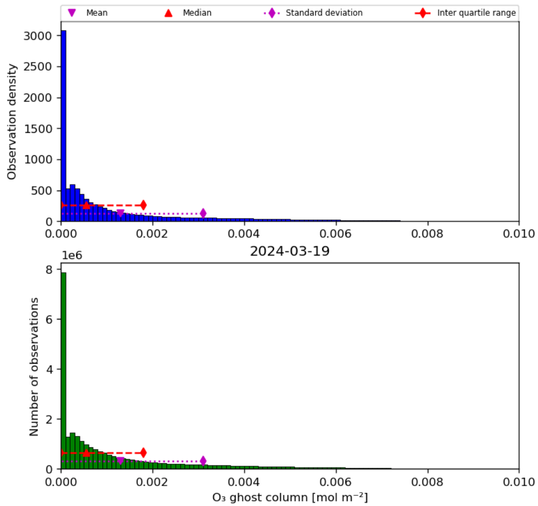
Figure 25: Histogram of “O 3 ghost column” for 2024-03-18 to 2024-03-20
