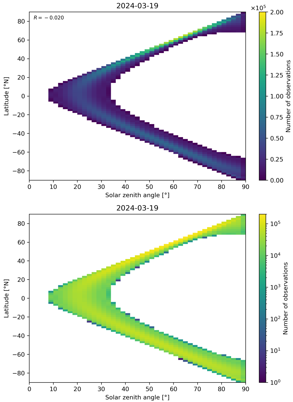
Figure 44: Scatter density plot of “Solar zenith angle” against “Latitude” for 2024-03-18 to 2024-03-20.
