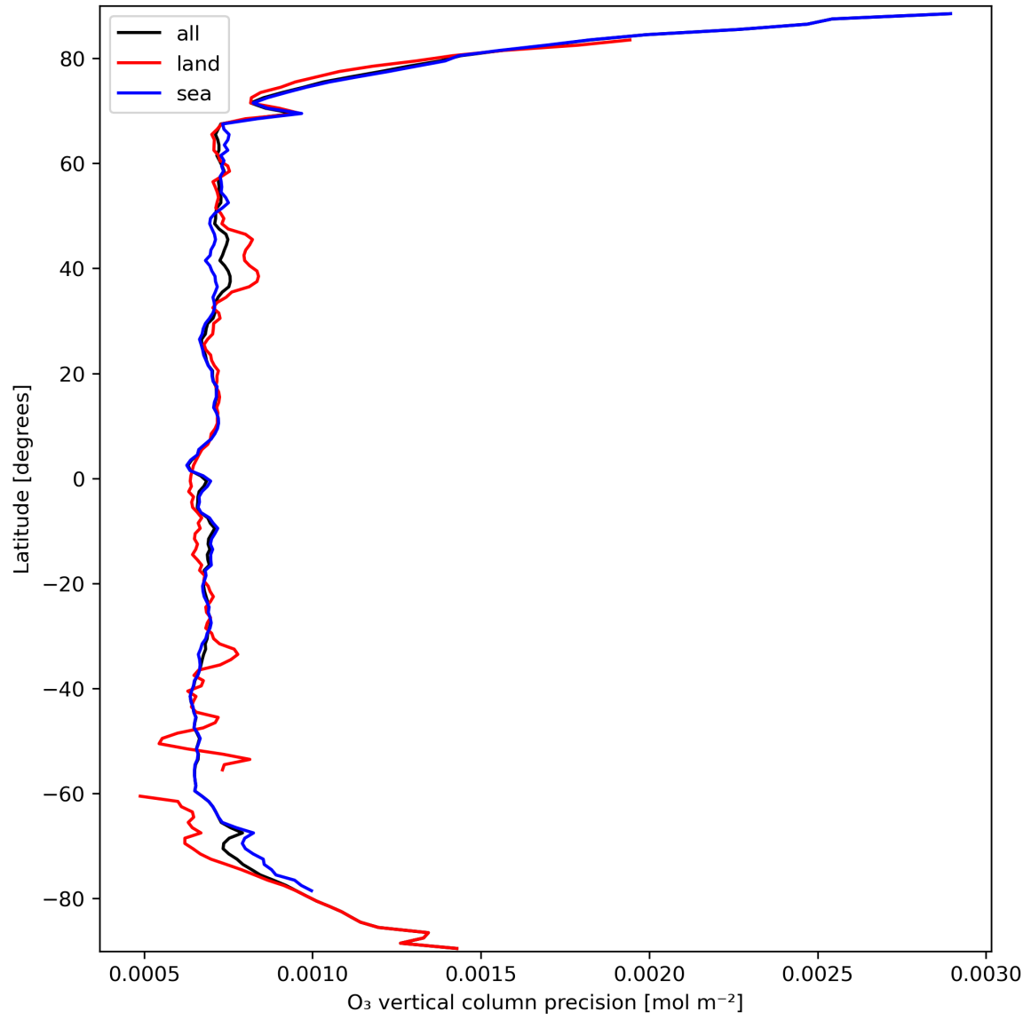
Figure 15: Zonal average of “O 3 vertical column precision” for 2024-03-18 to 2024-03-20.
