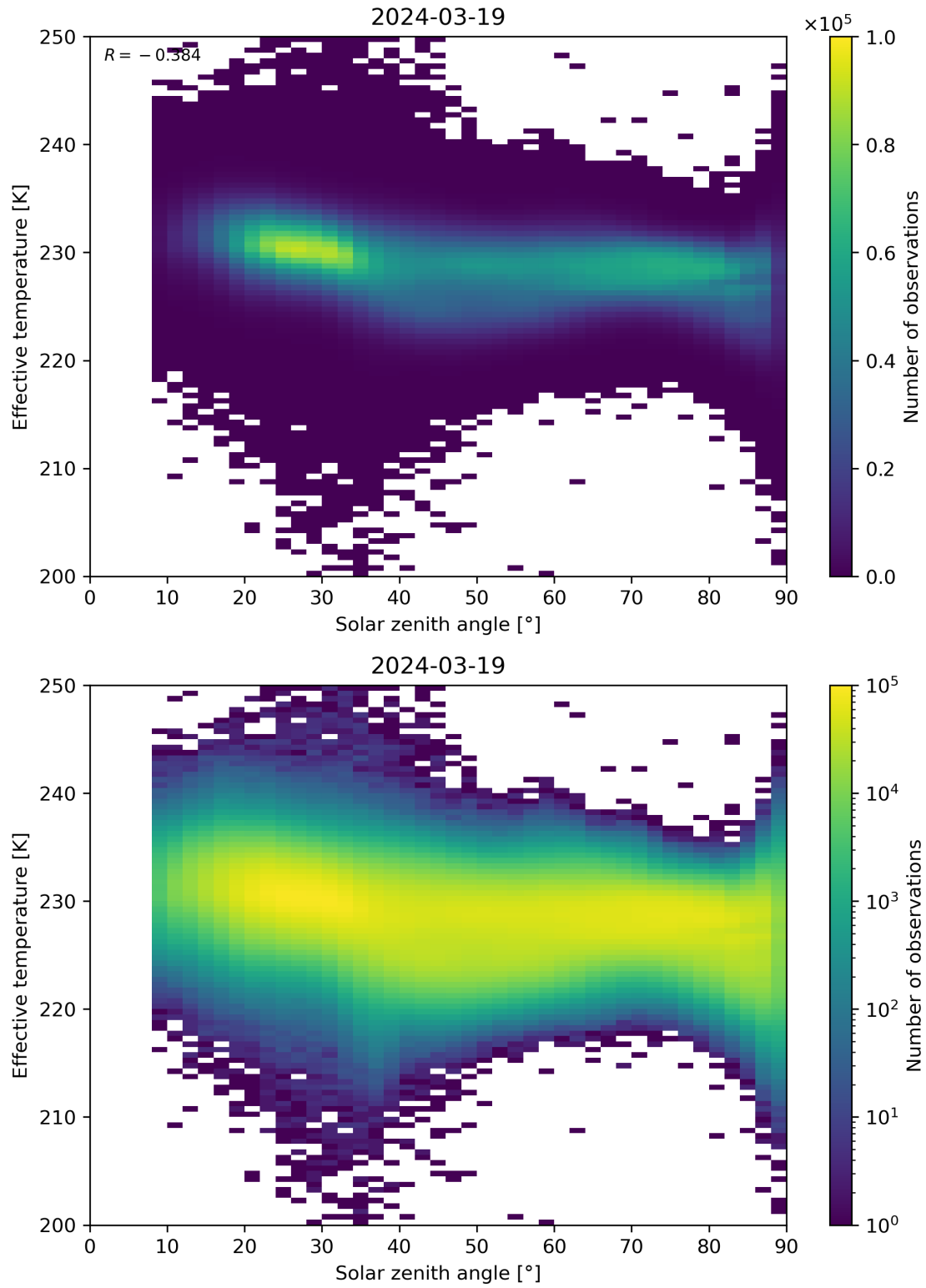
Figure 45: Scatter density plot of “Solar zenith angle” against “Effective temperature” for 2024-03-18 to 2024-03-20.
