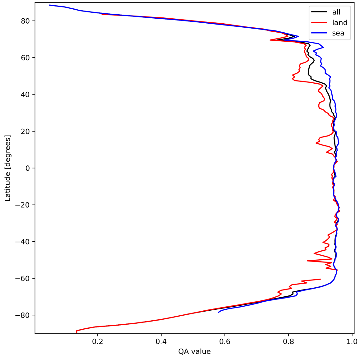
Figure 13: Zonal average of “QA value” for 2024-03-18 to 2024-03-20.
