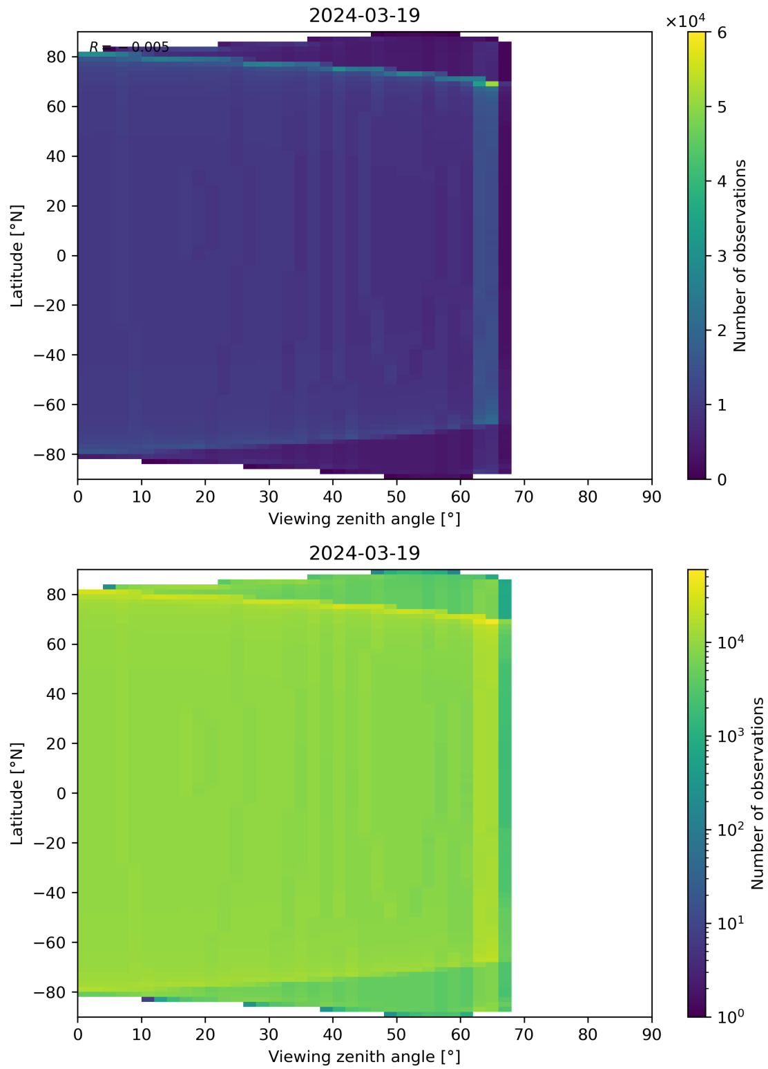
Figure 49: Scatter density plot of “Viewing zenith angle” against “Latitude” for 2024-03-18 to 2024-03-20.
