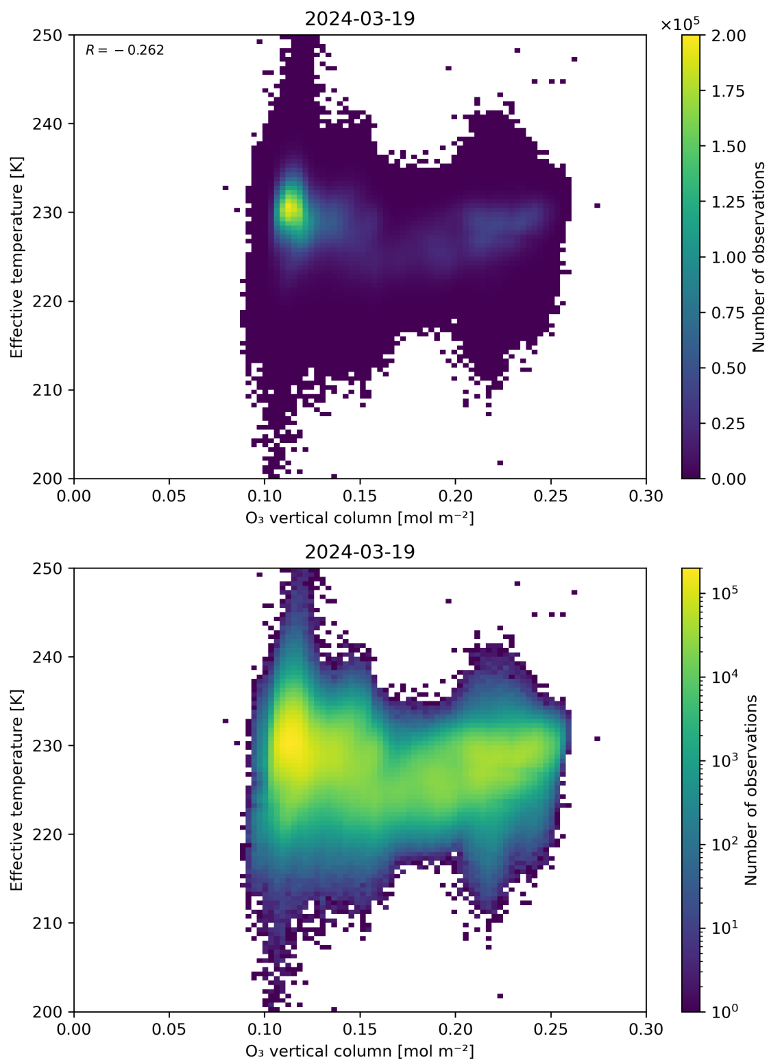
Figure 39: Scatter density plot of “O 3 vertical column” against “Effective temperature” for 2024-03-18 to 2024-03-20.
