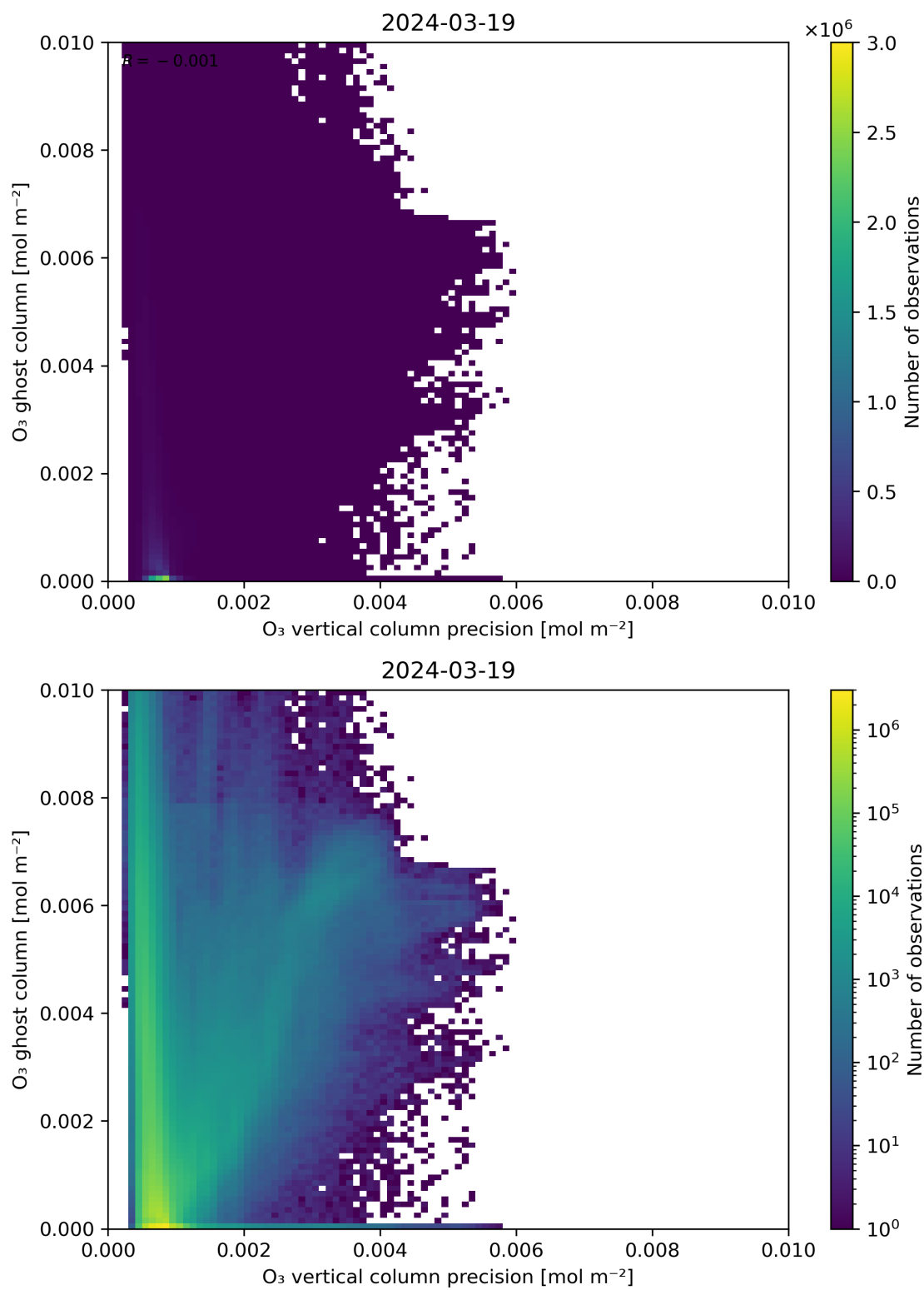
Figure 43: Scatter density plot of “ \text{O}_3 vertical column precision” against “ \text{O}_3 ghost column” for 2024-03-18 to 2024-03-20.
