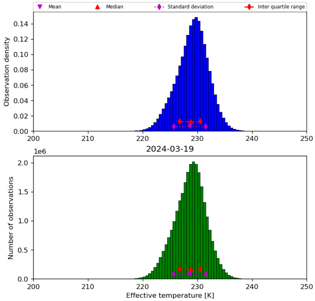
Figure 24: Histogram of “Effective temperature” for 2024-03-18 to 2024-03-20
