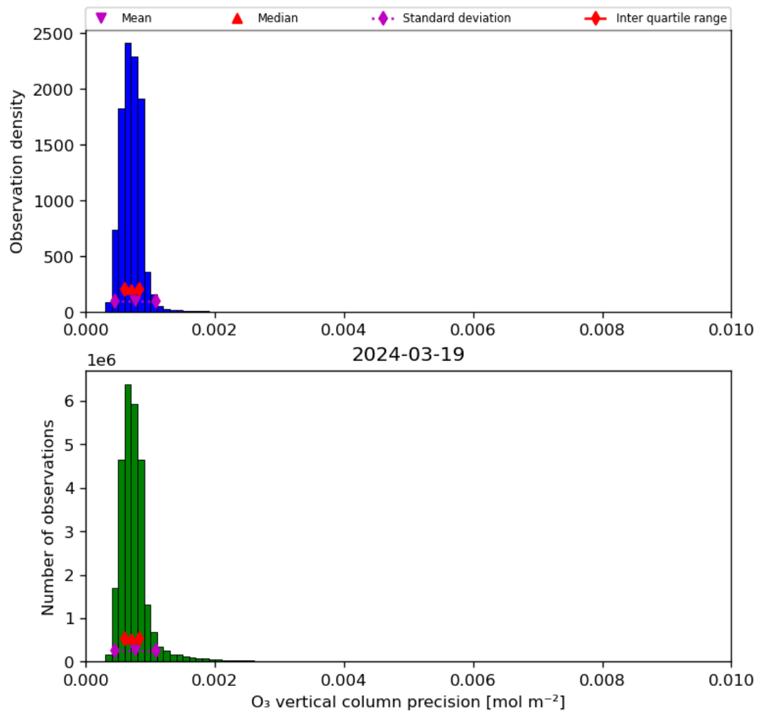
Figure 22: Histogram of “O 3 vertical column precision” for 2024-03-18 to 2024-03-20
