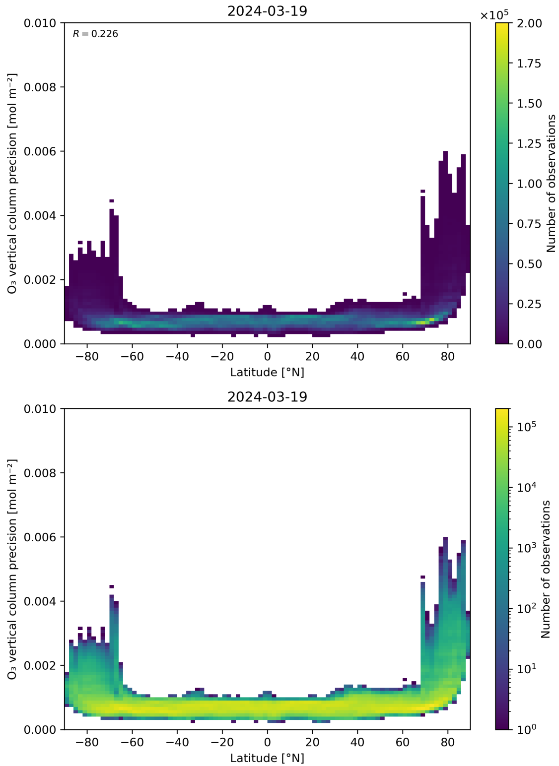
Figure 37: Scatter density plot of “Latitude” against “O 3 vertical column precision” for 2024-03-18 to 2024-03-20.
