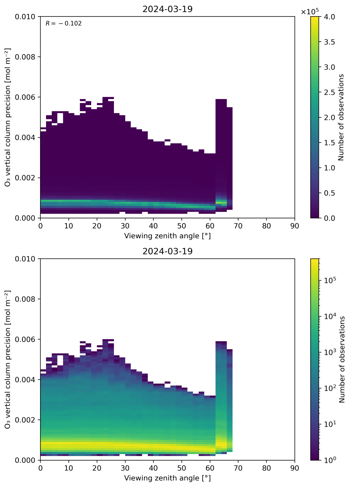
Figure 53: Scatter density plot of “Viewing zenith angle” against “O 3 vertical column precision” for 2024-03-18 to 2024-03-20.
