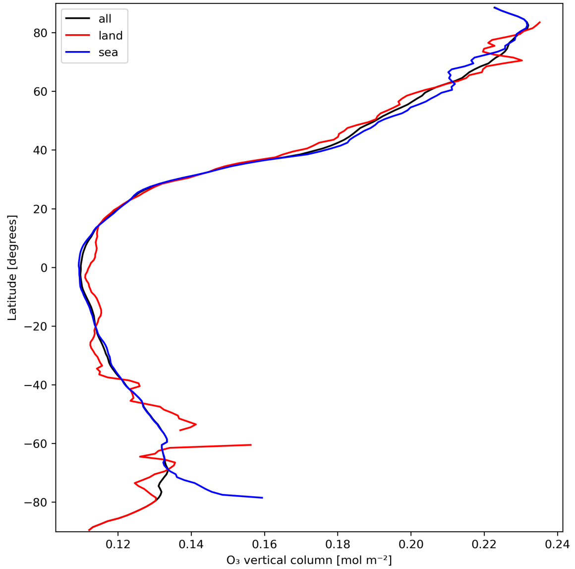
Figure 14: Zonal average of “O 3 vertical column” for 2024-03-18 to 2024-03-20.
