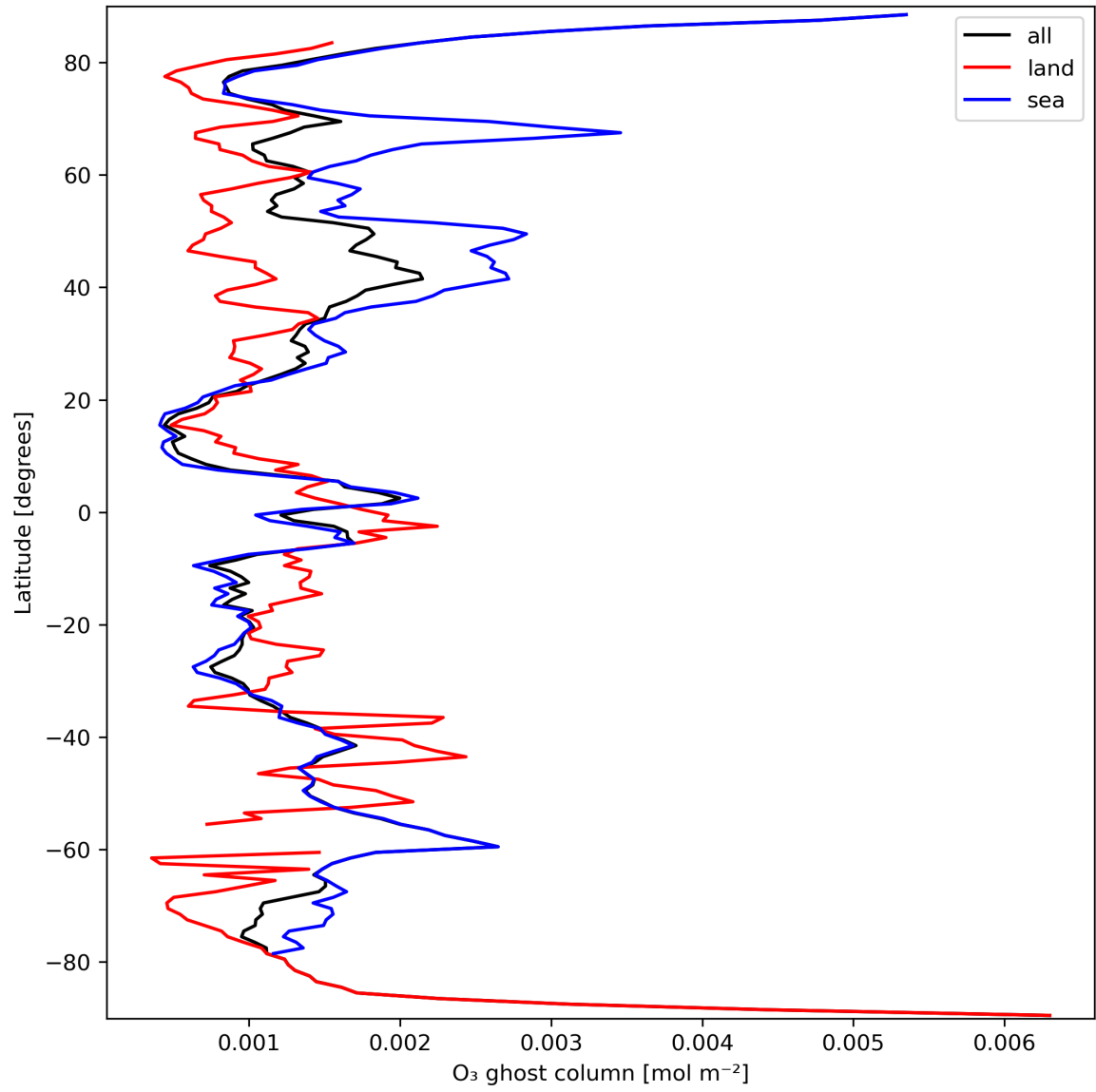
Figure 18: Zonal average of "O 3 ghost column" for 2024-03-18 to 2024-03-20.
