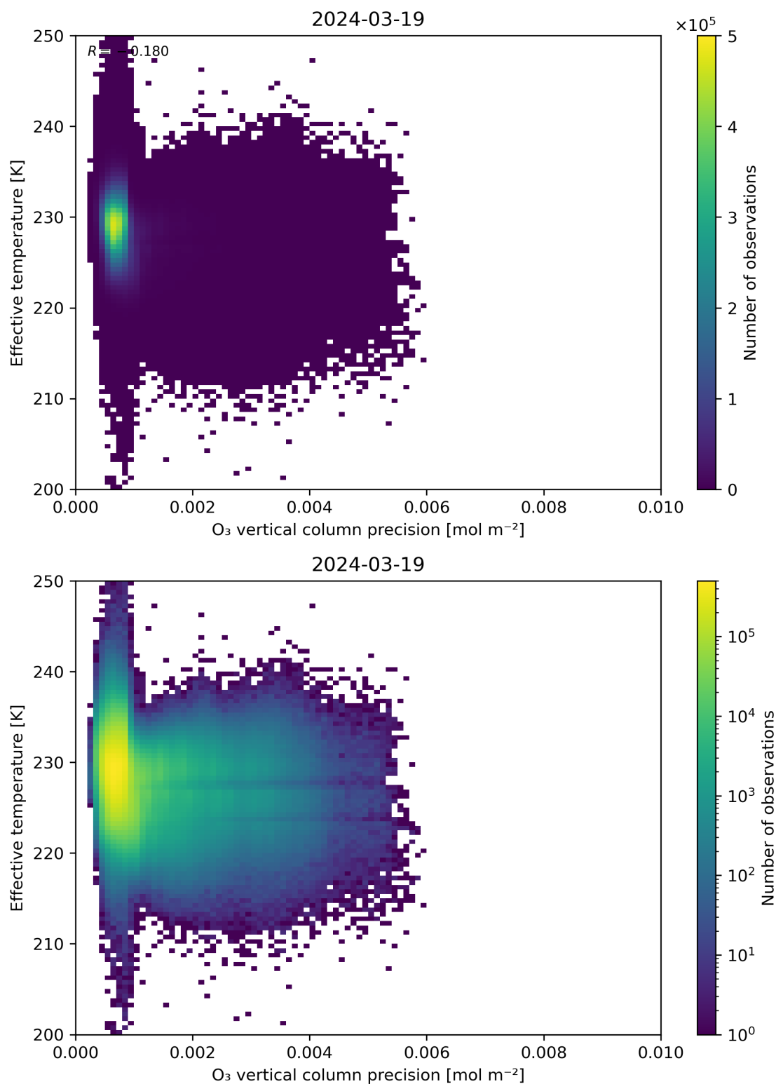
Figure 42: Scatter density plot of “O 3 vertical column precision” against “Effective temperature” for 2024-03-18 to 2024-03-20.
