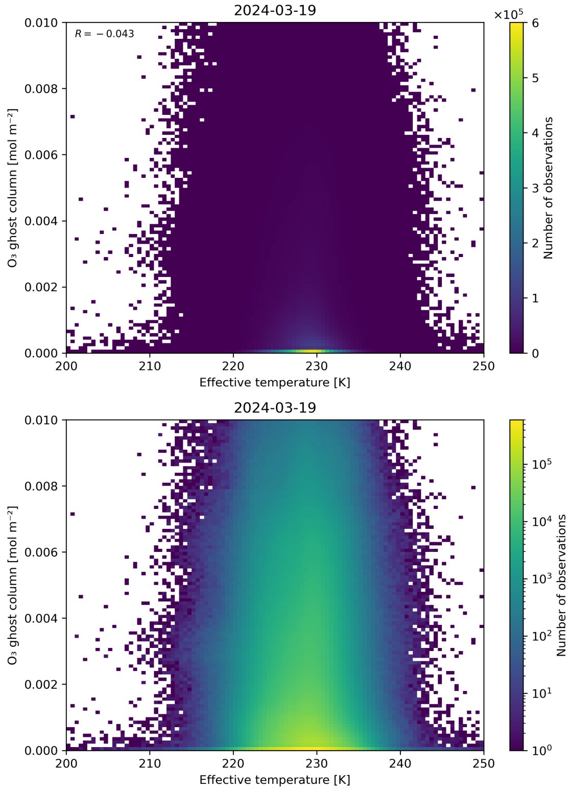
Figure 38: Scatter density plot of “Effective temperature” against “O 3 ghost column” for 2024-03-18 to 2024-03-20.
