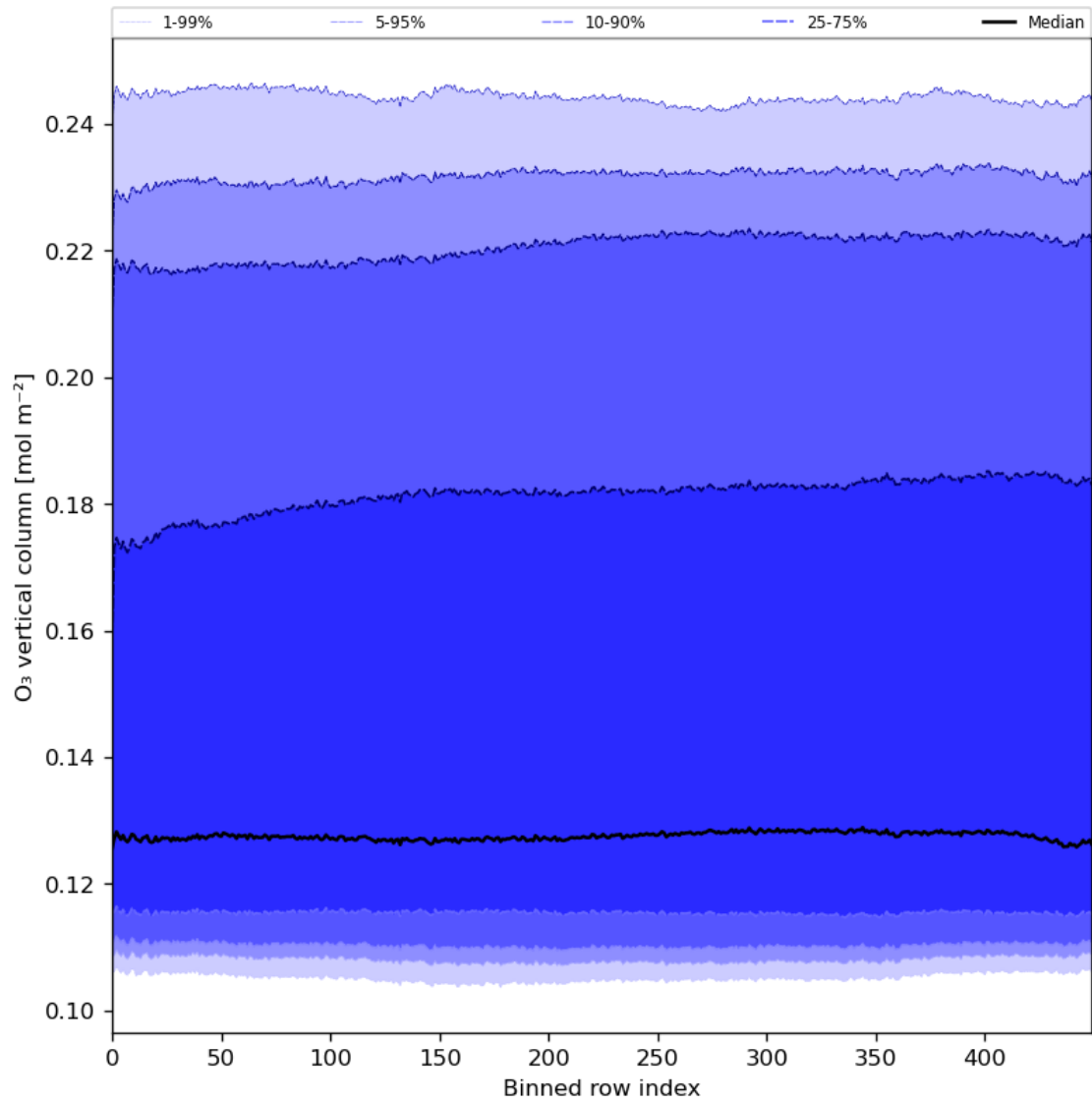
Figure 28: Along track statistics of “O 3 vertical column” for 2024-03-18 to 2024-03-20
