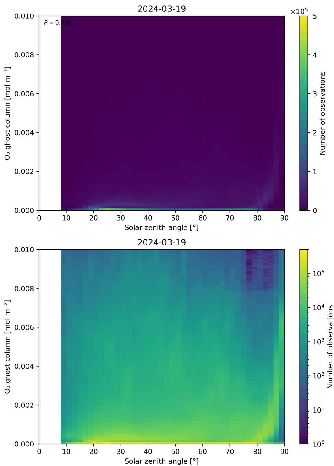
Figure 46: Scatter density plot of “Solar zenith angle” against “O 3 ghost column” for 2024-03-18 to 2024-03-20.
