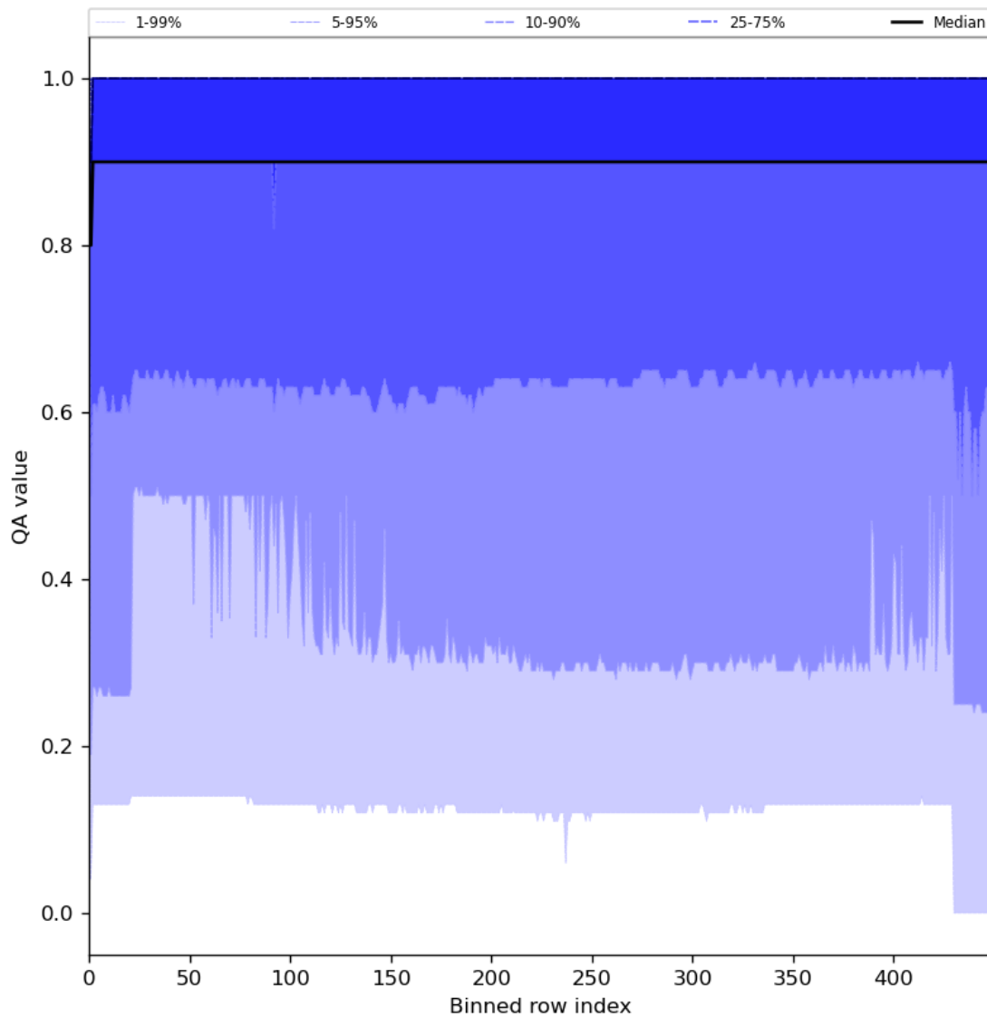
Figure 27: Along track statistics of “QA value” for 2024-03-18 to 2024-03-20
