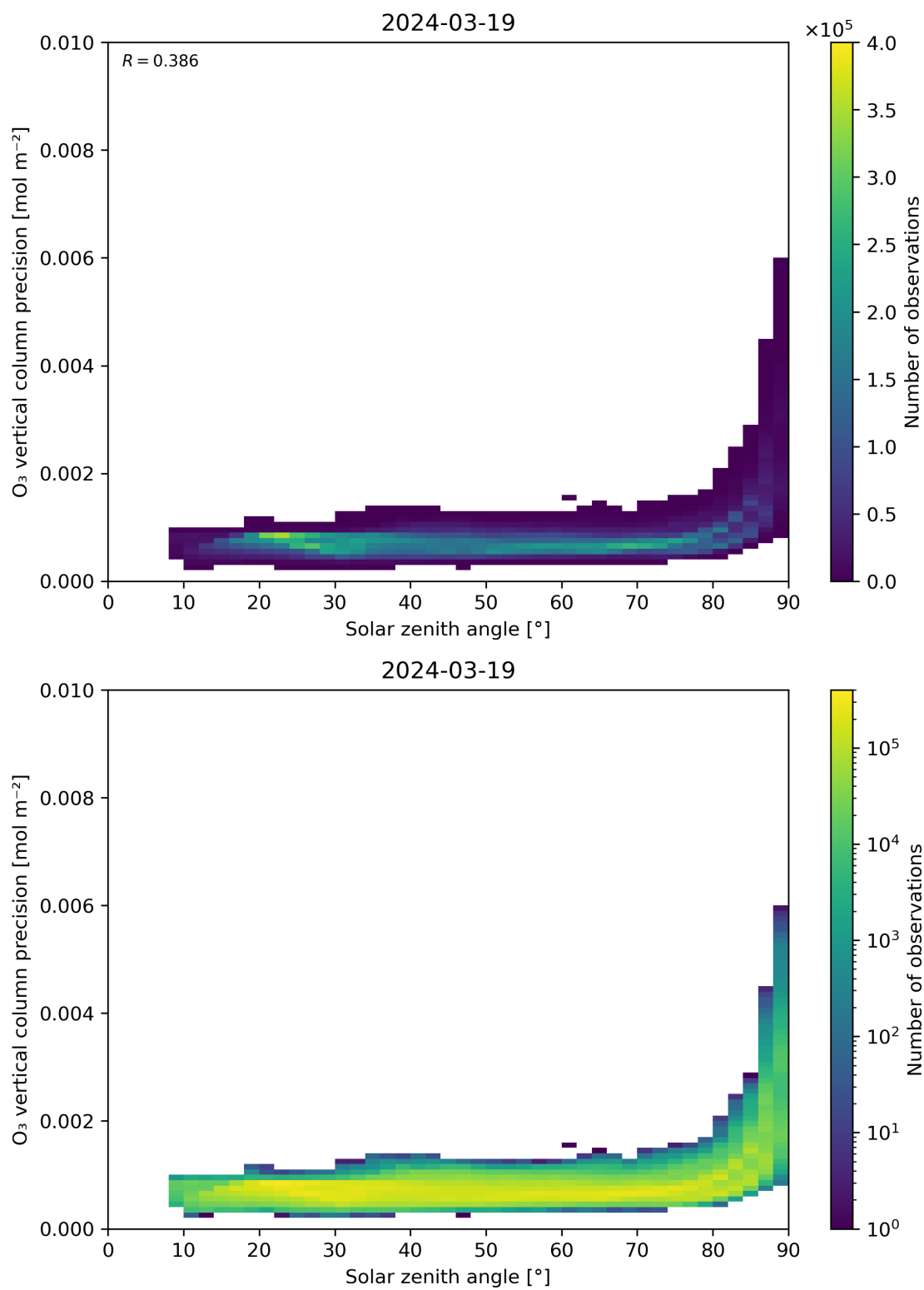
Figure 48: Scatter density plot of “Solar zenith angle” against “O 3 vertical column precision” for 2024-03-18 to 2024-03-20.
