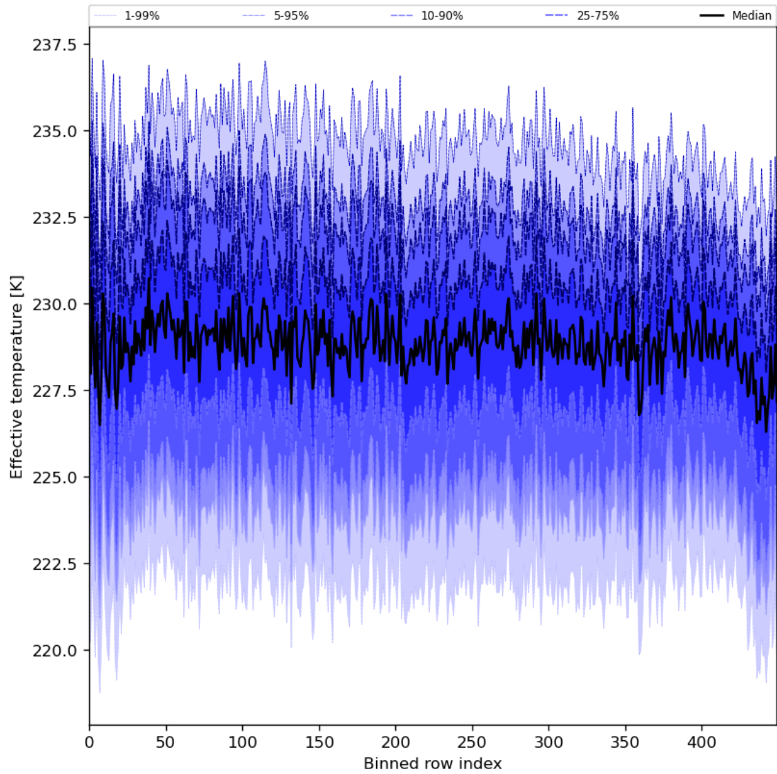
Figure 31: Along track statistics of “Effective temperature” for 2024-03-18 to 2024-03-20
