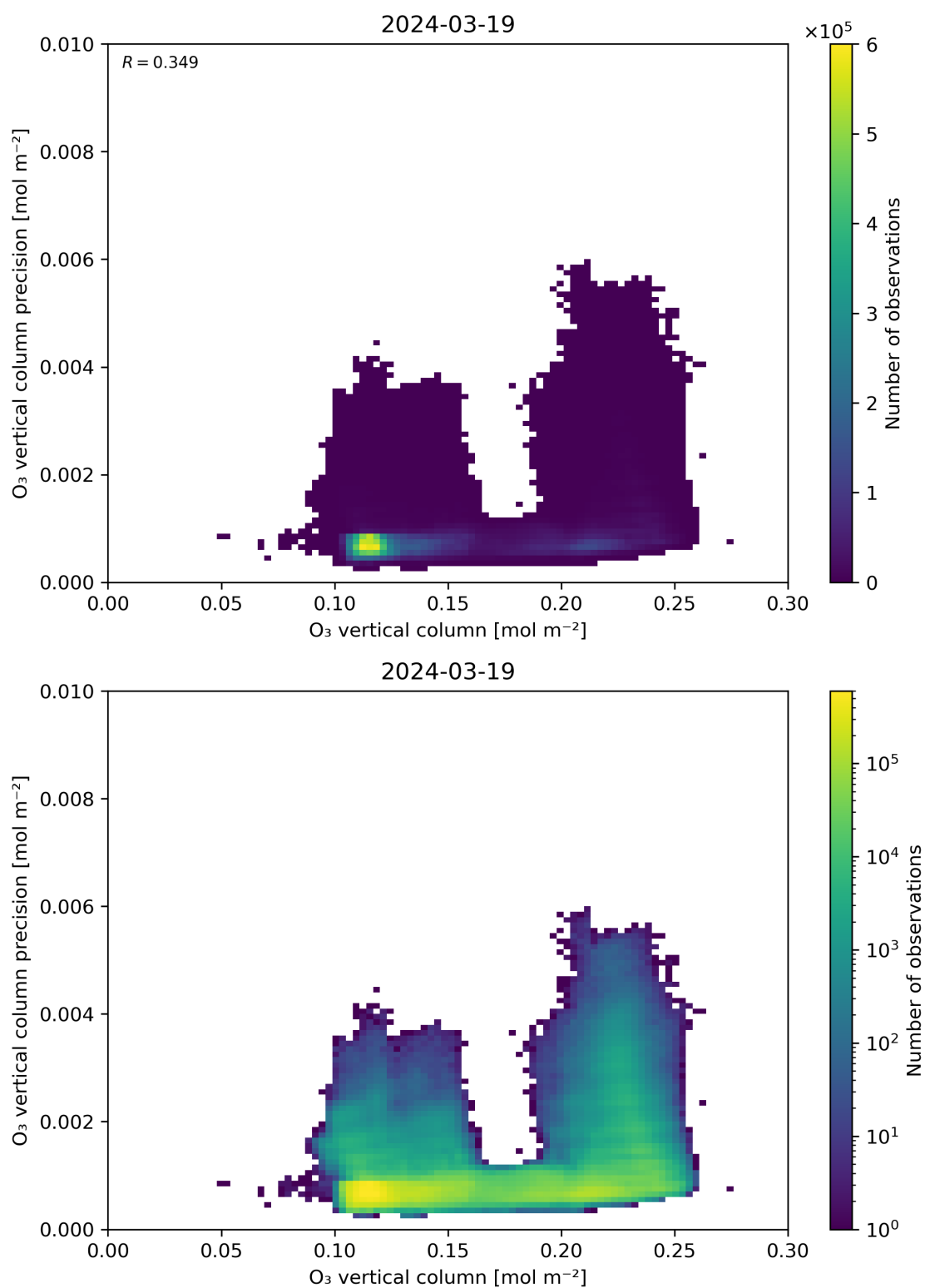
Figure 41: Scatter density plot of “O 3 vertical column” against “O 3 vertical column precision” for 2024-03-18 to 2024-03-20.
