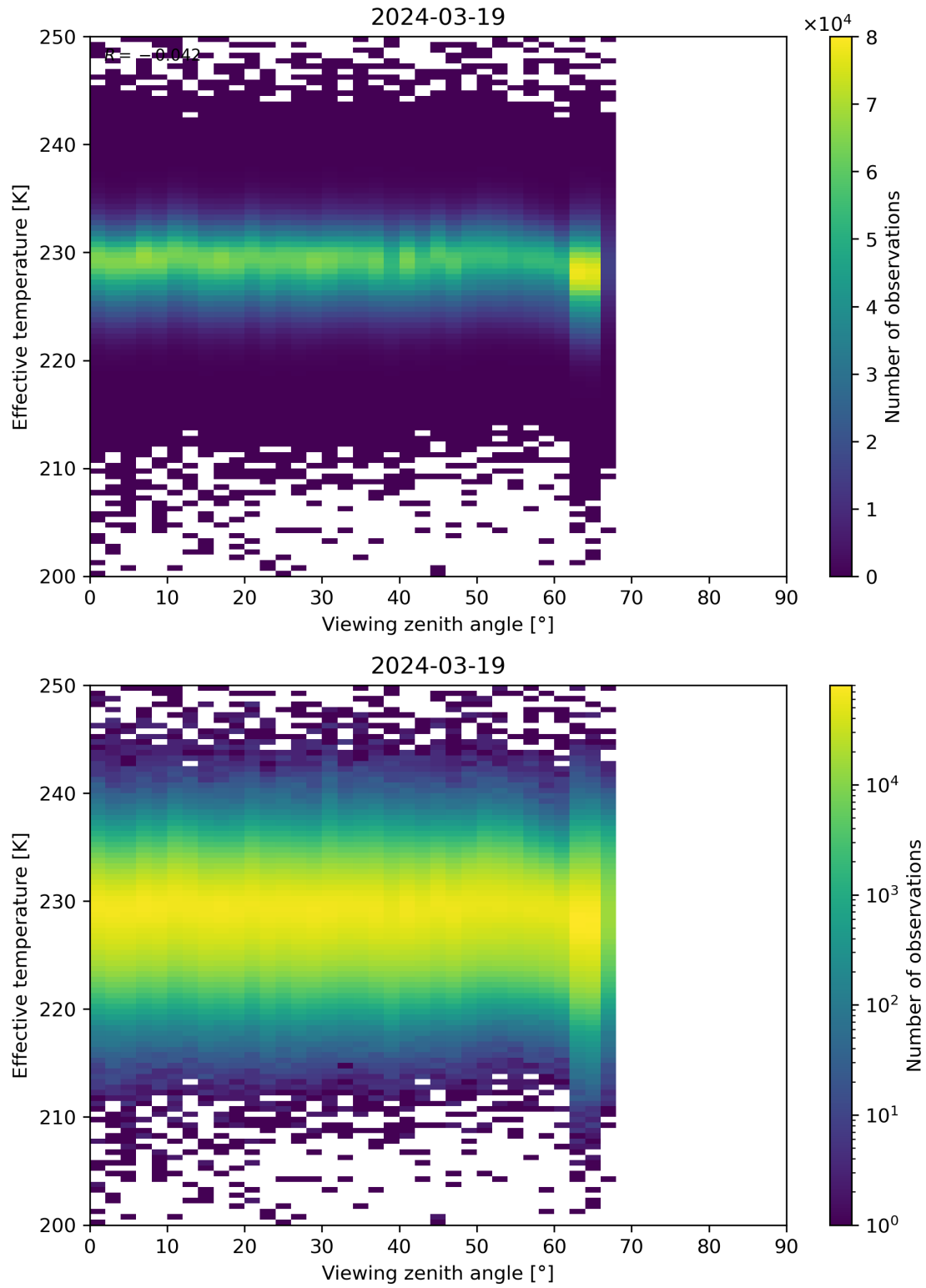
Figure 50: Scatter density plot of “Viewing zenith angle” against “Effective temperature” for 2024-03-18 to 2024-03-20.
