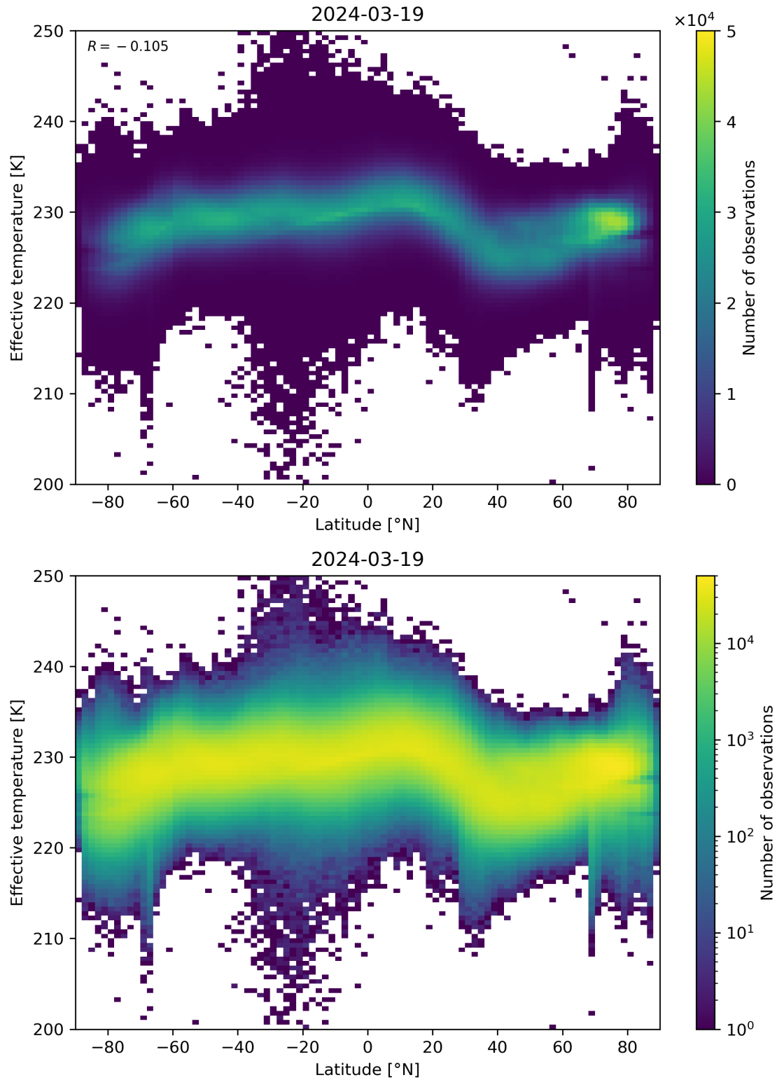
Figure 34: Scatter density plot of “Latitude” against “Effective temperature” for 2024-03-18 to 2024-03-20.
