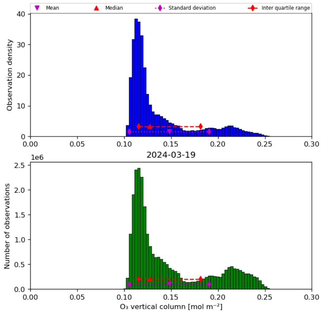
Figure 21: Histogram of “O 3 vertical column” for 2024-03-18 to 2024-03-20
