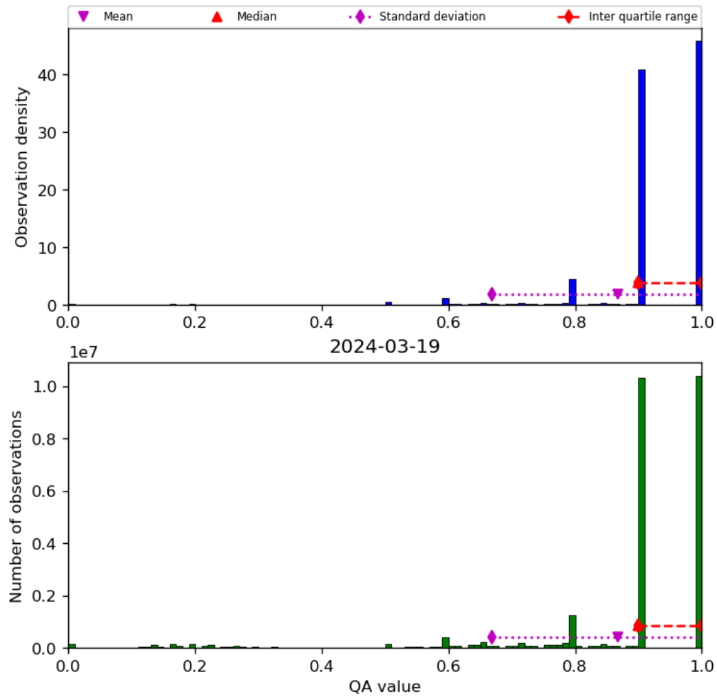
Figure 20: Histogram of “QA value” for 2024-03-18 to 2024-03-20
