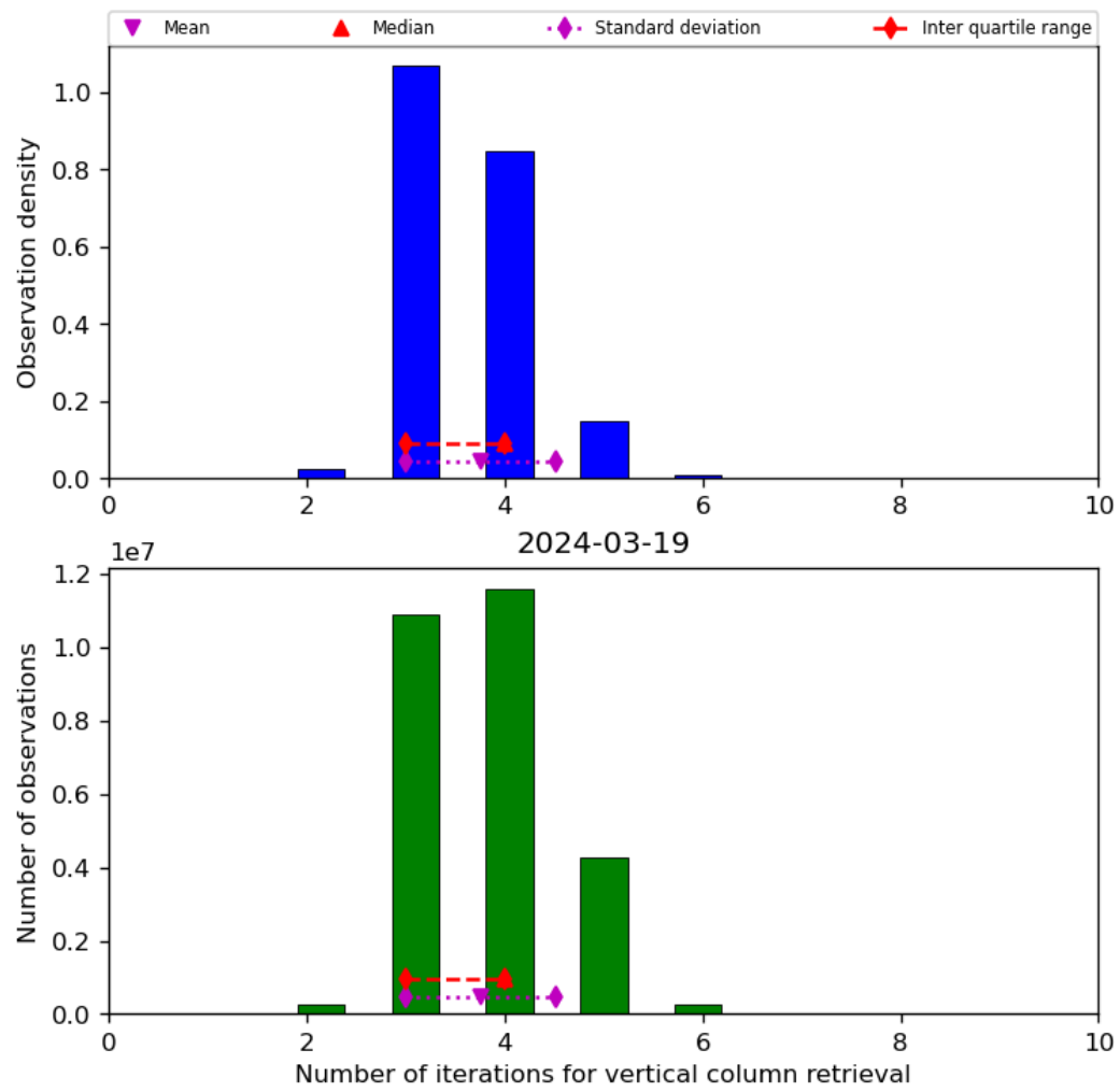
Figure 26: Histogram of “Number of iterations for vertical column retrieval” for 2024-03-18 to 2024-03-20
