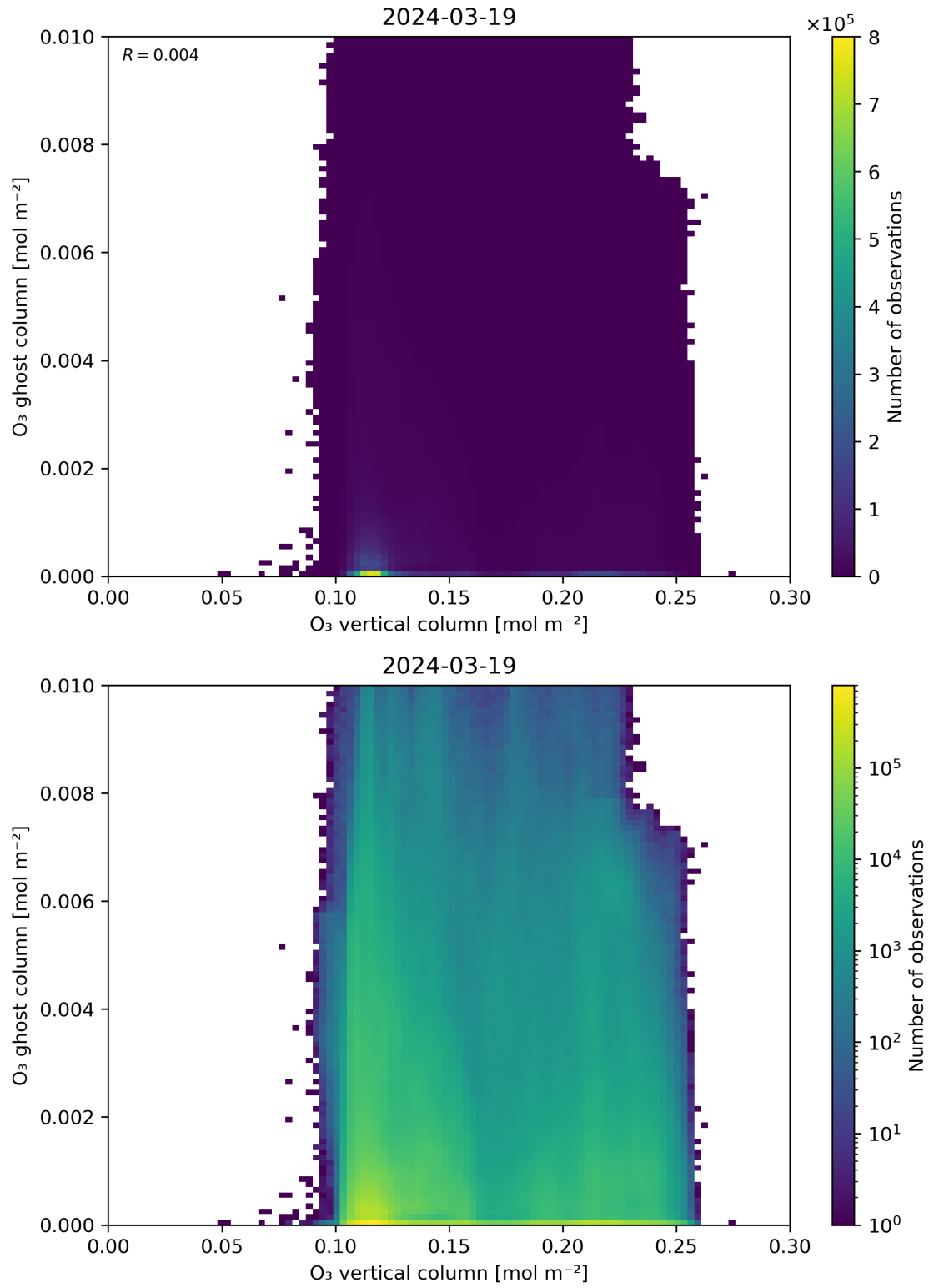
Figure 40: Scatter density plot of “O 3 vertical column” against “O 3 ghost column” for 2024-03-18 to 2024-03-20.
