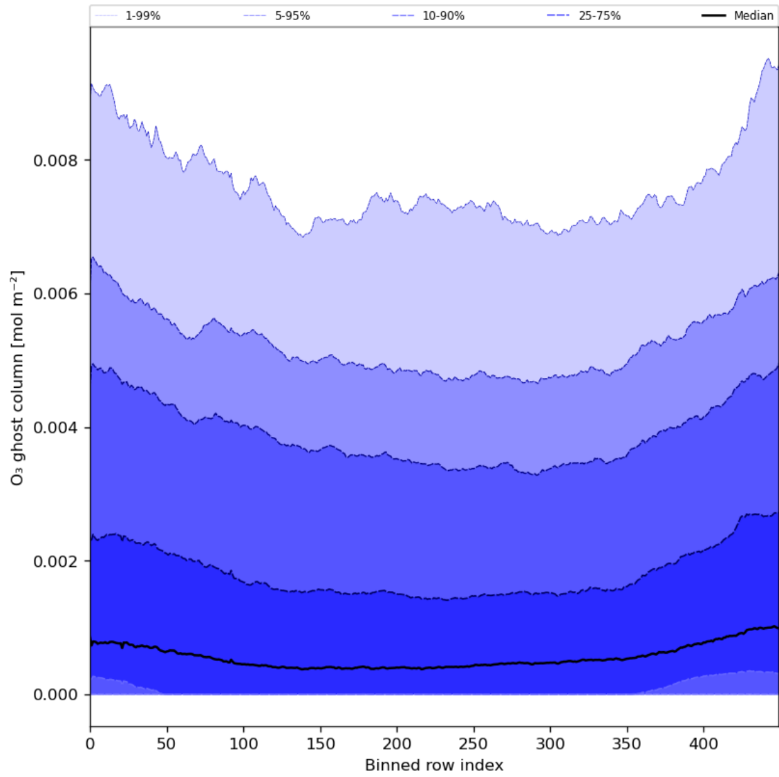
Figure 32: Along track statistics of “O 3 ghost column” for 2024-03-18 to 2024-03-20
