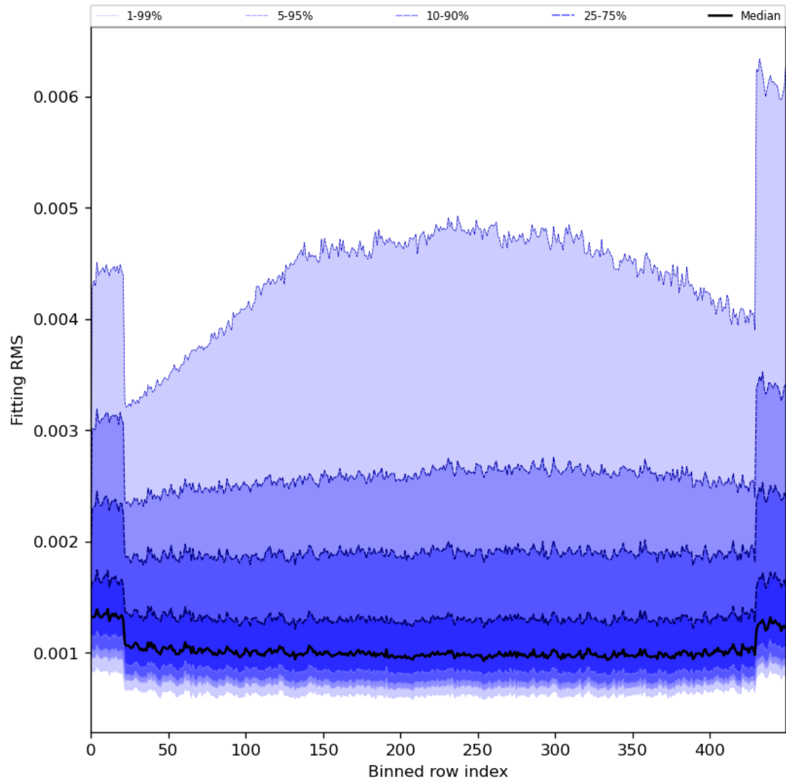
Figure 30: Along track statistics of “Fitting RMS” for 2024-03-18 to 2024-03-20
