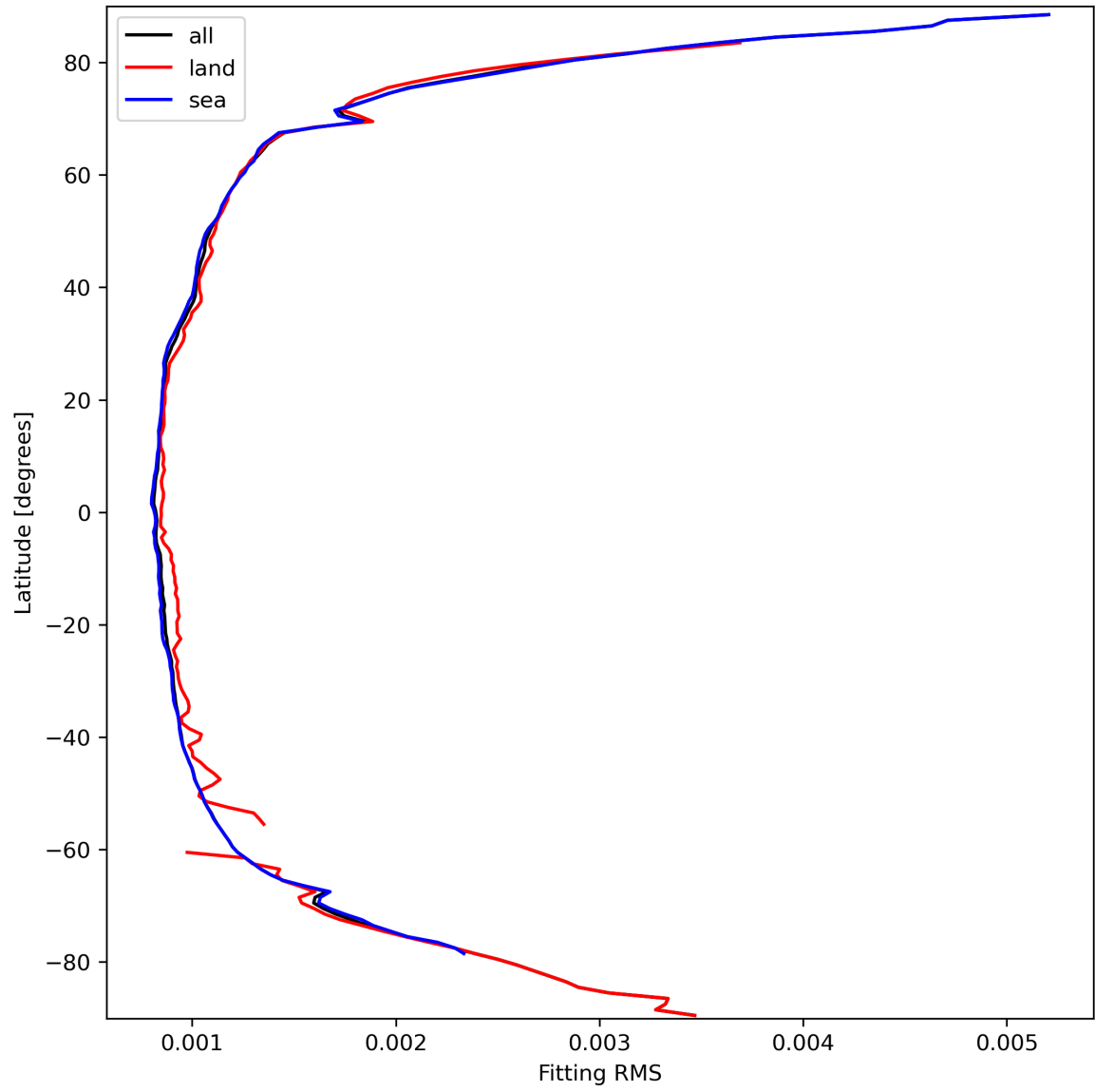
Figure 16: Zonal average of “Fitting RMS” for 2024-03-18 to 2024-03-20.
