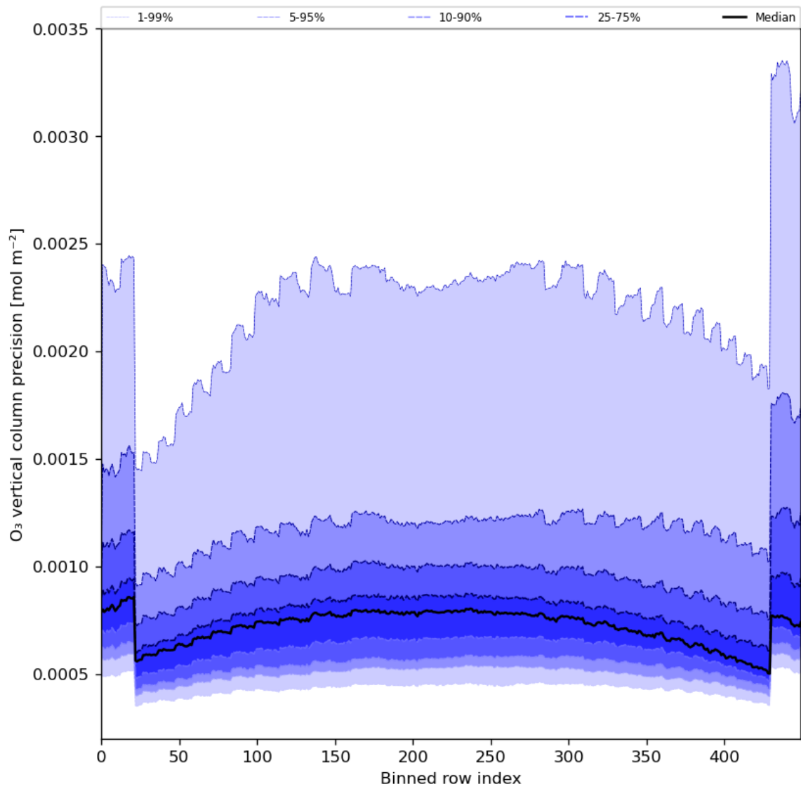
Figure 29: Along track statistics of “O 3 vertical column precision” for 2024-03-18 to 2024-03-20
