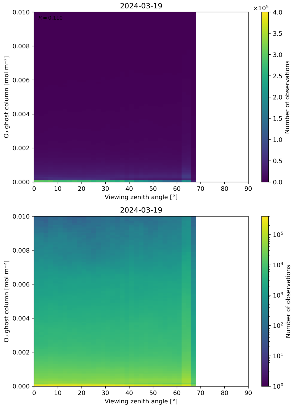
Figure 51: Scatter density plot of “Viewing zenith angle” against “O 3 ghost column” for 2024-03-18 to 2024-03-20.
