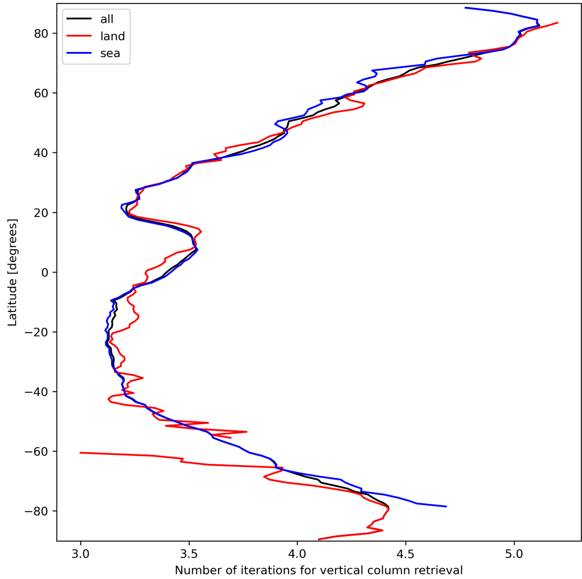
Figure 19: Zonal average of “Number of iterations for vertical column retrieval” for 2024-03-18 to 2024-03-20.
