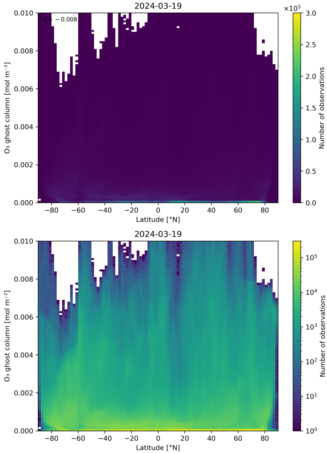
Figure 35: Scatter density plot of “Latitude” against “O 3 ghost column” for 2024-03-18 to 2024-03-20.
