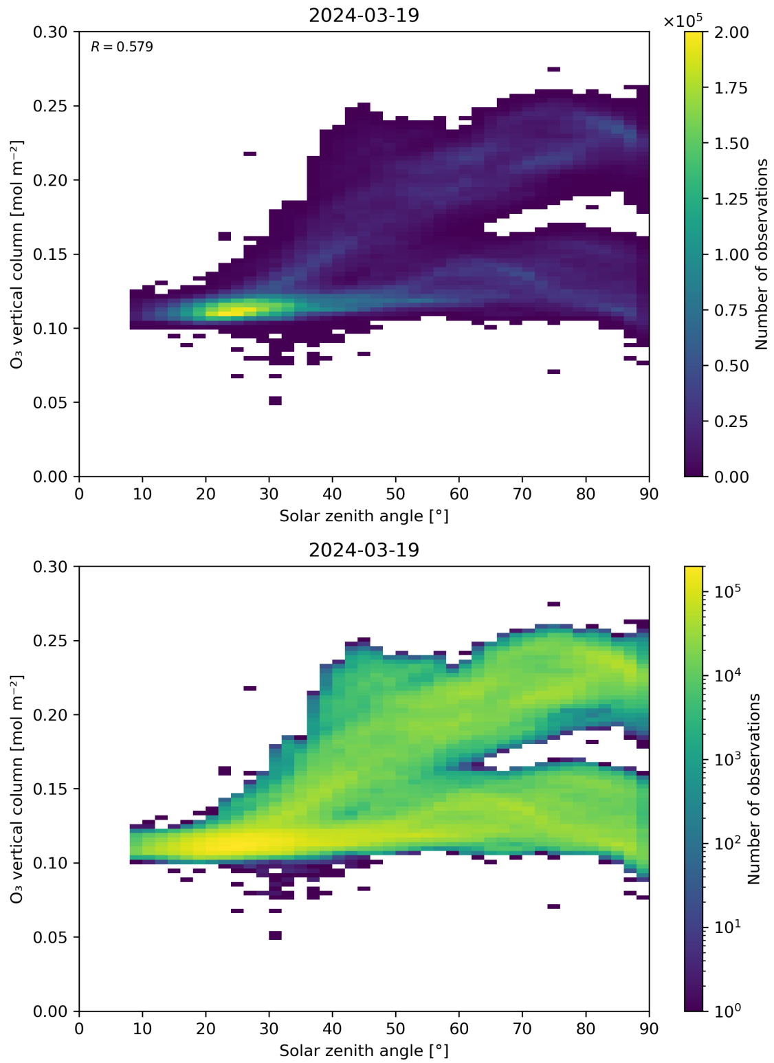
Figure 47: Scatter density plot of “Solar zenith angle” against “O 3 vertical column” for 2024-03-18 to 2024-03-20.
