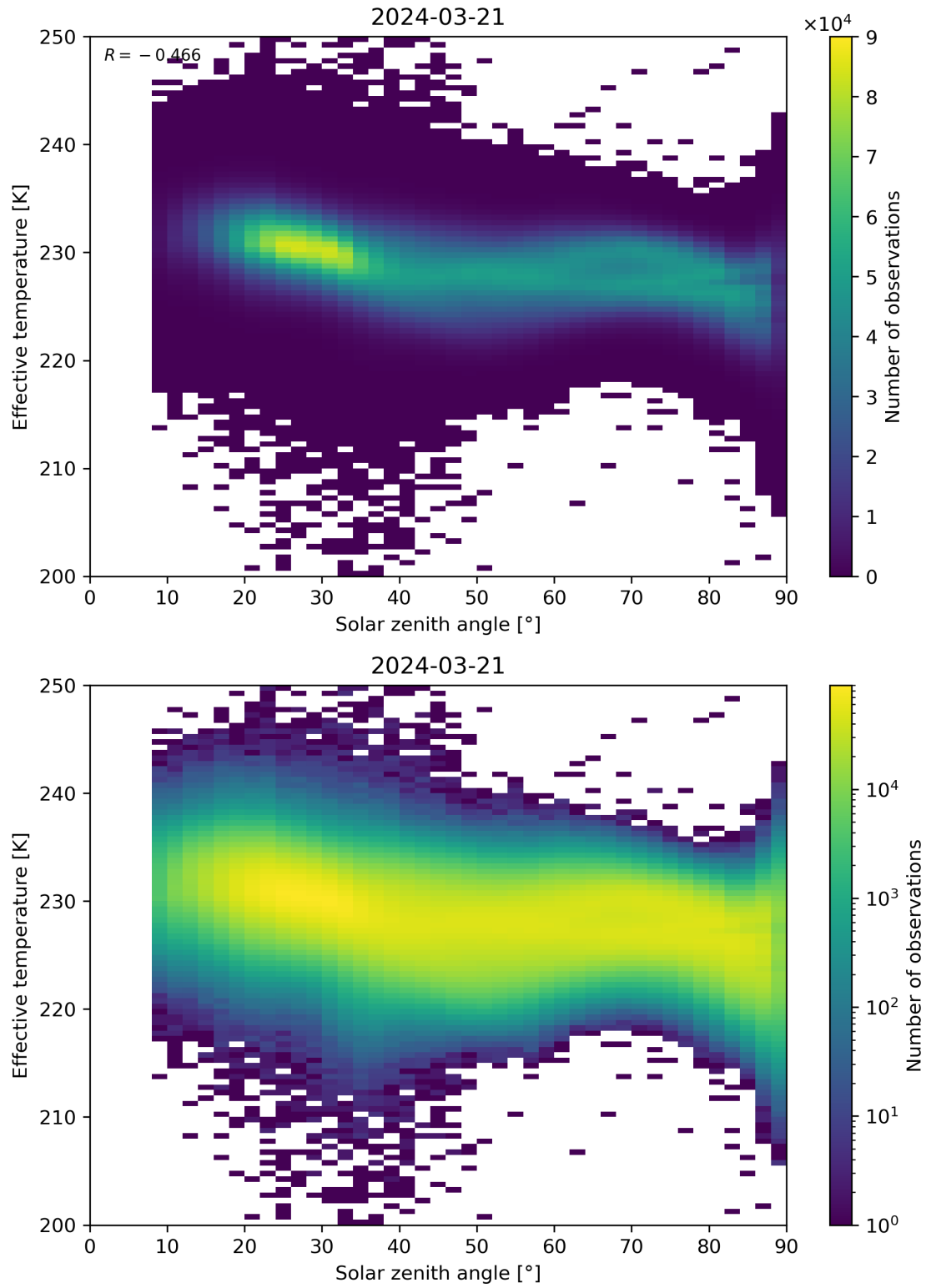
Figure 45: Scatter density plot of “Solar zenith angle” against “Effective temperature” for 2024-03-20 to 2024-03-22.
