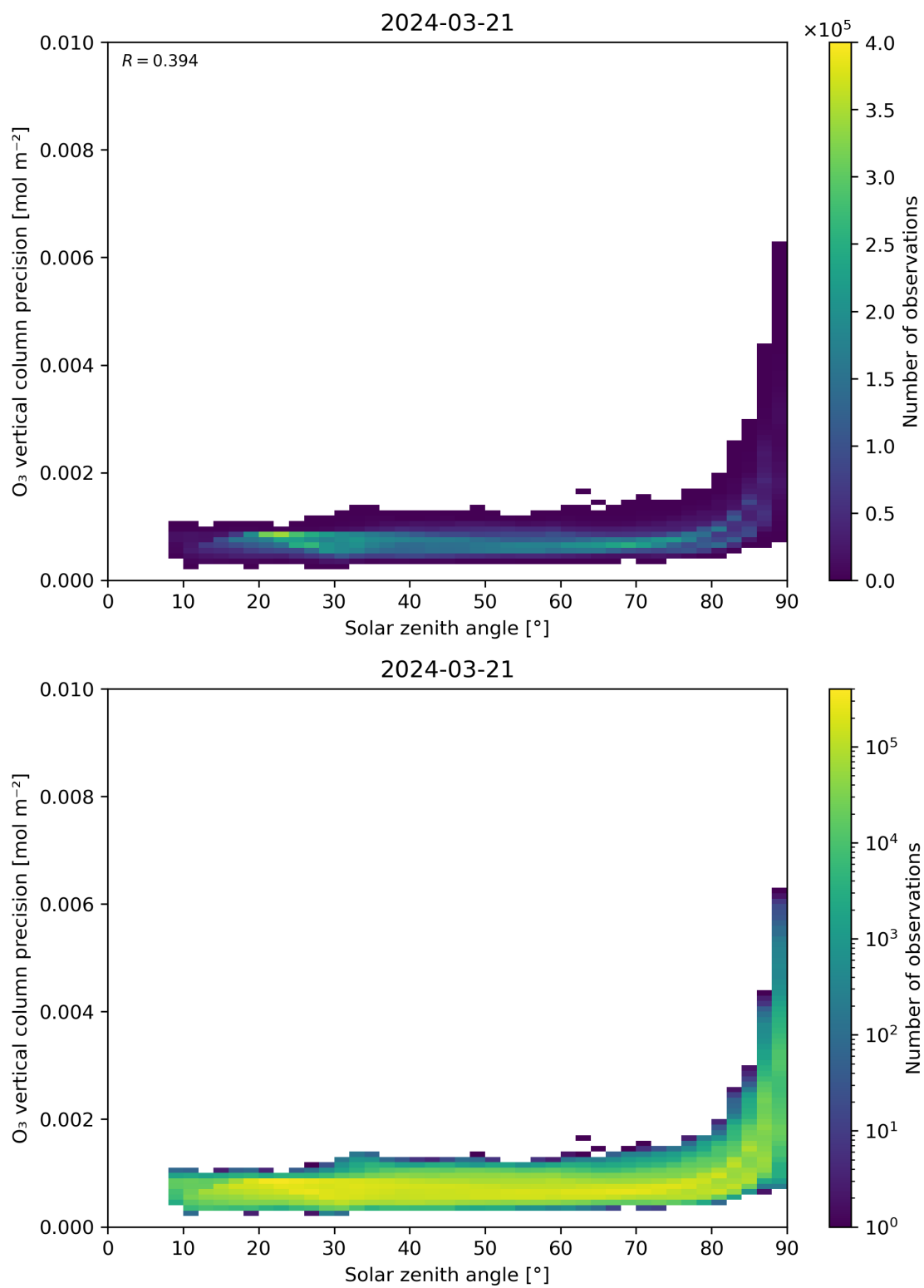
Figure 48: Scatter density plot of “Solar zenith angle” against “O 3 vertical column precision” for 2024-03-20 to 2024-03-22.
