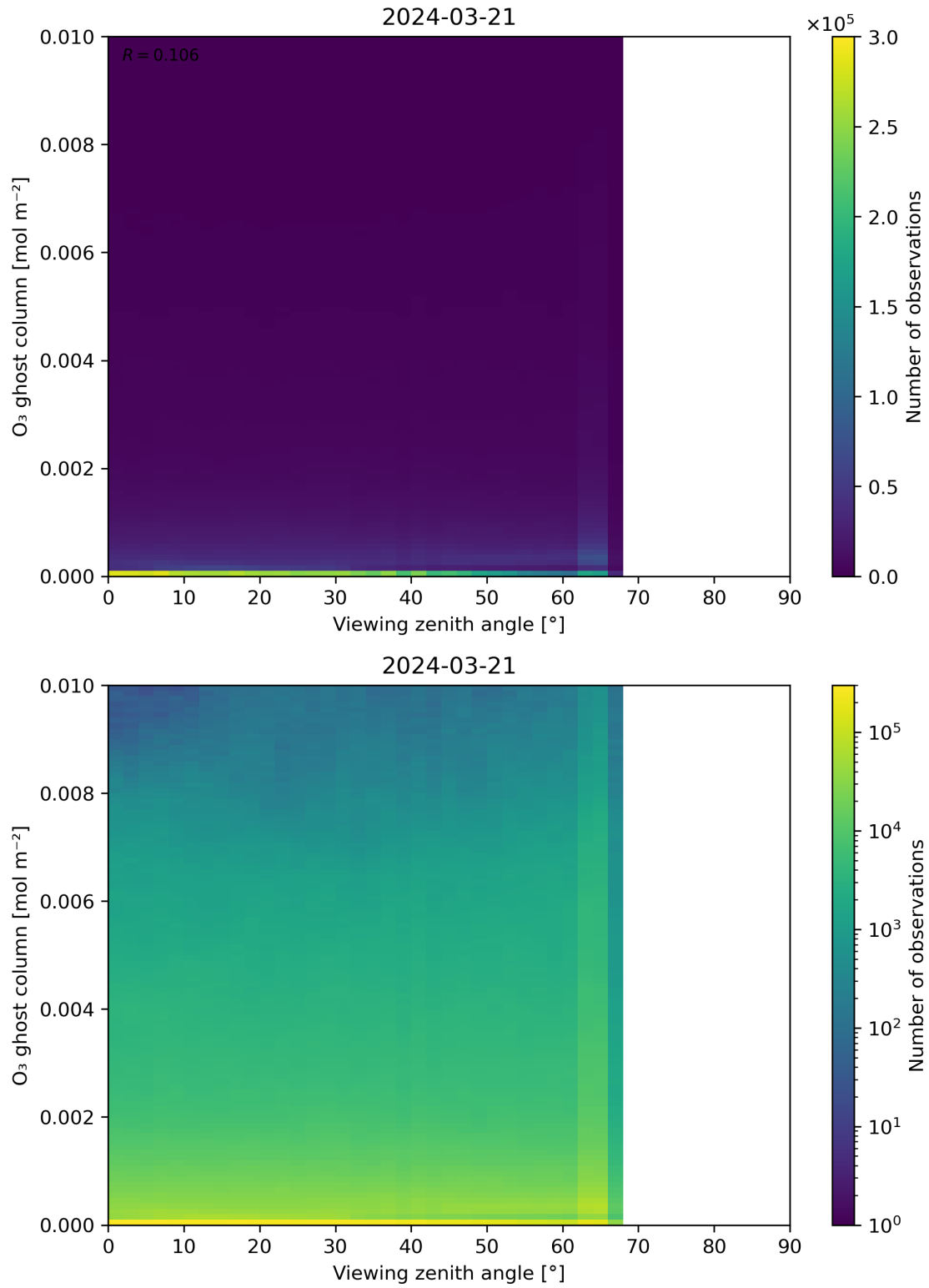
Figure 51: Scatter density plot of “Viewing zenith angle” against “O 3 ghost column” for 2024-03-20 to 2024-03-22.
