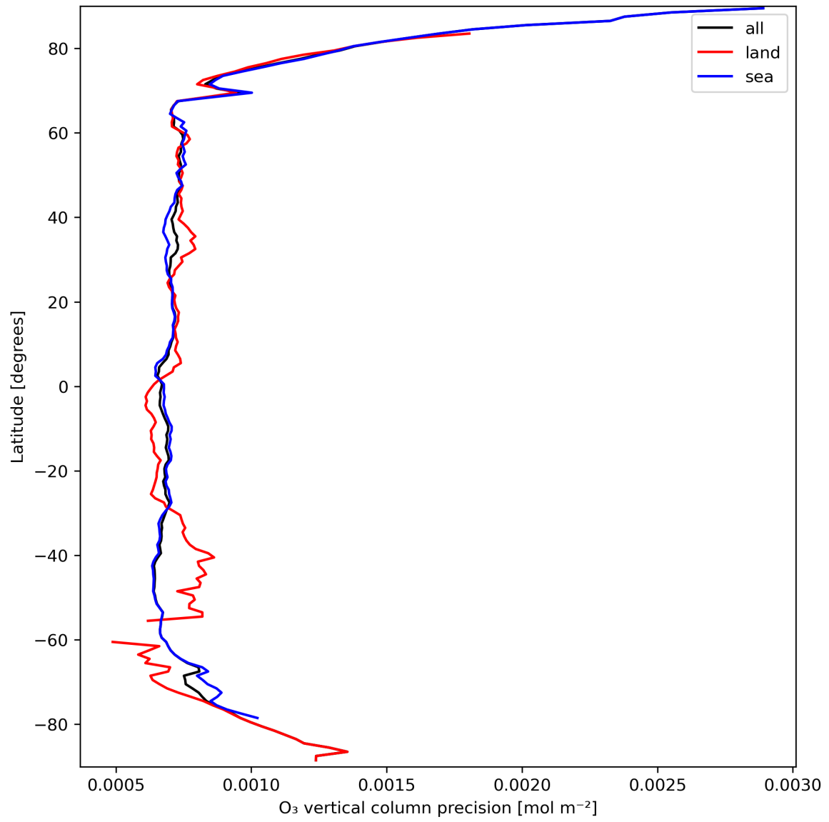
Figure 15: Zonal average of “O 3 vertical column precision” for 2024-03-20 to 2024-03-22.
