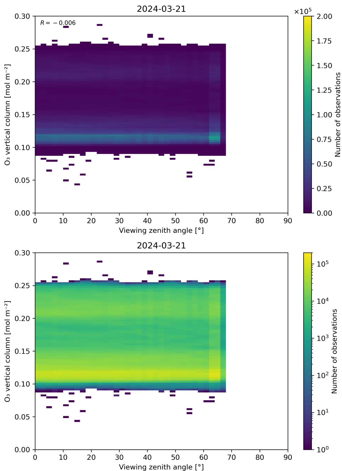
Figure 52: Scatter density plot of “Viewing zenith angle” against “O 3 vertical column” for 2024-03-20 to 2024-03-22.
