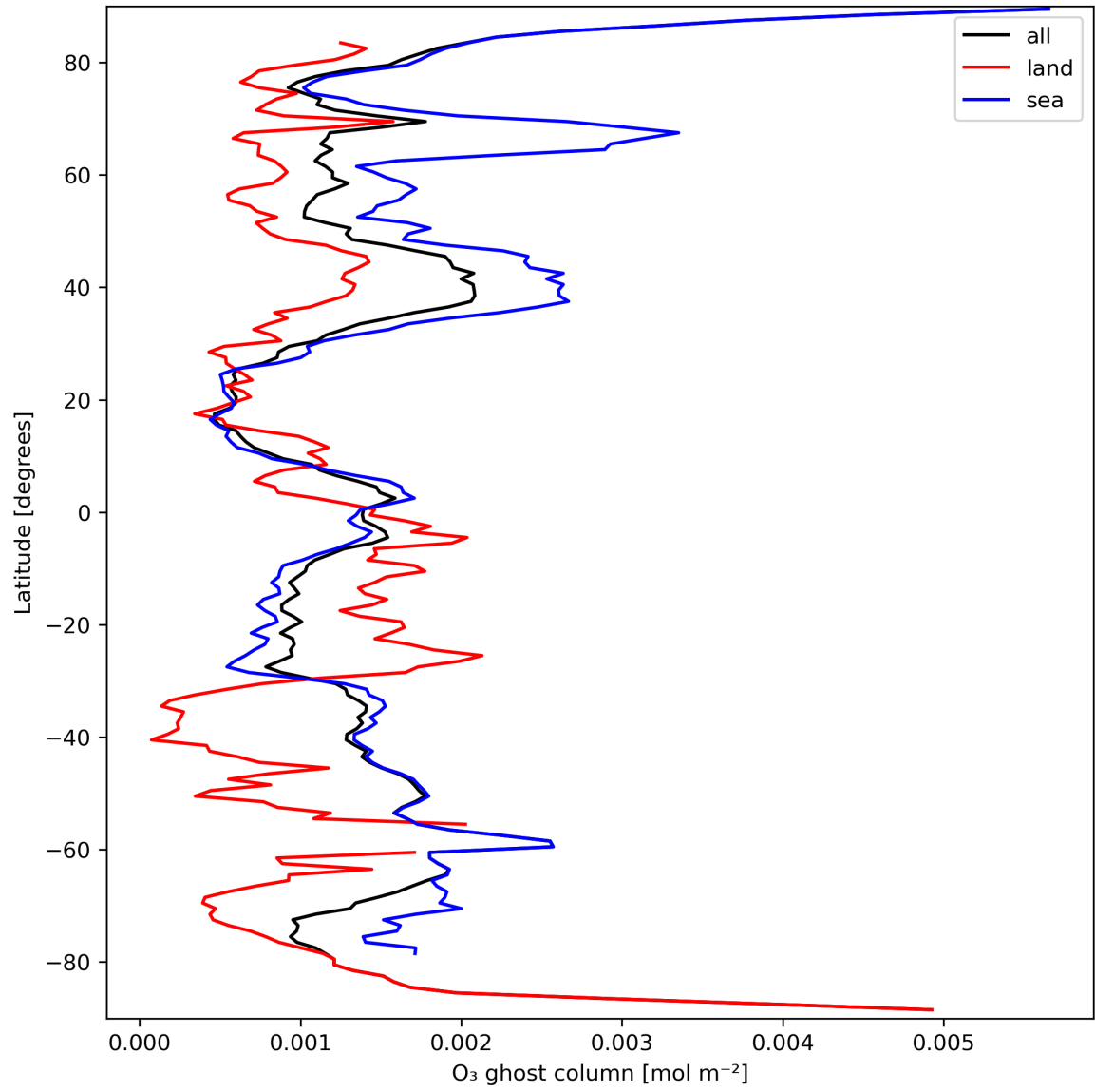
Figure 18: Zonal average of "O 3 ghost column" for 2024-03-20 to 2024-03-22.
