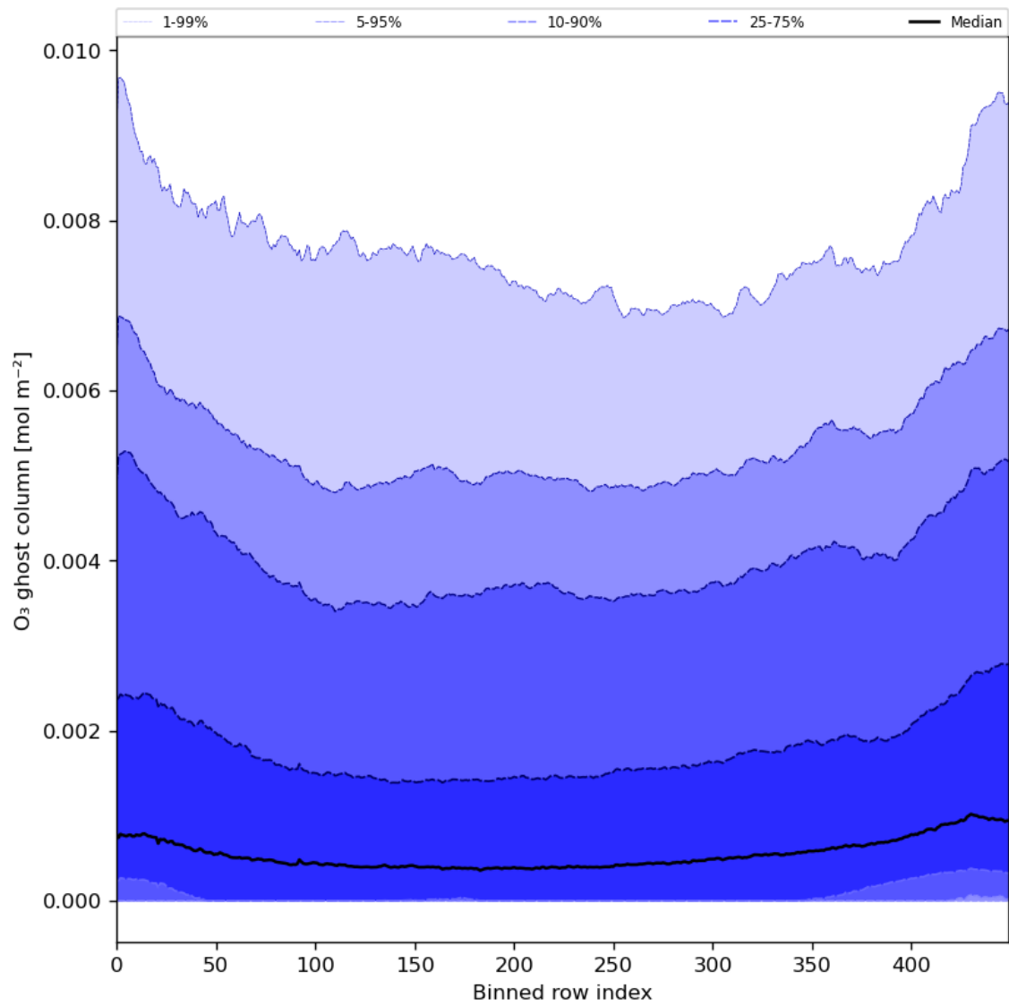
Figure 32: Along track statistics of “O 3 ghost column” for 2024-03-20 to 2024-03-22
