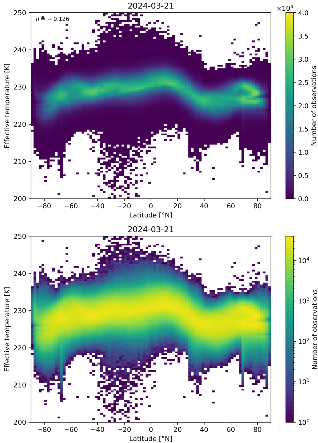
Figure 34: Scatter density plot of “Latitude” against “Effective temperature” for 2024-03-20 to 2024-03-22.
