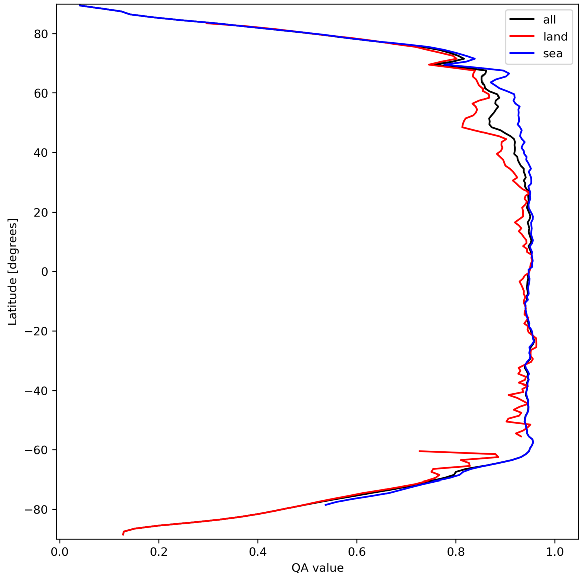
Figure 13: Zonal average of “QA value” for 2024-03-20 to 2024-03-22.
