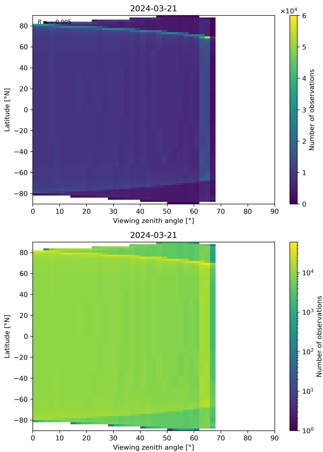
Figure 49: Scatter density plot of “Viewing zenith angle” against “Latitude” for 2024-03-20 to 2024-03-22.
