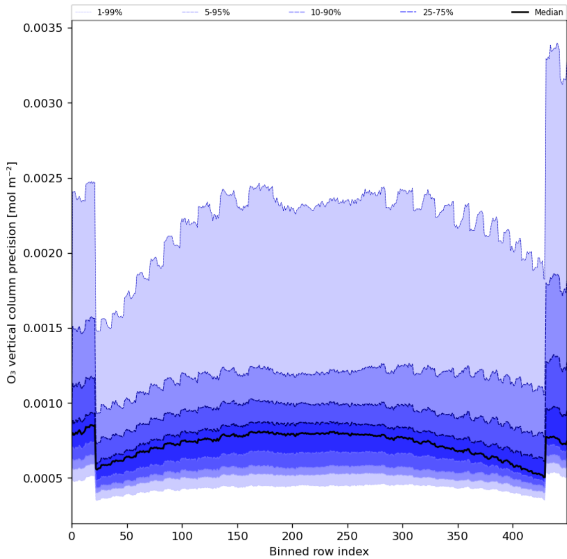
Figure 29: Along track statistics of “O 3 vertical column precision” for 2024-03-20 to 2024-03-22
