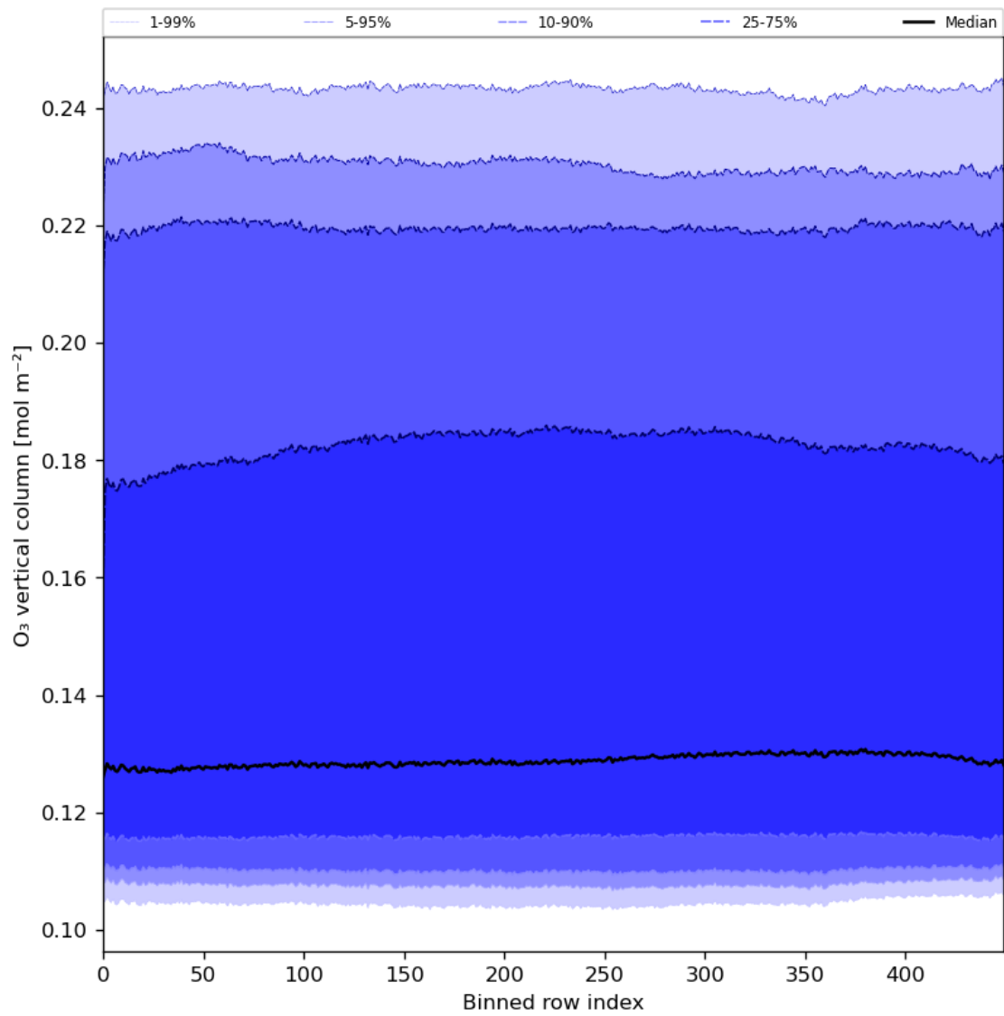
Figure 28: Along track statistics of “O 3 vertical column” for 2024-03-20 to 2024-03-22
