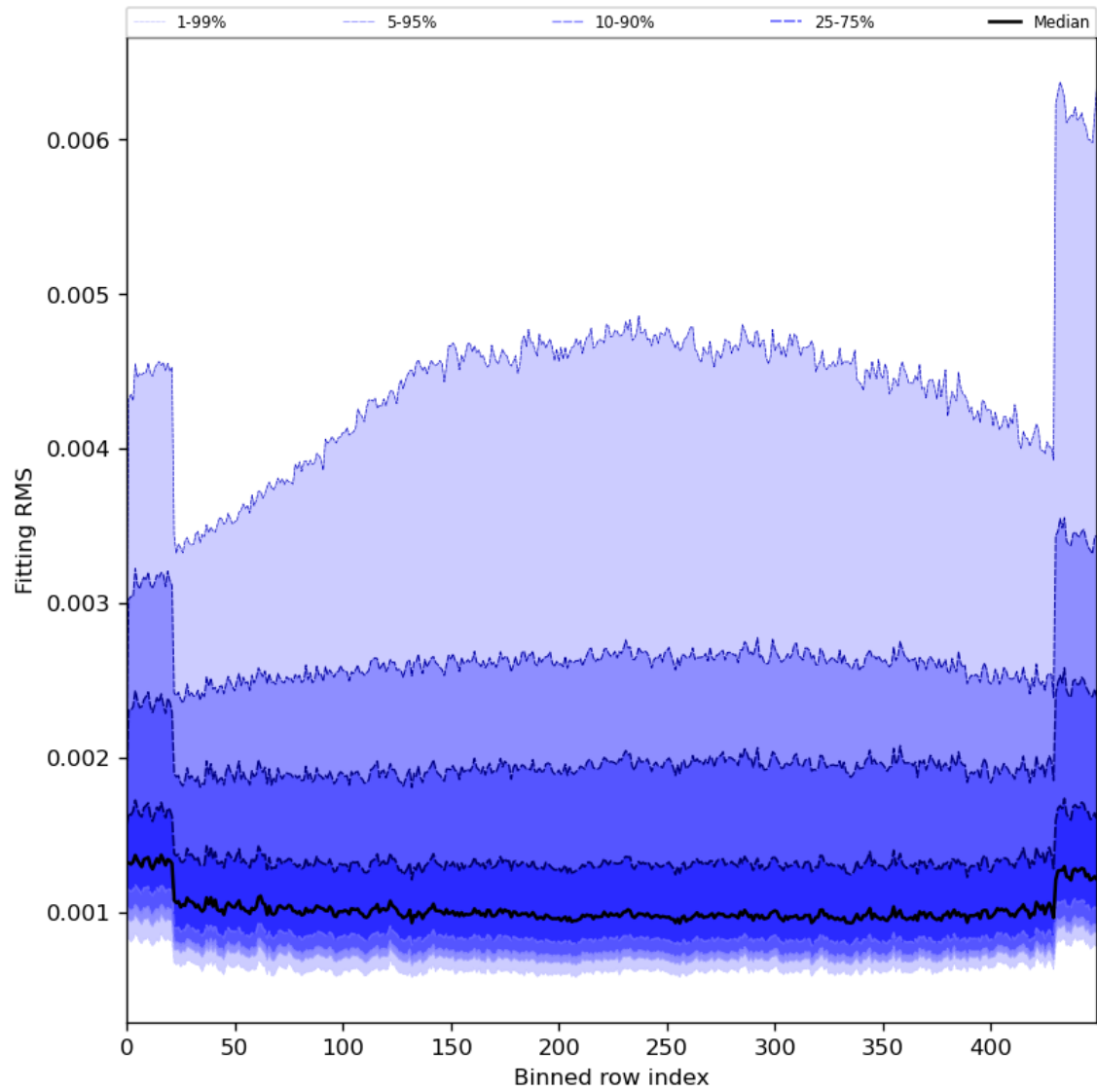
Figure 30: Along track statistics of “Fitting RMS” for 2024-03-20 to 2024-03-22
