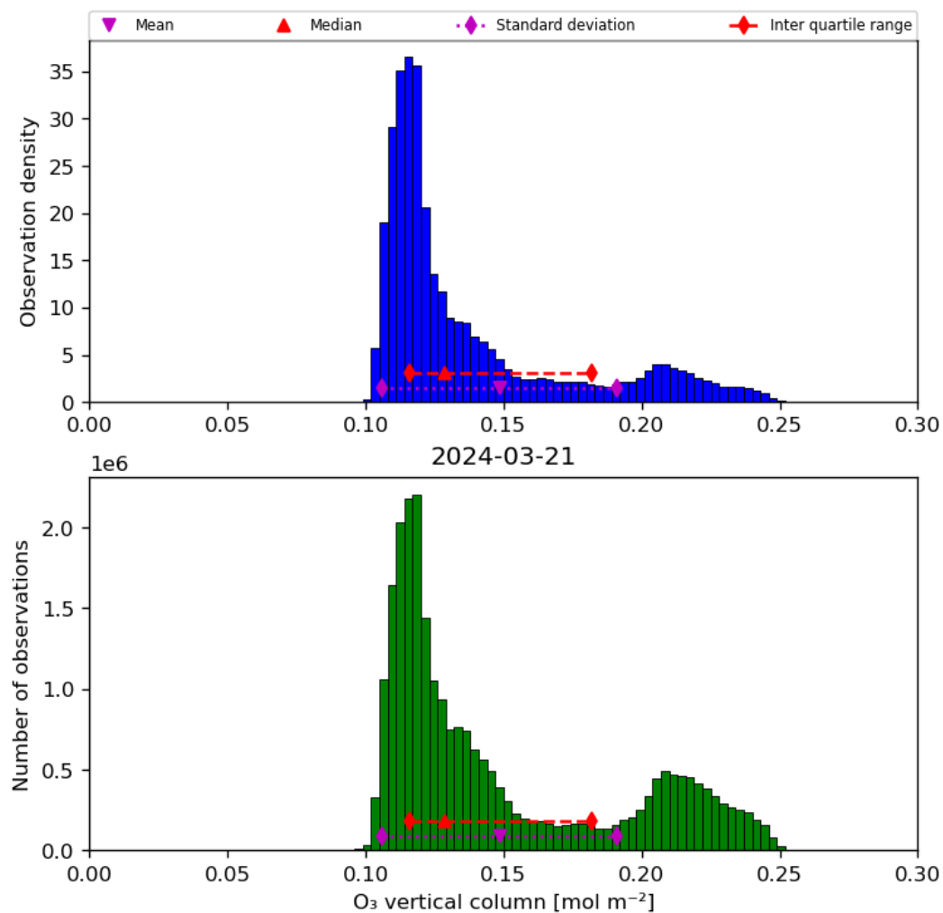
Figure 21: Histogram of “O 3 vertical column” for 2024-03-20 to 2024-03-22
