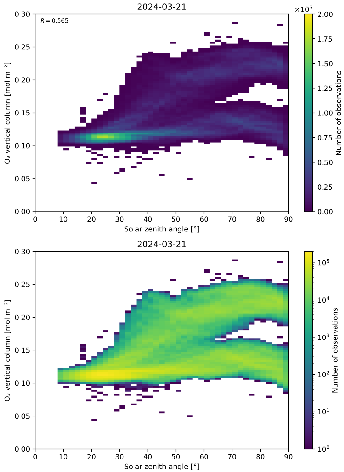
Figure 47: Scatter density plot of “Solar zenith angle” against “O 3 vertical column” for 2024-03-20 to 2024-03-22.
