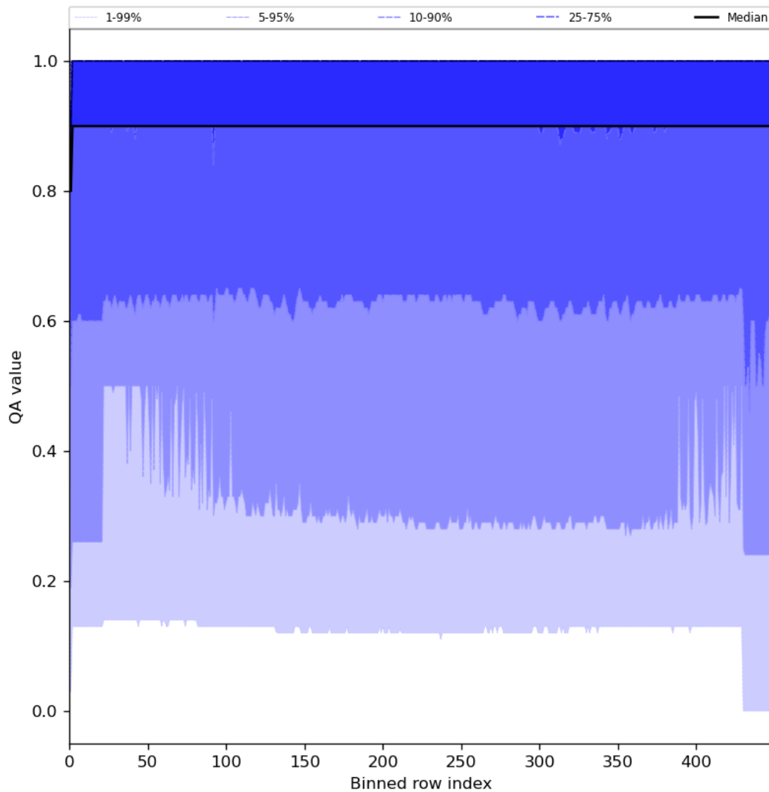
Figure 27: Along track statistics of “QA value” for 2024-03-20 to 2024-03-22
