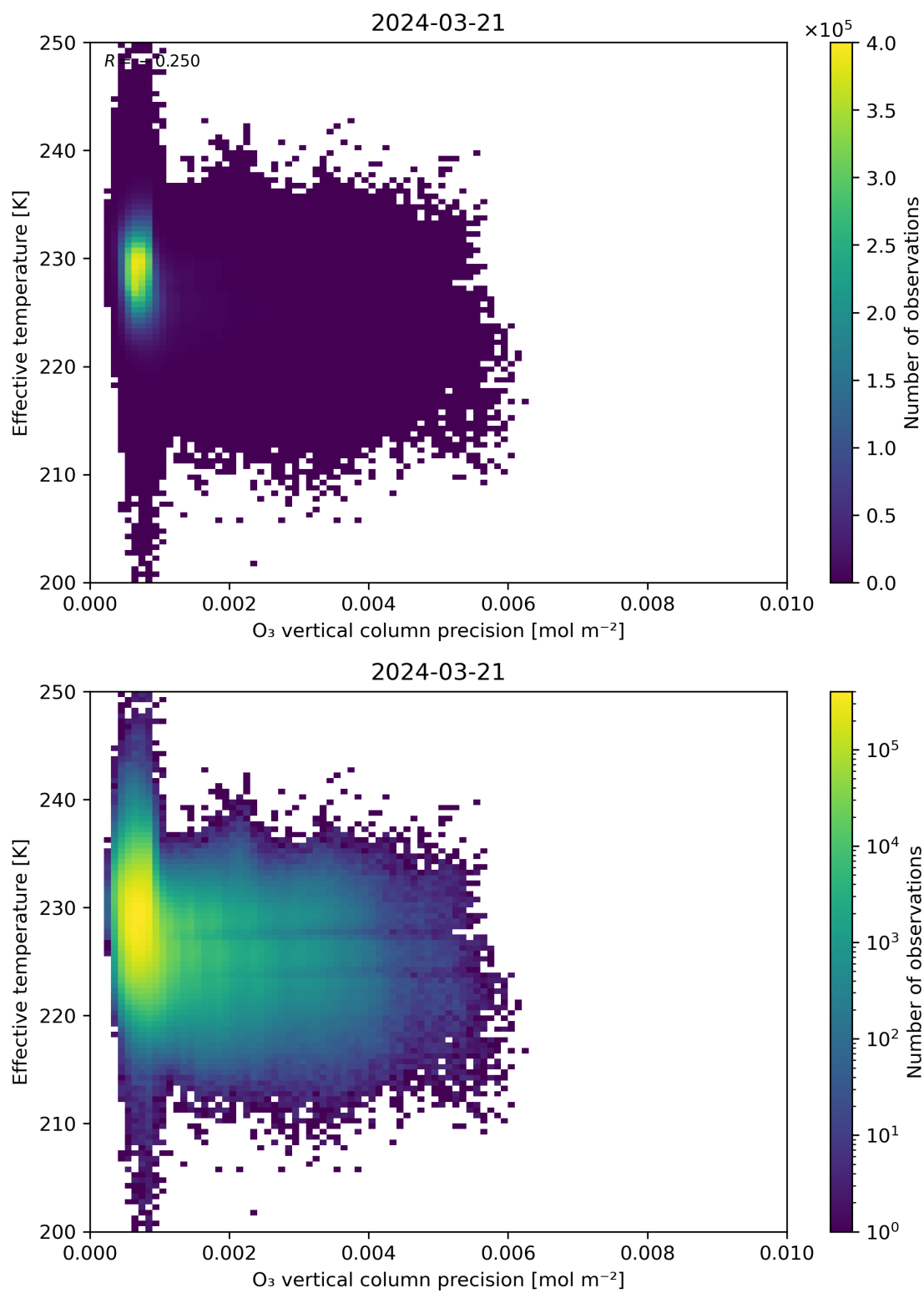
Figure 42: Scatter density plot of “O 3 vertical column precision” against “Effective temperature” for 2024-03-20 to 2024-03-22.
