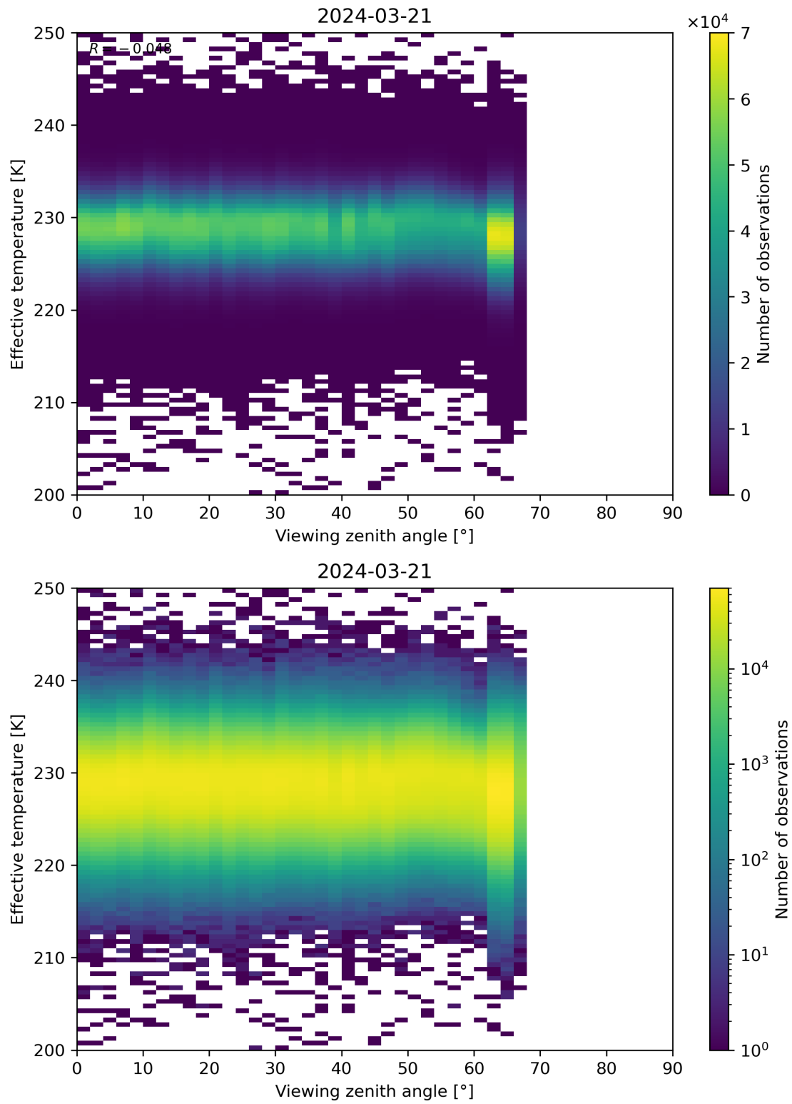
Figure 50: Scatter density plot of “Viewing zenith angle” against “Effective temperature” for 2024-03-20 to 2024-03-22.
