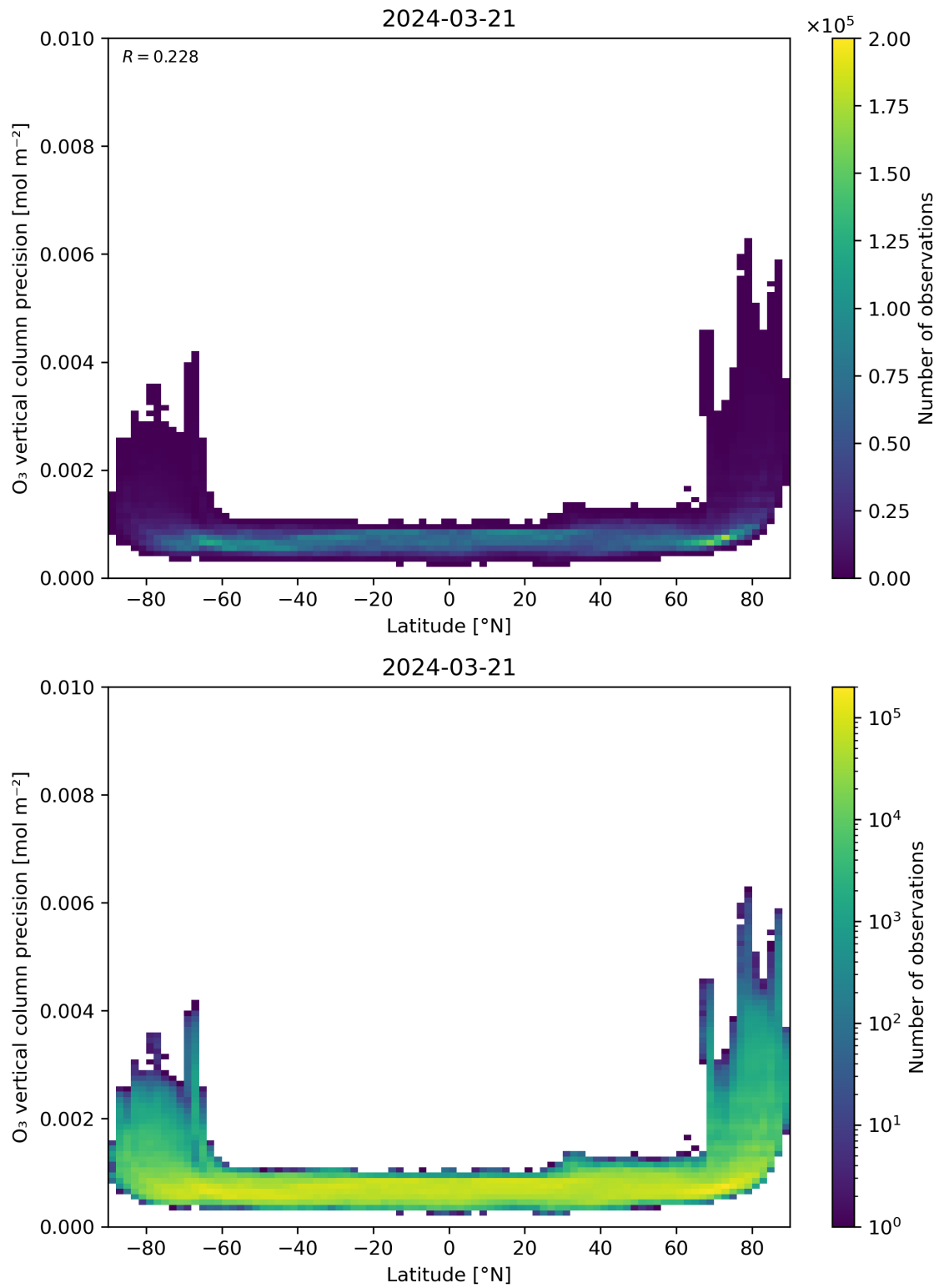
Figure 37: Scatter density plot of “Latitude” against “O 3 vertical column precision” for 2024-03-20 to 2024-03-22.
