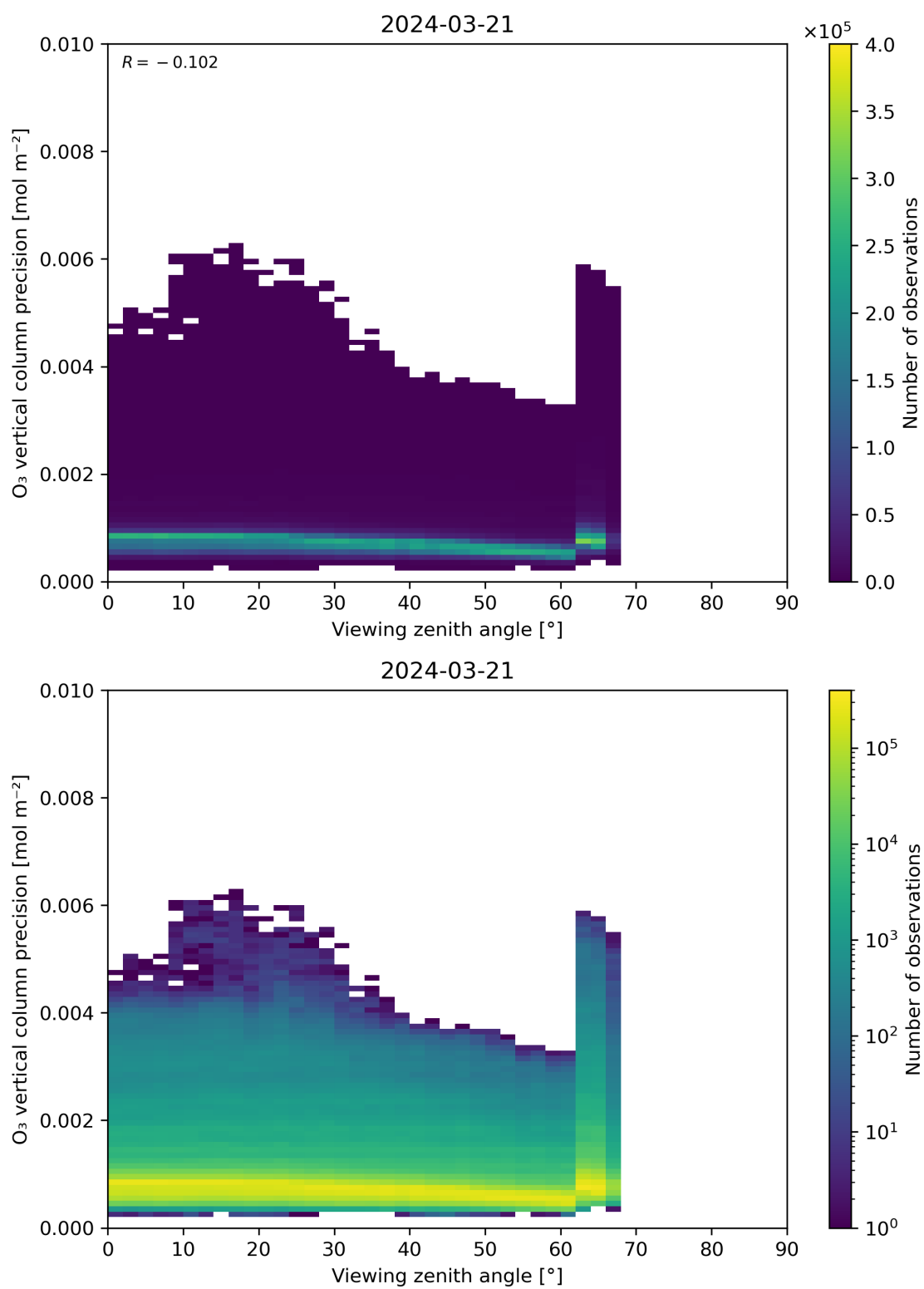
Figure 53: Scatter density plot of “Viewing zenith angle” against “O 3 vertical column precision” for 2024-03-20 to 2024-03-22.
