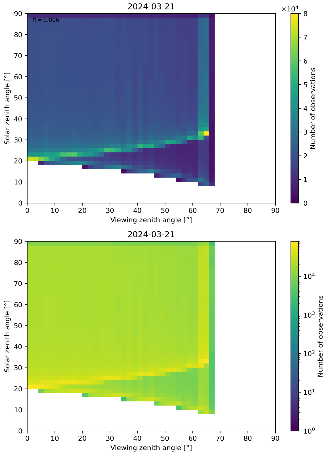
Figure 54: Scatter density plot of “Viewing zenith angle” against “Solar zenith angle” for 2024-03-20 to 2024-03-22.
