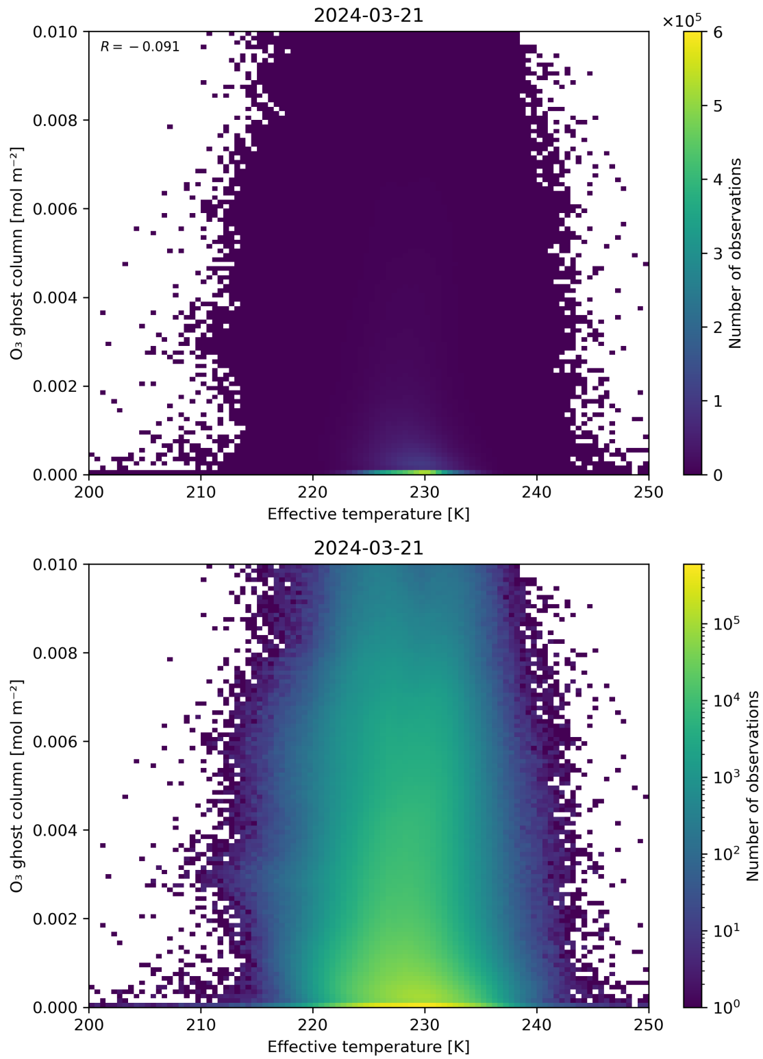
Figure 38: Scatter density plot of “Effective temperature” against “O 3 ghost column” for 2024-03-20 to 2024-03-22.
