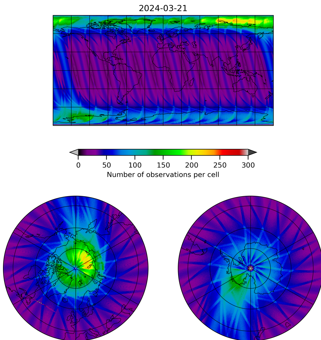
Figure 12: Map of the number of observations for 2024-03-20 to 2024-03-22
