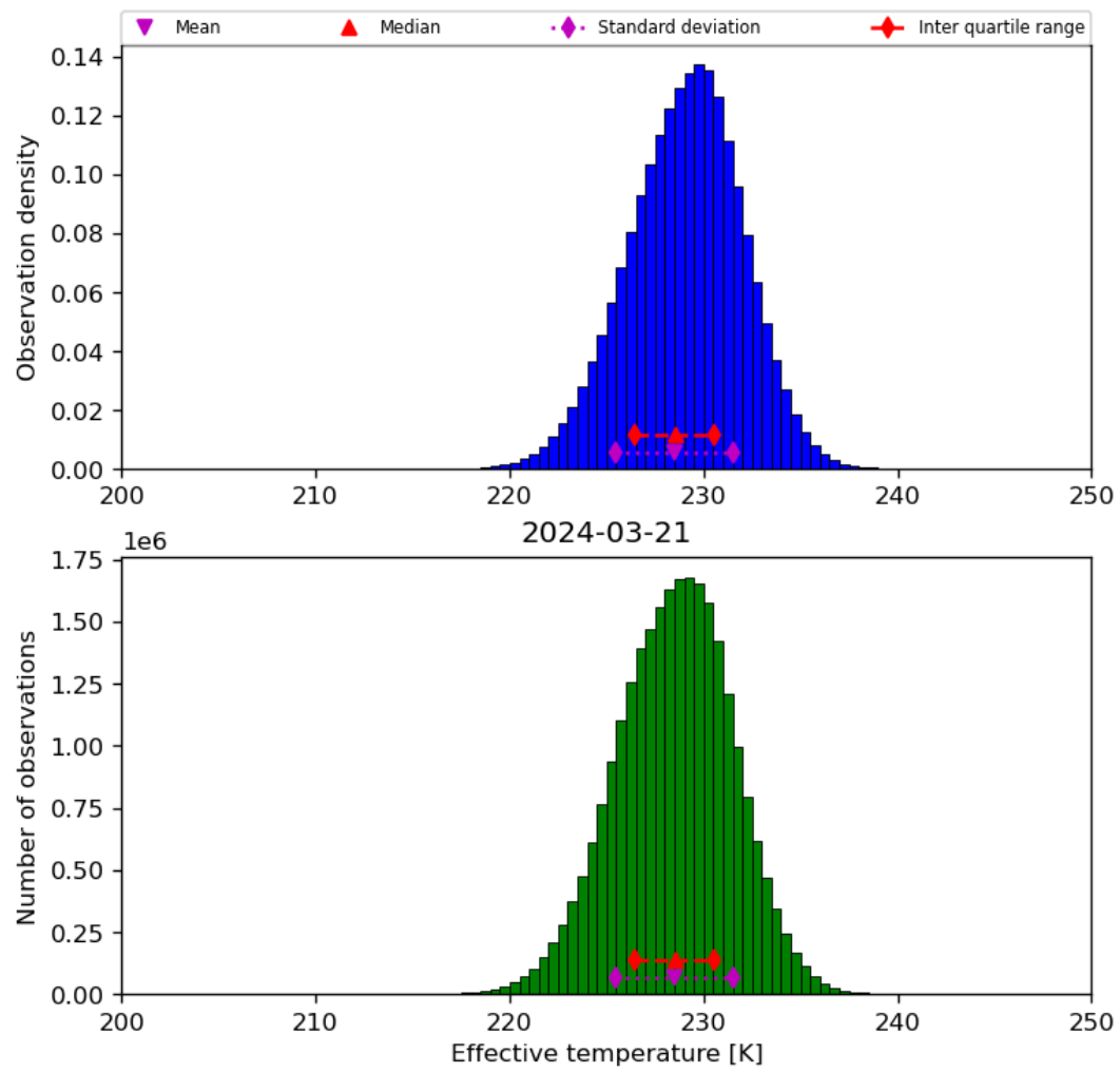
Figure 24: Histogram of “Effective temperature” for 2024-03-20 to 2024-03-22
