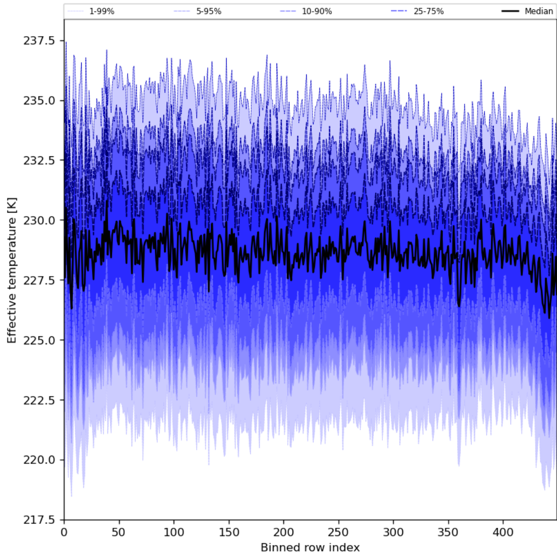
Figure 31: Along track statistics of “Effective temperature” for 2024-03-20 to 2024-03-22
