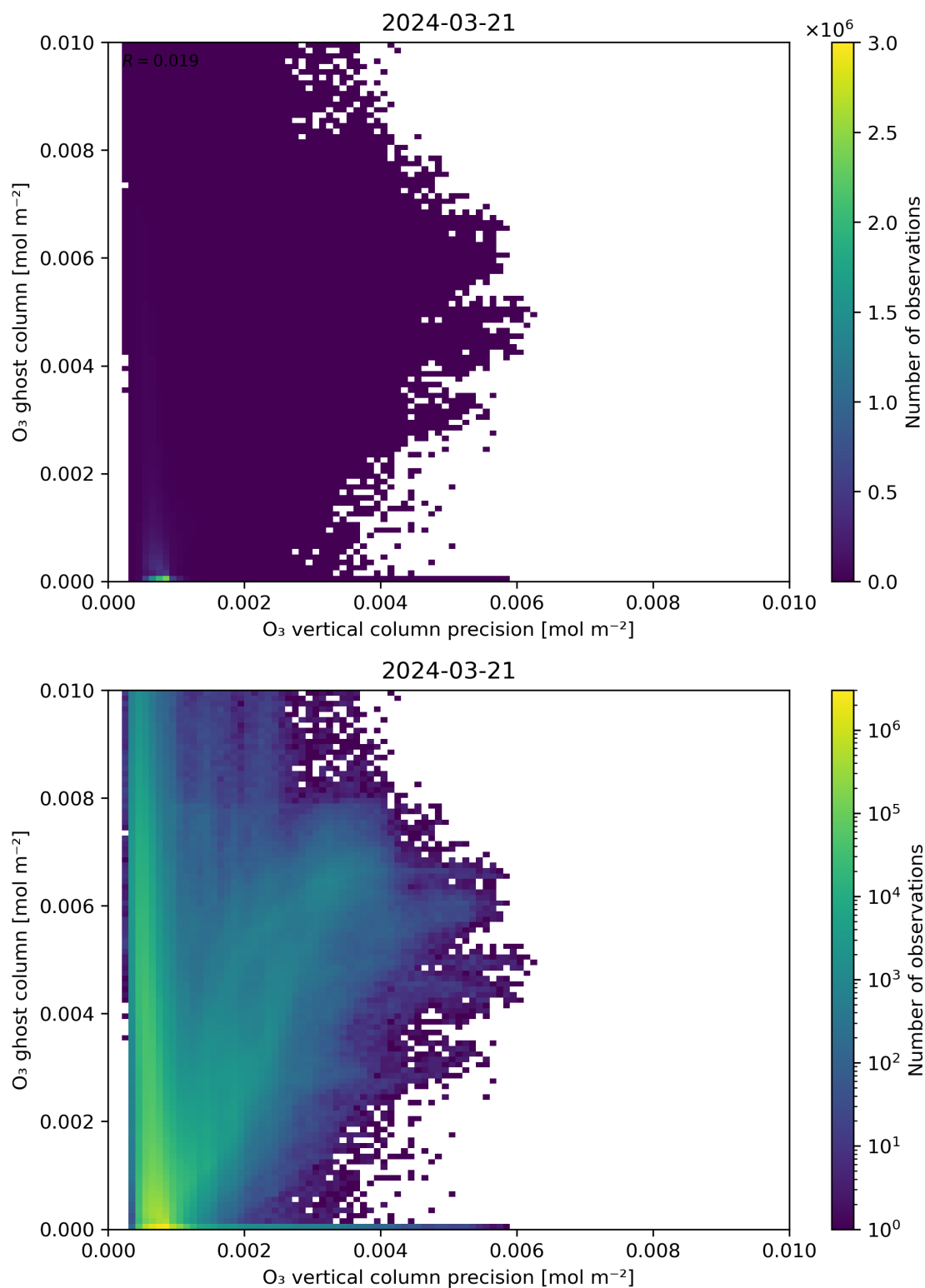
Figure 43: Scatter density plot of “ \text{O}_3 vertical column precision” against “ \text{O}_3 ghost column” for 2024-03-20 to 2024-03-22.
