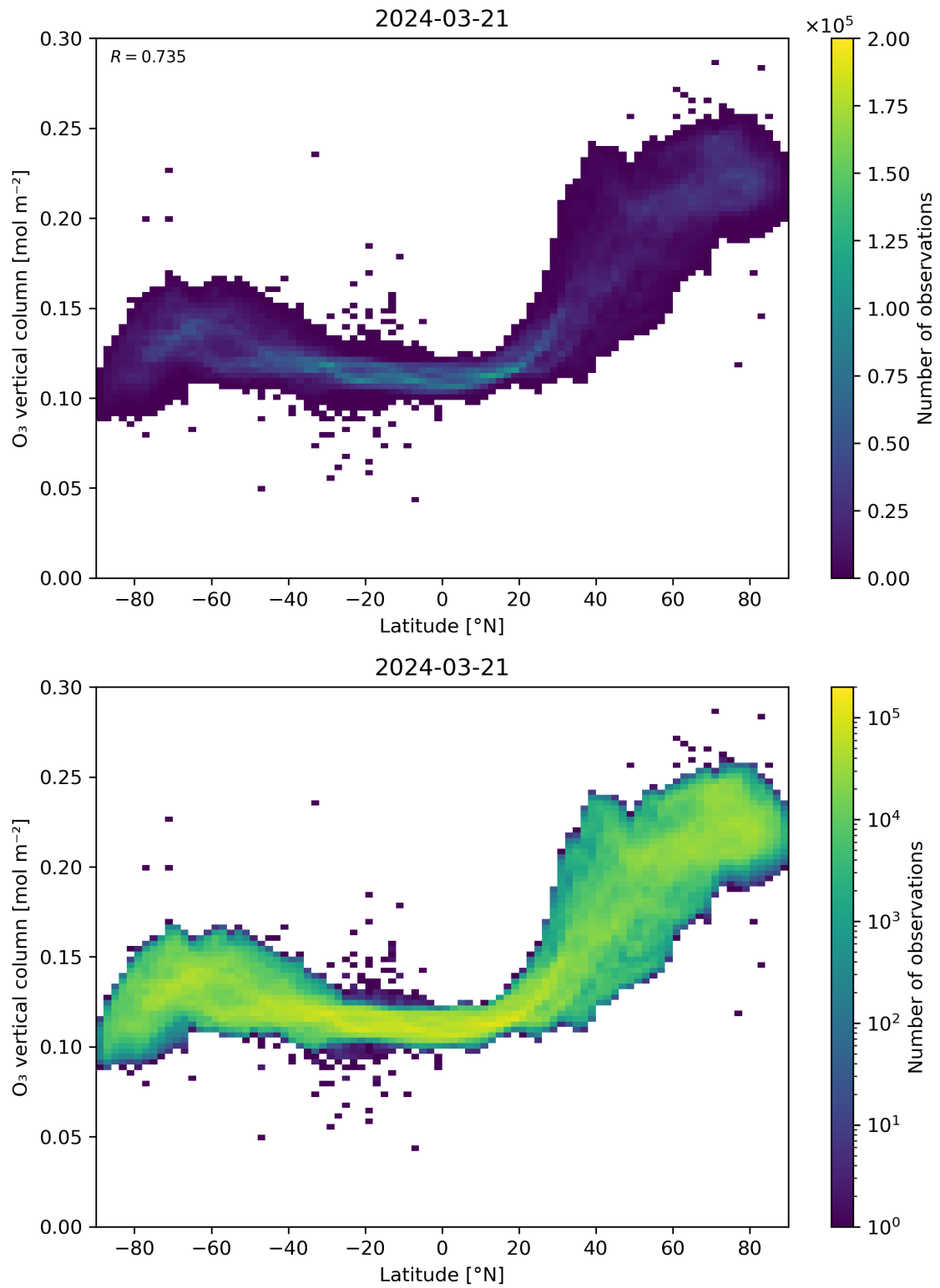
Figure 36: Scatter density plot of “Latitude” against “O 3 vertical column” for 2024-03-20 to 2024-03-22.
