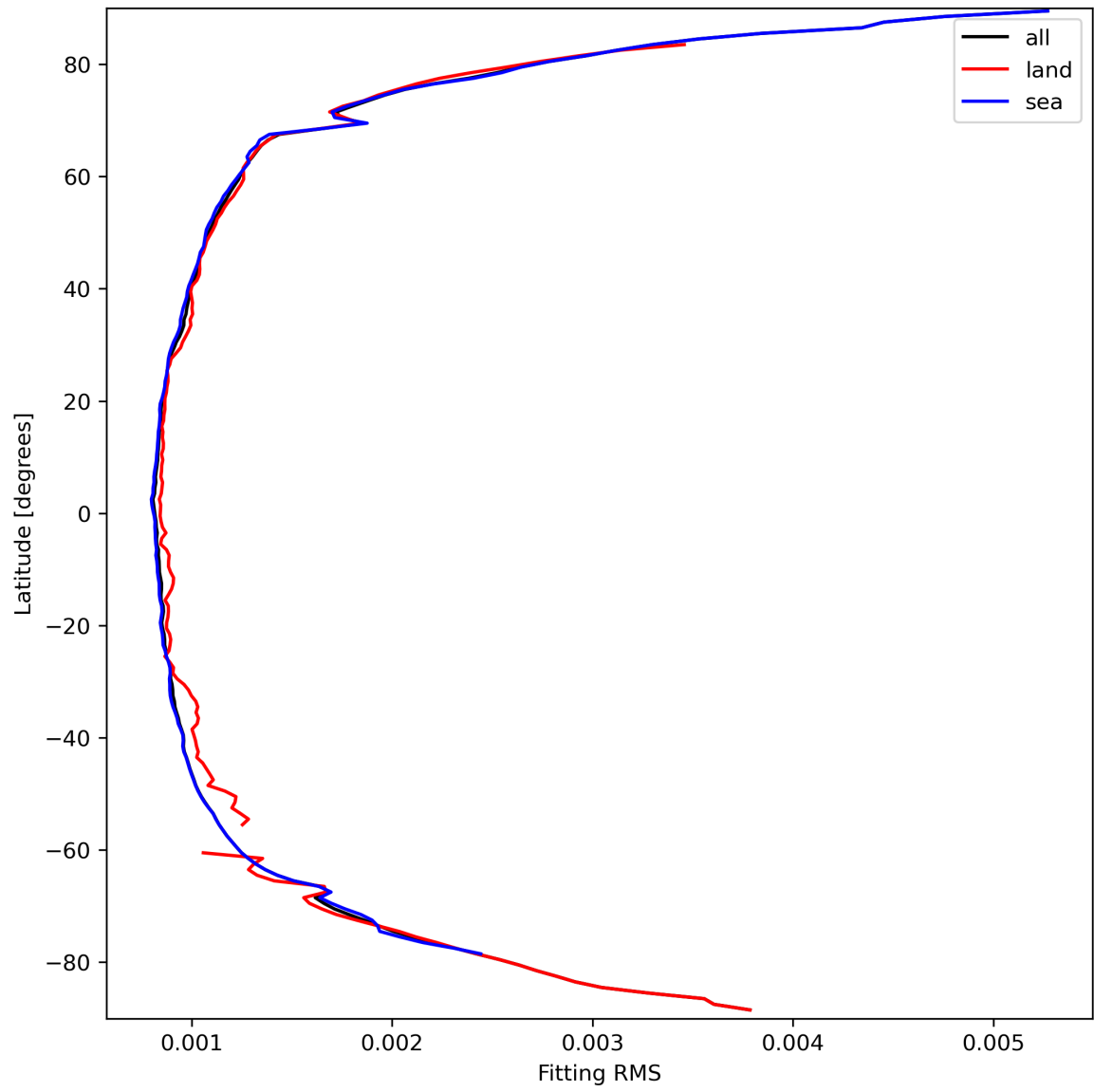
Figure 16: Zonal average of “Fitting RMS” for 2024-03-20 to 2024-03-22.
