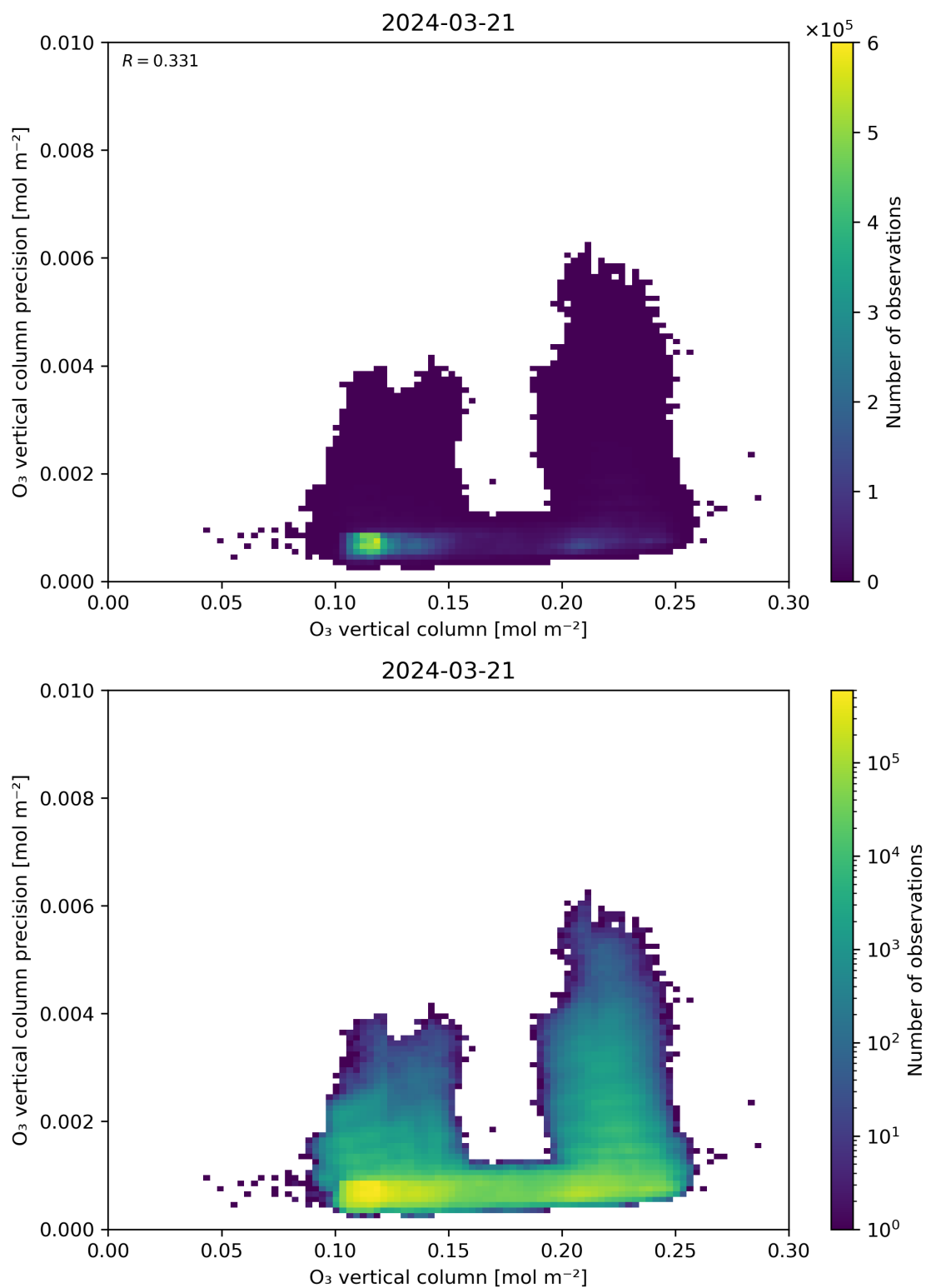
Figure 41: Scatter density plot of “O 3 vertical column” against “O 3 vertical column precision” for 2024-03-20 to 2024-03-22.
