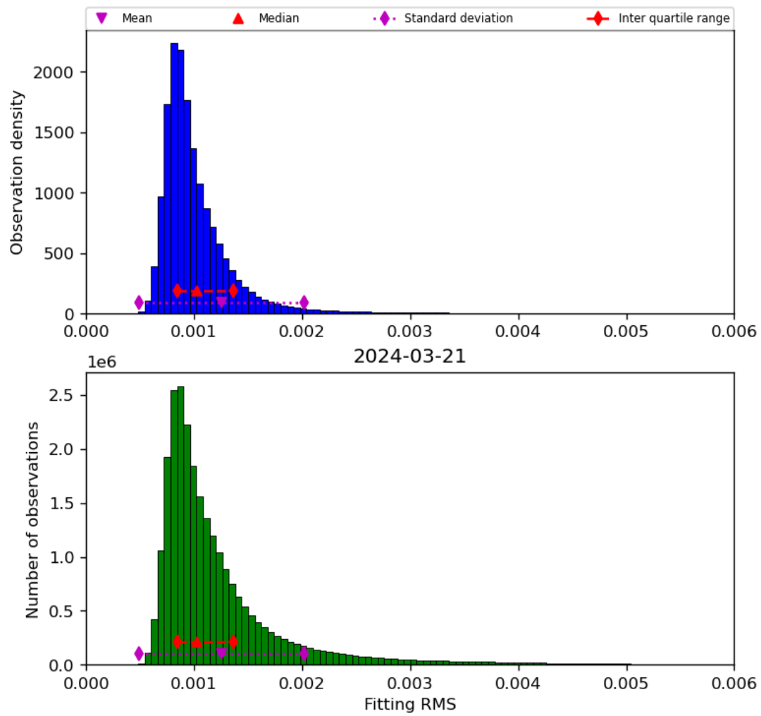
Figure 23: Histogram of “Fitting RMS” for 2024-03-20 to 2024-03-22
