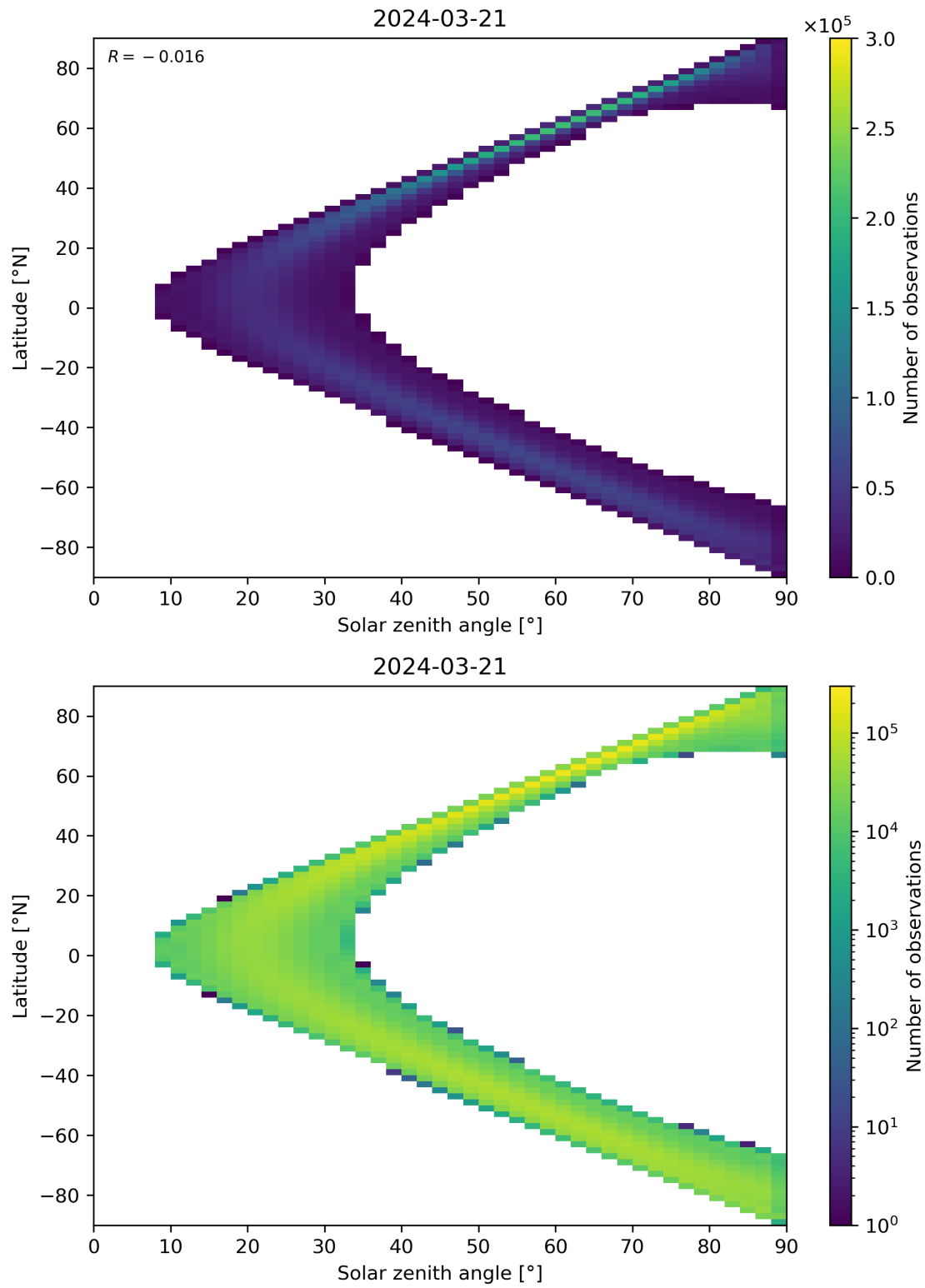
Figure 44: Scatter density plot of “Solar zenith angle” against “Latitude” for 2024-03-20 to 2024-03-22.
