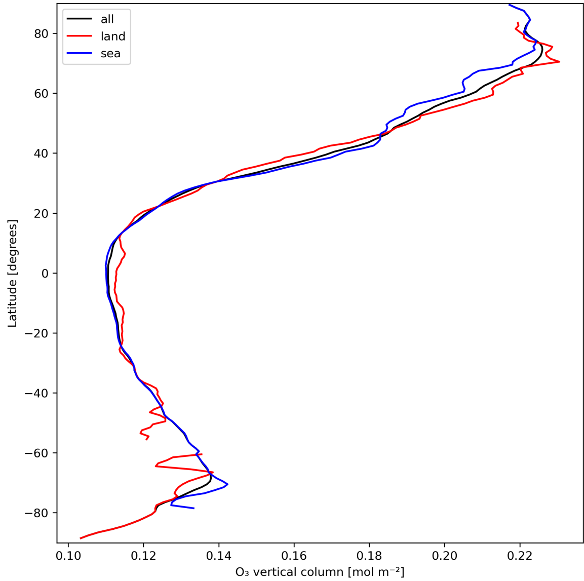
Figure 14: Zonal average of “O 3 vertical column” for 2024-03-20 to 2024-03-22.
