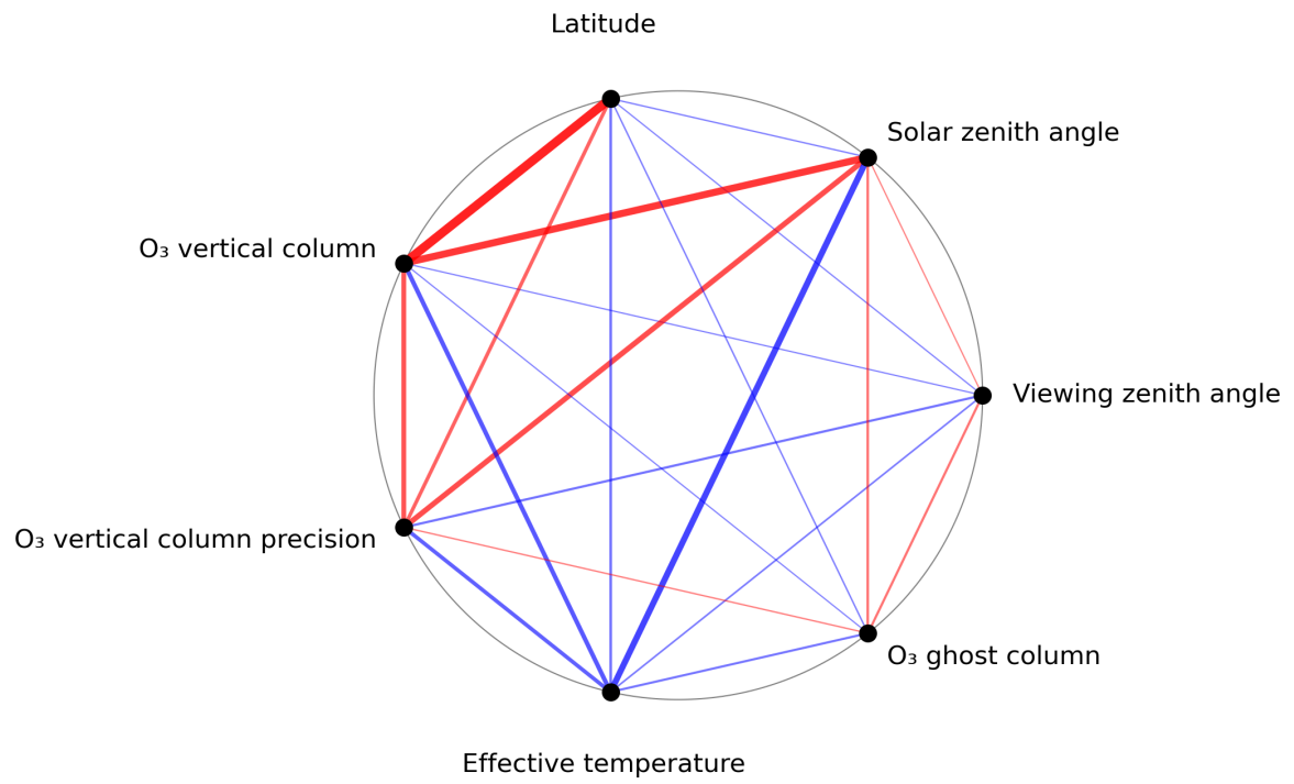
Figure 1: Map of correlation graph for 2024-03-20 to 2024-03-22.
