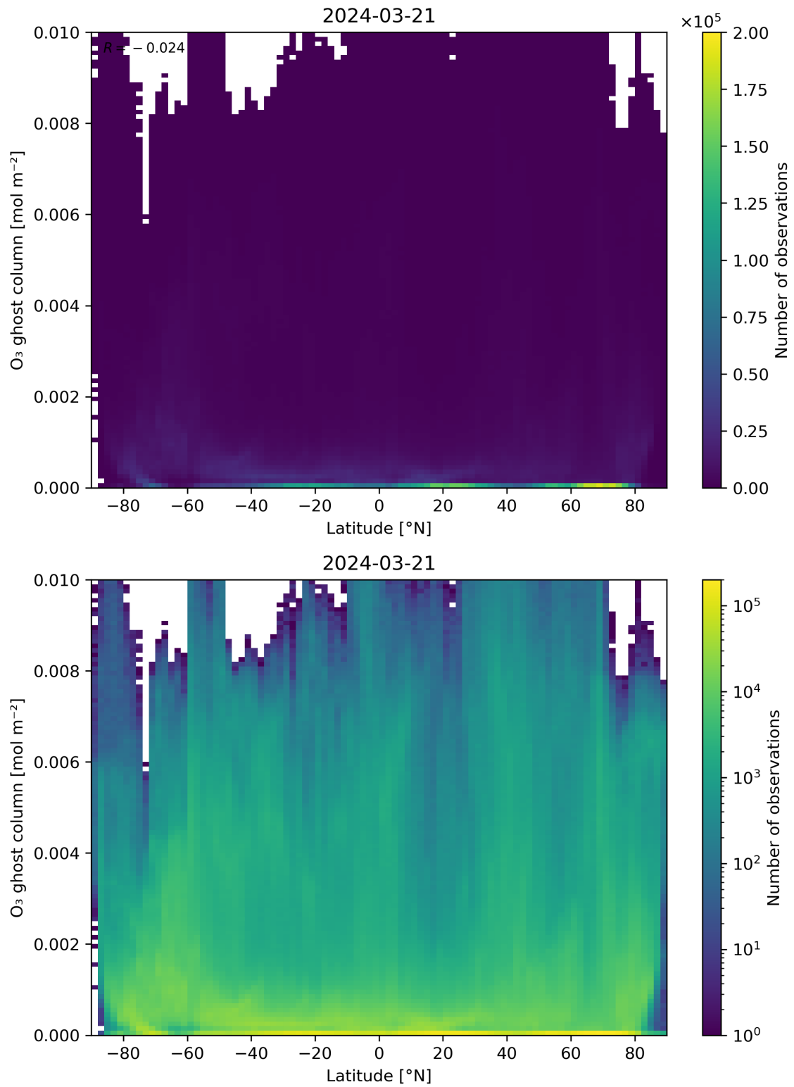
Figure 35: Scatter density plot of “Latitude” against “O 3 ghost column” for 2024-03-20 to 2024-03-22.
