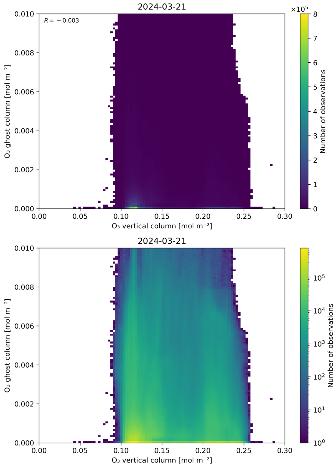
Figure 40: Scatter density plot of “O 3 vertical column” against “O 3 ghost column” for 2024-03-20 to 2024-03-22.
