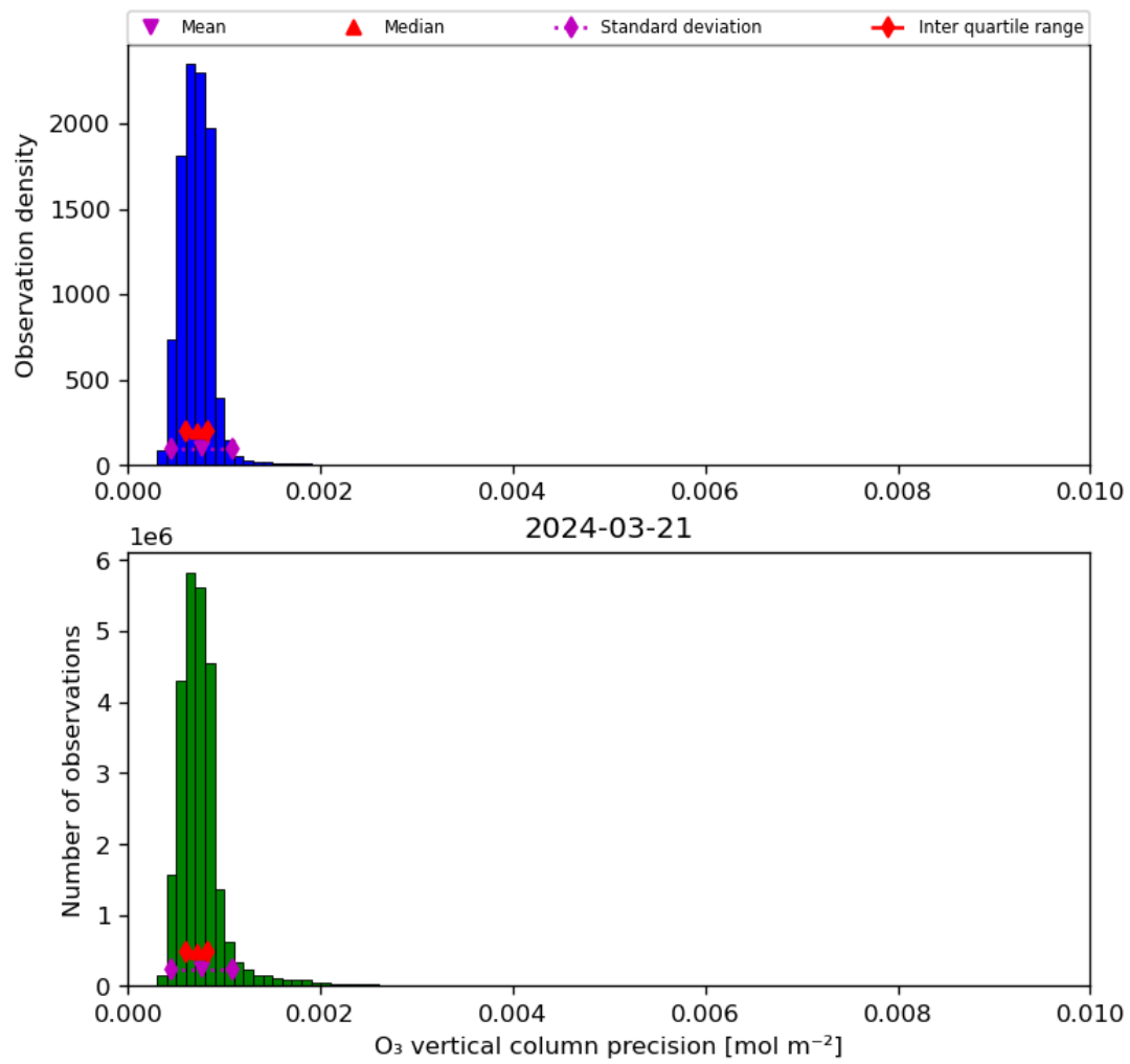
Figure 22: Histogram of “O 3 vertical column precision” for 2024-03-20 to 2024-03-22
