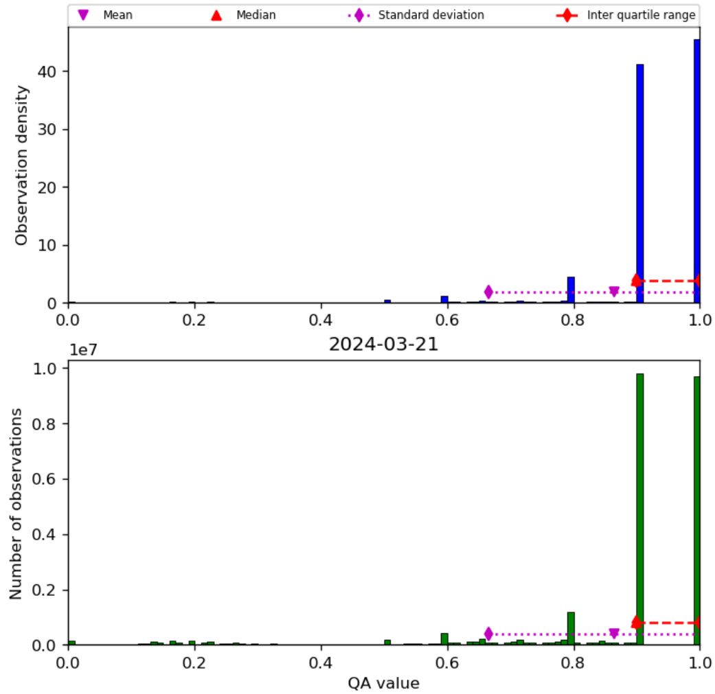
Figure 20: Histogram of “QA value” for 2024-03-20 to 2024-03-22
