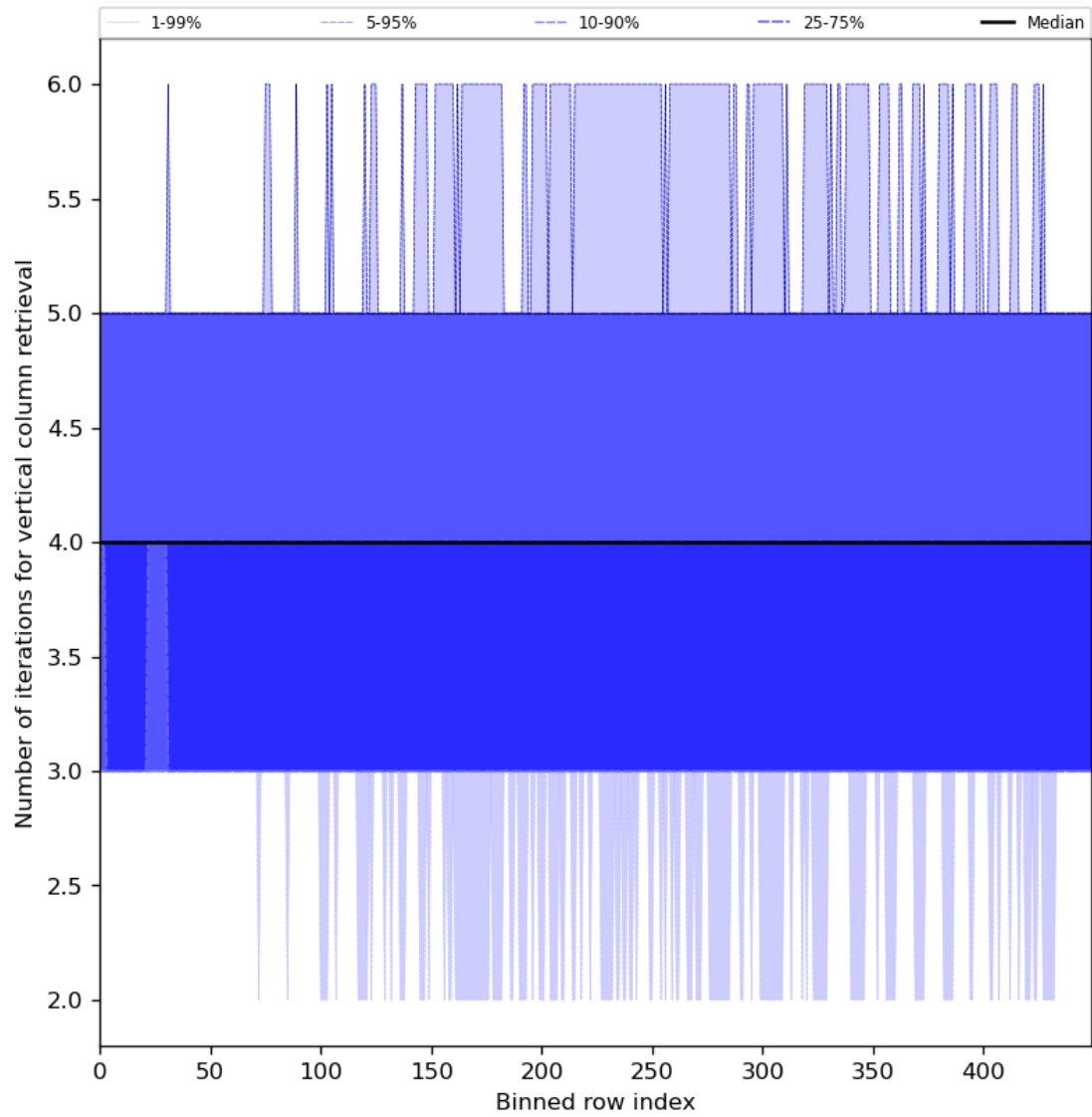
Figure 33: Along track statistics of “Number of iterations for vertical column retrieval” for 2024-03-20 to 2024-03-22
