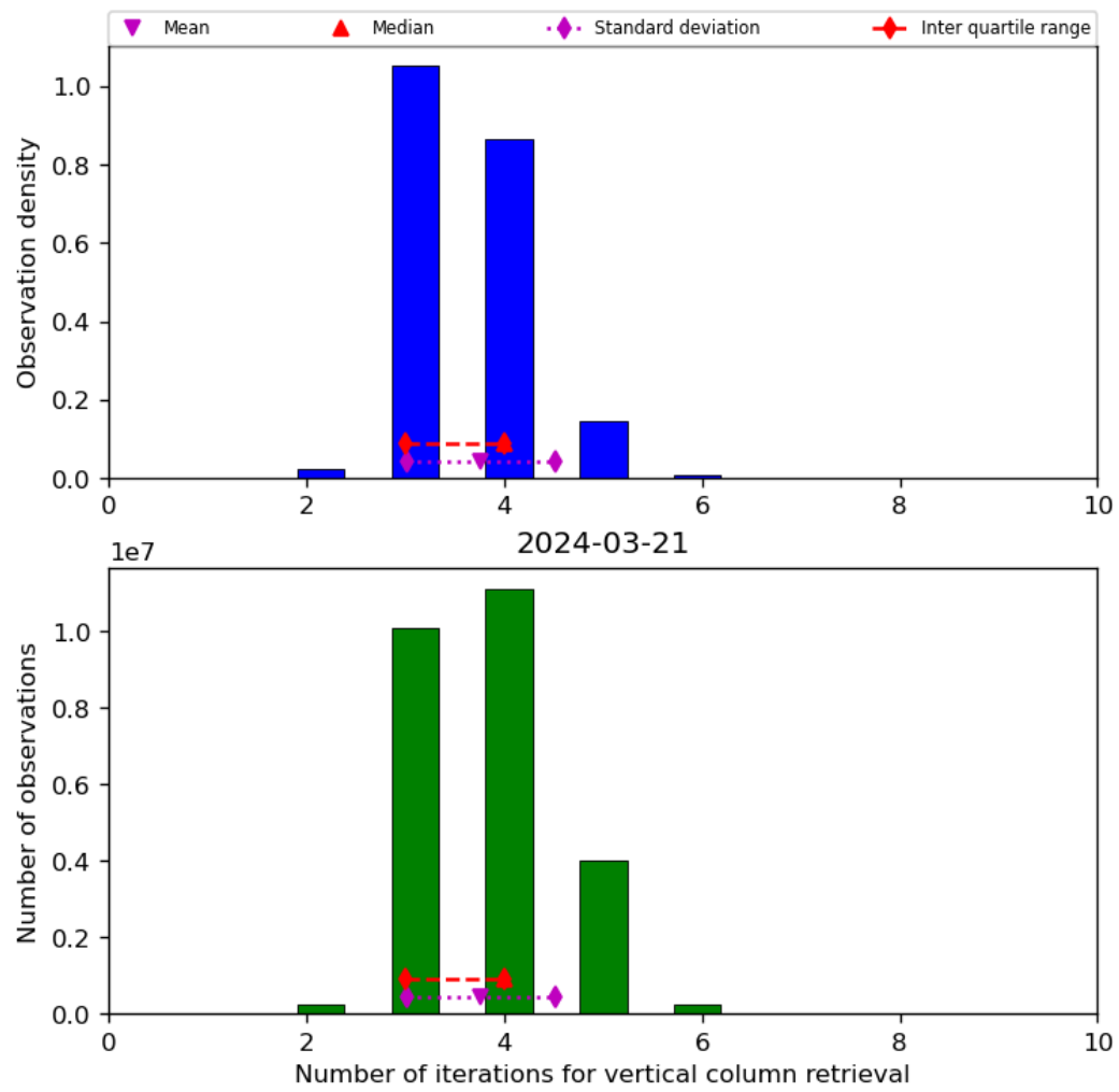
Figure 26: Histogram of “Number of iterations for vertical column retrieval” for 2024-03-20 to 2024-03-22
