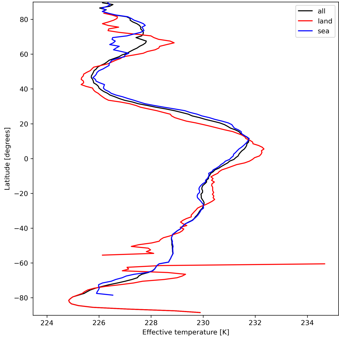
Figure 17: Zonal average of “Effective temperature” for 2024-03-20 to 2024-03-22.
