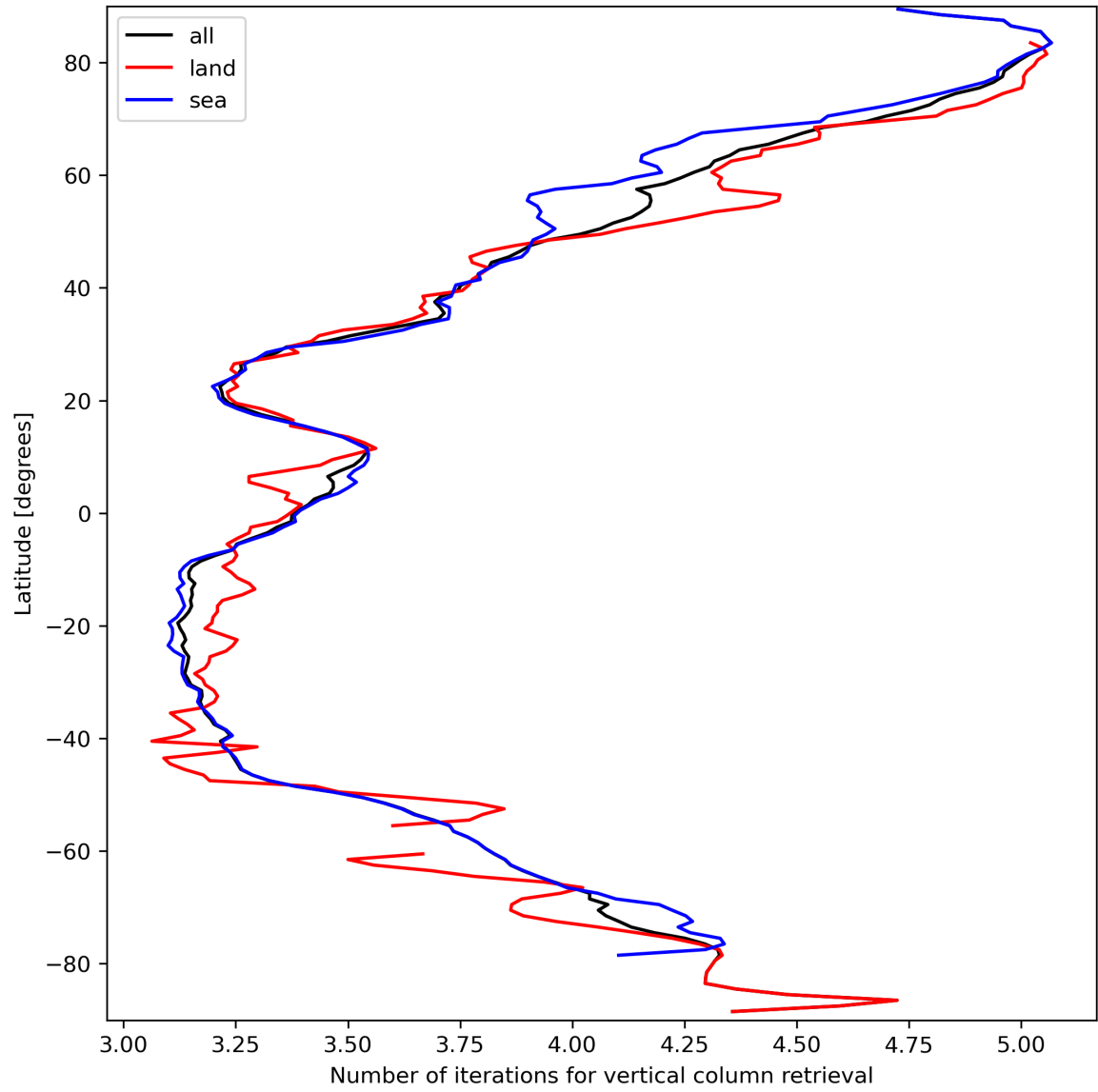
Figure 19: Zonal average of “Number of iterations for vertical column retrieval” for 2024-03-20 to 2024-03-22.
