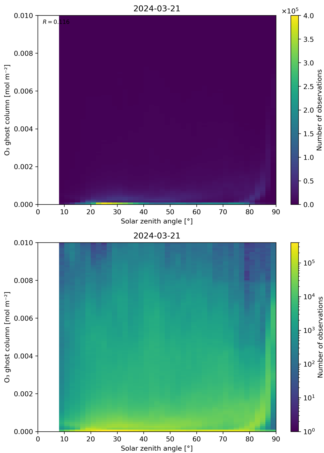
Figure 46: Scatter density plot of “Solar zenith angle” against “O 3 ghost column” for 2024-03-20 to 2024-03-22.
