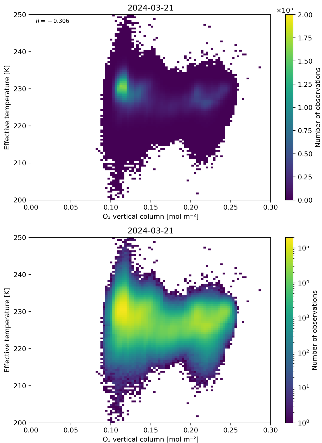
Figure 39: Scatter density plot of “O 3 vertical column” against “Effective temperature” for 2024-03-20 to 2024-03-22.
