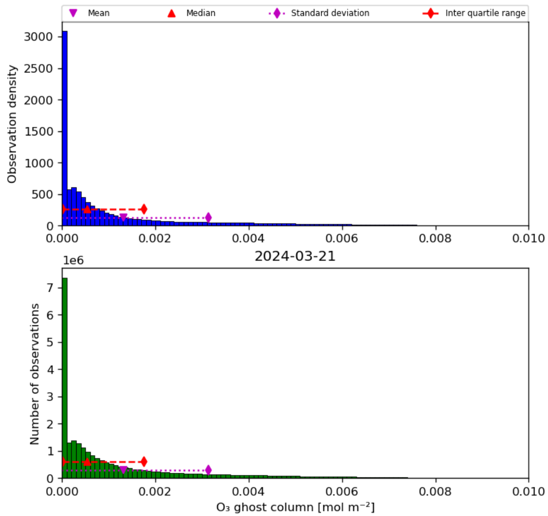
Figure 25: Histogram of “O 3 ghost column” for 2024-03-20 to 2024-03-22
