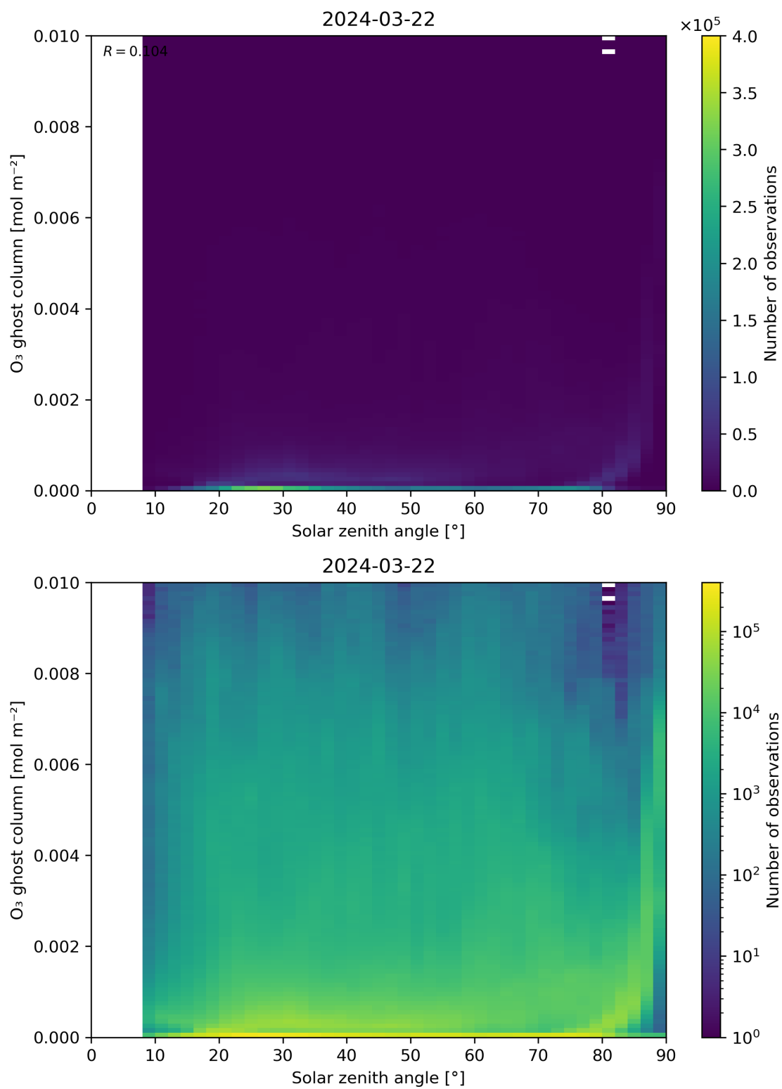
Figure 46: Scatter density plot of “Solar zenith angle” against “O 3 ghost column” for 2024-03-21 to 2024-03-22.
