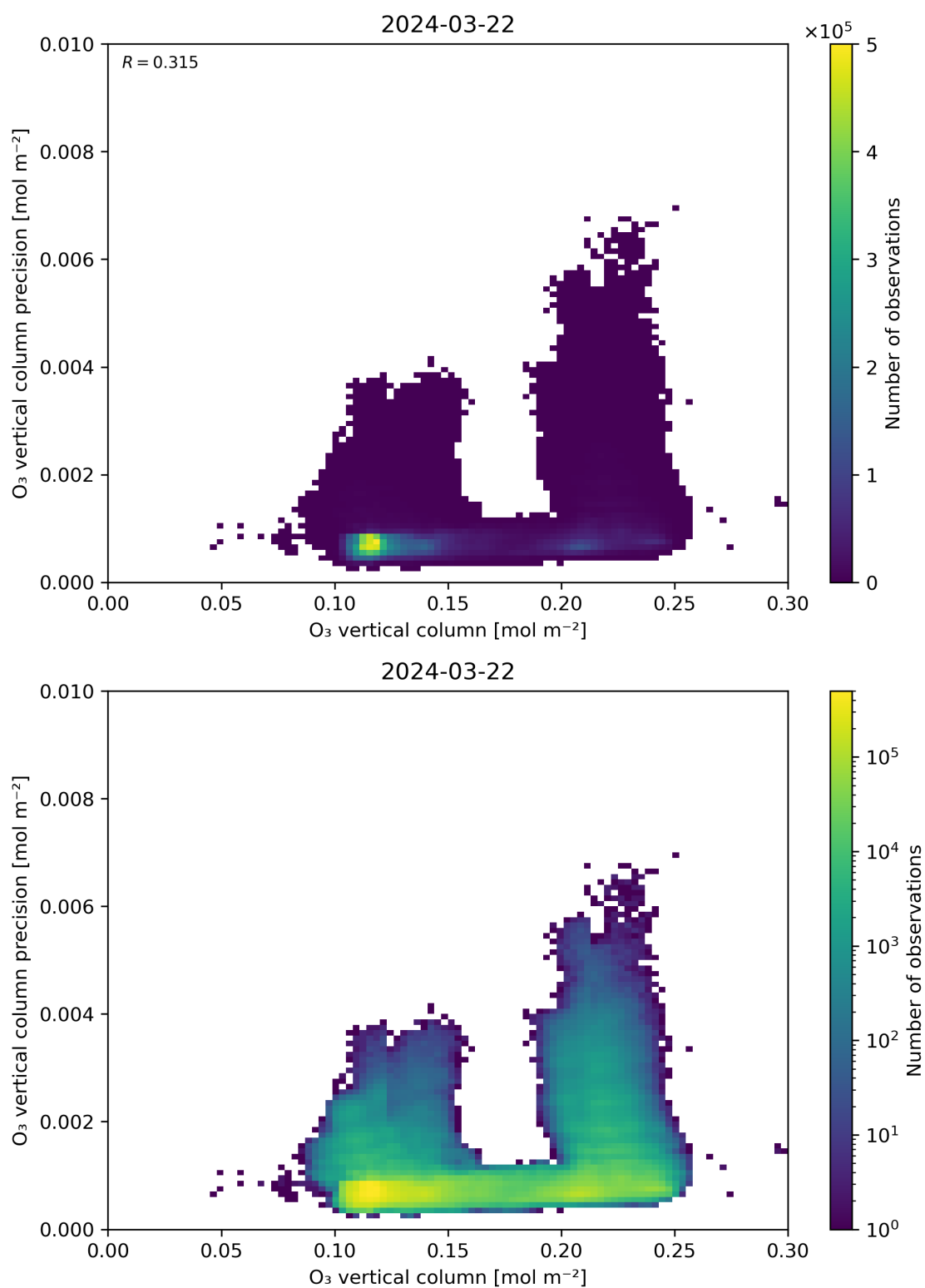
Figure 41: Scatter density plot of “O 3 vertical column” against “O 3 vertical column precision” for 2024-03-21 to 2024-03-22.
