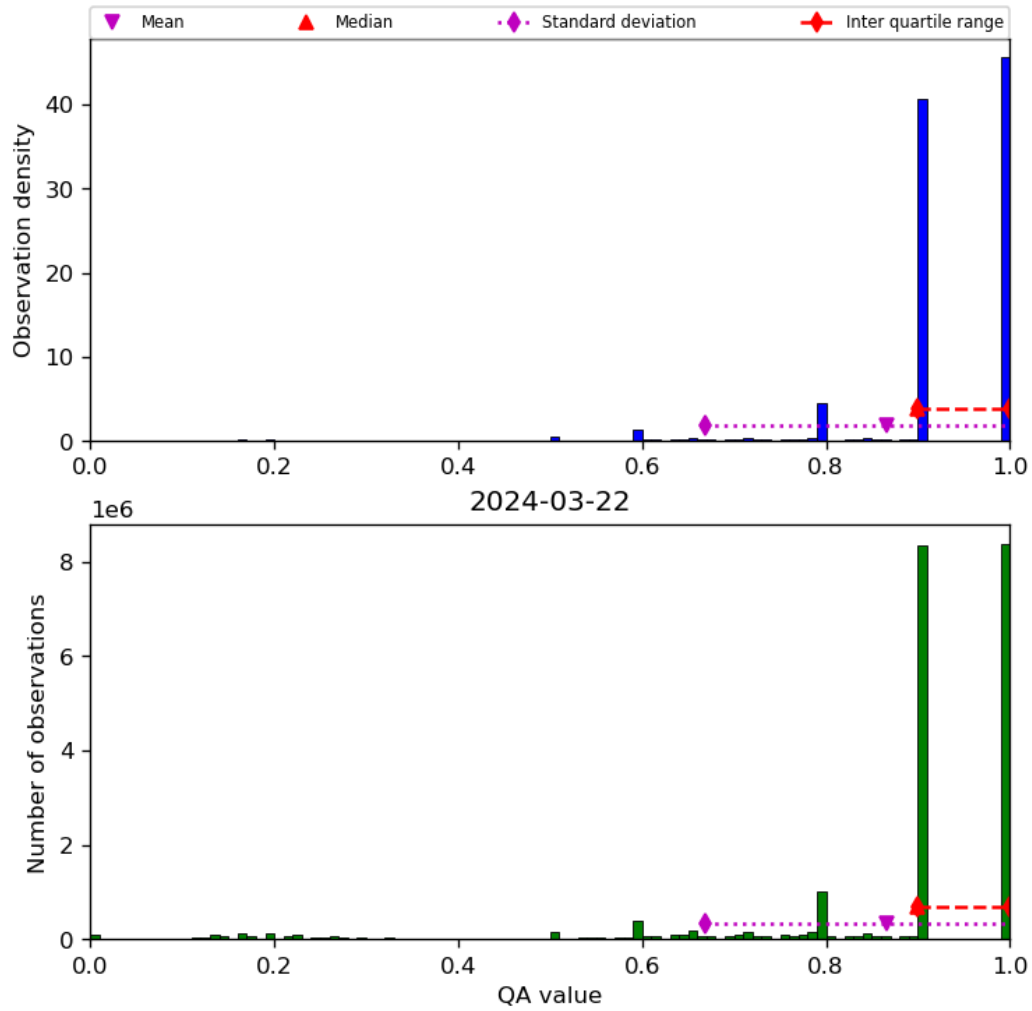
Figure 20: Histogram of “QA value” for 2024-03-21 to 2024-03-22
