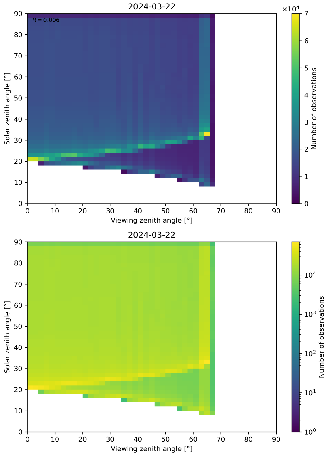
Figure 54: Scatter density plot of “Viewing zenith angle” against “Solar zenith angle” for 2024-03-21 to 2024-03-22.
