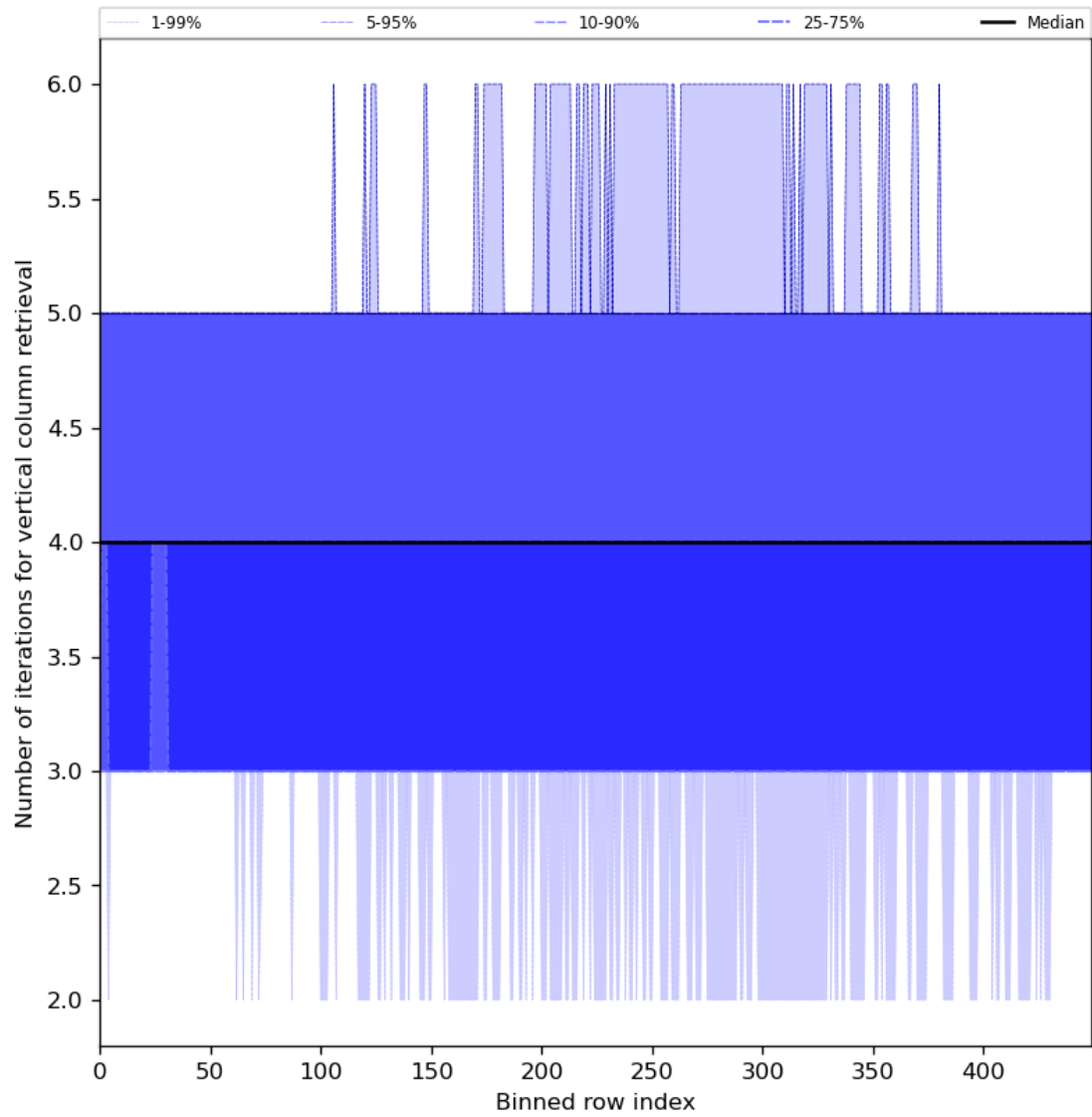
Figure 33: Along track statistics of “Number of iterations for vertical column retrieval” for 2024-03-21 to 2024-03-22
