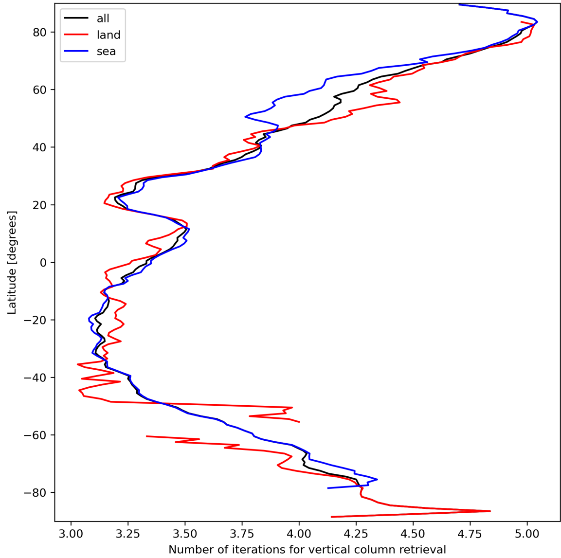
Figure 19: Zonal average of “Number of iterations for vertical column retrieval” for 2024-03-21 to 2024-03-22.
