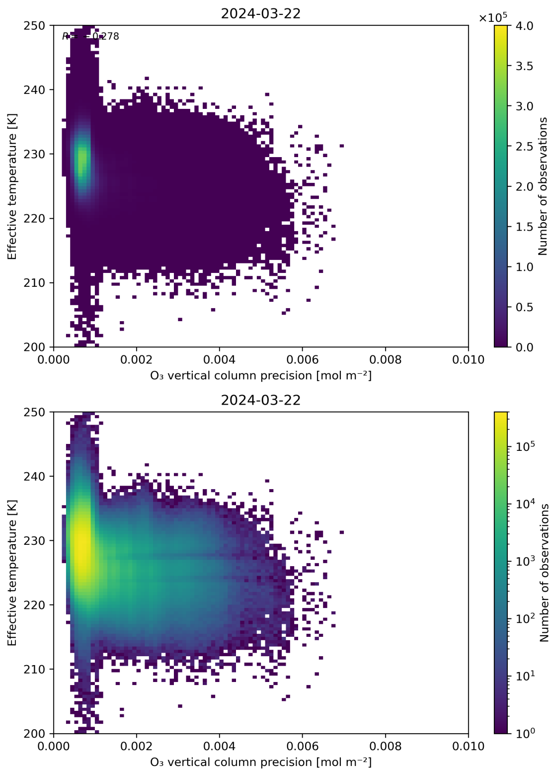
Figure 42: Scatter density plot of “O 3 vertical column precision” against “Effective temperature” for 2024-03-21 to 2024-03-22.
