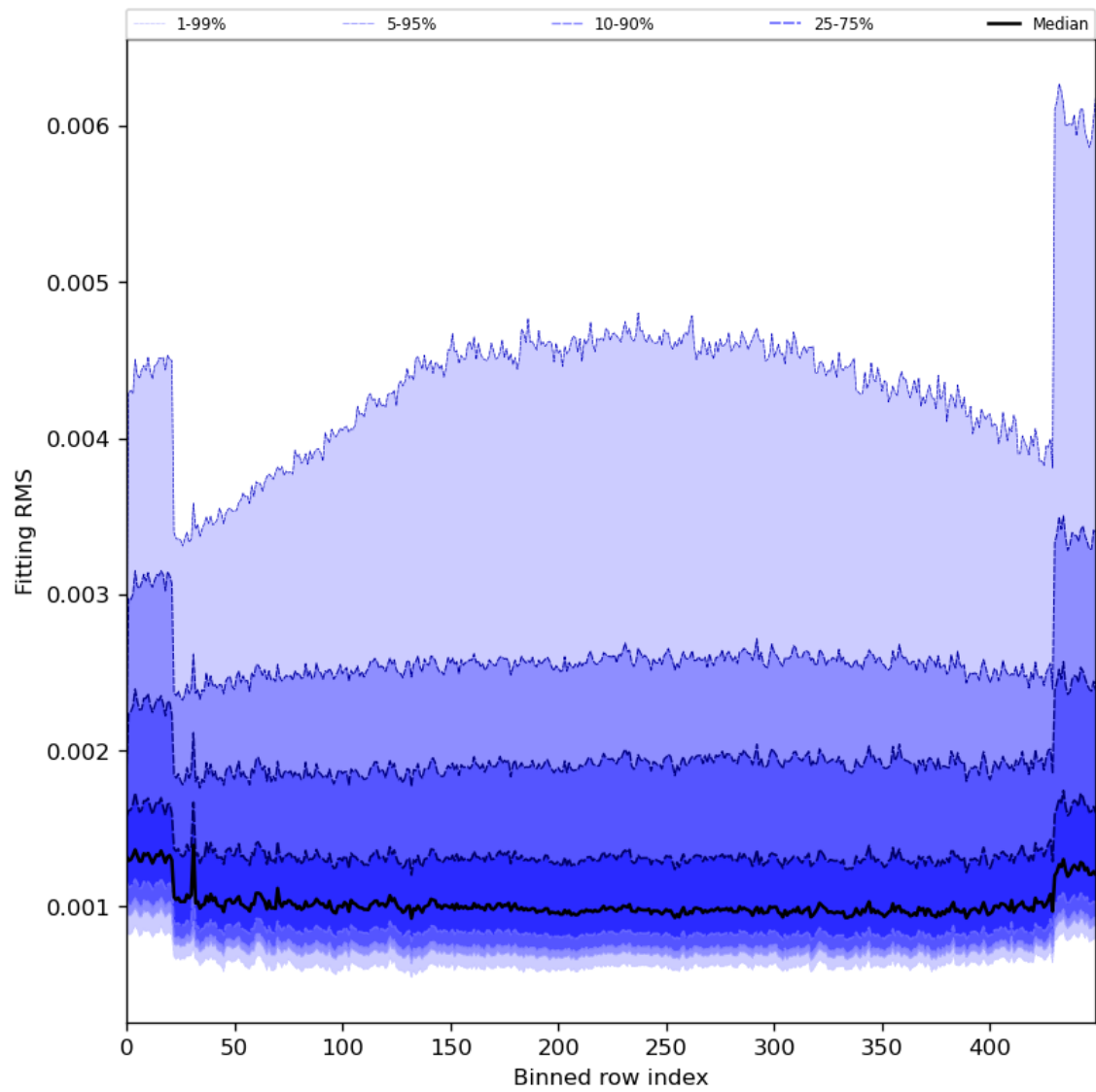
Figure 30: Along track statistics of “Fitting RMS” for 2024-03-21 to 2024-03-22
