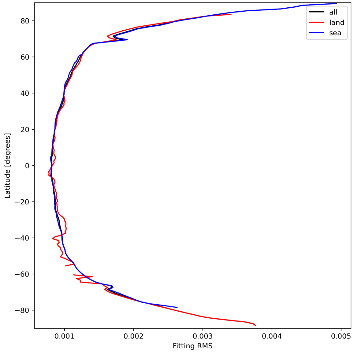
Figure 16: Zonal average of “Fitting RMS” for 2024-03-21 to 2024-03-22.
