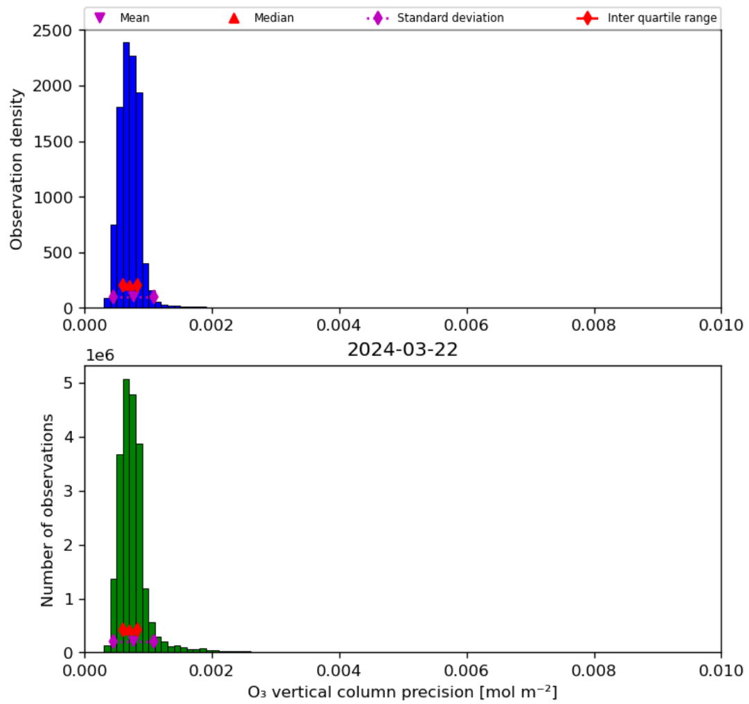
Figure 22: Histogram of “O 3 vertical column precision” for 2024-03-21 to 2024-03-22
