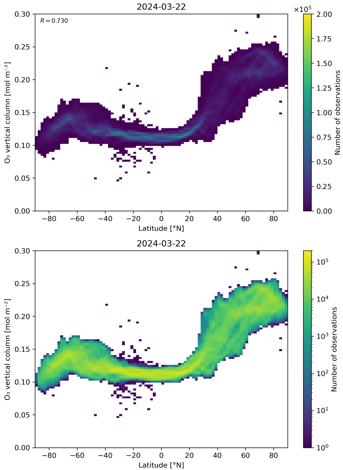
Figure 36: Scatter density plot of “Latitude” against “O 3 vertical column” for 2024-03-21 to 2024-03-22.
