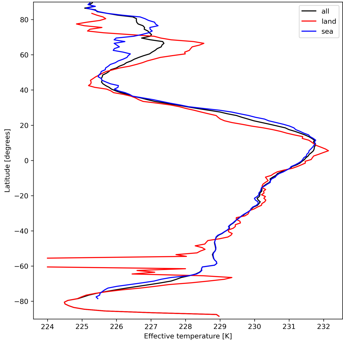
Figure 17: Zonal average of “Effective temperature” for 2024-03-21 to 2024-03-22.
