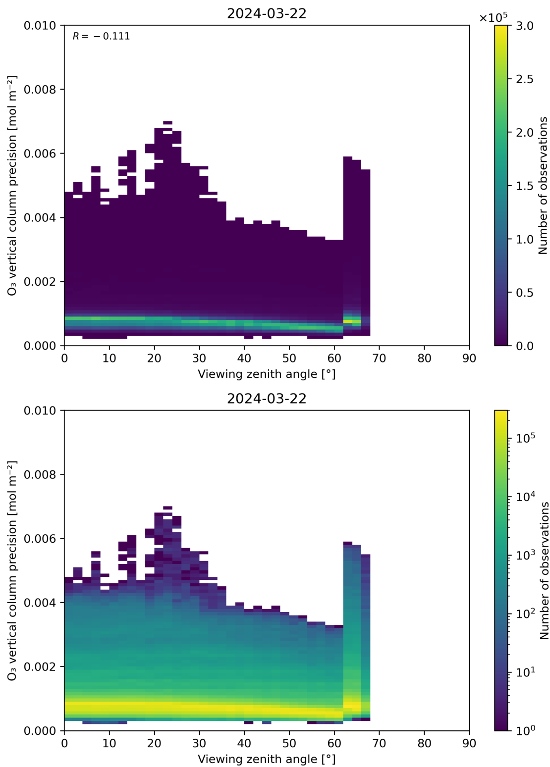
Figure 53: Scatter density plot of “Viewing zenith angle” against “O 3 vertical column precision” for 2024-03-21 to 2024-03-22.
