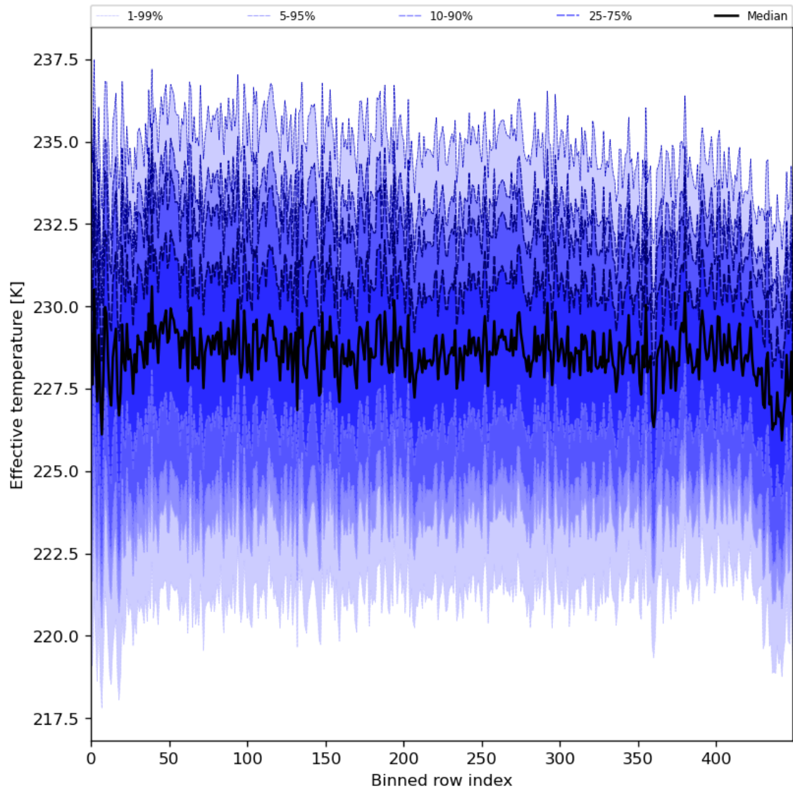
Figure 31: Along track statistics of “Effective temperature” for 2024-03-21 to 2024-03-22
