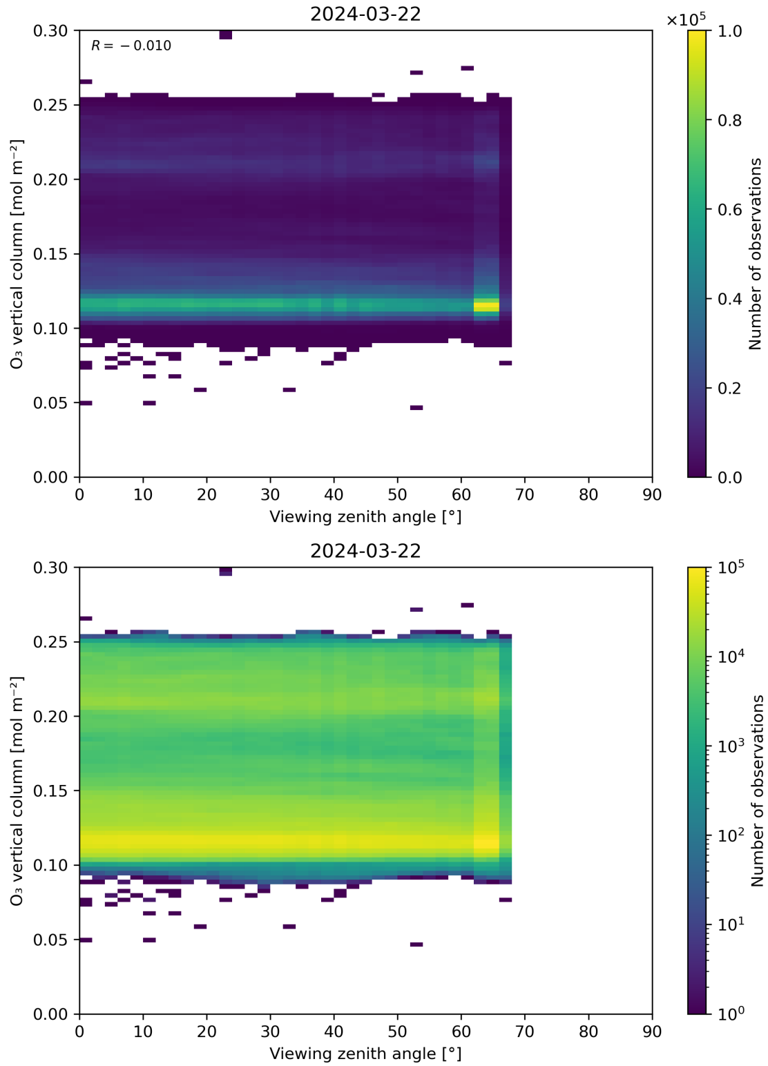
Figure 52: Scatter density plot of “Viewing zenith angle” against “O 3 vertical column” for 2024-03-21 to 2024-03-22.
