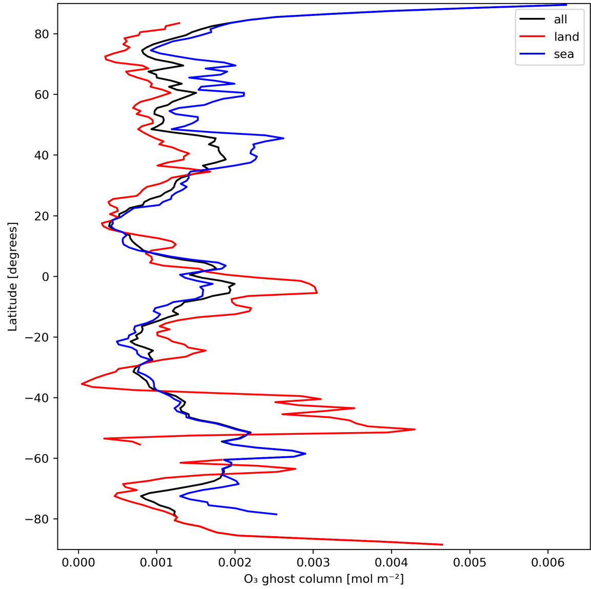
Figure 18: Zonal average of "O 3 ghost column" for 2024-03-21 to 2024-03-22.
