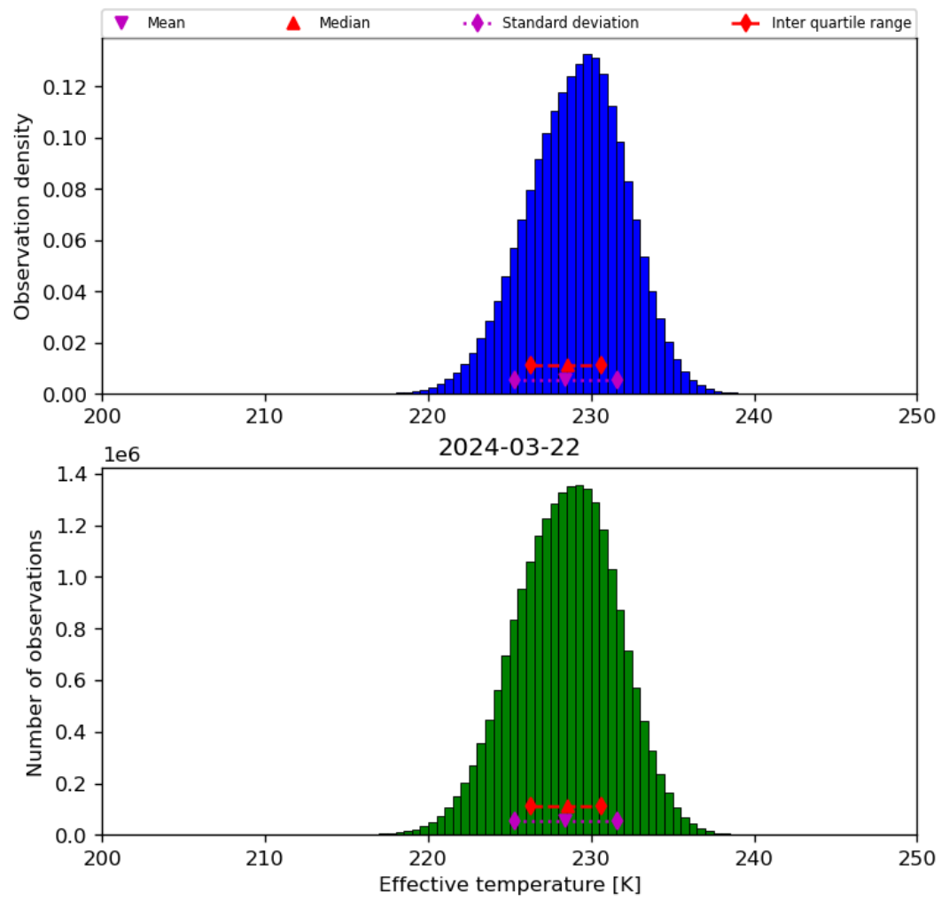
Figure 24: Histogram of “Effective temperature” for 2024-03-21 to 2024-03-22
