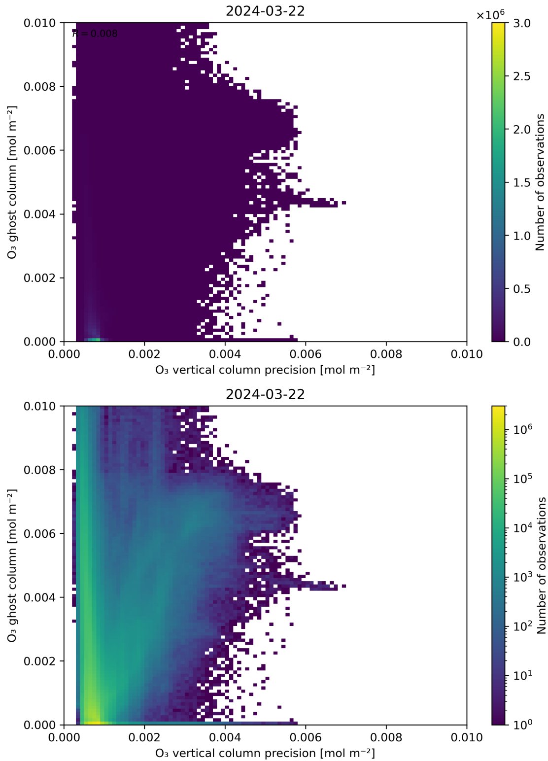
Figure 43: Scatter density plot of “ \text{O}_3 vertical column precision” against “ \text{O}_3 ghost column” for 2024-03-21 to 2024-03-22.
