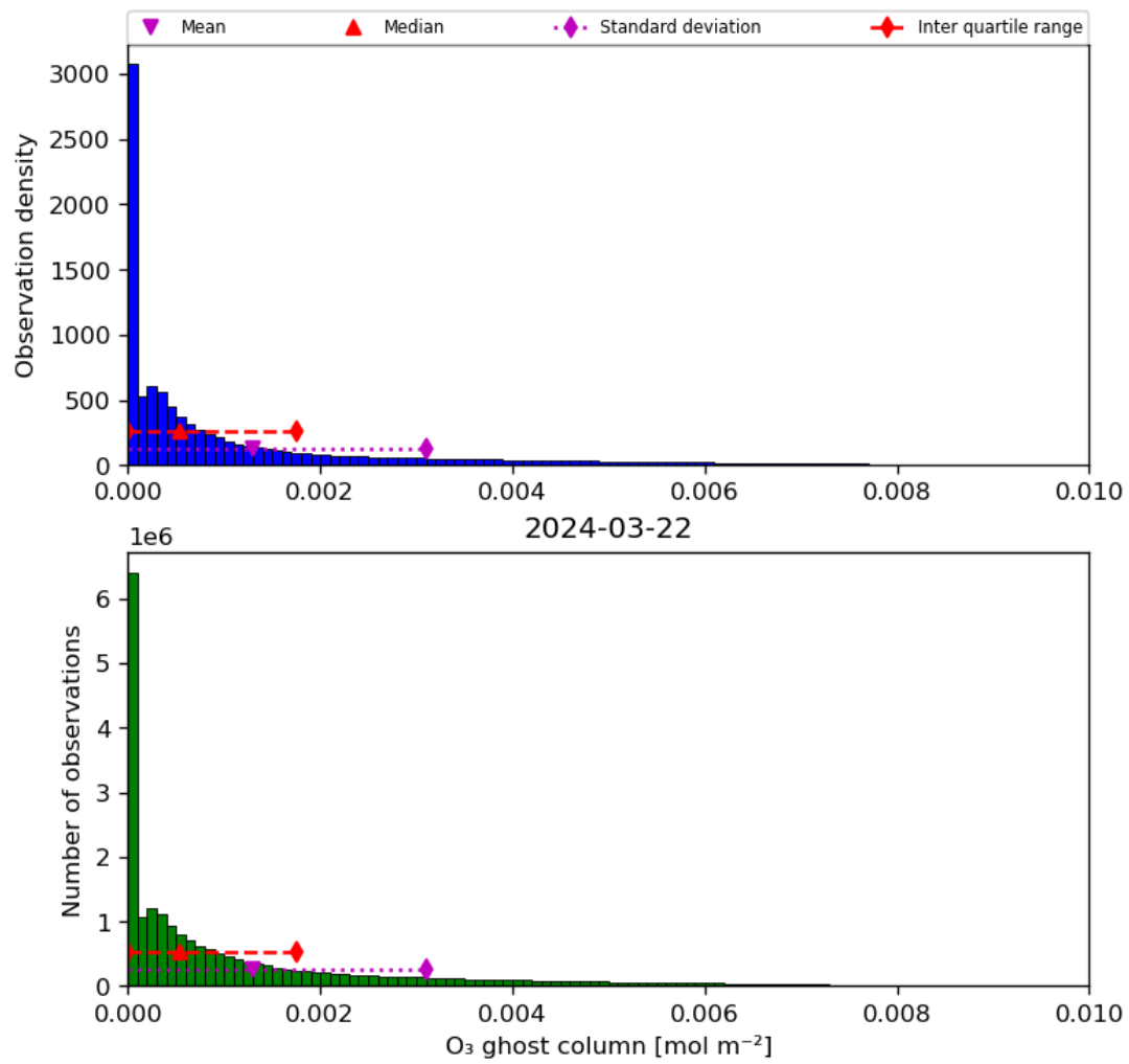
Figure 25: Histogram of "O 3 ghost column" for 2024-03-21 to 2024-03-22
