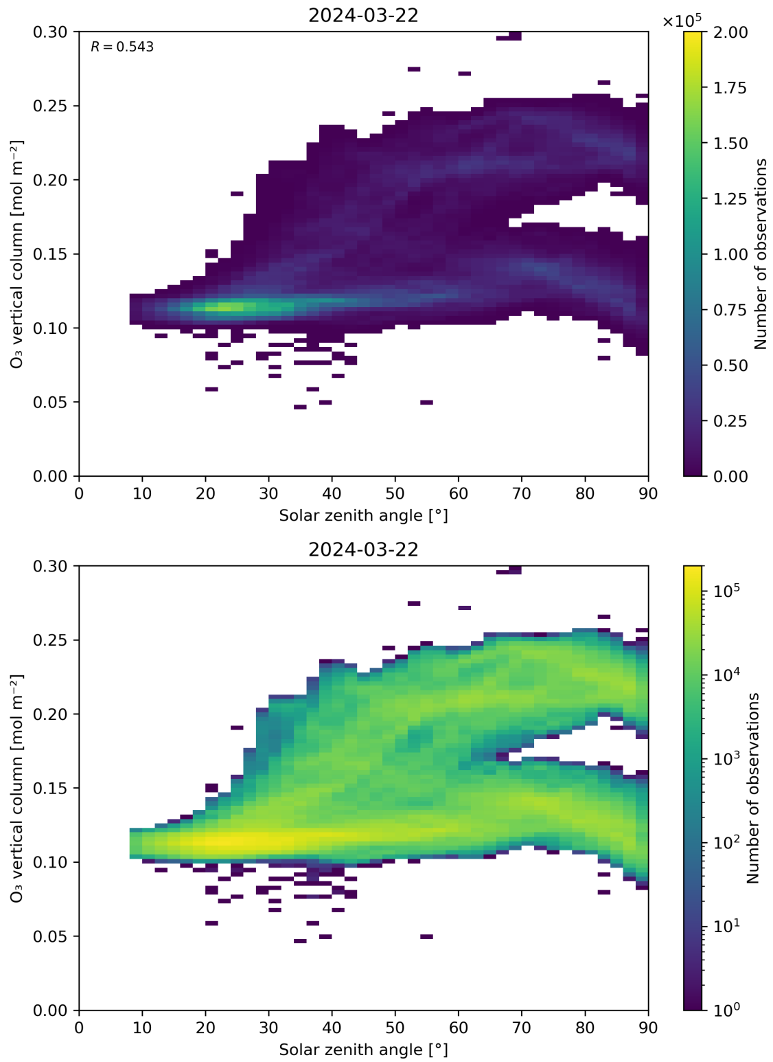
Figure 47: Scatter density plot of “Solar zenith angle” against “O 3 vertical column” for 2024-03-21 to 2024-03-22.
