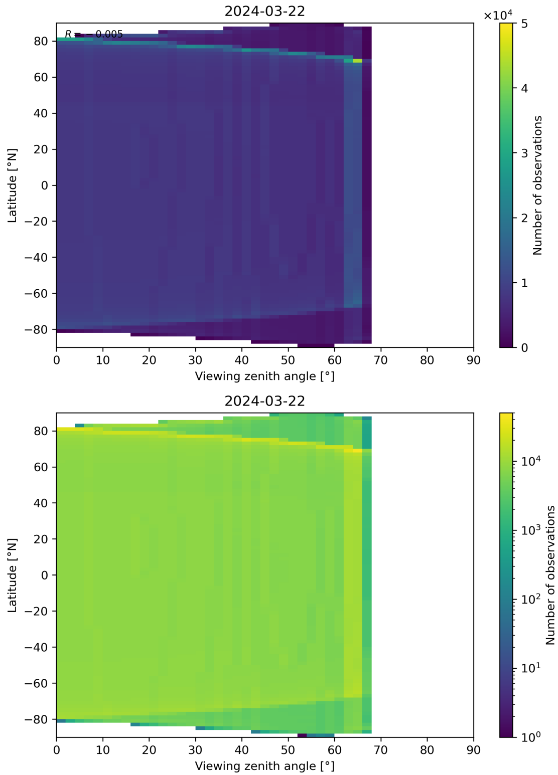
Figure 49: Scatter density plot of “Viewing zenith angle” against “Latitude” for 2024-03-21 to 2024-03-22.
