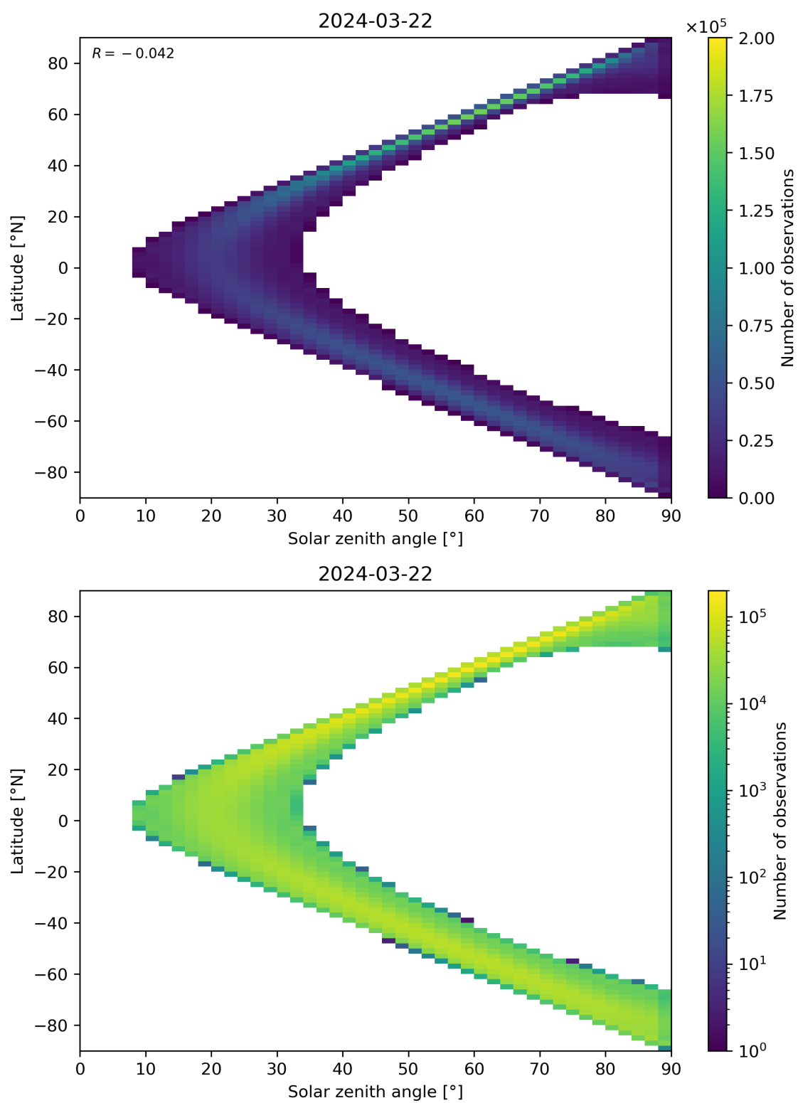
Figure 44: Scatter density plot of “Solar zenith angle” against “Latitude” for 2024-03-21 to 2024-03-22.
