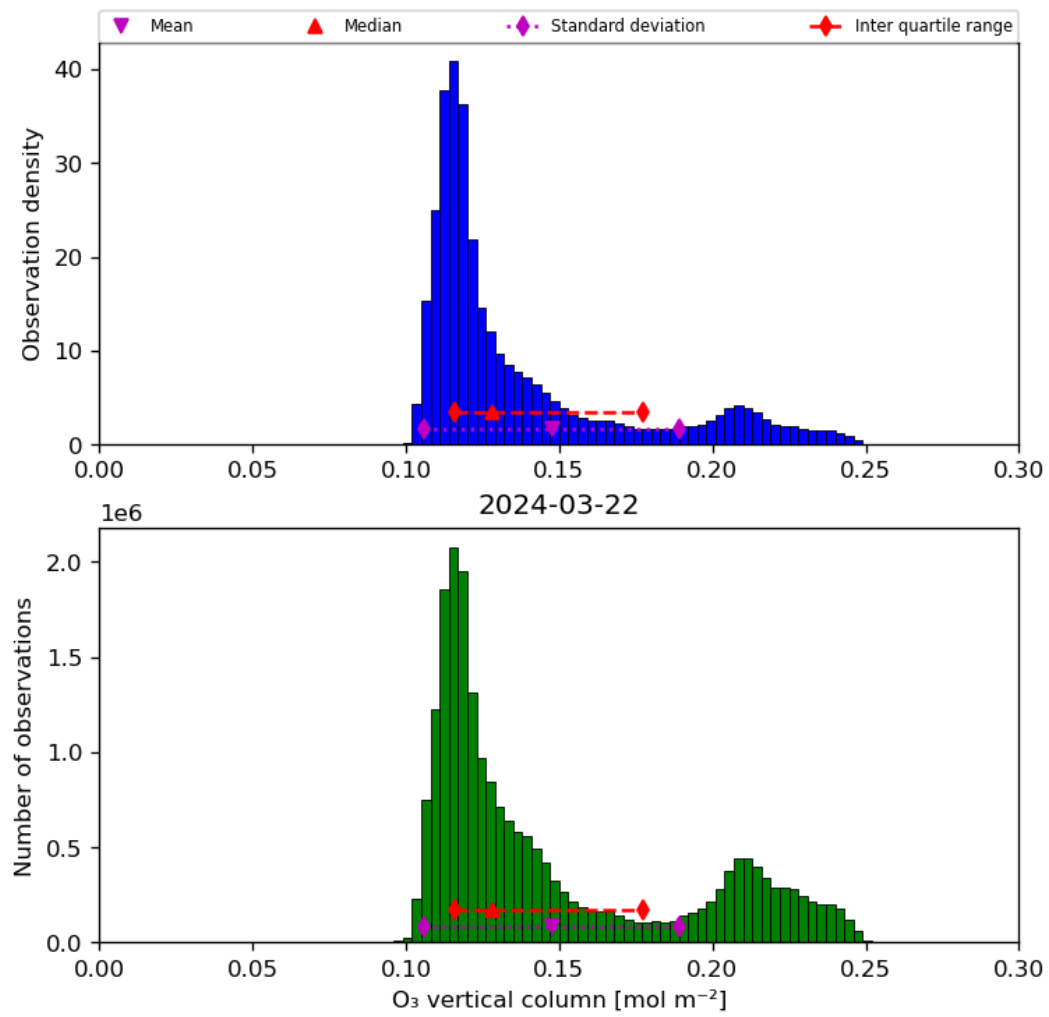
Figure 21: Histogram of “O 3 vertical column” for 2024-03-21 to 2024-03-22
