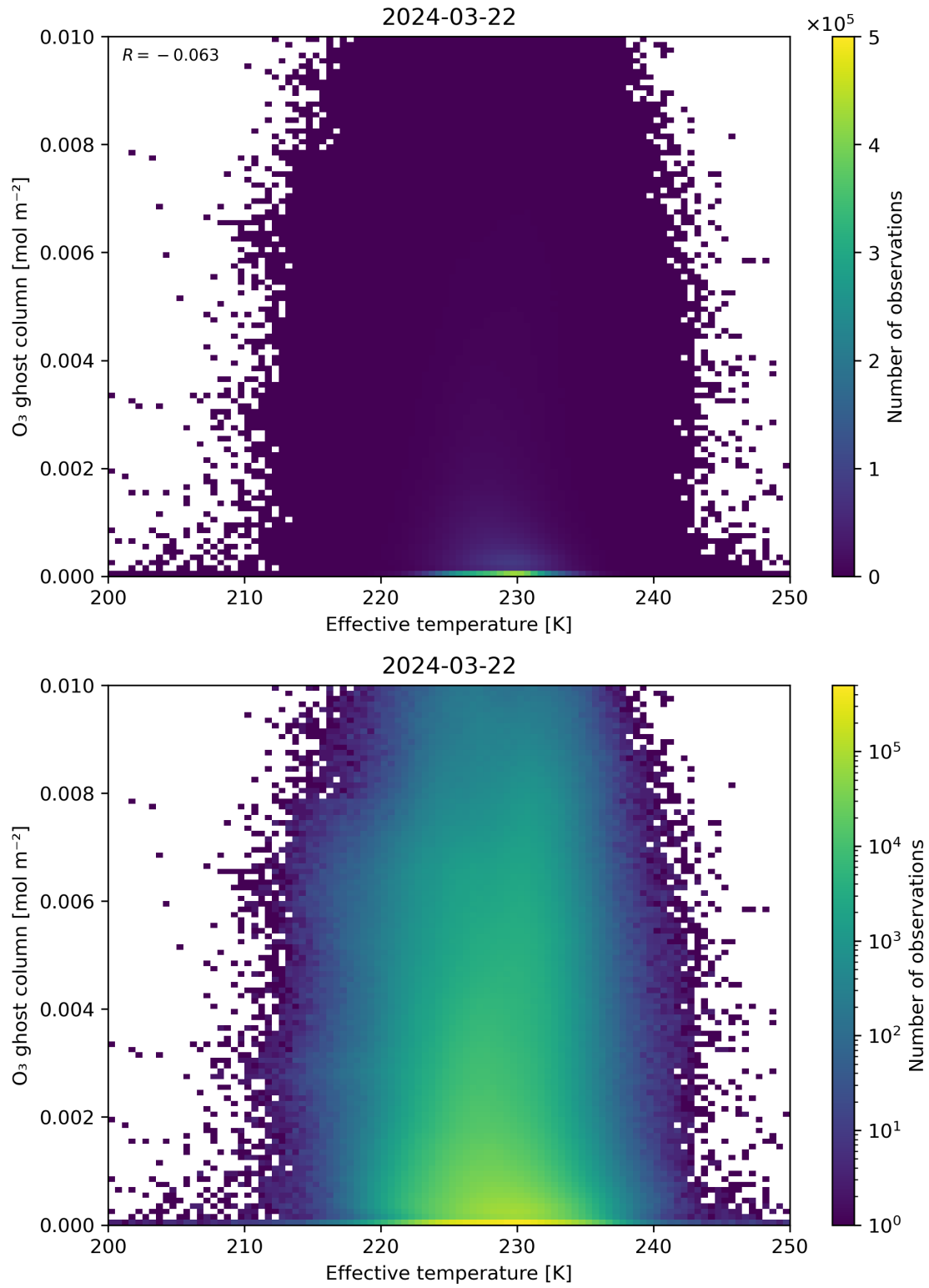
Figure 38: Scatter density plot of “Effective temperature” against “O 3 ghost column” for 2024-03-21 to 2024-03-22.
