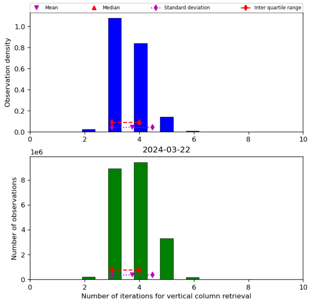
Figure 26: Histogram of “Number of iterations for vertical column retrieval” for 2024-03-21 to 2024-03-22
