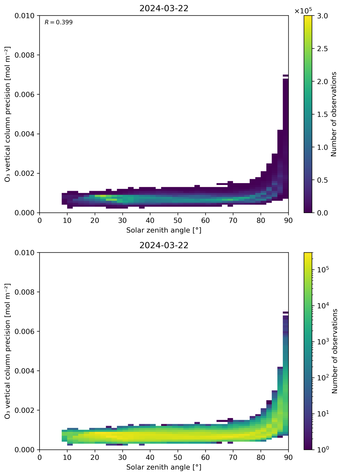
Figure 48: Scatter density plot of “Solar zenith angle” against “O 3 vertical column precision” for 2024-03-21 to 2024-03-22.
