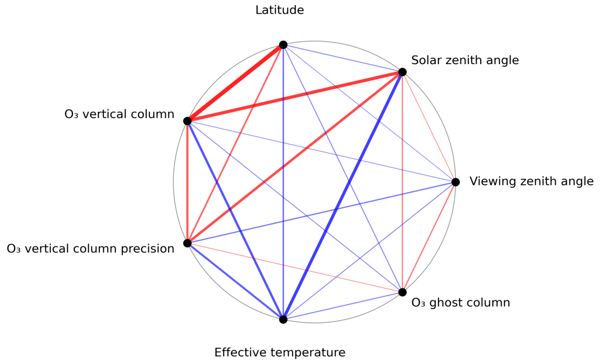
Figure 1: Map of correlation graph for 2024-03-21 to 2024-03-22.
