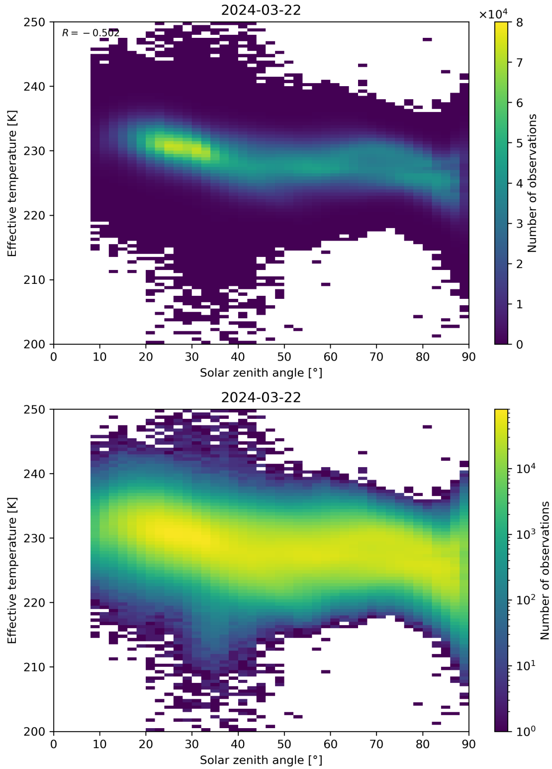
Figure 45: Scatter density plot of “Solar zenith angle” against “Effective temperature” for 2024-03-21 to 2024-03-22.
