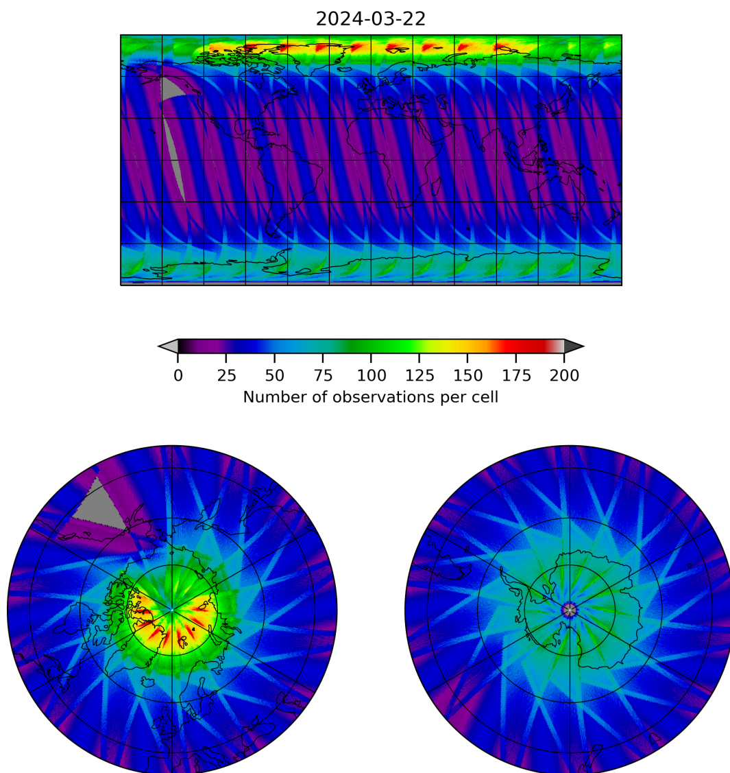
Figure 12: Map of the number of observations for 2024-03-21 to 2024-03-22
