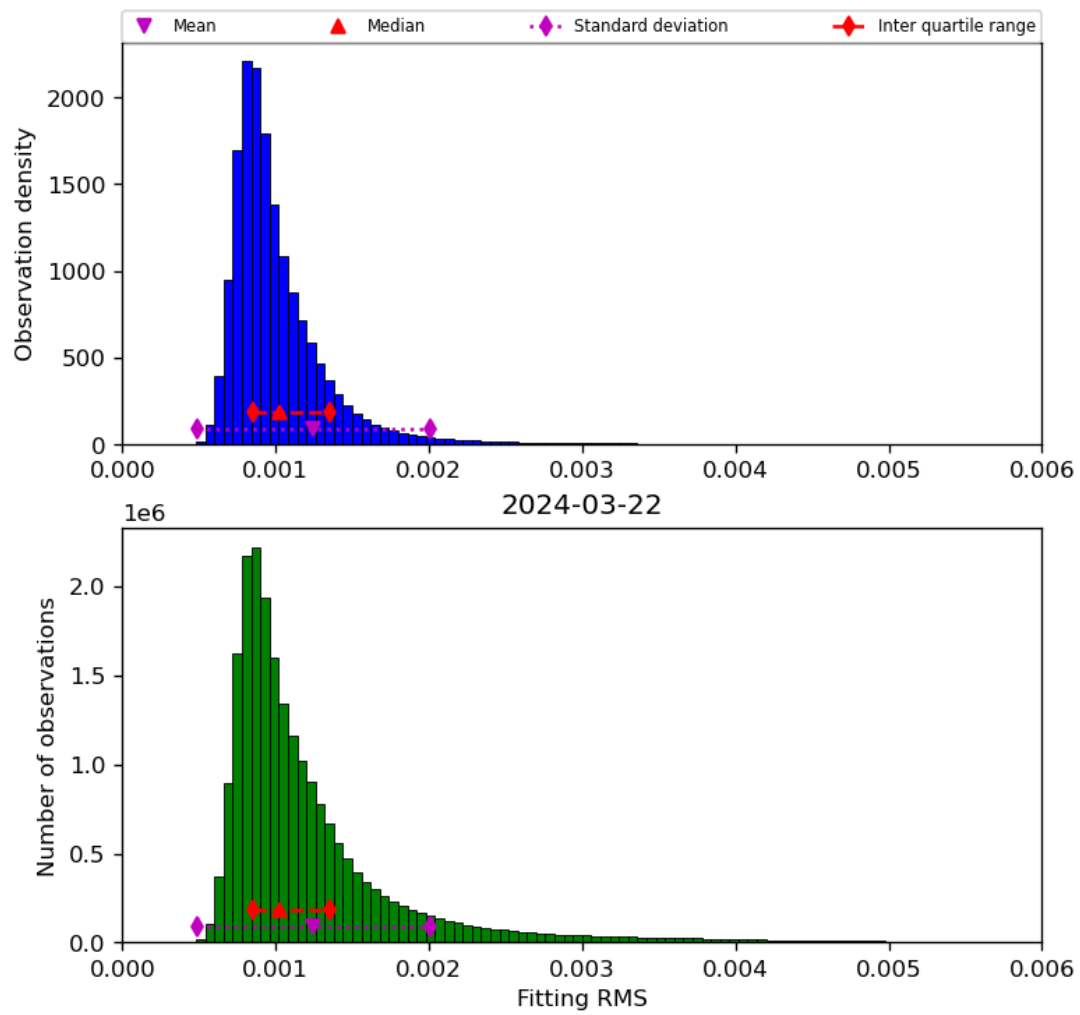
Figure 23: Histogram of “Fitting RMS” for 2024-03-21 to 2024-03-22
