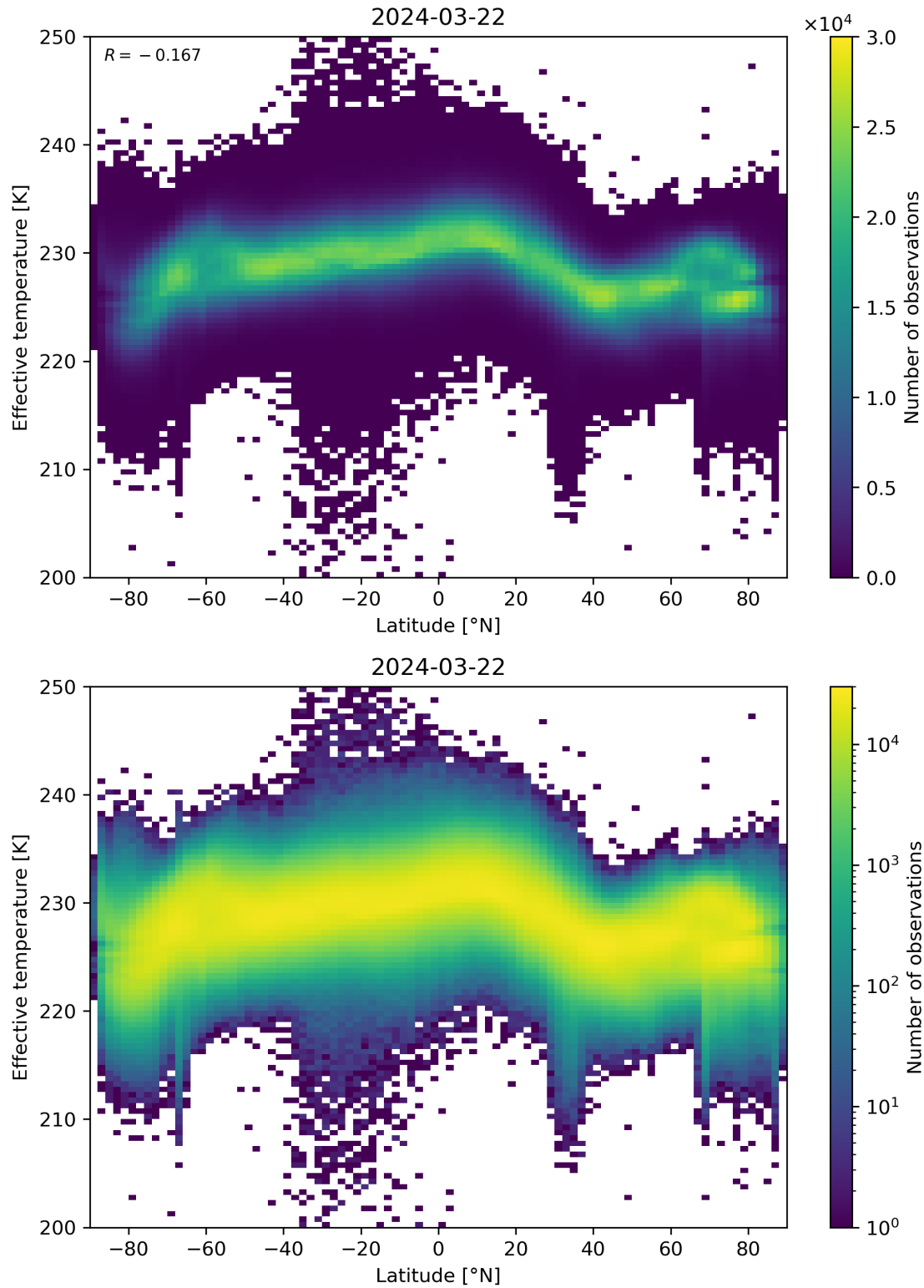
Figure 34: Scatter density plot of “Latitude” against “Effective temperature” for 2024-03-21 to 2024-03-22.
