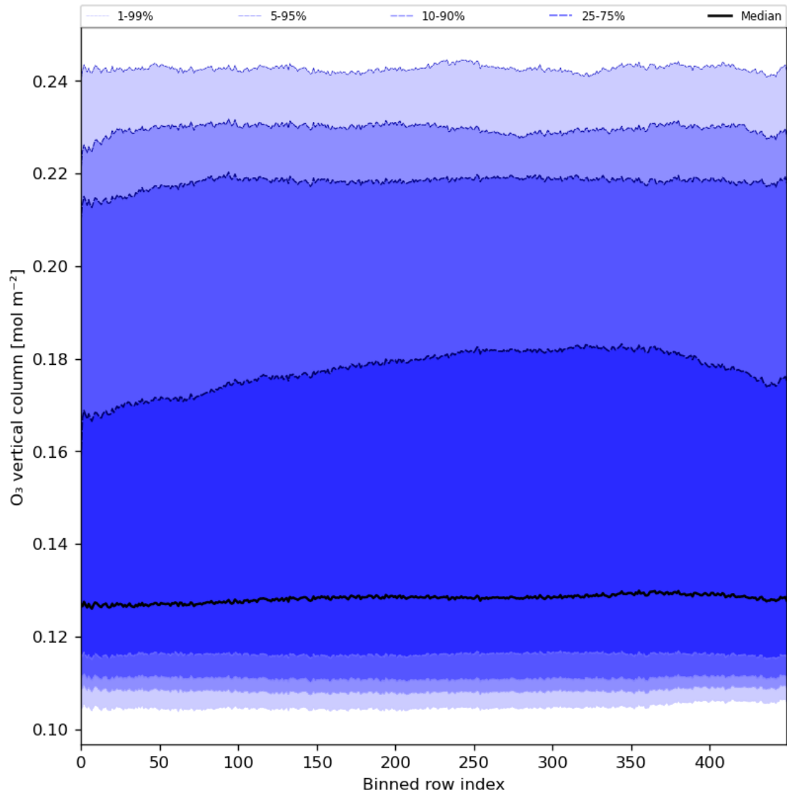
Figure 28: Along track statistics of “O 3 vertical column” for 2024-03-21 to 2024-03-22
