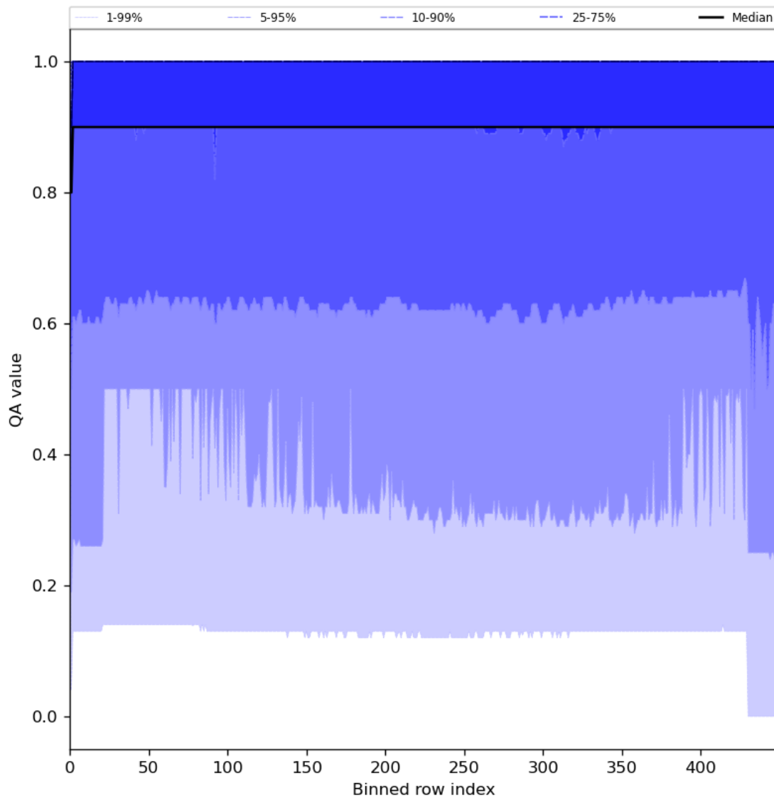
Figure 27: Along track statistics of “QA value” for 2024-03-21 to 2024-03-22
