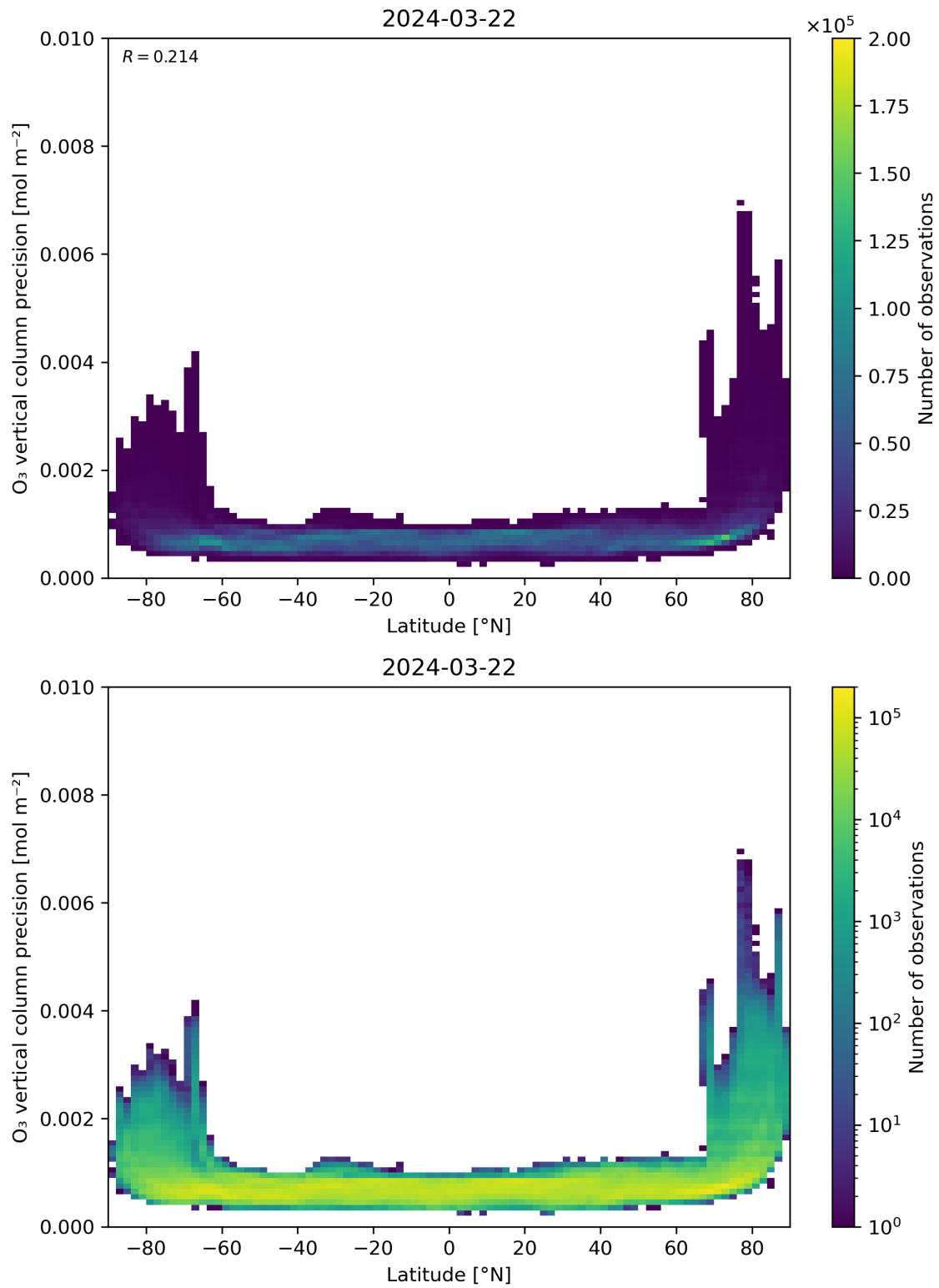
Figure 37: Scatter density plot of “Latitude” against “O 3 vertical column precision” for 2024-03-21 to 2024-03-22.
