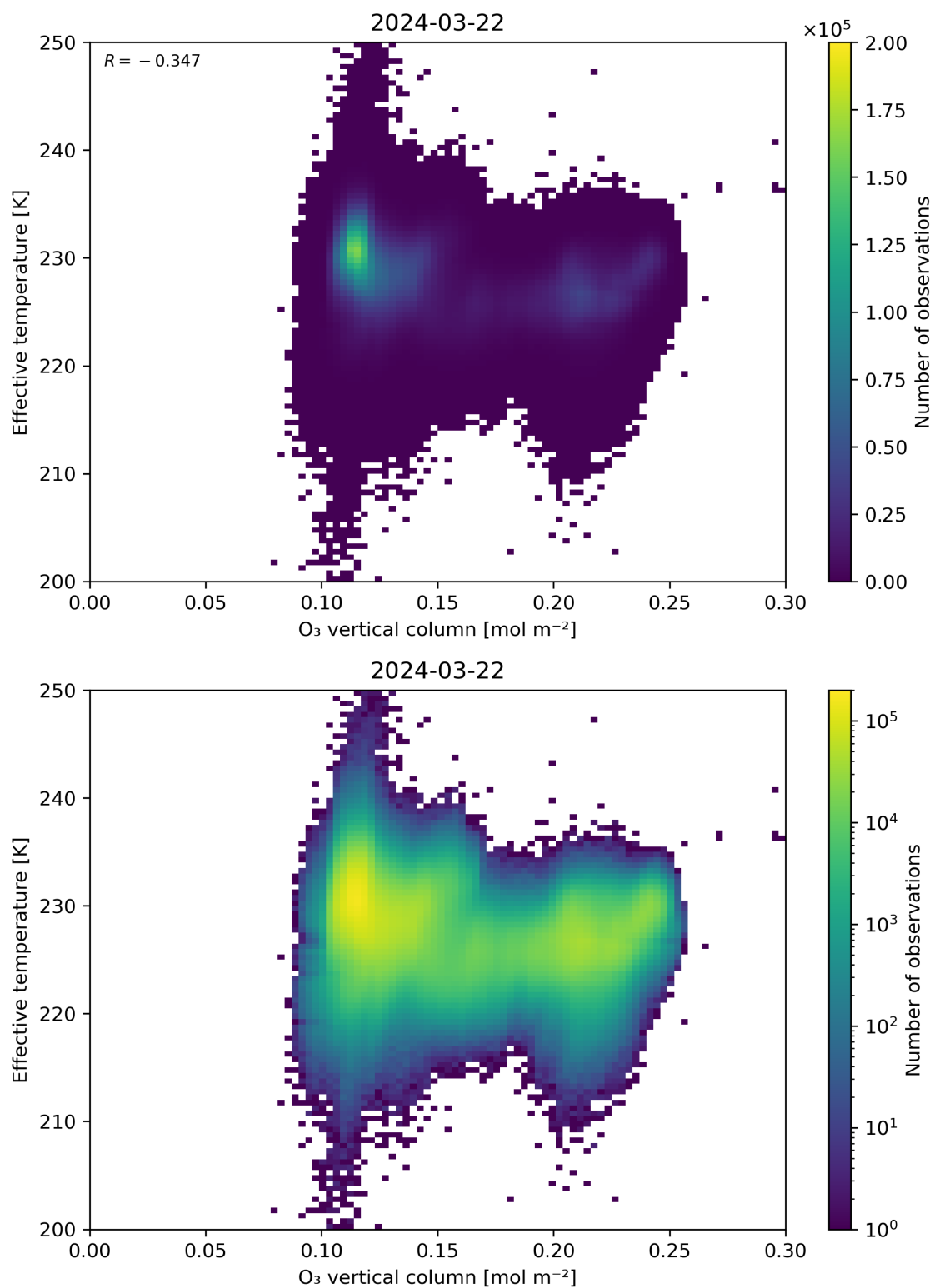
Figure 39: Scatter density plot of “O 3 vertical column” against “Effective temperature” for 2024-03-21 to 2024-03-22.
