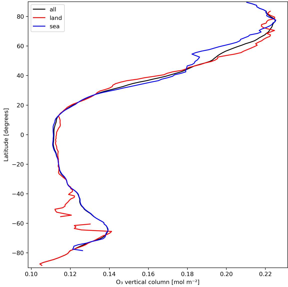
Figure 14: Zonal average of “O 3 vertical column” for 2024-03-21 to 2024-03-22.
