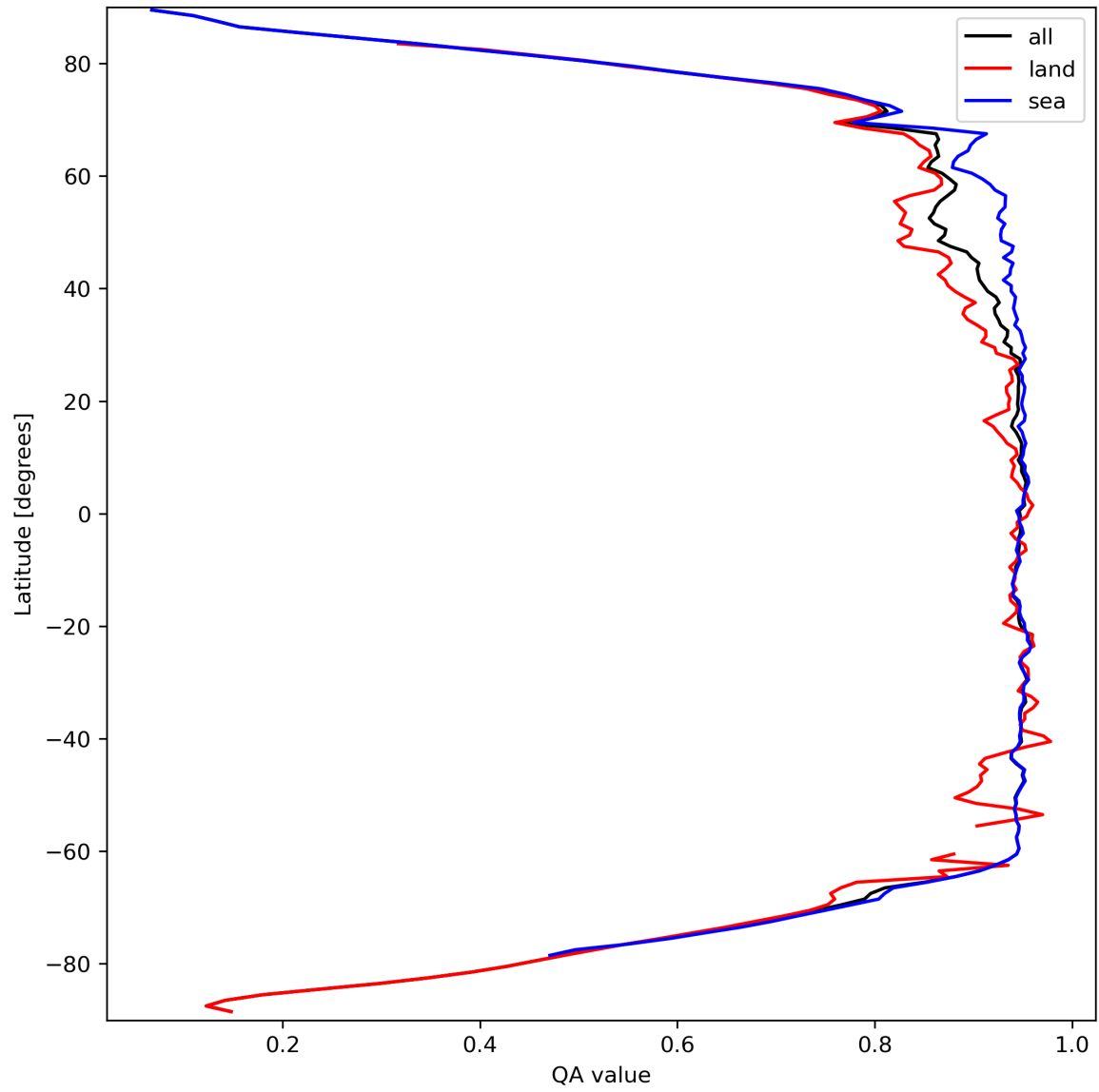
Figure 13: Zonal average of “QA value” for 2024-03-21 to 2024-03-22.
