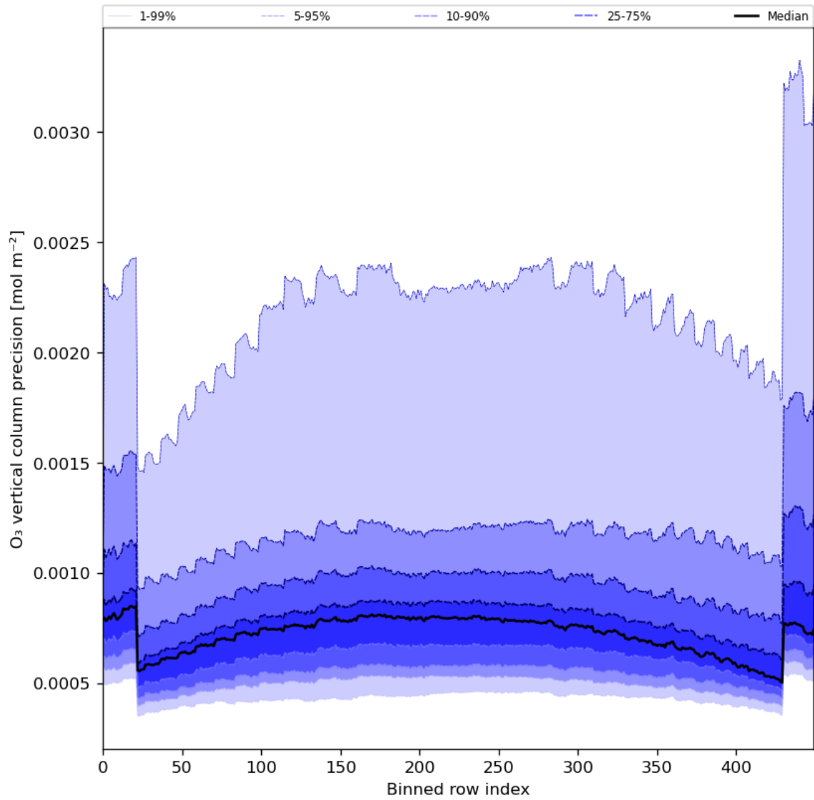
Figure 29: Along track statistics of “O 3 vertical column precision” for 2024-03-21 to 2024-03-22
