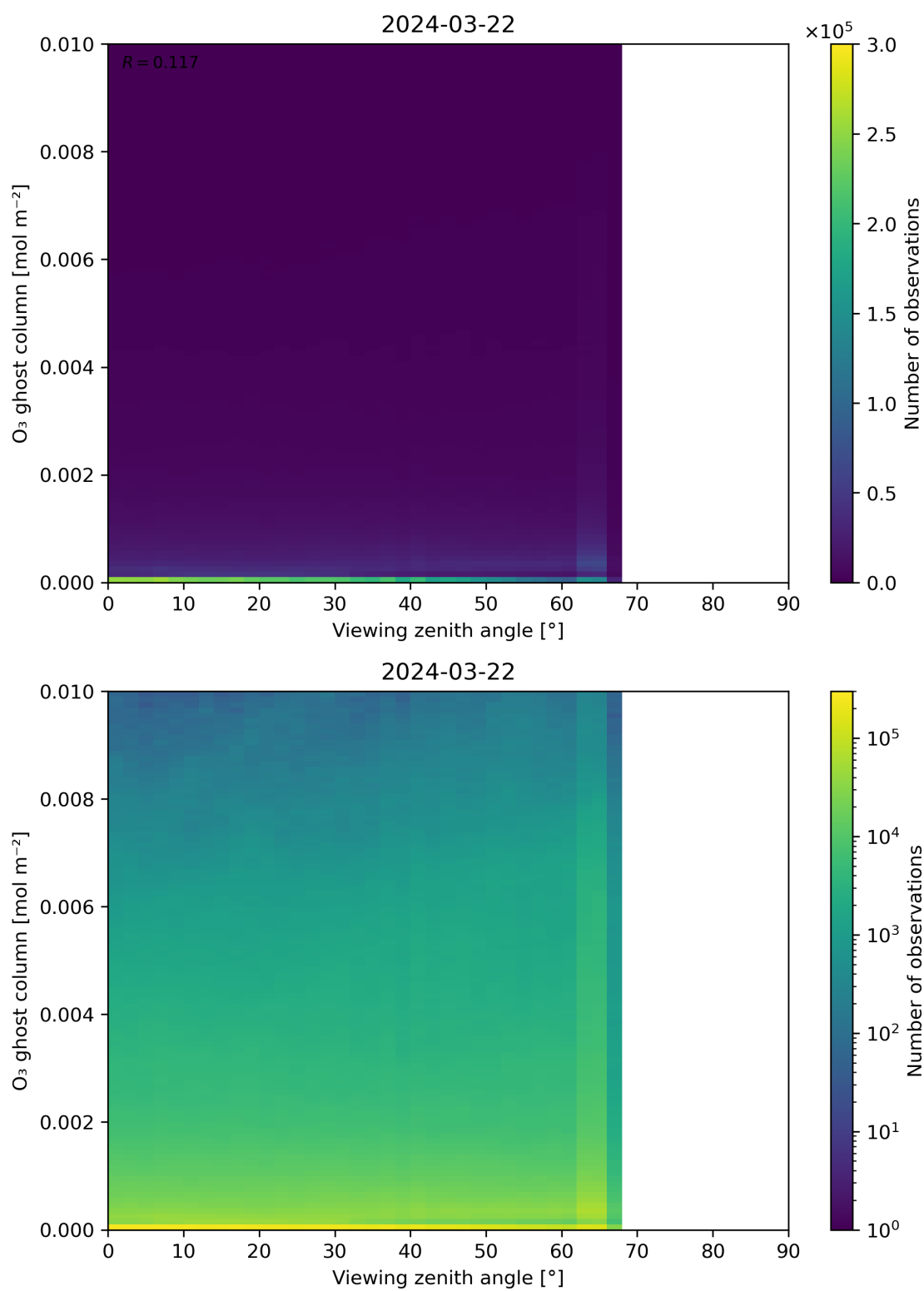
Figure 51: Scatter density plot of “Viewing zenith angle” against “O 3 ghost column” for 2024-03-21 to 2024-03-22.
