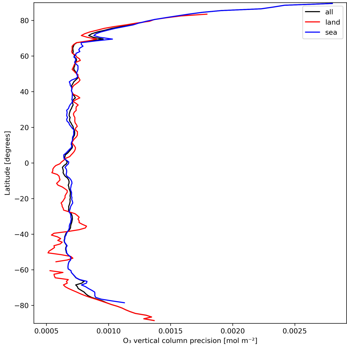
Figure 15: Zonal average of “O 3 vertical column precision” for 2024-03-21 to 2024-03-22.
