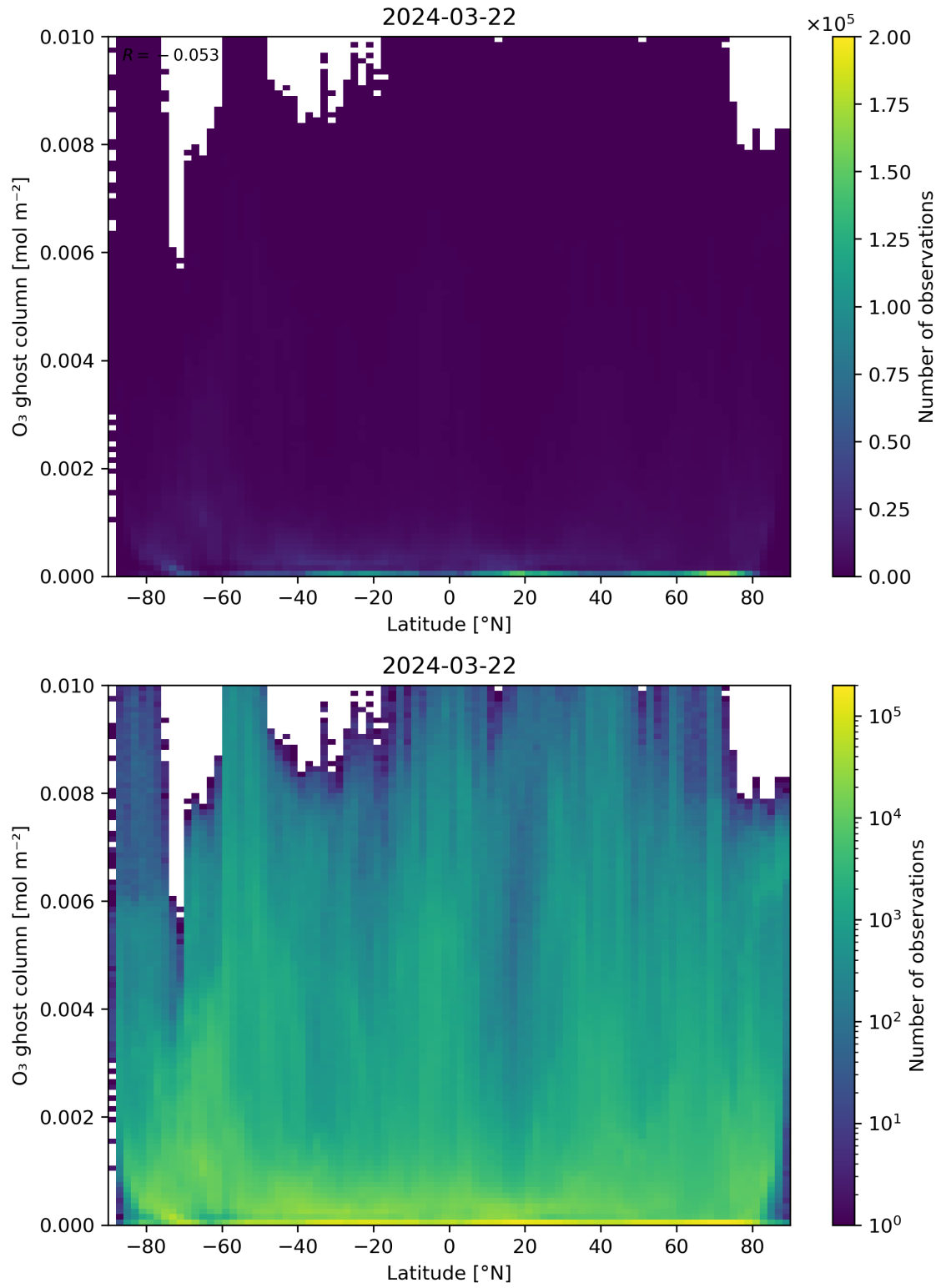
Figure 35: Scatter density plot of “Latitude” against “O 3 ghost column” for 2024-03-21 to 2024-03-22.
