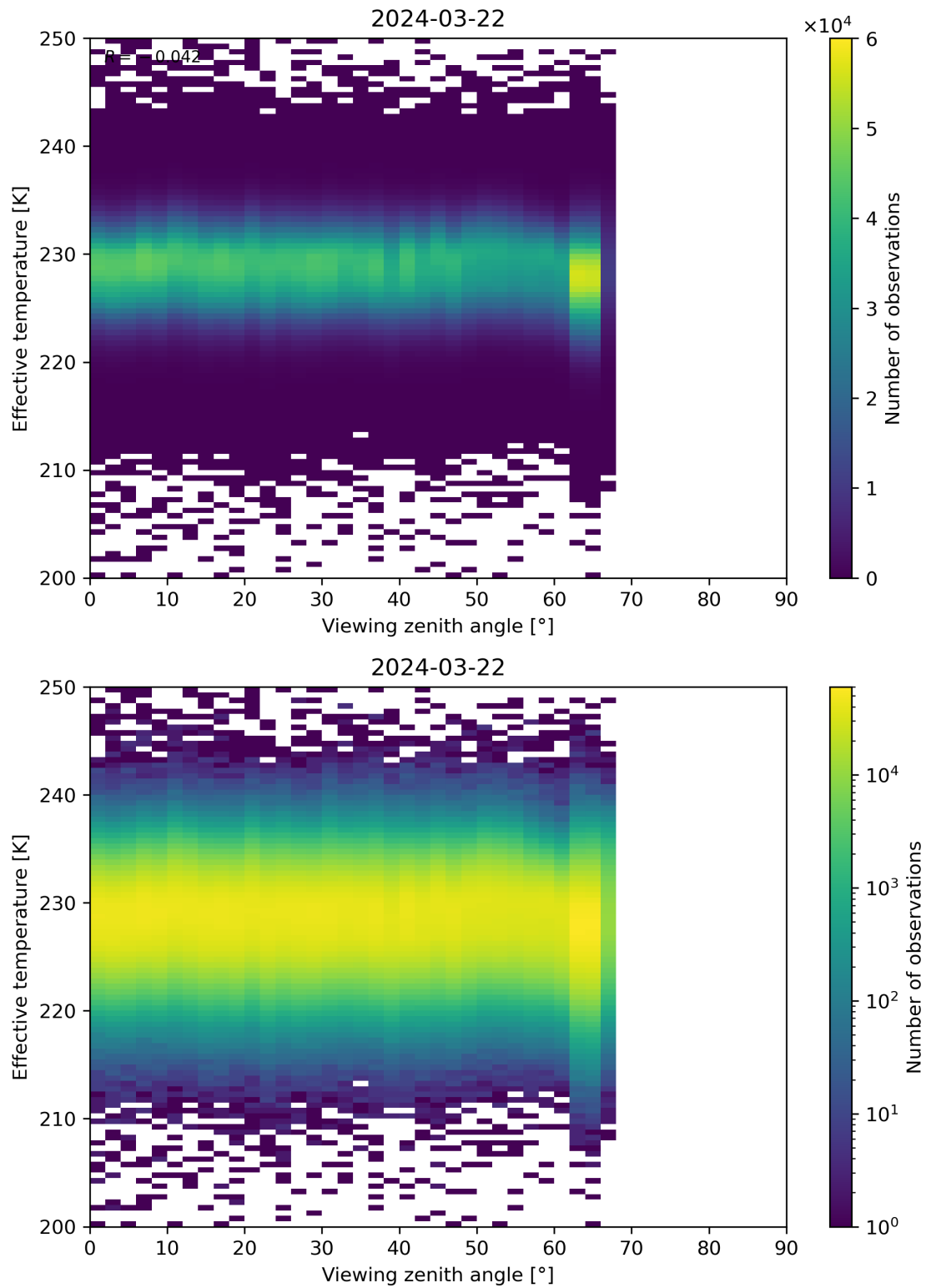
Figure 50: Scatter density plot of “Viewing zenith angle” against “Effective temperature” for 2024-03-21 to 2024-03-22.
