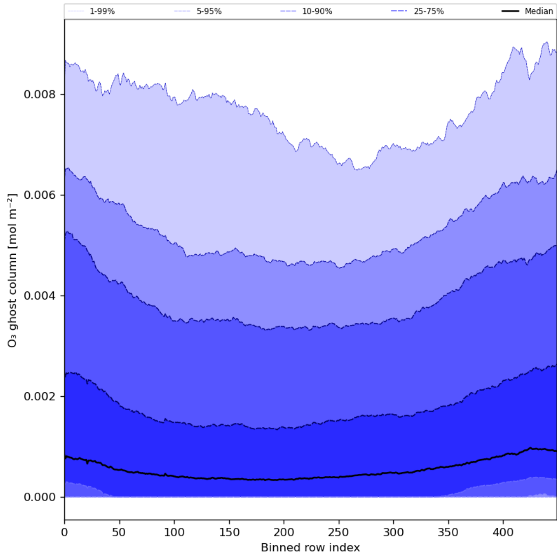
Figure 32: Along track statistics of “O 3 ghost column” for 2024-03-21 to 2024-03-22
