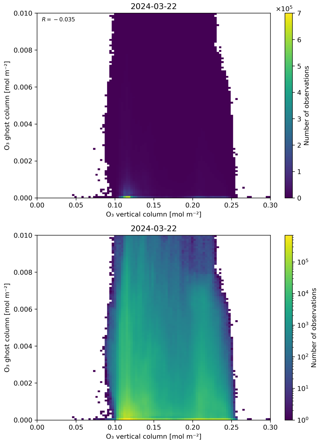
Figure 40: Scatter density plot of “O 3 vertical column” against “O 3 ghost column” for 2024-03-21 to 2024-03-22.
