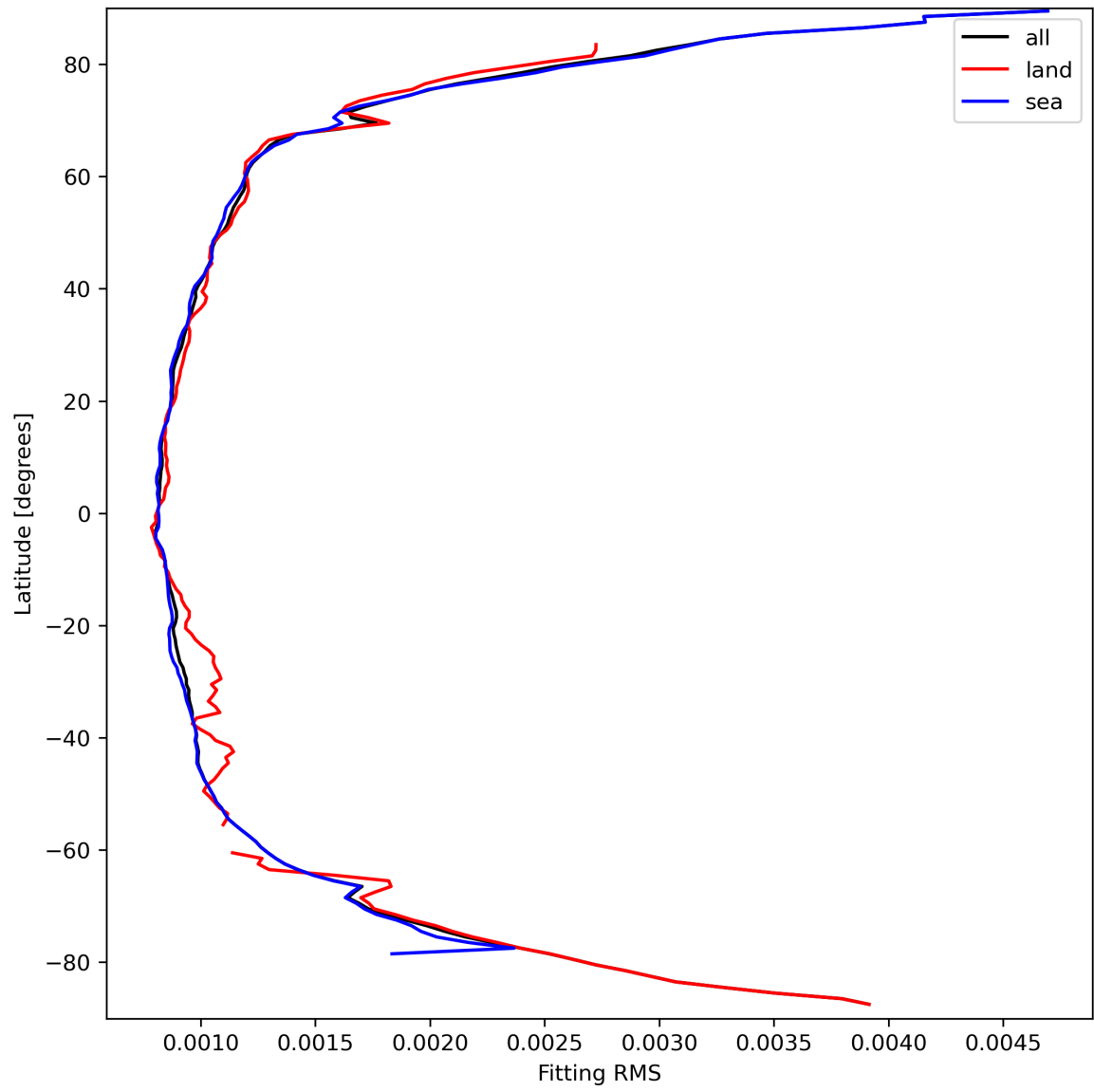
Figure 16: Zonal average of “Fitting RMS” for 2024-03-23 to 2024-03-24.
