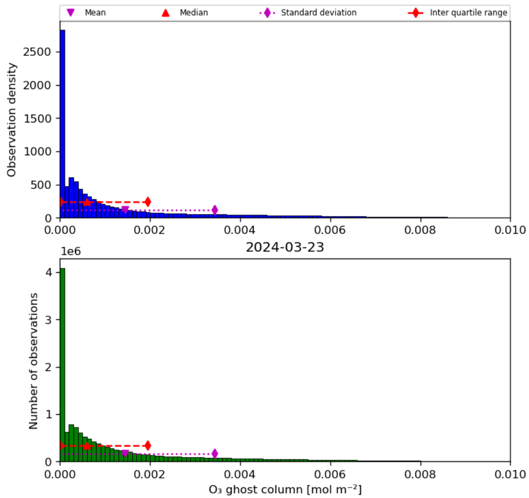
Figure 25: Histogram of “O 3 ghost column” for 2024-03-23 to 2024-03-24
