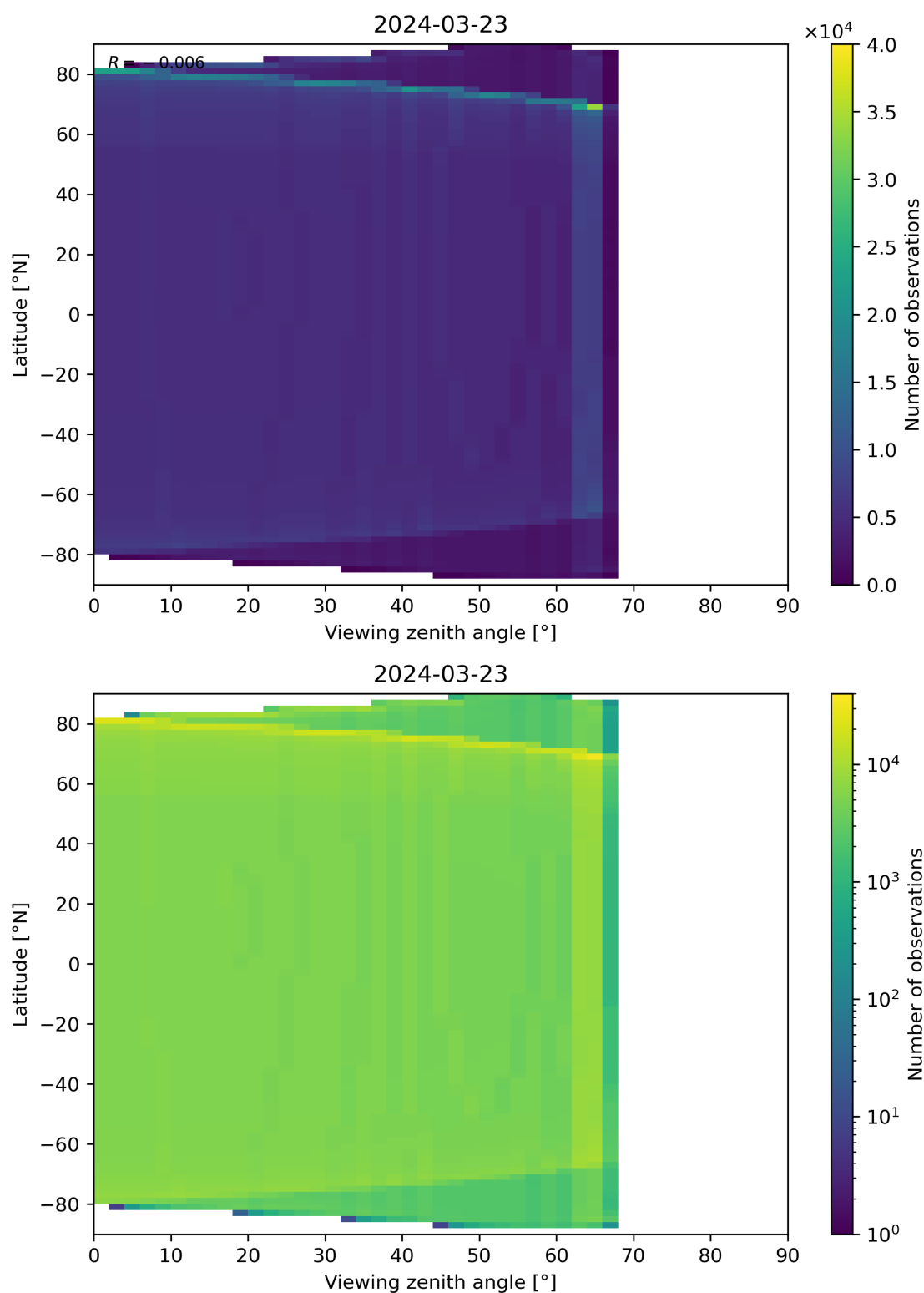
Figure 49: Scatter density plot of “Viewing zenith angle” against “Latitude” for 2024-03-23 to 2024-03-24.
