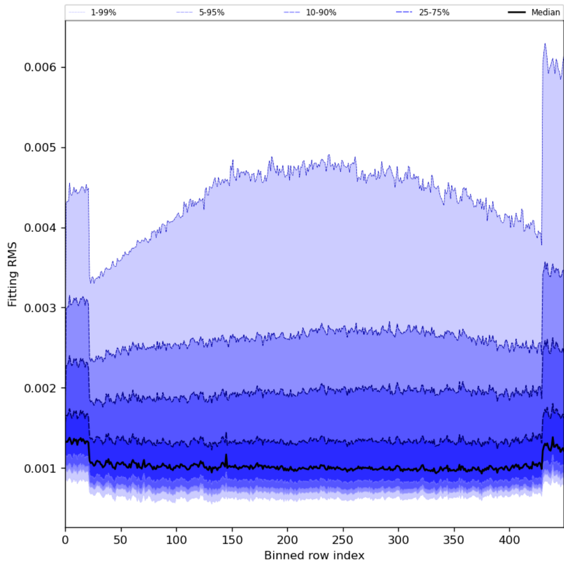
Figure 30: Along track statistics of “Fitting RMS” for 2024-03-23 to 2024-03-24
