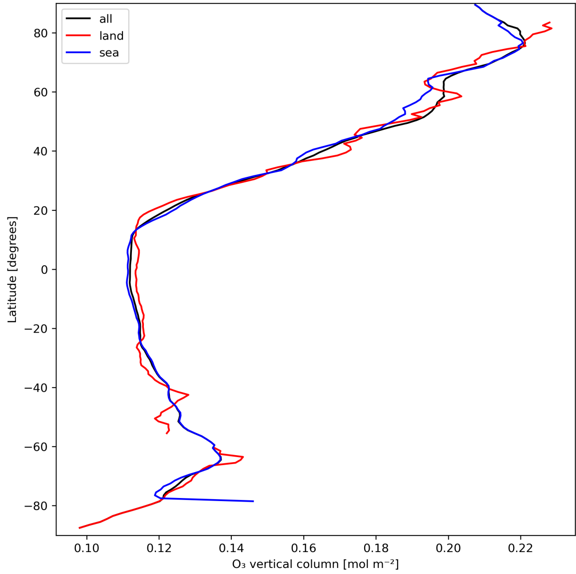
Figure 14: Zonal average of “O 3 vertical column” for 2024-03-23 to 2024-03-24.
