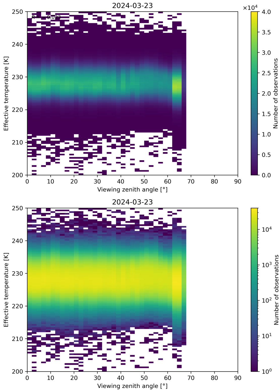
Figure 50: Scatter density plot of “Viewing zenith angle” against “Effective temperature” for 2024-03-23 to 2024-03-24.
