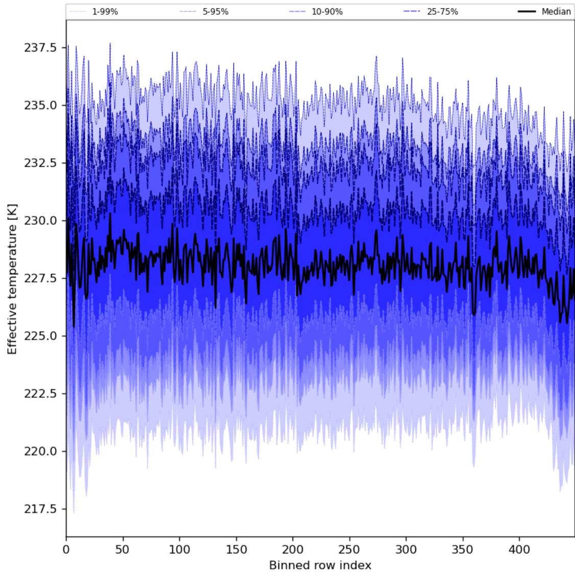
Figure 31: Along track statistics of “Effective temperature” for 2024-03-23 to 2024-03-24
