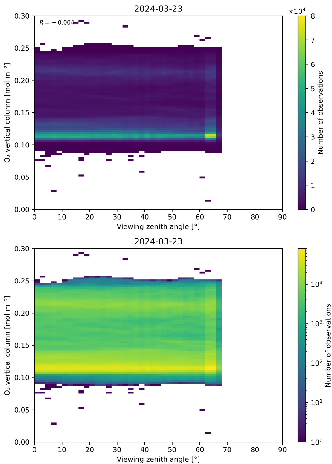
Figure 52: Scatter density plot of “Viewing zenith angle” against “O 3 vertical column” for 2024-03-23 to 2024-03-24.
