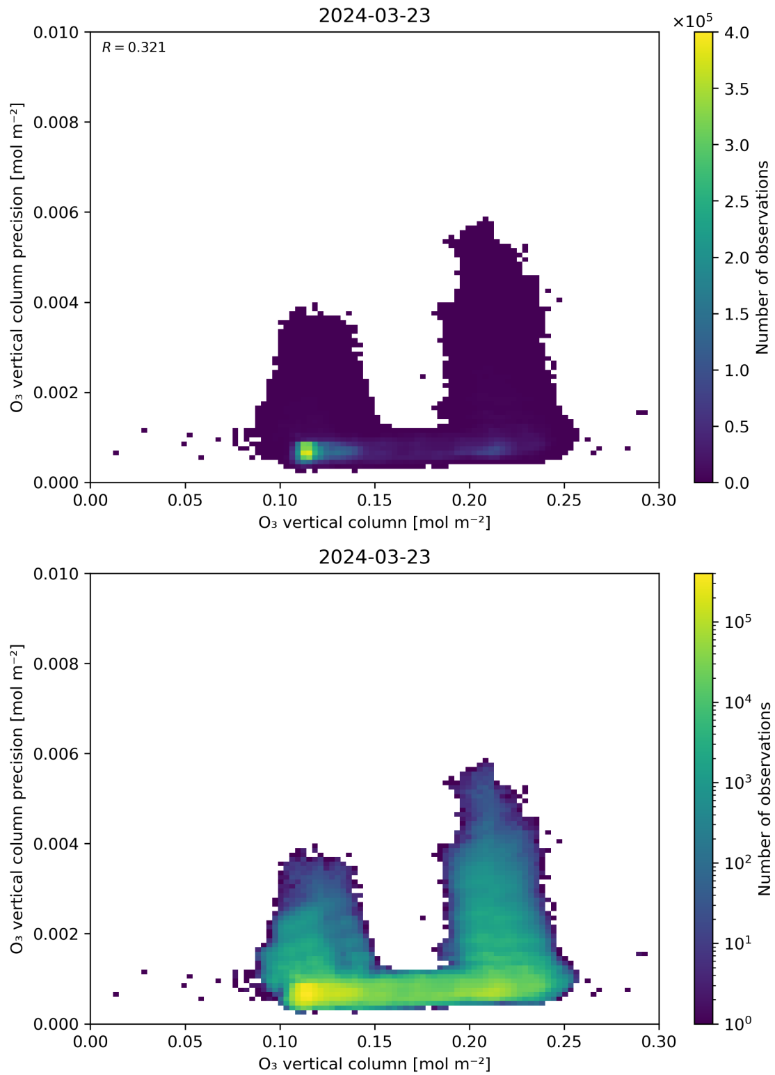
Figure 41: Scatter density plot of “O 3 vertical column” against “O 3 vertical column precision” for 2024-03-23 to 2024-03-24.
