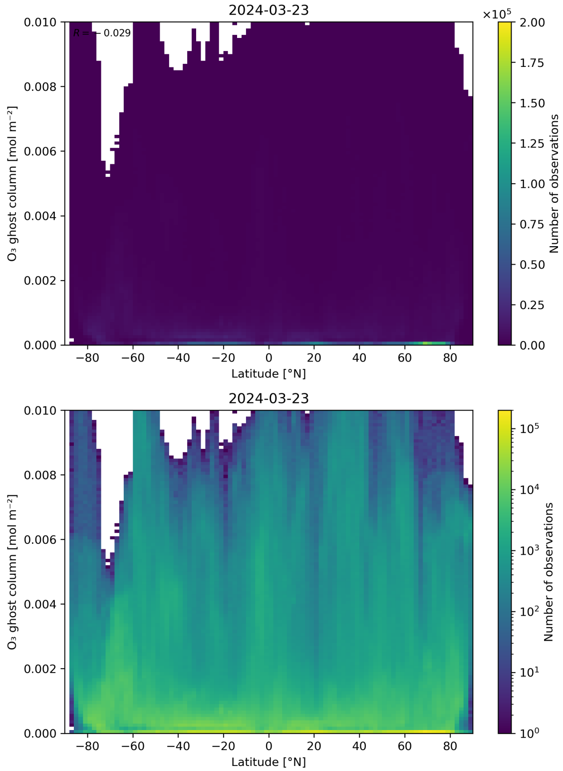
Figure 35: Scatter density plot of “Latitude” against “O 3 ghost column” for 2024-03-23 to 2024-03-24.
