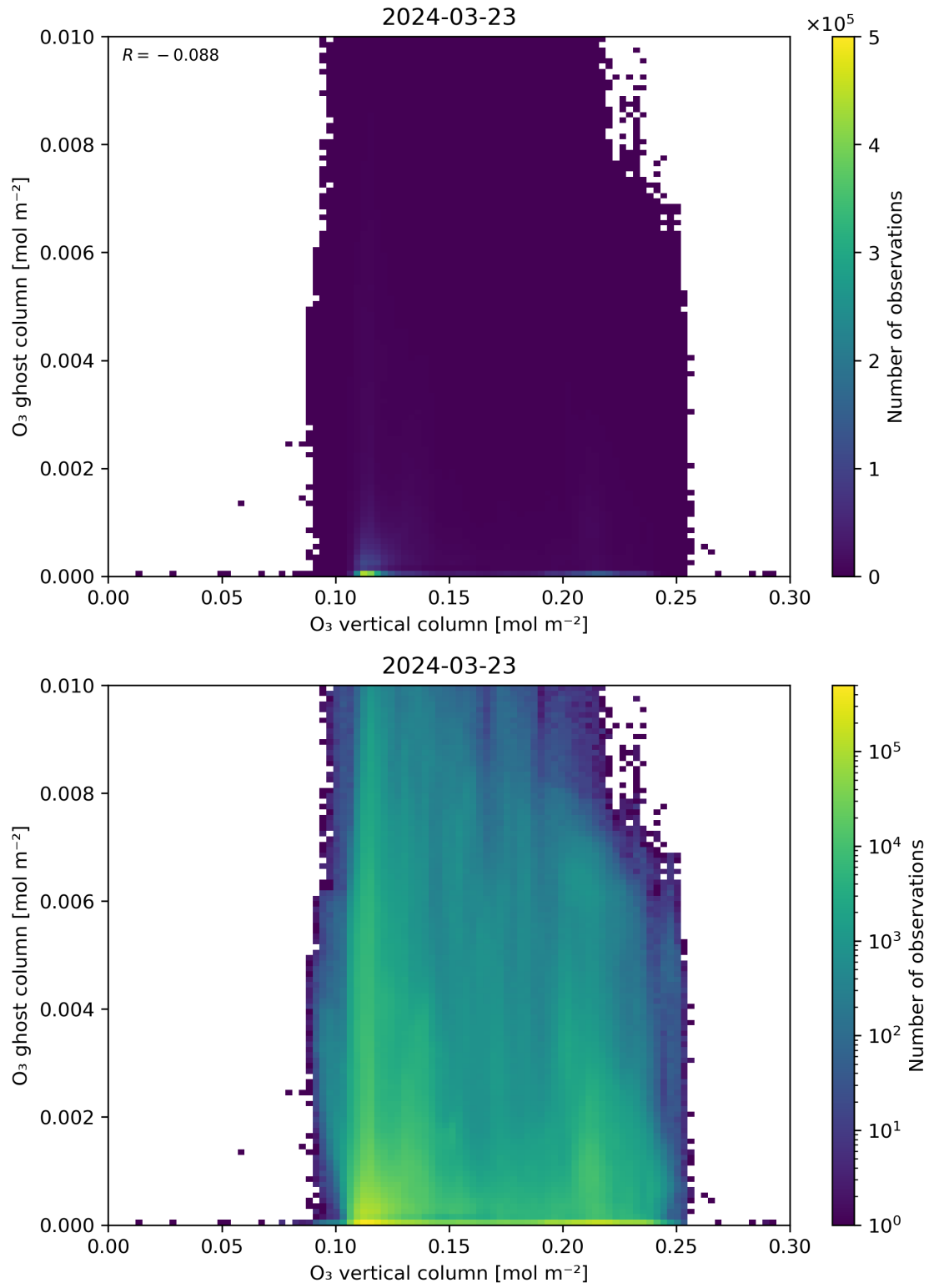
Figure 40: Scatter density plot of “O 3 vertical column” against “O 3 ghost column” for 2024-03-23 to 2024-03-24.
