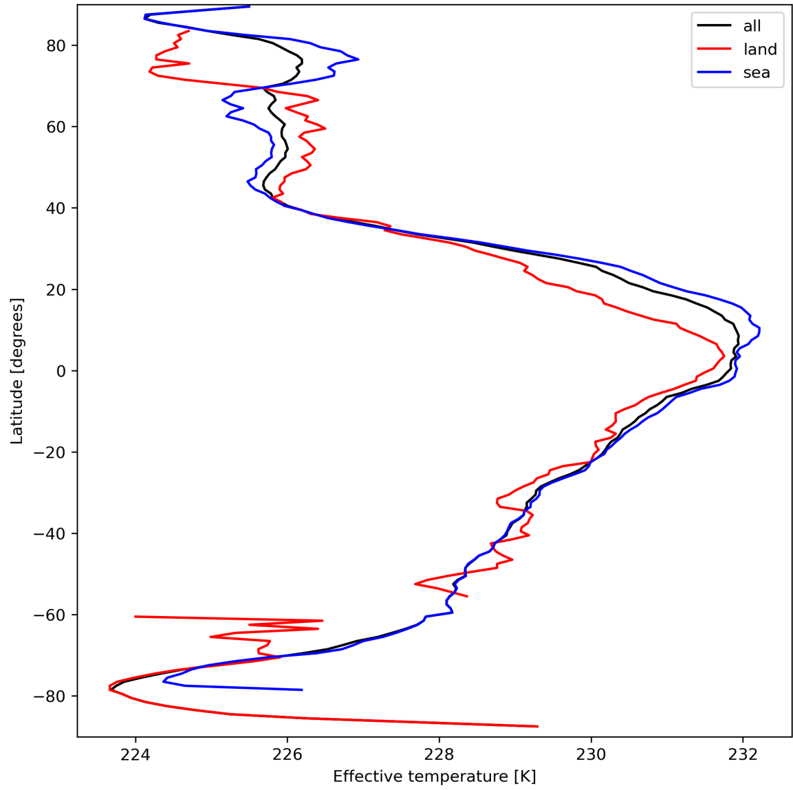
Figure 17: Zonal average of “Effective temperature” for 2024-03-23 to 2024-03-24.
