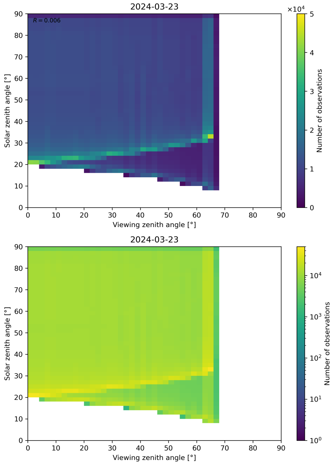
Figure 54: Scatter density plot of “Viewing zenith angle” against “Solar zenith angle” for 2024-03-23 to 2024-03-24.
