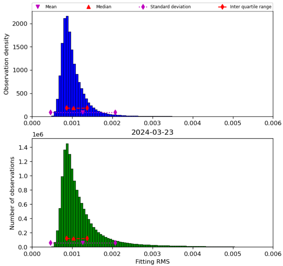
Figure 23: Histogram of “Fitting RMS” for 2024-03-23 to 2024-03-24
