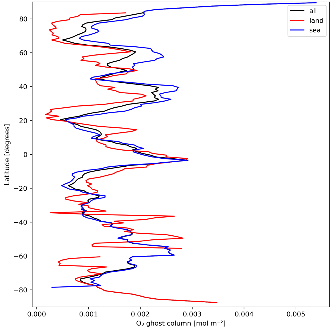
Figure 18: Zonal average of "O 3 ghost column" for 2024-03-23 to 2024-03-24.
