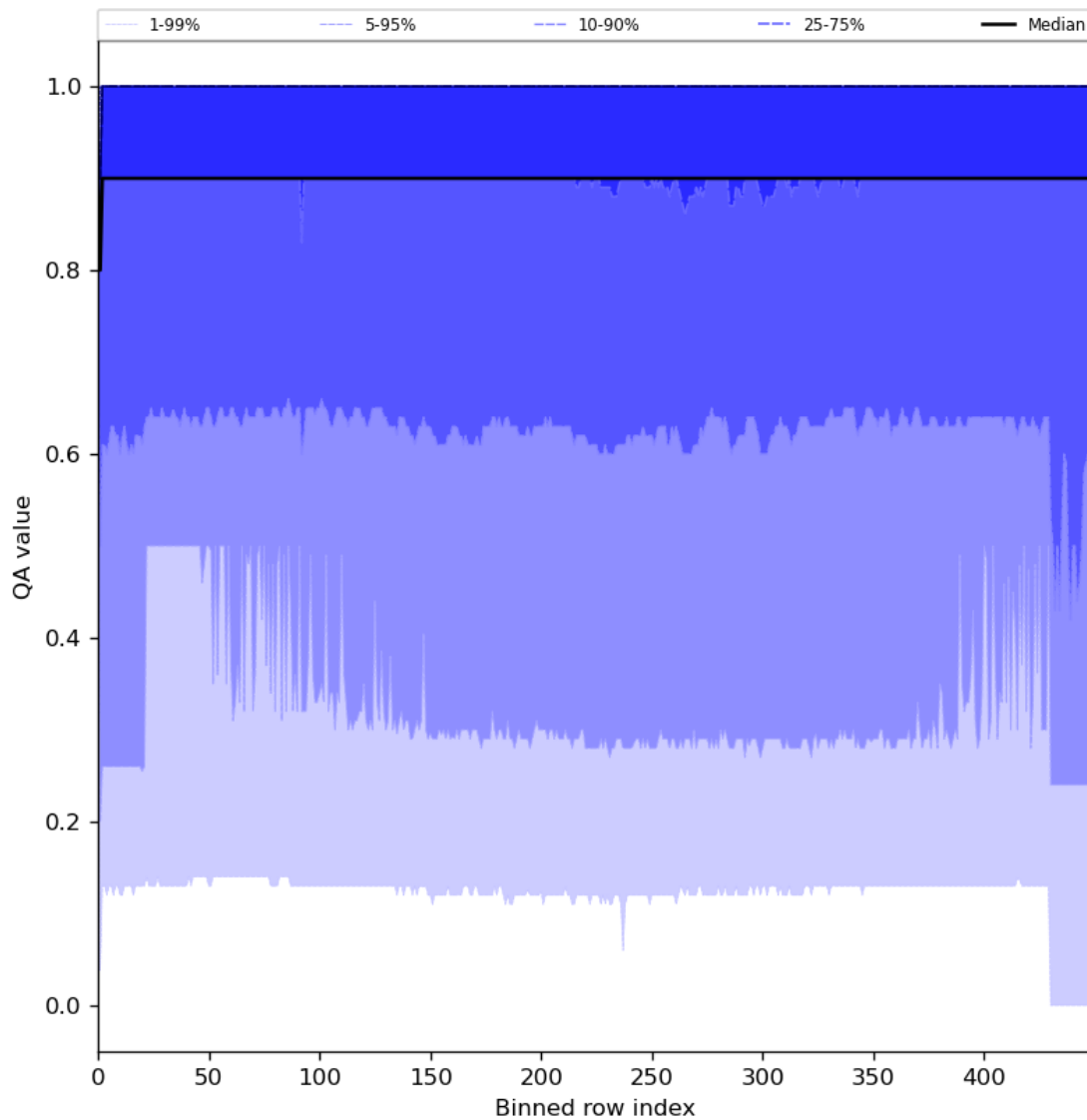
Figure 27: Along track statistics of “QA value” for 2024-03-23 to 2024-03-24
