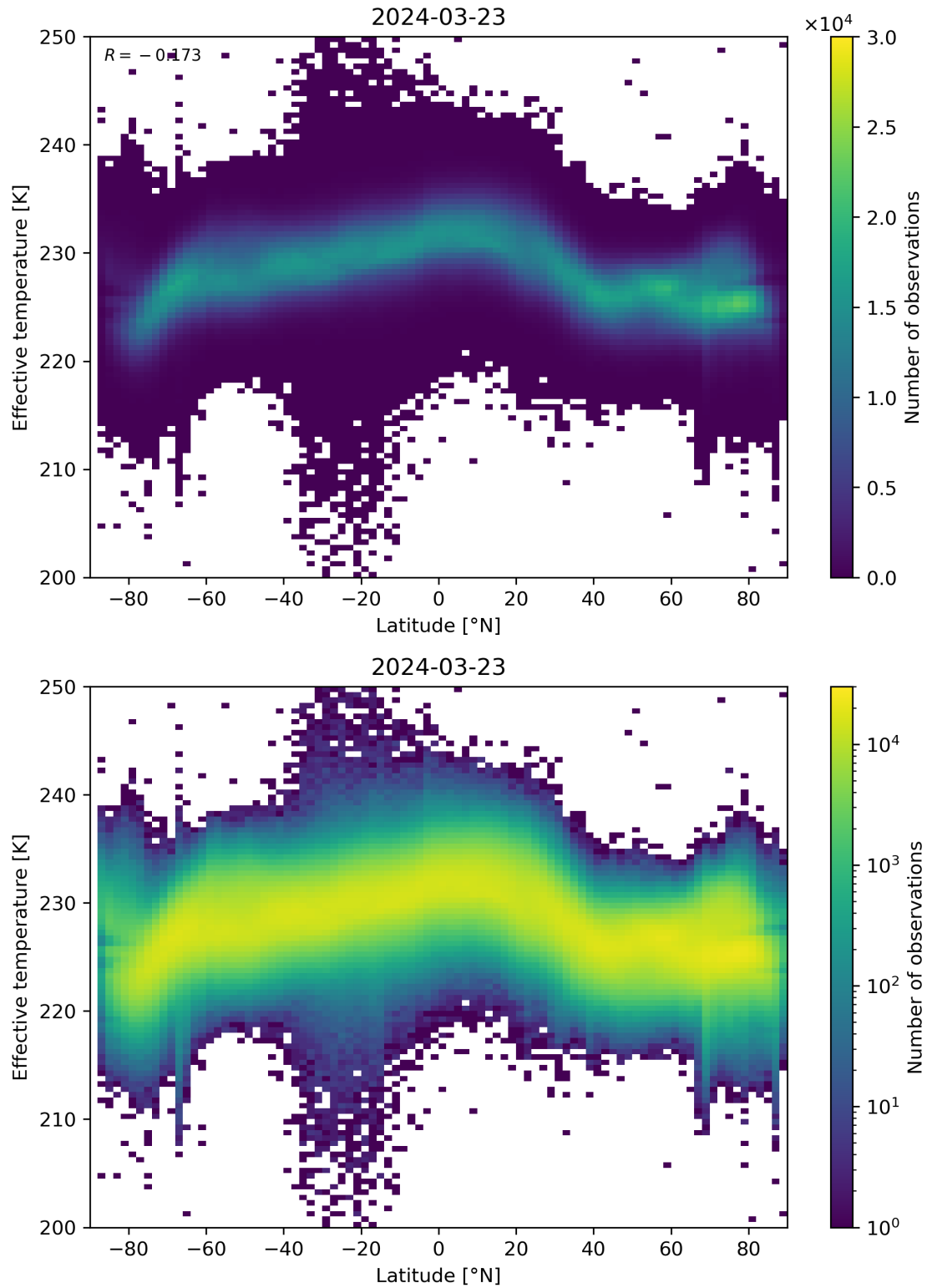
Figure 34: Scatter density plot of “Latitude” against “Effective temperature” for 2024-03-23 to 2024-03-24.
