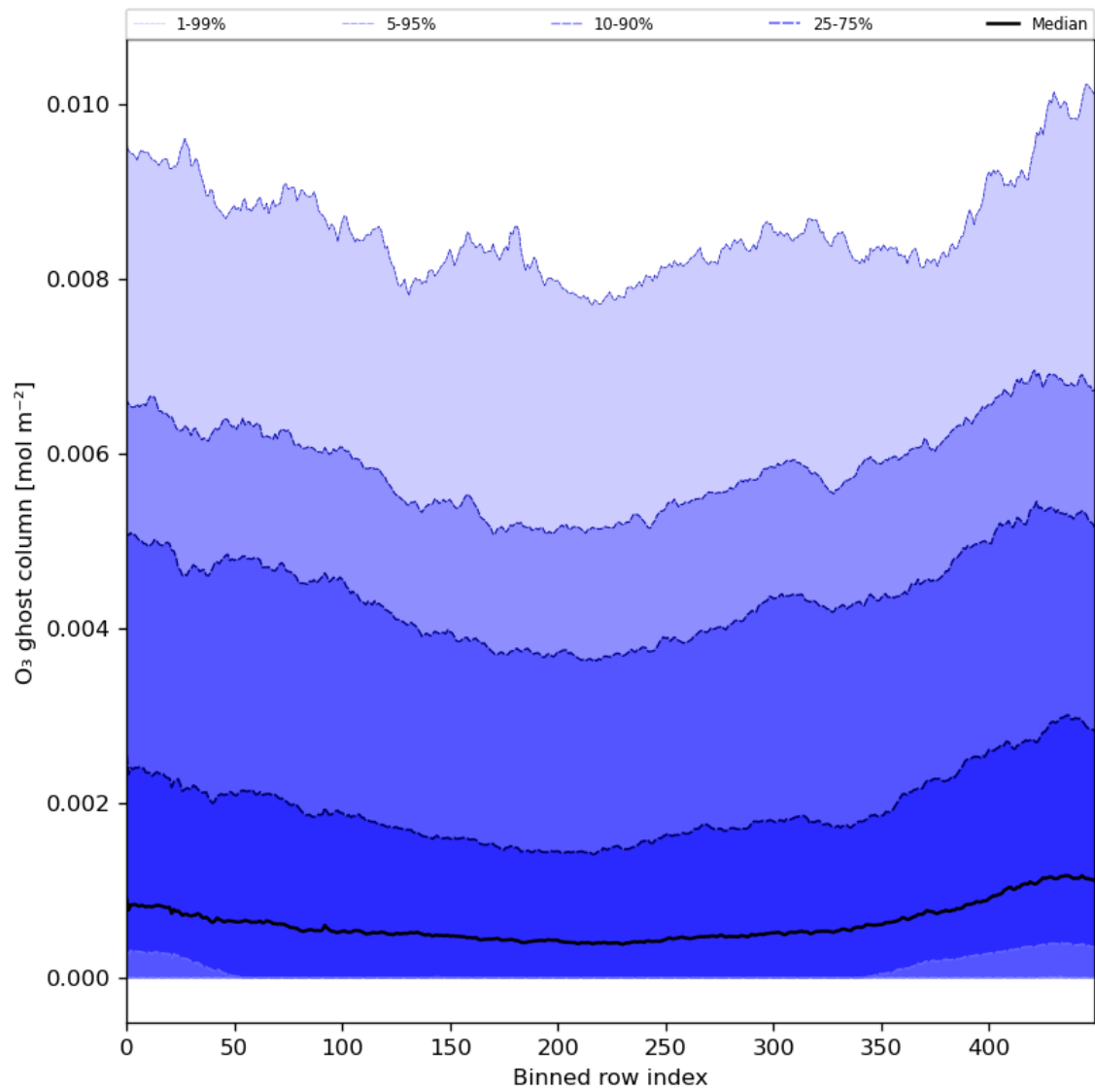
Figure 32: Along track statistics of “O 3 ghost column” for 2024-03-23 to 2024-03-24
