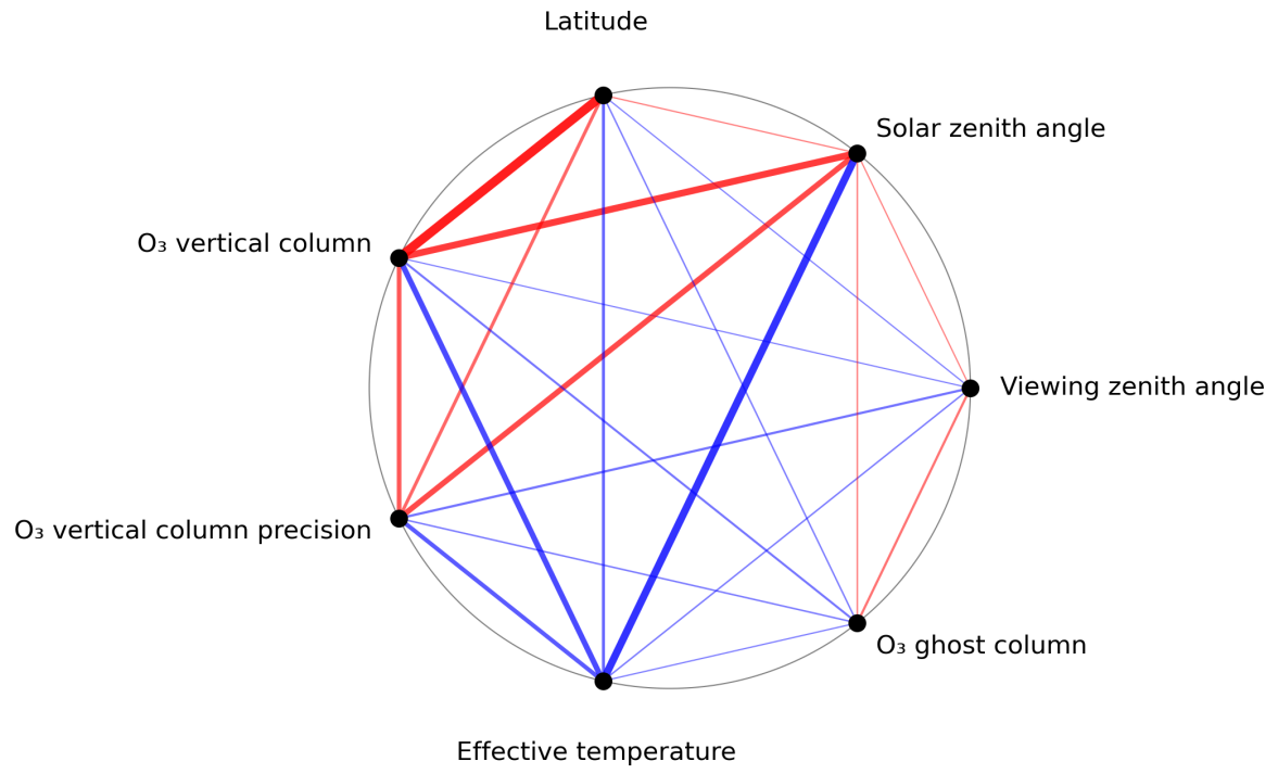
Figure 1: Map of correlation graph for 2024-03-23 to 2024-03-24.
