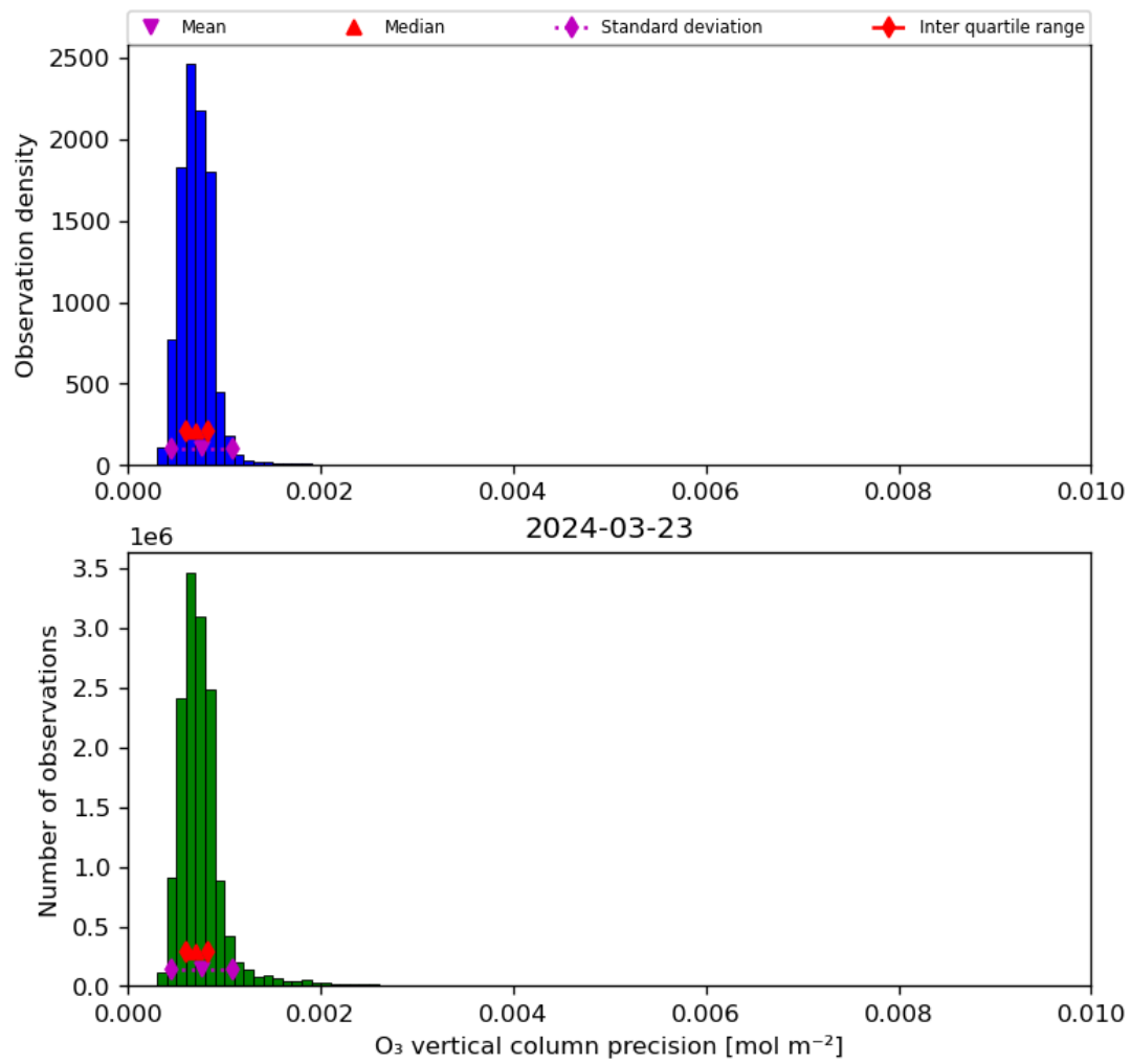
Figure 22: Histogram of “O 3 vertical column precision” for 2024-03-23 to 2024-03-24
