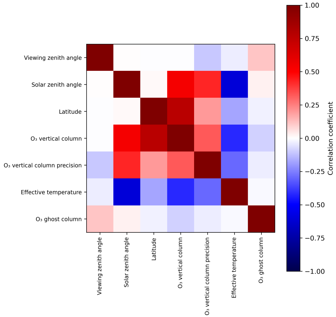
Figure 2: Map of correlation matrix for 2024-03-23 to 2024-03-24.
