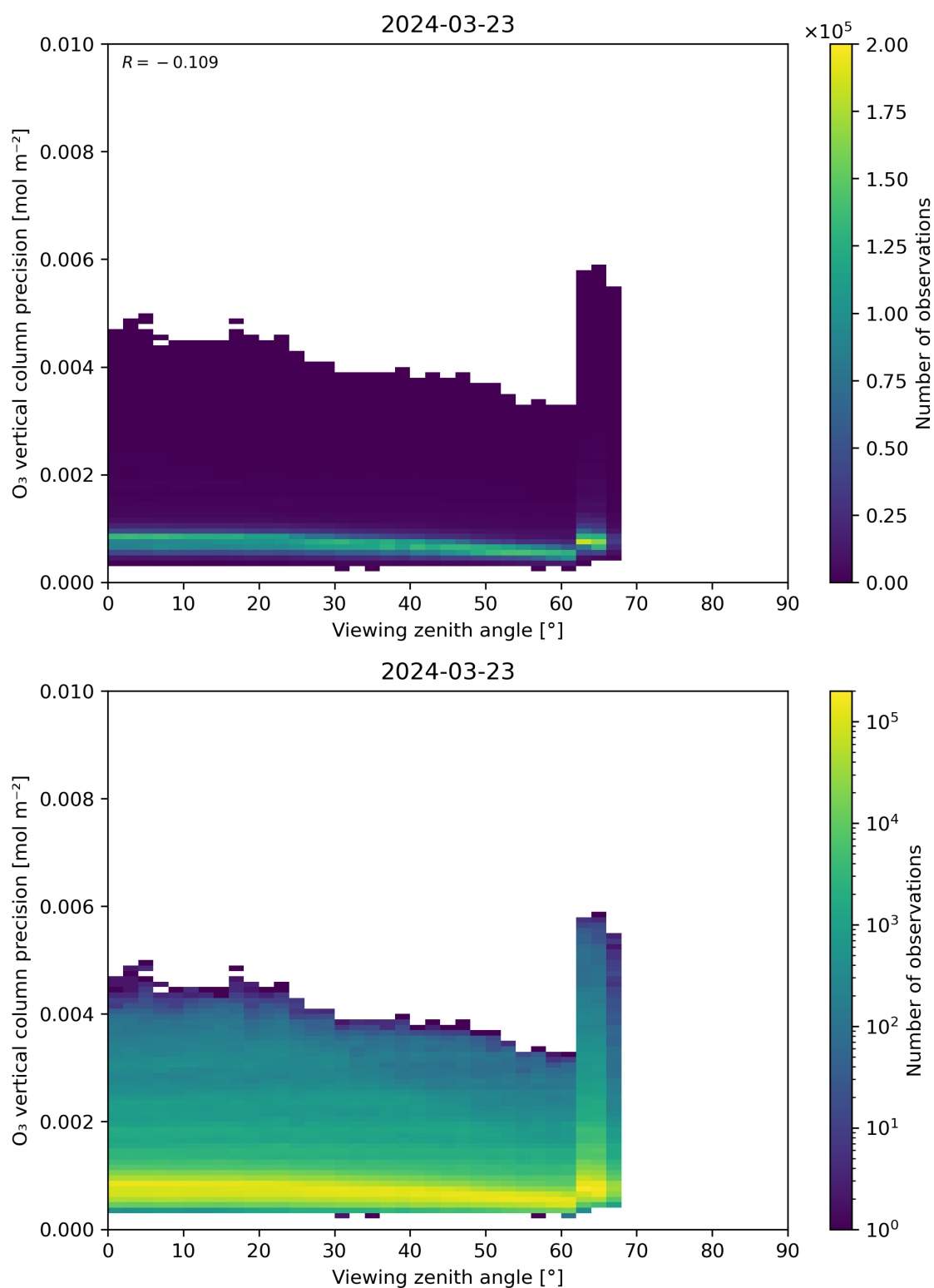
Figure 53: Scatter density plot of “Viewing zenith angle” against “O 3 vertical column precision” for 2024-03-23 to 2024-03-24.
