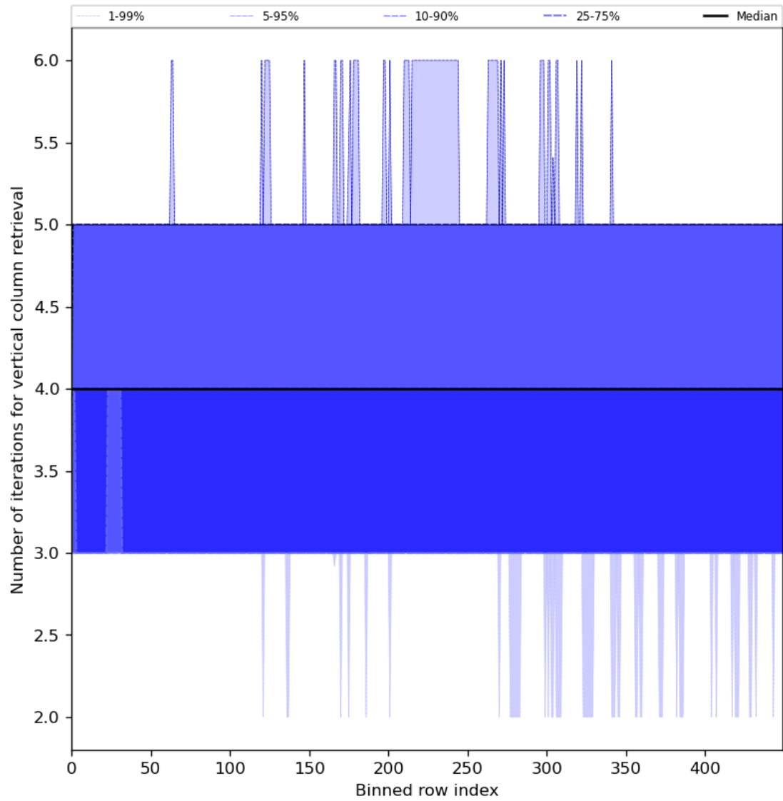
Figure 33: Along track statistics of “Number of iterations for vertical column retrieval” for 2024-03-23 to 2024-03-24
