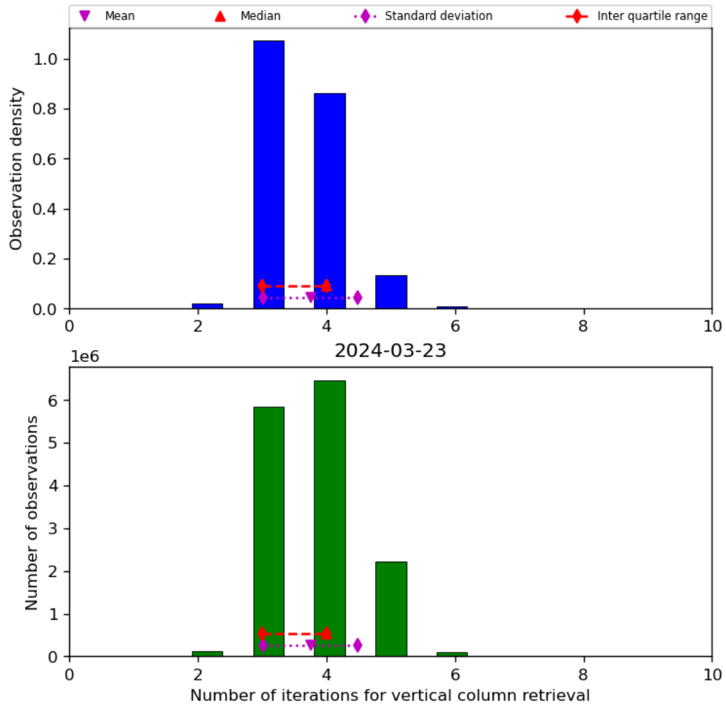
Figure 26: Histogram of “Number of iterations for vertical column retrieval” for 2024-03-23 to 2024-03-24
