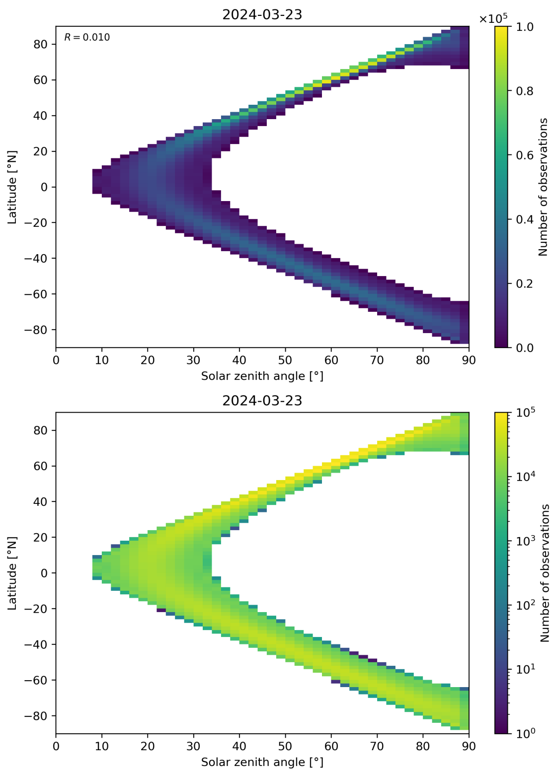
Figure 44: Scatter density plot of “Solar zenith angle” against “Latitude” for 2024-03-23 to 2024-03-24.
