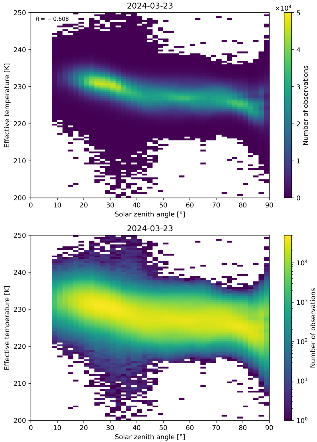
Figure 45: Scatter density plot of “Solar zenith angle” against “Effective temperature” for 2024-03-23 to 2024-03-24.
