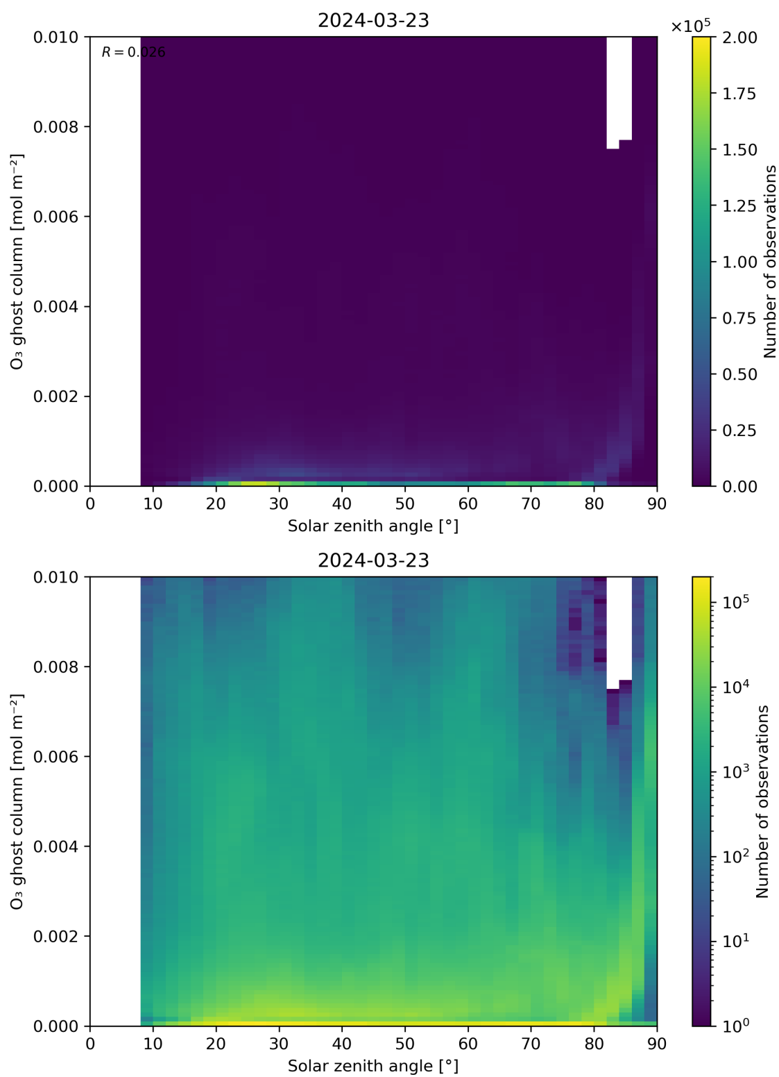
Figure 46: Scatter density plot of “Solar zenith angle” against “O 3 ghost column” for 2024-03-23 to 2024-03-24.
