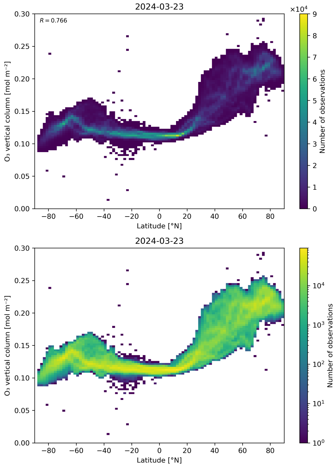
Figure 36: Scatter density plot of “Latitude” against “O 3 vertical column” for 2024-03-23 to 2024-03-24.
