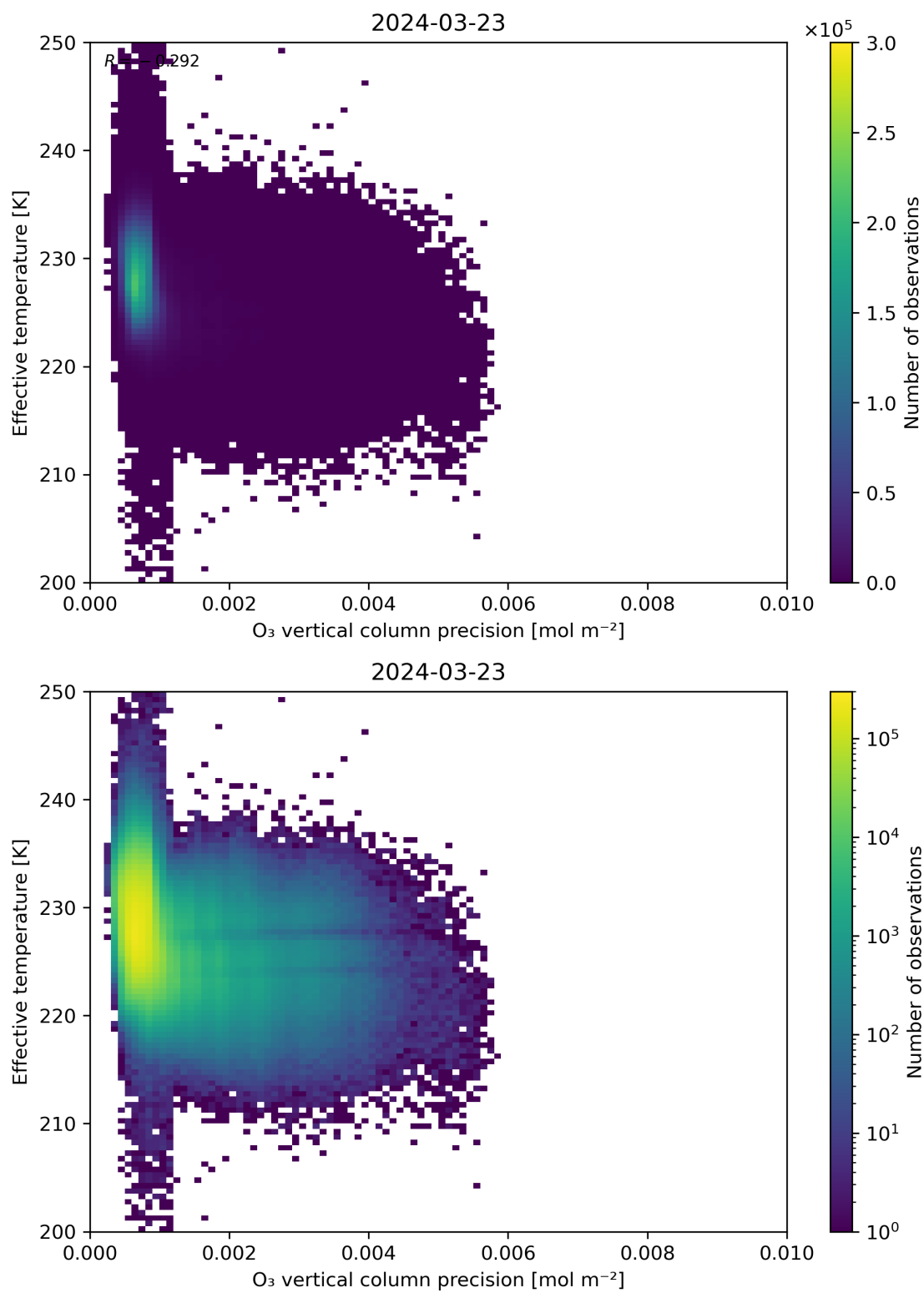
Figure 42: Scatter density plot of “O 3 vertical column precision” against “Effective temperature” for 2024-03-23 to 2024-03-24.
