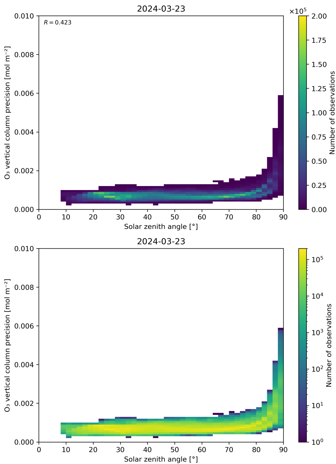
Figure 48: Scatter density plot of “Solar zenith angle” against “O 3 vertical column precision” for 2024-03-23 to 2024-03-24.
