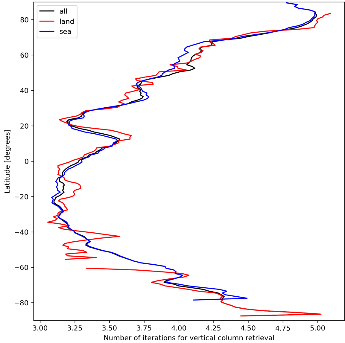
Figure 19: Zonal average of “Number of iterations for vertical column retrieval” for 2024-03-23 to 2024-03-24.
