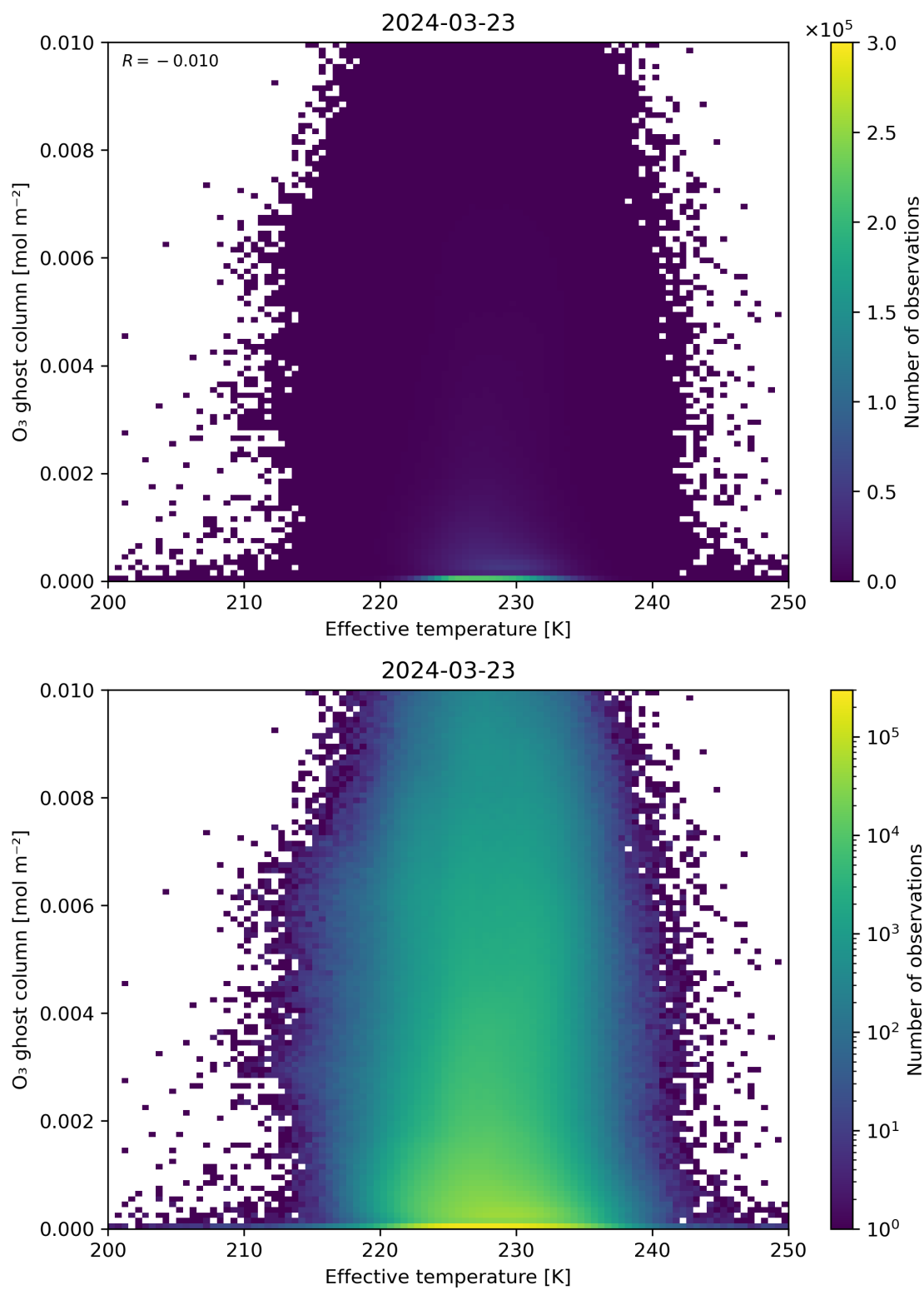
Figure 38: Scatter density plot of “Effective temperature” against “O 3 ghost column” for 2024-03-23 to 2024-03-24.
