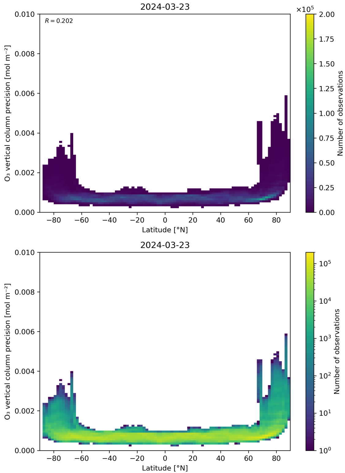
Figure 37: Scatter density plot of “Latitude” against “O 3 vertical column precision” for 2024-03-23 to 2024-03-24.
