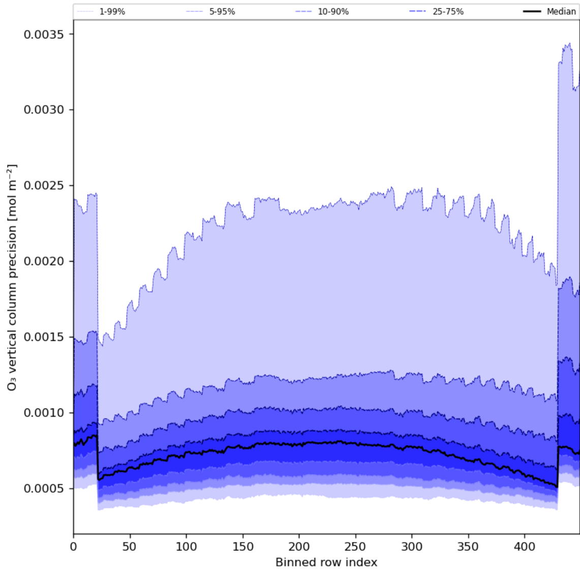
Figure 29: Along track statistics of “O 3 vertical column precision” for 2024-03-23 to 2024-03-24
