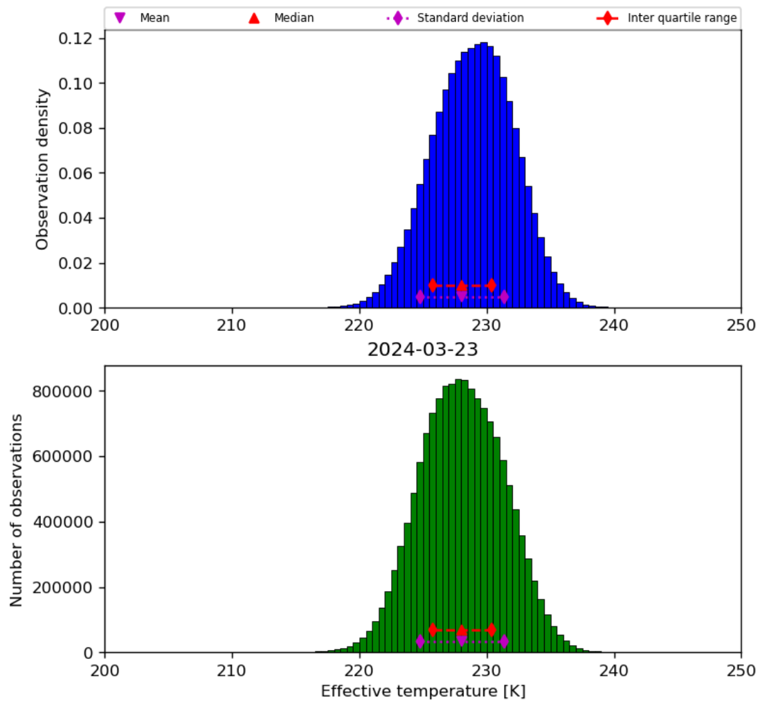
Figure 24: Histogram of “Effective temperature” for 2024-03-23 to 2024-03-24
