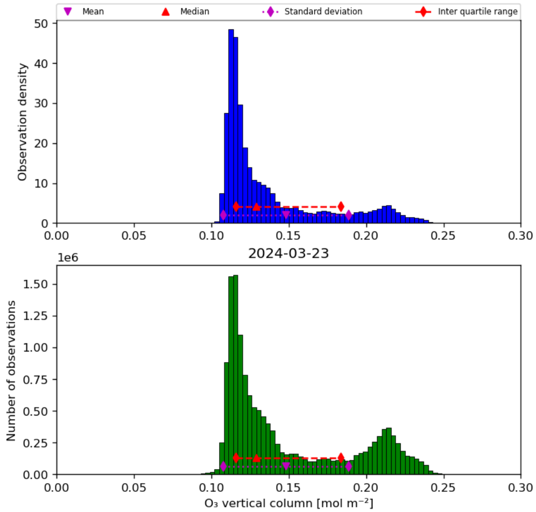
Figure 21: Histogram of “O 3 vertical column” for 2024-03-23 to 2024-03-24
