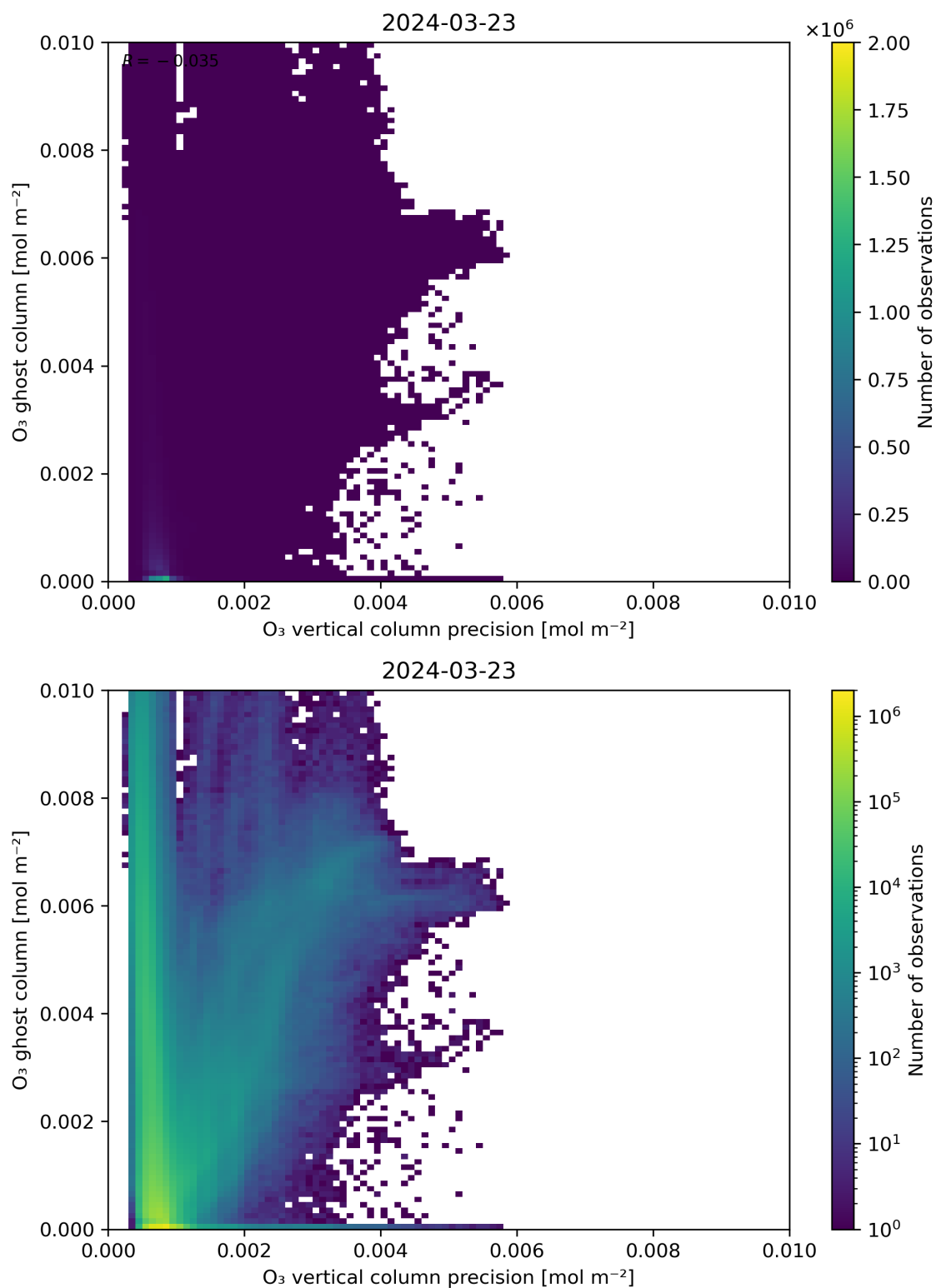
Figure 43: Scatter density plot of “ O_3 vertical column precision” against “ O_3 ghost column” for 2024-03-23 to 2024-03-24.
