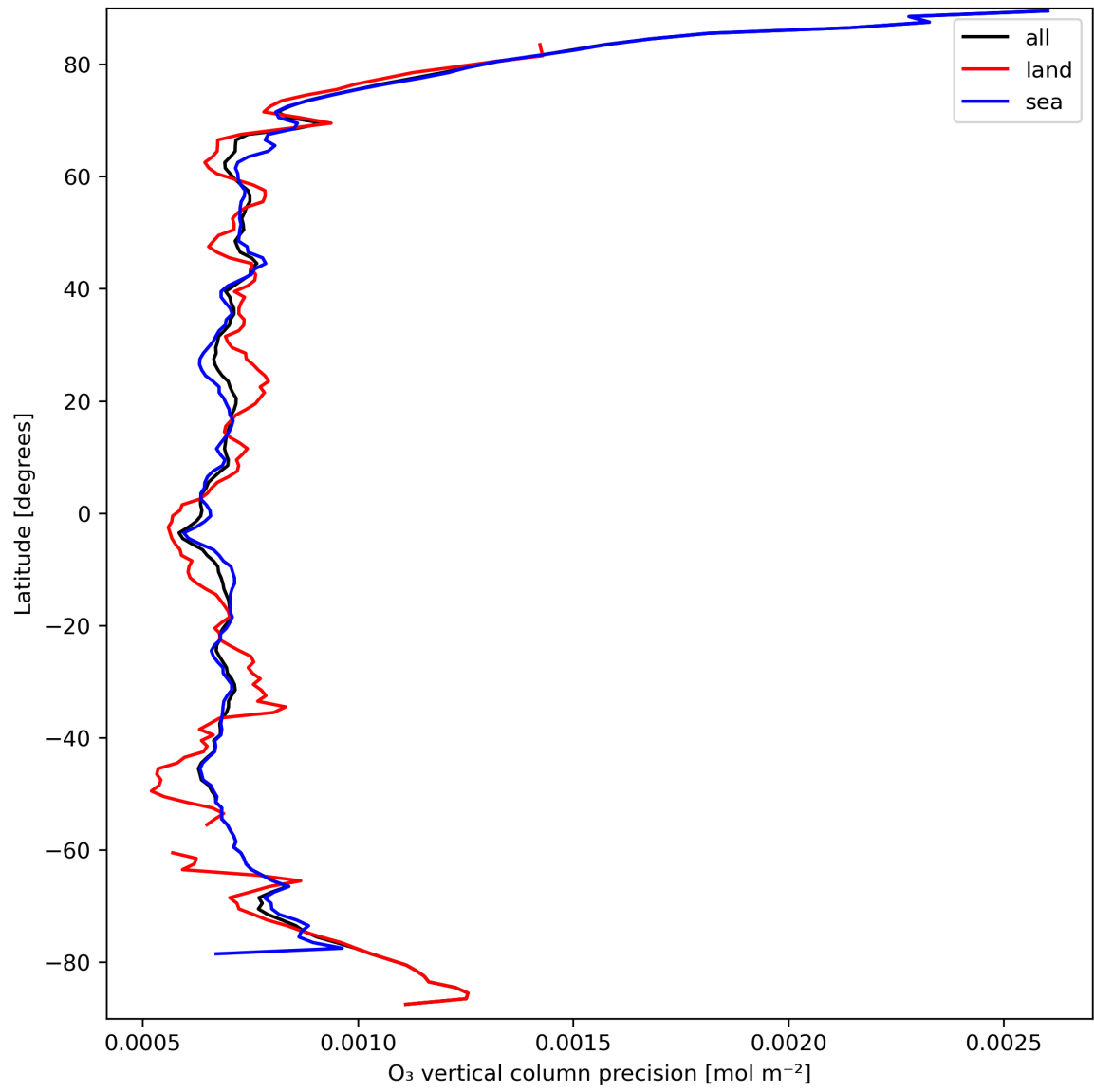
Figure 15: Zonal average of “O 3 vertical column precision” for 2024-03-23 to 2024-03-24.
