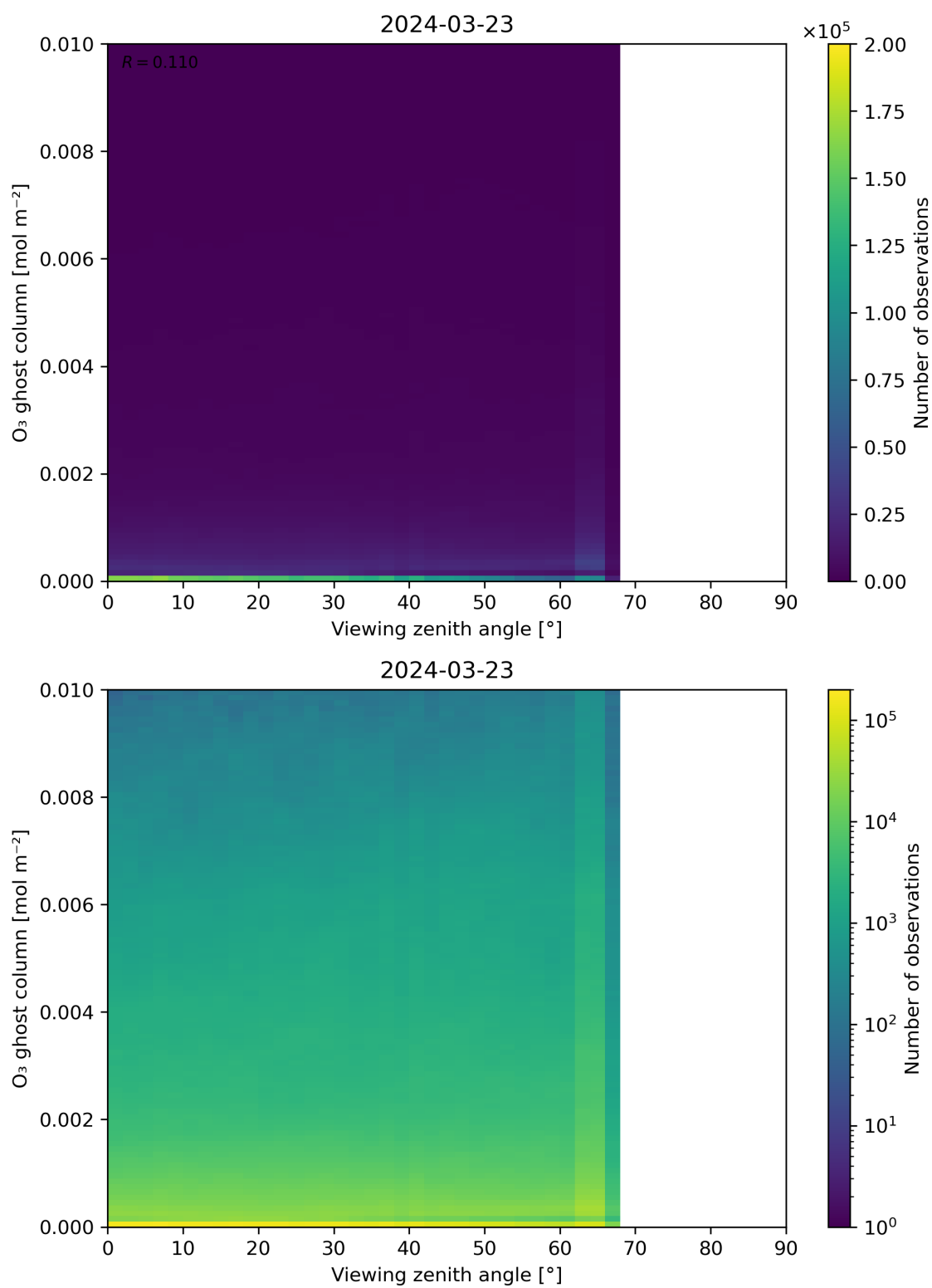
Figure 51: Scatter density plot of “Viewing zenith angle” against “O 3 ghost column” for 2024-03-23 to 2024-03-24.
