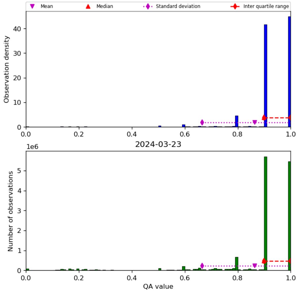
Figure 20: Histogram of “QA value” for 2024-03-23 to 2024-03-24
