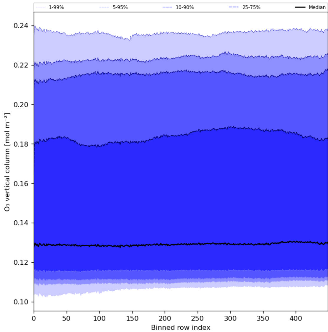
Figure 28: Along track statistics of “O 3 vertical column” for 2024-03-23 to 2024-03-24
