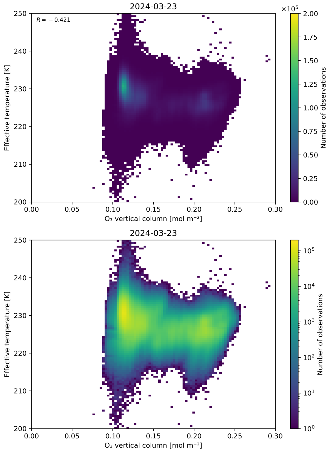
Figure 39: Scatter density plot of “O 3 vertical column” against “Effective temperature” for 2024-03-23 to 2024-03-24.
