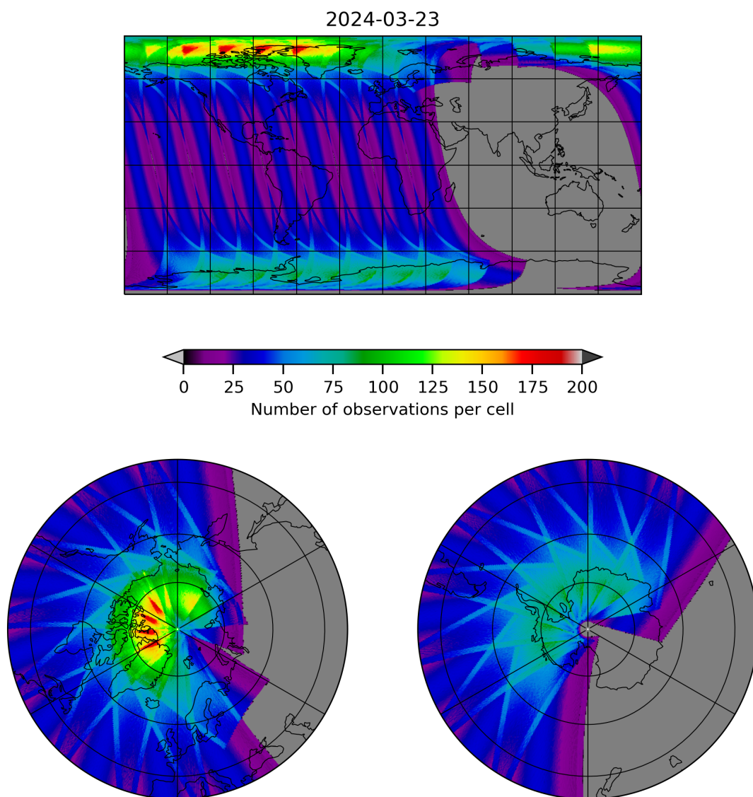
Figure 12: Map of the number of observations for 2024-03-23 to 2024-03-24
