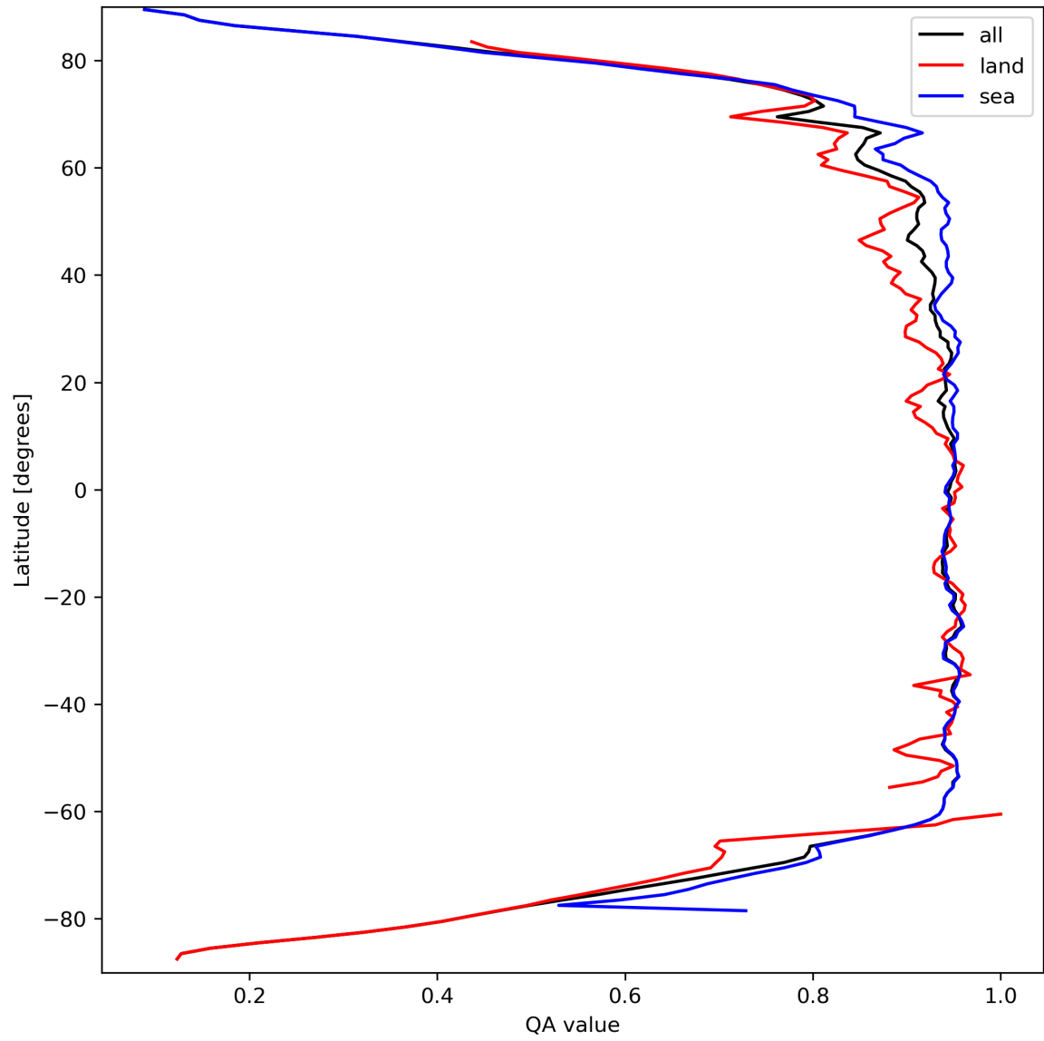
Figure 13: Zonal average of “QA value” for 2024-03-23 to 2024-03-24.
