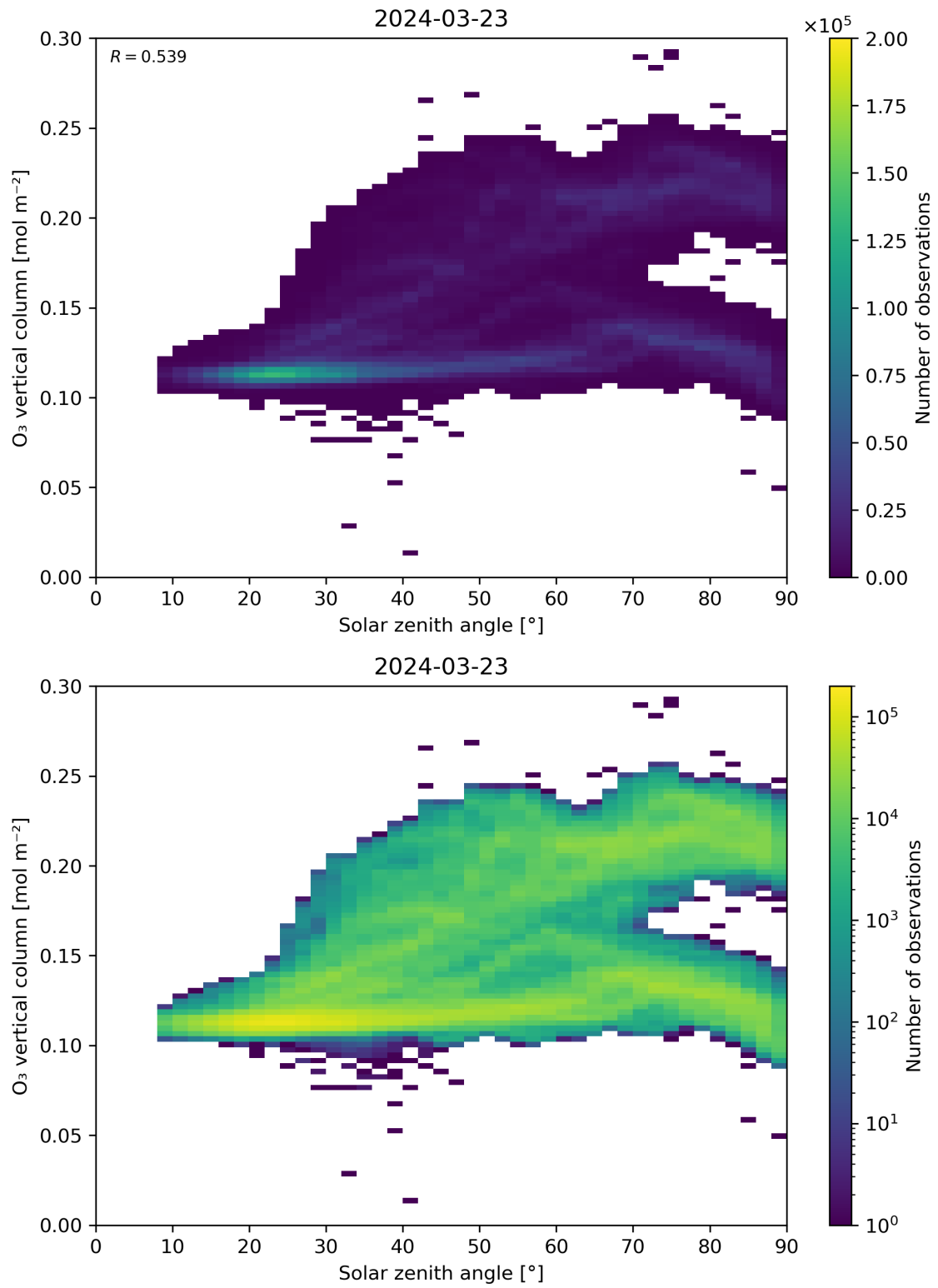
Figure 47: Scatter density plot of “Solar zenith angle” against “O 3 vertical column” for 2024-03-23 to 2024-03-24.
