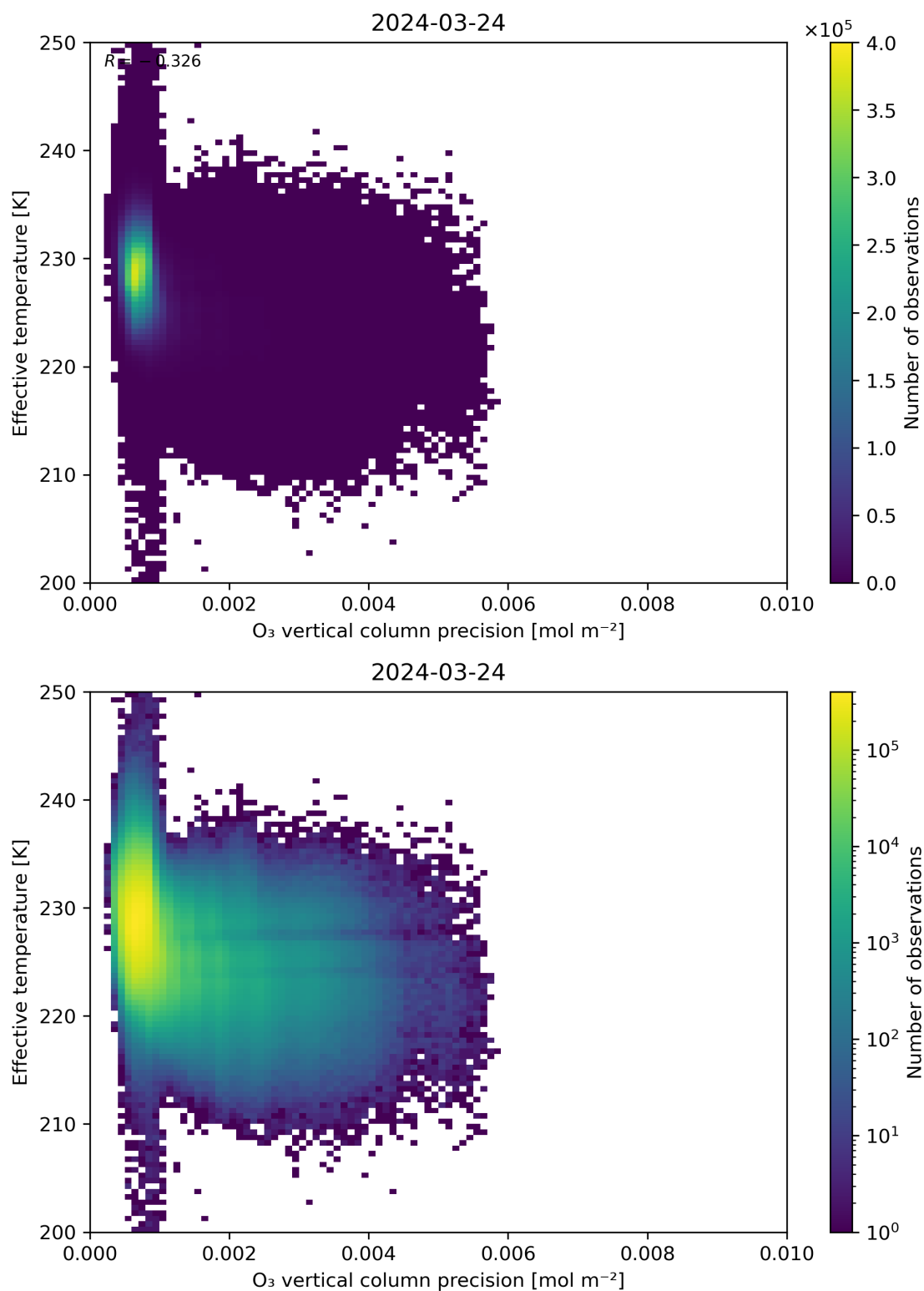
Figure 42: Scatter density plot of “O 3 vertical column precision” against “Effective temperature” for 2024-03-23 to 2024-03-25.
