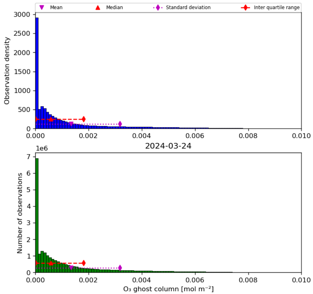
Figure 25: Histogram of “O 3 ghost column” for 2024-03-23 to 2024-03-25
