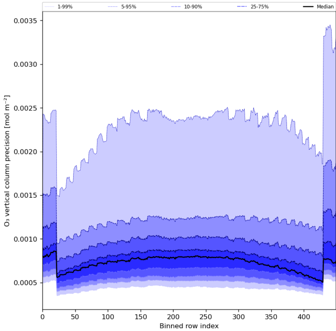
Figure 29: Along track statistics of “O 3 vertical column precision” for 2024-03-23 to 2024-03-25
