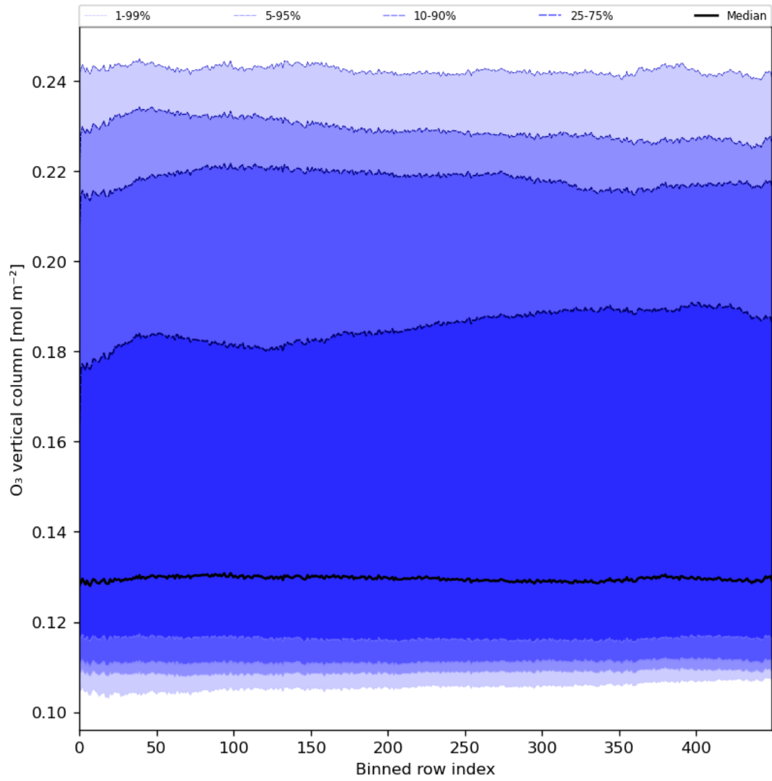
Figure 28: Along track statistics of "O 3 vertical column" for 2024-03-23 to 2024-03-25
