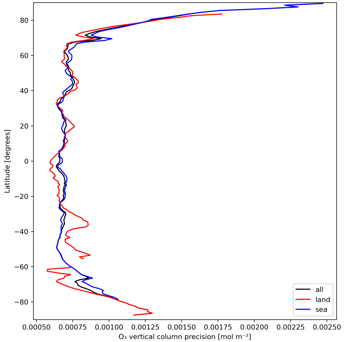
Figure 15: Zonal average of “O 3 vertical column precision” for 2024-03-23 to 2024-03-25.
