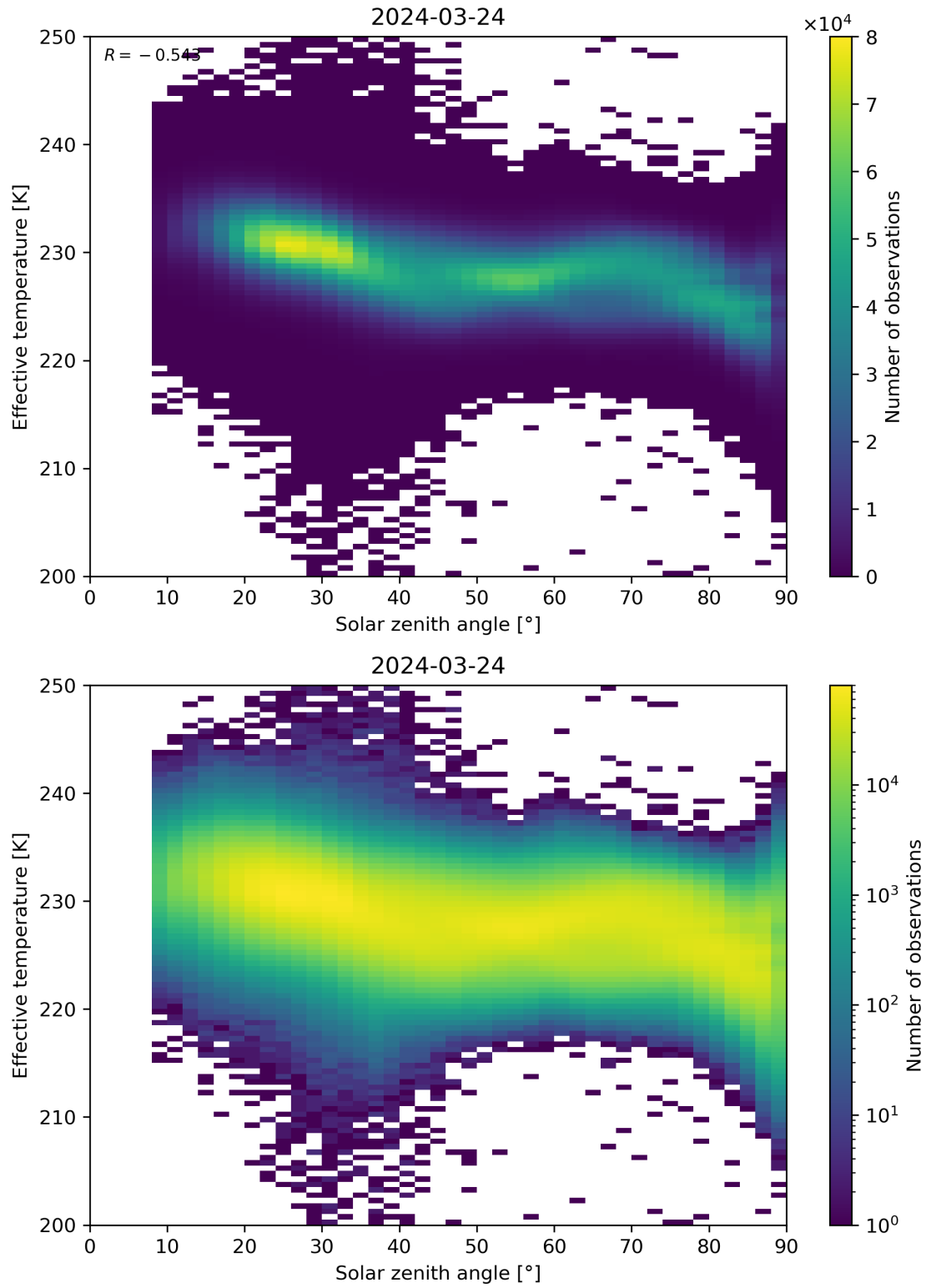
Figure 45: Scatter density plot of “Solar zenith angle” against “Effective temperature” for 2024-03-23 to 2024-03-25.
