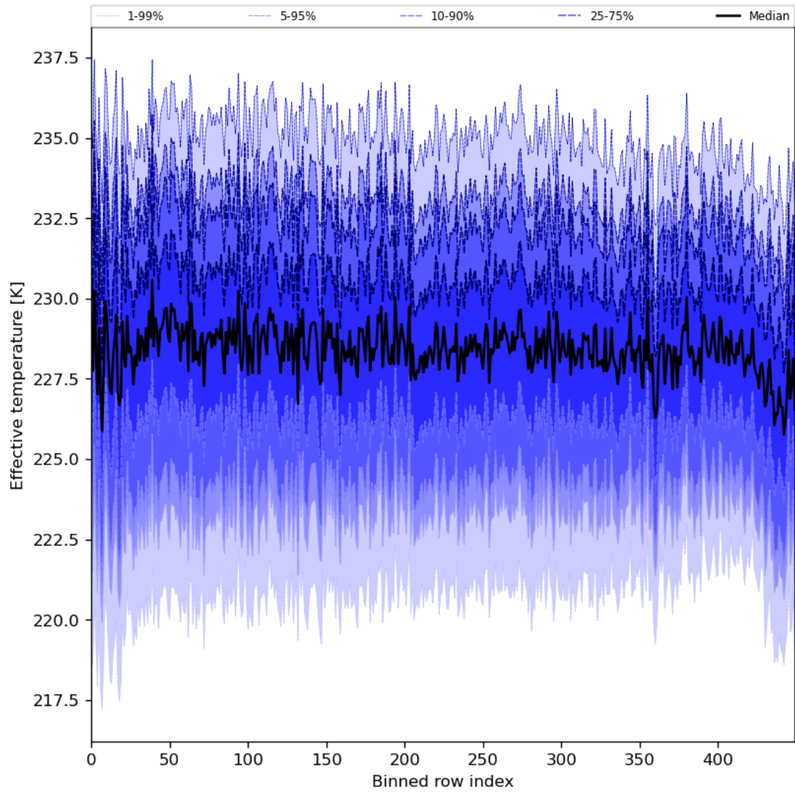
Figure 31: Along track statistics of “Effective temperature” for 2024-03-23 to 2024-03-25
