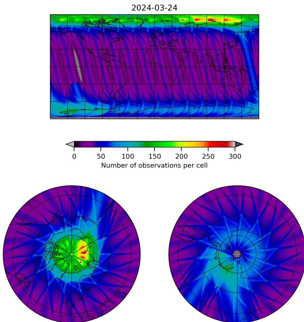
Figure 12: Map of the number of observations for 2024-03-23 to 2024-03-25
