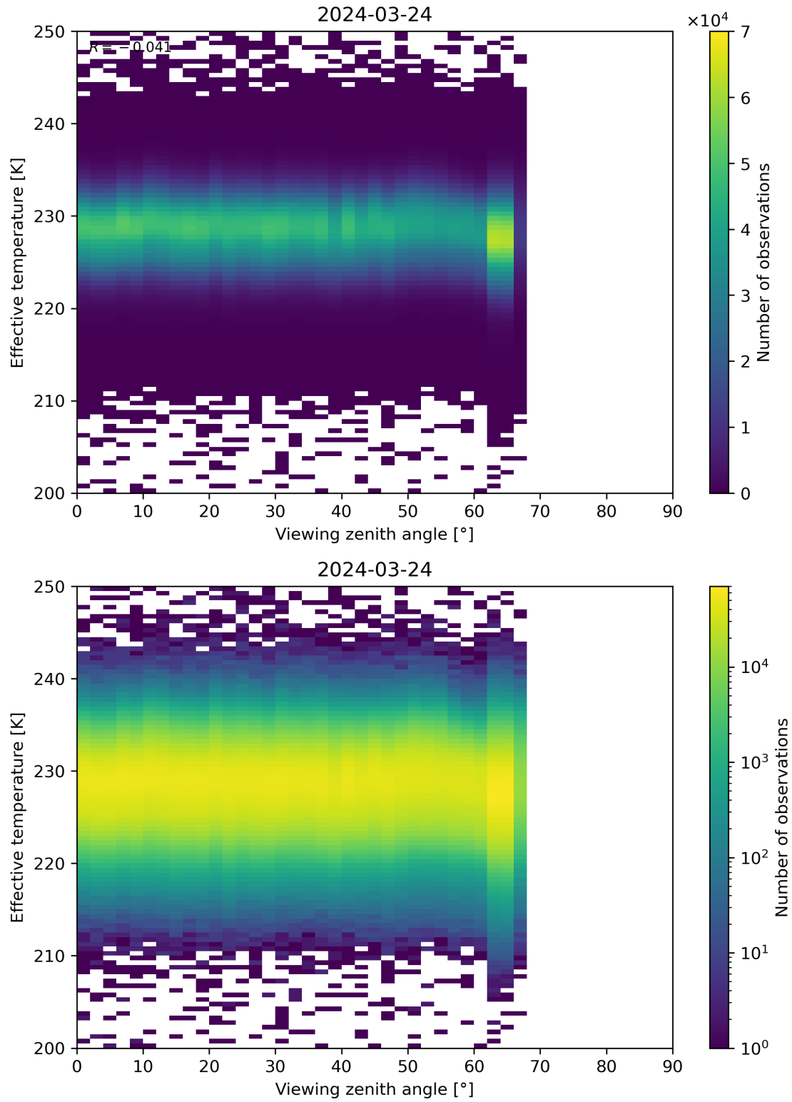
Figure 50: Scatter density plot of “Viewing zenith angle” against “Effective temperature” for 2024-03-23 to 2024-03-25.
