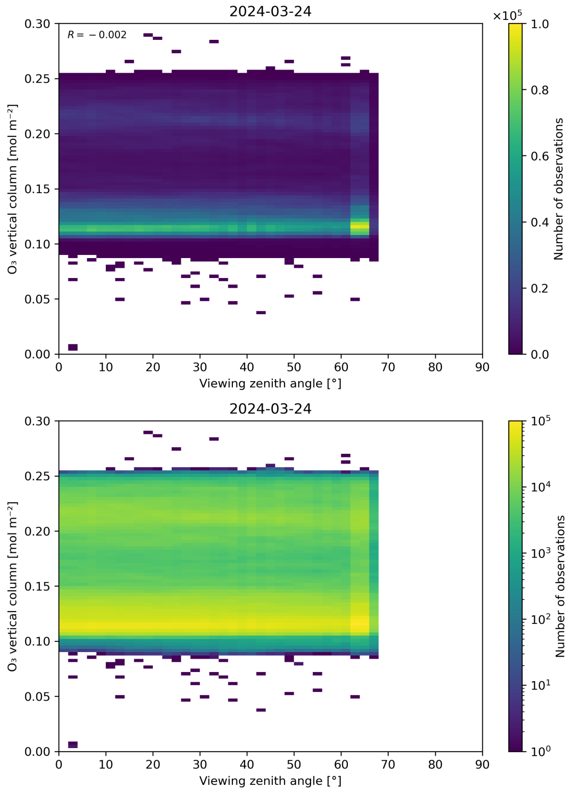
Figure 52: Scatter density plot of “Viewing zenith angle” against “O 3 vertical column” for 2024-03-23 to 2024-03-25.
