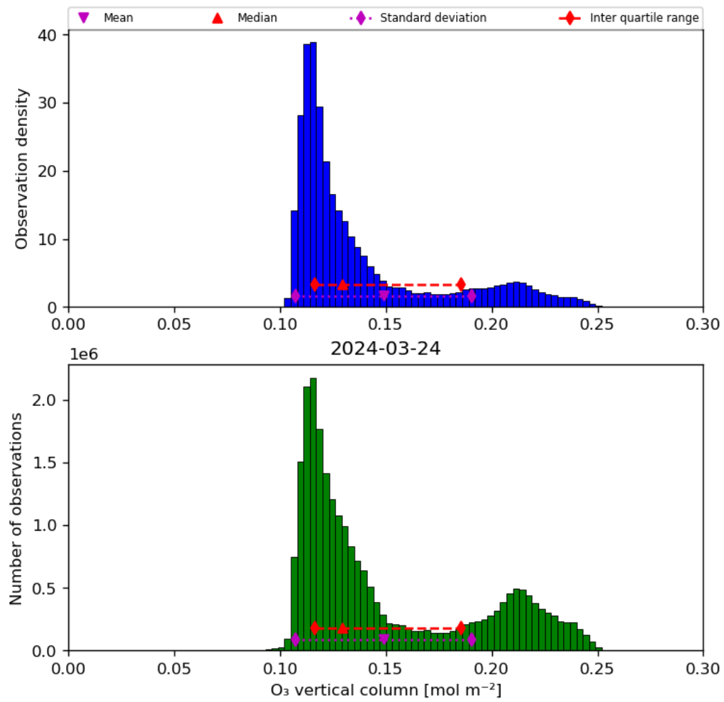
Figure 21: Histogram of “O 3 vertical column” for 2024-03-23 to 2024-03-25
