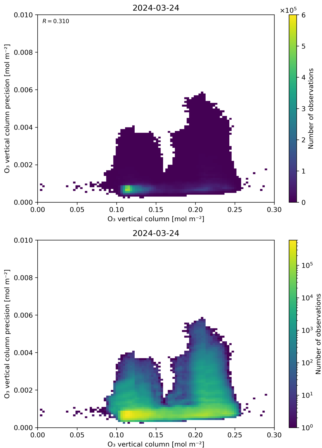
Figure 41: Scatter density plot of “O 3 vertical column” against “O 3 vertical column precision” for 2024-03-23 to 2024-03-25.
