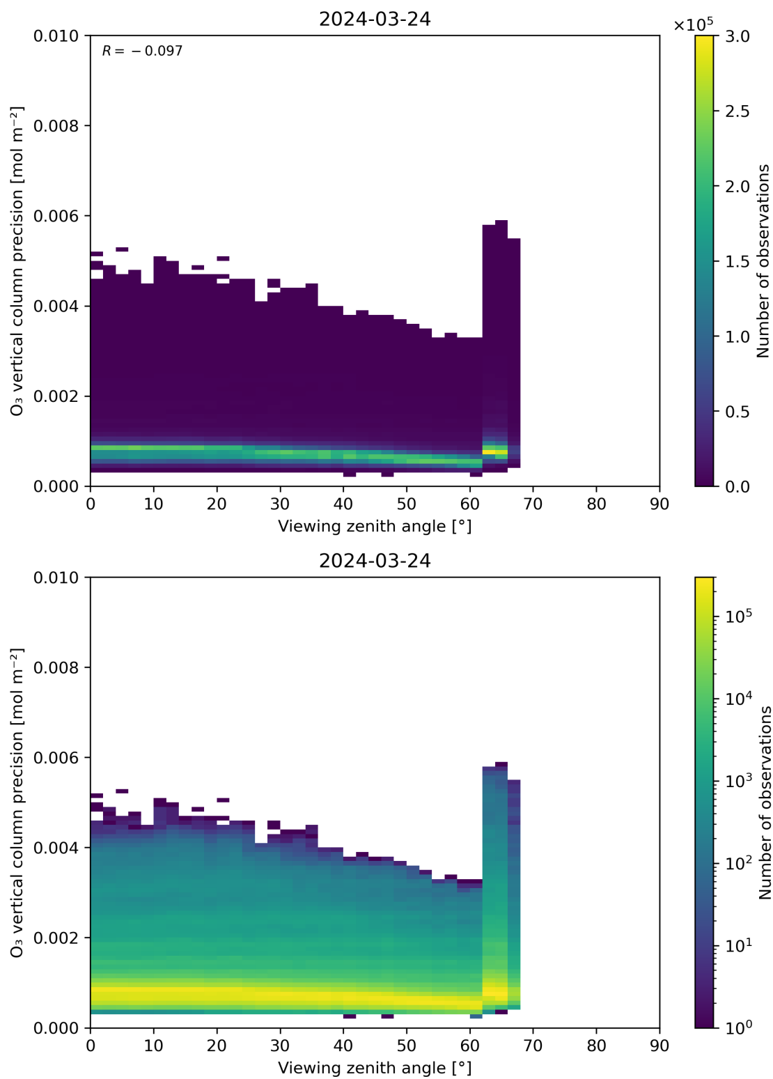
Figure 53: Scatter density plot of “Viewing zenith angle” against “O 3 vertical column precision” for 2024-03-23 to 2024-03-25.
