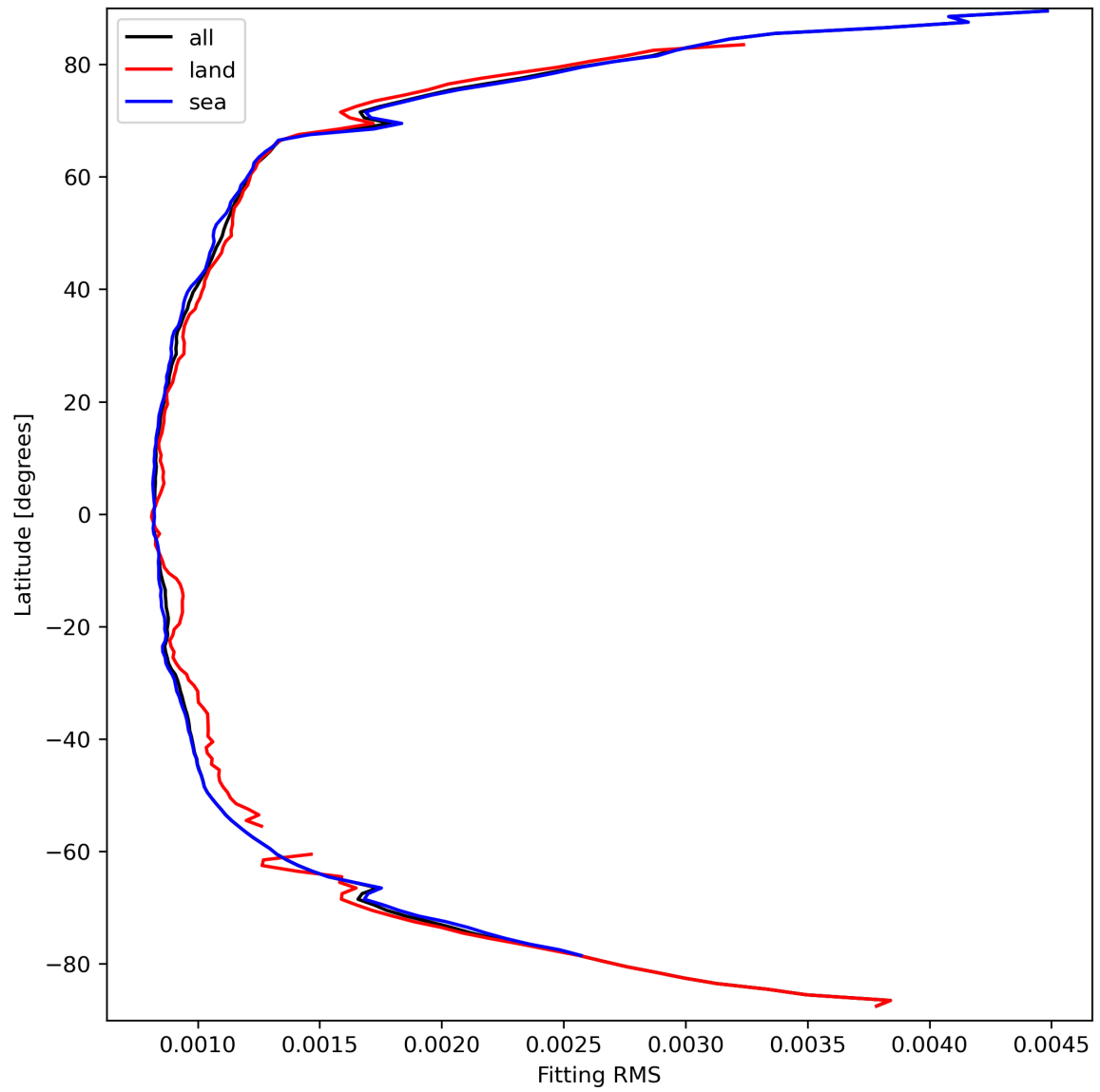
Figure 16: Zonal average of “Fitting RMS” for 2024-03-23 to 2024-03-25.
