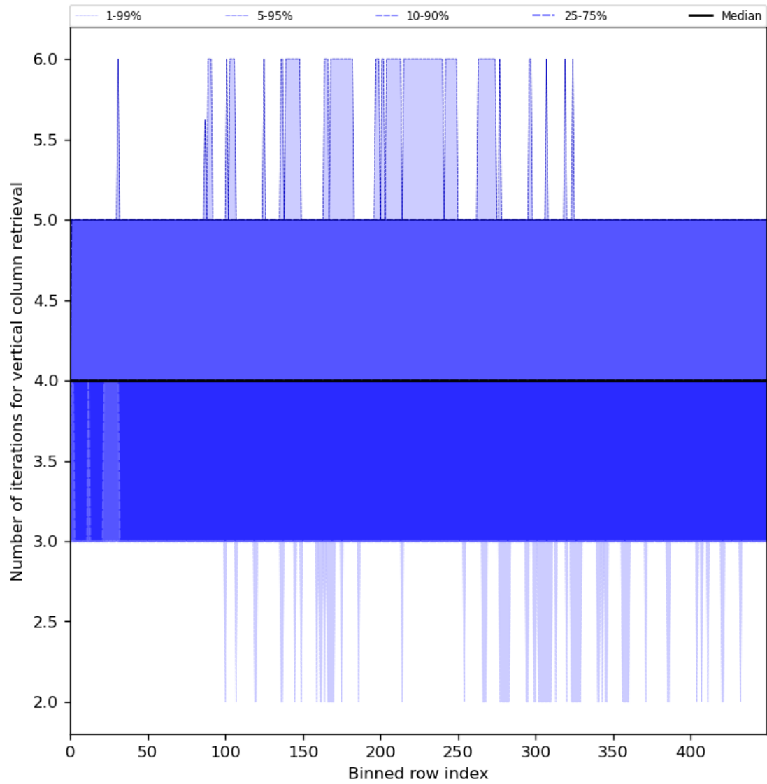
Figure 33: Along track statistics of “Number of iterations for vertical column retrieval” for 2024-03-23 to 2024-03-25
