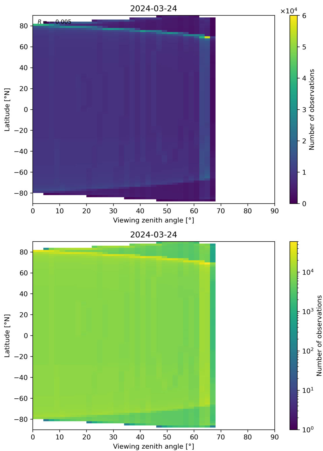
Figure 49: Scatter density plot of “Viewing zenith angle” against “Latitude” for 2024-03-23 to 2024-03-25.
