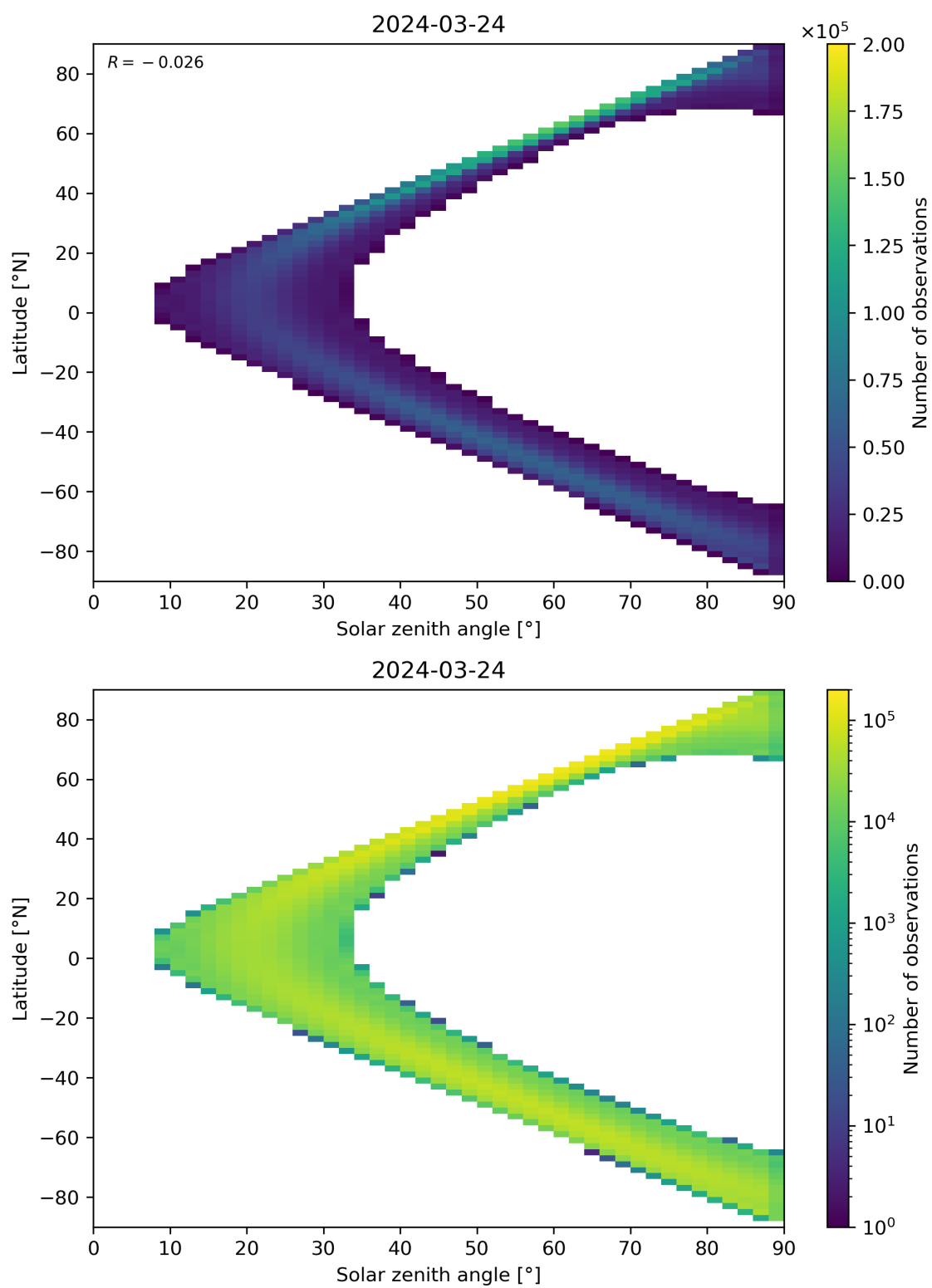
Figure 44: Scatter density plot of “Solar zenith angle” against “Latitude” for 2024-03-23 to 2024-03-25.
