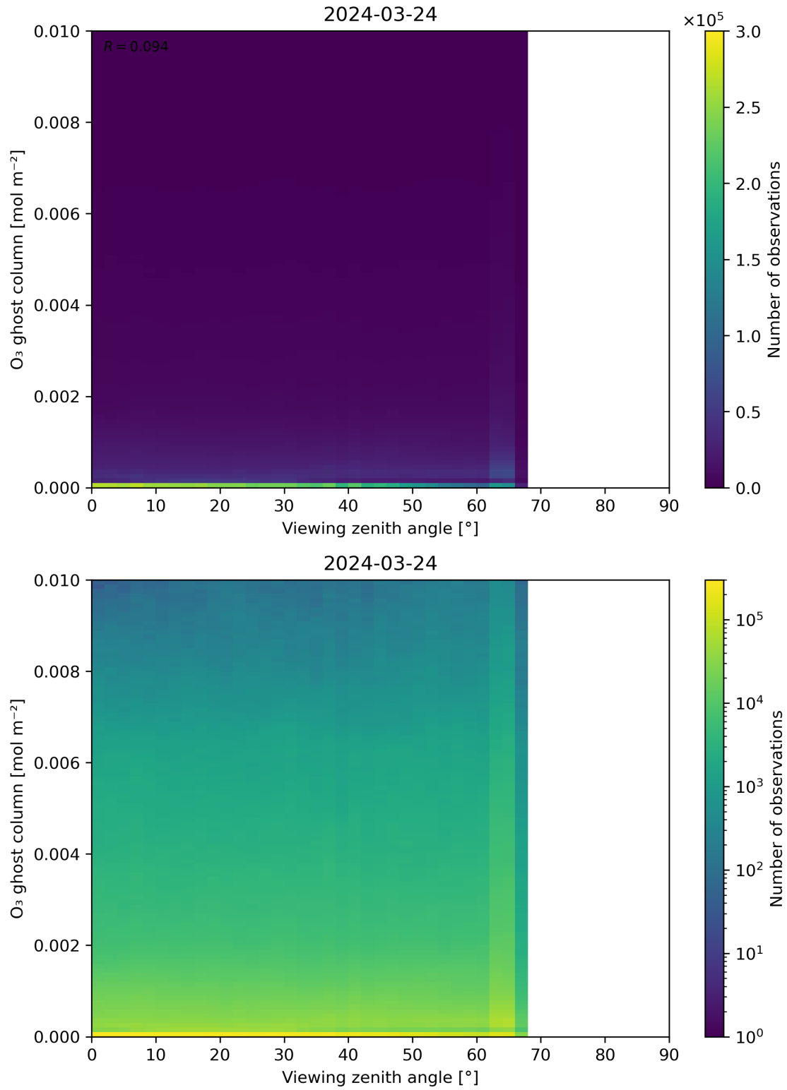
Figure 51: Scatter density plot of “Viewing zenith angle” against “O 3 ghost column” for 2024-03-23 to 2024-03-25.
