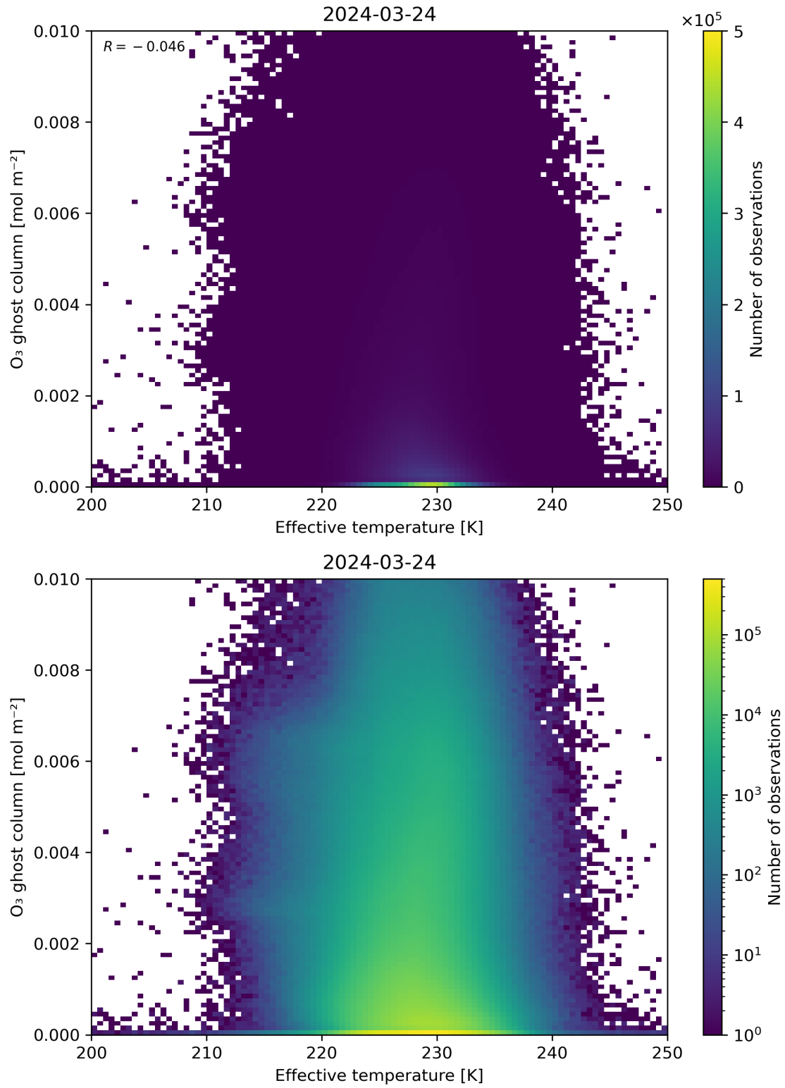
Figure 38: Scatter density plot of “Effective temperature” against “O 3 ghost column” for 2024-03-23 to 2024-03-25.
