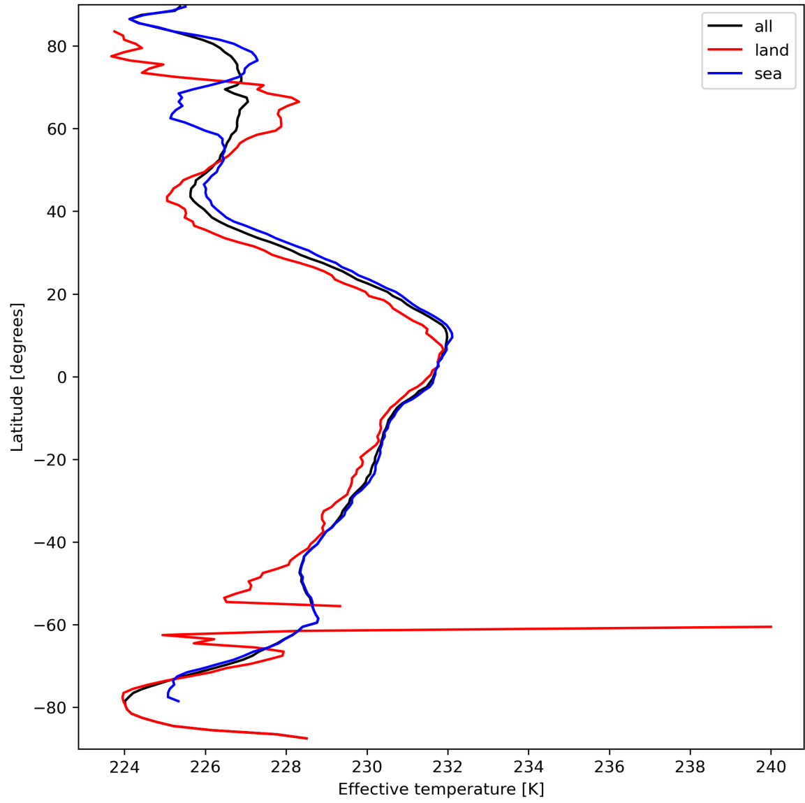
Figure 17: Zonal average of “Effective temperature” for 2024-03-23 to 2024-03-25.
