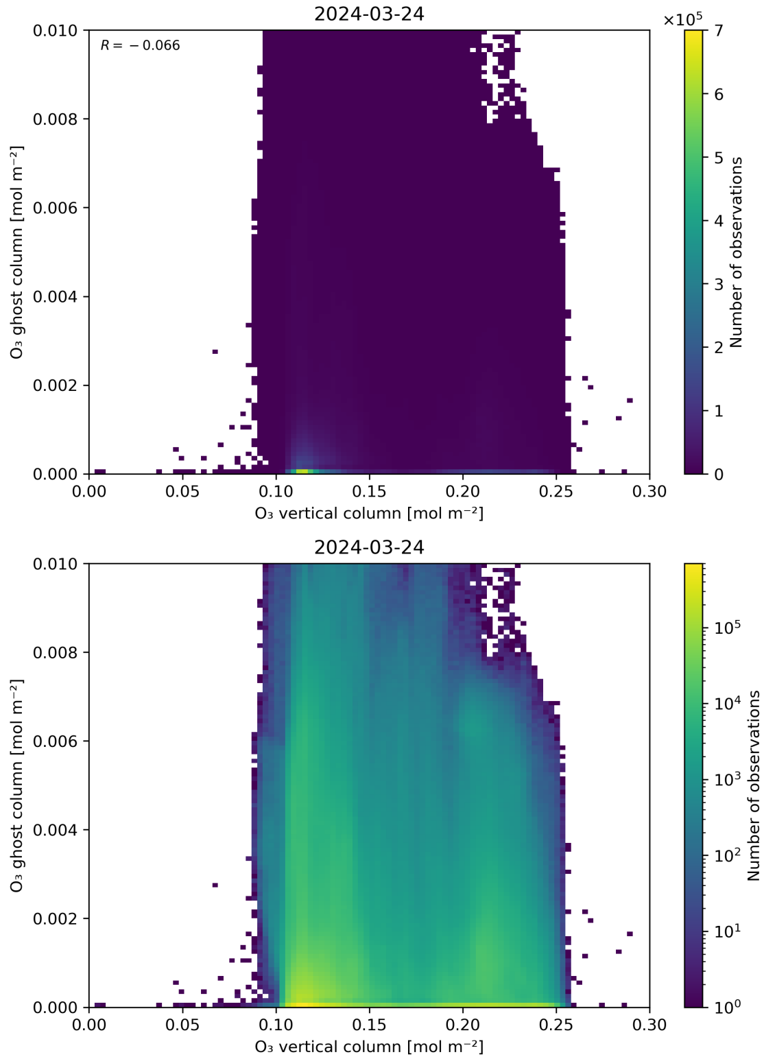
Figure 40: Scatter density plot of “O 3 vertical column” against “O 3 ghost column” for 2024-03-23 to 2024-03-25.
