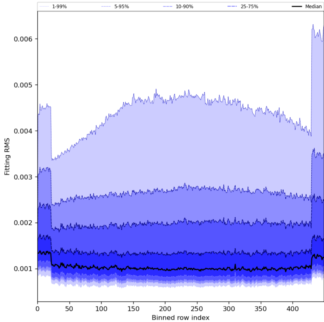
Figure 30: Along track statistics of “Fitting RMS” for 2024-03-23 to 2024-03-25
