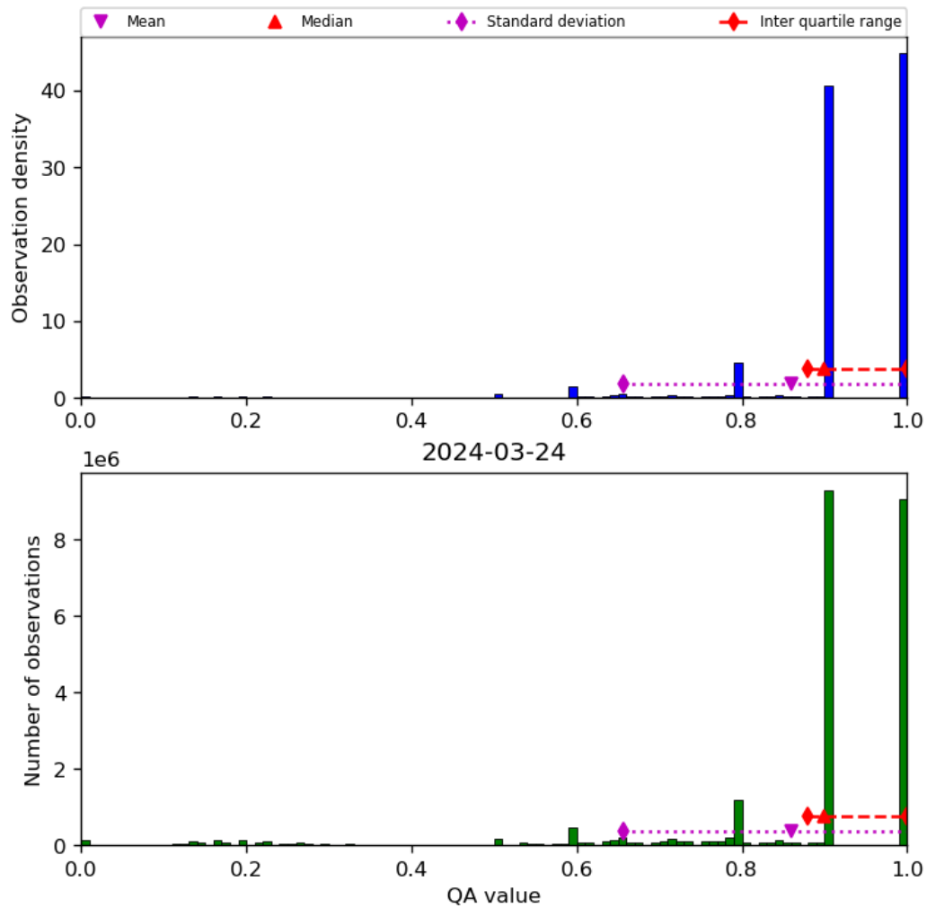
Figure 20: Histogram of “QA value” for 2024-03-23 to 2024-03-25
