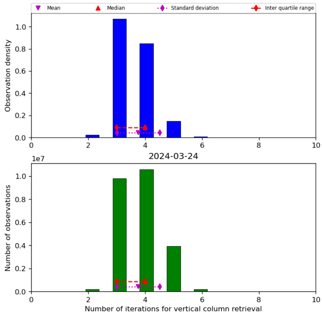
Figure 26: Histogram of “Number of iterations for vertical column retrieval” for 2024-03-23 to 2024-03-25
