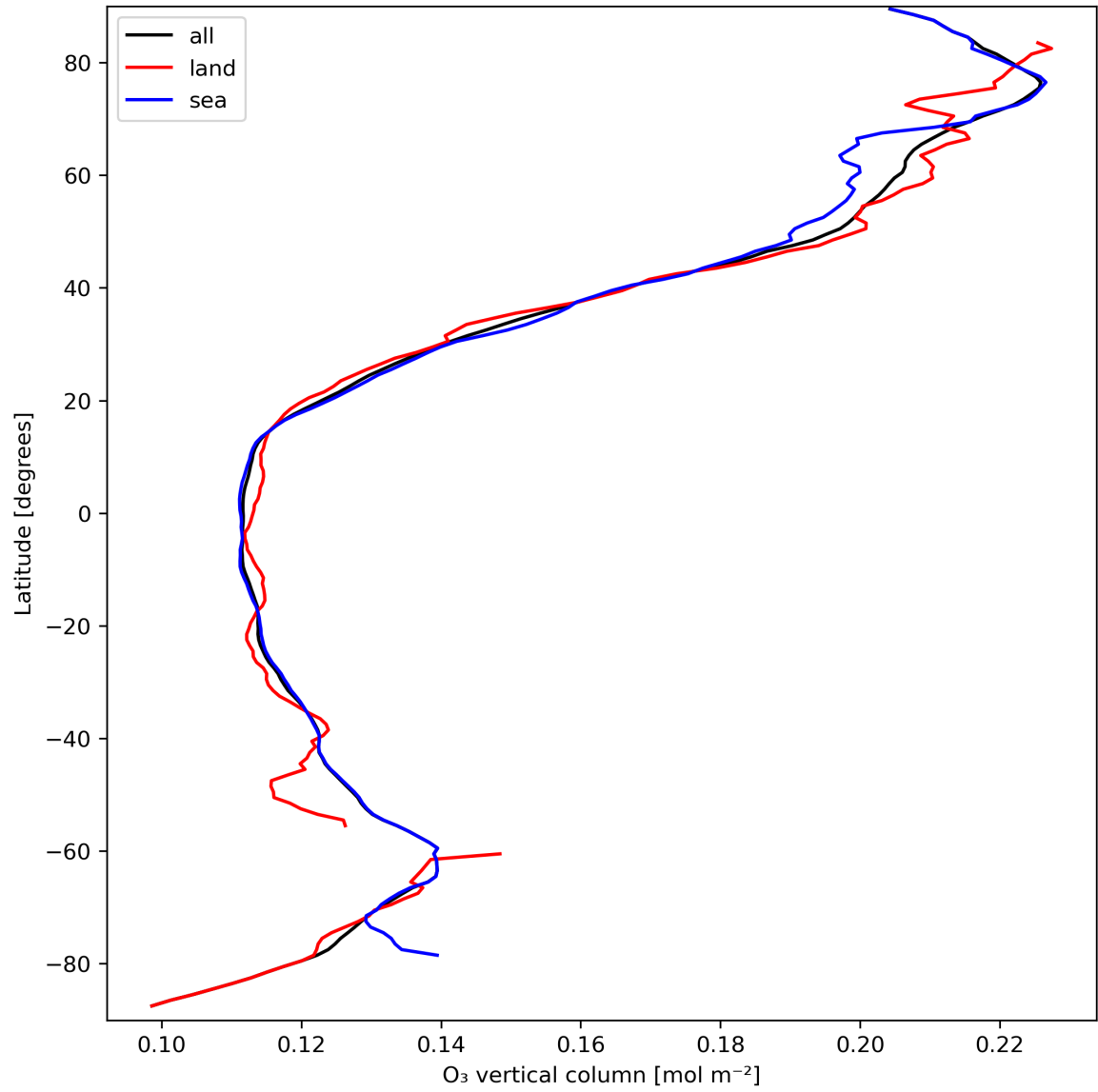
Figure 14: Zonal average of “O 3 vertical column” for 2024-03-23 to 2024-03-25.
