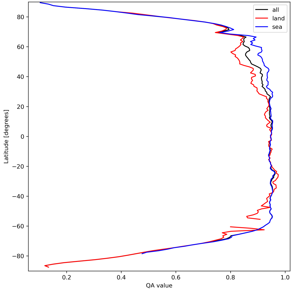
Figure 13: Zonal average of “QA value” for 2024-03-23 to 2024-03-25.
