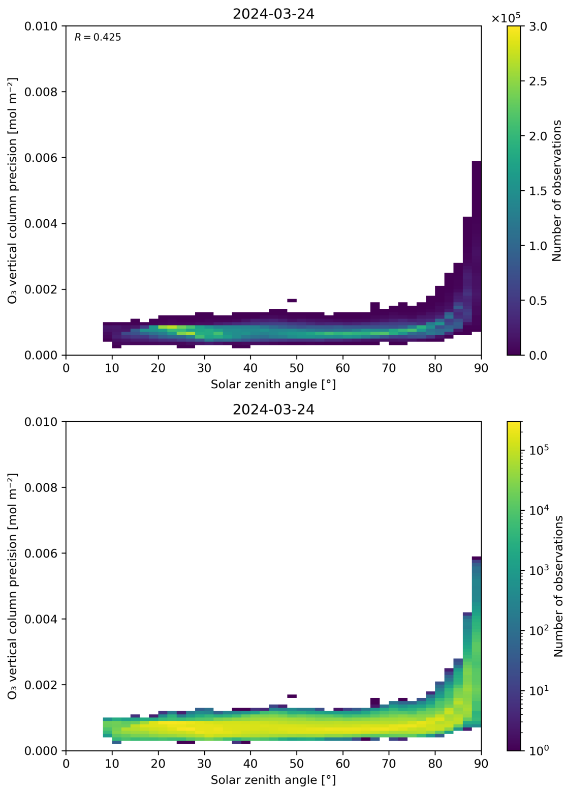
Figure 48: Scatter density plot of “Solar zenith angle” against “O 3 vertical column precision” for 2024-03-23 to 2024-03-25.
