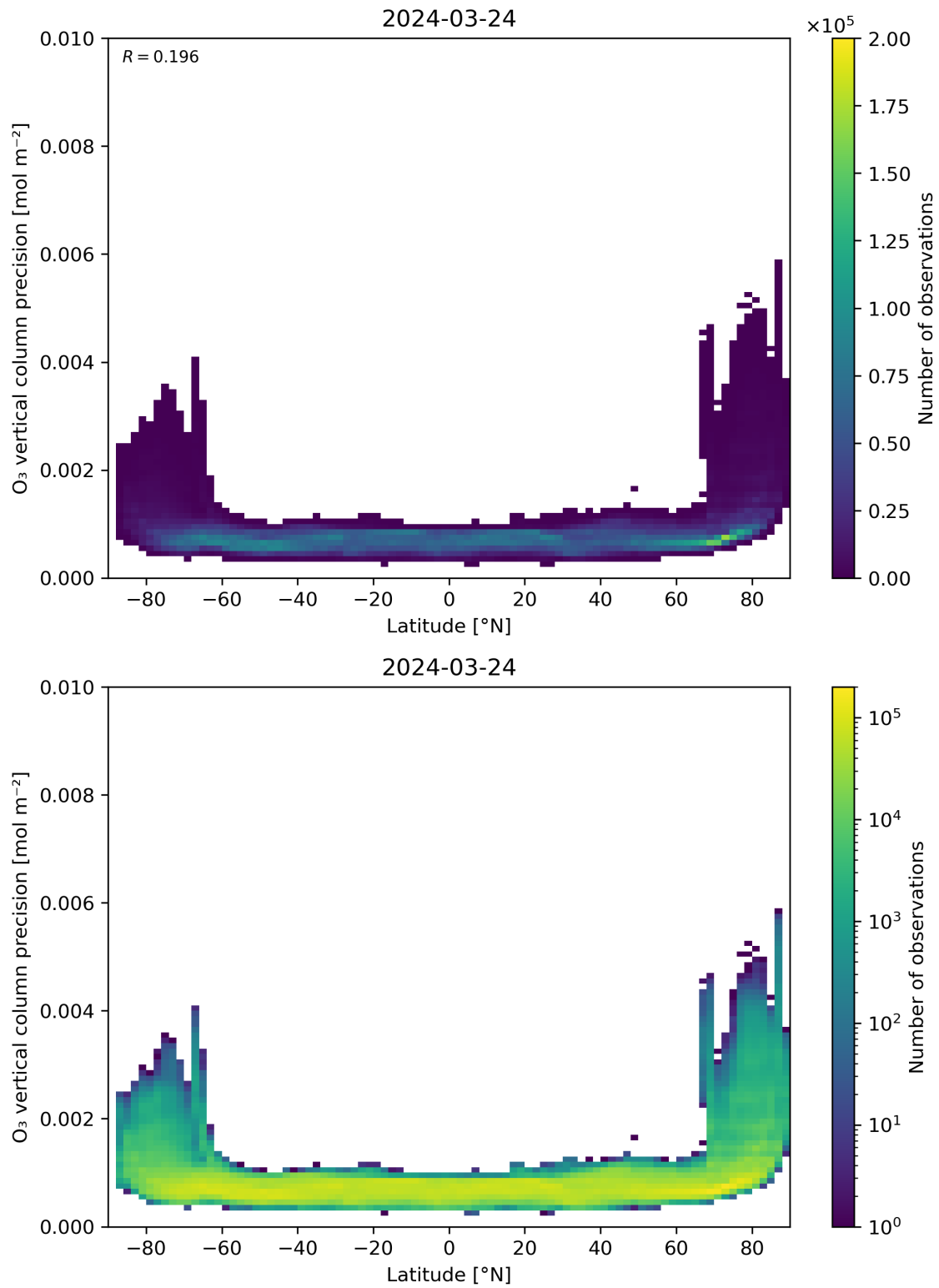
Figure 37: Scatter density plot of “Latitude” against “O 3 vertical column precision” for 2024-03-23 to 2024-03-25.
