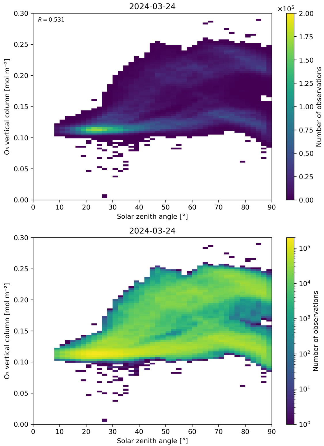
Figure 47: Scatter density plot of “Solar zenith angle” against “O 3 vertical column” for 2024-03-23 to 2024-03-25.
