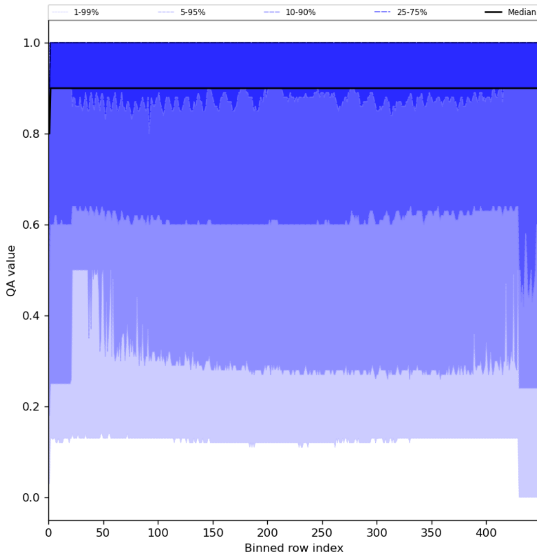
Figure 27: Along track statistics of “QA value” for 2024-03-23 to 2024-03-25
