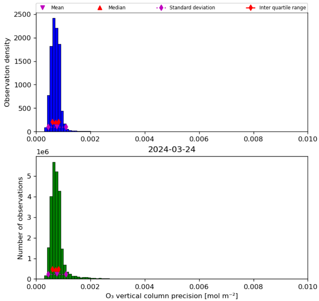
Figure 22: Histogram of “O 3 vertical column precision” for 2024-03-23 to 2024-03-25
