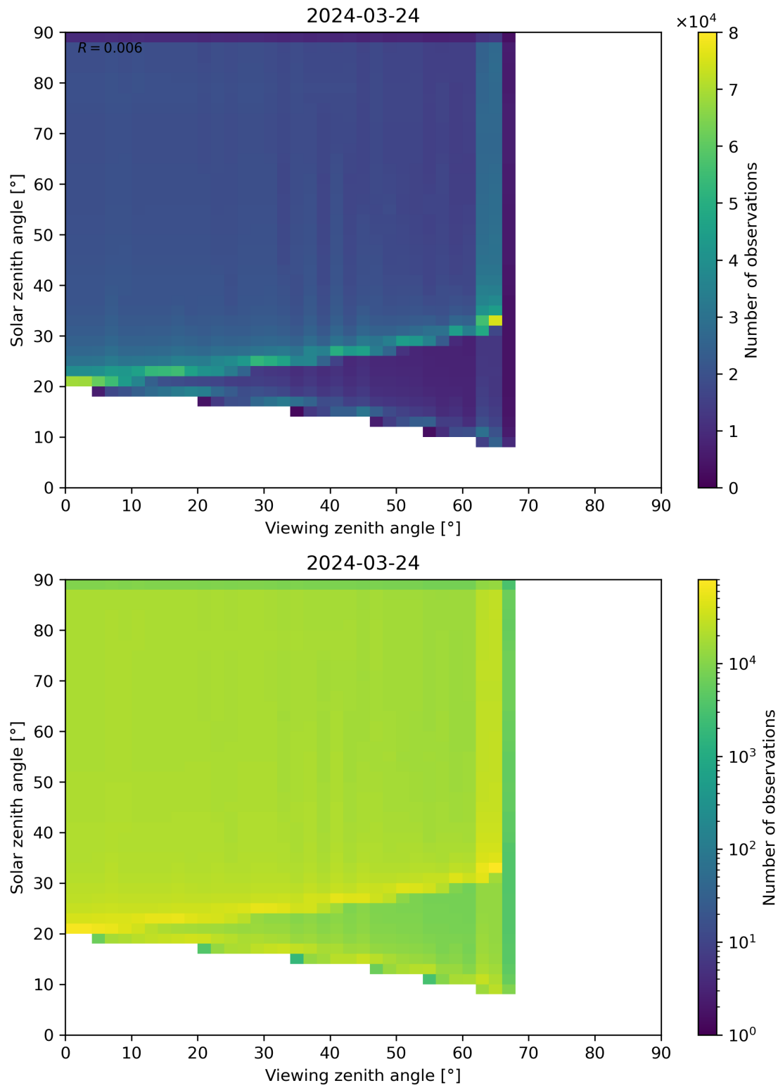
Figure 54: Scatter density plot of “Viewing zenith angle” against “Solar zenith angle” for 2024-03-23 to 2024-03-25.
