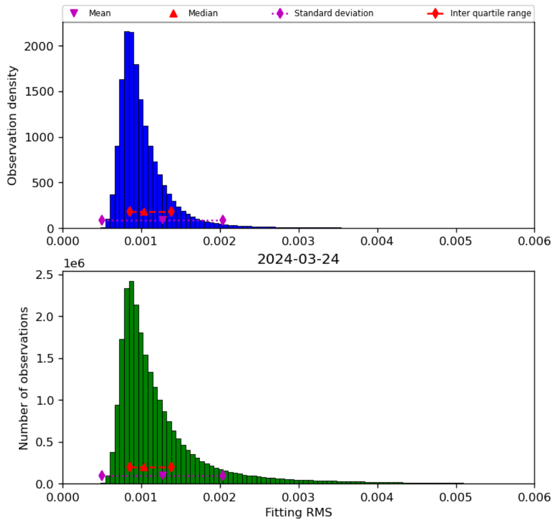
Figure 23: Histogram of “Fitting RMS” for 2024-03-23 to 2024-03-25
