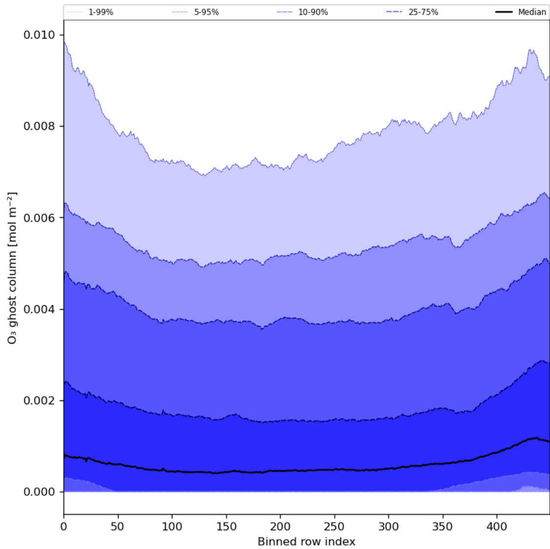
Figure 32: Along track statistics of “O 3 ghost column” for 2024-03-23 to 2024-03-25
