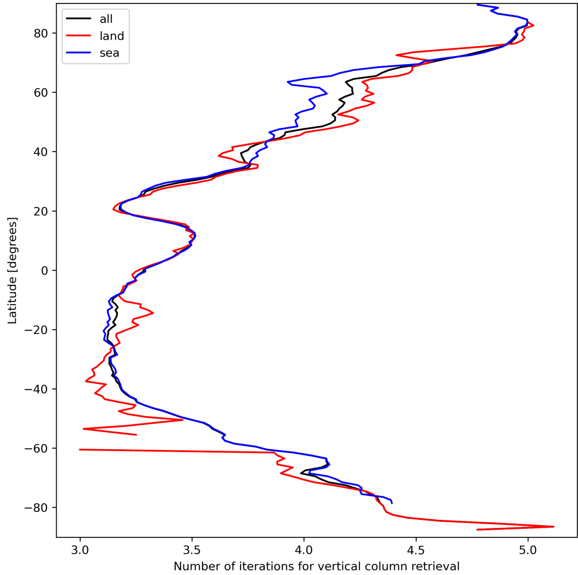
Figure 19: Zonal average of “Number of iterations for vertical column retrieval” for 2024-03-23 to 2024-03-25.
