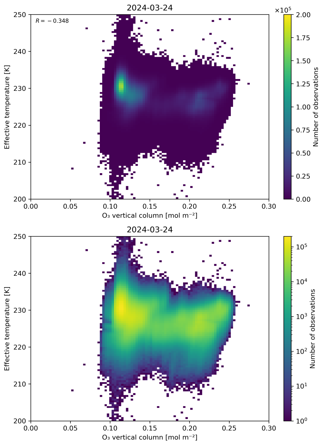
Figure 39: Scatter density plot of “O 3 vertical column” against “Effective temperature” for 2024-03-23 to 2024-03-25.
