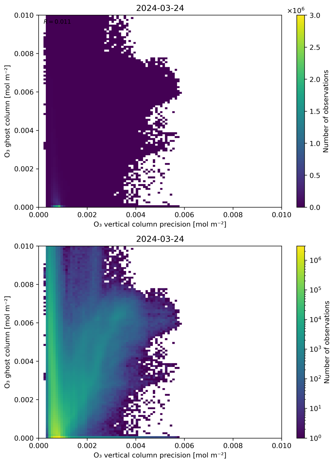
Figure 43: Scatter density plot of “O 3 vertical column precision” against “O 3 ghost column” for 2024-03-23 to 2024-03-25.
