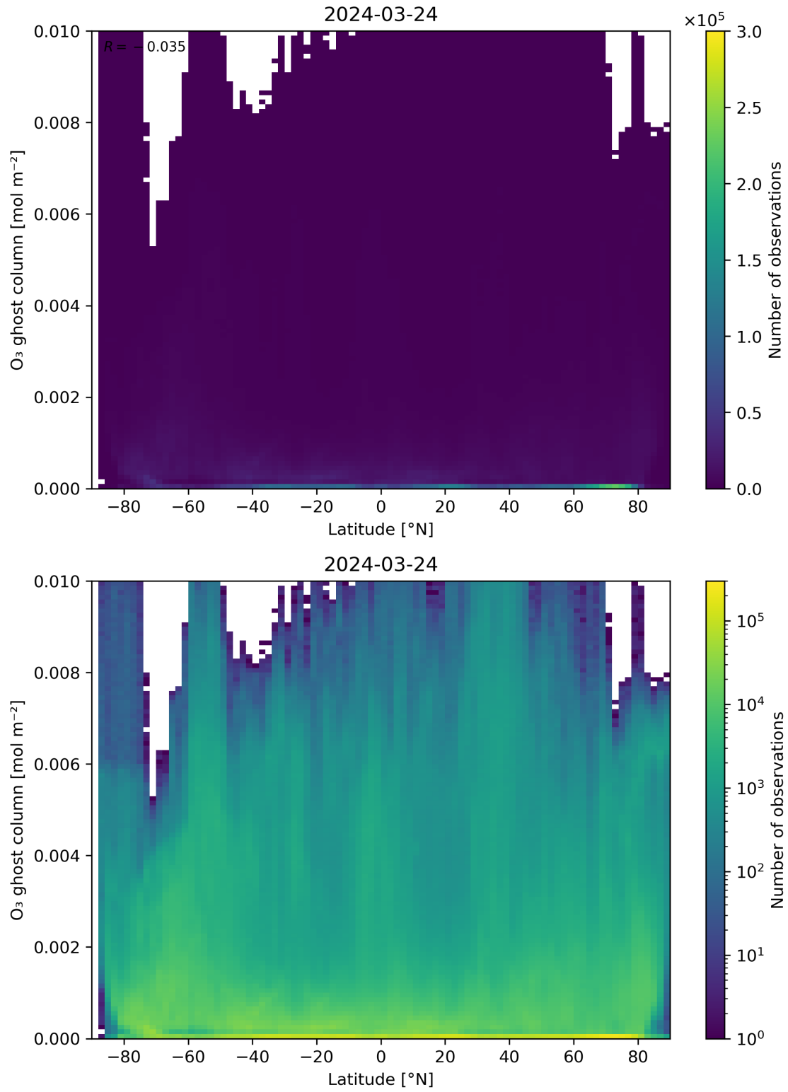
Figure 35: Scatter density plot of “Latitude” against “O 3 ghost column” for 2024-03-23 to 2024-03-25.
