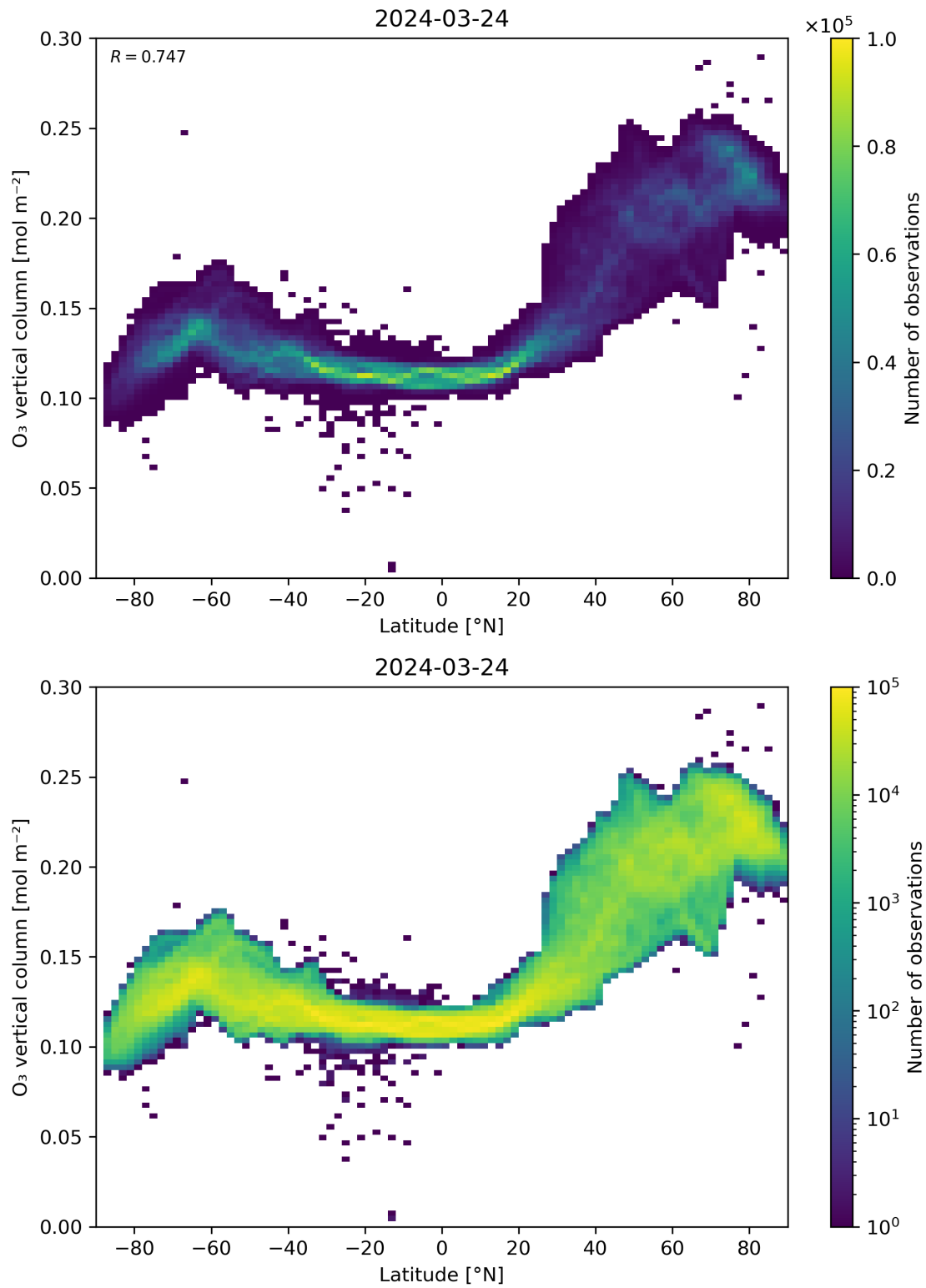
Figure 36: Scatter density plot of “Latitude” against “O 3 vertical column” for 2024-03-23 to 2024-03-25.
