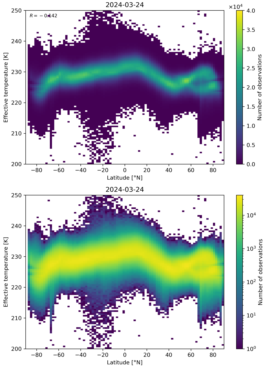
Figure 34: Scatter density plot of “Latitude” against “Effective temperature” for 2024-03-23 to 2024-03-25.
