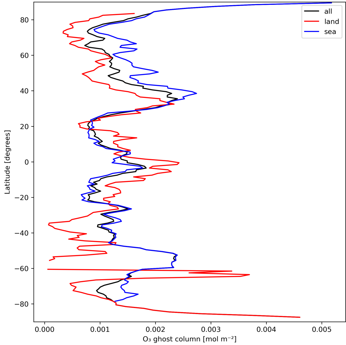
Figure 18: Zonal average of "O 3 ghost column" for 2024-03-23 to 2024-03-25.
