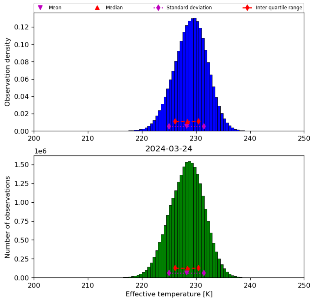
Figure 24: Histogram of “Effective temperature” for 2024-03-23 to 2024-03-25
