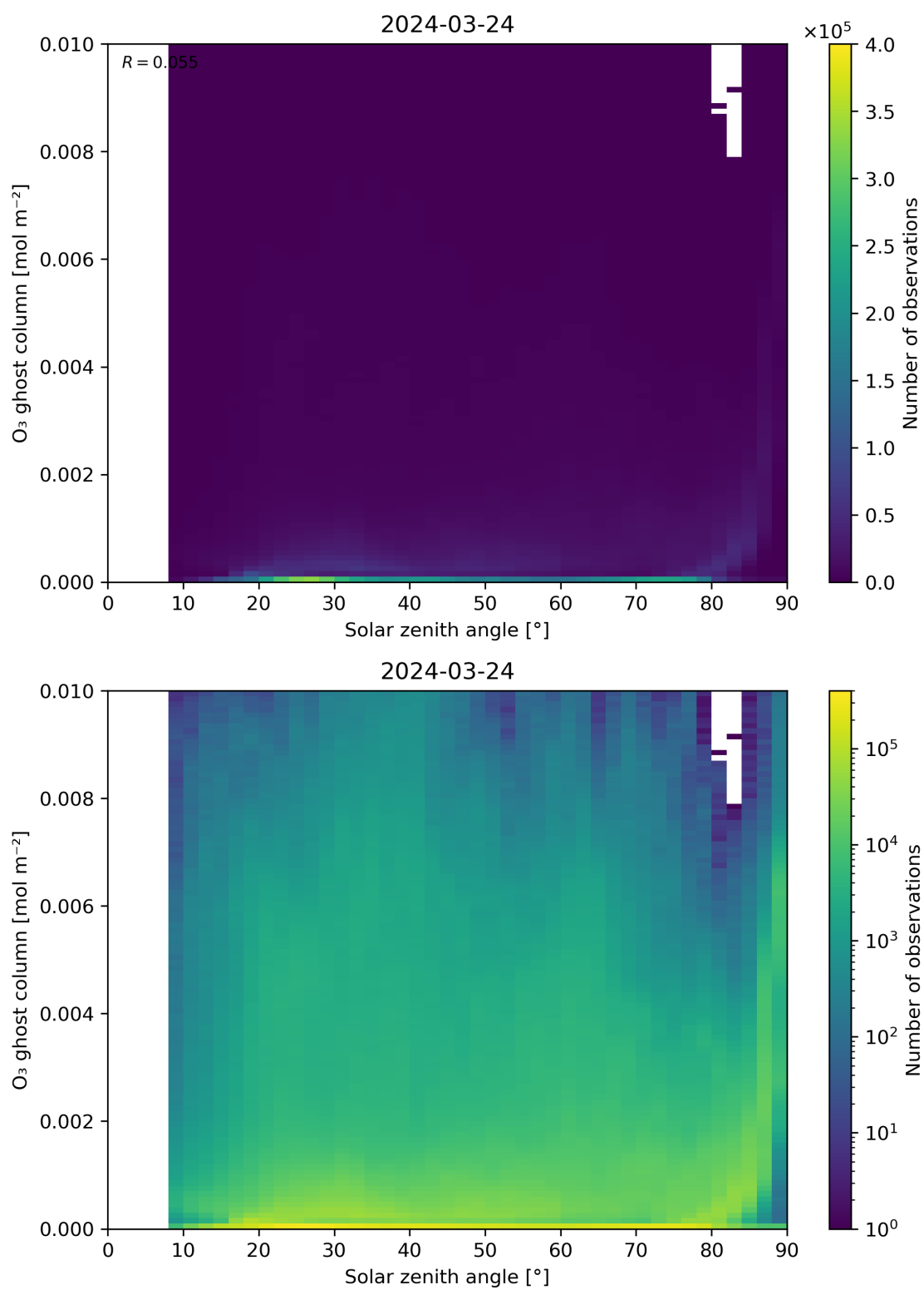
Figure 46: Scatter density plot of “Solar zenith angle” against “O 3 ghost column” for 2024-03-23 to 2024-03-25.
