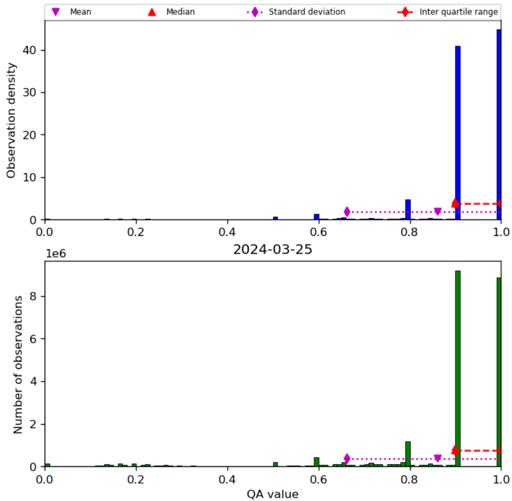
Figure 20: Histogram of “QA value” for 2024-03-25 to 2024-03-26
