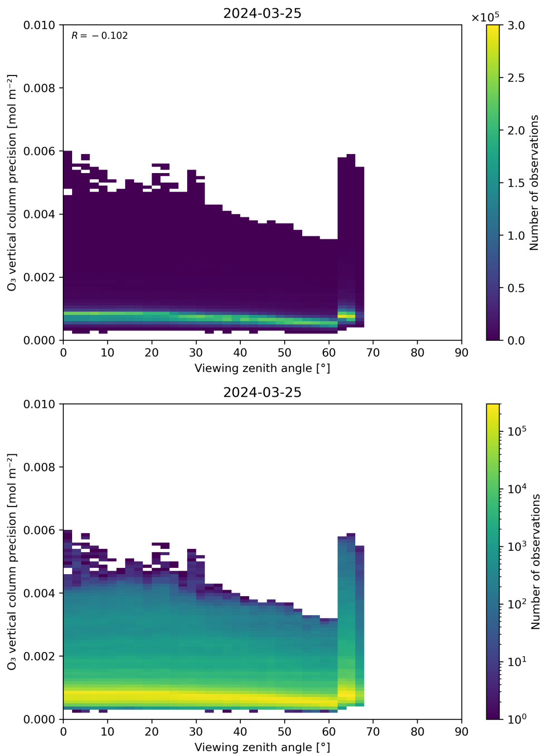
Figure 53: Scatter density plot of “Viewing zenith angle” against “O 3 vertical column precision” for 2024-03-25 to 2024-03-26.
