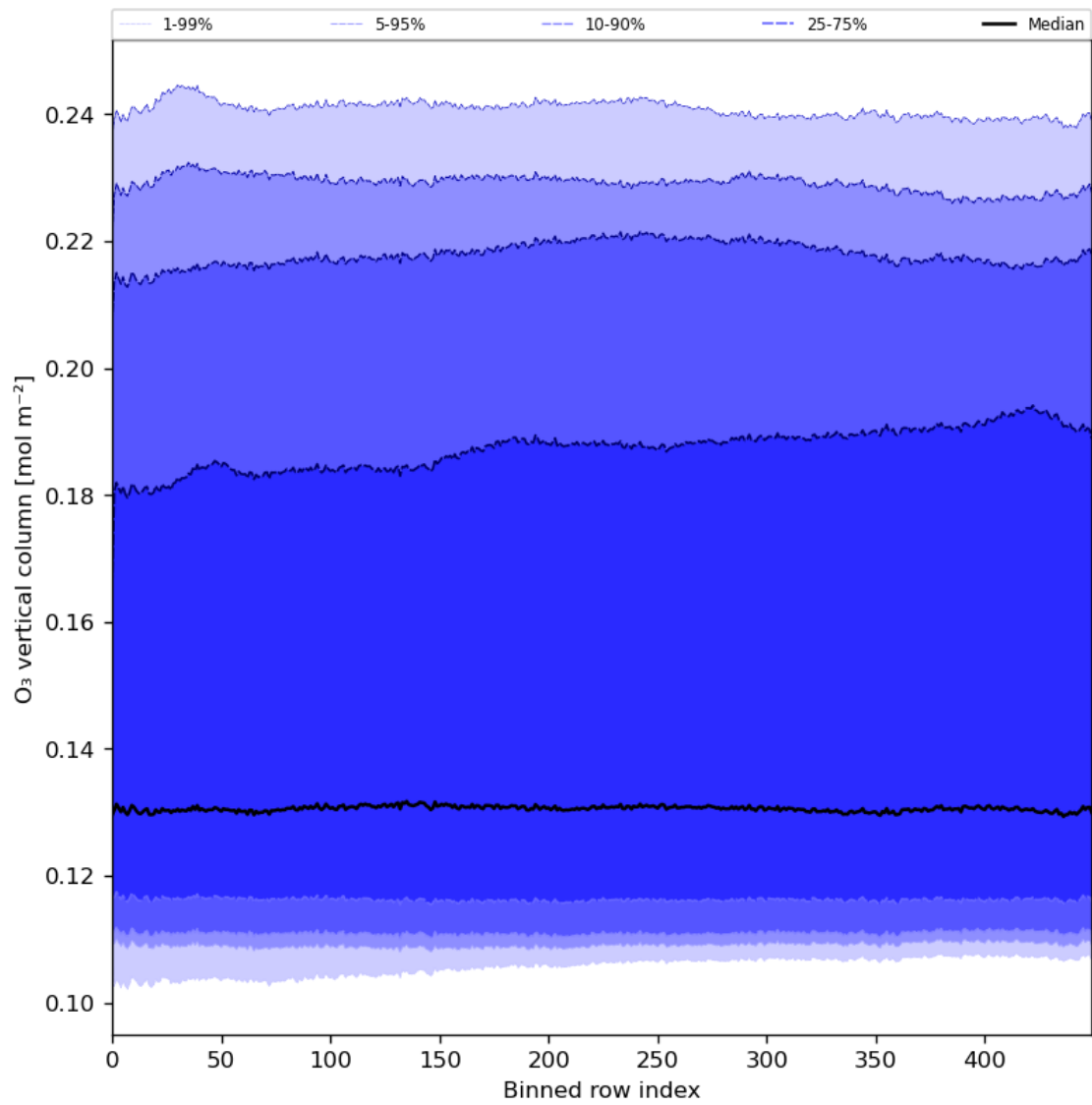
Figure 28: Along track statistics of “O 3 vertical column” for 2024-03-25 to 2024-03-26
