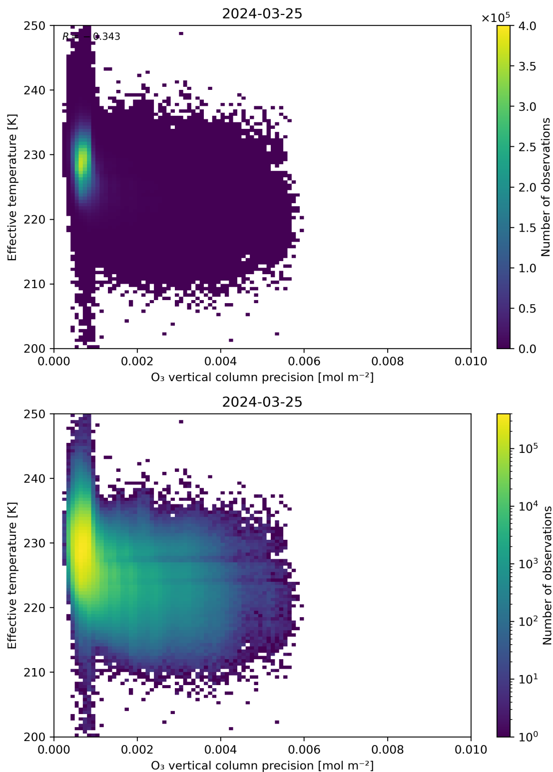
Figure 42: Scatter density plot of “O 3 vertical column precision” against “Effective temperature” for 2024-03-25 to 2024-03-26.
