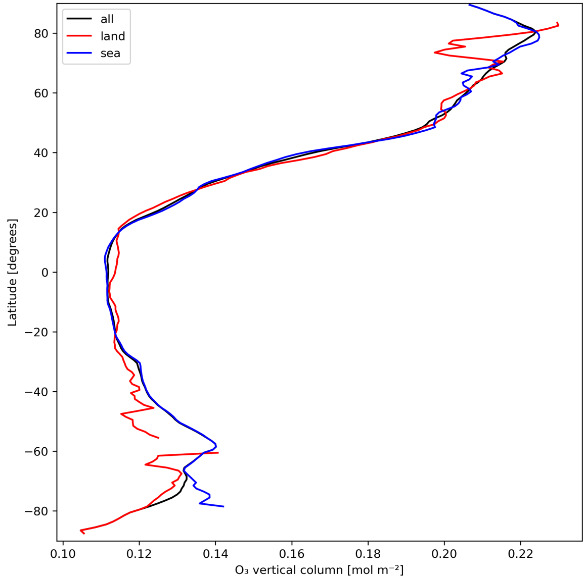
Figure 14: Zonal average of “O 3 vertical column” for 2024-03-25 to 2024-03-26.
