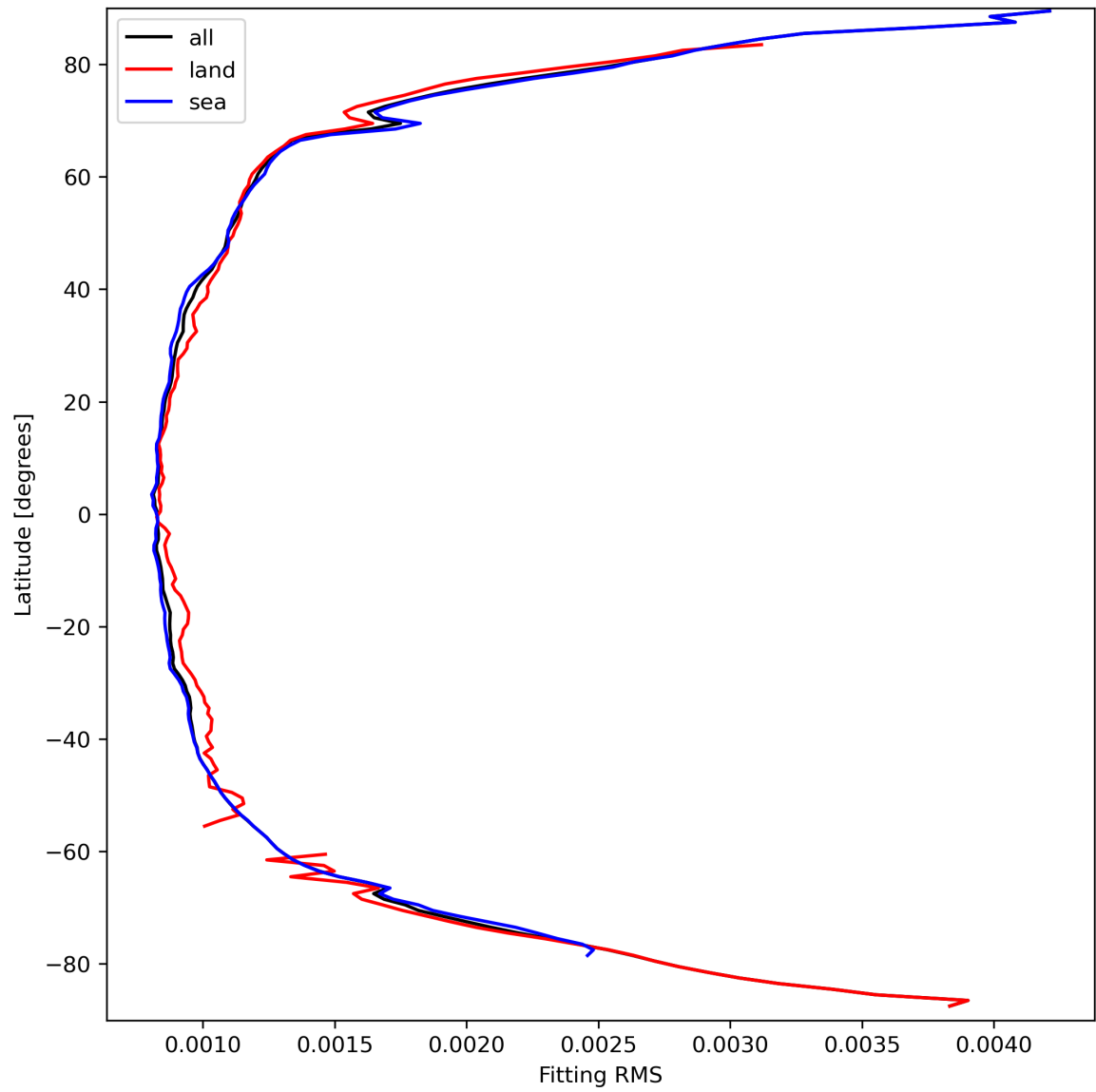
Figure 16: Zonal average of “Fitting RMS” for 2024-03-25 to 2024-03-26.
