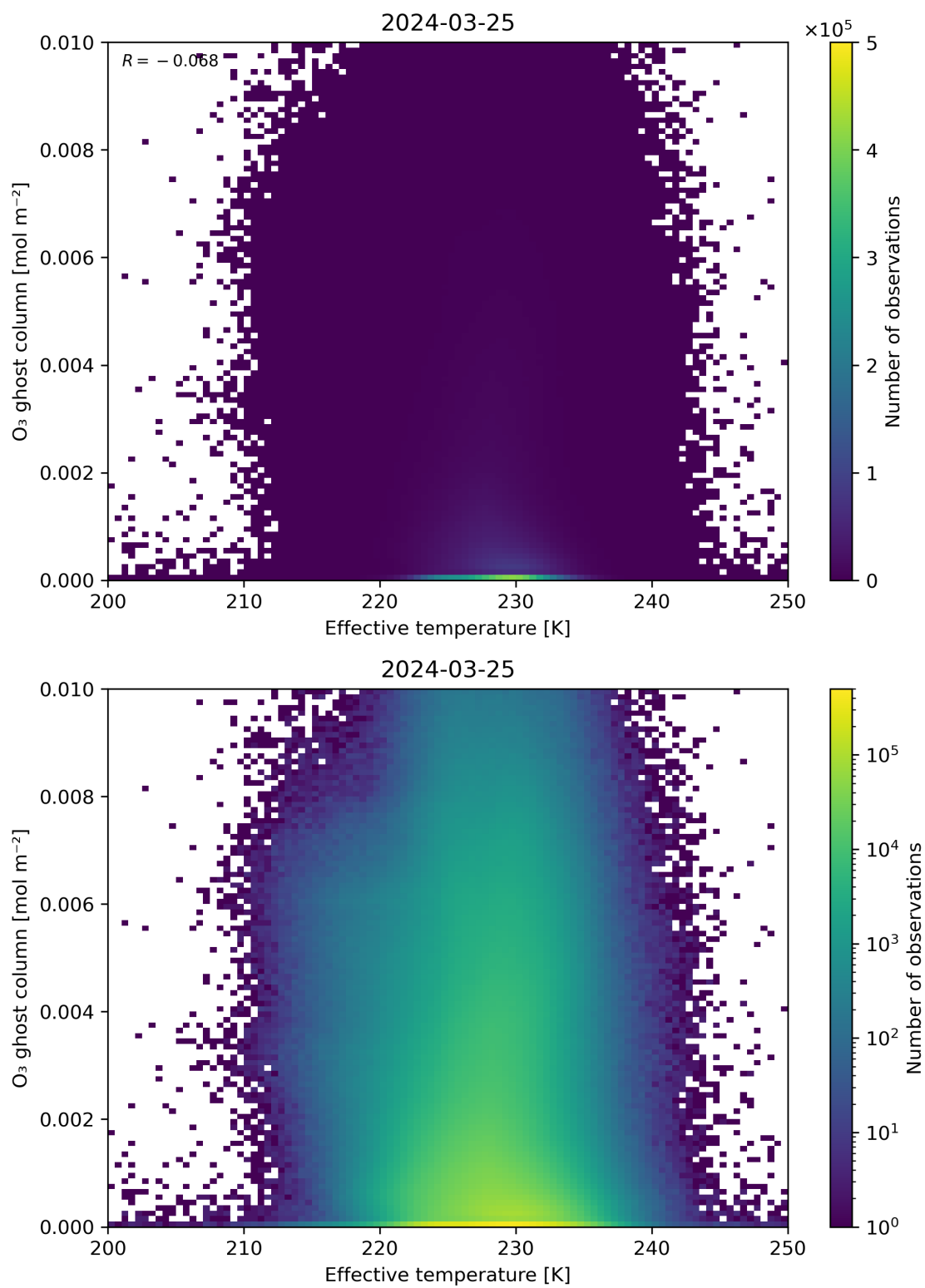
Figure 38: Scatter density plot of “Effective temperature” against “O 3 ghost column” for 2024-03-25 to 2024-03-26.
