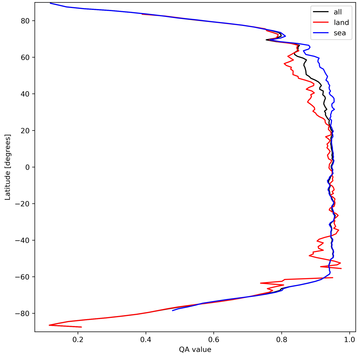
Figure 13: Zonal average of “QA value” for 2024-03-25 to 2024-03-26.
