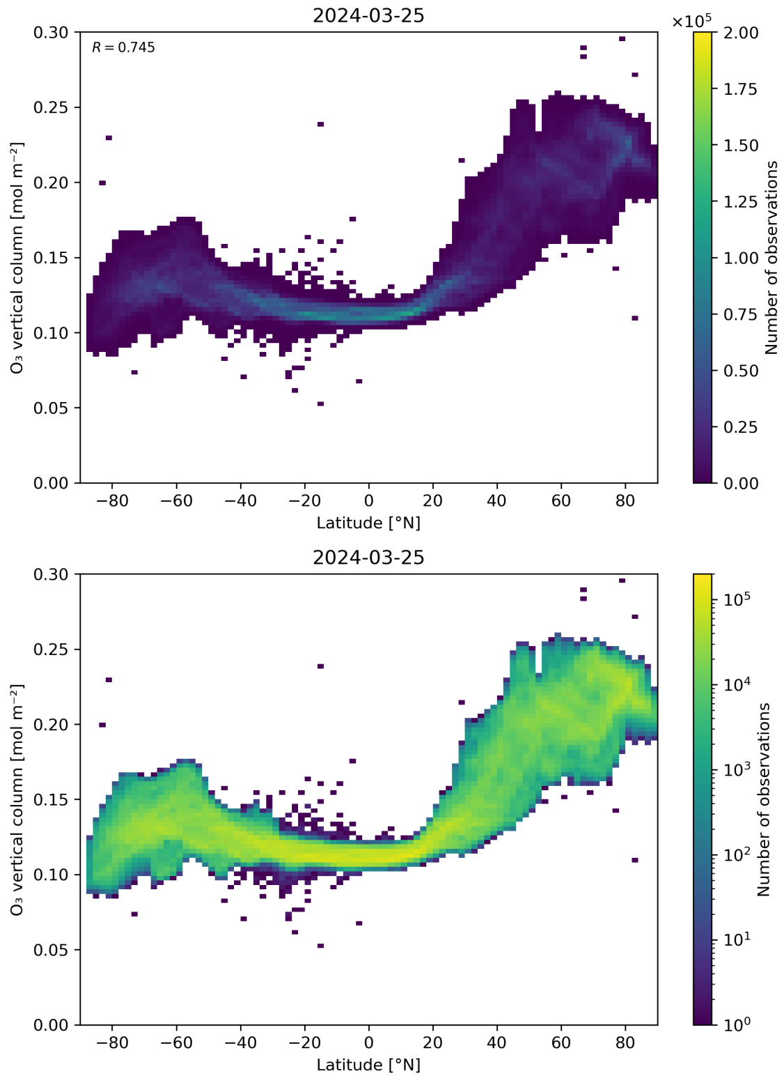
Figure 36: Scatter density plot of “Latitude” against “O 3 vertical column” for 2024-03-25 to 2024-03-26.
