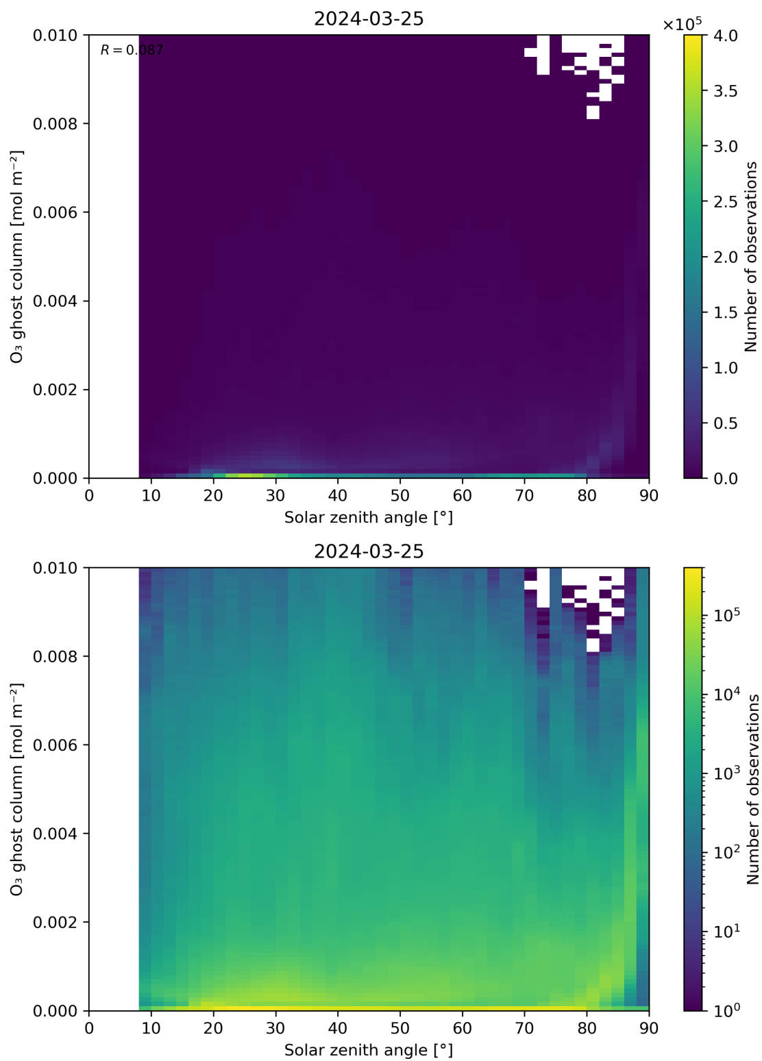
Figure 46: Scatter density plot of “Solar zenith angle” against “O 3 ghost column” for 2024-03-25 to 2024-03-26.
