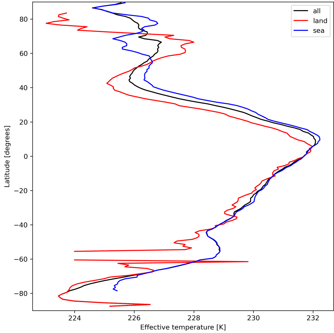
Figure 17: Zonal average of “Effective temperature” for 2024-03-25 to 2024-03-26.
