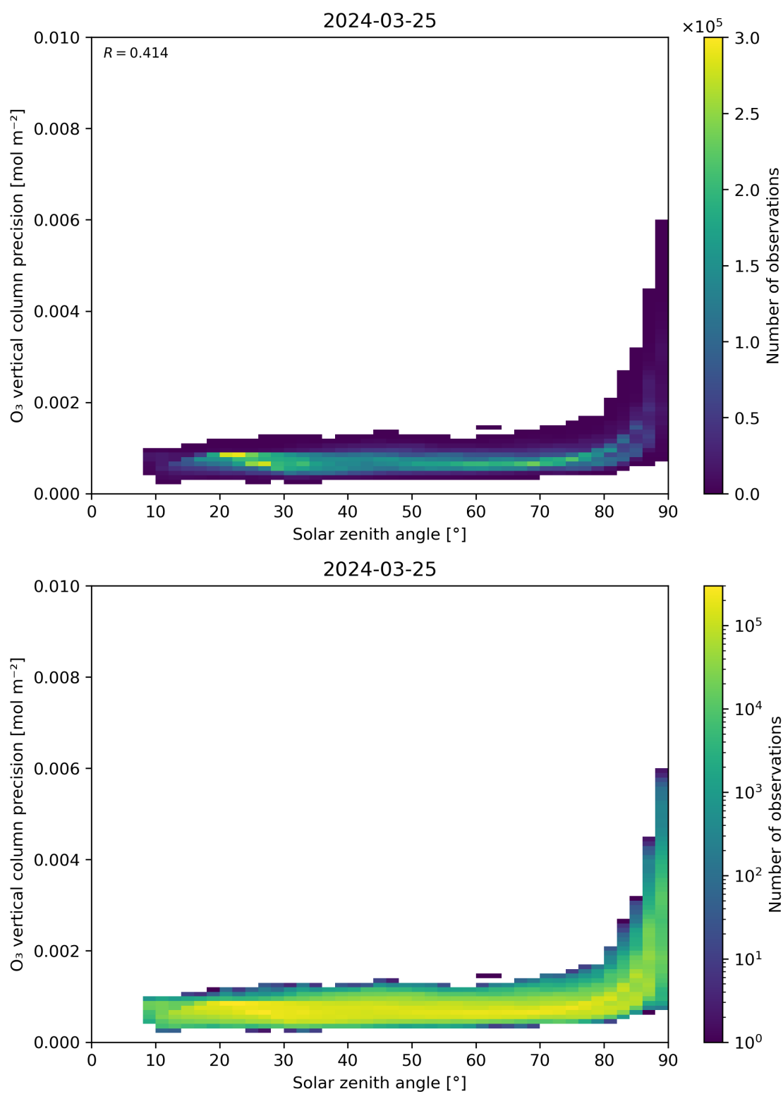
Figure 48: Scatter density plot of “Solar zenith angle” against “O 3 vertical column precision” for 2024-03-25 to 2024-03-26.
