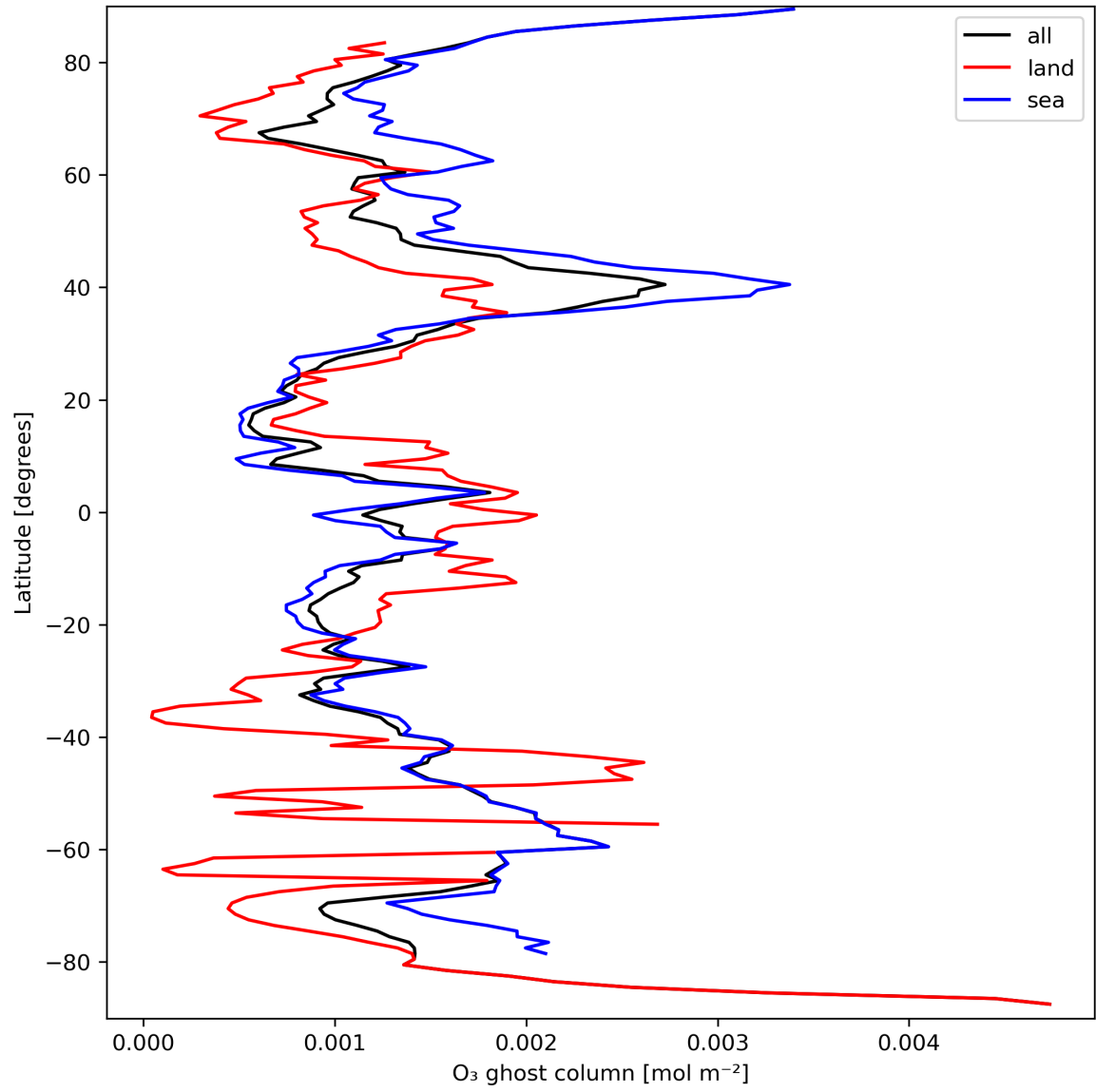
Figure 18: Zonal average of "O 3 ghost column" for 2024-03-25 to 2024-03-26.
