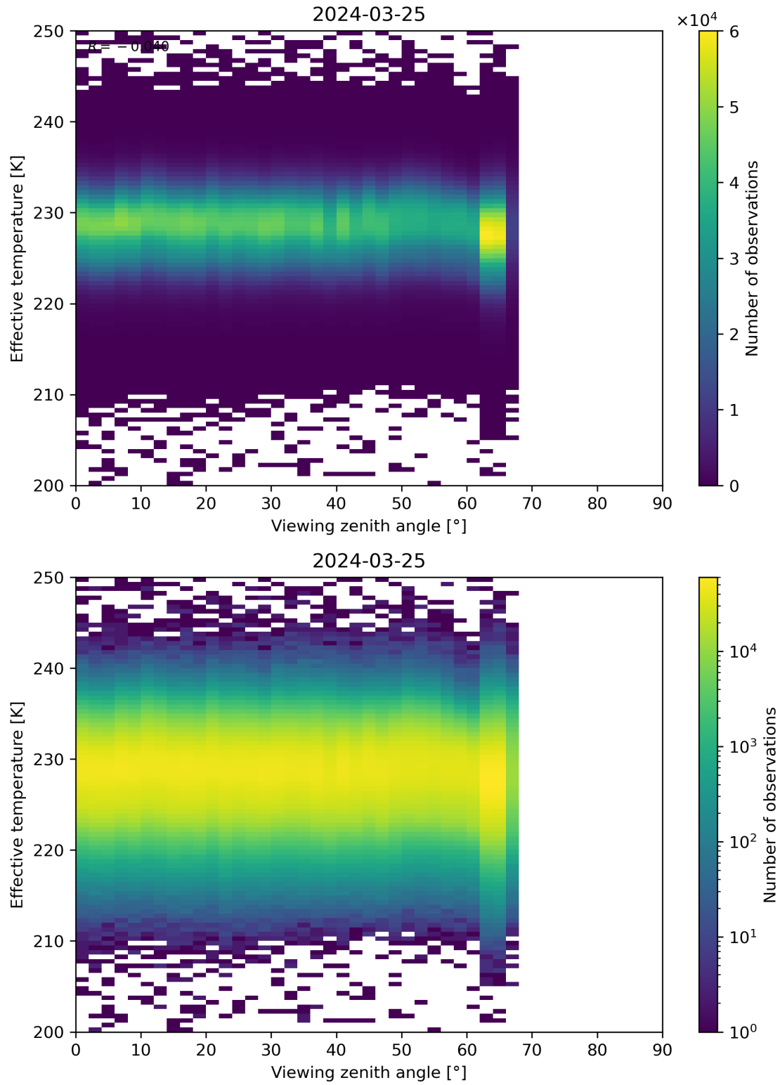
Figure 50: Scatter density plot of “Viewing zenith angle” against “Effective temperature” for 2024-03-25 to 2024-03-26.
