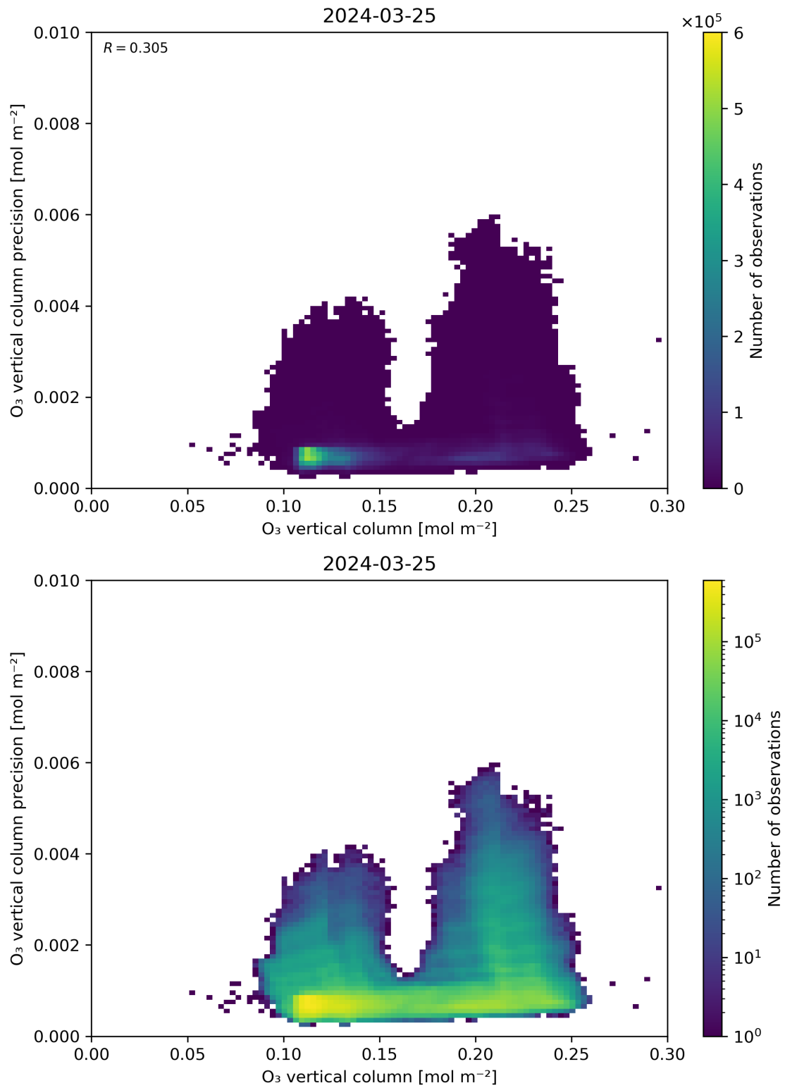
Figure 41: Scatter density plot of “O 3 vertical column” against “O 3 vertical column precision” for 2024-03-25 to 2024-03-26.
