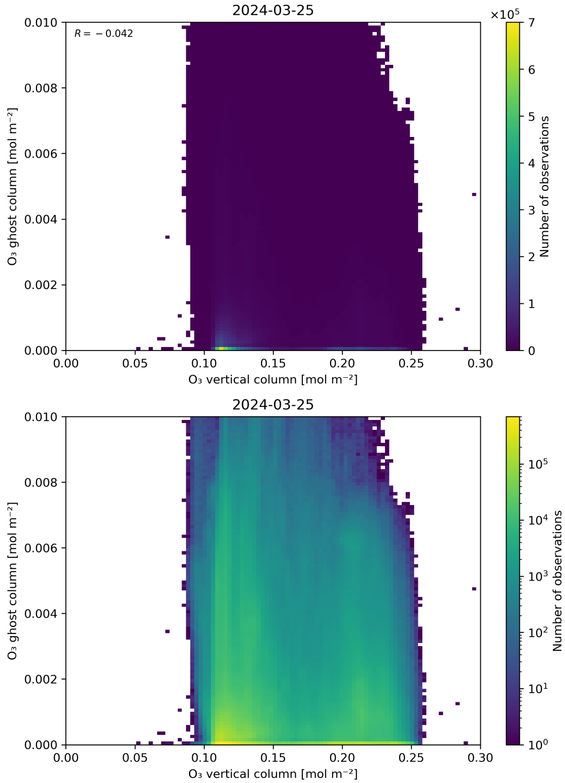
Figure 40: Scatter density plot of “O 3 vertical column” against “O 3 ghost column” for 2024-03-25 to 2024-03-26.
