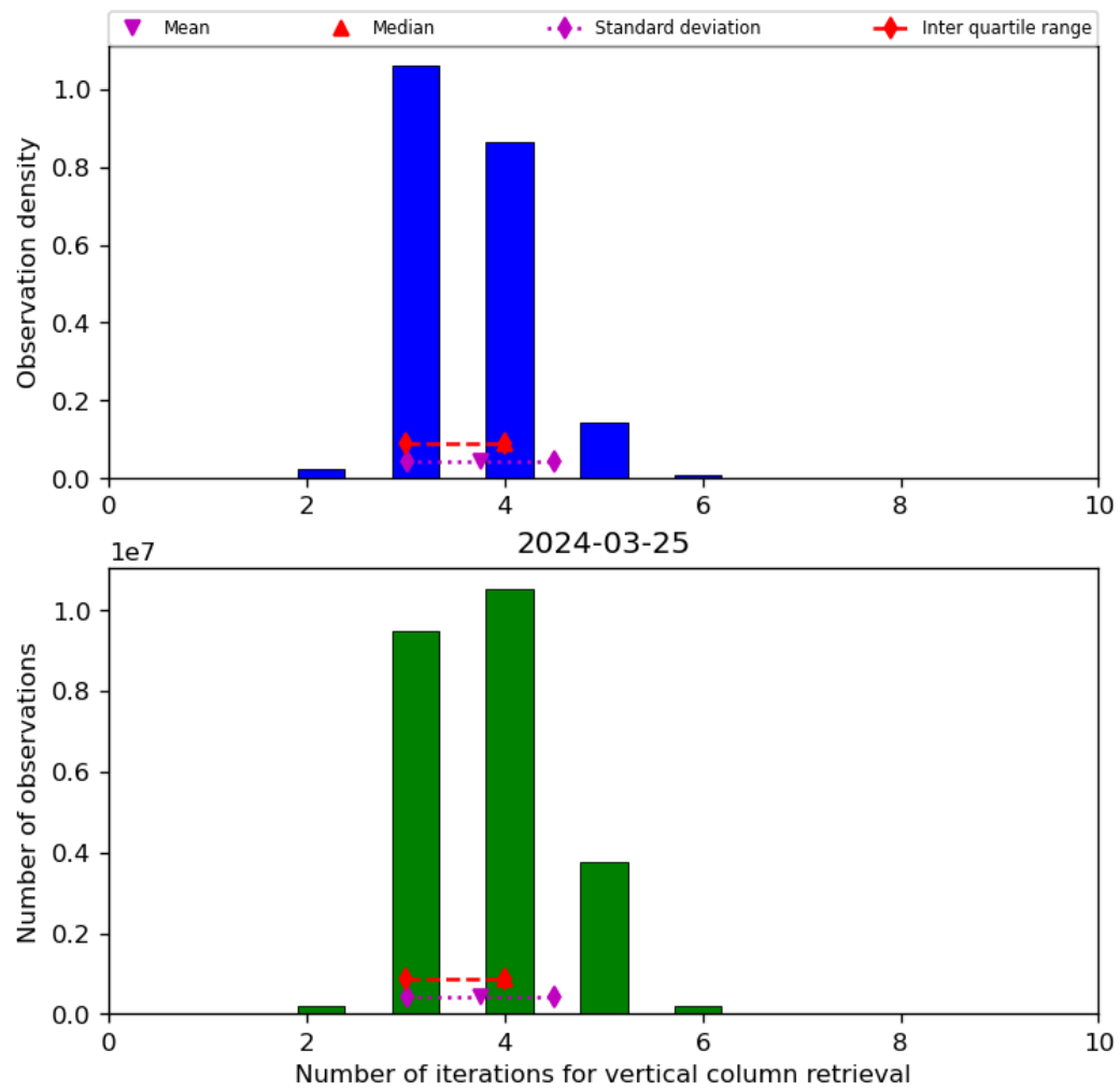
Figure 26: Histogram of “Number of iterations for vertical column retrieval” for 2024-03-25 to 2024-03-26
