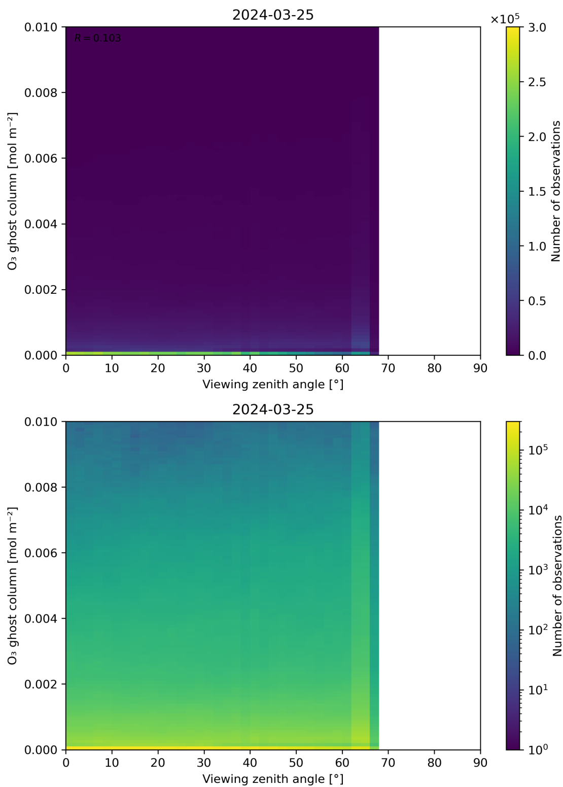
Figure 51: Scatter density plot of “Viewing zenith angle” against “O 3 ghost column” for 2024-03-25 to 2024-03-26.
