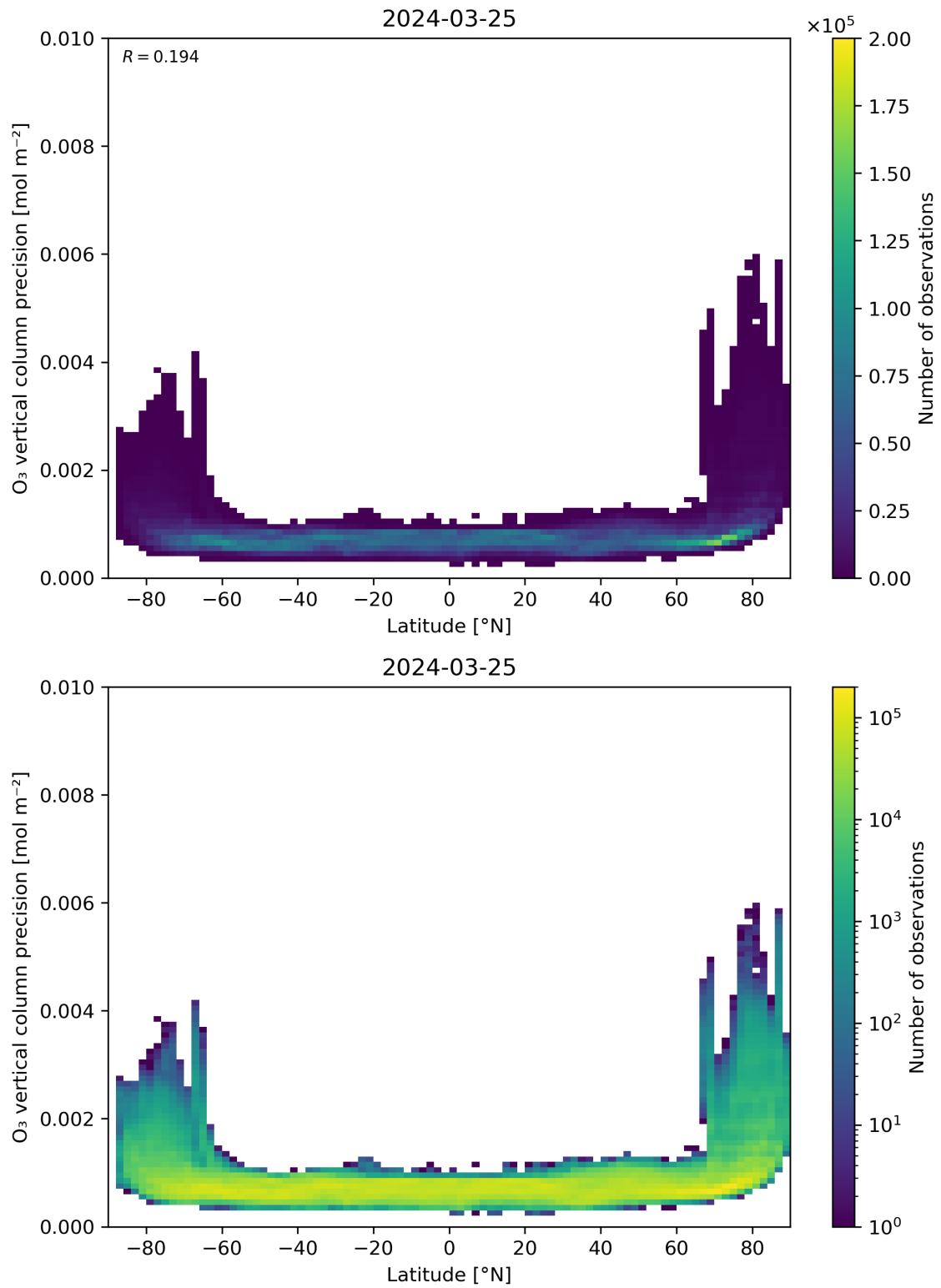
Figure 37: Scatter density plot of “Latitude” against “O 3 vertical column precision” for 2024-03-25 to 2024-03-26.
