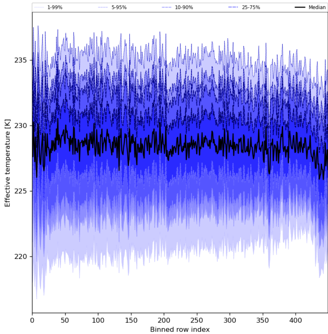
Figure 31: Along track statistics of “Effective temperature” for 2024-03-25 to 2024-03-26
