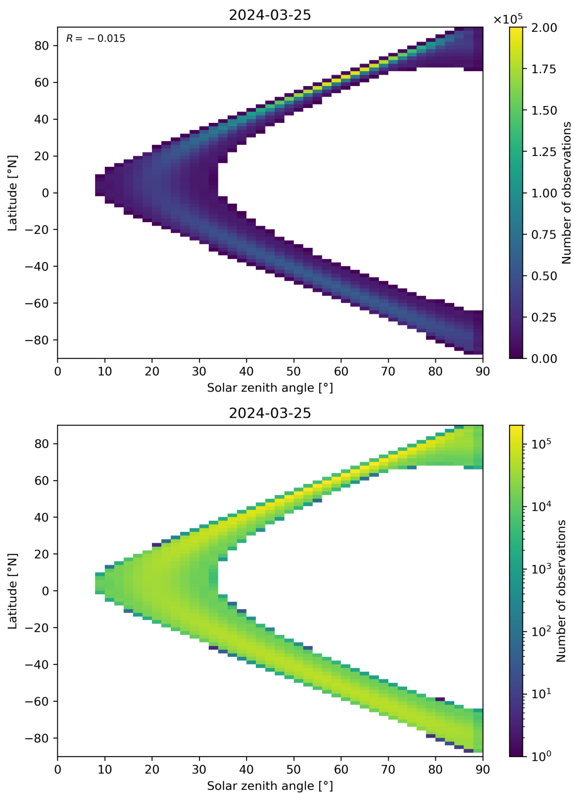
Figure 44: Scatter density plot of “Solar zenith angle” against “Latitude” for 2024-03-25 to 2024-03-26.
