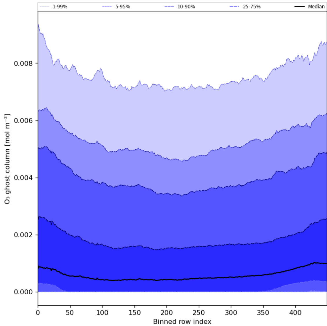
Figure 32: Along track statistics of “O 3 ghost column” for 2024-03-25 to 2024-03-26
