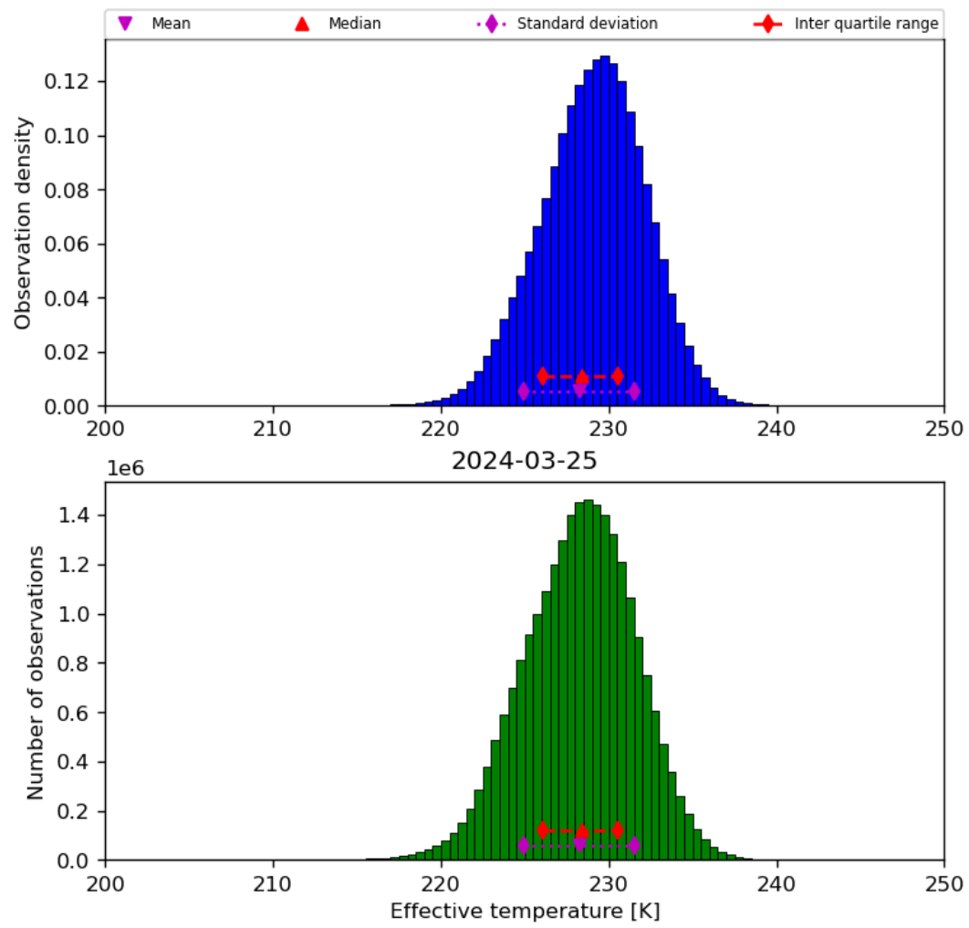
Figure 24: Histogram of “Effective temperature” for 2024-03-25 to 2024-03-26
