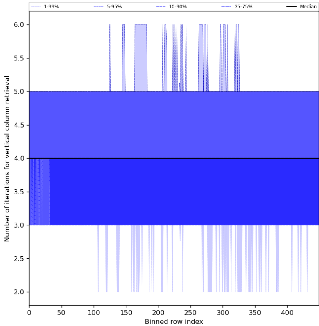
Figure 33: Along track statistics of “Number of iterations for vertical column retrieval” for 2024-03-25 to 2024-03-26
