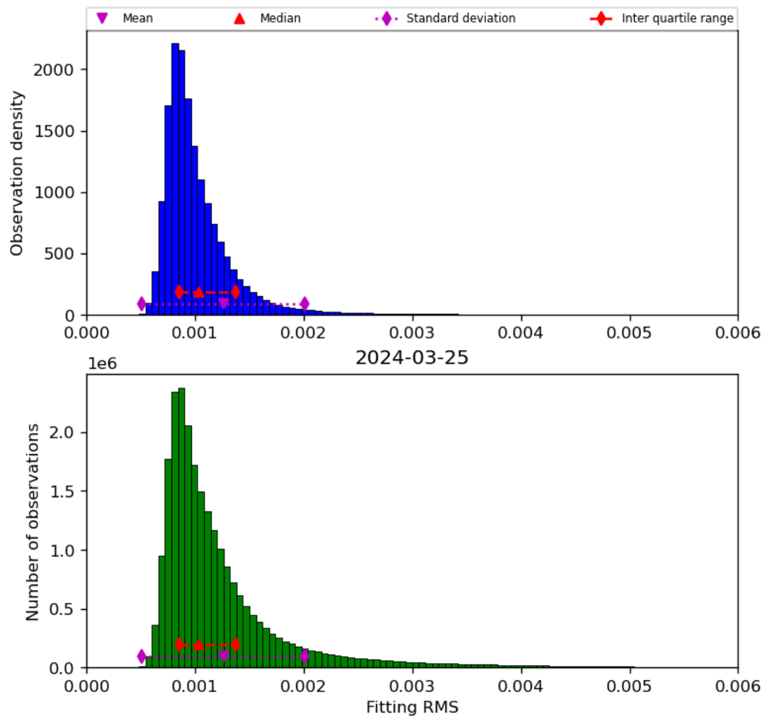
Figure 23: Histogram of “Fitting RMS” for 2024-03-25 to 2024-03-26
