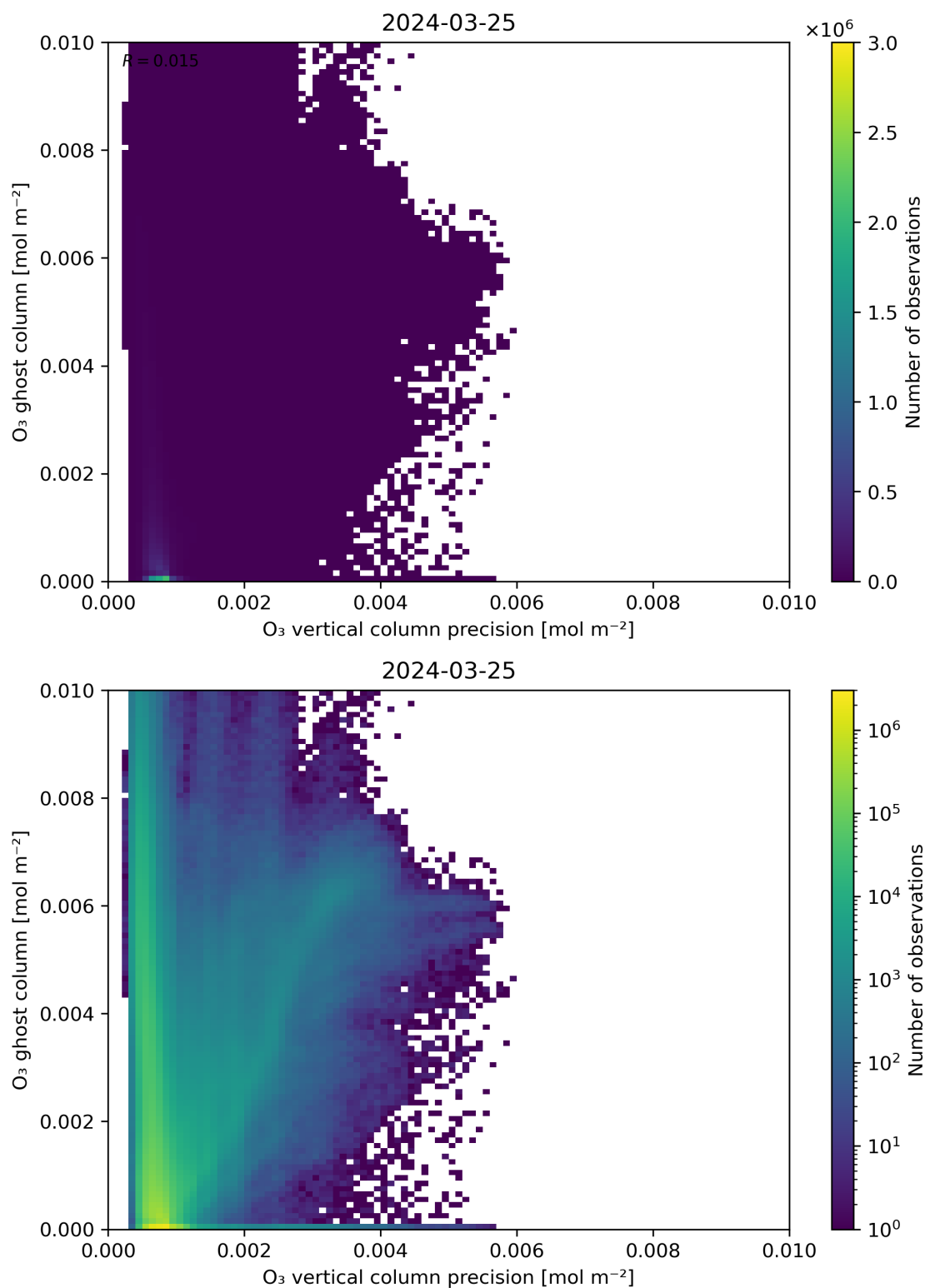
Figure 43: Scatter density plot of “O 3 vertical column precision” against “O 3 ghost column” for 2024-03-25 to 2024-03-26.
