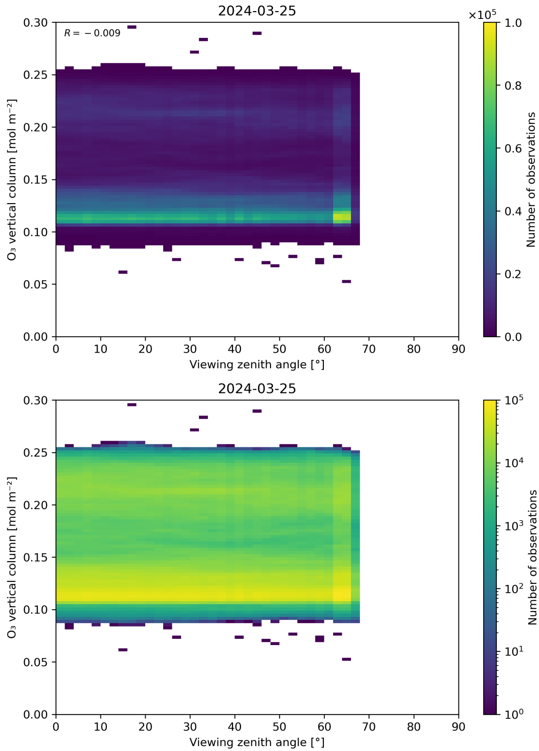
Figure 52: Scatter density plot of “Viewing zenith angle” against “O 3 vertical column” for 2024-03-25 to 2024-03-26.
