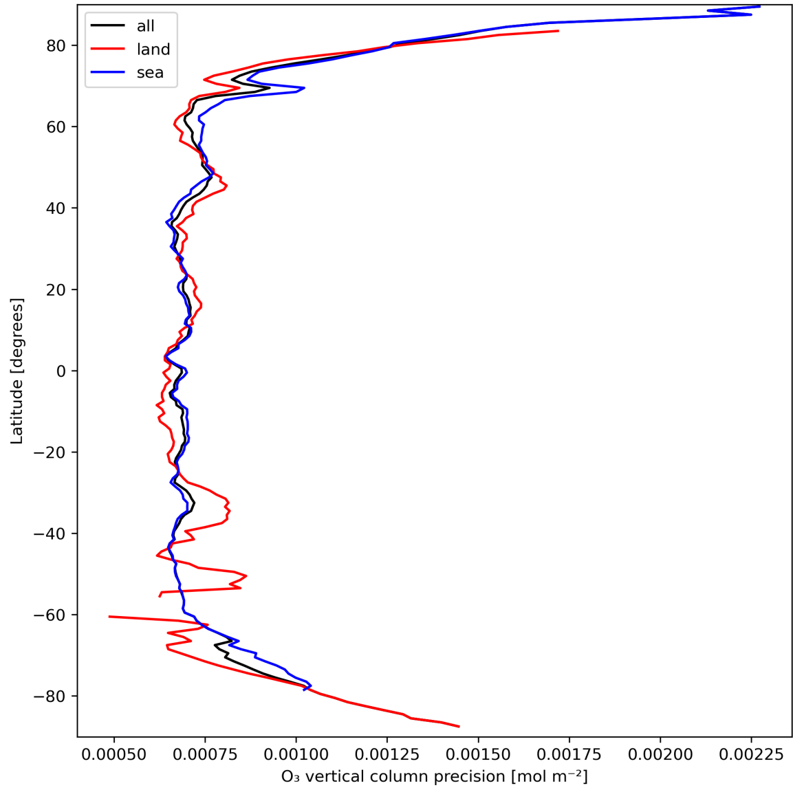
Figure 15: Zonal average of "O 3 vertical column precision" for 2024-03-25 to 2024-03-26.
