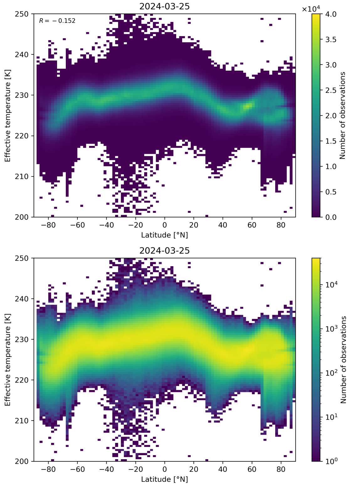
Figure 34: Scatter density plot of “Latitude” against “Effective temperature” for 2024-03-25 to 2024-03-26.
