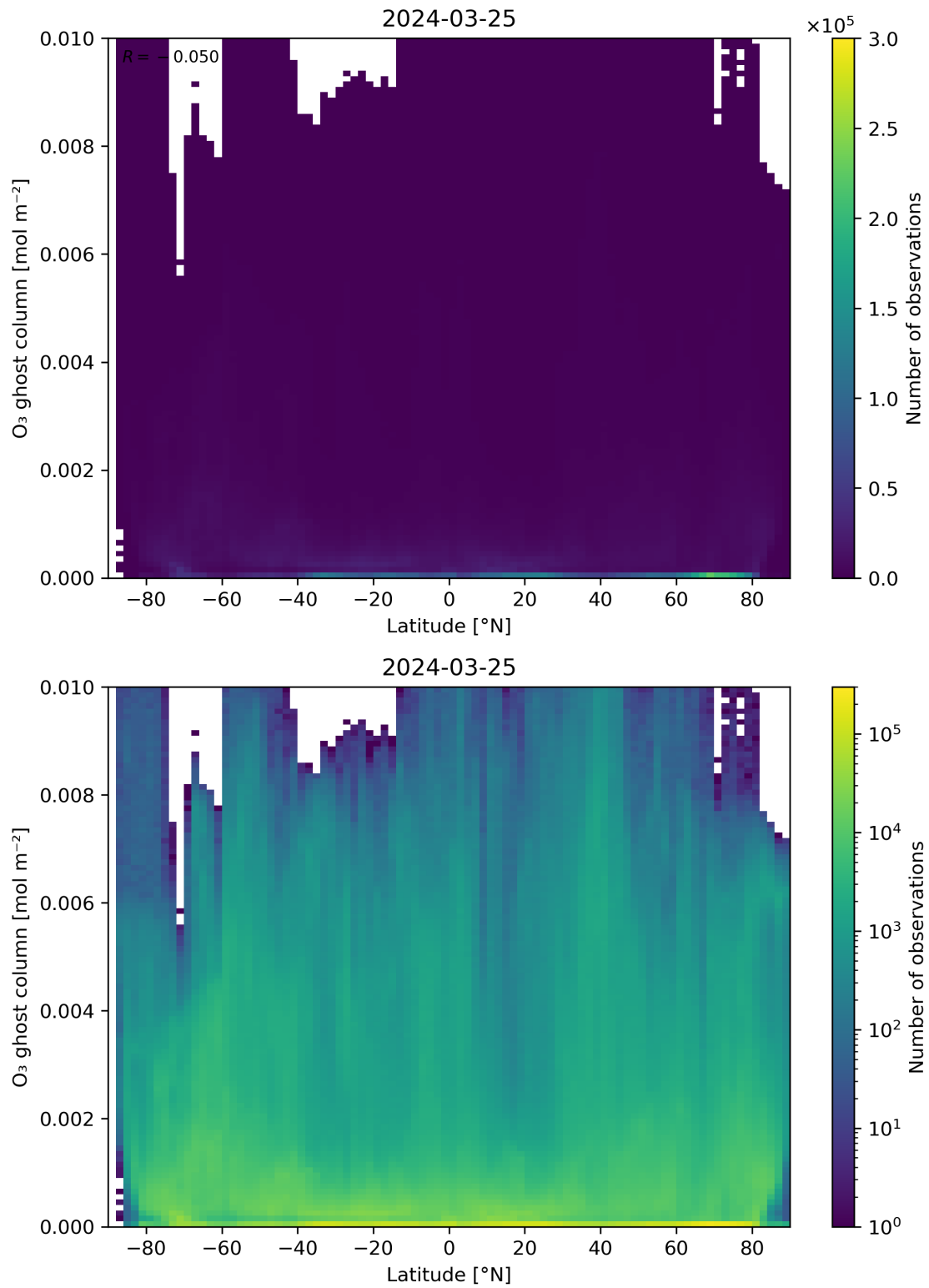
Figure 35: Scatter density plot of “Latitude” against “O 3 ghost column” for 2024-03-25 to 2024-03-26.
