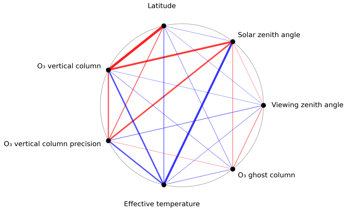
Figure 1: Map of correlation graph for 2024-03-25 to 2024-03-26.
