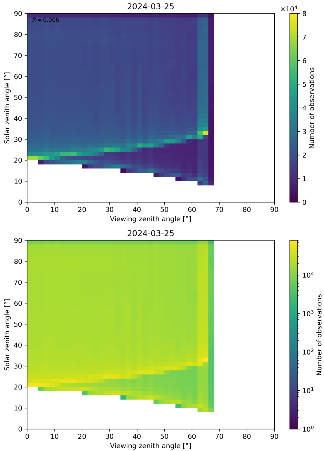
Figure 54: Scatter density plot of “Viewing zenith angle” against “Solar zenith angle” for 2024-03-25 to 2024-03-26.
