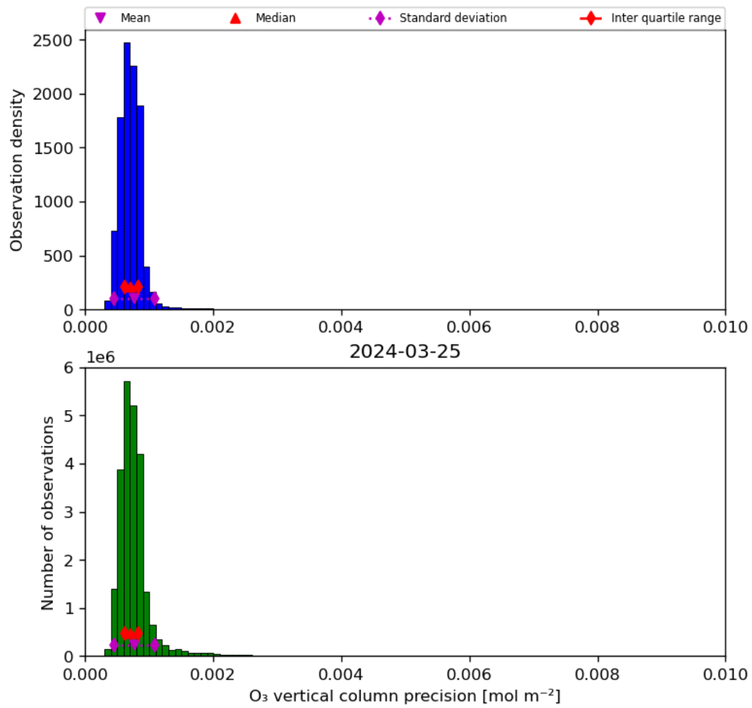
Figure 22: Histogram of “O 3 vertical column precision” for 2024-03-25 to 2024-03-26
