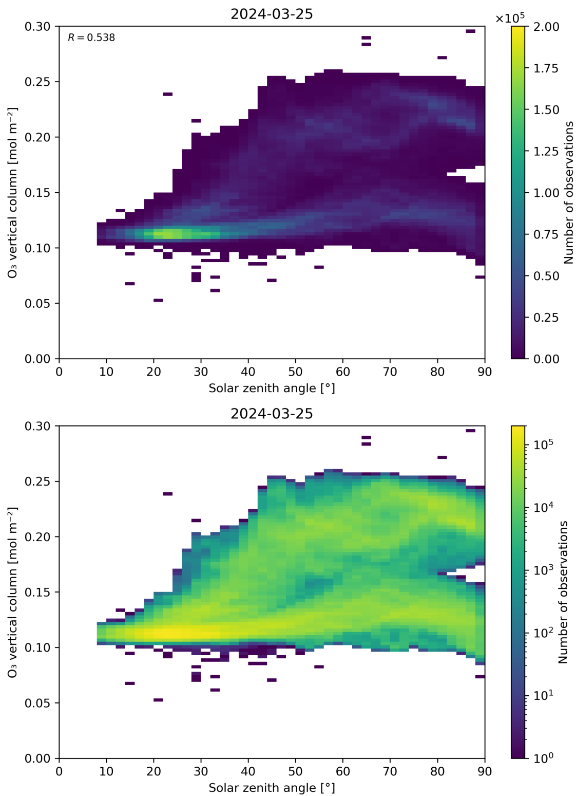
Figure 47: Scatter density plot of “Solar zenith angle” against “O 3 vertical column” for 2024-03-25 to 2024-03-26.
