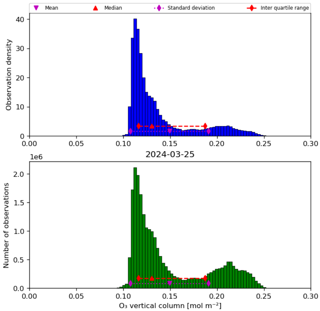
Figure 21: Histogram of “O 3 vertical column” for 2024-03-25 to 2024-03-26
