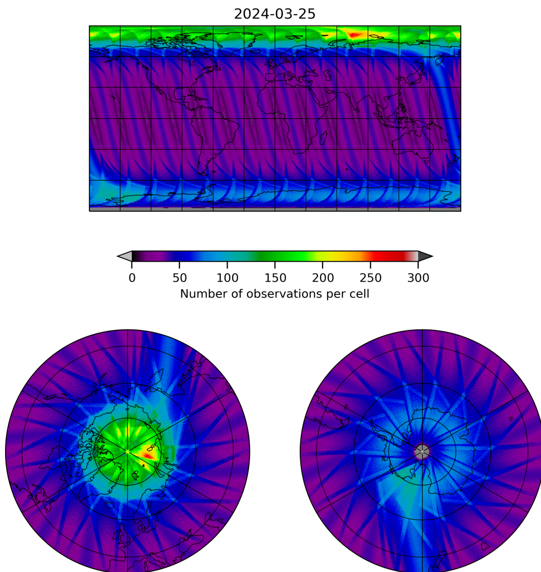
Figure 12: Map of the number of observations for 2024-03-25 to 2024-03-26
