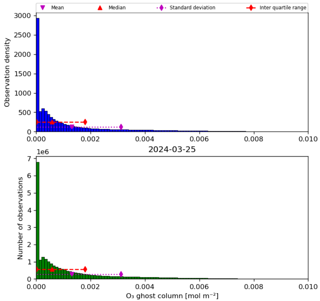
Figure 25: Histogram of “O 3 ghost column” for 2024-03-25 to 2024-03-26
