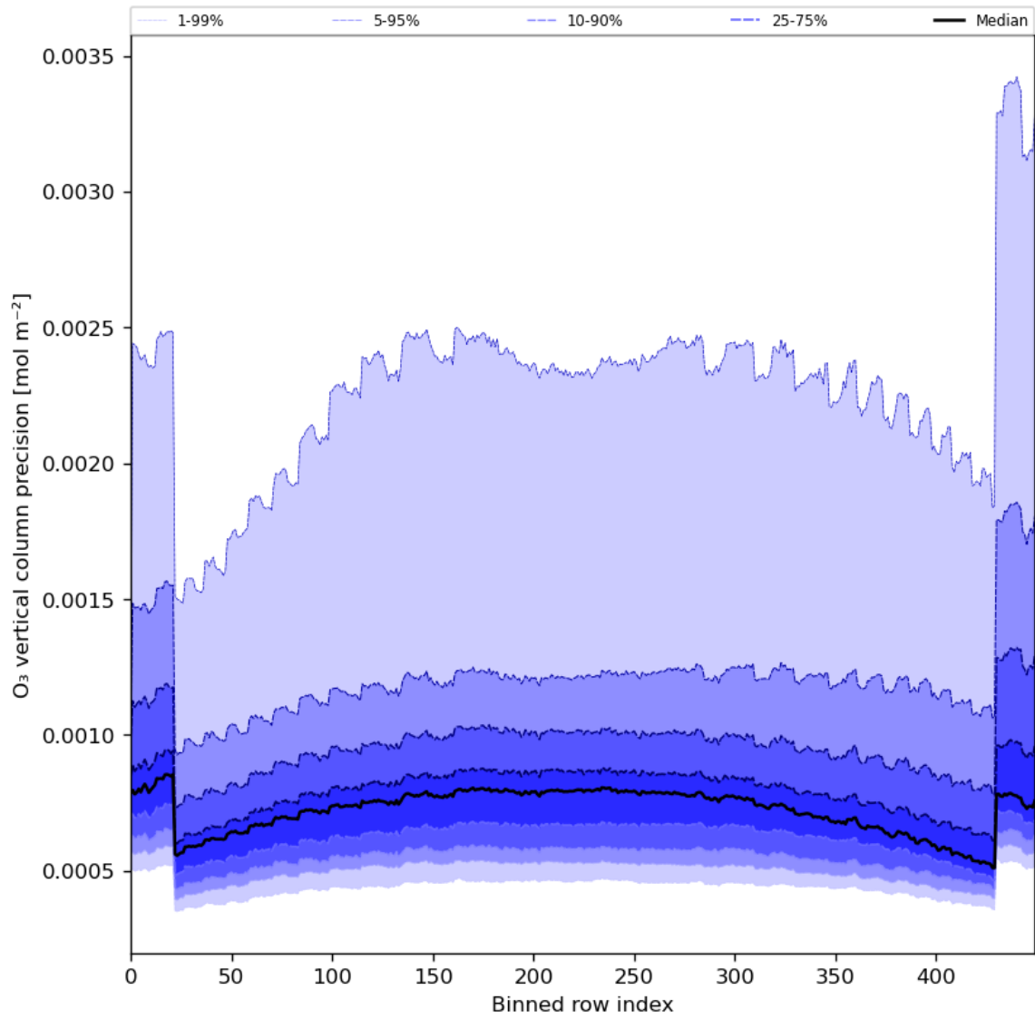
Figure 29: Along track statistics of “O 3 vertical column precision” for 2024-03-25 to 2024-03-26
