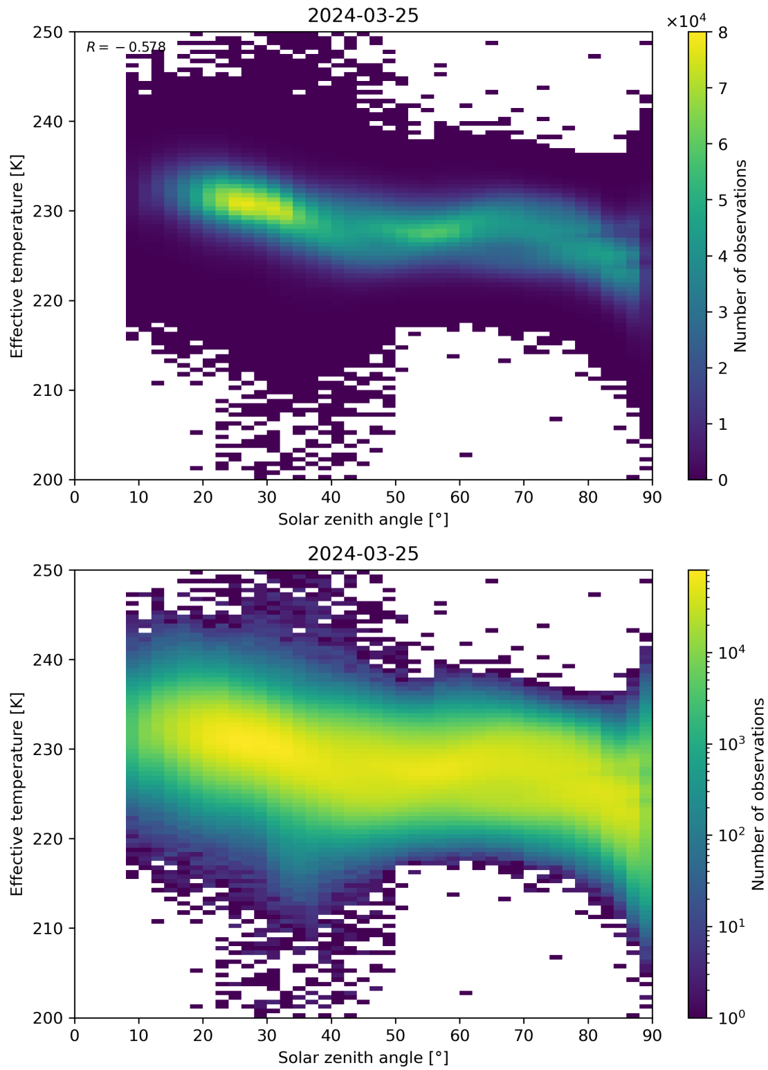
Figure 45: Scatter density plot of “Solar zenith angle” against “Effective temperature” for 2024-03-25 to 2024-03-26.
