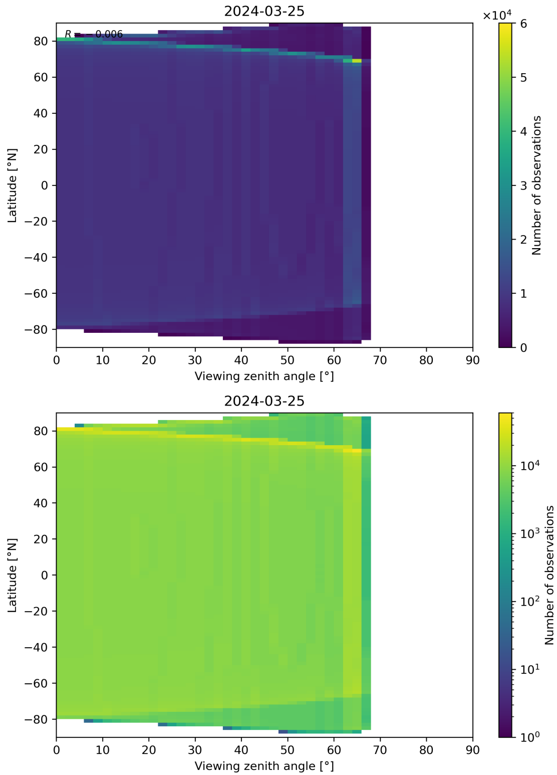
Figure 49: Scatter density plot of “Viewing zenith angle” against “Latitude” for 2024-03-25 to 2024-03-26.
