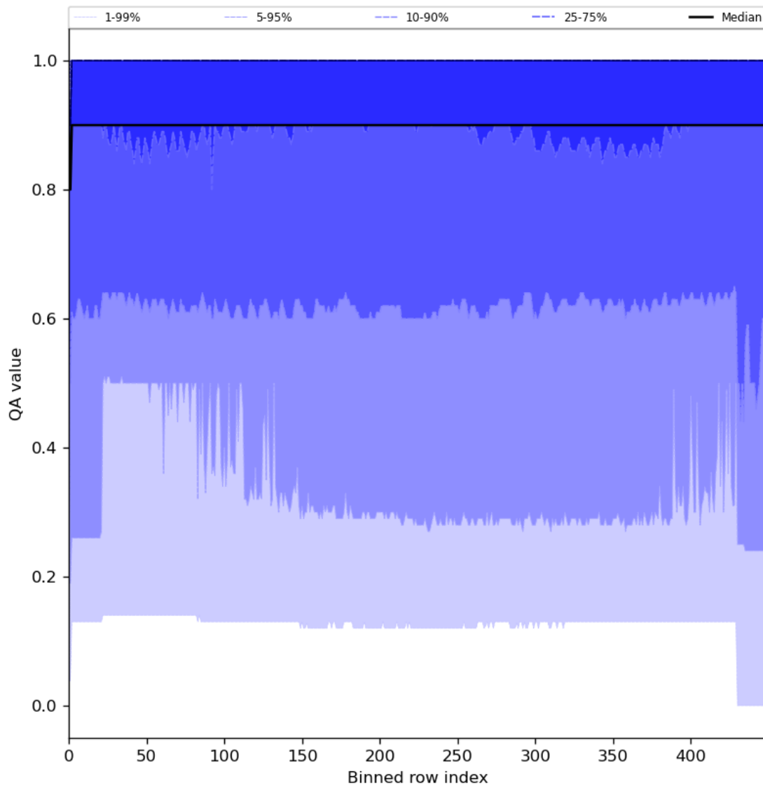
Figure 27: Along track statistics of “QA value” for 2024-03-25 to 2024-03-26
