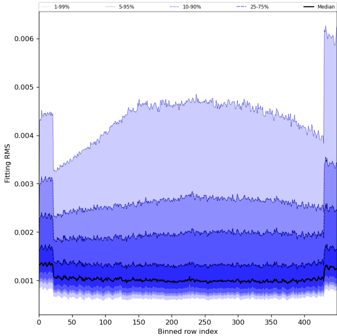
Figure 30: Along track statistics of “Fitting RMS” for 2024-03-25 to 2024-03-26
