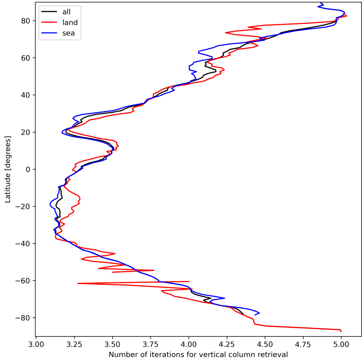
Figure 19: Zonal average of “Number of iterations for vertical column retrieval” for 2024-03-25 to 2024-03-26.
