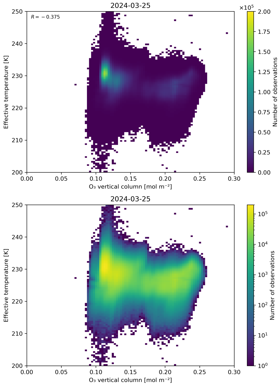
Figure 39: Scatter density plot of “O 3 vertical column” against “Effective temperature” for 2024-03-25 to 2024-03-26.
