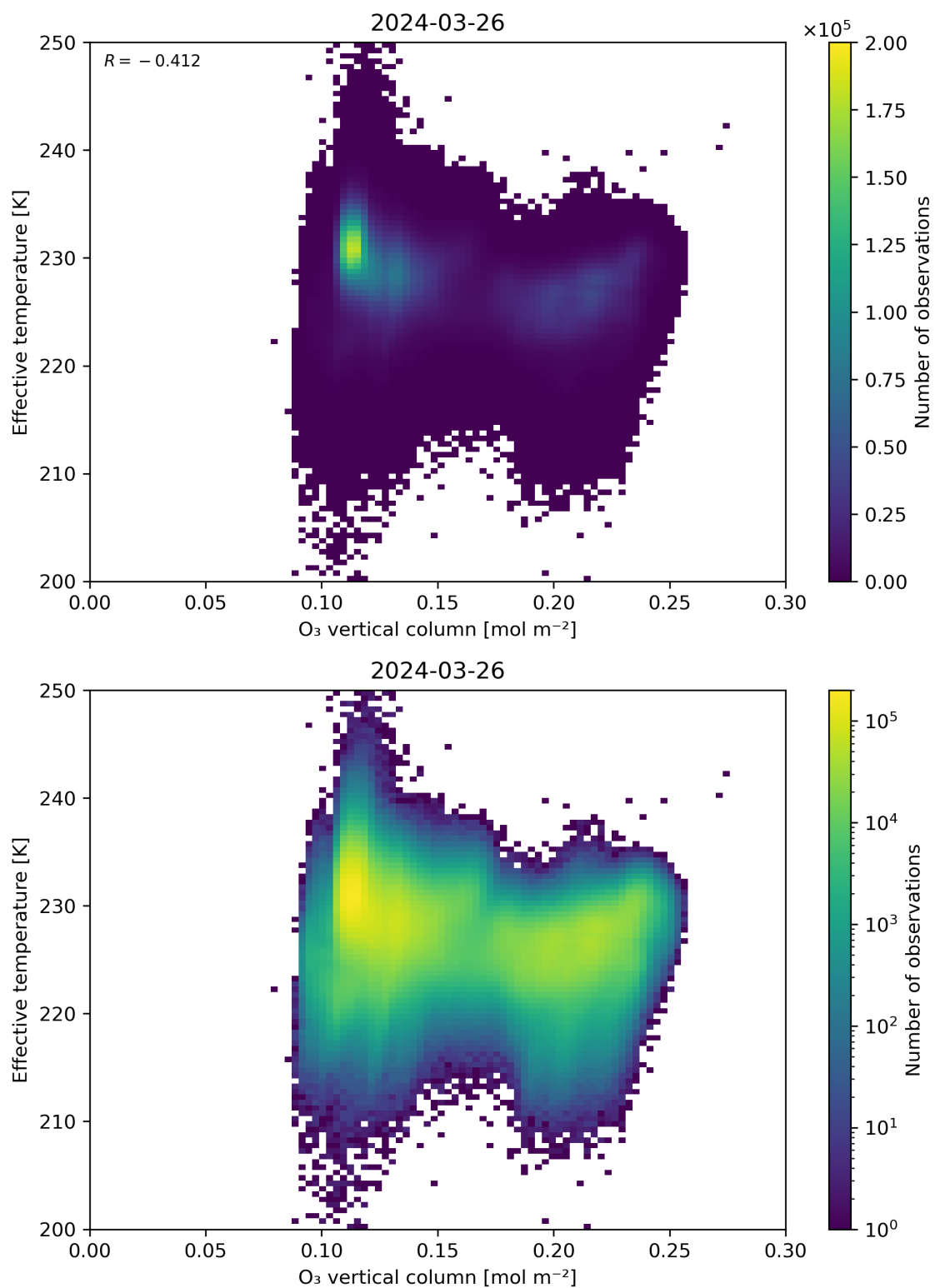
Figure 39: Scatter density plot of “O 3 vertical column” against “Effective temperature” for 2024-03-25 to 2024-03-27.
