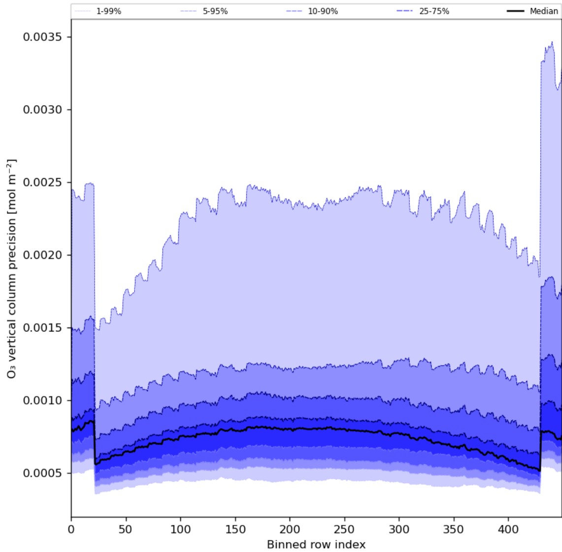
Figure 29: Along track statistics of “O 3 vertical column precision” for 2024-03-25 to 2024-03-27
