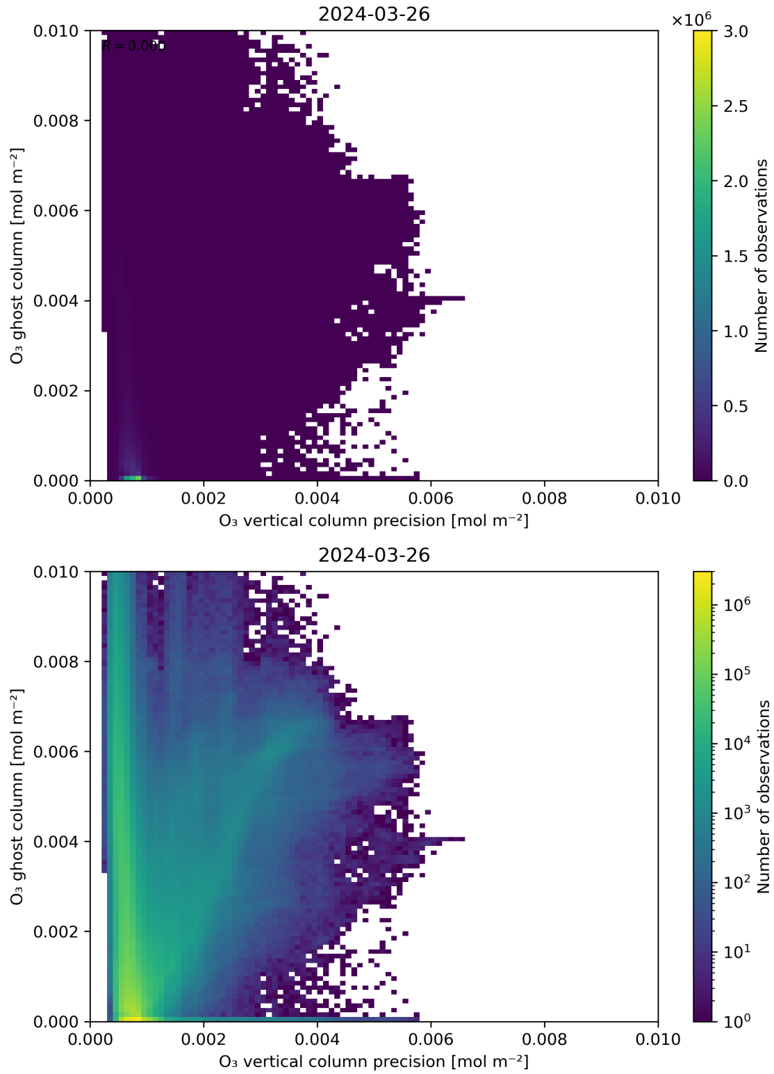
Figure 43: Scatter density plot of “O 3 vertical column precision” against “O 3 ghost column” for 2024-03-25 to 2024-03-27.
