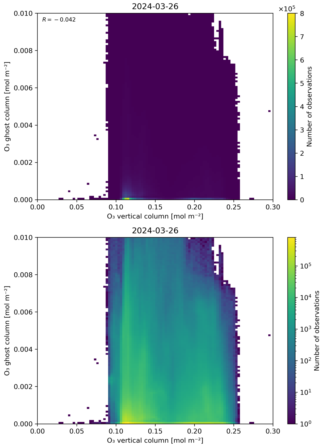
Figure 40: Scatter density plot of “O 3 vertical column” against “O 3 ghost column” for 2024-03-25 to 2024-03-27.
