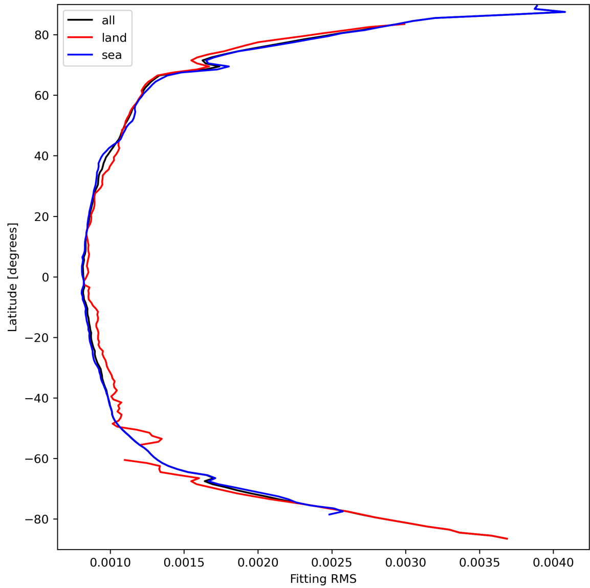
Figure 16: Zonal average of “Fitting RMS” for 2024-03-25 to 2024-03-27.
