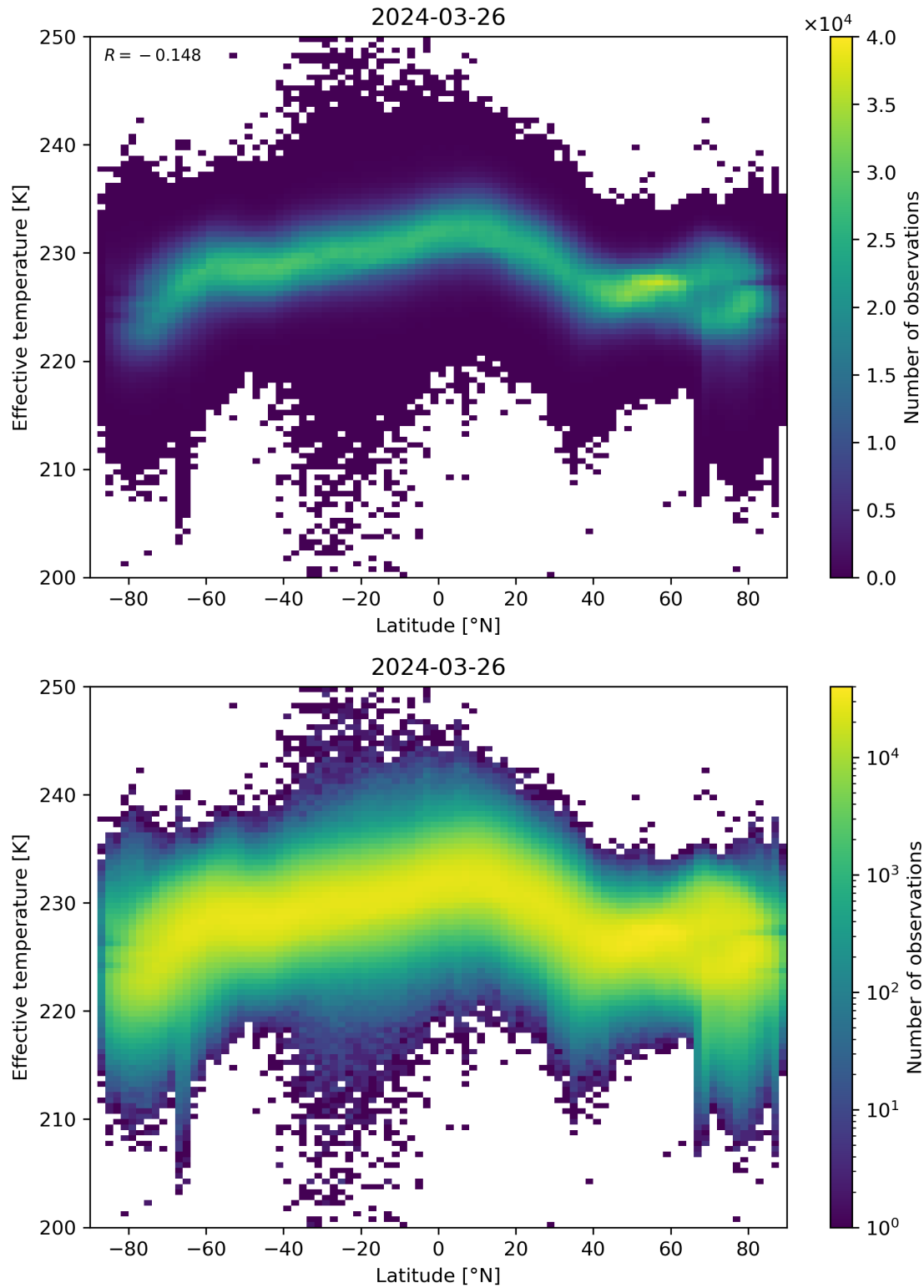
Figure 34: Scatter density plot of “Latitude” against “Effective temperature” for 2024-03-25 to 2024-03-27.
