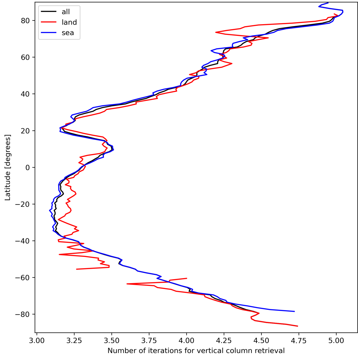
Figure 19: Zonal average of “Number of iterations for vertical column retrieval” for 2024-03-25 to 2024-03-27.
