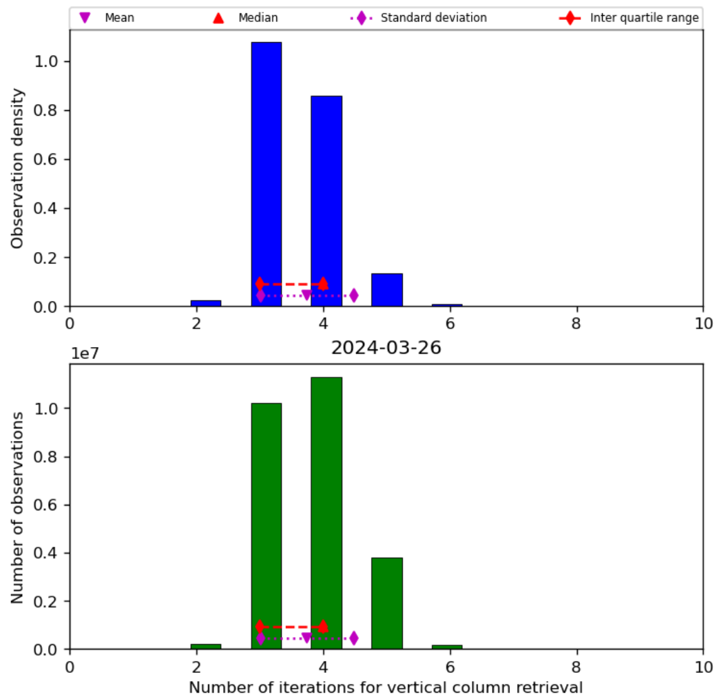
Figure 26: Histogram of “Number of iterations for vertical column retrieval” for 2024-03-25 to 2024-03-27
