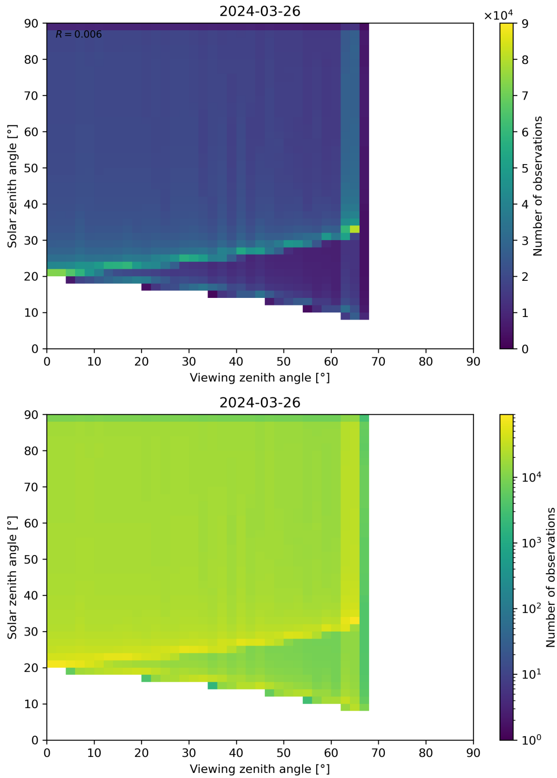
Figure 54: Scatter density plot of “Viewing zenith angle” against “Solar zenith angle” for 2024-03-25 to 2024-03-27.
