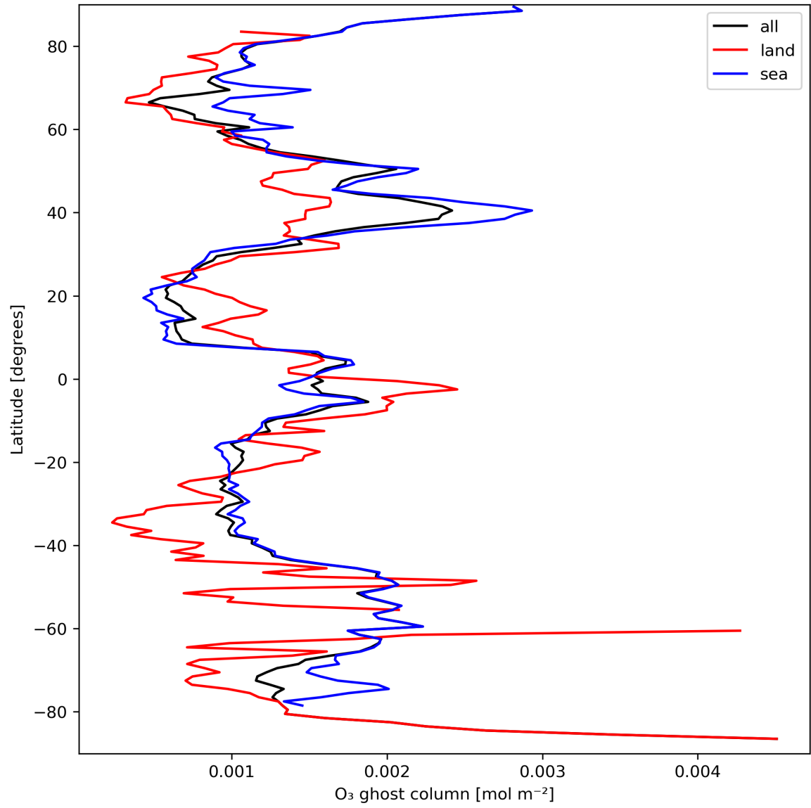
Figure 18: Zonal average of "O 3 ghost column" for 2024-03-25 to 2024-03-27.
