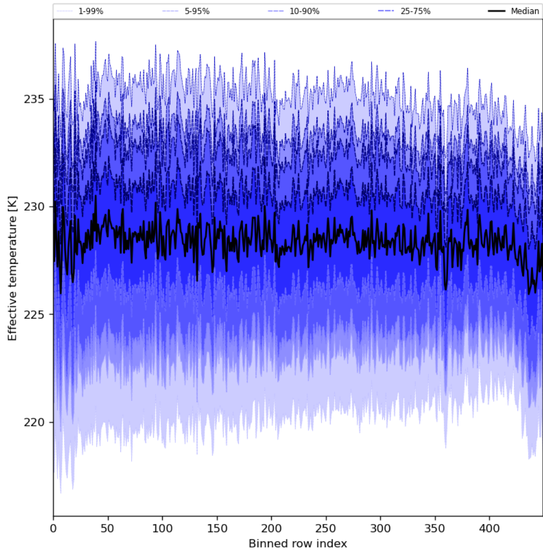
Figure 31: Along track statistics of “Effective temperature” for 2024-03-25 to 2024-03-27
