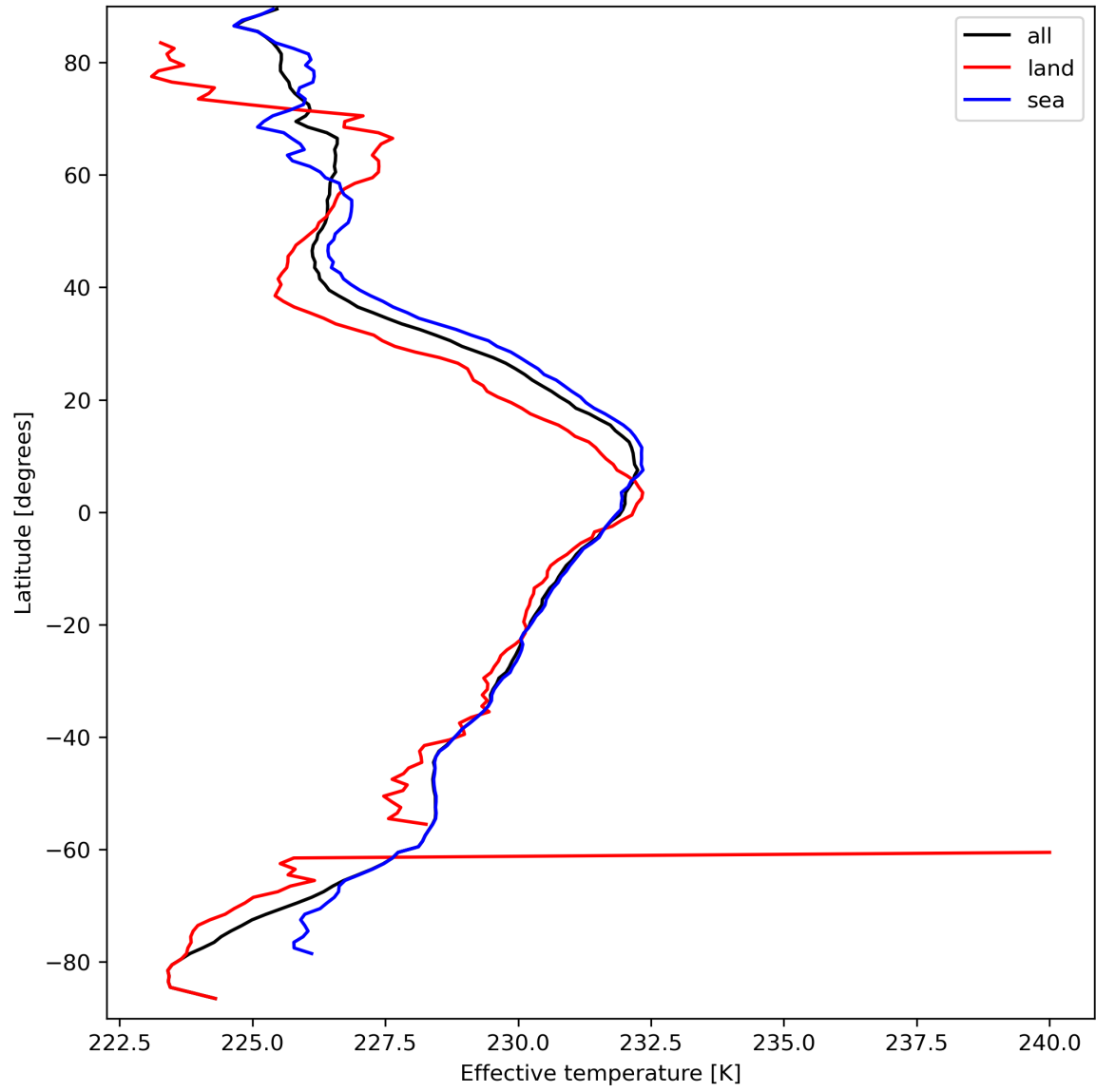
Figure 17: Zonal average of “Effective temperature” for 2024-03-25 to 2024-03-27.
