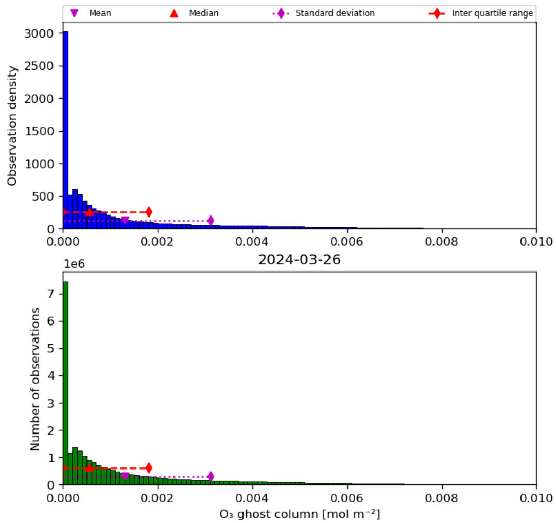
Figure 25: Histogram of “O 3 ghost column” for 2024-03-25 to 2024-03-27
