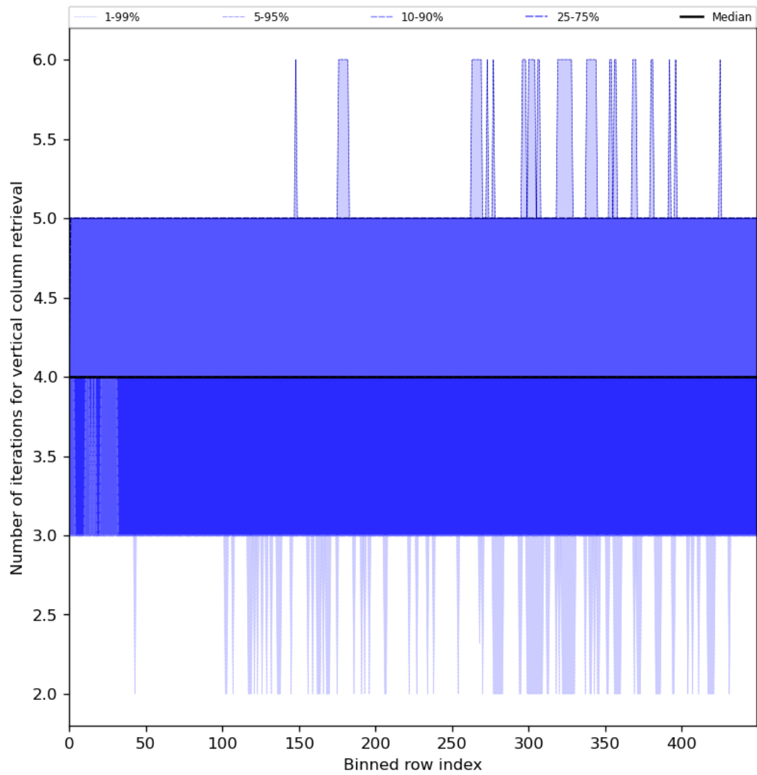
Figure 33: Along track statistics of “Number of iterations for vertical column retrieval” for 2024-03-25 to 2024-03-27
