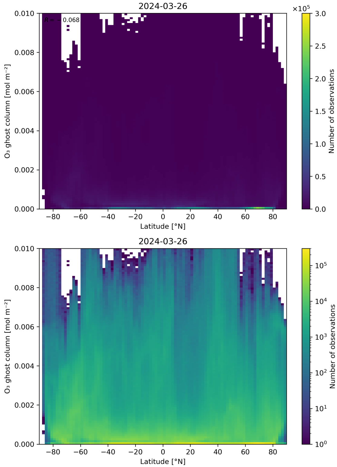
Figure 35: Scatter density plot of “Latitude” against “O 3 ghost column” for 2024-03-25 to 2024-03-27.
