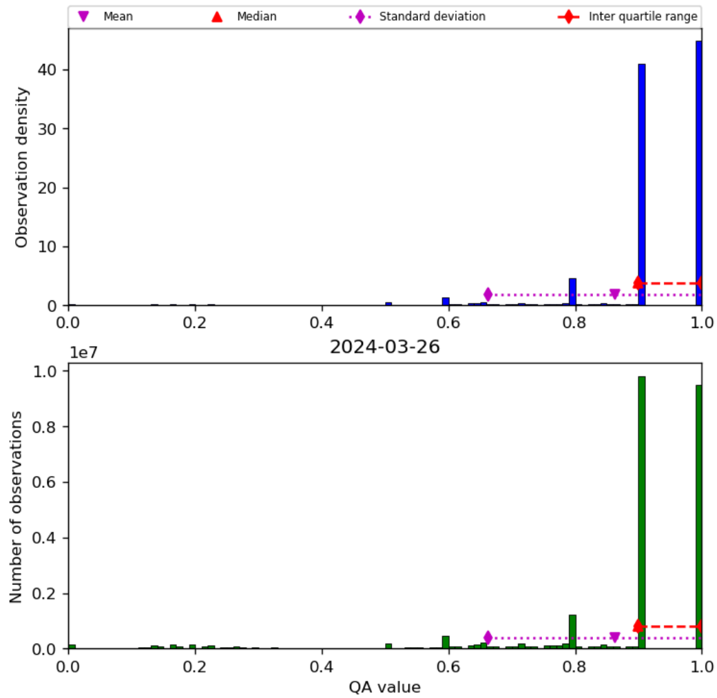
Figure 20: Histogram of “QA value” for 2024-03-25 to 2024-03-27
