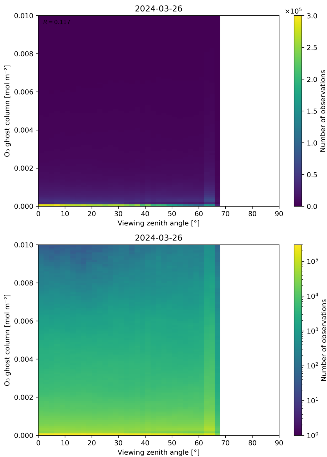
Figure 51: Scatter density plot of “Viewing zenith angle” against “O 3 ghost column” for 2024-03-25 to 2024-03-27.
