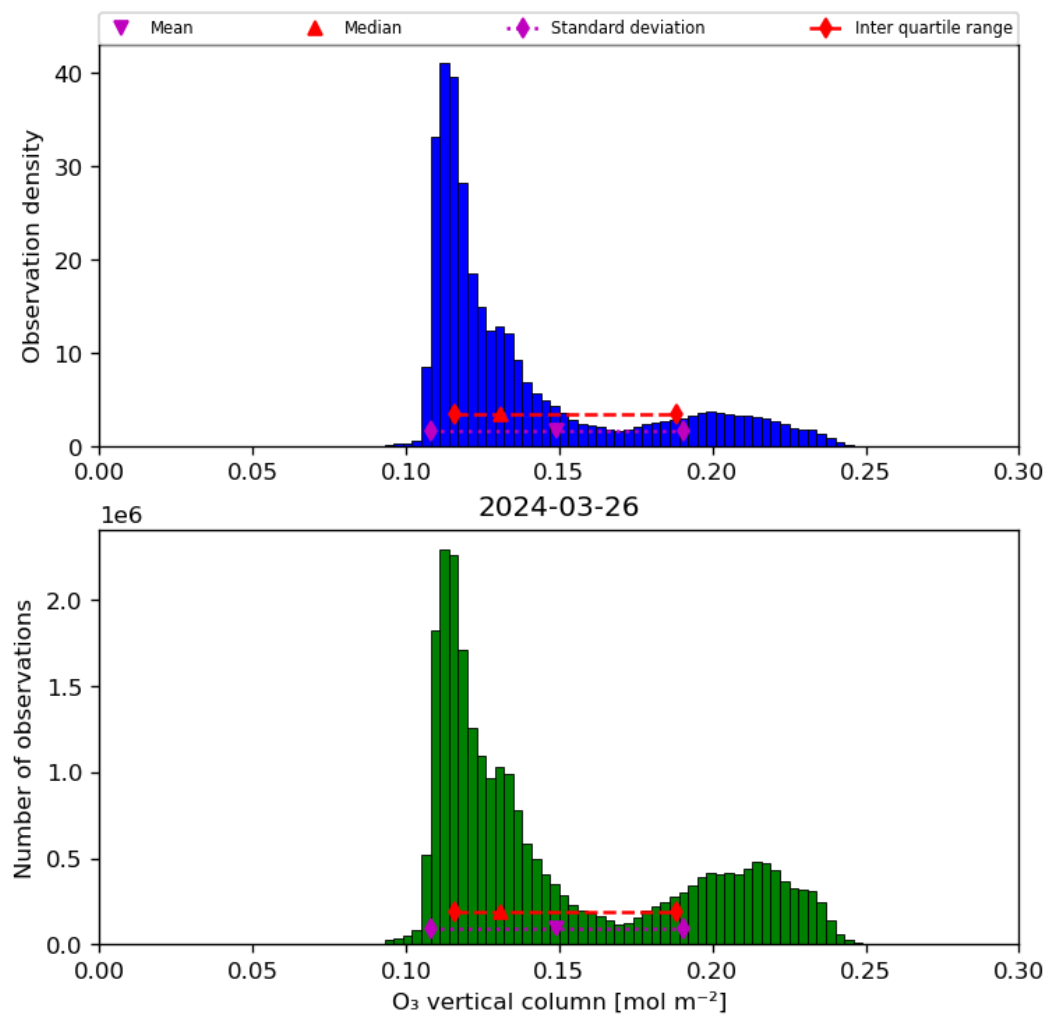
Figure 21: Histogram of “O 3 vertical column” for 2024-03-25 to 2024-03-27
