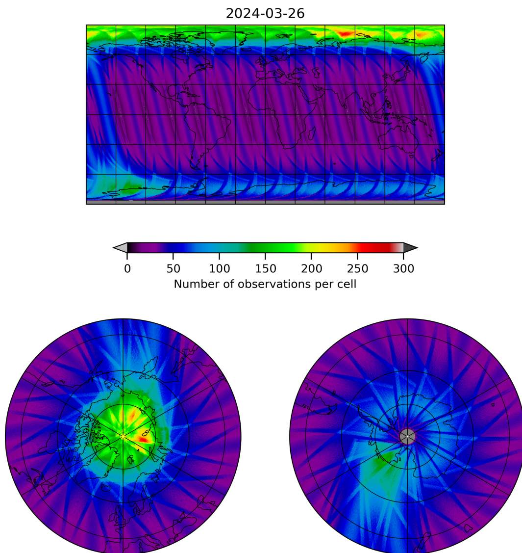
Figure 12: Map of the number of observations for 2024-03-25 to 2024-03-27
