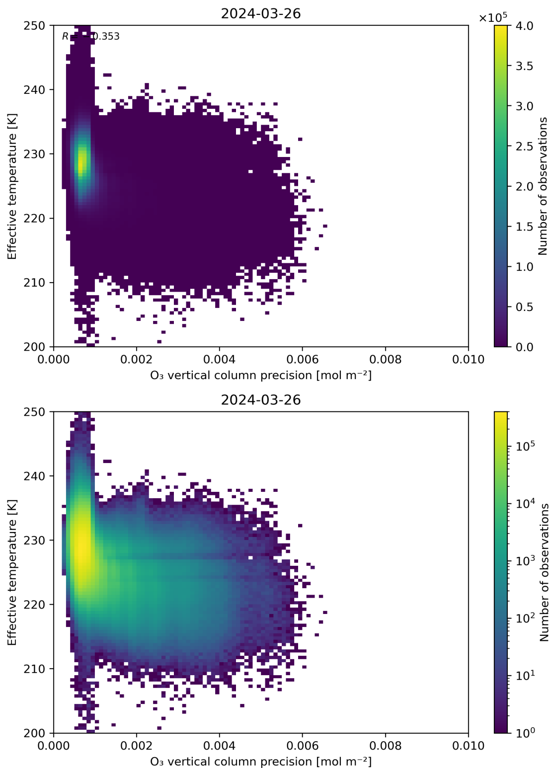
Figure 42: Scatter density plot of “O 3 vertical column precision” against “Effective temperature” for 2024-03-25 to 2024-03-27.
