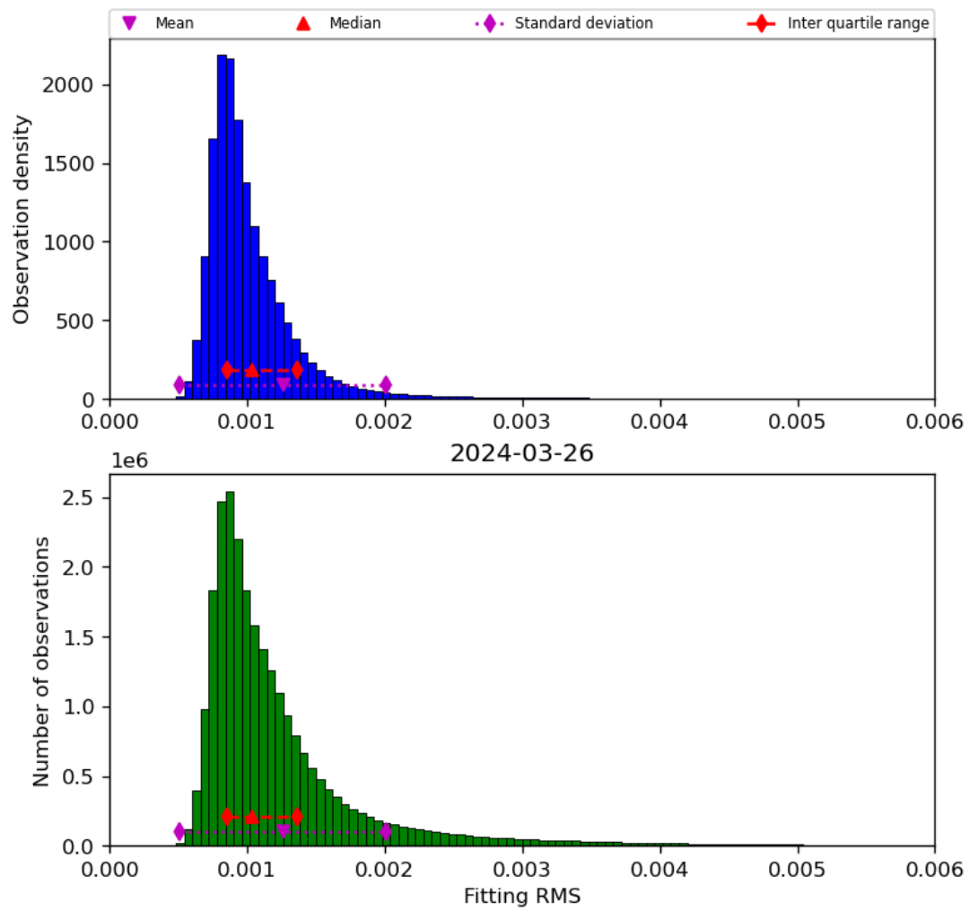
Figure 23: Histogram of “Fitting RMS” for 2024-03-25 to 2024-03-27
