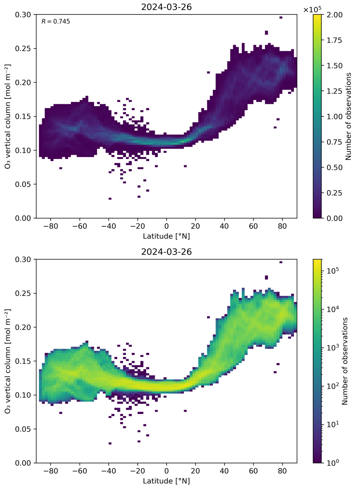
Figure 36: Scatter density plot of “Latitude” against “O 3 vertical column” for 2024-03-25 to 2024-03-27.
