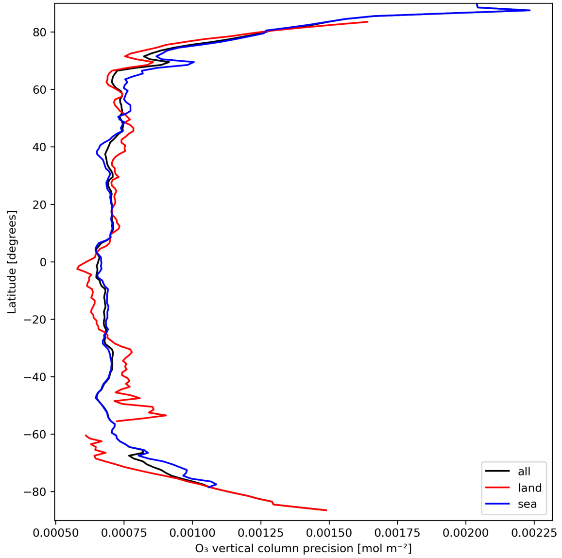
Figure 15: Zonal average of “O 3 vertical column precision” for 2024-03-25 to 2024-03-27.
