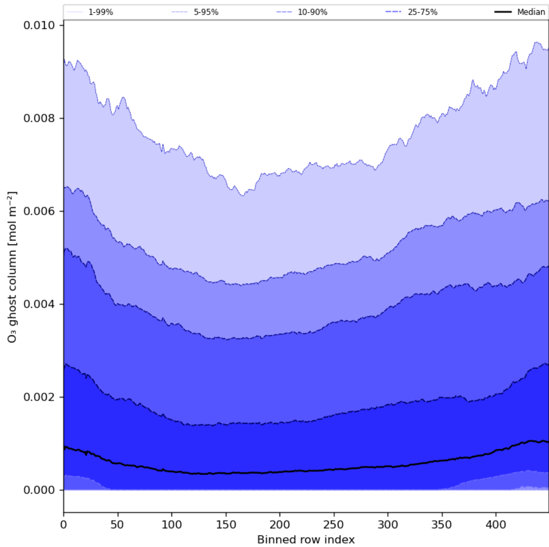
Figure 32: Along track statistics of “O 3 ghost column” for 2024-03-25 to 2024-03-27
