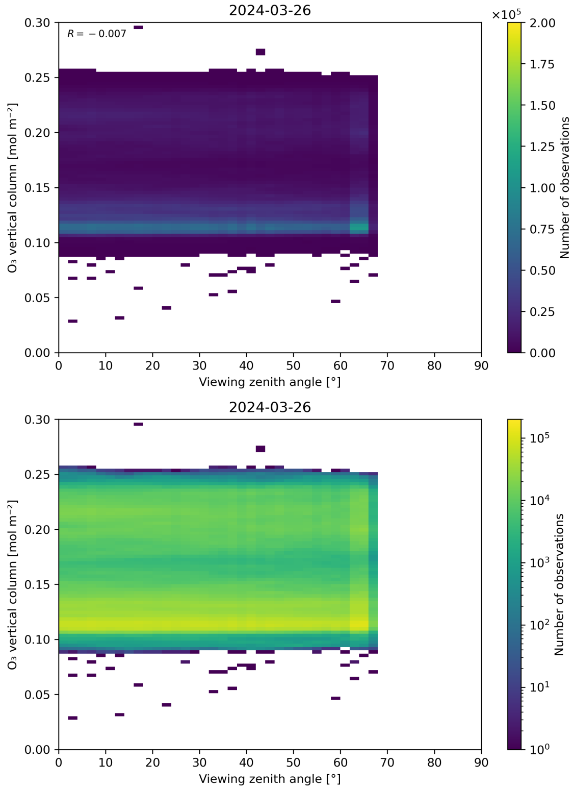
Figure 52: Scatter density plot of “Viewing zenith angle” against “O 3 vertical column” for 2024-03-25 to 2024-03-27.
