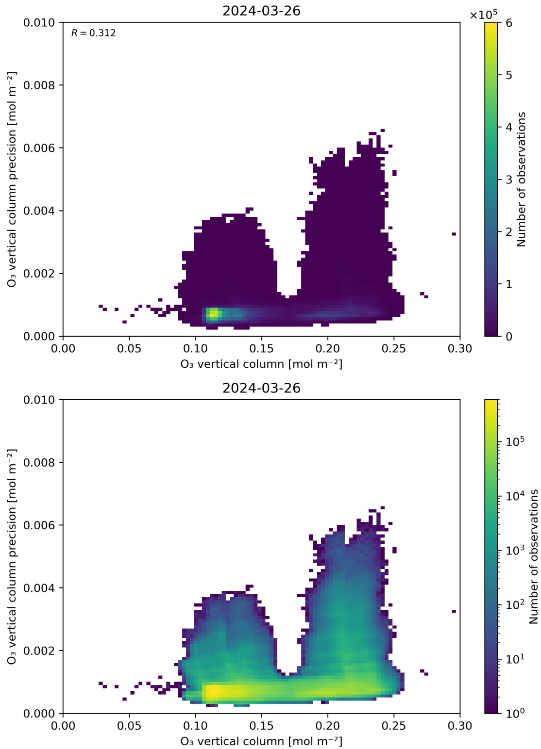
Figure 41: Scatter density plot of “O 3 vertical column” against “O 3 vertical column precision” for 2024-03-25 to 2024-03-27.
