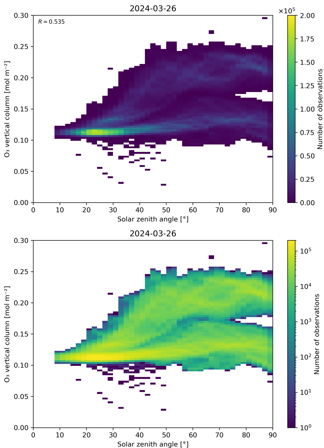
Figure 47: Scatter density plot of “Solar zenith angle” against “O 3 vertical column” for 2024-03-25 to 2024-03-27.
