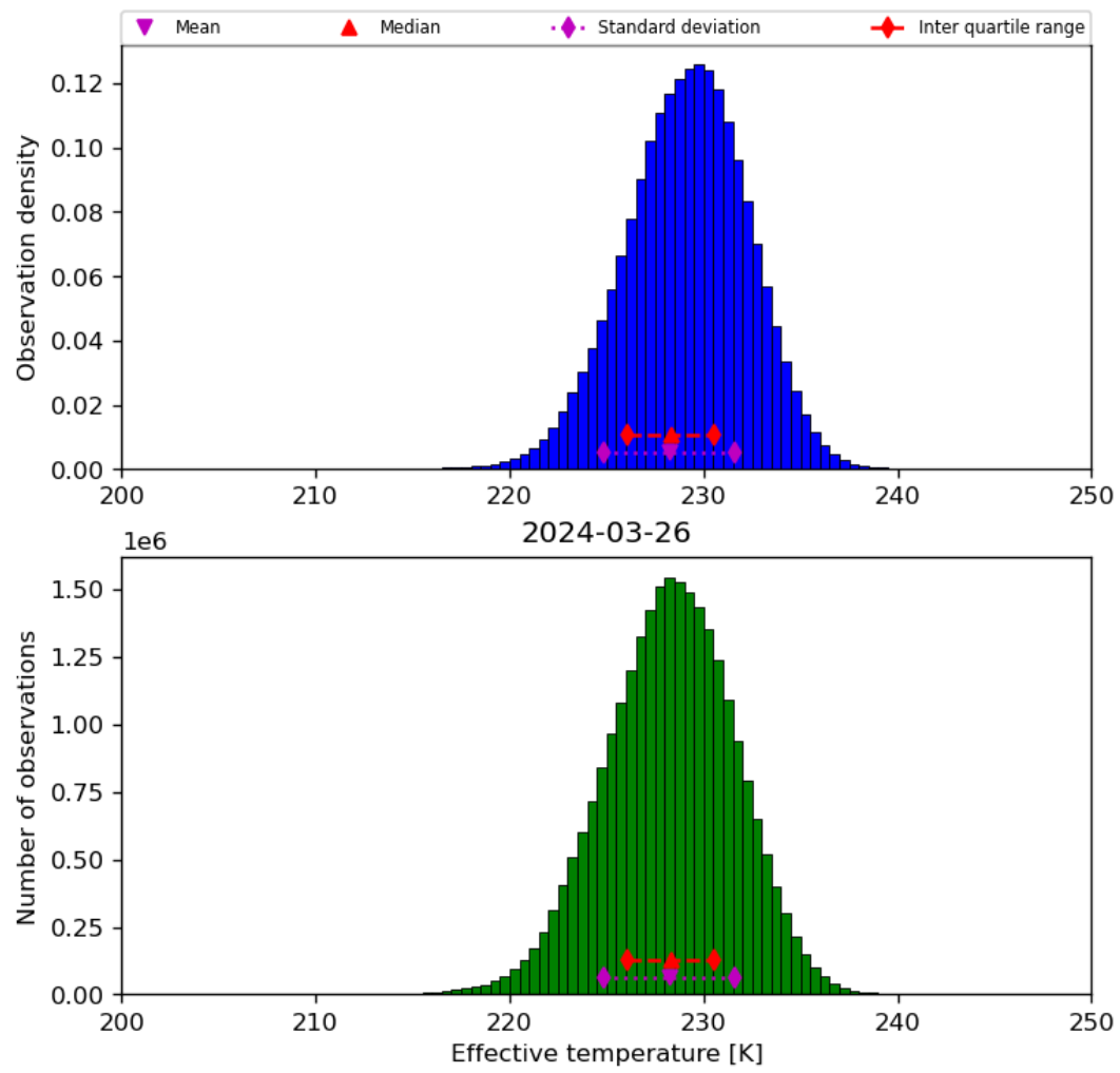
Figure 24: Histogram of “Effective temperature” for 2024-03-25 to 2024-03-27
