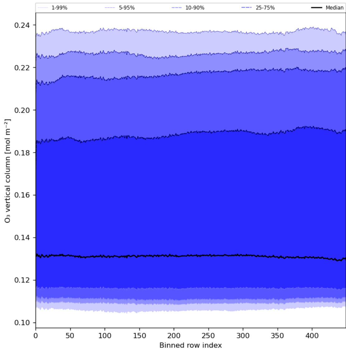
Figure 28: Along track statistics of “O 3 vertical column” for 2024-03-25 to 2024-03-27
