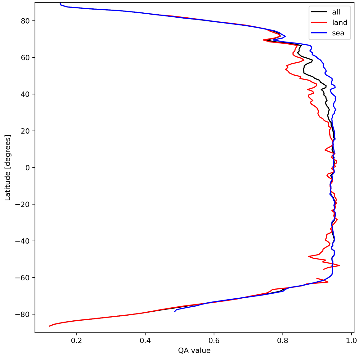
Figure 13: Zonal average of “QA value” for 2024-03-25 to 2024-03-27.
