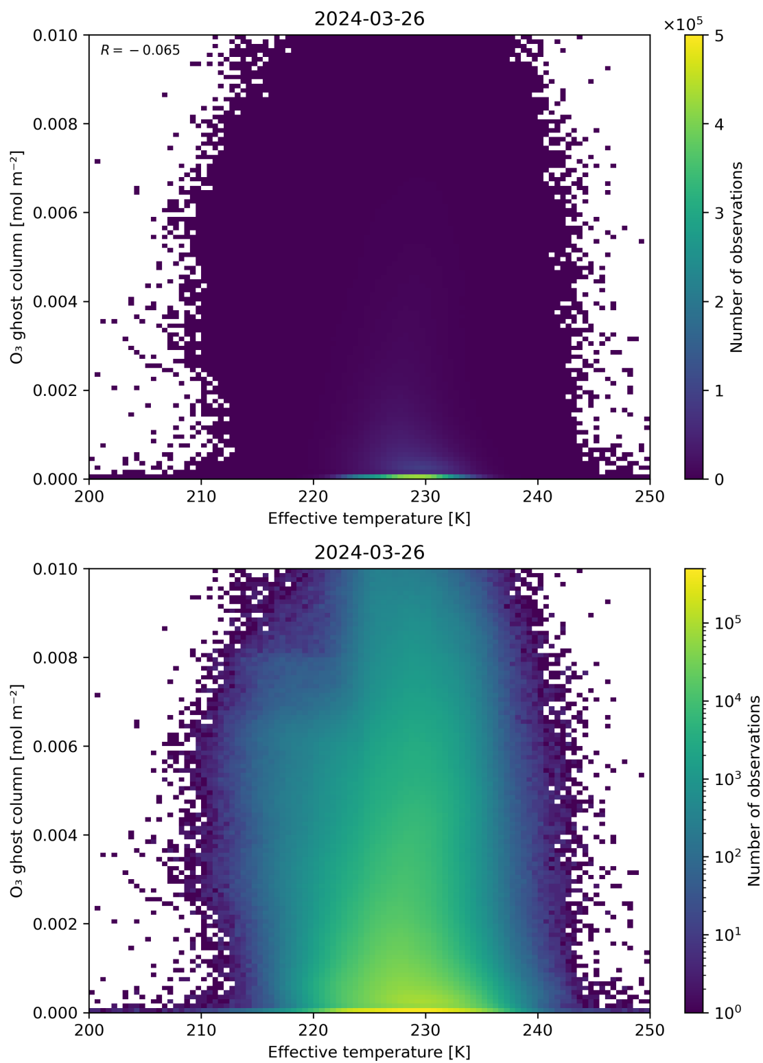
Figure 38: Scatter density plot of “Effective temperature” against “O 3 ghost column” for 2024-03-25 to 2024-03-27.
