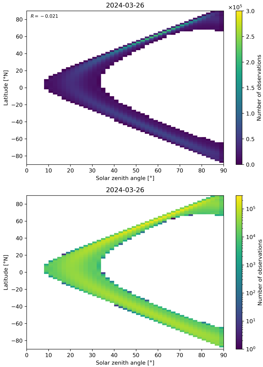
Figure 44: Scatter density plot of “Solar zenith angle” against “Latitude” for 2024-03-25 to 2024-03-27.
