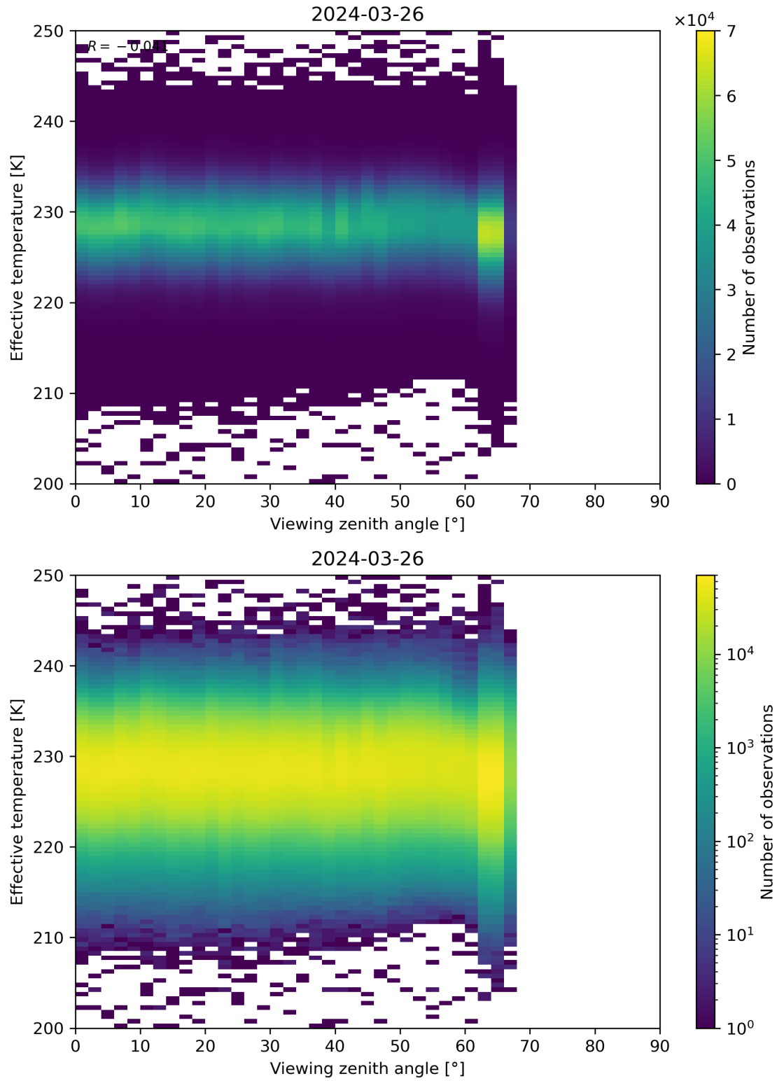
Figure 50: Scatter density plot of “Viewing zenith angle” against “Effective temperature” for 2024-03-25 to 2024-03-27.
