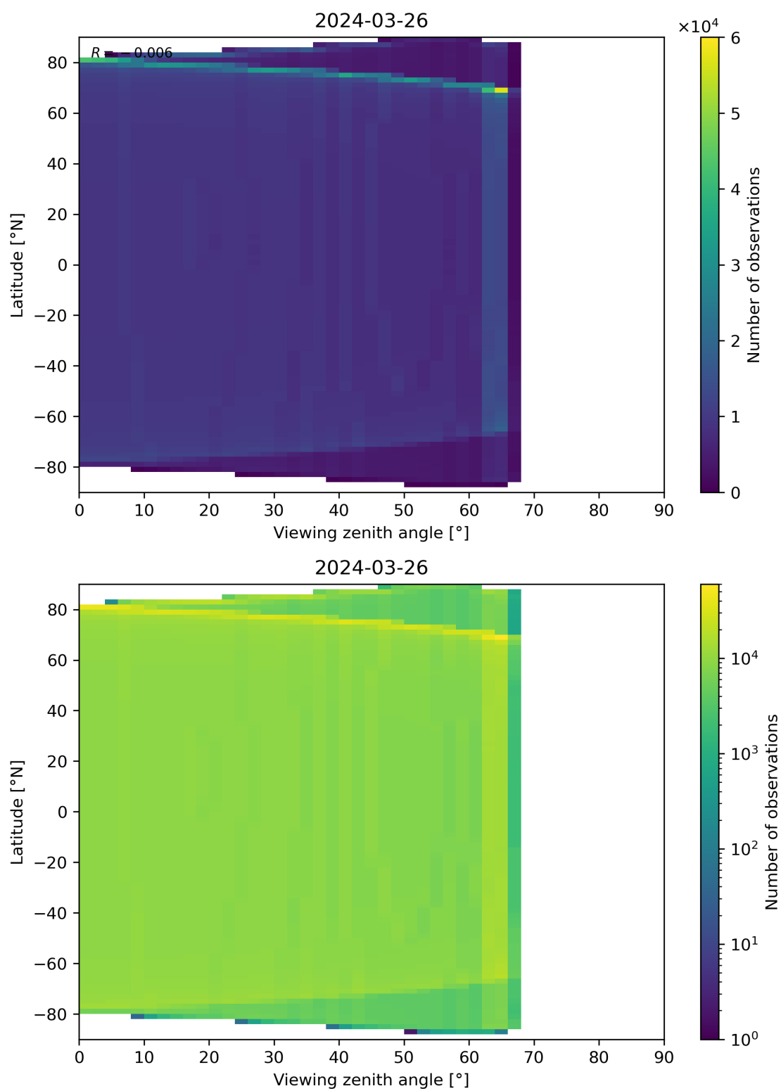
Figure 49: Scatter density plot of “Viewing zenith angle” against “Latitude” for 2024-03-25 to 2024-03-27.
