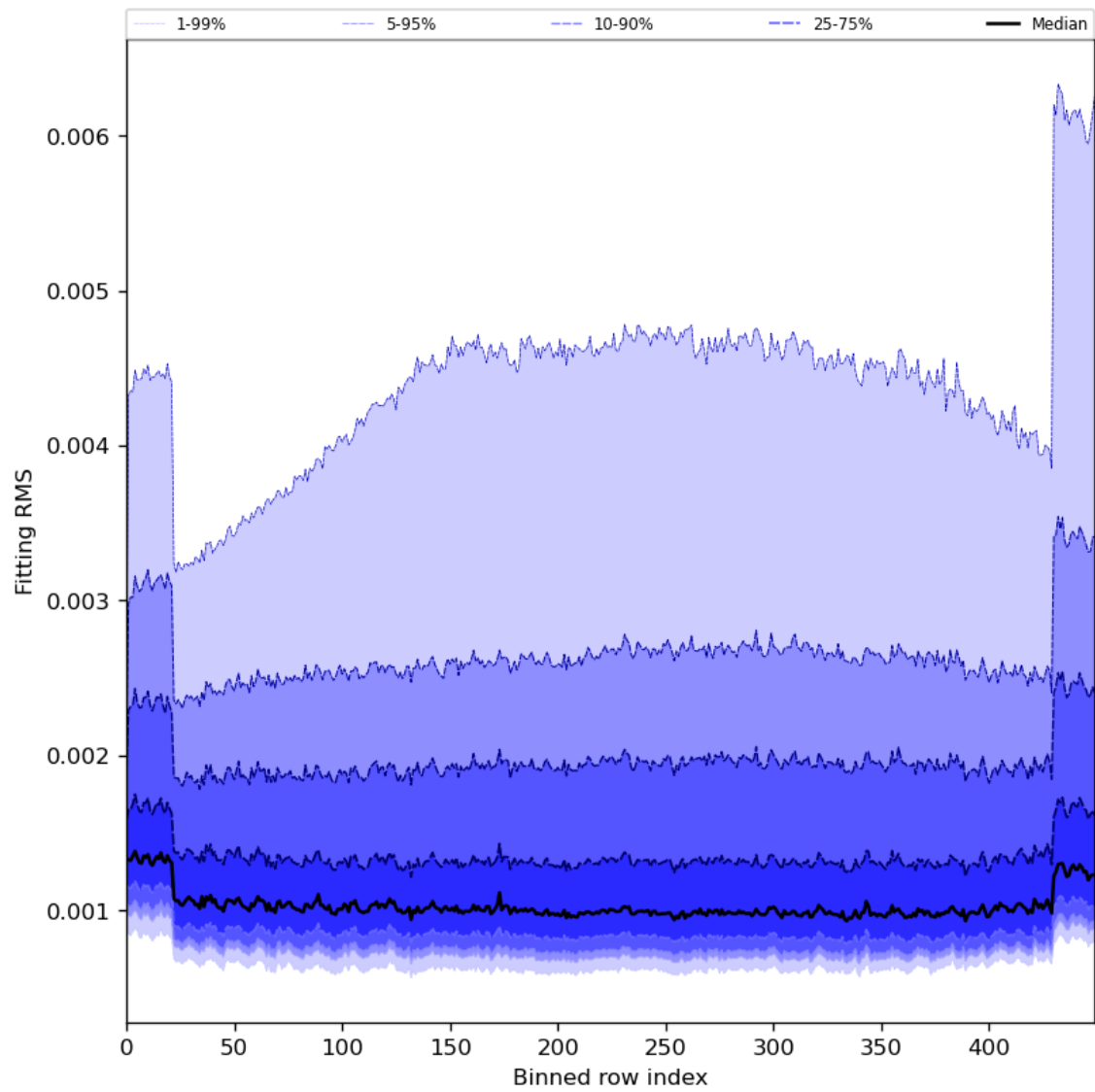
Figure 30: Along track statistics of “Fitting RMS” for 2024-03-25 to 2024-03-27
