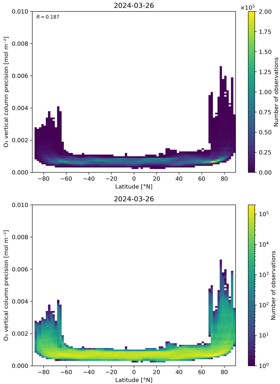
Figure 37: Scatter density plot of “Latitude” against “O 3 vertical column precision” for 2024-03-25 to 2024-03-27.
