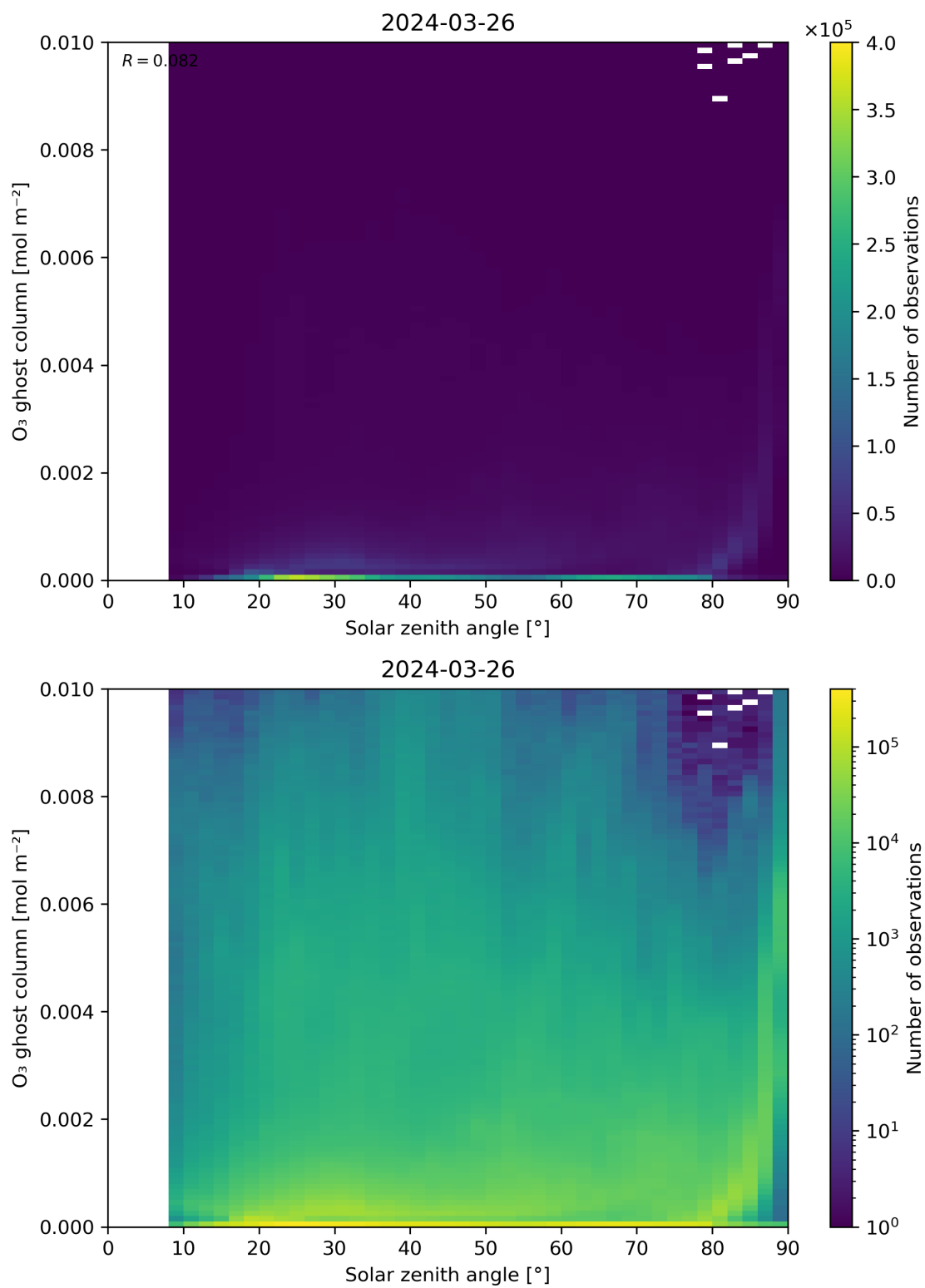
Figure 46: Scatter density plot of “Solar zenith angle” against “O 3 ghost column” for 2024-03-25 to 2024-03-27.
