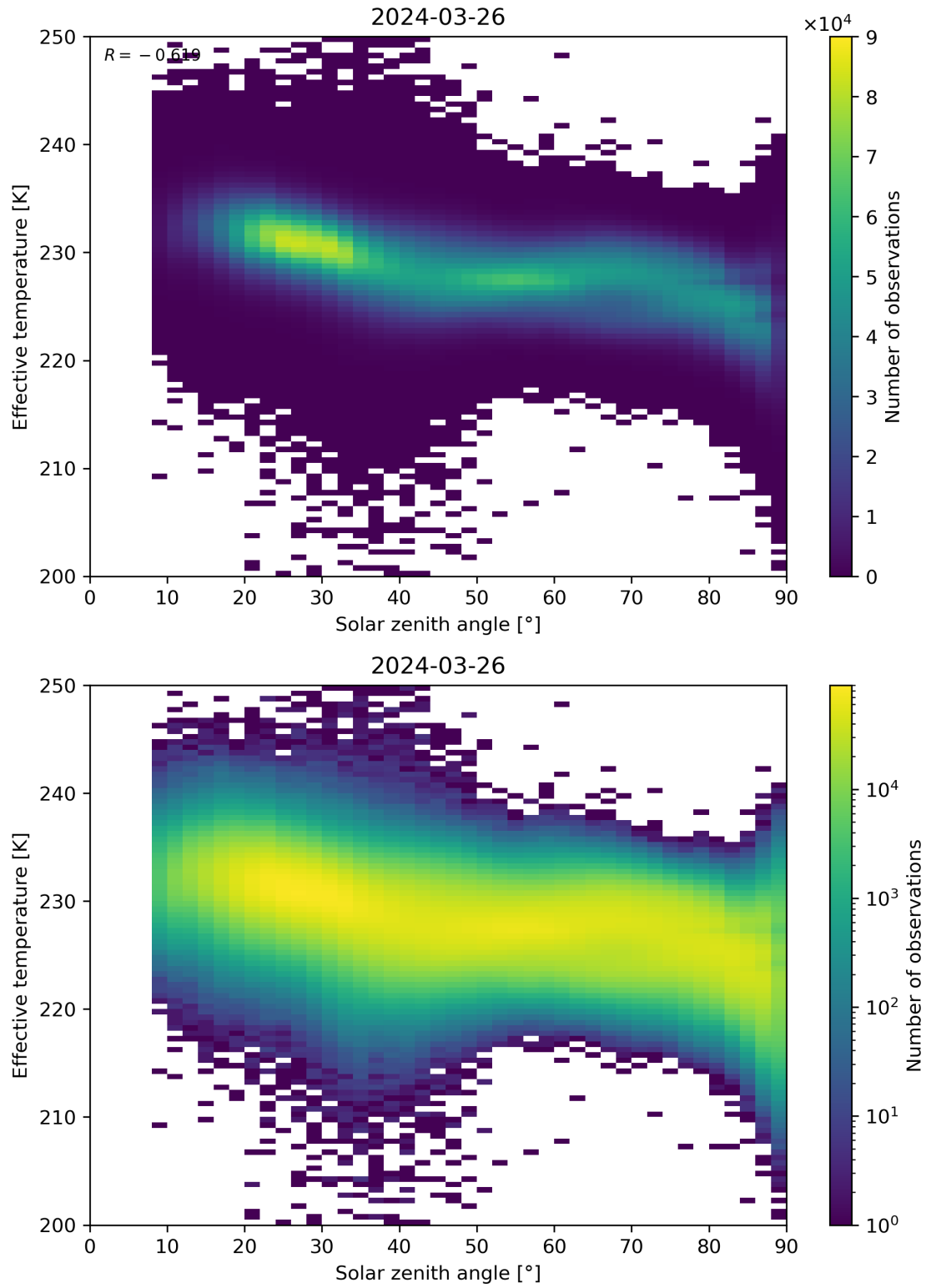
Figure 45: Scatter density plot of “Solar zenith angle” against “Effective temperature” for 2024-03-25 to 2024-03-27.
