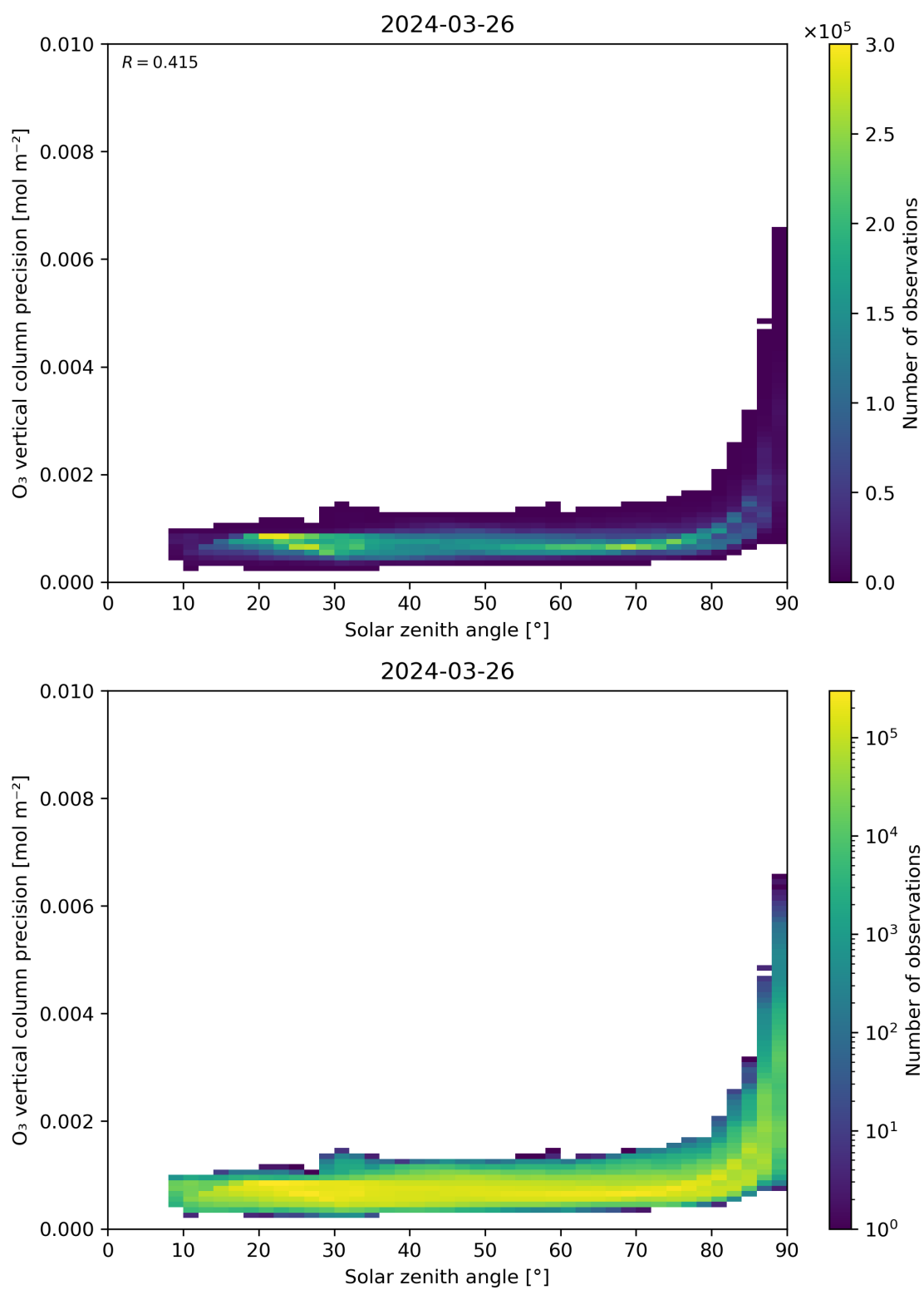
Figure 48: Scatter density plot of “Solar zenith angle” against “O 3 vertical column precision” for 2024-03-25 to 2024-03-27.
