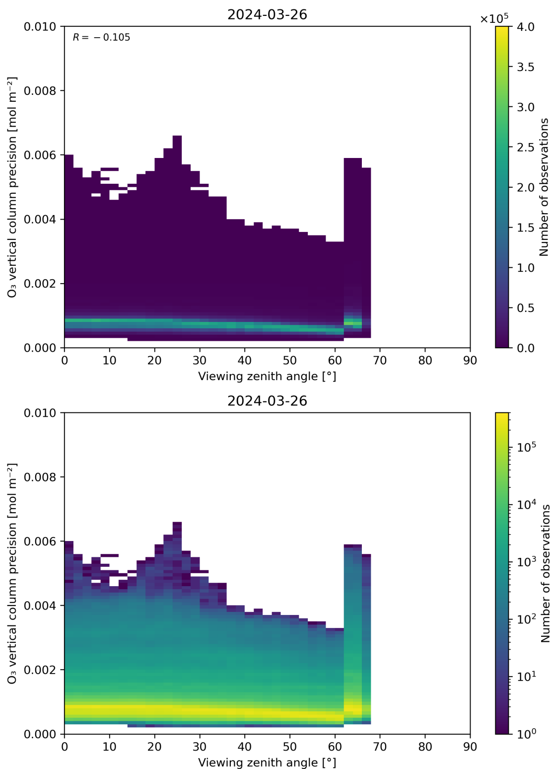
Figure 53: Scatter density plot of “Viewing zenith angle” against “O 3 vertical column precision” for 2024-03-25 to 2024-03-27.
