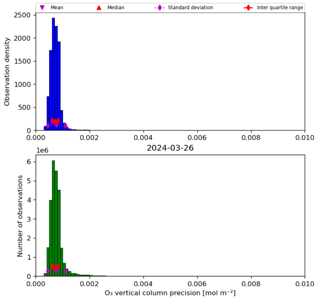
Figure 22: Histogram of “O 3 vertical column precision” for 2024-03-25 to 2024-03-27
