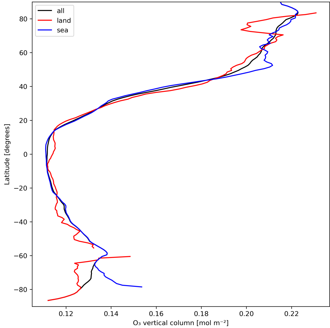
Figure 14: Zonal average of “O 3 vertical column” for 2024-03-25 to 2024-03-27.
