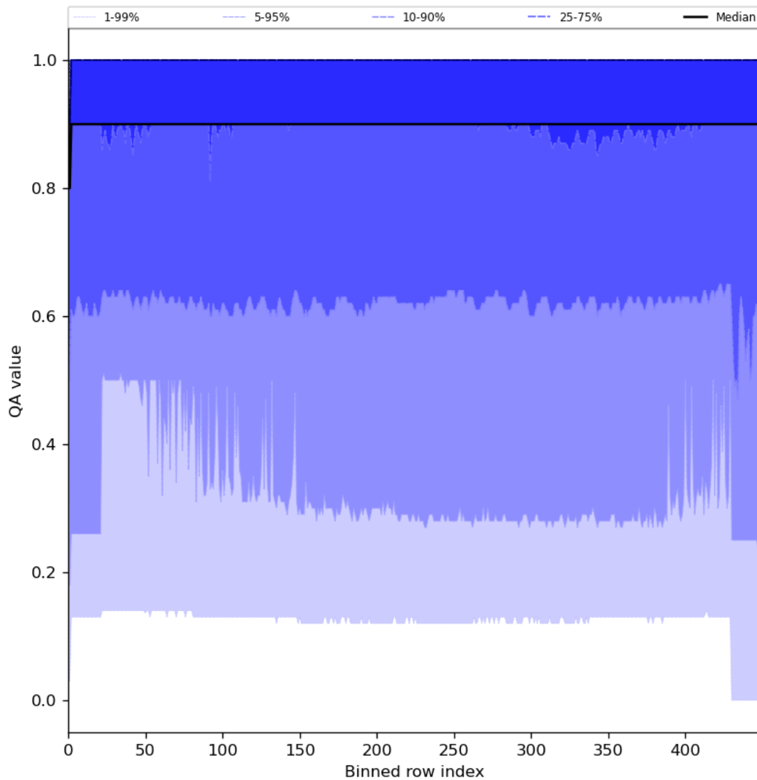
Figure 27: Along track statistics of “QA value” for 2024-03-25 to 2024-03-27
