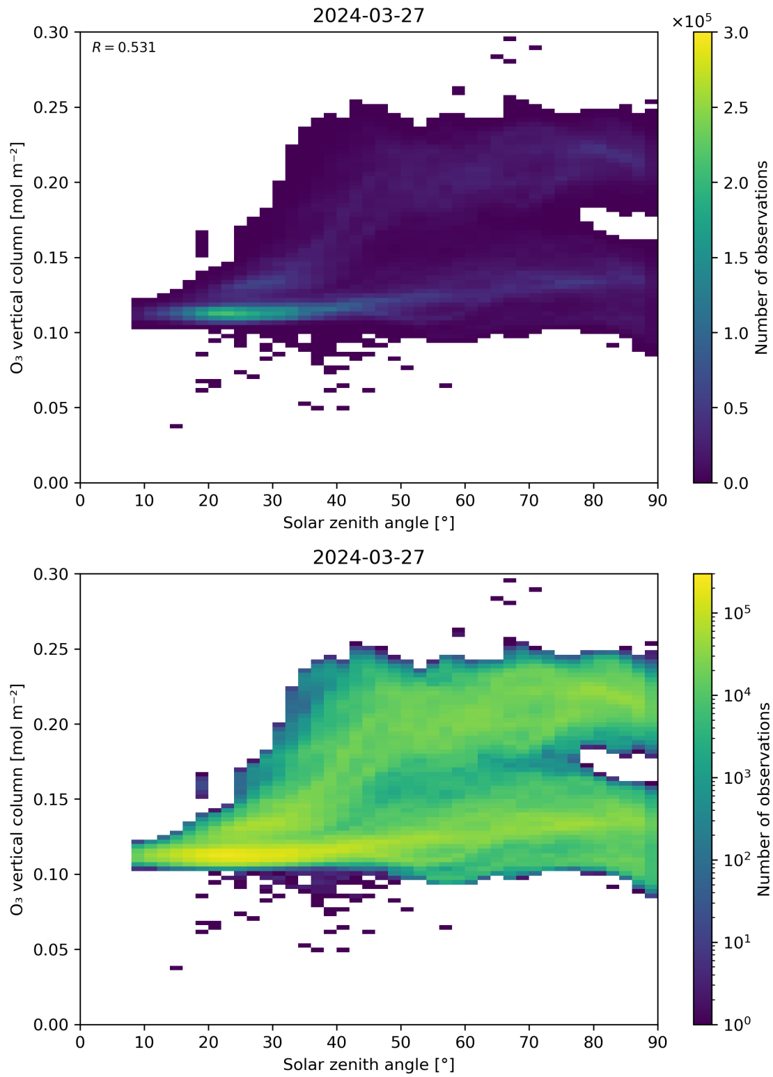
Figure 47: Scatter density plot of “Solar zenith angle” against “O 3 vertical column” for 2024-03-26 to 2024-03-28.
