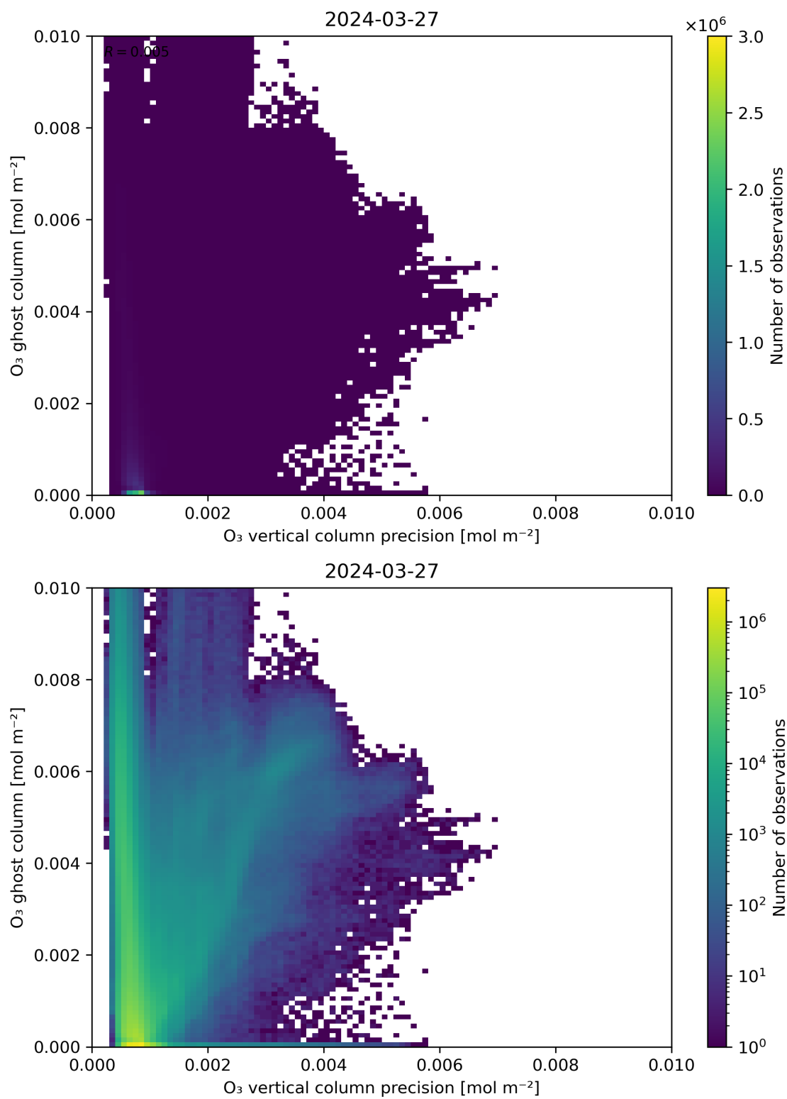
Figure 43: Scatter density plot of “O 3 vertical column precision” against “O 3 ghost column” for 2024-03-26 to 2024-03-28.
