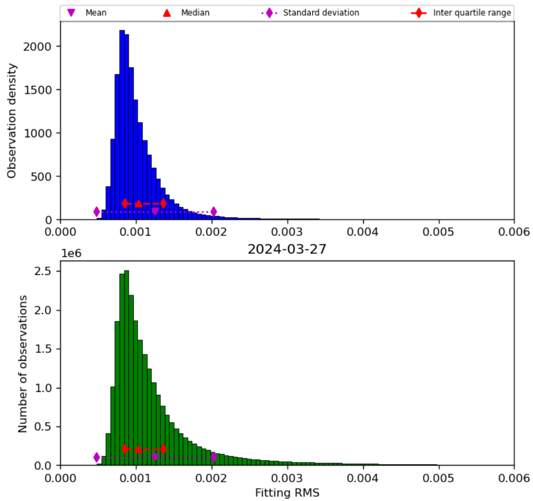
Figure 23: Histogram of “Fitting RMS” for 2024-03-26 to 2024-03-28
