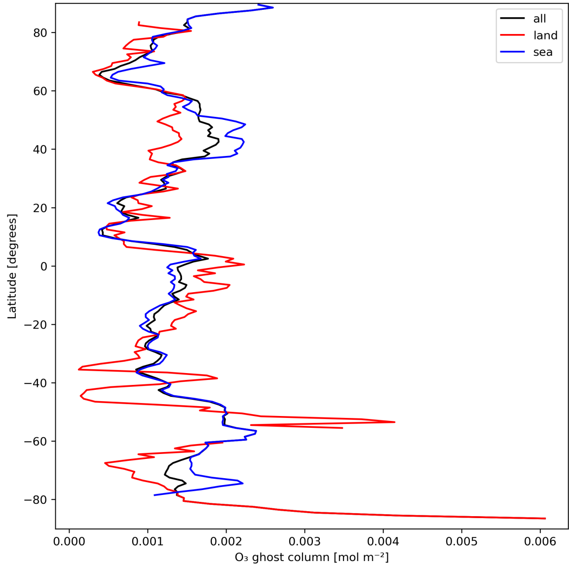
Figure 18: Zonal average of "O 3 ghost column" for 2024-03-26 to 2024-03-28.
