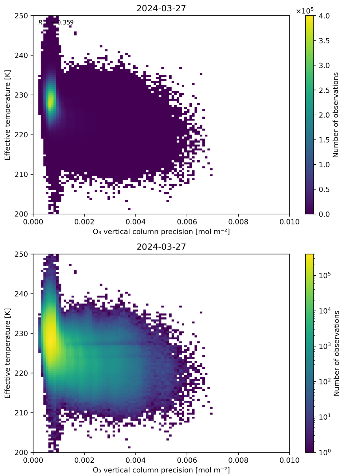
Figure 42: Scatter density plot of “O 3 vertical column precision” against “Effective temperature” for 2024-03-26 to 2024-03-28.
