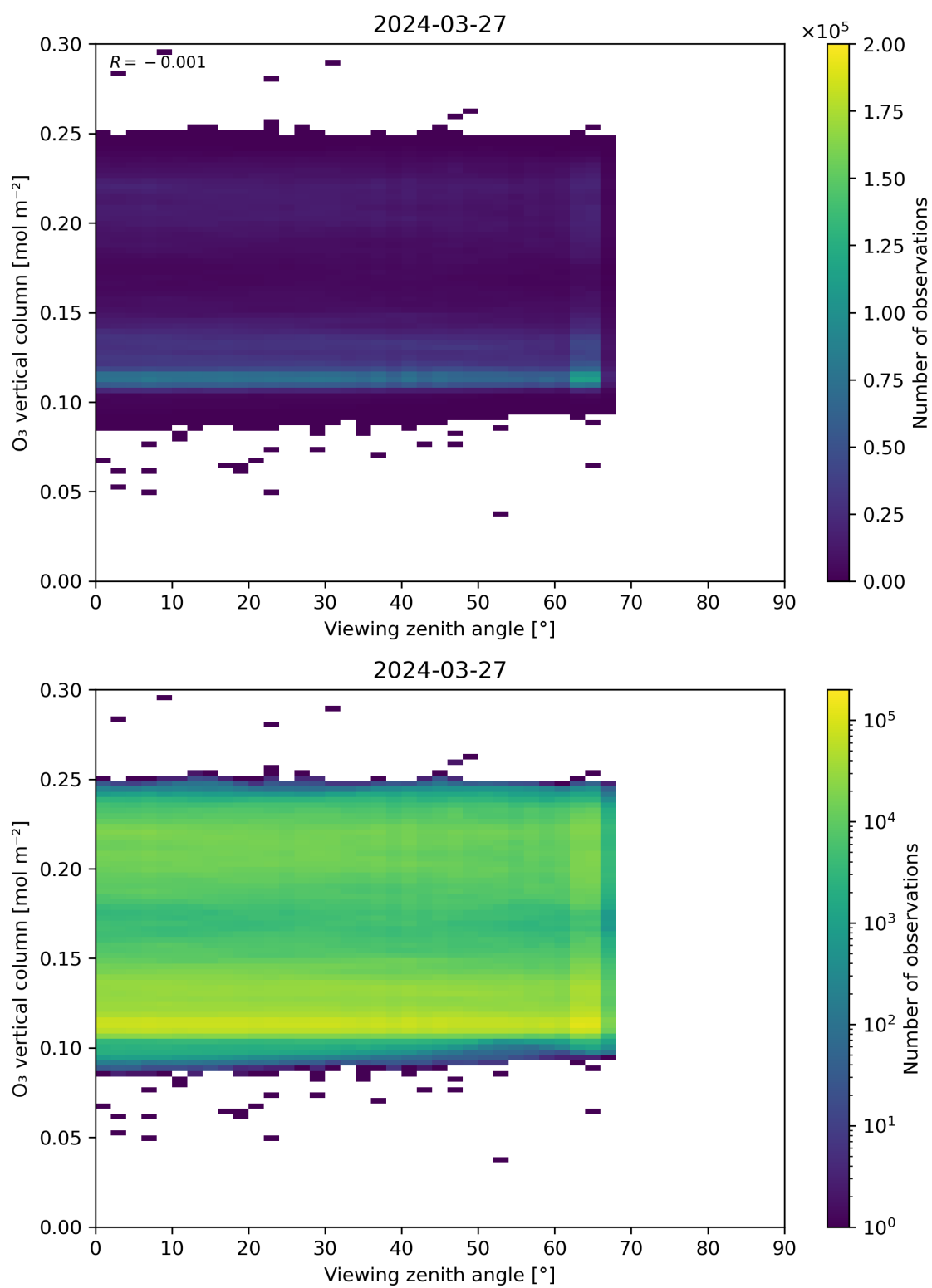
Figure 52: Scatter density plot of “Viewing zenith angle” against “O 3 vertical column” for 2024-03-26 to 2024-03-28.
