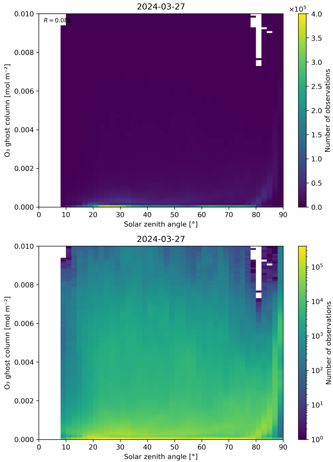
Figure 46: Scatter density plot of “Solar zenith angle” against “O 3 ghost column” for 2024-03-26 to 2024-03-28.
