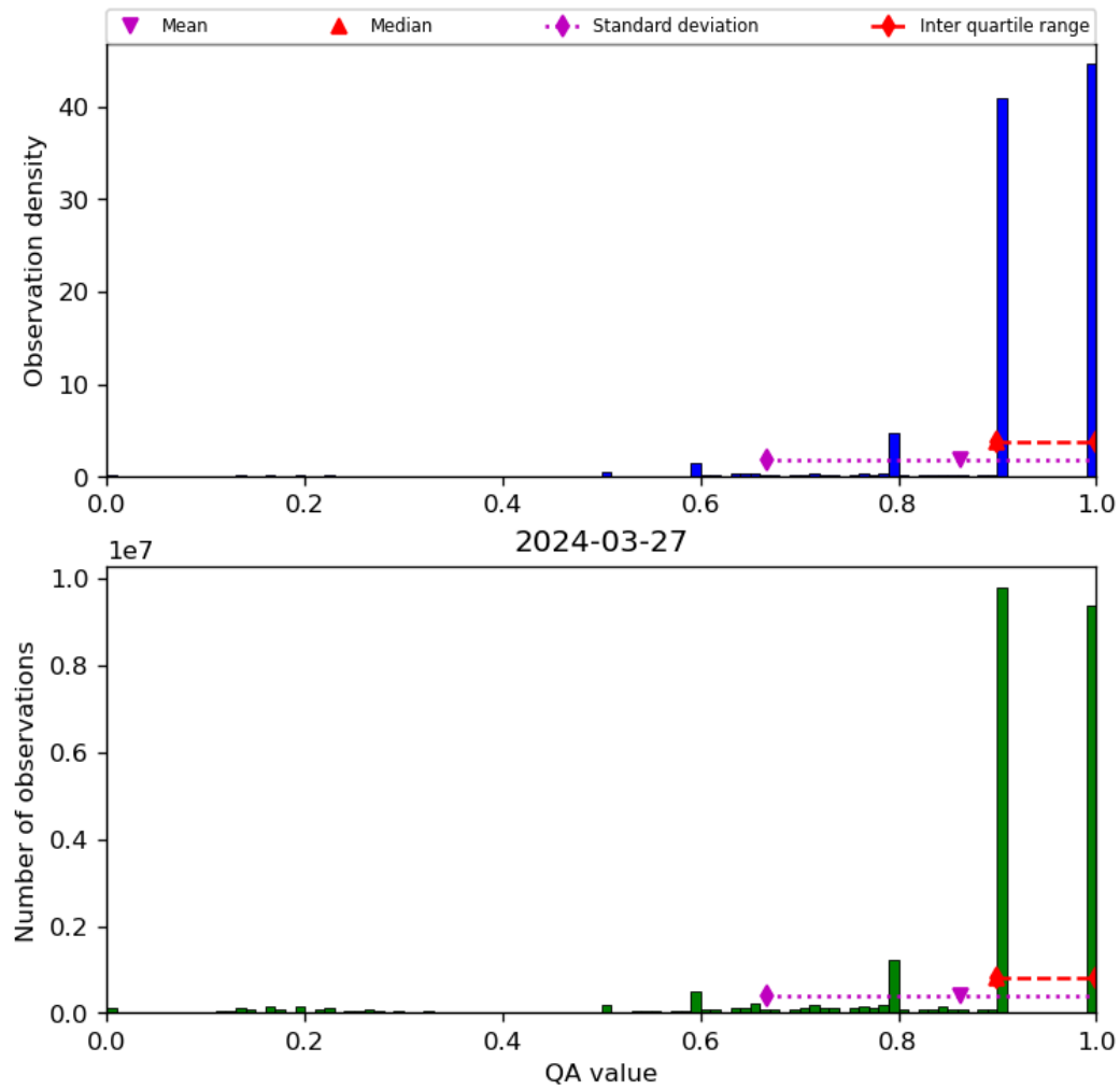
Figure 20: Histogram of “QA value” for 2024-03-26 to 2024-03-28
