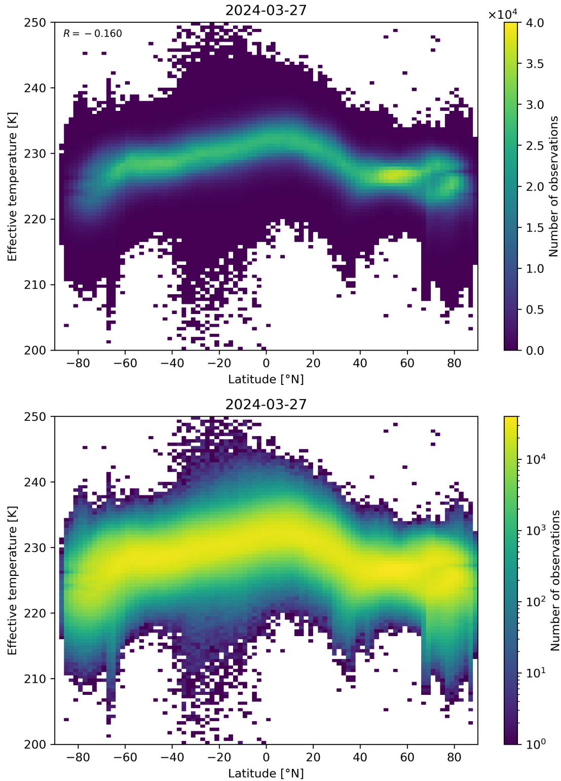
Figure 34: Scatter density plot of “Latitude” against “Effective temperature” for 2024-03-26 to 2024-03-28.
