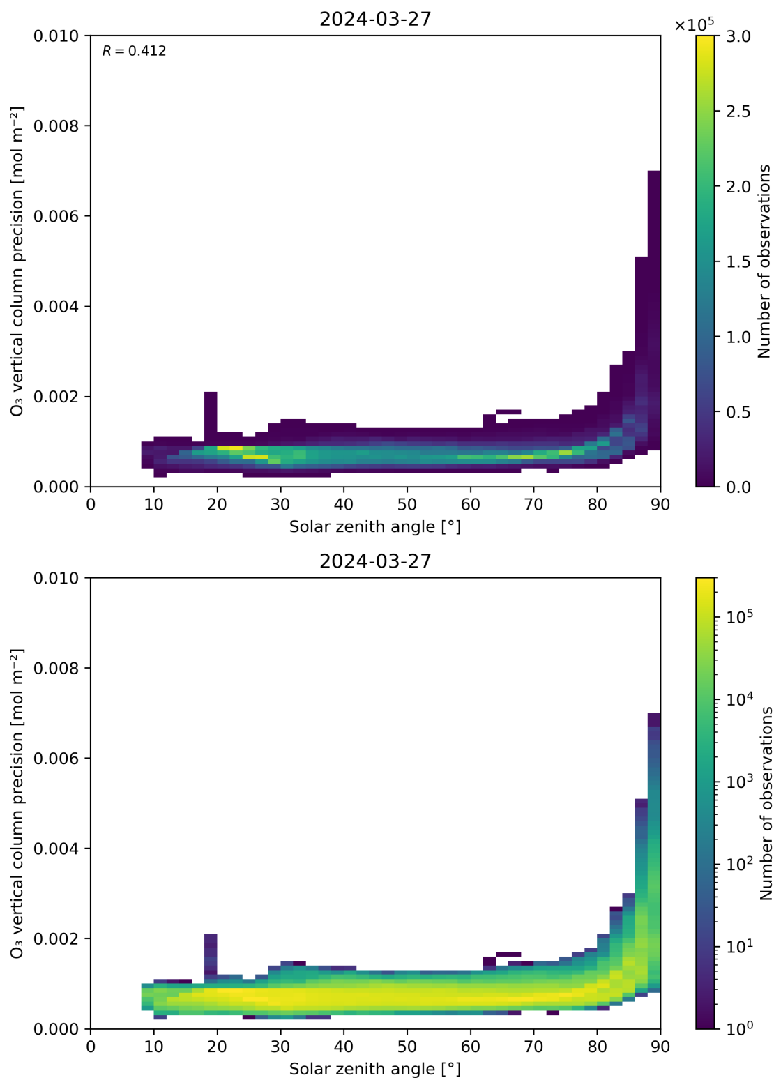
Figure 48: Scatter density plot of “Solar zenith angle” against “O 3 vertical column precision” for 2024-03-26 to 2024-03-28.
