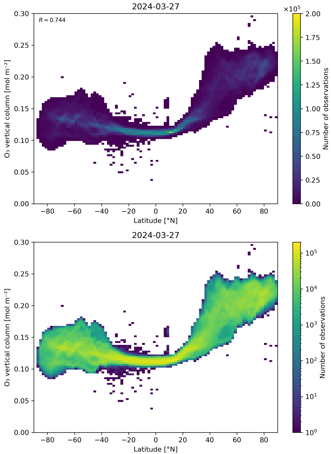
Figure 36: Scatter density plot of “Latitude” against “O 3 vertical column” for 2024-03-26 to 2024-03-28.
