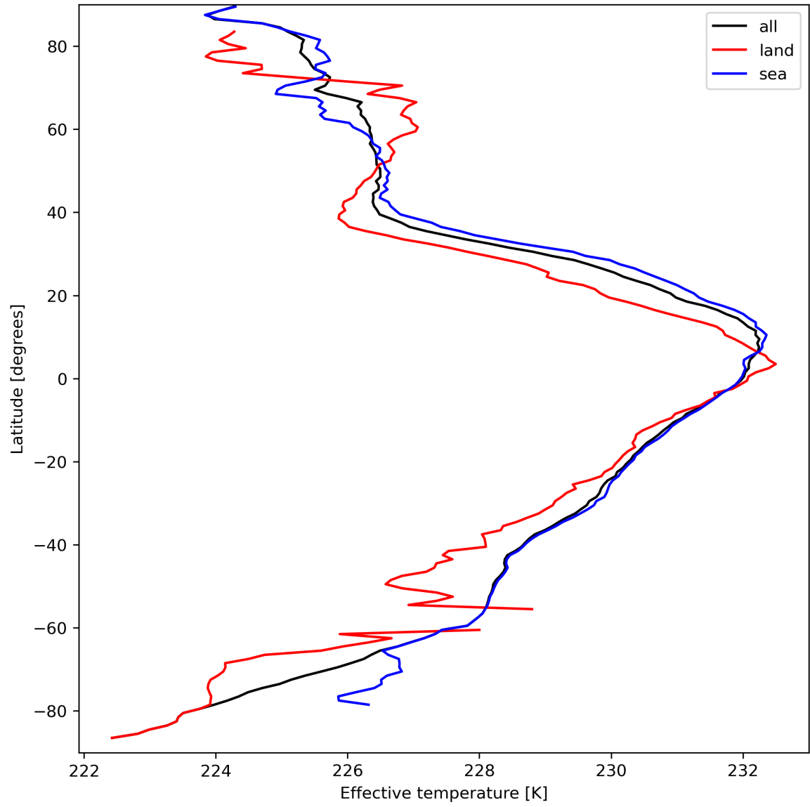
Figure 17: Zonal average of “Effective temperature” for 2024-03-26 to 2024-03-28.
