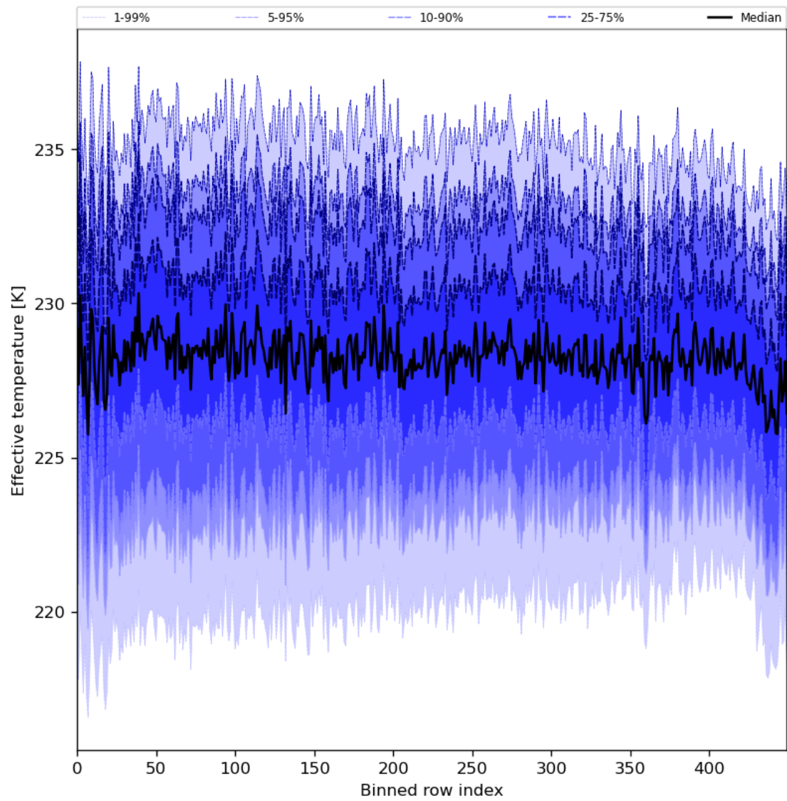
Figure 31: Along track statistics of “Effective temperature” for 2024-03-26 to 2024-03-28
