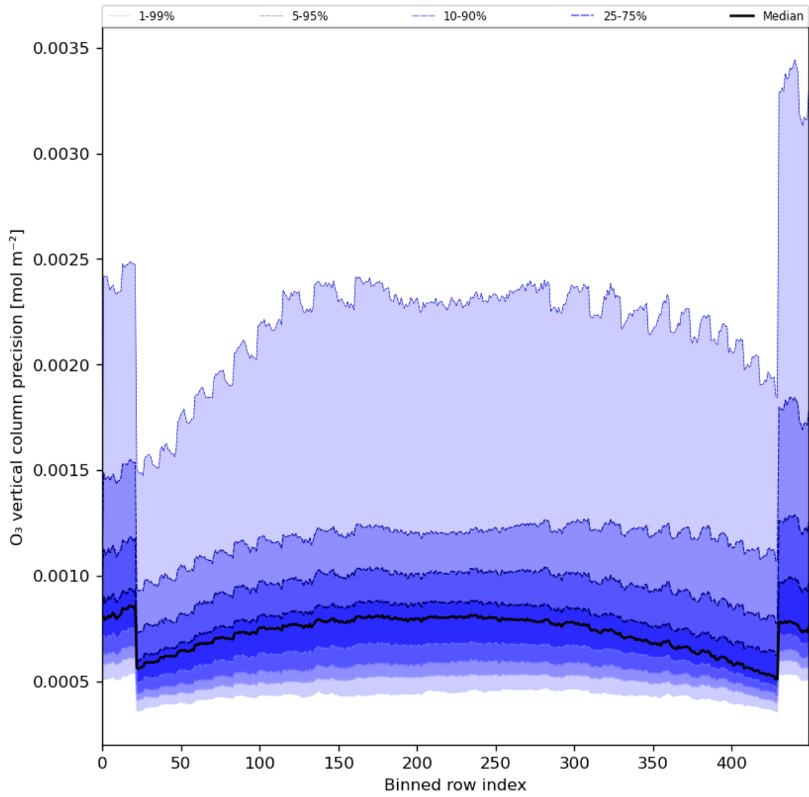
Figure 29: Along track statistics of “O 3 vertical column precision” for 2024-03-26 to 2024-03-28
