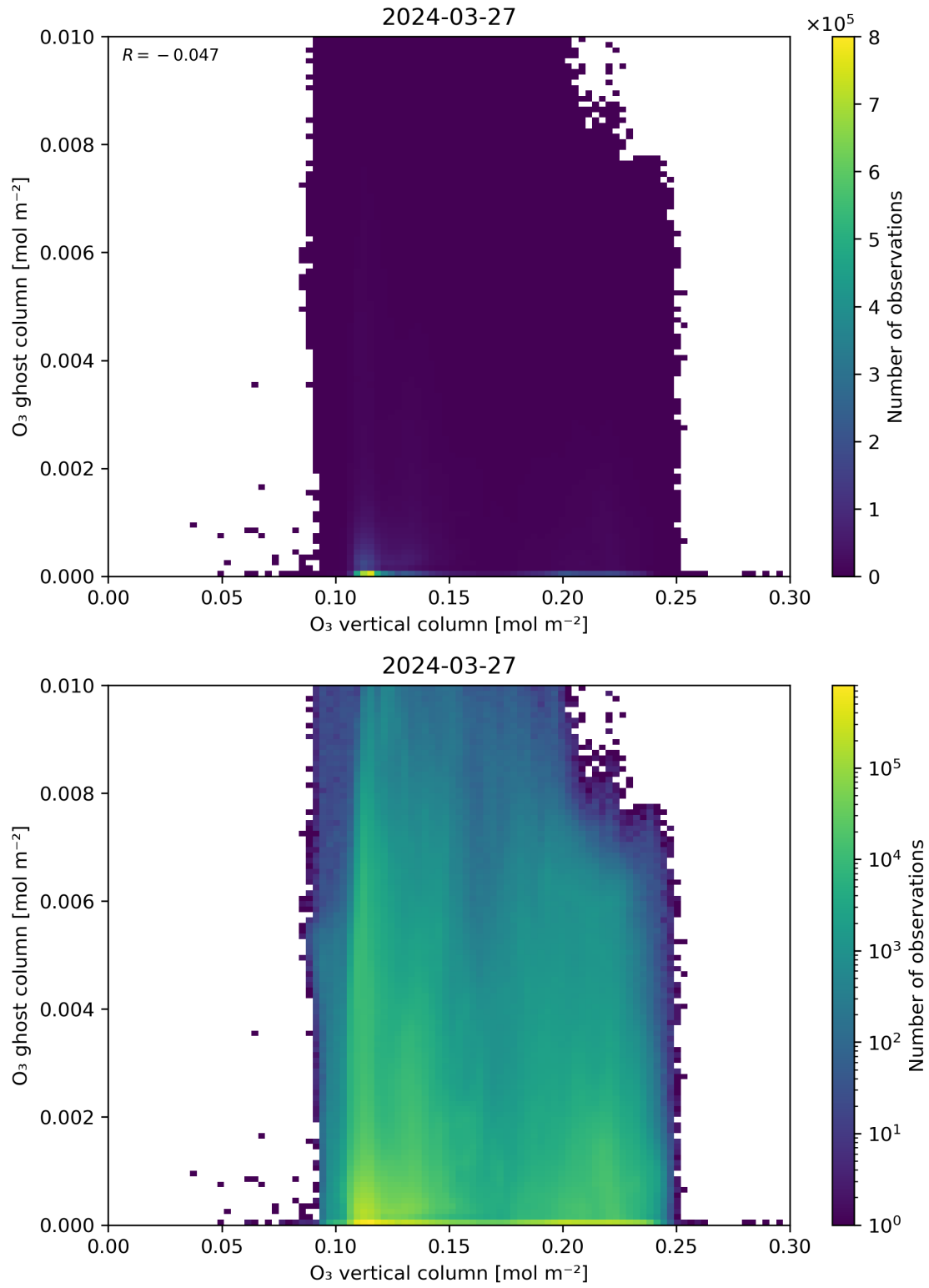
Figure 40: Scatter density plot of “O 3 vertical column” against “O 3 ghost column” for 2024-03-26 to 2024-03-28.
