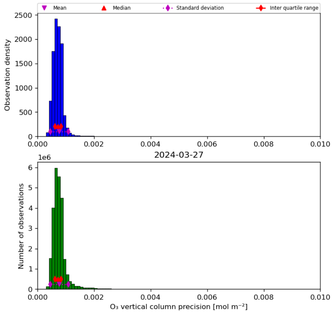
Figure 22: Histogram of “O 3 vertical column precision” for 2024-03-26 to 2024-03-28
