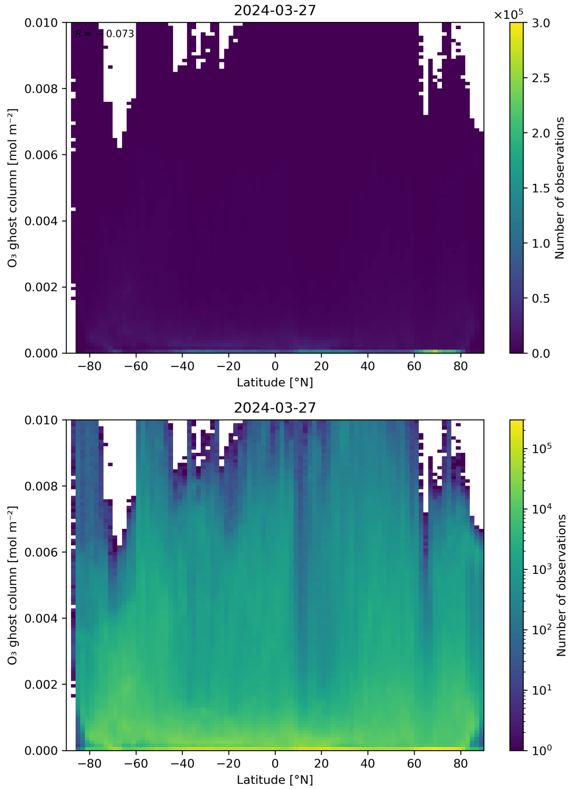
Figure 35: Scatter density plot of “Latitude” against “O 3 ghost column” for 2024-03-26 to 2024-03-28.
