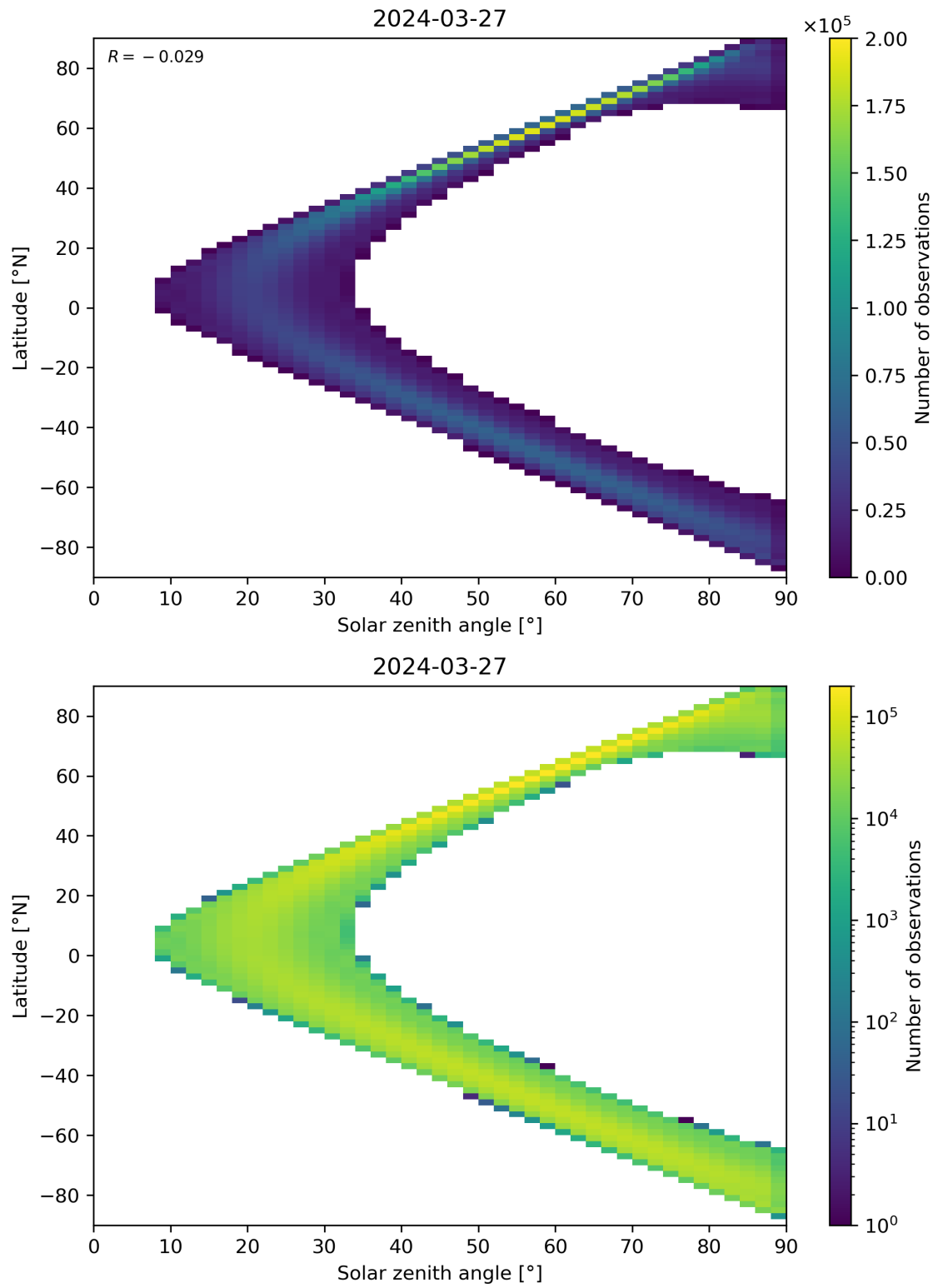
Figure 44: Scatter density plot of “Solar zenith angle” against “Latitude” for 2024-03-26 to 2024-03-28.
