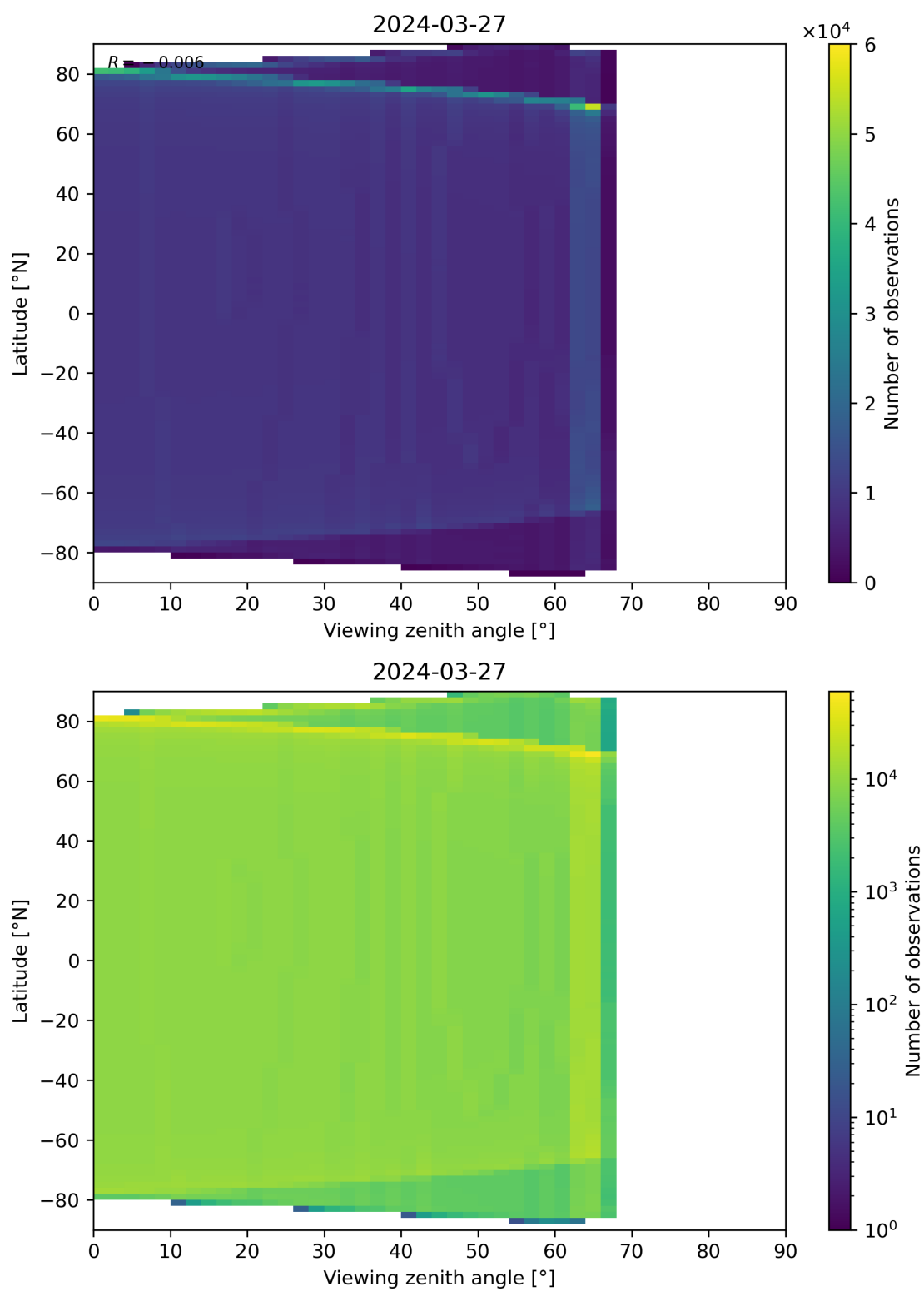
Figure 49: Scatter density plot of “Viewing zenith angle” against “Latitude” for 2024-03-26 to 2024-03-28.
