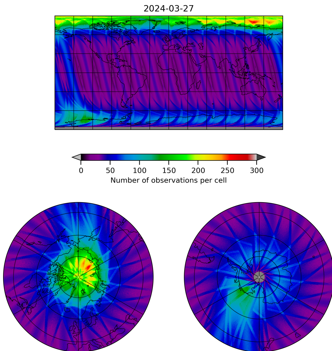
Figure 12: Map of the number of observations for 2024-03-26 to 2024-03-28
