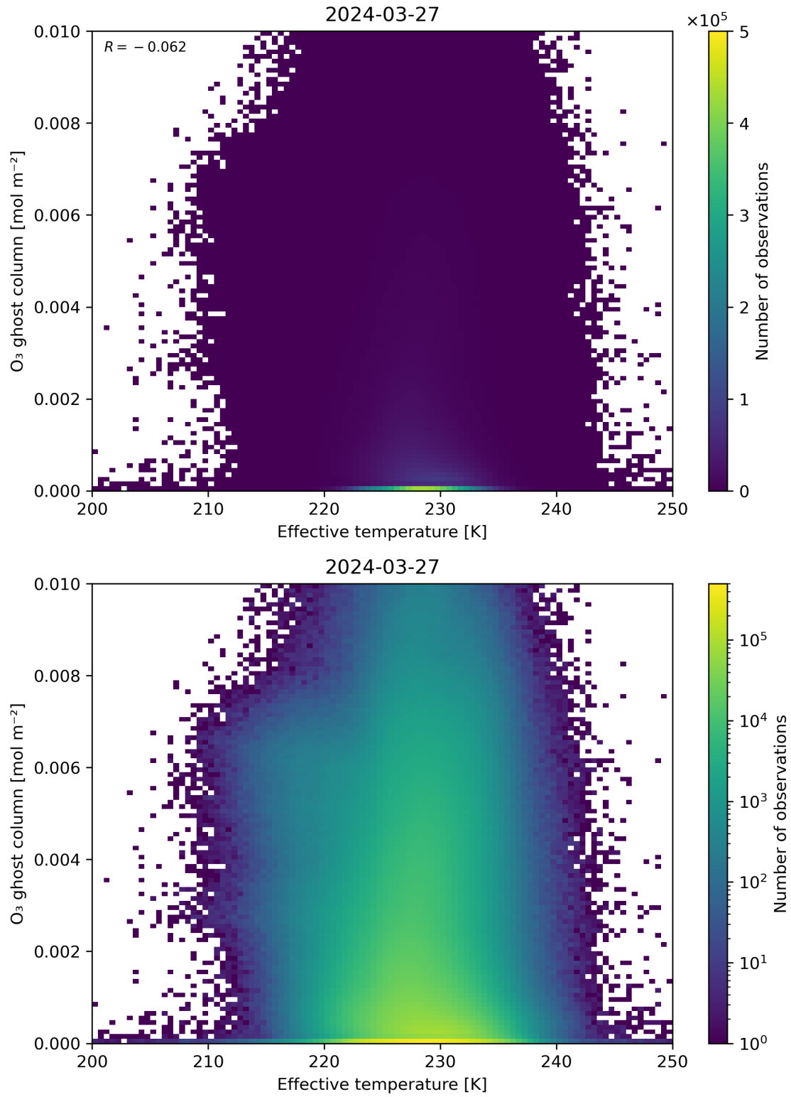
Figure 38: Scatter density plot of “Effective temperature” against “O 3 ghost column” for 2024-03-26 to 2024-03-28.
