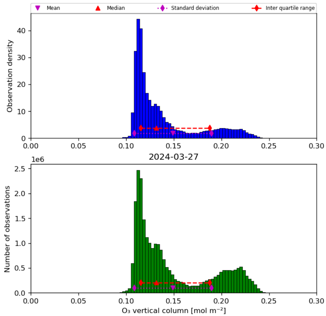
Figure 21: Histogram of “O 3 vertical column” for 2024-03-26 to 2024-03-28
