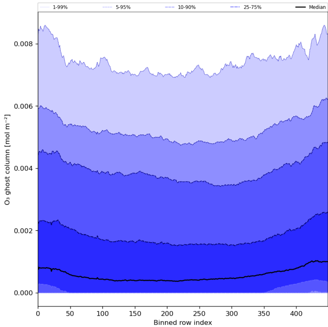
Figure 32: Along track statistics of “O 3 ghost column” for 2024-03-26 to 2024-03-28
