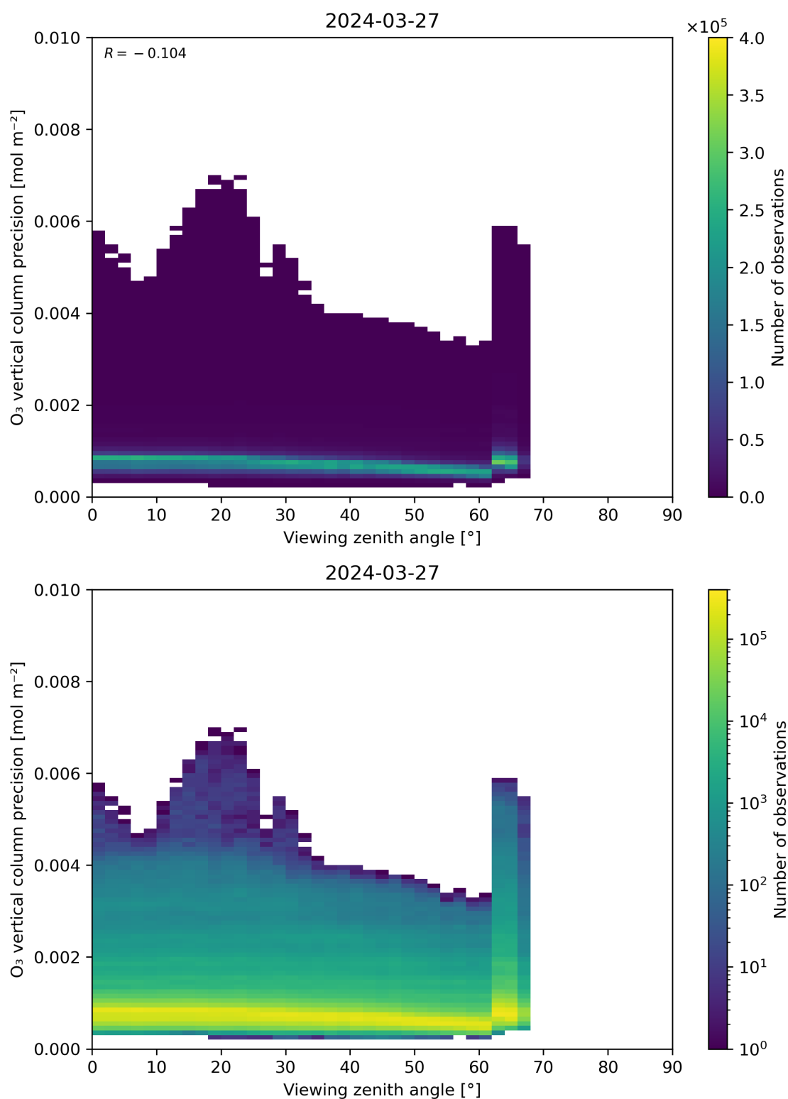
Figure 53: Scatter density plot of “Viewing zenith angle” against “O 3 vertical column precision” for 2024-03-26 to 2024-03-28.
