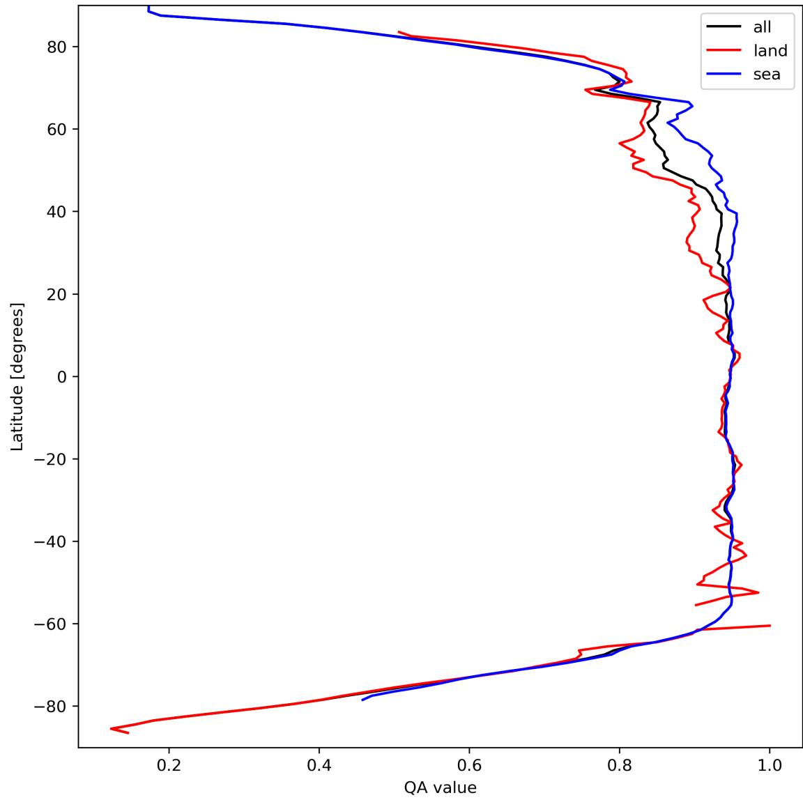
Figure 13: Zonal average of “QA value” for 2024-03-26 to 2024-03-28.
