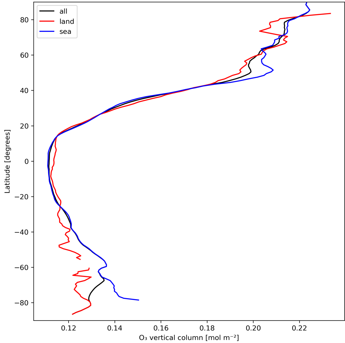
Figure 14: Zonal average of “O 3 vertical column” for 2024-03-26 to 2024-03-28.
