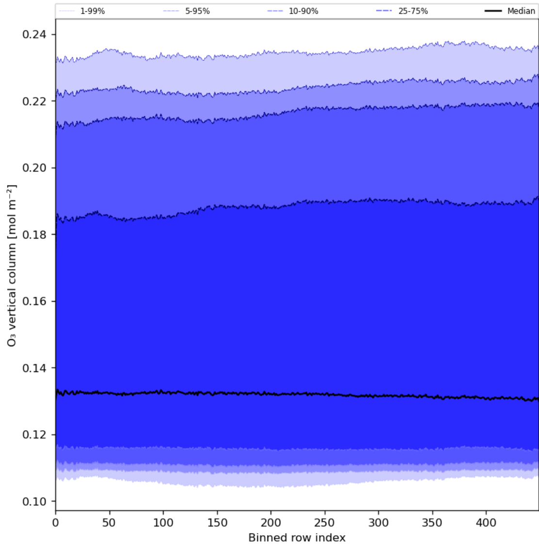
Figure 28: Along track statistics of “O 3 vertical column” for 2024-03-26 to 2024-03-28
