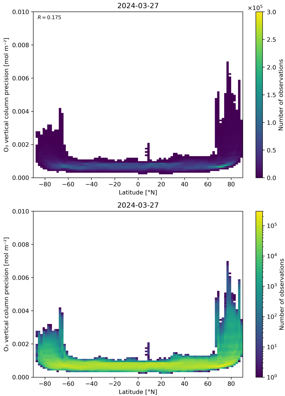
Figure 37: Scatter density plot of “Latitude” against “O 3 vertical column precision” for 2024-03-26 to 2024-03-28.
