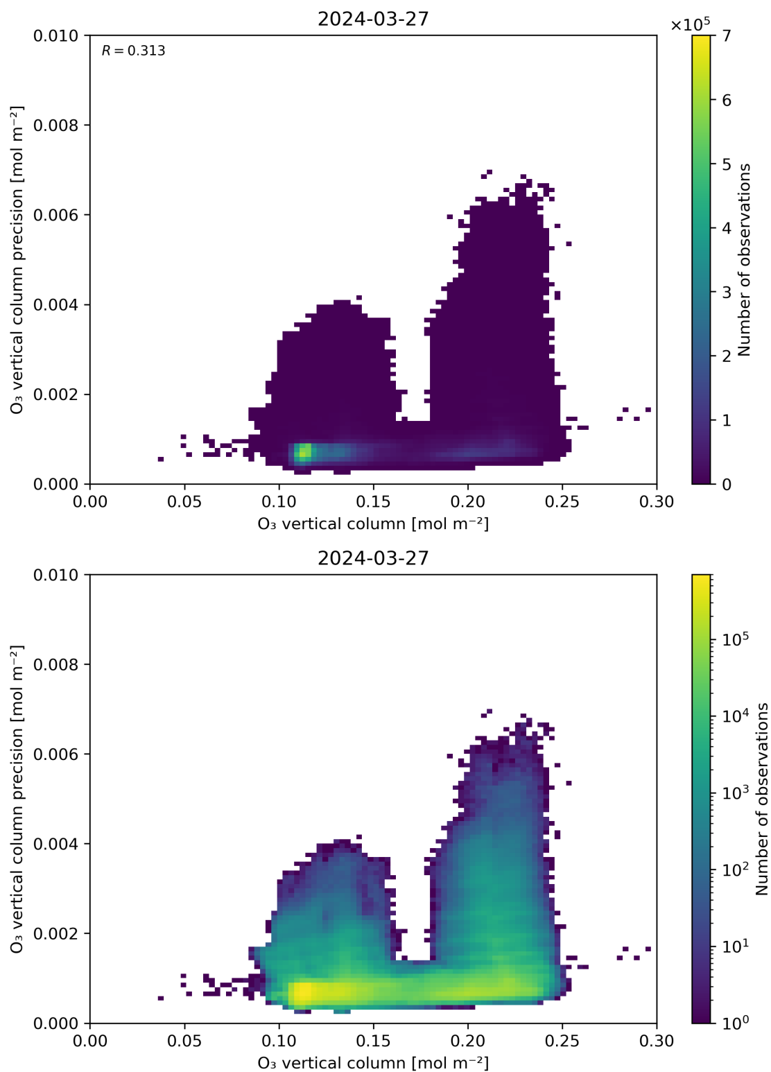
Figure 41: Scatter density plot of “O 3 vertical column” against “O 3 vertical column precision” for 2024-03-26 to 2024-03-28.
