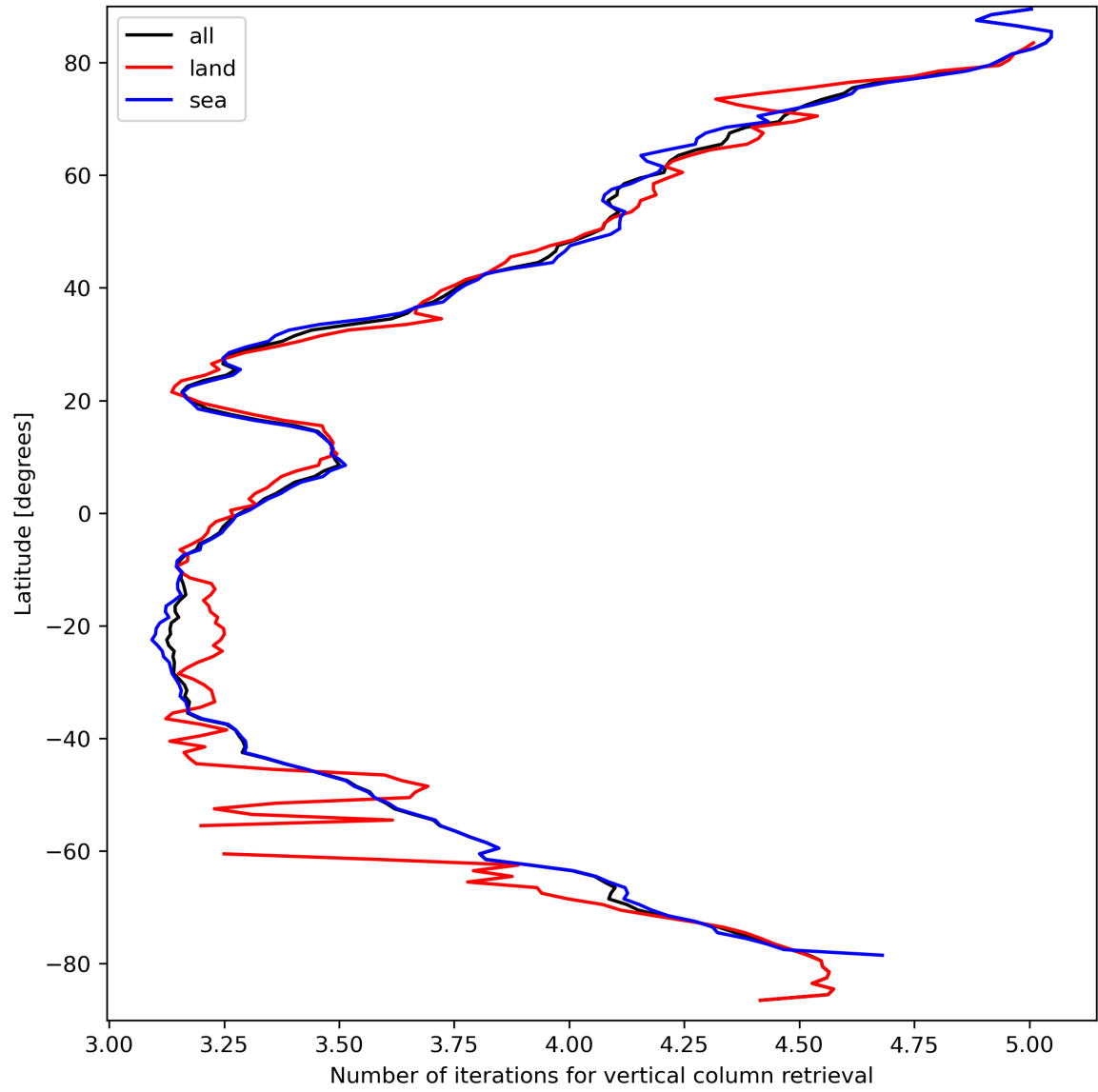
Figure 19: Zonal average of “Number of iterations for vertical column retrieval” for 2024-03-26 to 2024-03-28.
