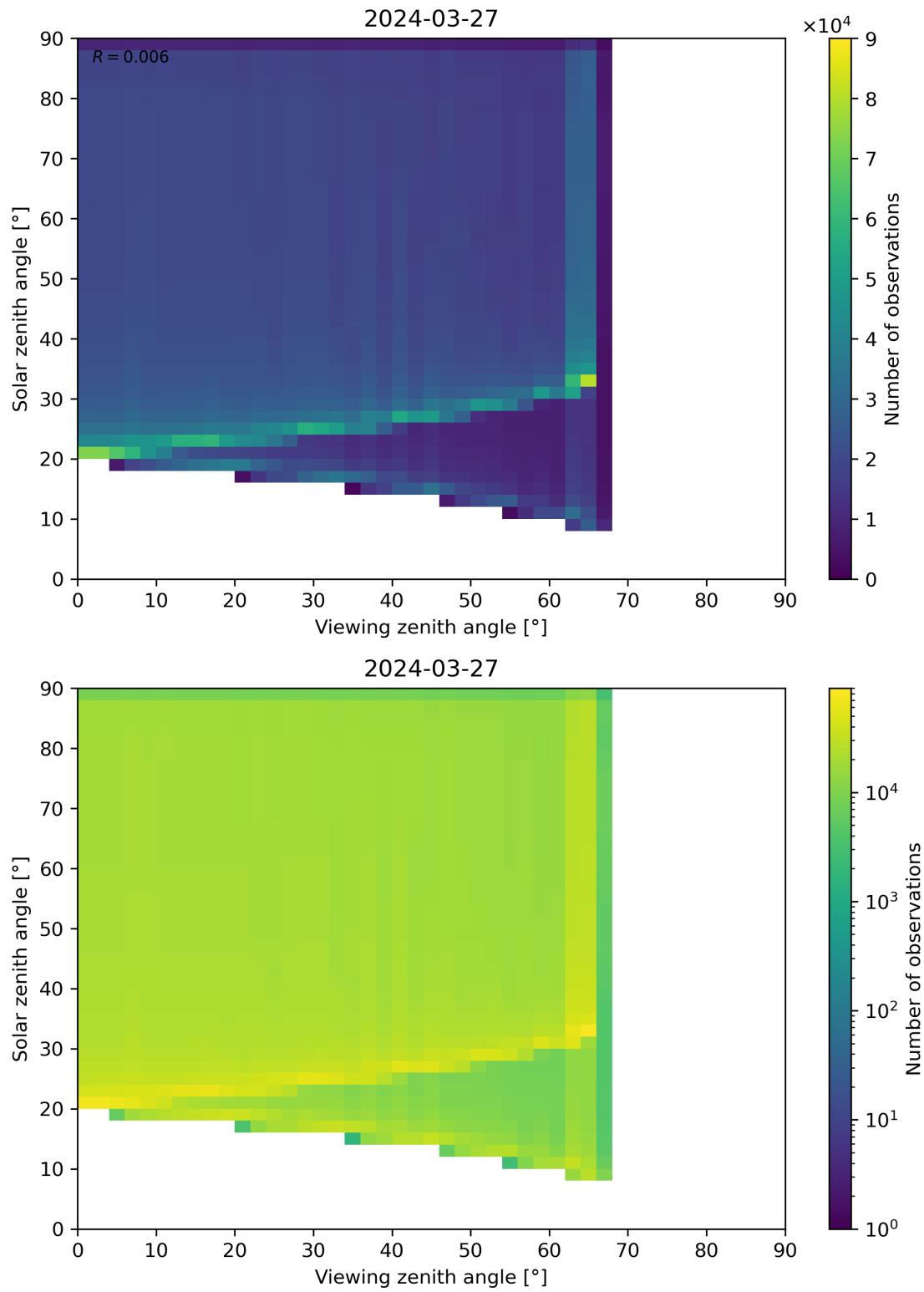
Figure 54: Scatter density plot of “Viewing zenith angle” against “Solar zenith angle” for 2024-03-26 to 2024-03-28.
