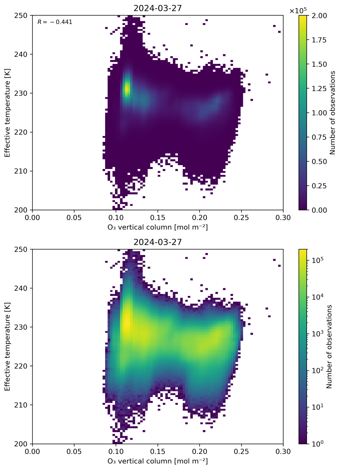
Figure 39: Scatter density plot of “O 3 vertical column” against “Effective temperature” for 2024-03-26 to 2024-03-28.
