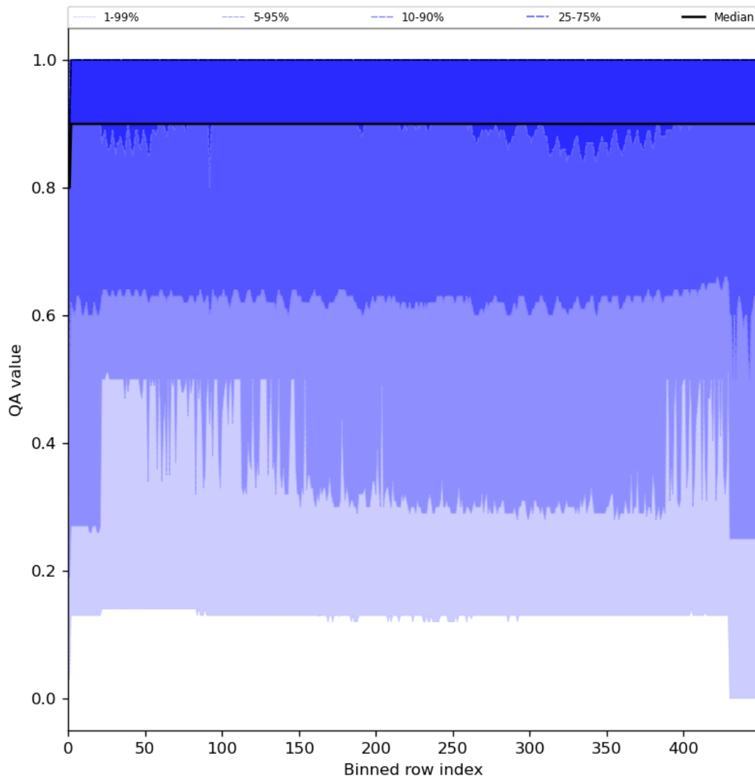
Figure 27: Along track statistics of “QA value” for 2024-03-26 to 2024-03-28
