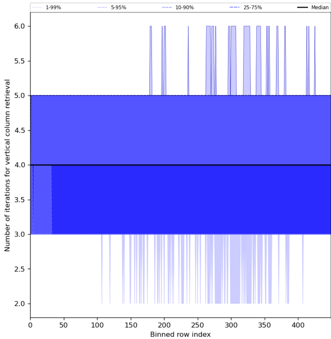
Figure 33: Along track statistics of “Number of iterations for vertical column retrieval” for 2024-03-26 to 2024-03-28
