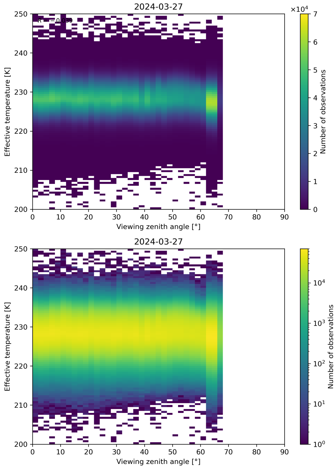
Figure 50: Scatter density plot of “Viewing zenith angle” against “Effective temperature” for 2024-03-26 to 2024-03-28.
