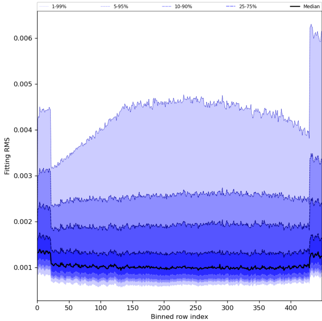
Figure 30: Along track statistics of “Fitting RMS” for 2024-03-26 to 2024-03-28
