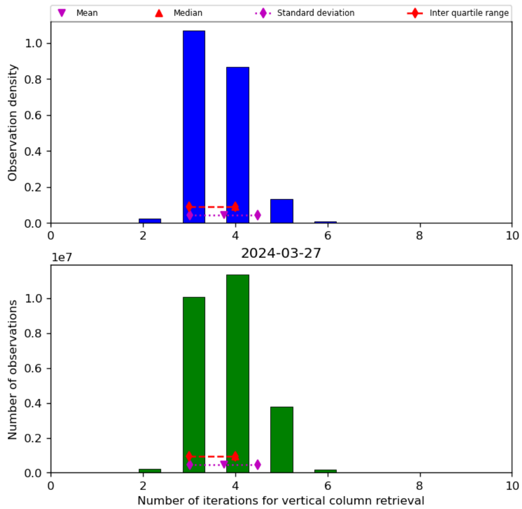
Figure 26: Histogram of “Number of iterations for vertical column retrieval” for 2024-03-26 to 2024-03-28
