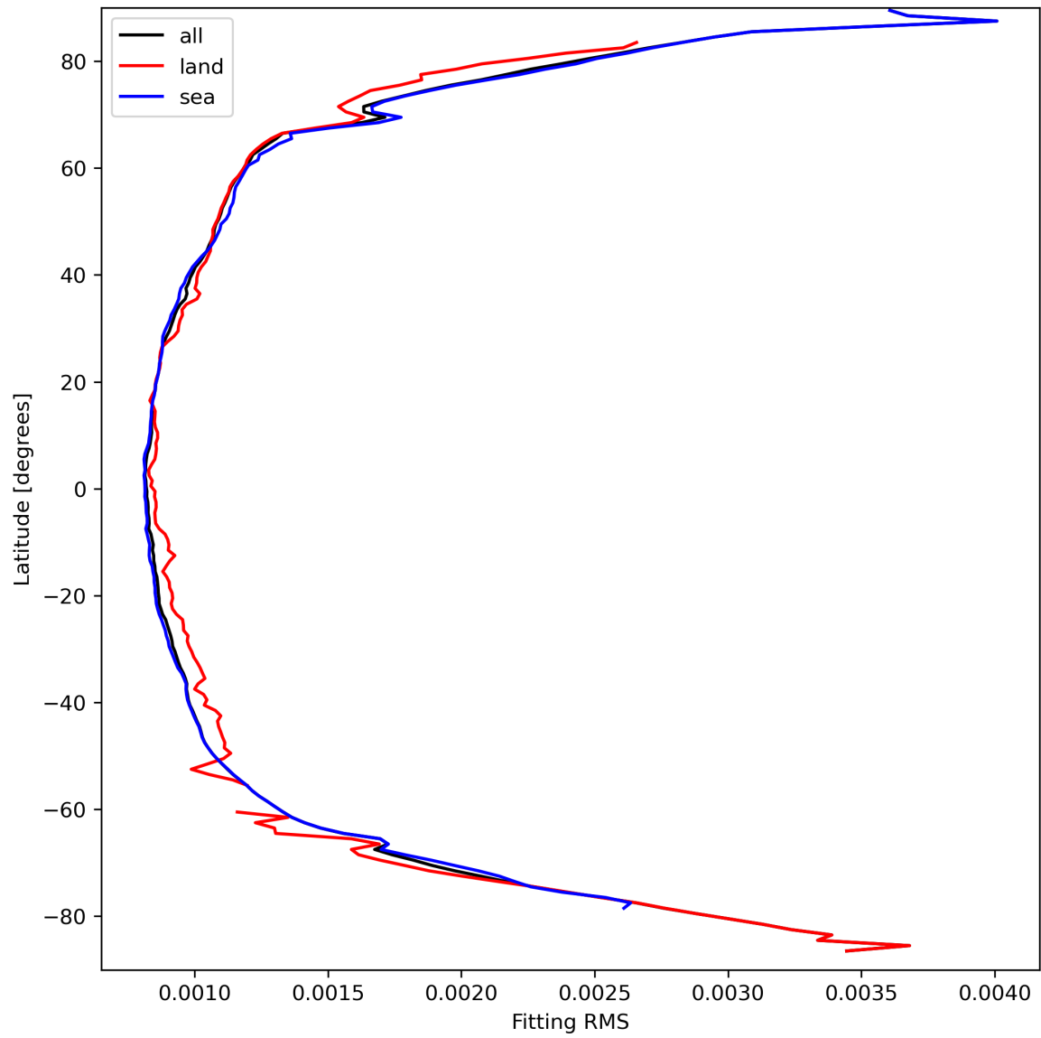
Figure 16: Zonal average of “Fitting RMS” for 2024-03-26 to 2024-03-28.
