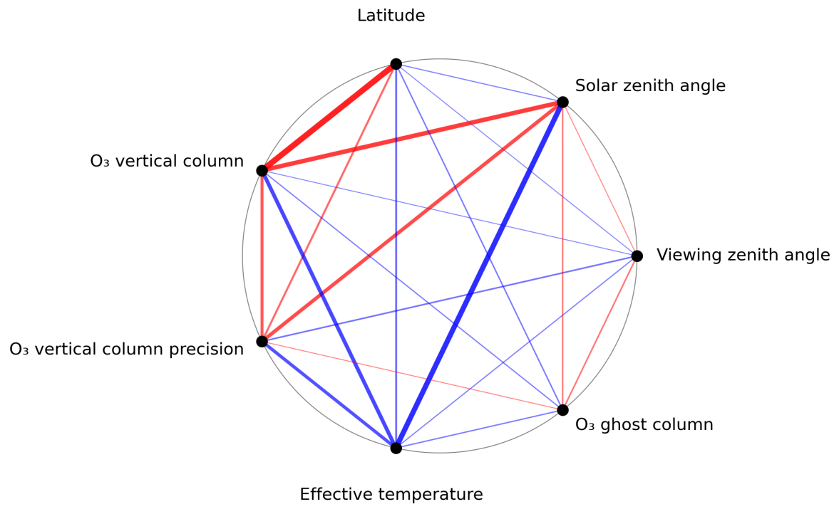
Figure 1: Map of correlation graph for 2024-03-26 to 2024-03-28.
