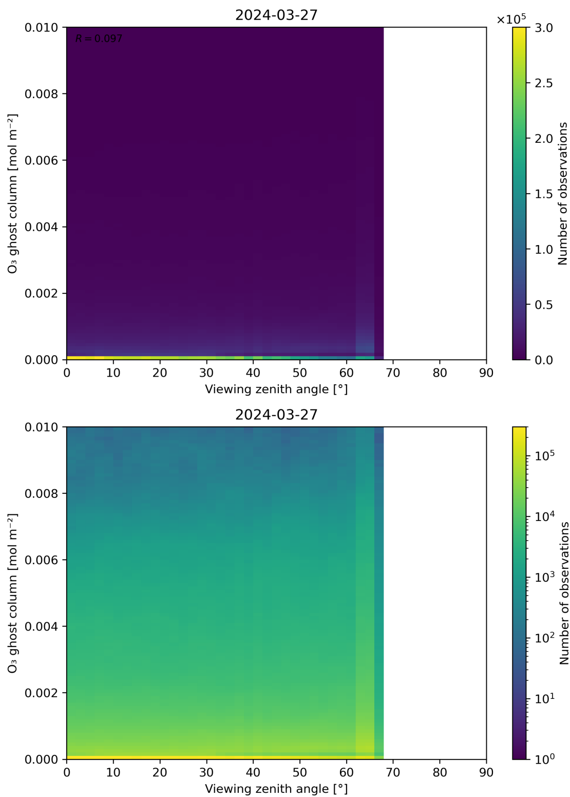
Figure 51: Scatter density plot of “Viewing zenith angle” against “O 3 ghost column” for 2024-03-26 to 2024-03-28.
