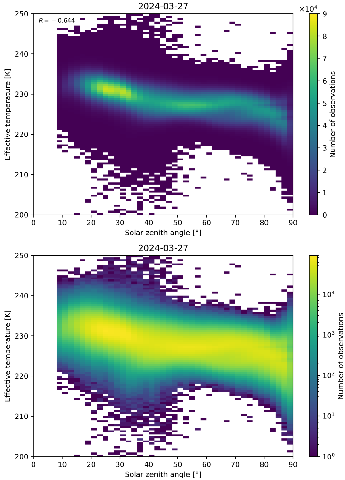
Figure 45: Scatter density plot of “Solar zenith angle” against “Effective temperature” for 2024-03-26 to 2024-03-28.
