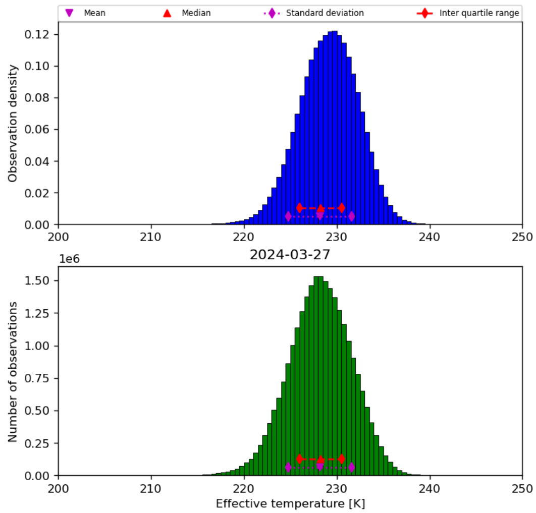
Figure 24: Histogram of “Effective temperature” for 2024-03-26 to 2024-03-28
