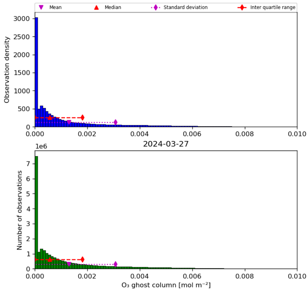
Figure 25: Histogram of “O 3 ghost column” for 2024-03-26 to 2024-03-28
