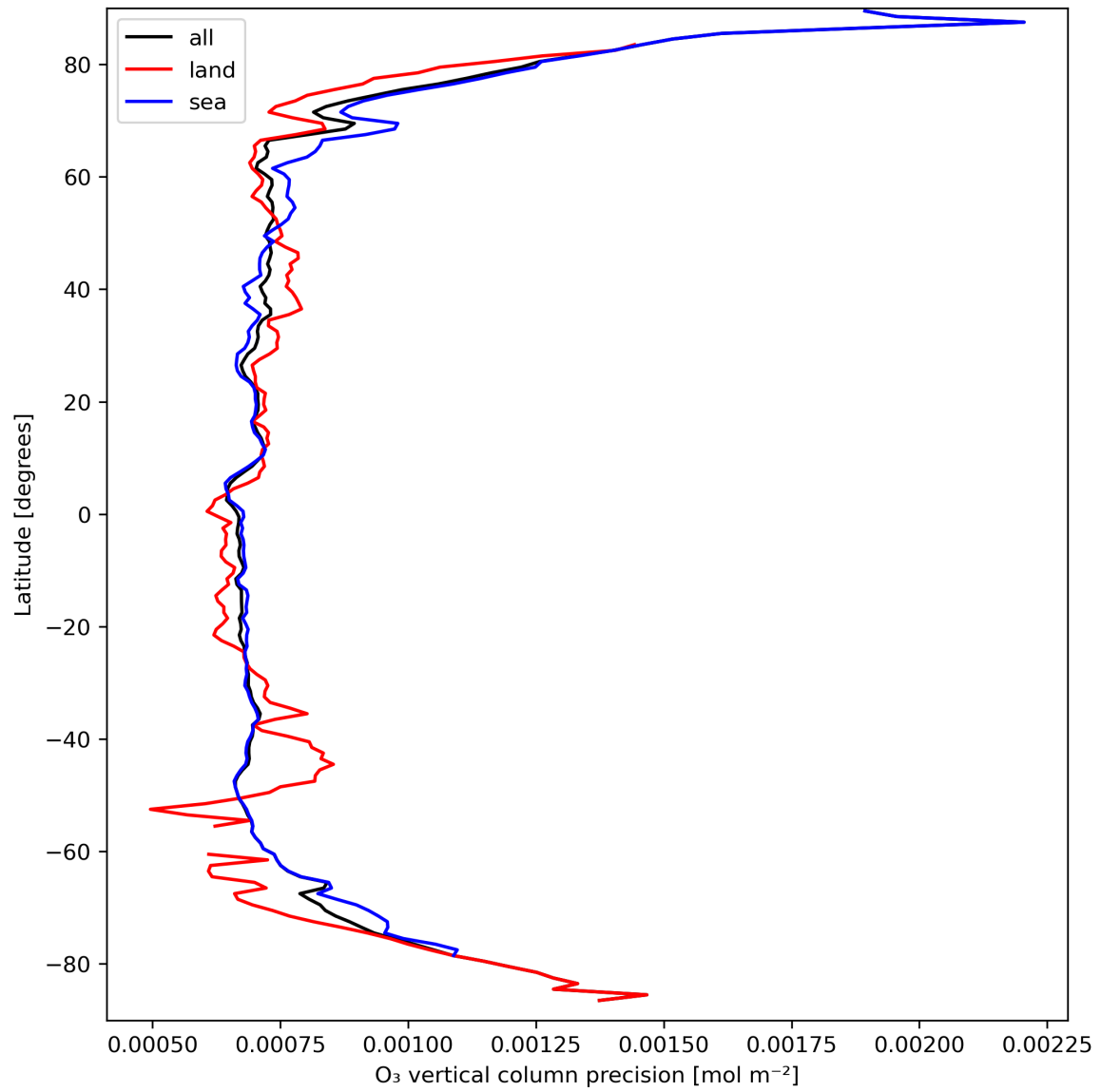
Figure 15: Zonal average of "O 3 vertical column precision" for 2024-03-26 to 2024-03-28.
