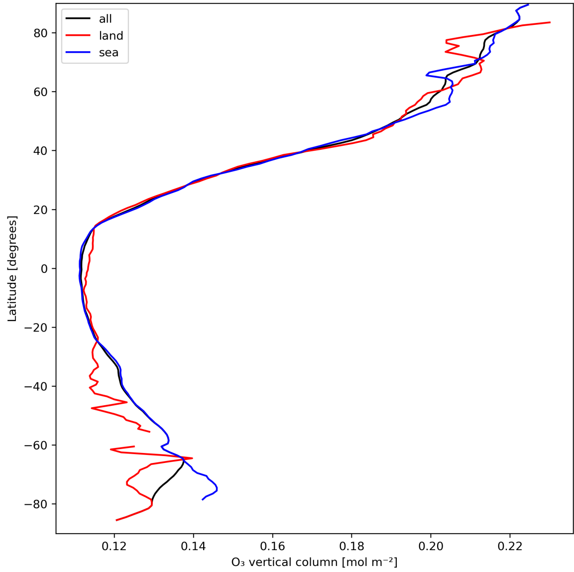
Figure 14: Zonal average of “O 3 vertical column” for 2024-03-27 to 2024-03-29.
