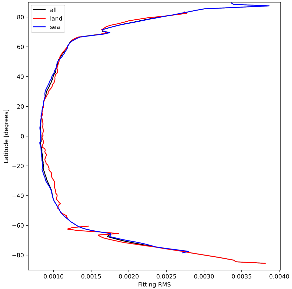
Figure 16: Zonal average of “Fitting RMS” for 2024-03-27 to 2024-03-29.
