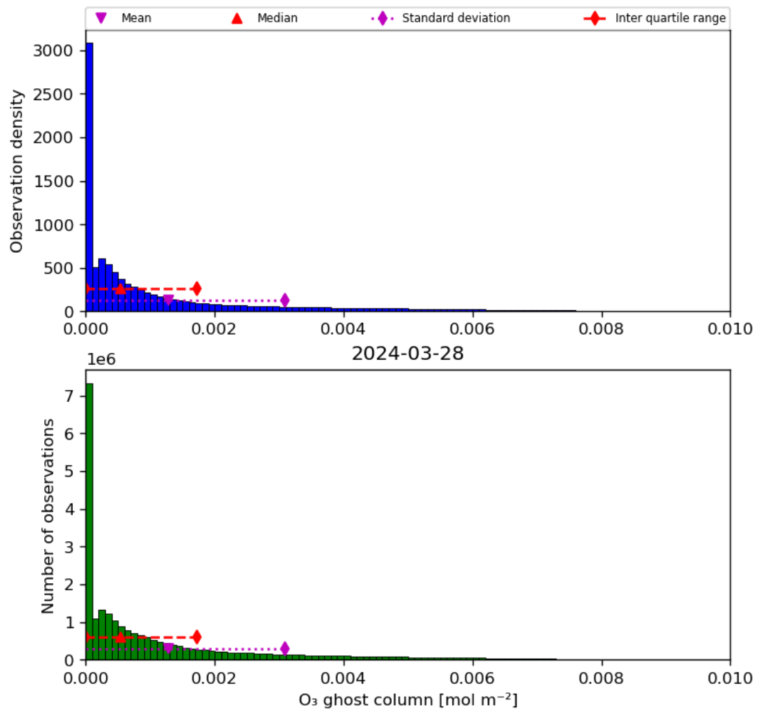
Figure 25: Histogram of “O 3 ghost column” for 2024-03-27 to 2024-03-29
