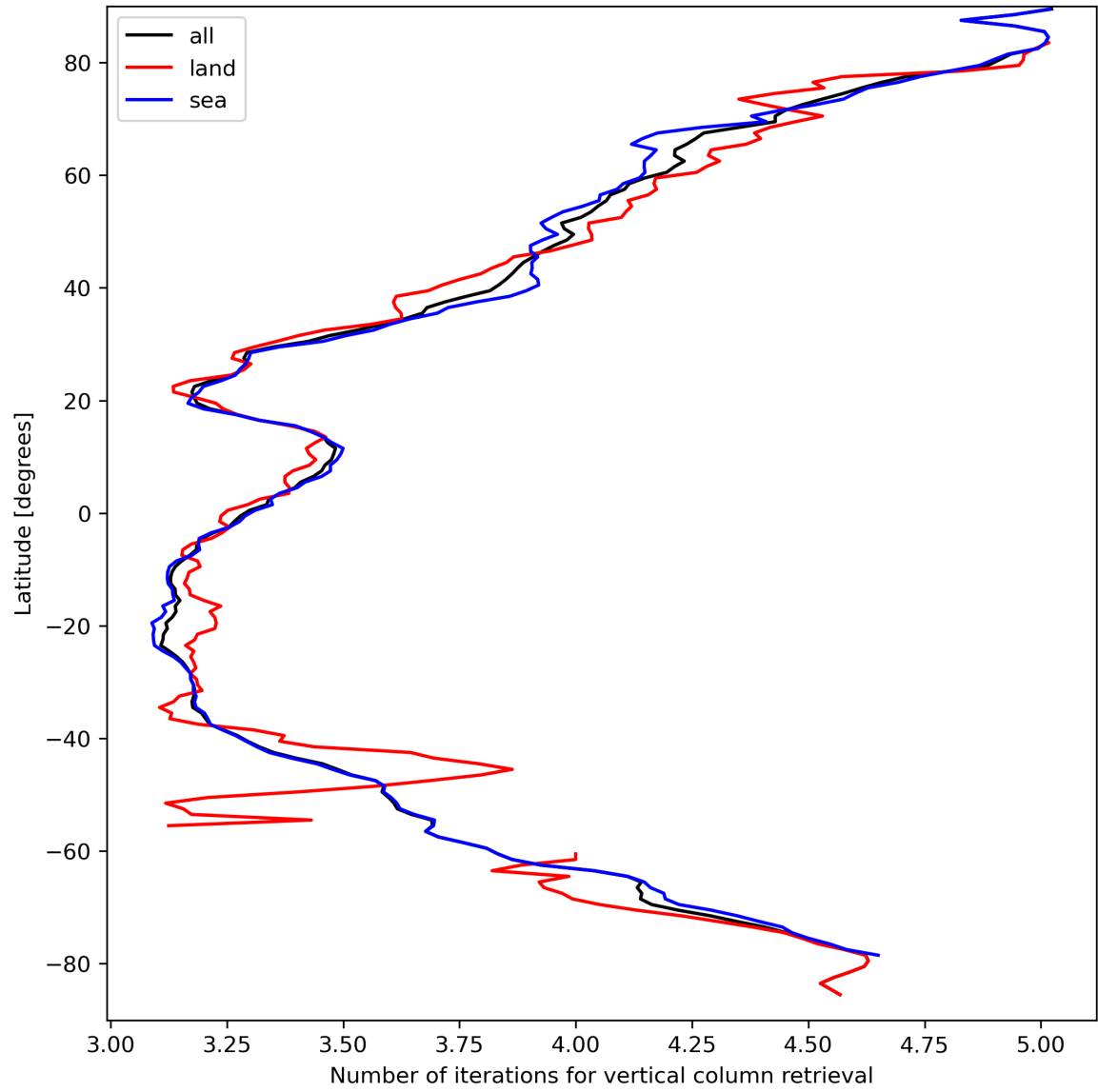
Figure 19: Zonal average of “Number of iterations for vertical column retrieval” for 2024-03-27 to 2024-03-29.
