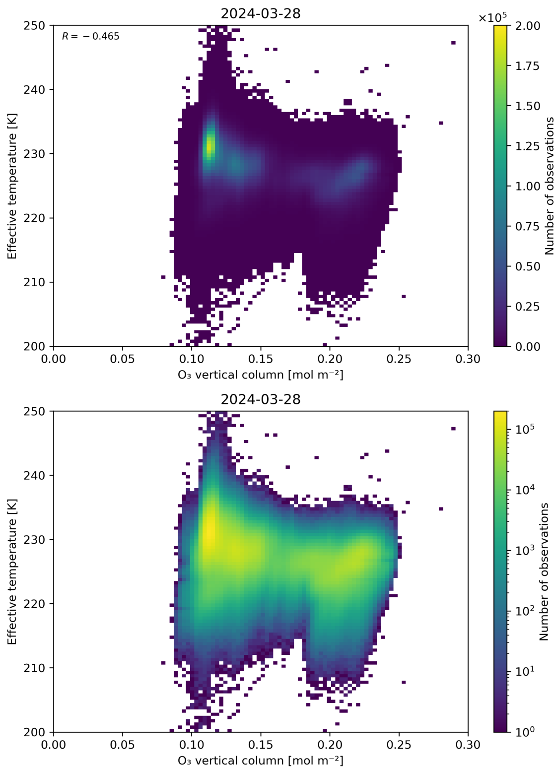
Figure 39: Scatter density plot of “O 3 vertical column” against “Effective temperature” for 2024-03-27 to 2024-03-29.
