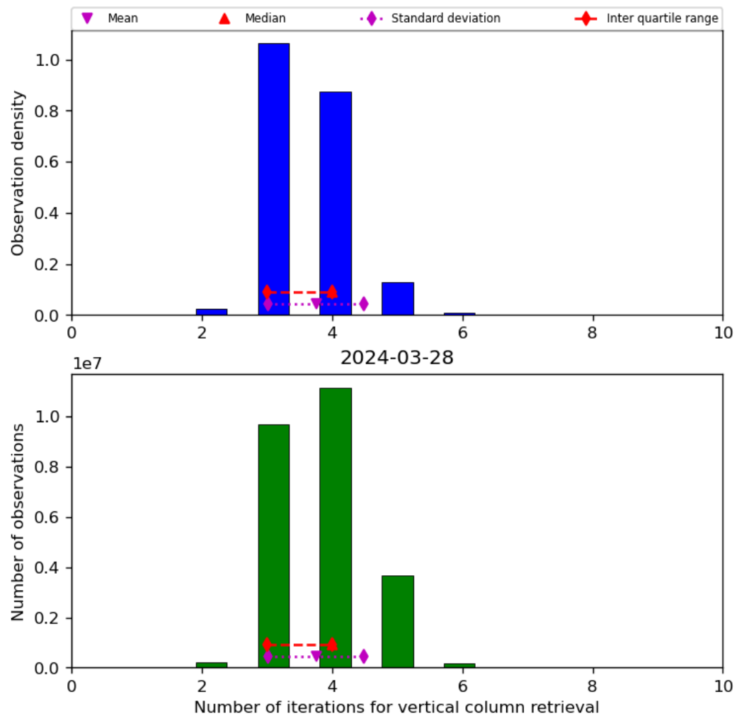
Figure 26: Histogram of “Number of iterations for vertical column retrieval” for 2024-03-27 to 2024-03-29
