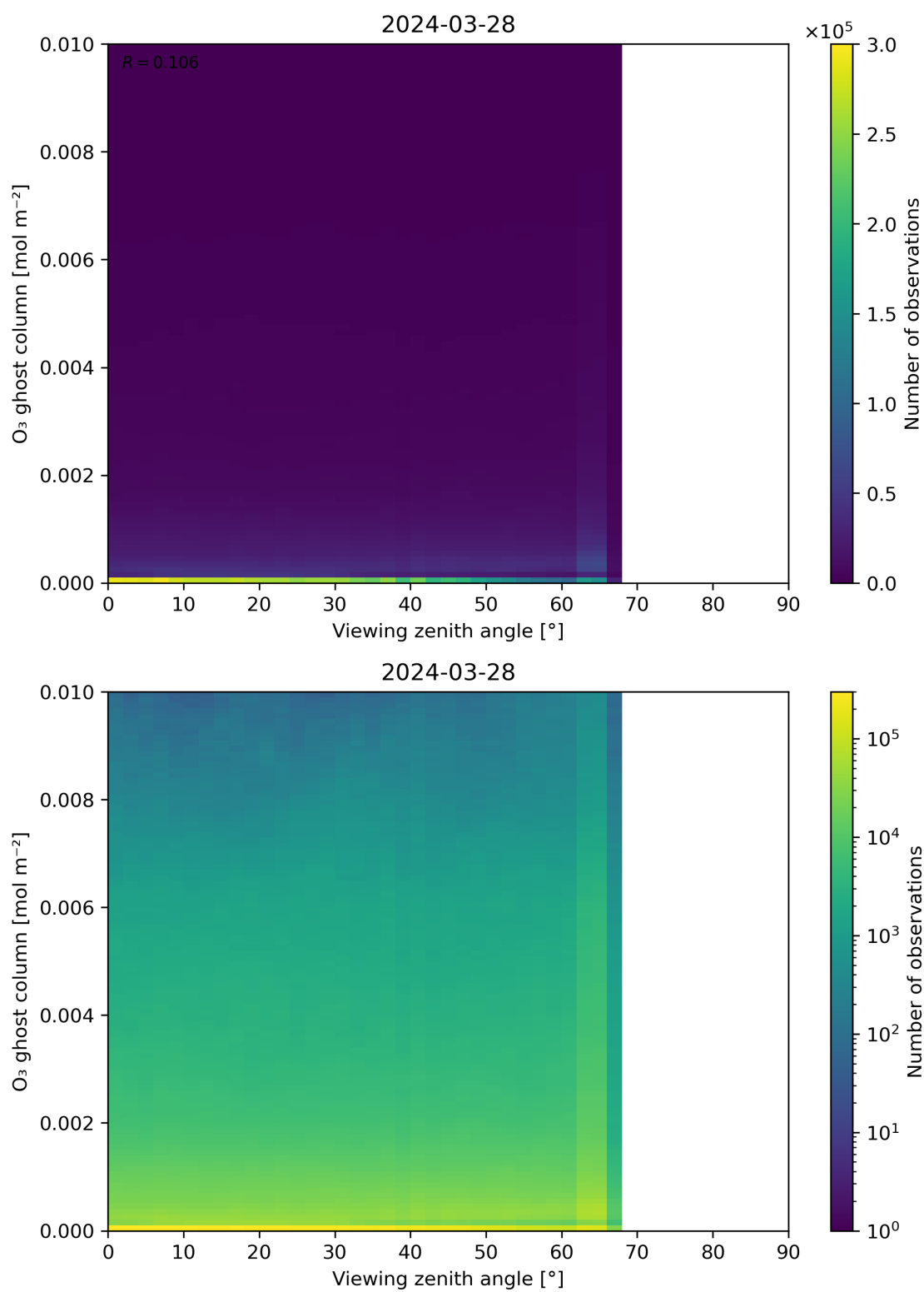
Figure 51: Scatter density plot of “Viewing zenith angle” against “O 3 ghost column” for 2024-03-27 to 2024-03-29.
