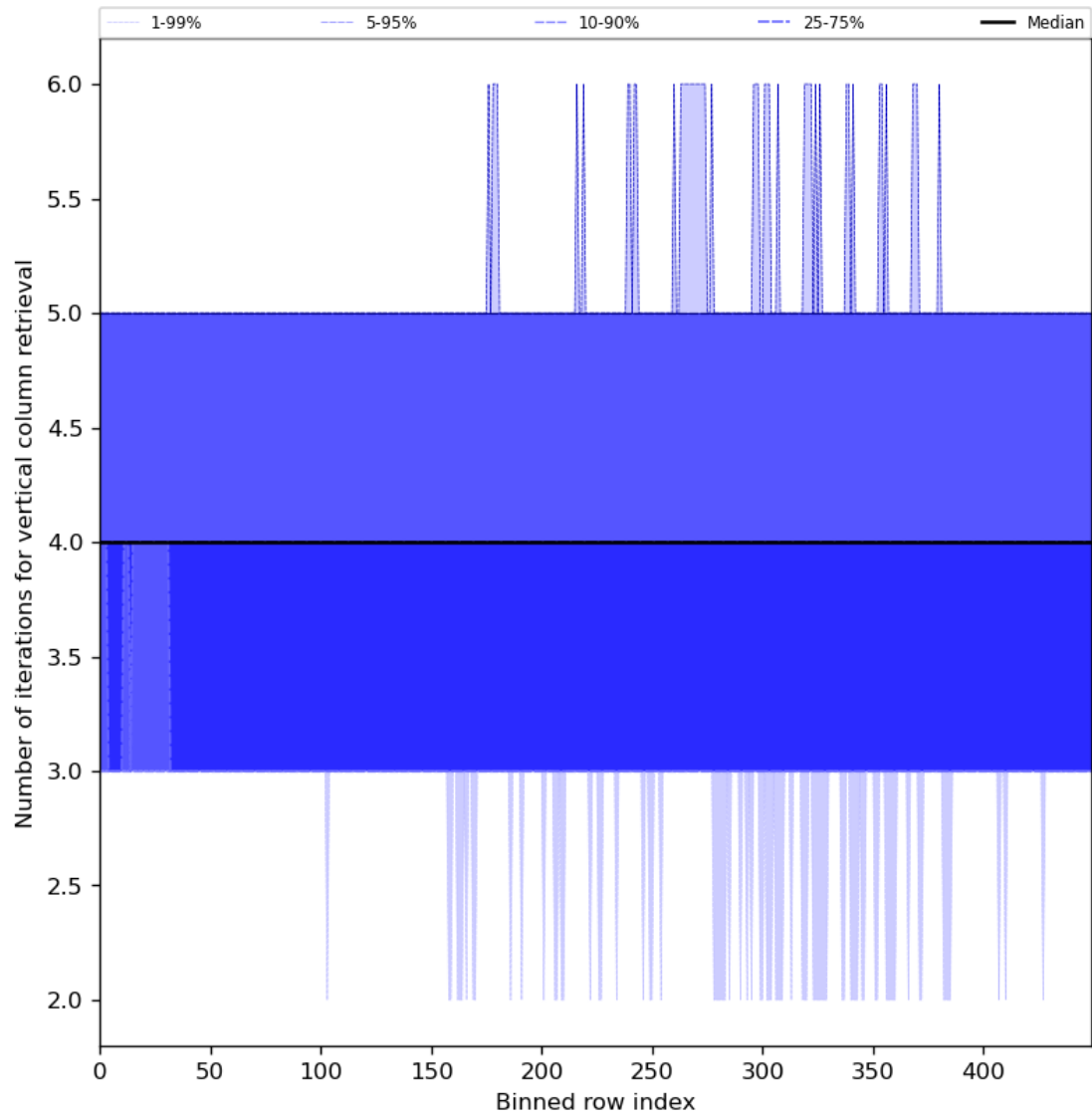
Figure 33: Along track statistics of “Number of iterations for vertical column retrieval” for 2024-03-27 to 2024-03-29
