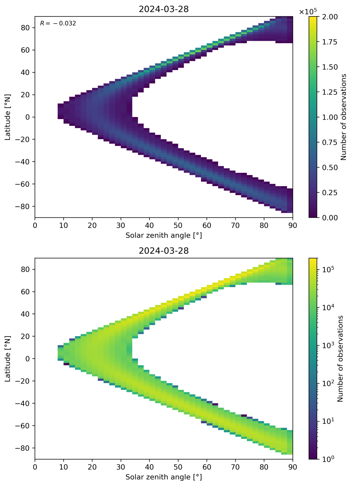
Figure 44: Scatter density plot of “Solar zenith angle” against “Latitude” for 2024-03-27 to 2024-03-29.
