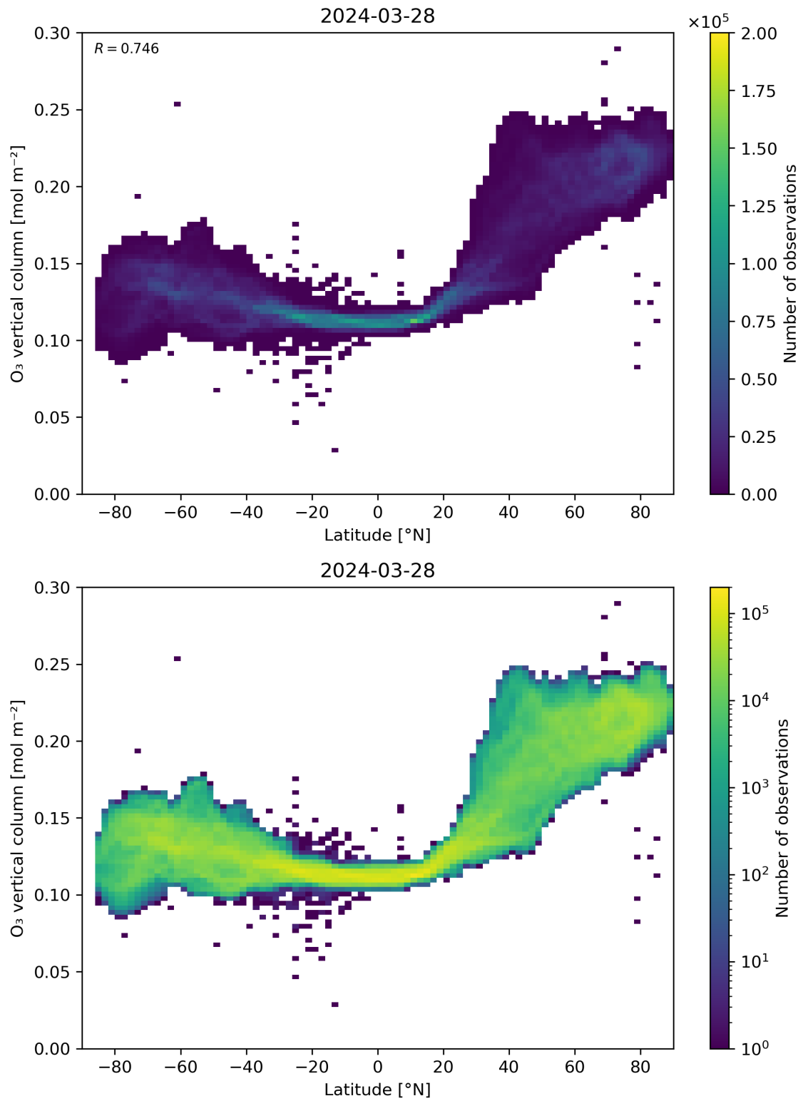
Figure 36: Scatter density plot of “Latitude” against “O 3 vertical column” for 2024-03-27 to 2024-03-29.
