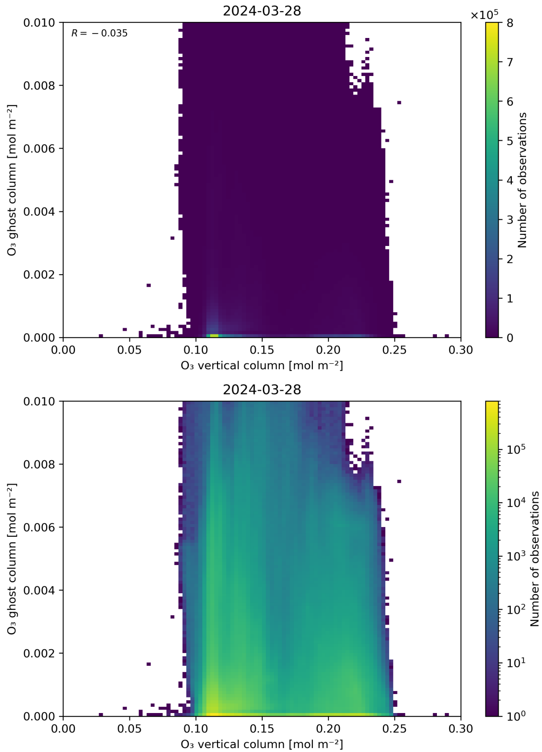
Figure 40: Scatter density plot of “O 3 vertical column” against “O 3 ghost column” for 2024-03-27 to 2024-03-29.
