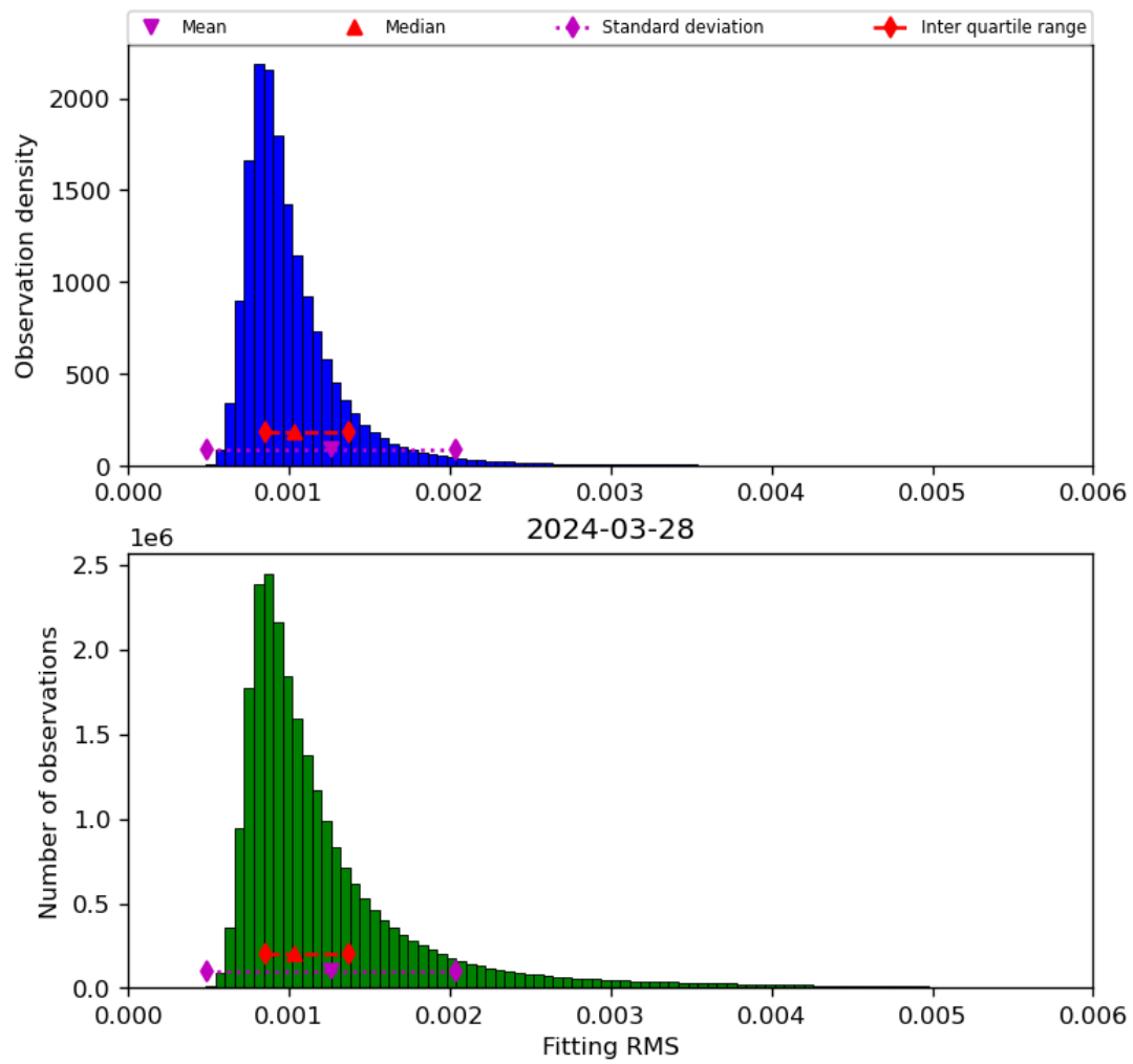
Figure 23: Histogram of “Fitting RMS” for 2024-03-27 to 2024-03-29
