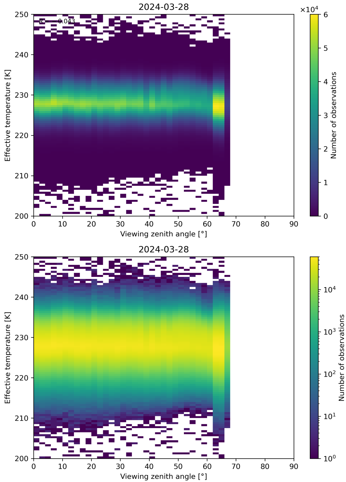
Figure 50: Scatter density plot of “Viewing zenith angle” against “Effective temperature” for 2024-03-27 to 2024-03-29.
