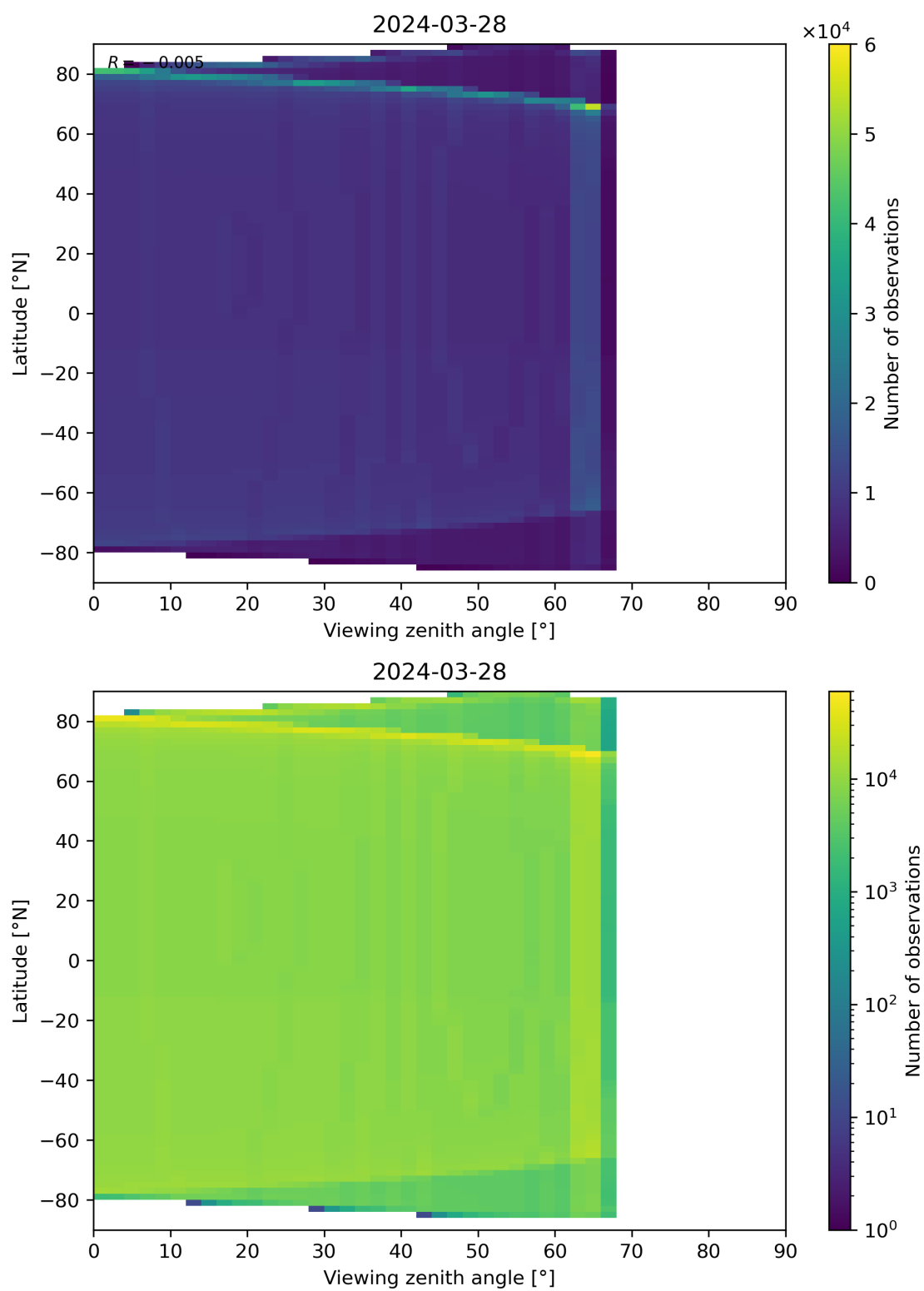
Figure 49: Scatter density plot of “Viewing zenith angle” against “Latitude” for 2024-03-27 to 2024-03-29.
