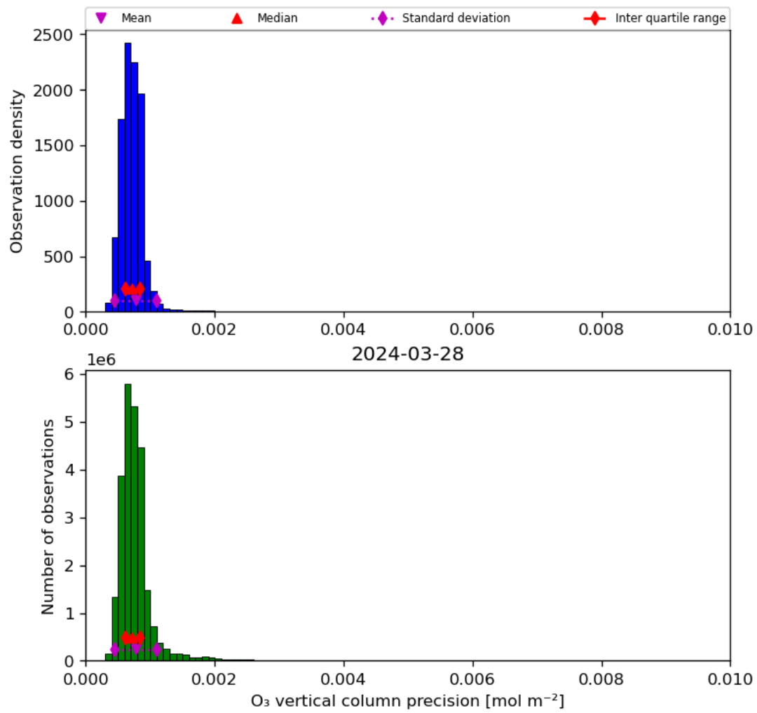
Figure 22: Histogram of “O 3 vertical column precision” for 2024-03-27 to 2024-03-29
