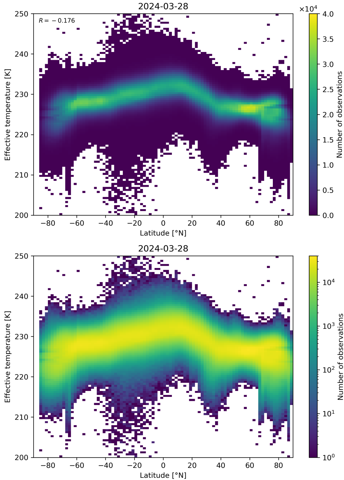
Figure 34: Scatter density plot of “Latitude” against “Effective temperature” for 2024-03-27 to 2024-03-29.
