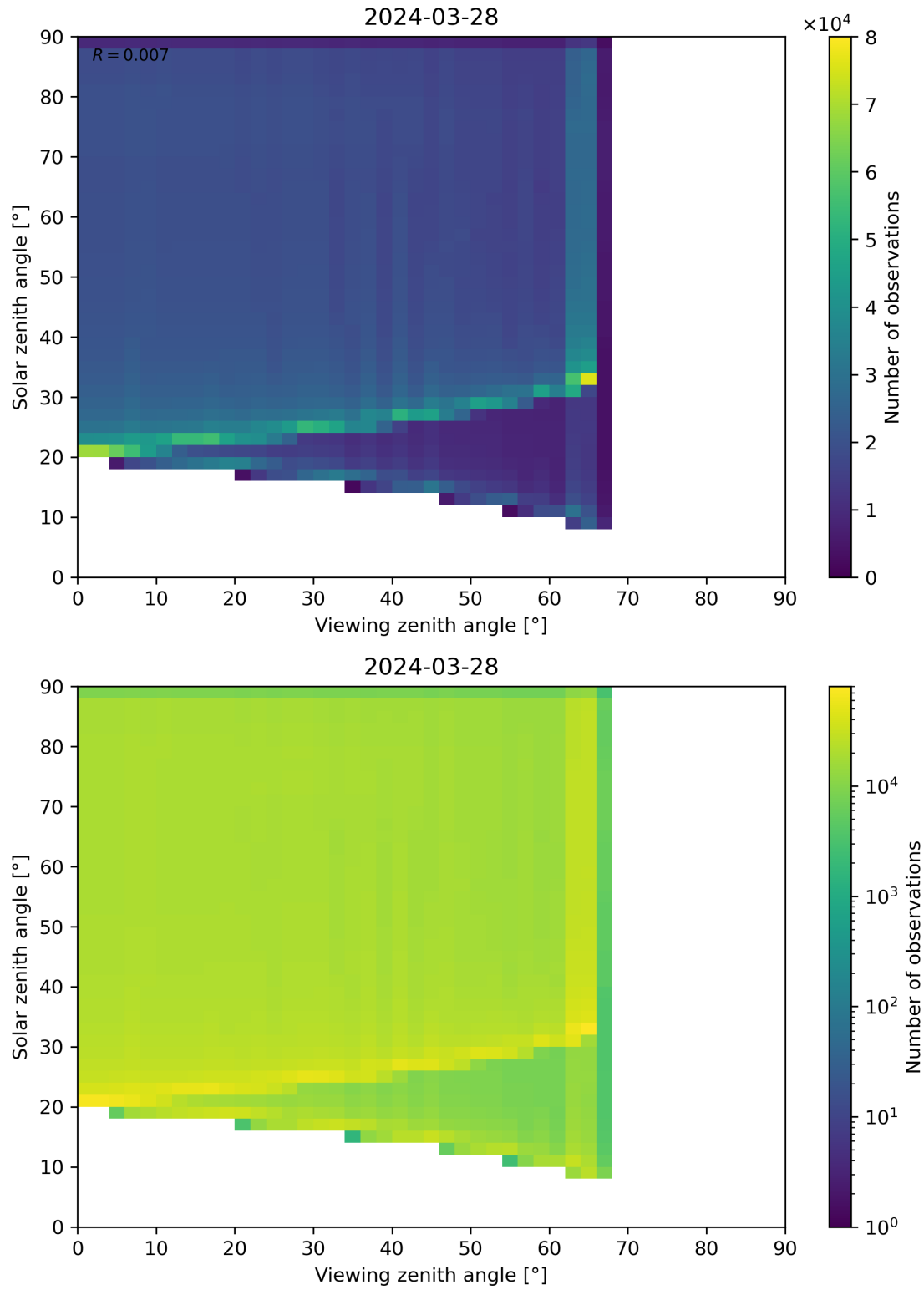
Figure 54: Scatter density plot of “Viewing zenith angle” against “Solar zenith angle” for 2024-03-27 to 2024-03-29.
