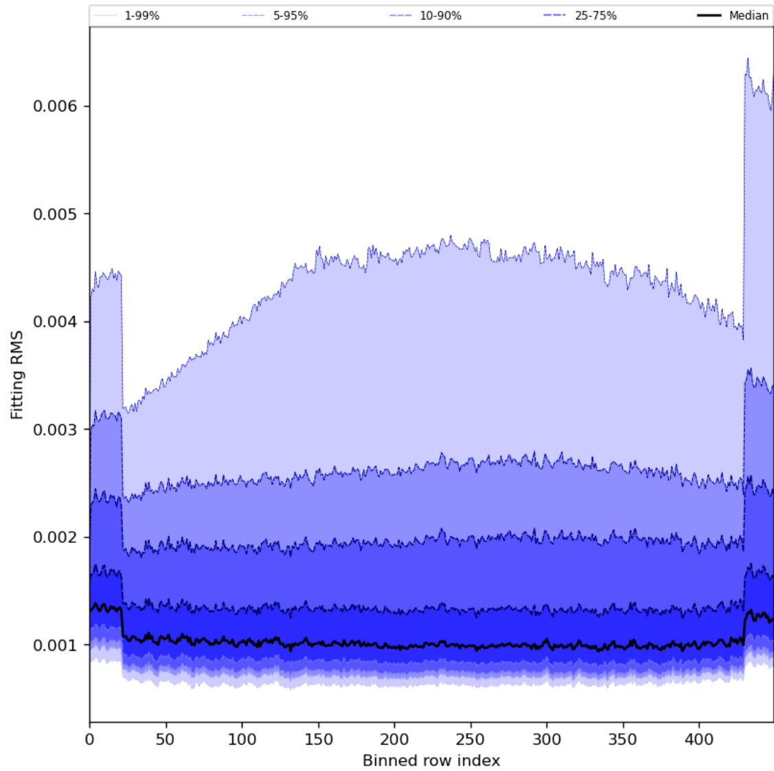
Figure 30: Along track statistics of “Fitting RMS” for 2024-03-27 to 2024-03-29
