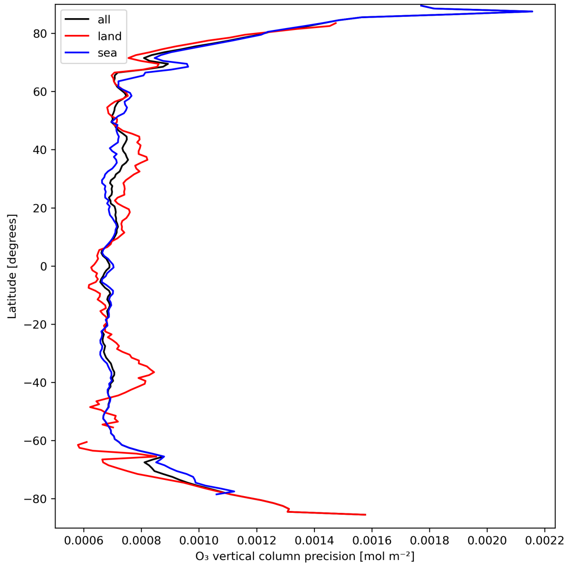
Figure 15: Zonal average of "O 3 vertical column precision" for 2024-03-27 to 2024-03-29.
