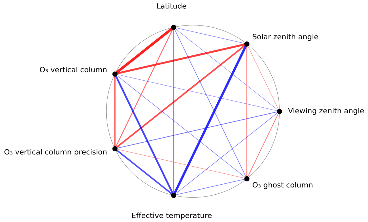
Figure 1: Map of correlation graph for 2024-03-27 to 2024-03-29.
