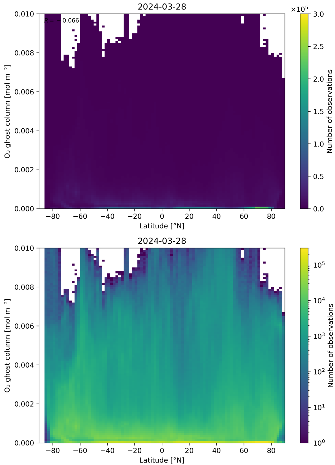
Figure 35: Scatter density plot of “Latitude” against “O 3 ghost column” for 2024-03-27 to 2024-03-29.
