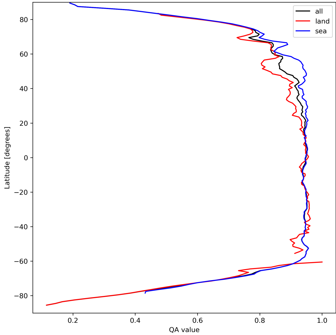
Figure 13: Zonal average of “QA value” for 2024-03-27 to 2024-03-29.
