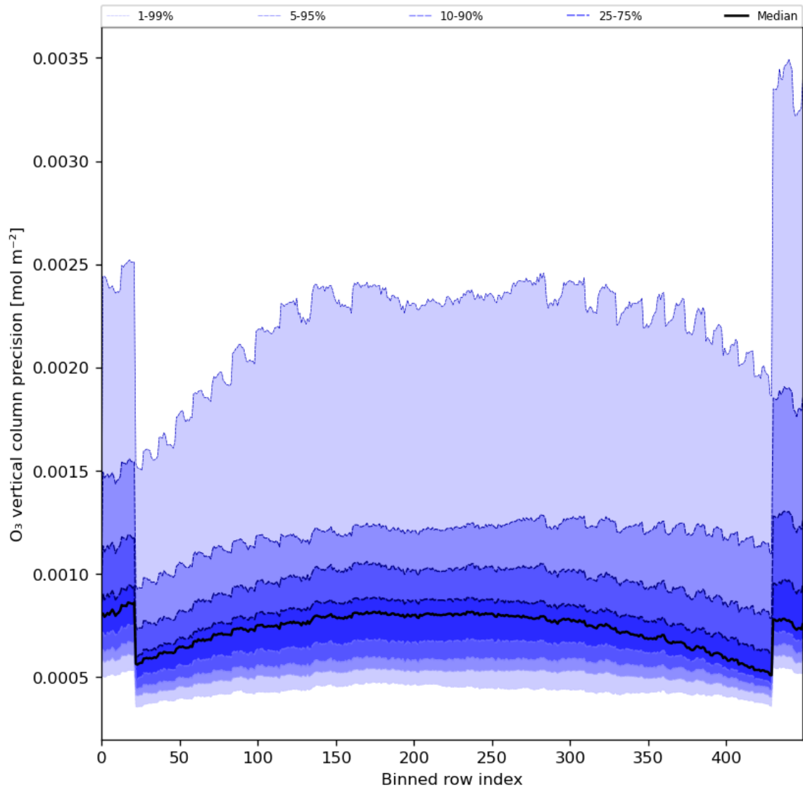
Figure 29: Along track statistics of “O 3 vertical column precision” for 2024-03-27 to 2024-03-29
