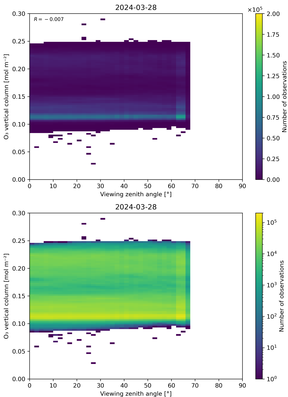
Figure 52: Scatter density plot of “Viewing zenith angle” against “O 3 vertical column” for 2024-03-27 to 2024-03-29.
