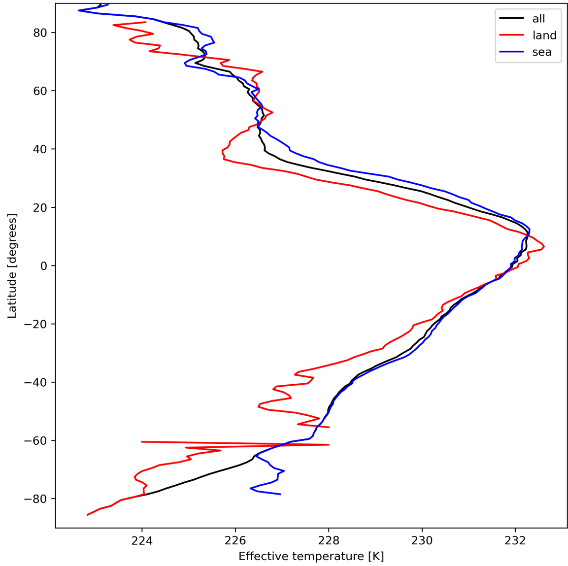
Figure 17: Zonal average of “Effective temperature” for 2024-03-27 to 2024-03-29.
