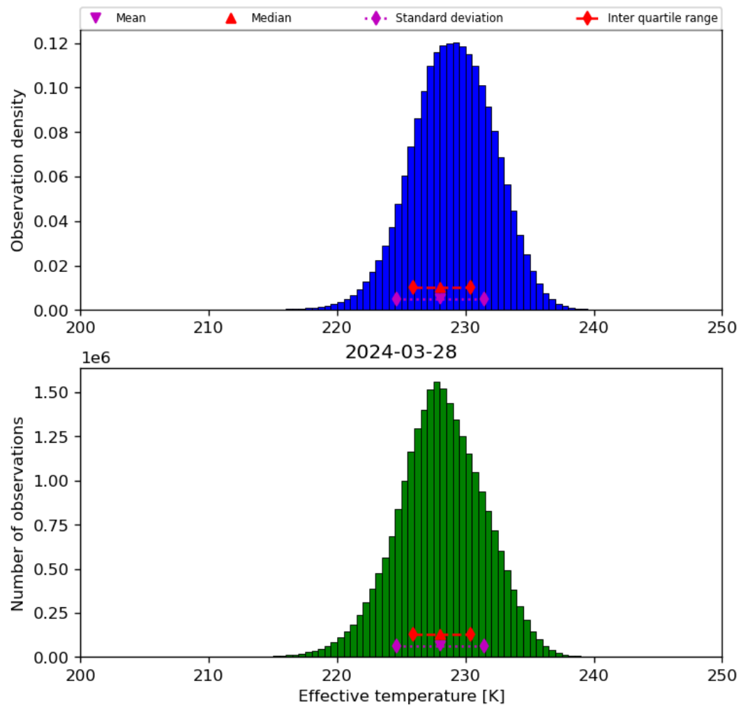
Figure 24: Histogram of “Effective temperature” for 2024-03-27 to 2024-03-29
