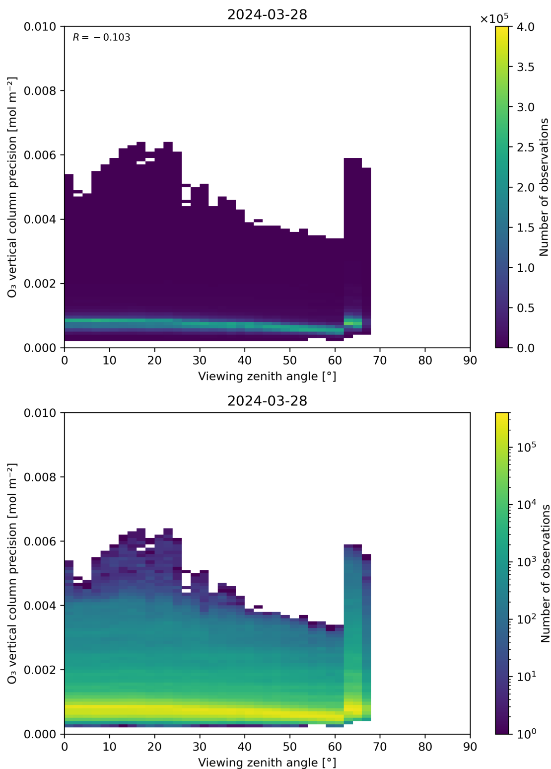
Figure 53: Scatter density plot of “Viewing zenith angle” against “O 3 vertical column precision” for 2024-03-27 to 2024-03-29.
