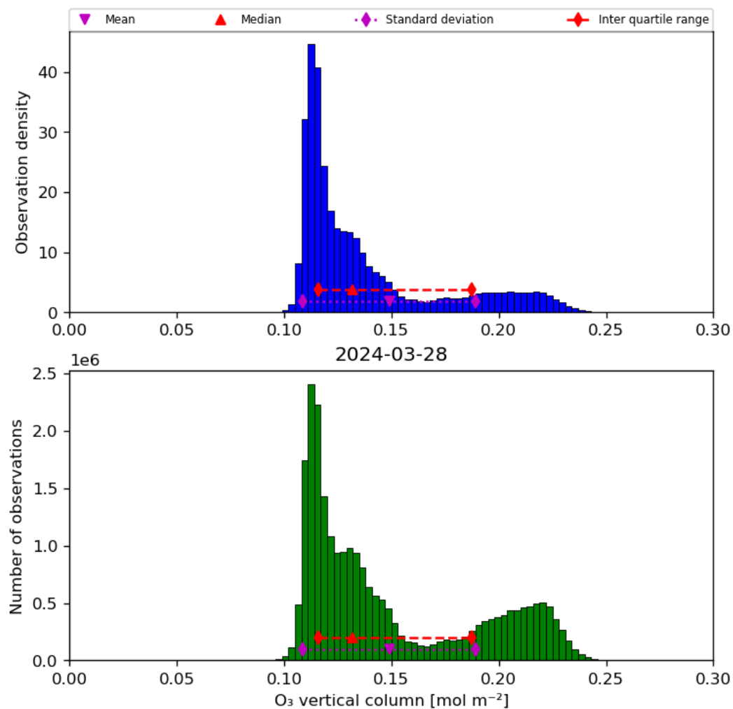
Figure 21: Histogram of “O 3 vertical column” for 2024-03-27 to 2024-03-29
