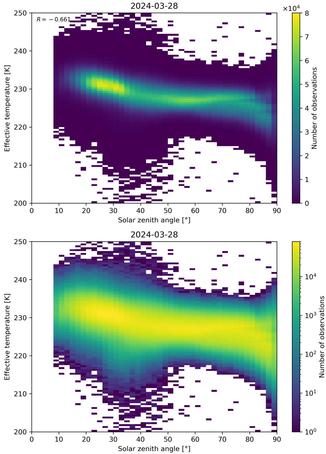
Figure 45: Scatter density plot of “Solar zenith angle” against “Effective temperature” for 2024-03-27 to 2024-03-29.
