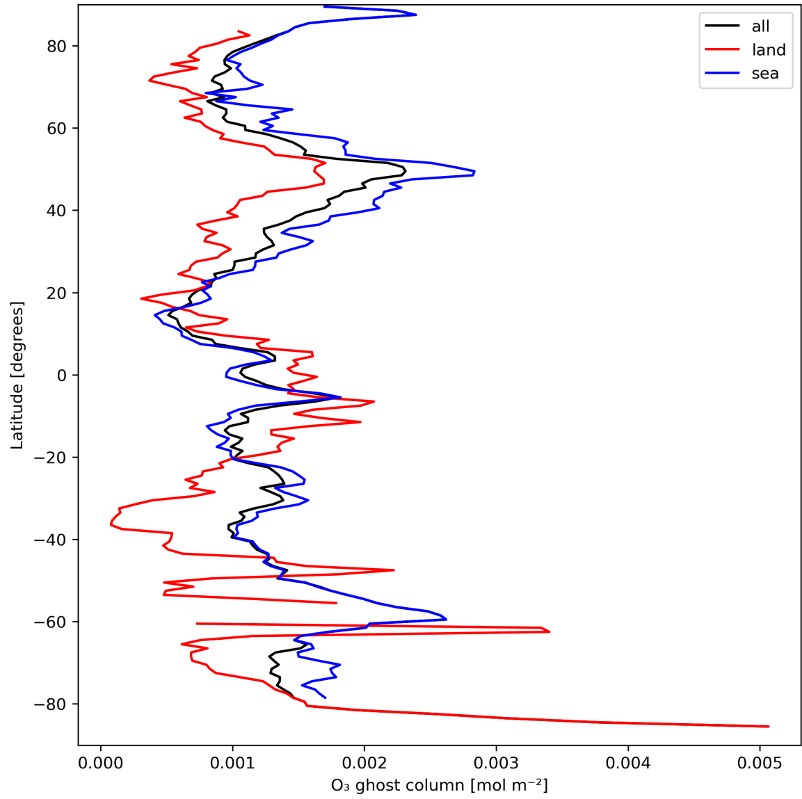
Figure 18: Zonal average of "O 3 ghost column" for 2024-03-27 to 2024-03-29.
