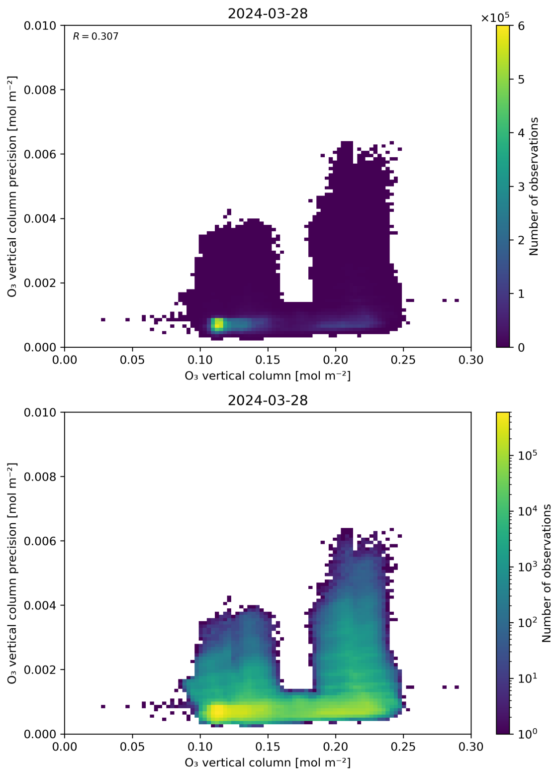
Figure 41: Scatter density plot of “O 3 vertical column” against “O 3 vertical column precision” for 2024-03-27 to 2024-03-29.
