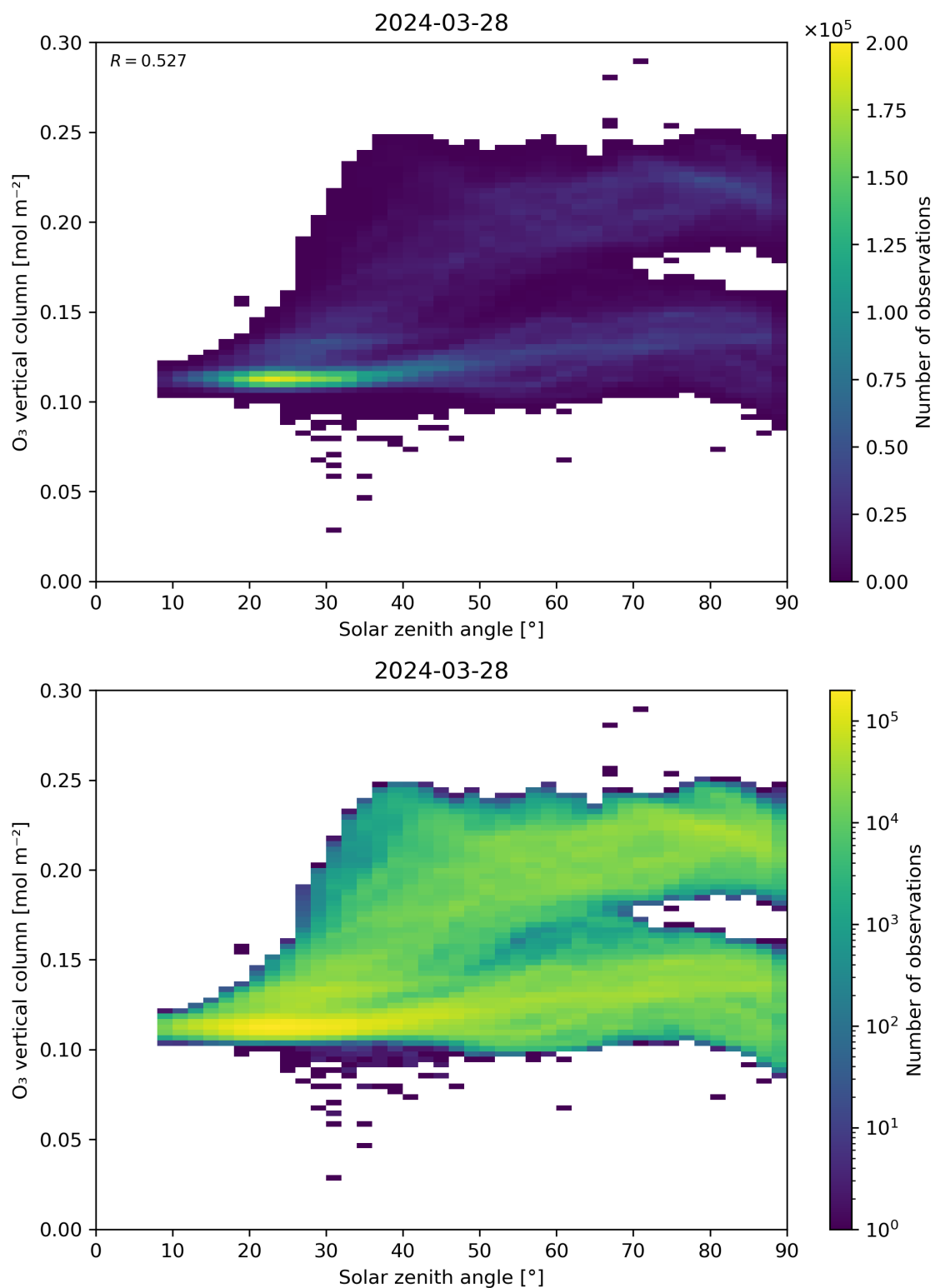
Figure 47: Scatter density plot of “Solar zenith angle” against “O 3 vertical column” for 2024-03-27 to 2024-03-29.
