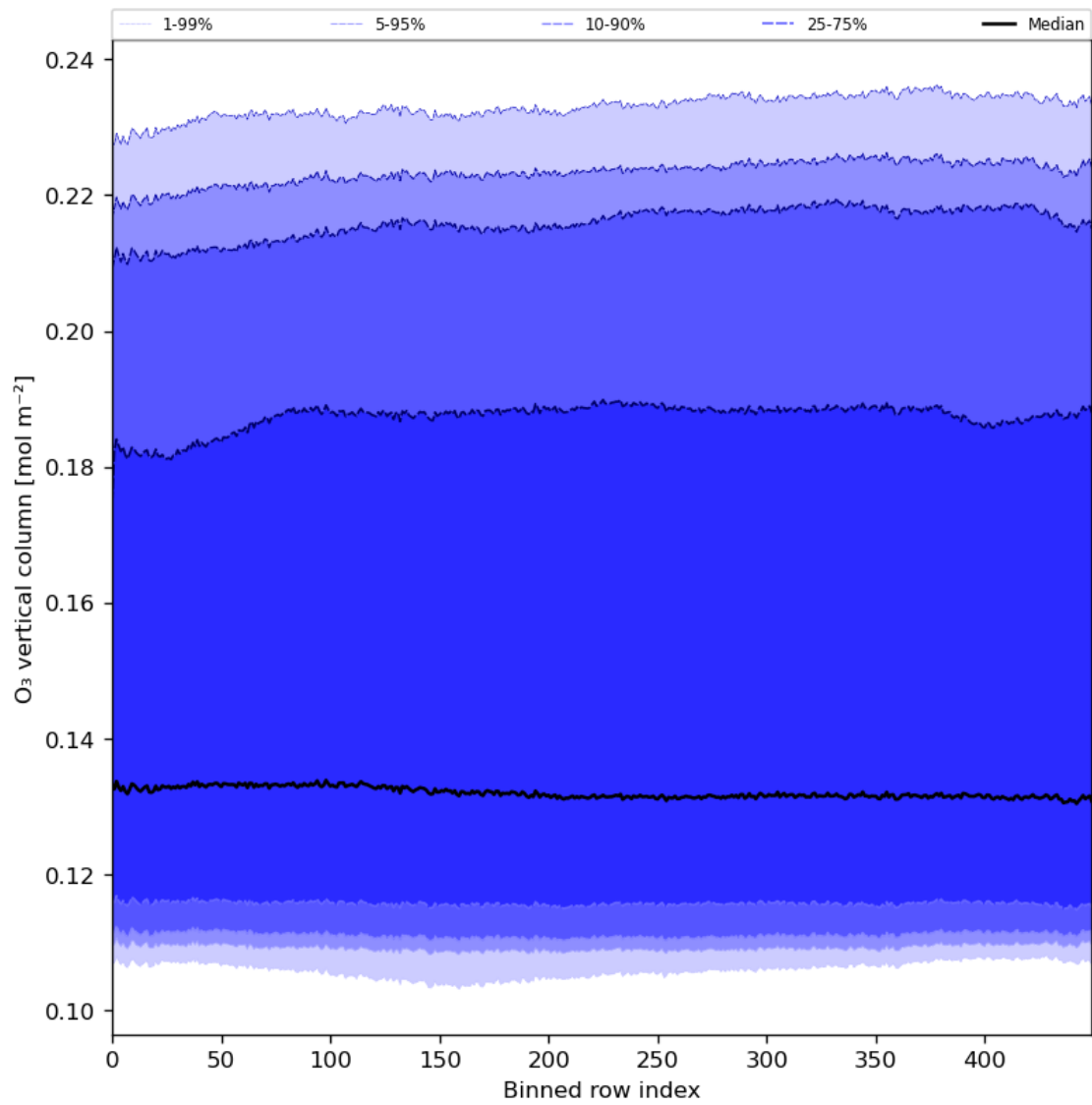
Figure 28: Along track statistics of “ O_3 vertical column” for 2024-03-27 to 2024-03-29
