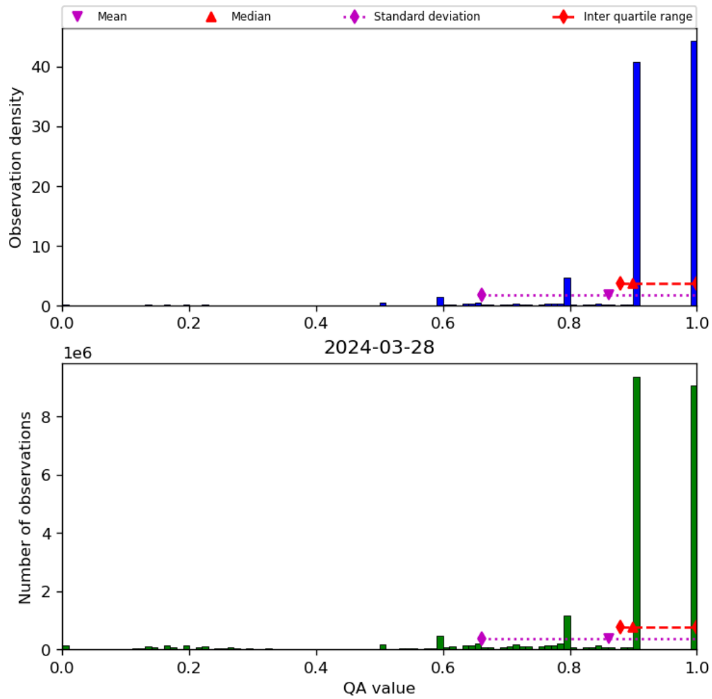
Figure 20: Histogram of “QA value” for 2024-03-27 to 2024-03-29
