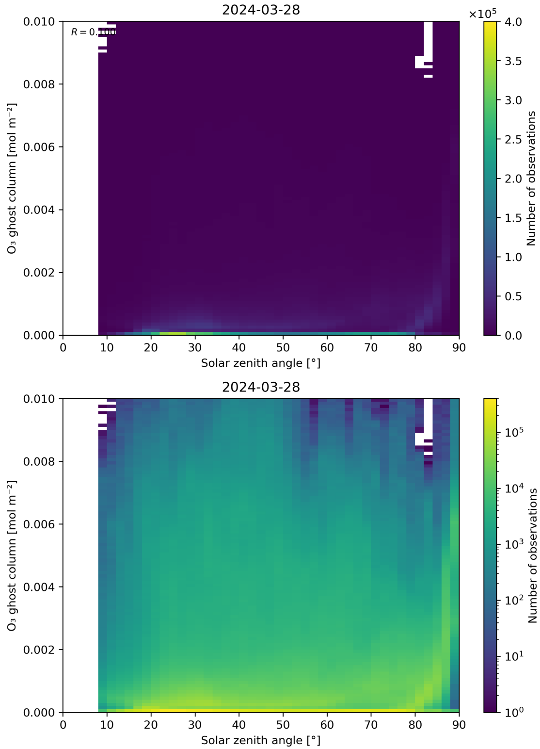
Figure 46: Scatter density plot of “Solar zenith angle” against “O 3 ghost column” for 2024-03-27 to 2024-03-29.
