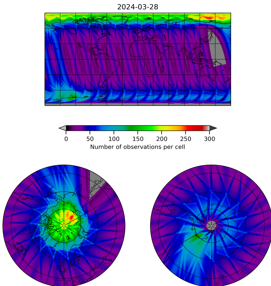
Figure 12: Map of the number of observations for 2024-03-27 to 2024-03-29
