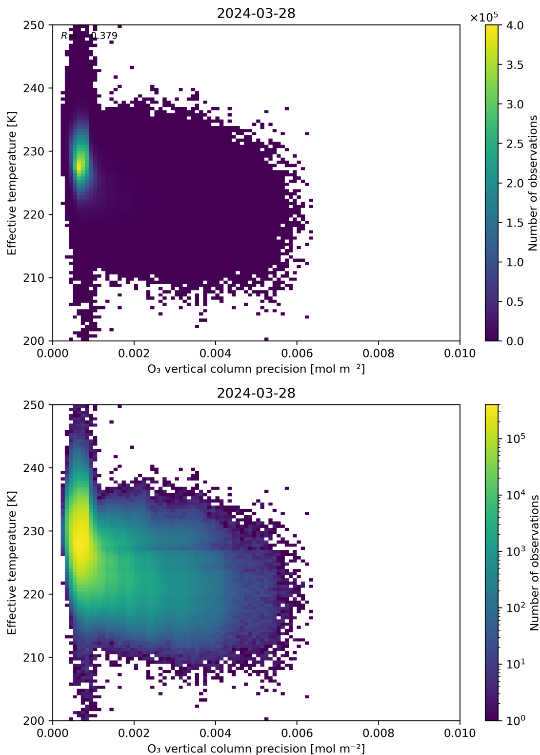
Figure 42: Scatter density plot of “O 3 vertical column precision” against “Effective temperature” for 2024-03-27 to 2024-03-29.
