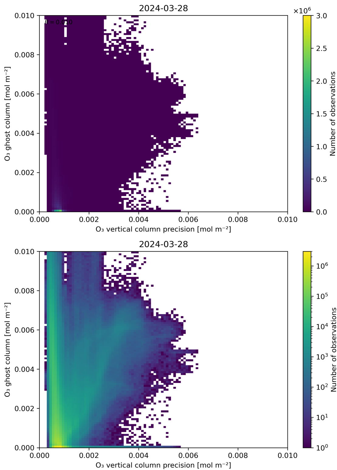
Figure 43: Scatter density plot of “O 3 vertical column precision” against “O 3 ghost column” for 2024-03-27 to 2024-03-29.
