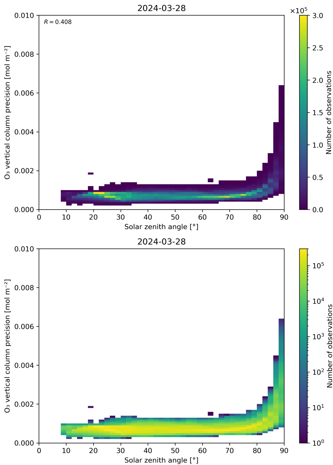
Figure 48: Scatter density plot of “Solar zenith angle” against “O 3 vertical column precision” for 2024-03-27 to 2024-03-29.
