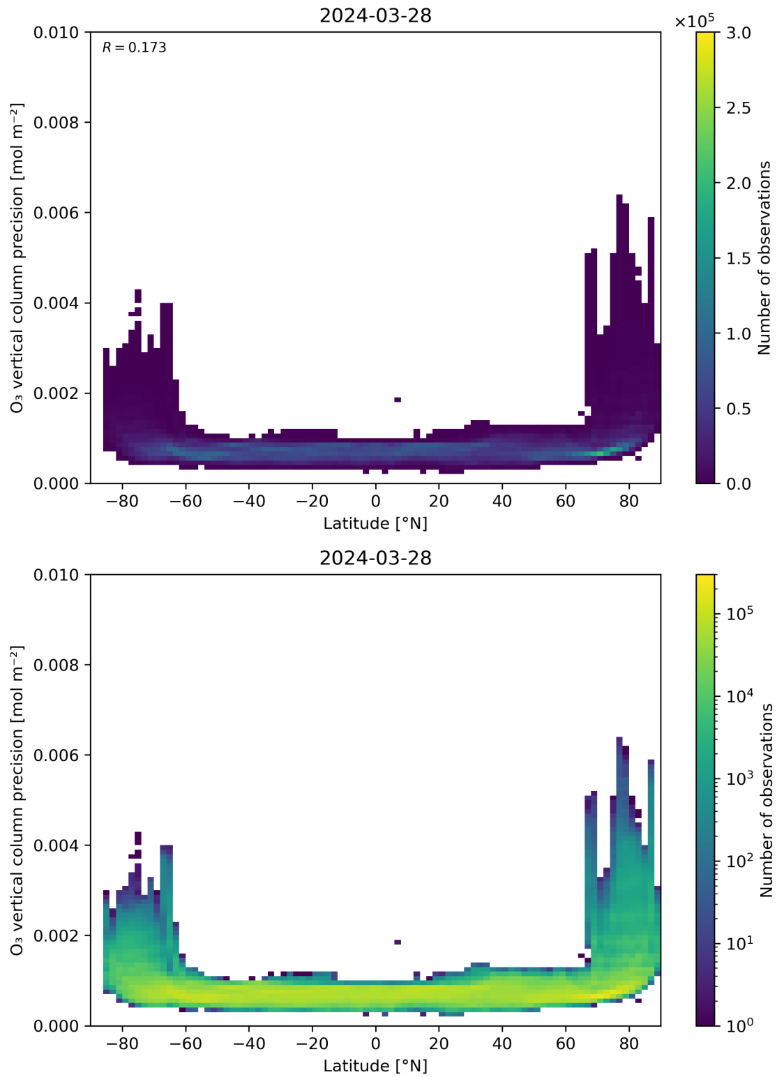
Figure 37: Scatter density plot of “Latitude” against “O 3 vertical column precision” for 2024-03-27 to 2024-03-29.
