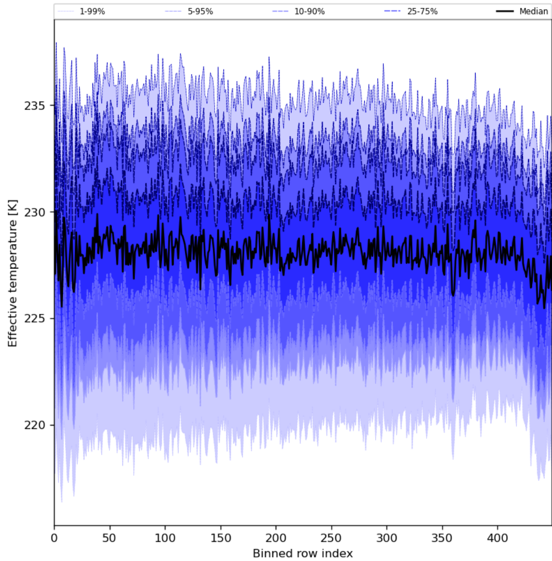
Figure 31: Along track statistics of “Effective temperature” for 2024-03-27 to 2024-03-29
