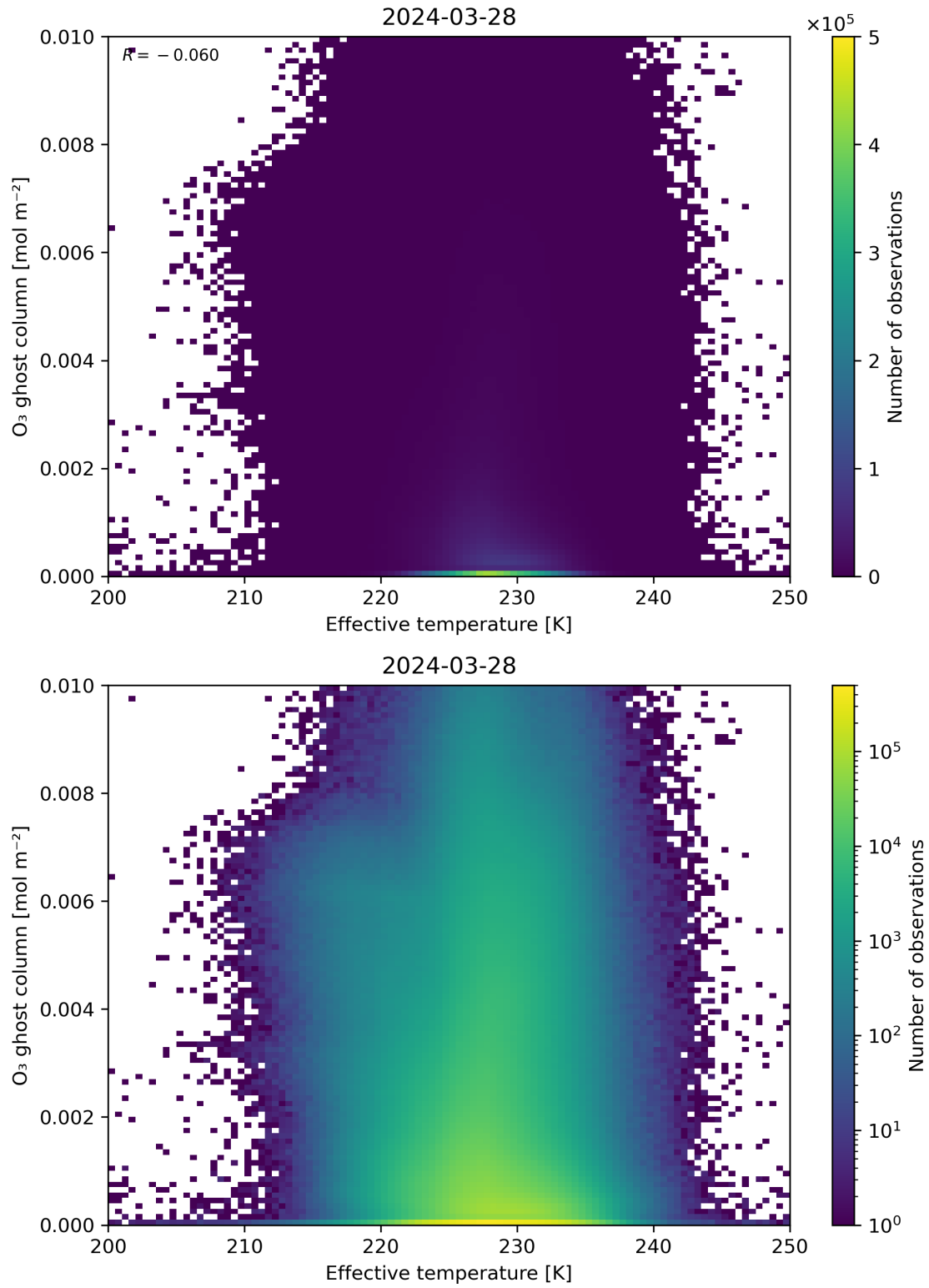
Figure 38: Scatter density plot of “Effective temperature” against “O 3 ghost column” for 2024-03-27 to 2024-03-29.
