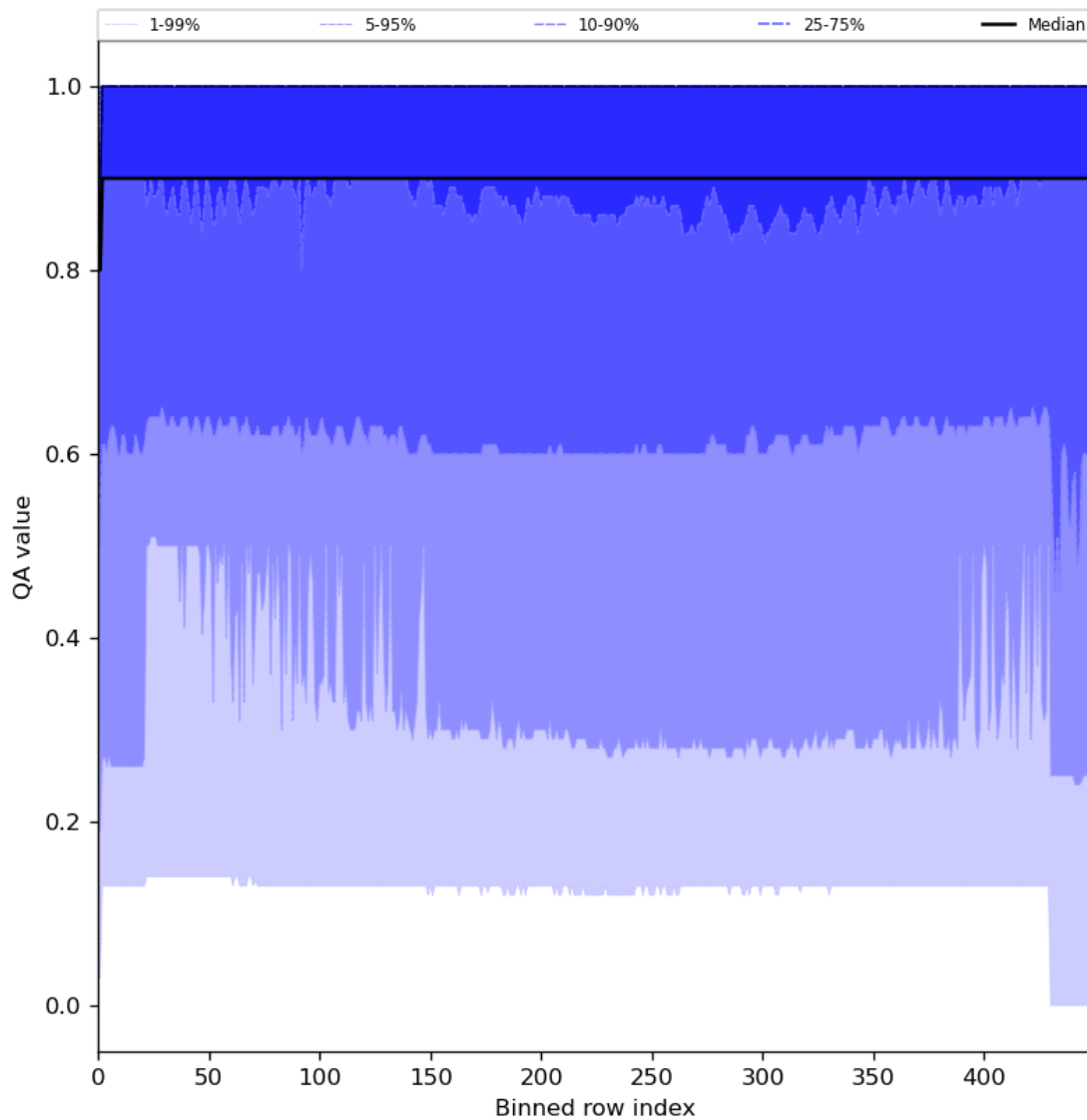
Figure 27: Along track statistics of “QA value” for 2024-03-27 to 2024-03-29
