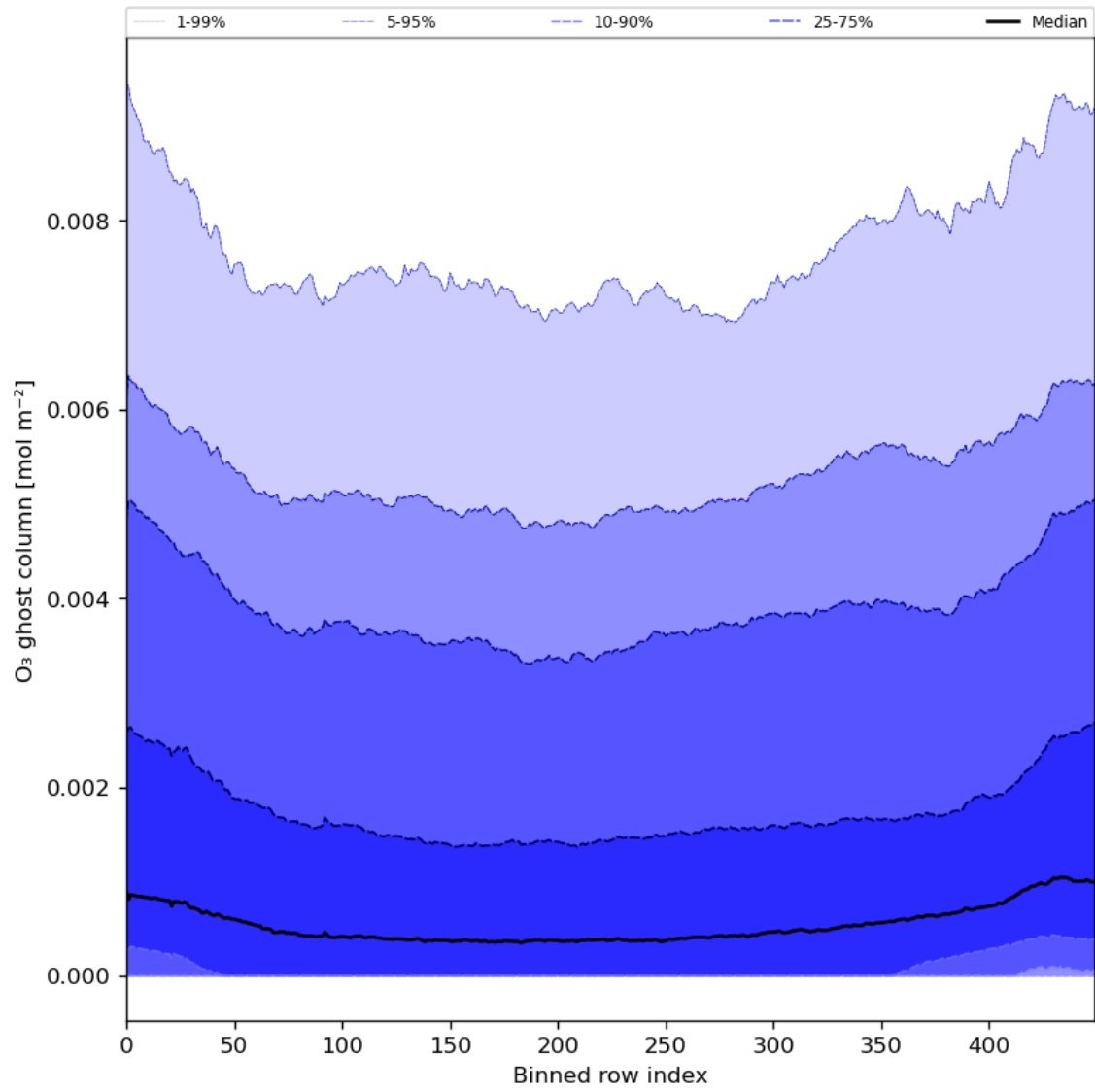
Figure 32: Along track statistics of “O 3 ghost column” for 2024-03-27 to 2024-03-29
