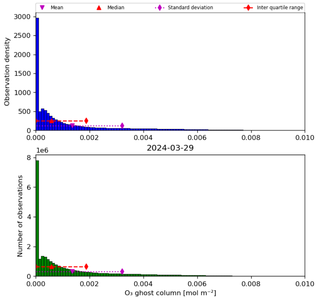
Figure 25: Histogram of “O 3 ghost column” for 2024-03-28 to 2024-03-30
