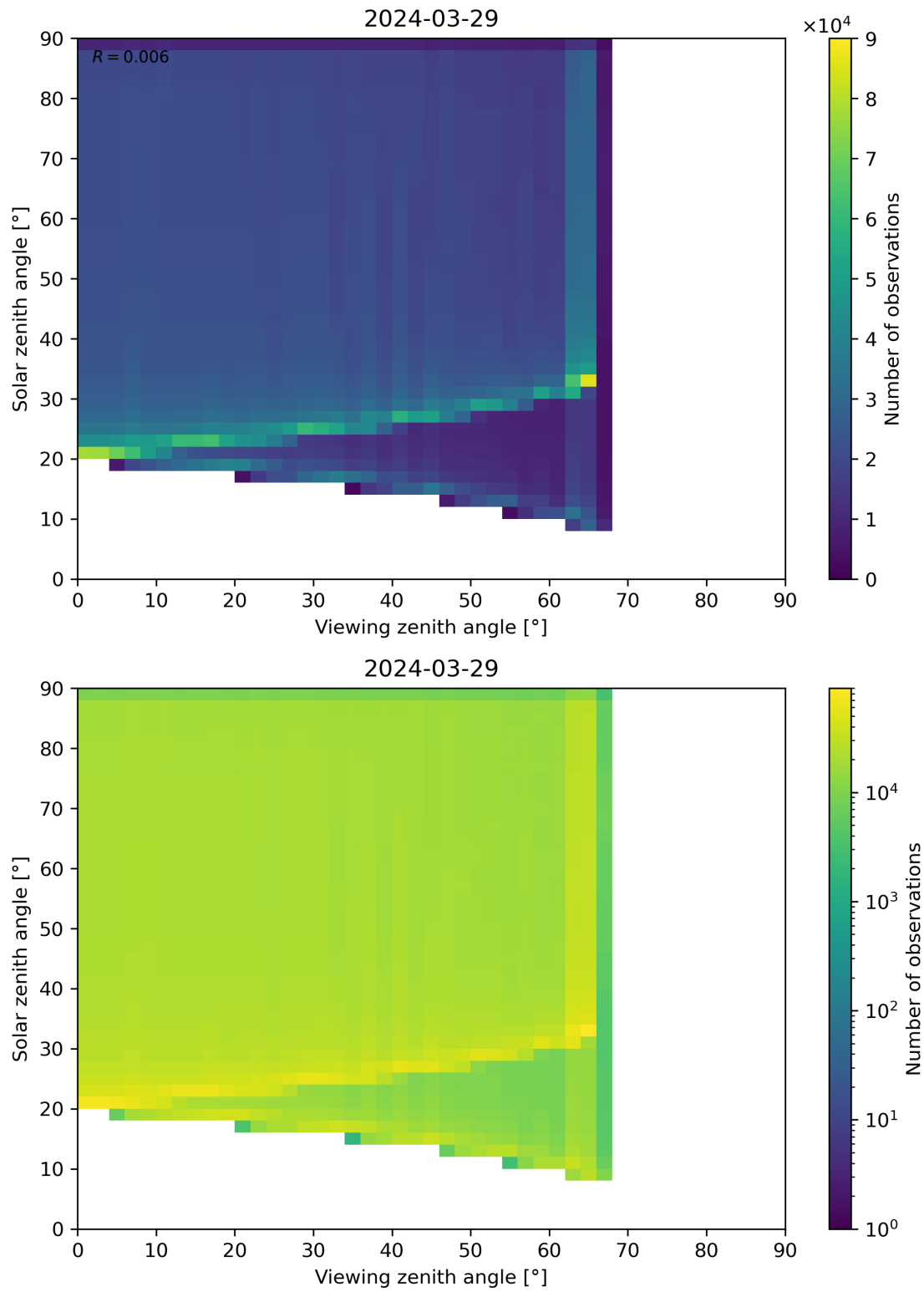
Figure 54: Scatter density plot of “Viewing zenith angle” against “Solar zenith angle” for 2024-03-28 to 2024-03-30.
