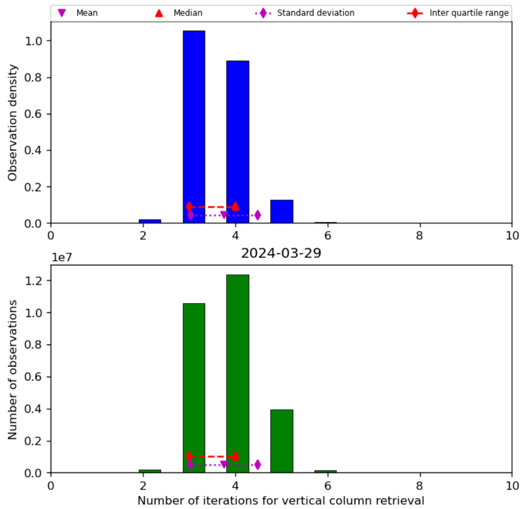
Figure 26: Histogram of “Number of iterations for vertical column retrieval” for 2024-03-28 to 2024-03-30
