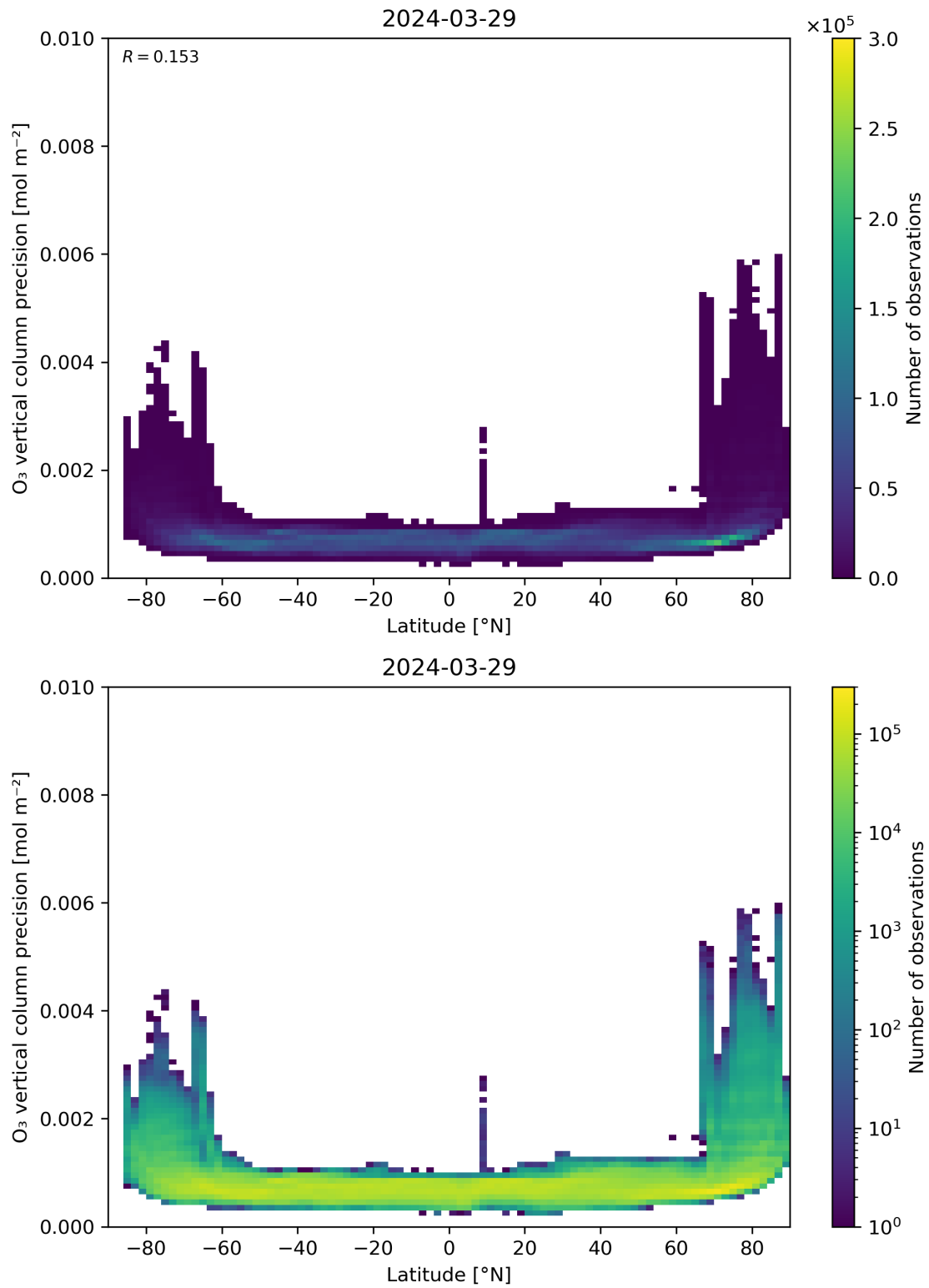
Figure 37: Scatter density plot of “Latitude” against “O 3 vertical column precision” for 2024-03-28 to 2024-03-30.
