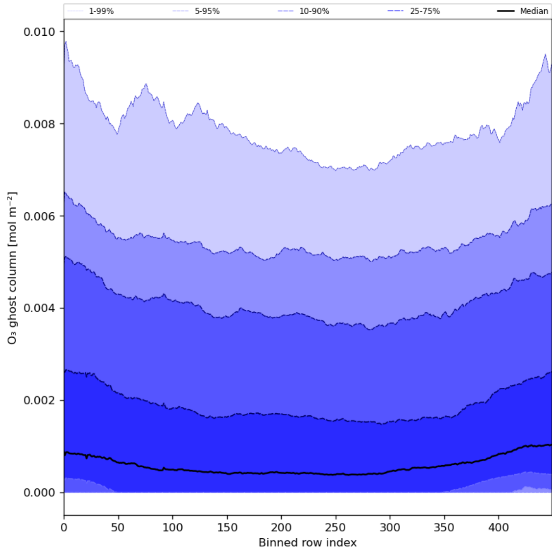
Figure 32: Along track statistics of “O 3 ghost column” for 2024-03-28 to 2024-03-30
