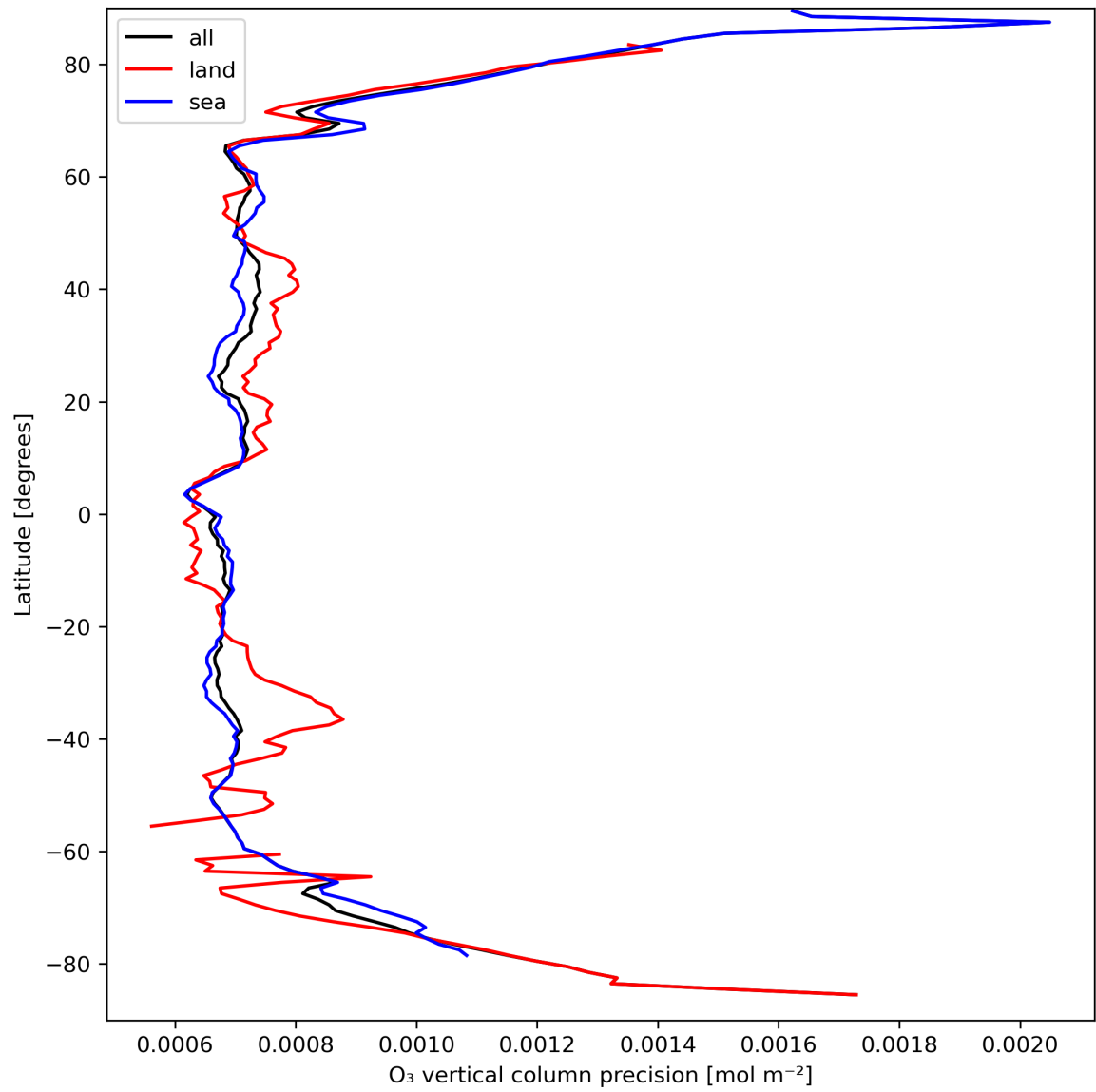
Figure 15: Zonal average of “O 3 vertical column precision” for 2024-03-28 to 2024-03-30.
