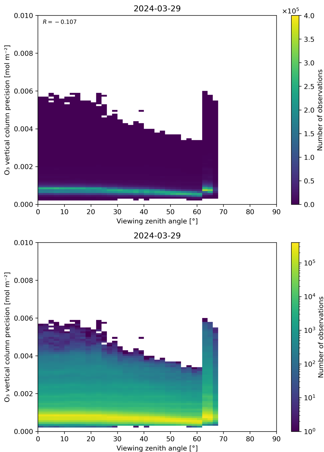
Figure 53: Scatter density plot of “Viewing zenith angle” against “O 3 vertical column precision” for 2024-03-28 to 2024-03-30.
