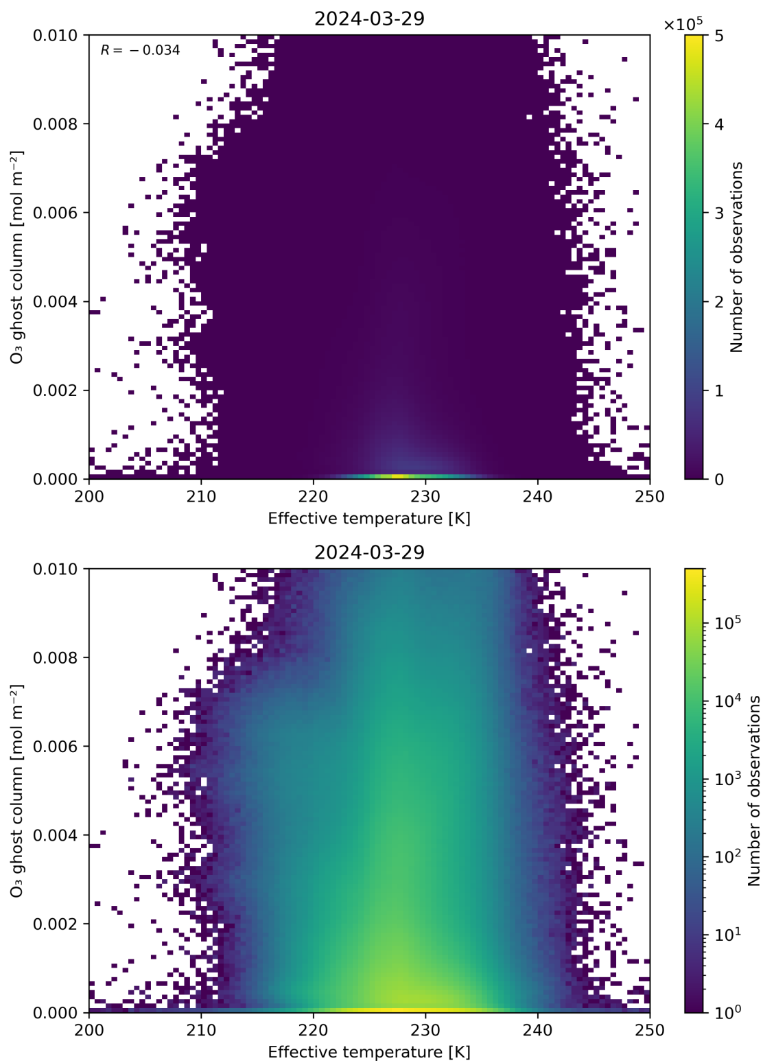
Figure 38: Scatter density plot of “Effective temperature” against “O 3 ghost column” for 2024-03-28 to 2024-03-30.
