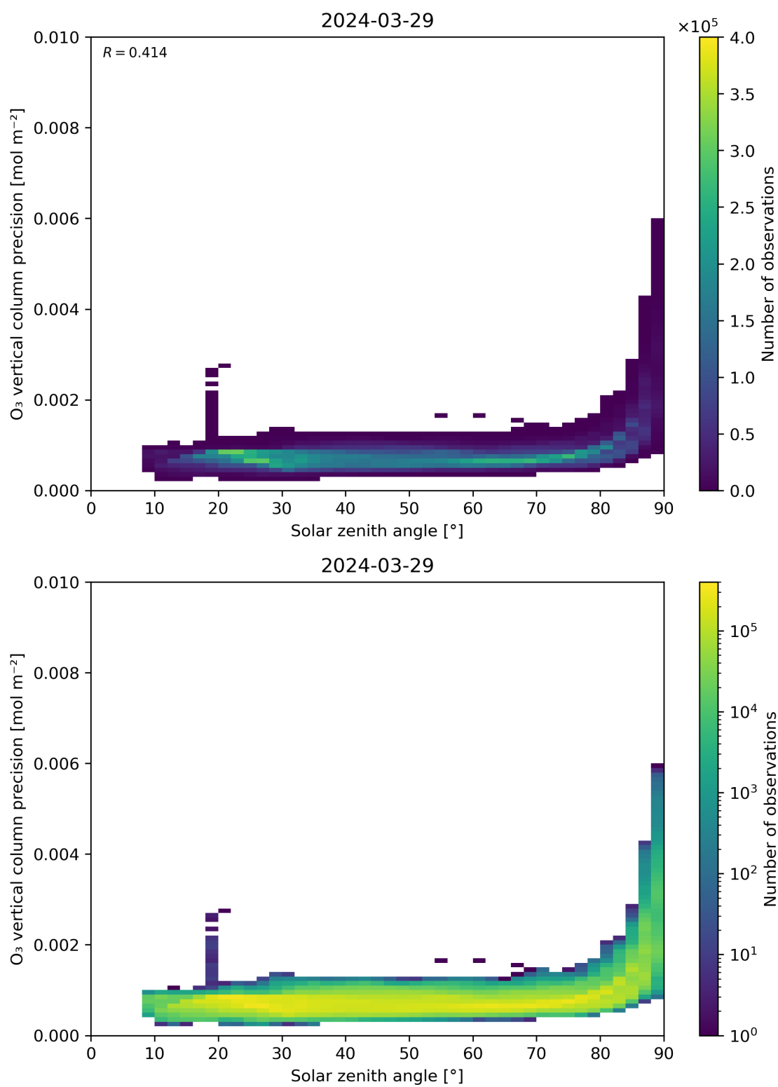
Figure 48: Scatter density plot of “Solar zenith angle” against “O 3 vertical column precision” for 2024-03-28 to 2024-03-30.
