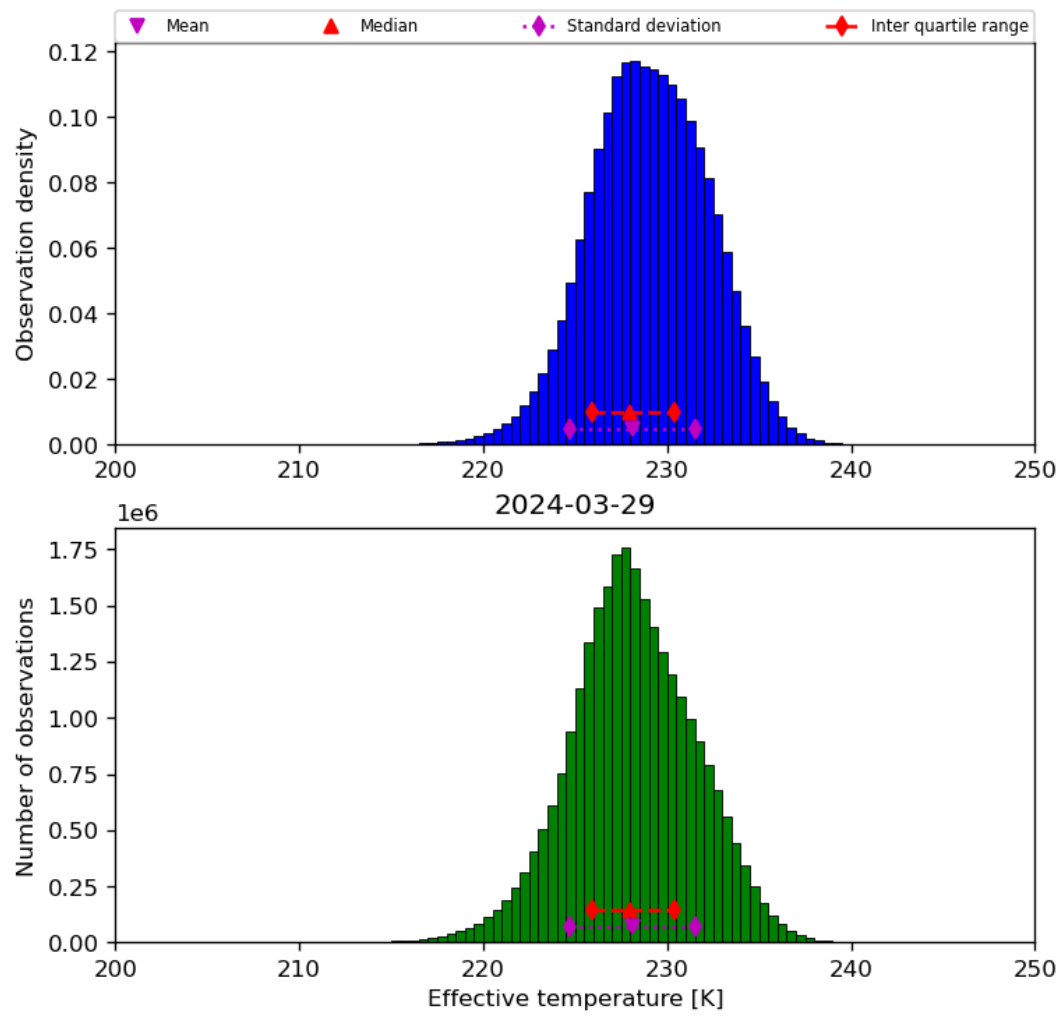
Figure 24: Histogram of “Effective temperature” for 2024-03-28 to 2024-03-30
