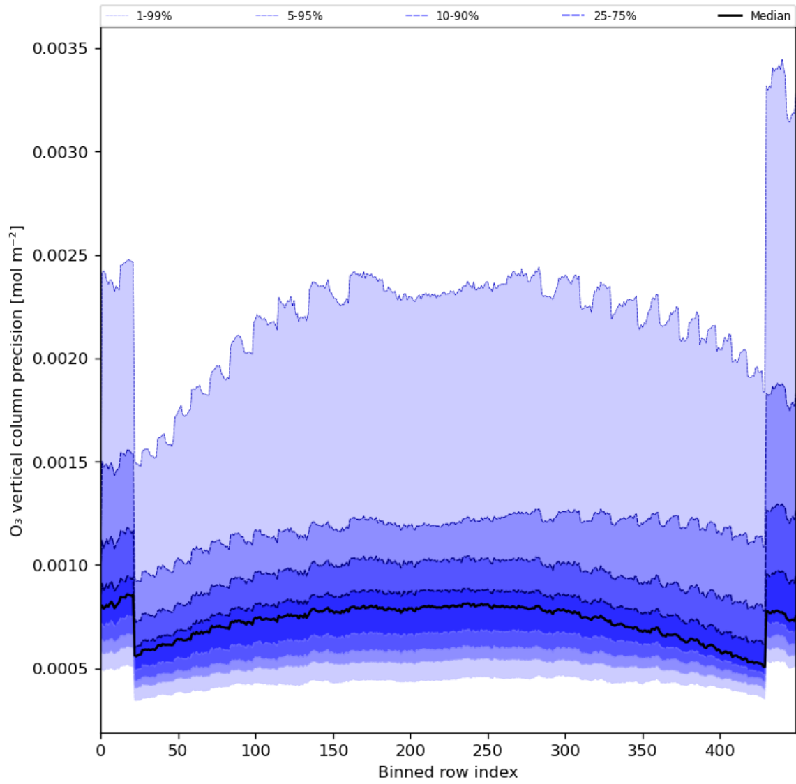
Figure 29: Along track statistics of “O 3 vertical column precision” for 2024-03-28 to 2024-03-30
