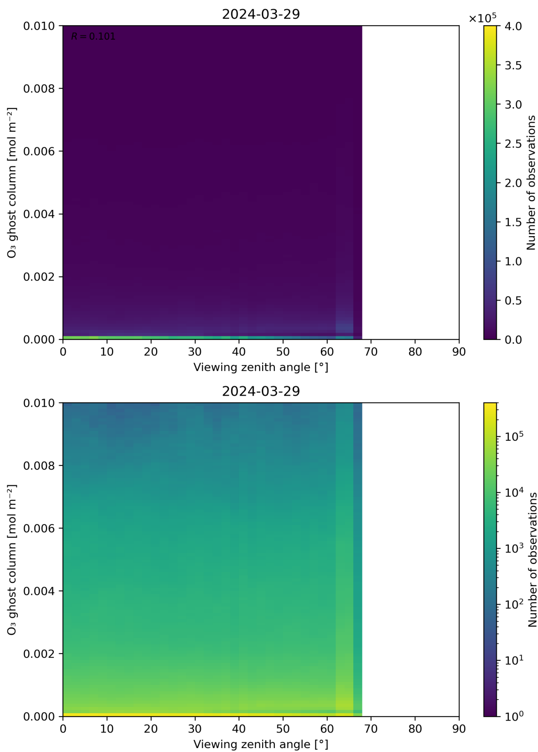
Figure 51: Scatter density plot of “Viewing zenith angle” against “O 3 ghost column” for 2024-03-28 to 2024-03-30.
