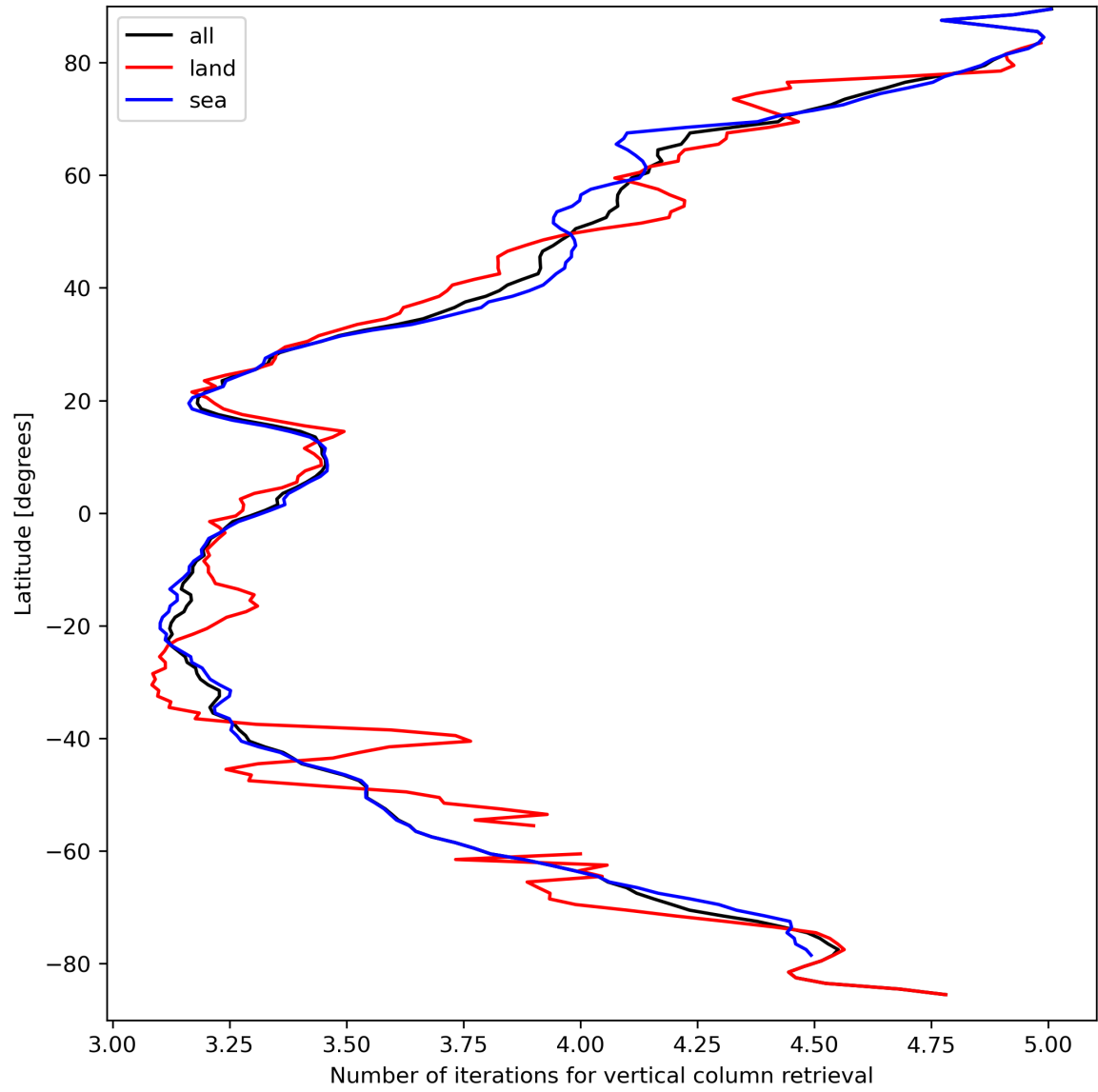
Figure 19: Zonal average of “Number of iterations for vertical column retrieval” for 2024-03-28 to 2024-03-30.
