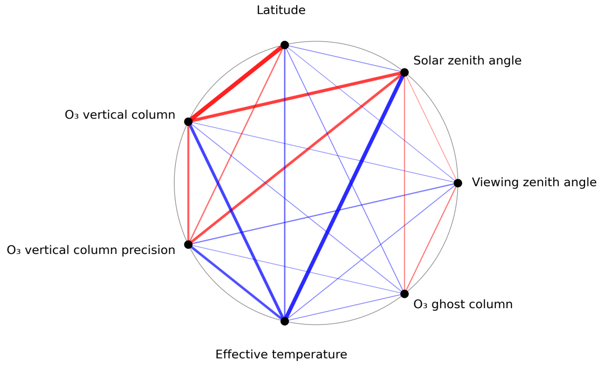
Figure 1: Map of correlation graph for 2024-03-28 to 2024-03-30.
