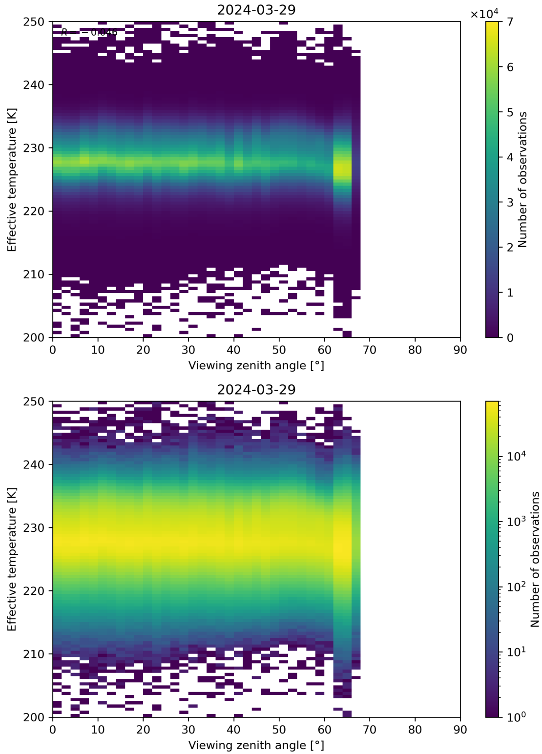
Figure 50: Scatter density plot of “Viewing zenith angle” against “Effective temperature” for 2024-03-28 to 2024-03-30.
