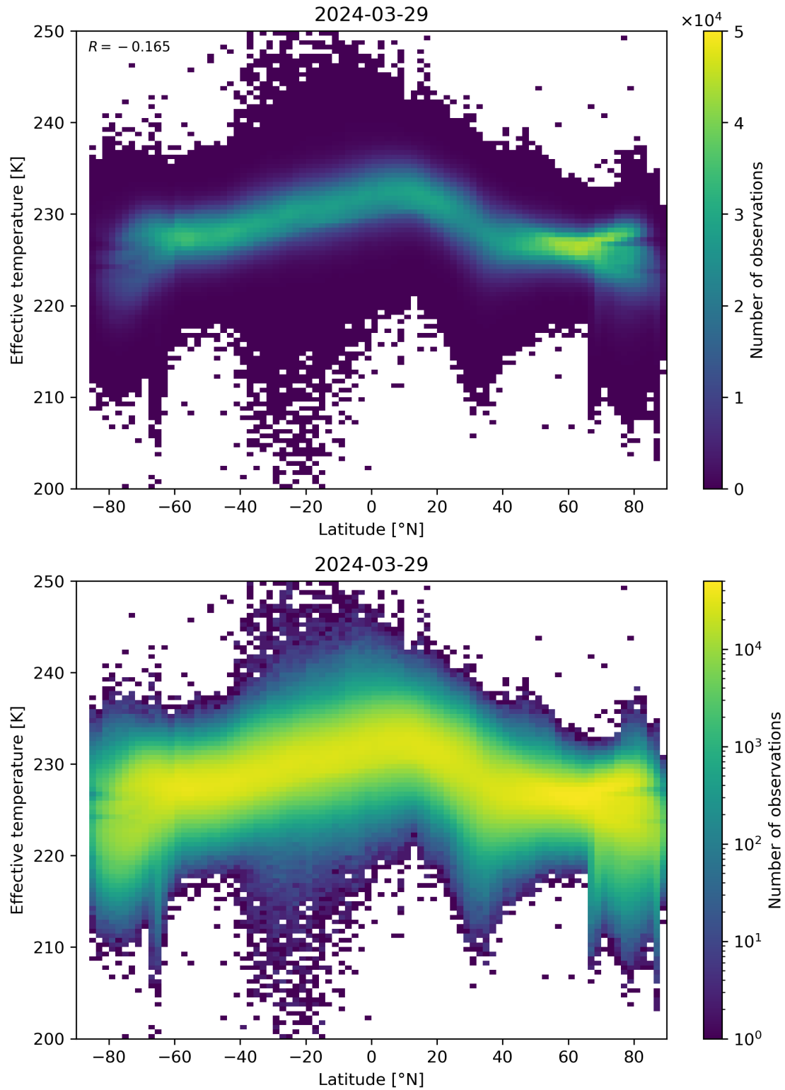
Figure 34: Scatter density plot of “Latitude” against “Effective temperature” for 2024-03-28 to 2024-03-30.
