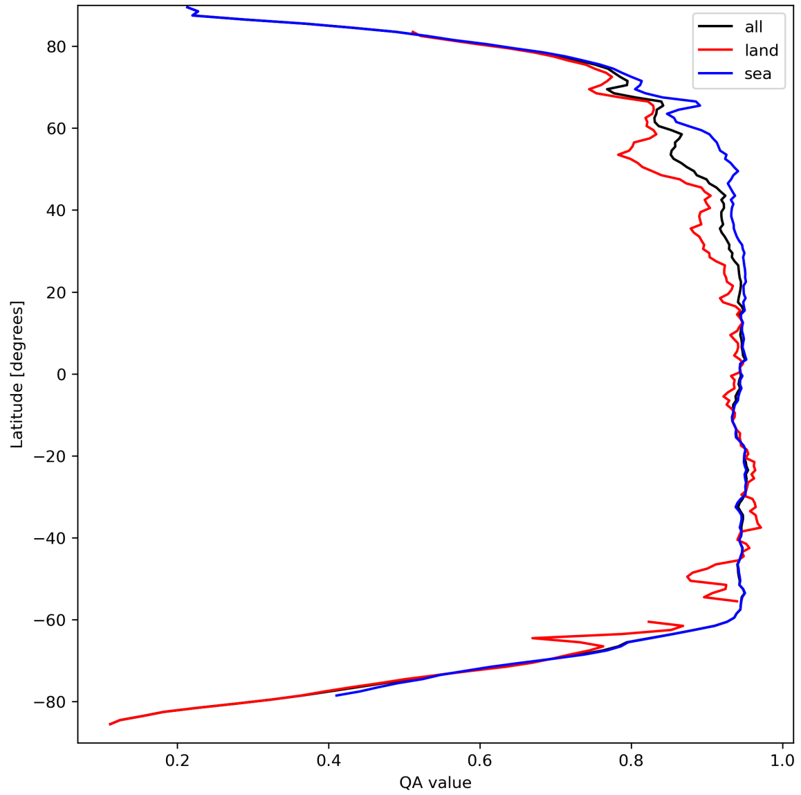
Figure 13: Zonal average of “QA value” for 2024-03-28 to 2024-03-30.
