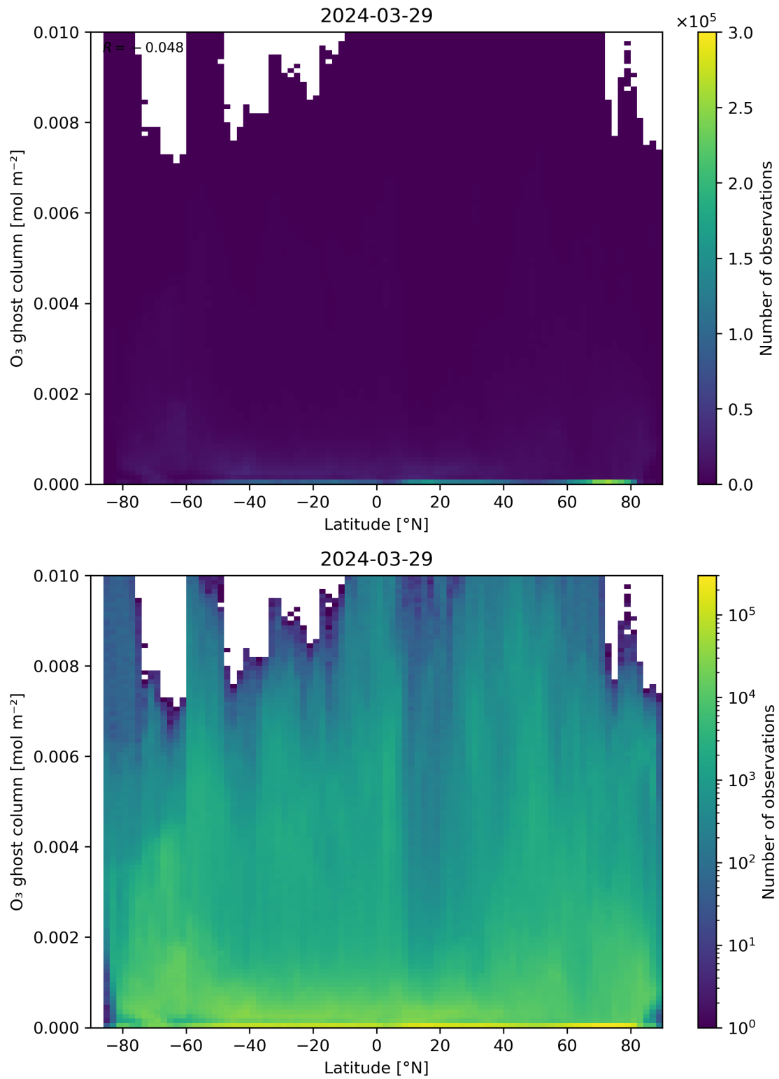
Figure 35: Scatter density plot of “Latitude” against “O 3 ghost column” for 2024-03-28 to 2024-03-30.
