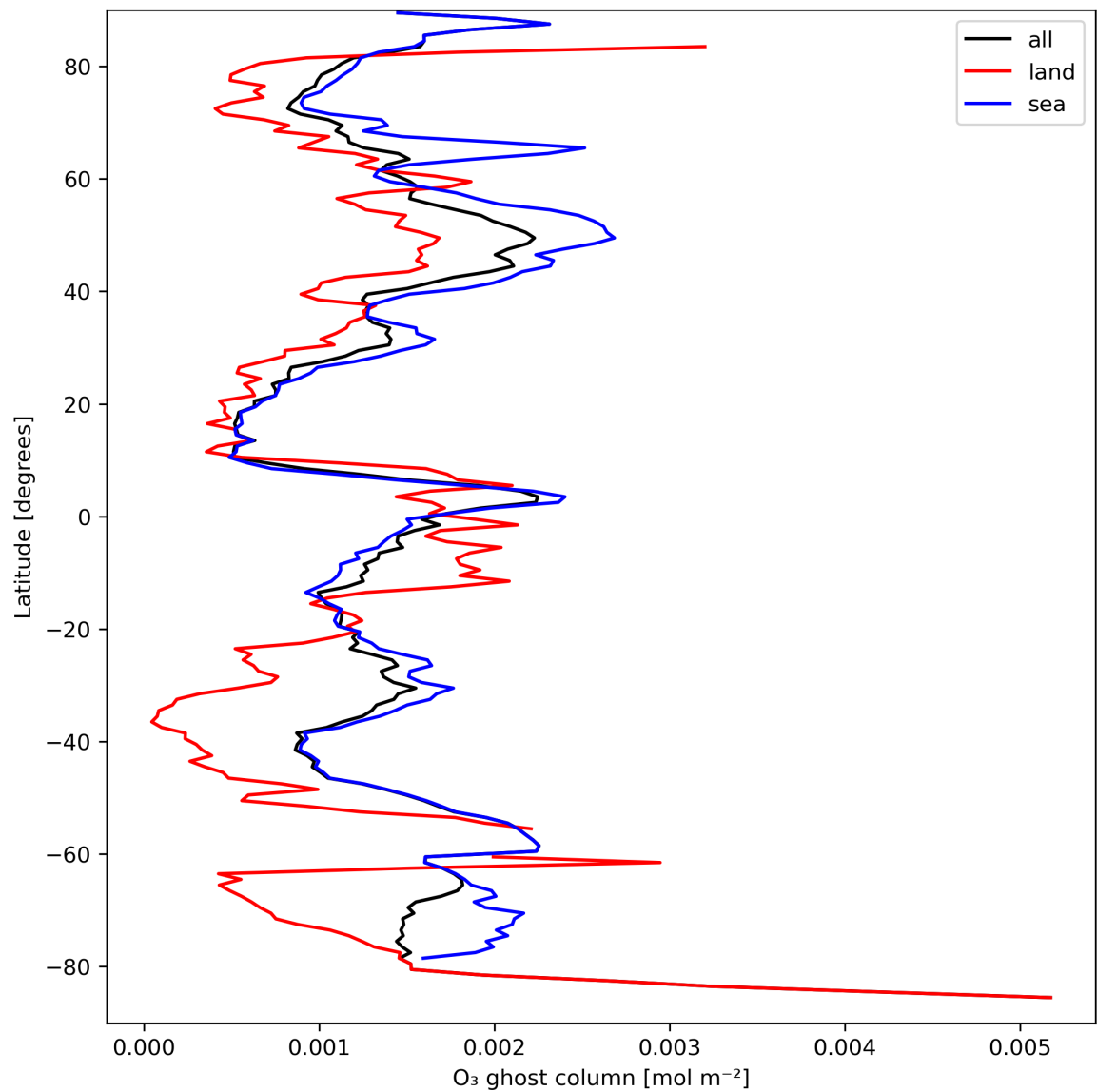
Figure 18: Zonal average of “O 3 ghost column” for 2024-03-28 to 2024-03-30.
