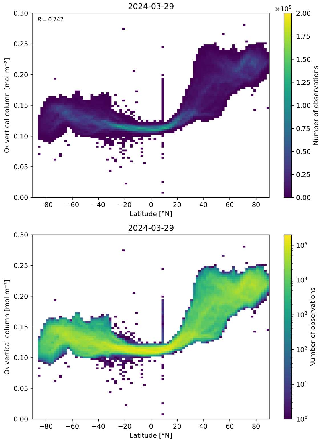
Figure 36: Scatter density plot of “Latitude” against “O 3 vertical column” for 2024-03-28 to 2024-03-30.
