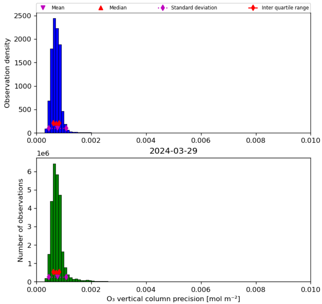
Figure 22: Histogram of “O 3 vertical column precision” for 2024-03-28 to 2024-03-30
