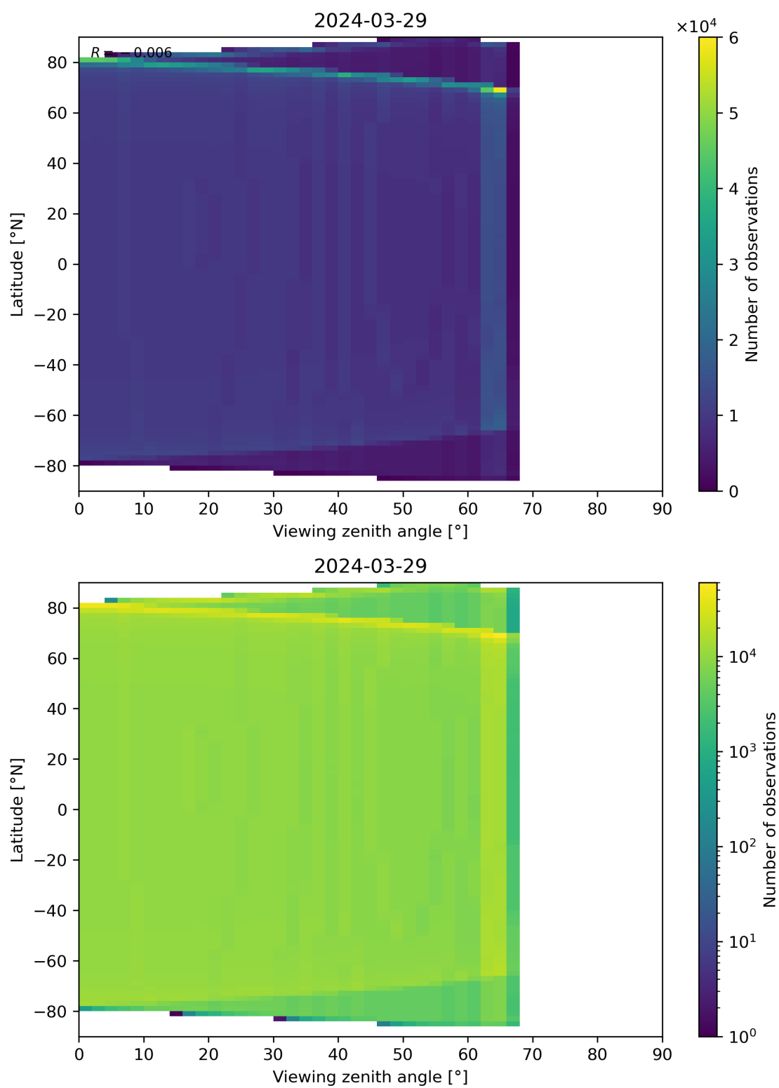
Figure 49: Scatter density plot of “Viewing zenith angle” against “Latitude” for 2024-03-28 to 2024-03-30.
