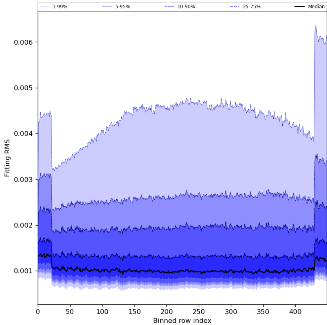
Figure 30: Along track statistics of “Fitting RMS” for 2024-03-28 to 2024-03-30
