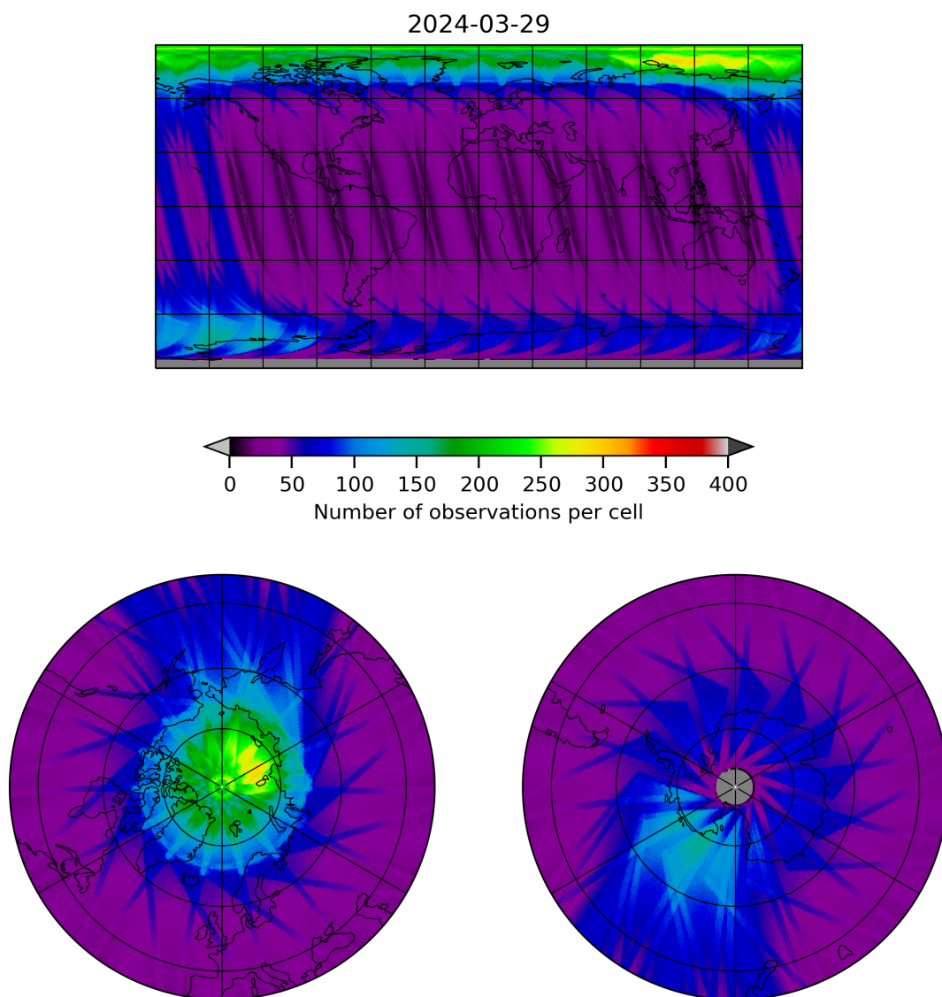
Figure 12: Map of the number of observations for 2024-03-28 to 2024-03-30
