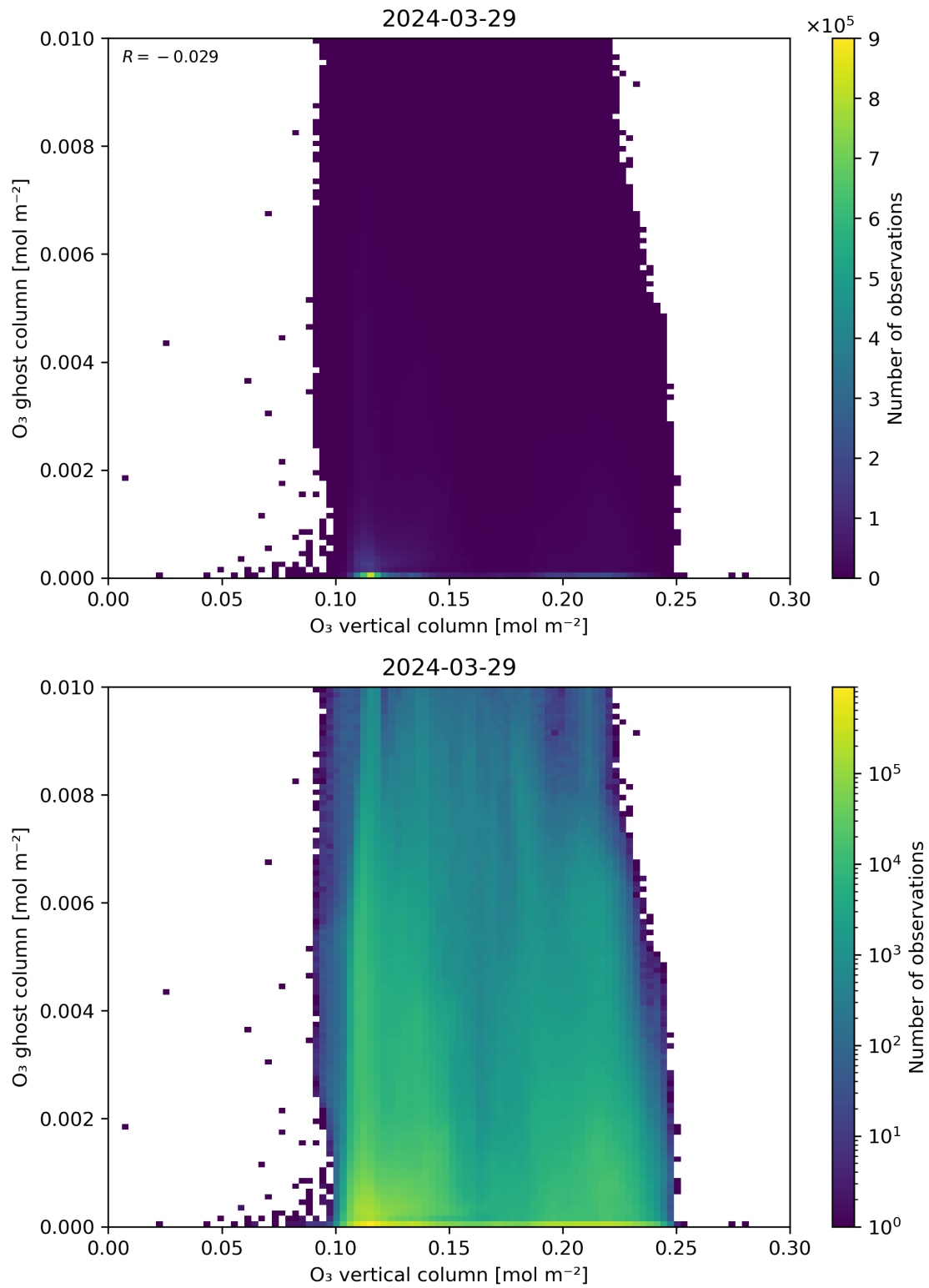
Figure 40: Scatter density plot of “O 3 vertical column” against “O 3 ghost column” for 2024-03-28 to 2024-03-30.
