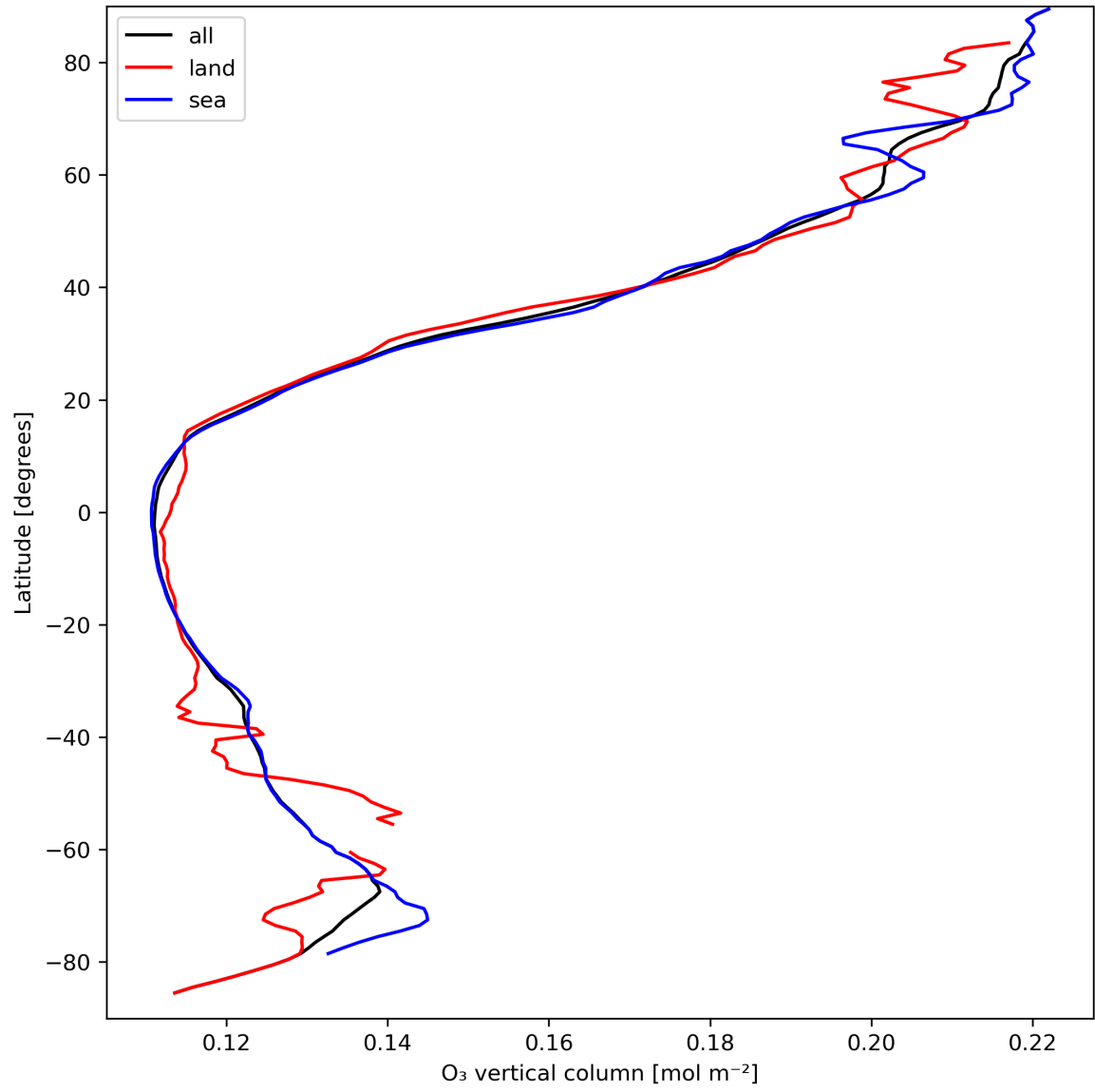
Figure 14: Zonal average of “O 3 vertical column” for 2024-03-28 to 2024-03-30.
