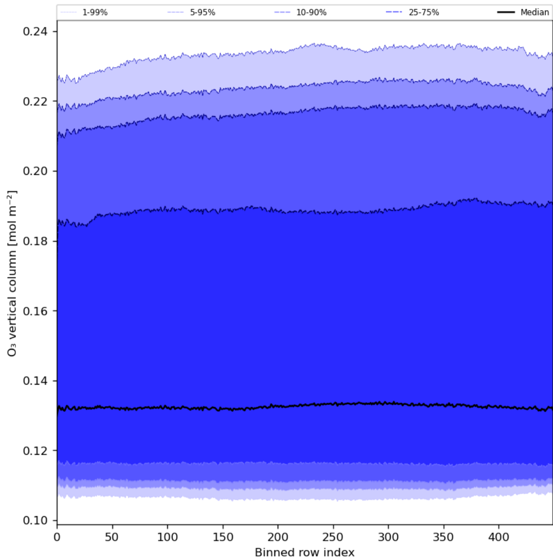
Figure 28: Along track statistics of “O 3 vertical column” for 2024-03-28 to 2024-03-30
