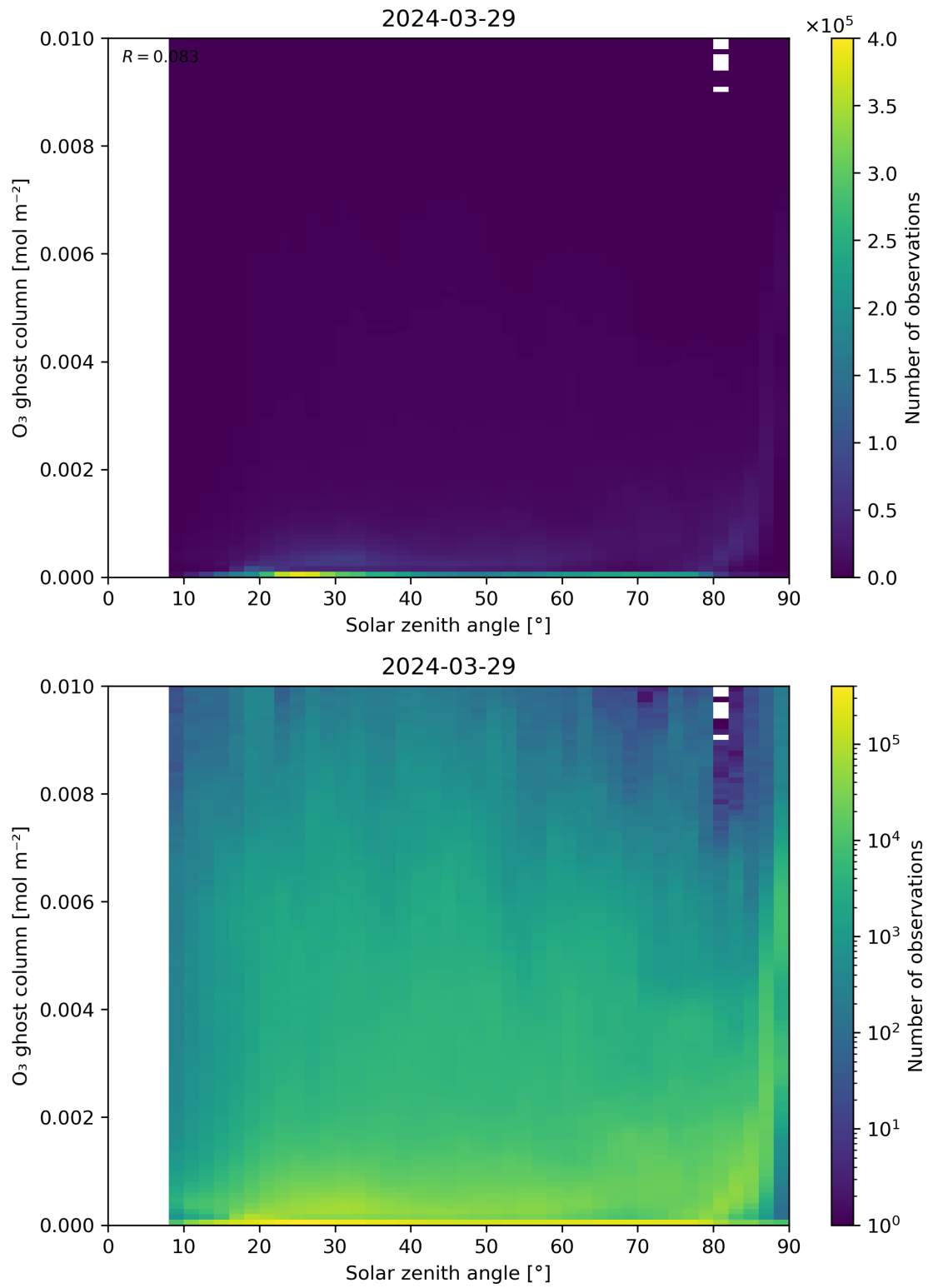
Figure 46: Scatter density plot of “Solar zenith angle” against “O 3 ghost column” for 2024-03-28 to 2024-03-30.
