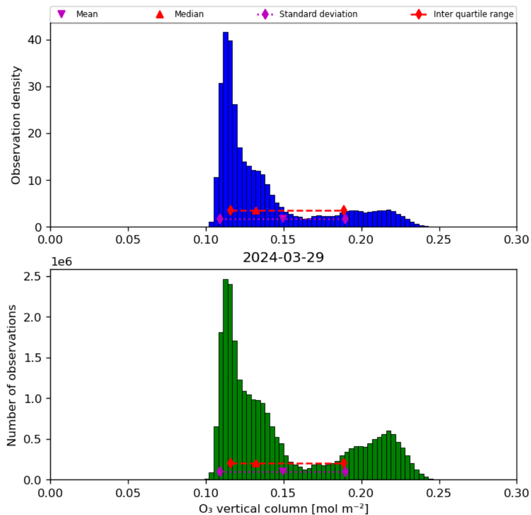
Figure 21: Histogram of “O 3 vertical column” for 2024-03-28 to 2024-03-30
