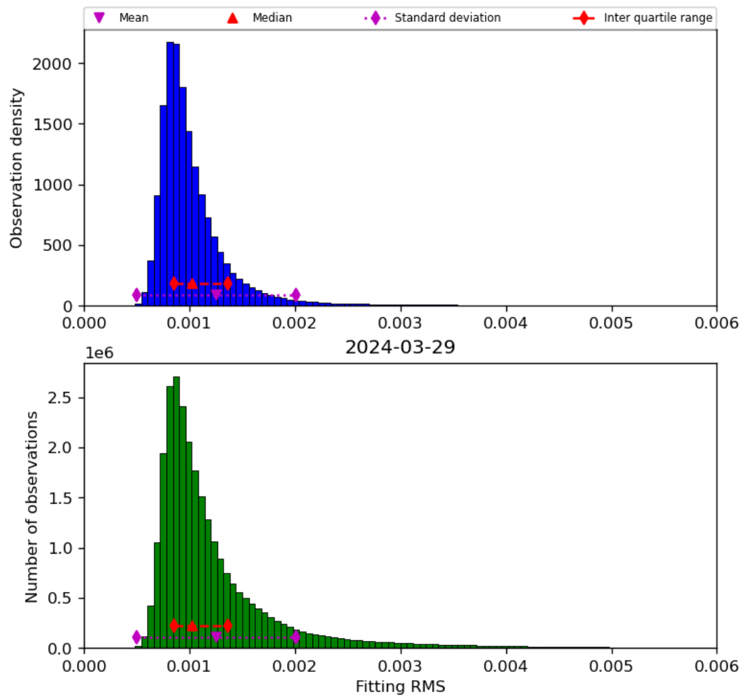
Figure 23: Histogram of “Fitting RMS” for 2024-03-28 to 2024-03-30
