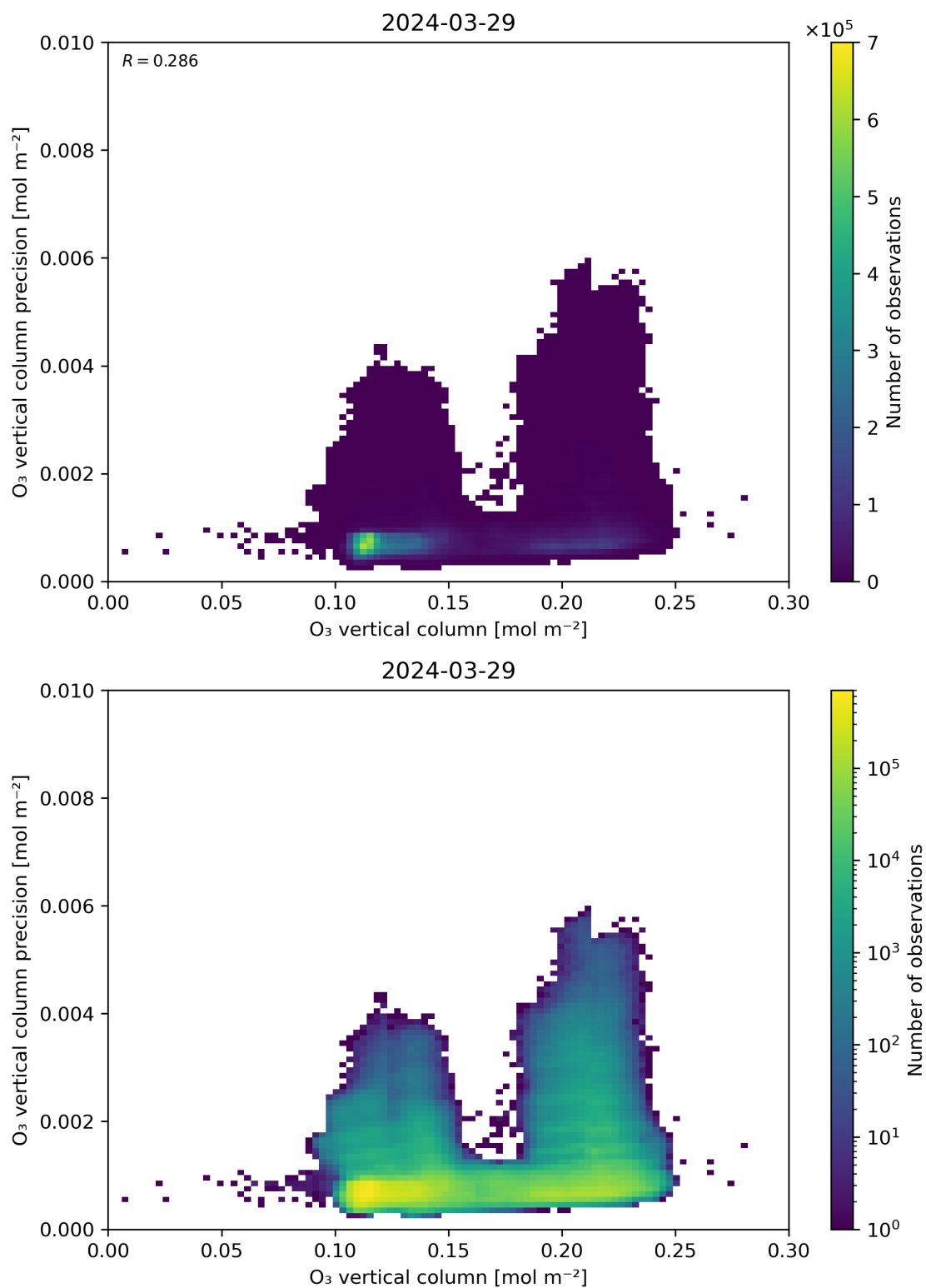
Figure 41: Scatter density plot of “O 3 vertical column” against “O 3 vertical column precision” for 2024-03-28 to 2024-03-30.
