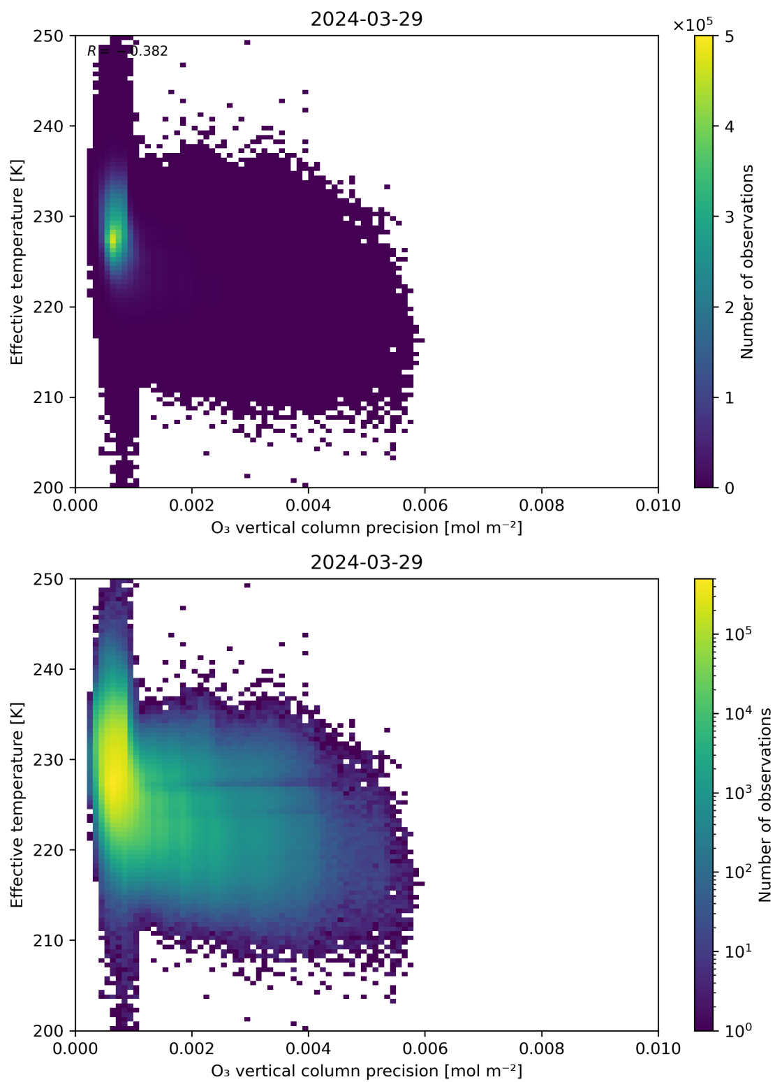
Figure 42: Scatter density plot of “O 3 vertical column precision” against “Effective temperature” for 2024-03-28 to 2024-03-30.
