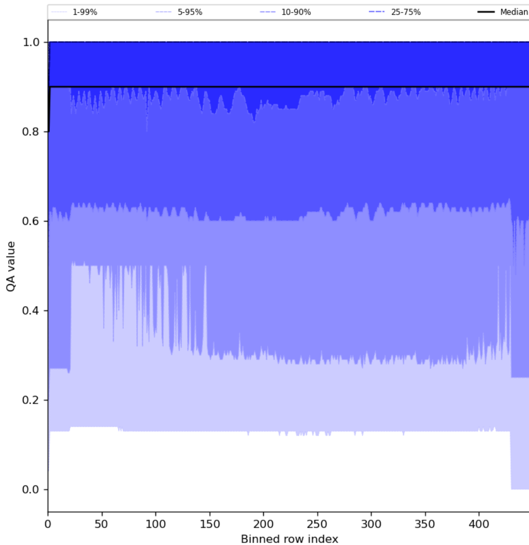
Figure 27: Along track statistics of “QA value” for 2024-03-28 to 2024-03-30
