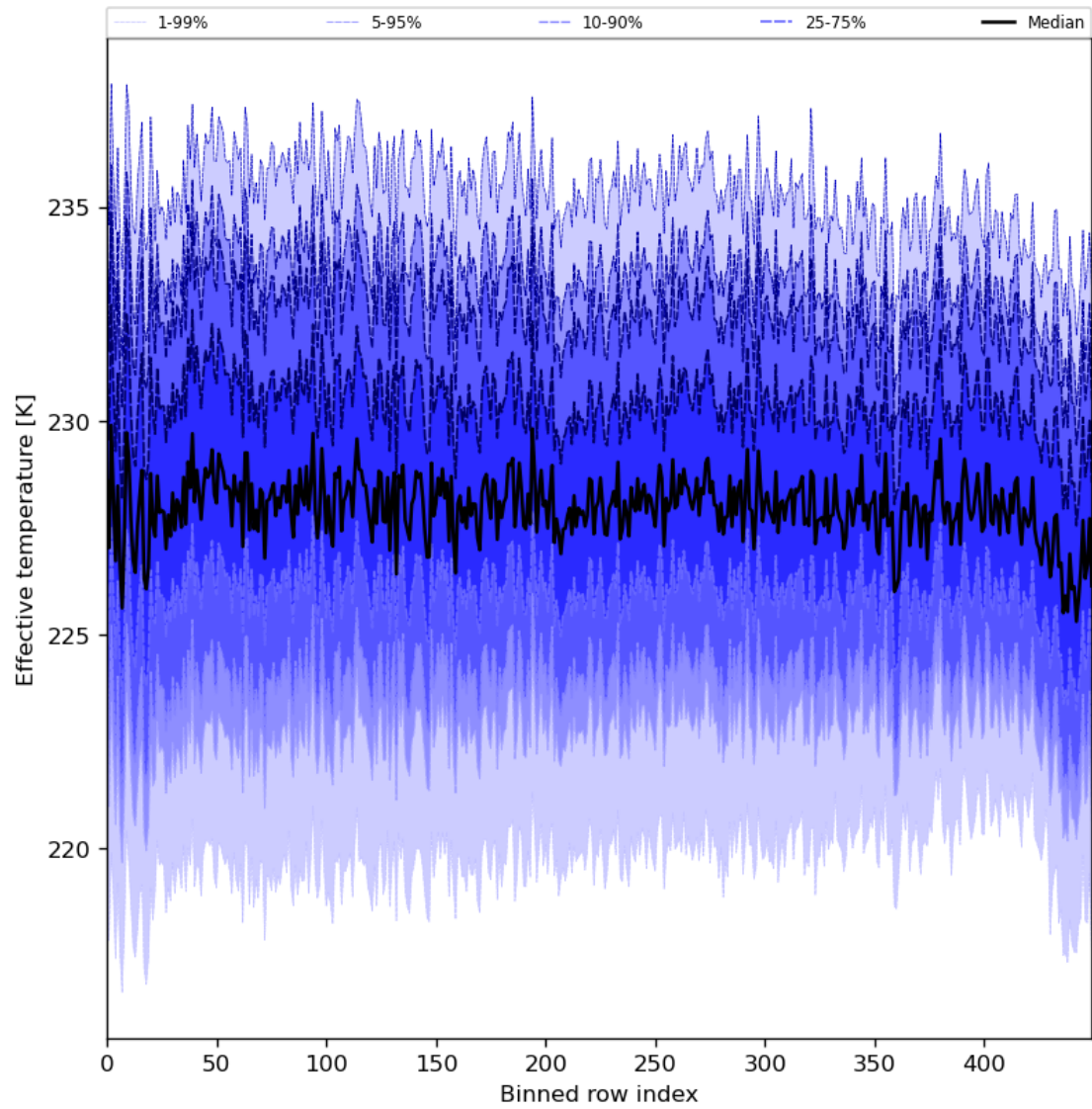
Figure 31: Along track statistics of “Effective temperature” for 2024-03-28 to 2024-03-30
