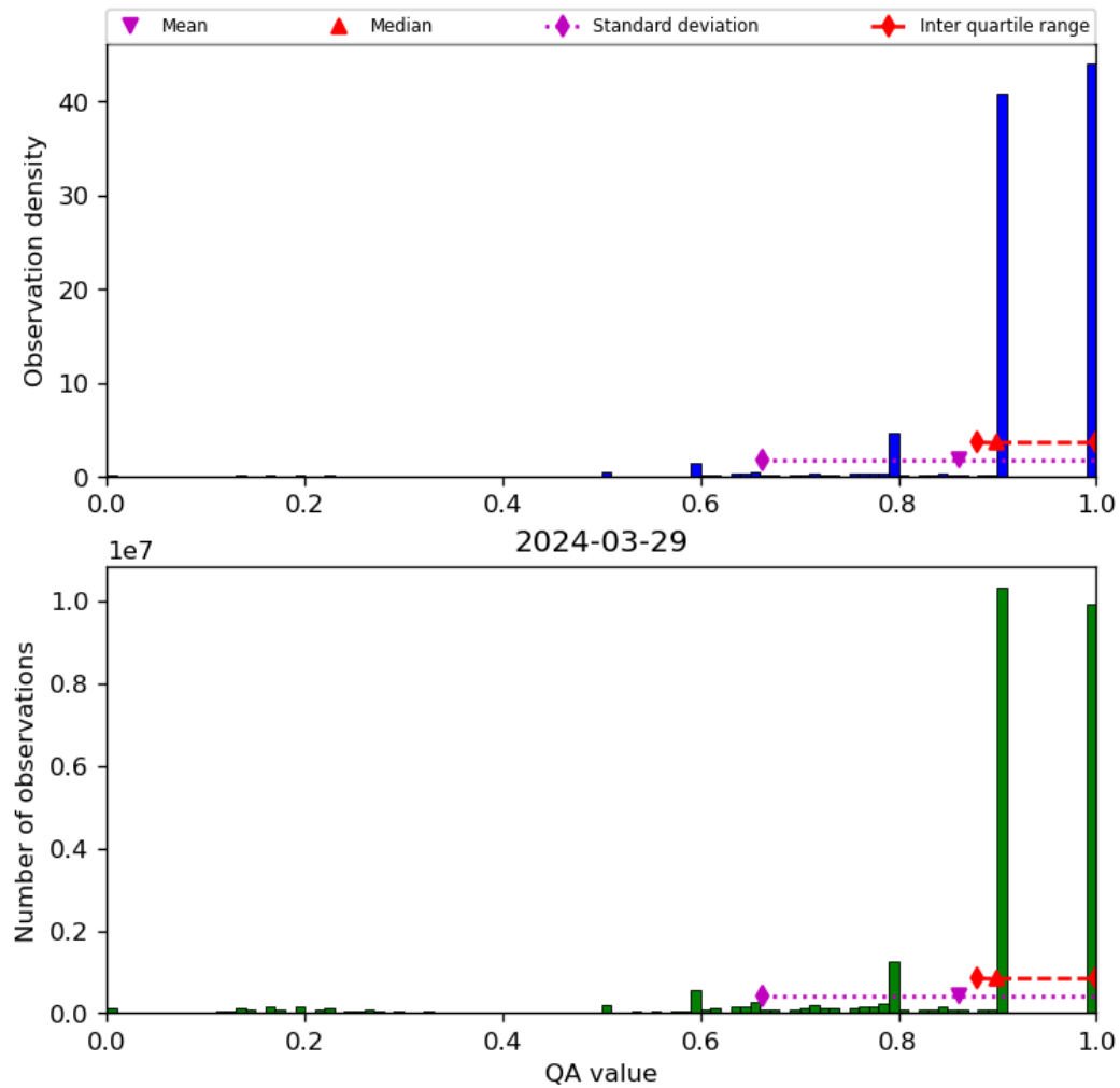
Figure 20: Histogram of “QA value” for 2024-03-28 to 2024-03-30
