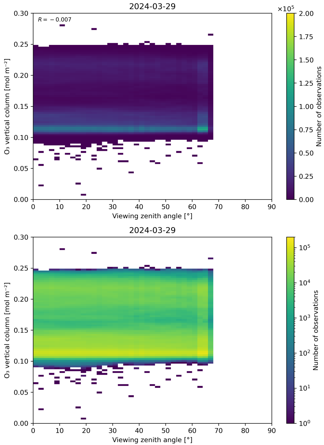
Figure 52: Scatter density plot of “Viewing zenith angle” against “O 3 vertical column” for 2024-03-28 to 2024-03-30.
