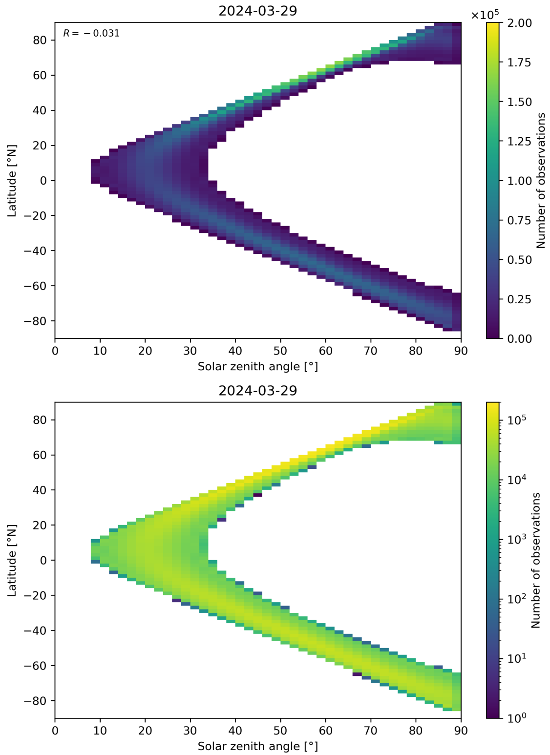
Figure 44: Scatter density plot of “Solar zenith angle” against “Latitude” for 2024-03-28 to 2024-03-30.
