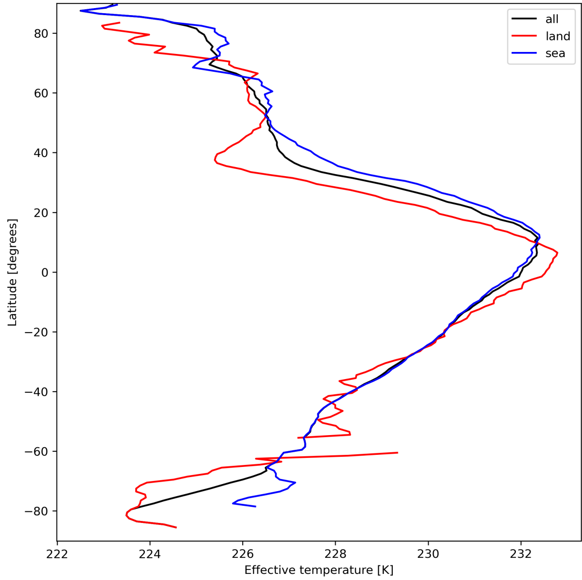
Figure 17: Zonal average of “Effective temperature” for 2024-03-28 to 2024-03-30.
