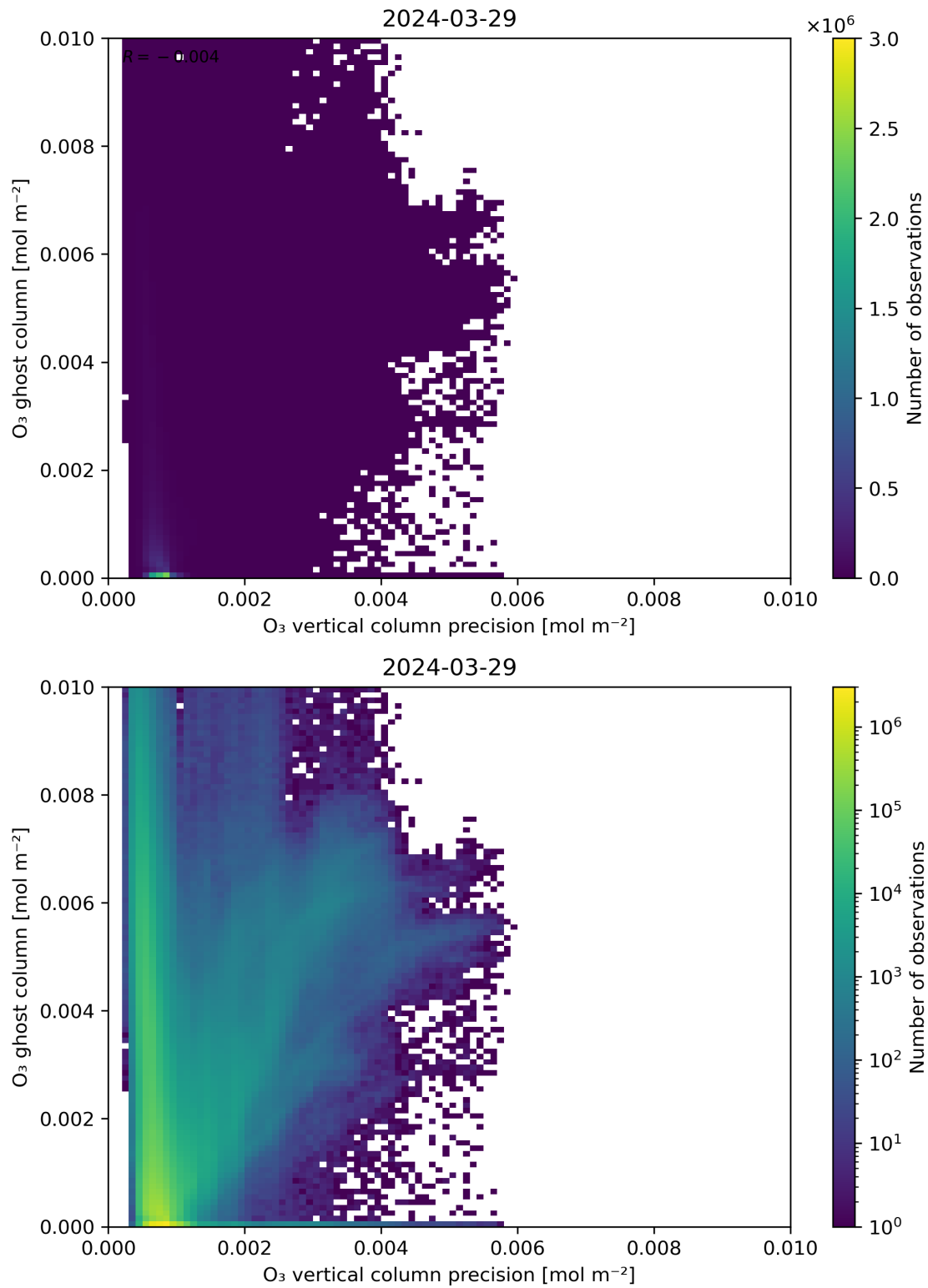
Figure 43: Scatter density plot of “ \text{O}_3 vertical column precision” against “ \text{O}_3 ghost column” for 2024-03-28 to 2024-03-30.
