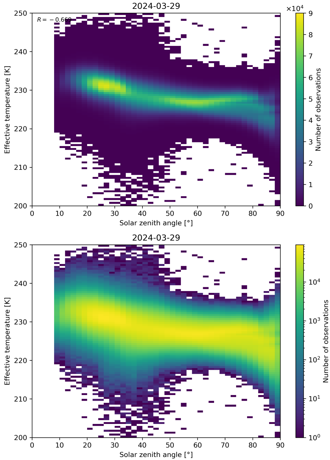
Figure 45: Scatter density plot of “Solar zenith angle” against “Effective temperature” for 2024-03-28 to 2024-03-30.
