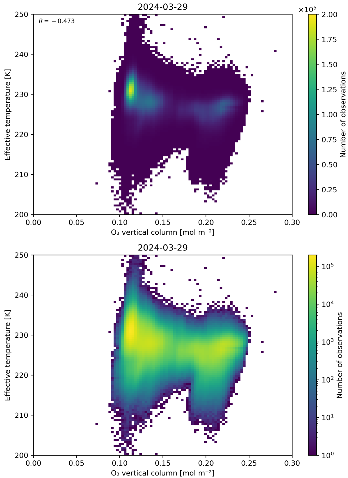
Figure 39: Scatter density plot of “O 3 vertical column” against “Effective temperature” for 2024-03-28 to 2024-03-30.
