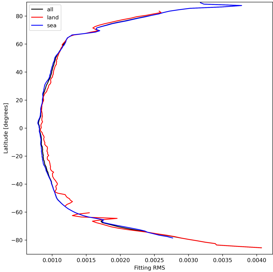
Figure 16: Zonal average of “Fitting RMS” for 2024-03-28 to 2024-03-30.
