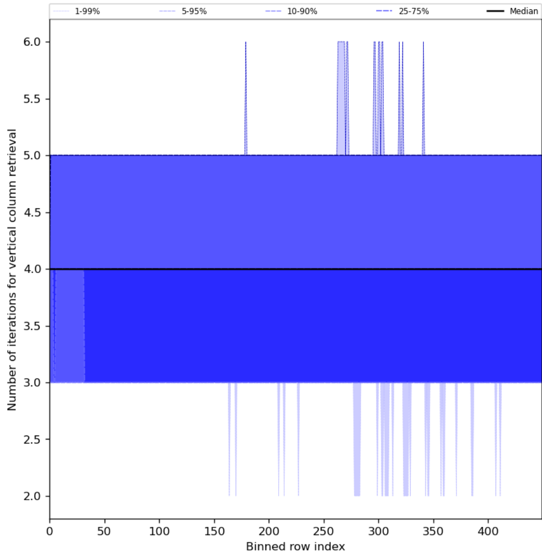
Figure 33: Along track statistics of “Number of iterations for vertical column retrieval” for 2024-03-28 to 2024-03-30
