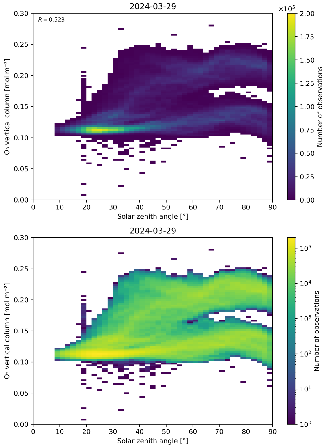
Figure 47: Scatter density plot of “Solar zenith angle” against “O 3 vertical column” for 2024-03-28 to 2024-03-30.
