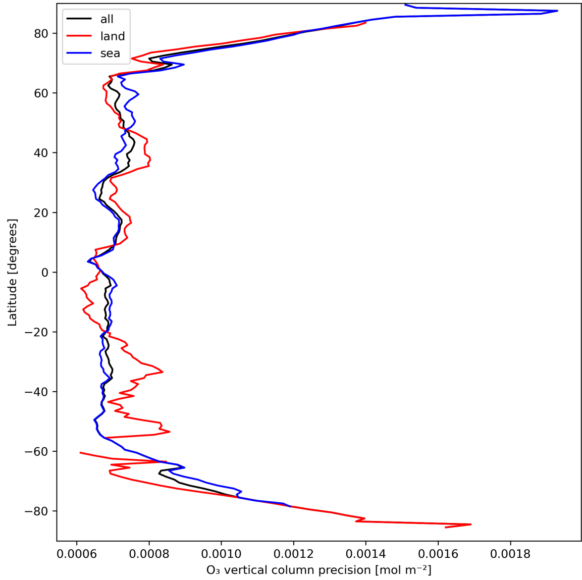
Figure 15: Zonal average of “O 3 vertical column precision” for 2024-03-30 to 2024-03-31.
