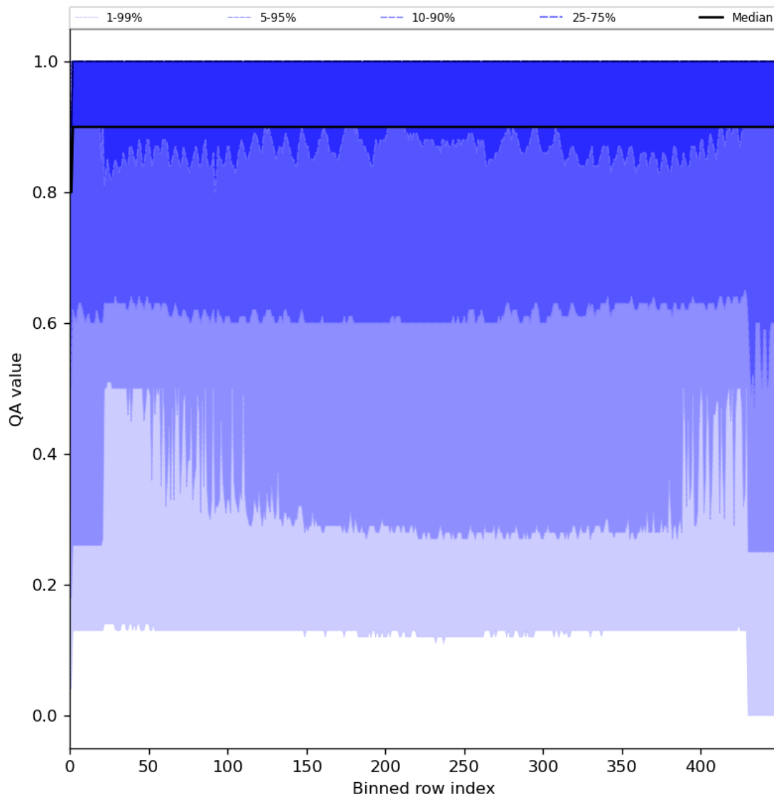
Figure 27: Along track statistics of “QA value” for 2024-03-30 to 2024-03-31
