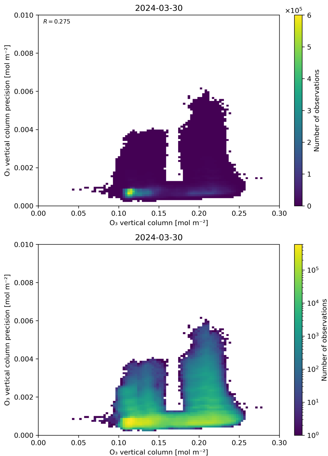
Figure 41: Scatter density plot of “O 3 vertical column” against “O 3 vertical column precision” for 2024-03-30 to 2024-03-31.
