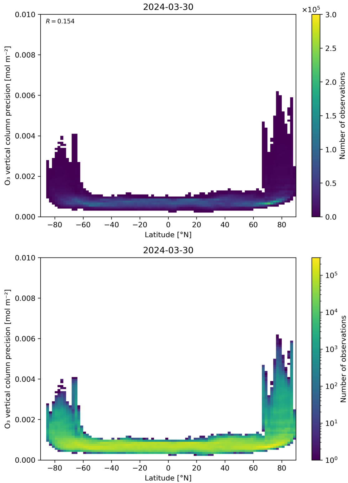
Figure 37: Scatter density plot of “Latitude” against “O 3 vertical column precision” for 2024-03-30 to 2024-03-31.
