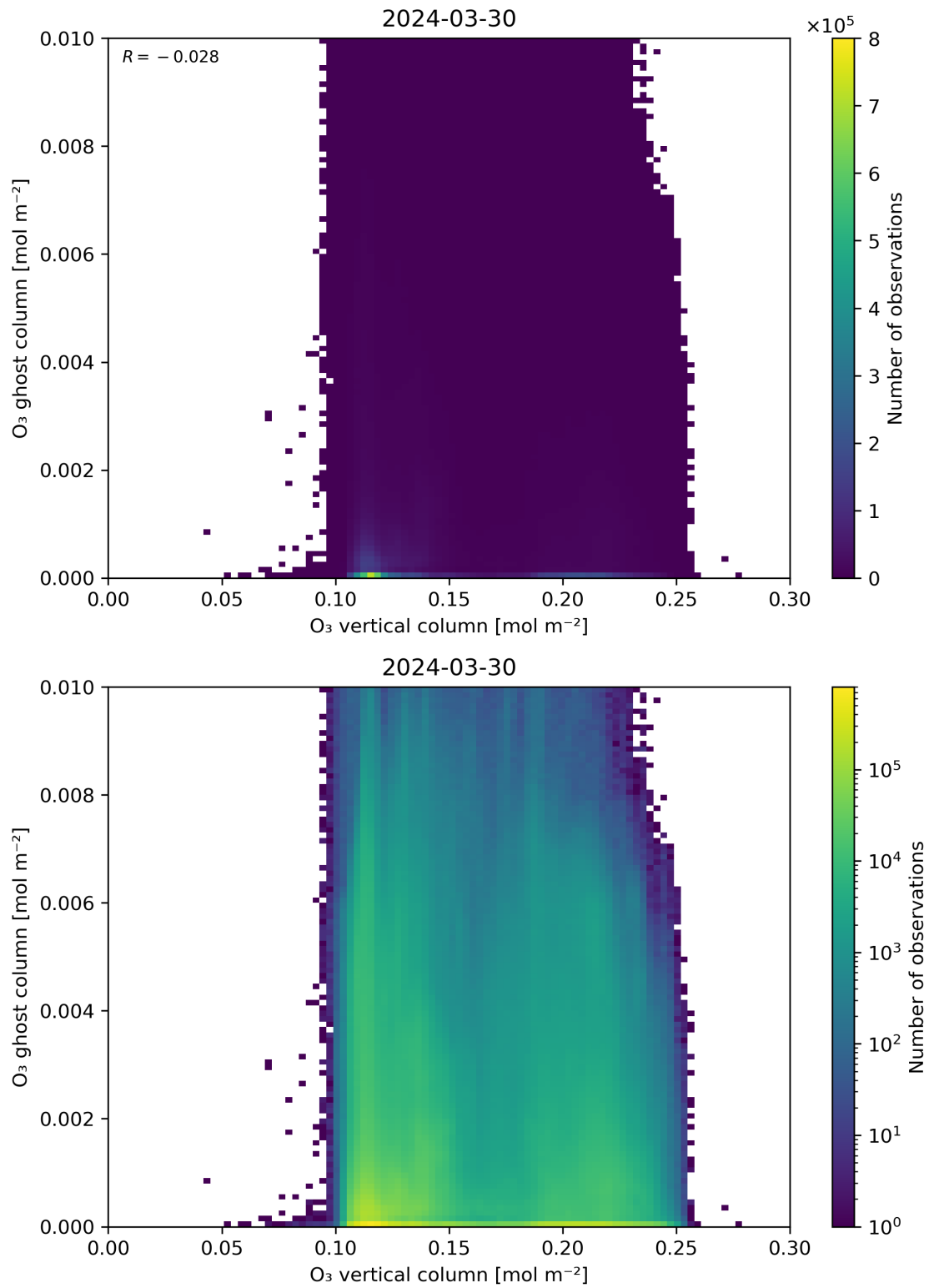
Figure 40: Scatter density plot of “O 3 vertical column” against “O 3 ghost column” for 2024-03-30 to 2024-03-31.
