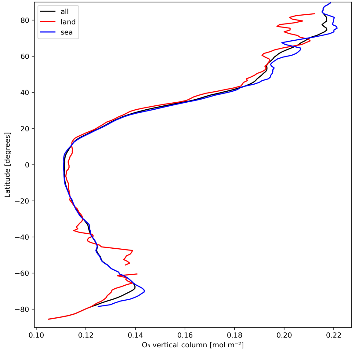
Figure 14: Zonal average of “O 3 vertical column” for 2024-03-30 to 2024-03-31.
