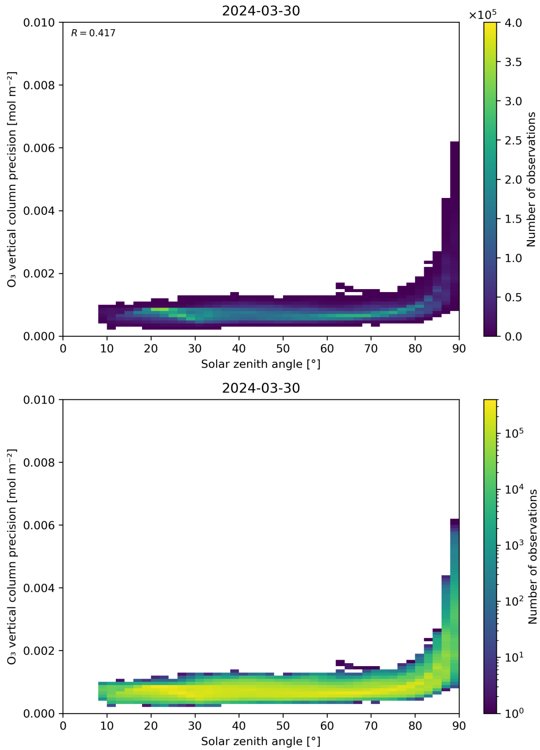
Figure 48: Scatter density plot of “Solar zenith angle” against “O 3 vertical column precision” for 2024-03-30 to 2024-03-31.
