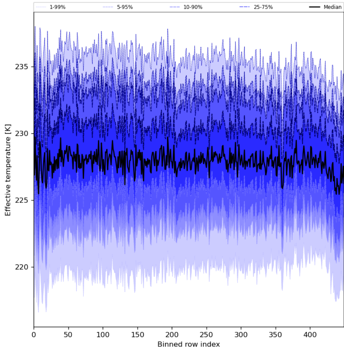
Figure 31: Along track statistics of “Effective temperature” for 2024-03-30 to 2024-03-31
