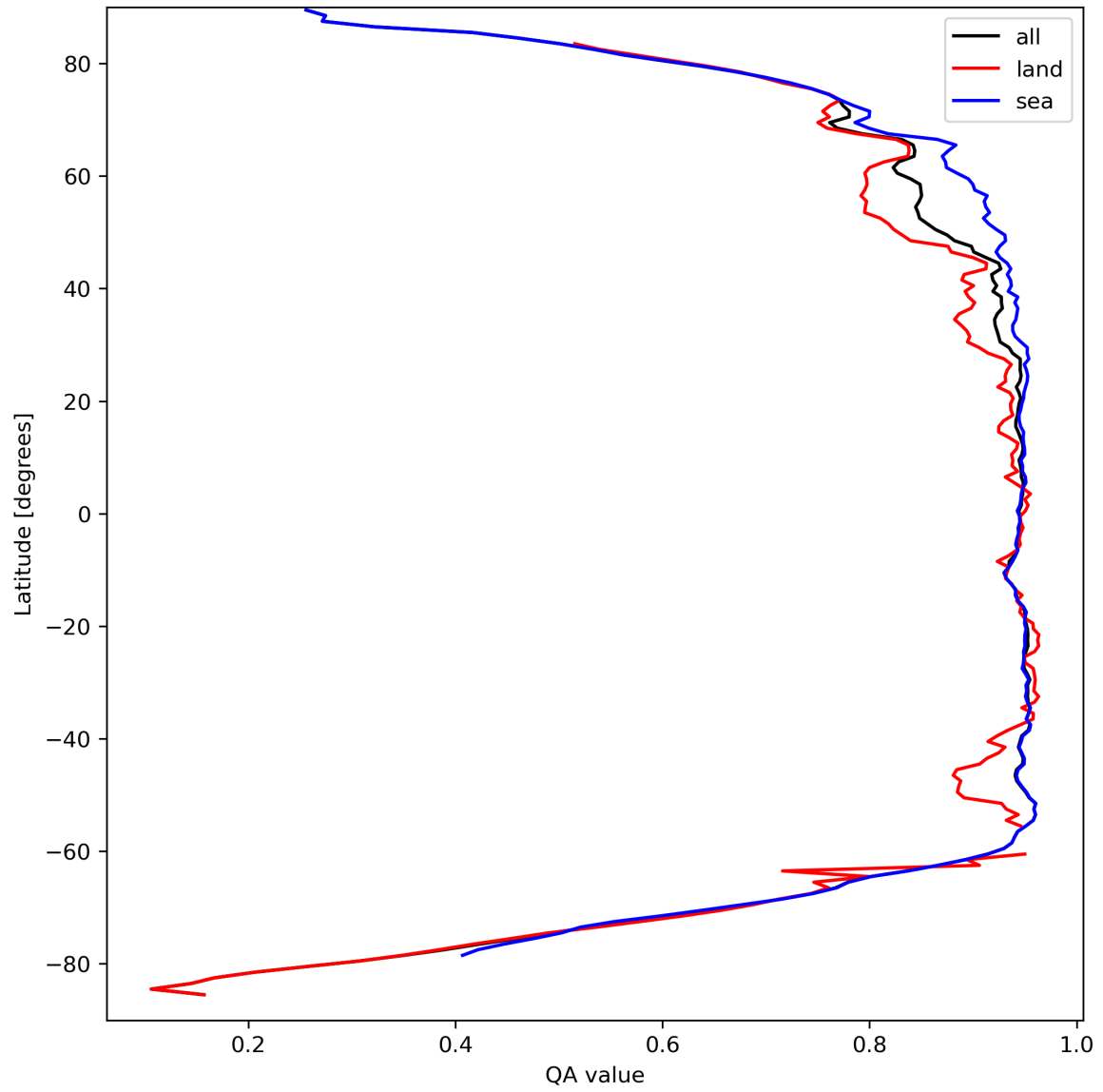
Figure 13: Zonal average of “QA value” for 2024-03-30 to 2024-03-31.
