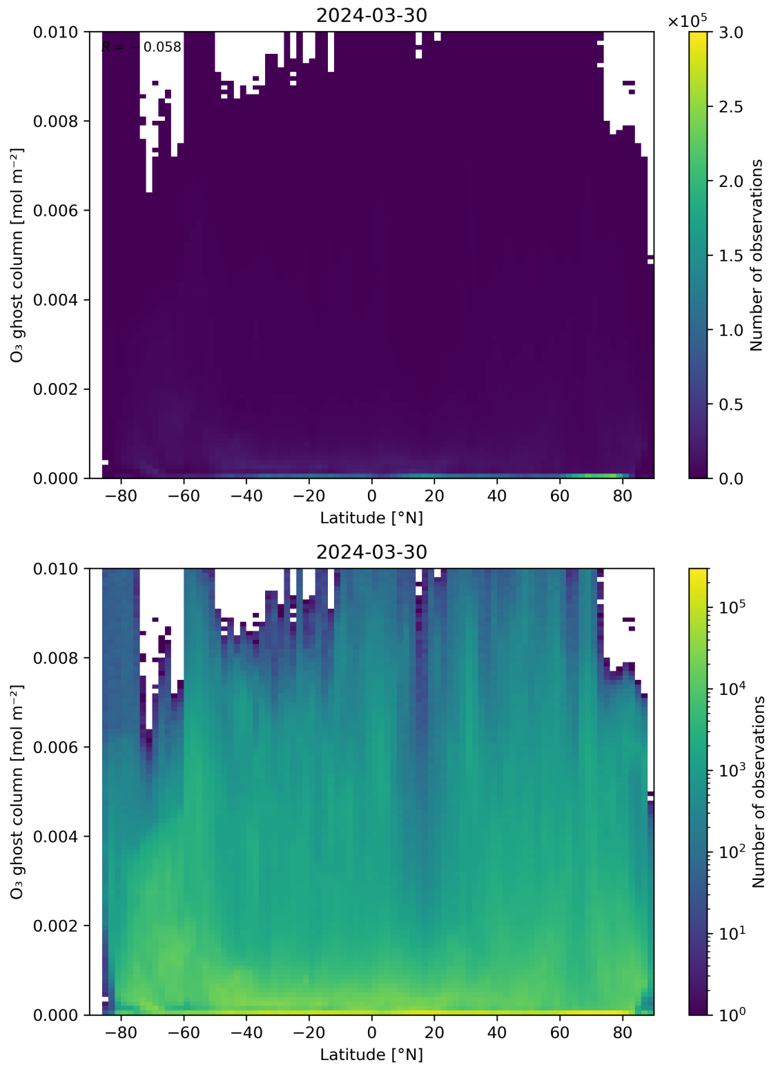
Figure 35: Scatter density plot of “Latitude” against “O 3 ghost column” for 2024-03-30 to 2024-03-31.
