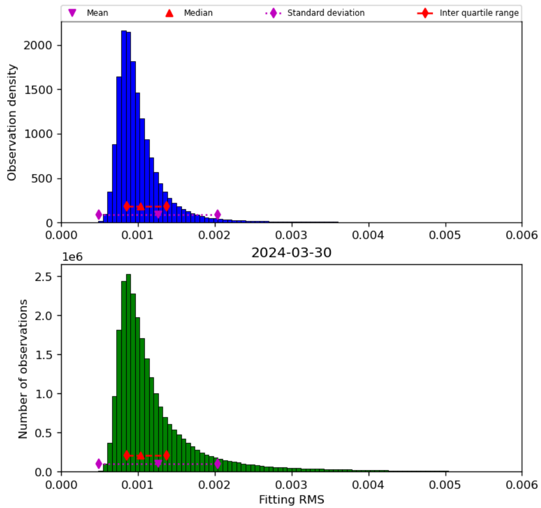
Figure 23: Histogram of “Fitting RMS” for 2024-03-30 to 2024-03-31
