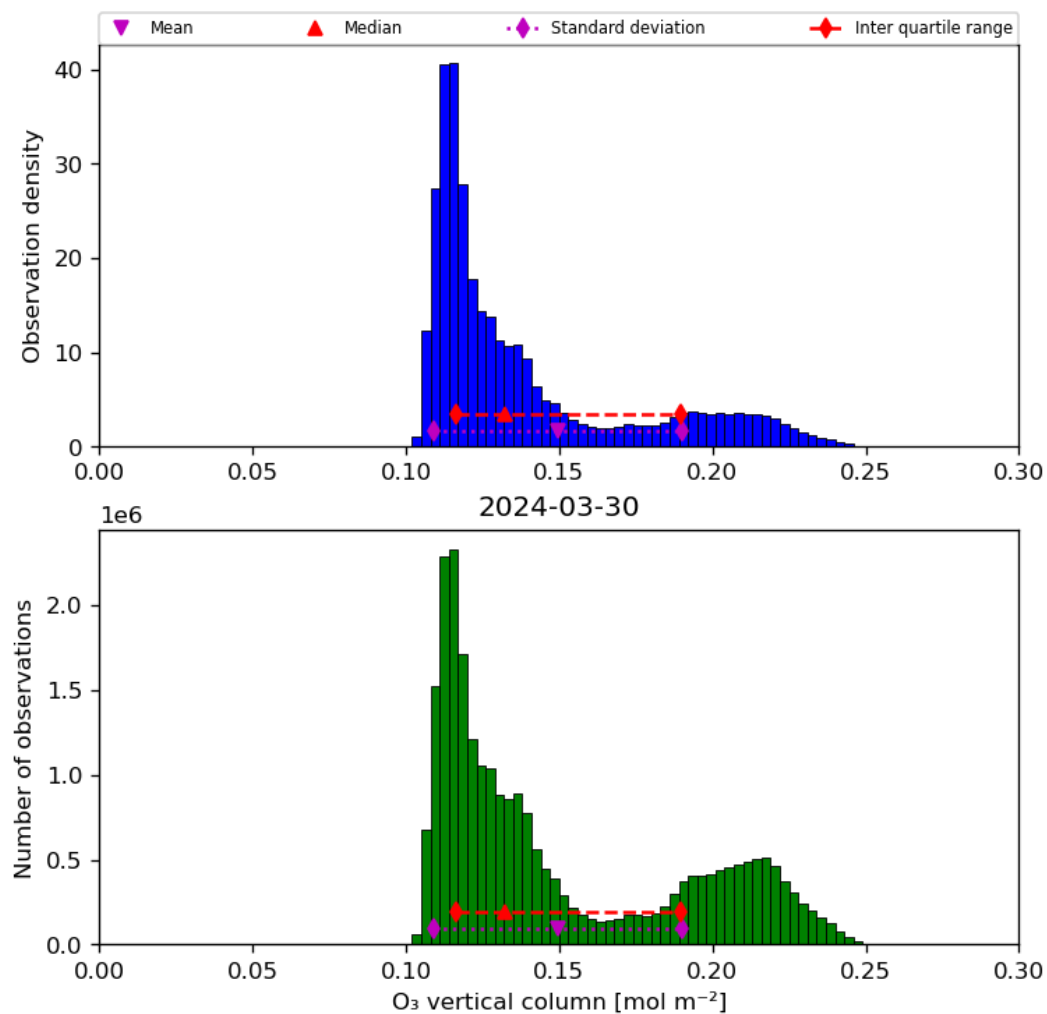
Figure 21: Histogram of “O 3 vertical column” for 2024-03-30 to 2024-03-31
