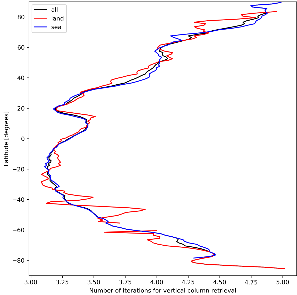
Figure 19: Zonal average of “Number of iterations for vertical column retrieval” for 2024-03-30 to 2024-03-31.
