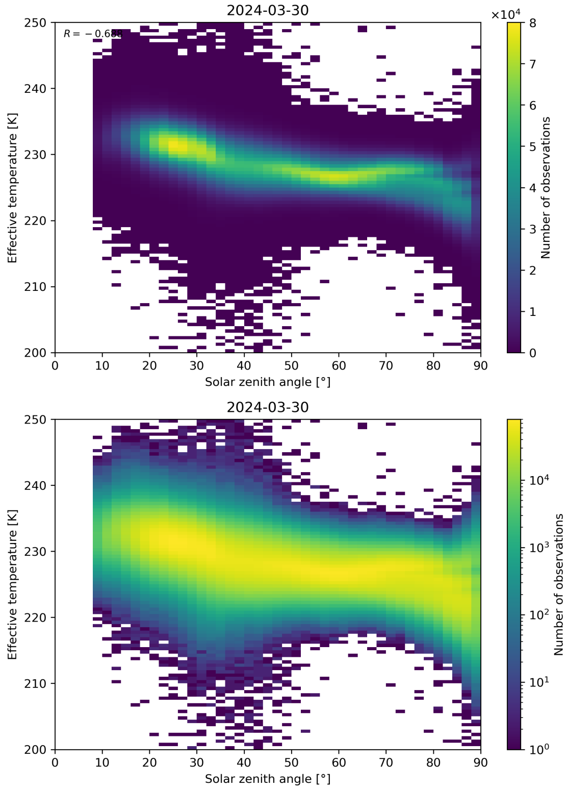
Figure 45: Scatter density plot of “Solar zenith angle” against “Effective temperature” for 2024-03-30 to 2024-03-31.
