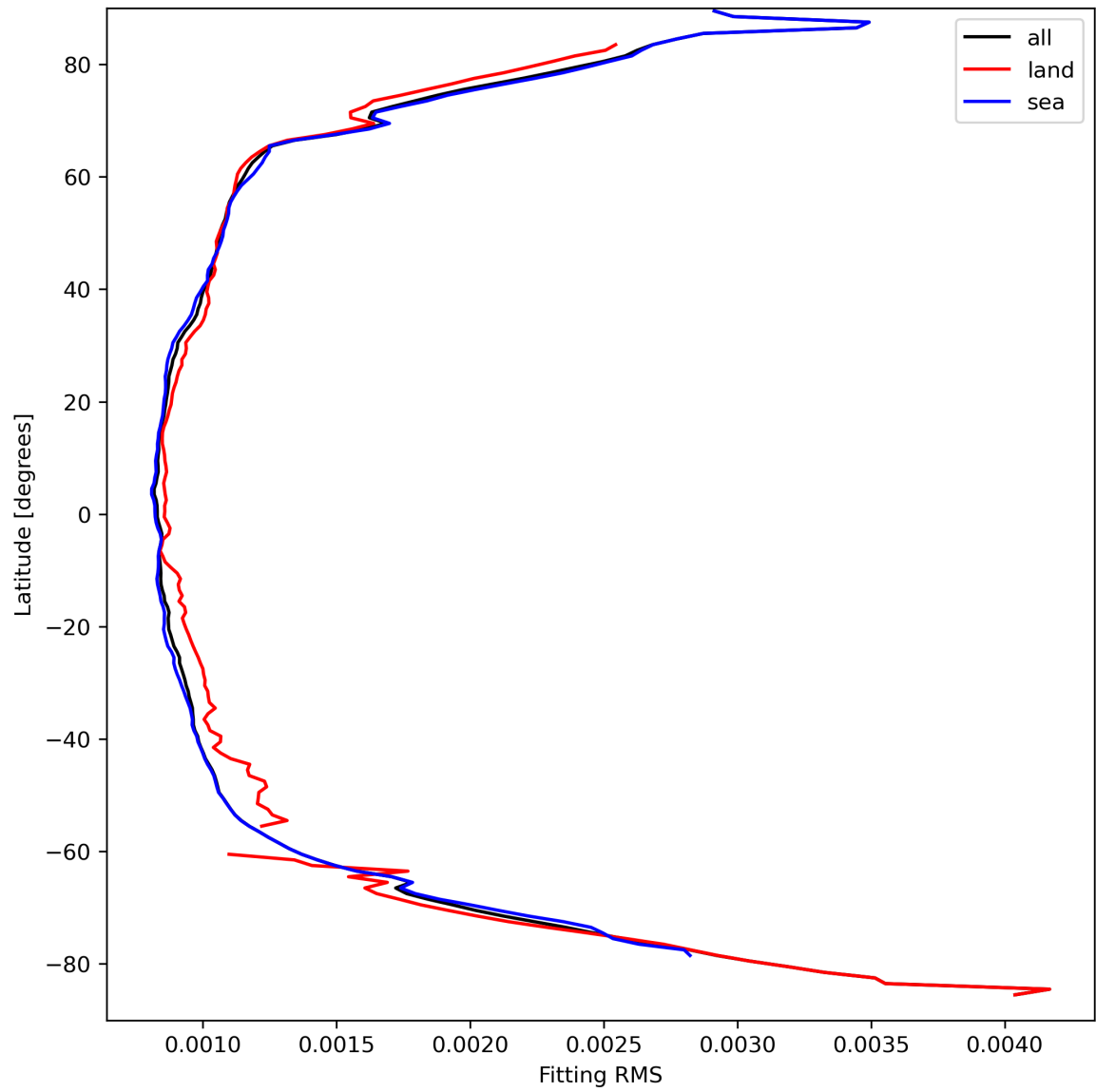
Figure 16: Zonal average of “Fitting RMS” for 2024-03-30 to 2024-03-31.
