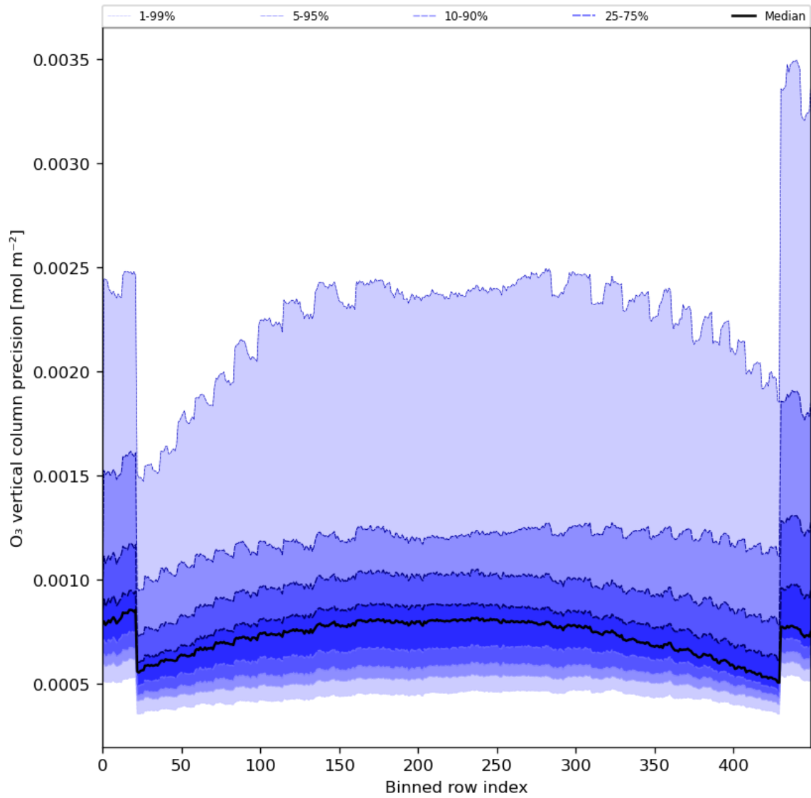
Figure 29: Along track statistics of “O 3 vertical column precision” for 2024-03-30 to 2024-03-31
