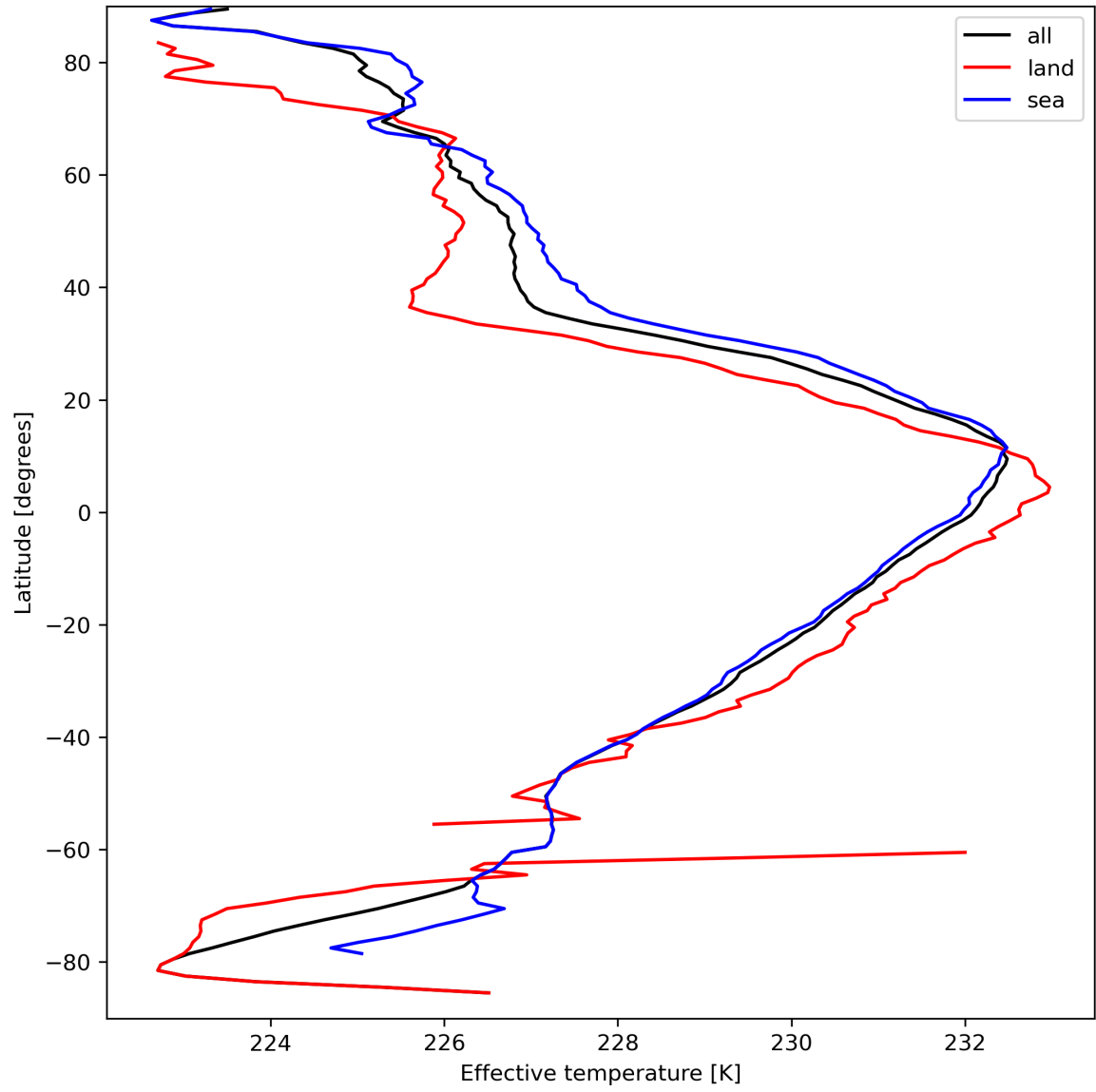
Figure 17: Zonal average of “Effective temperature” for 2024-03-30 to 2024-03-31.
