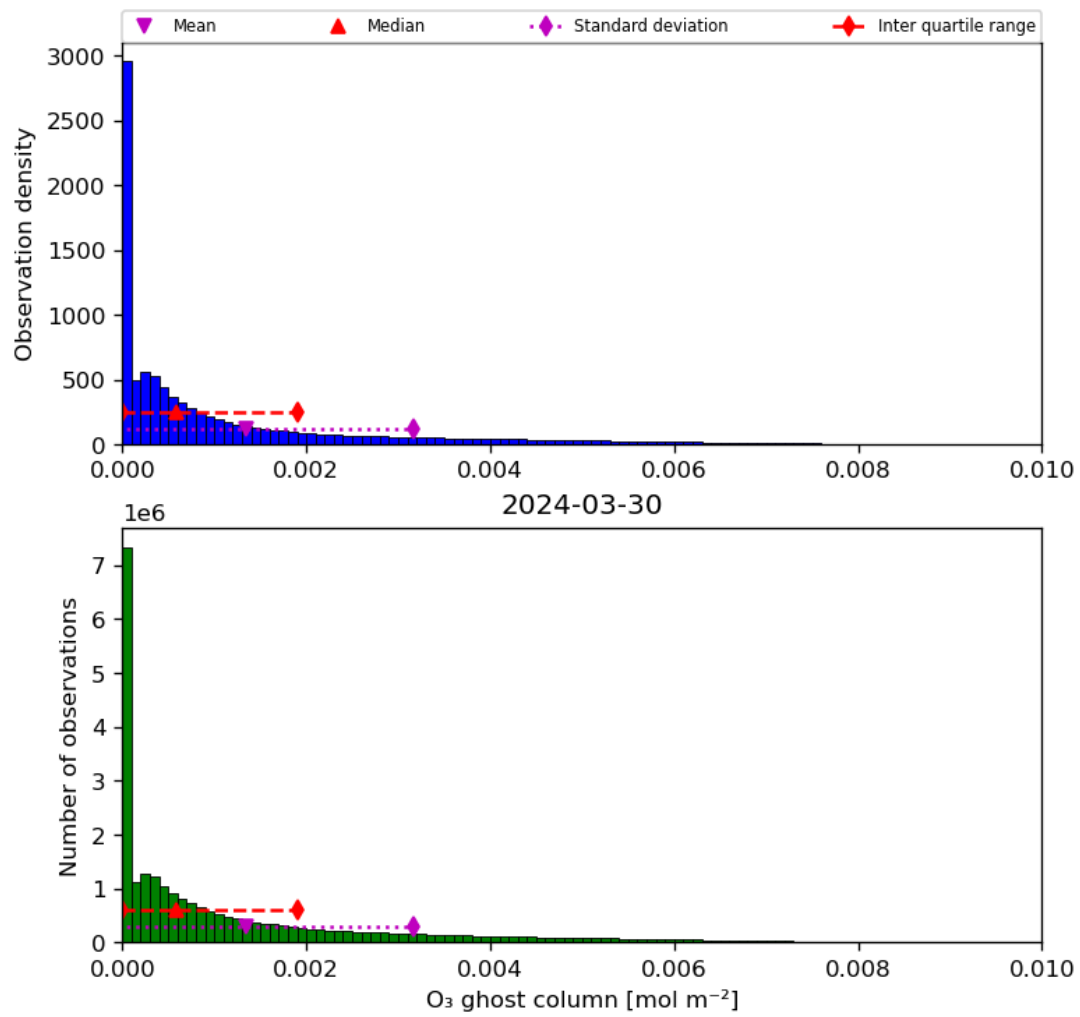
Figure 25: Histogram of “O 3 ghost column” for 2024-03-30 to 2024-03-31
