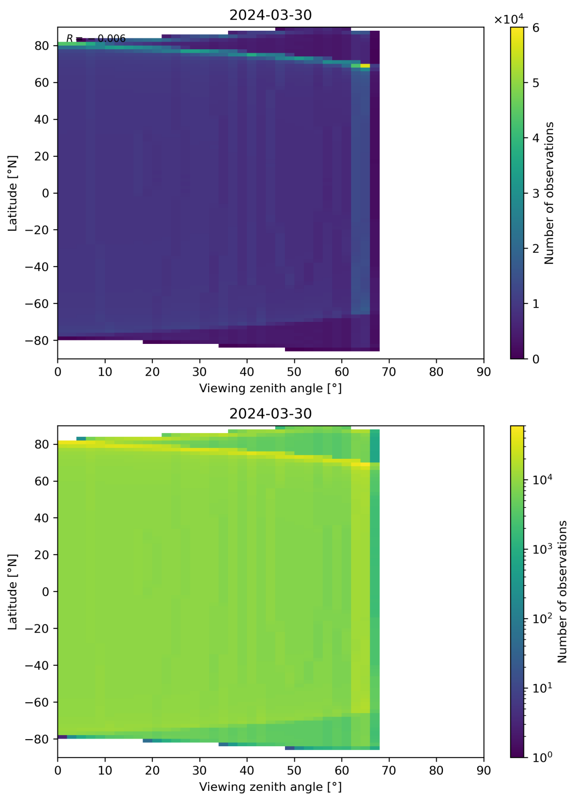
Figure 49: Scatter density plot of “Viewing zenith angle” against “Latitude” for 2024-03-30 to 2024-03-31.
