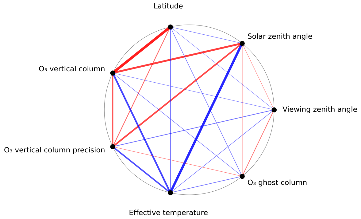
Figure 1: Map of correlation graph for 2024-03-30 to 2024-03-31.
