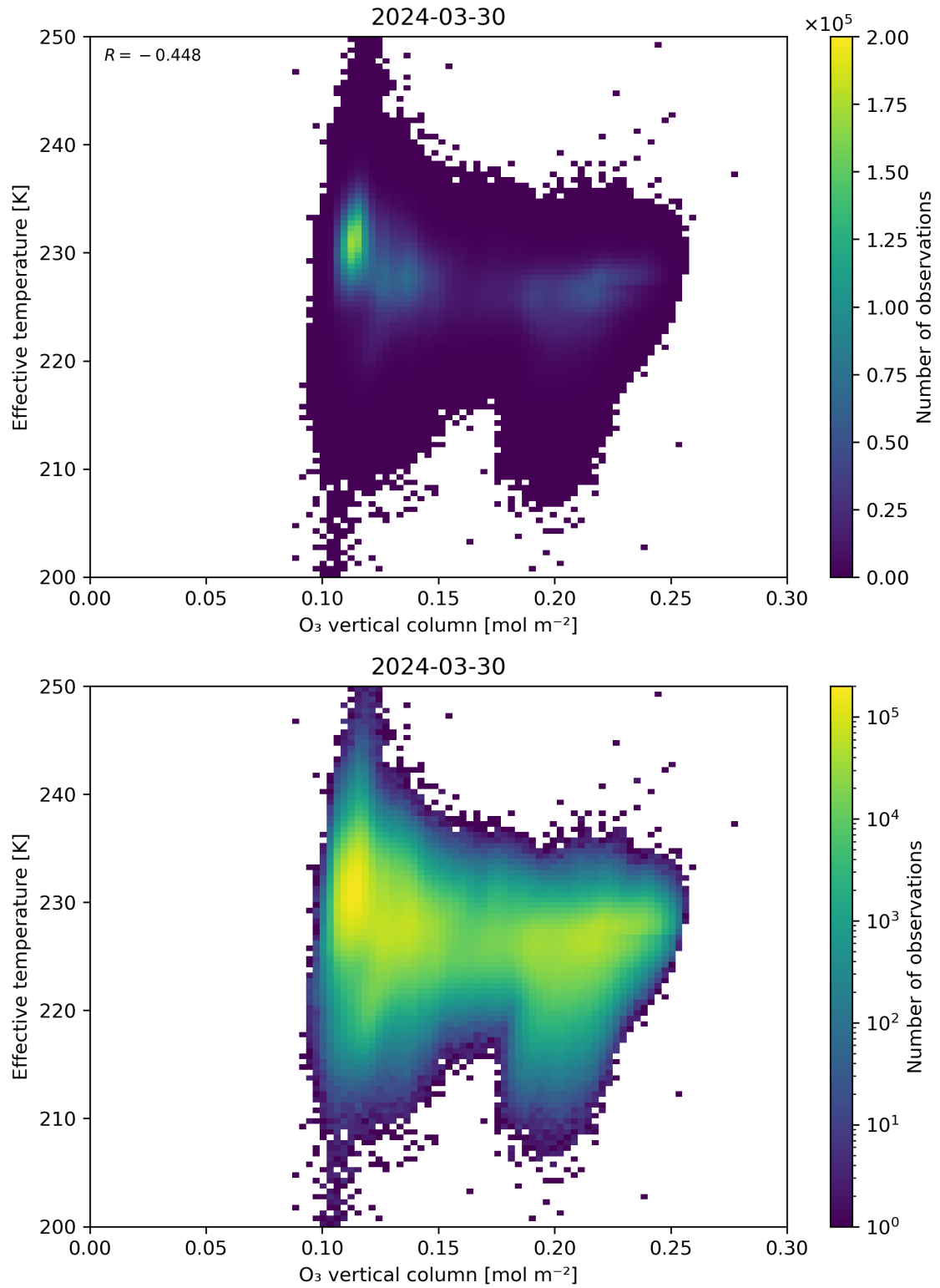
Figure 39: Scatter density plot of “O 3 vertical column” against “Effective temperature” for 2024-03-30 to 2024-03-31.
