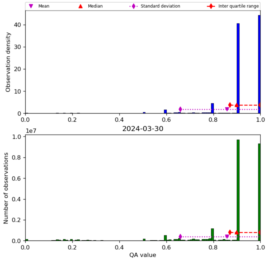
Figure 20: Histogram of “QA value” for 2024-03-30 to 2024-03-31
