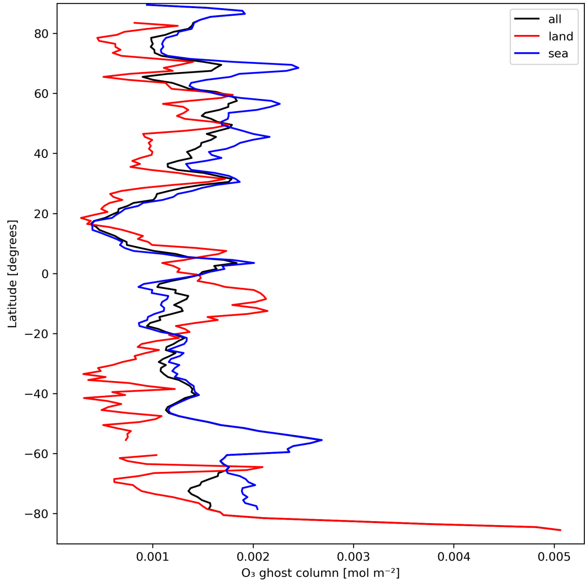
Figure 18: Zonal average of "O 3 ghost column" for 2024-03-30 to 2024-03-31.
