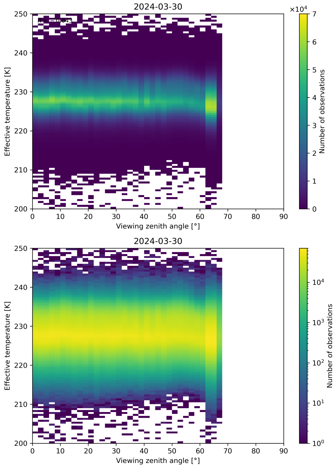
Figure 50: Scatter density plot of “Viewing zenith angle” against “Effective temperature” for 2024-03-30 to 2024-03-31.
