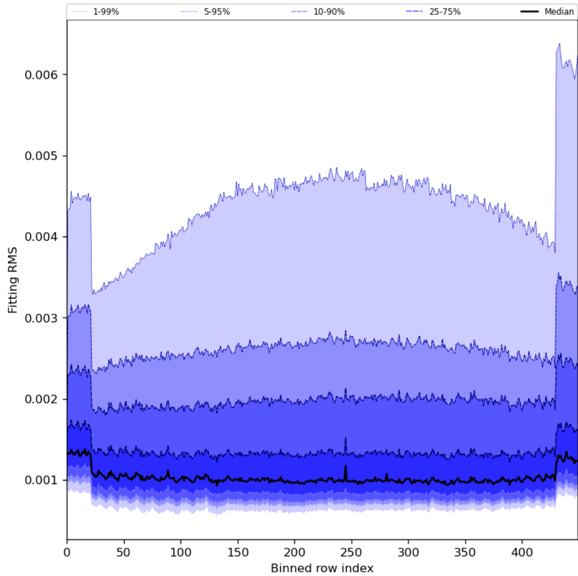
Figure 30: Along track statistics of “Fitting RMS” for 2024-03-30 to 2024-03-31
