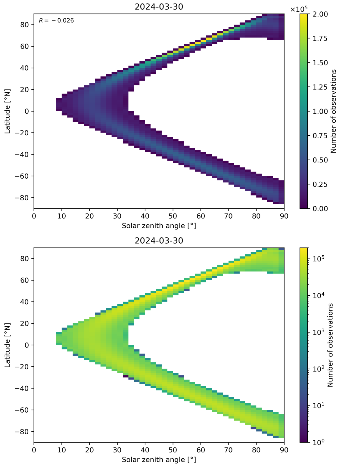
Figure 44: Scatter density plot of “Solar zenith angle” against “Latitude” for 2024-03-30 to 2024-03-31.
