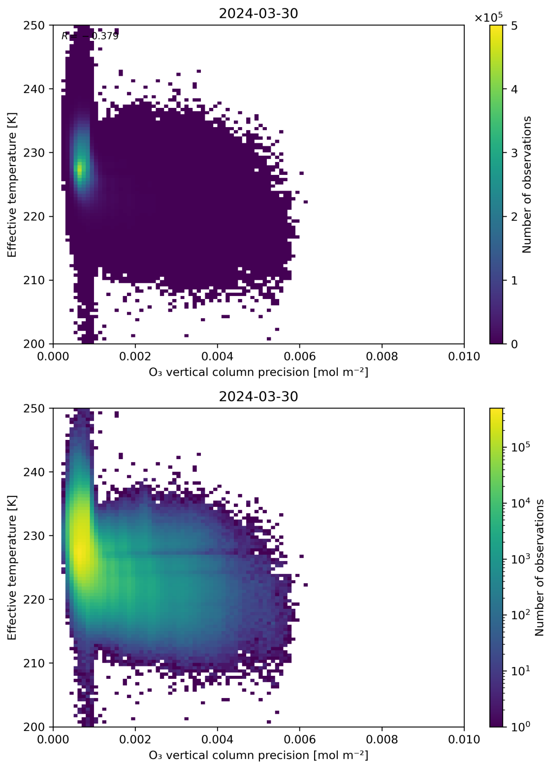
Figure 42: Scatter density plot of “O 3 vertical column precision” against “Effective temperature” for 2024-03-30 to 2024-03-31.
