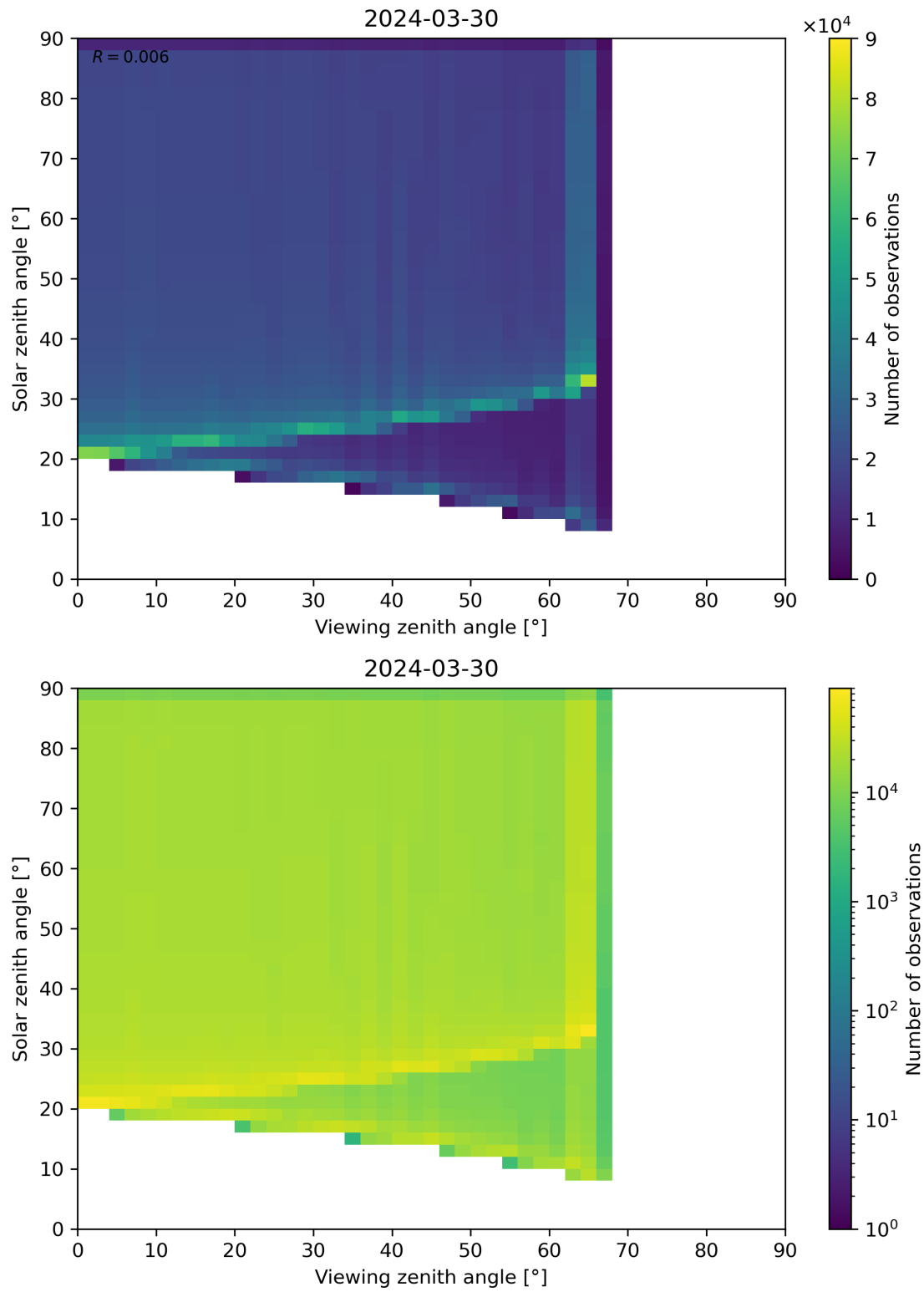
Figure 54: Scatter density plot of “Viewing zenith angle” against “Solar zenith angle” for 2024-03-30 to 2024-03-31.
