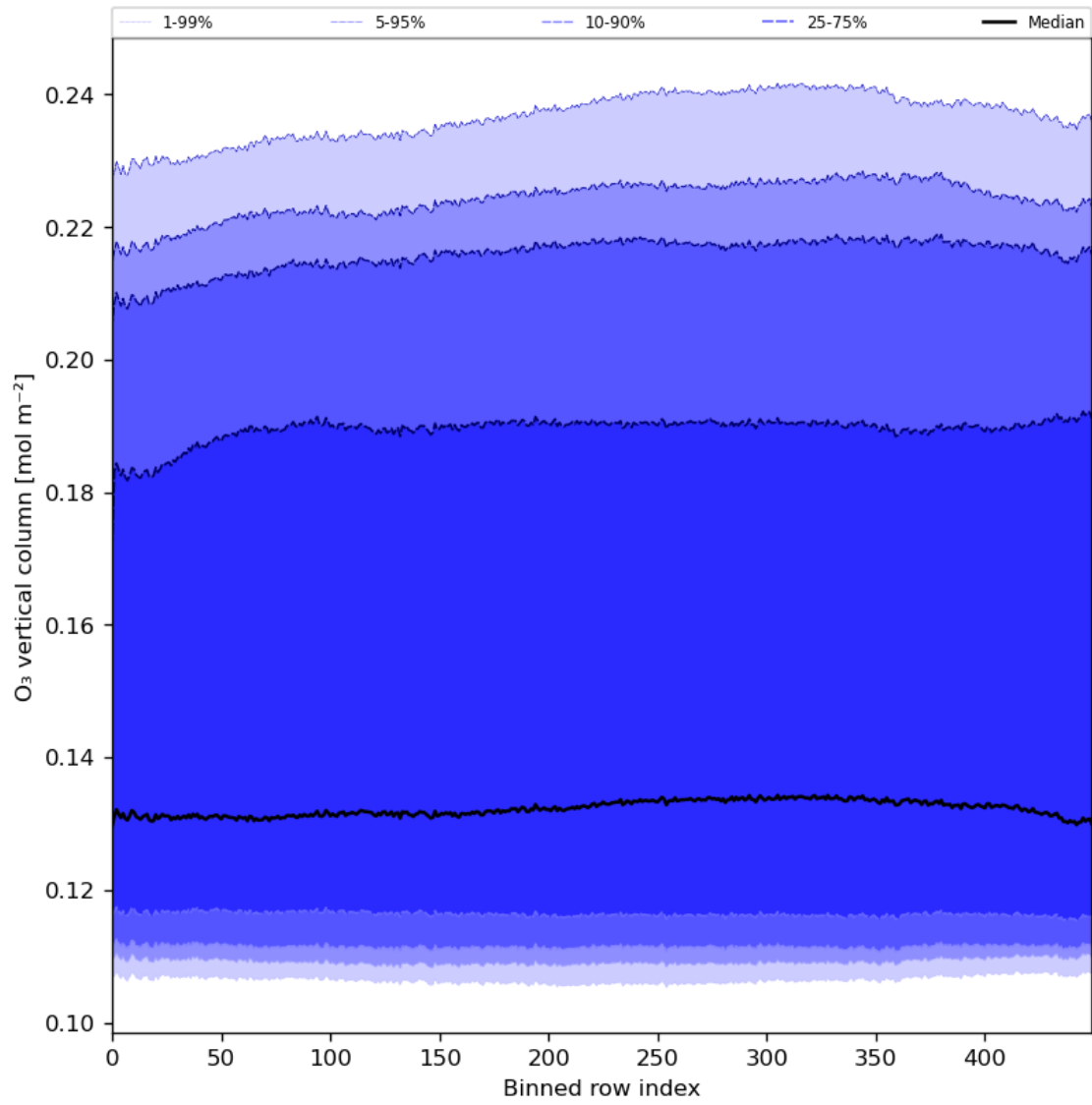
Figure 28: Along track statistics of “O 3 vertical column” for 2024-03-30 to 2024-03-31
