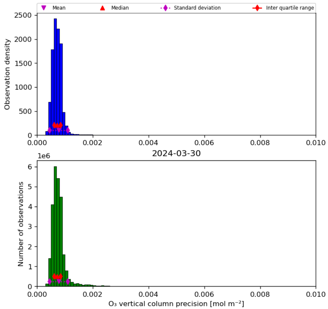
Figure 22: Histogram of “O 3 vertical column precision” for 2024-03-30 to 2024-03-31
