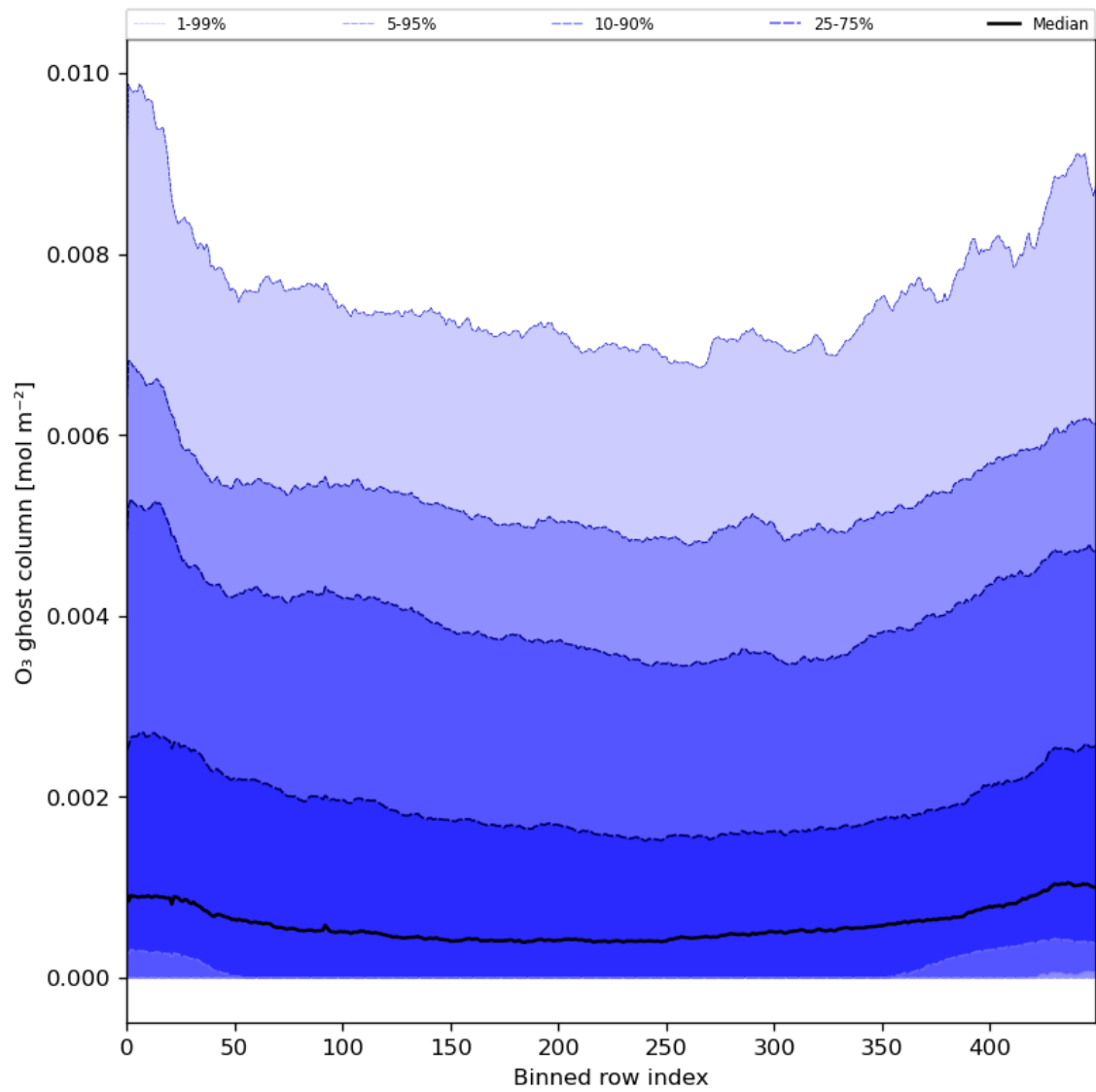
Figure 32: Along track statistics of “O 3 ghost column” for 2024-03-30 to 2024-03-31
