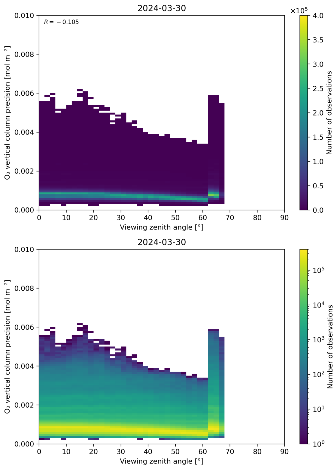
Figure 53: Scatter density plot of “Viewing zenith angle” against “O 3 vertical column precision” for 2024-03-30 to 2024-03-31.
