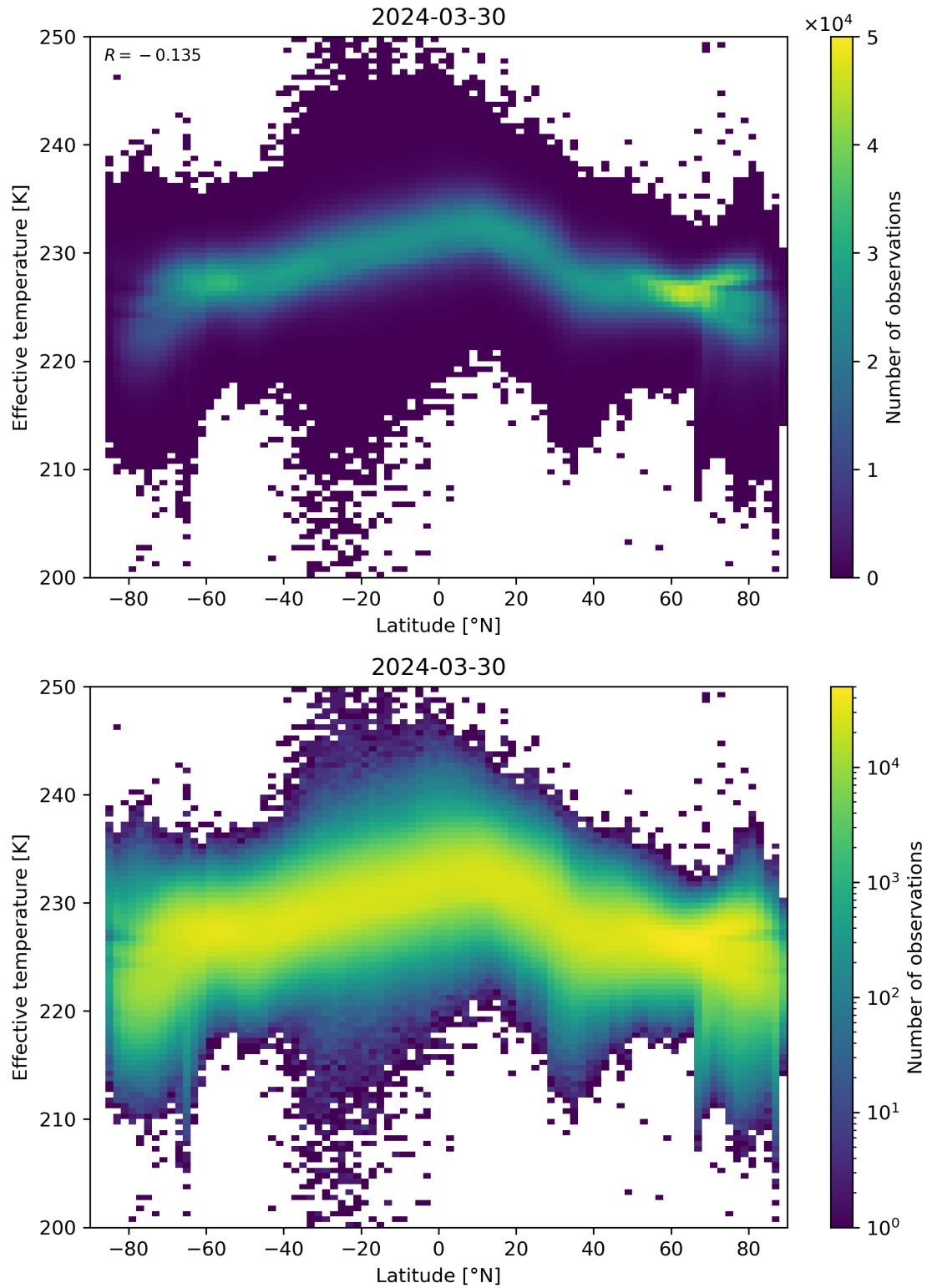
Figure 34: Scatter density plot of “Latitude” against “Effective temperature” for 2024-03-30 to 2024-03-31.
