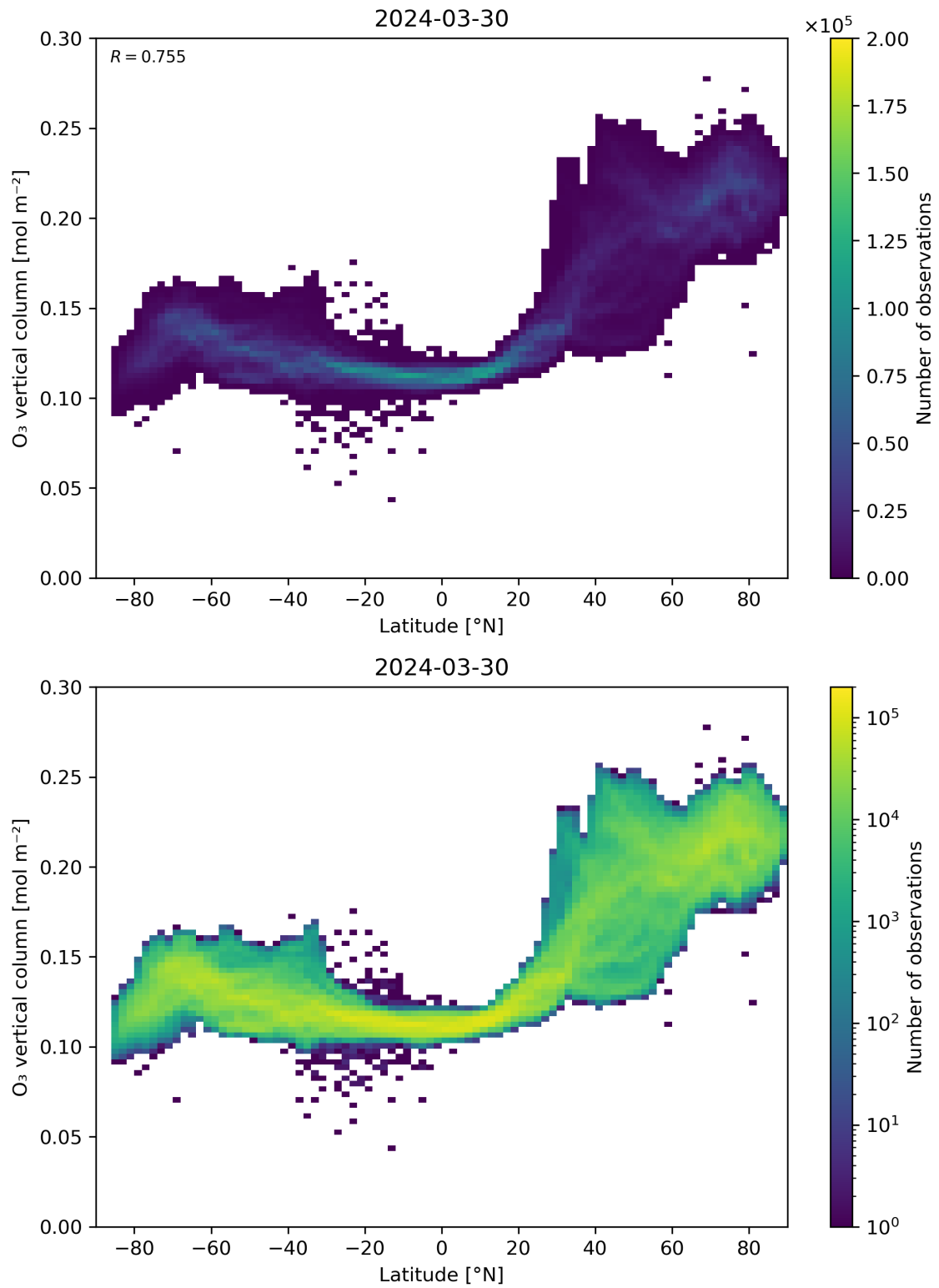
Figure 36: Scatter density plot of “Latitude” against “O 3 vertical column” for 2024-03-30 to 2024-03-31.
