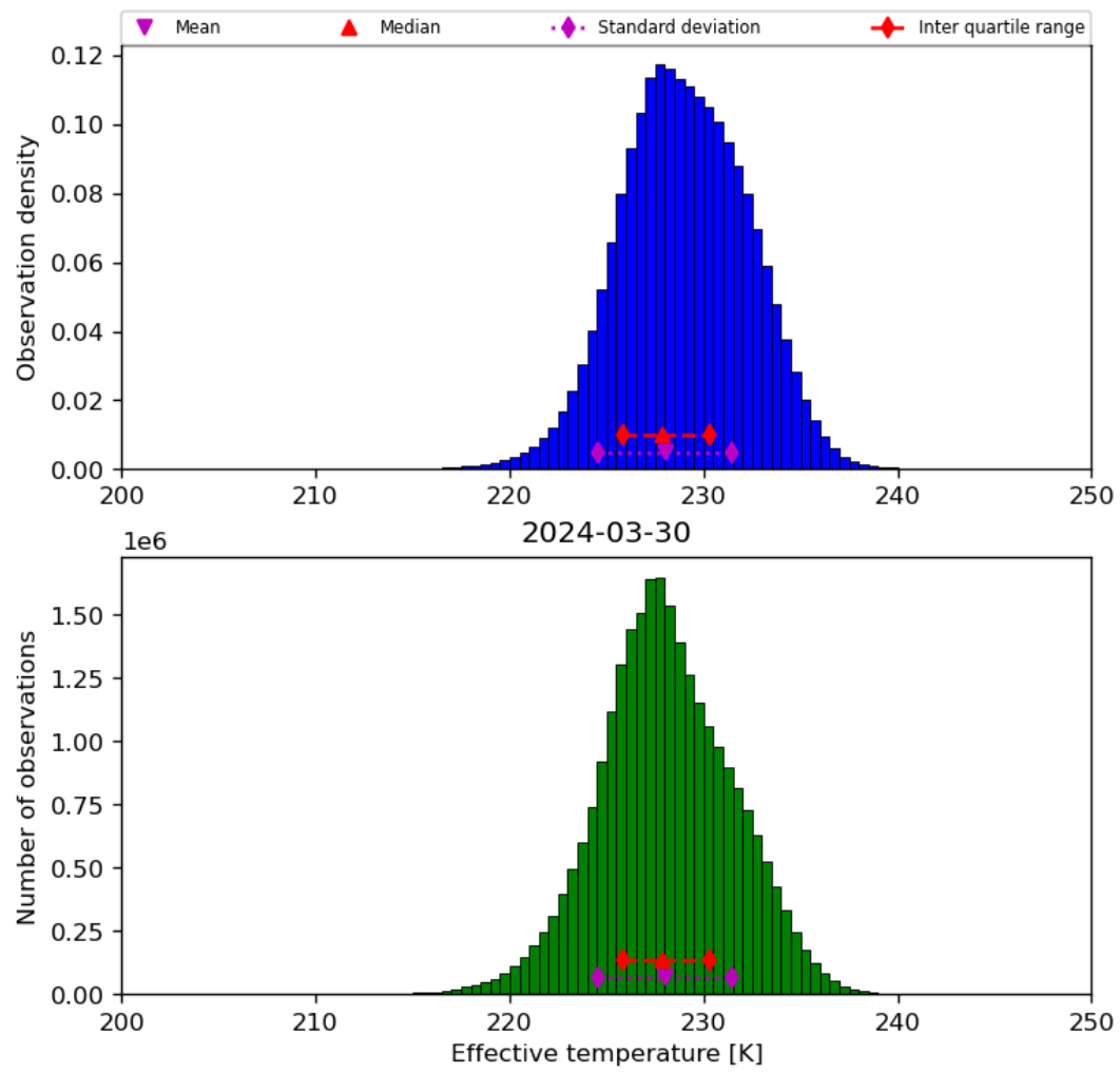
Figure 24: Histogram of “Effective temperature” for 2024-03-30 to 2024-03-31
