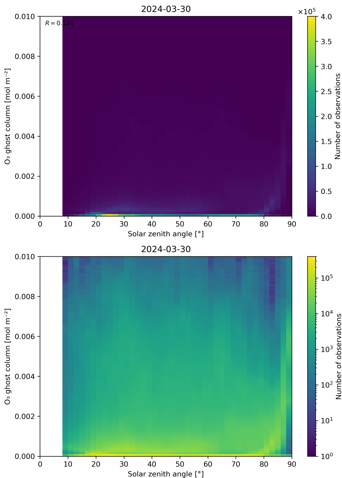
Figure 46: Scatter density plot of “Solar zenith angle” against “O 3 ghost column” for 2024-03-30 to 2024-03-31.
