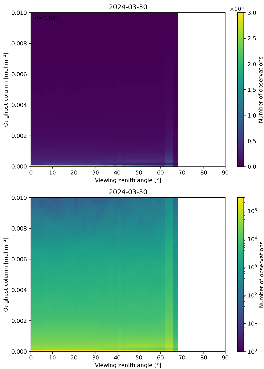
Figure 51: Scatter density plot of “Viewing zenith angle” against “O 3 ghost column” for 2024-03-30 to 2024-03-31.
