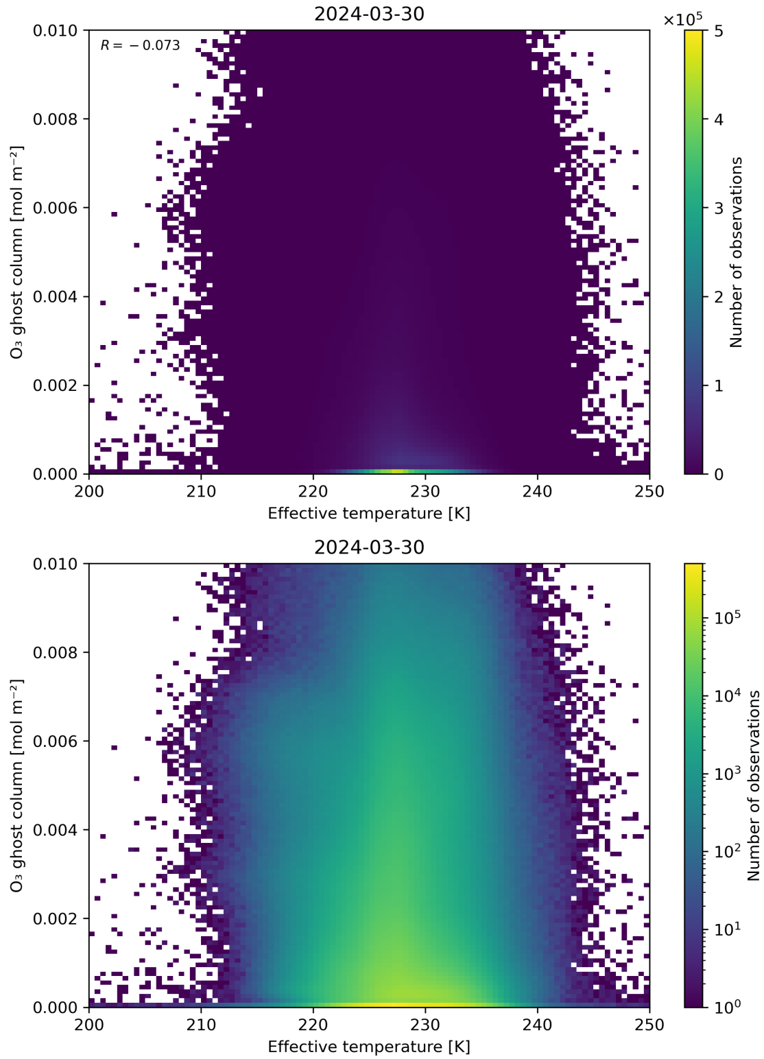
Figure 38: Scatter density plot of “Effective temperature” against “O 3 ghost column” for 2024-03-30 to 2024-03-31.
