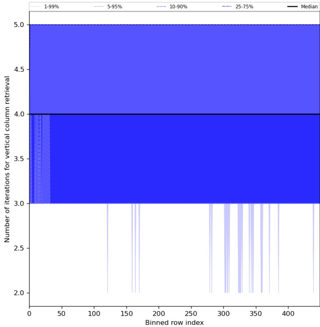
Figure 33: Along track statistics of “Number of iterations for vertical column retrieval” for 2024-03-30 to 2024-03-31
