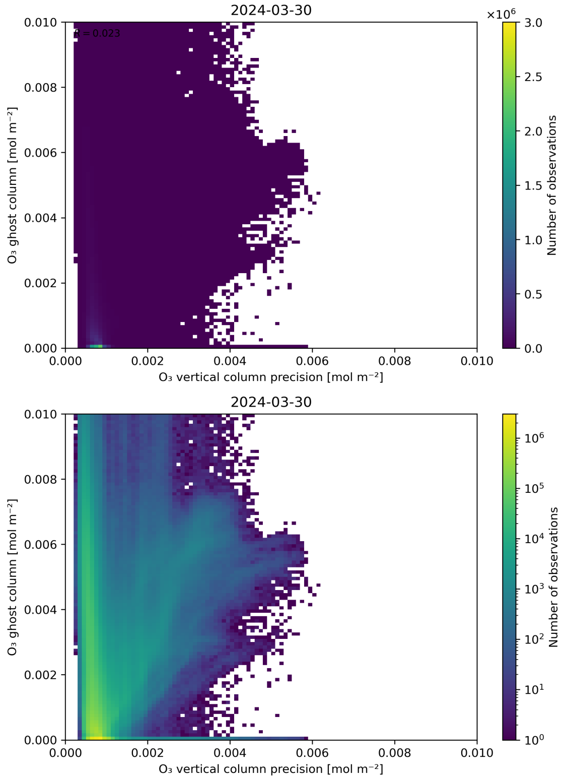
Figure 43: Scatter density plot of “O 3 vertical column precision” against “O 3 ghost column” for 2024-03-30 to 2024-03-31.
