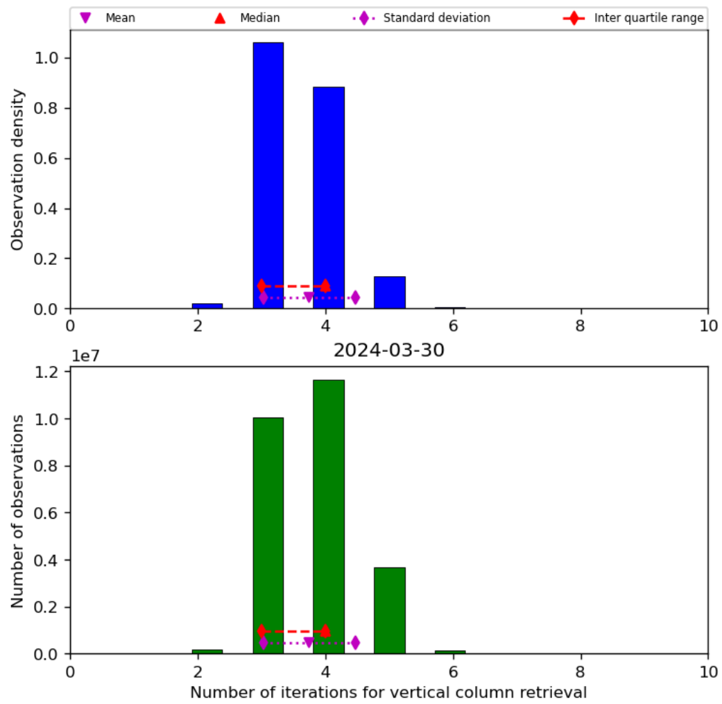
Figure 26: Histogram of “Number of iterations for vertical column retrieval” for 2024-03-30 to 2024-03-31
