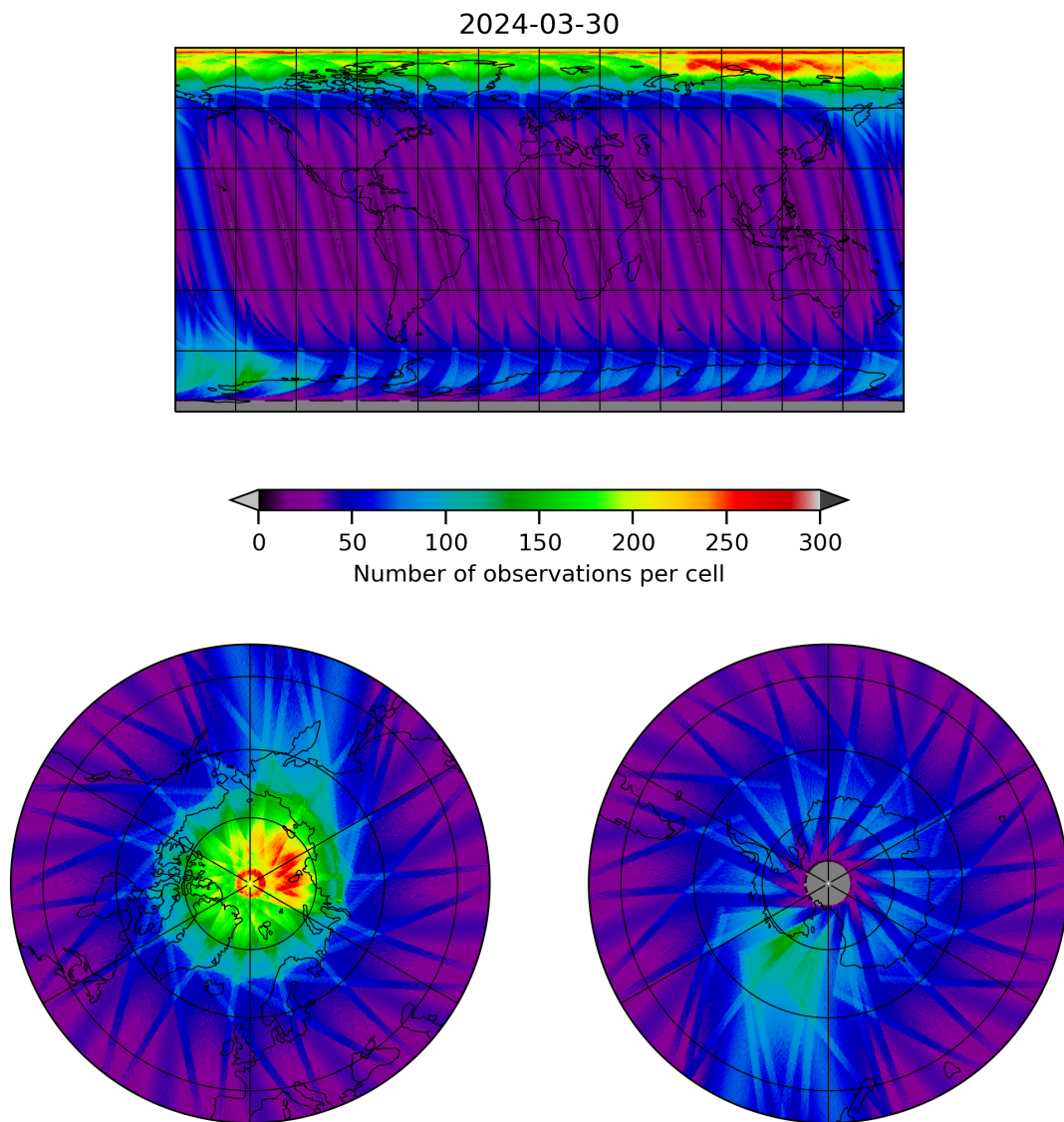
Figure 12: Map of the number of observations for 2024-03-30 to 2024-03-31
