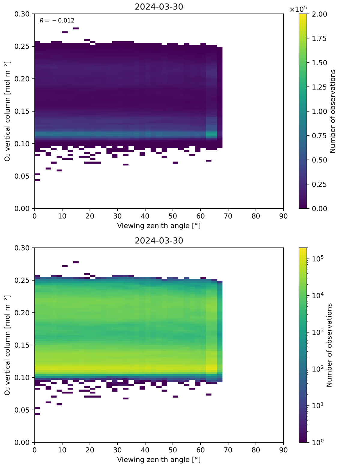
Figure 52: Scatter density plot of “Viewing zenith angle” against “O 3 vertical column” for 2024-03-30 to 2024-03-31.
