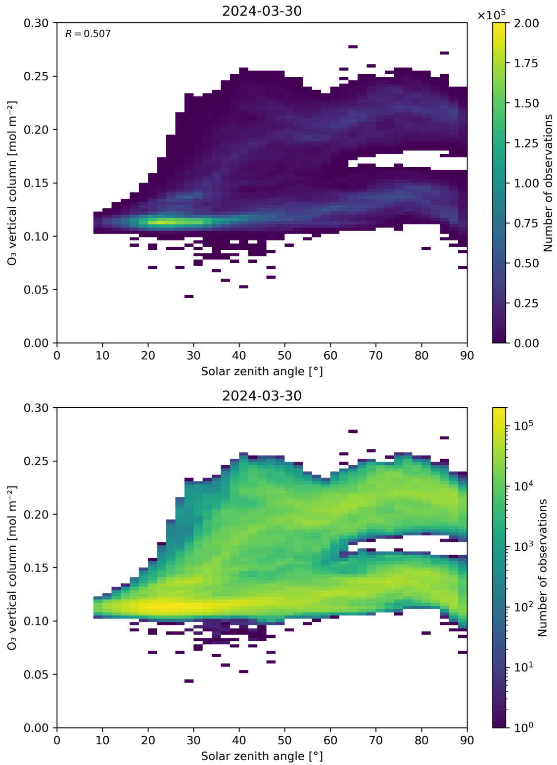
Figure 47: Scatter density plot of “Solar zenith angle” against “O 3 vertical column” for 2024-03-30 to 2024-03-31.
