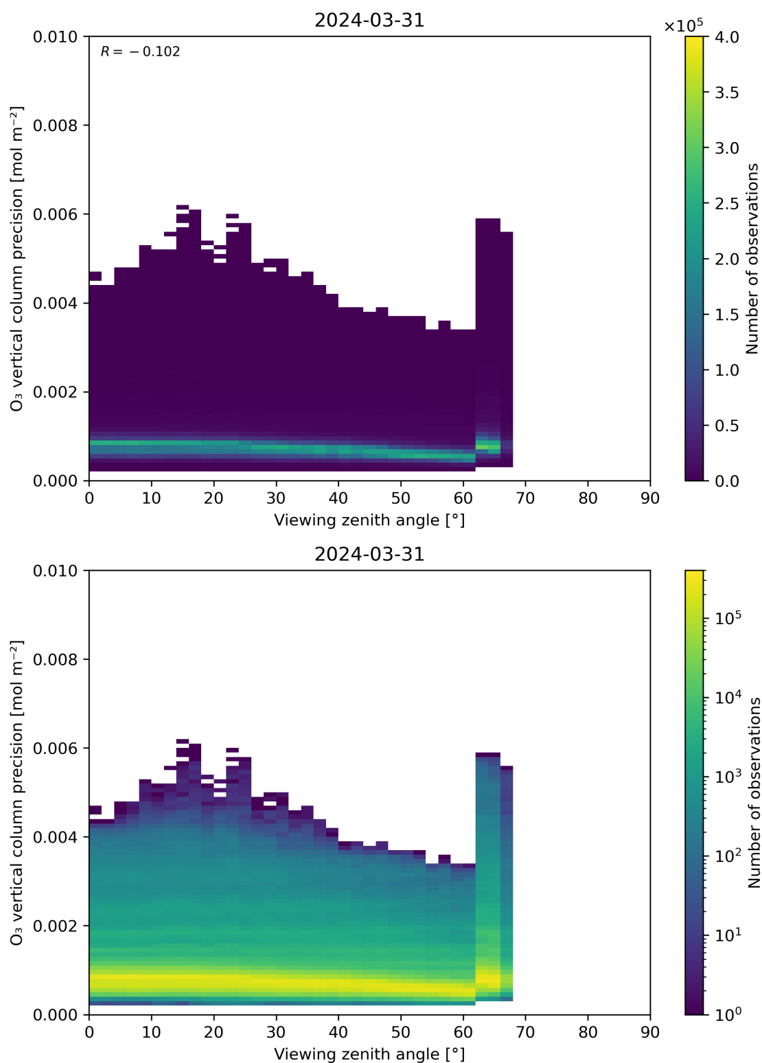
Figure 53: Scatter density plot of “Viewing zenith angle” against “O 3 vertical column precision” for 2024-03-31 to 2024-04-01.
