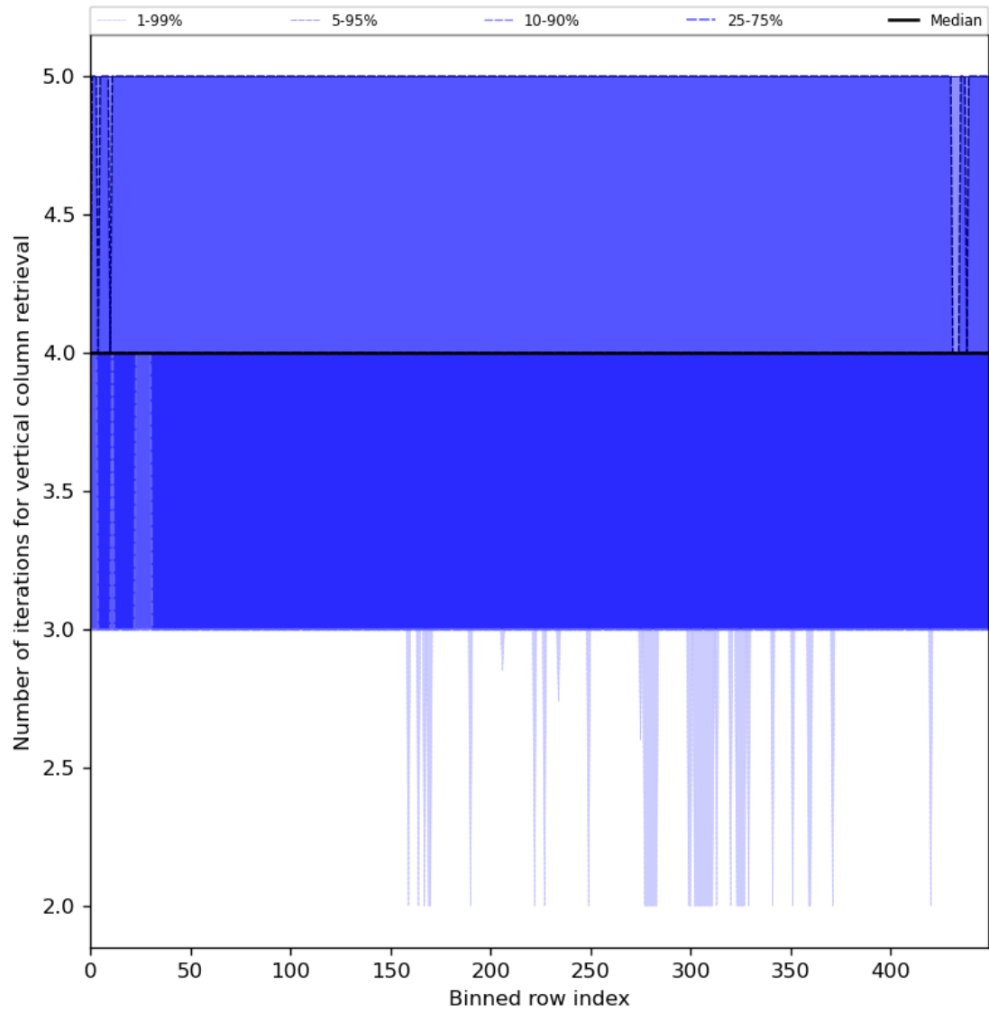
Figure 33: Along track statistics of “Number of iterations for vertical column retrieval” for 2024-03-31 to 2024-04-01
