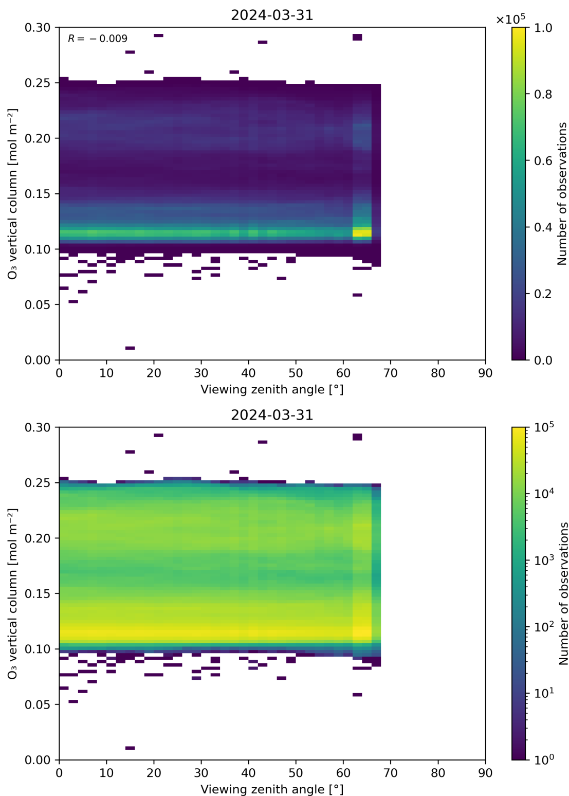
Figure 52: Scatter density plot of “Viewing zenith angle” against “O 3 vertical column” for 2024-03-31 to 2024-04-01.
