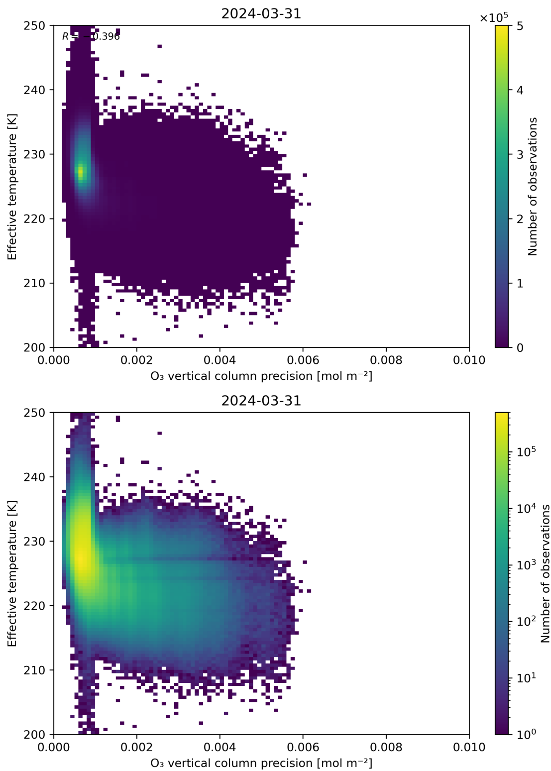
Figure 42: Scatter density plot of “O 3 vertical column precision” against “Effective temperature” for 2024-03-31 to 2024-04-01.
