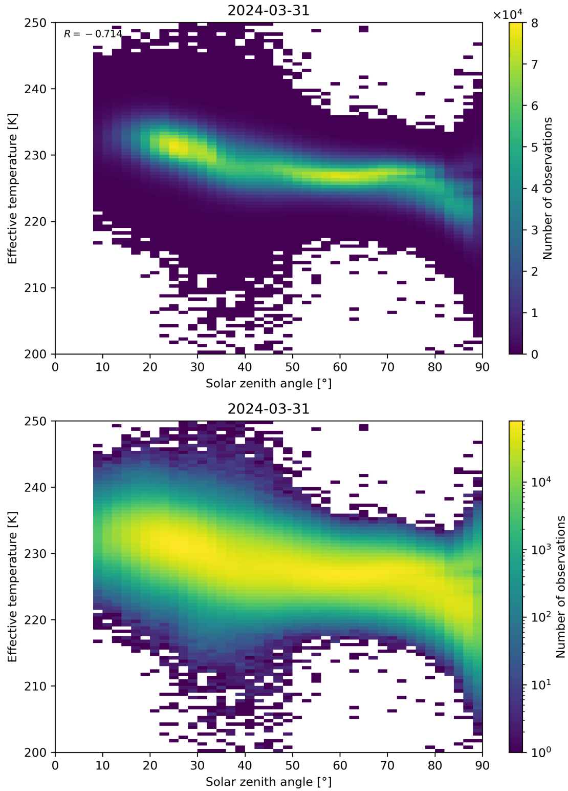
Figure 45: Scatter density plot of “Solar zenith angle” against “Effective temperature” for 2024-03-31 to 2024-04-01.
