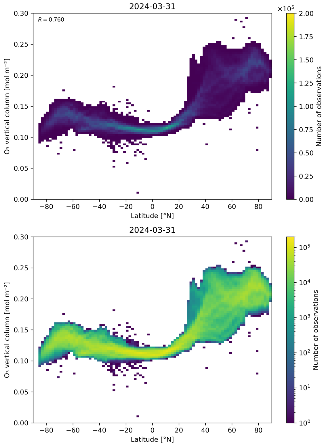
Figure 36: Scatter density plot of “Latitude” against “O 3 vertical column” for 2024-03-31 to 2024-04-01.
