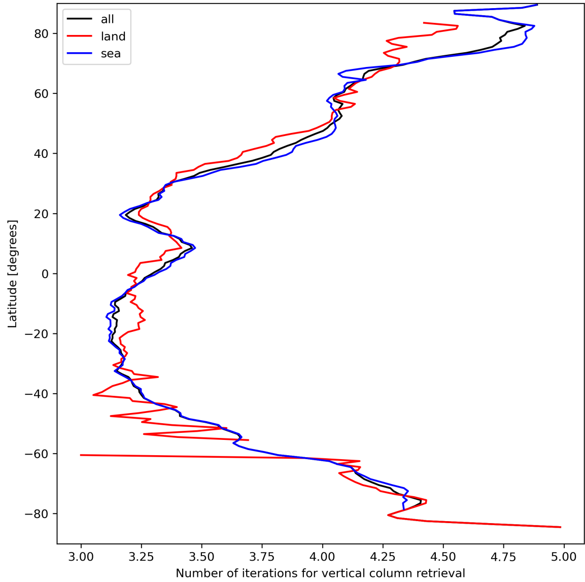
Figure 19: Zonal average of “Number of iterations for vertical column retrieval” for 2024-03-31 to 2024-04-01.
