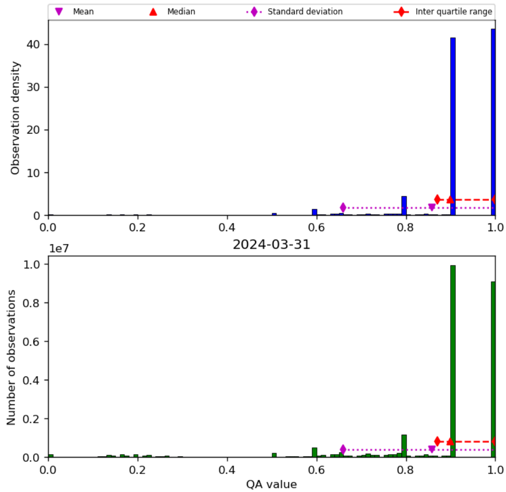
Figure 20: Histogram of “QA value” for 2024-03-31 to 2024-04-01
