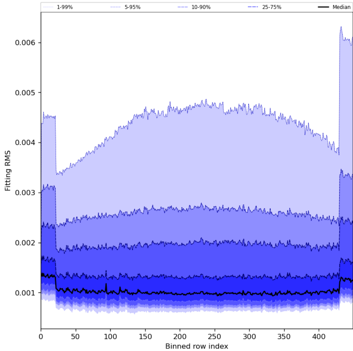
Figure 30: Along track statistics of “Fitting RMS” for 2024-03-31 to 2024-04-01
