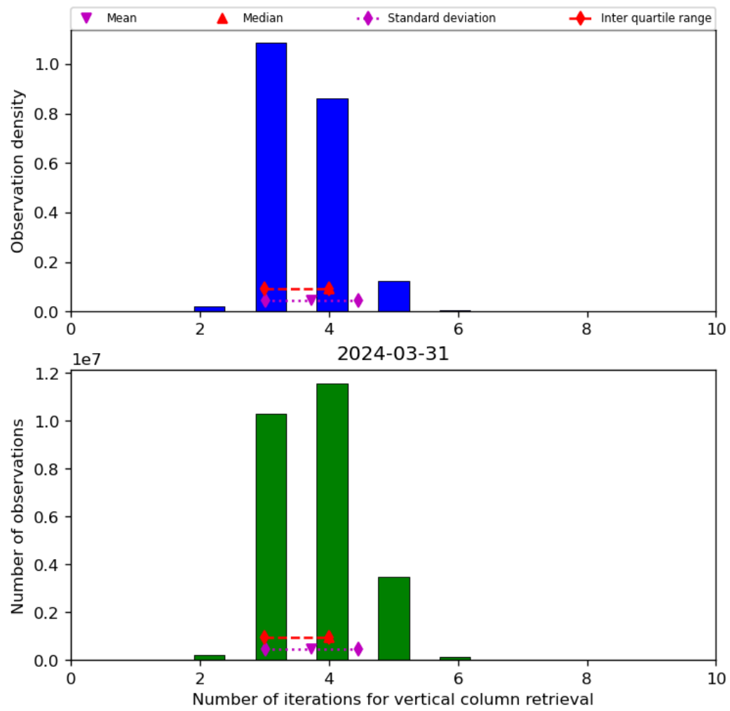
Figure 26: Histogram of “Number of iterations for vertical column retrieval” for 2024-03-31 to 2024-04-01
