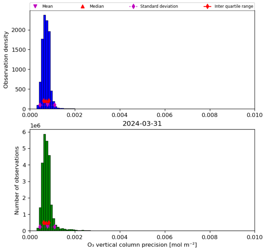
Figure 22: Histogram of “O 3 vertical column precision” for 2024-03-31 to 2024-04-01
