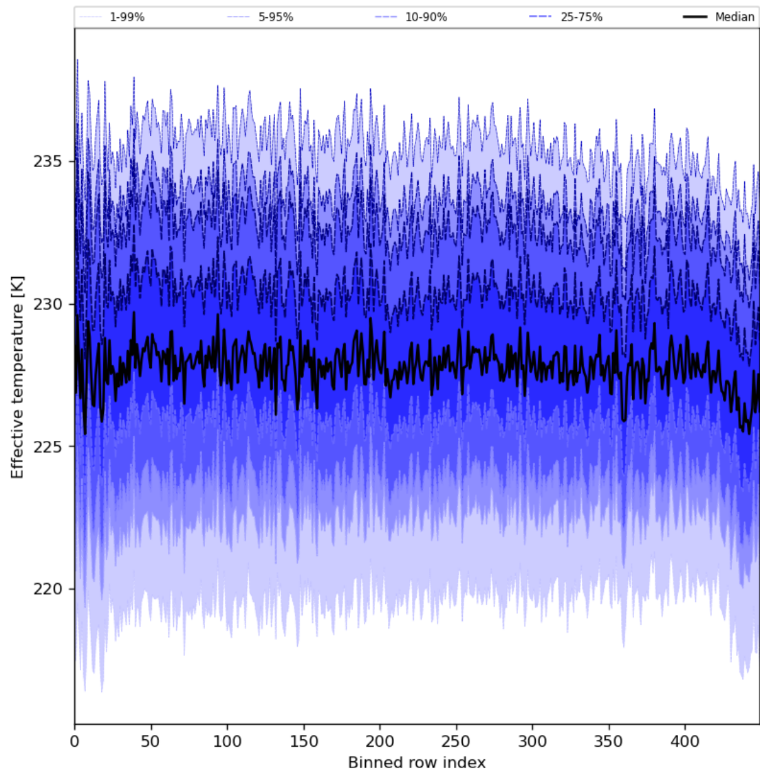
Figure 31: Along track statistics of “Effective temperature” for 2024-03-31 to 2024-04-01
