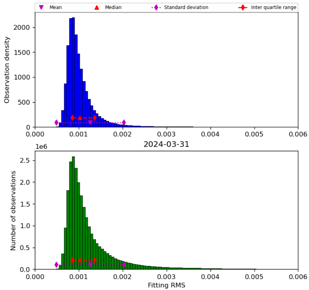
Figure 23: Histogram of “Fitting RMS” for 2024-03-31 to 2024-04-01
