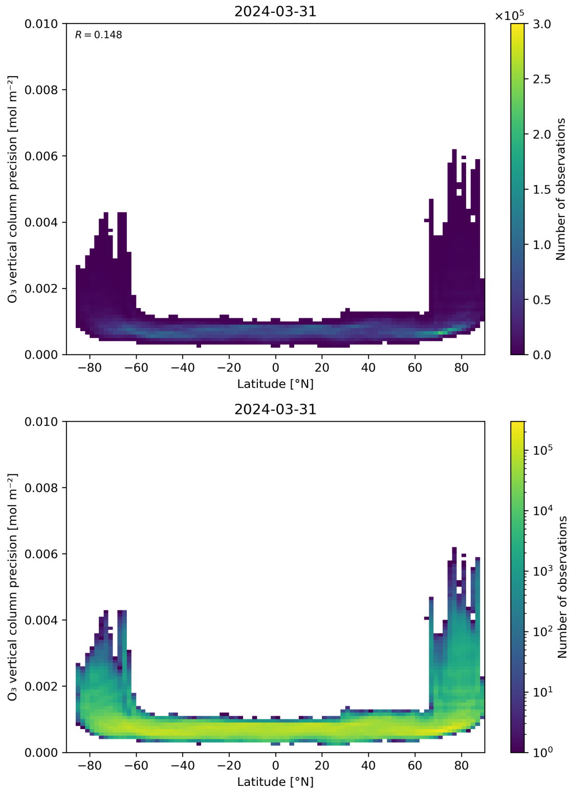
Figure 37: Scatter density plot of “Latitude” against “O 3 vertical column precision” for 2024-03-31 to 2024-04-01.
