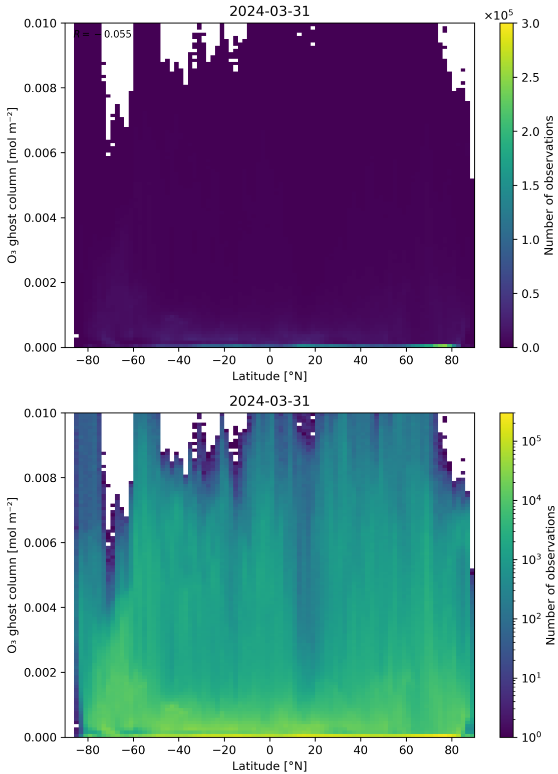
Figure 35: Scatter density plot of “Latitude” against “O 3 ghost column” for 2024-03-31 to 2024-04-01.
