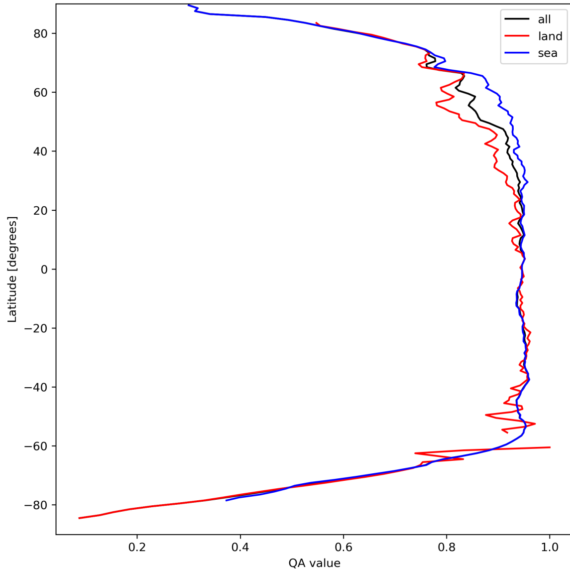
Figure 13: Zonal average of “QA value” for 2024-03-31 to 2024-04-01.
