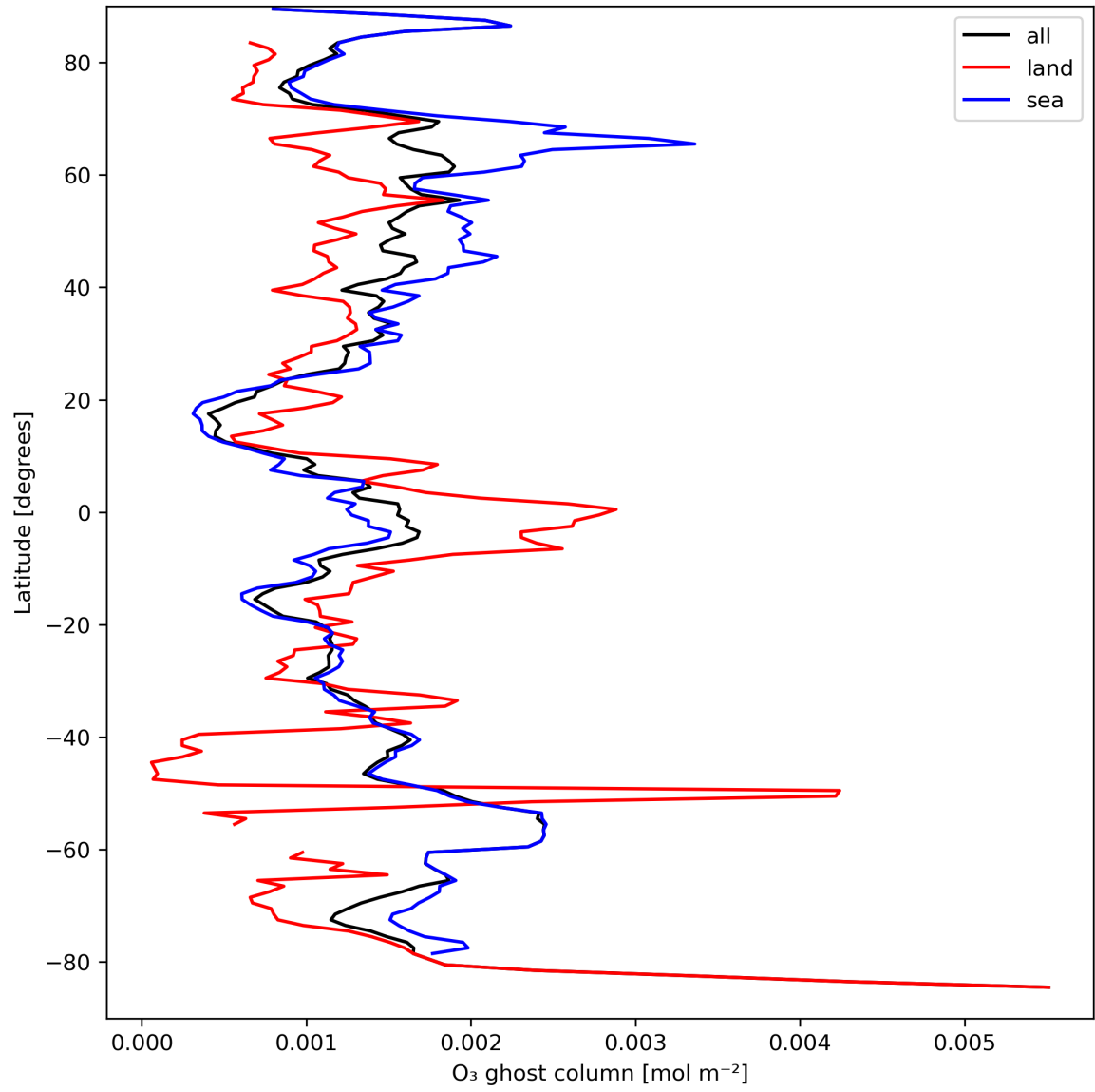
Figure 18: Zonal average of "O 3 ghost column" for 2024-03-31 to 2024-04-01.
