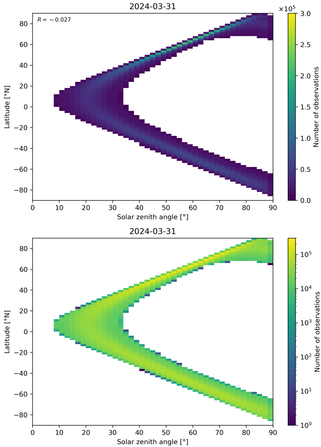
Figure 44: Scatter density plot of “Solar zenith angle” against “Latitude” for 2024-03-31 to 2024-04-01.
