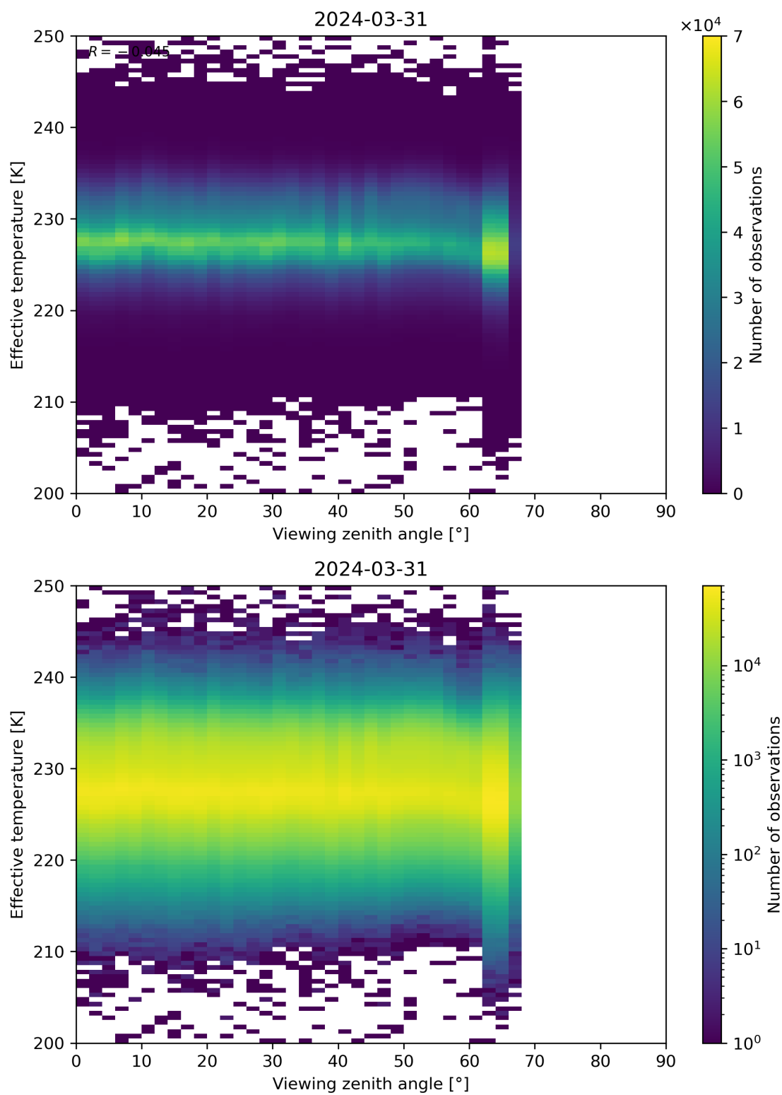
Figure 50: Scatter density plot of “Viewing zenith angle” against “Effective temperature” for 2024-03-31 to 2024-04-01.
