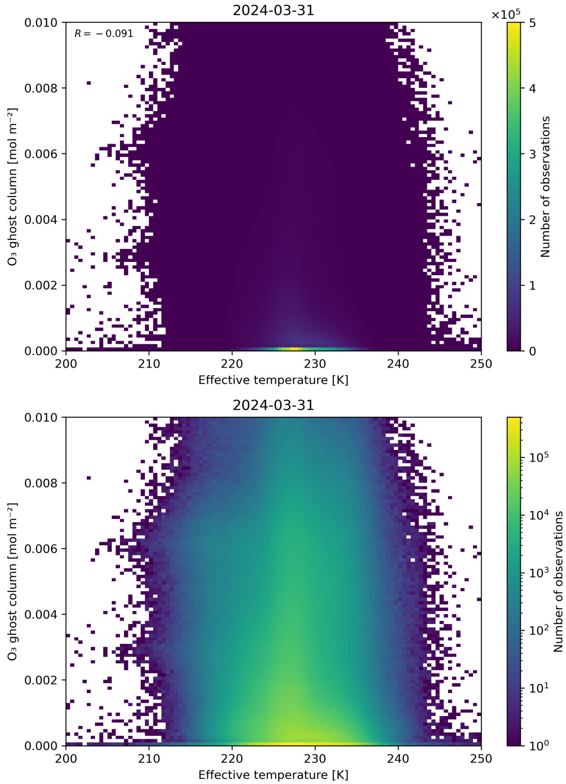
Figure 38: Scatter density plot of “Effective temperature” against “O 3 ghost column” for 2024-03-31 to 2024-04-01.
