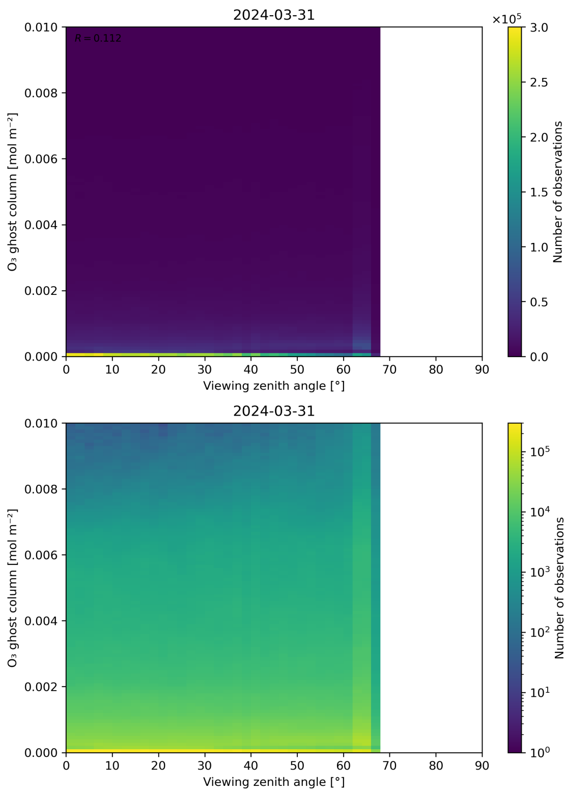
Figure 51: Scatter density plot of “Viewing zenith angle” against “O 3 ghost column” for 2024-03-31 to 2024-04-01.
