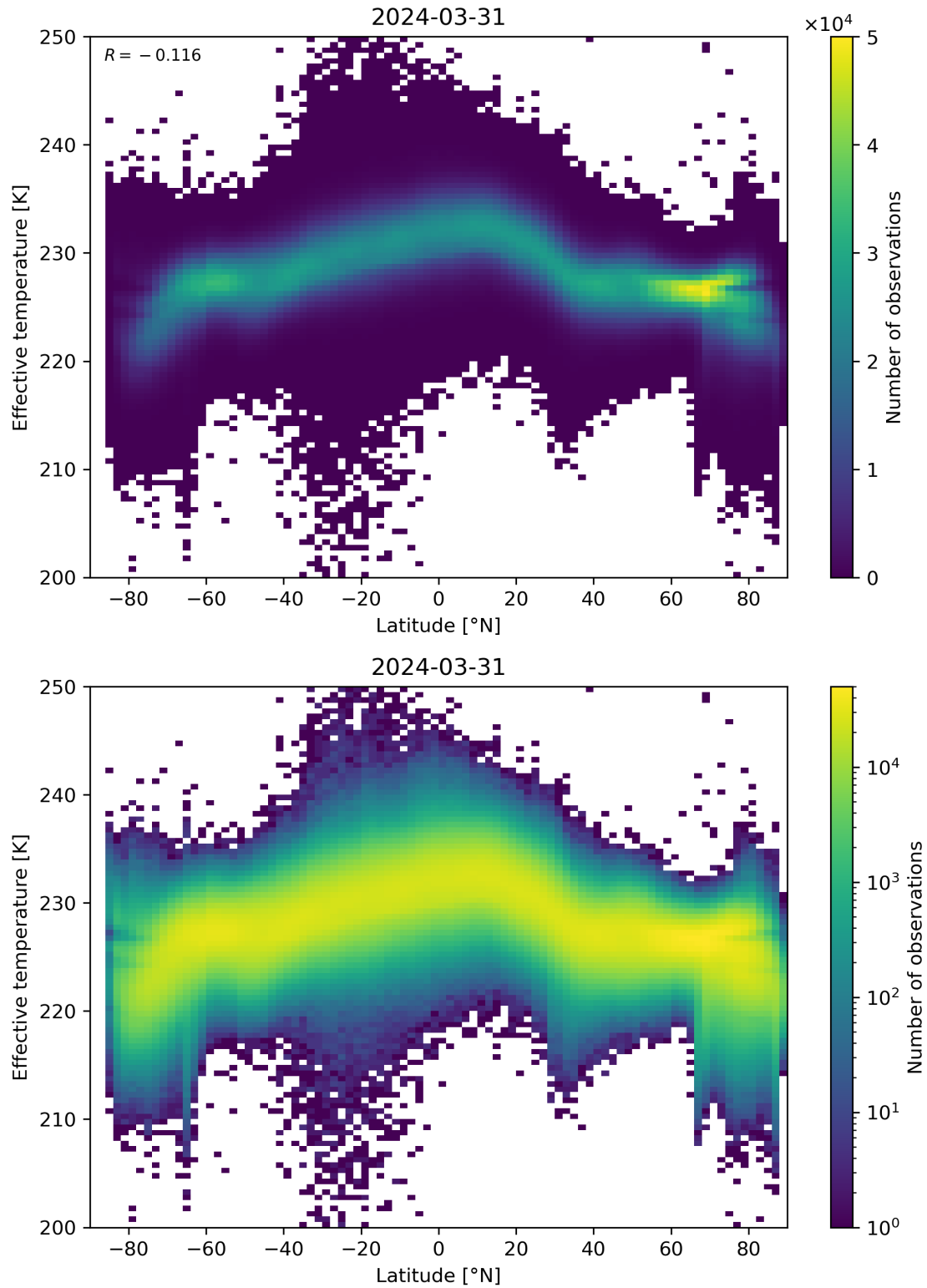
Figure 34: Scatter density plot of “Latitude” against “Effective temperature” for 2024-03-31 to 2024-04-01.
