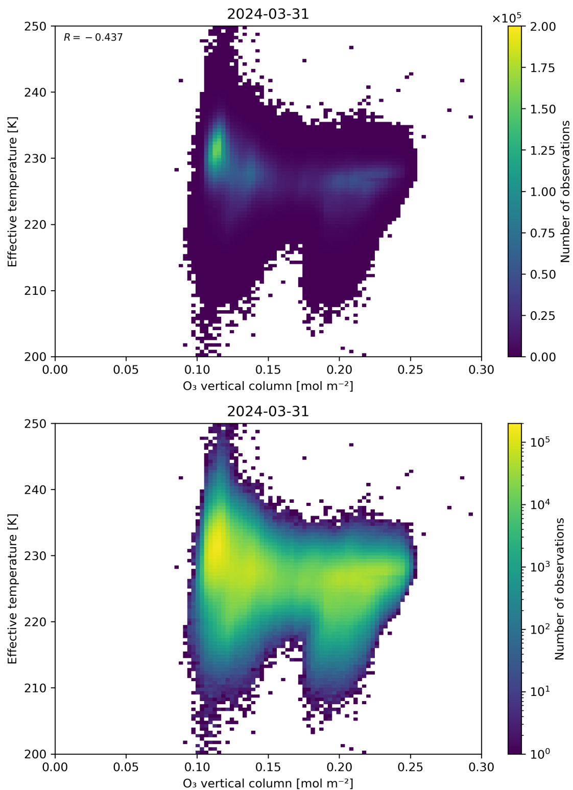
Figure 39: Scatter density plot of “O 3 vertical column” against “Effective temperature” for 2024-03-31 to 2024-04-01.
