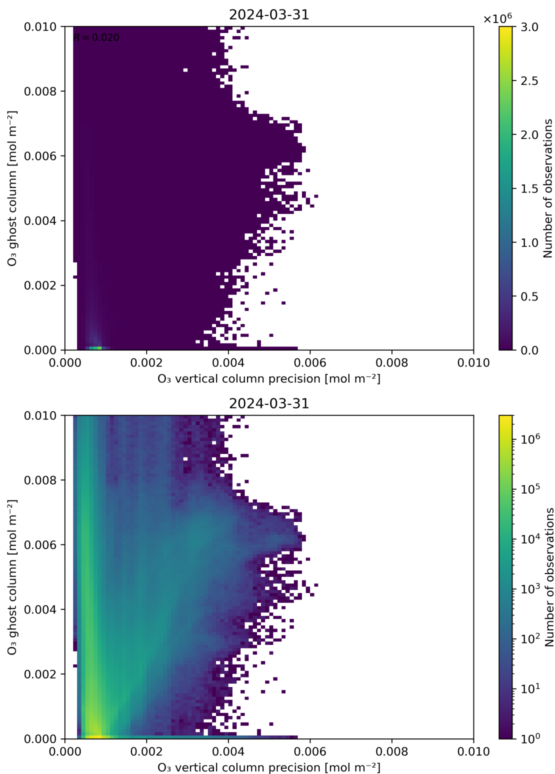
Figure 43: Scatter density plot of “O 3 vertical column precision” against “O 3 ghost column” for 2024-03-31 to 2024-04-01.
