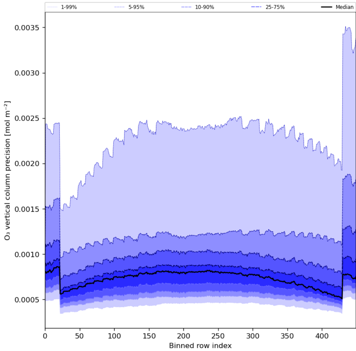
Figure 29: Along track statistics of “O 3 vertical column precision” for 2024-03-31 to 2024-04-01
