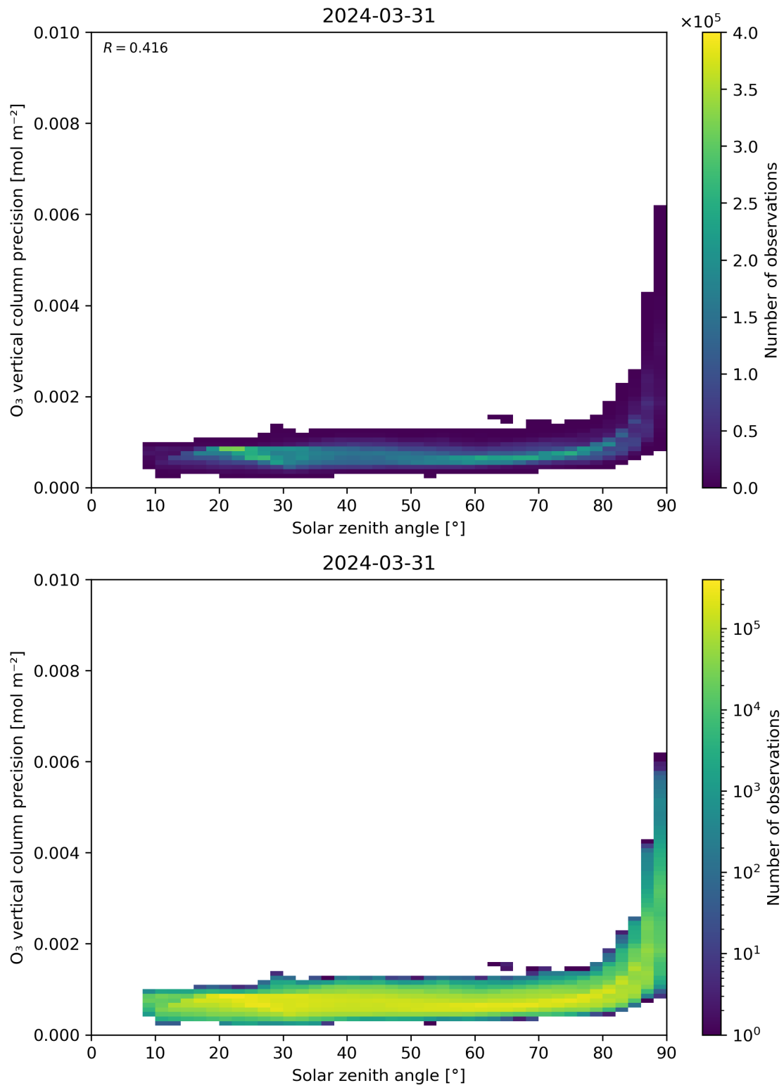
Figure 48: Scatter density plot of “Solar zenith angle” against “O 3 vertical column precision” for 2024-03-31 to 2024-04-01.
