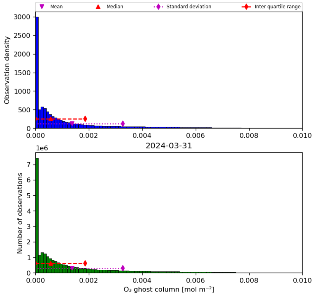
Figure 25: Histogram of “O 3 ghost column” for 2024-03-31 to 2024-04-01
