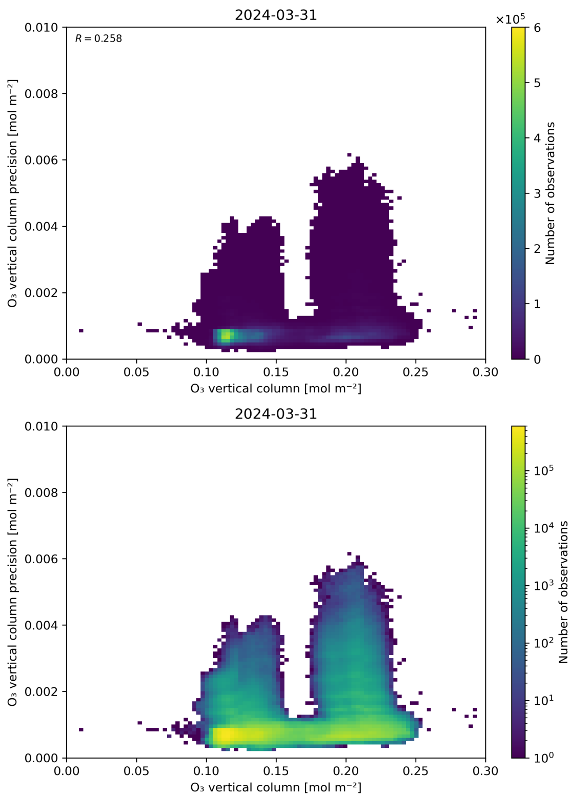
Figure 41: Scatter density plot of “O 3 vertical column” against “O 3 vertical column precision” for 2024-03-31 to 2024-04-01.
