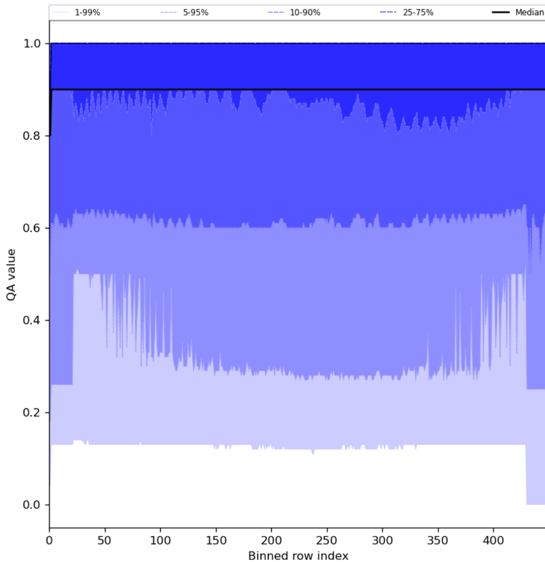
Figure 27: Along track statistics of “QA value” for 2024-03-31 to 2024-04-01
