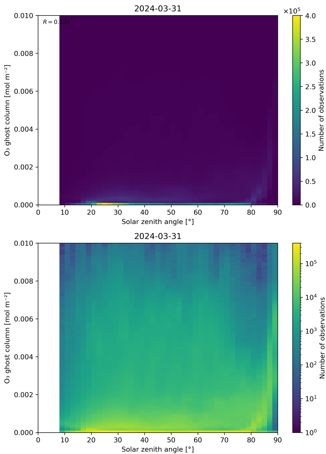
Figure 46: Scatter density plot of “Solar zenith angle” against “O 3 ghost column” for 2024-03-31 to 2024-04-01.
