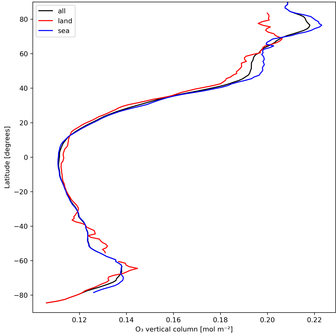
Figure 14: Zonal average of “O 3 vertical column” for 2024-03-31 to 2024-04-01.
