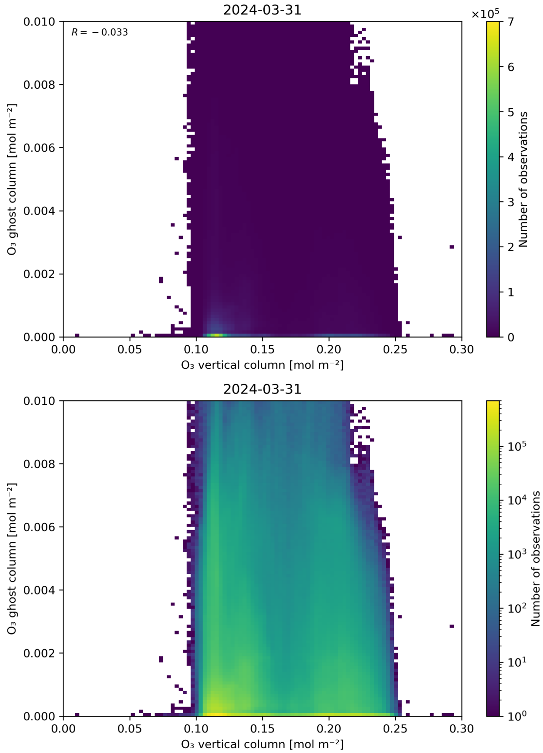
Figure 40: Scatter density plot of “O 3 vertical column” against “O 3 ghost column” for 2024-03-31 to 2024-04-01.
