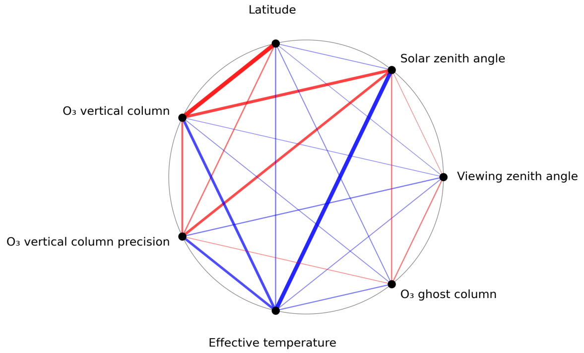
Figure 1: Map of correlation graph for 2024-03-31 to 2024-04-01.
