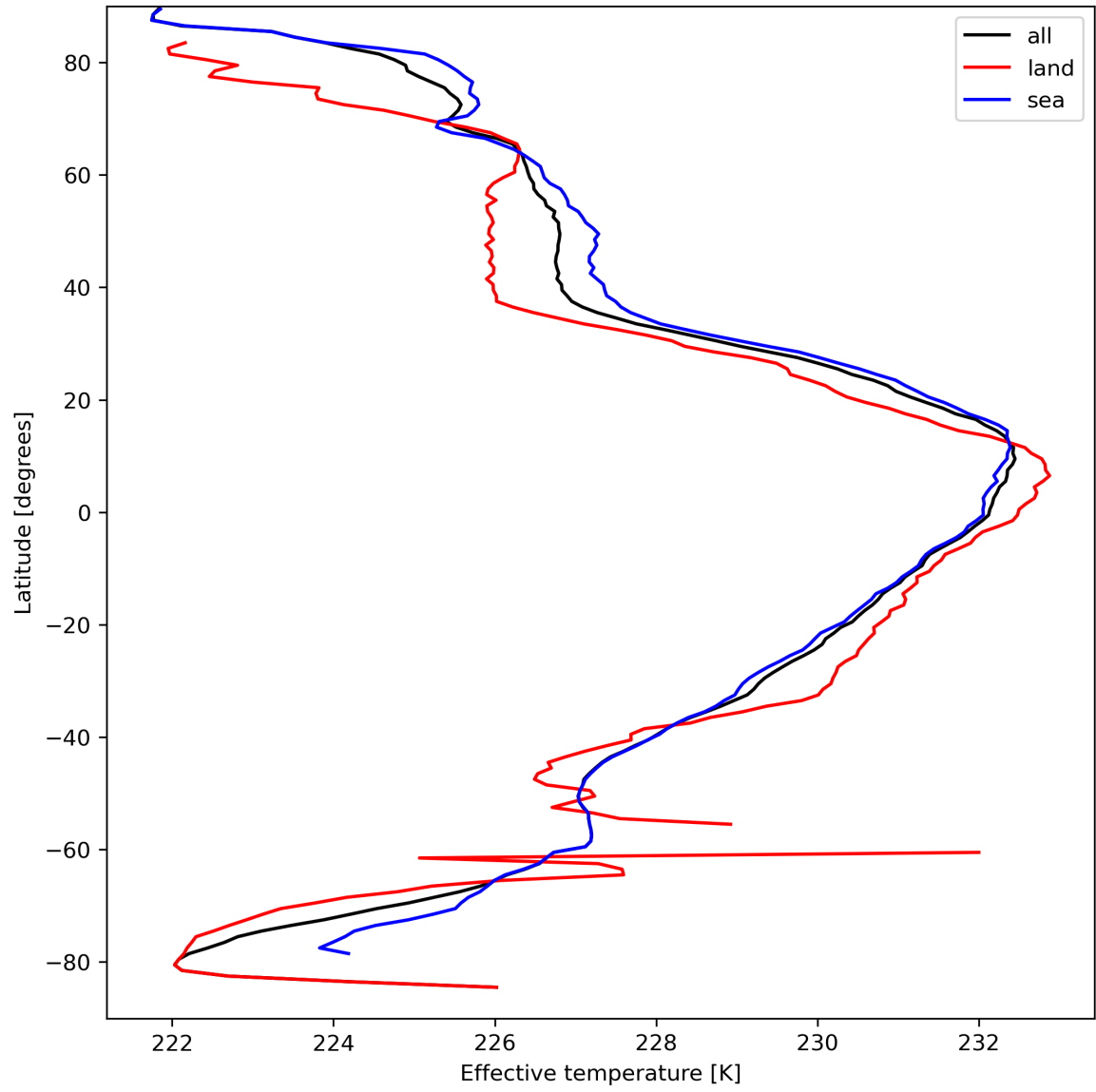
Figure 17: Zonal average of “Effective temperature” for 2024-03-31 to 2024-04-01.
