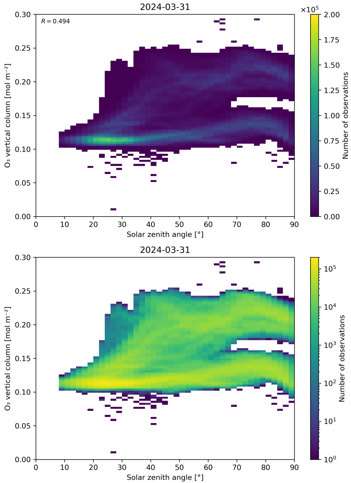
Figure 47: Scatter density plot of “Solar zenith angle” against “O 3 vertical column” for 2024-03-31 to 2024-04-01.
