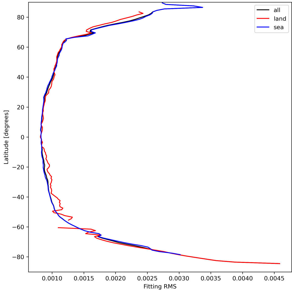
Figure 16: Zonal average of “Fitting RMS” for 2024-03-31 to 2024-04-01.
