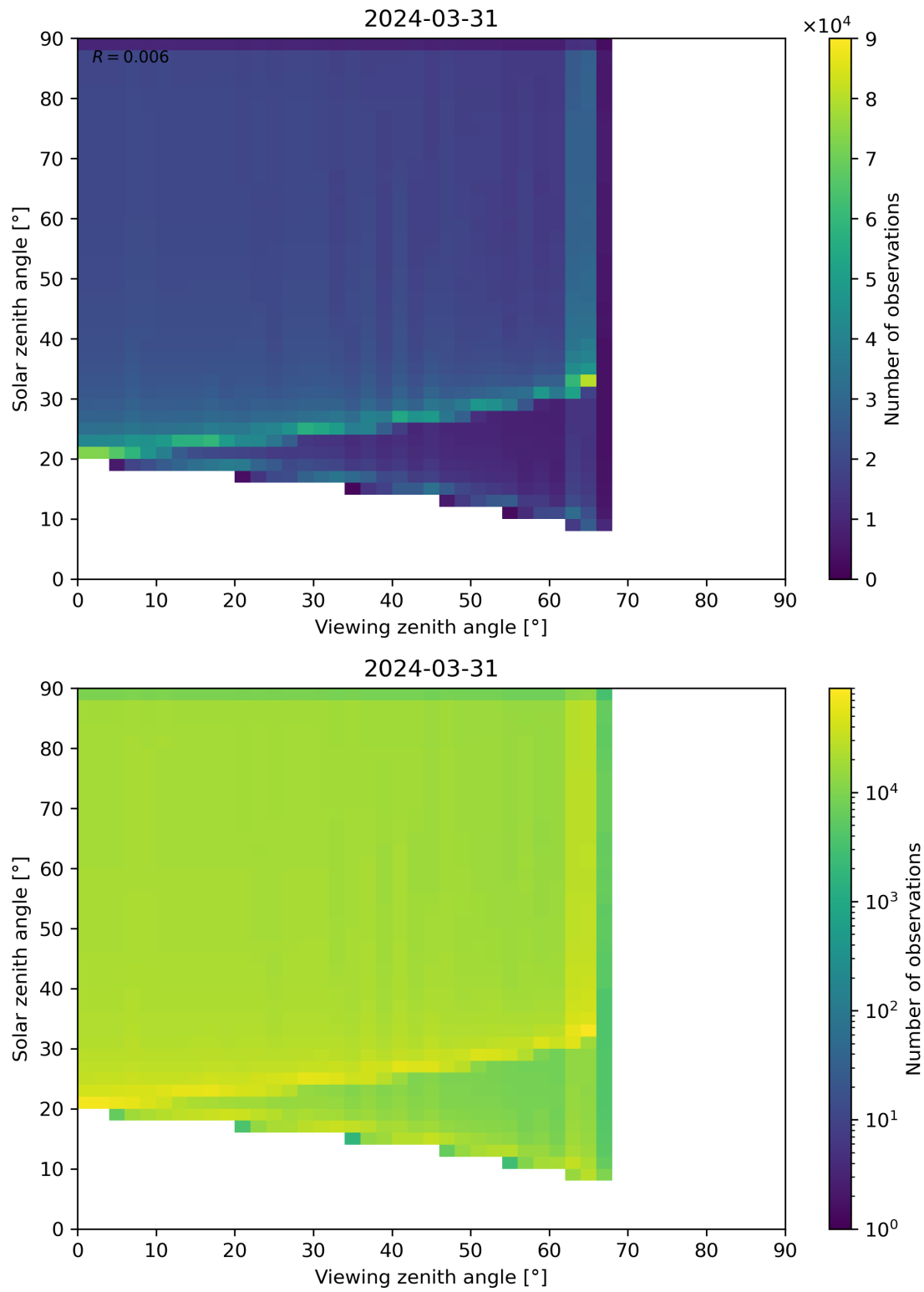
Figure 54: Scatter density plot of “Viewing zenith angle” against “Solar zenith angle” for 2024-03-31 to 2024-04-01.
