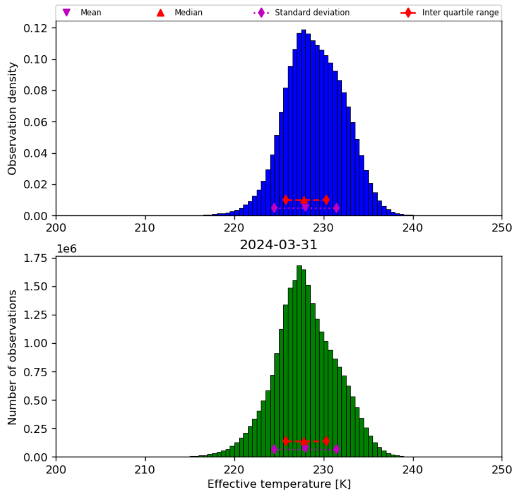
Figure 24: Histogram of “Effective temperature” for 2024-03-31 to 2024-04-01
