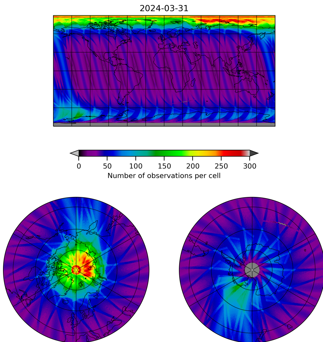
Figure 12: Map of the number of observations for 2024-03-31 to 2024-04-01
