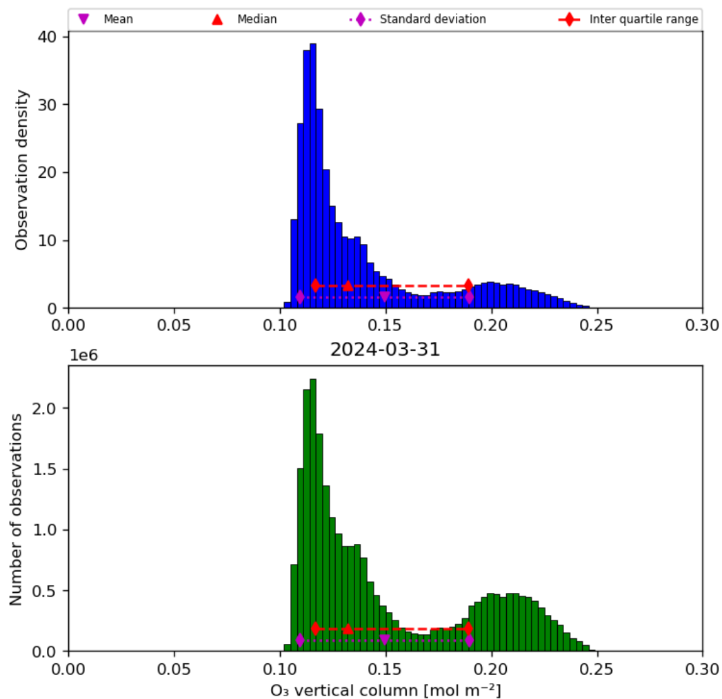
Figure 21: Histogram of “O 3 vertical column” for 2024-03-31 to 2024-04-01
