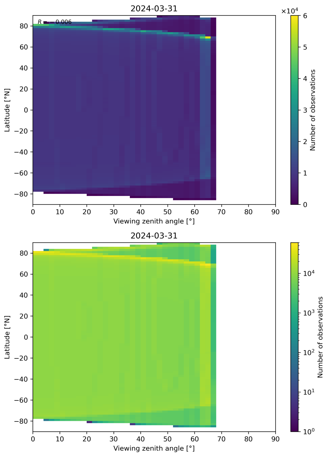
Figure 49: Scatter density plot of “Viewing zenith angle” against “Latitude” for 2024-03-31 to 2024-04-01.
