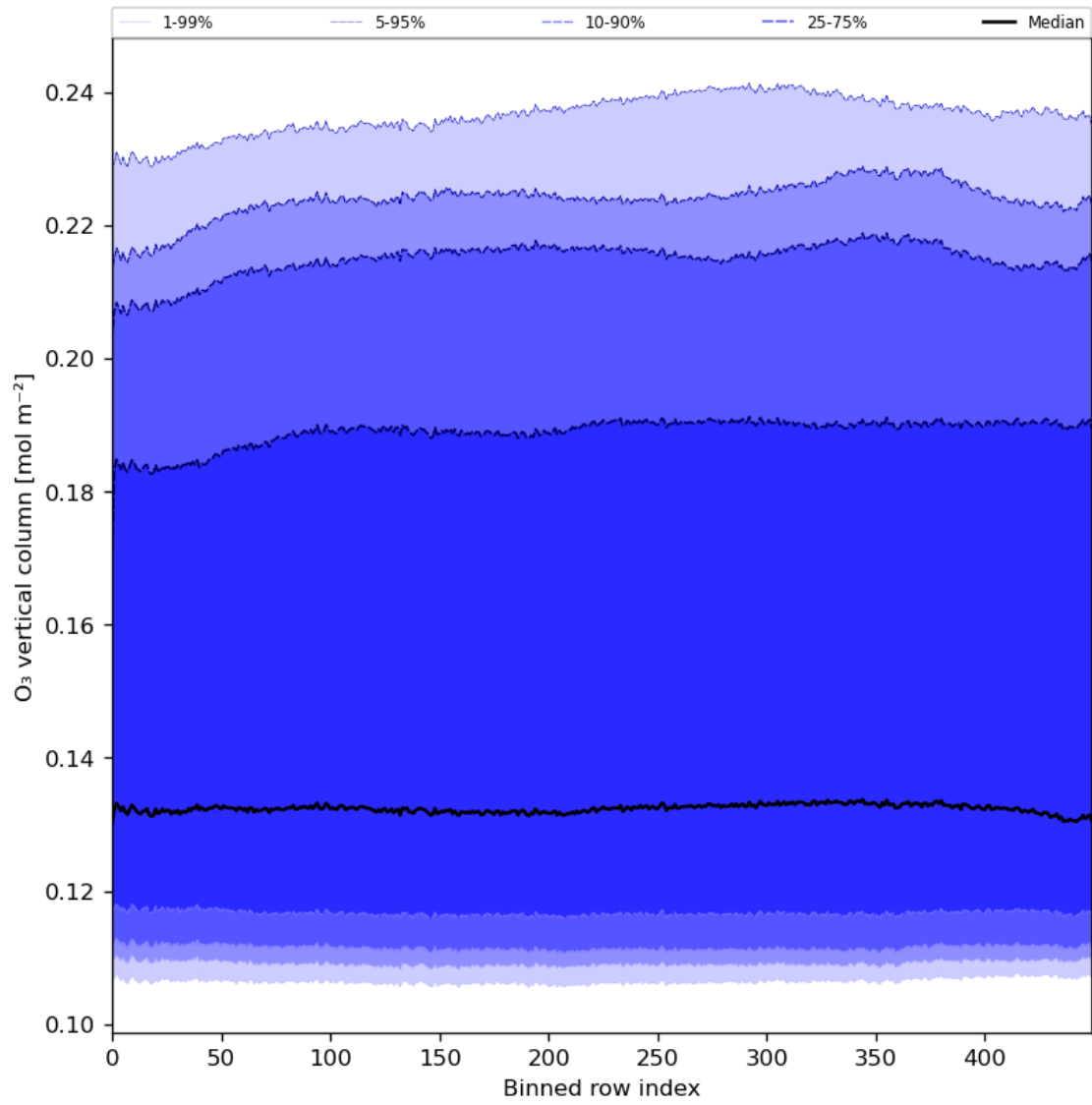
Figure 28: Along track statistics of “O 3 vertical column” for 2024-03-31 to 2024-04-01
