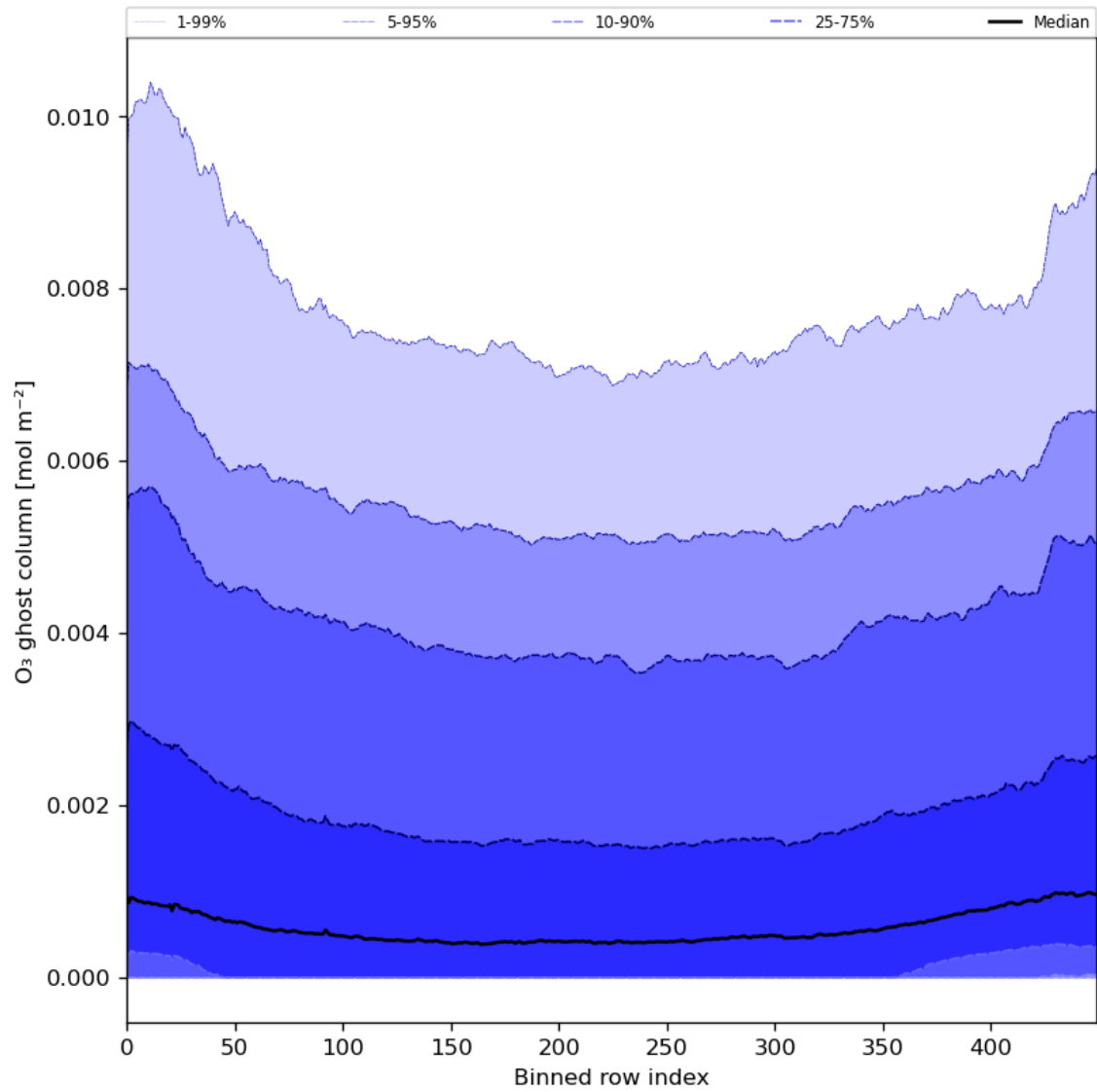
Figure 32: Along track statistics of "O 3 ghost column" for 2024-03-31 to 2024-04-01
