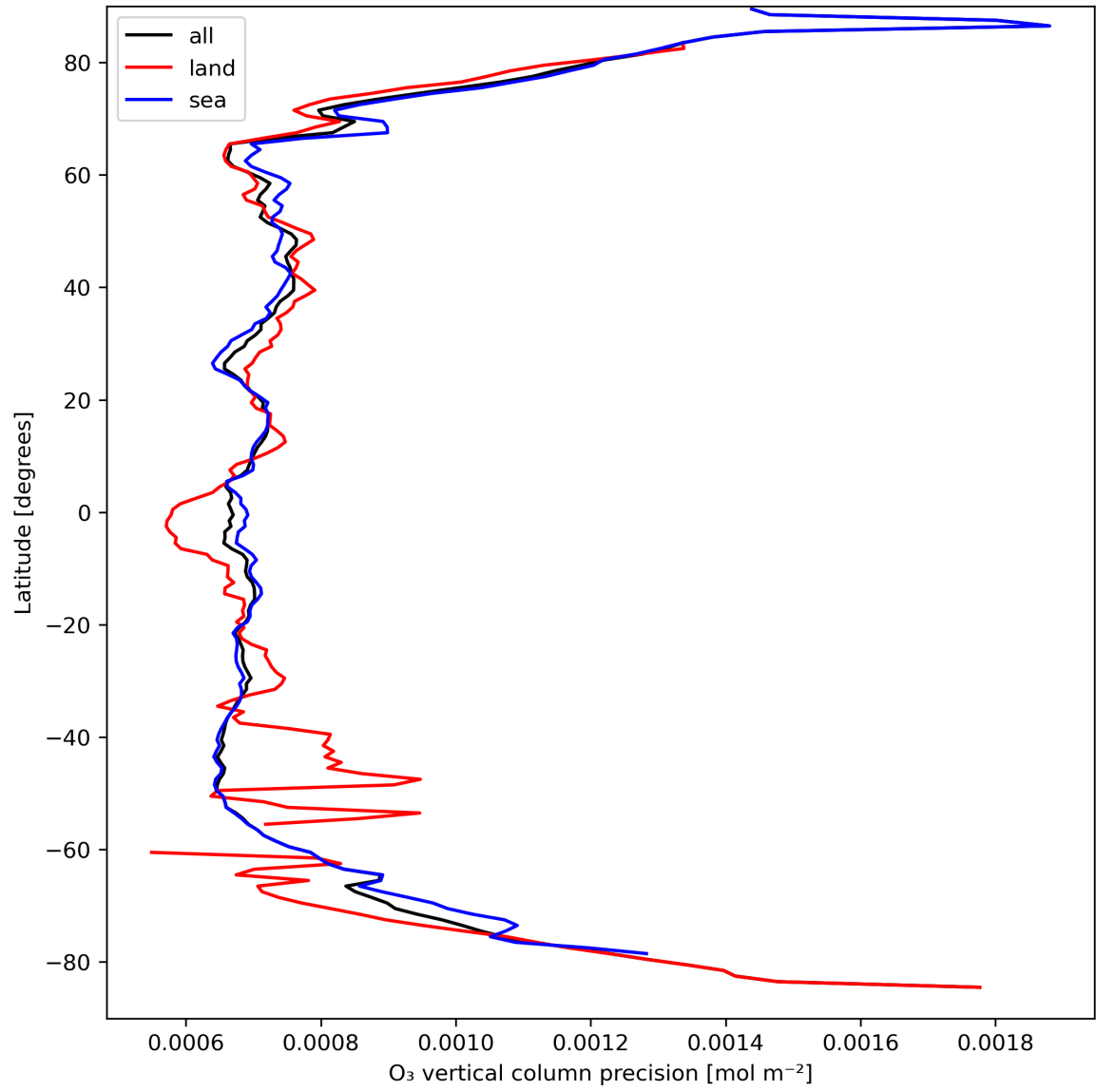
Figure 15: Zonal average of “O 3 vertical column precision” for 2024-03-31 to 2024-04-01.
