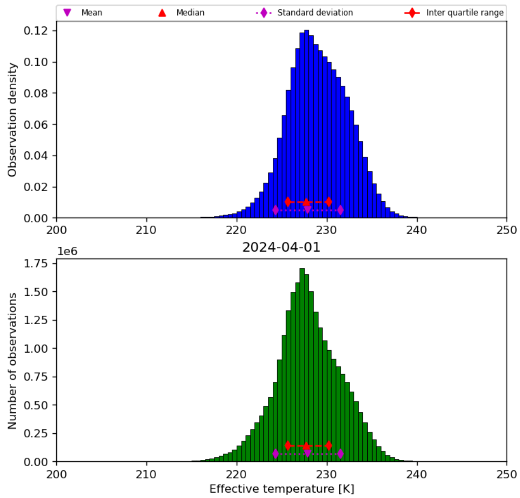
Figure 24: Histogram of “Effective temperature” for 2024-03-31 to 2024-04-02
