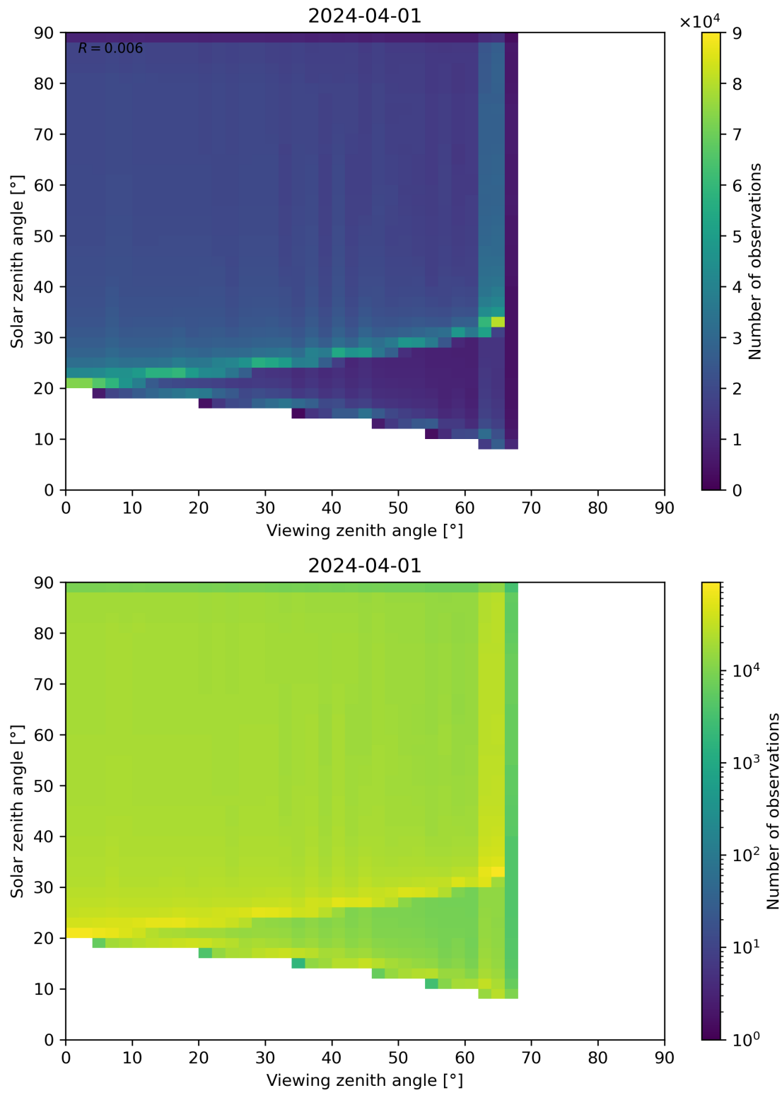
Figure 54: Scatter density plot of “Viewing zenith angle” against “Solar zenith angle” for 2024-03-31 to 2024-04-02.
