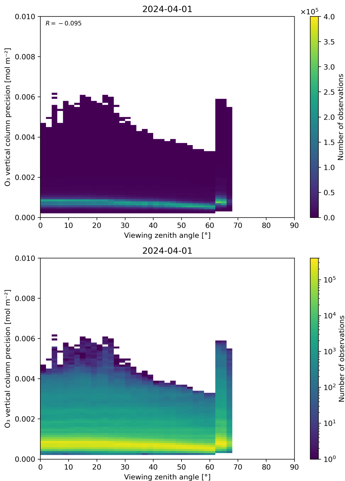
Figure 53: Scatter density plot of “Viewing zenith angle” against “O 3 vertical column precision” for 2024-03-31 to 2024-04-02.
