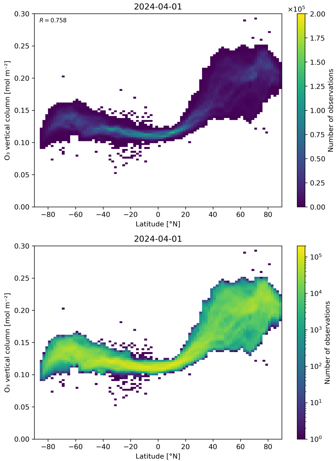
Figure 36: Scatter density plot of “Latitude” against “O 3 vertical column” for 2024-03-31 to 2024-04-02.
