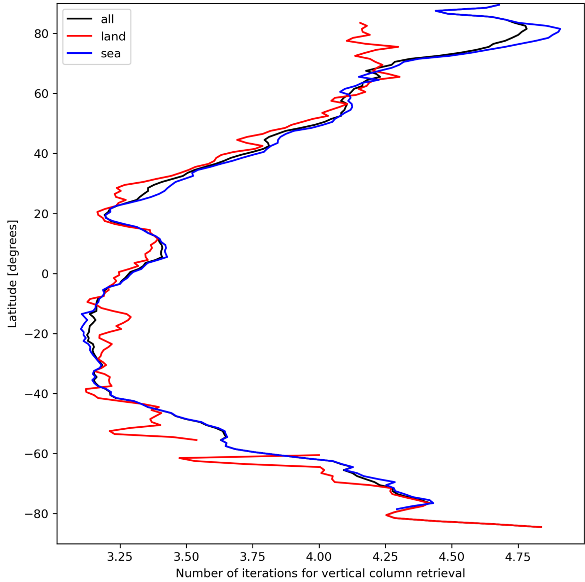
Figure 19: Zonal average of “Number of iterations for vertical column retrieval” for 2024-03-31 to 2024-04-02.
