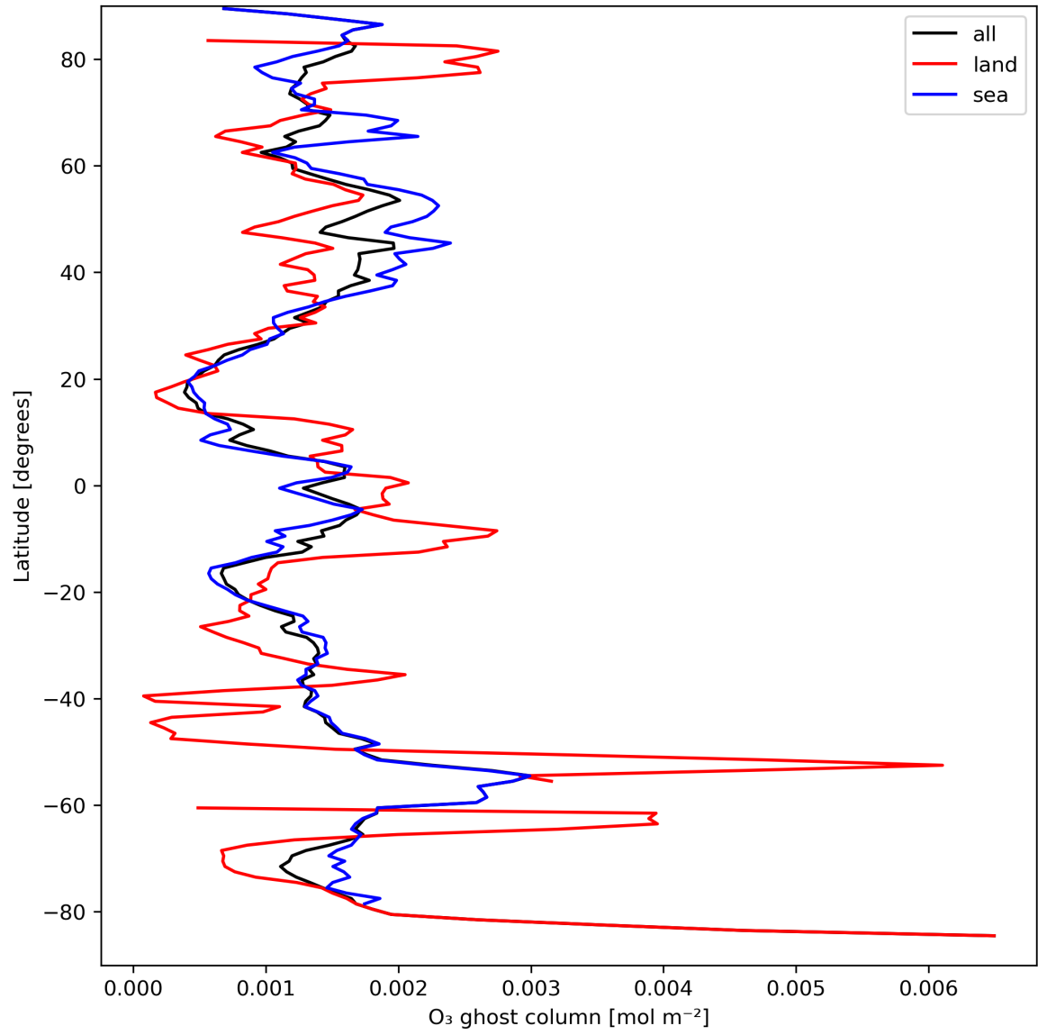
Figure 18: Zonal average of "O 3 ghost column" for 2024-03-31 to 2024-04-02.
