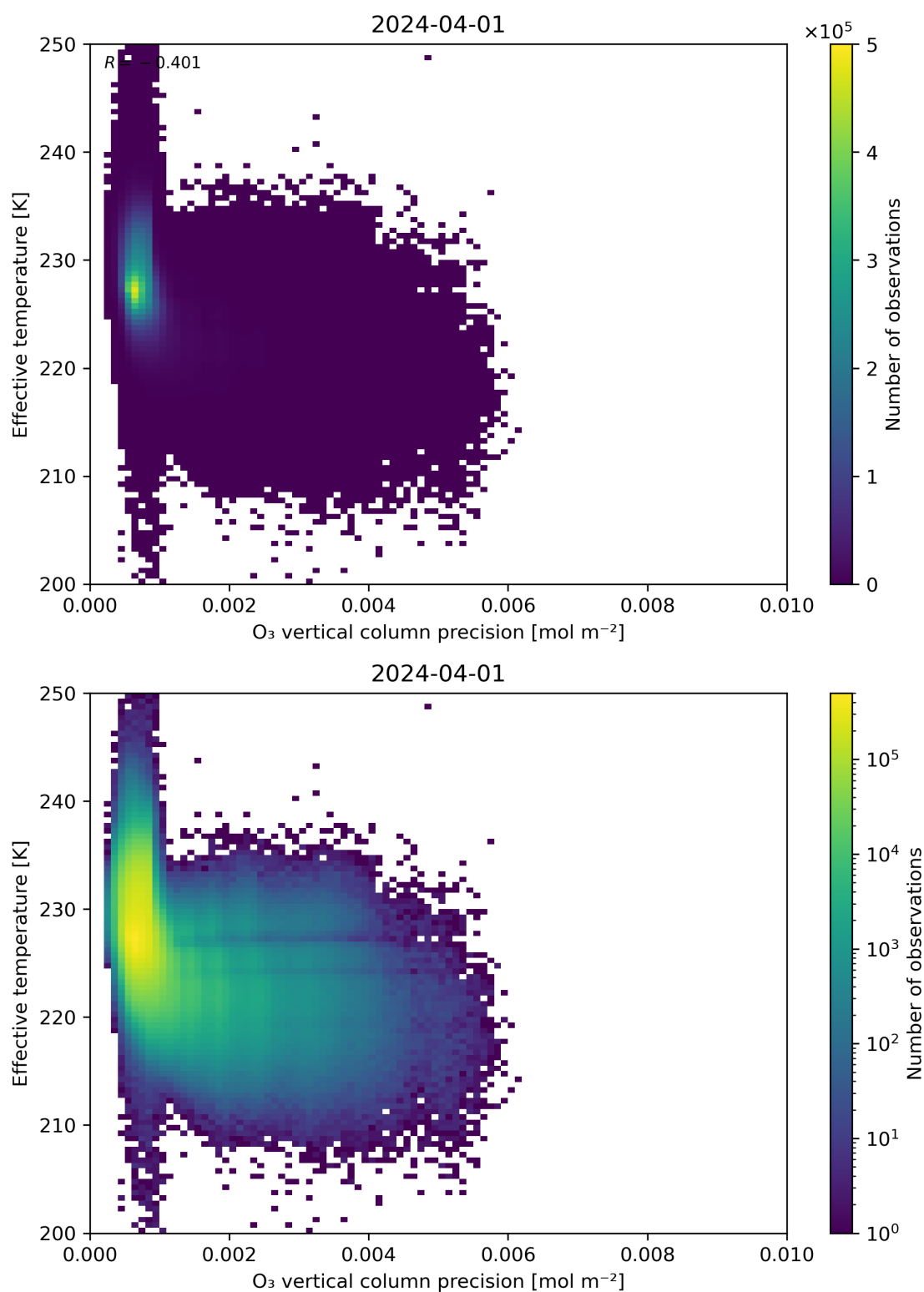
Figure 42: Scatter density plot of “O 3 vertical column precision” against “Effective temperature” for 2024-03-31 to 2024-04-02.
