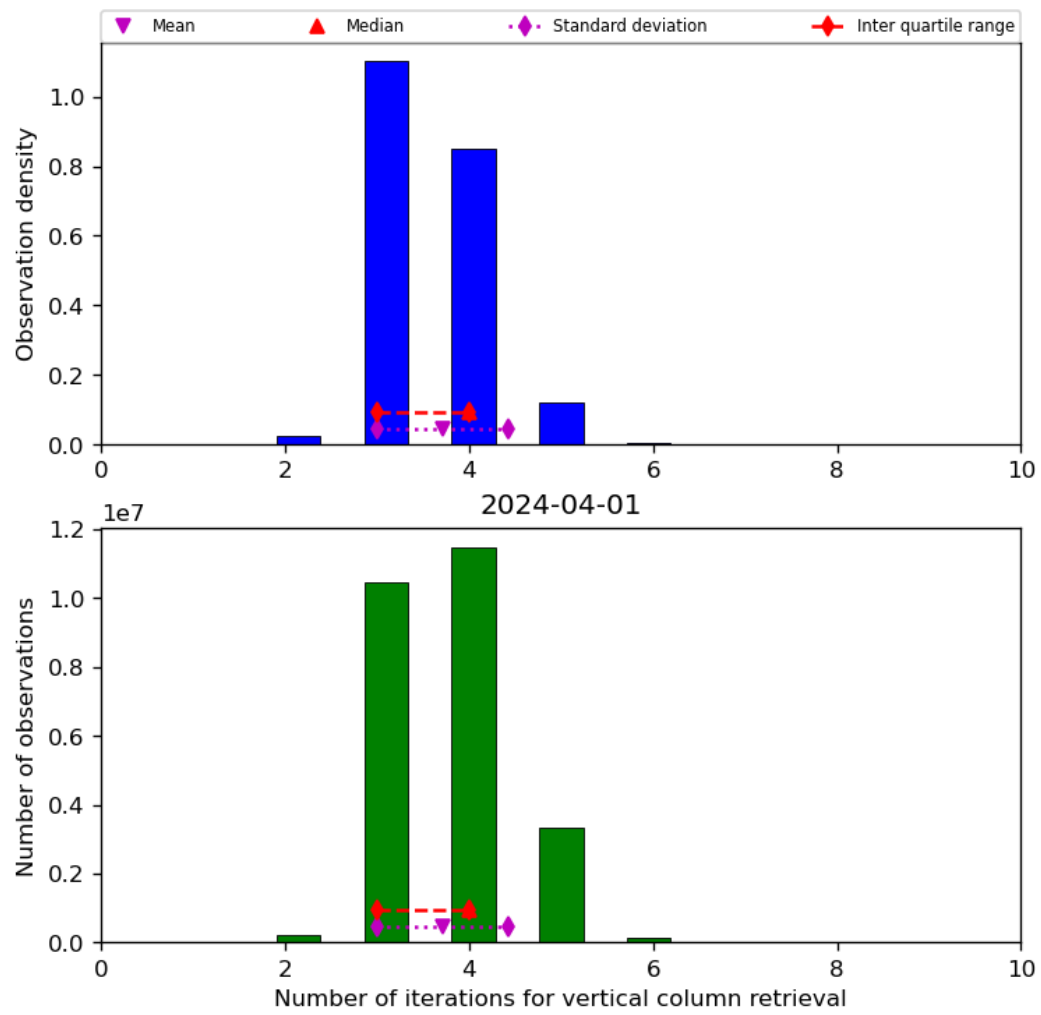
Figure 26: Histogram of “Number of iterations for vertical column retrieval” for 2024-03-31 to 2024-04-02
