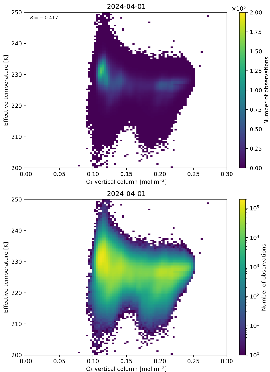
Figure 39: Scatter density plot of “O 3 vertical column” against “Effective temperature” for 2024-03-31 to 2024-04-02.
