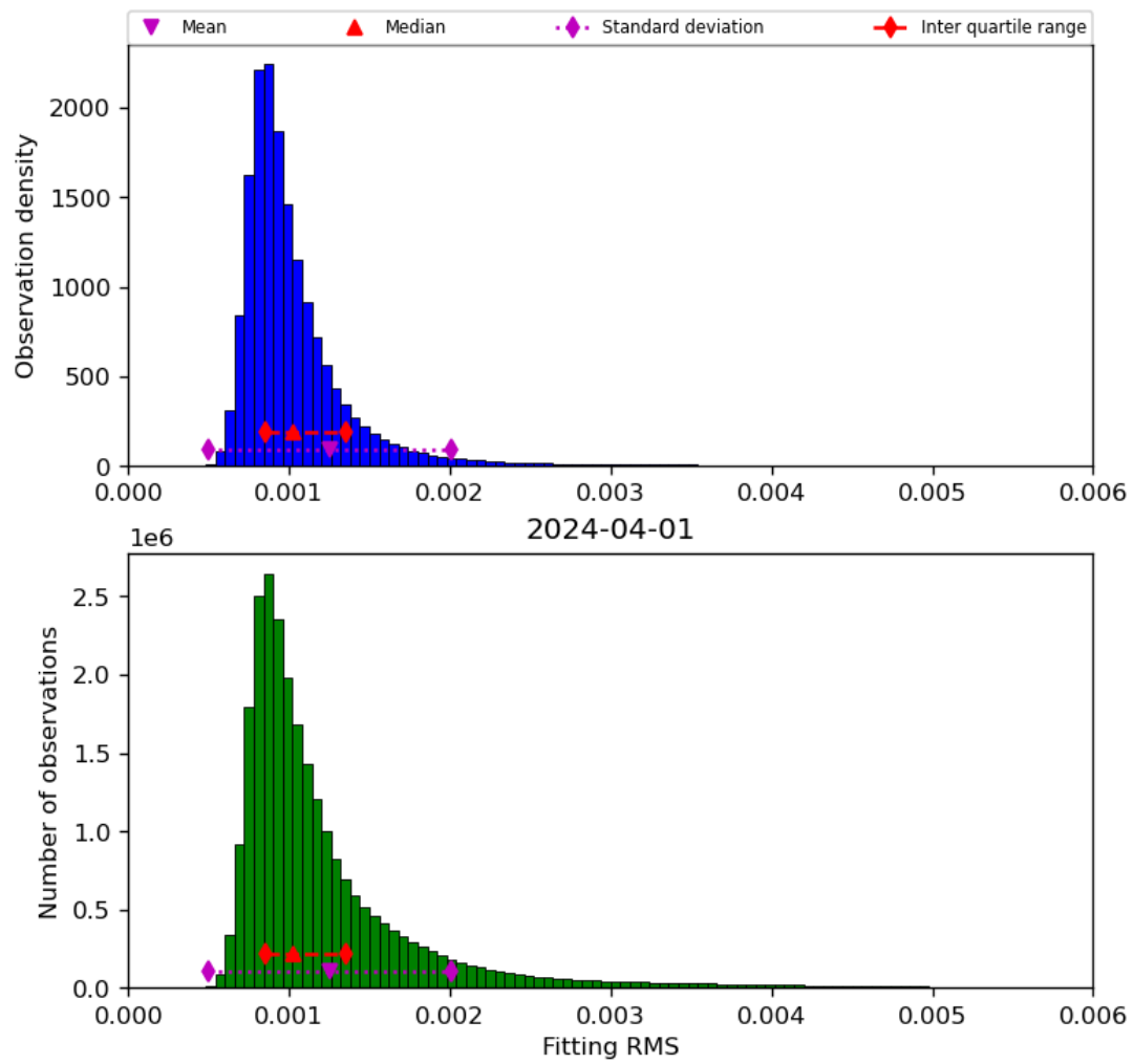
Figure 23: Histogram of “Fitting RMS” for 2024-03-31 to 2024-04-02
