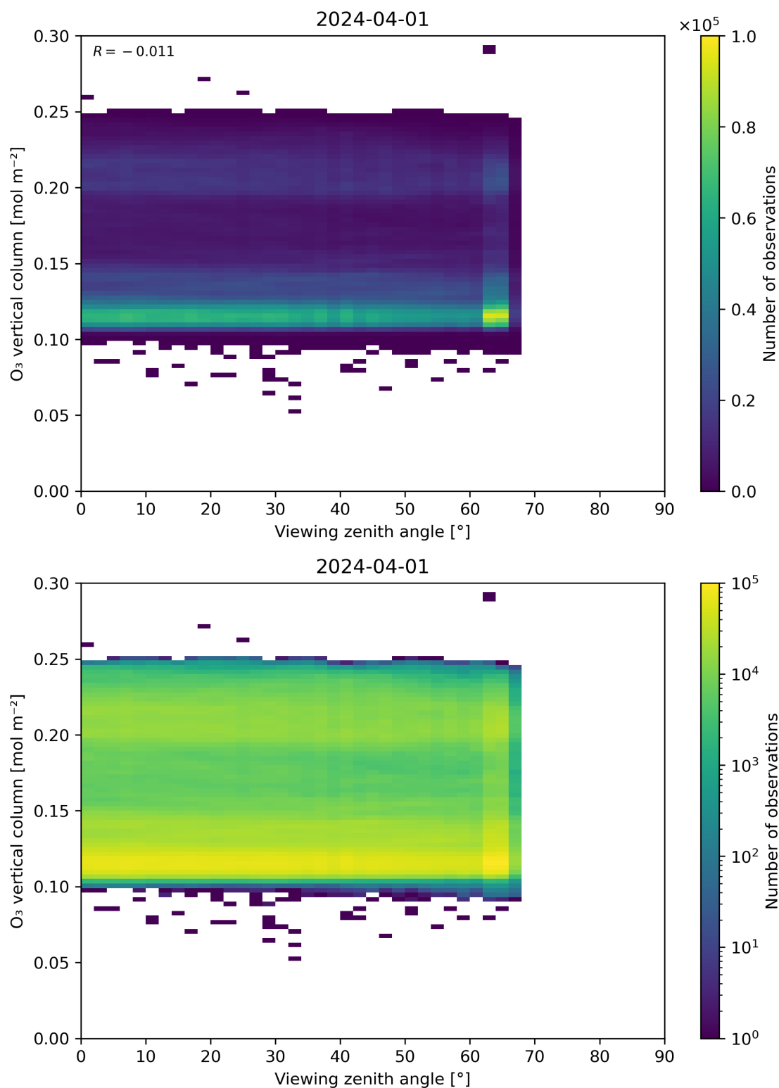
Figure 52: Scatter density plot of “Viewing zenith angle” against “O 3 vertical column” for 2024-03-31 to 2024-04-02.
