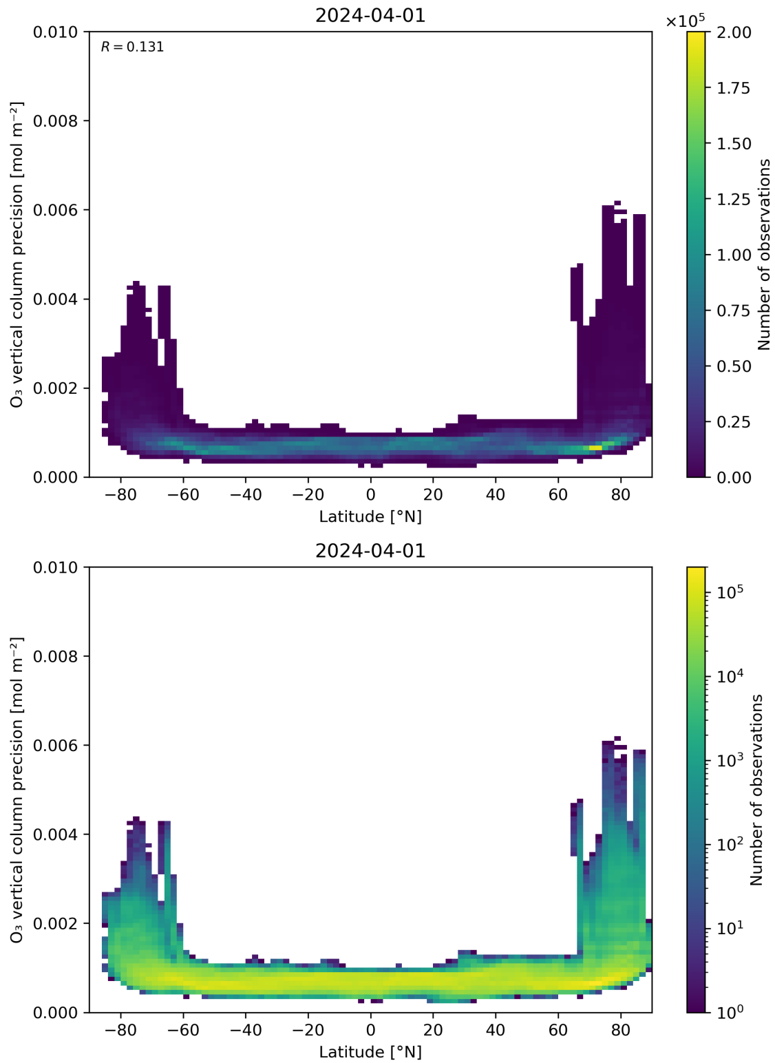
Figure 37: Scatter density plot of “Latitude” against “O 3 vertical column precision” for 2024-03-31 to 2024-04-02.
