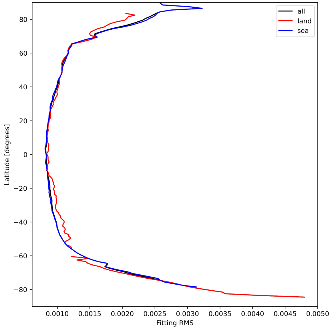
Figure 16: Zonal average of “Fitting RMS” for 2024-03-31 to 2024-04-02.
