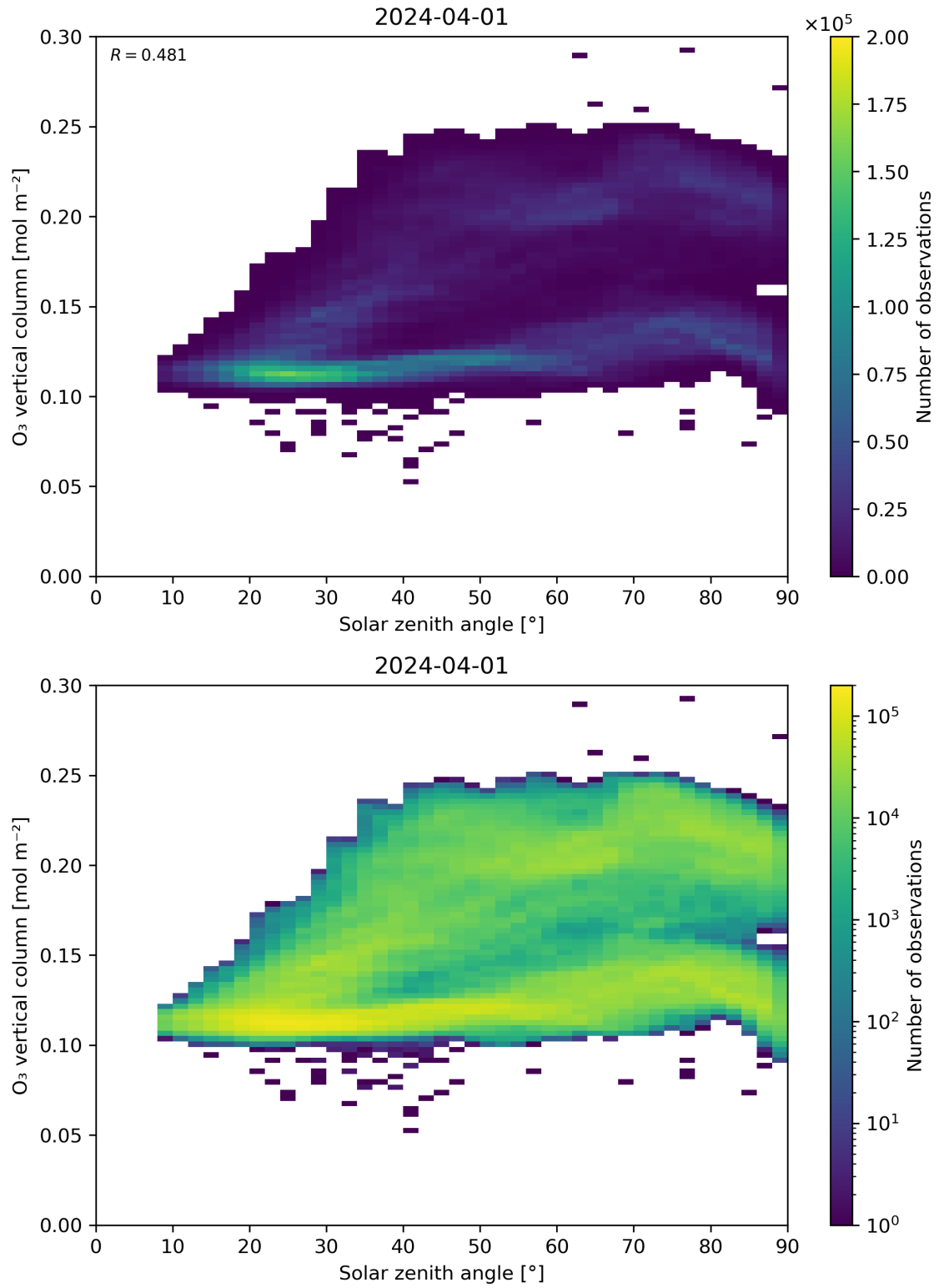
Figure 47: Scatter density plot of “Solar zenith angle” against “O 3 vertical column” for 2024-03-31 to 2024-04-02.
