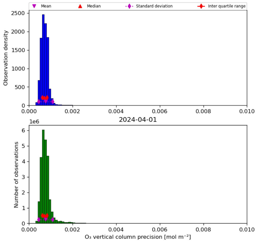
Figure 22: Histogram of “O 3 vertical column precision” for 2024-03-31 to 2024-04-02
