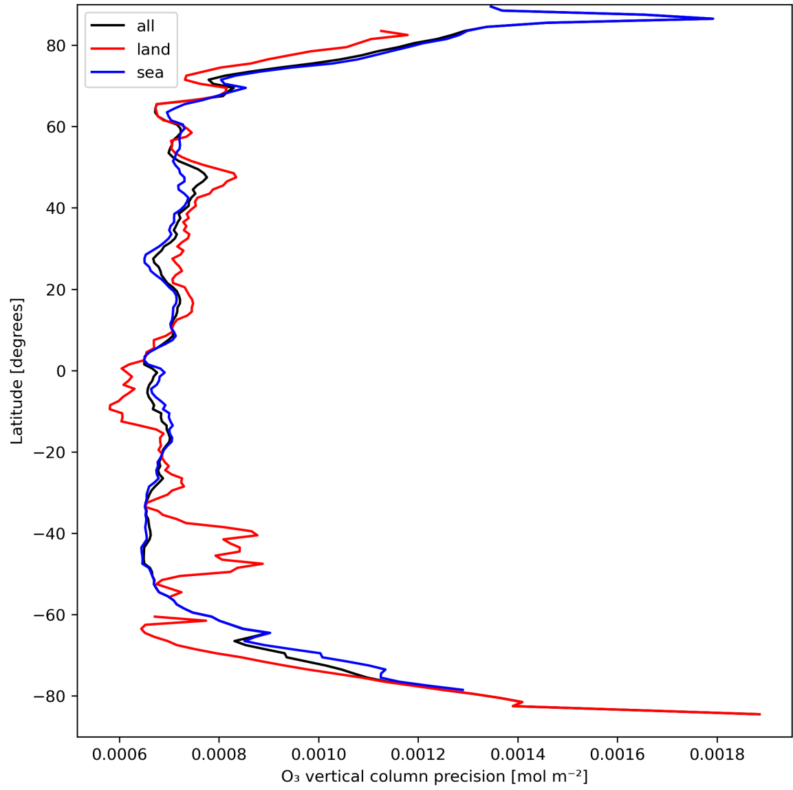
Figure 15: Zonal average of “O 3 vertical column precision” for 2024-03-31 to 2024-04-02.
