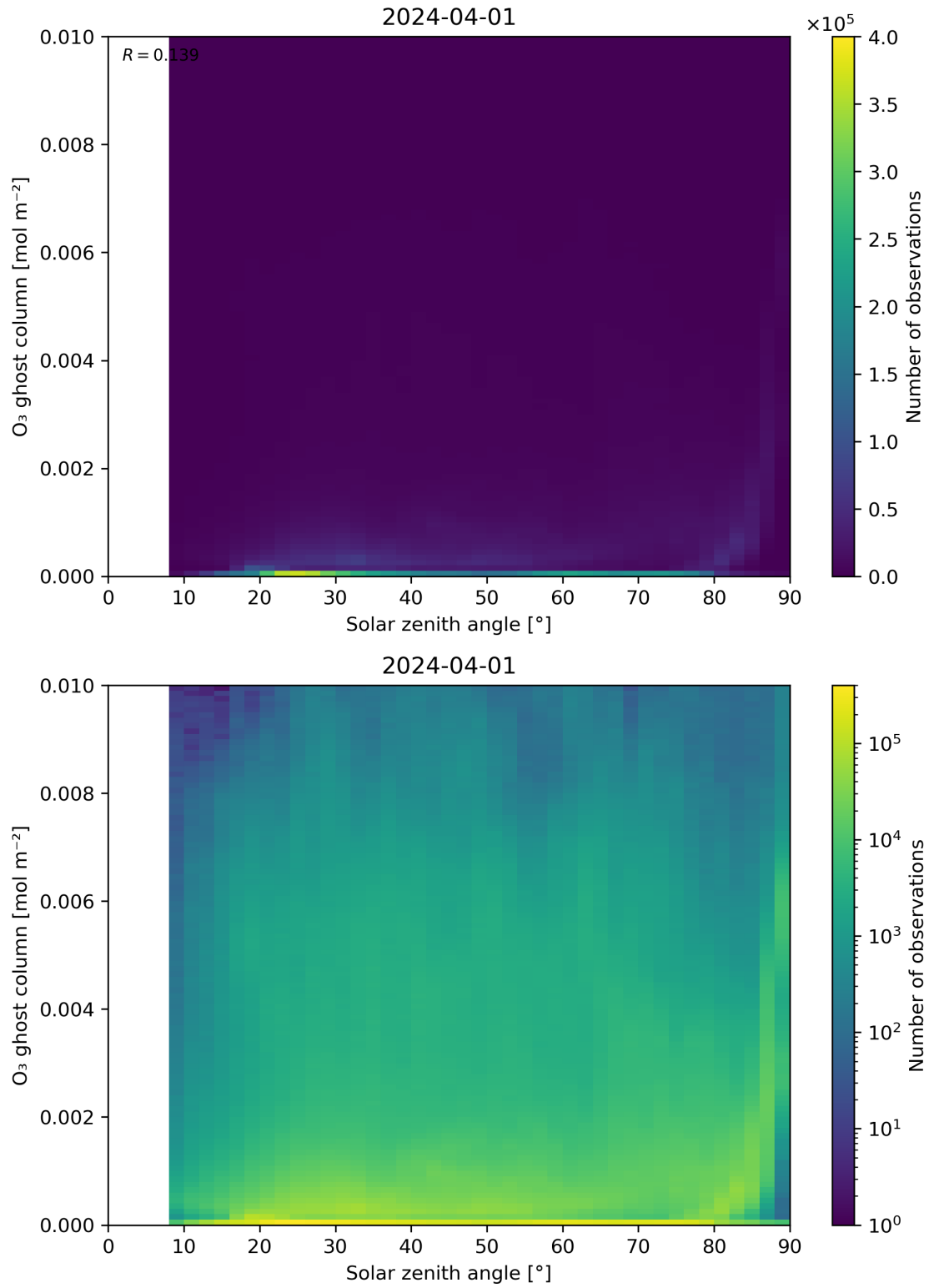
Figure 46: Scatter density plot of “Solar zenith angle” against “O 3 ghost column” for 2024-03-31 to 2024-04-02.
