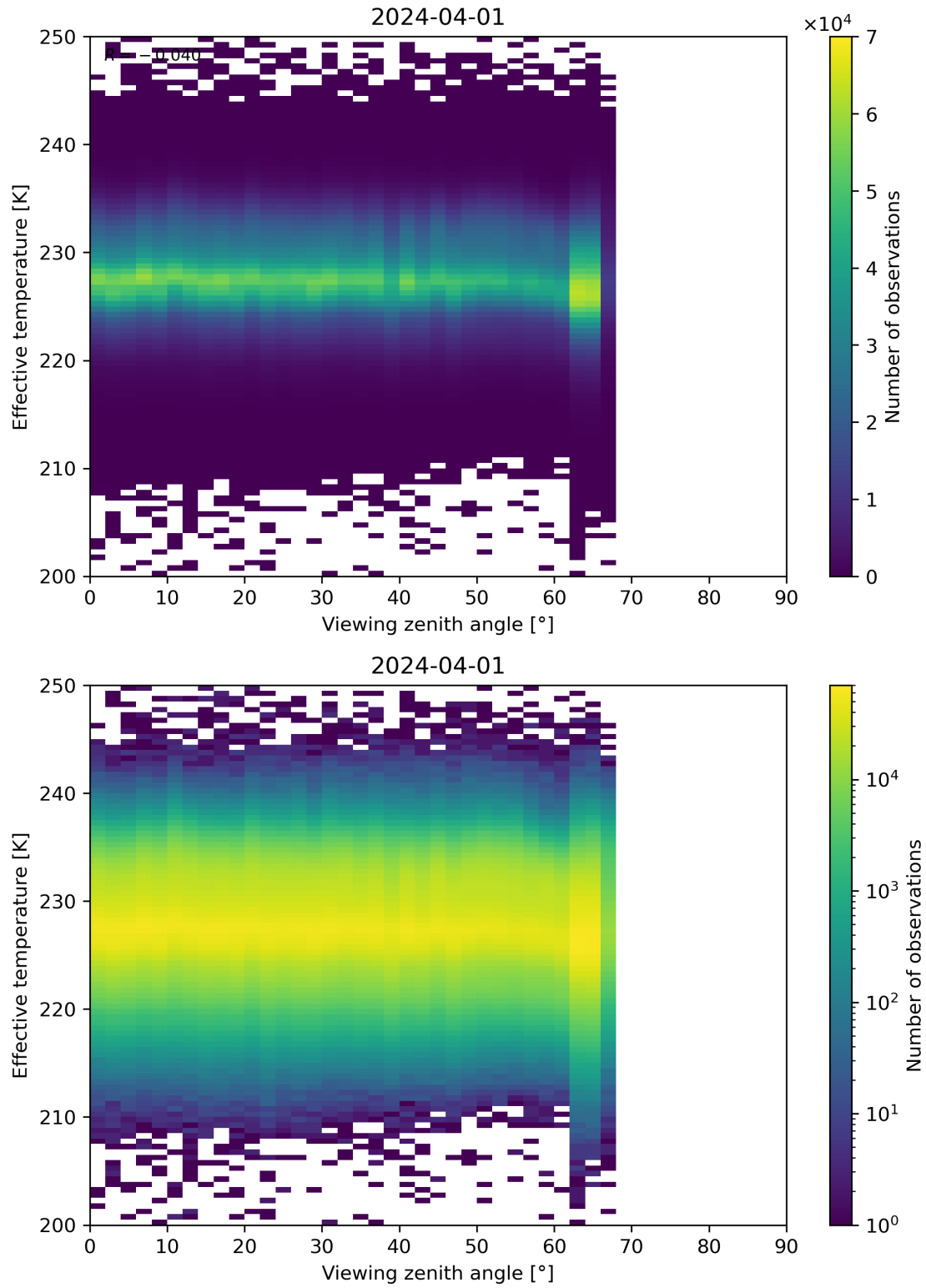
Figure 50: Scatter density plot of “Viewing zenith angle” against “Effective temperature” for 2024-03-31 to 2024-04-02.
