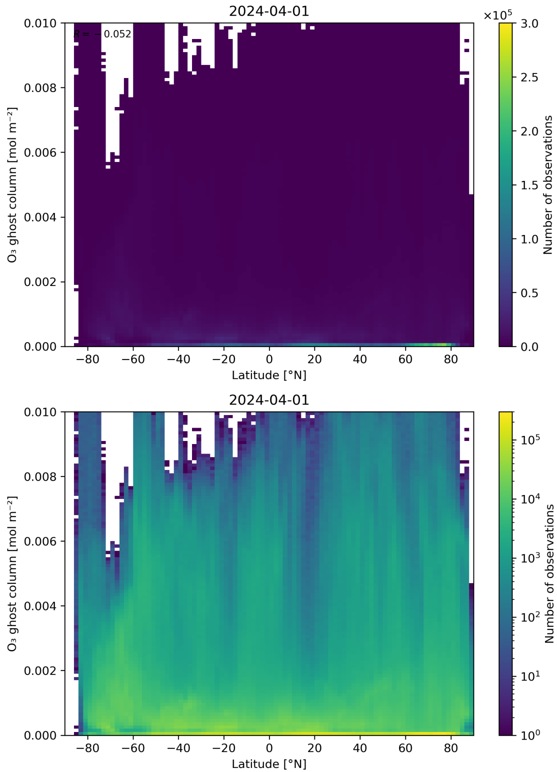
Figure 35: Scatter density plot of “Latitude” against “O 3 ghost column” for 2024-03-31 to 2024-04-02.
