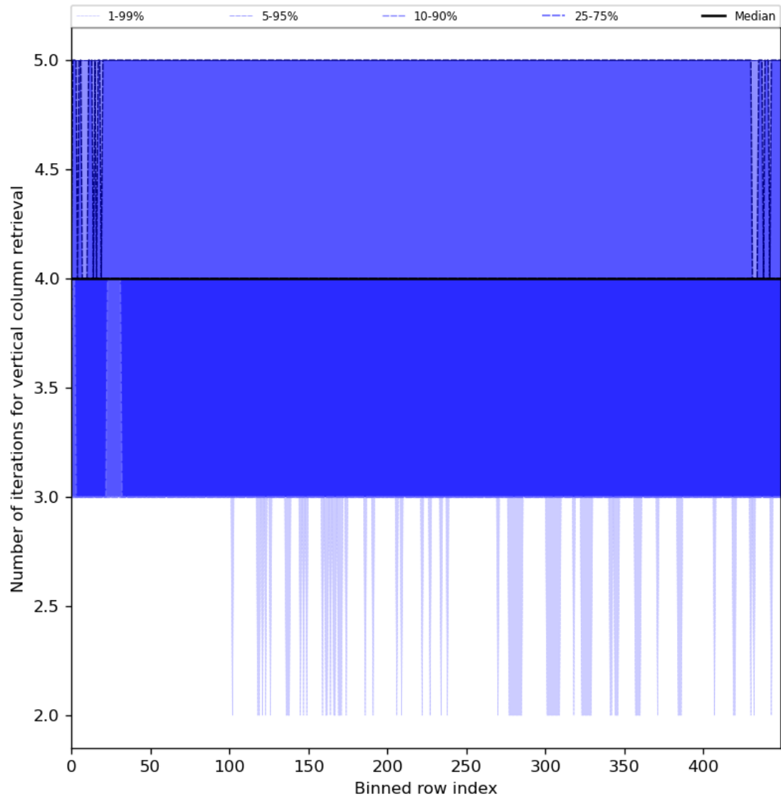
Figure 33: Along track statistics of “Number of iterations for vertical column retrieval” for 2024-03-31 to 2024-04-02
