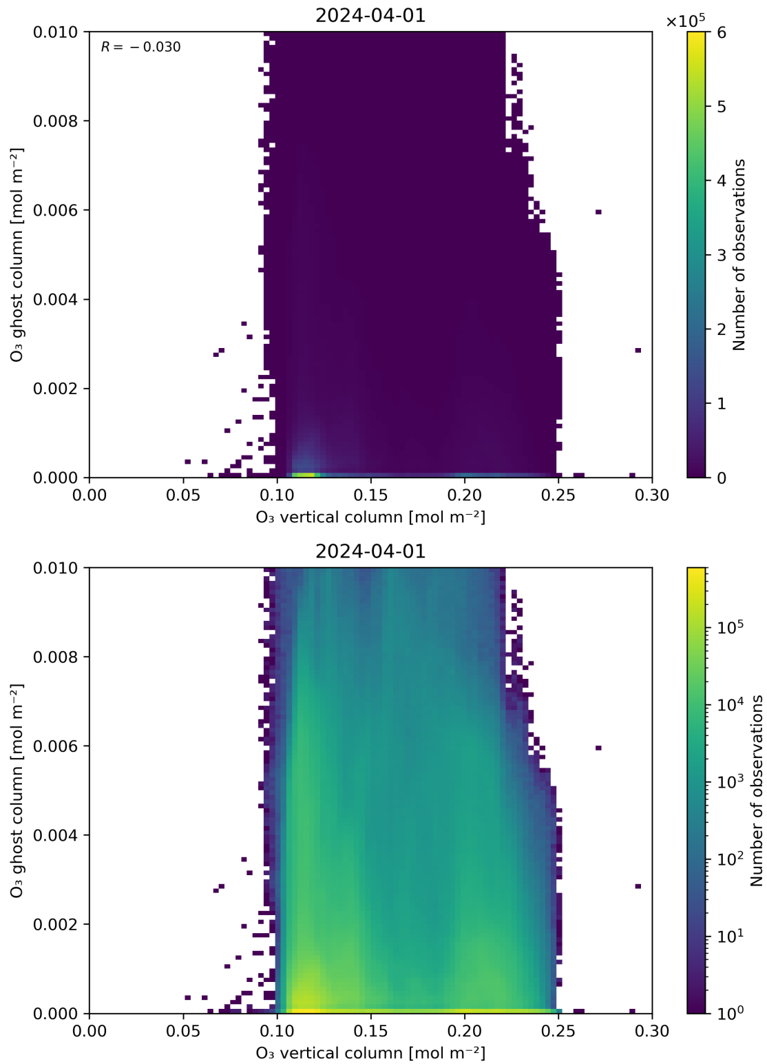
Figure 40: Scatter density plot of “O 3 vertical column” against “O 3 ghost column” for 2024-03-31 to 2024-04-02.
