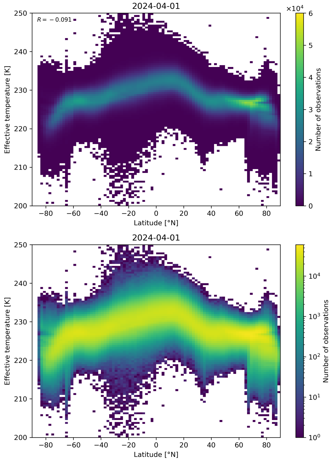
Figure 34: Scatter density plot of “Latitude” against “Effective temperature” for 2024-03-31 to 2024-04-02.
