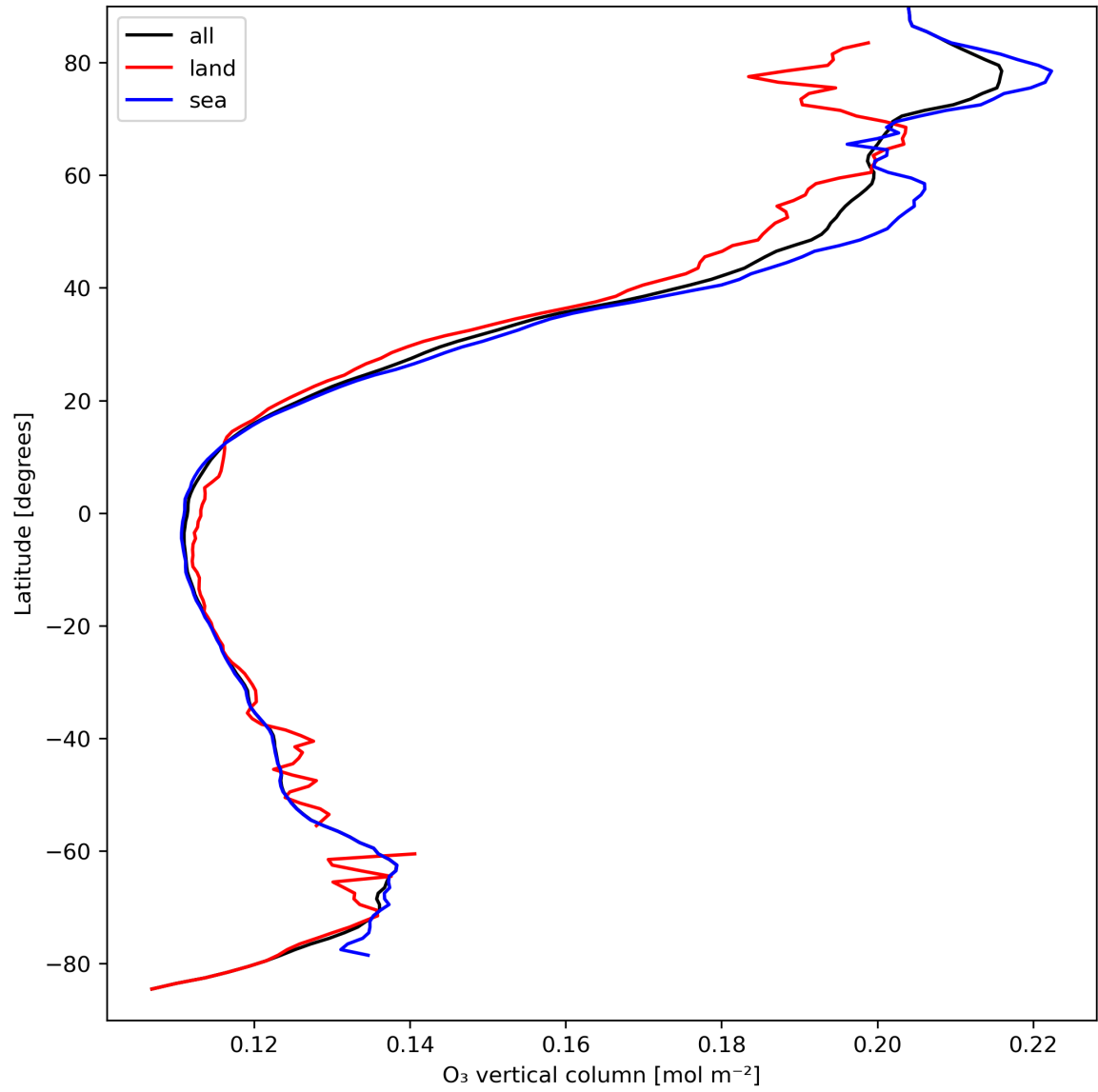
Figure 14: Zonal average of “O 3 vertical column” for 2024-03-31 to 2024-04-02.
