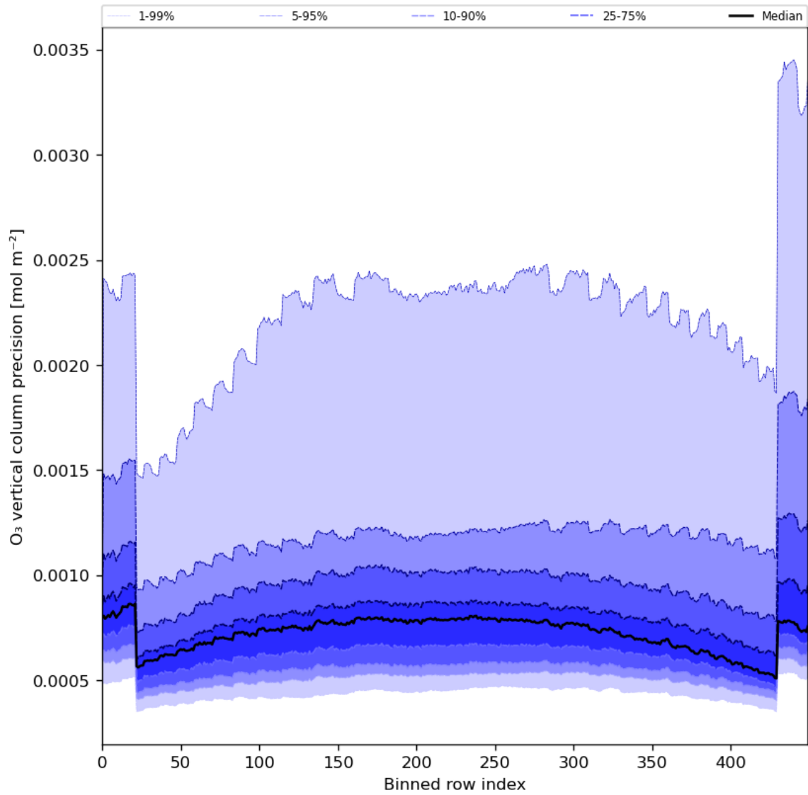
Figure 29: Along track statistics of “O 3 vertical column precision” for 2024-03-31 to 2024-04-02
