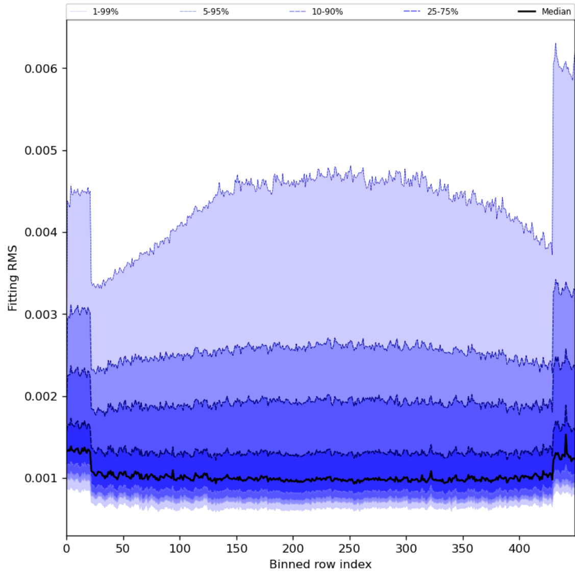
Figure 30: Along track statistics of “Fitting RMS” for 2024-03-31 to 2024-04-02
