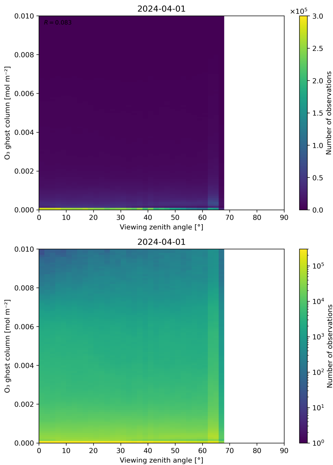
Figure 51: Scatter density plot of “Viewing zenith angle” against “O 3 ghost column” for 2024-03-31 to 2024-04-02.
