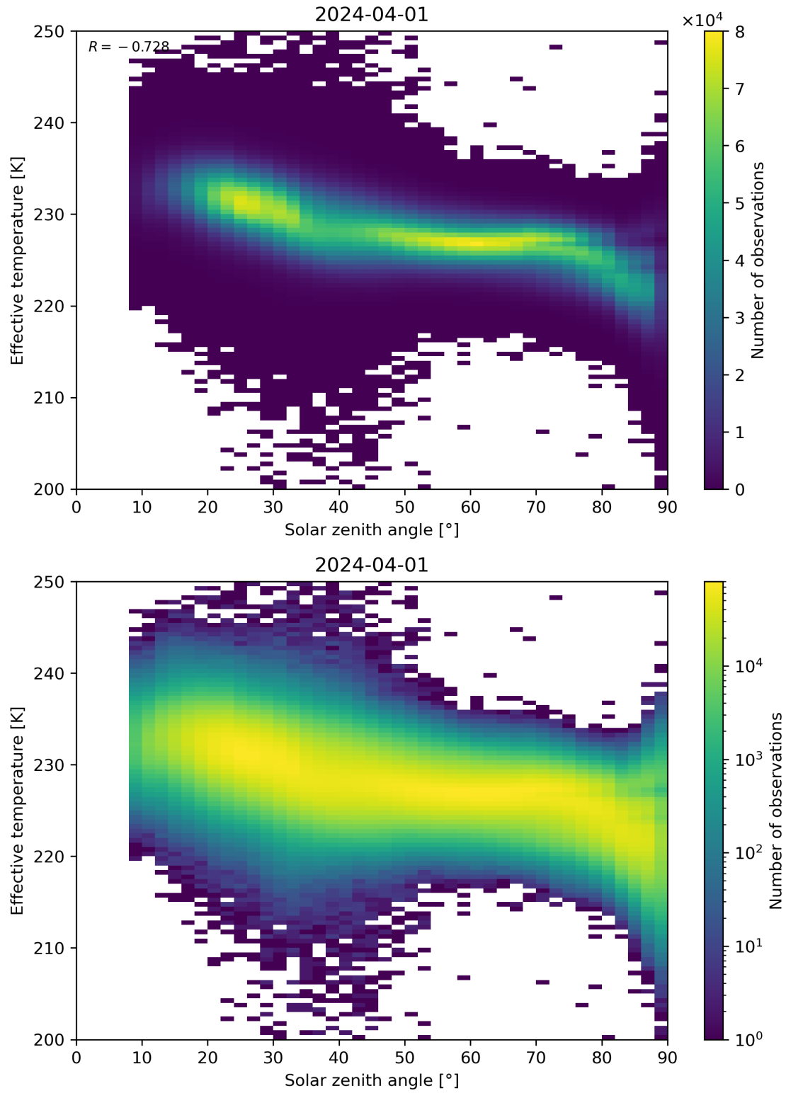
Figure 45: Scatter density plot of “Solar zenith angle” against “Effective temperature” for 2024-03-31 to 2024-04-02.
