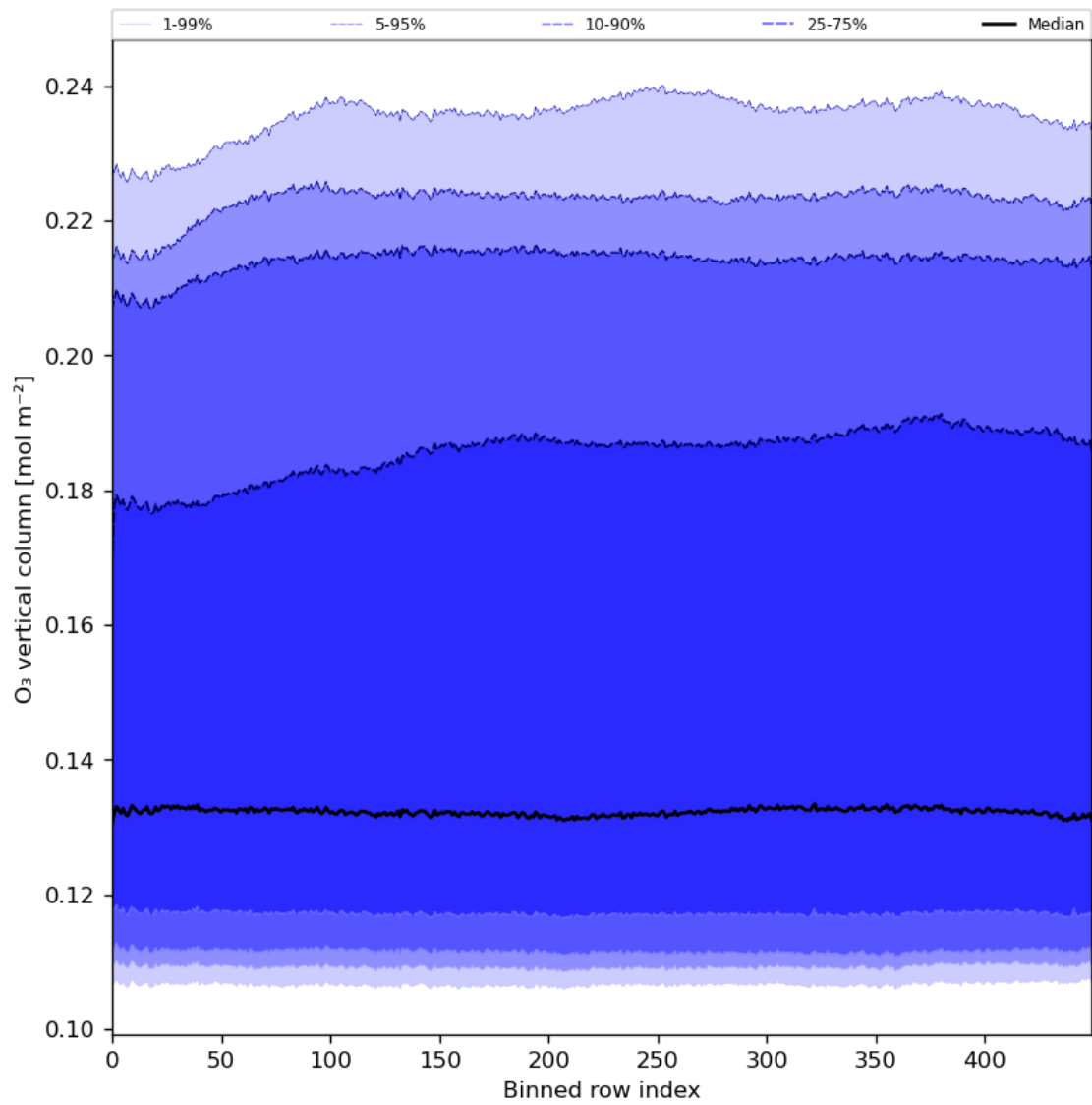
Figure 28: Along track statistics of “O 3 vertical column” for 2024-03-31 to 2024-04-02
