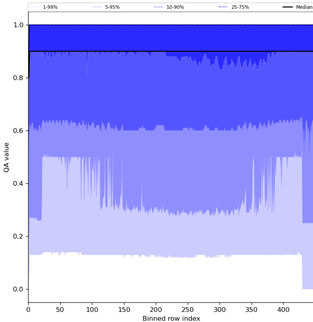
Figure 27: Along track statistics of “QA value” for 2024-03-31 to 2024-04-02
