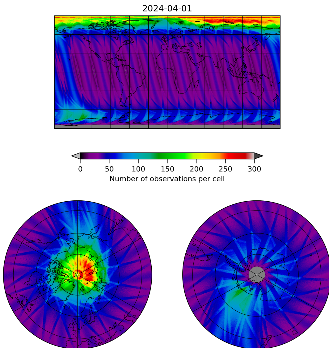
Figure 12: Map of the number of observations for 2024-03-31 to 2024-04-02
