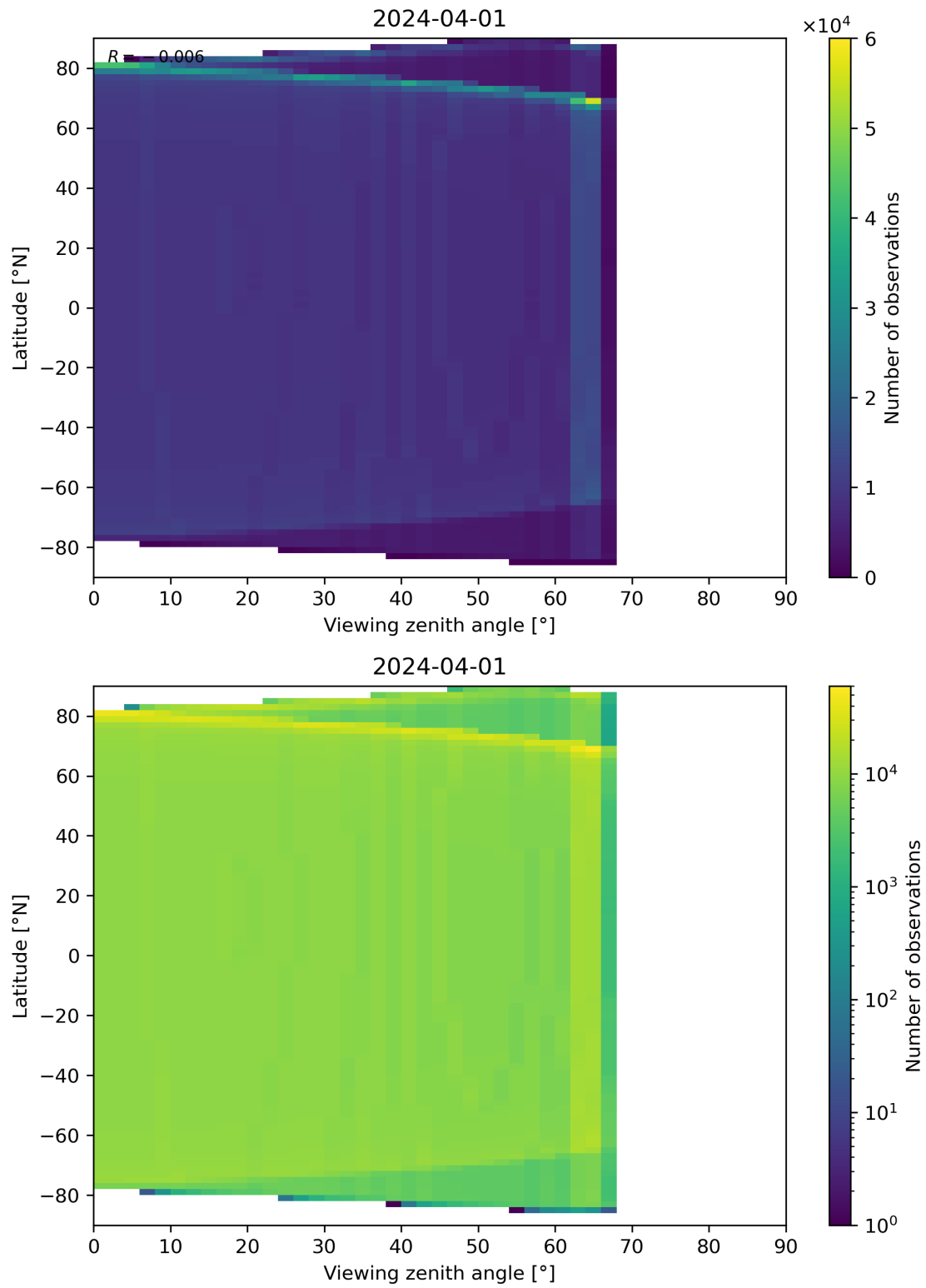
Figure 49: Scatter density plot of “Viewing zenith angle” against “Latitude” for 2024-03-31 to 2024-04-02.
