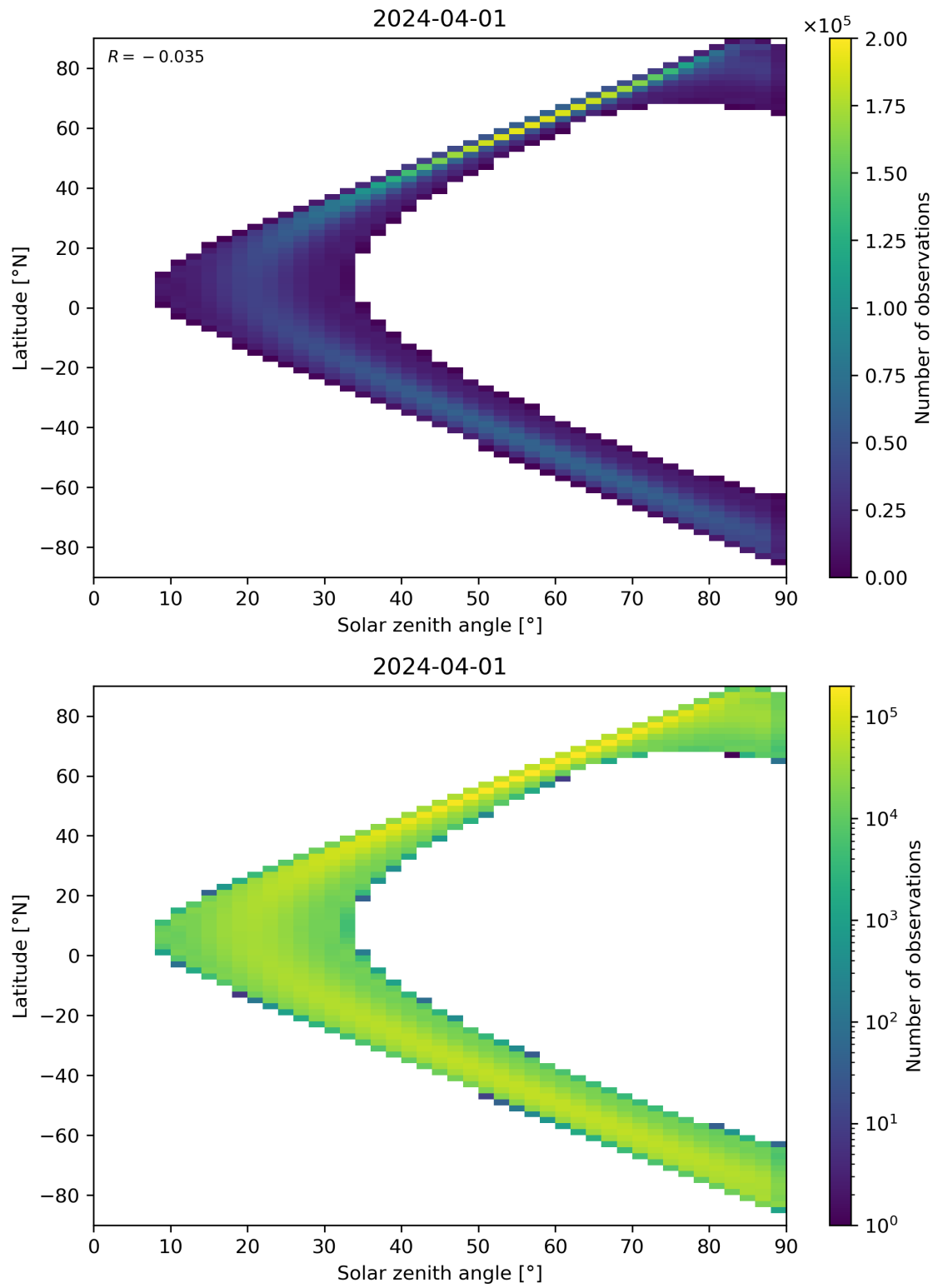
Figure 44: Scatter density plot of “Solar zenith angle” against “Latitude” for 2024-03-31 to 2024-04-02.
