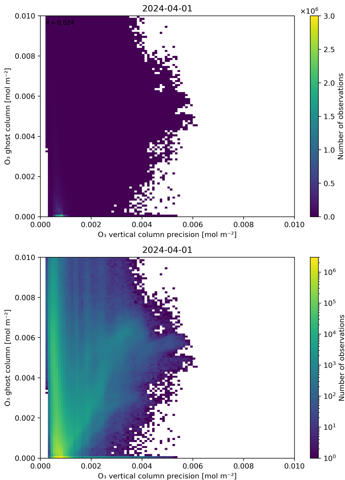
Figure 43: Scatter density plot of “ O_3 vertical column precision” against “ O_3 ghost column” for 2024-03-31 to 2024-04-02.
