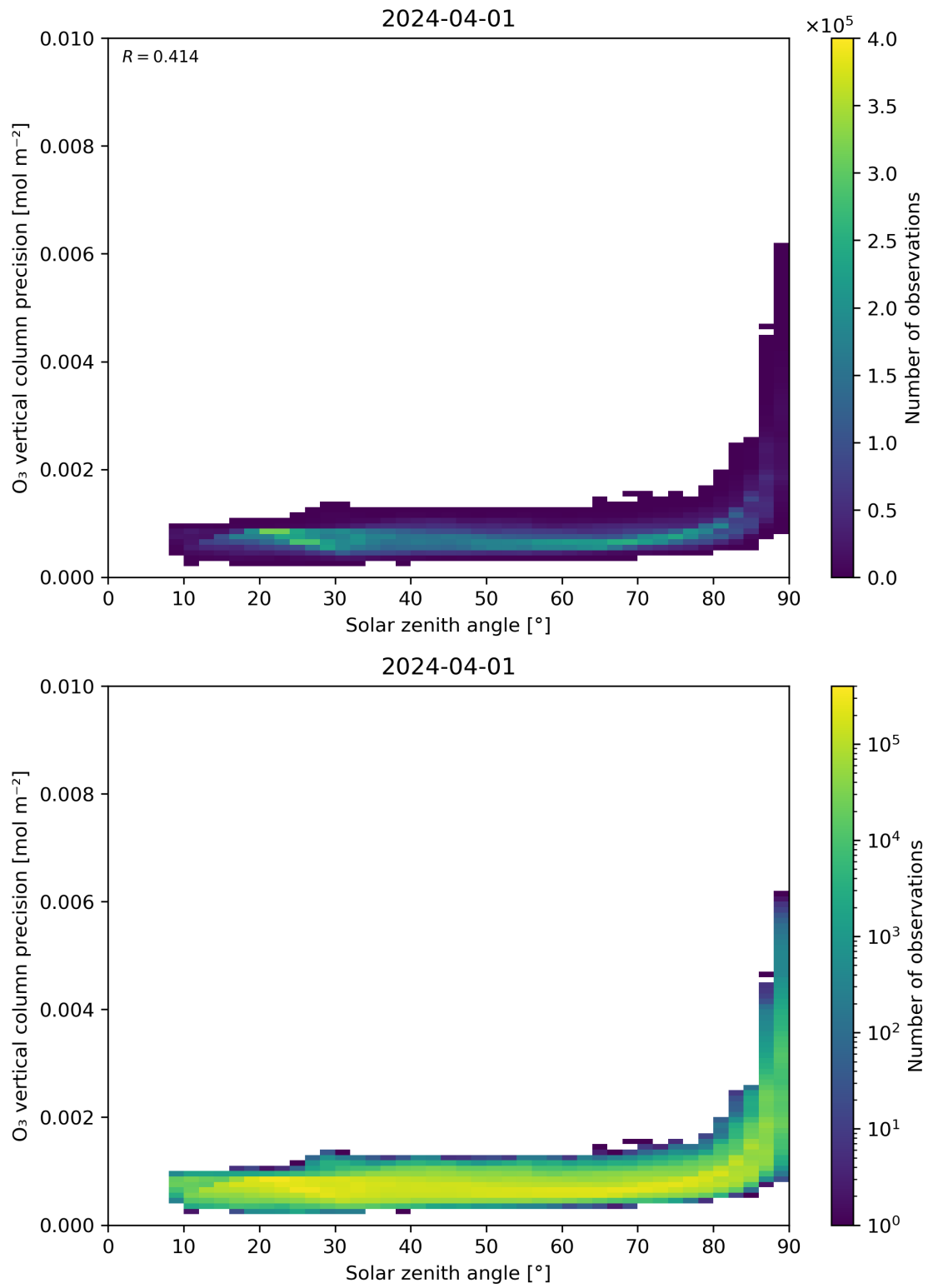
Figure 48: Scatter density plot of “Solar zenith angle” against “O 3 vertical column precision” for 2024-03-31 to 2024-04-02.
