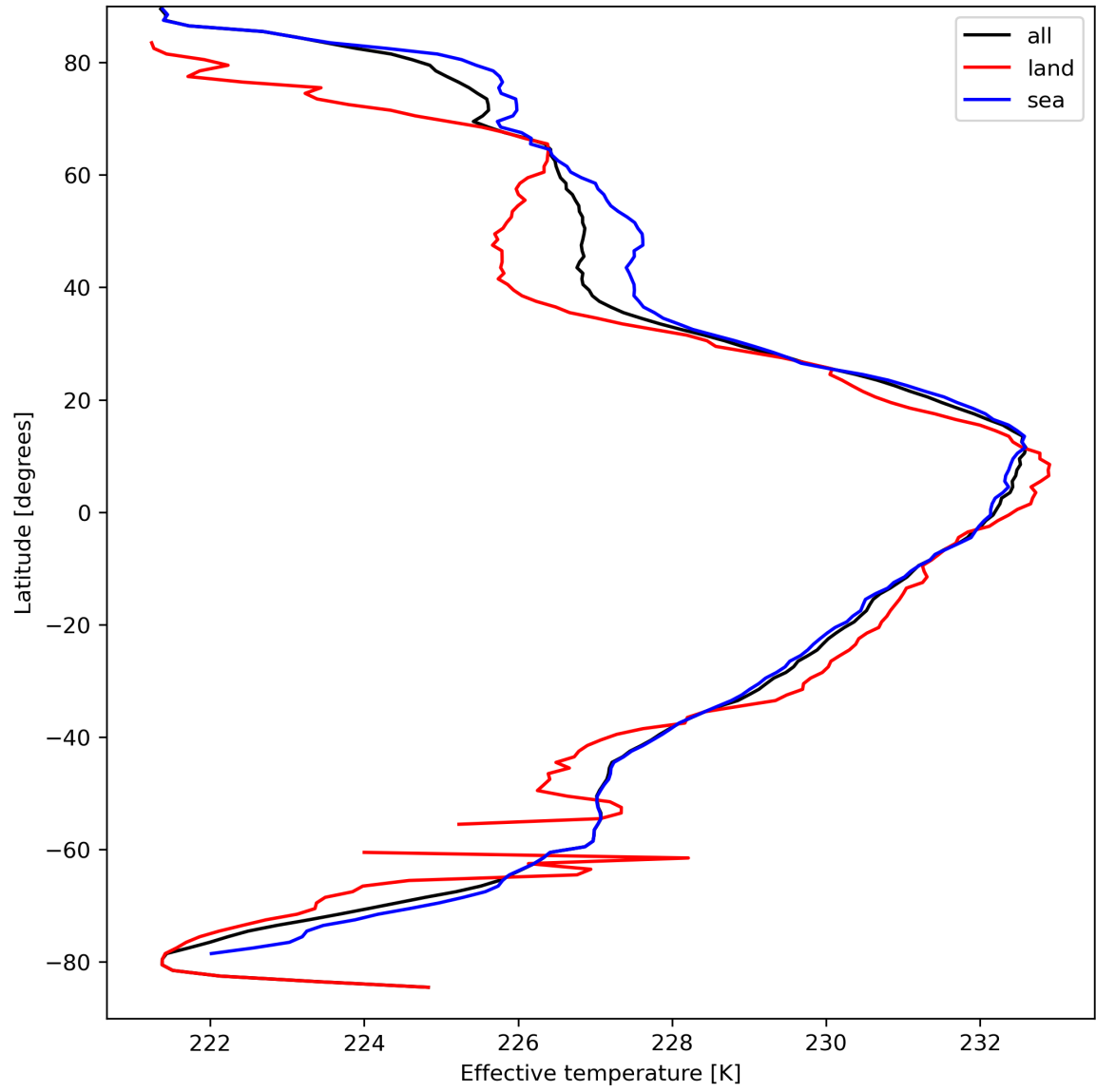
Figure 17: Zonal average of “Effective temperature” for 2024-03-31 to 2024-04-02.
