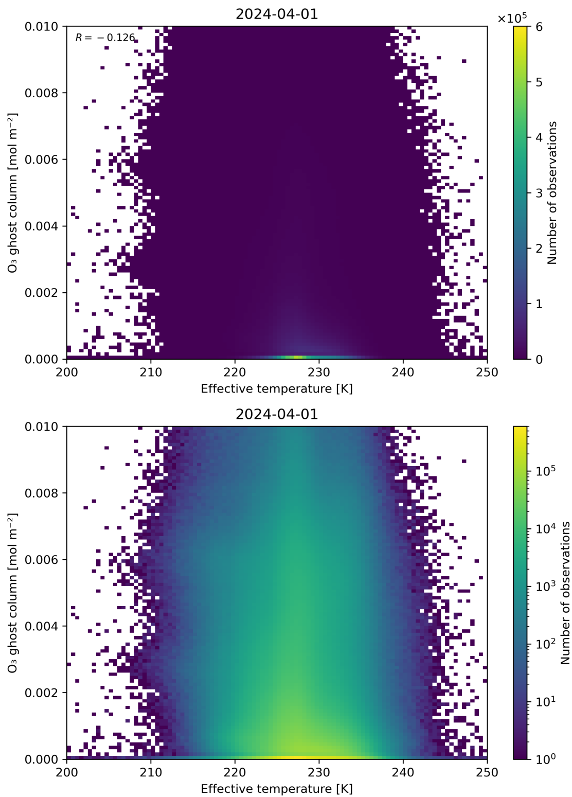
Figure 38: Scatter density plot of “Effective temperature” against “O 3 ghost column” for 2024-03-31 to 2024-04-02.
