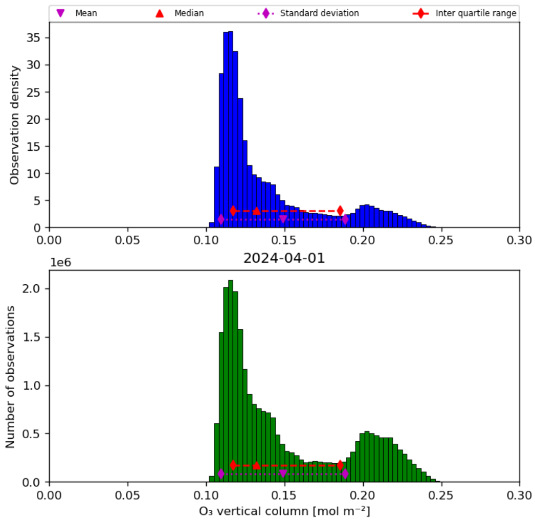
Figure 21: Histogram of “O 3 vertical column” for 2024-03-31 to 2024-04-02
