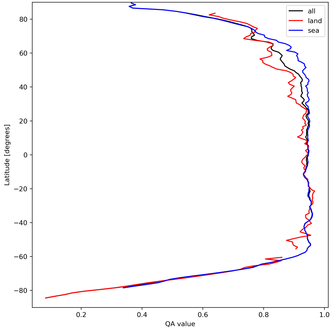
Figure 13: Zonal average of “QA value” for 2024-03-31 to 2024-04-02.
