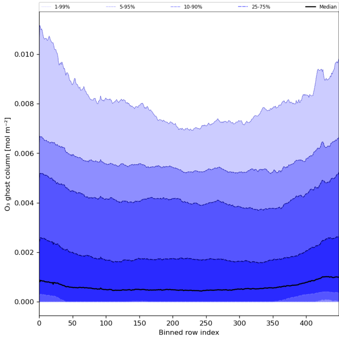
Figure 32: Along track statistics of “O 3 ghost column” for 2024-03-31 to 2024-04-02
