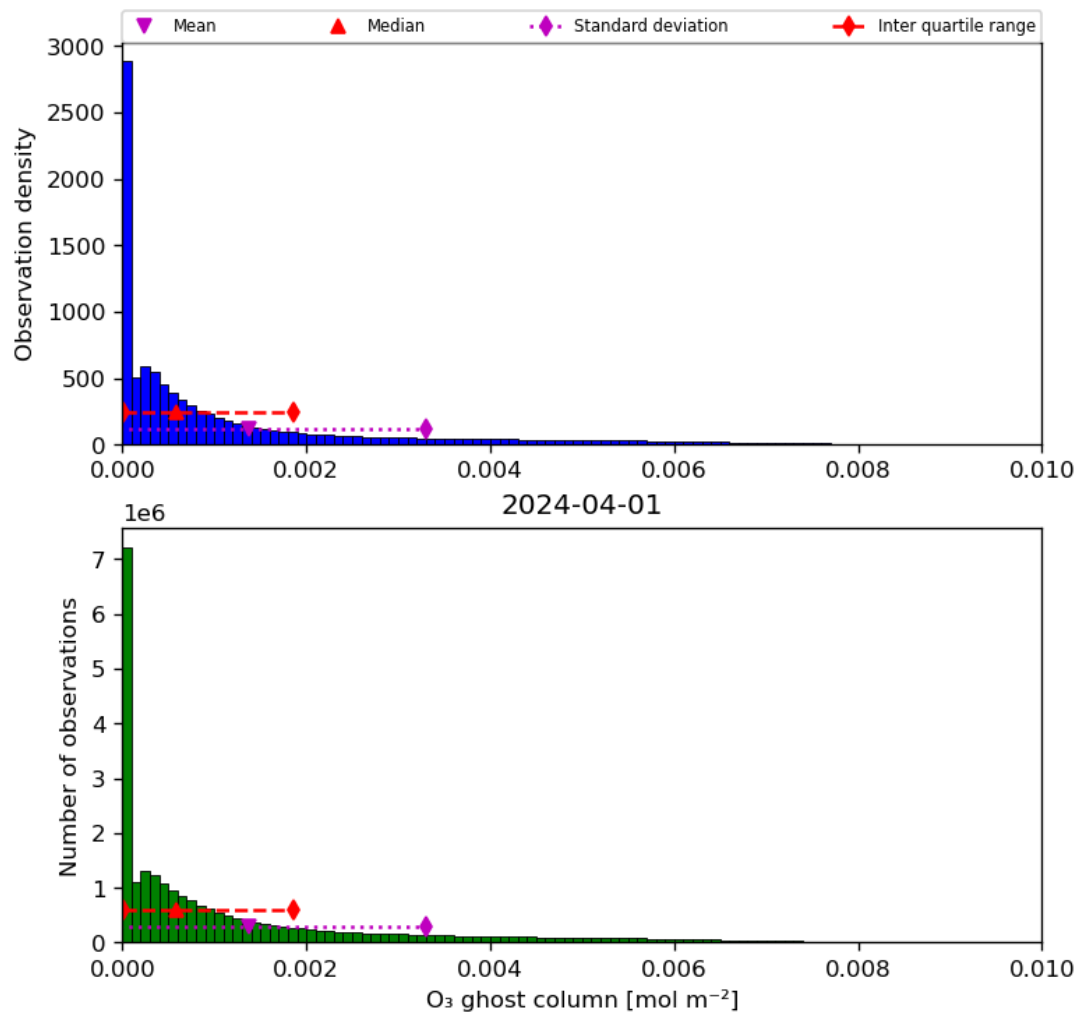
Figure 25: Histogram of “O 3 ghost column” for 2024-03-31 to 2024-04-02
