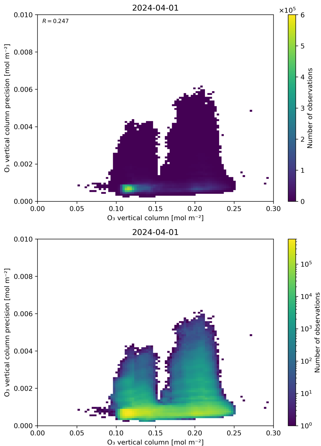
Figure 41: Scatter density plot of “O 3 vertical column” against “O 3 vertical column precision” for 2024-03-31 to 2024-04-02.
