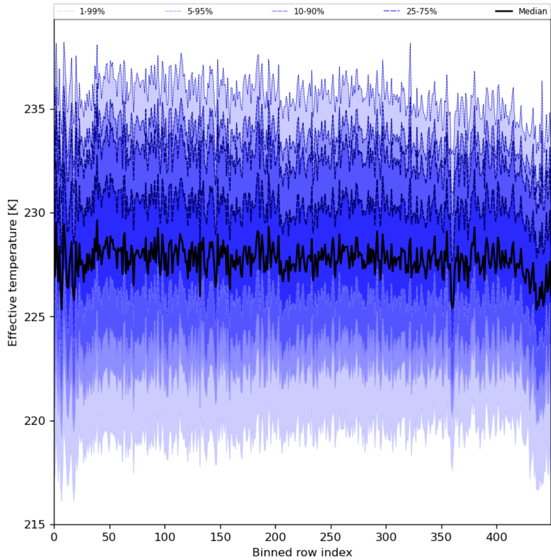
Figure 31: Along track statistics of “Effective temperature” for 2024-03-31 to 2024-04-02
