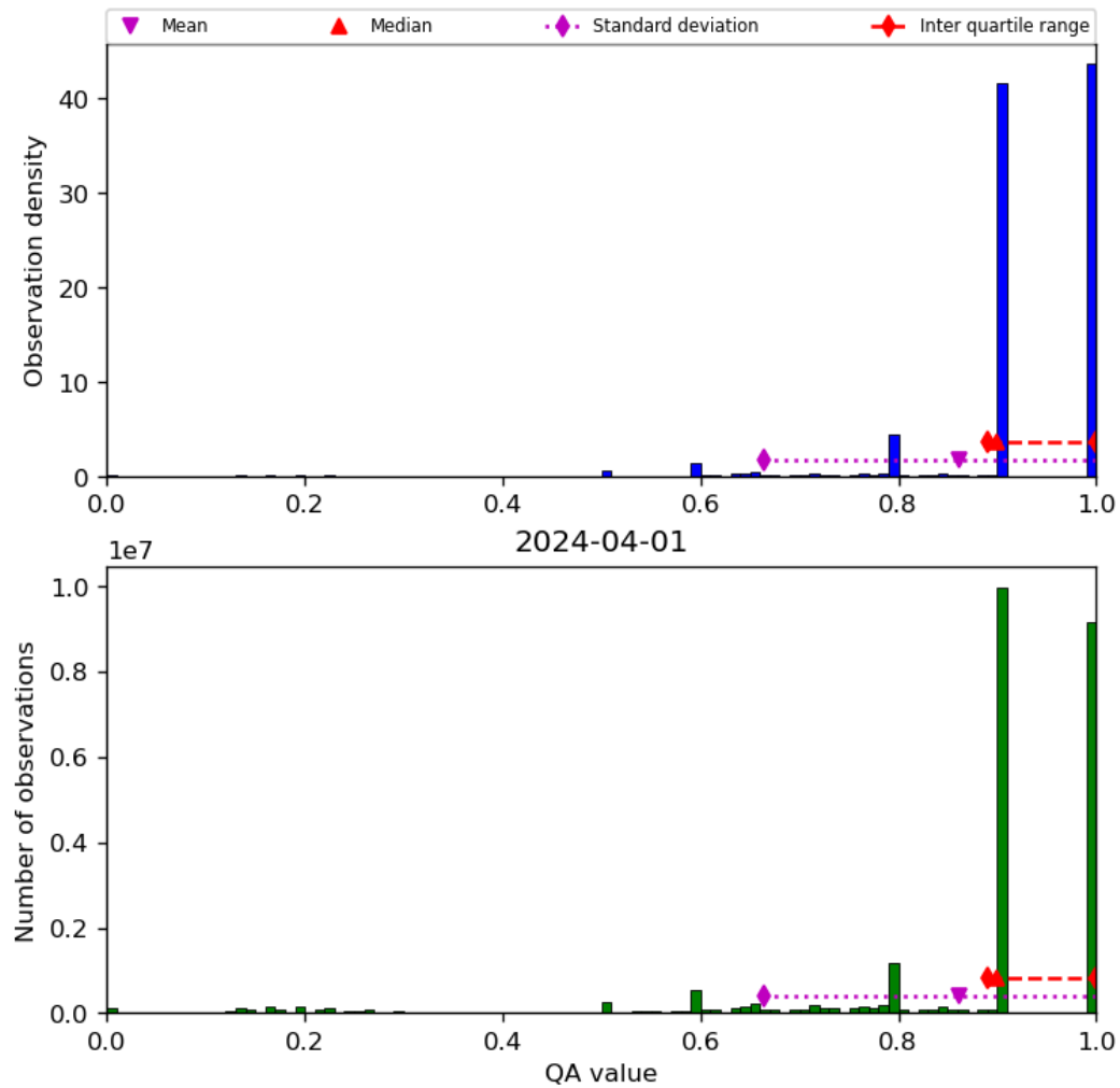
Figure 20: Histogram of “QA value” for 2024-03-31 to 2024-04-02
