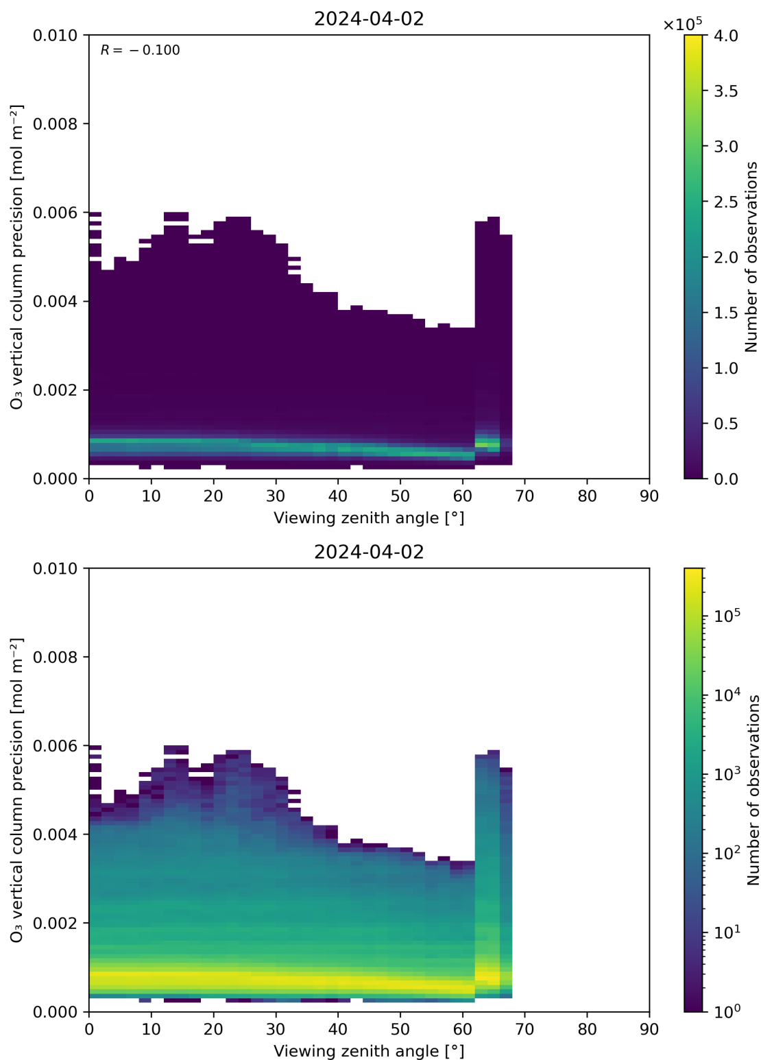
Figure 53: Scatter density plot of “Viewing zenith angle” against “O 3 vertical column precision” for 2024-04-01 to 2024-04-03.
