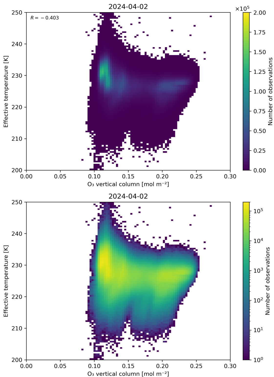
Figure 39: Scatter density plot of “O 3 vertical column” against “Effective temperature” for 2024-04-01 to 2024-04-03.
