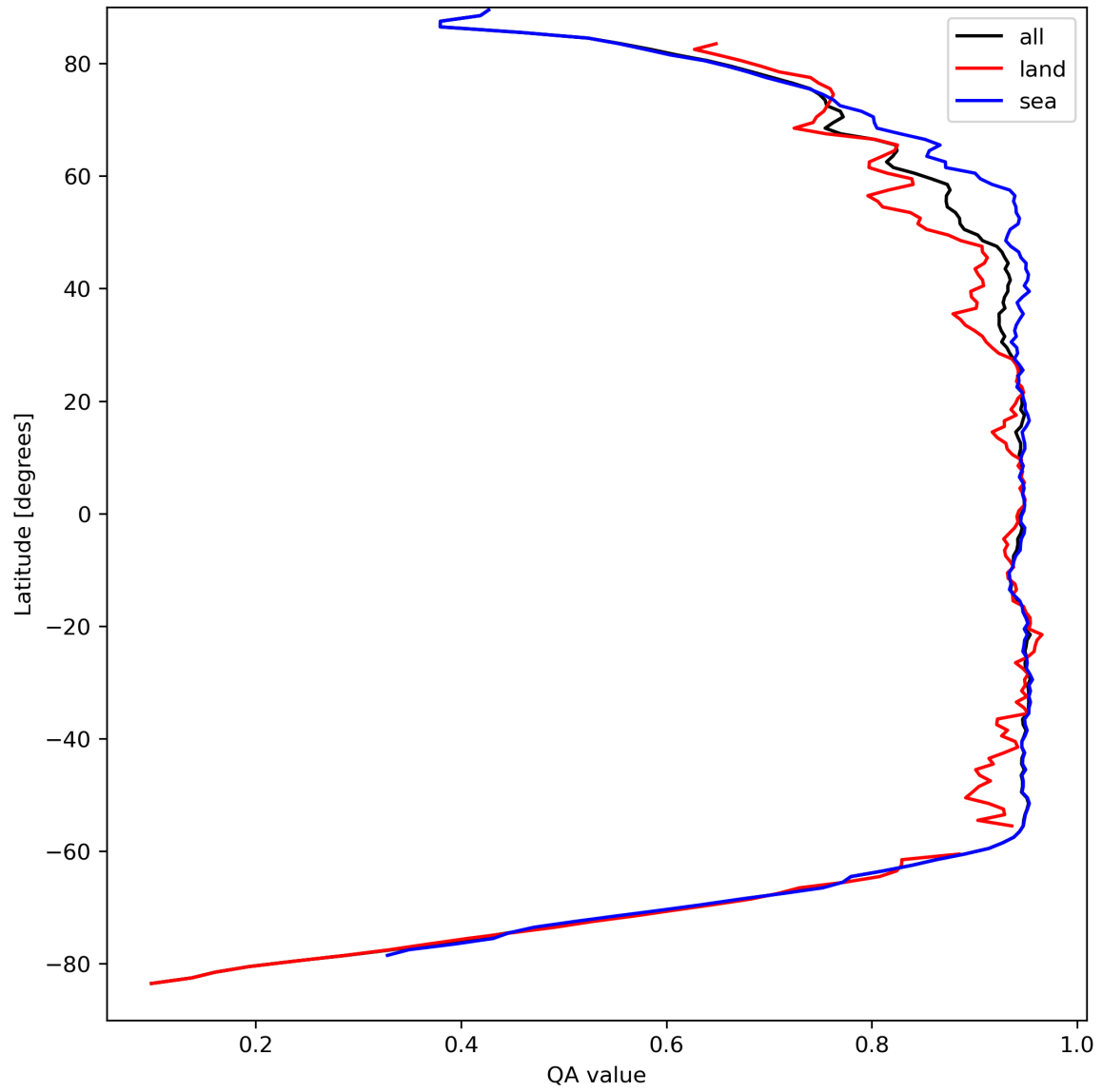
Figure 13: Zonal average of “QA value” for 2024-04-01 to 2024-04-03.
