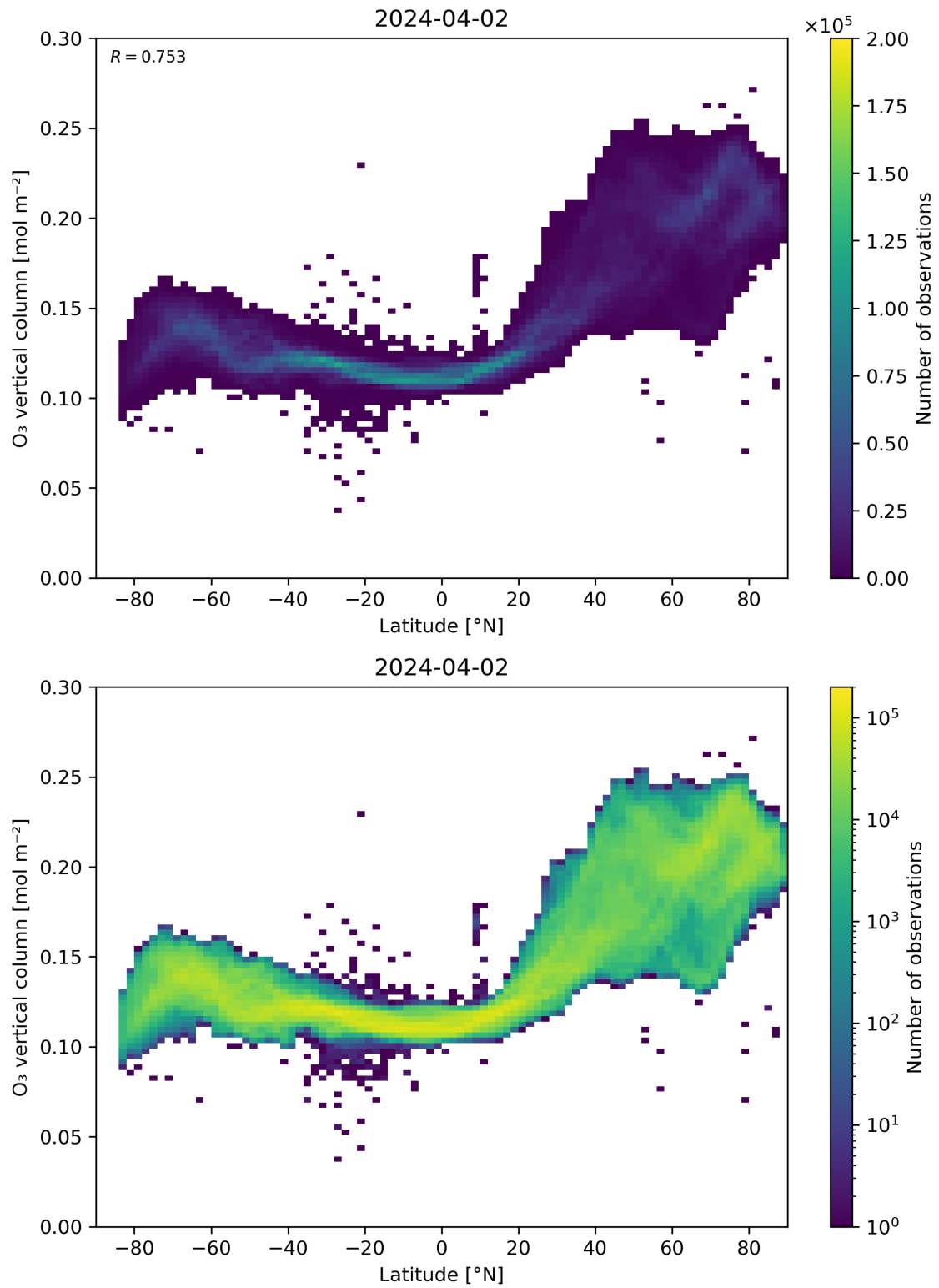
Figure 36: Scatter density plot of “Latitude” against “O 3 vertical column” for 2024-04-01 to 2024-04-03.
