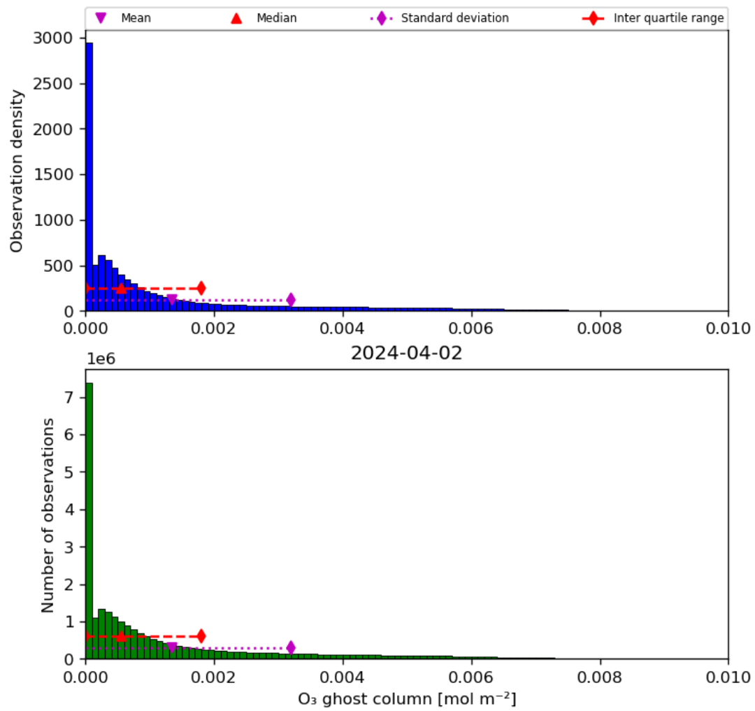
Figure 25: Histogram of “O 3 ghost column” for 2024-04-01 to 2024-04-03
