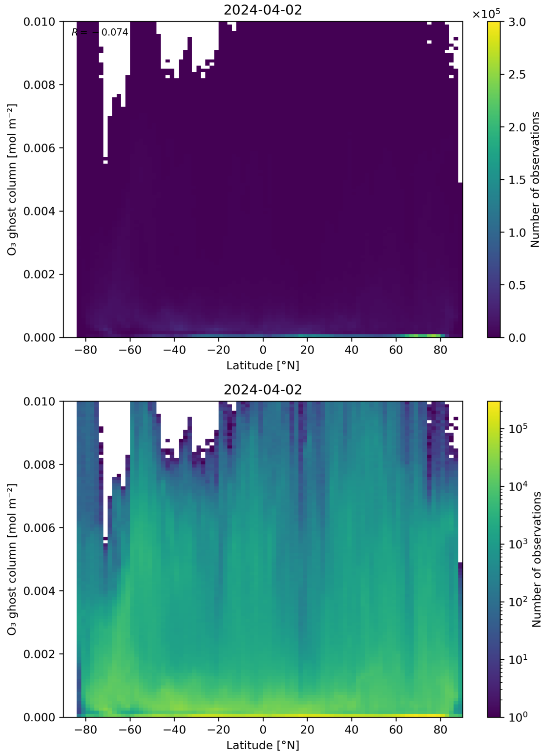
Figure 35: Scatter density plot of “Latitude” against “O 3 ghost column” for 2024-04-01 to 2024-04-03.
