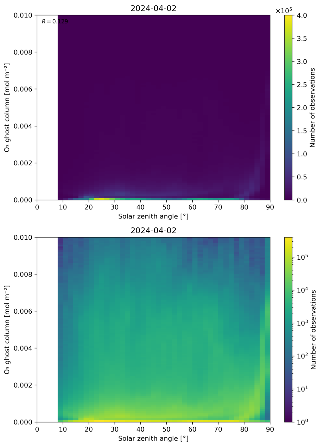
Figure 46: Scatter density plot of “Solar zenith angle” against “O 3 ghost column” for 2024-04-01 to 2024-04-03.
