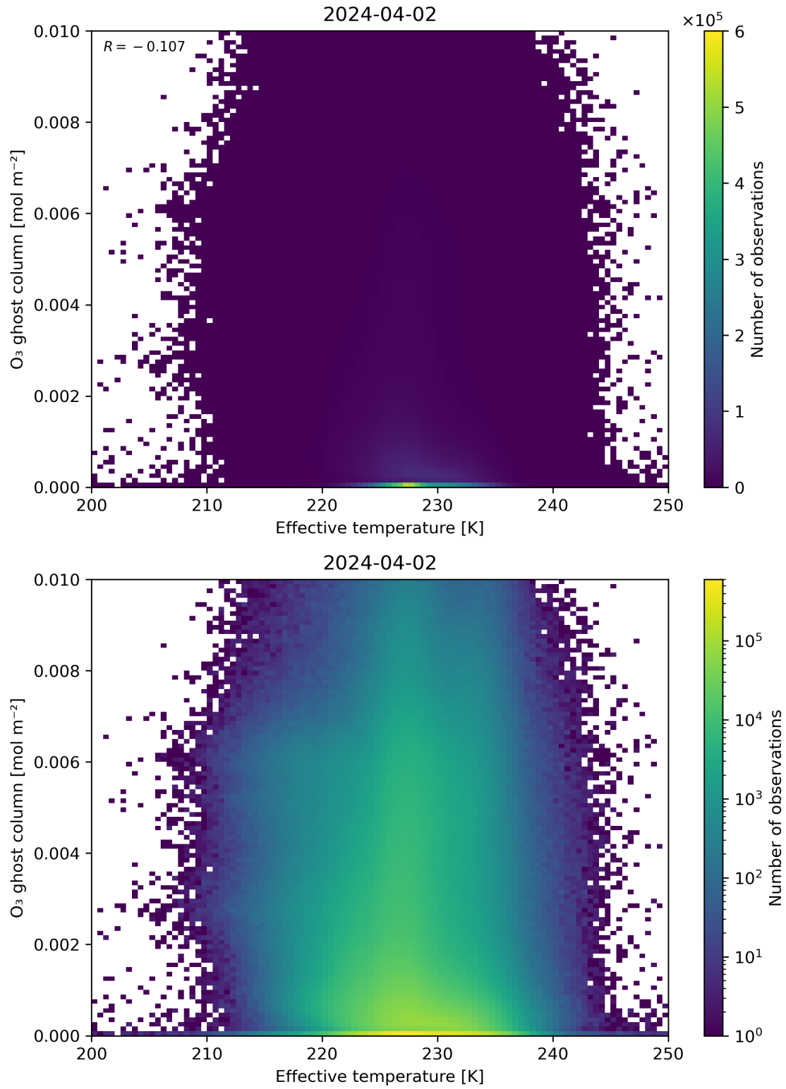
Figure 38: Scatter density plot of “Effective temperature” against “O 3 ghost column” for 2024-04-01 to 2024-04-03.
