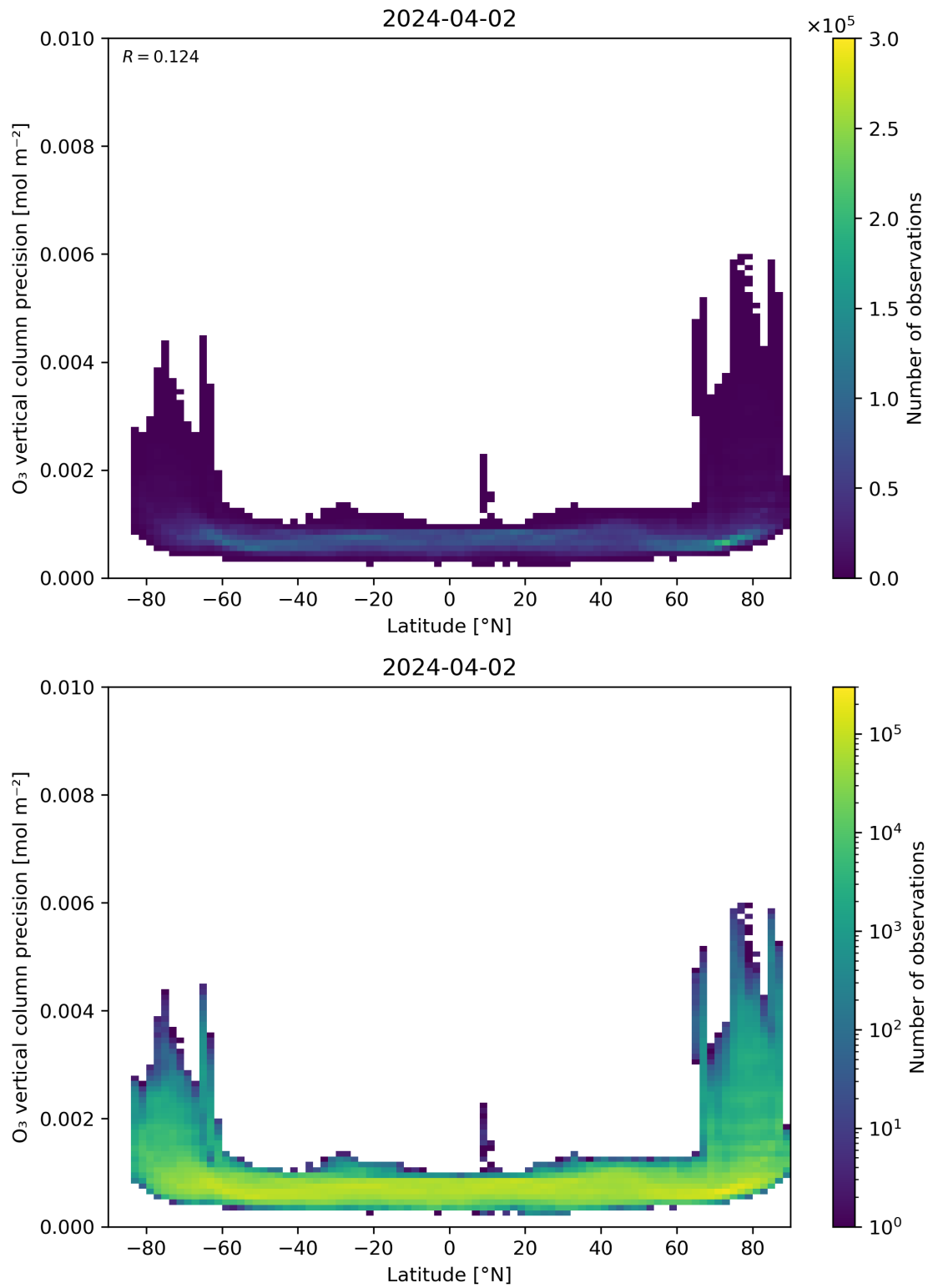
Figure 37: Scatter density plot of “Latitude” against “O 3 vertical column precision” for 2024-04-01 to 2024-04-03.
