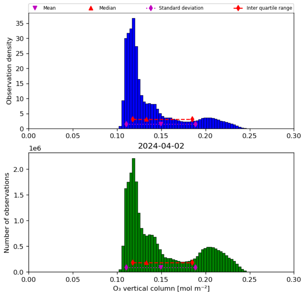
Figure 21: Histogram of “O 3 vertical column” for 2024-04-01 to 2024-04-03
