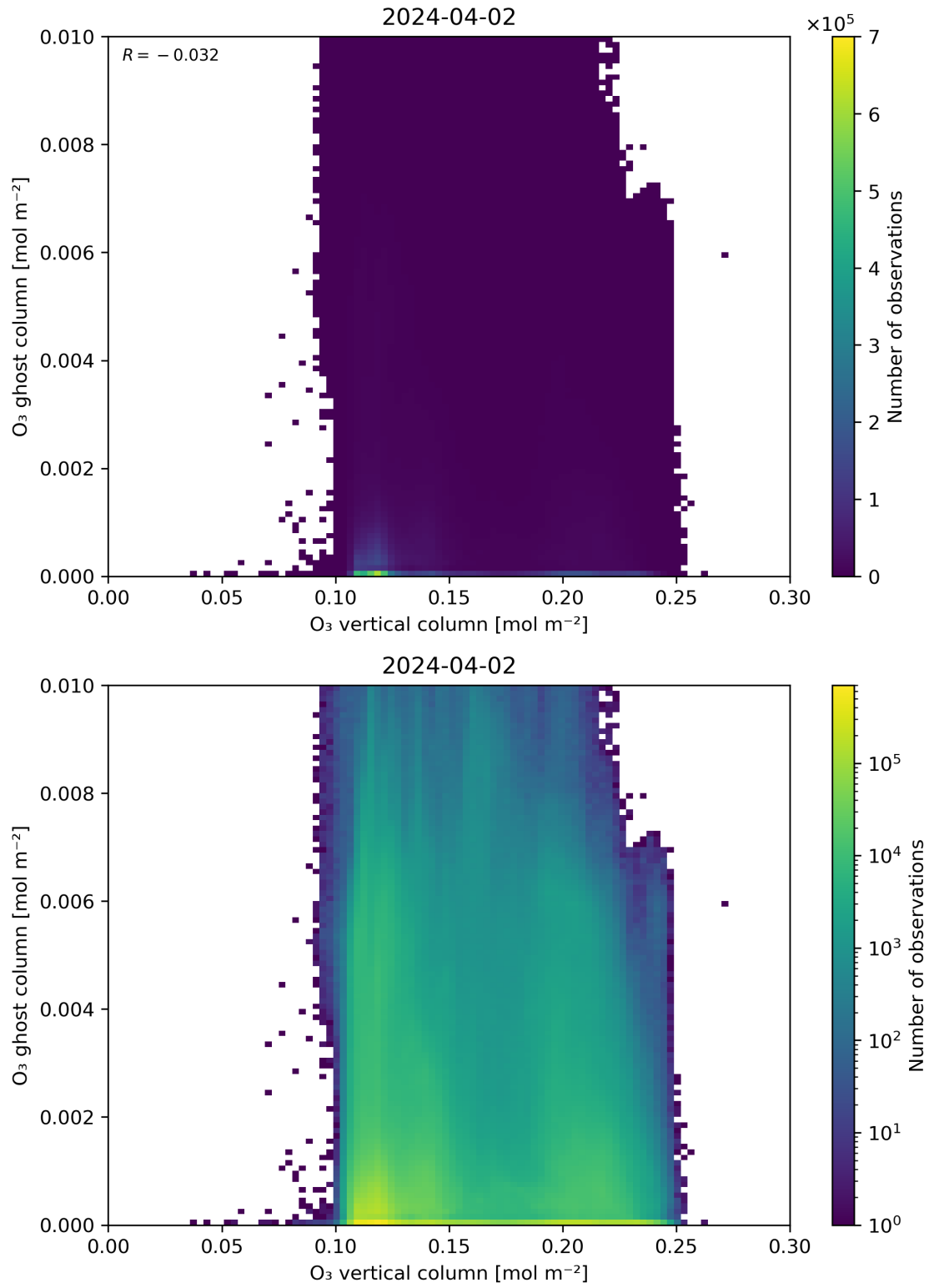
Figure 40: Scatter density plot of “O 3 vertical column” against “O 3 ghost column” for 2024-04-01 to 2024-04-03.
