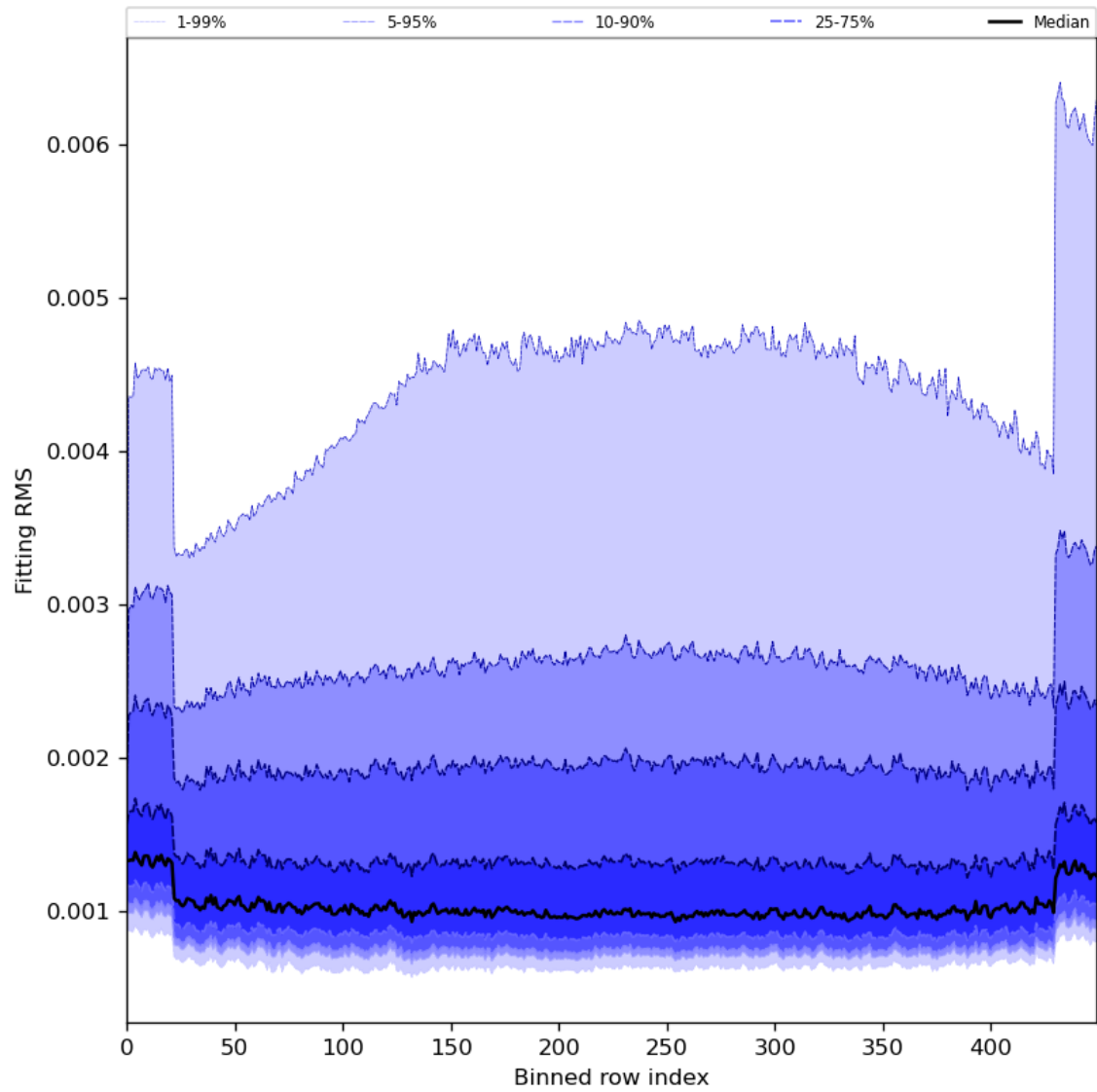
Figure 30: Along track statistics of “Fitting RMS” for 2024-04-01 to 2024-04-03
