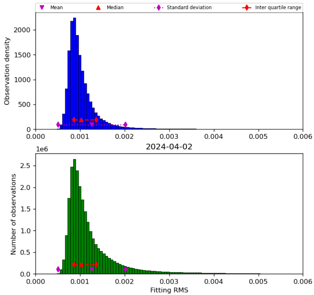
Figure 23: Histogram of “Fitting RMS” for 2024-04-01 to 2024-04-03
