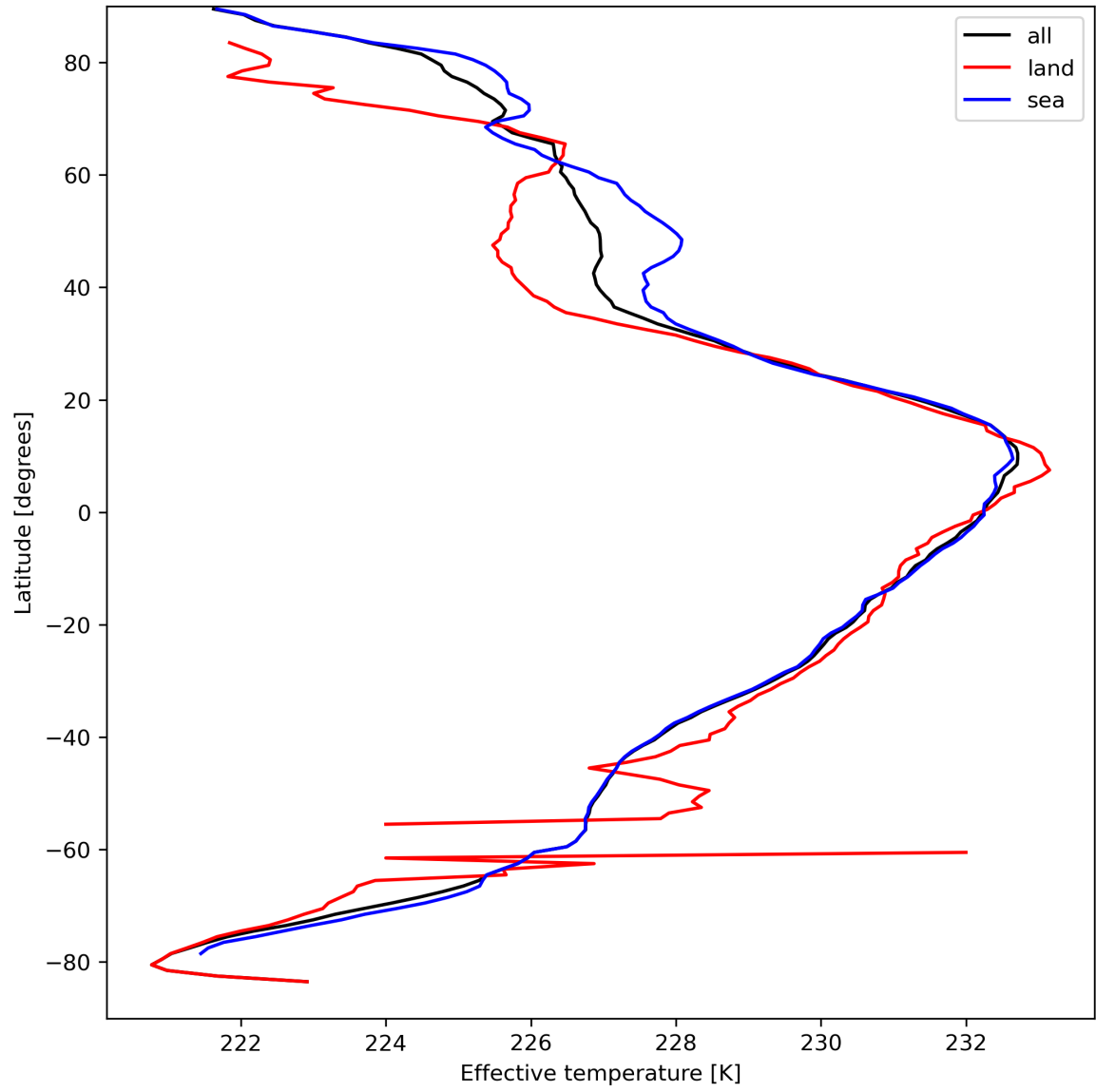
Figure 17: Zonal average of “Effective temperature” for 2024-04-01 to 2024-04-03.
