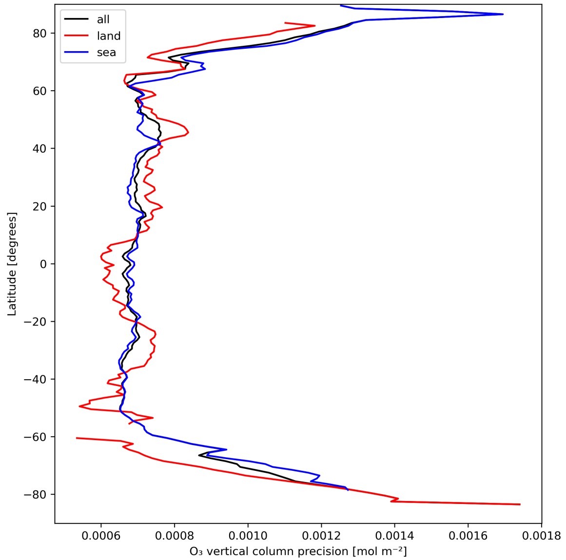
Figure 15: Zonal average of "O 3 vertical column precision" for 2024-04-01 to 2024-04-03.
