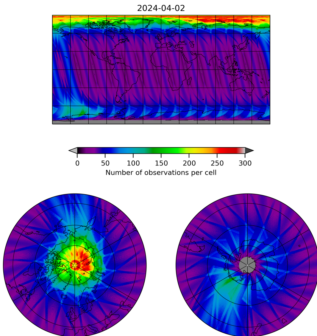
Figure 12: Map of the number of observations for 2024-04-01 to 2024-04-03
