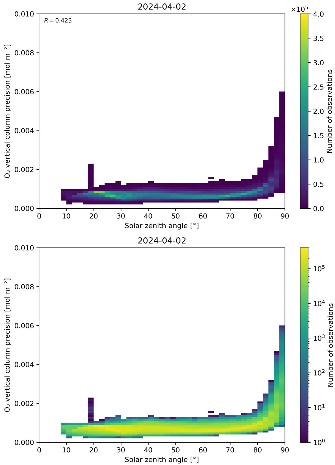
Figure 48: Scatter density plot of “Solar zenith angle” against “O 3 vertical column precision” for 2024-04-01 to 2024-04-03.
