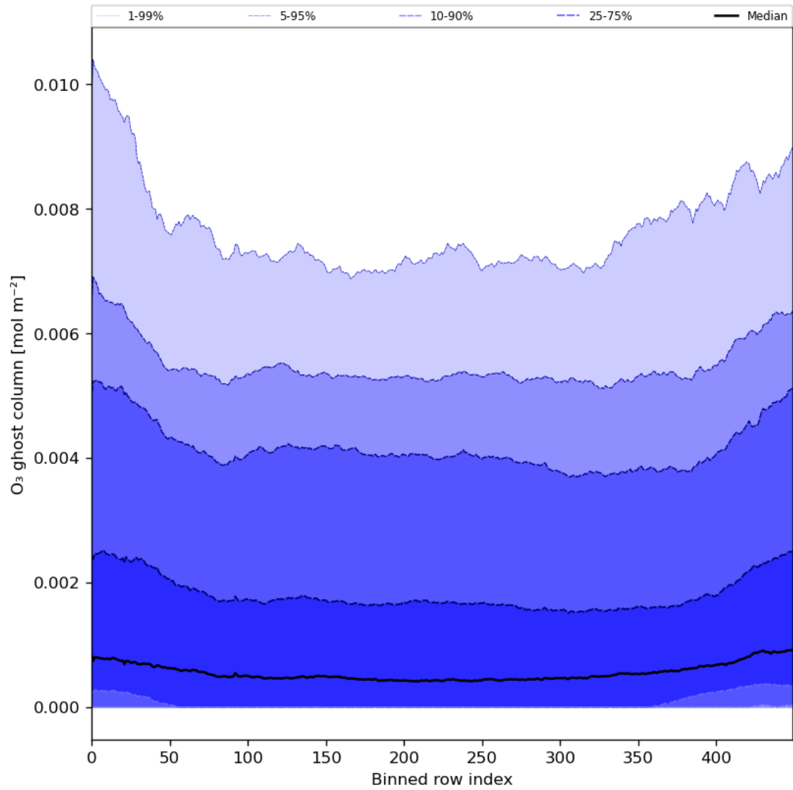
Figure 32: Along track statistics of “O 3 ghost column” for 2024-04-01 to 2024-04-03
