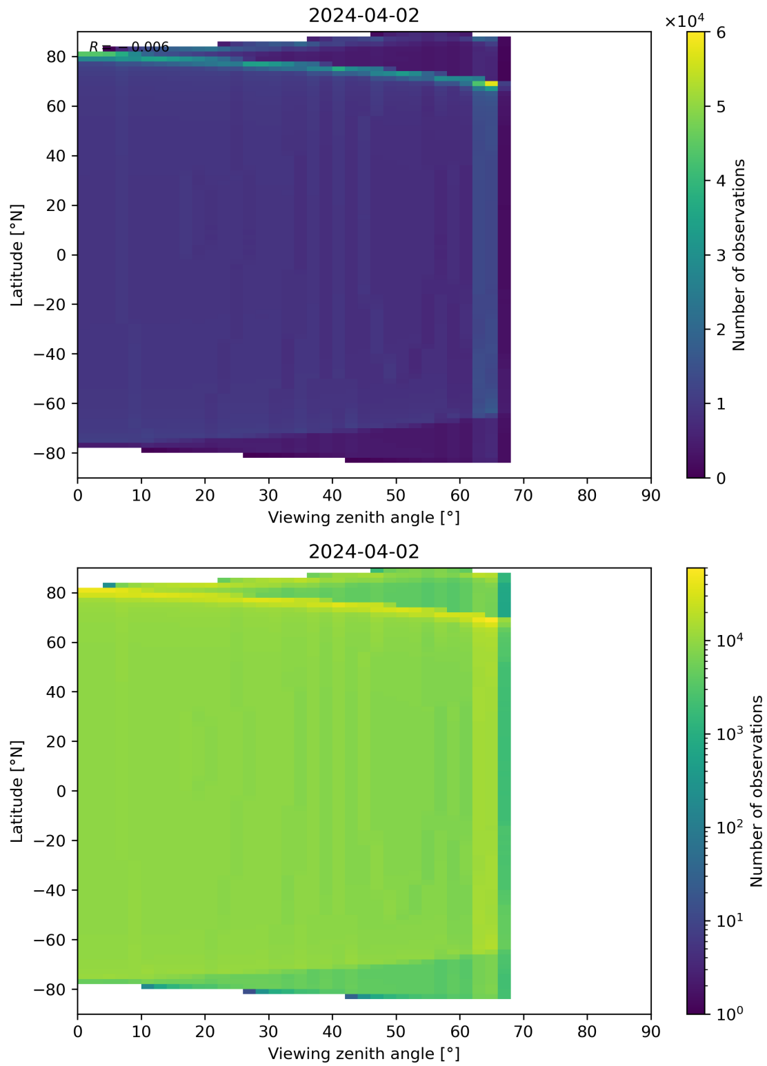
Figure 49: Scatter density plot of “Viewing zenith angle” against “Latitude” for 2024-04-01 to 2024-04-03.
