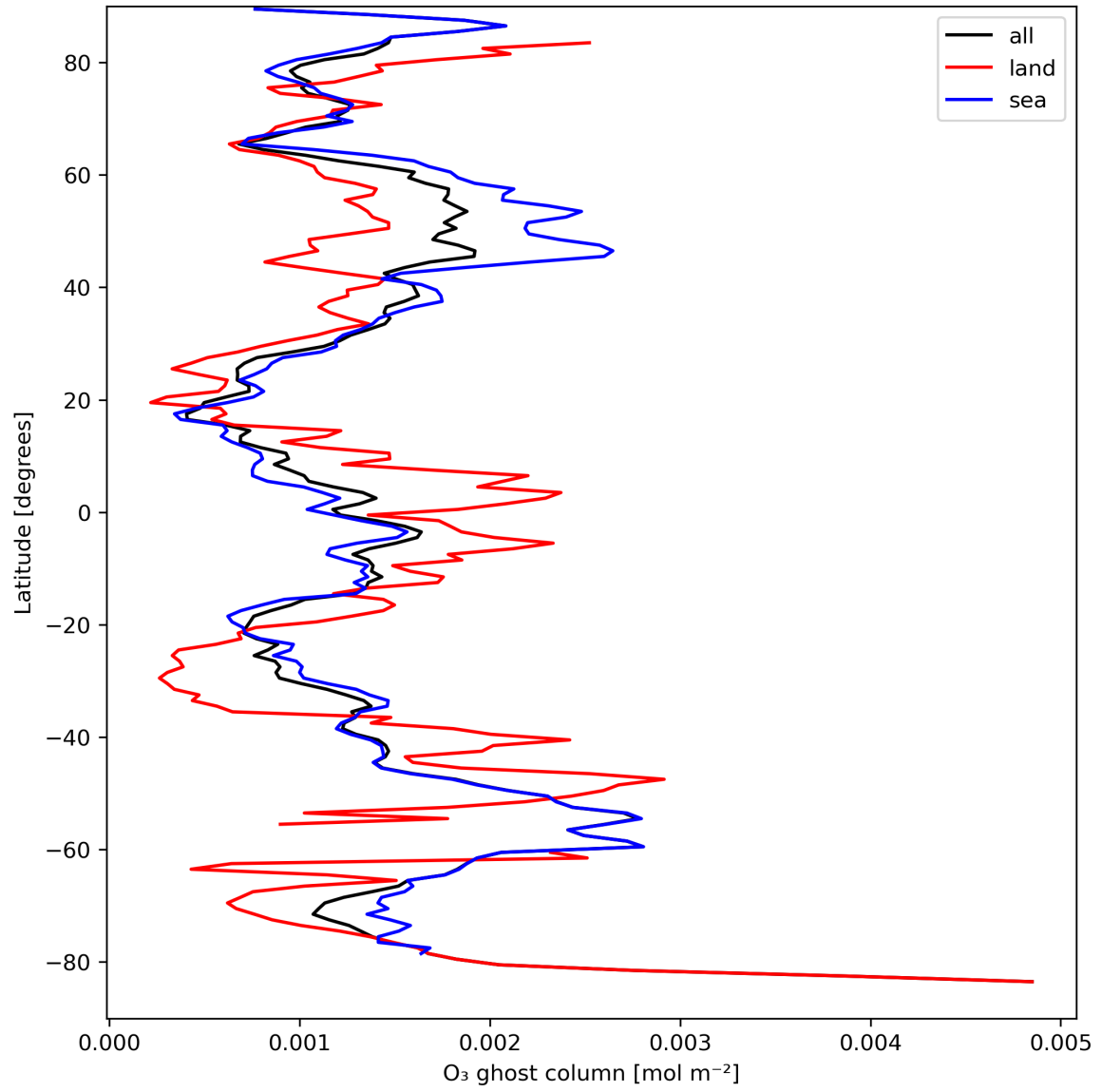
Figure 18: Zonal average of "O 3 ghost column" for 2024-04-01 to 2024-04-03.
