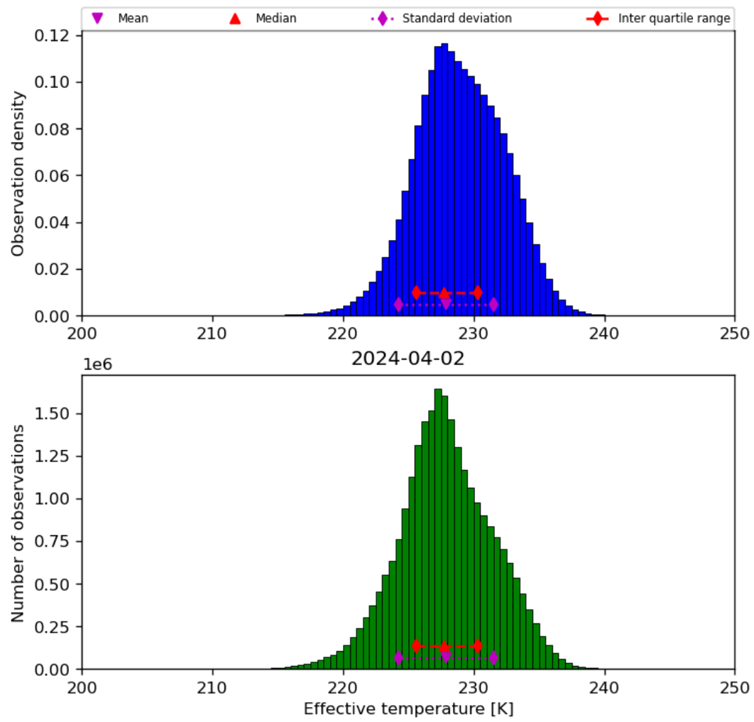
Figure 24: Histogram of “Effective temperature” for 2024-04-01 to 2024-04-03
