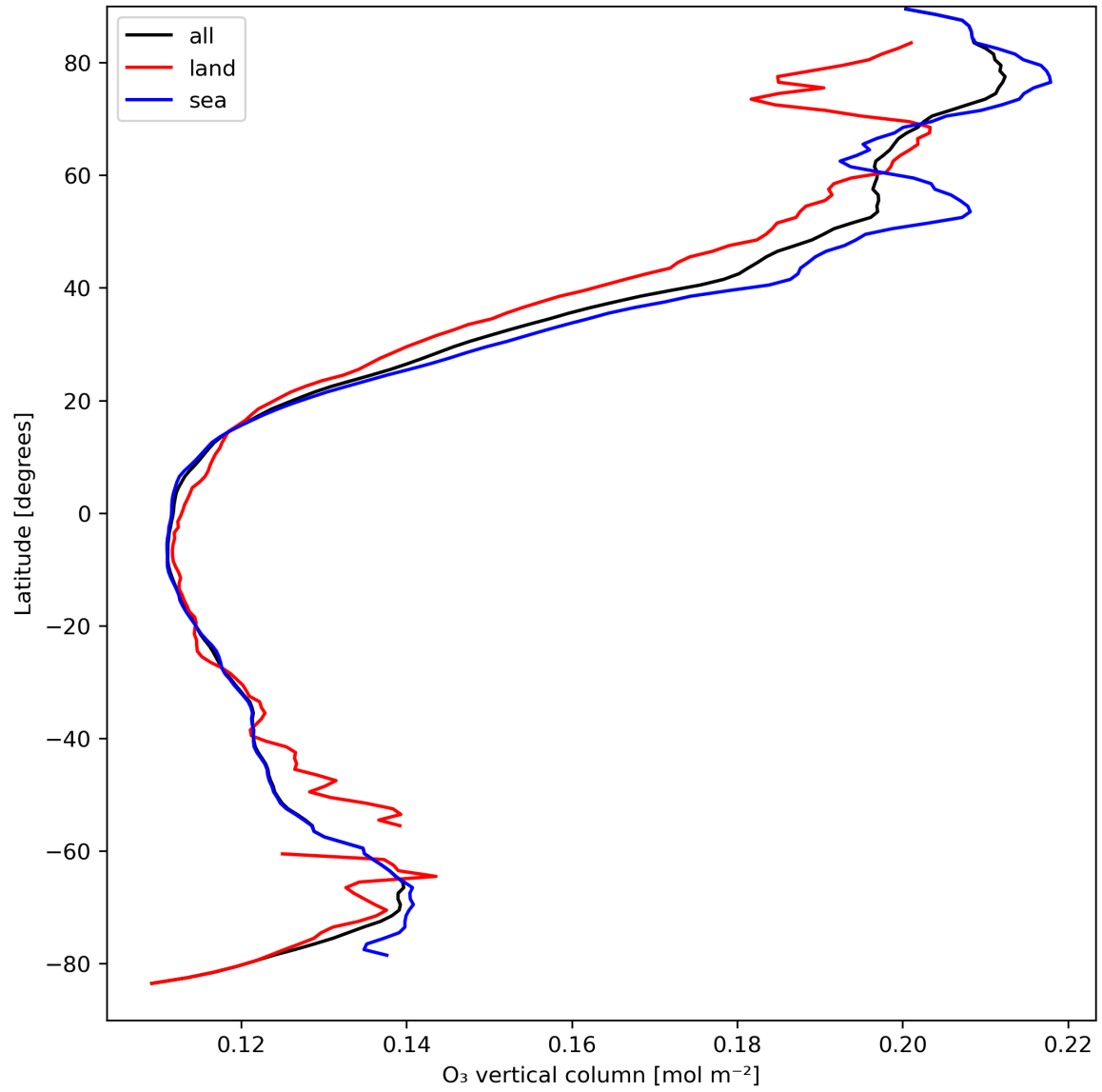
Figure 14: Zonal average of “O 3 vertical column” for 2024-04-01 to 2024-04-03.
