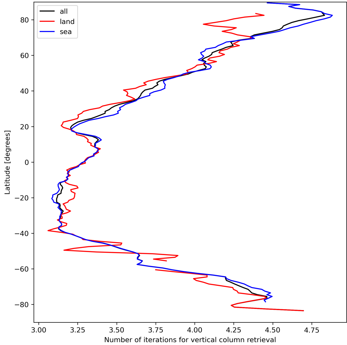
Figure 19: Zonal average of “Number of iterations for vertical column retrieval” for 2024-04-01 to 2024-04-03.
