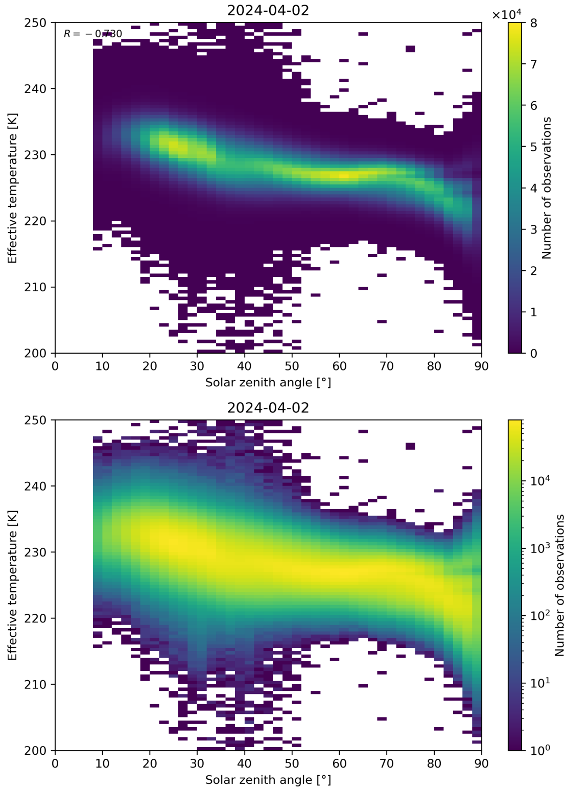
Figure 45: Scatter density plot of “Solar zenith angle” against “Effective temperature” for 2024-04-01 to 2024-04-03.
