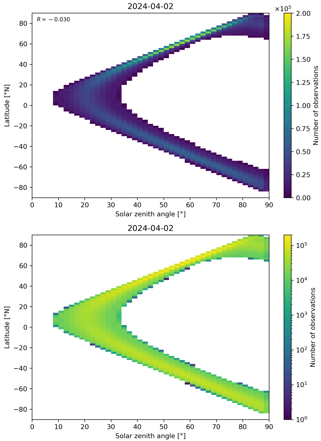
Figure 44: Scatter density plot of “Solar zenith angle” against “Latitude” for 2024-04-01 to 2024-04-03.
