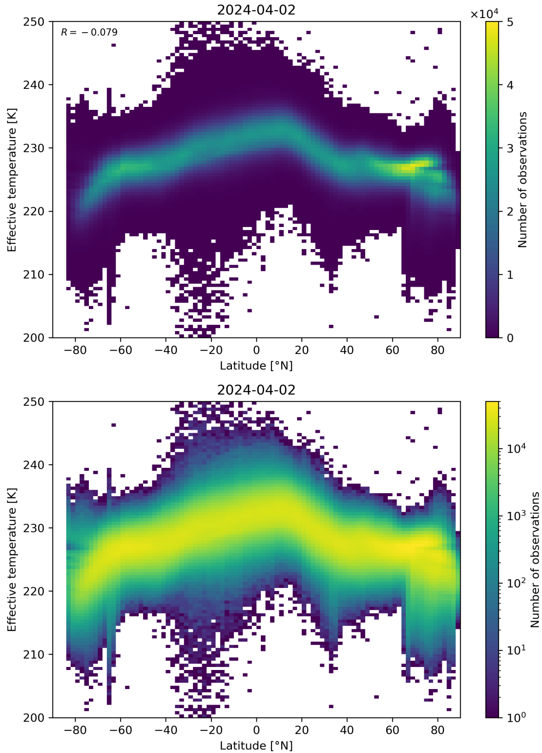
Figure 34: Scatter density plot of “Latitude” against “Effective temperature” for 2024-04-01 to 2024-04-03.
