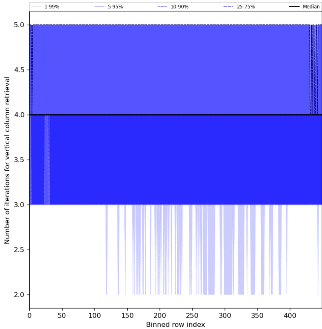
Figure 33: Along track statistics of “Number of iterations for vertical column retrieval” for 2024-04-01 to 2024-04-03
