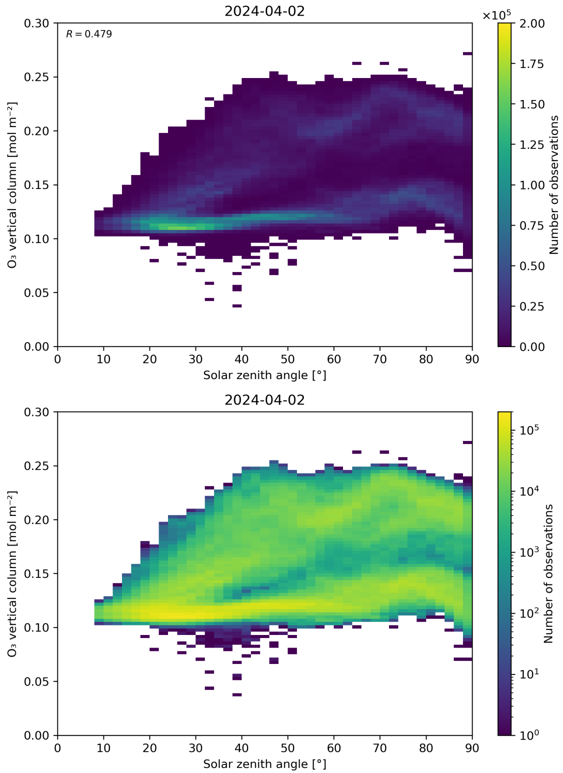
Figure 47: Scatter density plot of “Solar zenith angle” against “O 3 vertical column” for 2024-04-01 to 2024-04-03.
