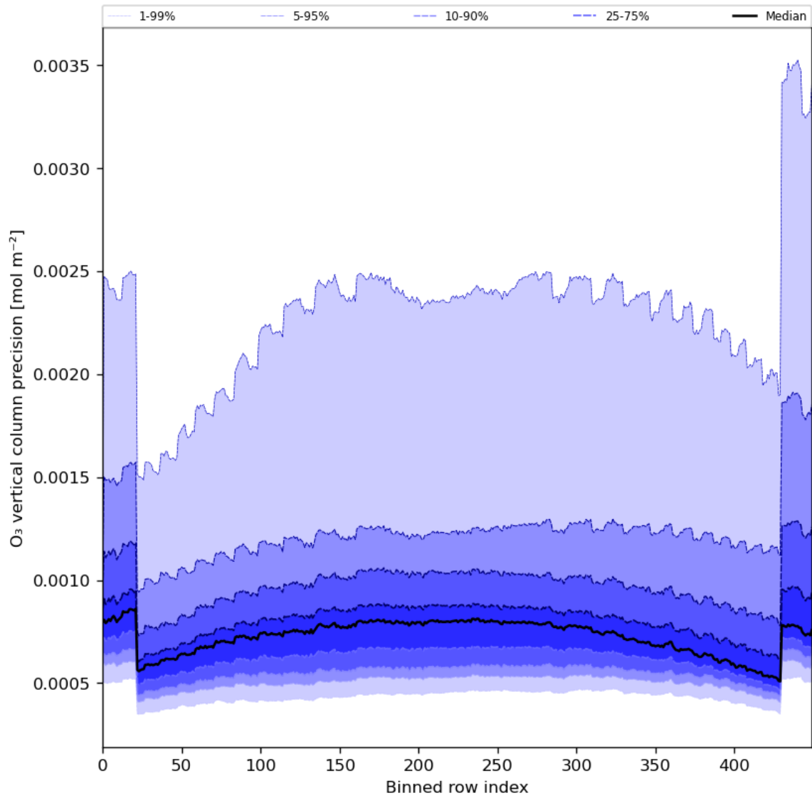
Figure 29: Along track statistics of “O 3 vertical column precision” for 2024-04-01 to 2024-04-03
