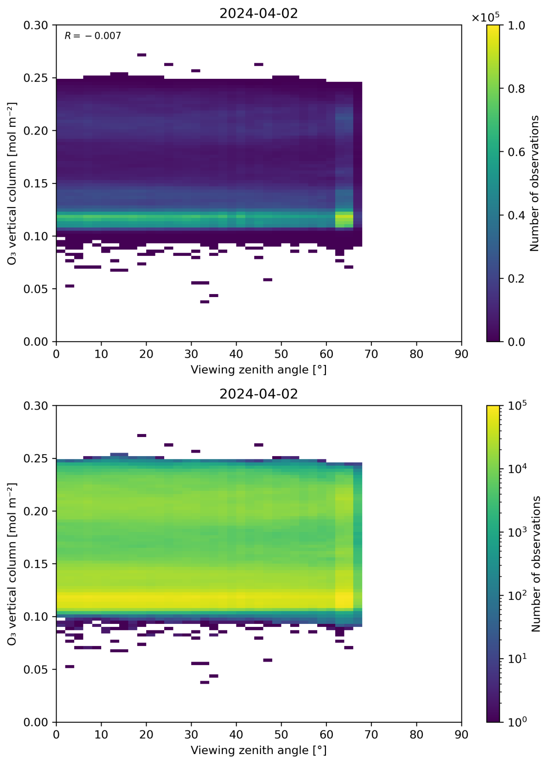
Figure 52: Scatter density plot of “Viewing zenith angle” against “O 3 vertical column” for 2024-04-01 to 2024-04-03.
