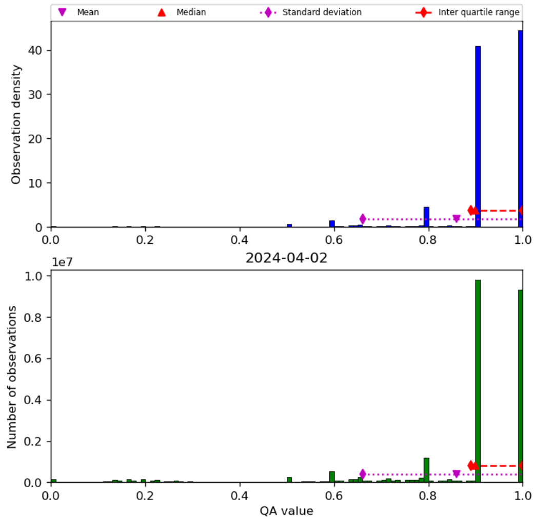
Figure 20: Histogram of “QA value” for 2024-04-01 to 2024-04-03
