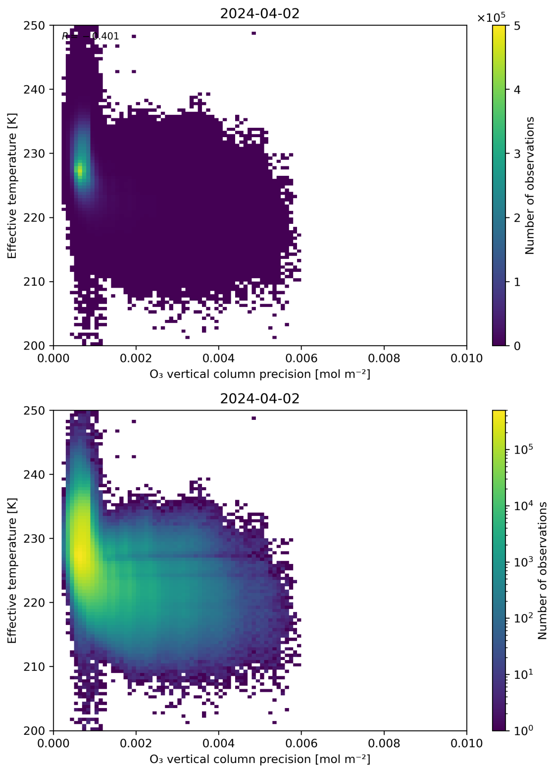
Figure 42: Scatter density plot of “O 3 vertical column precision” against “Effective temperature” for 2024-04-01 to 2024-04-03.
