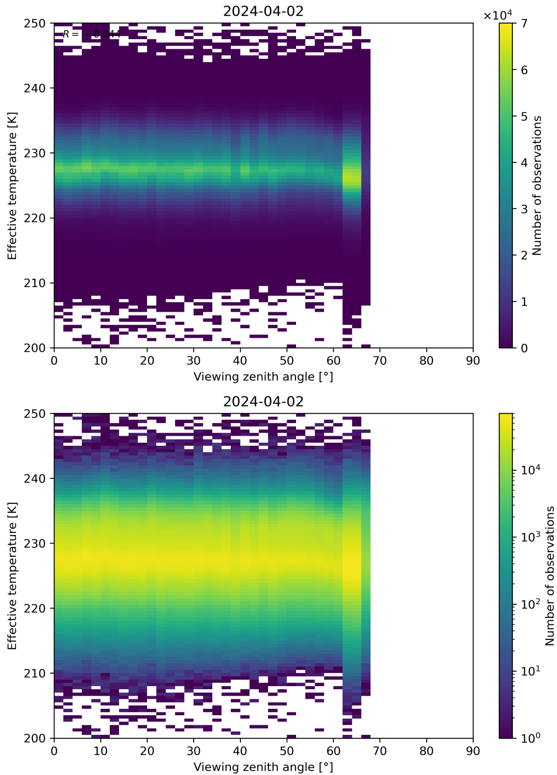
Figure 50: Scatter density plot of “Viewing zenith angle” against “Effective temperature” for 2024-04-01 to 2024-04-03.
