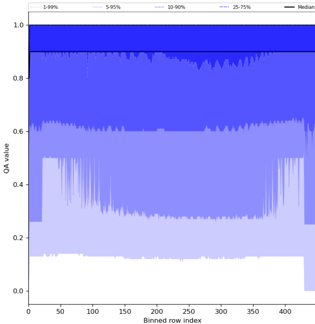
Figure 27: Along track statistics of “QA value” for 2024-04-01 to 2024-04-03
