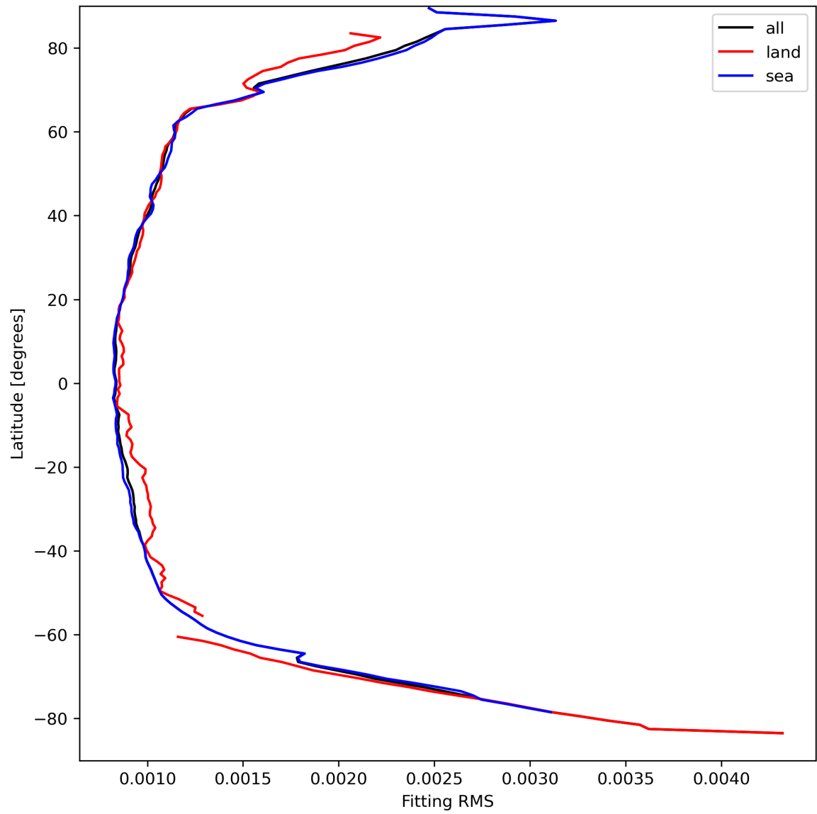
Figure 16: Zonal average of “Fitting RMS” for 2024-04-01 to 2024-04-03.
