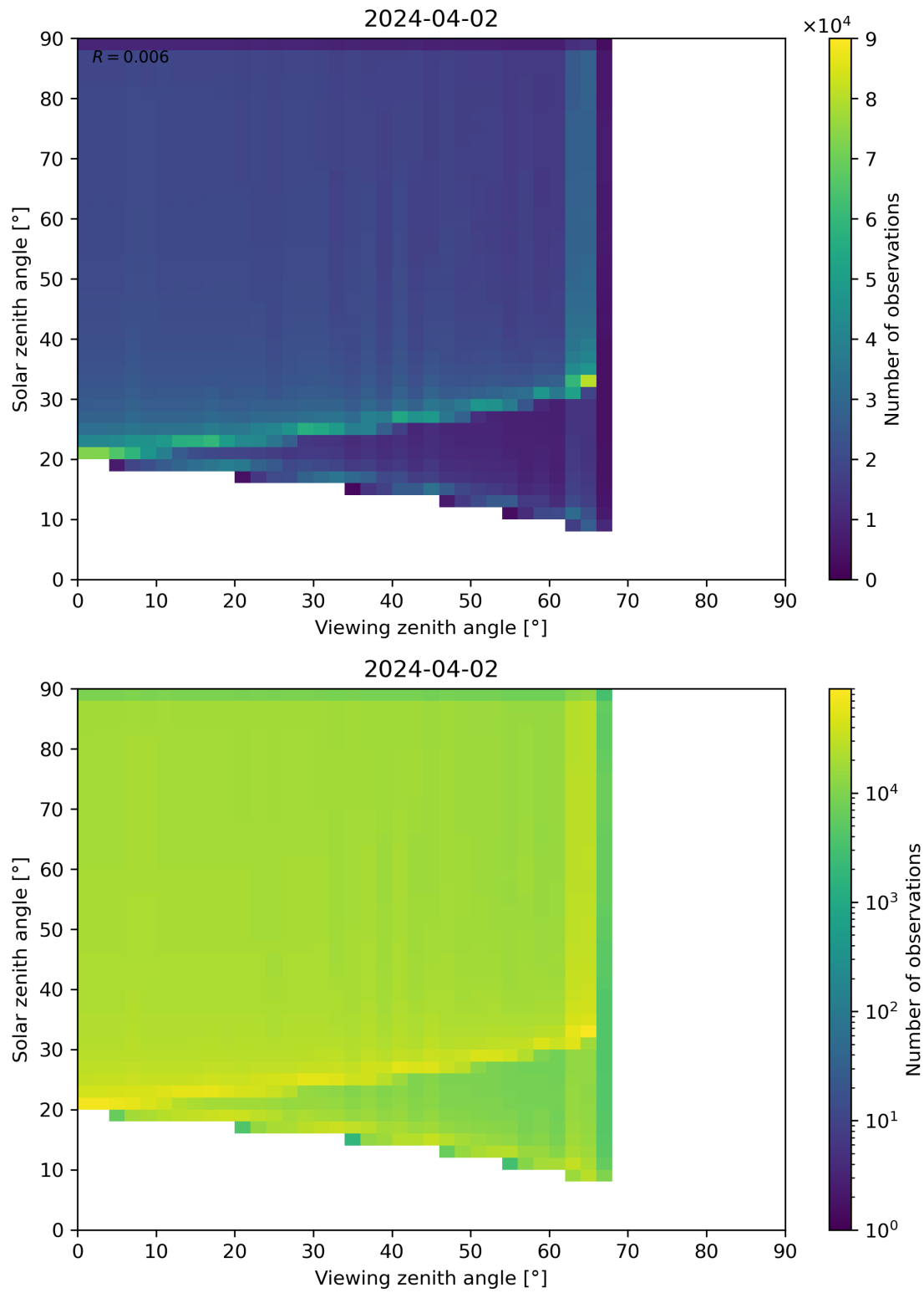
Figure 54: Scatter density plot of “Viewing zenith angle” against “Solar zenith angle” for 2024-04-01 to 2024-04-03.
