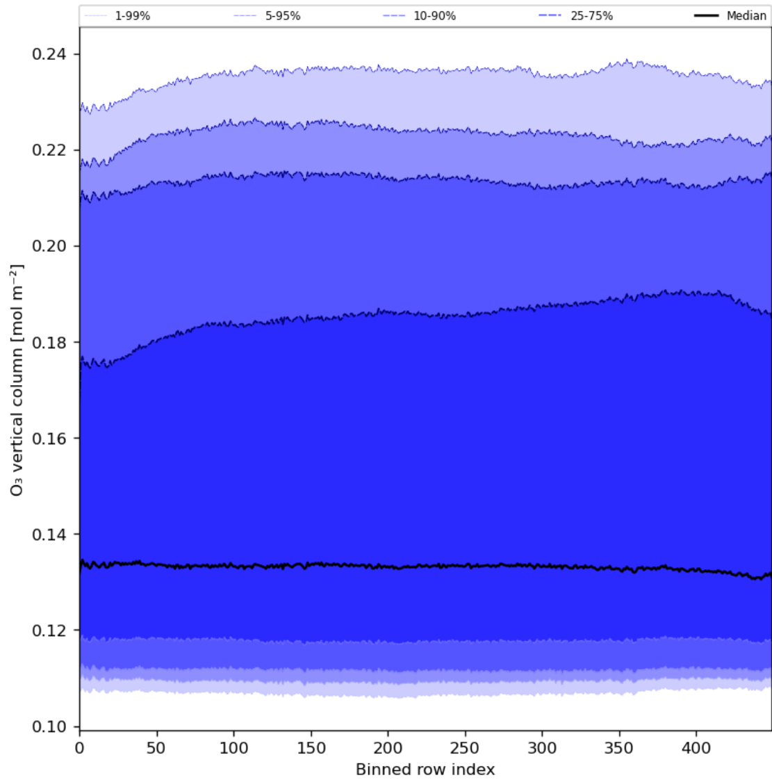
Figure 28: Along track statistics of “O 3 vertical column” for 2024-04-01 to 2024-04-03
