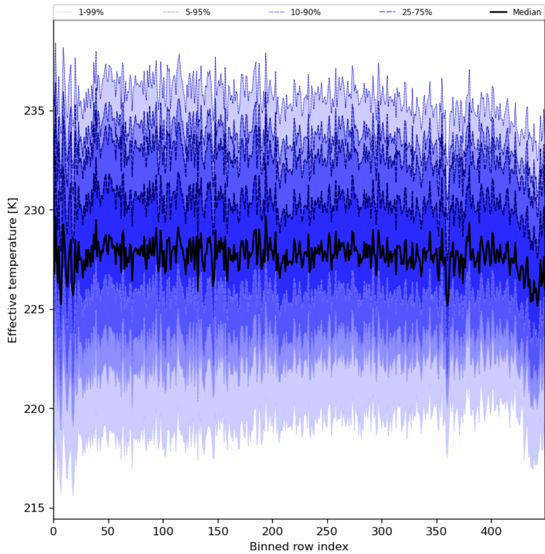
Figure 31: Along track statistics of “Effective temperature” for 2024-04-01 to 2024-04-03
