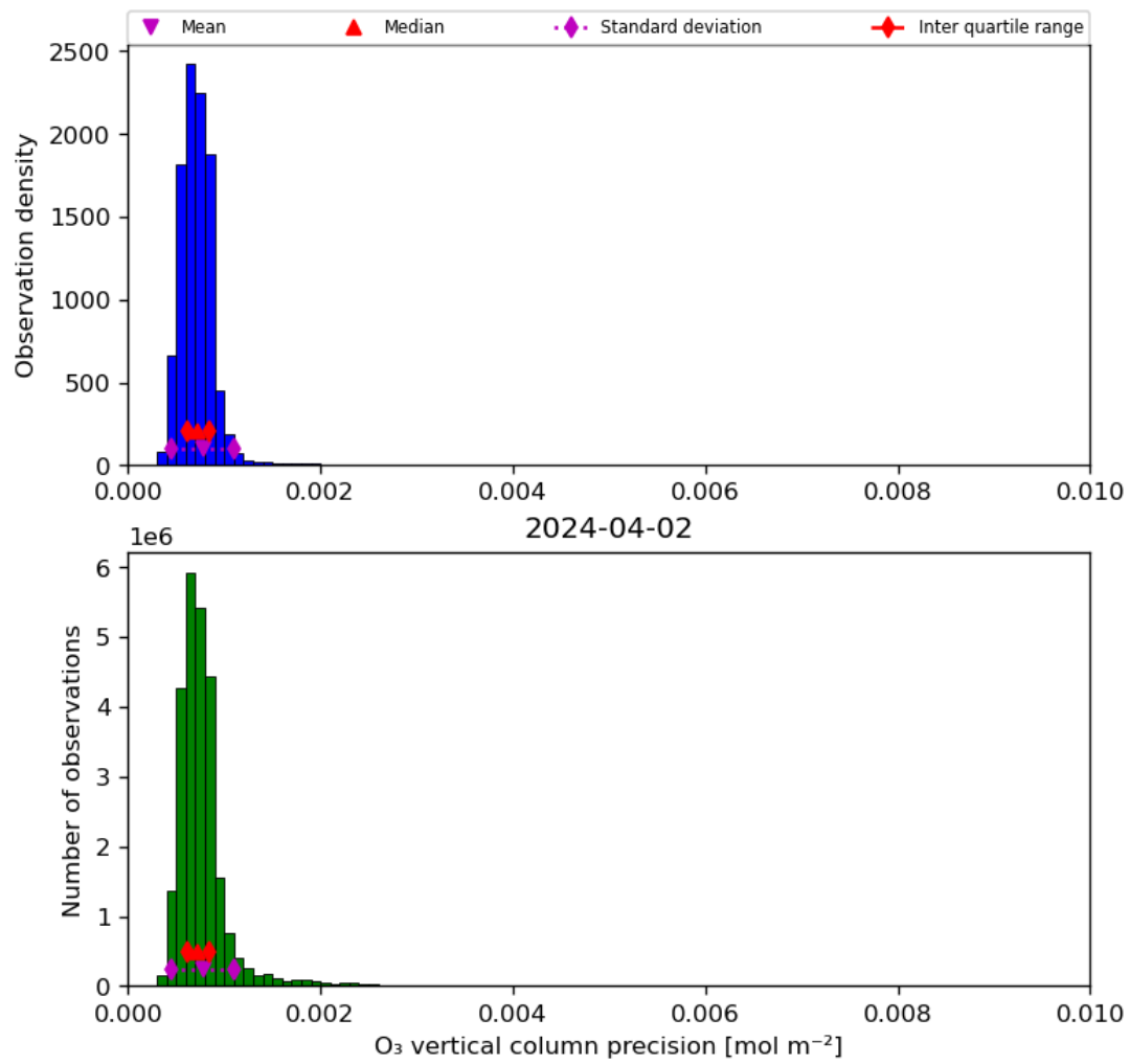
Figure 22: Histogram of “O 3 vertical column precision” for 2024-04-01 to 2024-04-03
