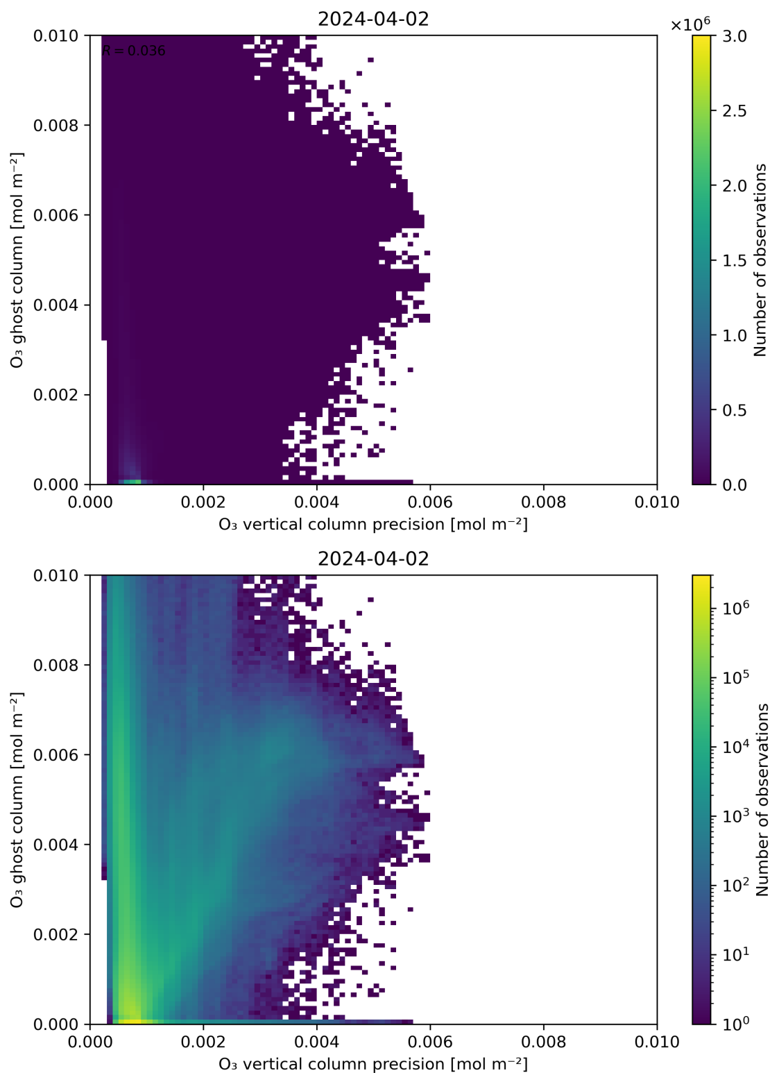
Figure 43: Scatter density plot of “ \text{O}_3 vertical column precision” against “ \text{O}_3 ghost column” for 2024-04-01 to 2024-04-03.
