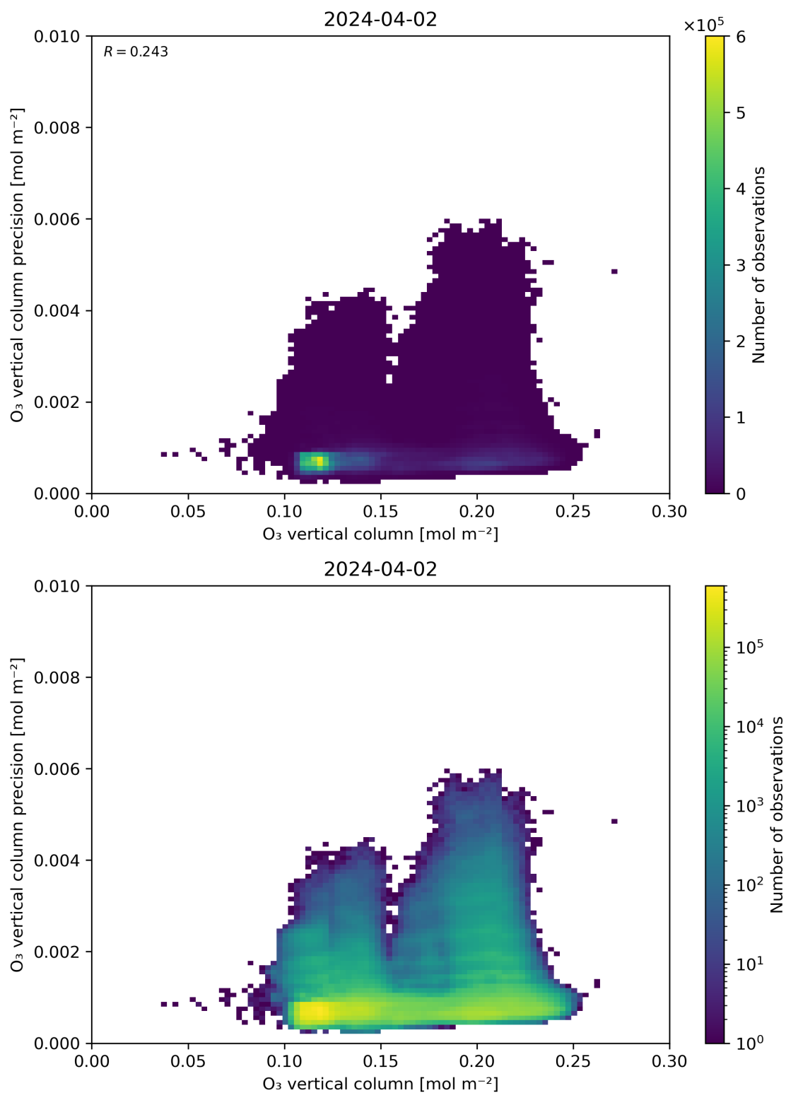
Figure 41: Scatter density plot of “O 3 vertical column” against “O 3 vertical column precision” for 2024-04-01 to 2024-04-03.
