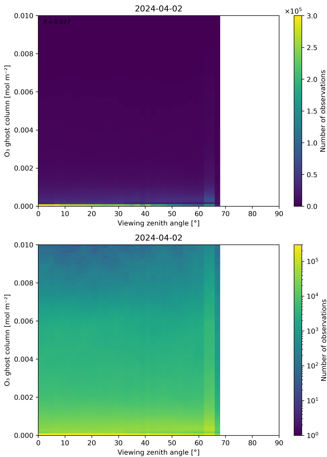
Figure 51: Scatter density plot of “Viewing zenith angle” against “O 3 ghost column” for 2024-04-01 to 2024-04-03.
