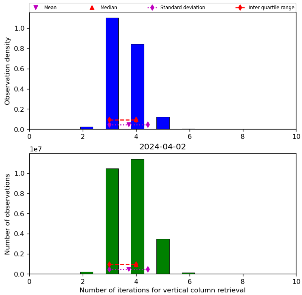
Figure 26: Histogram of “Number of iterations for vertical column retrieval” for 2024-04-01 to 2024-04-03
