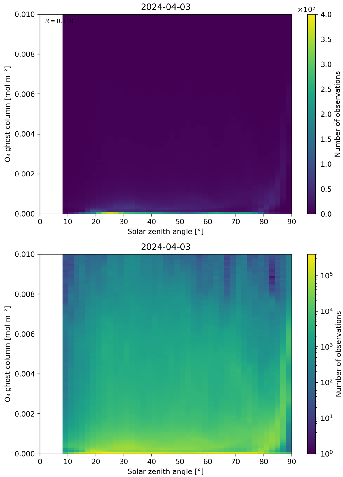
Figure 46: Scatter density plot of “Solar zenith angle” against “O 3 ghost column” for 2024-04-02 to 2024-04-04.
