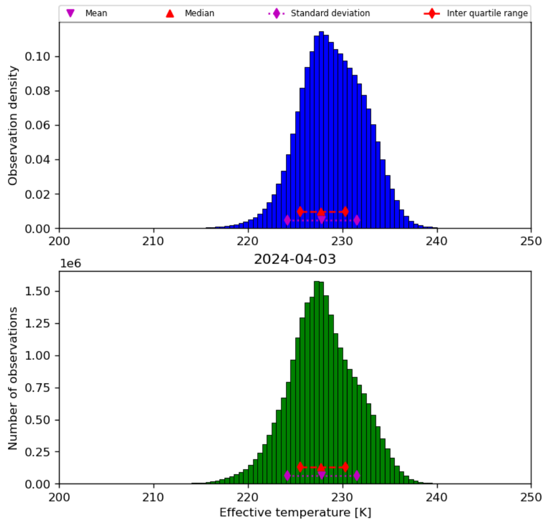
Figure 24: Histogram of “Effective temperature” for 2024-04-02 to 2024-04-04
