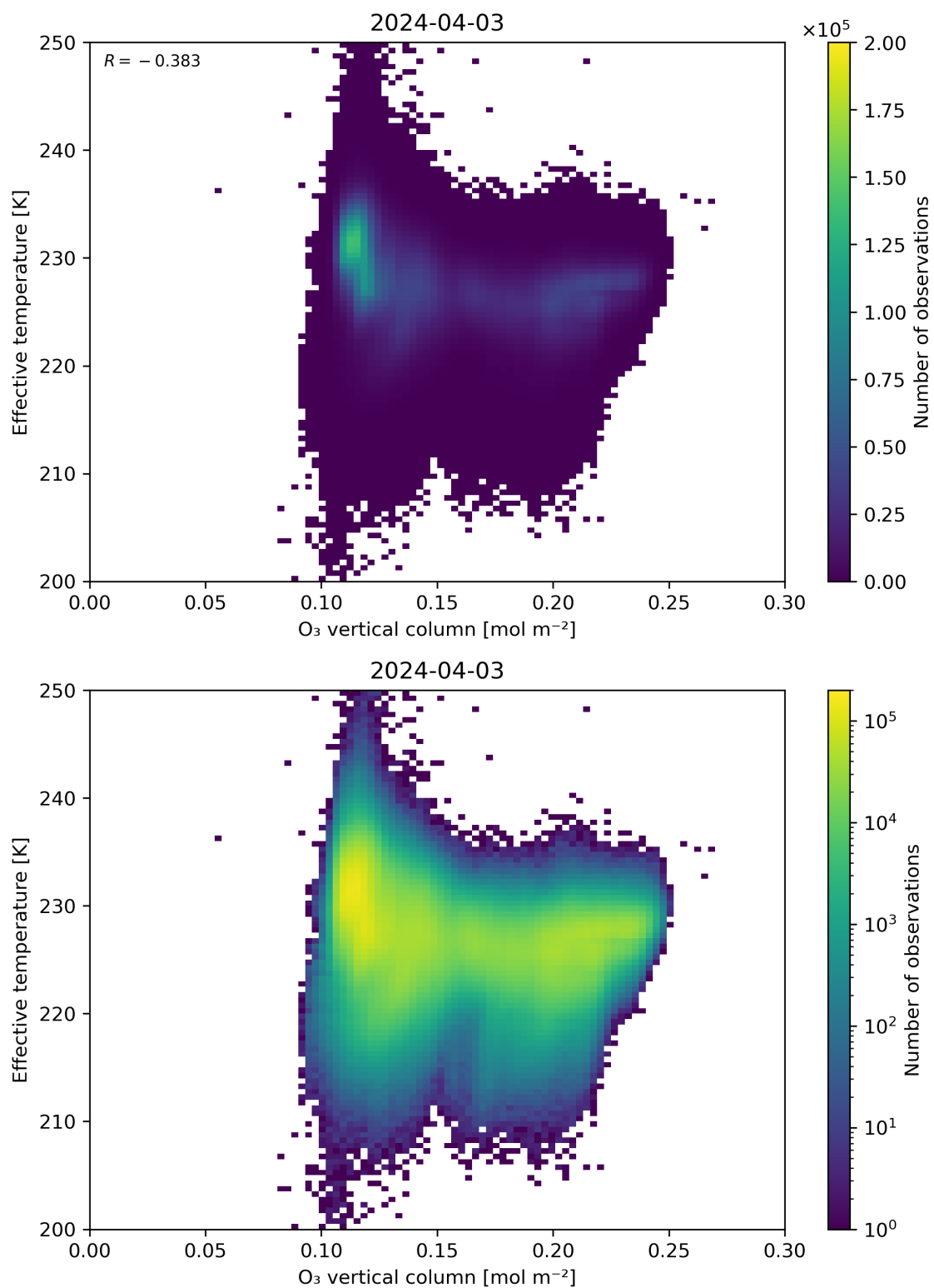
Figure 39: Scatter density plot of “O 3 vertical column” against “Effective temperature” for 2024-04-02 to 2024-04-04.
