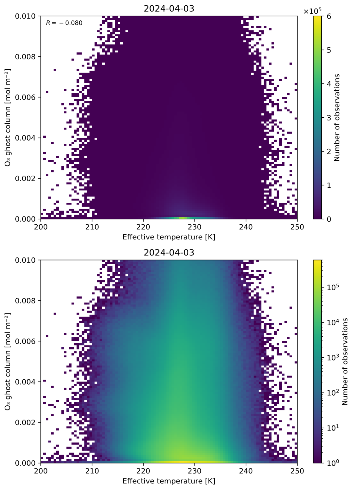
Figure 38: Scatter density plot of “Effective temperature” against “O 3 ghost column” for 2024-04-02 to 2024-04-04.
