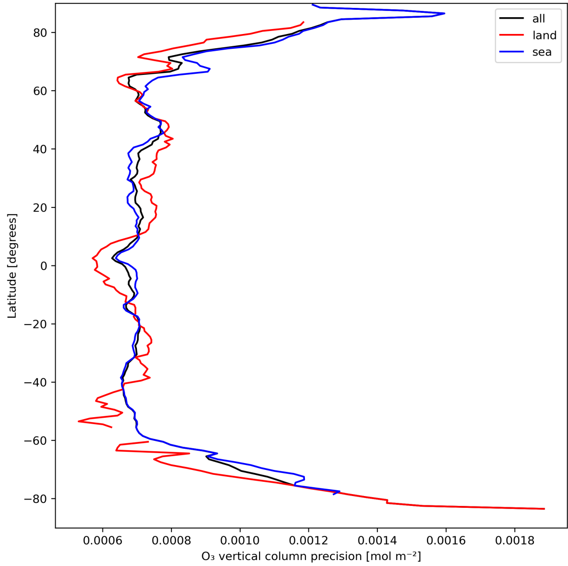
Figure 15: Zonal average of “O 3 vertical column precision” for 2024-04-02 to 2024-04-04.
