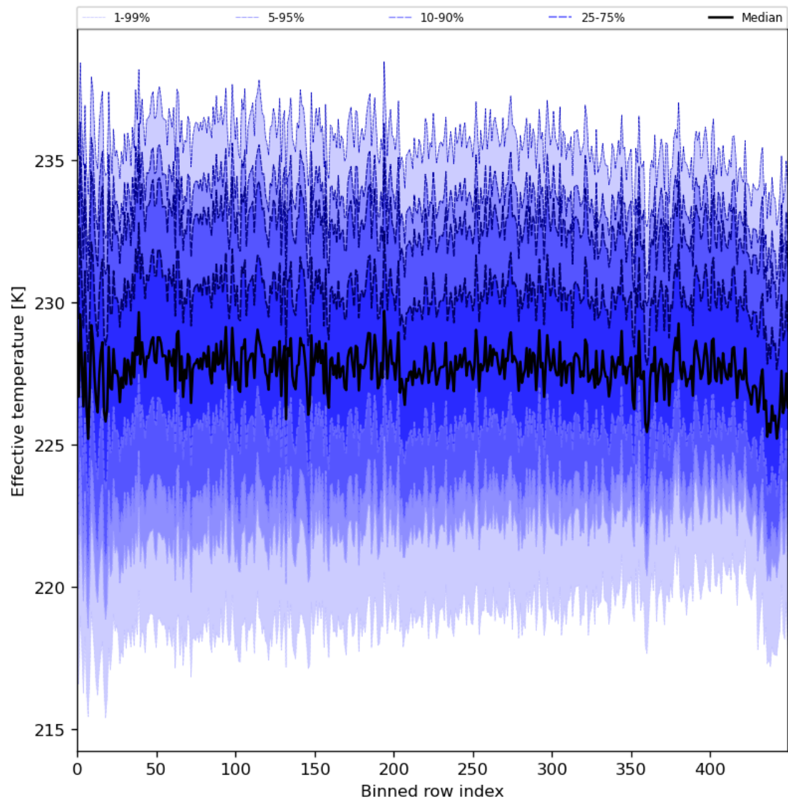
Figure 31: Along track statistics of “Effective temperature” for 2024-04-02 to 2024-04-04
