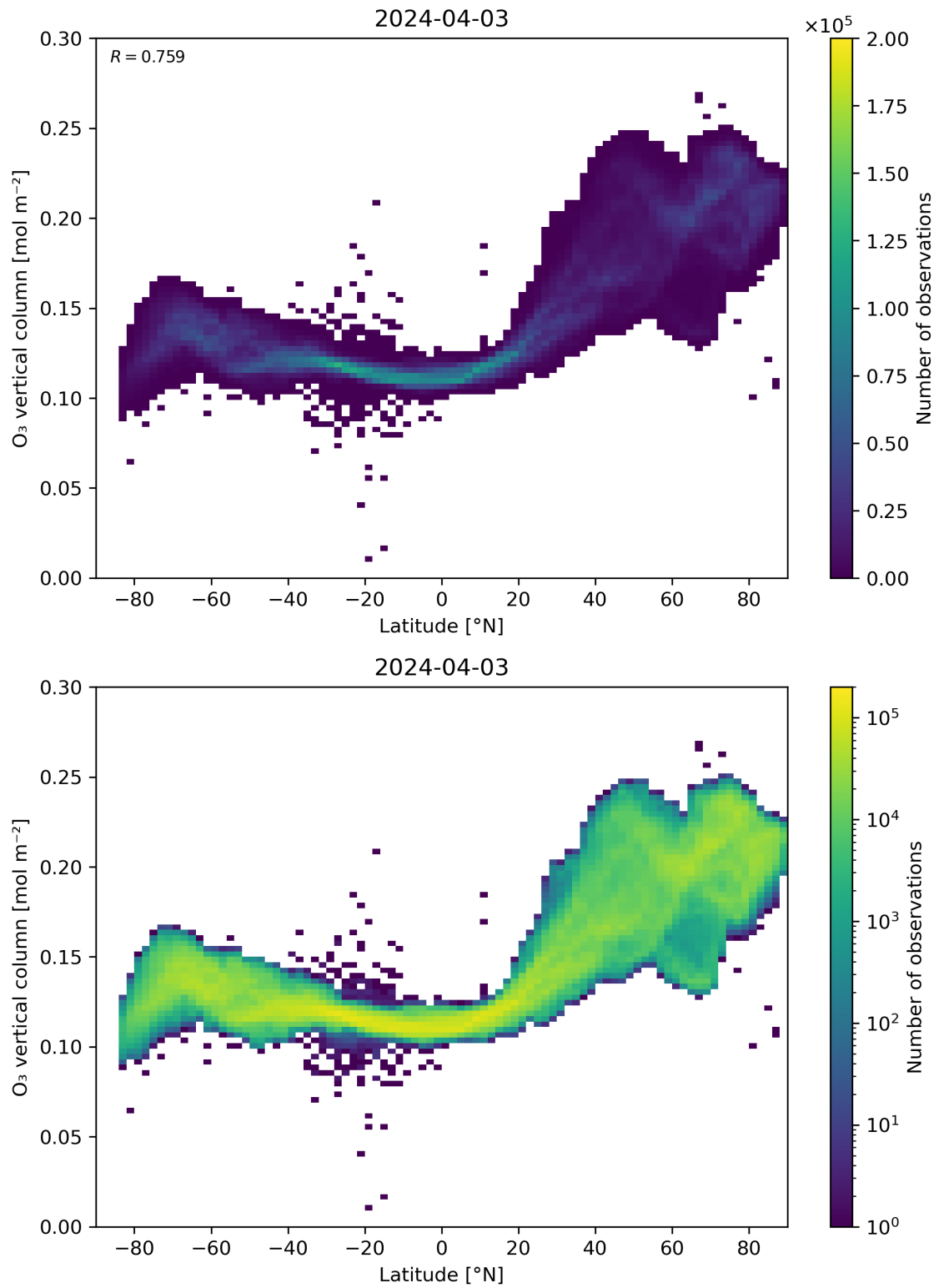
Figure 36: Scatter density plot of “Latitude” against “O 3 vertical column” for 2024-04-02 to 2024-04-04.
