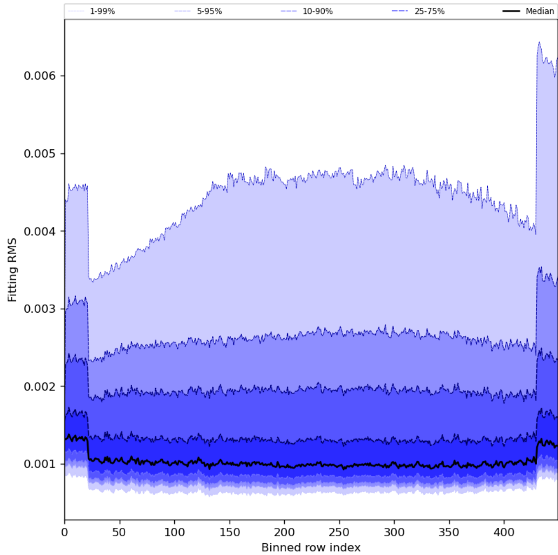
Figure 30: Along track statistics of “Fitting RMS” for 2024-04-02 to 2024-04-04
