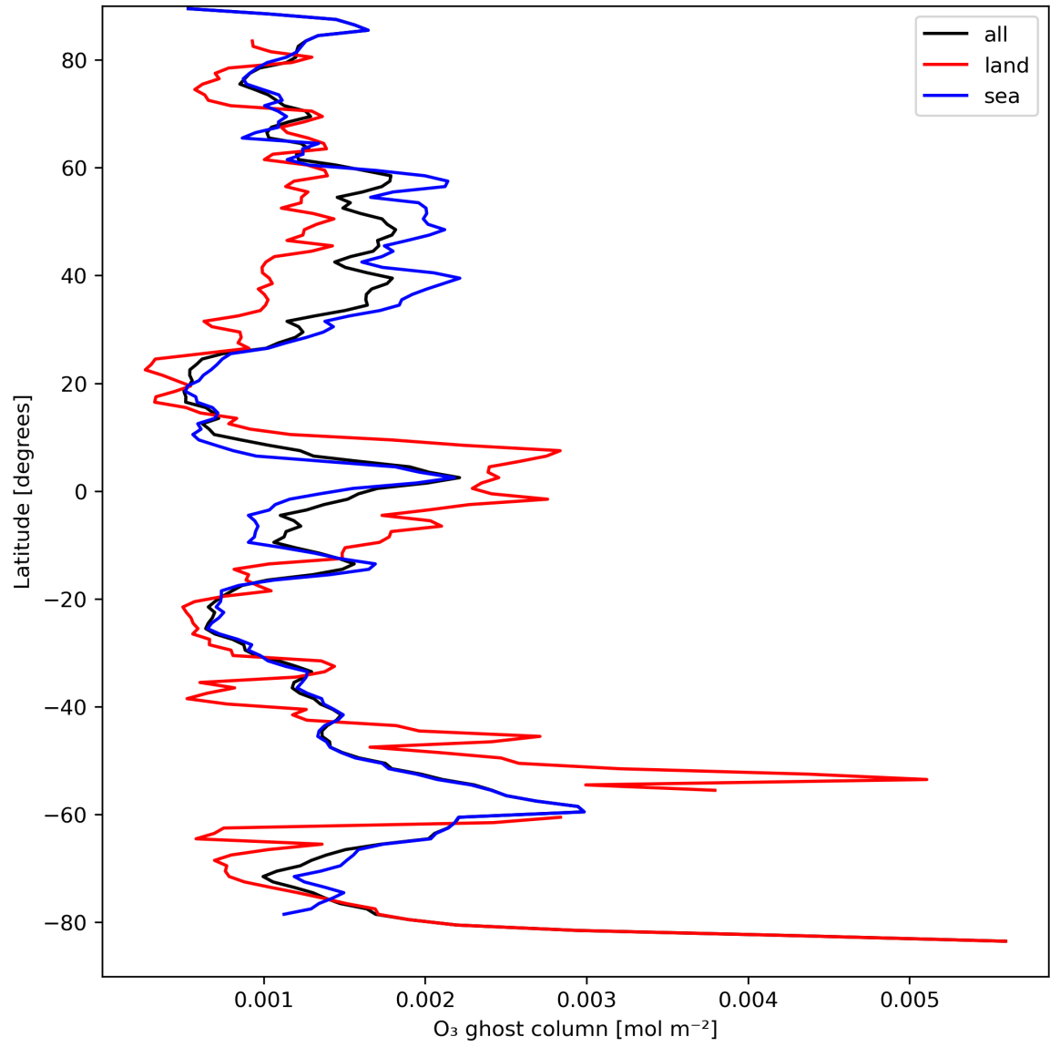
Figure 18: Zonal average of “O 3 ghost column” for 2024-04-02 to 2024-04-04.
