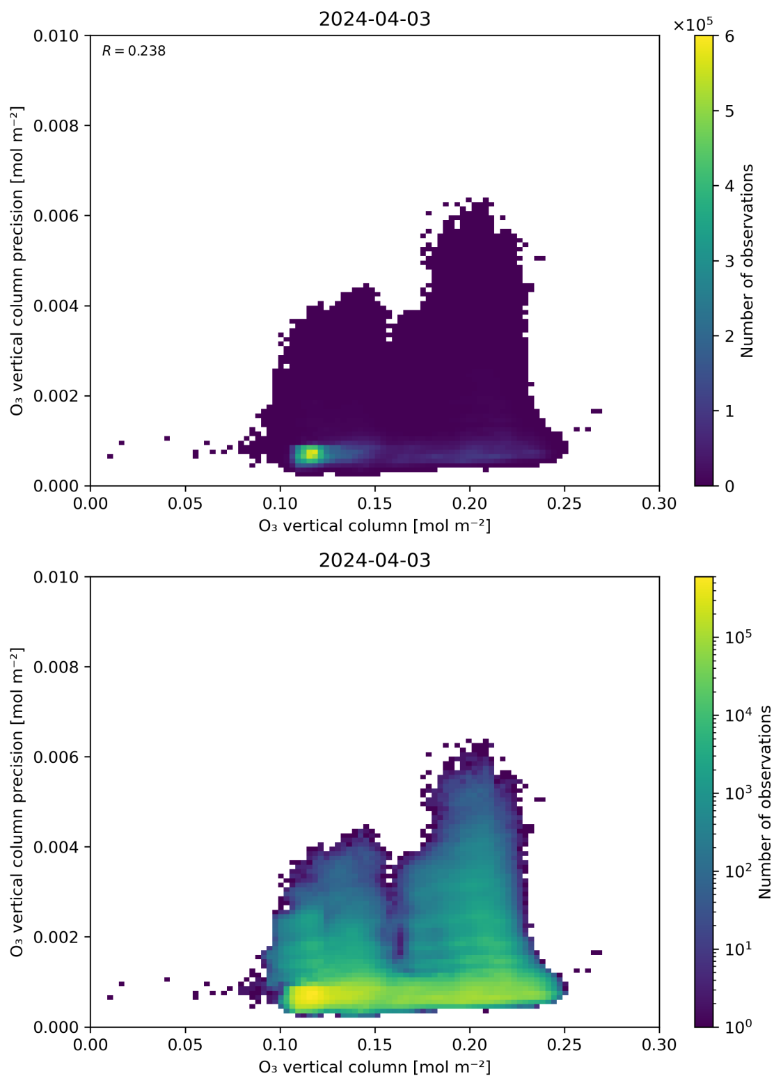
Figure 41: Scatter density plot of “O 3 vertical column” against “O 3 vertical column precision” for 2024-04-02 to 2024-04-04.
