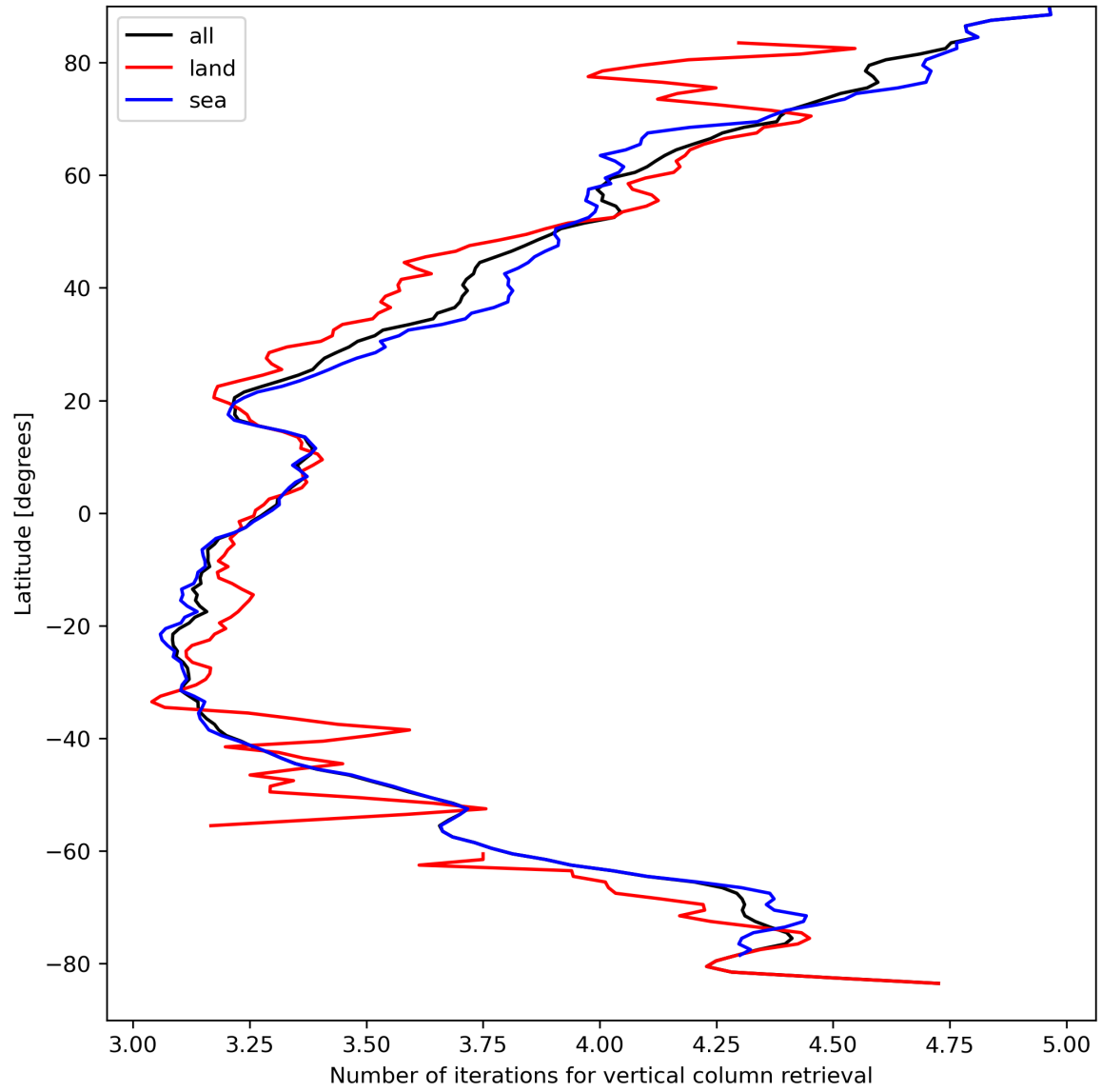
Figure 19: Zonal average of “Number of iterations for vertical column retrieval” for 2024-04-02 to 2024-04-04.
