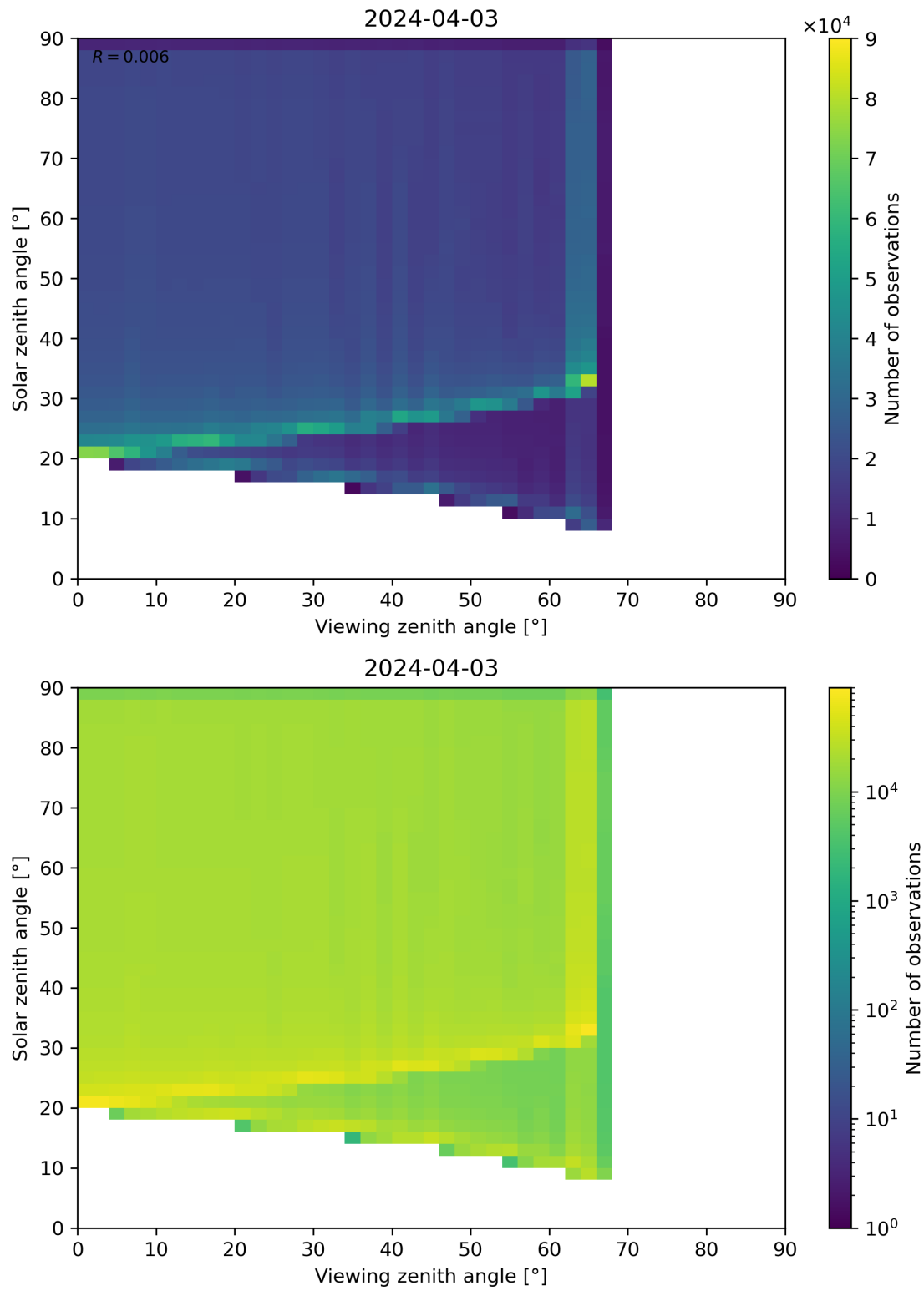
Figure 54: Scatter density plot of “Viewing zenith angle” against “Solar zenith angle” for 2024-04-02 to 2024-04-04.
