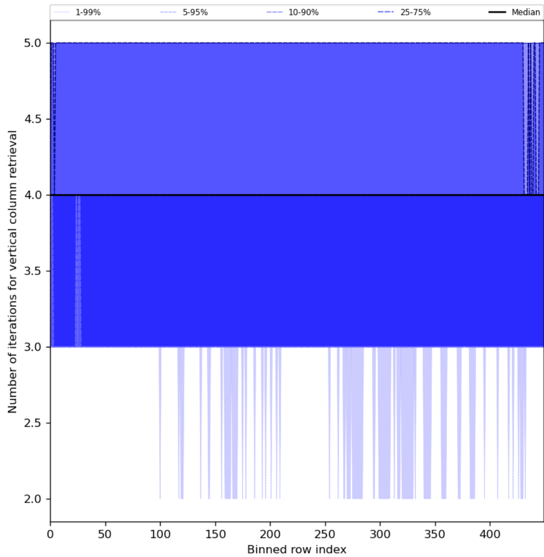
Figure 33: Along track statistics of “Number of iterations for vertical column retrieval” for 2024-04-02 to 2024-04-04
