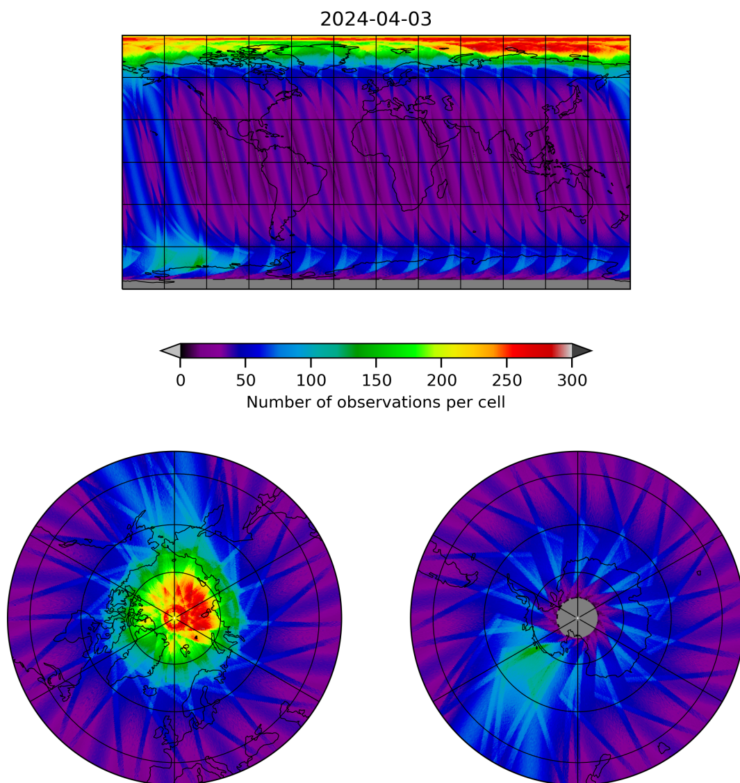
Figure 12: Map of the number of observations for 2024-04-02 to 2024-04-04
