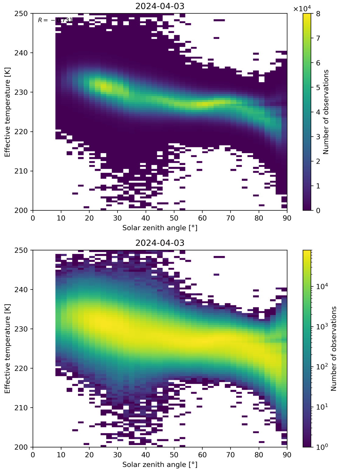
Figure 45: Scatter density plot of “Solar zenith angle” against “Effective temperature” for 2024-04-02 to 2024-04-04.
