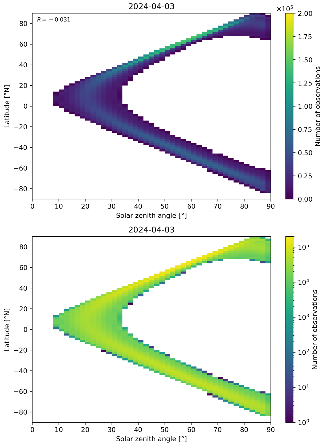
Figure 44: Scatter density plot of “Solar zenith angle” against “Latitude” for 2024-04-02 to 2024-04-04.
