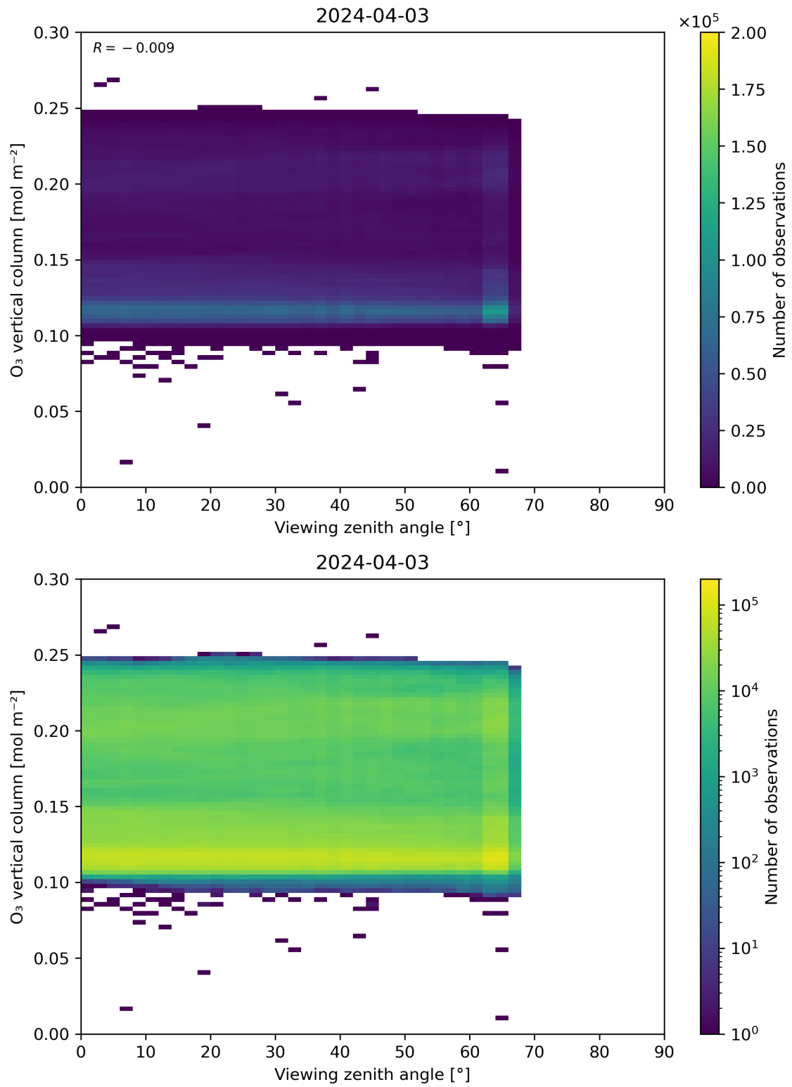
Figure 52: Scatter density plot of “Viewing zenith angle” against “O 3 vertical column” for 2024-04-02 to 2024-04-04.
