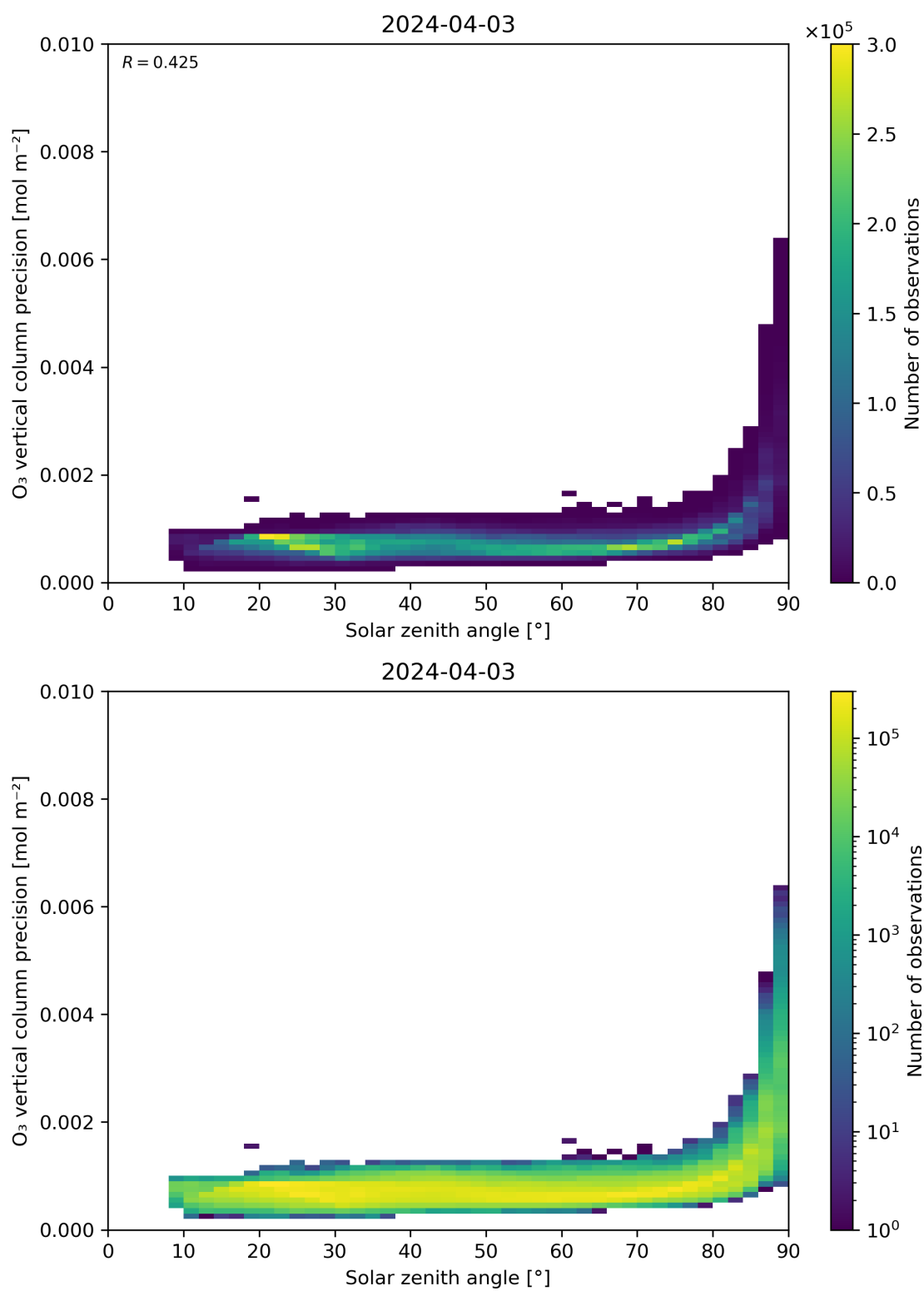
Figure 48: Scatter density plot of “Solar zenith angle” against “O 3 vertical column precision” for 2024-04-02 to 2024-04-04.
