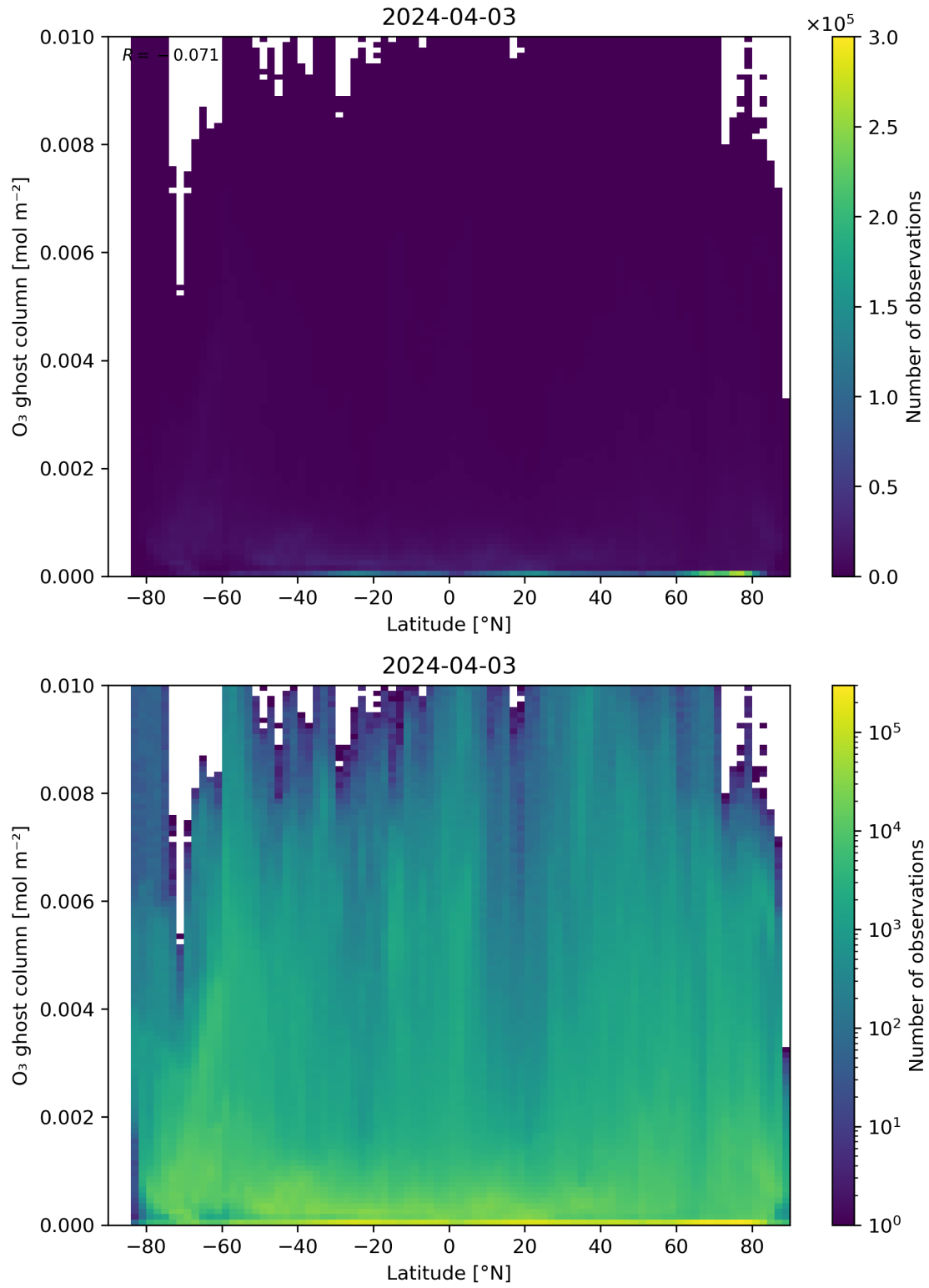
Figure 35: Scatter density plot of “Latitude” against “O 3 ghost column” for 2024-04-02 to 2024-04-04.
