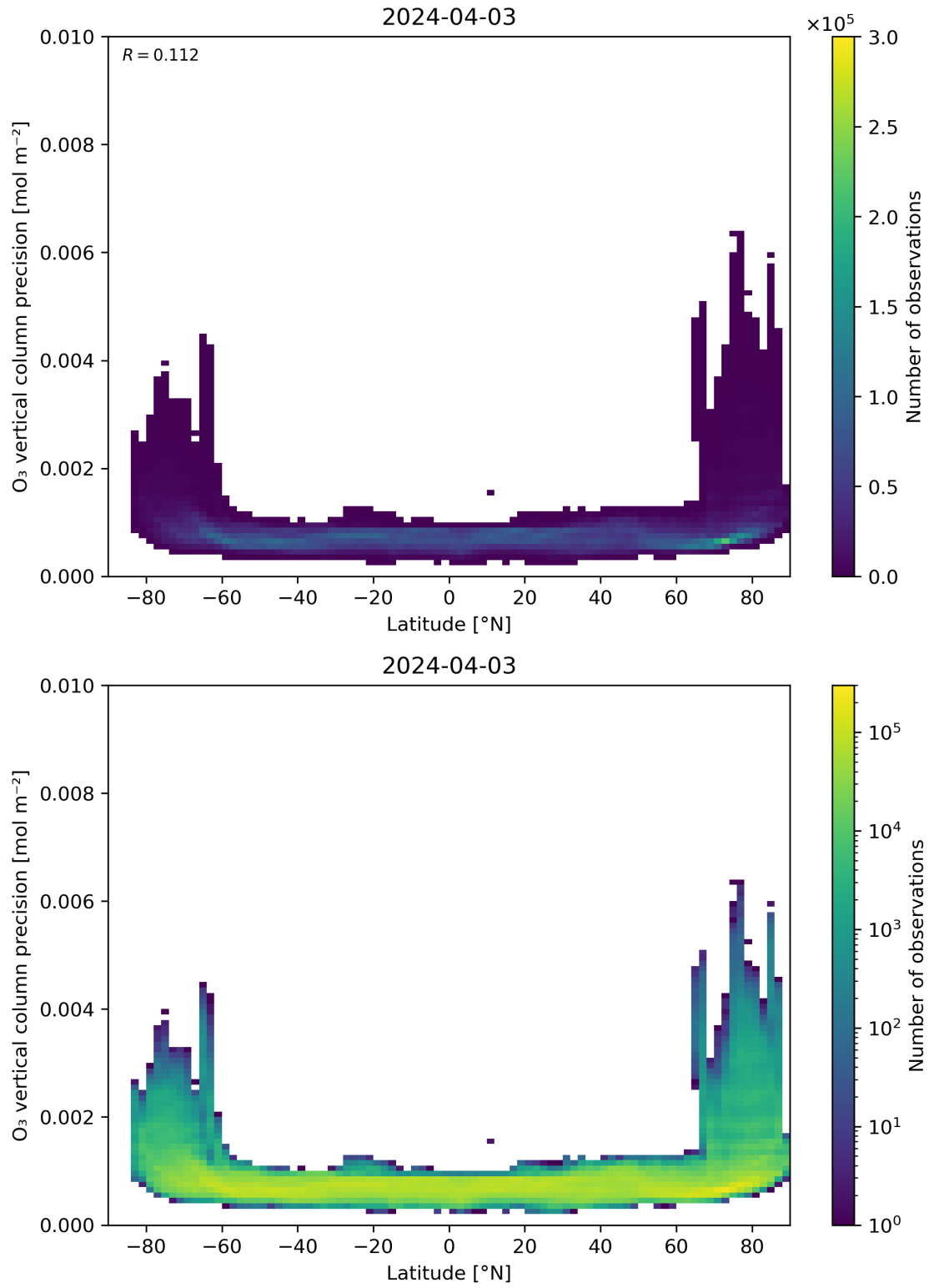
Figure 37: Scatter density plot of “Latitude” against “O 3 vertical column precision” for 2024-04-02 to 2024-04-04.
