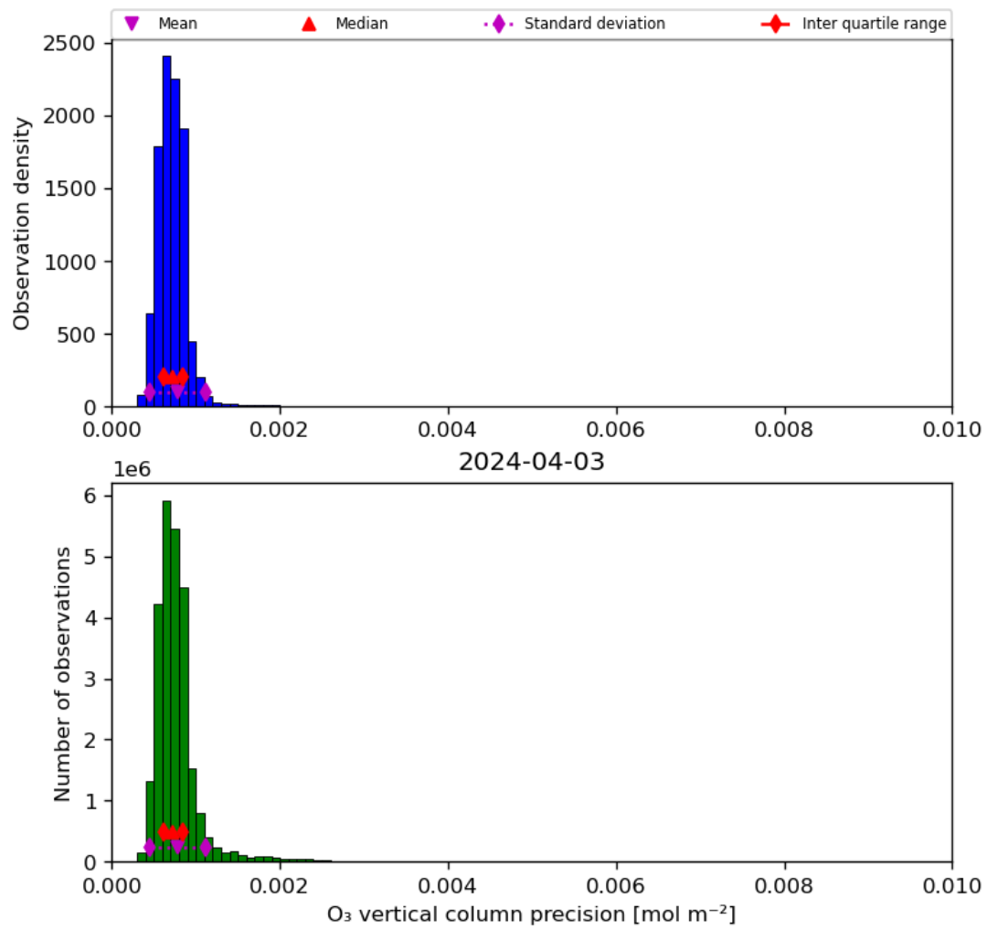
Figure 22: Histogram of “O 3 vertical column precision” for 2024-04-02 to 2024-04-04
