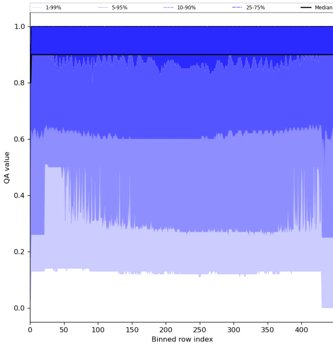
Figure 27: Along track statistics of “QA value” for 2024-04-02 to 2024-04-04
