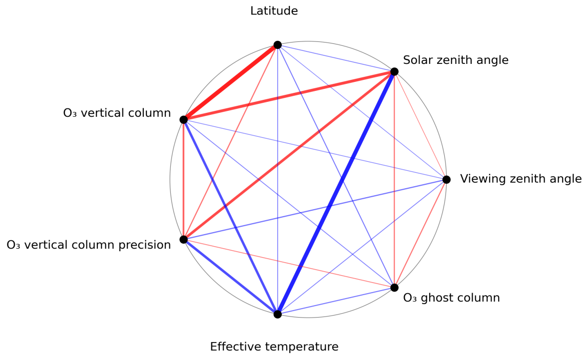
Figure 1: Map of correlation graph for 2024-04-02 to 2024-04-04.
