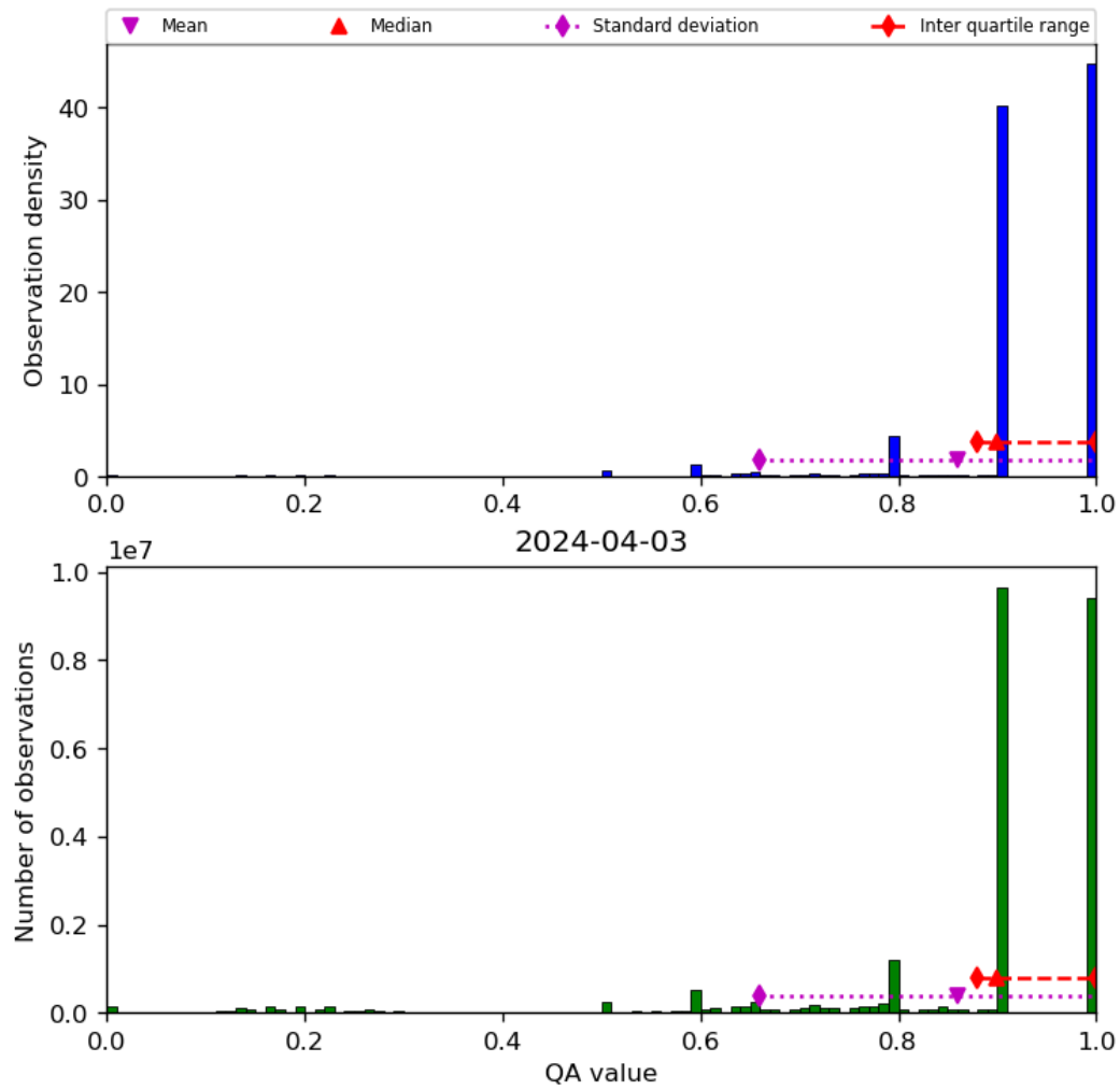
Figure 20: Histogram of “QA value” for 2024-04-02 to 2024-04-04
