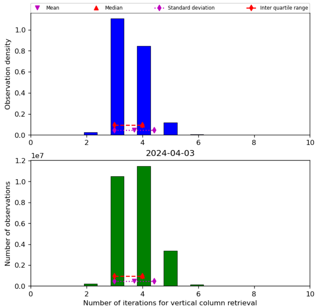
Figure 26: Histogram of “Number of iterations for vertical column retrieval” for 2024-04-02 to 2024-04-04
