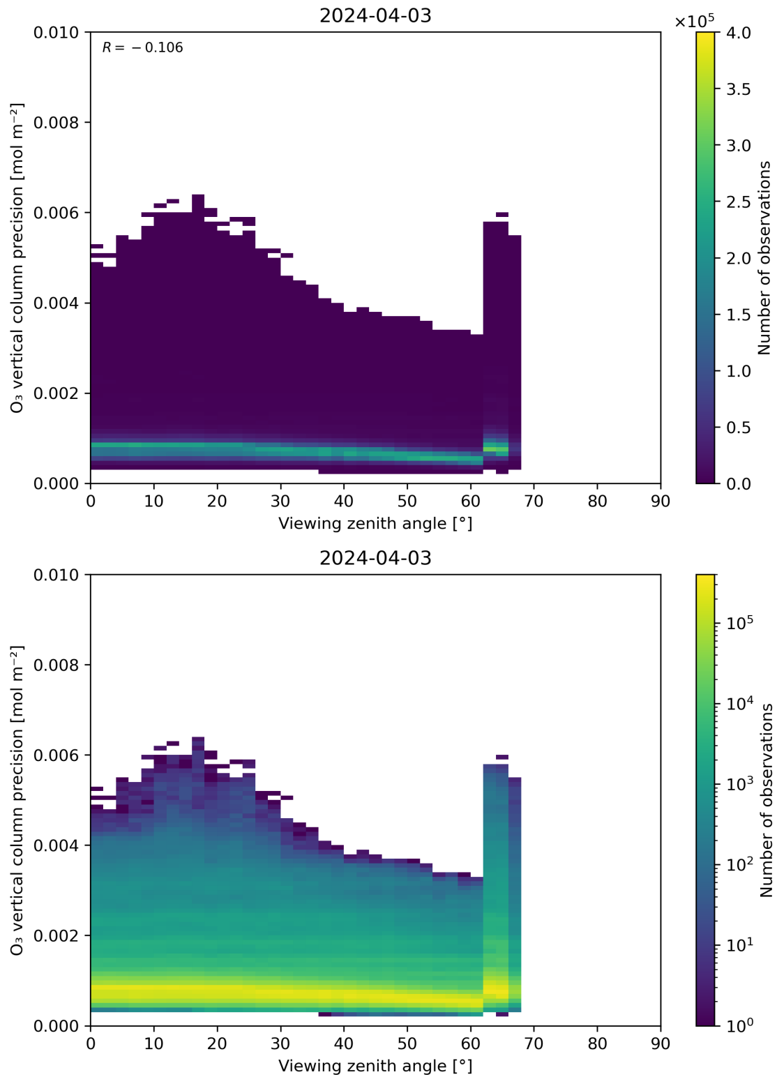
Figure 53: Scatter density plot of “Viewing zenith angle” against “O 3 vertical column precision” for 2024-04-02 to 2024-04-04.
