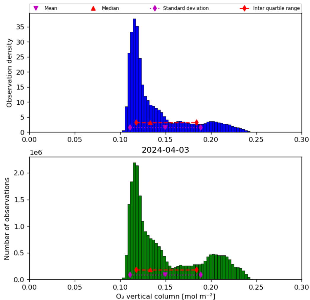
Figure 21: Histogram of “O 3 vertical column” for 2024-04-02 to 2024-04-04
