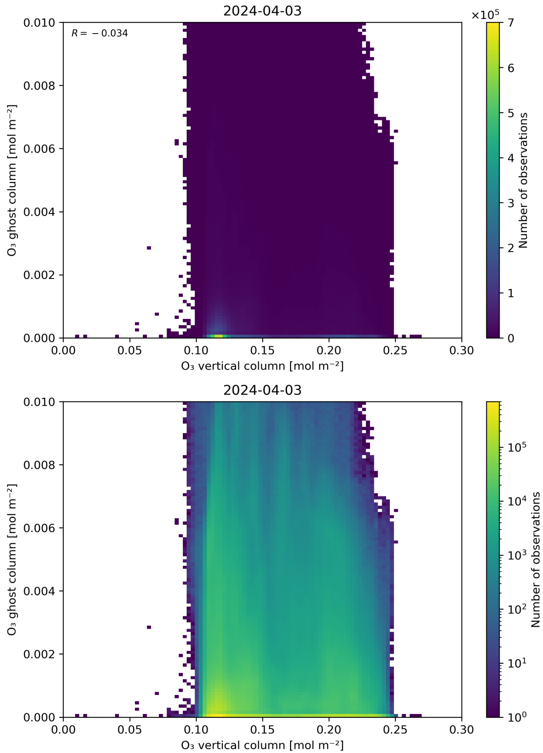
Figure 40: Scatter density plot of “O 3 vertical column” against “O 3 ghost column” for 2024-04-02 to 2024-04-04.
