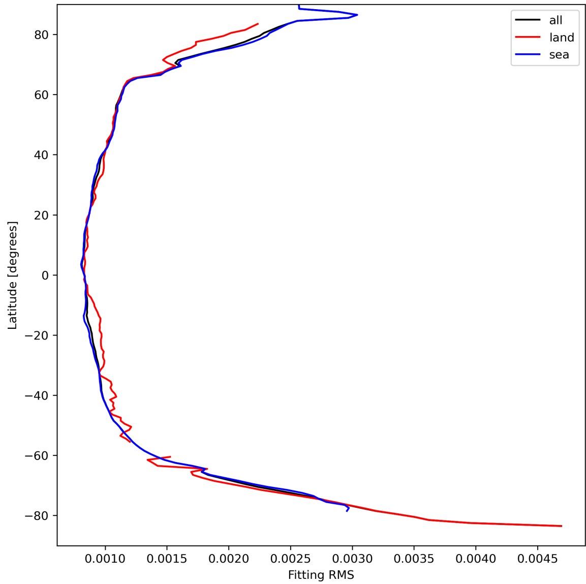
Figure 16: Zonal average of “Fitting RMS” for 2024-04-02 to 2024-04-04.
