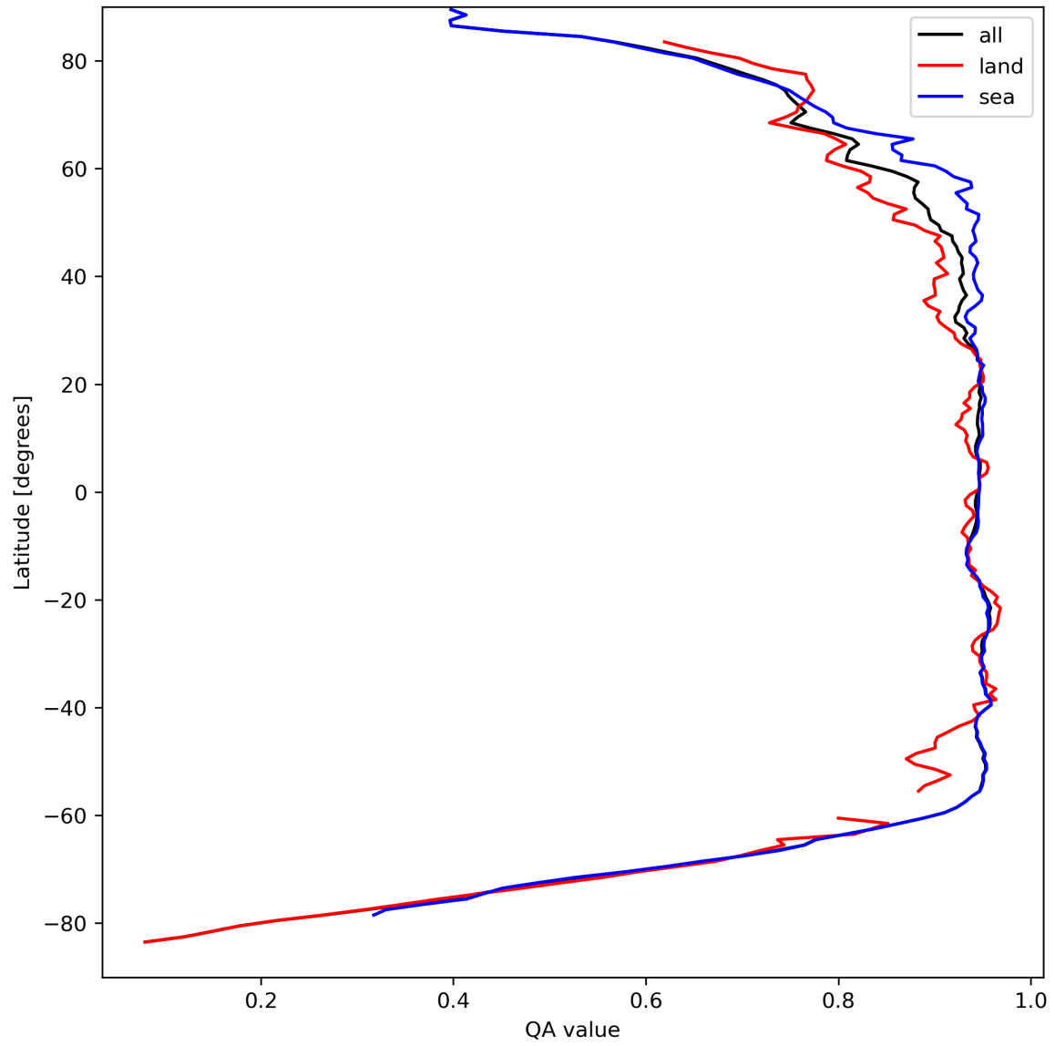
Figure 13: Zonal average of “QA value” for 2024-04-02 to 2024-04-04.
