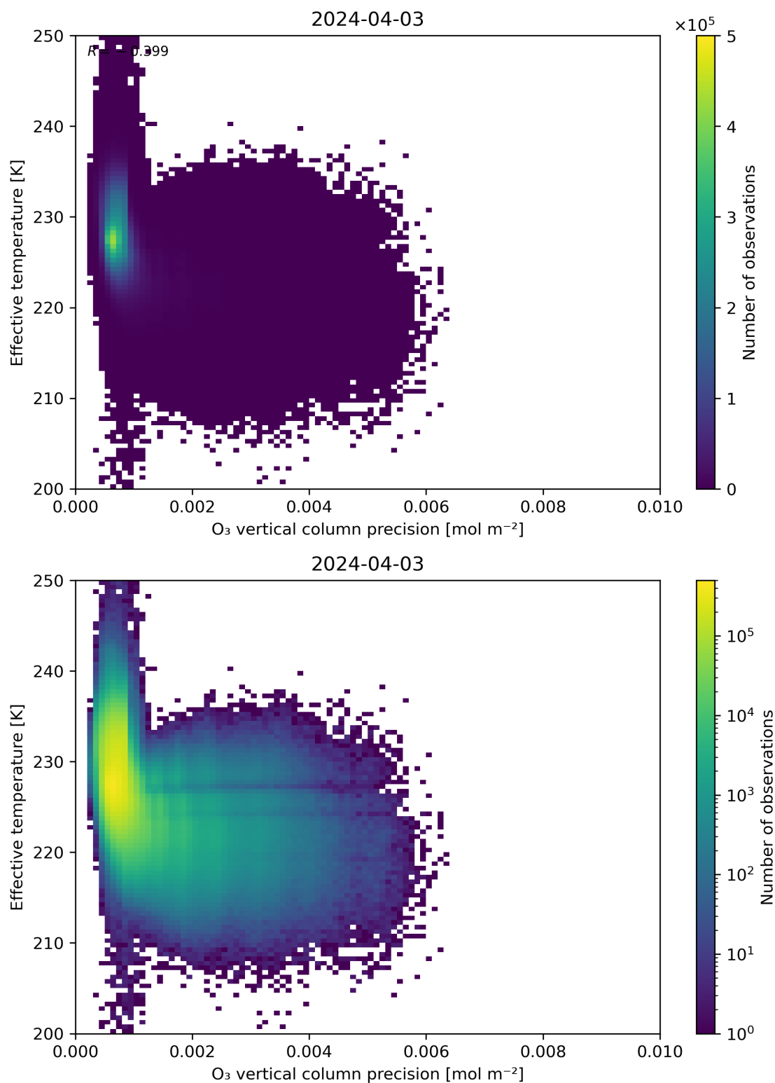
Figure 42: Scatter density plot of “O 3 vertical column precision” against “Effective temperature” for 2024-04-02 to 2024-04-04.
