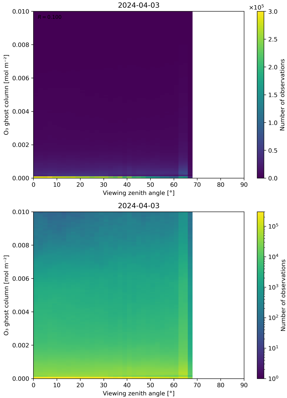
Figure 51: Scatter density plot of “Viewing zenith angle” against “O 3 ghost column” for 2024-04-02 to 2024-04-04.
