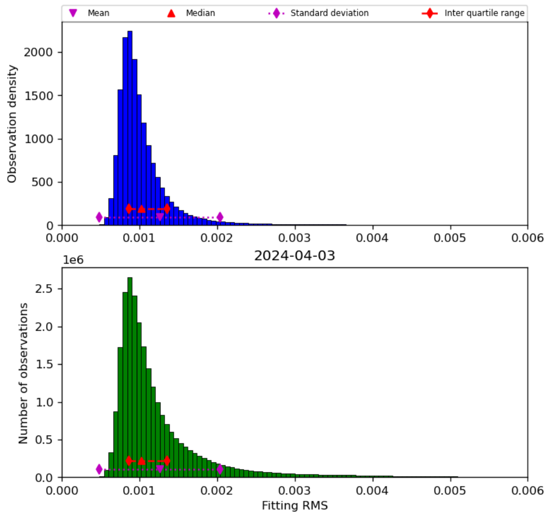
Figure 23: Histogram of “Fitting RMS” for 2024-04-02 to 2024-04-04
