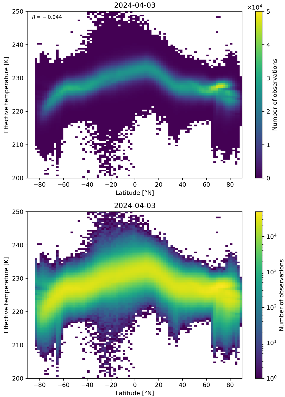
Figure 34: Scatter density plot of “Latitude” against “Effective temperature” for 2024-04-02 to 2024-04-04.
