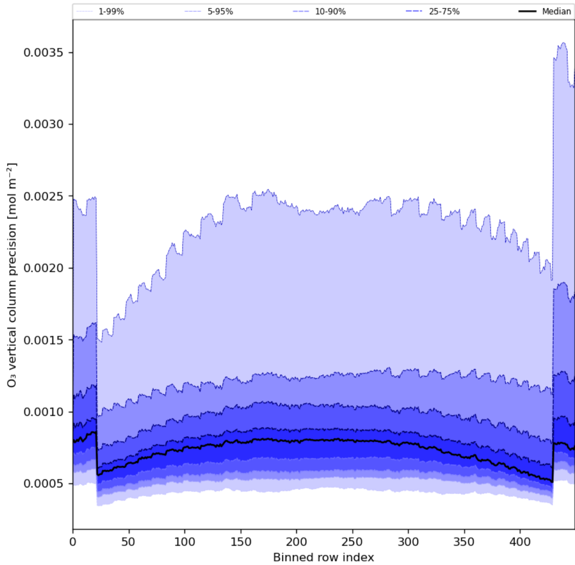
Figure 29: Along track statistics of “O 3 vertical column precision” for 2024-04-02 to 2024-04-04
