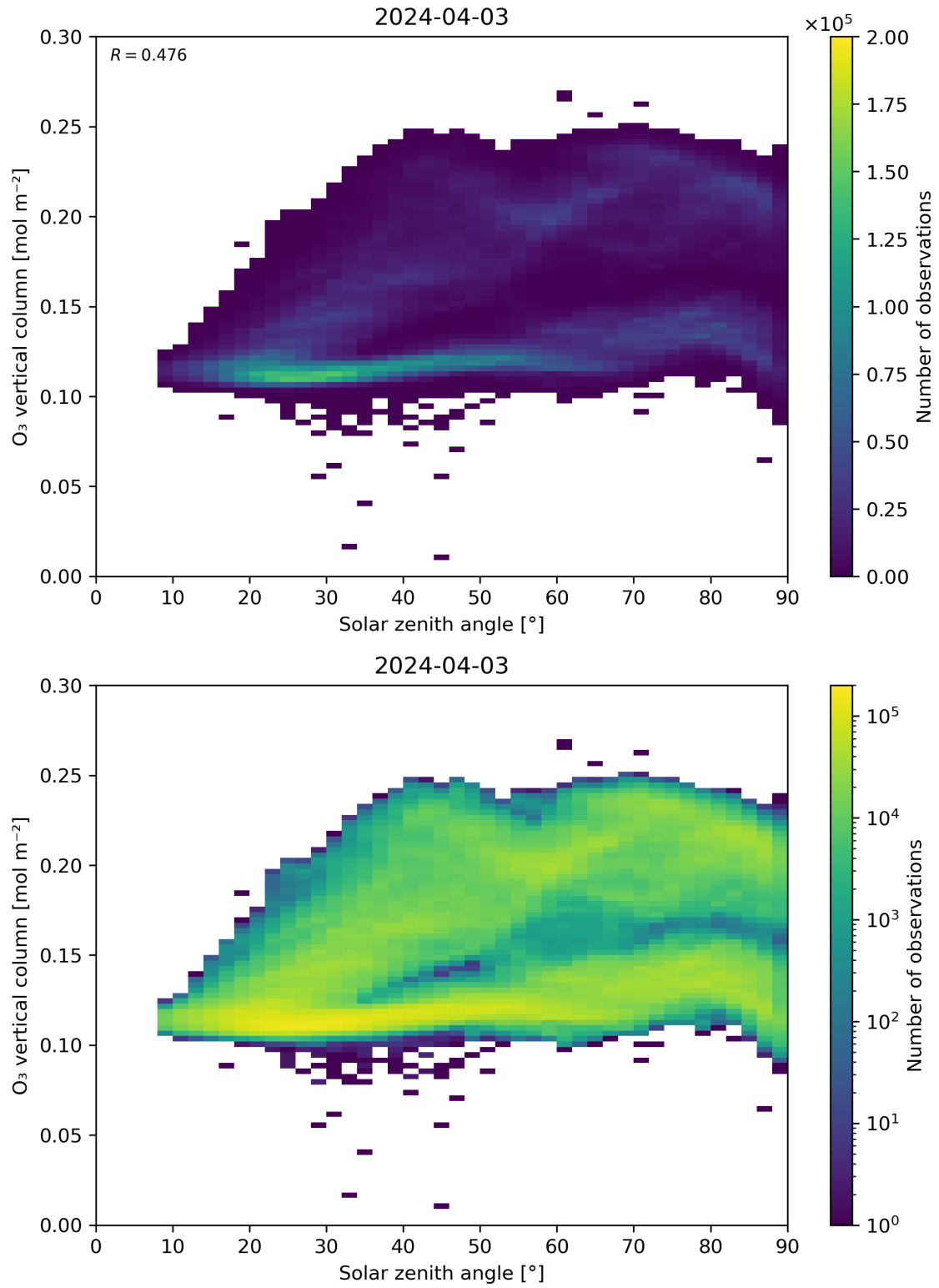
Figure 47: Scatter density plot of “Solar zenith angle” against “O 3 vertical column” for 2024-04-02 to 2024-04-04.
