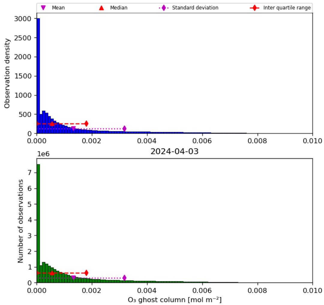
Figure 25: Histogram of “O 3 ghost column” for 2024-04-02 to 2024-04-04
