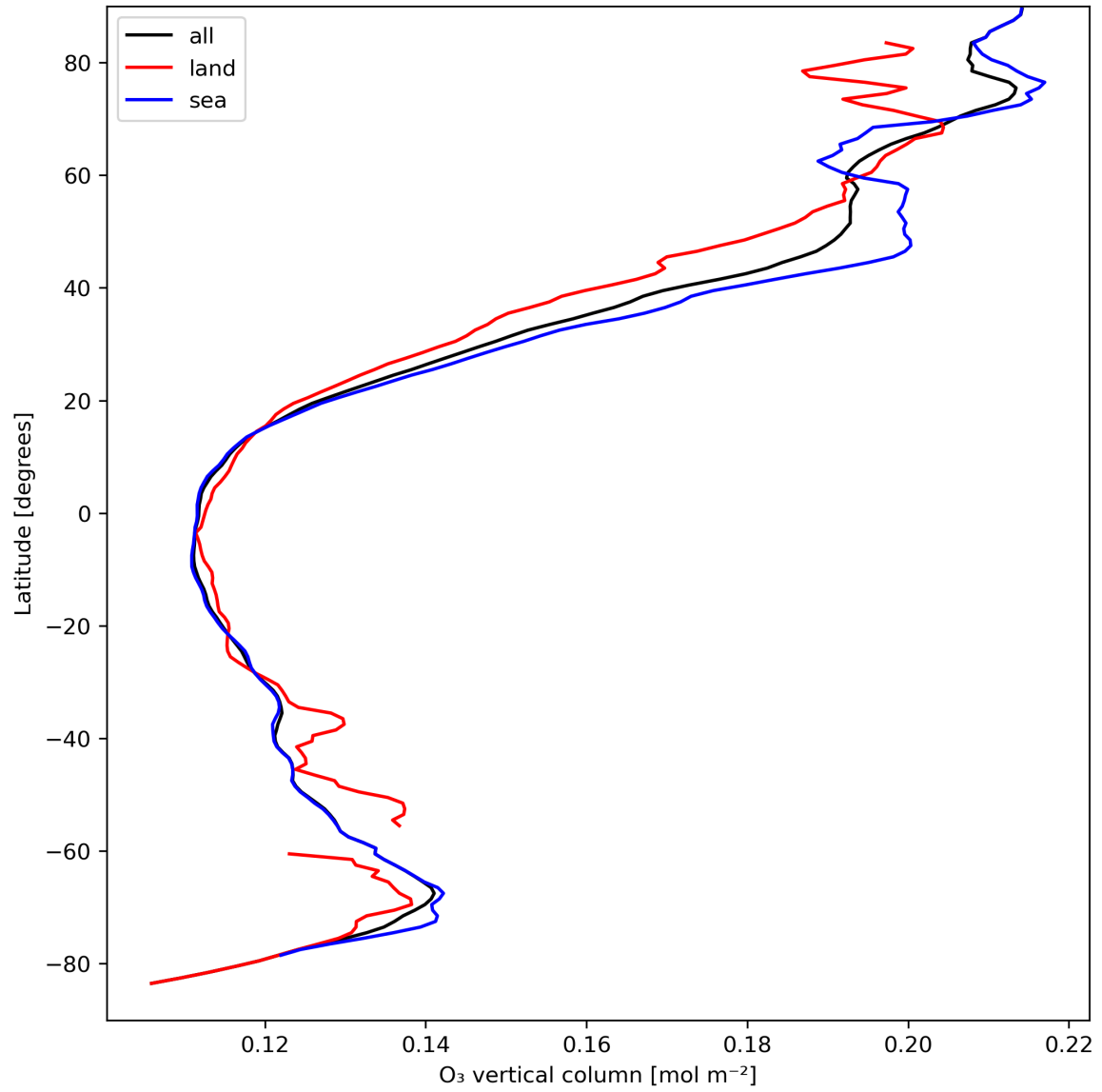
Figure 14: Zonal average of “O 3 vertical column” for 2024-04-02 to 2024-04-04.
