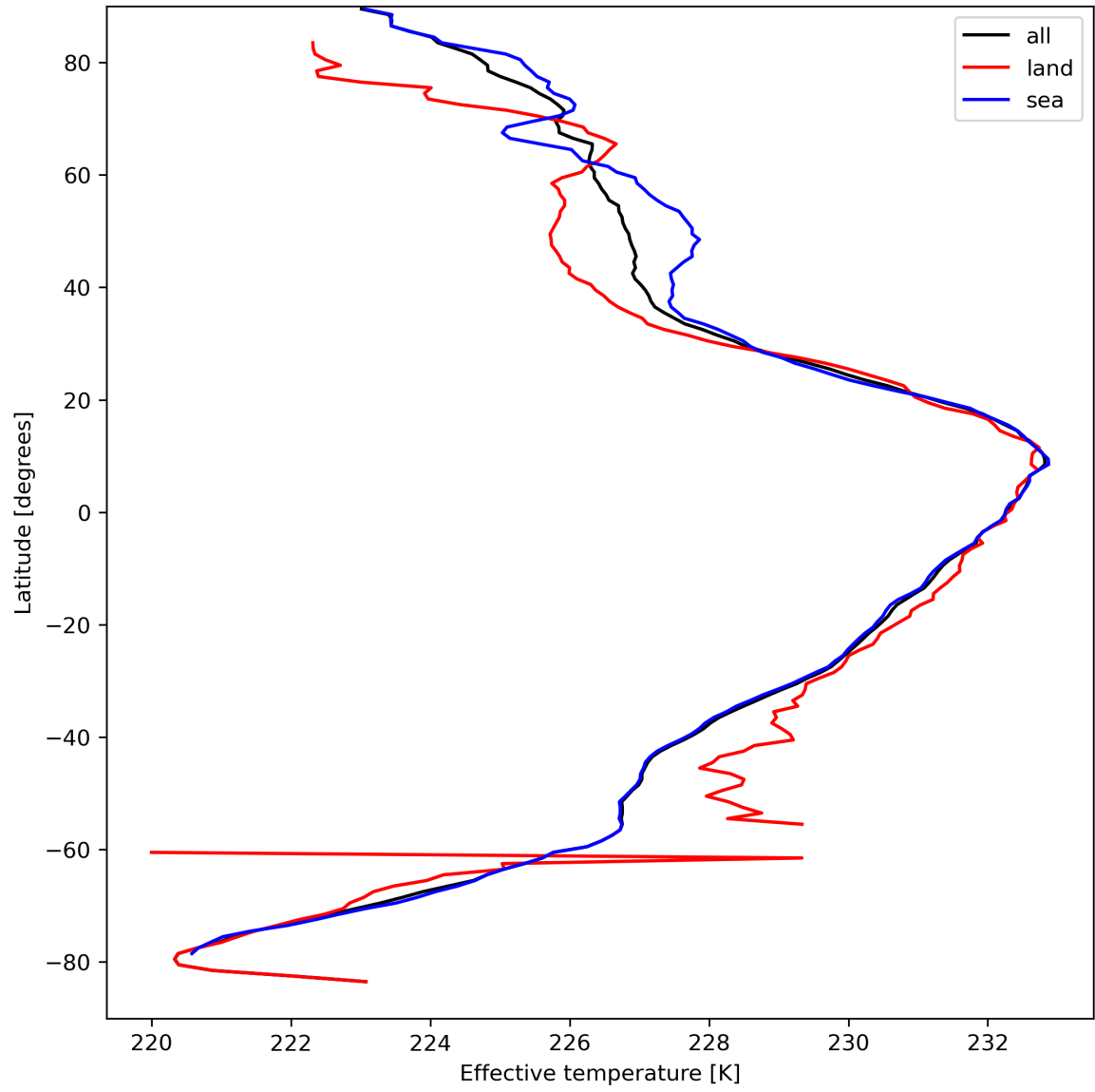
Figure 17: Zonal average of “Effective temperature” for 2024-04-02 to 2024-04-04.
