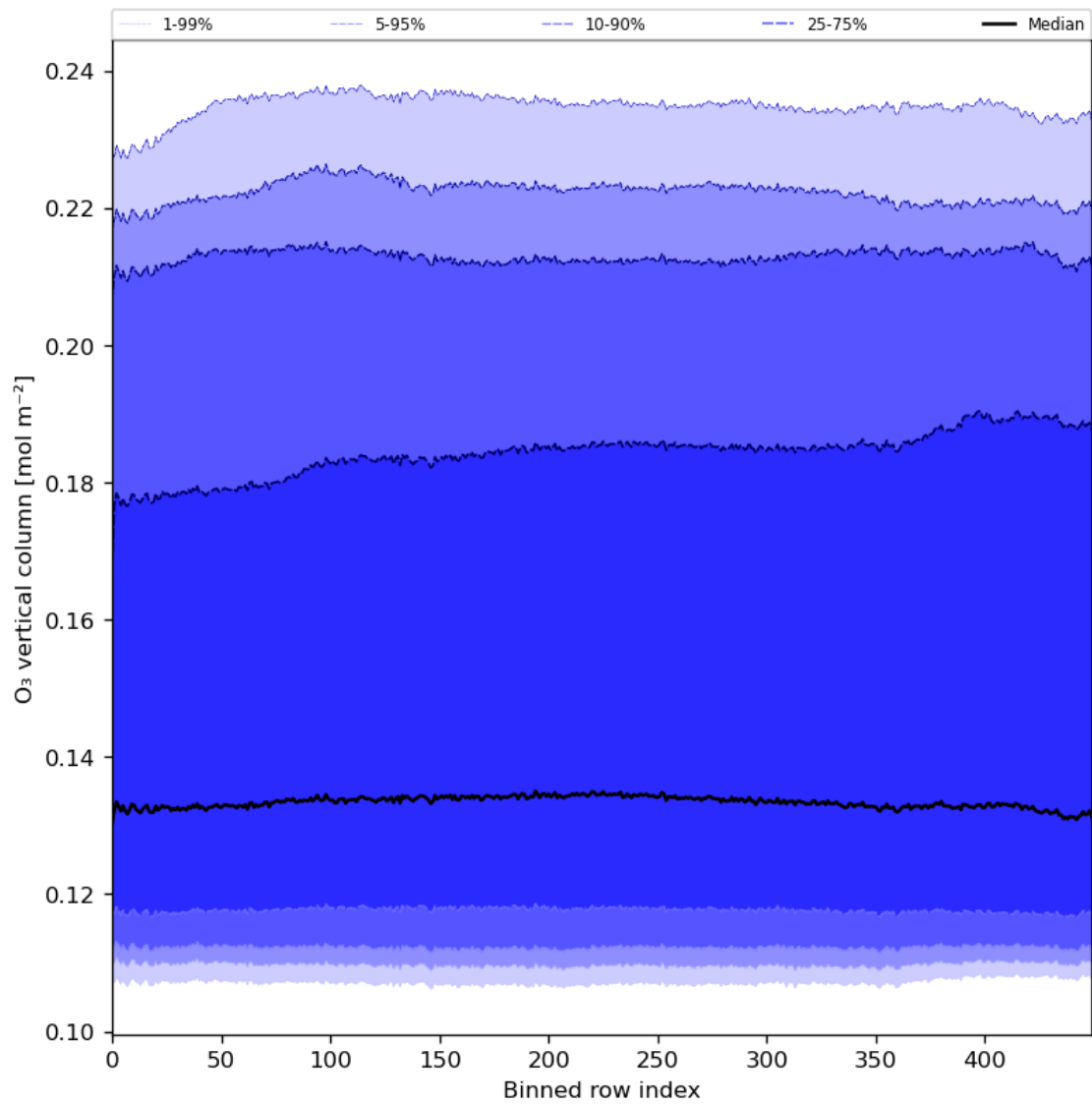
Figure 28: Along track statistics of “O 3 vertical column” for 2024-04-02 to 2024-04-04
