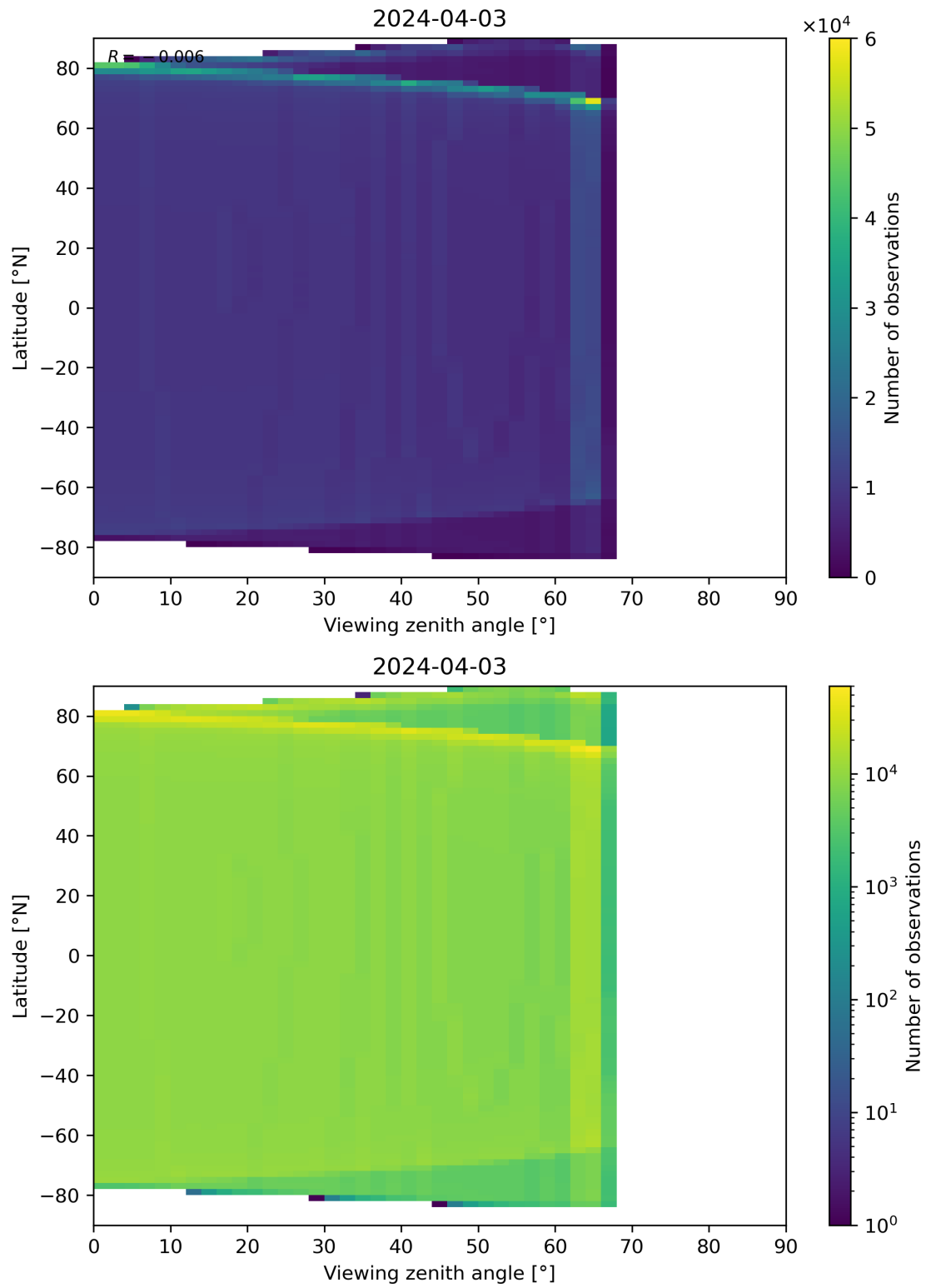
Figure 49: Scatter density plot of “Viewing zenith angle” against “Latitude” for 2024-04-02 to 2024-04-04.
