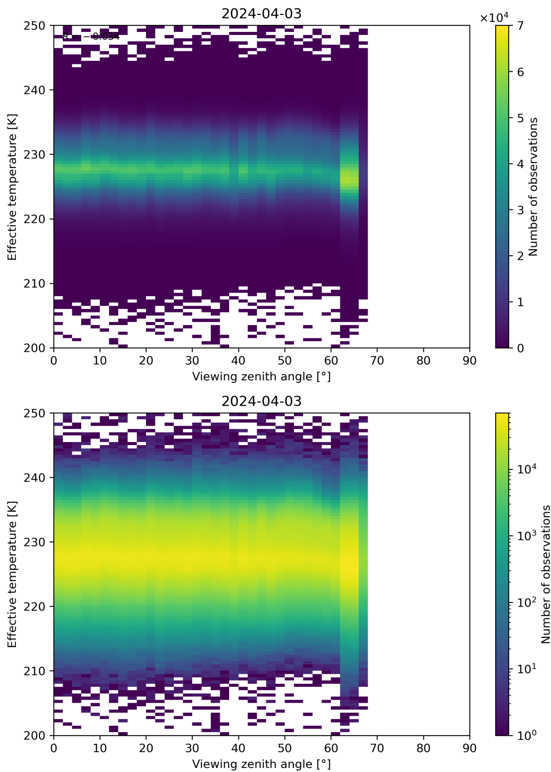
Figure 50: Scatter density plot of “Viewing zenith angle” against “Effective temperature” for 2024-04-02 to 2024-04-04.
