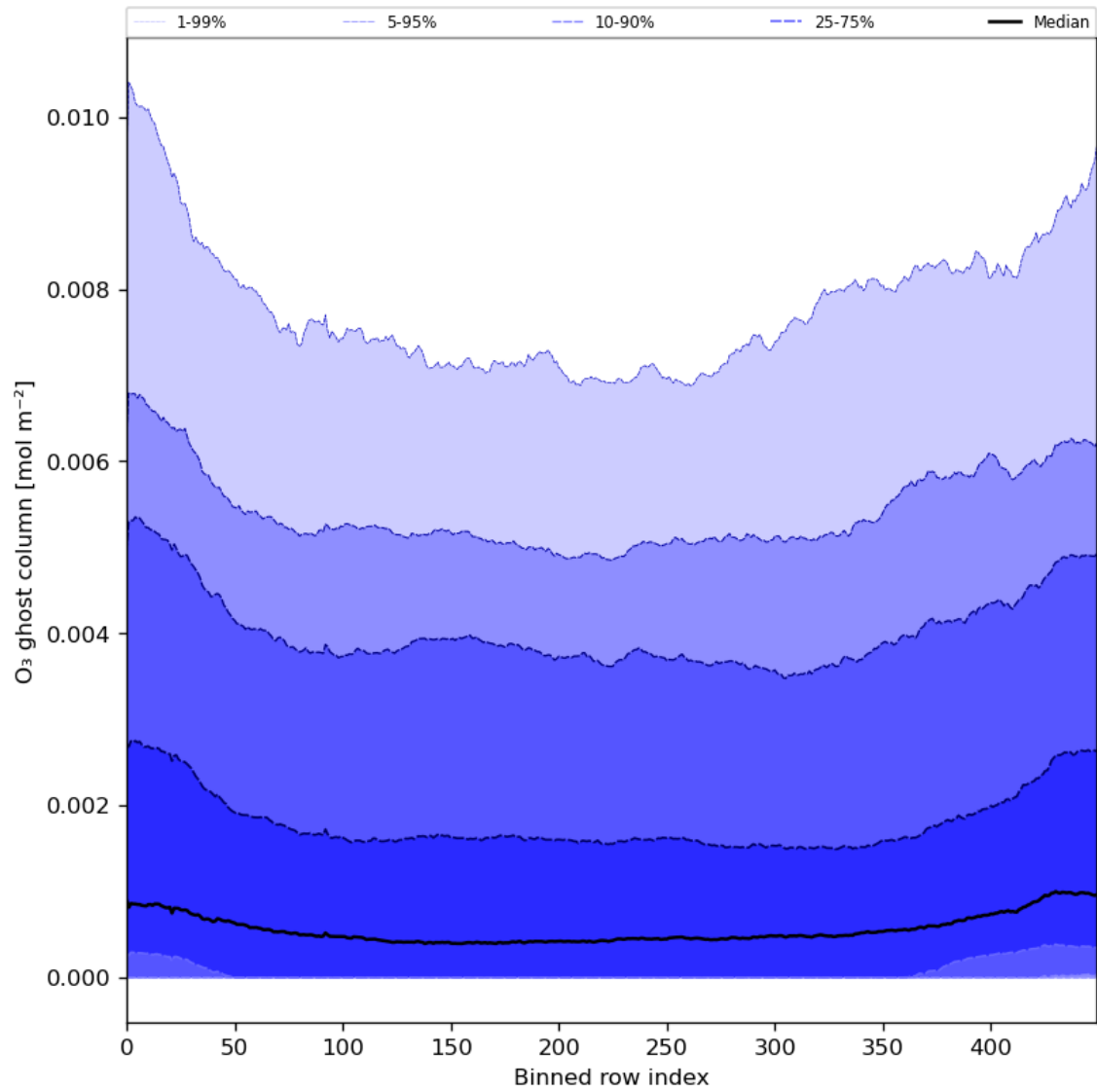
Figure 32: Along track statistics of “O 3 ghost column” for 2024-04-02 to 2024-04-04
