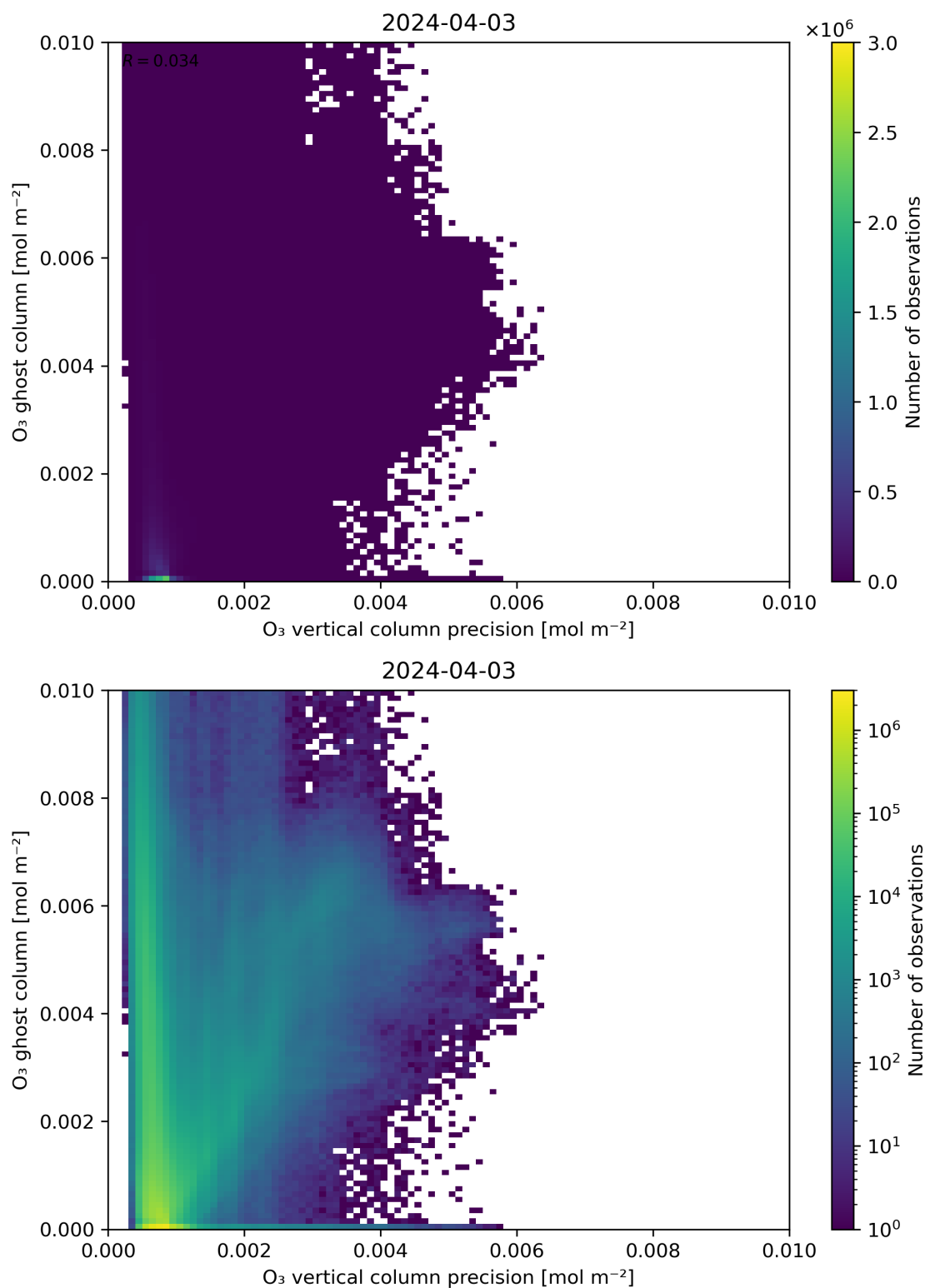
Figure 43: Scatter density plot of “ \text{O}_3 vertical column precision” against “ \text{O}_3 ghost column” for 2024-04-02 to 2024-04-04.
