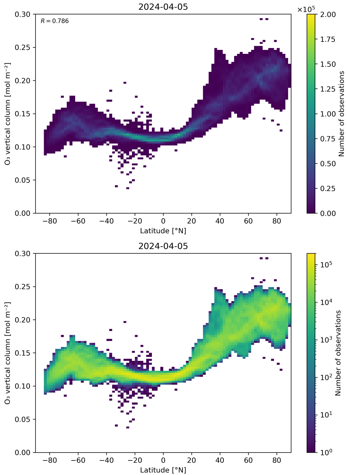
Figure 36: Scatter density plot of “Latitude” against “O 3 vertical column” for 2024-04-05 to 2024-04-06.
