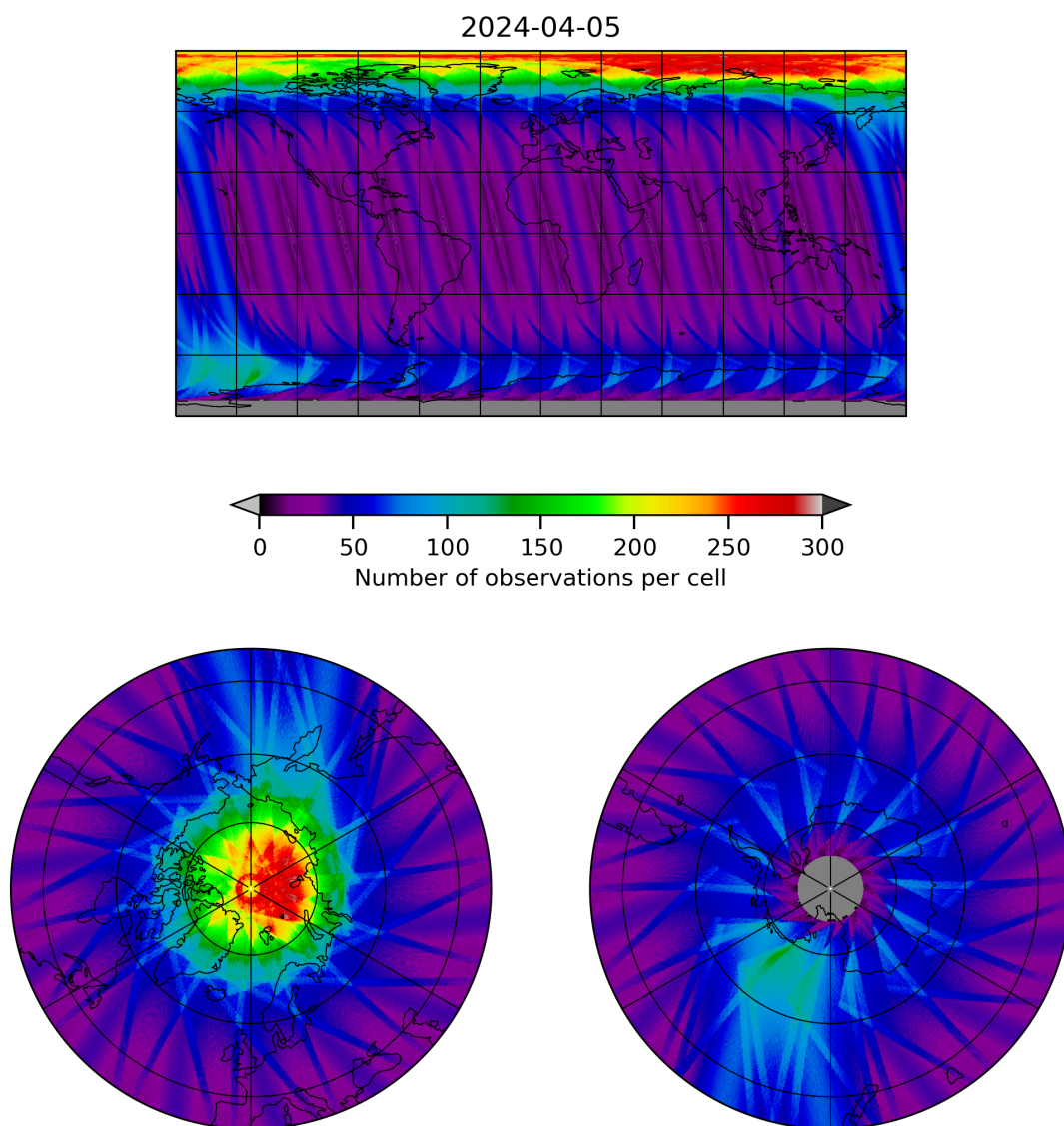
Figure 12: Map of the number of observations for 2024-04-05 to 2024-04-06
