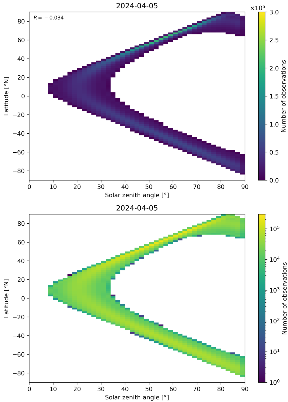
Figure 44: Scatter density plot of “Solar zenith angle” against “Latitude” for 2024-04-05 to 2024-04-06.
