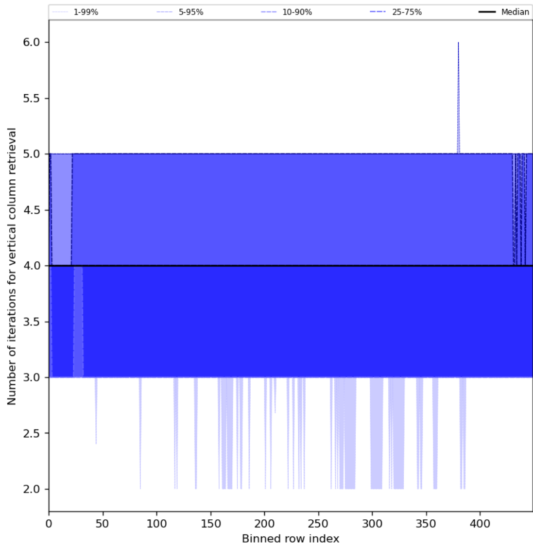
Figure 33: Along track statistics of “Number of iterations for vertical column retrieval” for 2024-04-05 to 2024-04-06
