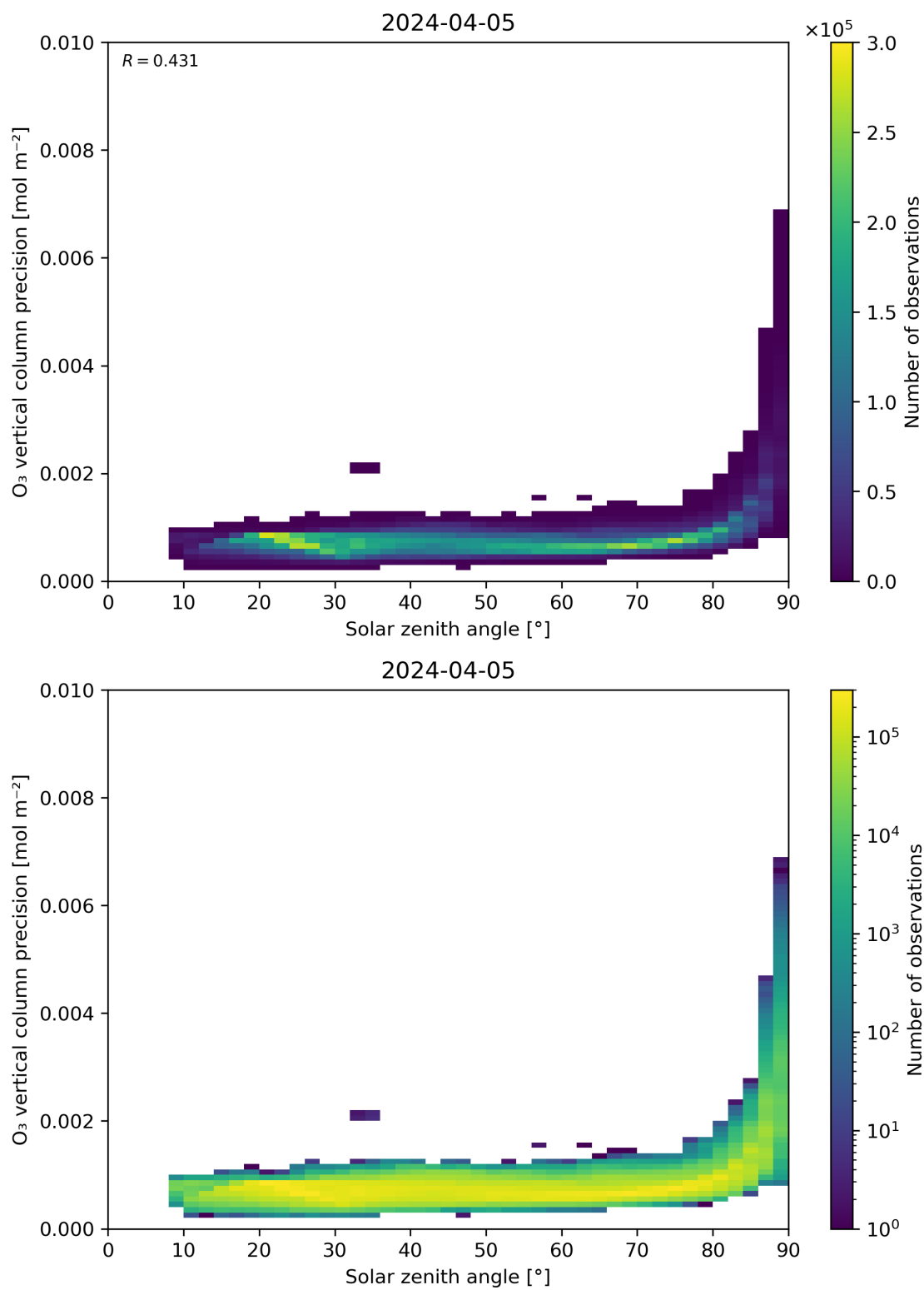
Figure 48: Scatter density plot of “Solar zenith angle” against “O 3 vertical column precision” for 2024-04-05 to 2024-04-06.
