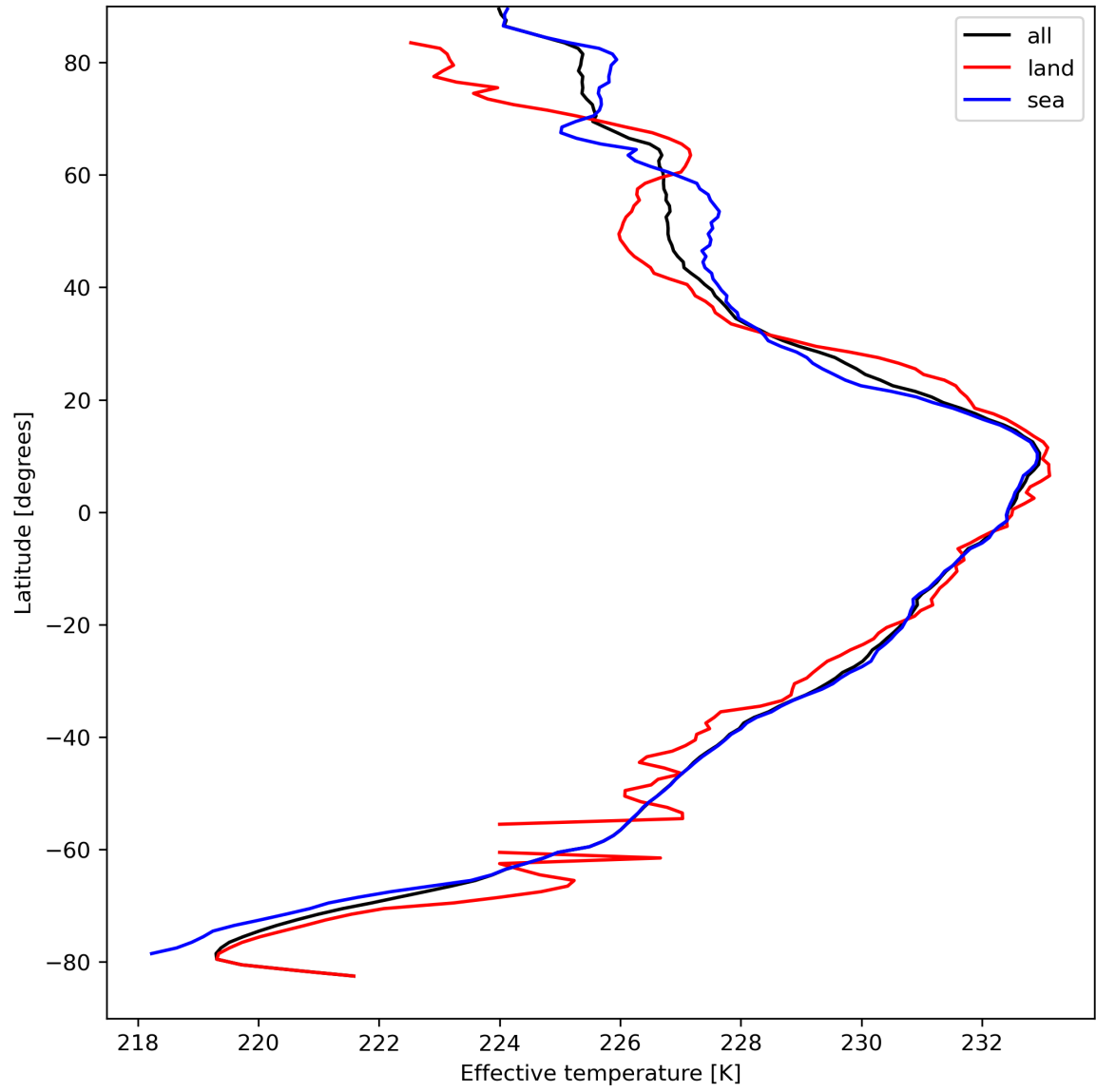
Figure 17: Zonal average of "Effective temperature" for 2024-04-05 to 2024-04-06.
