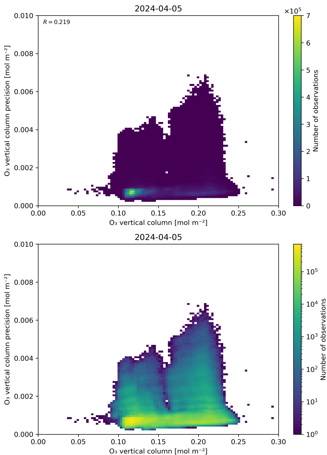
Figure 41: Scatter density plot of “O 3 vertical column” against “O 3 vertical column precision” for 2024-04-05 to 2024-04-06.
