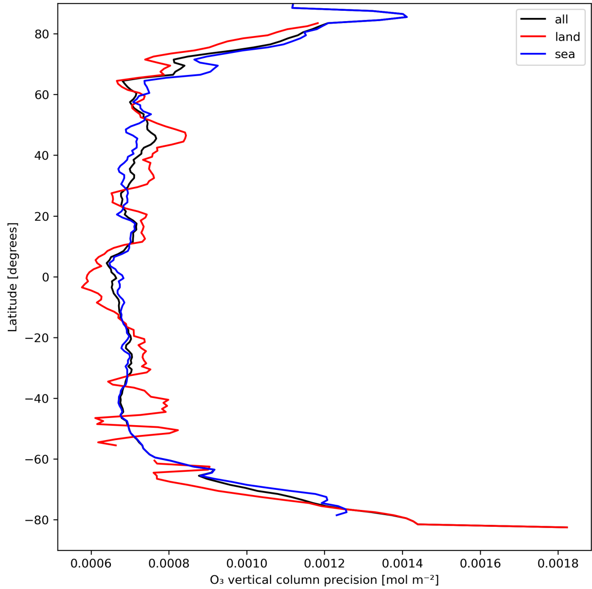
Figure 15: Zonal average of "O 3 vertical column precision" for 2024-04-05 to 2024-04-06.
