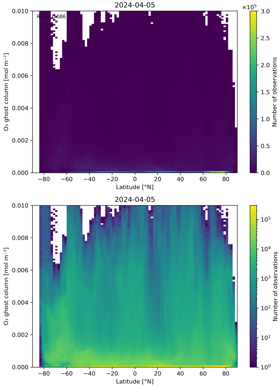
Figure 35: Scatter density plot of “Latitude” against “O 3 ghost column” for 2024-04-05 to 2024-04-06.
