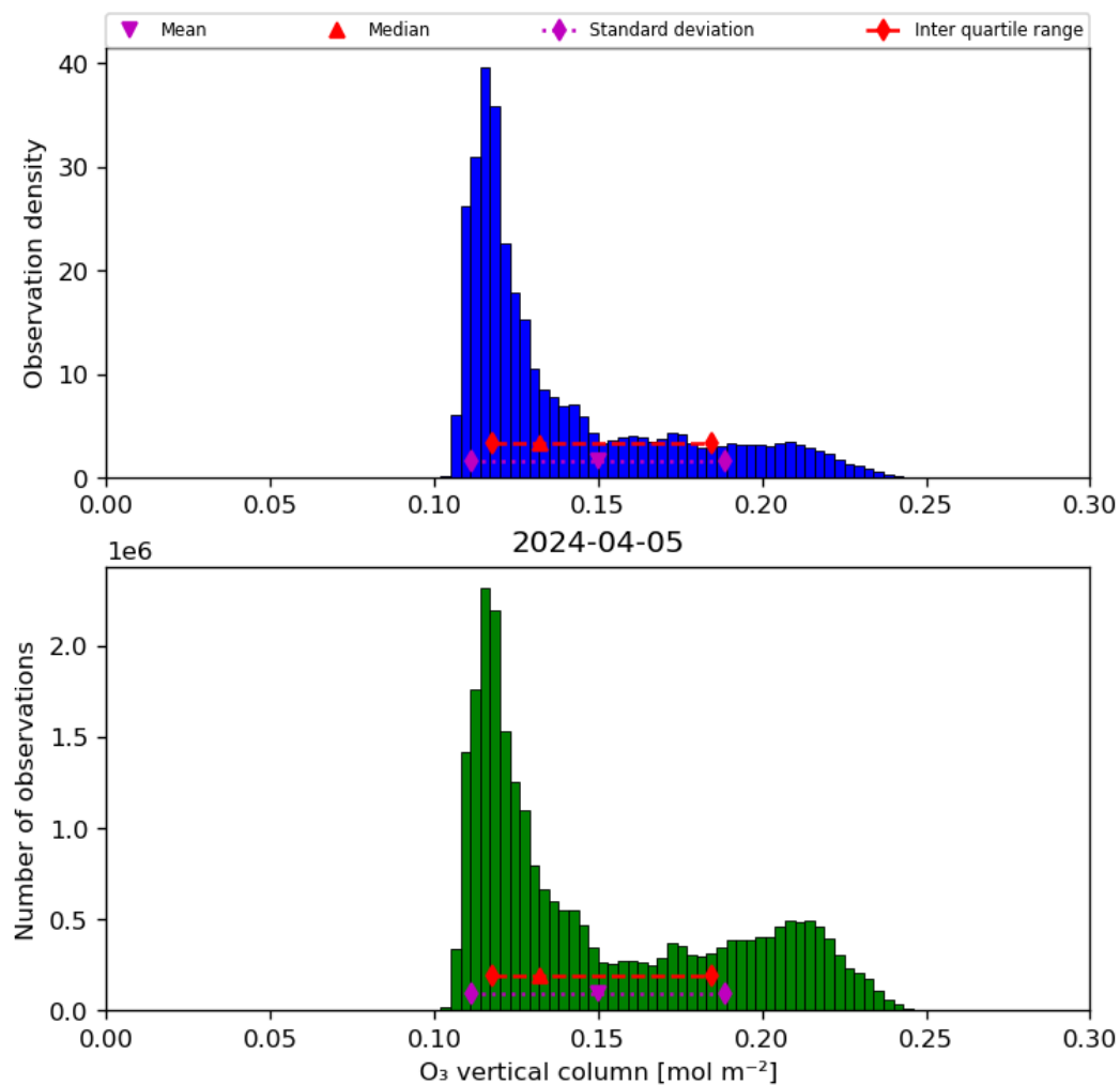
Figure 21: Histogram of “O 3 vertical column” for 2024-04-05 to 2024-04-06
