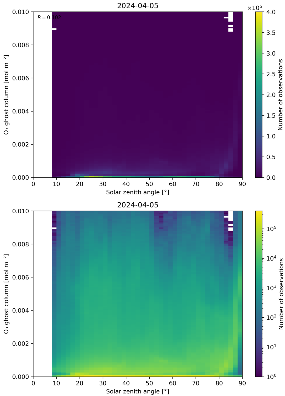
Figure 46: Scatter density plot of “Solar zenith angle” against “O 3 ghost column” for 2024-04-05 to 2024-04-06.
