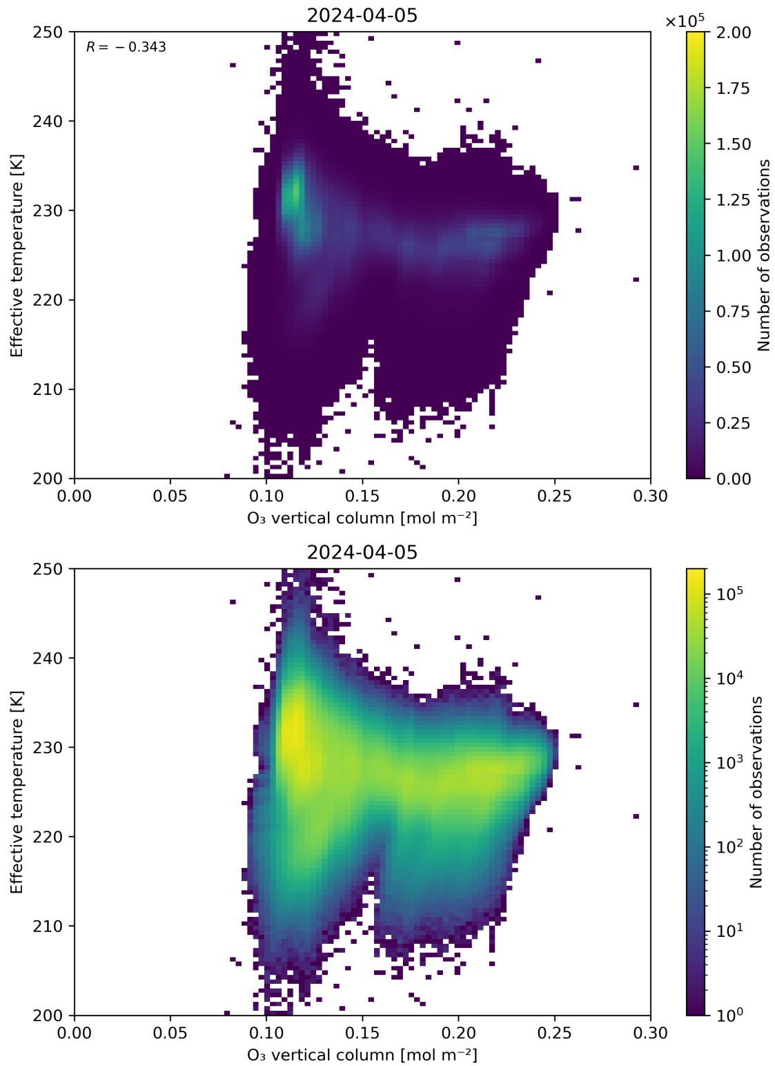
Figure 39: Scatter density plot of “O 3 vertical column” against “Effective temperature” for 2024-04-05 to 2024-04-06.
