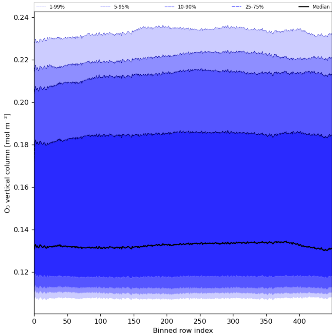
Figure 28: Along track statistics of “O 3 vertical column” for 2024-04-05 to 2024-04-06
