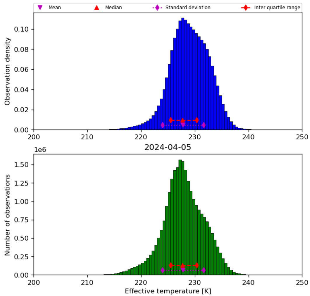
Figure 24: Histogram of “Effective temperature” for 2024-04-05 to 2024-04-06
