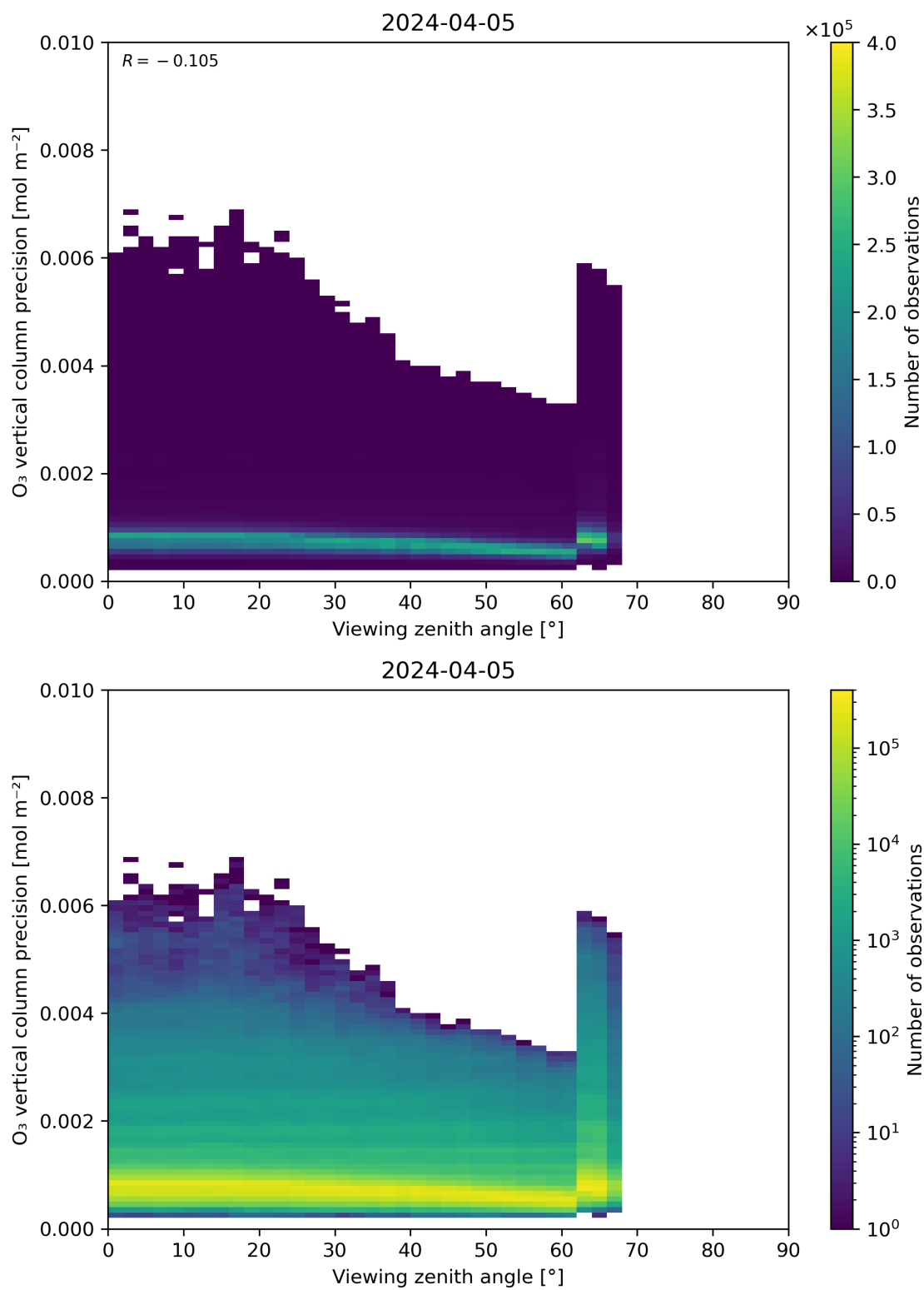
Figure 53: Scatter density plot of “Viewing zenith angle” against “O 3 vertical column precision” for 2024-04-05 to 2024-04-06.
