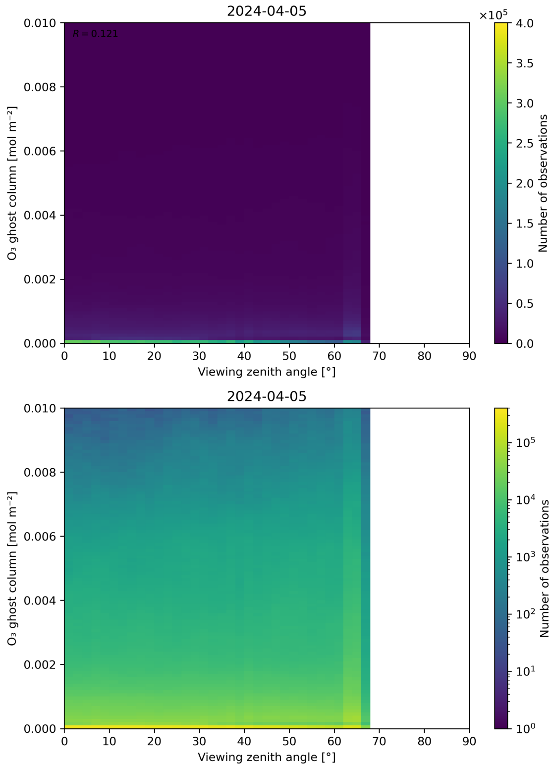
Figure 51: Scatter density plot of “Viewing zenith angle” against “O 3 ghost column” for 2024-04-05 to 2024-04-06.
