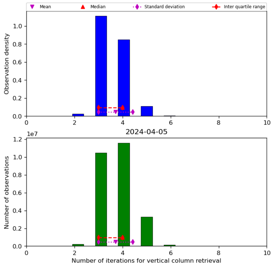
Figure 26: Histogram of “Number of iterations for vertical column retrieval” for 2024-04-05 to 2024-04-06
