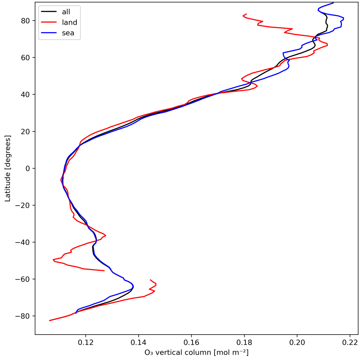
Figure 14: Zonal average of “O 3 vertical column” for 2024-04-05 to 2024-04-06.
