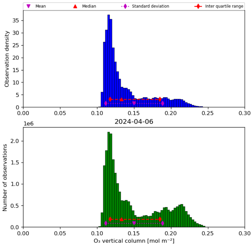
Figure 21: Histogram of “O 3 vertical column” for 2024-04-05 to 2024-04-07
