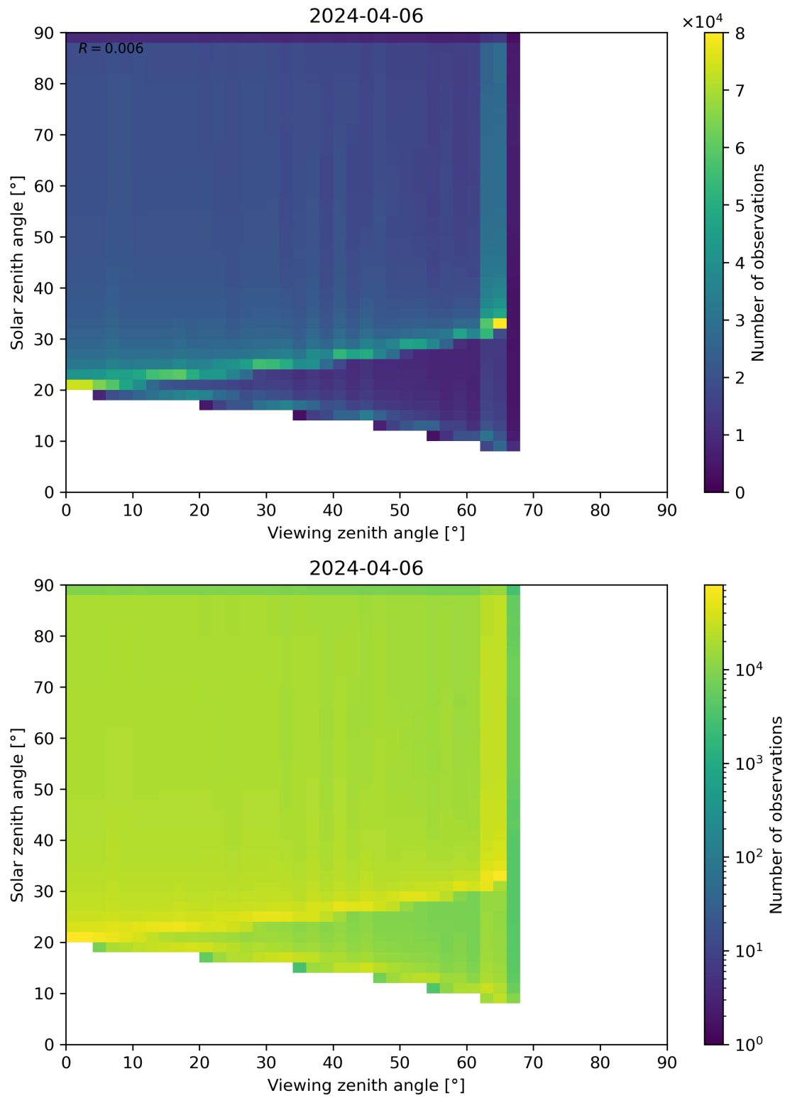
Figure 54: Scatter density plot of “Viewing zenith angle” against “Solar zenith angle” for 2024-04-05 to 2024-04-07.
