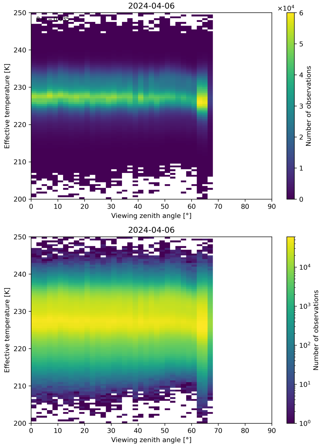
Figure 50: Scatter density plot of “Viewing zenith angle” against “Effective temperature” for 2024-04-05 to 2024-04-07.
