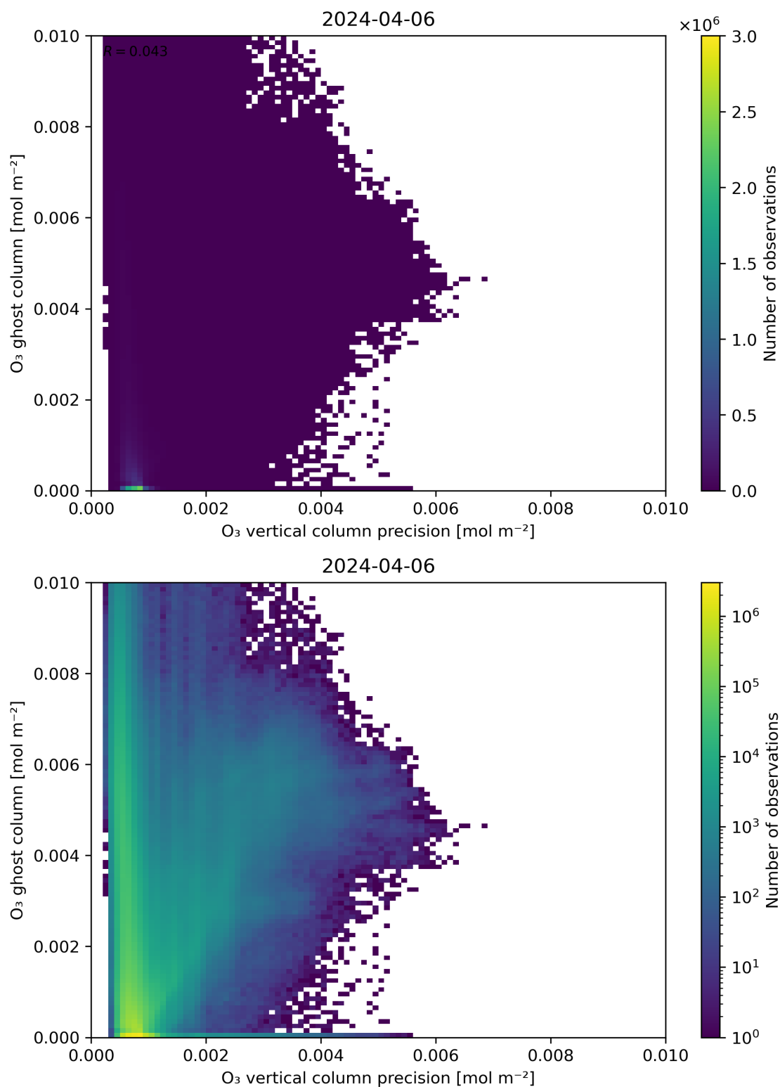
Figure 43: Scatter density plot of “ \text{O}_3 vertical column precision” against “ \text{O}_3 ghost column” for 2024-04-05 to 2024-04-07.
