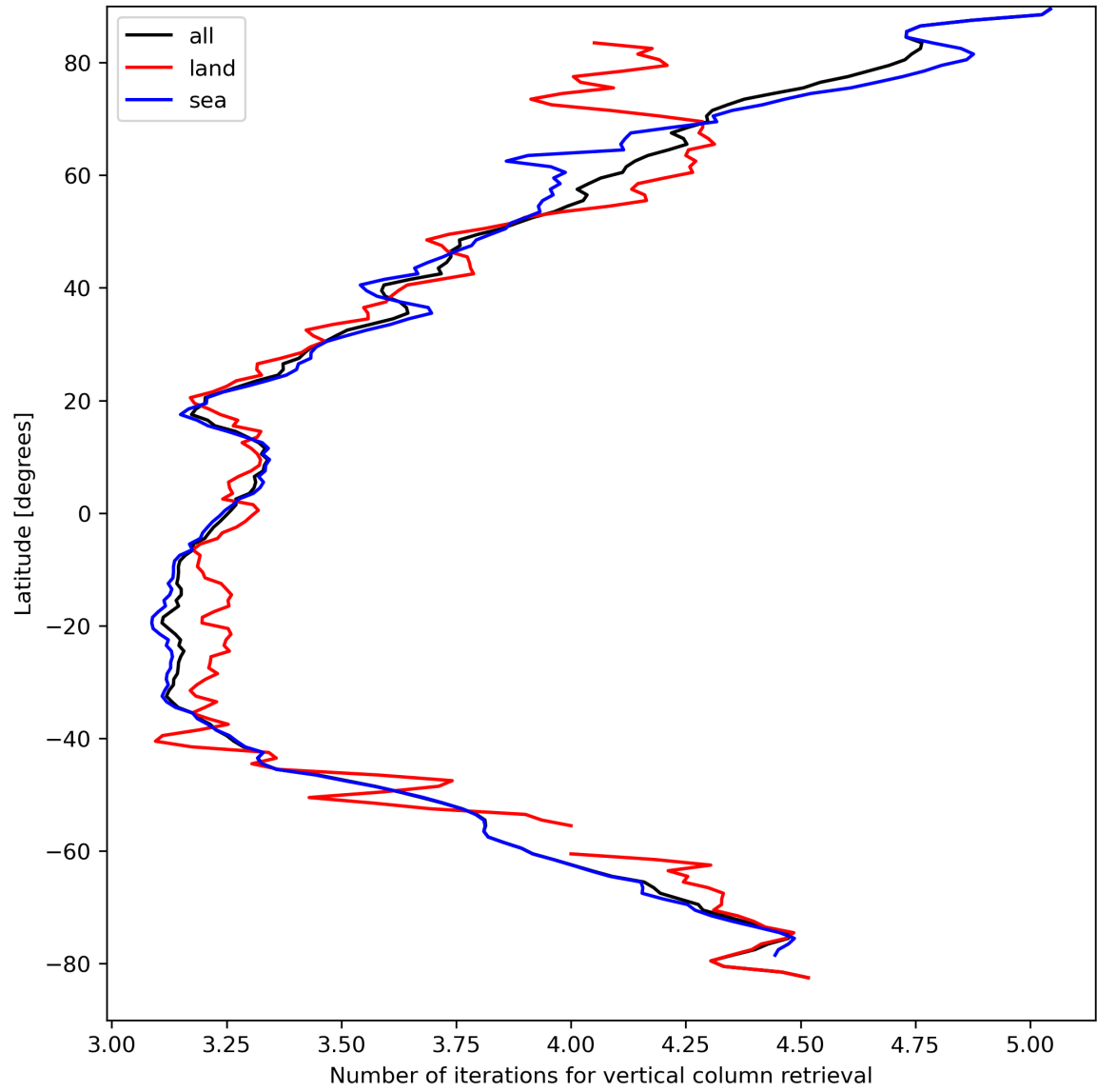
Figure 19: Zonal average of “Number of iterations for vertical column retrieval” for 2024-04-05 to 2024-04-07.
