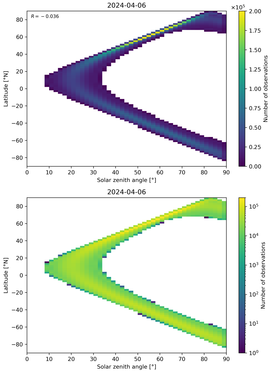
Figure 44: Scatter density plot of “Solar zenith angle” against “Latitude” for 2024-04-05 to 2024-04-07.
