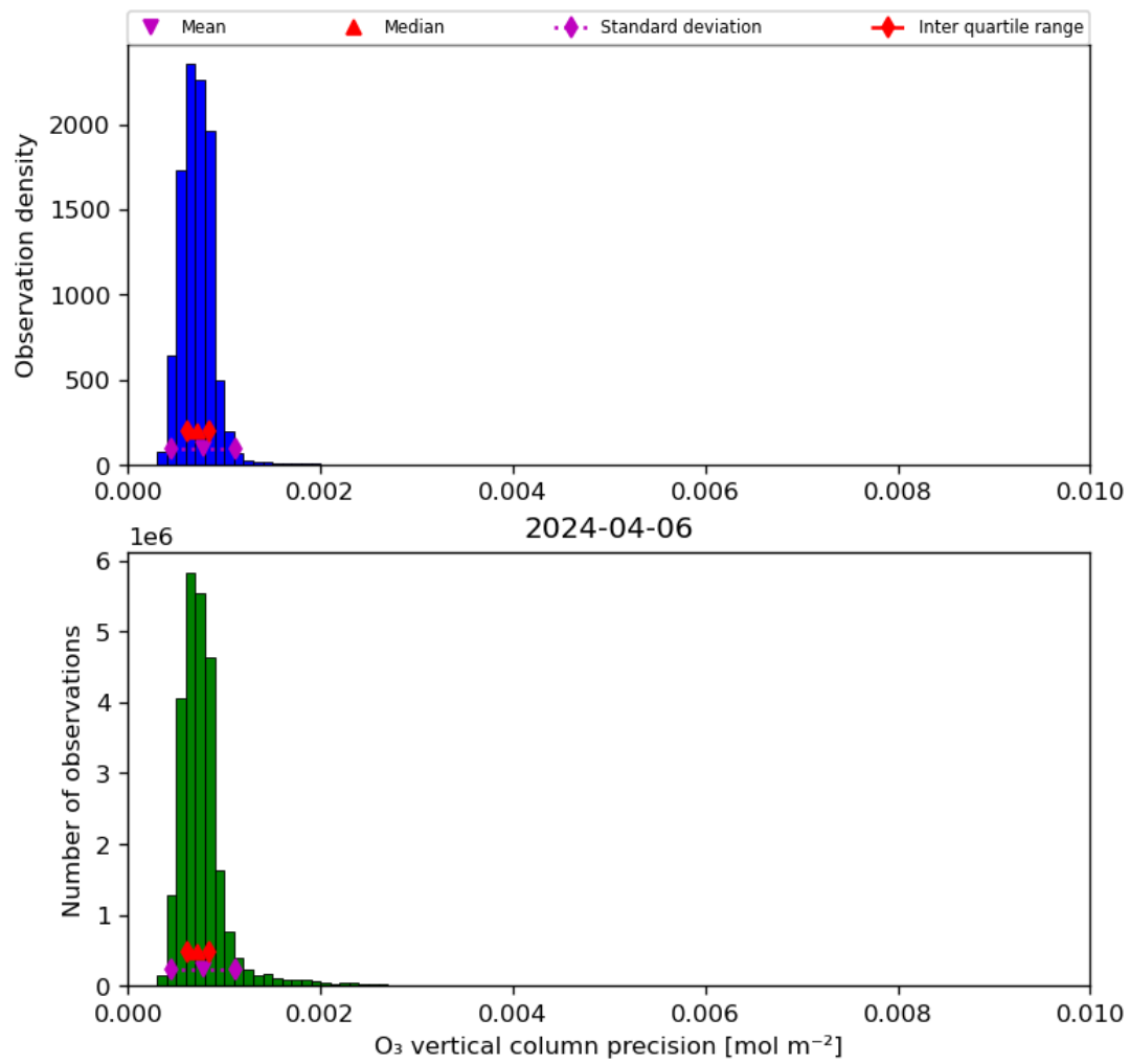
Figure 22: Histogram of “O 3 vertical column precision” for 2024-04-05 to 2024-04-07
