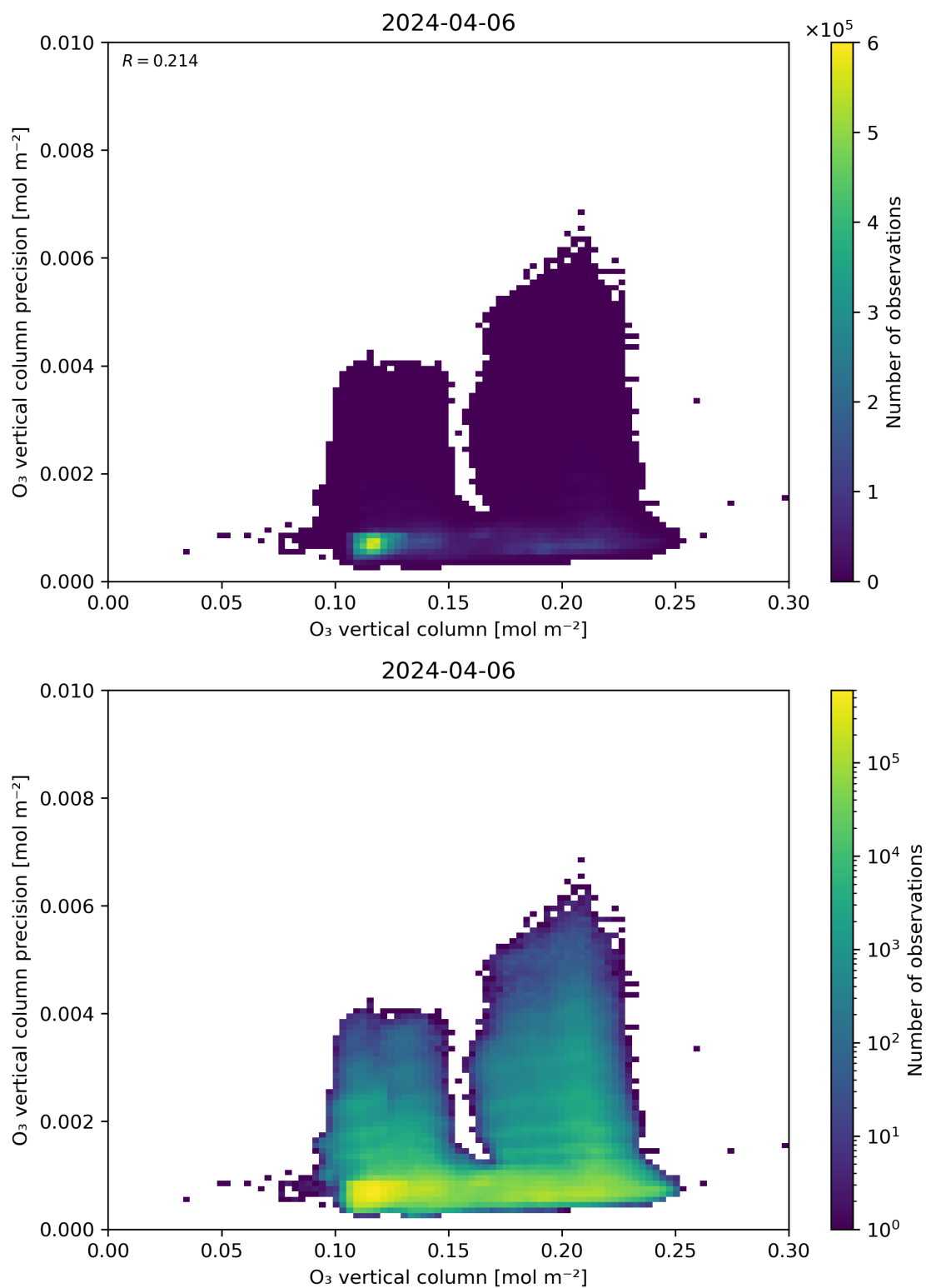
Figure 41: Scatter density plot of “O 3 vertical column” against “O 3 vertical column precision” for 2024-04-05 to 2024-04-07.
