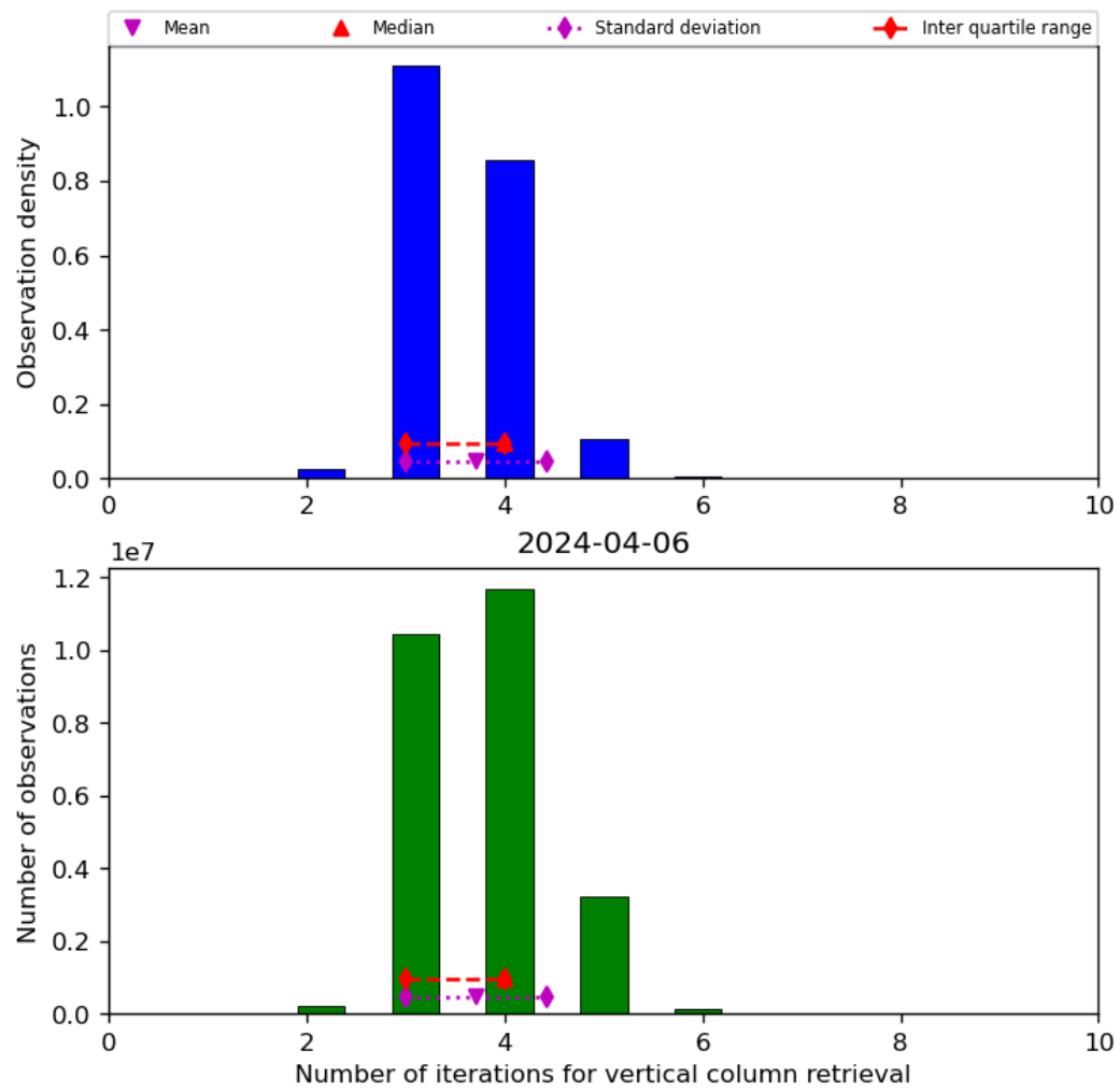
Figure 26: Histogram of “Number of iterations for vertical column retrieval” for 2024-04-05 to 2024-04-07
