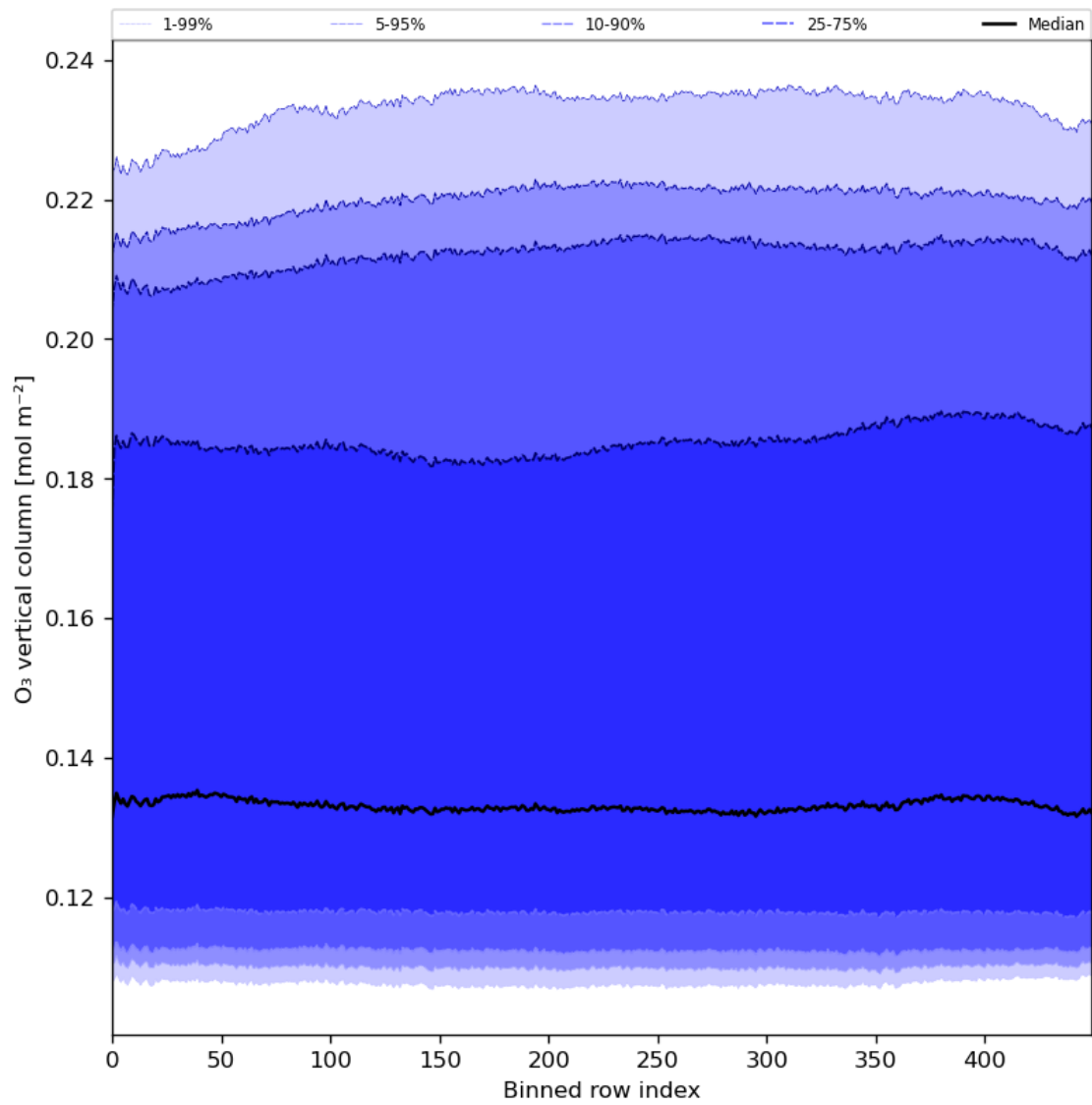
Figure 28: Along track statistics of “O 3 vertical column” for 2024-04-05 to 2024-04-07
