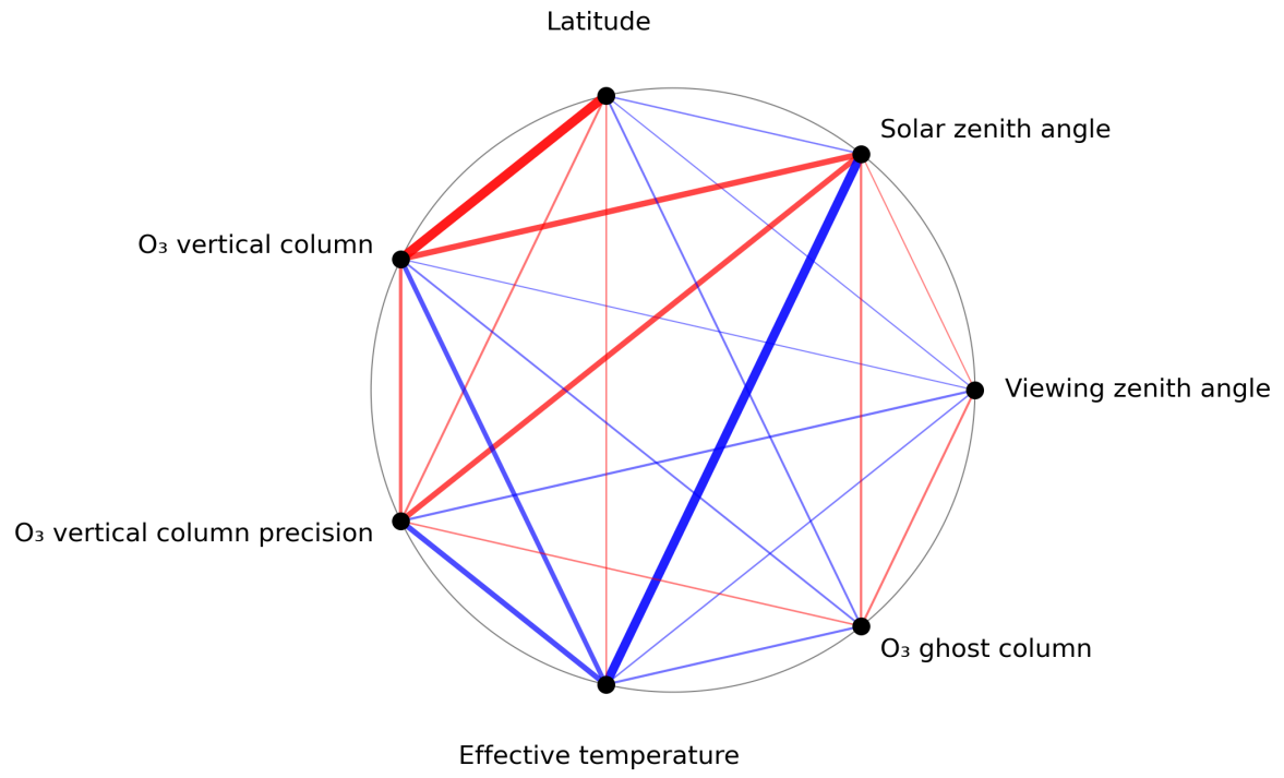
Figure 1: Map of correlation graph for 2024-04-05 to 2024-04-07.
