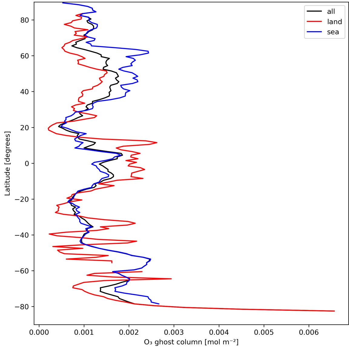
Figure 18: Zonal average of "O 3 ghost column" for 2024-04-05 to 2024-04-07.
