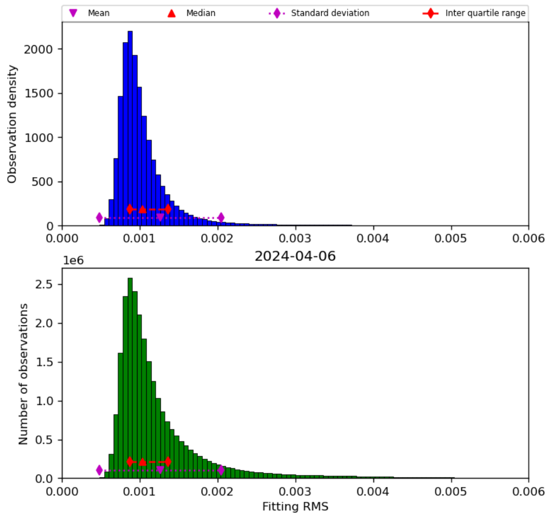
Figure 23: Histogram of “Fitting RMS” for 2024-04-05 to 2024-04-07
