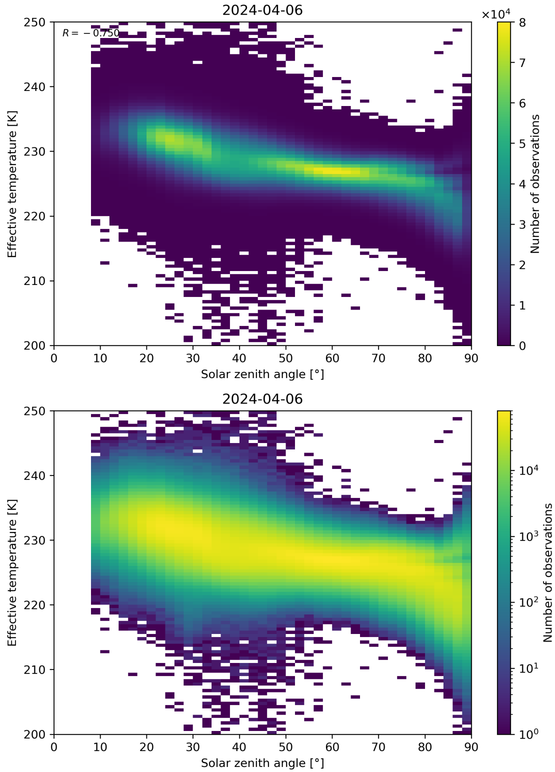
Figure 45: Scatter density plot of “Solar zenith angle” against “Effective temperature” for 2024-04-05 to 2024-04-07.
