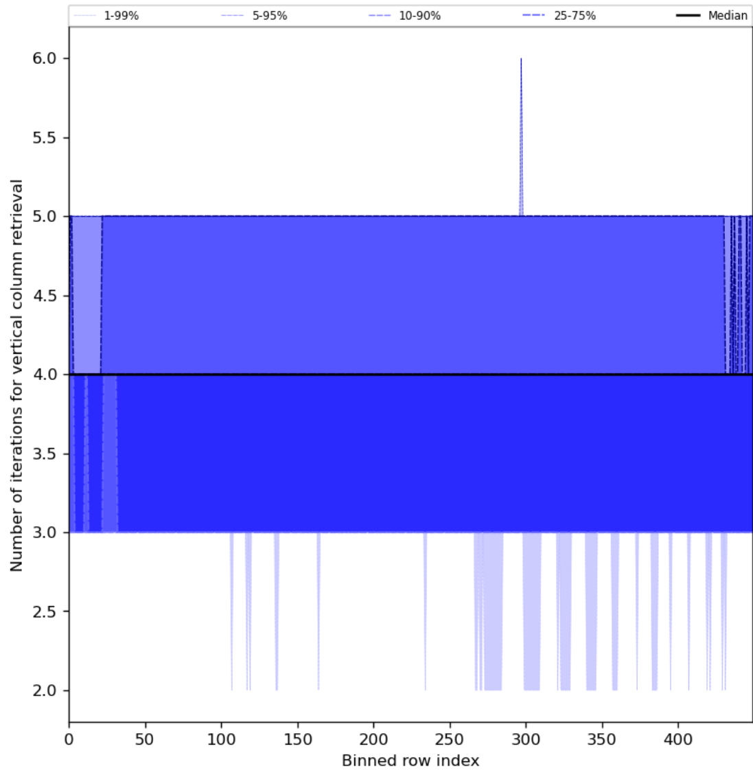
Figure 33: Along track statistics of “Number of iterations for vertical column retrieval” for 2024-04-05 to 2024-04-07
