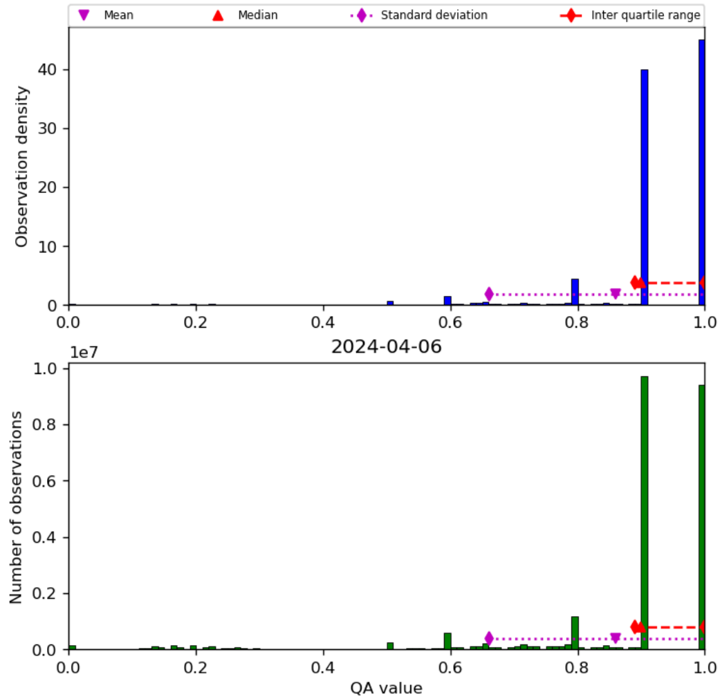
Figure 20: Histogram of “QA value” for 2024-04-05 to 2024-04-07
