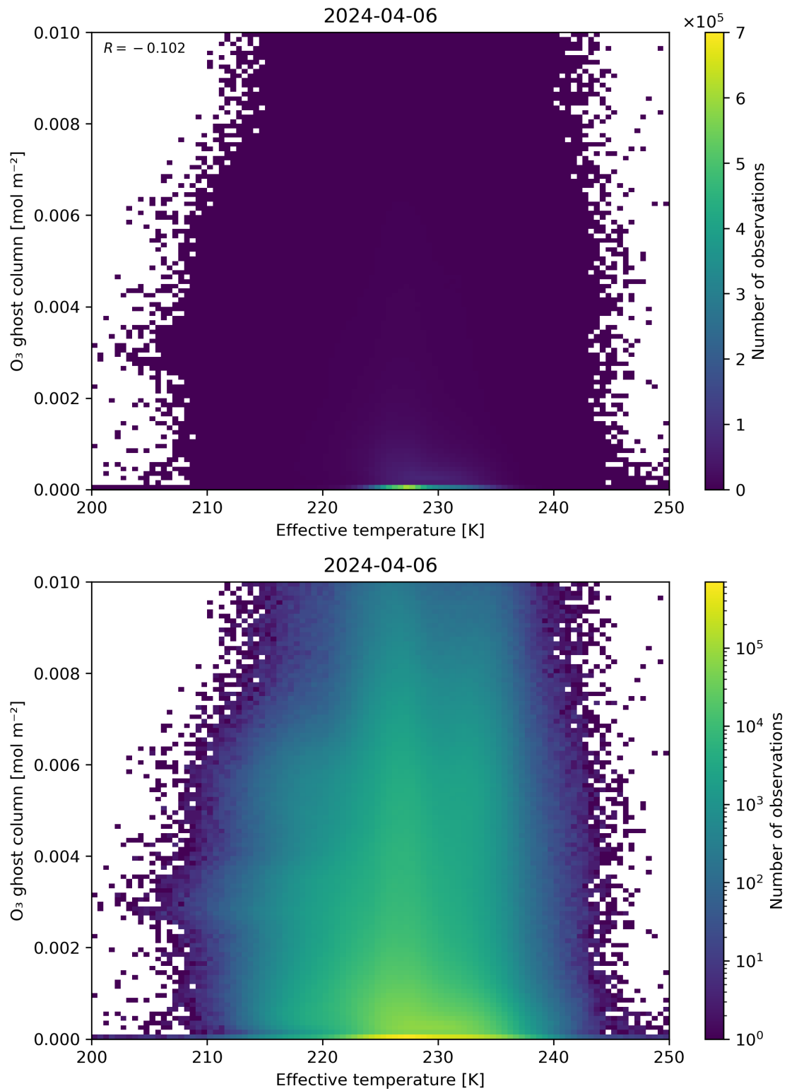
Figure 38: Scatter density plot of “Effective temperature” against “O 3 ghost column” for 2024-04-05 to 2024-04-07.
