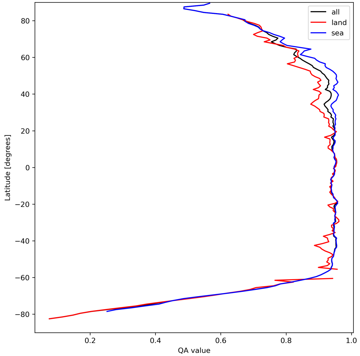
Figure 13: Zonal average of “QA value” for 2024-04-05 to 2024-04-07.
