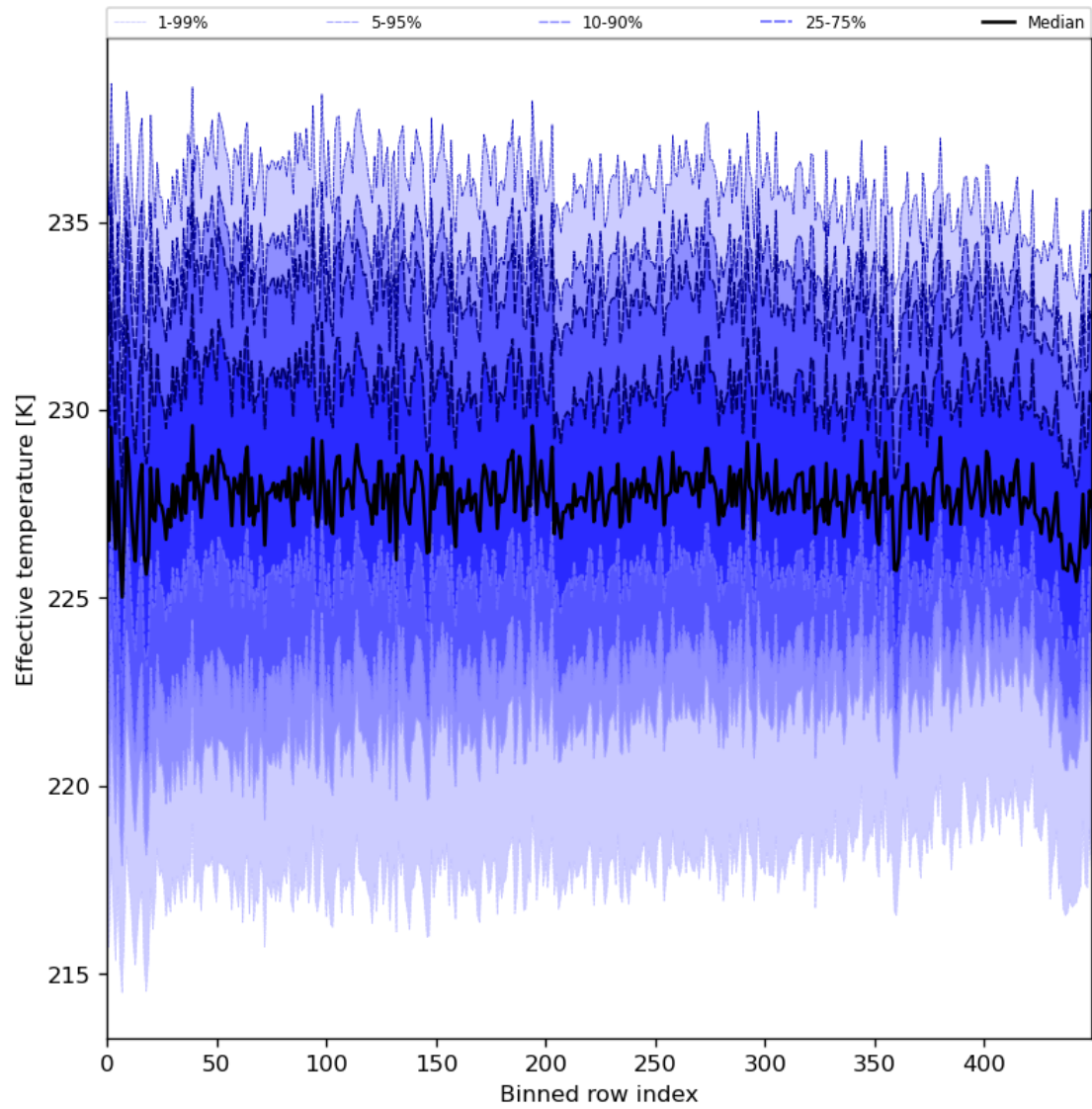
Figure 31: Along track statistics of “Effective temperature” for 2024-04-05 to 2024-04-07
