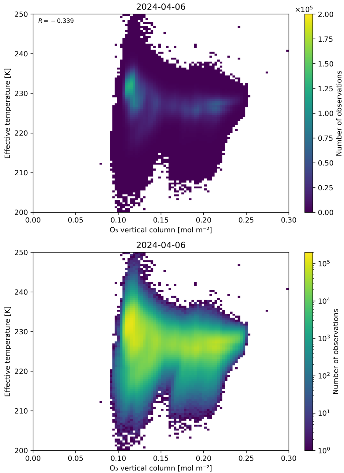
Figure 39: Scatter density plot of “O 3 vertical column” against “Effective temperature” for 2024-04-05 to 2024-04-07.
