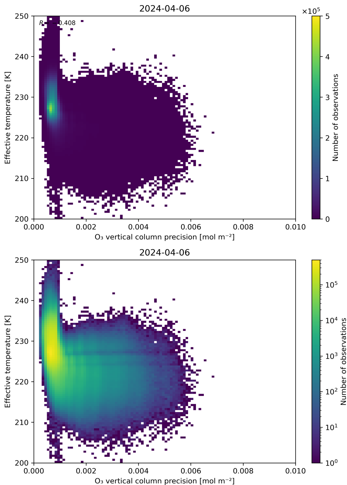
Figure 42: Scatter density plot of “O 3 vertical column precision” against “Effective temperature” for 2024-04-05 to 2024-04-07.
