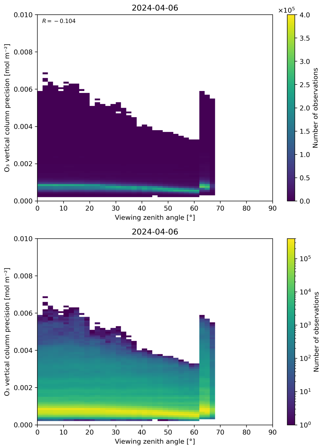
Figure 53: Scatter density plot of “Viewing zenith angle” against “O 3 vertical column precision” for 2024-04-05 to 2024-04-07.
