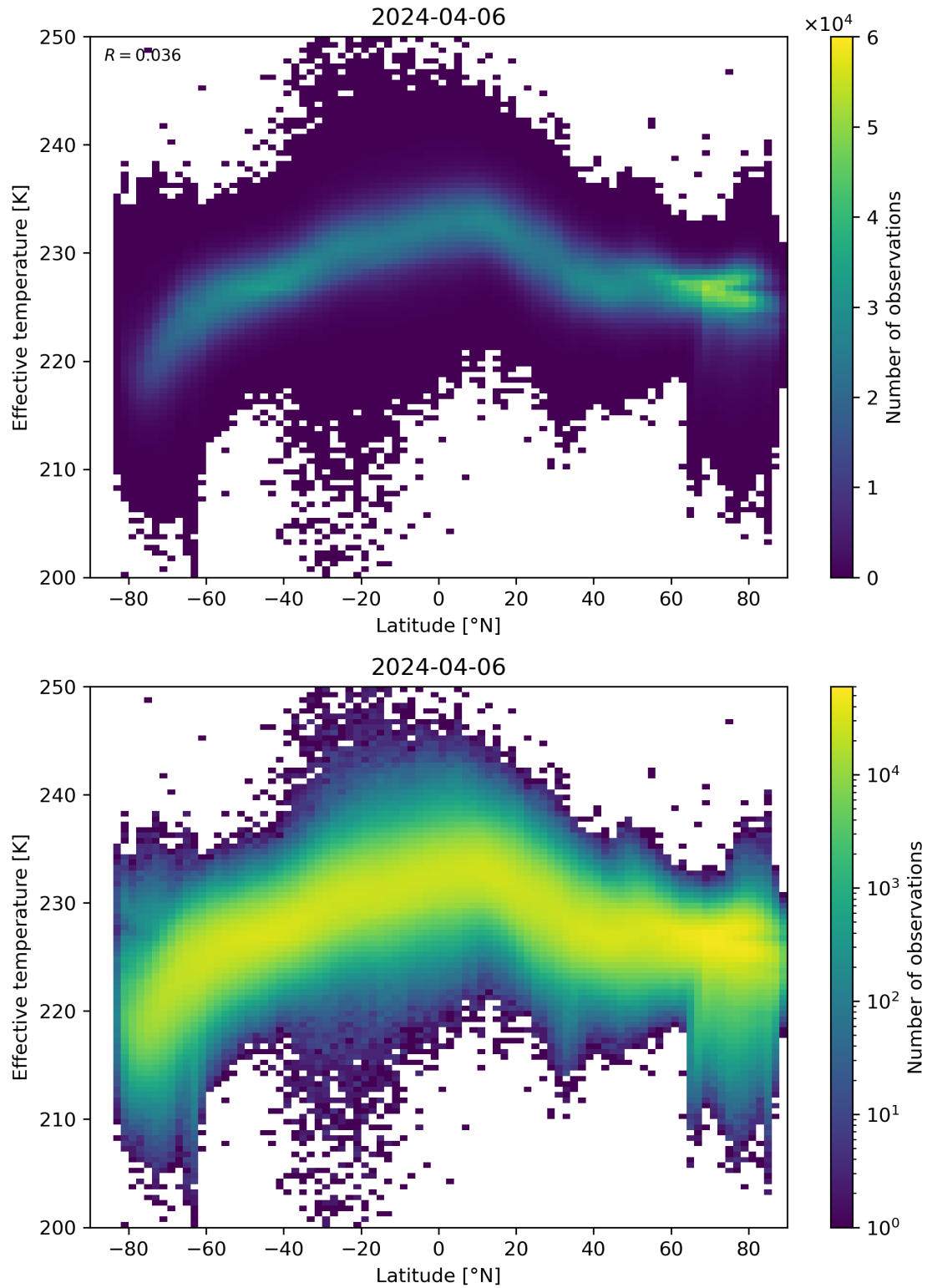
Figure 34: Scatter density plot of “Latitude” against “Effective temperature” for 2024-04-05 to 2024-04-07.
