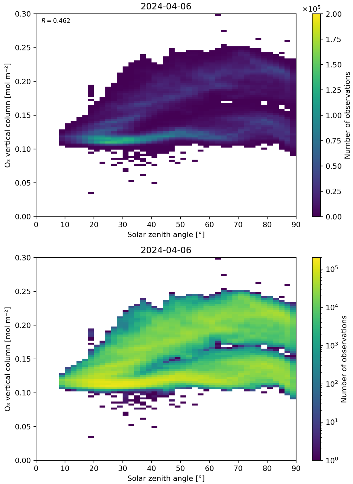
Figure 47: Scatter density plot of “Solar zenith angle” against “O 3 vertical column” for 2024-04-05 to 2024-04-07.
