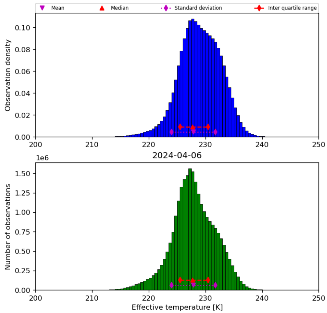
Figure 24: Histogram of “Effective temperature” for 2024-04-05 to 2024-04-07
