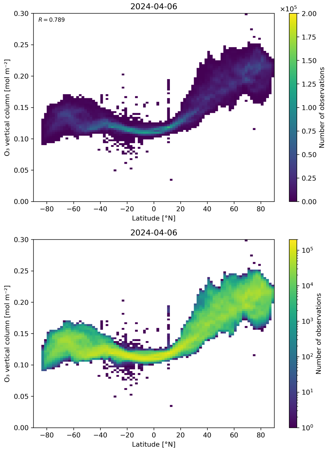
Figure 36: Scatter density plot of “Latitude” against “O 3 vertical column” for 2024-04-05 to 2024-04-07.
