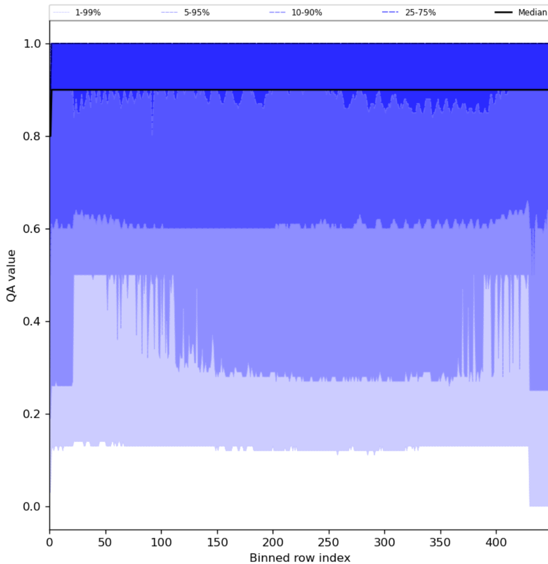
Figure 27: Along track statistics of “QA value” for 2024-04-05 to 2024-04-07
