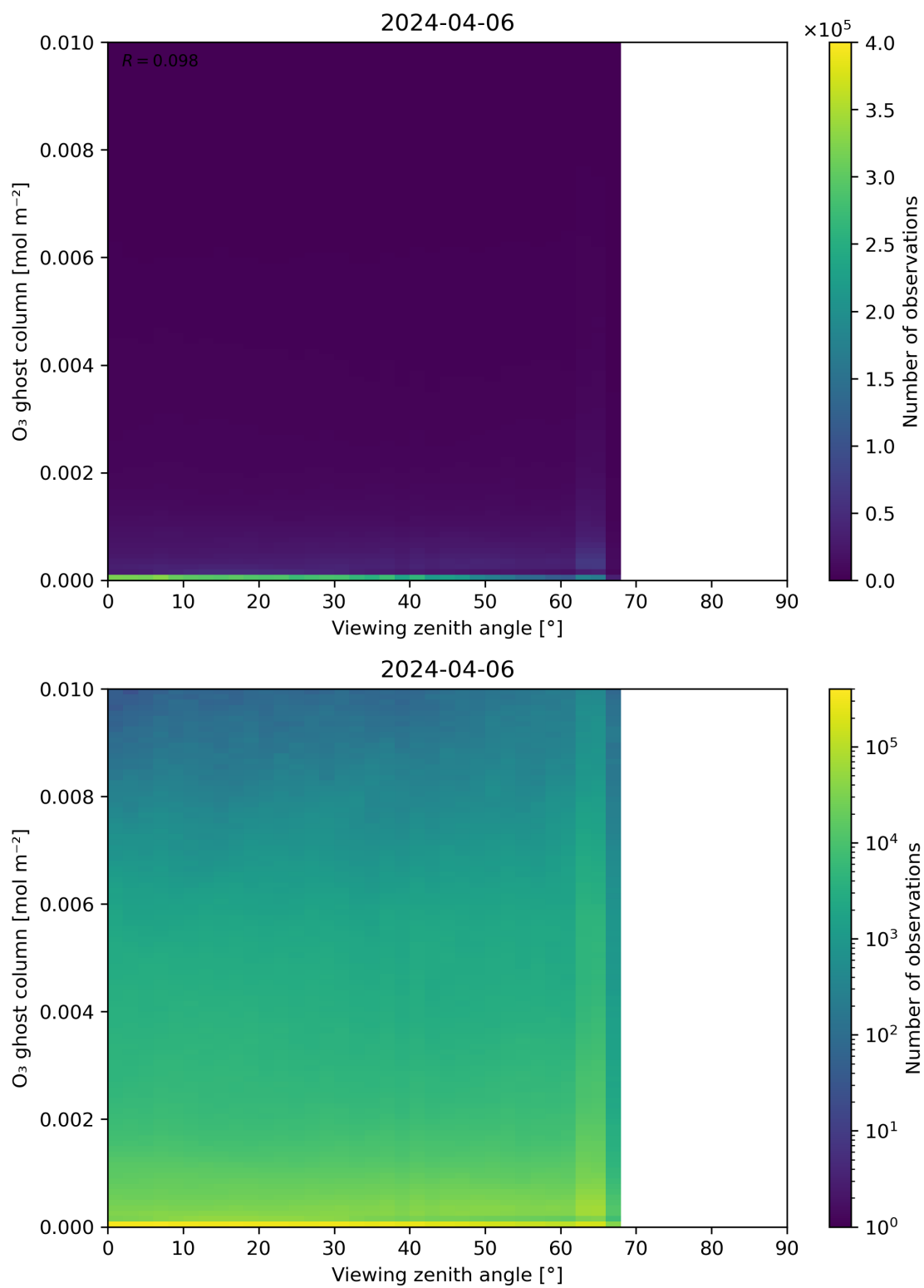
Figure 51: Scatter density plot of “Viewing zenith angle” against “O 3 ghost column” for 2024-04-05 to 2024-04-07.
