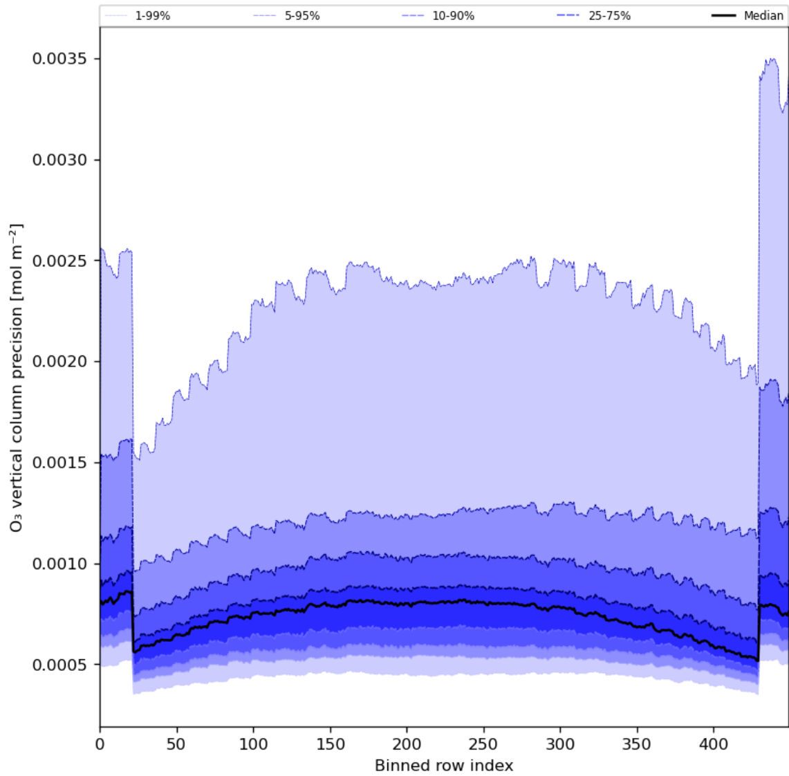
Figure 29: Along track statistics of “O 3 vertical column precision” for 2024-04-05 to 2024-04-07
