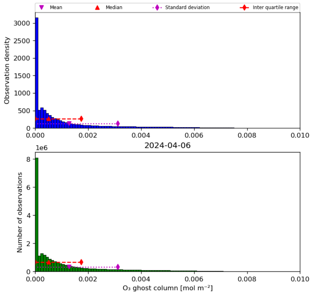
Figure 25: Histogram of “O 3 ghost column” for 2024-04-05 to 2024-04-07
