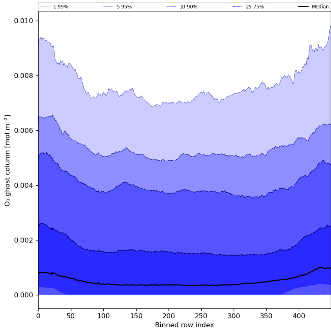
Figure 32: Along track statistics of “O 3 ghost column” for 2024-04-05 to 2024-04-07
