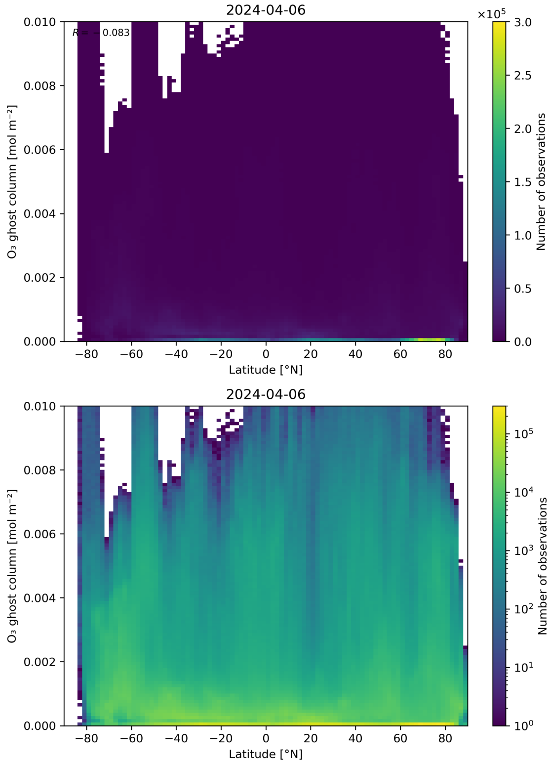
Figure 35: Scatter density plot of “Latitude” against “O 3 ghost column” for 2024-04-05 to 2024-04-07.
