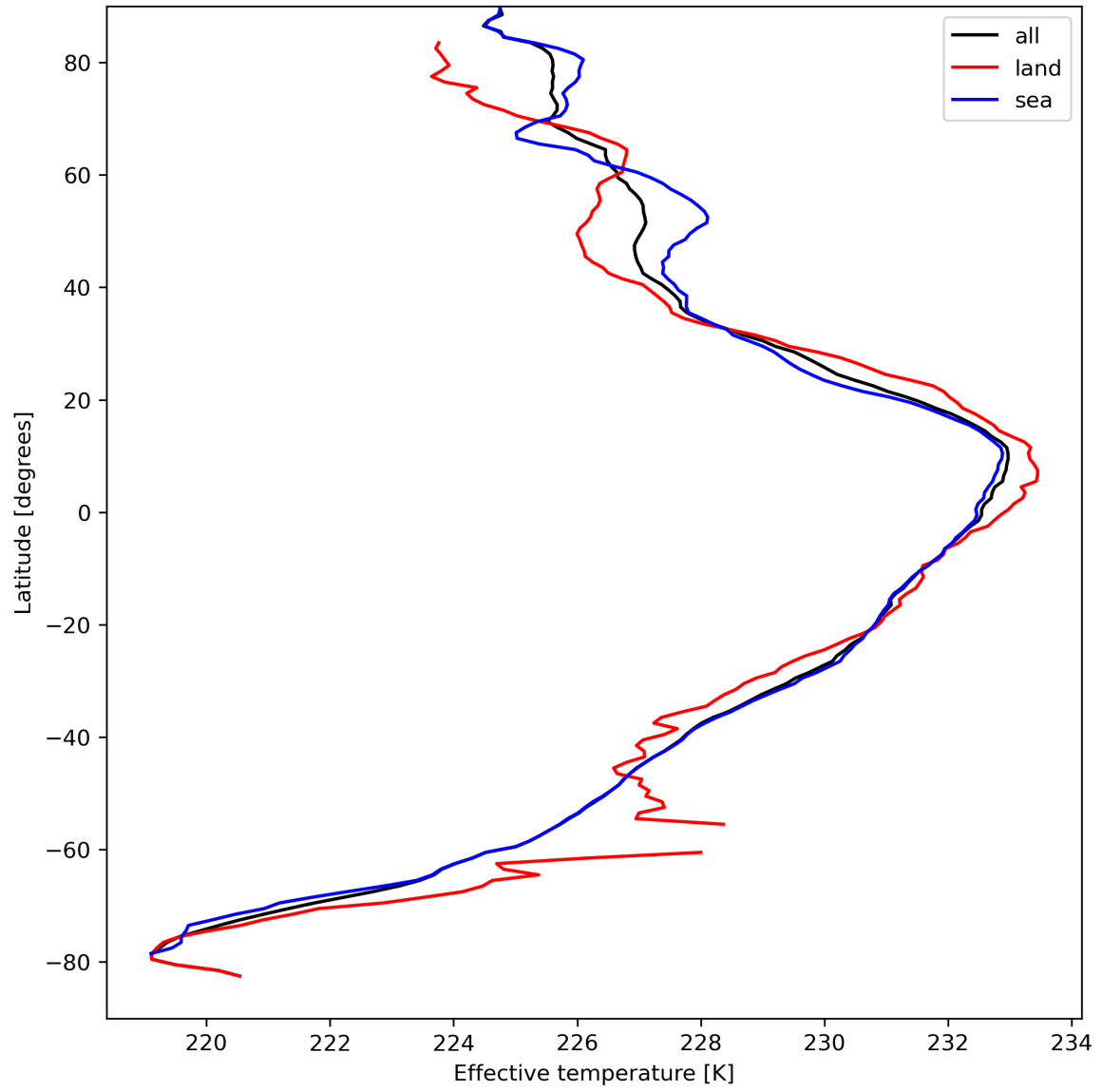
Figure 17: Zonal average of “Effective temperature” for 2024-04-05 to 2024-04-07.
