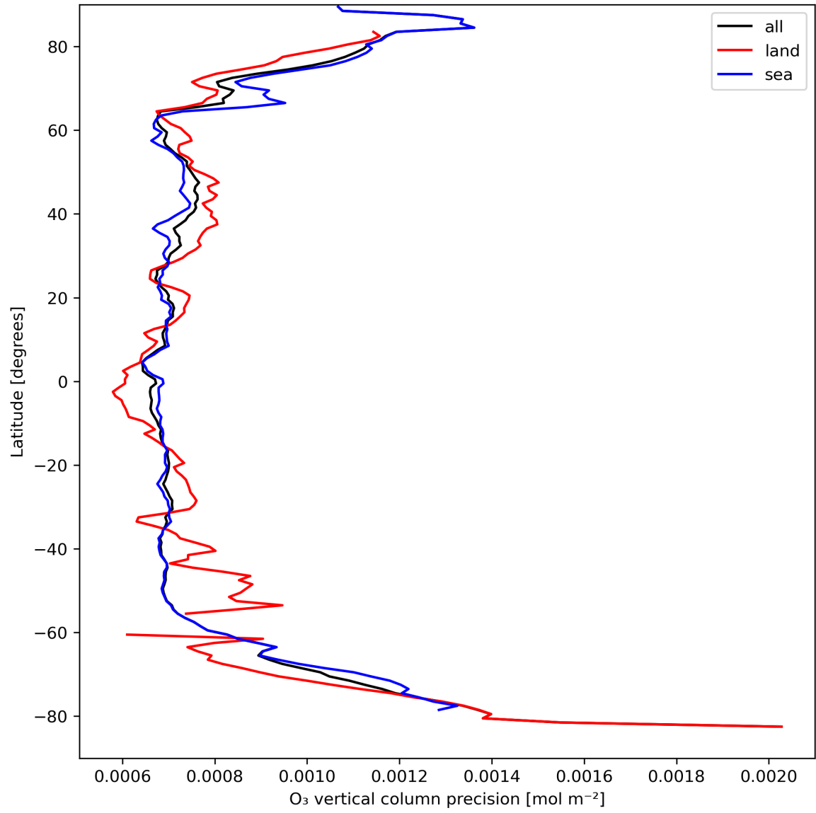
Figure 15: Zonal average of “O 3 vertical column precision” for 2024-04-05 to 2024-04-07.
