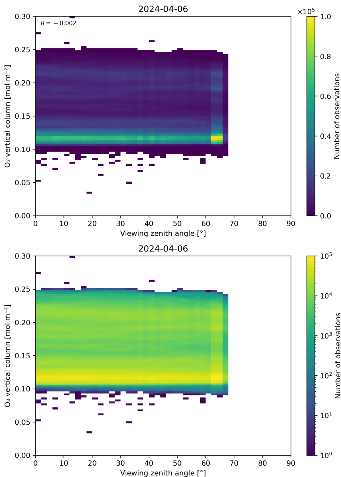
Figure 52: Scatter density plot of “Viewing zenith angle” against “O 3 vertical column” for 2024-04-05 to 2024-04-07.
