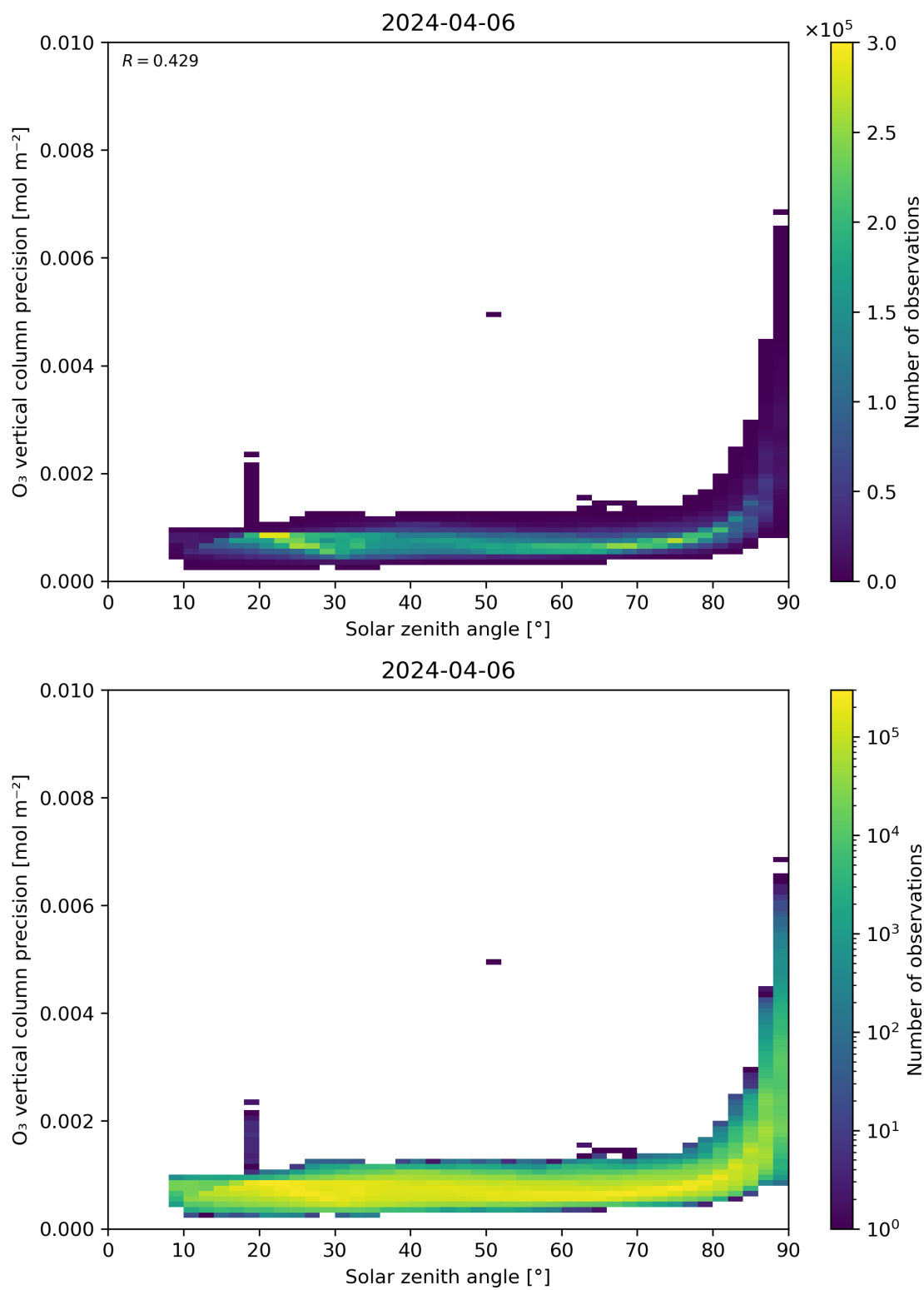
Figure 48: Scatter density plot of “Solar zenith angle” against “O 3 vertical column precision” for 2024-04-05 to 2024-04-07.
