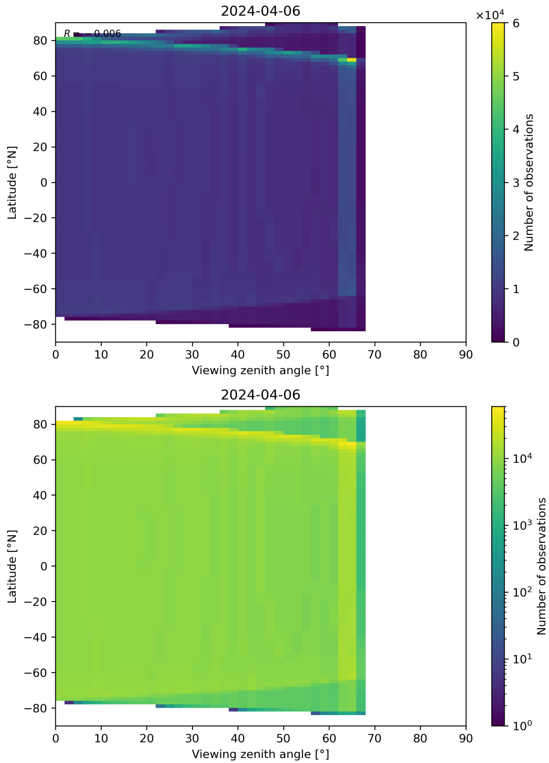
Figure 49: Scatter density plot of “Viewing zenith angle” against “Latitude” for 2024-04-05 to 2024-04-07.
