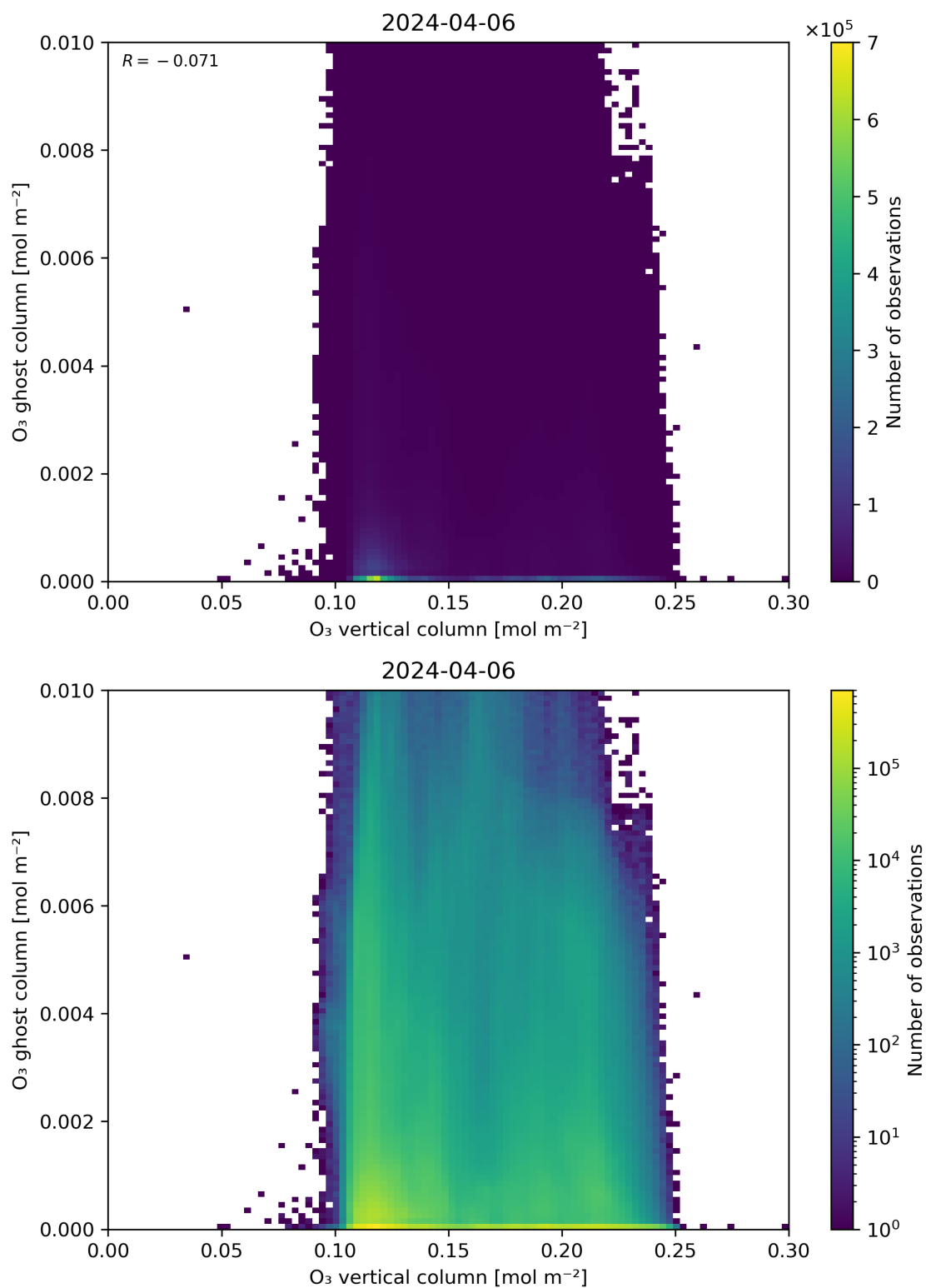
Figure 40: Scatter density plot of “O 3 vertical column” against “O 3 ghost column” for 2024-04-05 to 2024-04-07.
