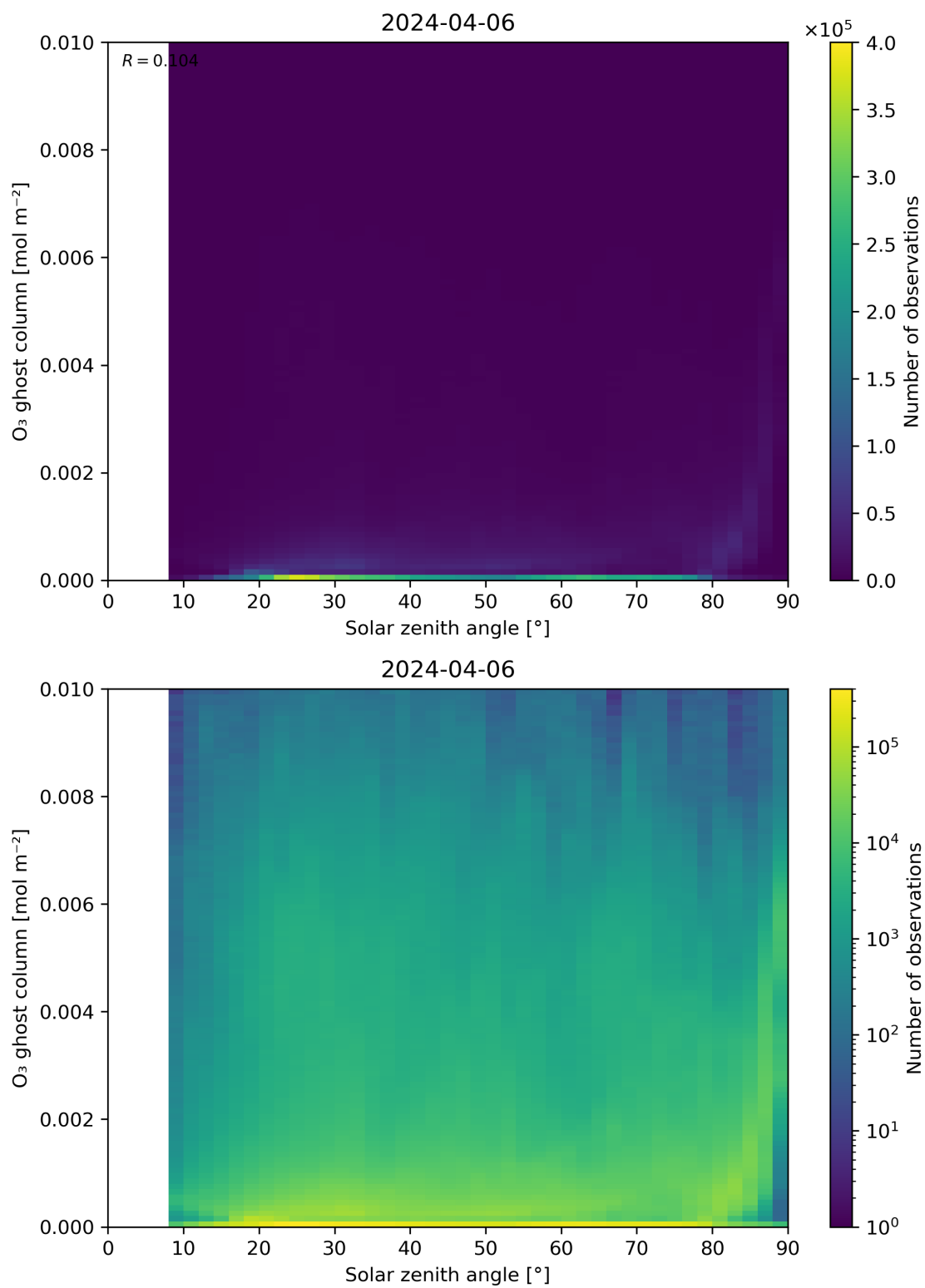
Figure 46: Scatter density plot of “Solar zenith angle” against “O 3 ghost column” for 2024-04-05 to 2024-04-07.
