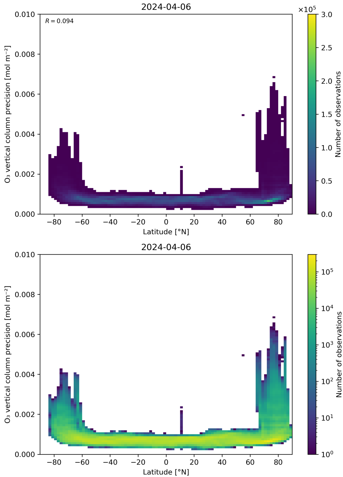
Figure 37: Scatter density plot of “Latitude” against “O 3 vertical column precision” for 2024-04-05 to 2024-04-07.
