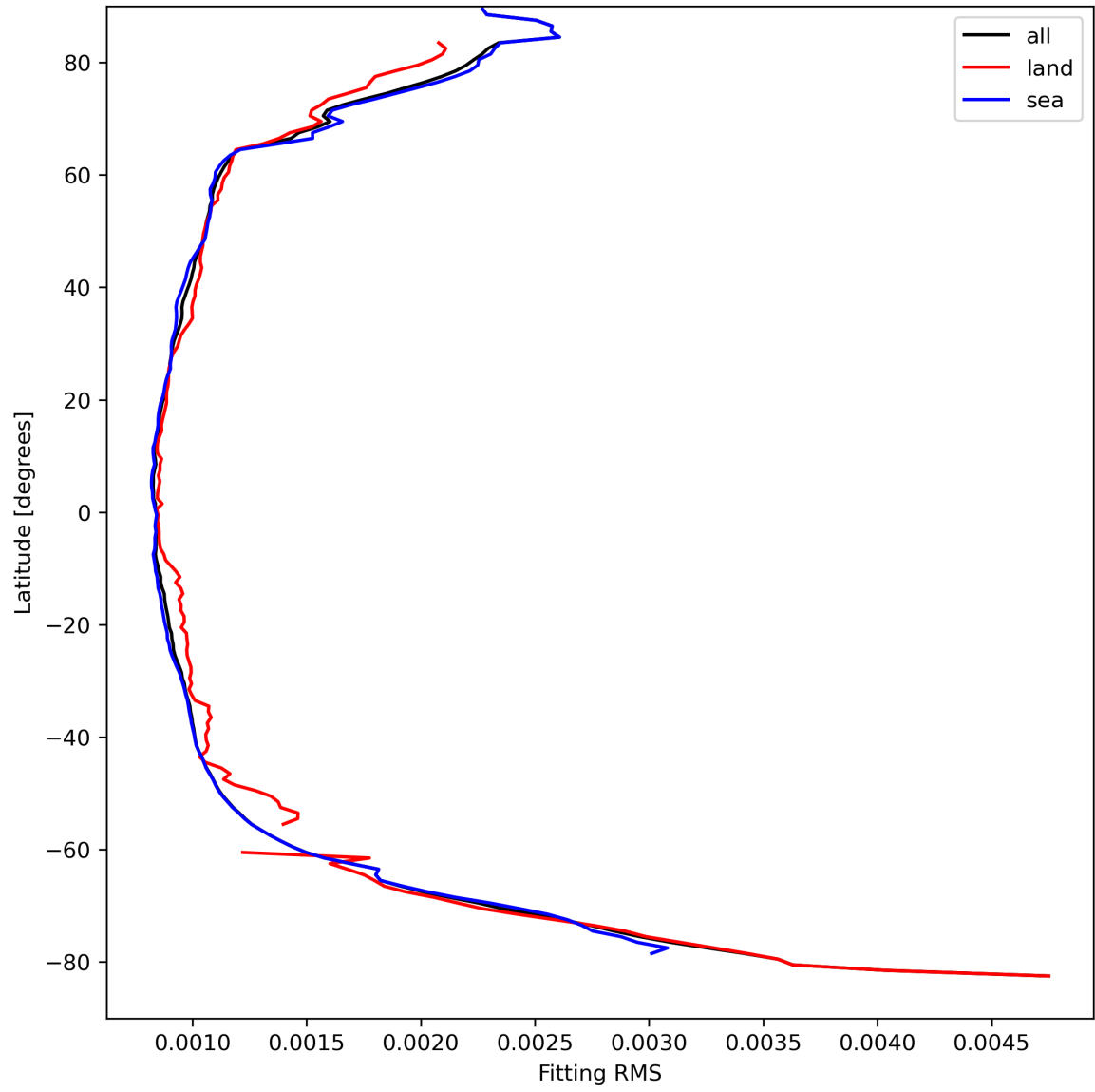
Figure 16: Zonal average of “Fitting RMS” for 2024-04-05 to 2024-04-07.
