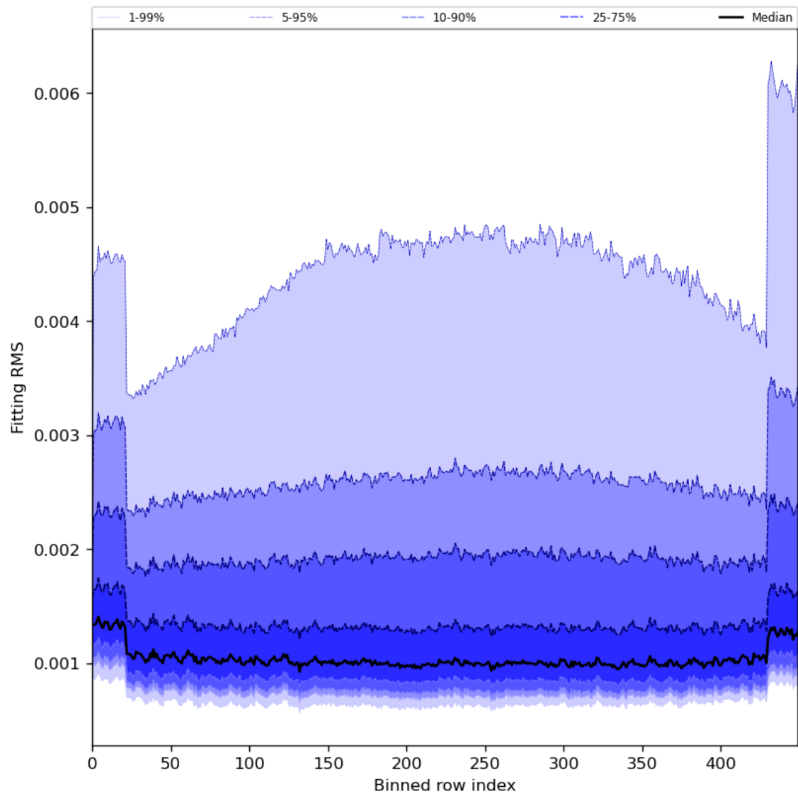
Figure 30: Along track statistics of “Fitting RMS” for 2024-04-05 to 2024-04-07
