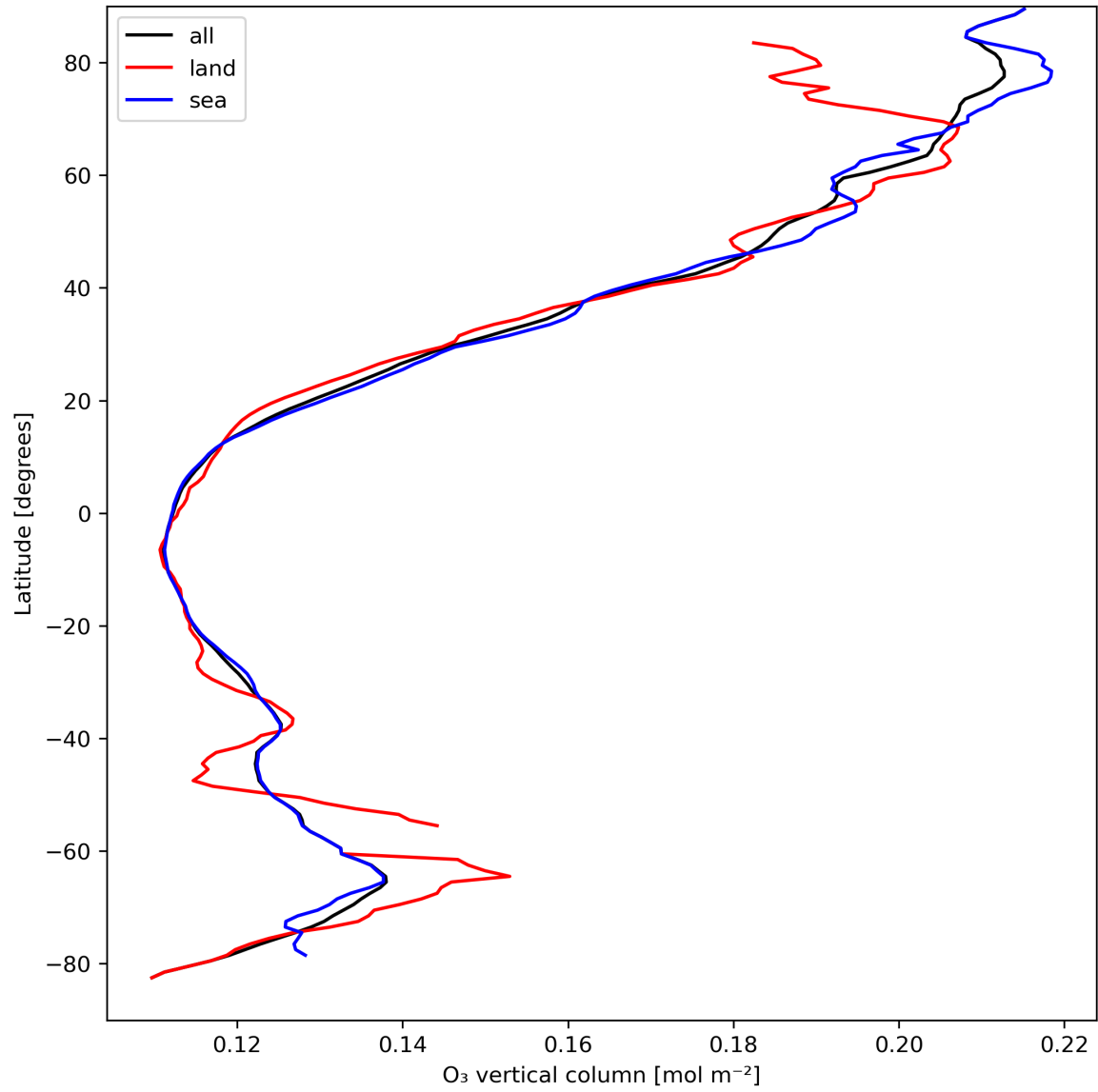
Figure 14: Zonal average of “O 3 vertical column” for 2024-04-05 to 2024-04-07.
