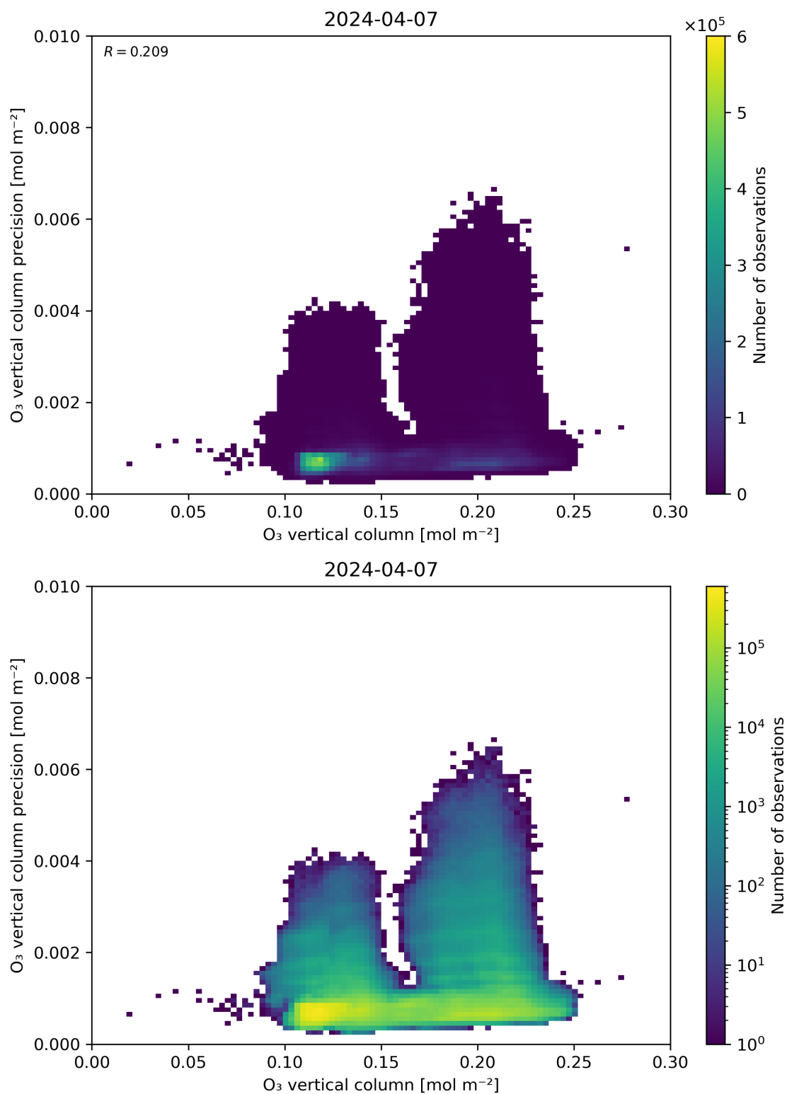
Figure 41: Scatter density plot of “O 3 vertical column” against “O 3 vertical column precision” for 2024-04-06 to 2024-04-08.
