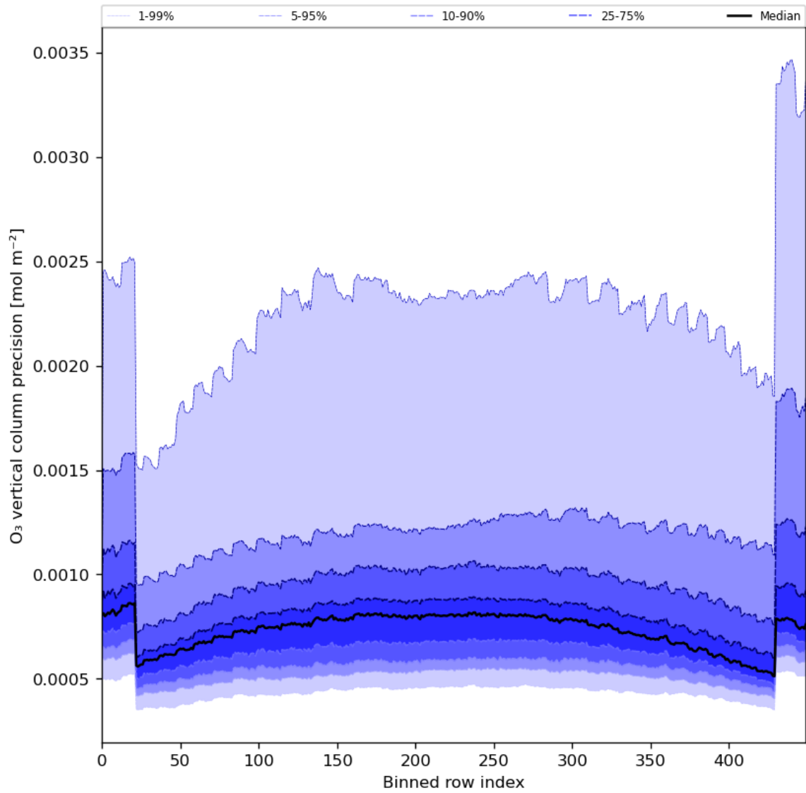
Figure 29: Along track statistics of “O 3 vertical column precision” for 2024-04-06 to 2024-04-08
