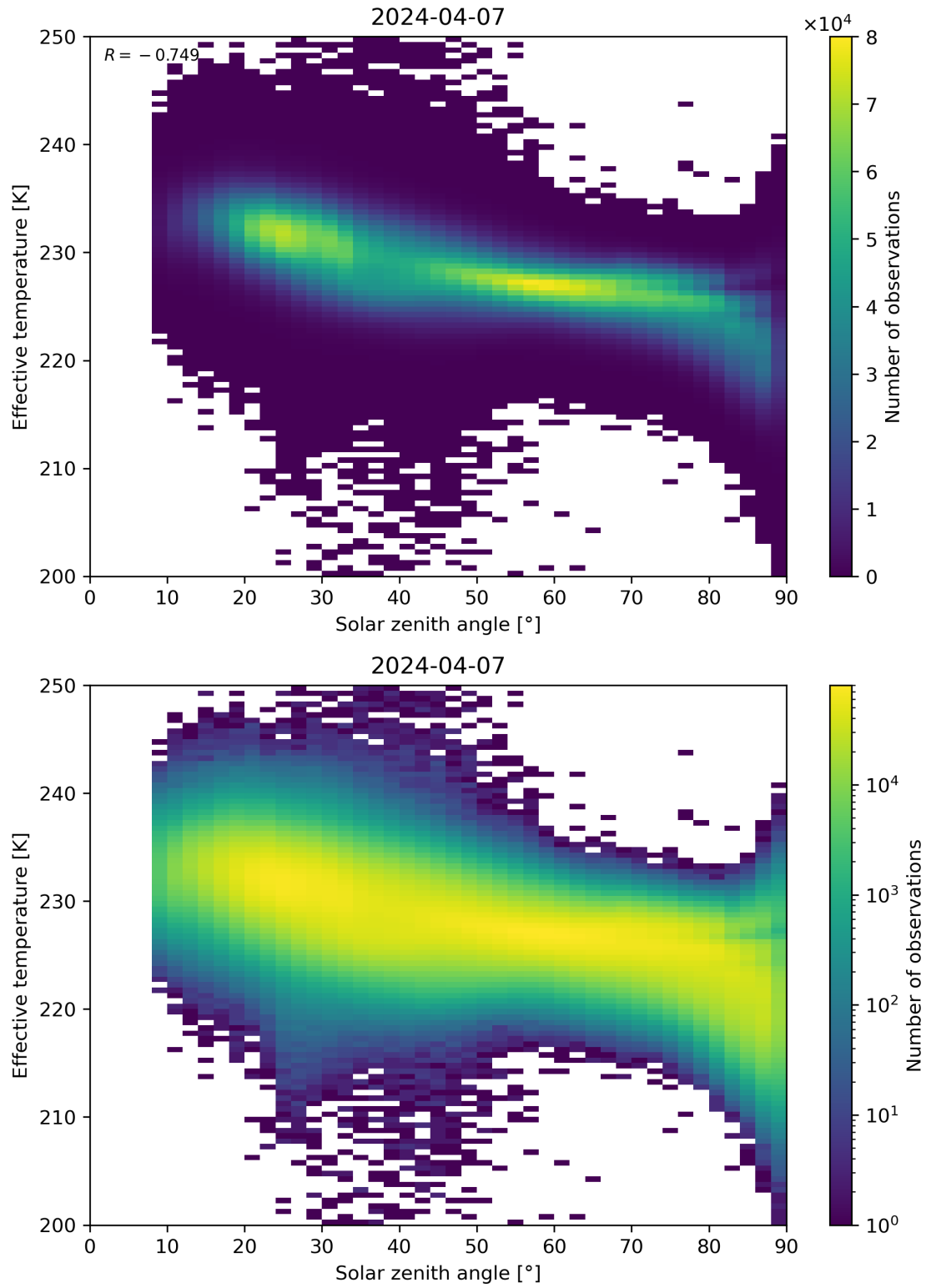
Figure 45: Scatter density plot of “Solar zenith angle” against “Effective temperature” for 2024-04-06 to 2024-04-08.
