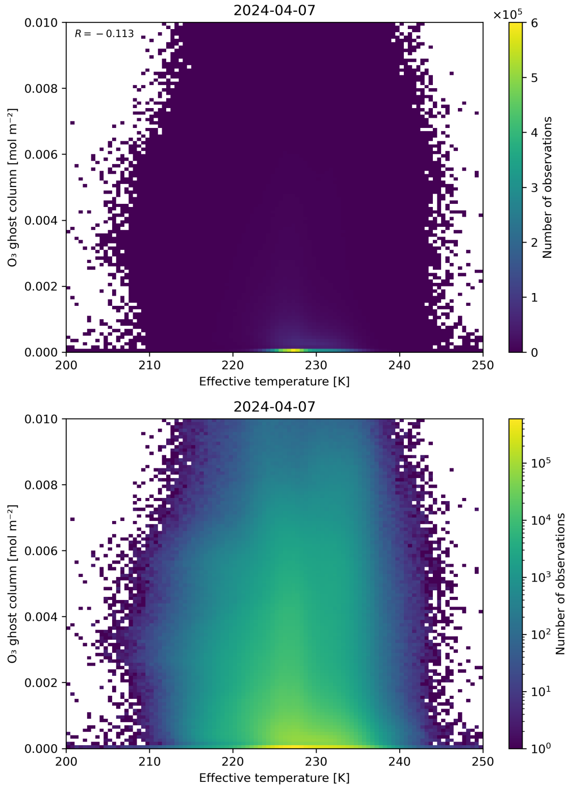
Figure 38: Scatter density plot of “Effective temperature” against “O 3 ghost column” for 2024-04-06 to 2024-04-08.
