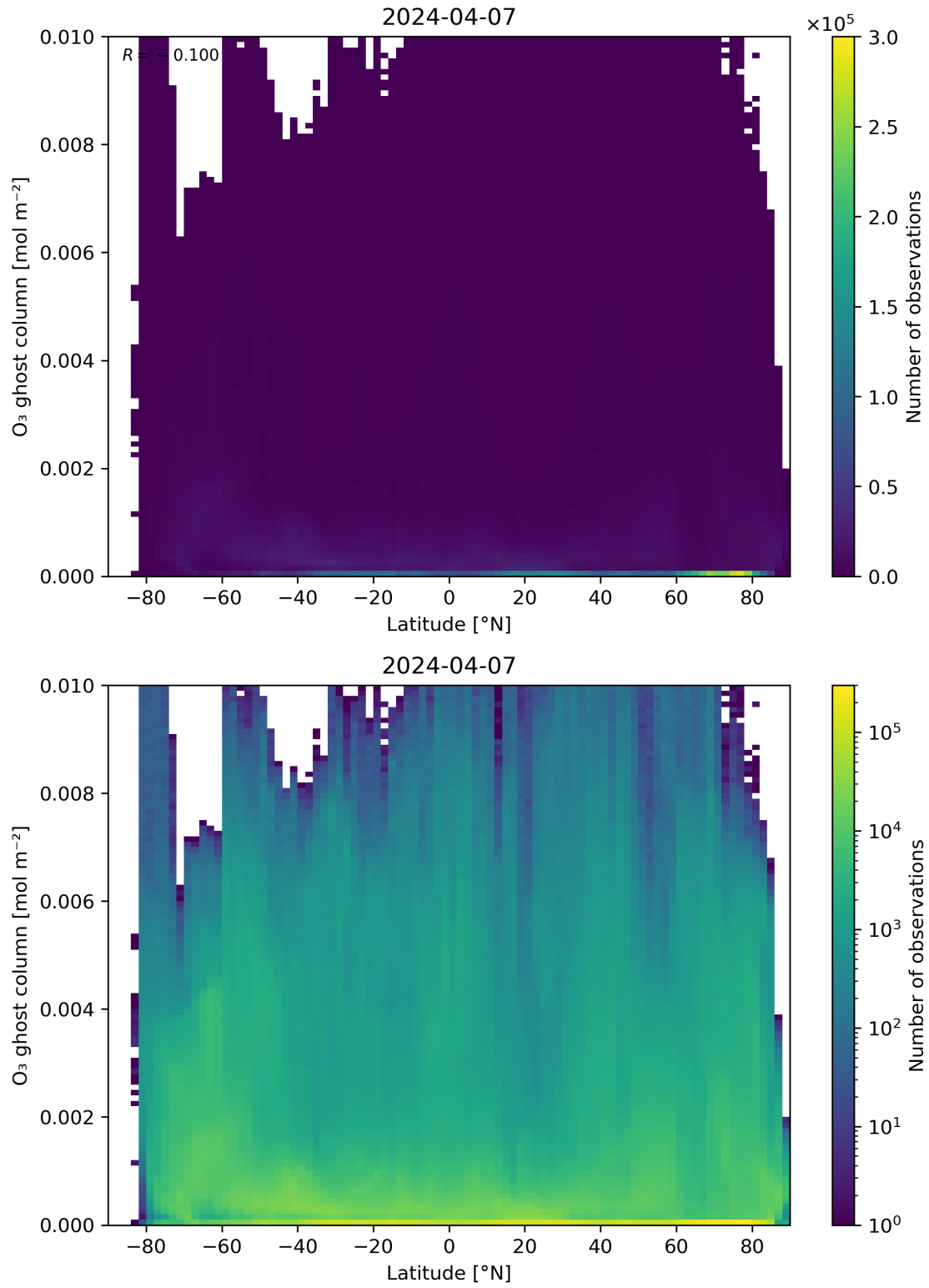
Figure 35: Scatter density plot of “Latitude” against “O 3 ghost column” for 2024-04-06 to 2024-04-08.
