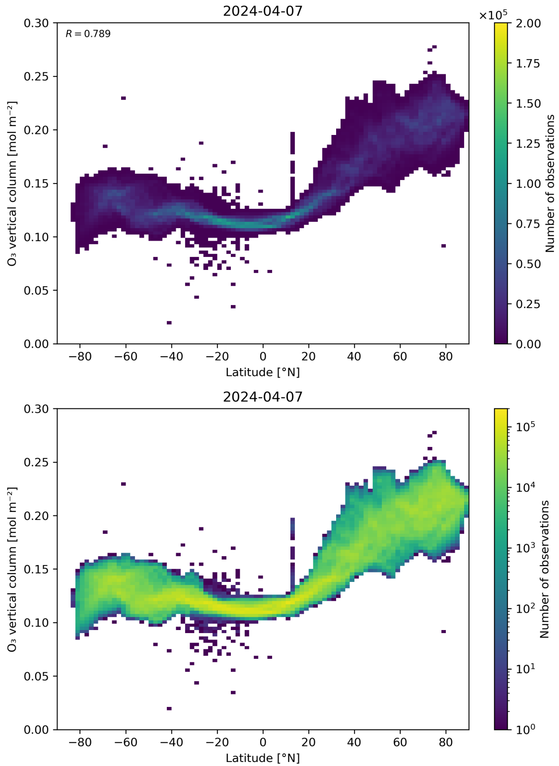
Figure 36: Scatter density plot of “Latitude” against “O 3 vertical column” for 2024-04-06 to 2024-04-08.
