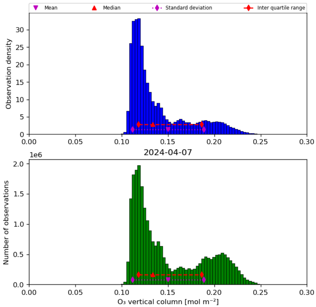
Figure 21: Histogram of “O 3 vertical column” for 2024-04-06 to 2024-04-08
