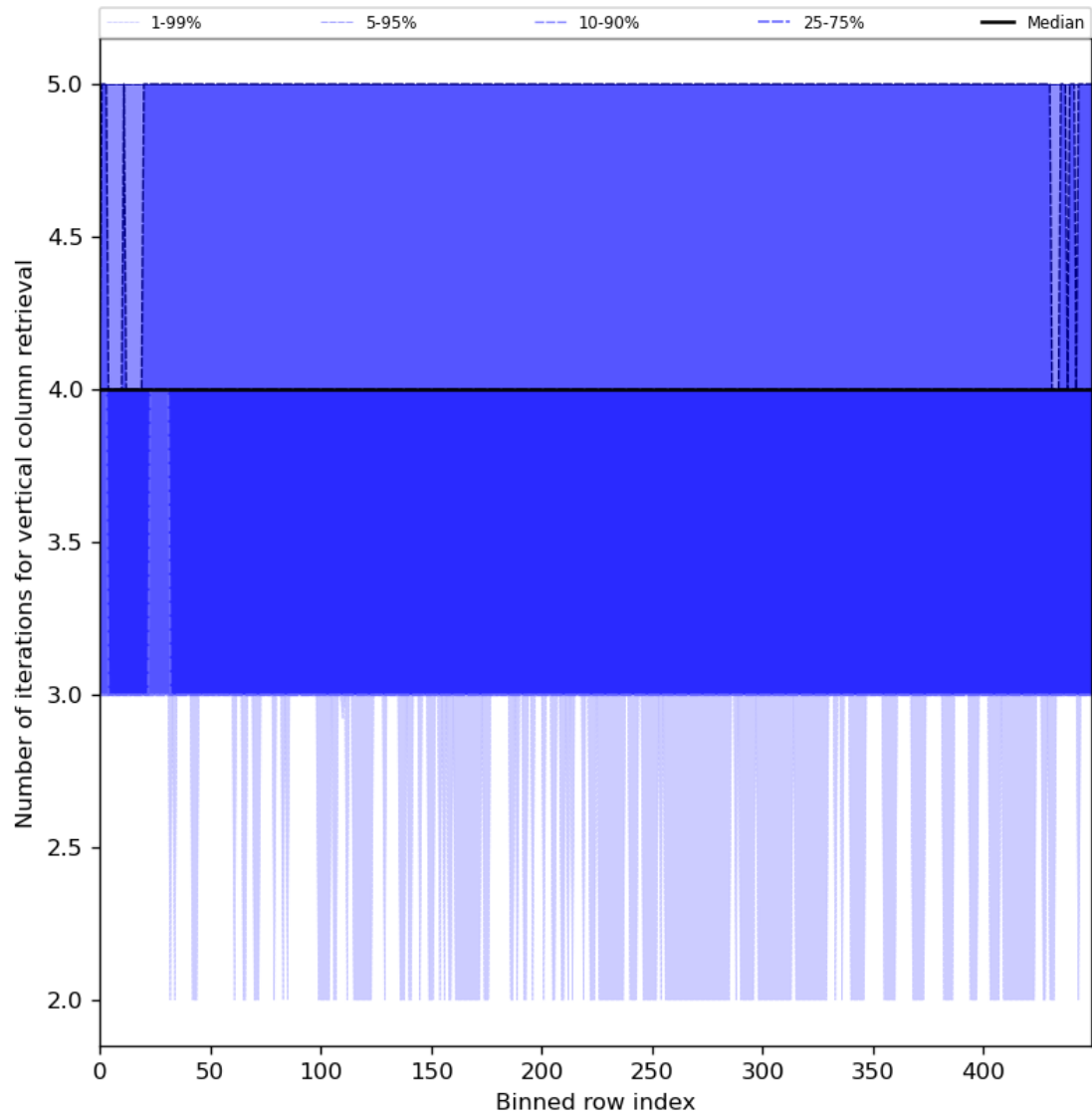
Figure 33: Along track statistics of “Number of iterations for vertical column retrieval” for 2024-04-06 to 2024-04-08
