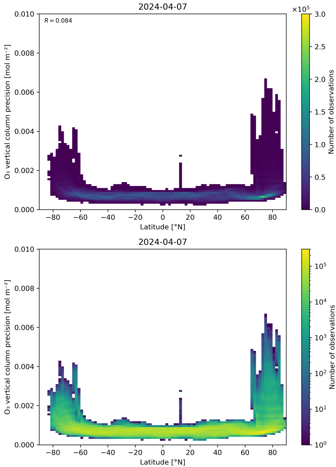
Figure 37: Scatter density plot of “Latitude” against “O 3 vertical column precision” for 2024-04-06 to 2024-04-08.
