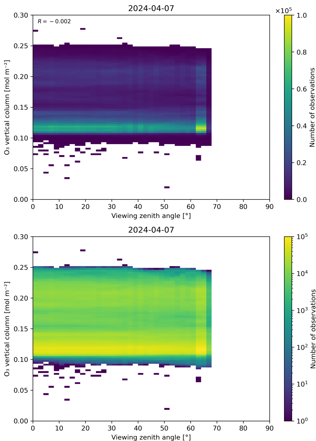
Figure 52: Scatter density plot of “Viewing zenith angle” against “O 3 vertical column” for 2024-04-06 to 2024-04-08.
