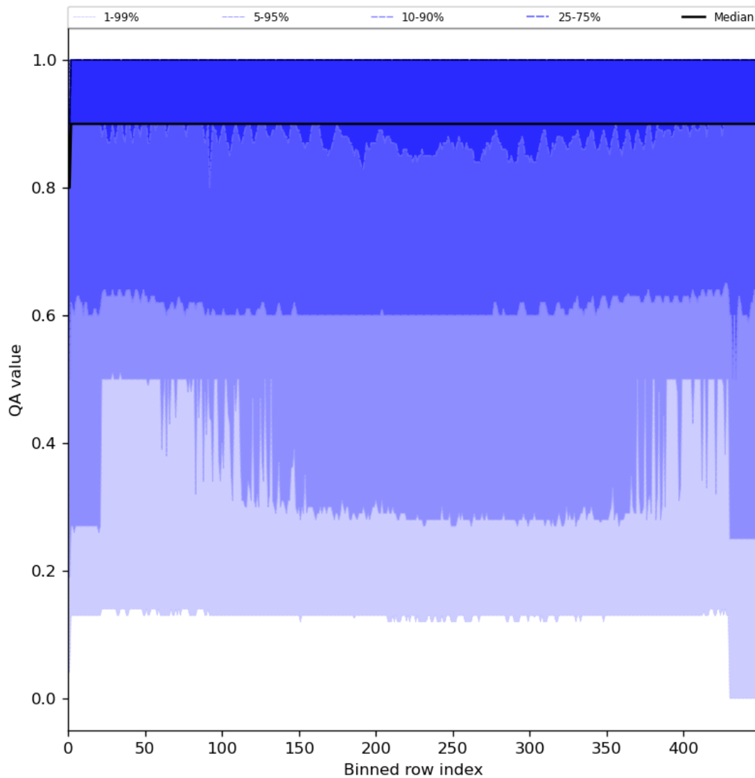
Figure 27: Along track statistics of “QA value” for 2024-04-06 to 2024-04-08
