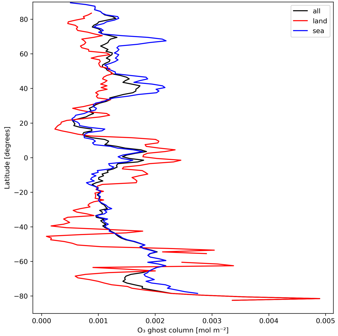
Figure 18: Zonal average of “O 3 ghost column” for 2024-04-06 to 2024-04-08.
