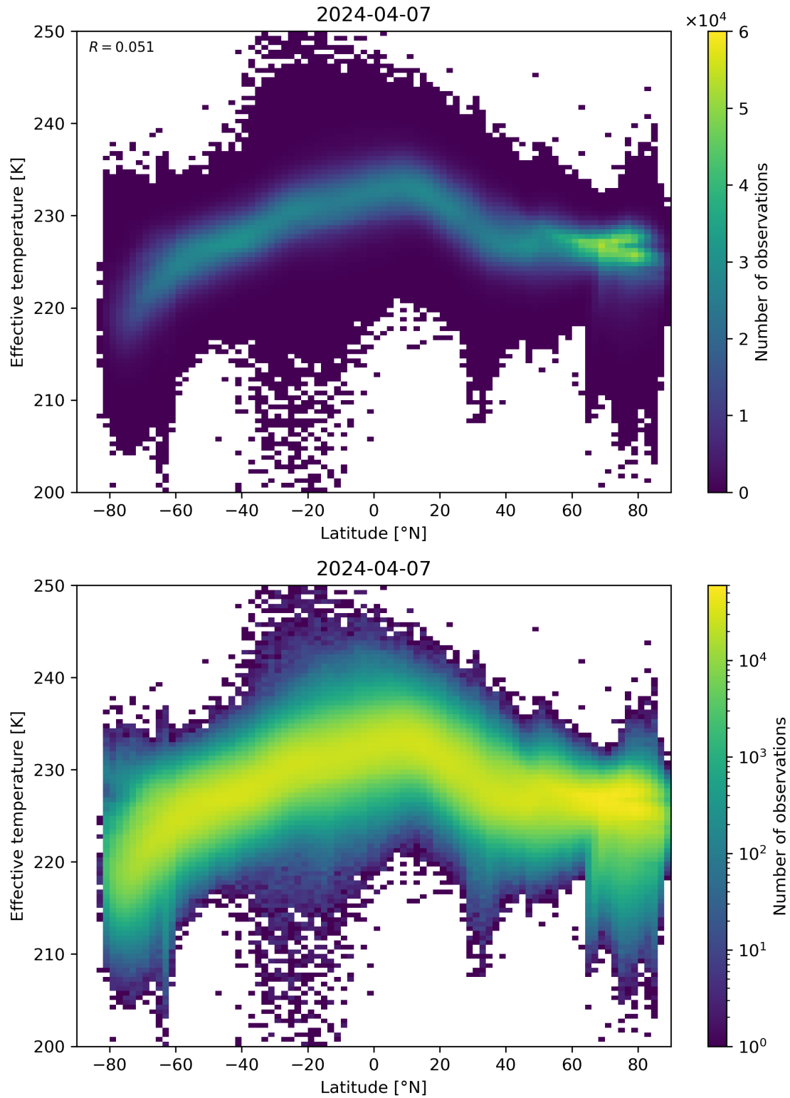
Figure 34: Scatter density plot of “Latitude” against “Effective temperature” for 2024-04-06 to 2024-04-08.
