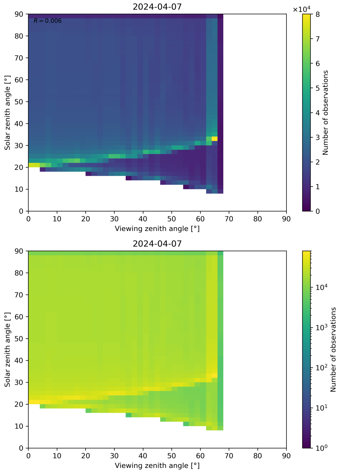
Figure 54: Scatter density plot of “Viewing zenith angle” against “Solar zenith angle” for 2024-04-06 to 2024-04-08.
