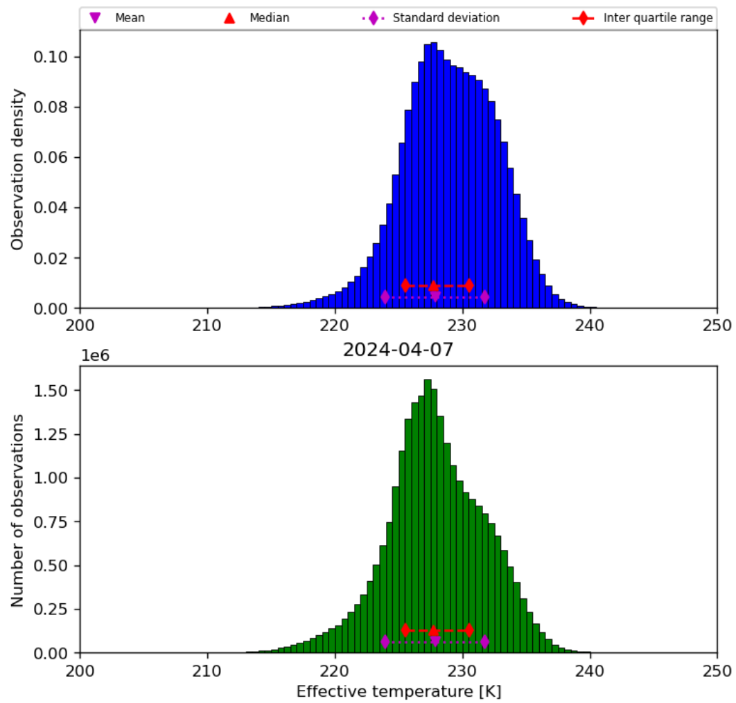
Figure 24: Histogram of “Effective temperature” for 2024-04-06 to 2024-04-08
