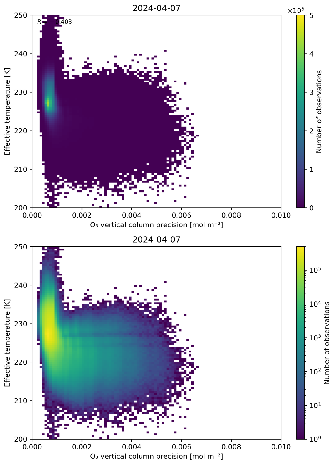
Figure 42: Scatter density plot of “O 3 vertical column precision” against “Effective temperature” for 2024-04-06 to 2024-04-08.
