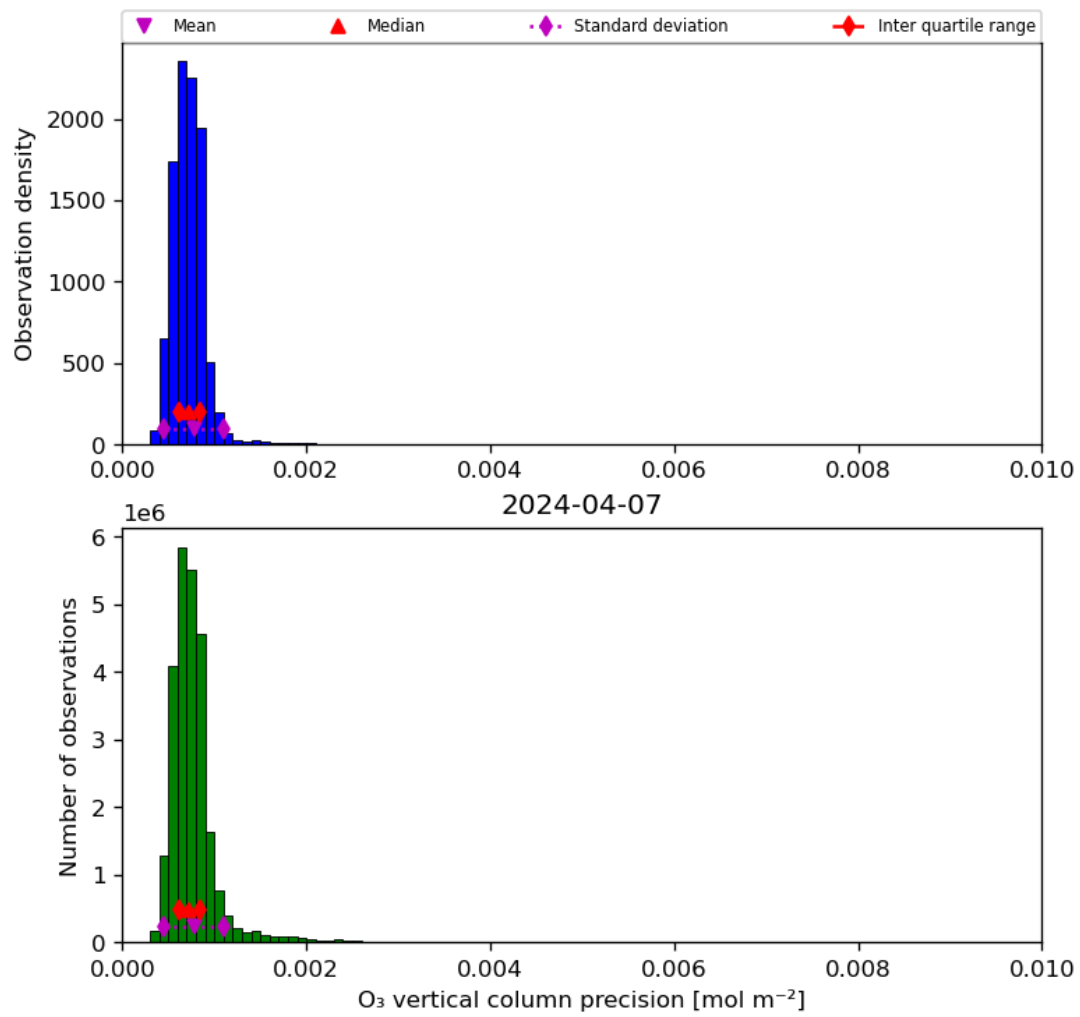
Figure 22: Histogram of “O 3 vertical column precision” for 2024-04-06 to 2024-04-08
