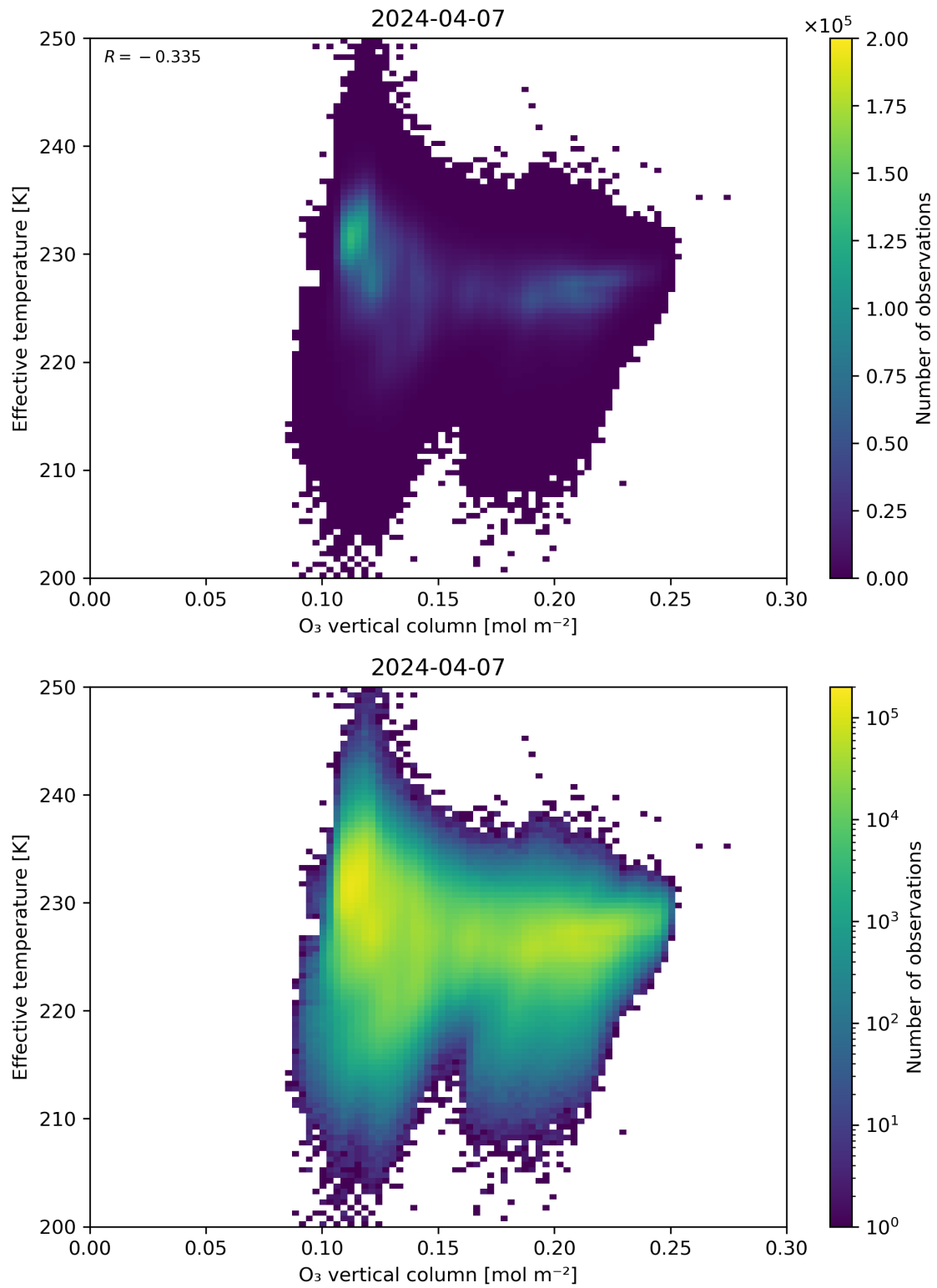
Figure 39: Scatter density plot of “O 3 vertical column” against “Effective temperature” for 2024-04-06 to 2024-04-08.
