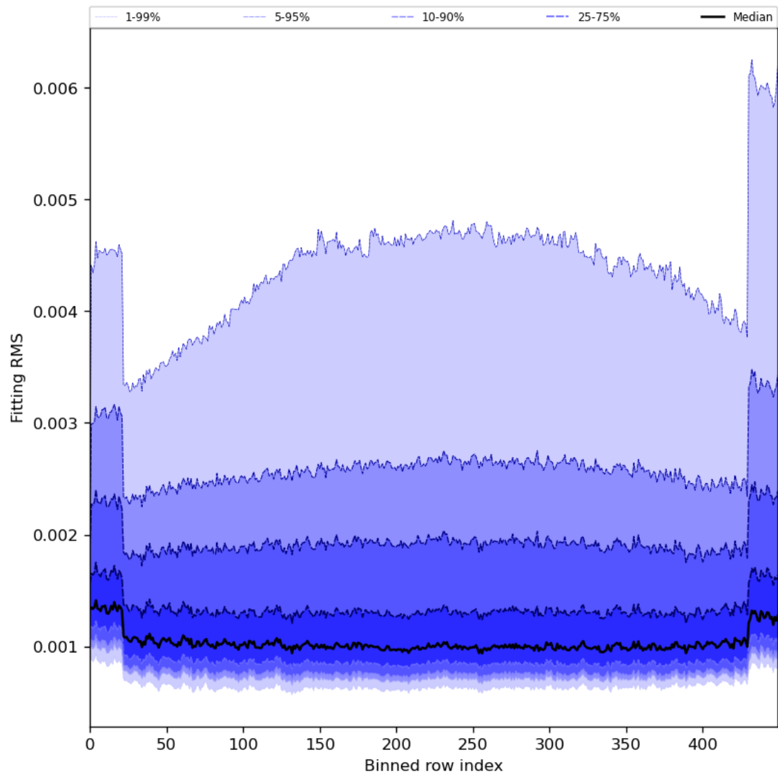
Figure 30: Along track statistics of “Fitting RMS” for 2024-04-06 to 2024-04-08
