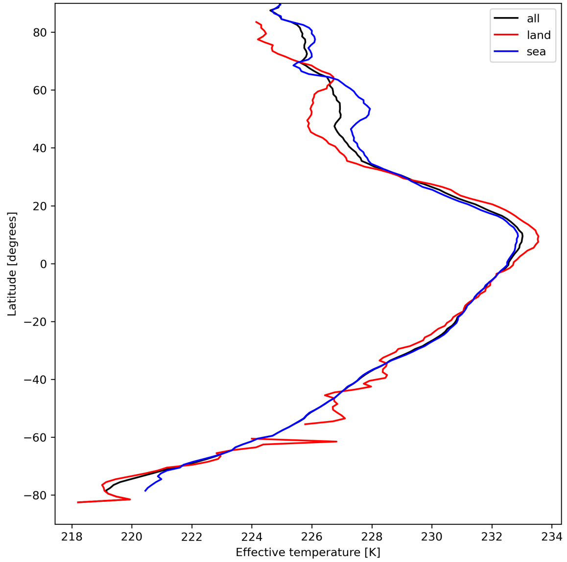
Figure 17: Zonal average of "Effective temperature" for 2024-04-06 to 2024-04-08.
