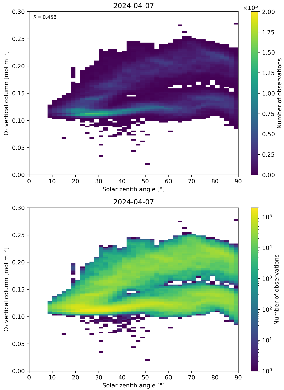
Figure 47: Scatter density plot of “Solar zenith angle” against “O 3 vertical column” for 2024-04-06 to 2024-04-08.
