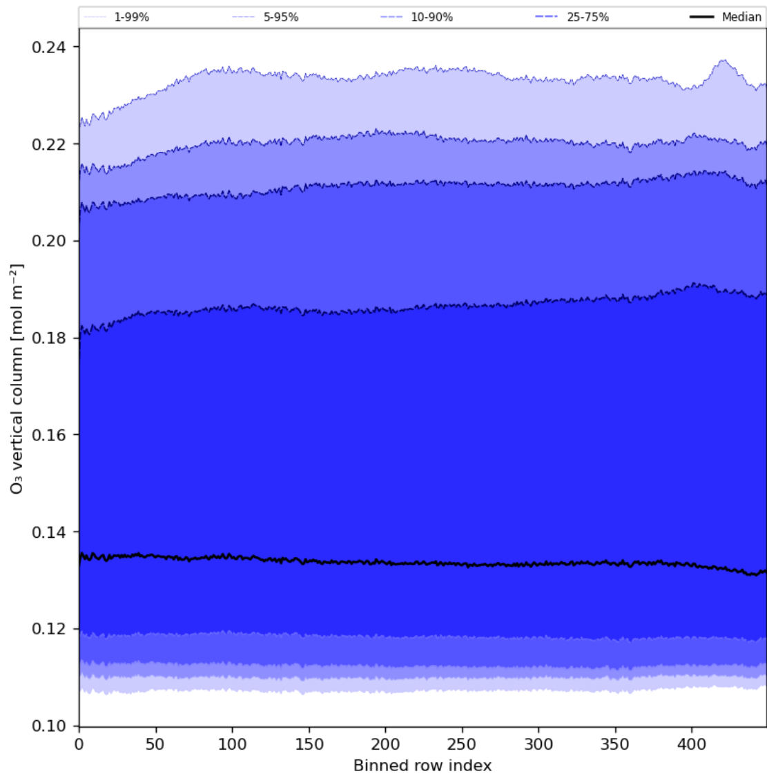
Figure 28: Along track statistics of “O 3 vertical column” for 2024-04-06 to 2024-04-08
