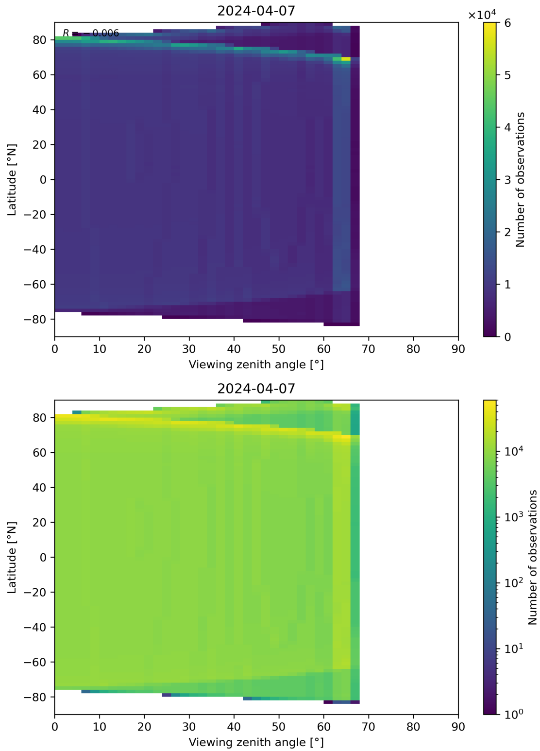
Figure 49: Scatter density plot of “Viewing zenith angle” against “Latitude” for 2024-04-06 to 2024-04-08.
