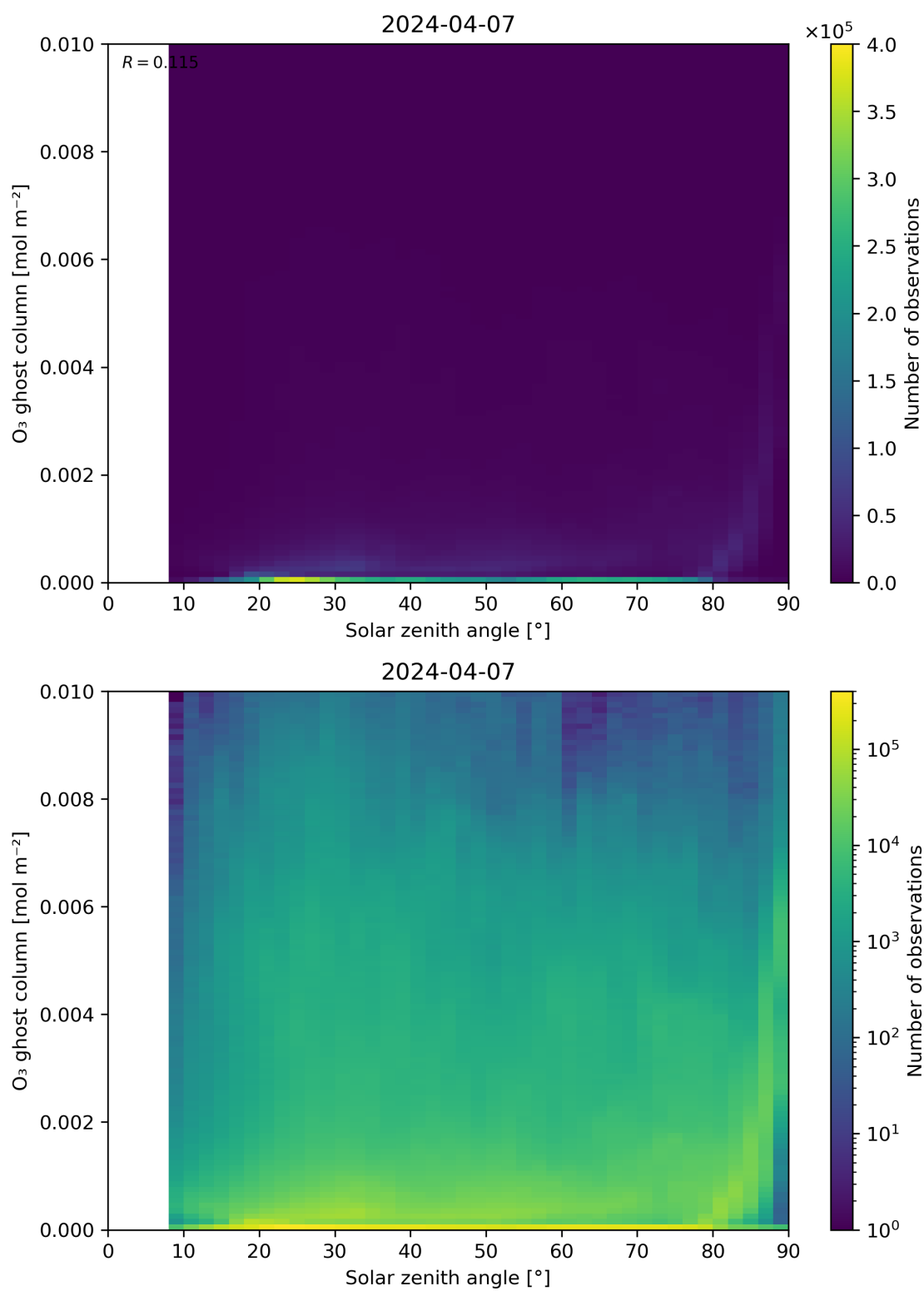
Figure 46: Scatter density plot of “Solar zenith angle” against “O 3 ghost column” for 2024-04-06 to 2024-04-08.
