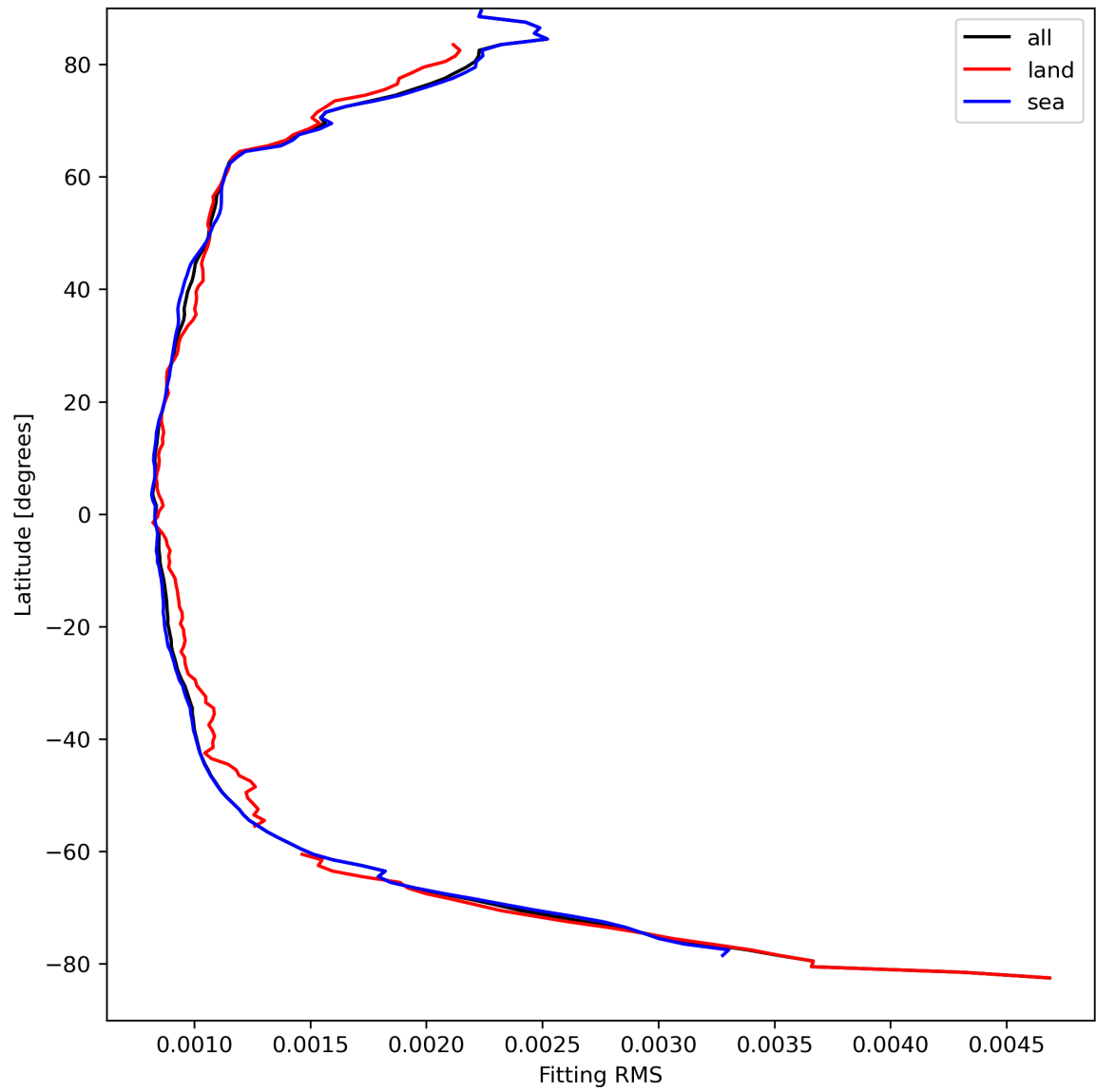
Figure 16: Zonal average of “Fitting RMS” for 2024-04-06 to 2024-04-08.
