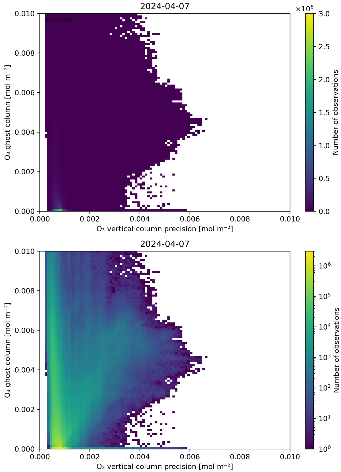
Figure 43: Scatter density plot of “ \text{O}_3 vertical column precision” against “ \text{O}_3 ghost column” for 2024-04-06 to 2024-04-08.
