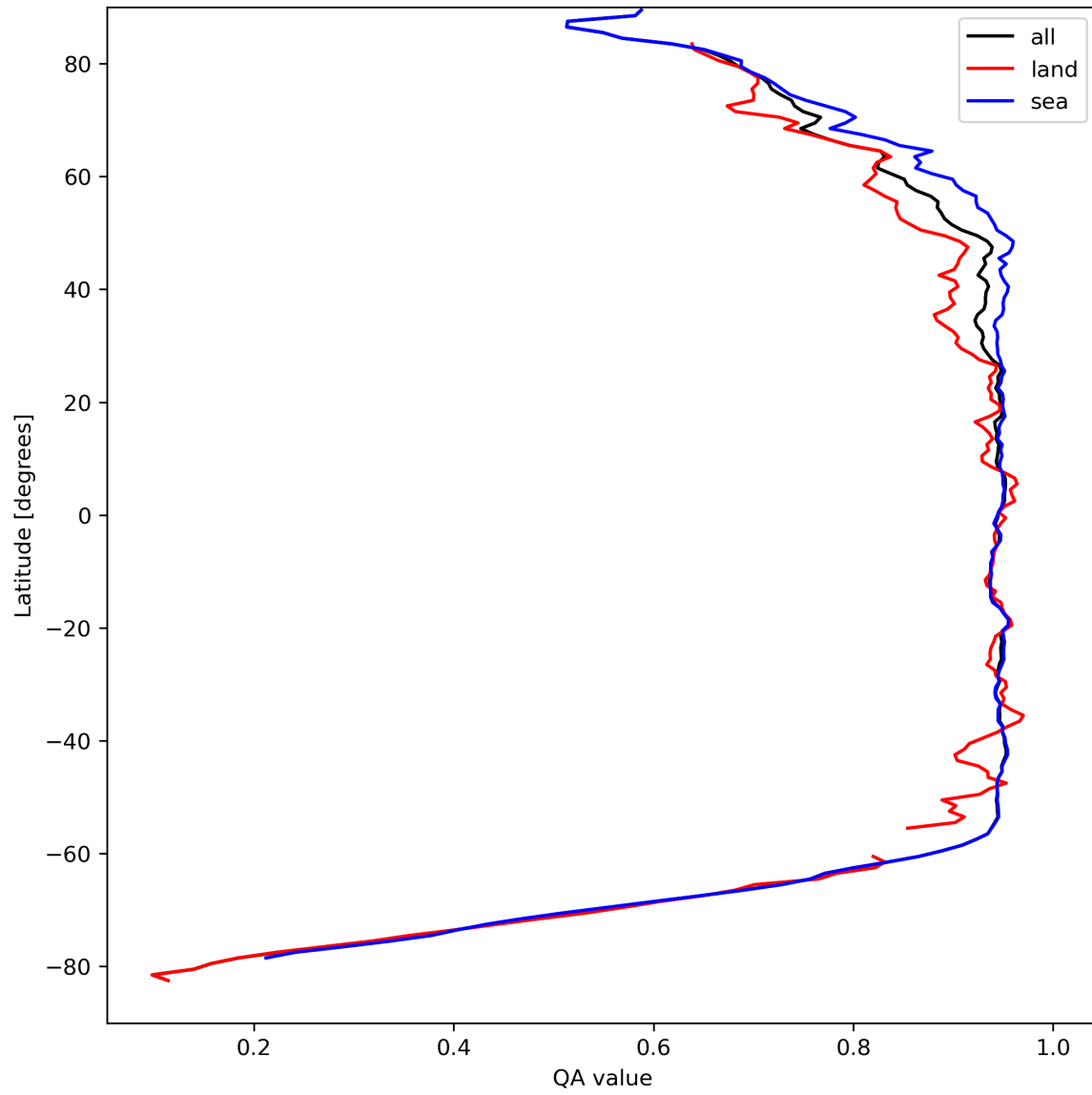
Figure 13: Zonal average of “QA value” for 2024-04-06 to 2024-04-08.
