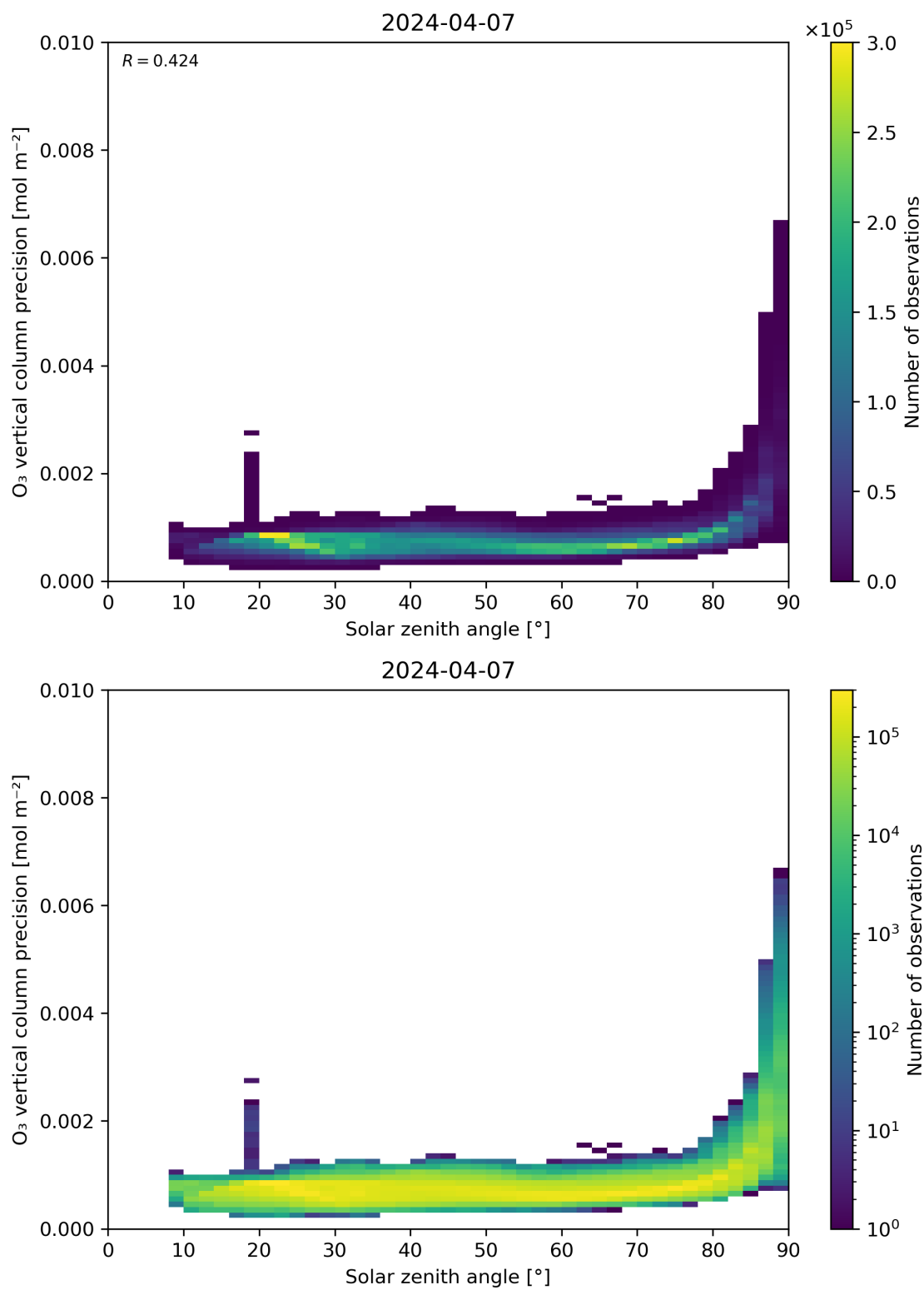
Figure 48: Scatter density plot of “Solar zenith angle” against “O 3 vertical column precision” for 2024-04-06 to 2024-04-08.
