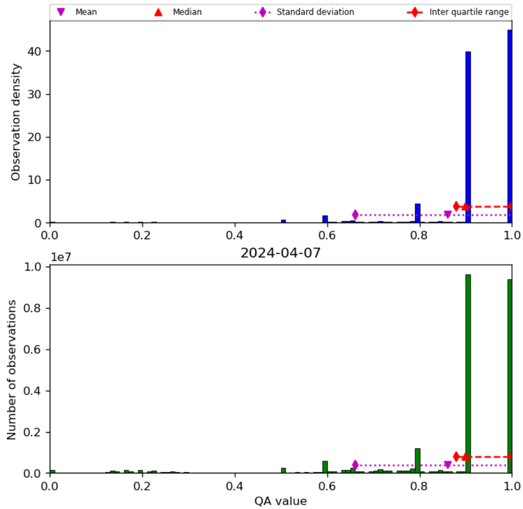
Figure 20: Histogram of “QA value” for 2024-04-06 to 2024-04-08
