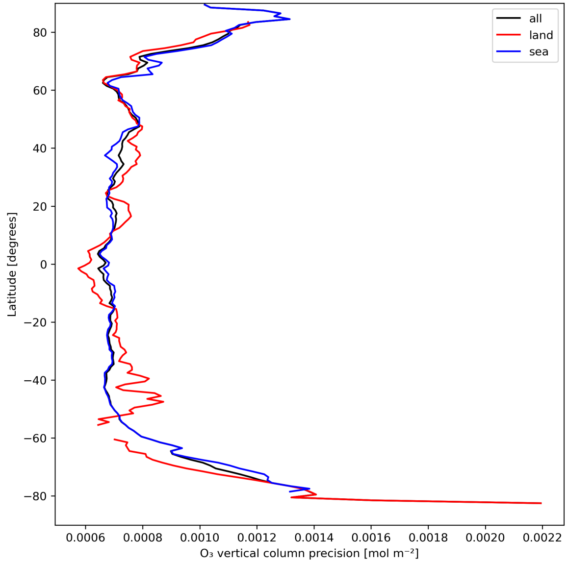
Figure 15: Zonal average of “O 3 vertical column precision” for 2024-04-06 to 2024-04-08.
