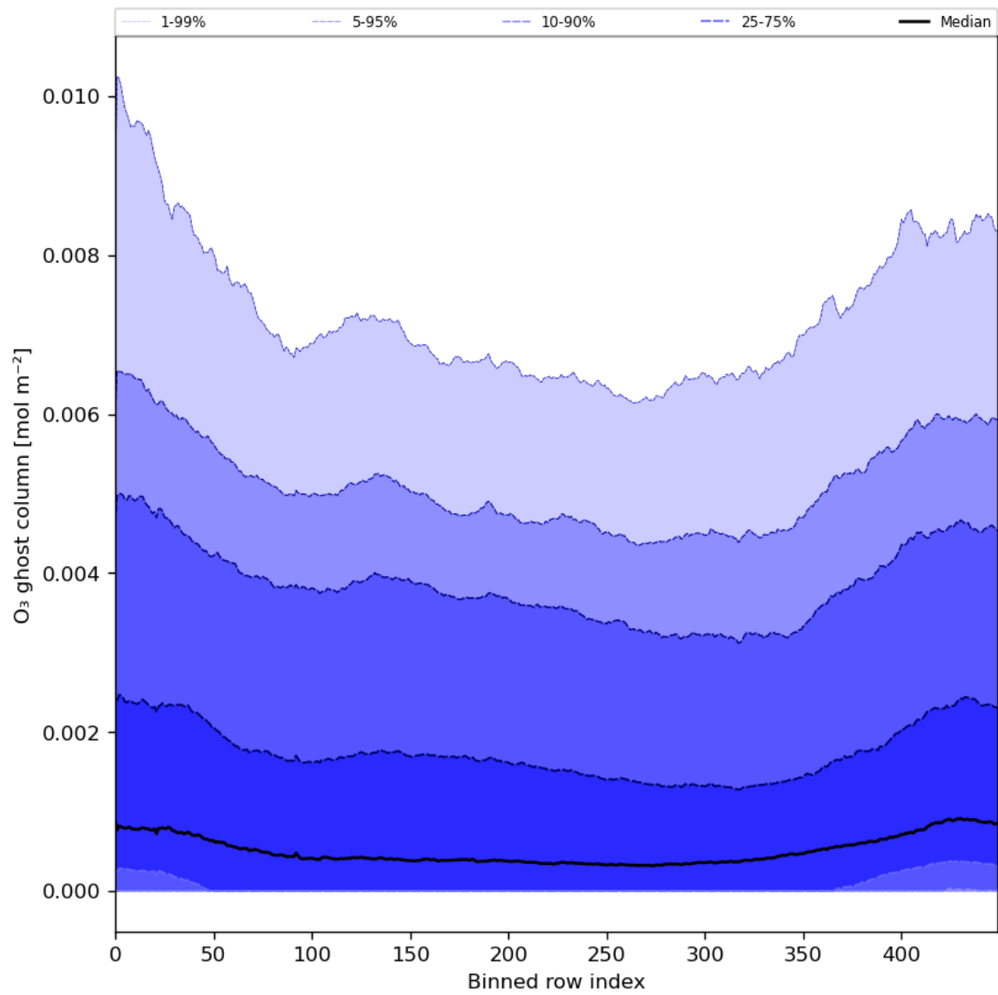
Figure 32: Along track statistics of “O 3 ghost column” for 2024-04-06 to 2024-04-08
