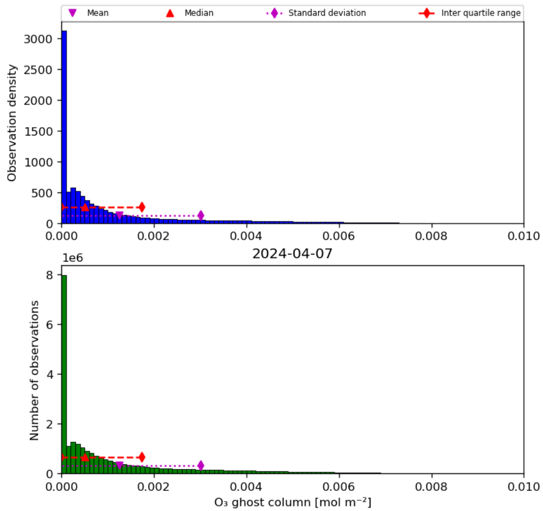
Figure 25: Histogram of “O 3 ghost column” for 2024-04-06 to 2024-04-08
