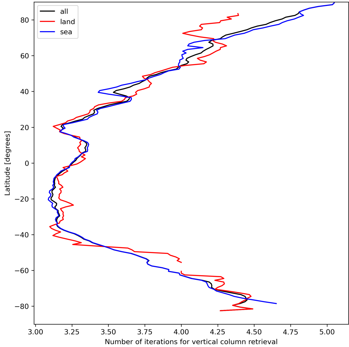
Figure 19: Zonal average of “Number of iterations for vertical column retrieval” for 2024-04-06 to 2024-04-08.
