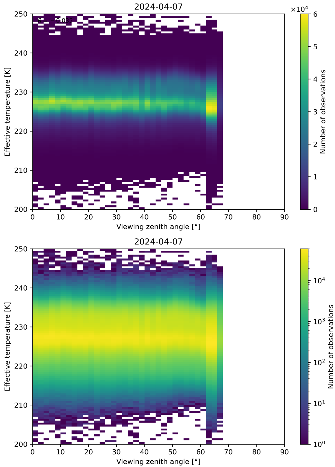
Figure 50: Scatter density plot of “Viewing zenith angle” against “Effective temperature” for 2024-04-06 to 2024-04-08.
