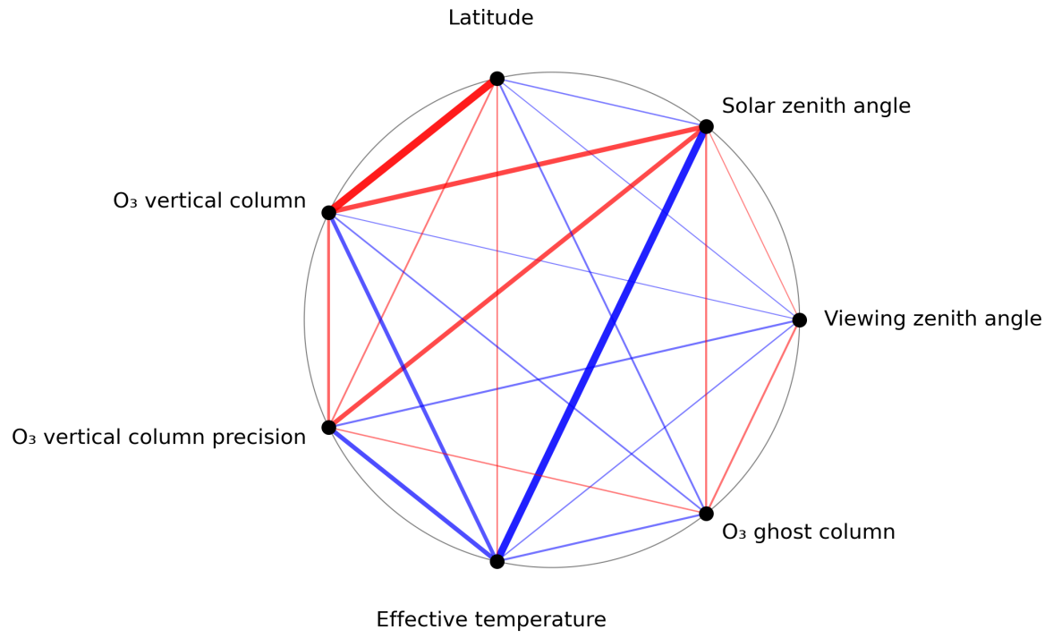
Figure 1: Map of correlation graph for 2024-04-06 to 2024-04-08.
