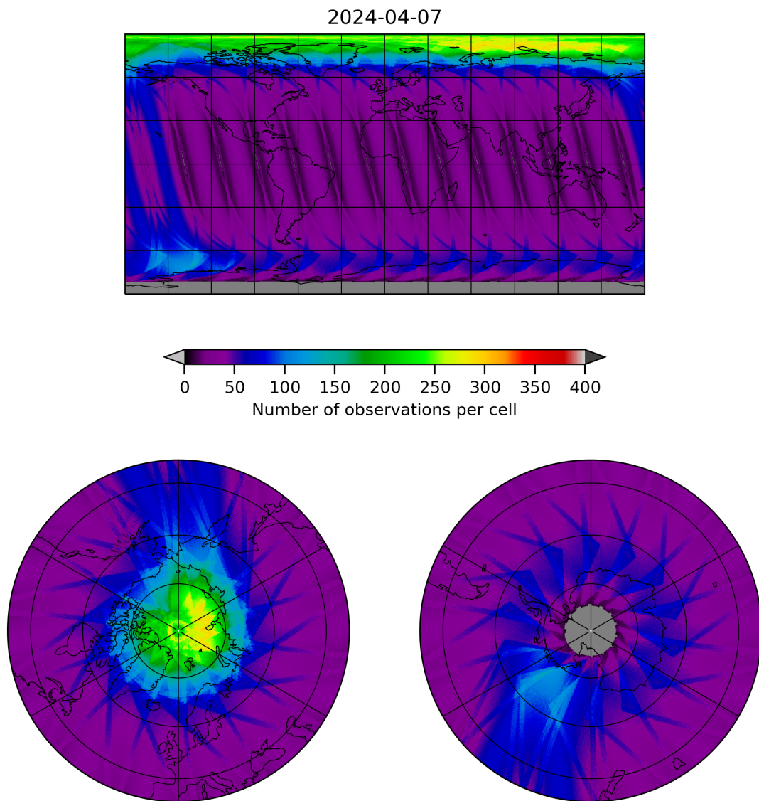
Figure 12: Map of the number of observations for 2024-04-06 to 2024-04-08
