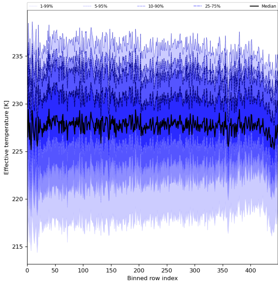
Figure 31: Along track statistics of “Effective temperature” for 2024-04-06 to 2024-04-08
