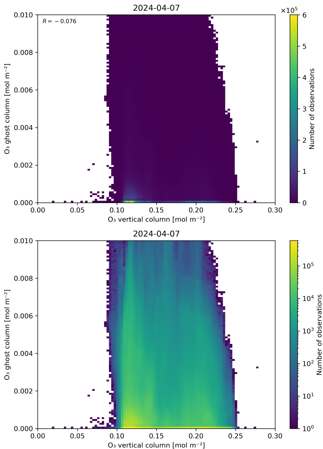
Figure 40: Scatter density plot of “O 3 vertical column” against “O 3 ghost column” for 2024-04-06 to 2024-04-08.
