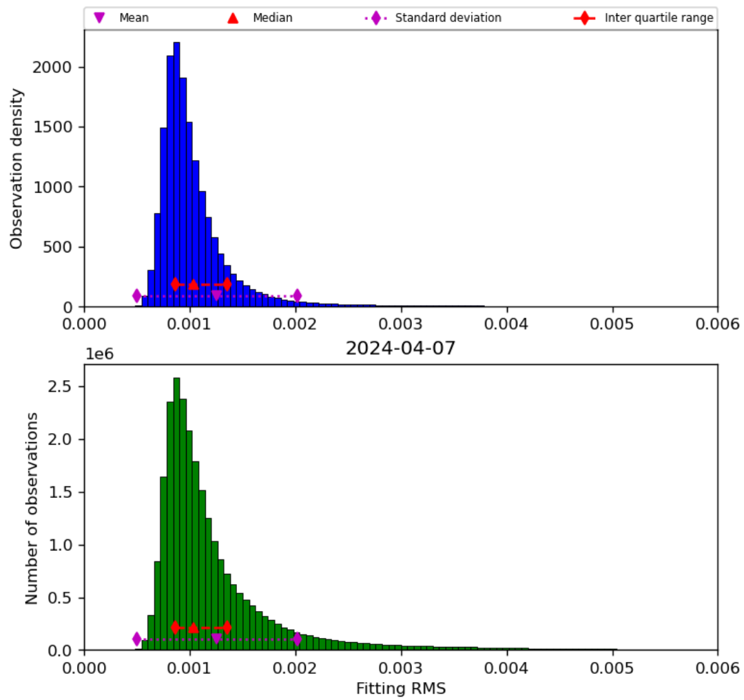
Figure 23: Histogram of “Fitting RMS” for 2024-04-06 to 2024-04-08
