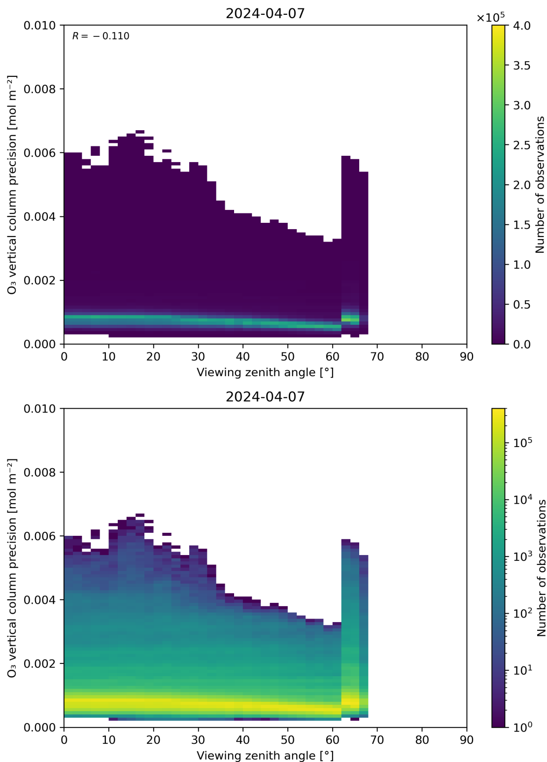
Figure 53: Scatter density plot of “Viewing zenith angle” against “O 3 vertical column precision” for 2024-04-06 to 2024-04-08.
