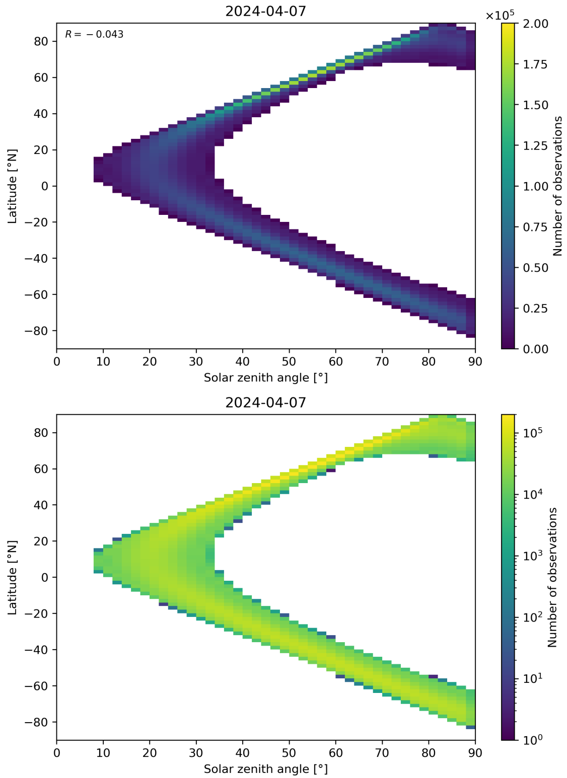
Figure 44: Scatter density plot of “Solar zenith angle” against “Latitude” for 2024-04-06 to 2024-04-08.
