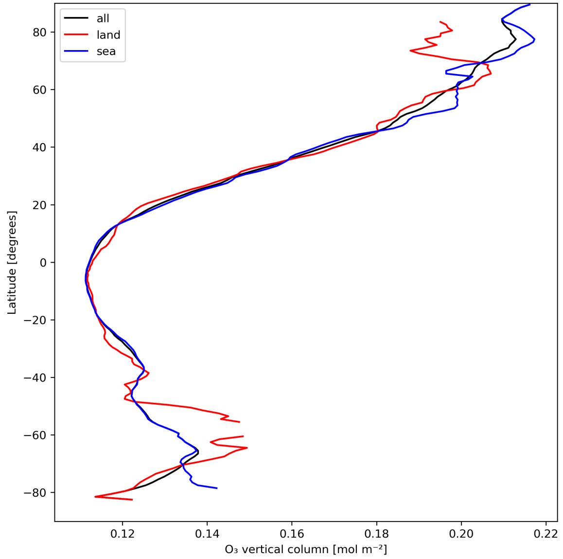
Figure 14: Zonal average of “O 3 vertical column” for 2024-04-06 to 2024-04-08.
