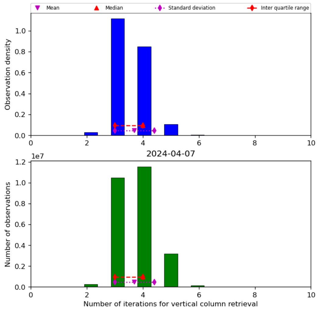
Figure 26: Histogram of “Number of iterations for vertical column retrieval” for 2024-04-06 to 2024-04-08
