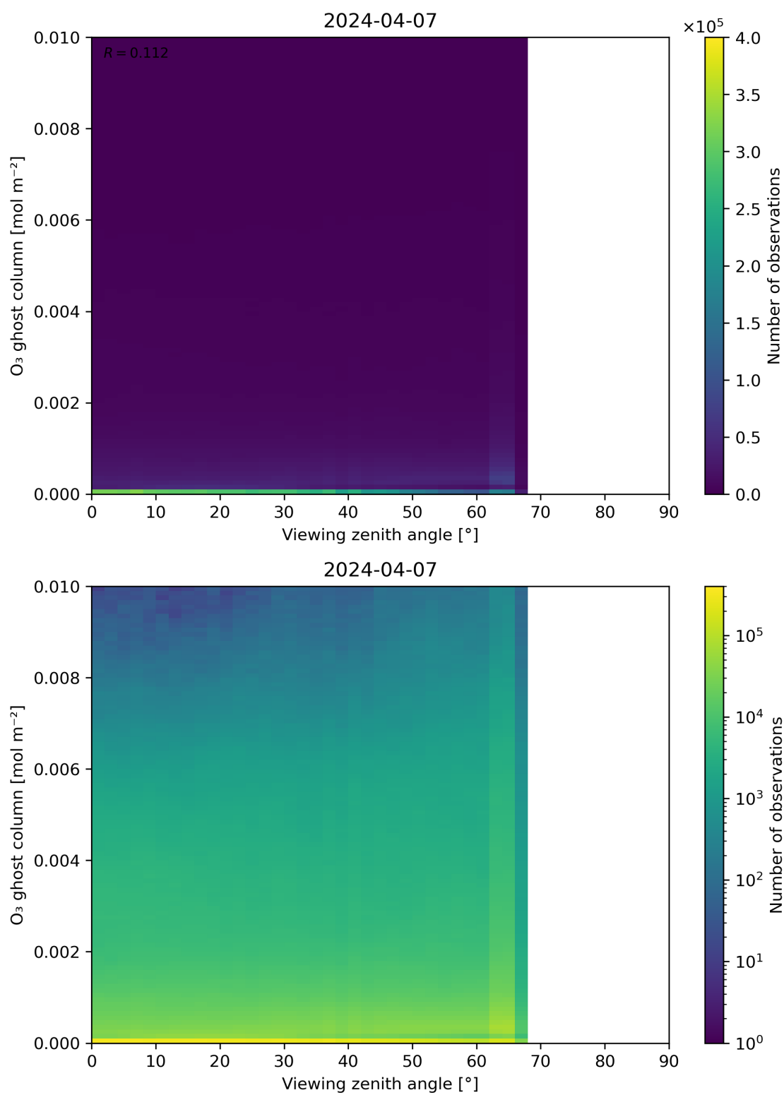
Figure 51: Scatter density plot of “Viewing zenith angle” against “O 3 ghost column” for 2024-04-06 to 2024-04-08.
