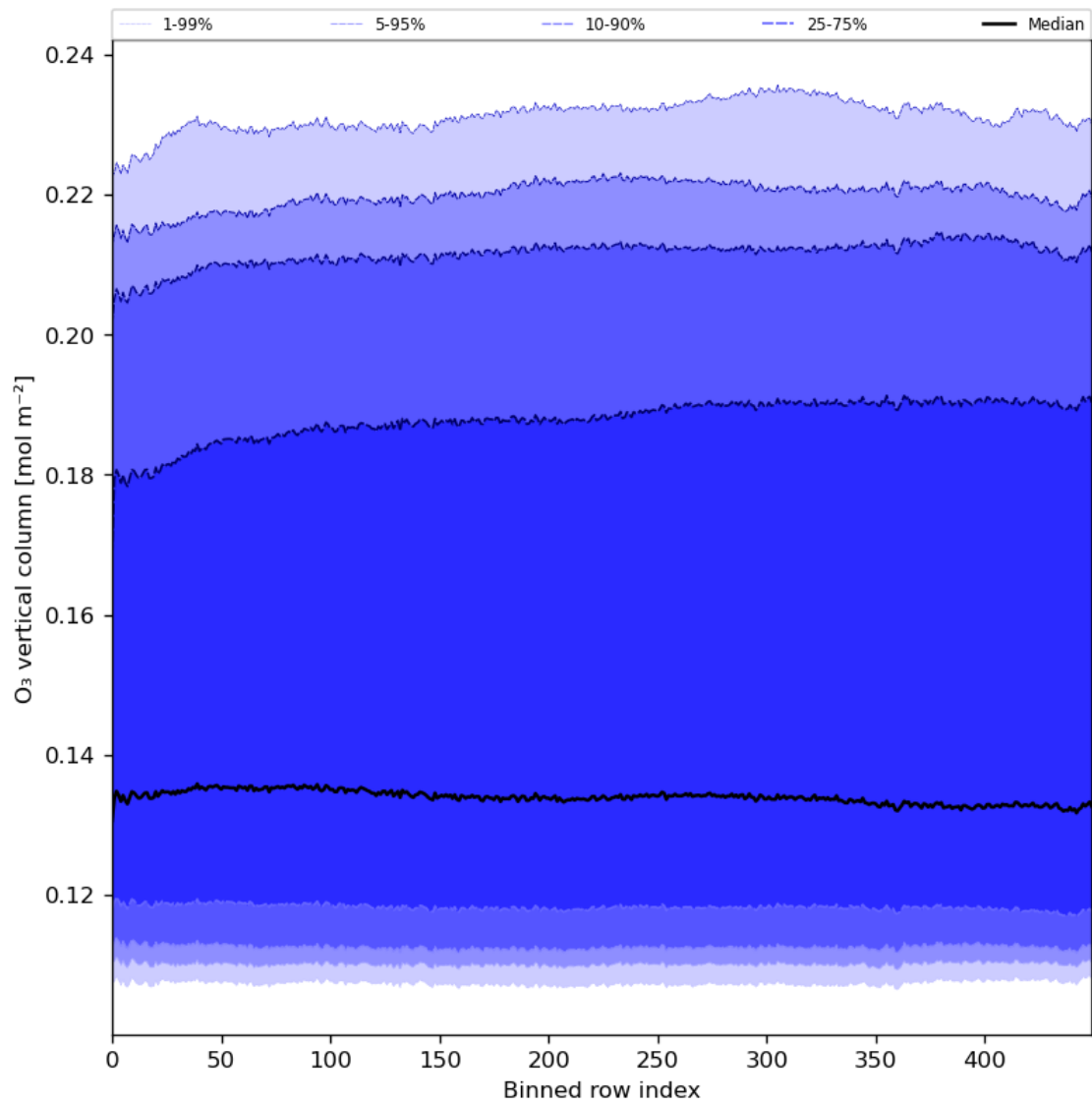
Figure 28: Along track statistics of “O 3 vertical column” for 2024-04-07 to 2024-04-09
