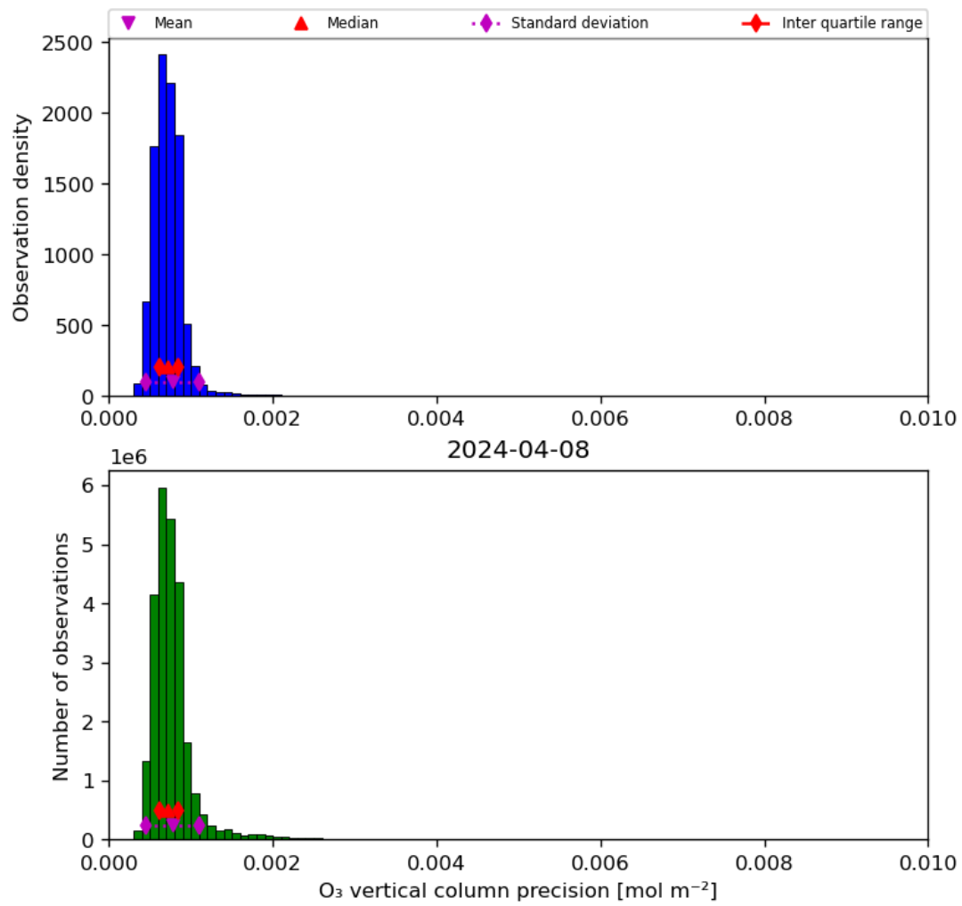
Figure 22: Histogram of “O 3 vertical column precision” for 2024-04-07 to 2024-04-09
