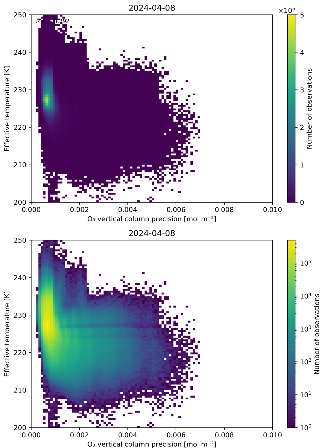
Figure 42: Scatter density plot of “O 3 vertical column precision” against “Effective temperature” for 2024-04-07 to 2024-04-09.
