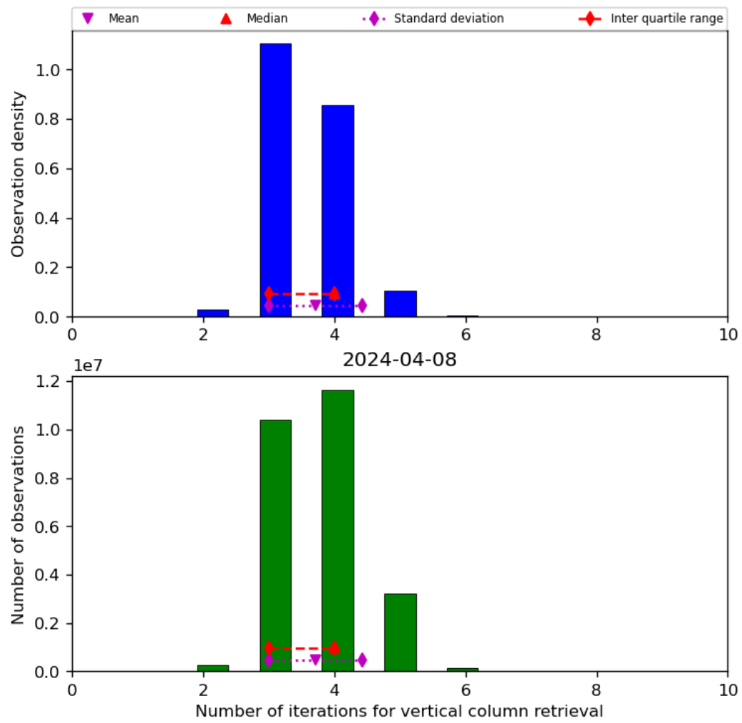
Figure 26: Histogram of “Number of iterations for vertical column retrieval” for 2024-04-07 to 2024-04-09
