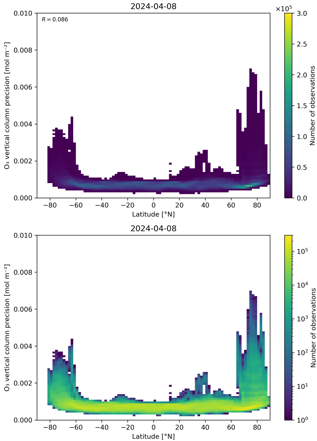
Figure 37: Scatter density plot of “Latitude” against “O 3 vertical column precision” for 2024-04-07 to 2024-04-09.
