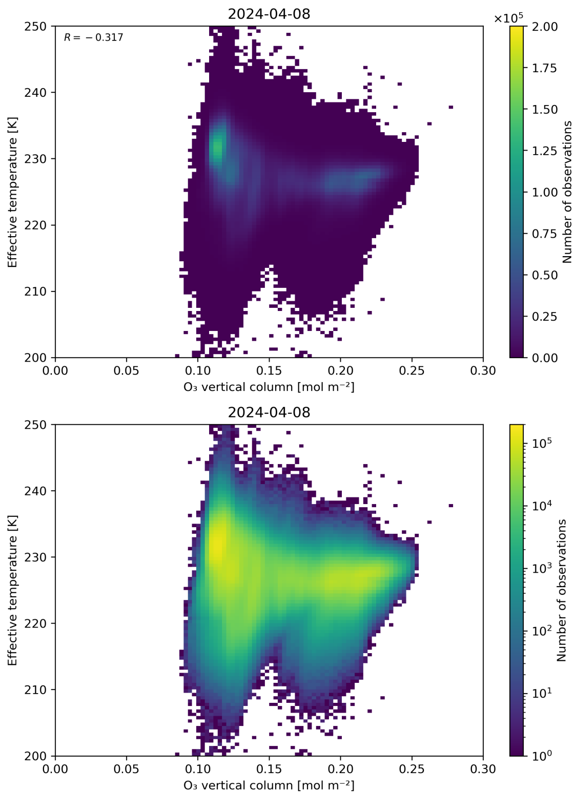
Figure 39: Scatter density plot of “O 3 vertical column” against “Effective temperature” for 2024-04-07 to 2024-04-09.
