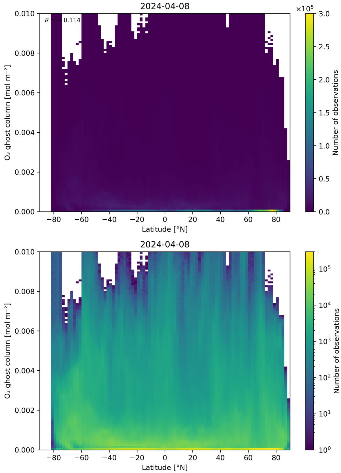
Figure 35: Scatter density plot of “Latitude” against “O 3 ghost column” for 2024-04-07 to 2024-04-09.
