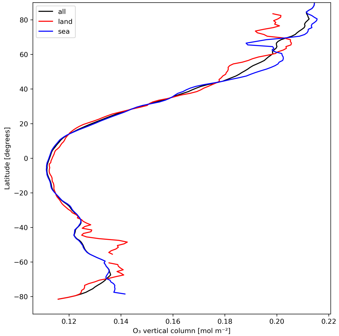
Figure 14: Zonal average of “O 3 vertical column” for 2024-04-07 to 2024-04-09.
