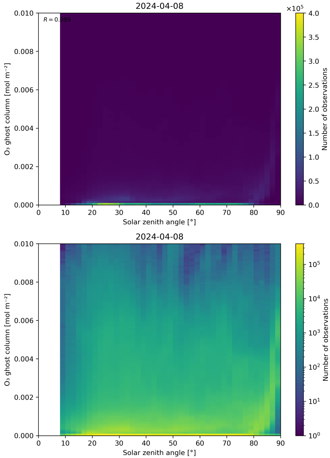
Figure 46: Scatter density plot of “Solar zenith angle” against “O 3 ghost column” for 2024-04-07 to 2024-04-09.
