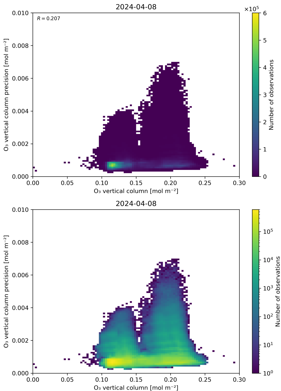
Figure 41: Scatter density plot of “O 3 vertical column” against “O 3 vertical column precision” for 2024-04-07 to 2024-04-09.
