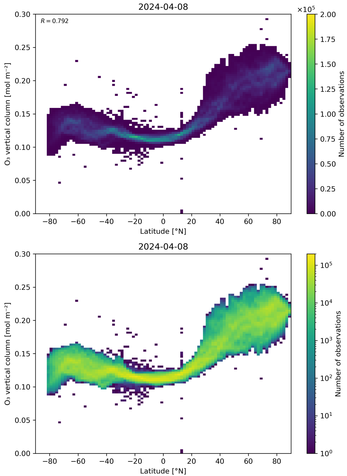
Figure 36: Scatter density plot of “Latitude” against “O 3 vertical column” for 2024-04-07 to 2024-04-09.
