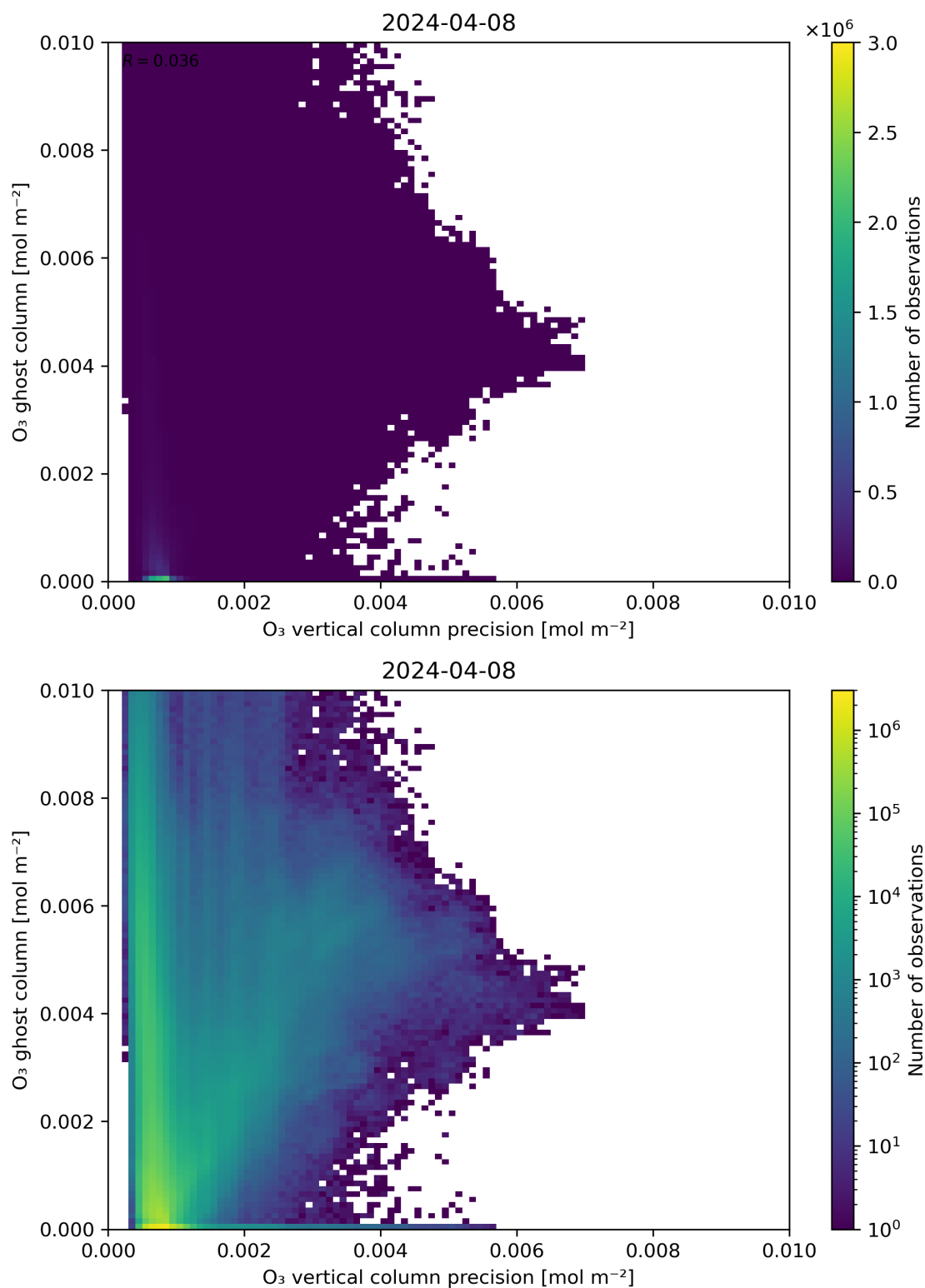
Figure 43: Scatter density plot of “ O_3 vertical column precision” against “ O_3 ghost column” for 2024-04-07 to 2024-04-09.
