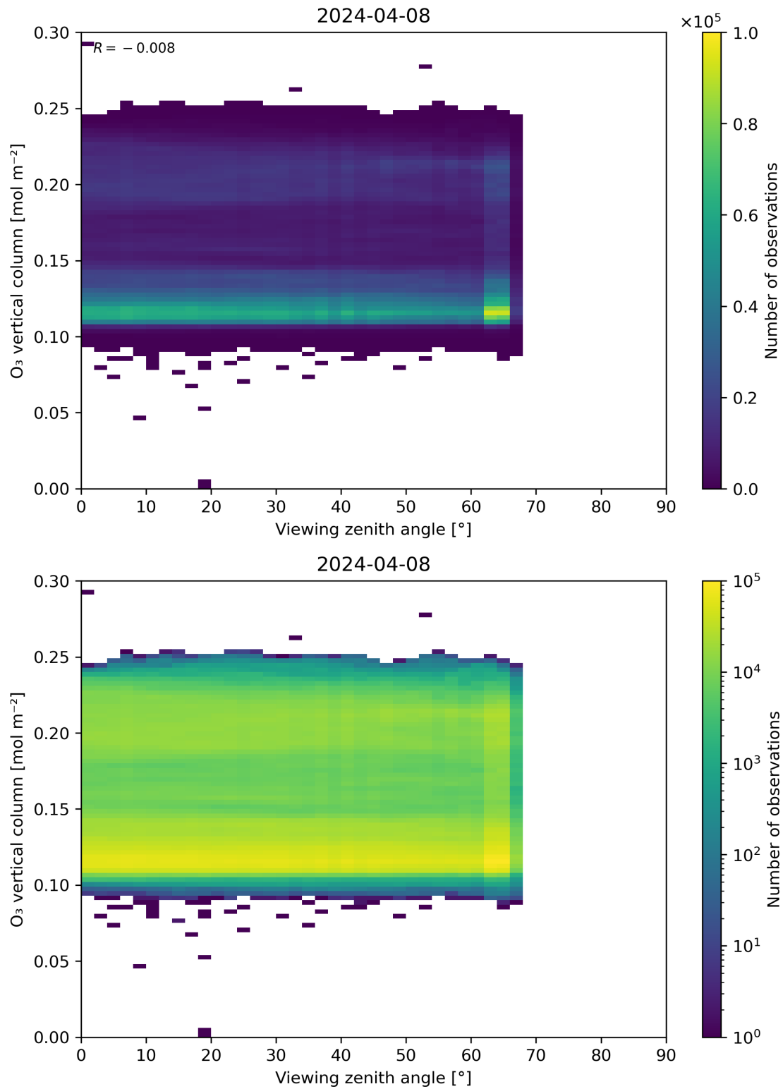
Figure 52: Scatter density plot of “Viewing zenith angle” against “O 3 vertical column” for 2024-04-07 to 2024-04-09.
