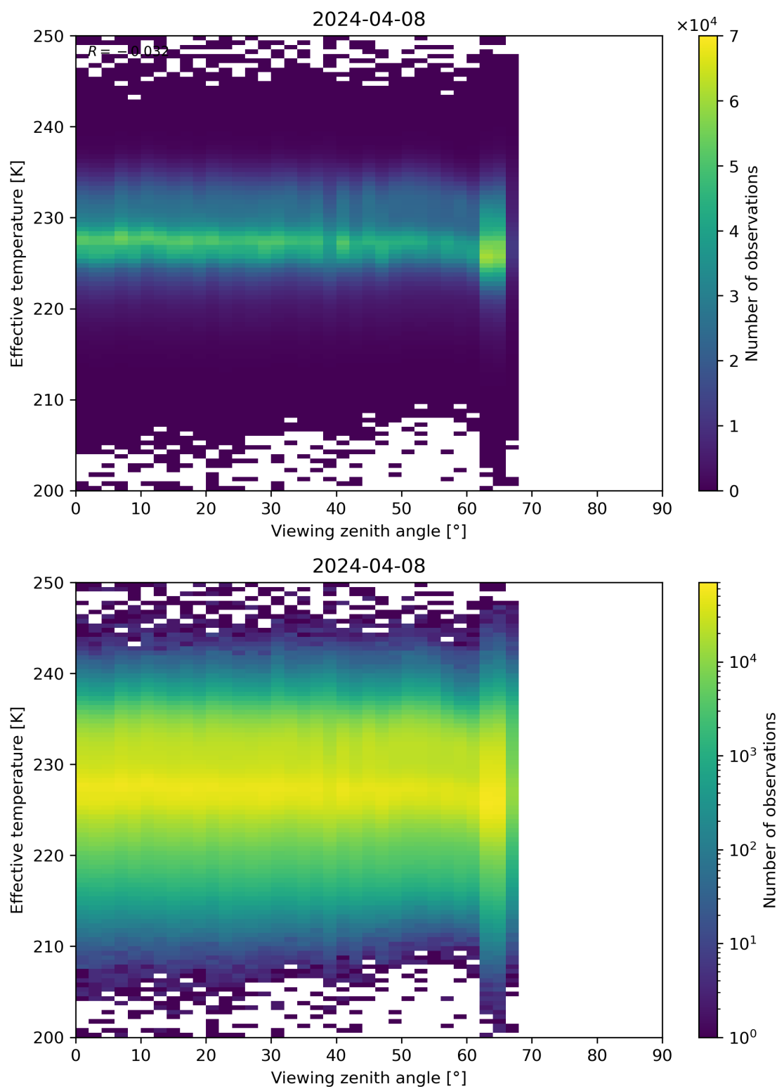
Figure 50: Scatter density plot of “Viewing zenith angle” against “Effective temperature” for 2024-04-07 to 2024-04-09.
