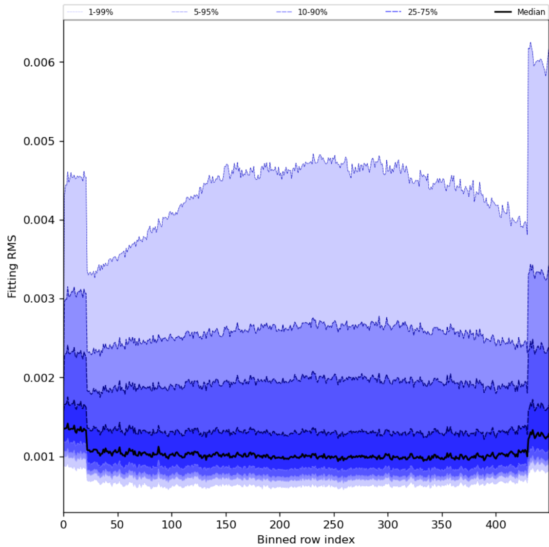
Figure 30: Along track statistics of “Fitting RMS” for 2024-04-07 to 2024-04-09
