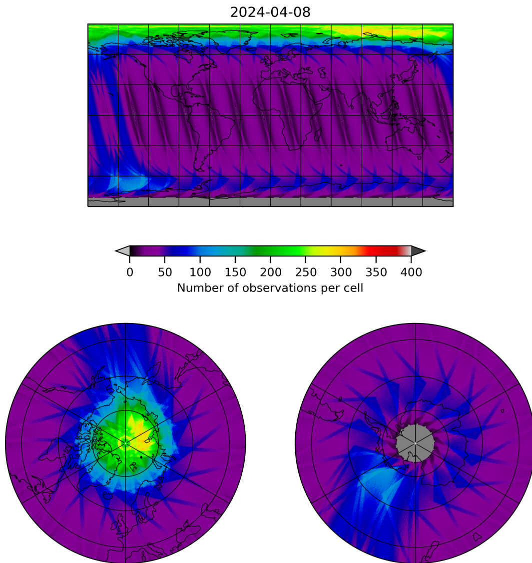
Figure 12: Map of the number of observations for 2024-04-07 to 2024-04-09
