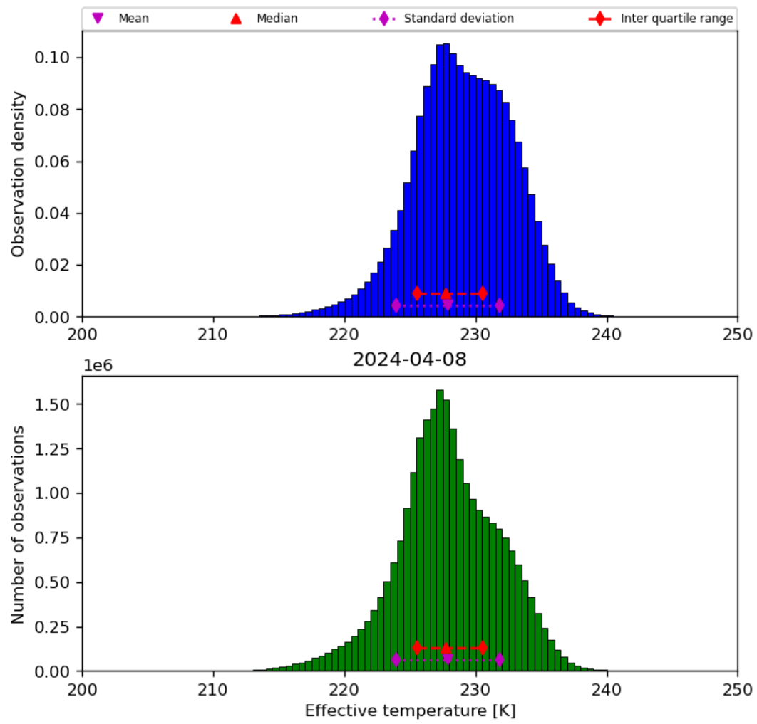
Figure 24: Histogram of “Effective temperature” for 2024-04-07 to 2024-04-09
