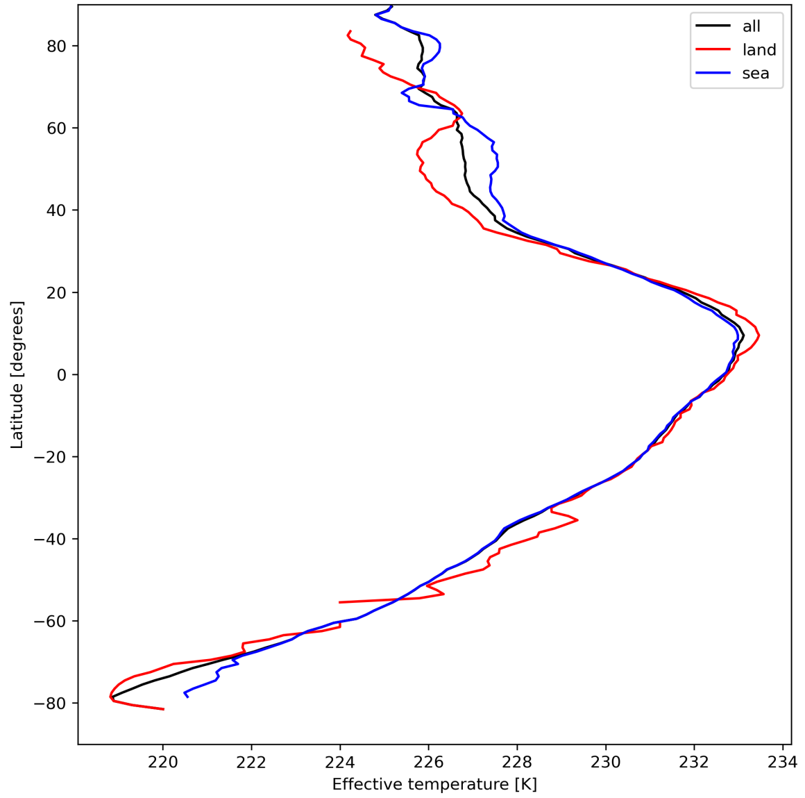
Figure 17: Zonal average of “Effective temperature” for 2024-04-07 to 2024-04-09.
