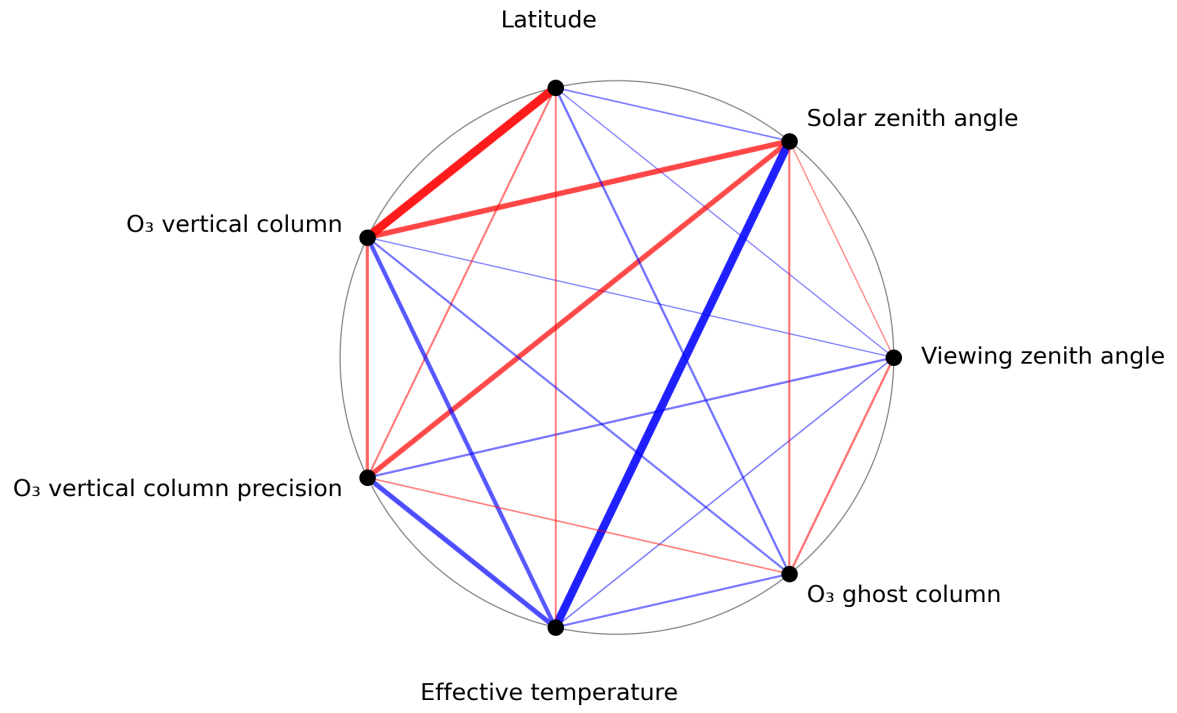
Figure 1: Map of correlation graph for 2024-04-07 to 2024-04-09.
