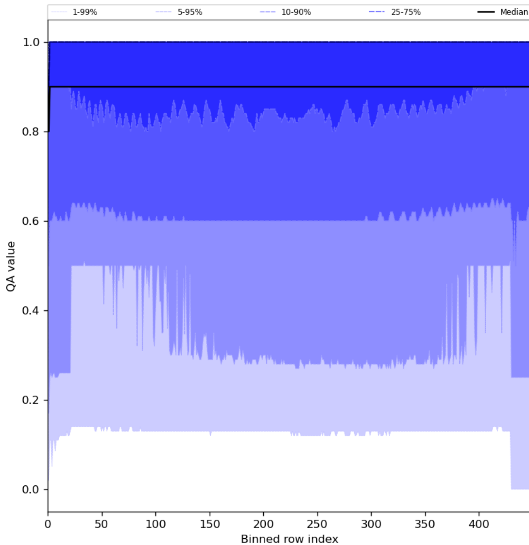
Figure 27: Along track statistics of “QA value” for 2024-04-07 to 2024-04-09
