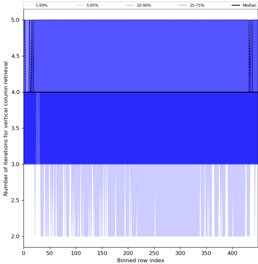
Figure 33: Along track statistics of “Number of iterations for vertical column retrieval” for 2024-04-07 to 2024-04-09
