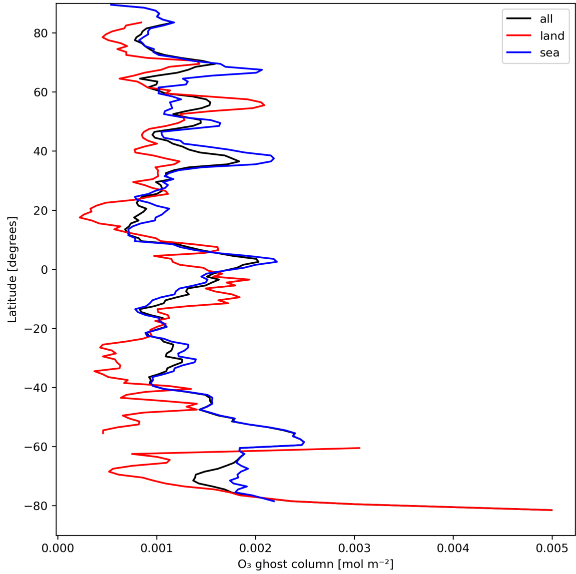
Figure 18: Zonal average of "O 3 ghost column" for 2024-04-07 to 2024-04-09.
