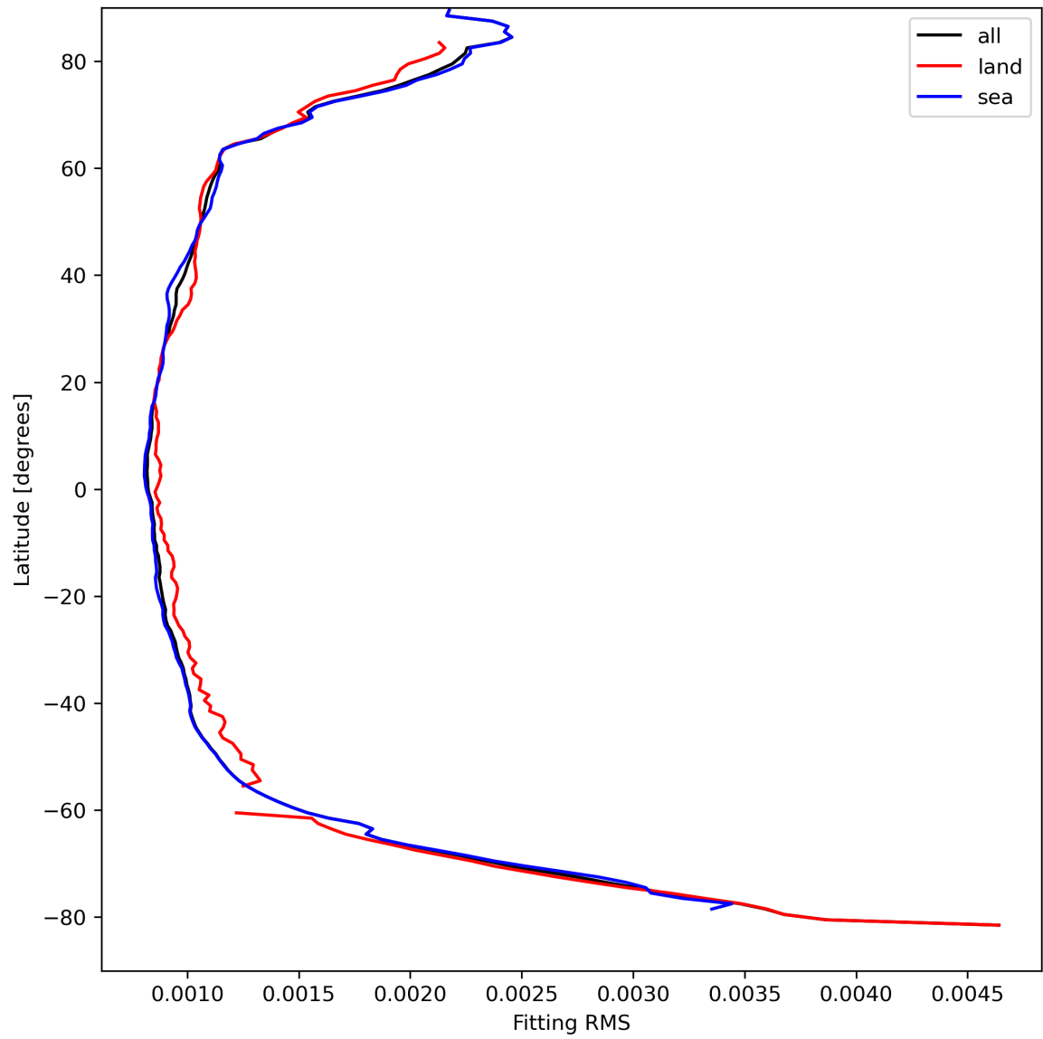
Figure 16: Zonal average of “Fitting RMS” for 2024-04-07 to 2024-04-09.
