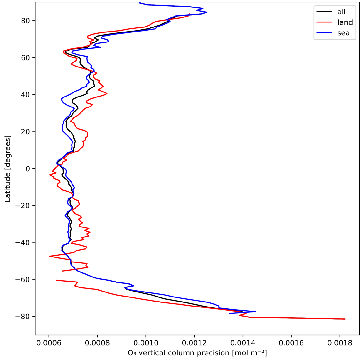
Figure 15: Zonal average of "O 3 vertical column precision" for 2024-04-07 to 2024-04-09.
