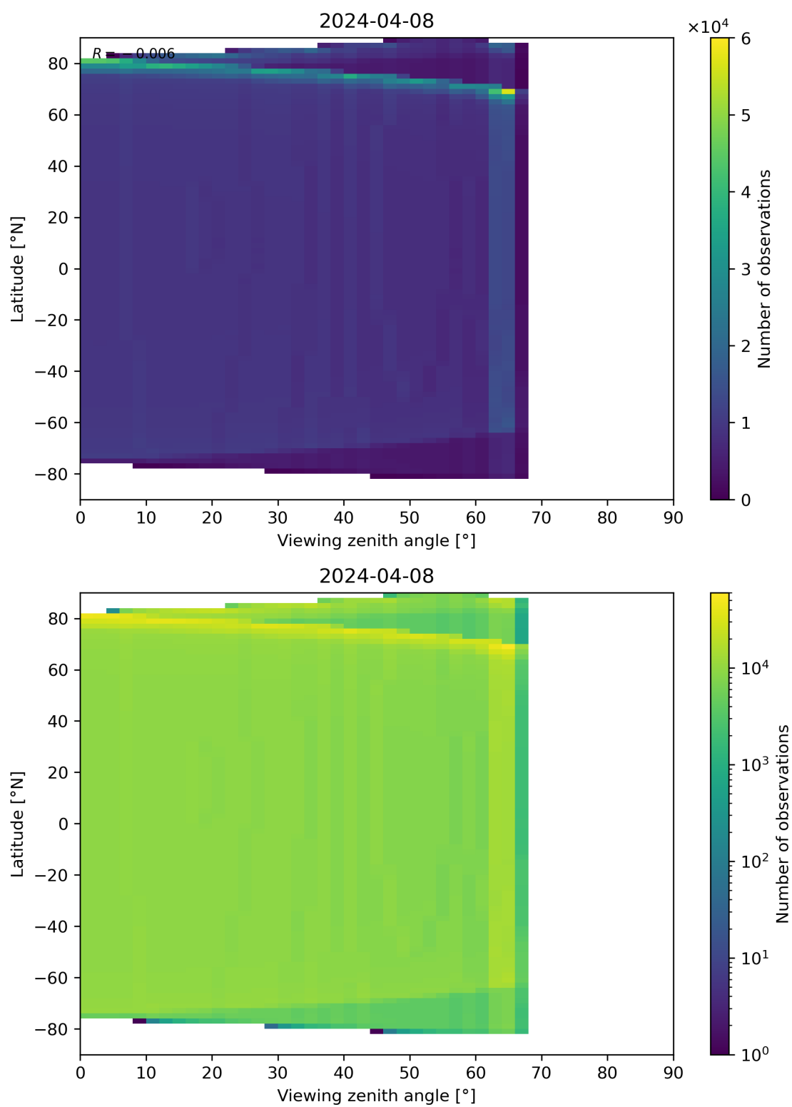
Figure 49: Scatter density plot of “Viewing zenith angle” against “Latitude” for 2024-04-07 to 2024-04-09.
