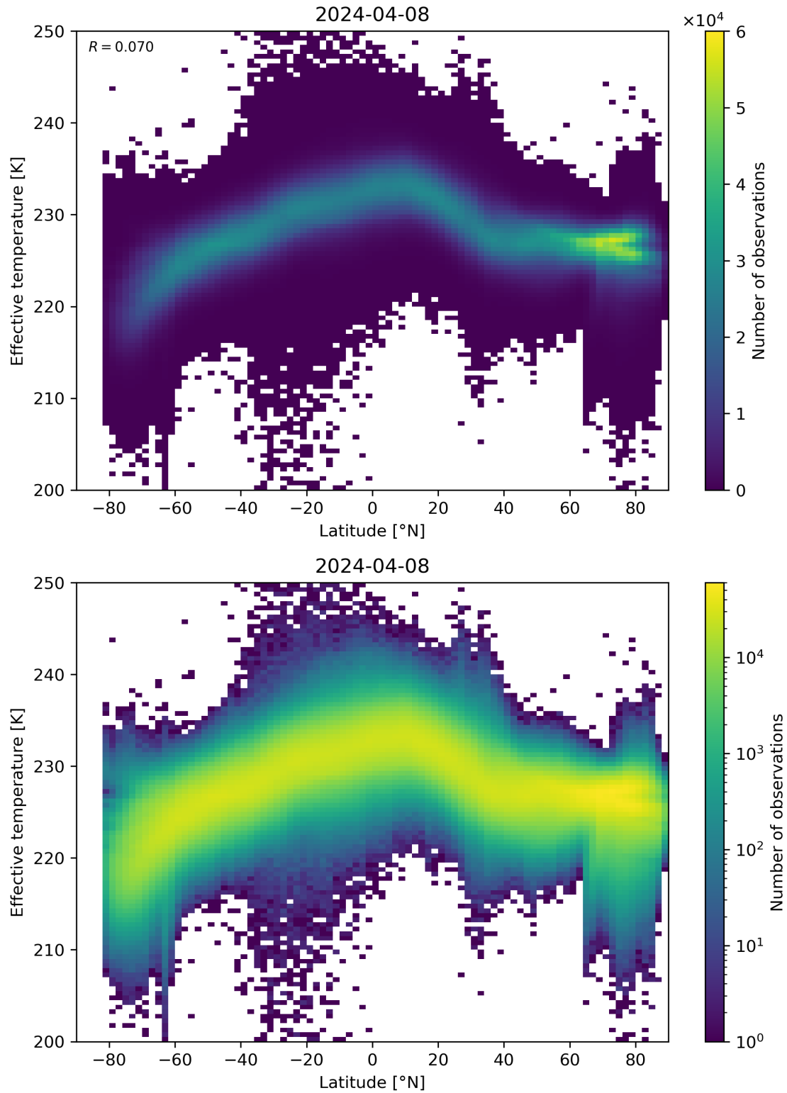
Figure 34: Scatter density plot of “Latitude” against “Effective temperature” for 2024-04-07 to 2024-04-09.
