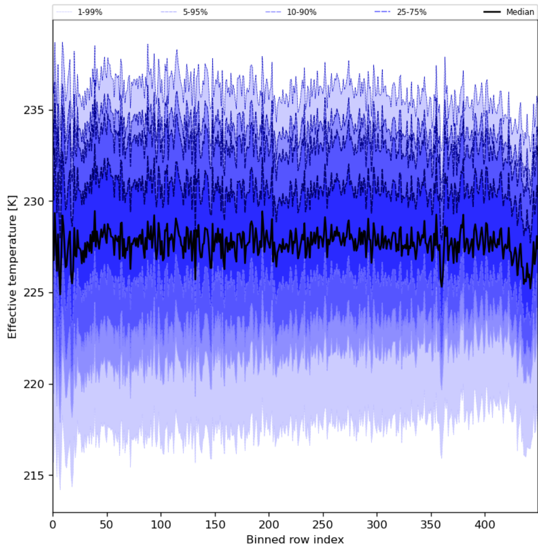
Figure 31: Along track statistics of “Effective temperature” for 2024-04-07 to 2024-04-09
