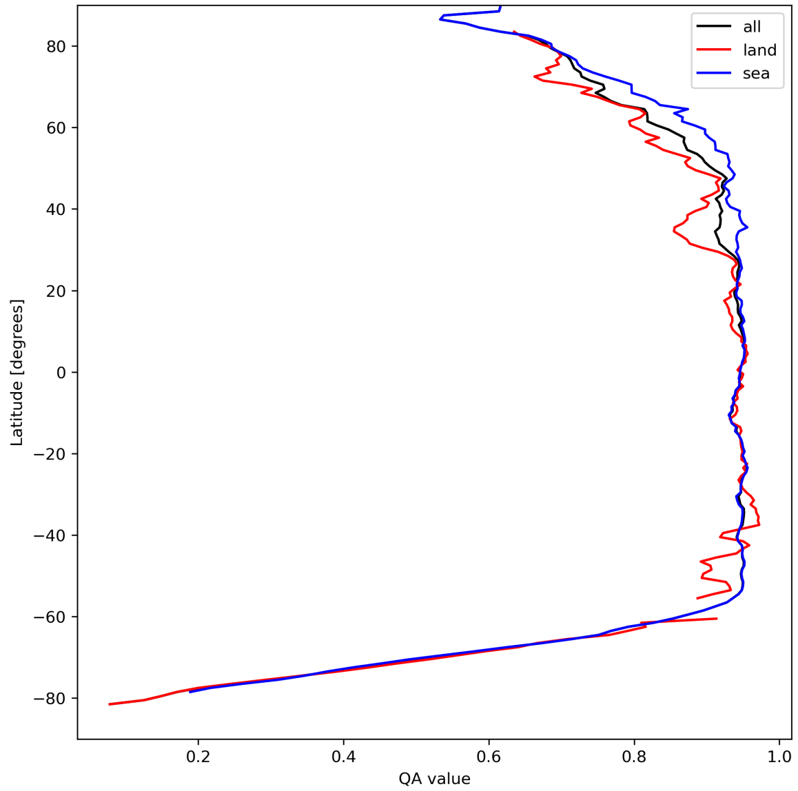
Figure 13: Zonal average of “QA value” for 2024-04-07 to 2024-04-09.
