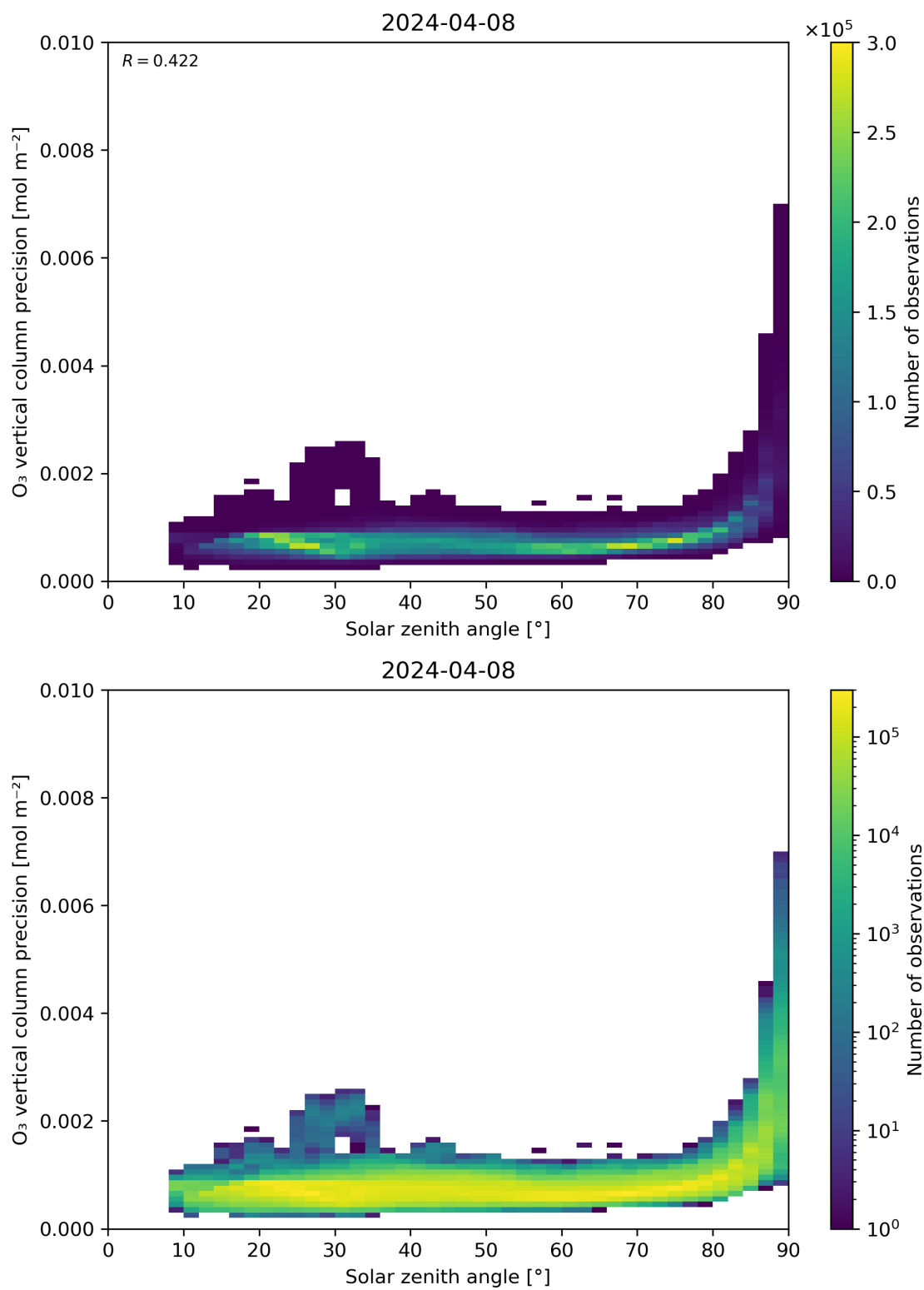
Figure 48: Scatter density plot of “Solar zenith angle” against “O 3 vertical column precision” for 2024-04-07 to 2024-04-09.
