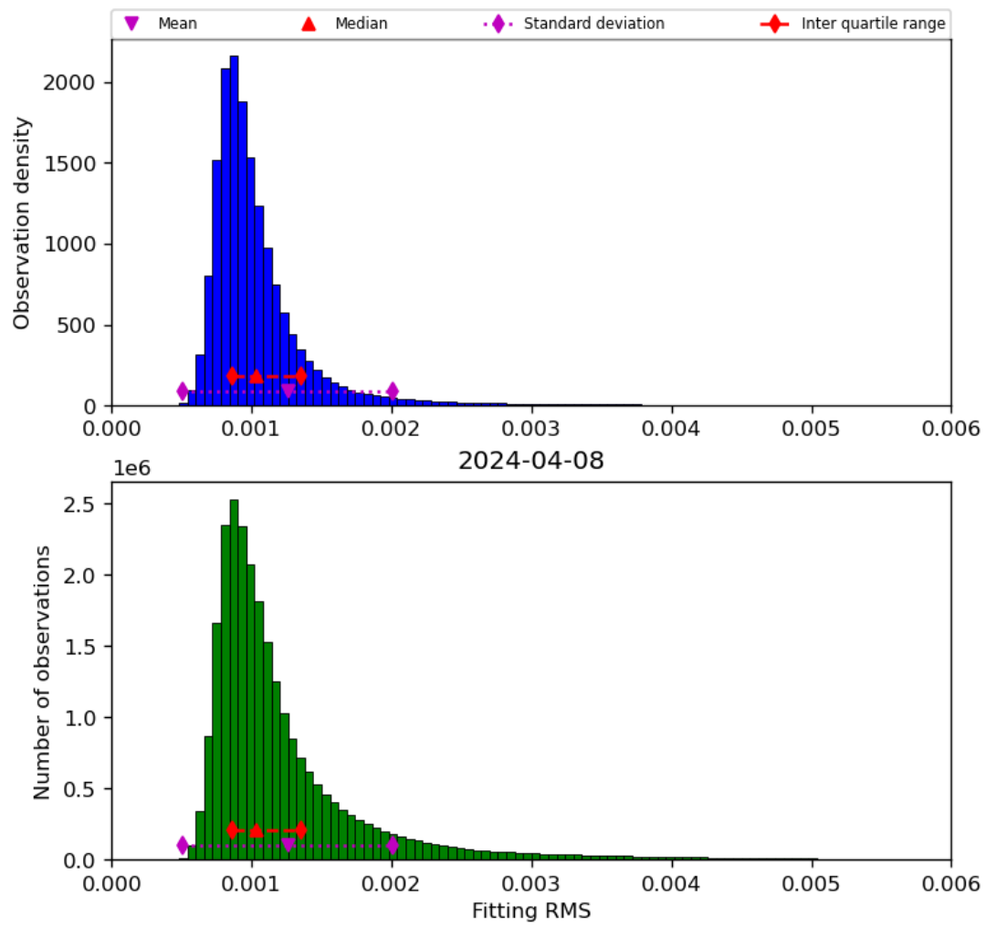
Figure 23: Histogram of “Fitting RMS” for 2024-04-07 to 2024-04-09
