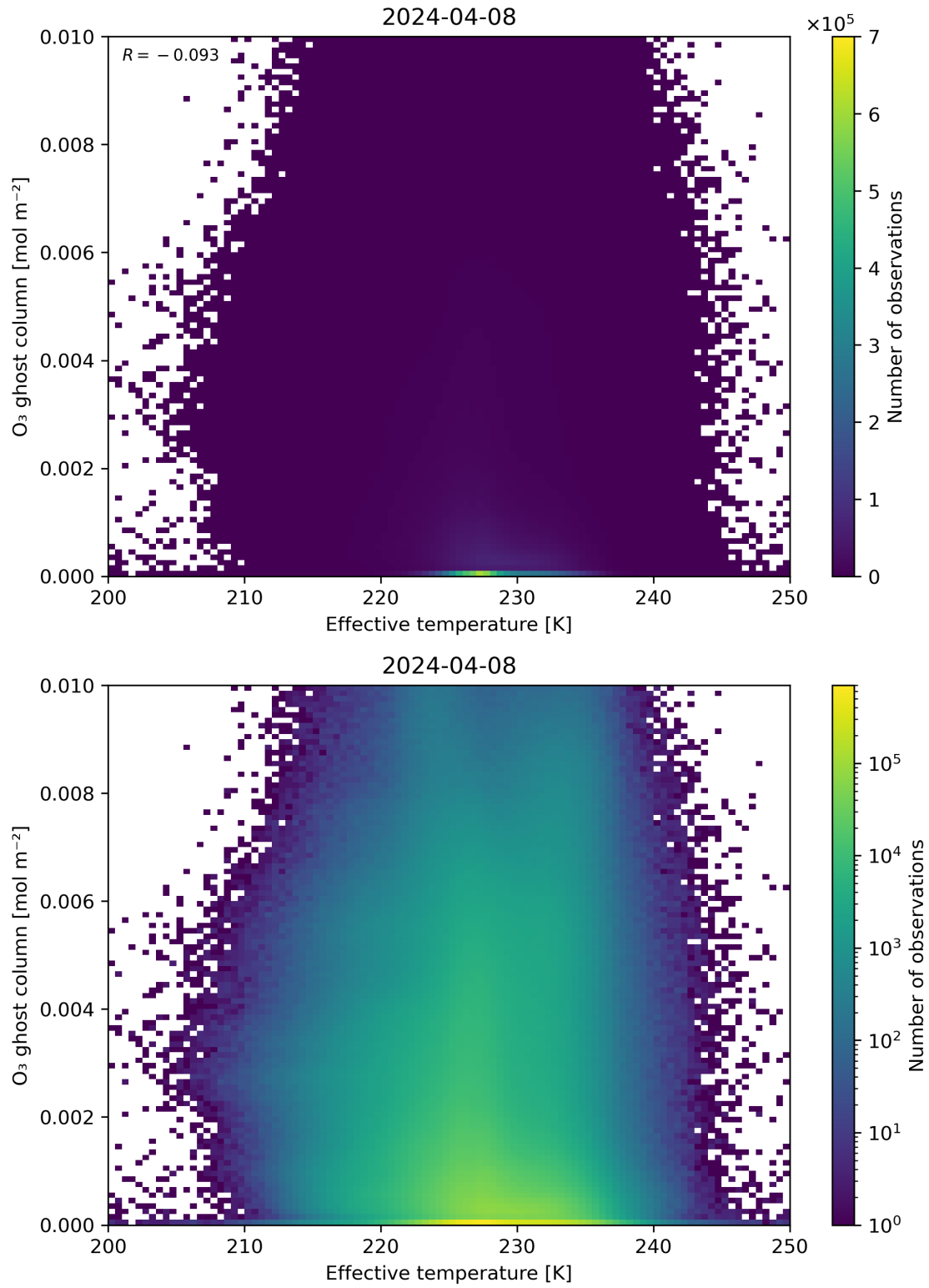
Figure 38: Scatter density plot of “Effective temperature” against “O 3 ghost column” for 2024-04-07 to 2024-04-09.
