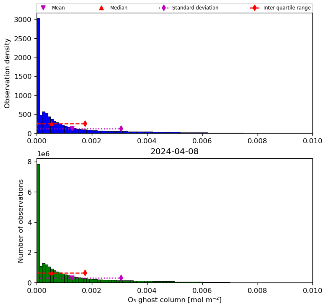
Figure 25: Histogram of “O 3 ghost column” for 2024-04-07 to 2024-04-09
