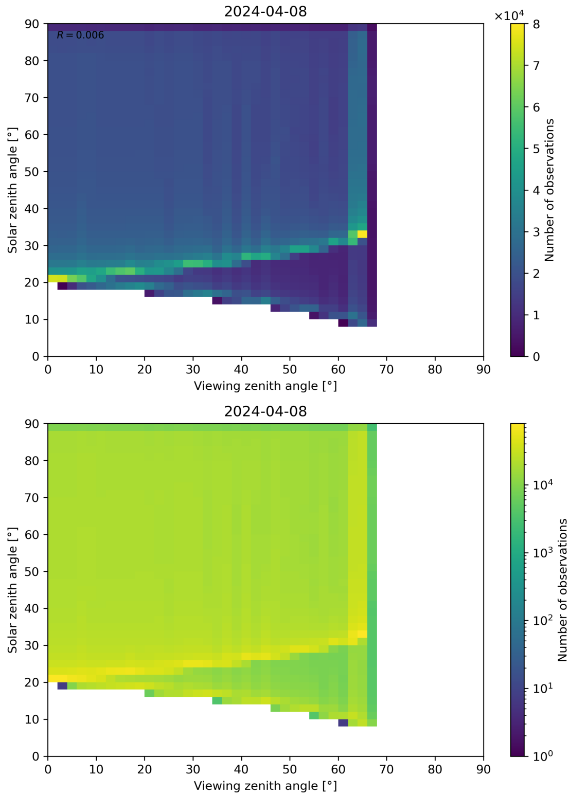
Figure 54: Scatter density plot of “Viewing zenith angle” against “Solar zenith angle” for 2024-04-07 to 2024-04-09.
