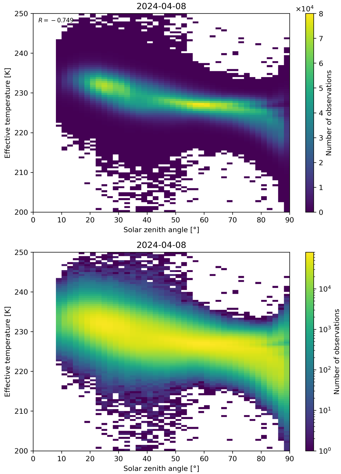
Figure 45: Scatter density plot of “Solar zenith angle” against “Effective temperature” for 2024-04-07 to 2024-04-09.
