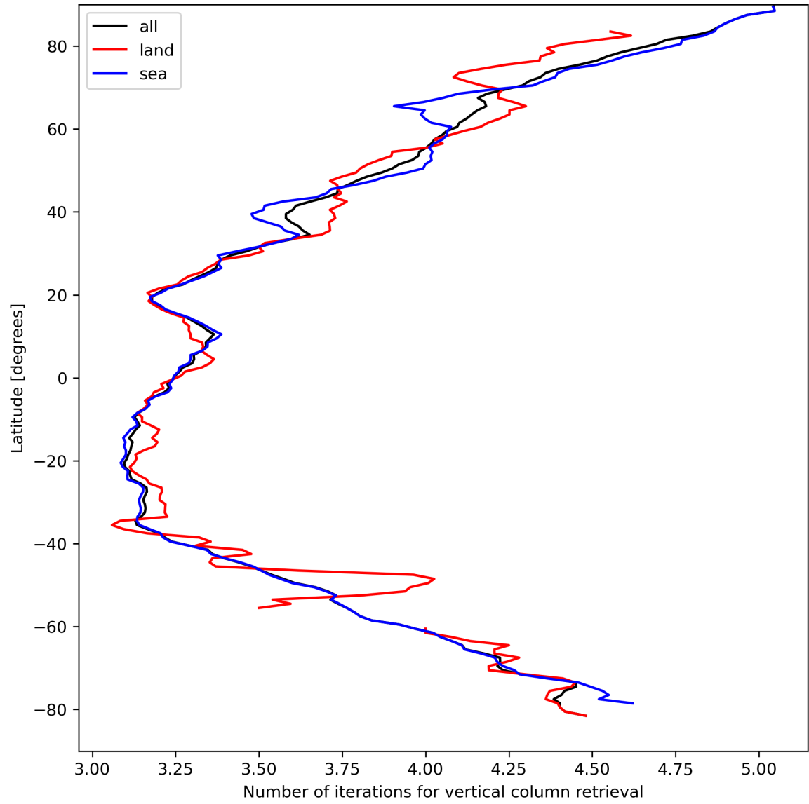
Figure 19: Zonal average of “Number of iterations for vertical column retrieval” for 2024-04-07 to 2024-04-09.
