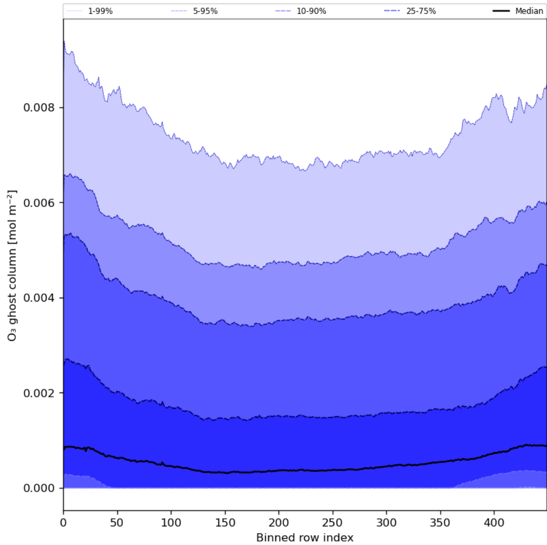
Figure 32: Along track statistics of “O 3 ghost column” for 2024-04-07 to 2024-04-09
