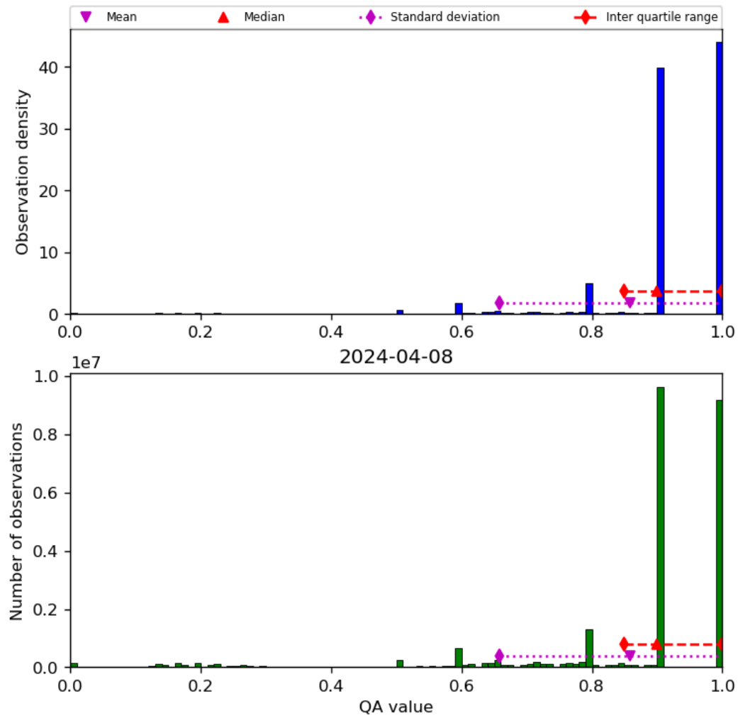
Figure 20: Histogram of “QA value” for 2024-04-07 to 2024-04-09
