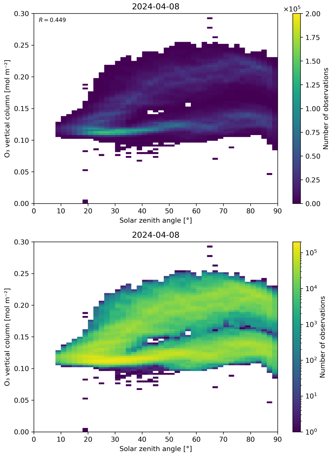
Figure 47: Scatter density plot of “Solar zenith angle” against “O 3 vertical column” for 2024-04-07 to 2024-04-09.
