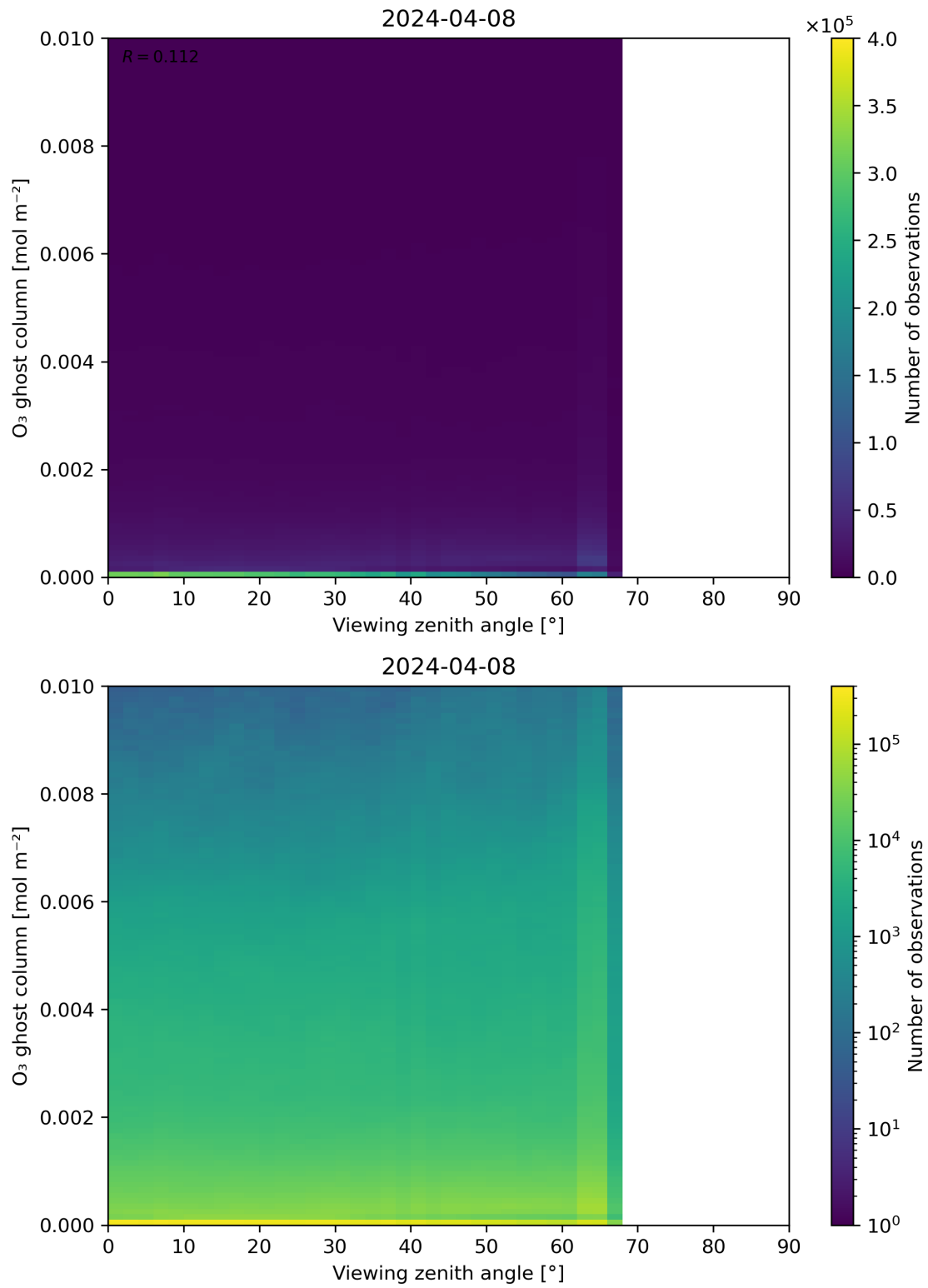
Figure 51: Scatter density plot of “Viewing zenith angle” against “O 3 ghost column” for 2024-04-07 to 2024-04-09.
