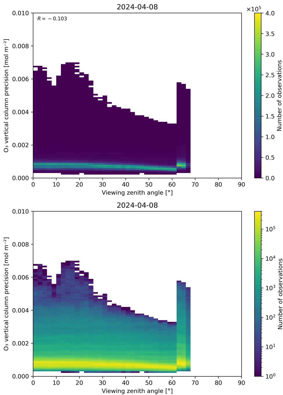
Figure 53: Scatter density plot of “Viewing zenith angle” against “O 3 vertical column precision” for 2024-04-07 to 2024-04-09.
