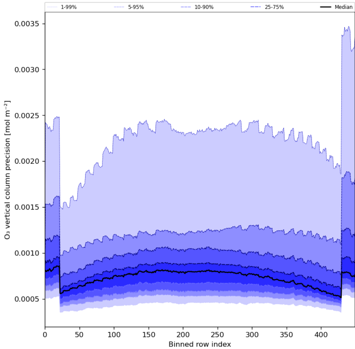
Figure 29: Along track statistics of “O 3 vertical column precision” for 2024-04-07 to 2024-04-09
