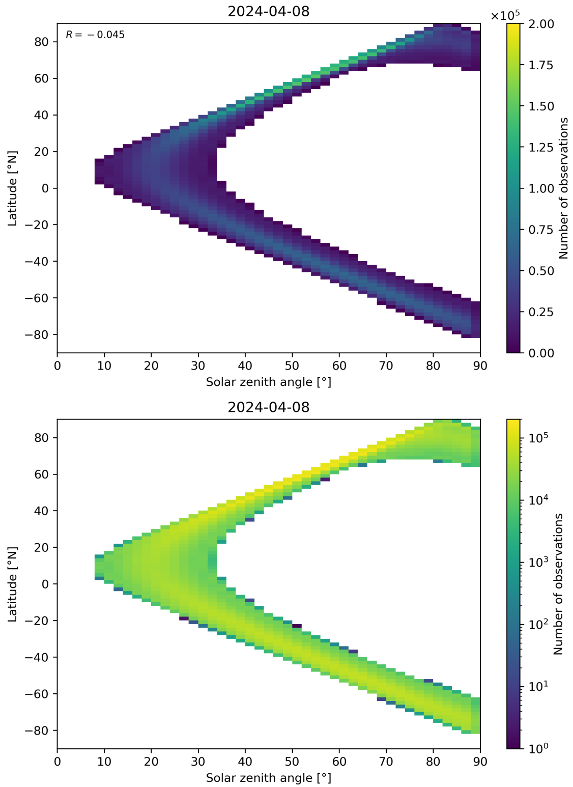
Figure 44: Scatter density plot of “Solar zenith angle” against “Latitude” for 2024-04-07 to 2024-04-09.
