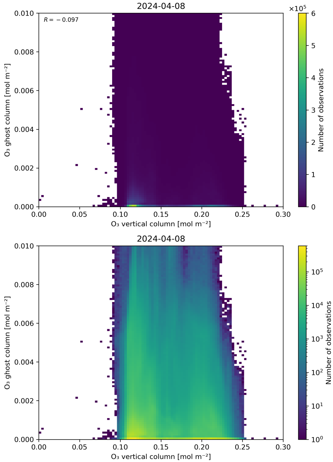
Figure 40: Scatter density plot of “O 3 vertical column” against “O 3 ghost column” for 2024-04-07 to 2024-04-09.
