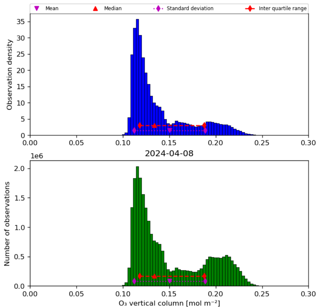
Figure 21: Histogram of “O 3 vertical column” for 2024-04-07 to 2024-04-09
