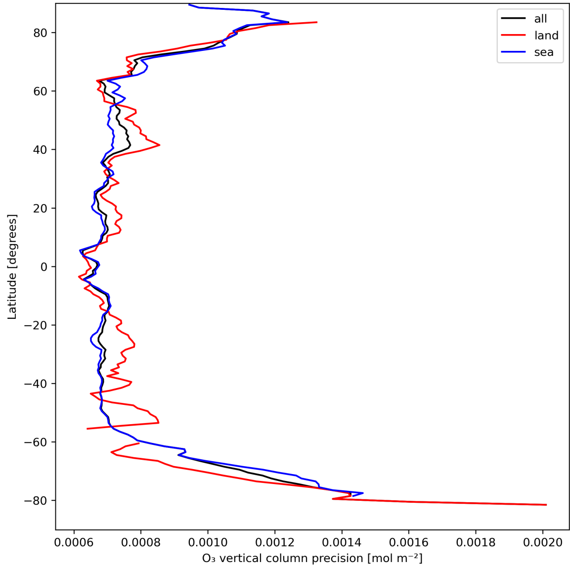
Figure 15: Zonal average of "O 3 vertical column precision" for 2024-04-08 to 2024-04-10.
