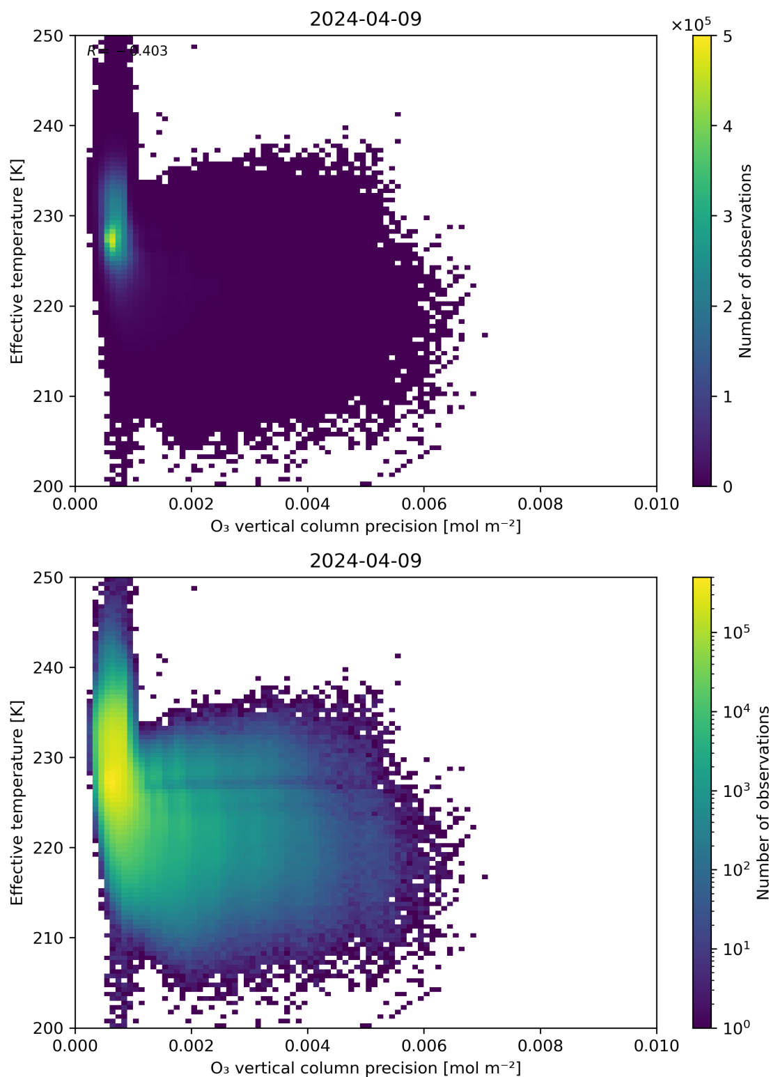
Figure 42: Scatter density plot of “O 3 vertical column precision” against “Effective temperature” for 2024-04-08 to 2024-04-10.
