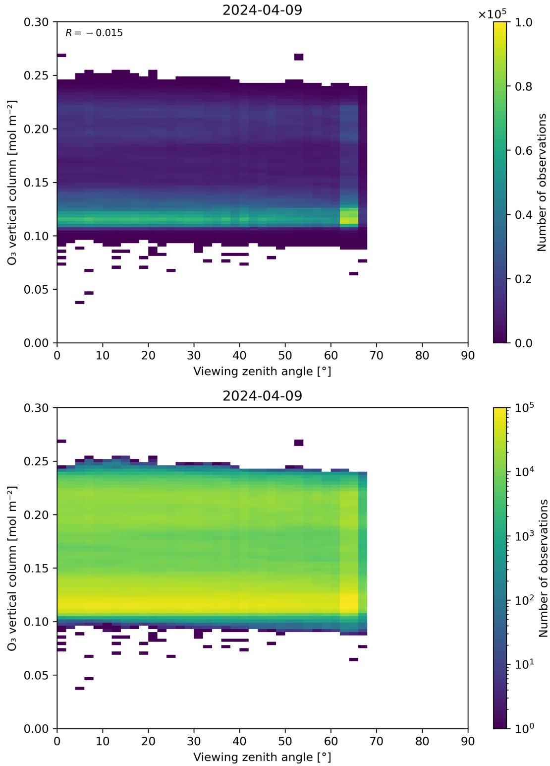
Figure 52: Scatter density plot of “Viewing zenith angle” against “O 3 vertical column” for 2024-04-08 to 2024-04-10.
