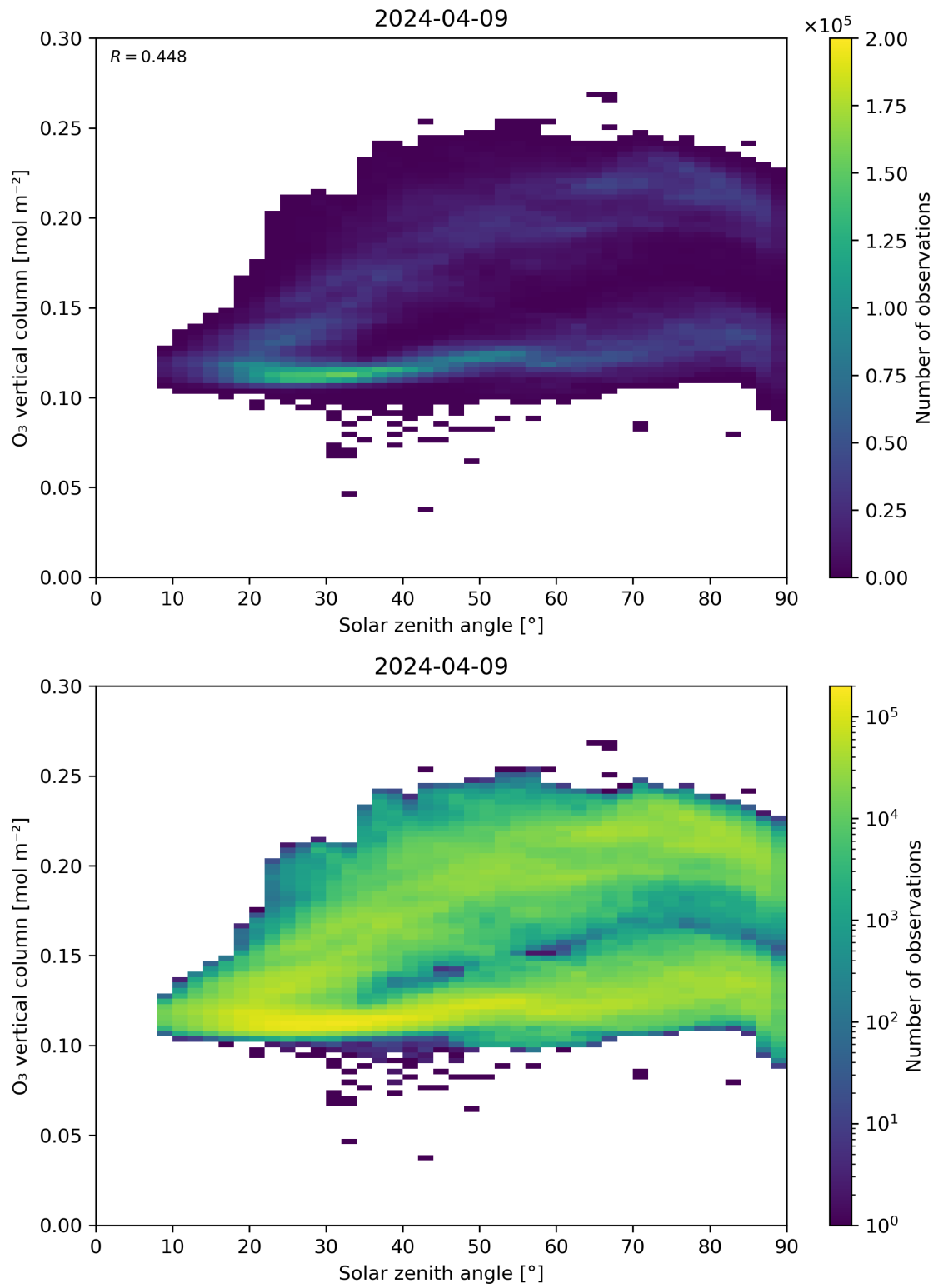
Figure 47: Scatter density plot of “Solar zenith angle” against “O 3 vertical column” for 2024-04-08 to 2024-04-10.
