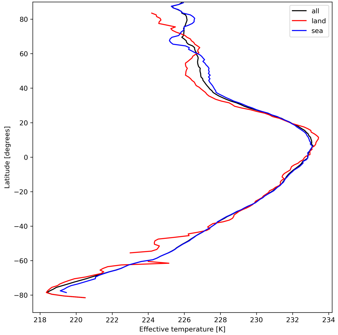
Figure 17: Zonal average of “Effective temperature” for 2024-04-08 to 2024-04-10.
