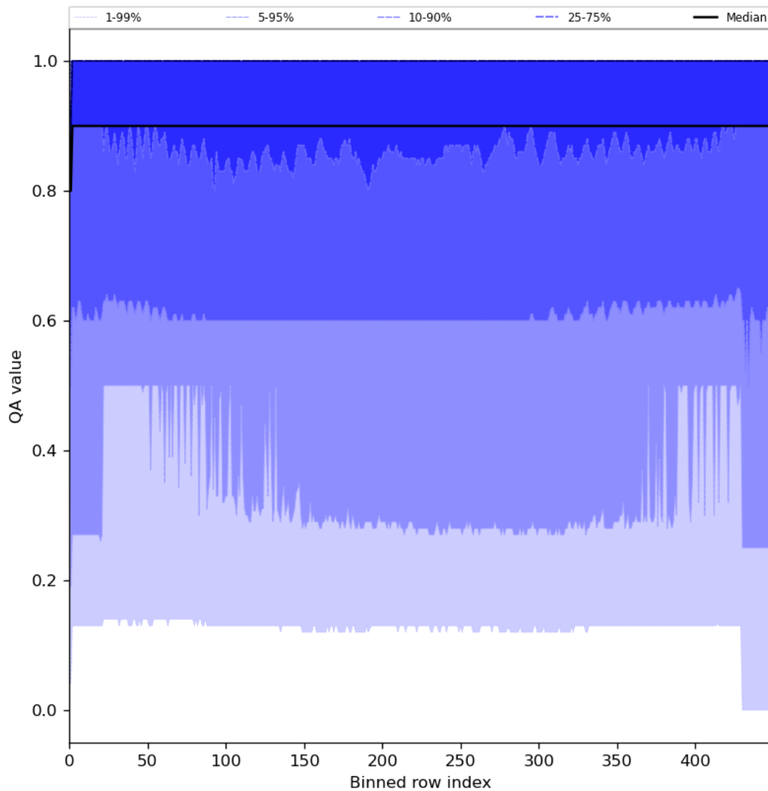
Figure 27: Along track statistics of “QA value” for 2024-04-08 to 2024-04-10
