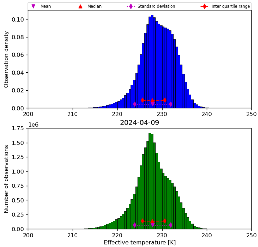
Figure 24: Histogram of “Effective temperature” for 2024-04-08 to 2024-04-10
