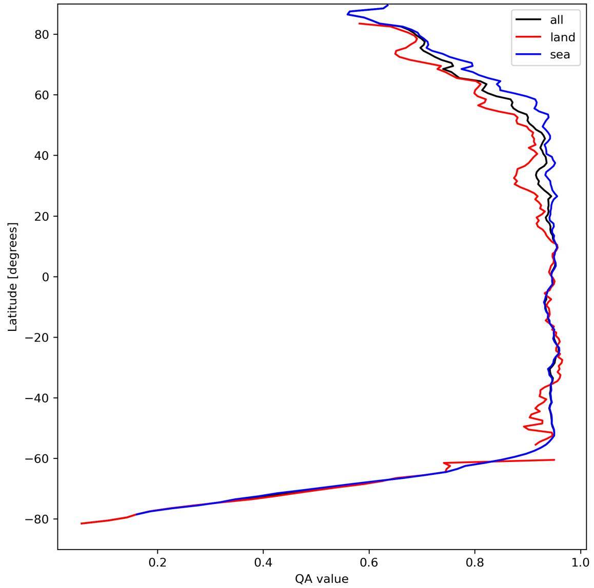
Figure 13: Zonal average of “QA value” for 2024-04-08 to 2024-04-10.
