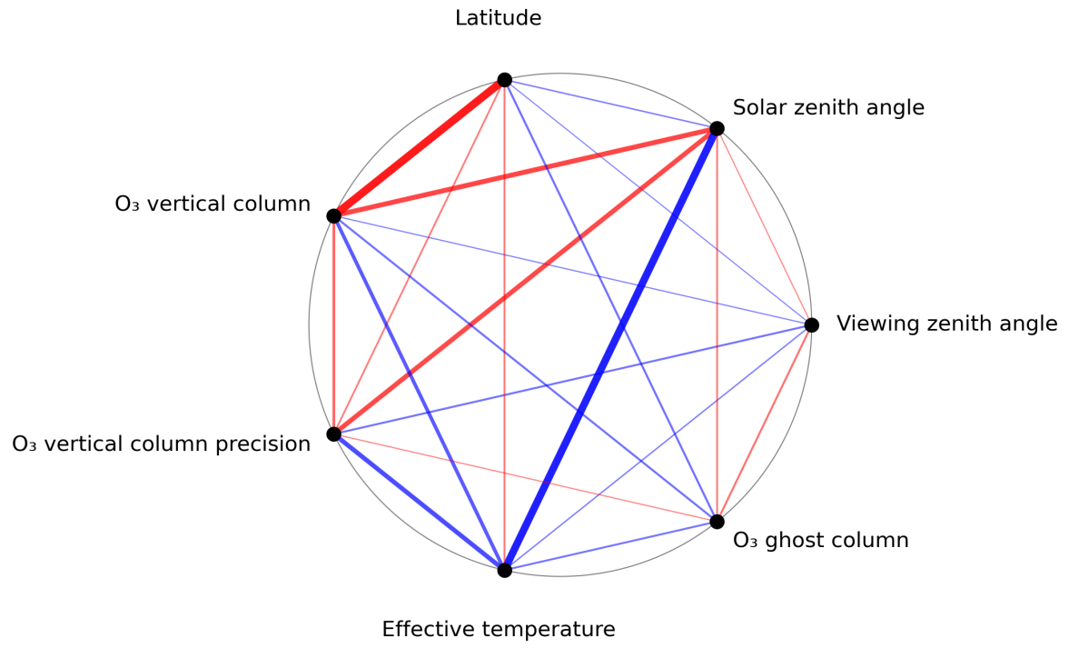
Figure 1: Map of correlation graph for 2024-04-08 to 2024-04-10.
