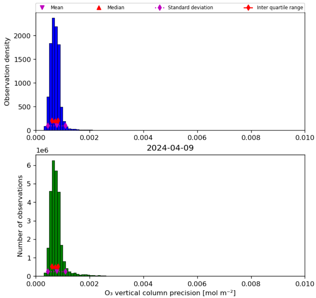
Figure 22: Histogram of “O 3 vertical column precision” for 2024-04-08 to 2024-04-10
