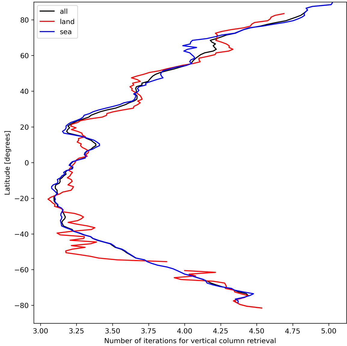
Figure 19: Zonal average of “Number of iterations for vertical column retrieval” for 2024-04-08 to 2024-04-10.
