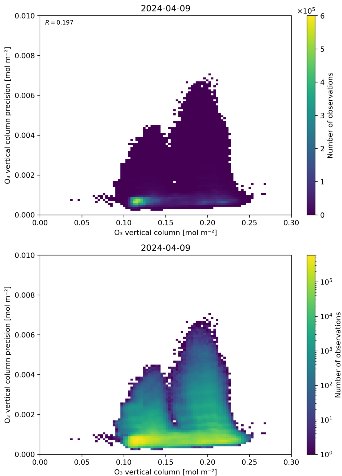
Figure 41: Scatter density plot of “O 3 vertical column” against “O 3 vertical column precision” for 2024-04-08 to 2024-04-10.
