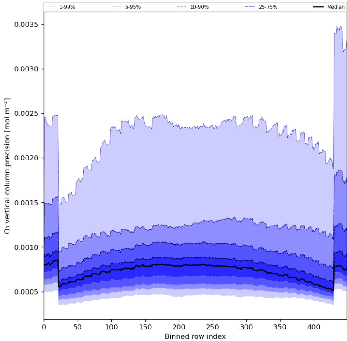
Figure 29: Along track statistics of “O 3 vertical column precision” for 2024-04-08 to 2024-04-10
