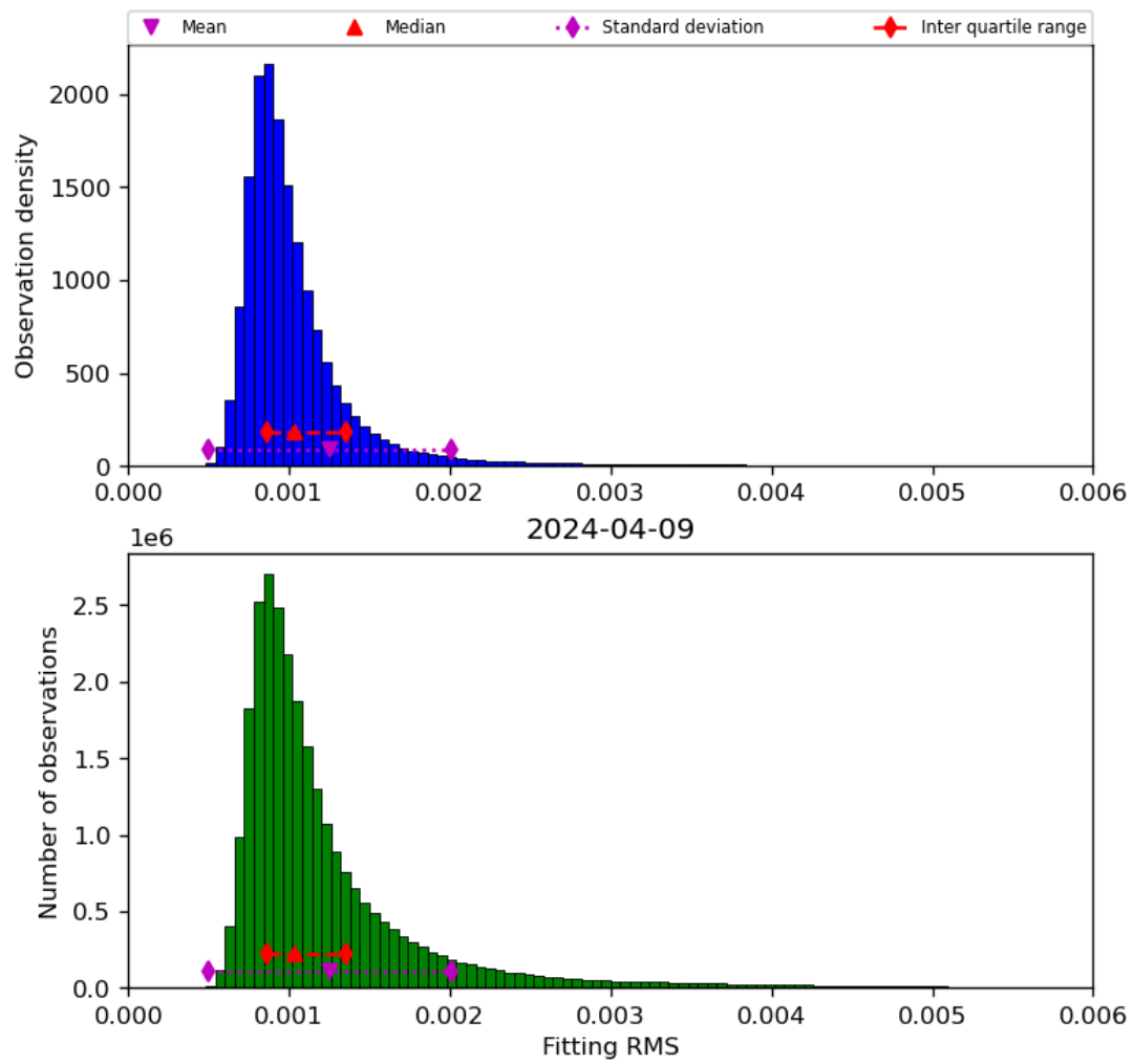
Figure 23: Histogram of “Fitting RMS” for 2024-04-08 to 2024-04-10
