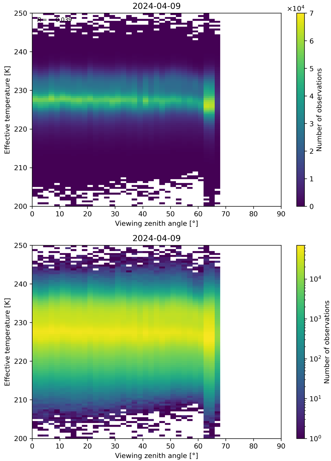
Figure 50: Scatter density plot of “Viewing zenith angle” against “Effective temperature” for 2024-04-08 to 2024-04-10.
