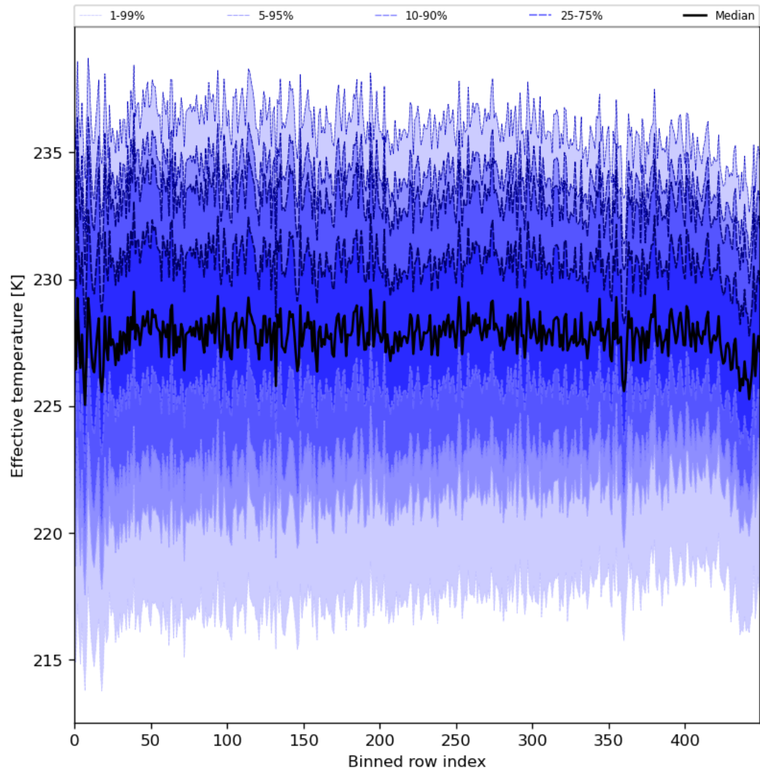
Figure 31: Along track statistics of “Effective temperature” for 2024-04-08 to 2024-04-10
