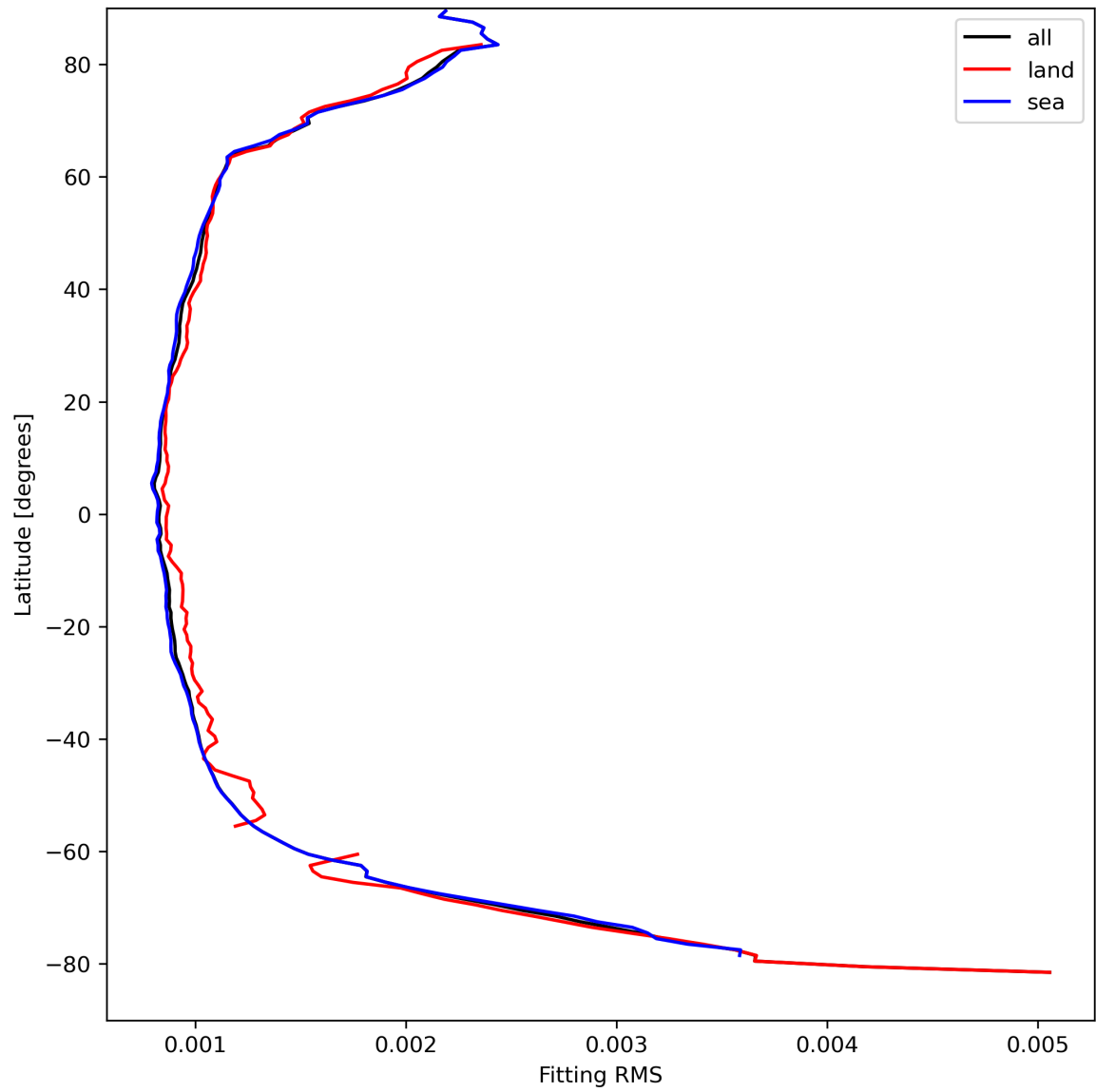
Figure 16: Zonal average of “Fitting RMS” for 2024-04-08 to 2024-04-10.
