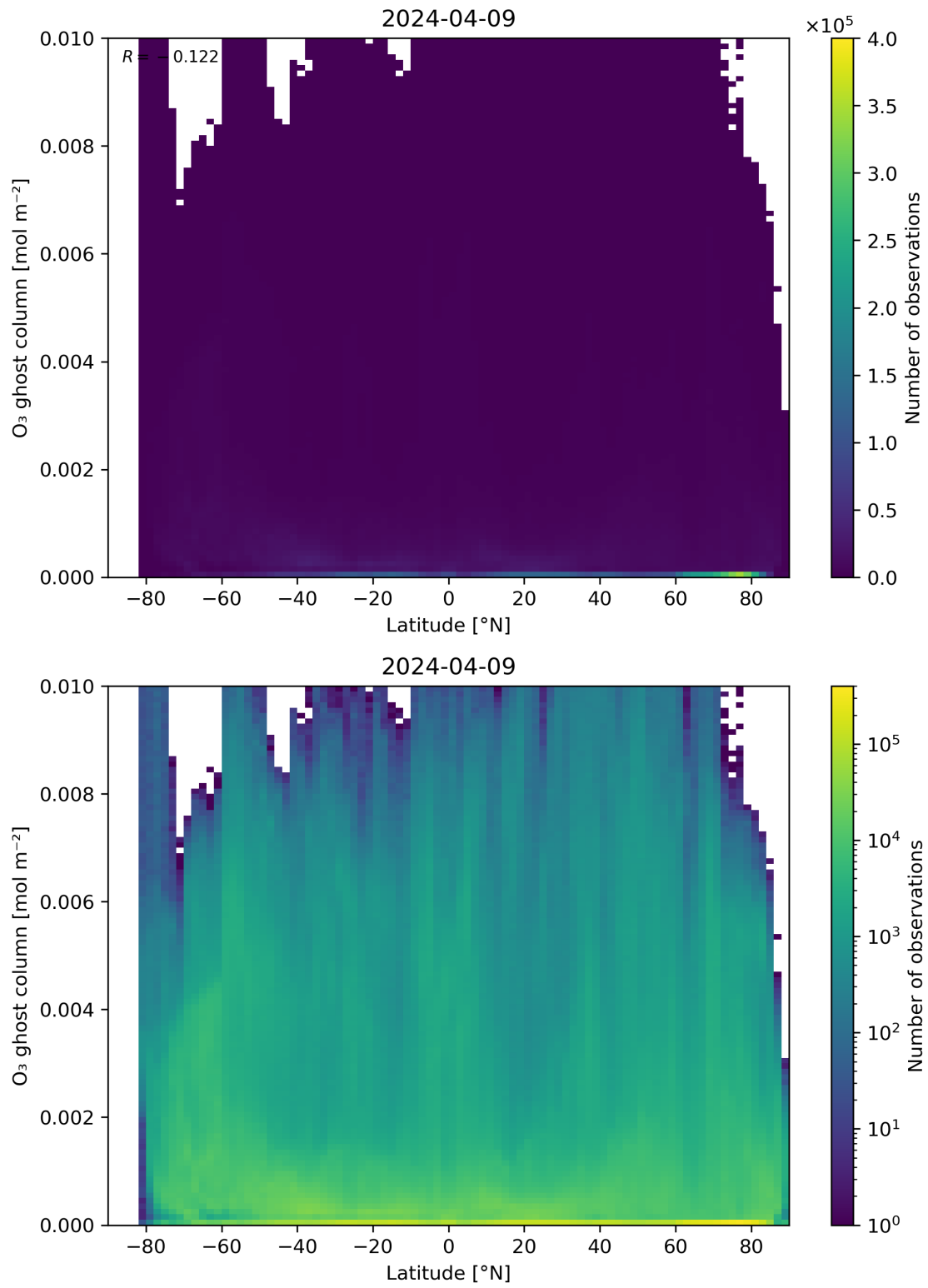
Figure 35: Scatter density plot of “Latitude” against “O 3 ghost column” for 2024-04-08 to 2024-04-10.
