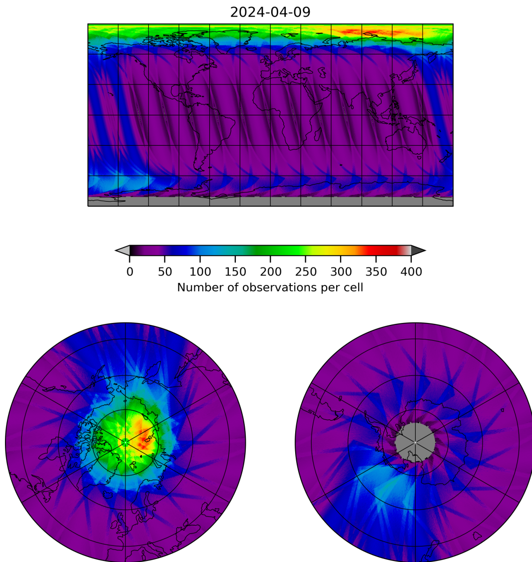
Figure 12: Map of the number of observations for 2024-04-08 to 2024-04-10
