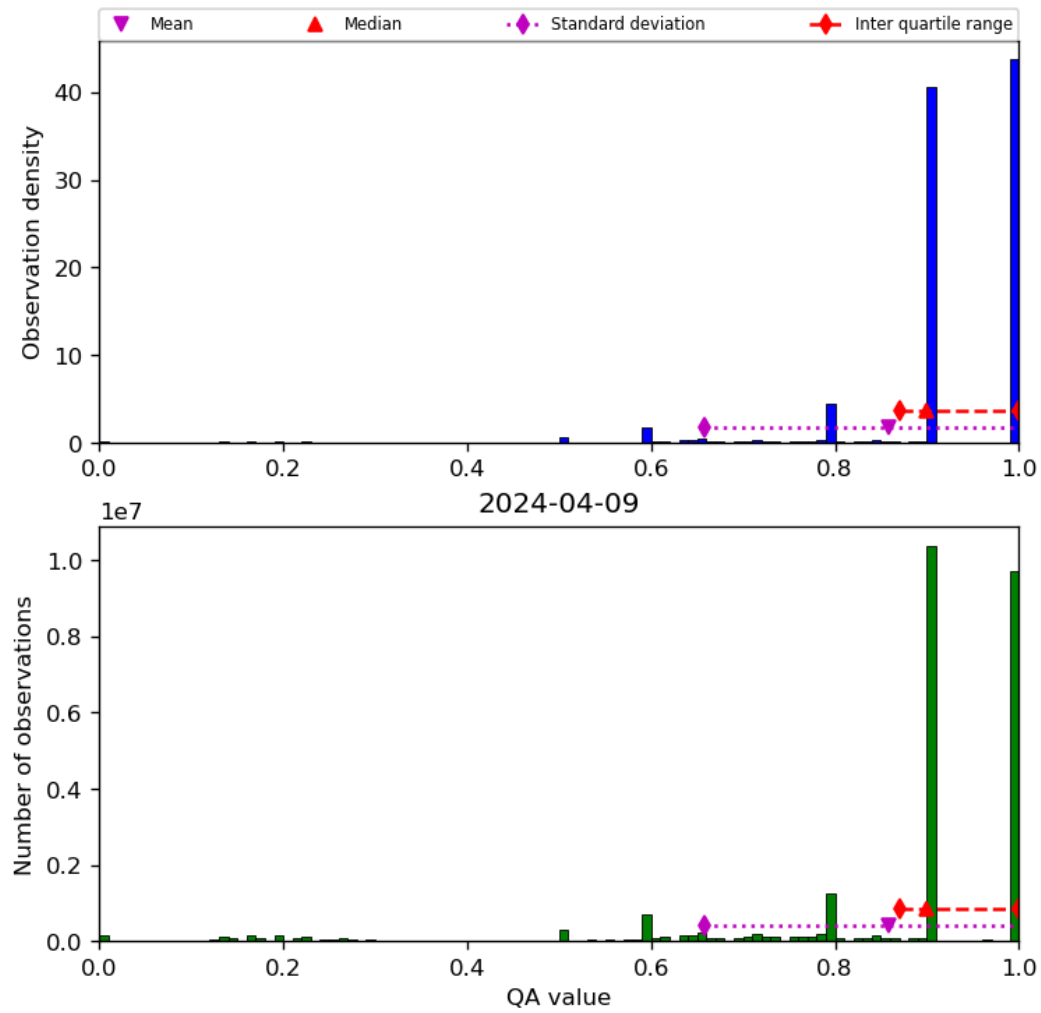
Figure 20: Histogram of “QA value” for 2024-04-08 to 2024-04-10
