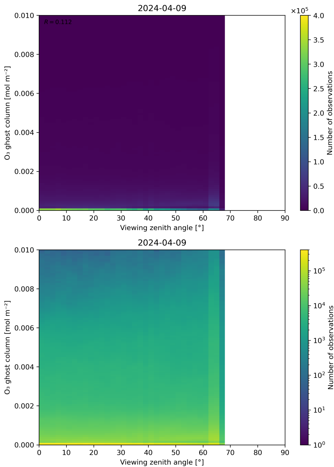
Figure 51: Scatter density plot of “Viewing zenith angle” against “O 3 ghost column” for 2024-04-08 to 2024-04-10.
