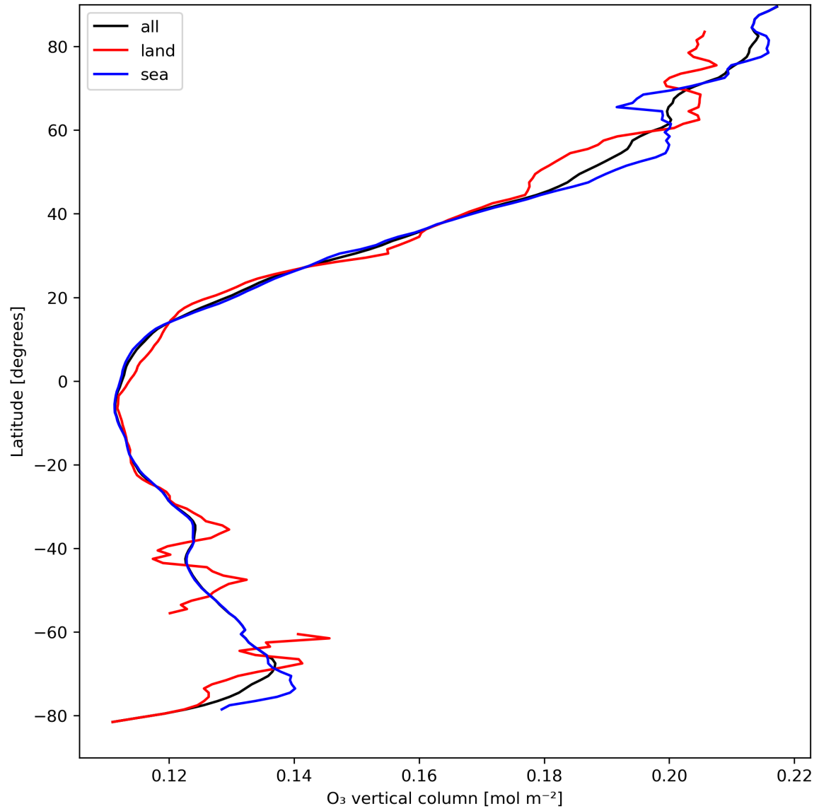
Figure 14: Zonal average of “O 3 vertical column” for 2024-04-08 to 2024-04-10.
