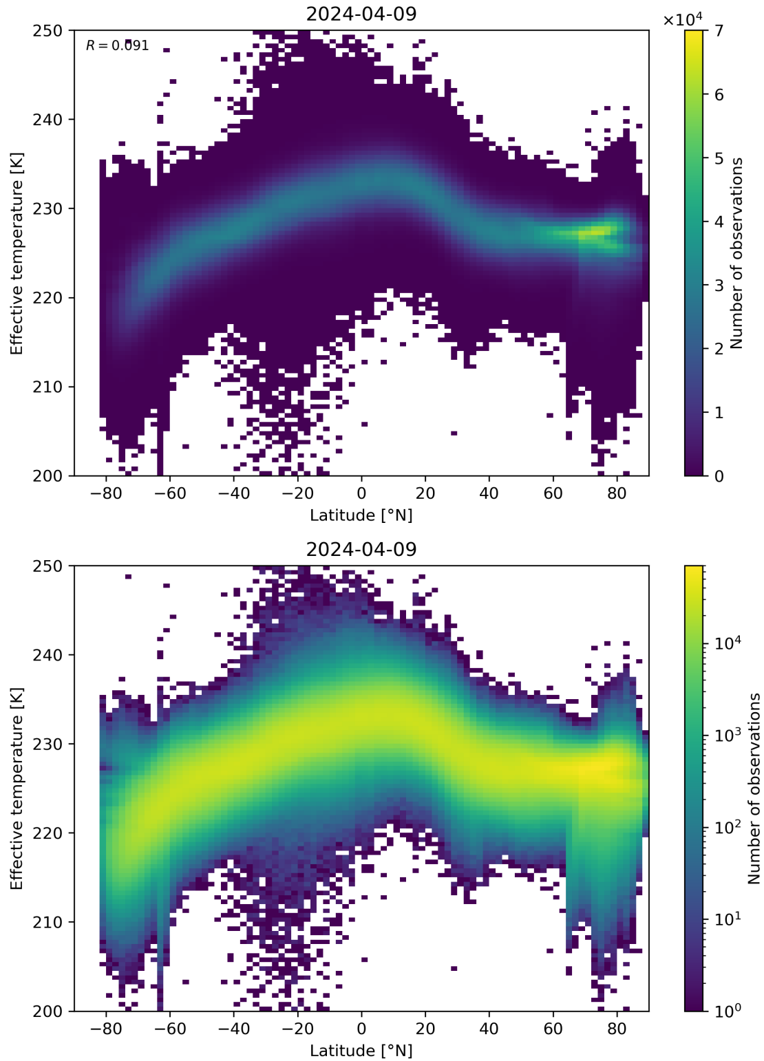
Figure 34: Scatter density plot of “Latitude” against “Effective temperature” for 2024-04-08 to 2024-04-10.
