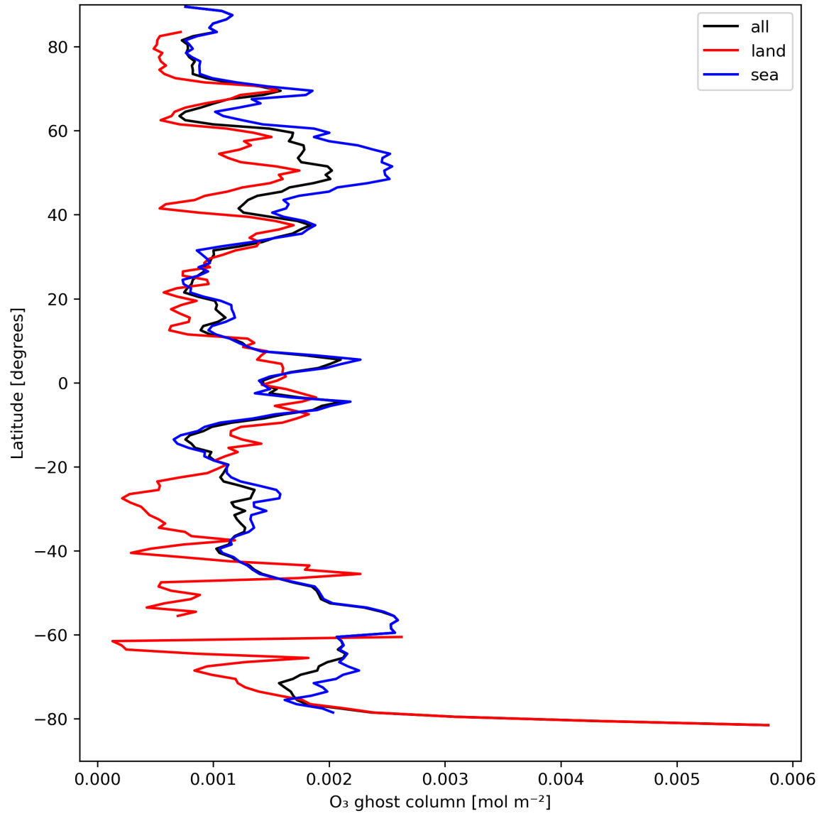
Figure 18: Zonal average of "O 3 ghost column" for 2024-04-08 to 2024-04-10.
