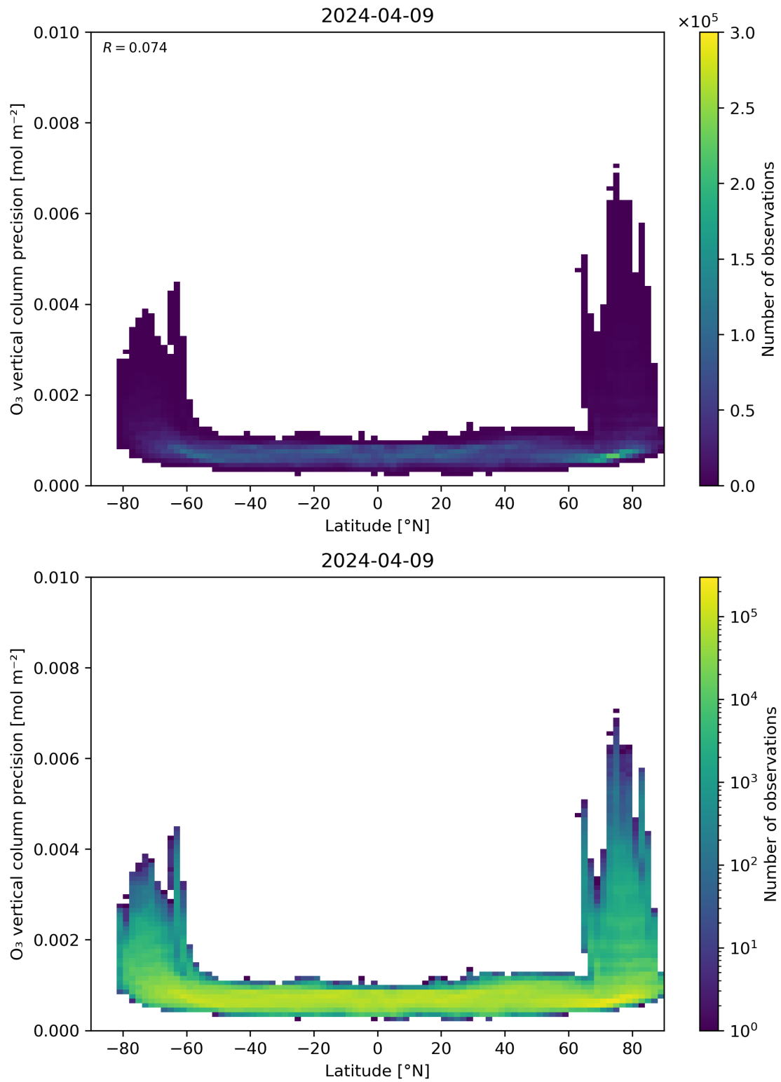
Figure 37: Scatter density plot of “Latitude” against “O 3 vertical column precision” for 2024-04-08 to 2024-04-10.
