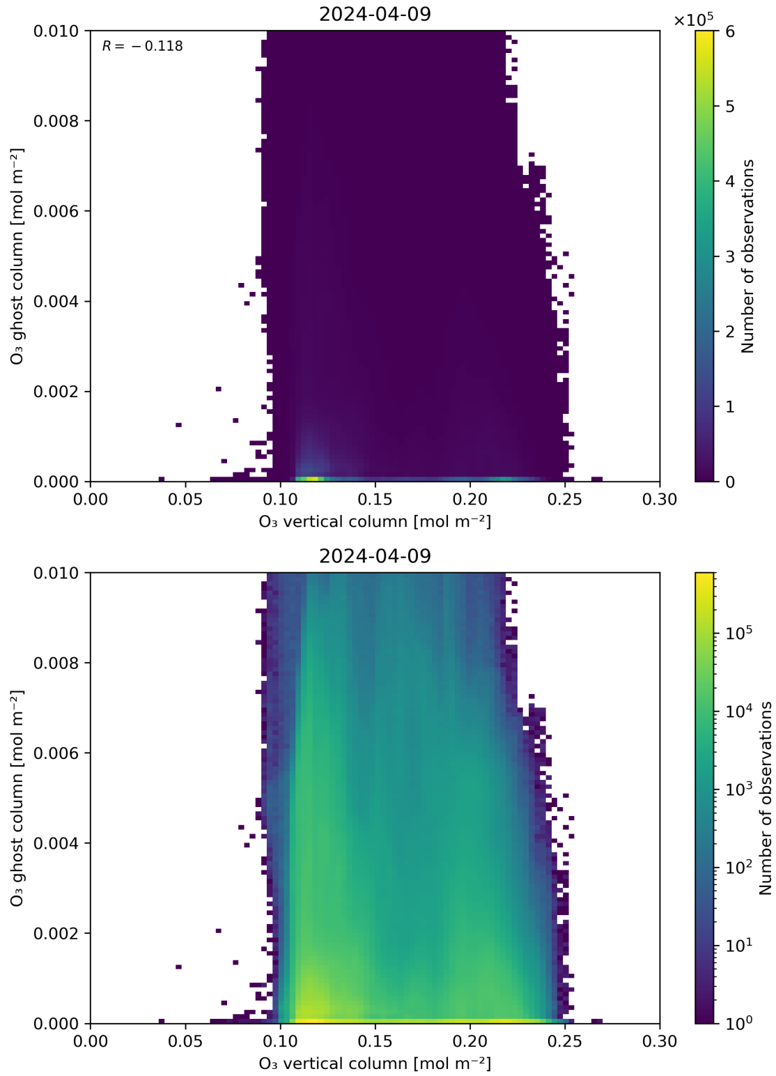
Figure 40: Scatter density plot of “O 3 vertical column” against “O 3 ghost column” for 2024-04-08 to 2024-04-10.
