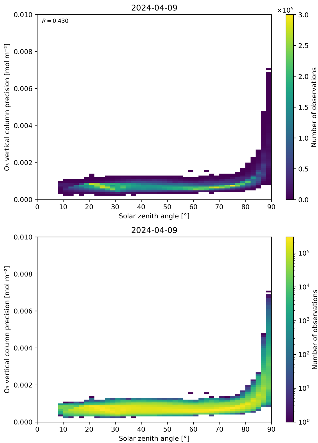
Figure 48: Scatter density plot of “Solar zenith angle” against “O 3 vertical column precision” for 2024-04-08 to 2024-04-10.
