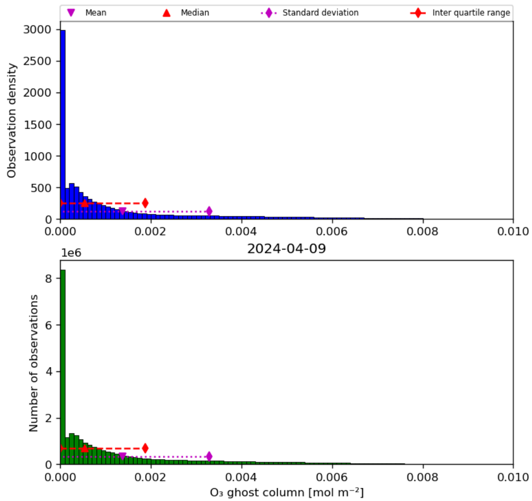
Figure 25: Histogram of “O 3 ghost column” for 2024-04-08 to 2024-04-10
