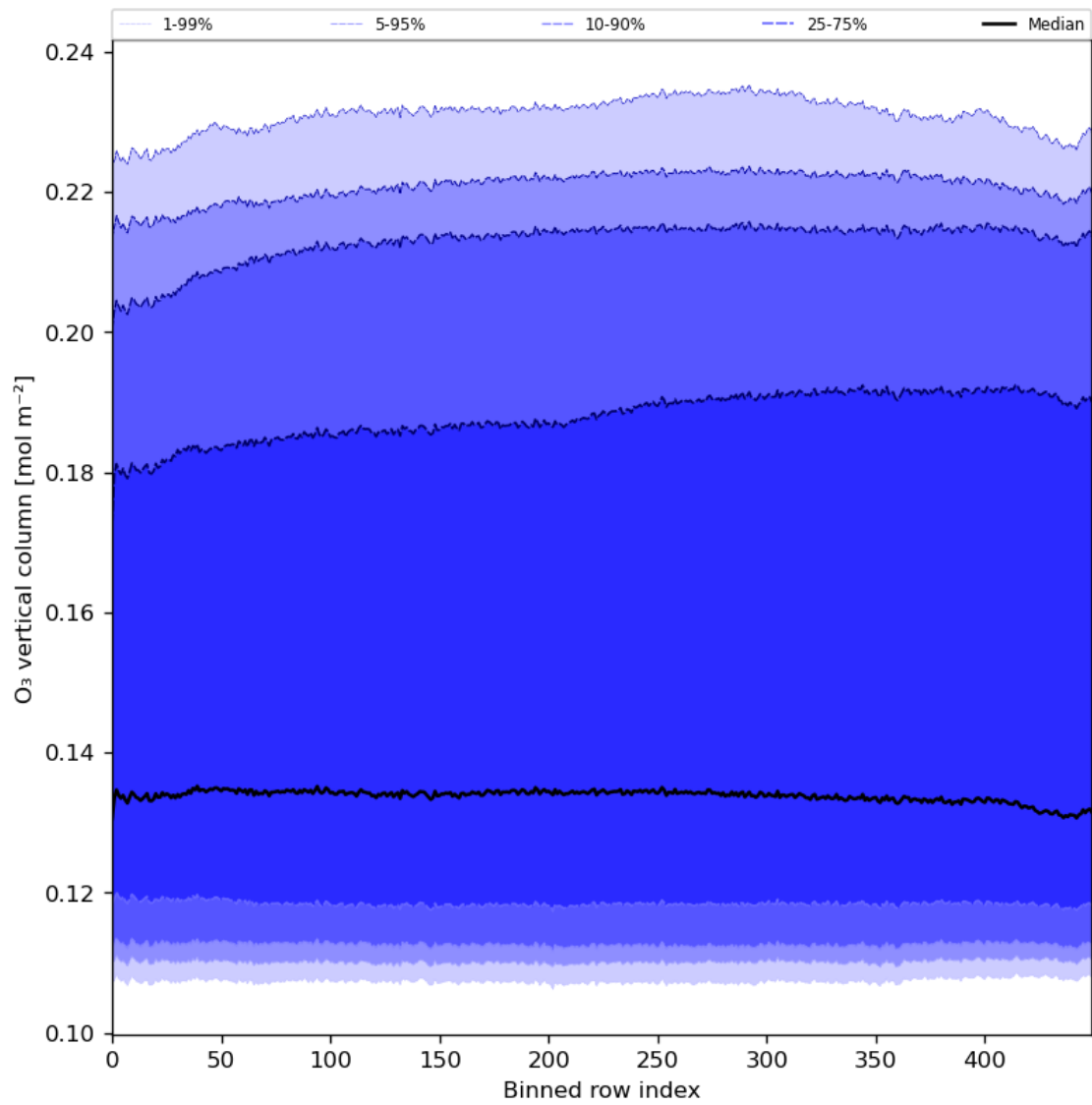
Figure 28: Along track statistics of “O 3 vertical column” for 2024-04-08 to 2024-04-10
