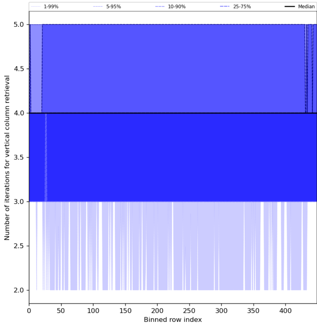
Figure 33: Along track statistics of “Number of iterations for vertical column retrieval” for 2024-04-08 to 2024-04-10
