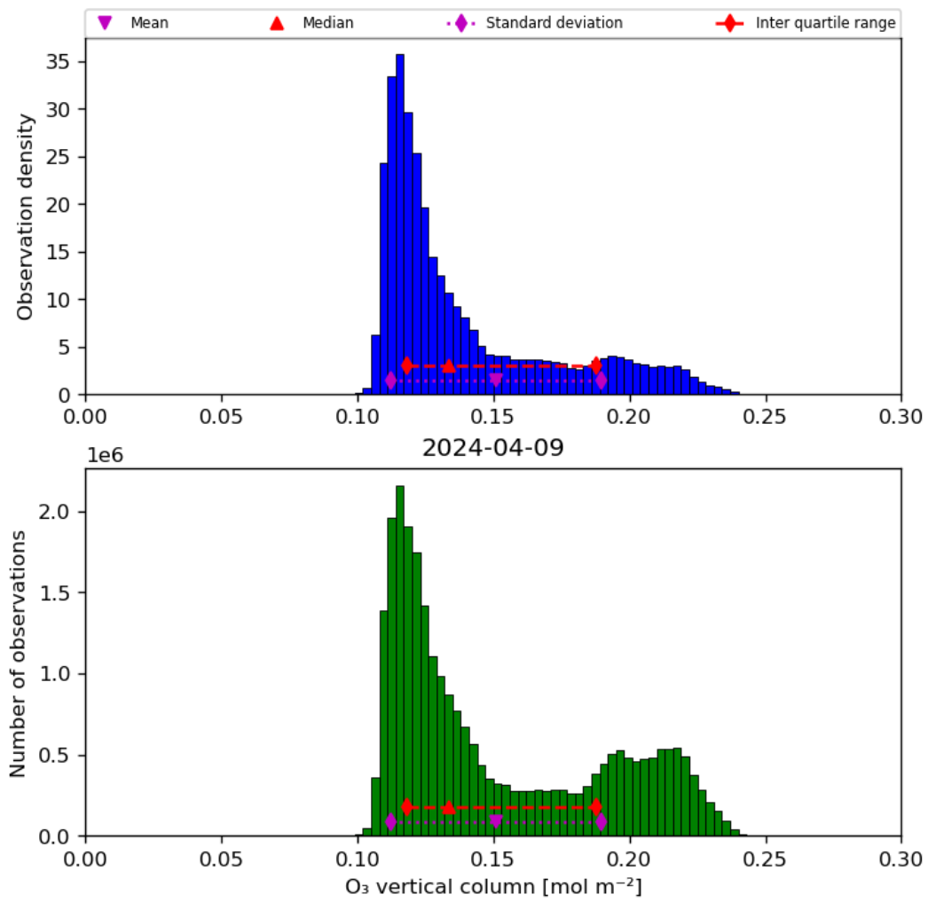
Figure 21: Histogram of “O 3 vertical column” for 2024-04-08 to 2024-04-10
