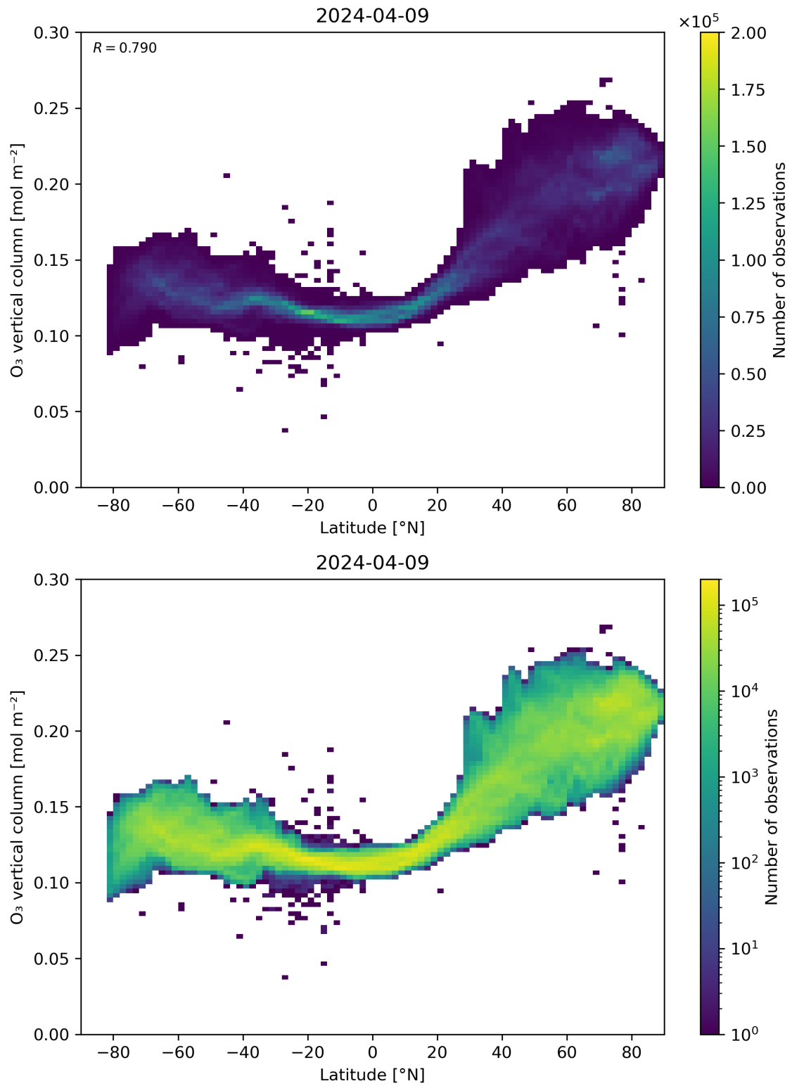
Figure 36: Scatter density plot of “Latitude” against “O 3 vertical column” for 2024-04-08 to 2024-04-10.
