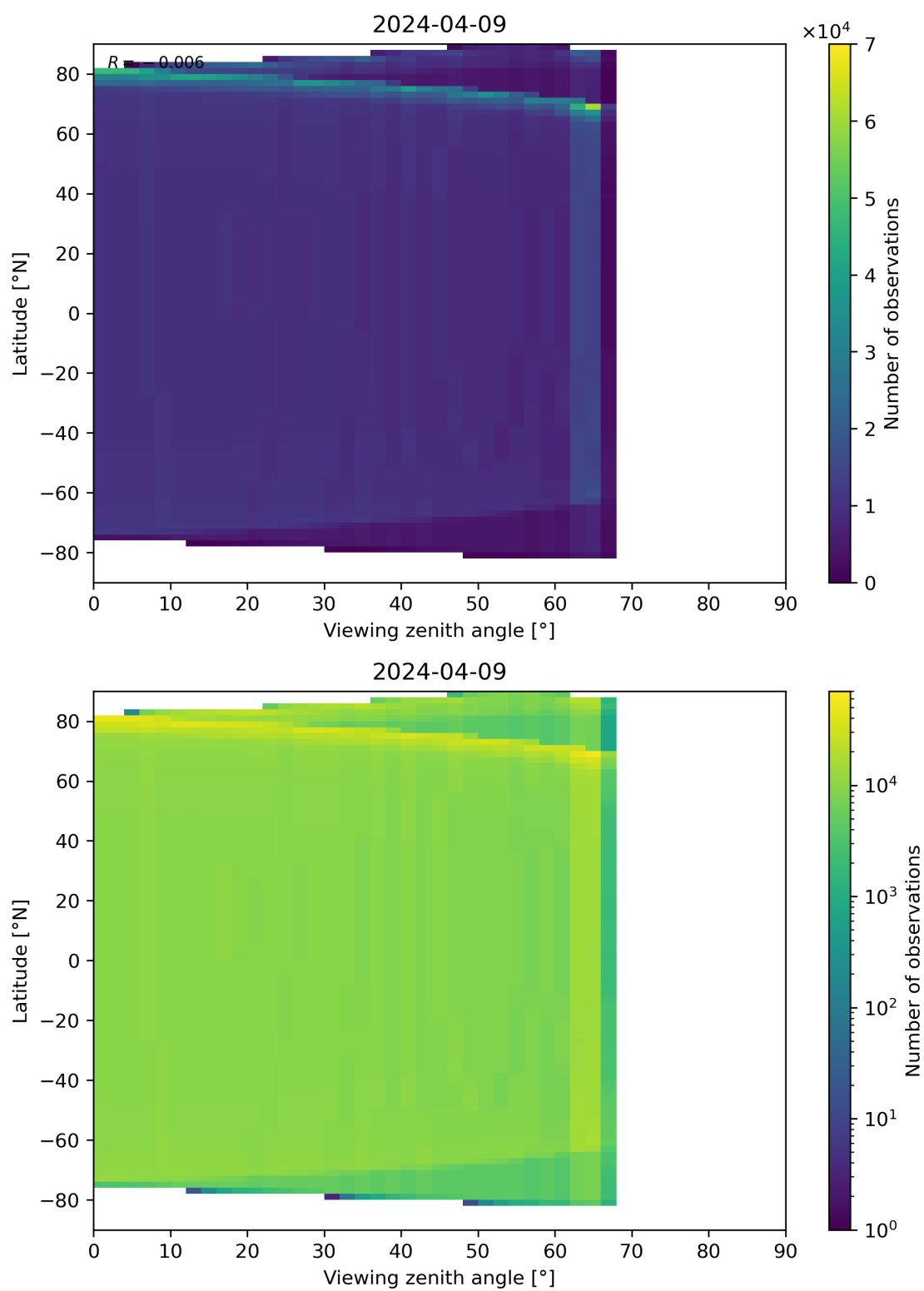
Figure 49: Scatter density plot of “Viewing zenith angle” against “Latitude” for 2024-04-08 to 2024-04-10.
