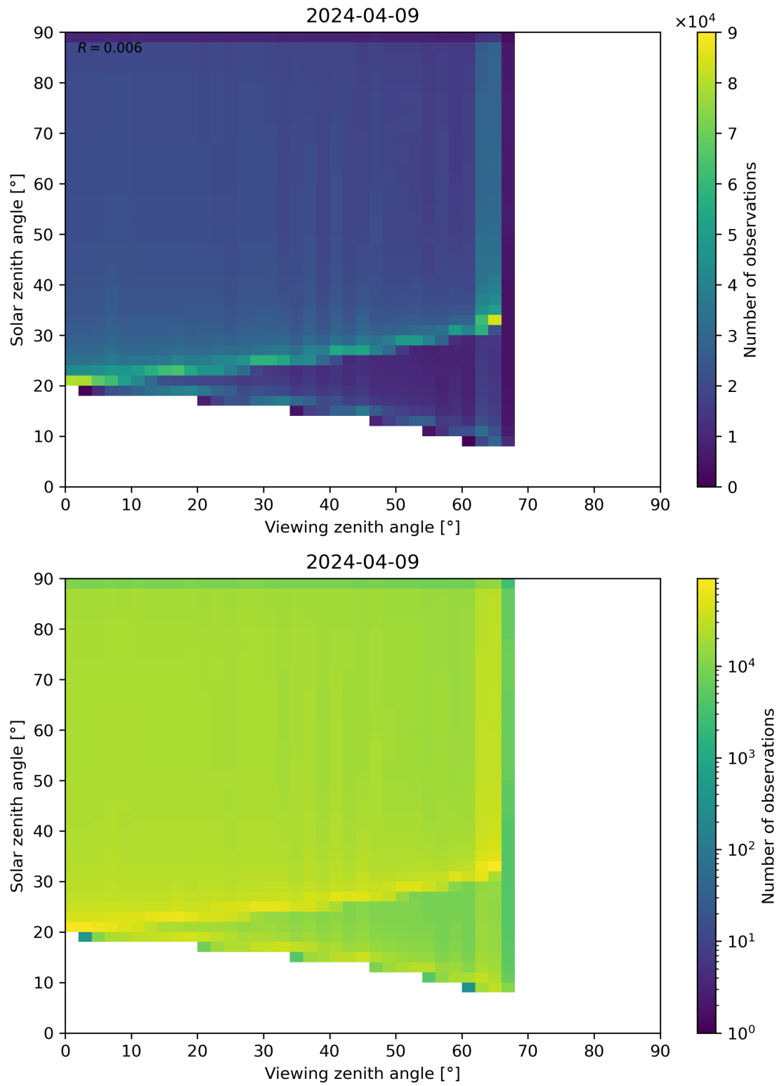
Figure 54: Scatter density plot of “Viewing zenith angle” against “Solar zenith angle” for 2024-04-08 to 2024-04-10.
