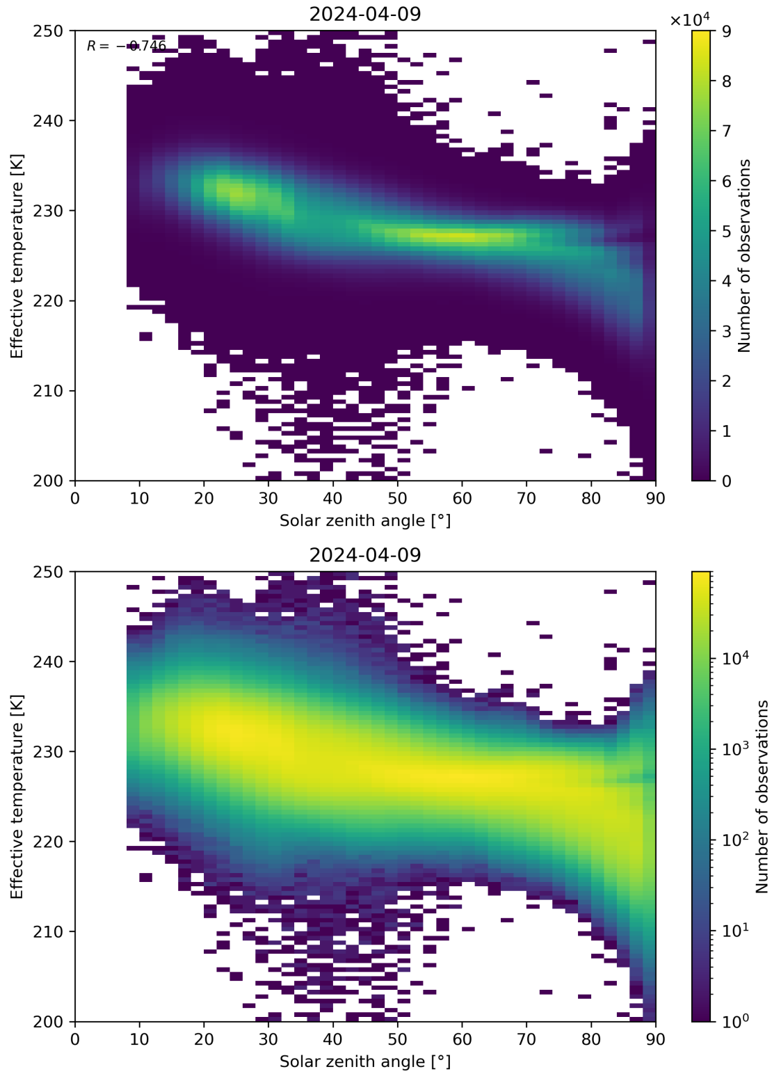
Figure 45: Scatter density plot of “Solar zenith angle” against “Effective temperature” for 2024-04-08 to 2024-04-10.
