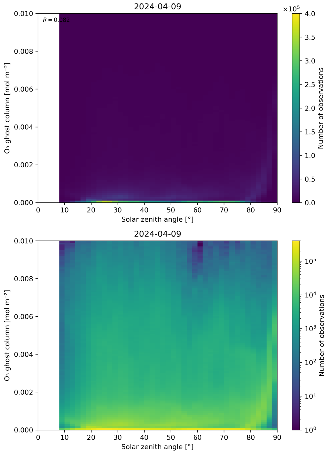
Figure 46: Scatter density plot of “Solar zenith angle” against “O 3 ghost column” for 2024-04-08 to 2024-04-10.
