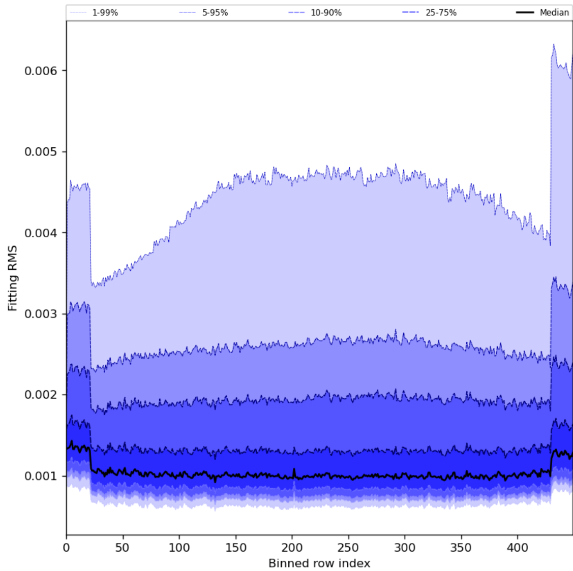
Figure 30: Along track statistics of “Fitting RMS” for 2024-04-08 to 2024-04-10
