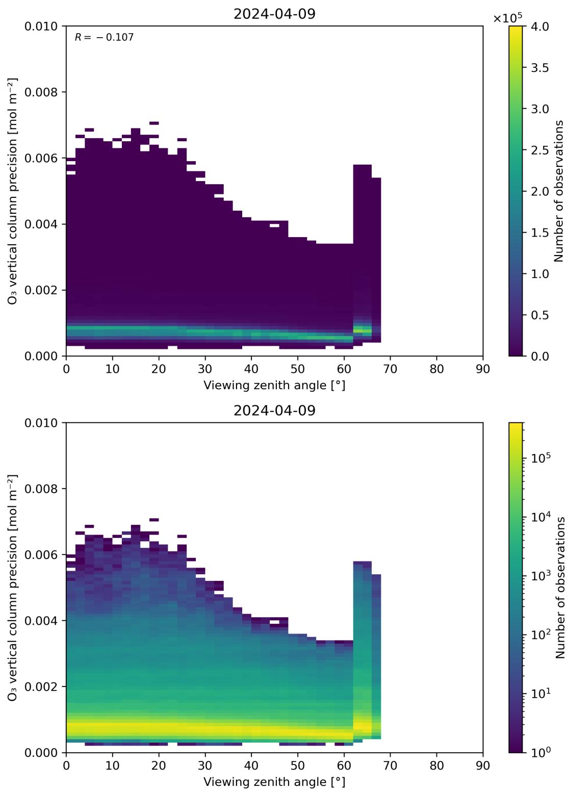
Figure 53: Scatter density plot of “Viewing zenith angle” against “O 3 vertical column precision” for 2024-04-08 to 2024-04-10.
