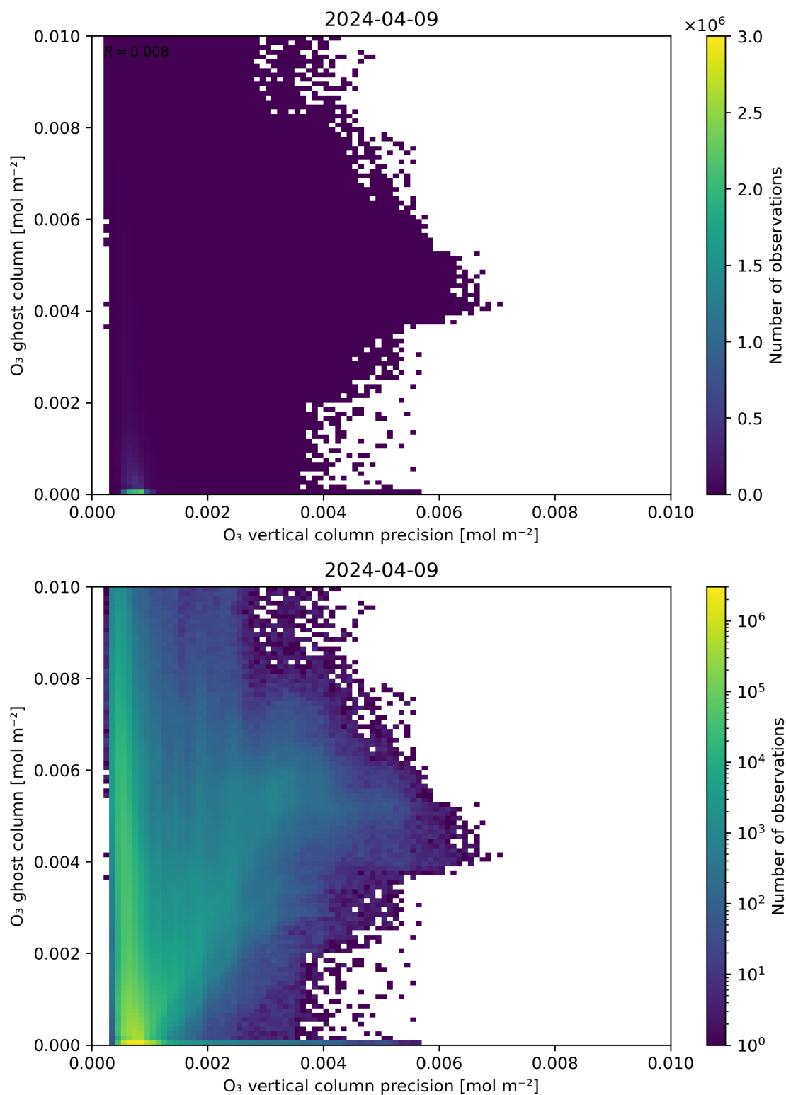
Figure 43: Scatter density plot of “ \text{O}_3 vertical column precision” against “ \text{O}_3 ghost column” for 2024-04-08 to 2024-04-10.
