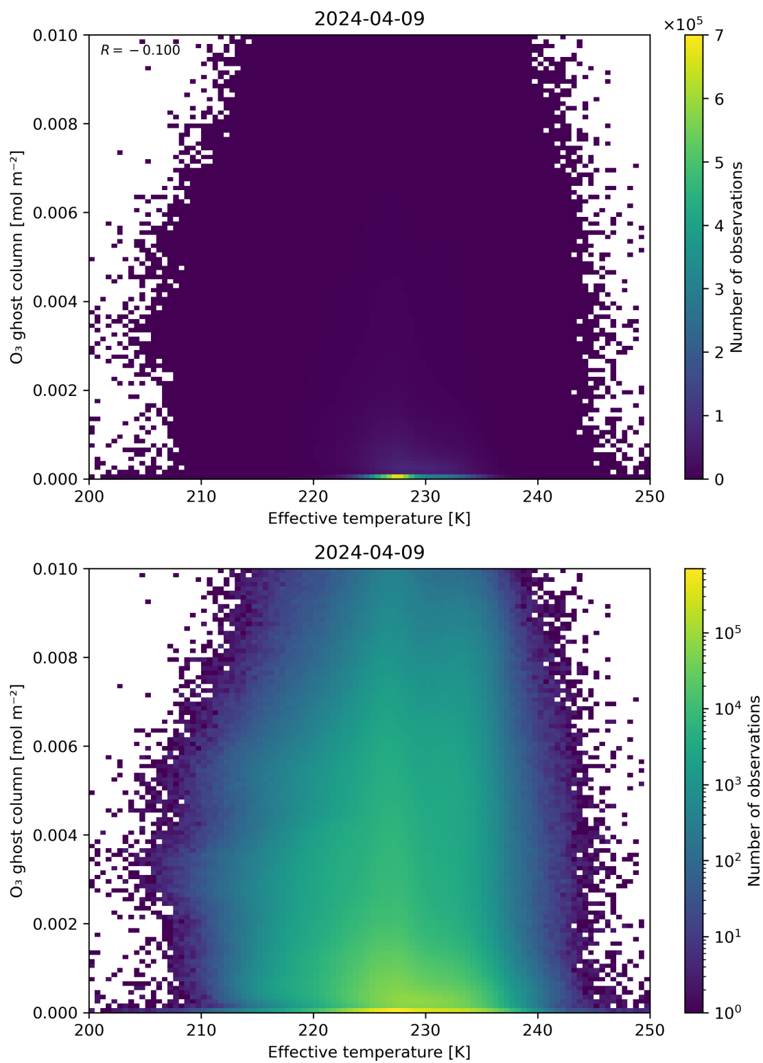
Figure 38: Scatter density plot of “Effective temperature” against “O 3 ghost column” for 2024-04-08 to 2024-04-10.
