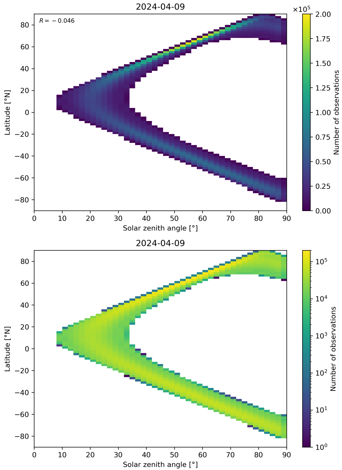
Figure 44: Scatter density plot of “Solar zenith angle” against “Latitude” for 2024-04-08 to 2024-04-10.
