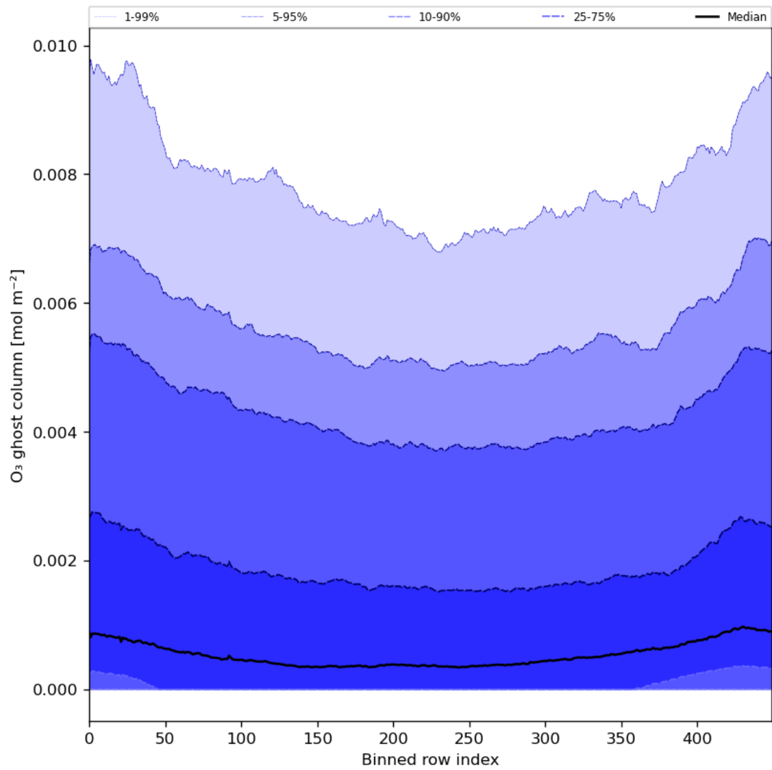
Figure 32: Along track statistics of “O 3 ghost column” for 2024-04-08 to 2024-04-10
