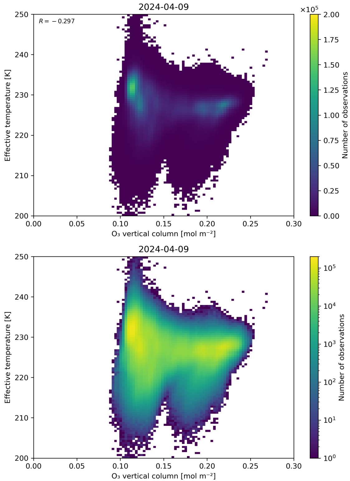
Figure 39: Scatter density plot of “O 3 vertical column” against “Effective temperature” for 2024-04-08 to 2024-04-10.
