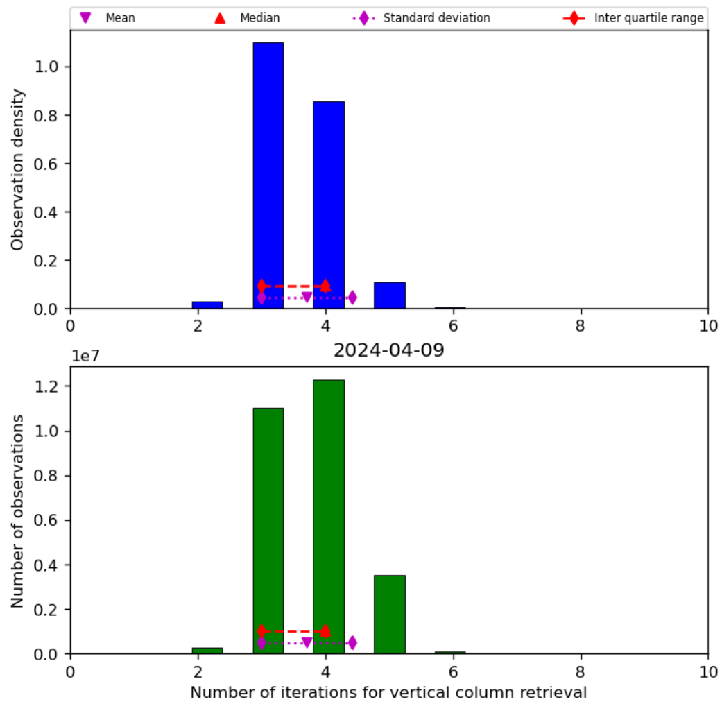
Figure 26: Histogram of “Number of iterations for vertical column retrieval” for 2024-04-08 to 2024-04-10
