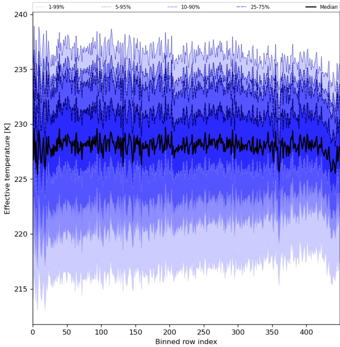
Figure 31: Along track statistics of “Effective temperature” for 2024-04-10 to 2024-04-12
