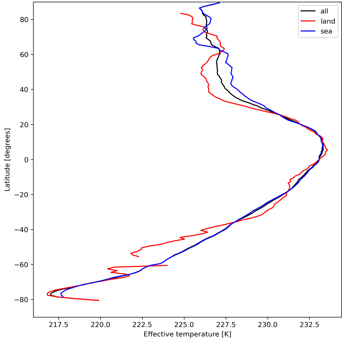
Figure 17: Zonal average of “Effective temperature” for 2024-04-10 to 2024-04-12.
