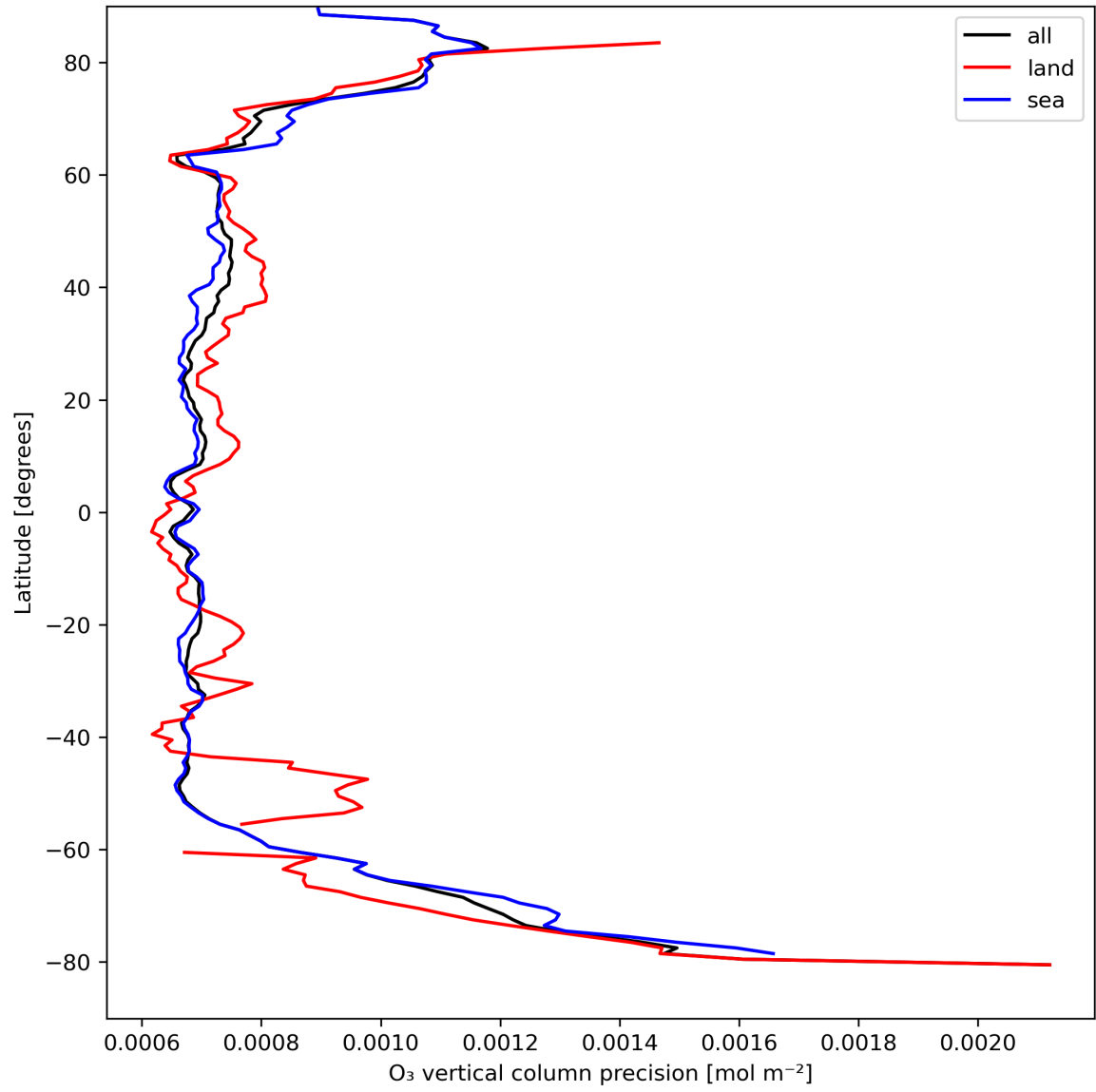
Figure 15: Zonal average of "O 3 vertical column precision" for 2024-04-10 to 2024-04-12.
