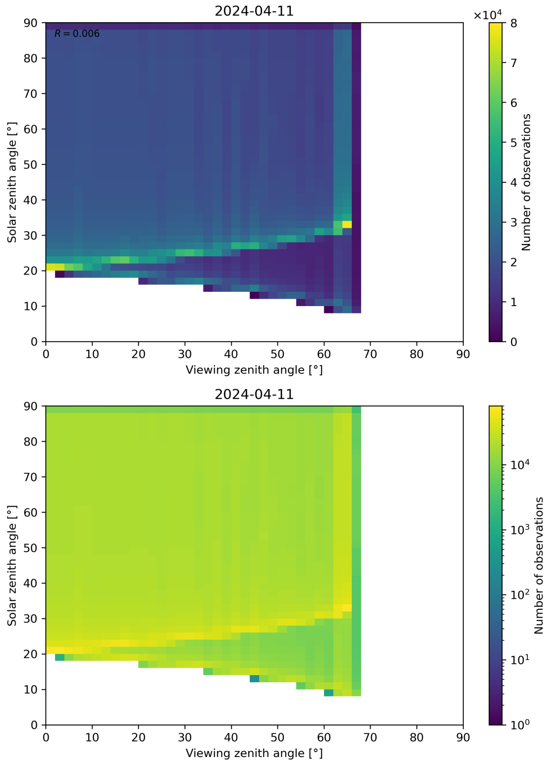
Figure 54: Scatter density plot of “Viewing zenith angle” against “Solar zenith angle” for 2024-04-10 to 2024-04-12.
