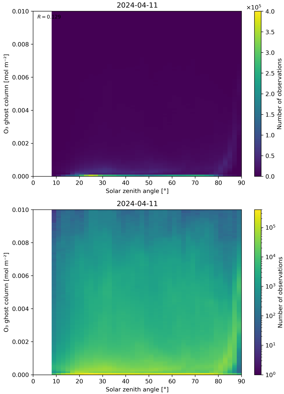
Figure 46: Scatter density plot of “Solar zenith angle” against “O 3 ghost column” for 2024-04-10 to 2024-04-12.
