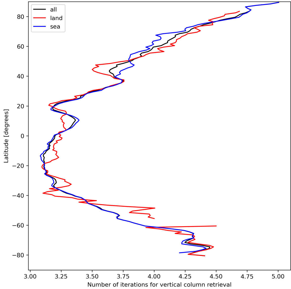
Figure 19: Zonal average of “Number of iterations for vertical column retrieval” for 2024-04-10 to 2024-04-12.
