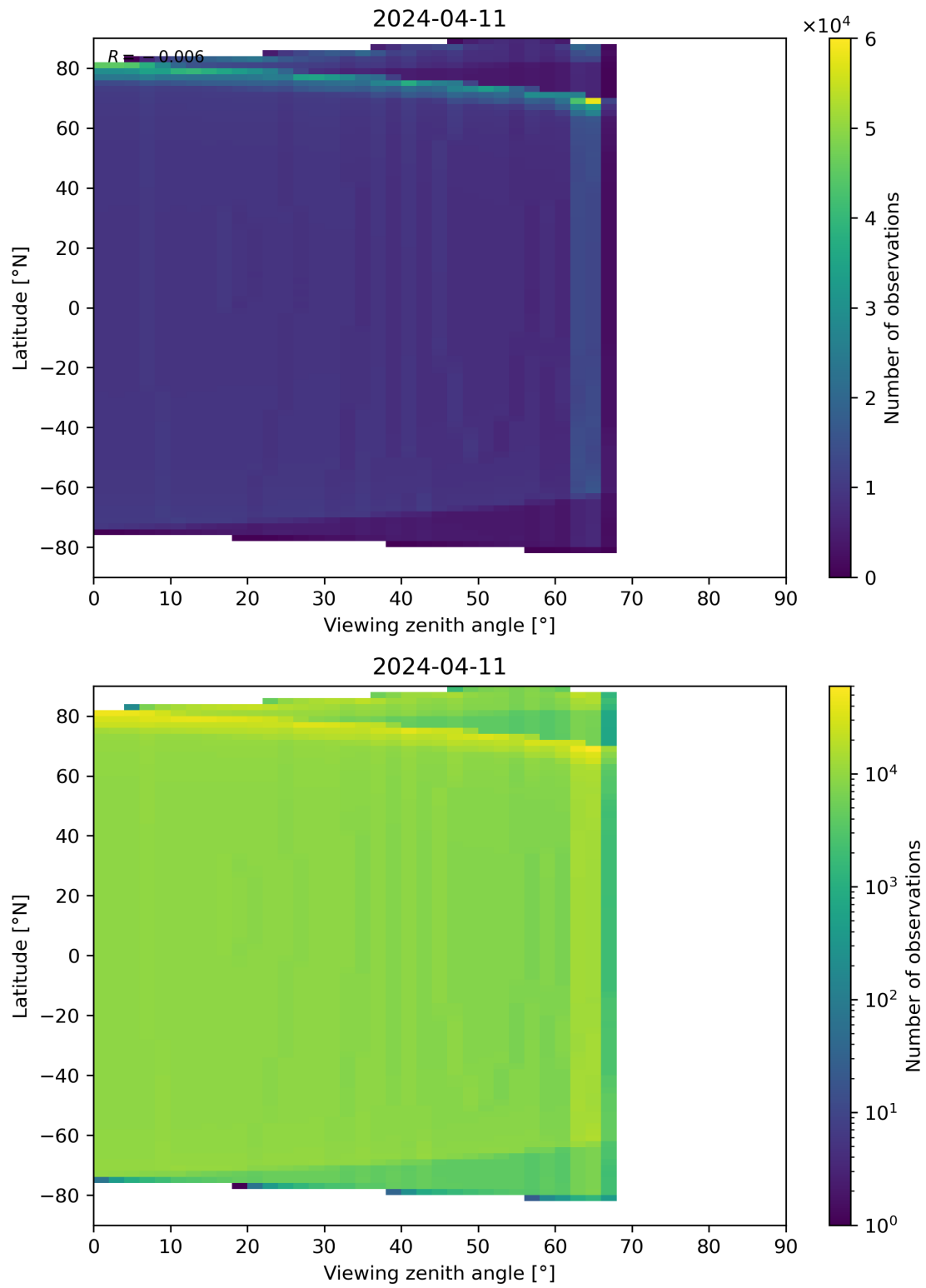
Figure 49: Scatter density plot of “Viewing zenith angle” against “Latitude” for 2024-04-10 to 2024-04-12.
