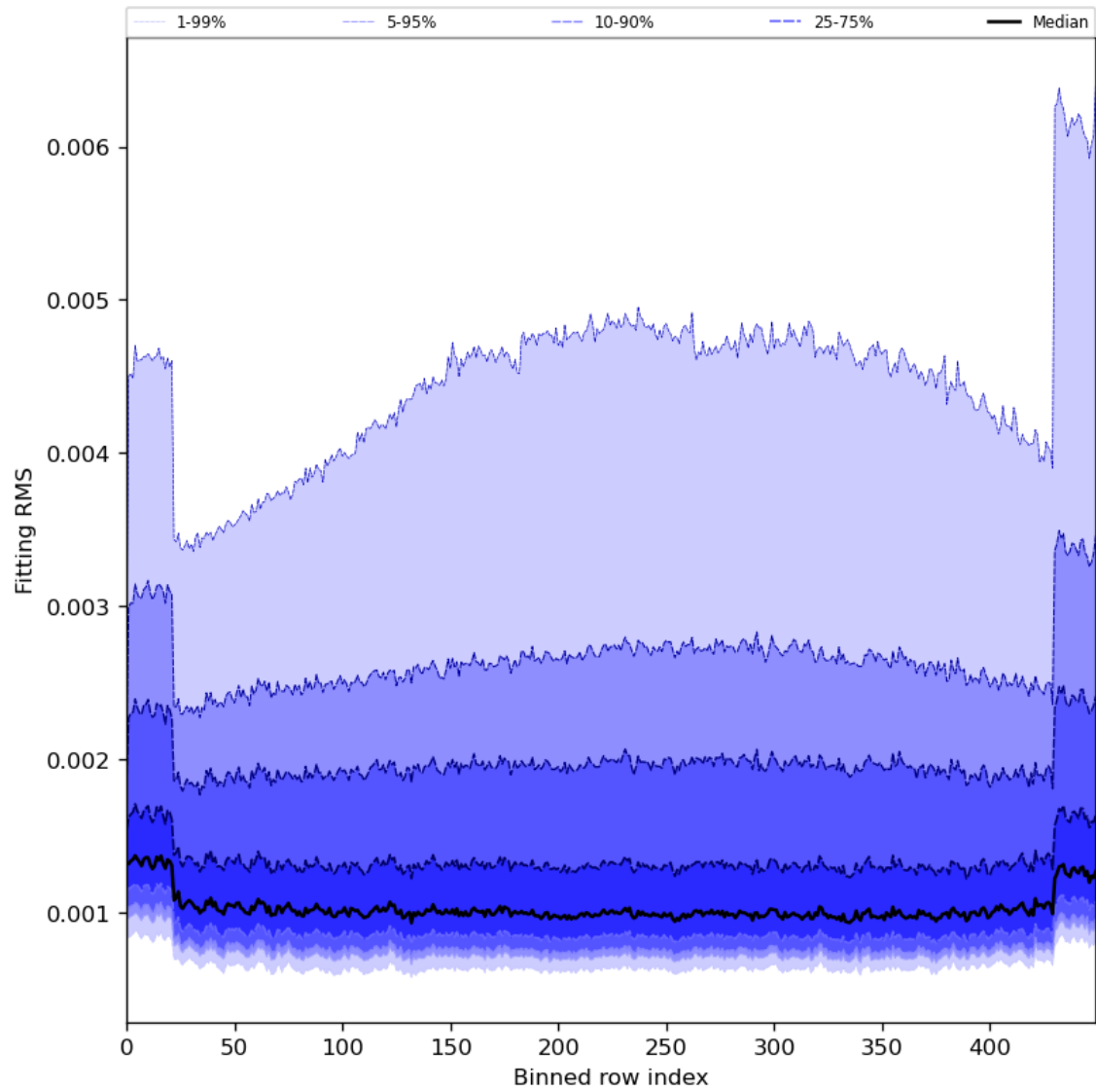
Figure 30: Along track statistics of “Fitting RMS” for 2024-04-10 to 2024-04-12
