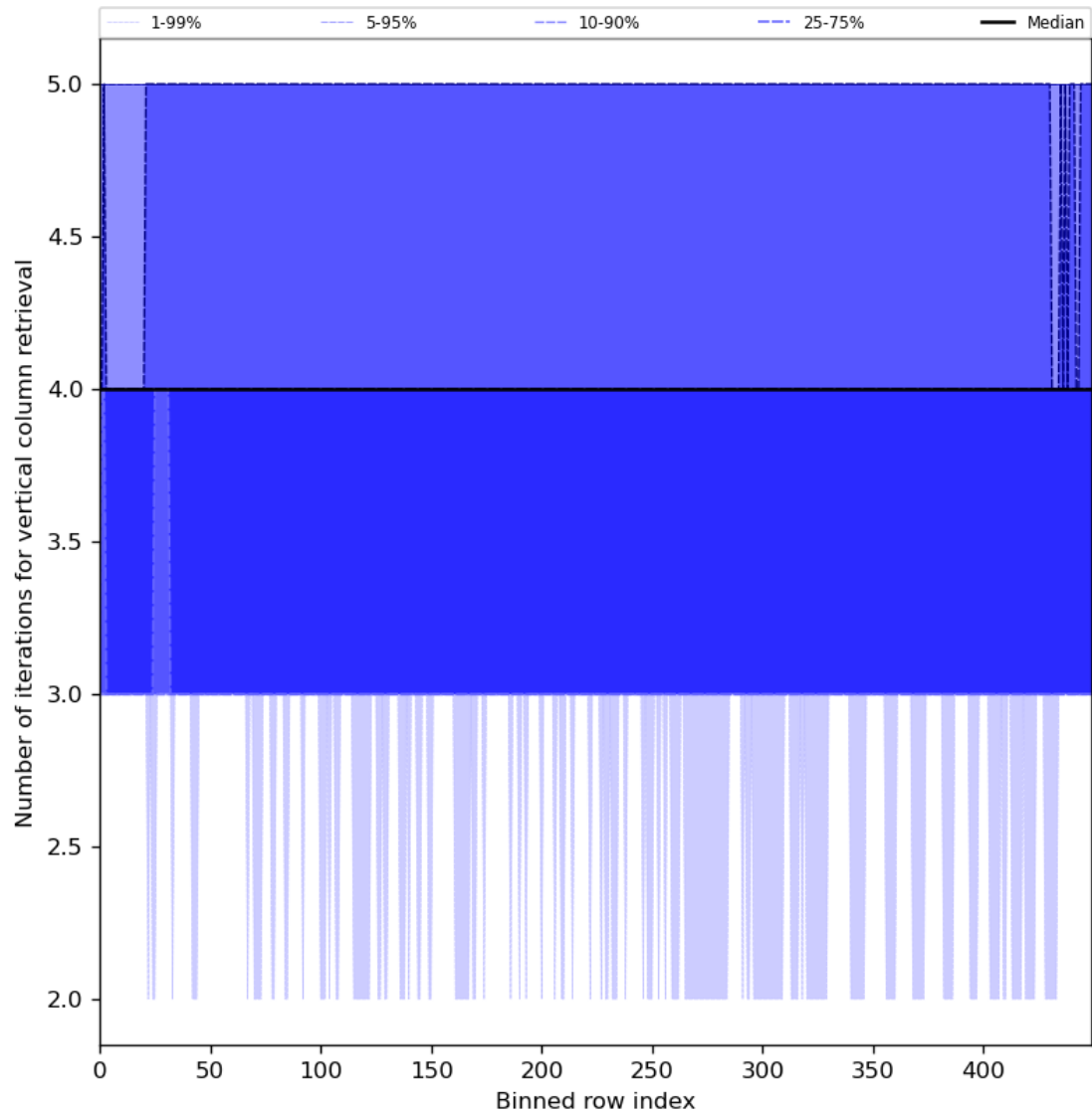
Figure 33: Along track statistics of “Number of iterations for vertical column retrieval” for 2024-04-10 to 2024-04-12
