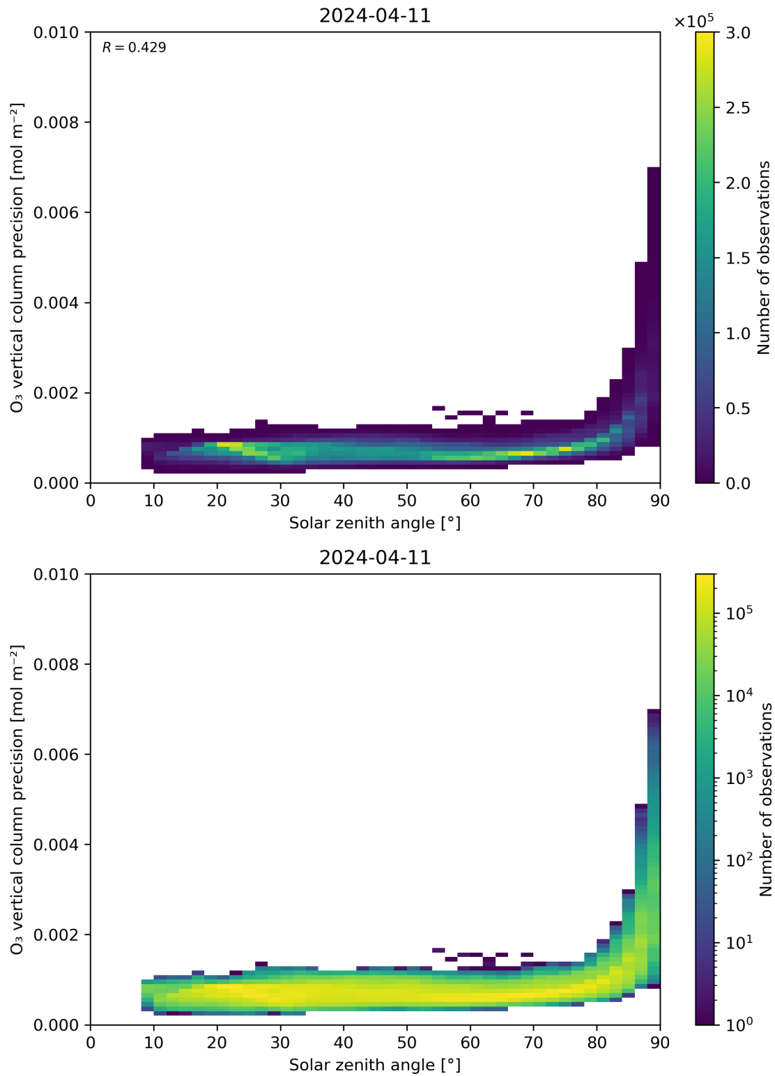
Figure 48: Scatter density plot of “Solar zenith angle” against “O 3 vertical column precision” for 2024-04-10 to 2024-04-12.
