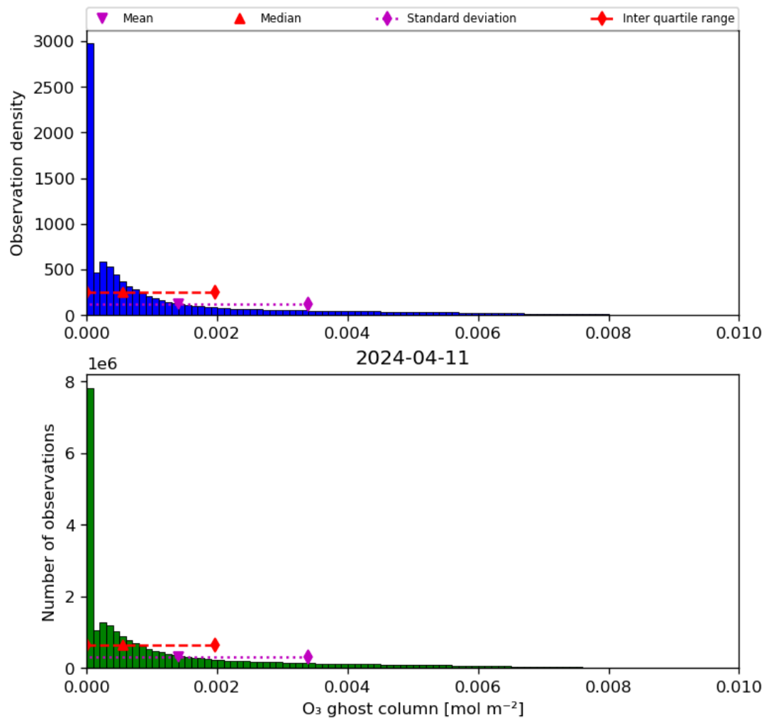
Figure 25: Histogram of “O 3 ghost column” for 2024-04-10 to 2024-04-12
