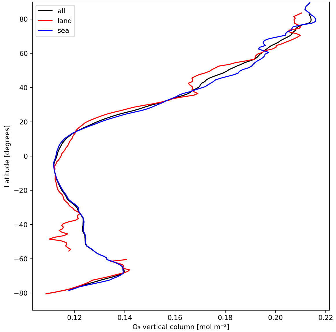
Figure 14: Zonal average of “O 3 vertical column” for 2024-04-10 to 2024-04-12.
