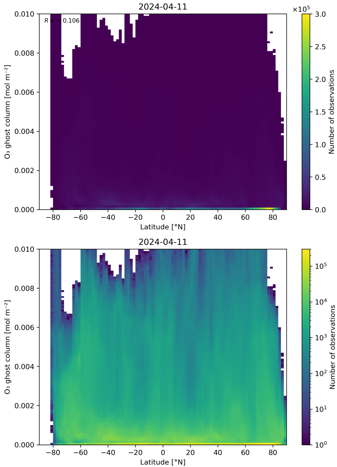
Figure 35: Scatter density plot of “Latitude” against “O 3 ghost column” for 2024-04-10 to 2024-04-12.
