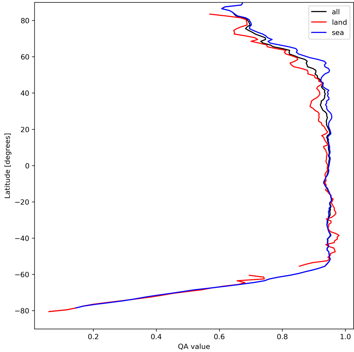
Figure 13: Zonal average of “QA value” for 2024-04-10 to 2024-04-12.
