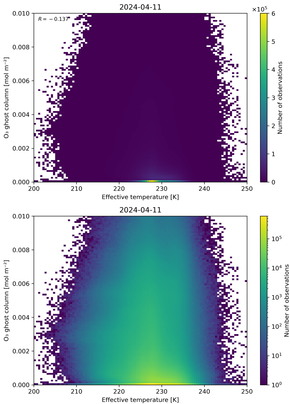
Figure 38: Scatter density plot of “Effective temperature” against “O 3 ghost column” for 2024-04-10 to 2024-04-12.
