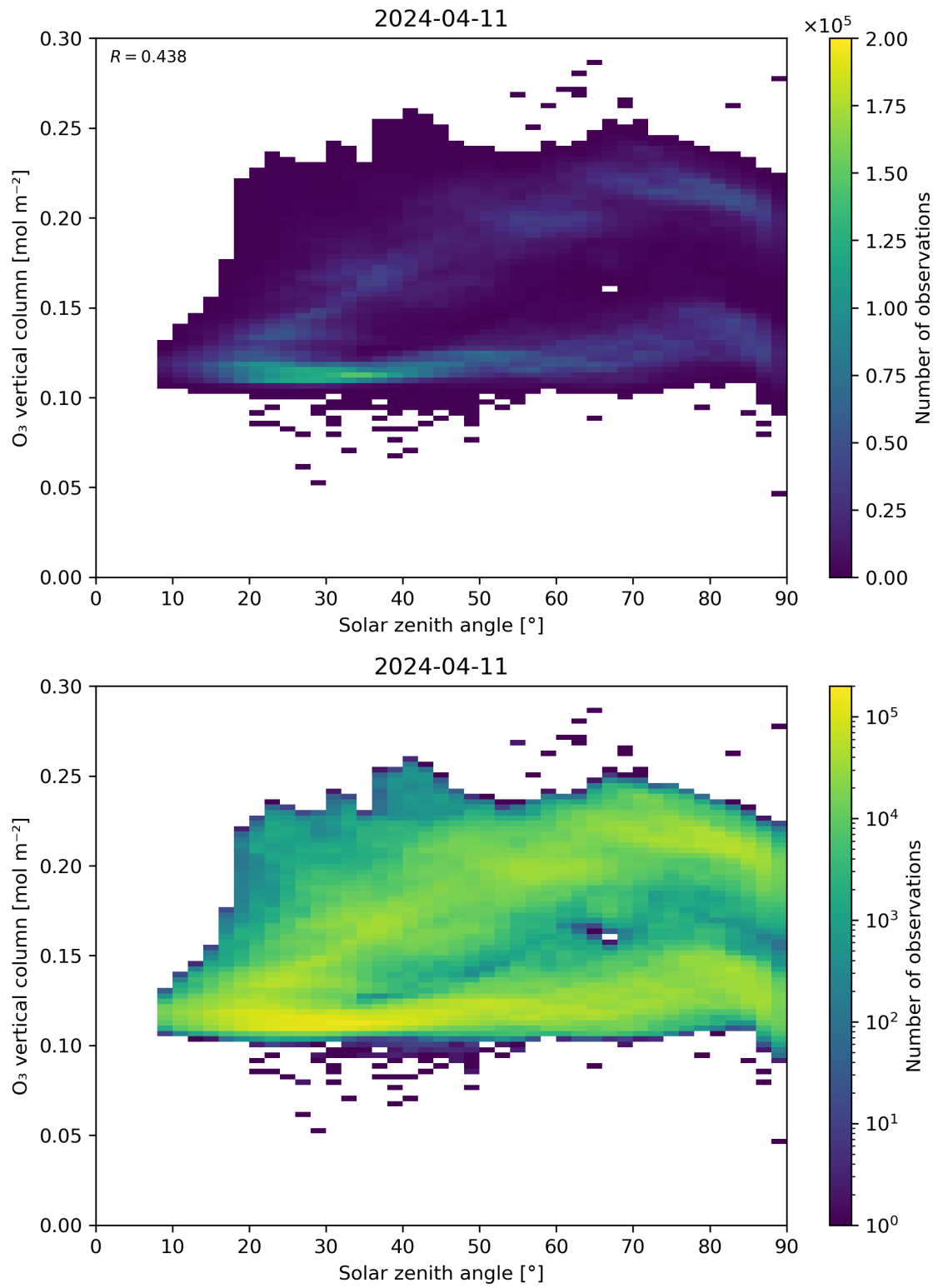
Figure 47: Scatter density plot of “Solar zenith angle” against “O 3 vertical column” for 2024-04-10 to 2024-04-12.
