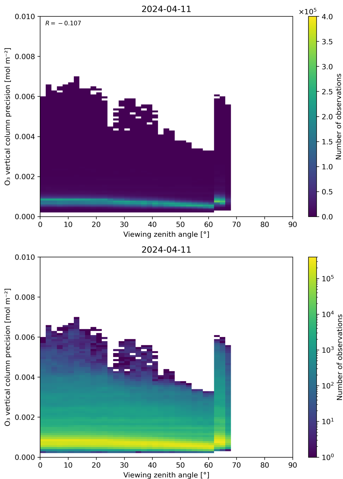
Figure 53: Scatter density plot of “Viewing zenith angle” against “O 3 vertical column precision” for 2024-04-10 to 2024-04-12.
