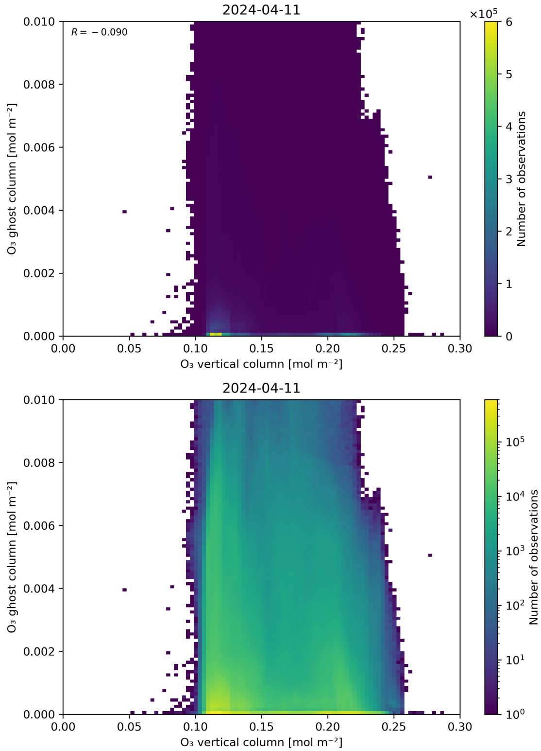
Figure 40: Scatter density plot of “O 3 vertical column” against “O 3 ghost column” for 2024-04-10 to 2024-04-12.
