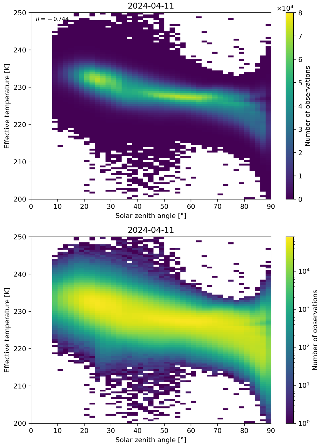
Figure 45: Scatter density plot of “Solar zenith angle” against “Effective temperature” for 2024-04-10 to 2024-04-12.
