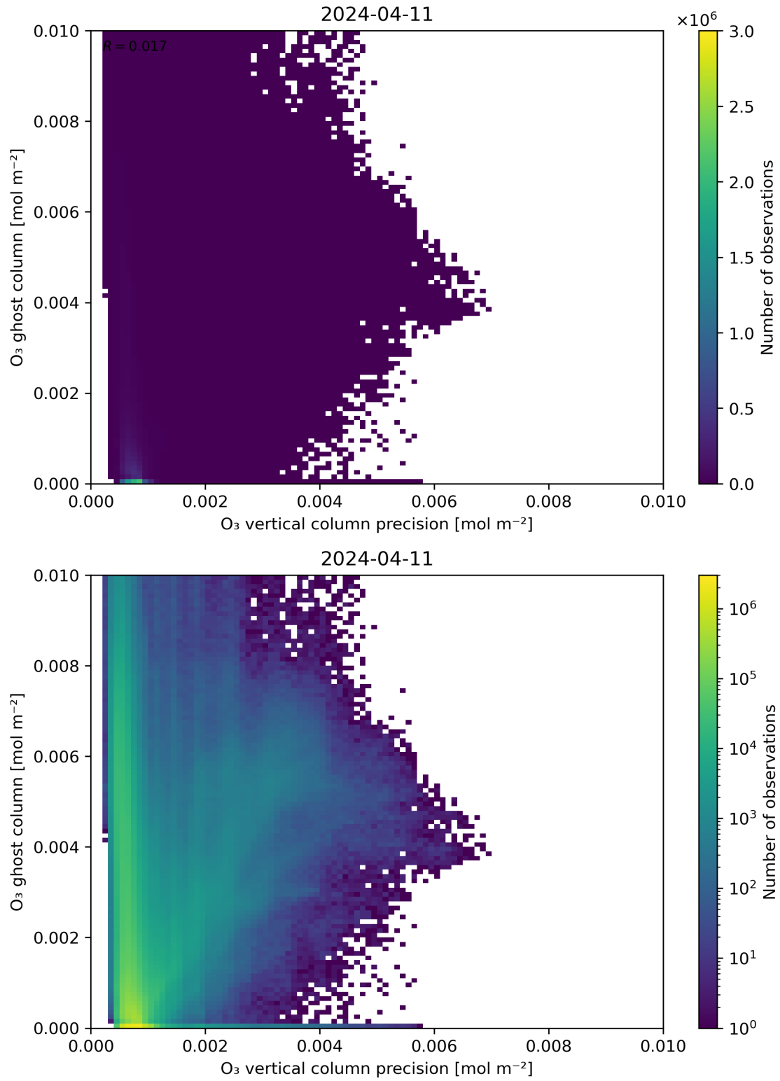
Figure 43: Scatter density plot of “ \text{O}_3 vertical column precision” against “ \text{O}_3 ghost column” for 2024-04-10 to 2024-04-12.
