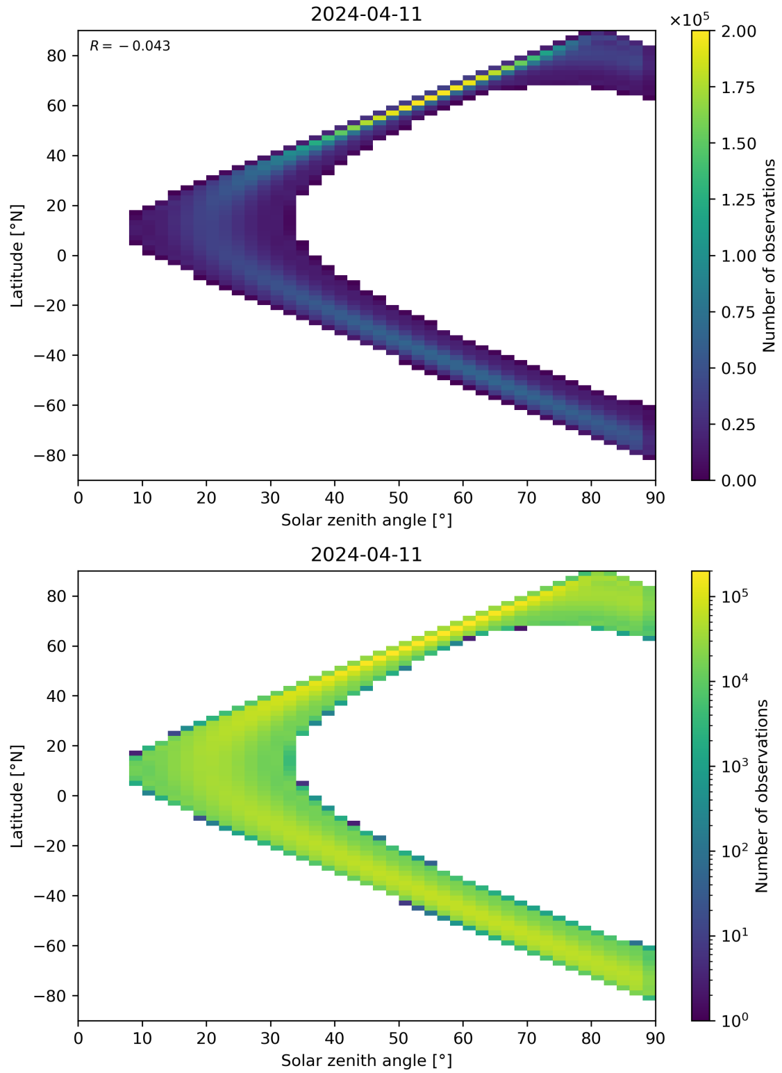
Figure 44: Scatter density plot of “Solar zenith angle” against “Latitude” for 2024-04-10 to 2024-04-12.
