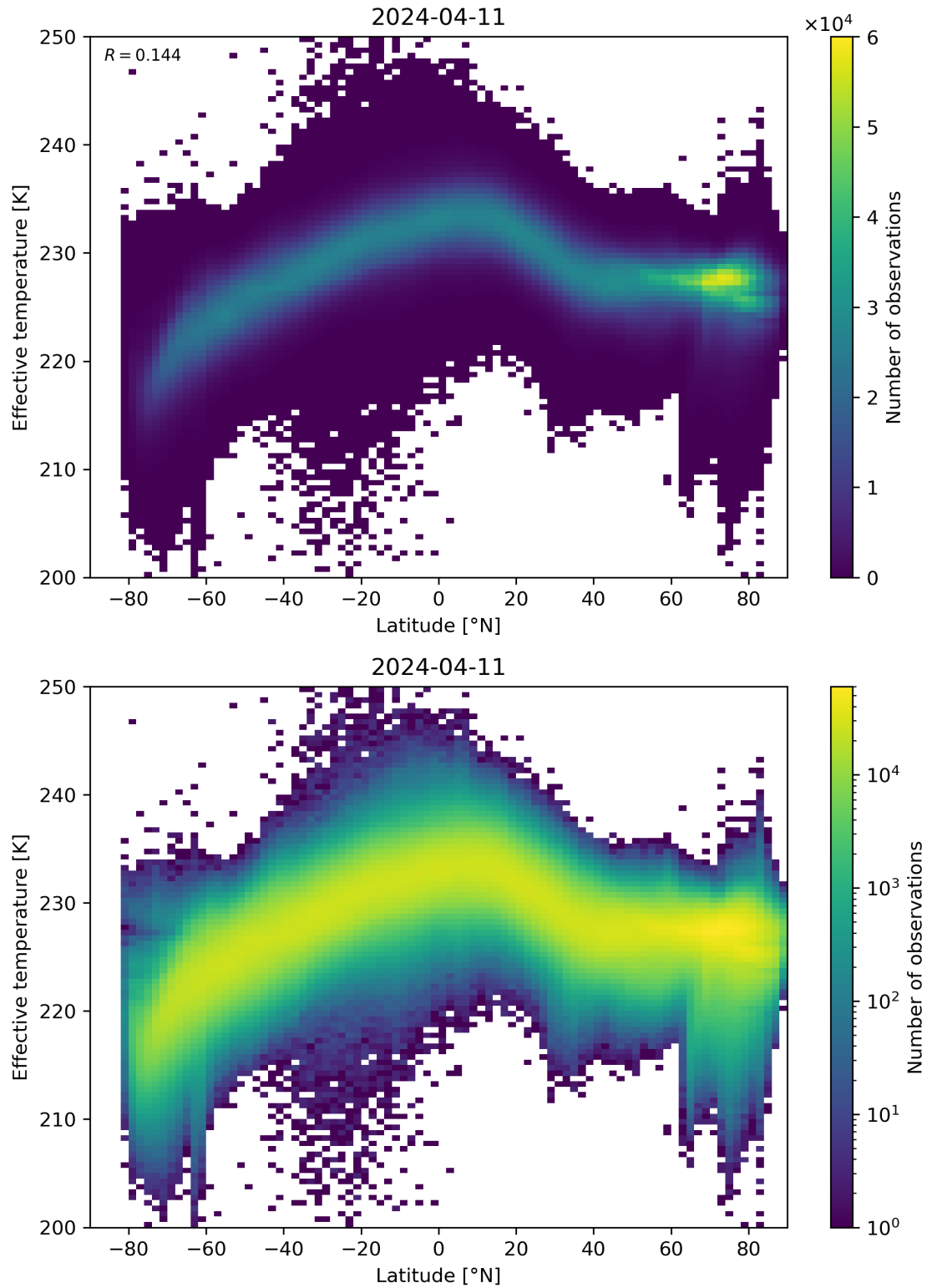
Figure 34: Scatter density plot of “Latitude” against “Effective temperature” for 2024-04-10 to 2024-04-12.
