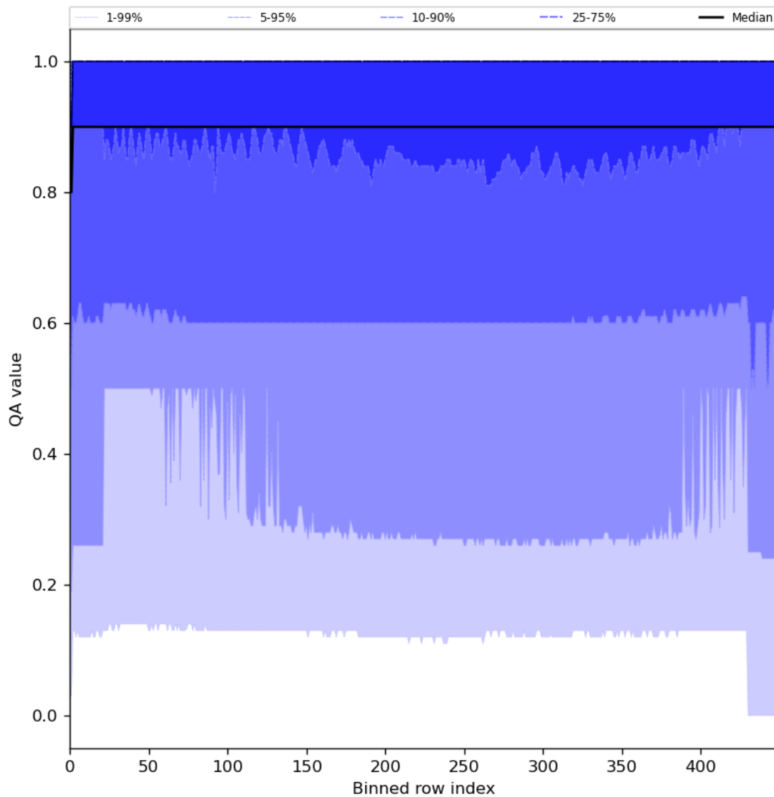
Figure 27: Along track statistics of “QA value” for 2024-04-10 to 2024-04-12
