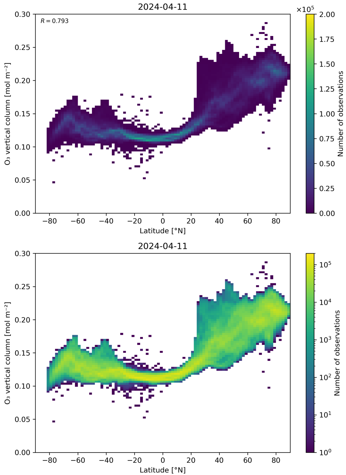
Figure 36: Scatter density plot of “Latitude” against “O 3 vertical column” for 2024-04-10 to 2024-04-12.
