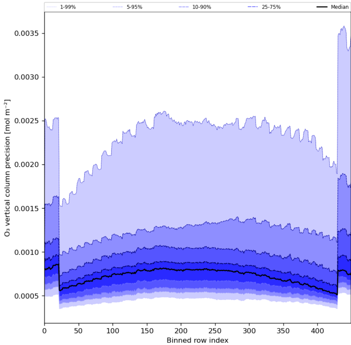
Figure 29: Along track statistics of “O 3 vertical column precision” for 2024-04-10 to 2024-04-12
