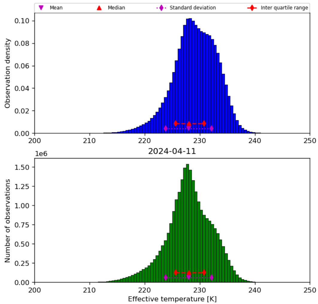
Figure 24: Histogram of “Effective temperature” for 2024-04-10 to 2024-04-12
