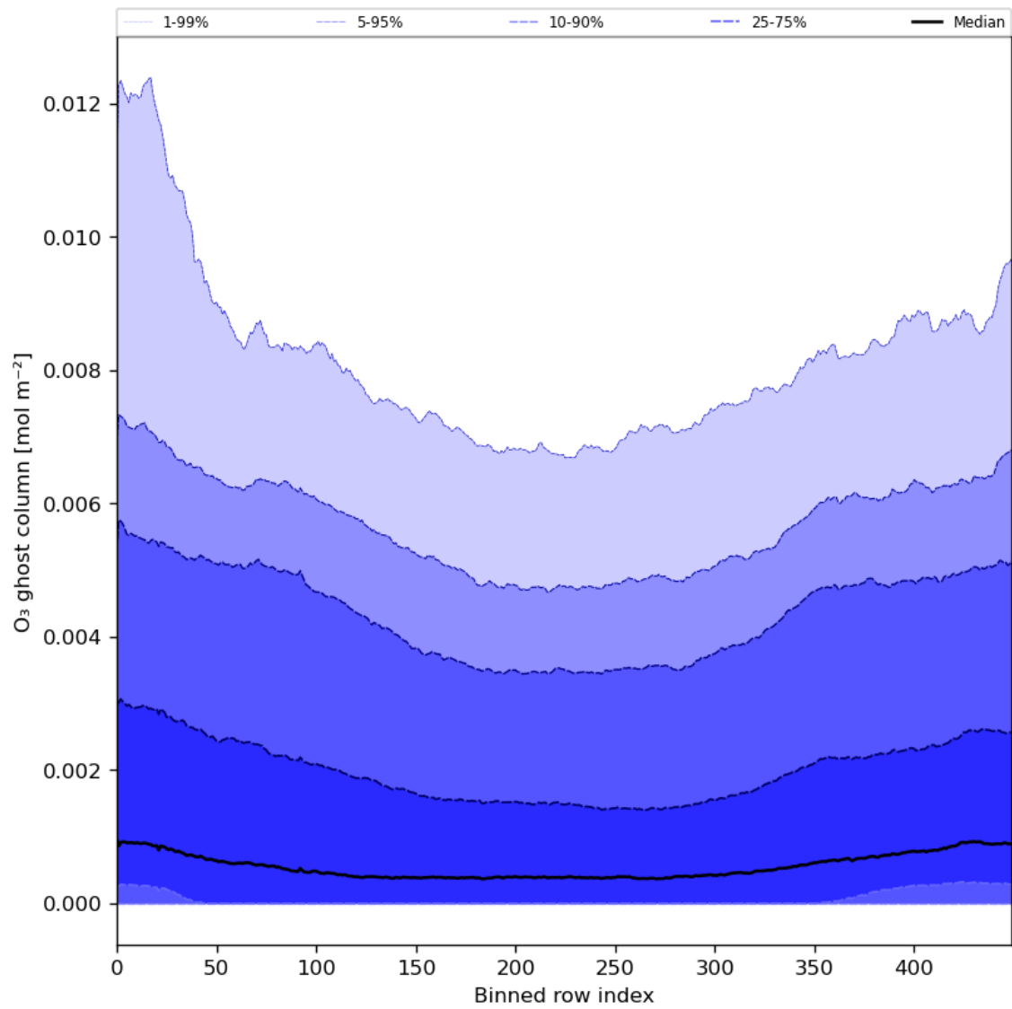
Figure 32: Along track statistics of “O 3 ghost column” for 2024-04-10 to 2024-04-12
