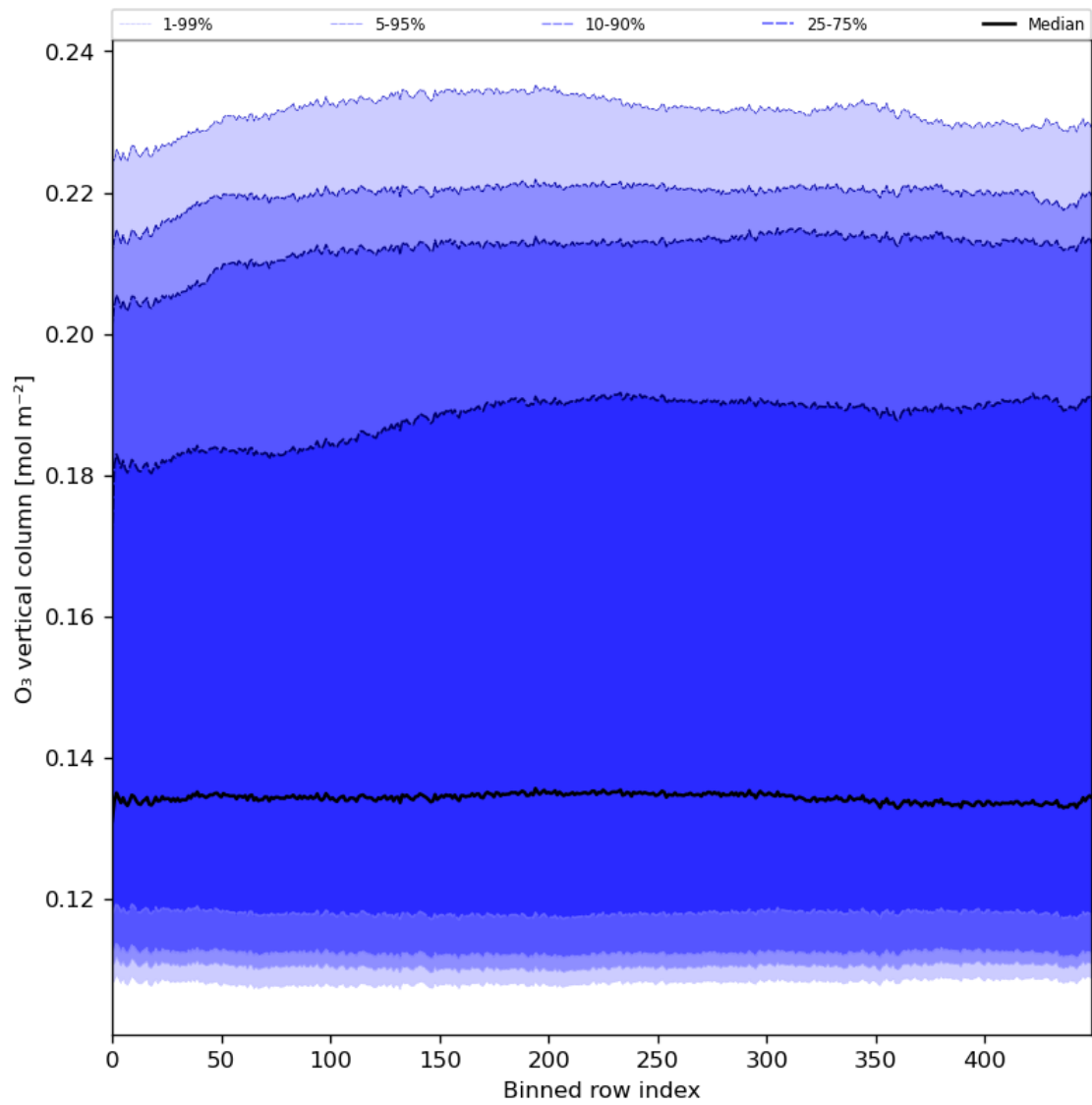
Figure 28: Along track statistics of “O 3 vertical column” for 2024-04-10 to 2024-04-12
