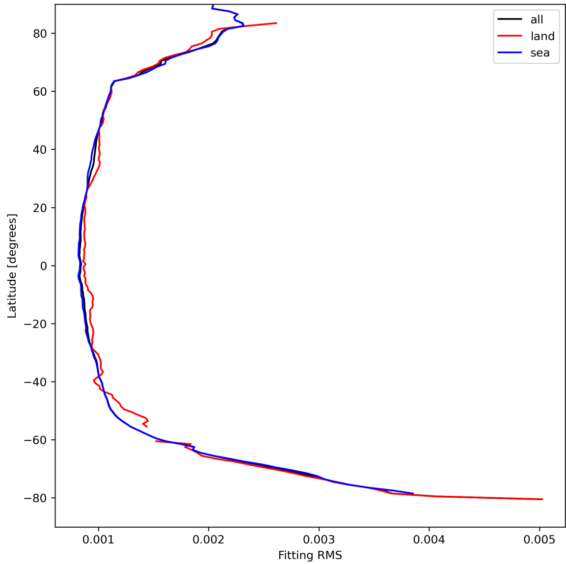
Figure 16: Zonal average of “Fitting RMS” for 2024-04-10 to 2024-04-12.
