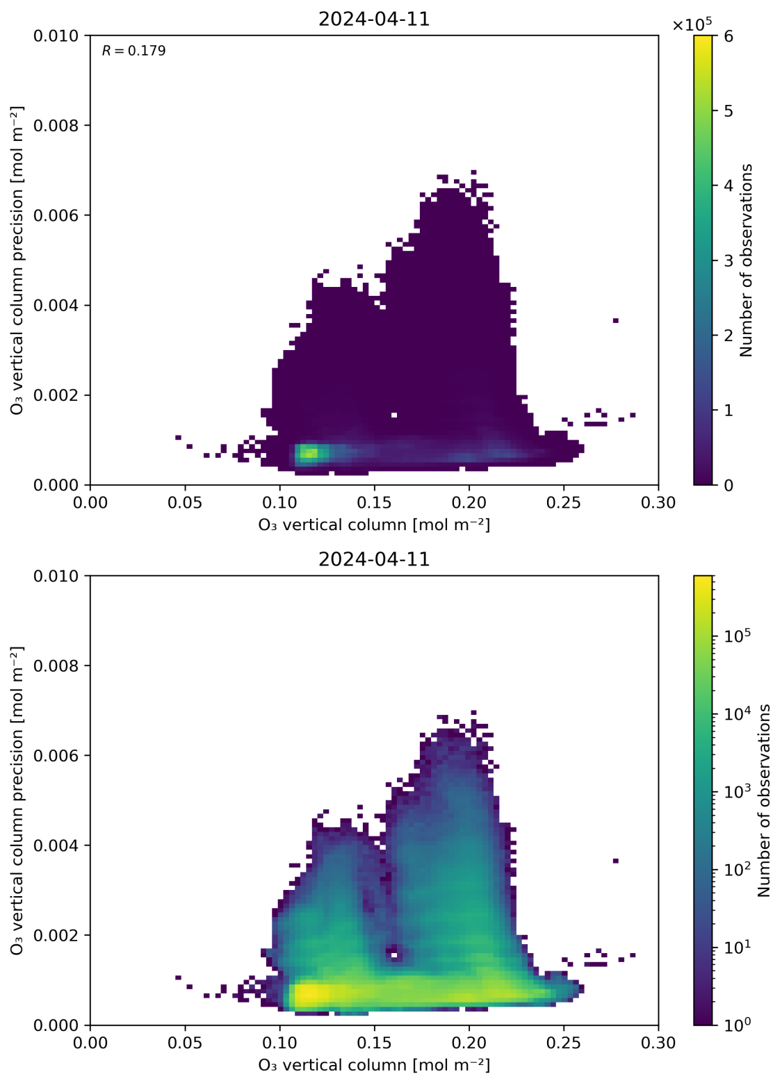
Figure 41: Scatter density plot of “O 3 vertical column” against “O 3 vertical column precision” for 2024-04-10 to 2024-04-12.
