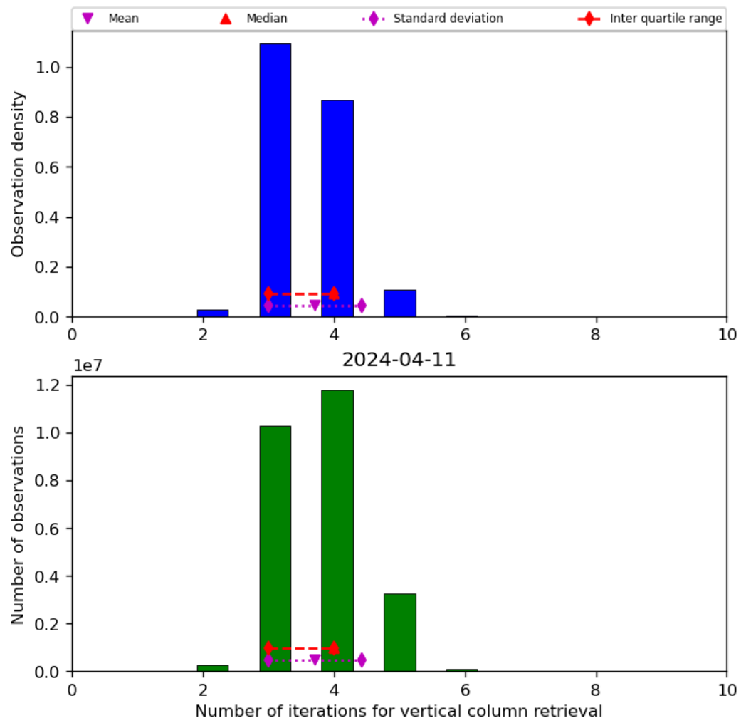
Figure 26: Histogram of “Number of iterations for vertical column retrieval” for 2024-04-10 to 2024-04-12
