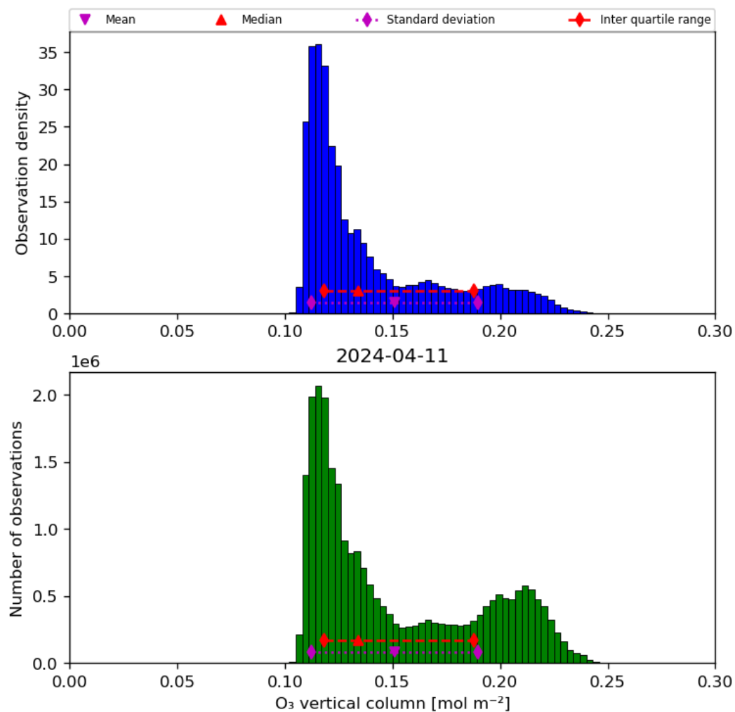
Figure 21: Histogram of “O 3 vertical column” for 2024-04-10 to 2024-04-12
