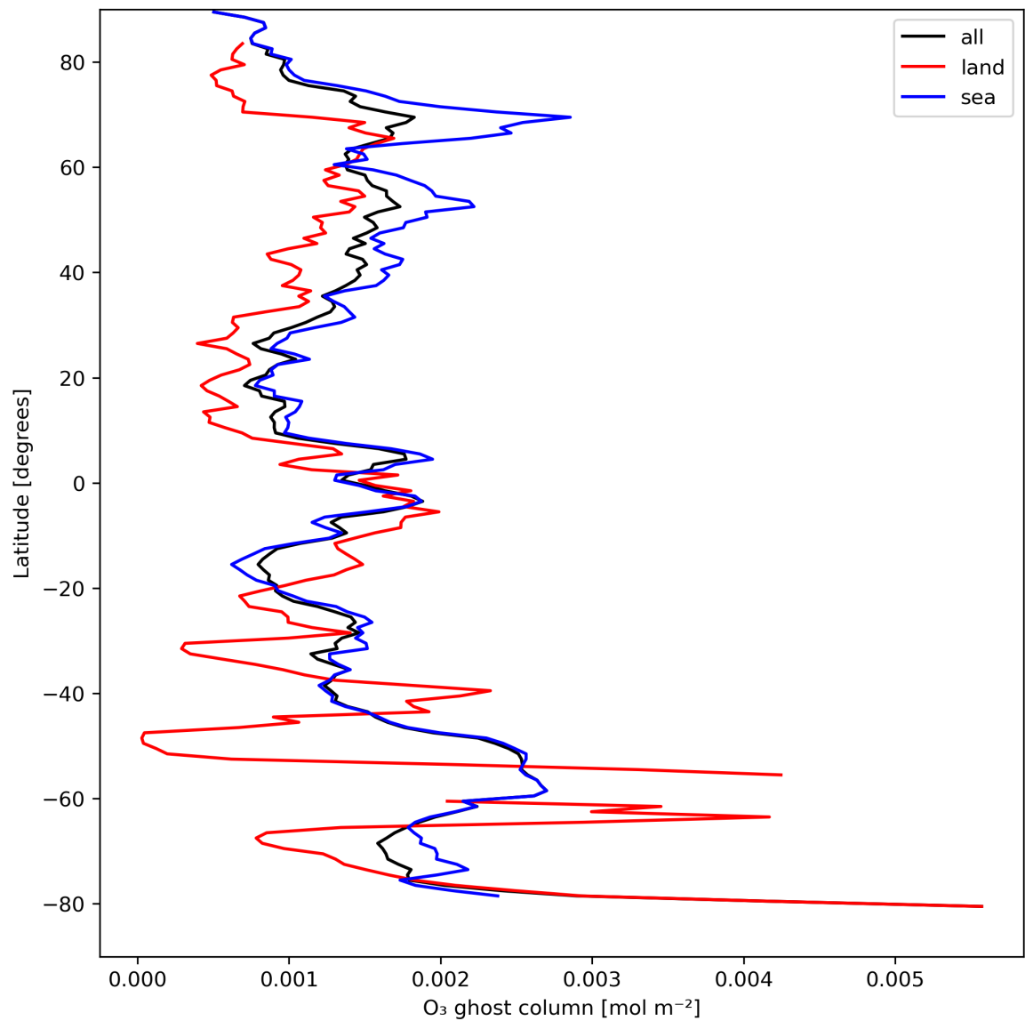
Figure 18: Zonal average of “O 3 ghost column” for 2024-04-10 to 2024-04-12.
