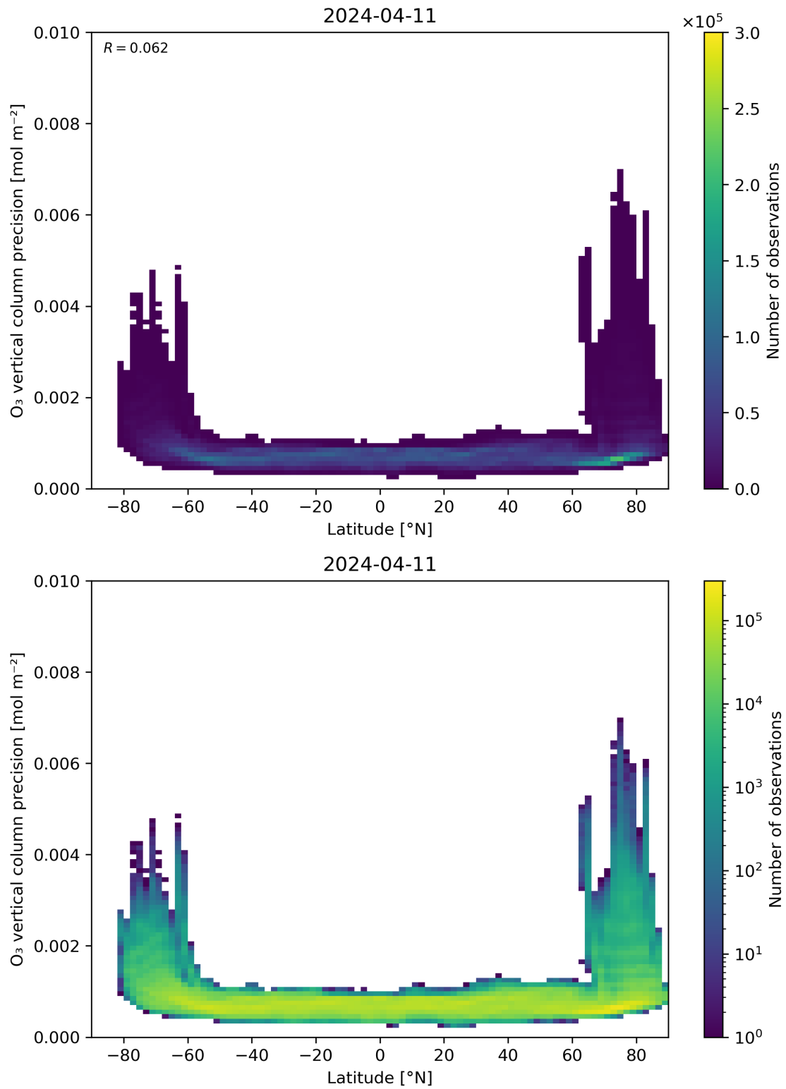
Figure 37: Scatter density plot of “Latitude” against “O 3 vertical column precision” for 2024-04-10 to 2024-04-12.
