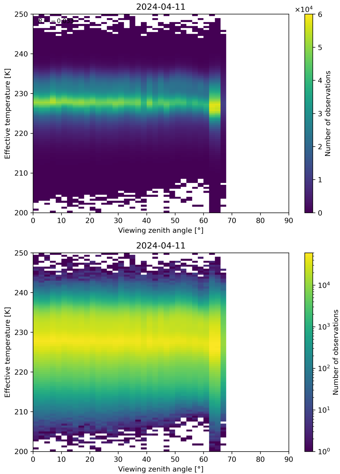
Figure 50: Scatter density plot of “Viewing zenith angle” against “Effective temperature” for 2024-04-10 to 2024-04-12.
