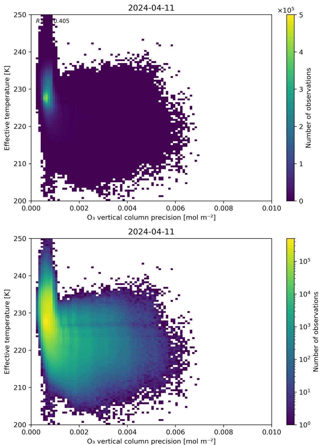
Figure 42: Scatter density plot of “O 3 vertical column precision” against “Effective temperature” for 2024-04-10 to 2024-04-12.
