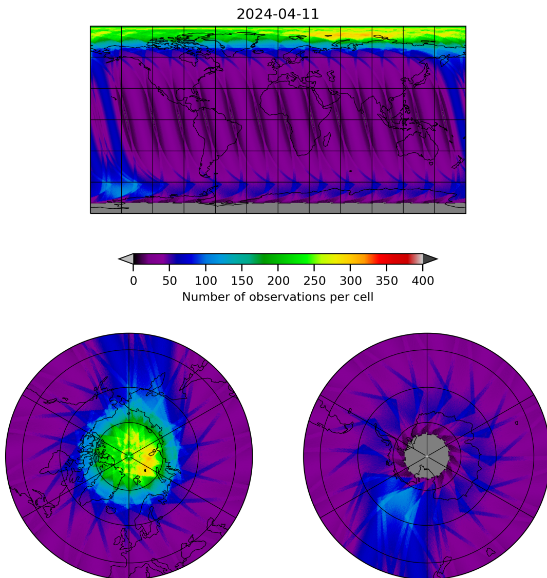
Figure 12: Map of the number of observations for 2024-04-10 to 2024-04-12
