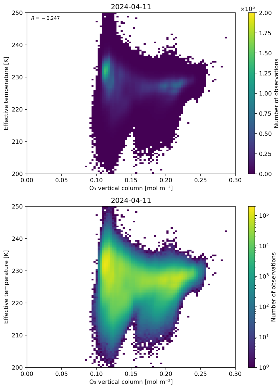
Figure 39: Scatter density plot of “O 3 vertical column” against “Effective temperature” for 2024-04-10 to 2024-04-12.
