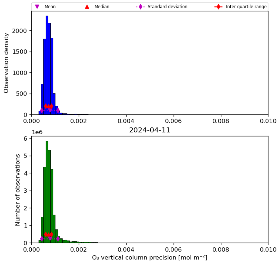
Figure 22: Histogram of “O 3 vertical column precision” for 2024-04-10 to 2024-04-12
