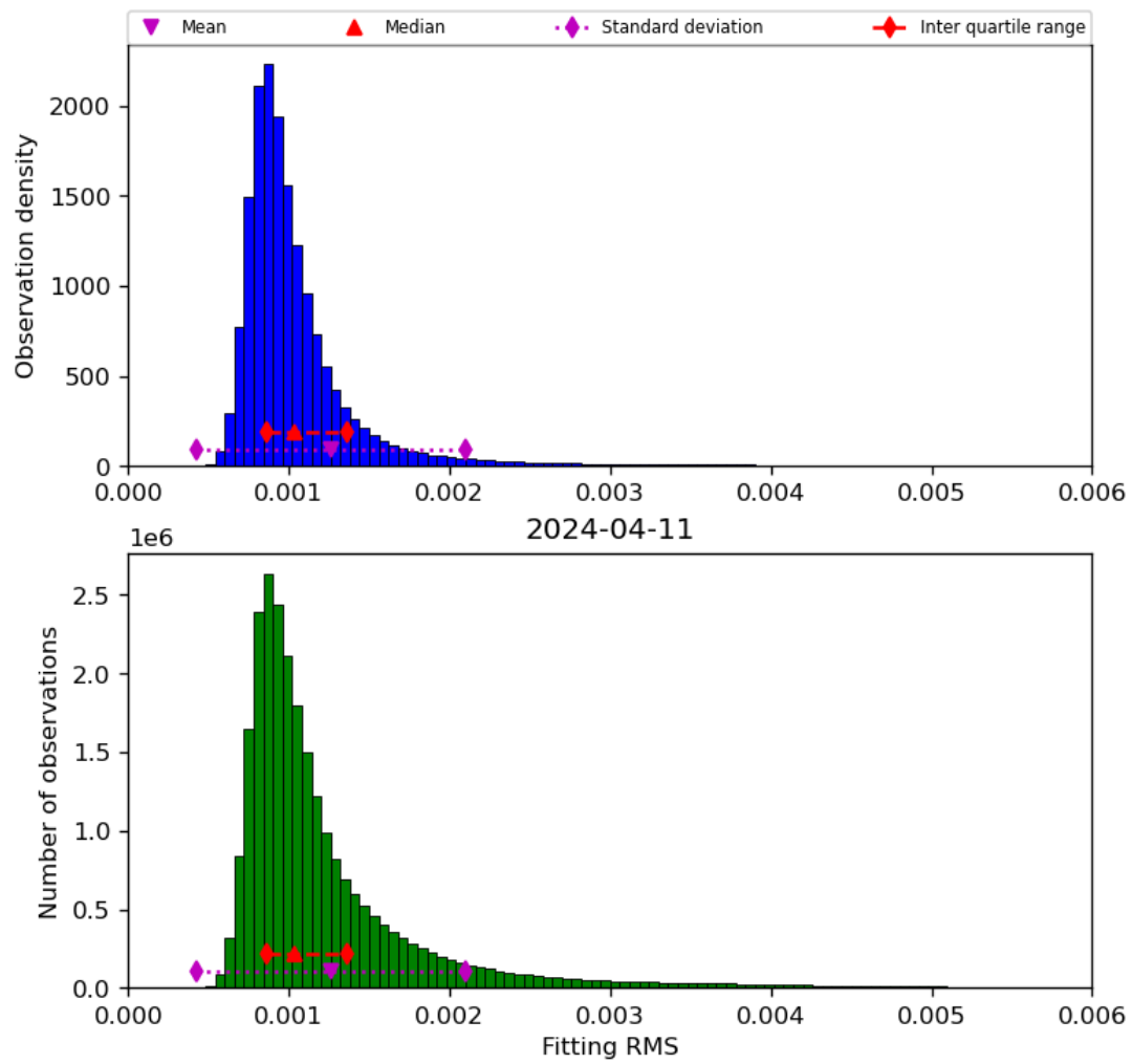
Figure 23: Histogram of “Fitting RMS” for 2024-04-10 to 2024-04-12
