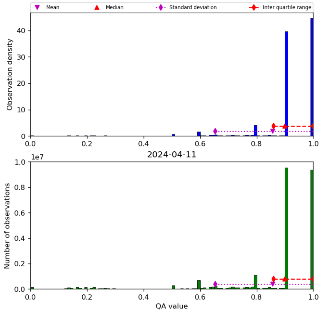
Figure 20: Histogram of “QA value” for 2024-04-10 to 2024-04-12
