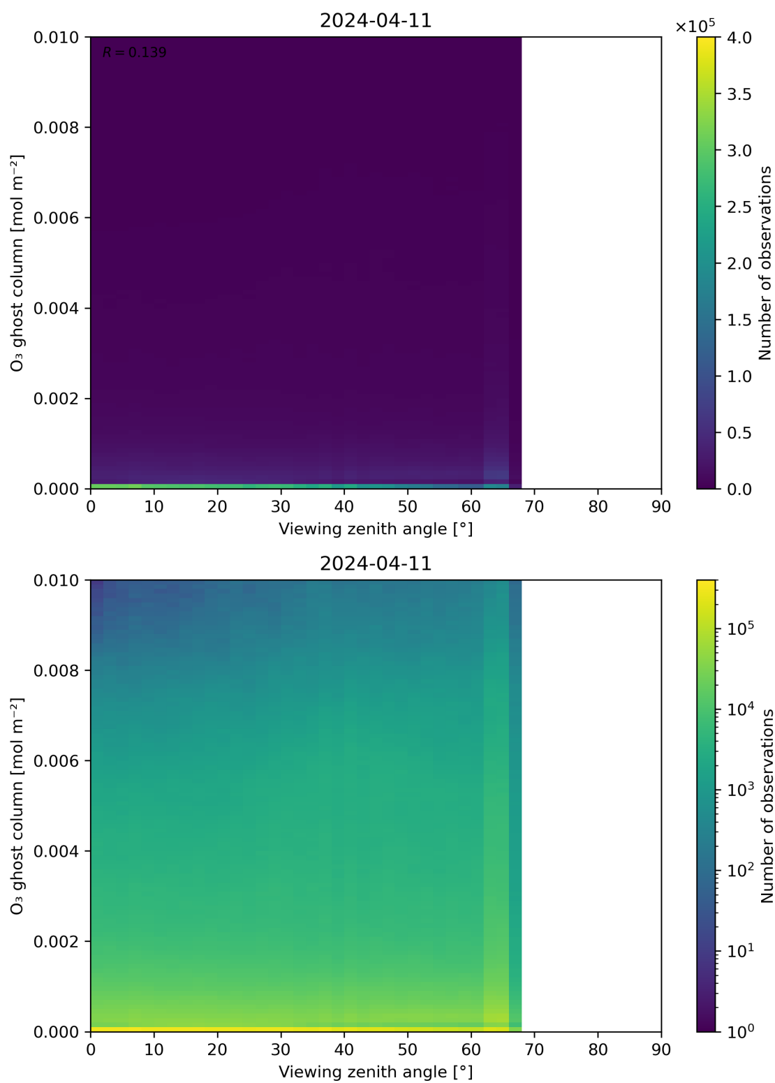
Figure 51: Scatter density plot of “Viewing zenith angle” against “O 3 ghost column” for 2024-04-10 to 2024-04-12.
