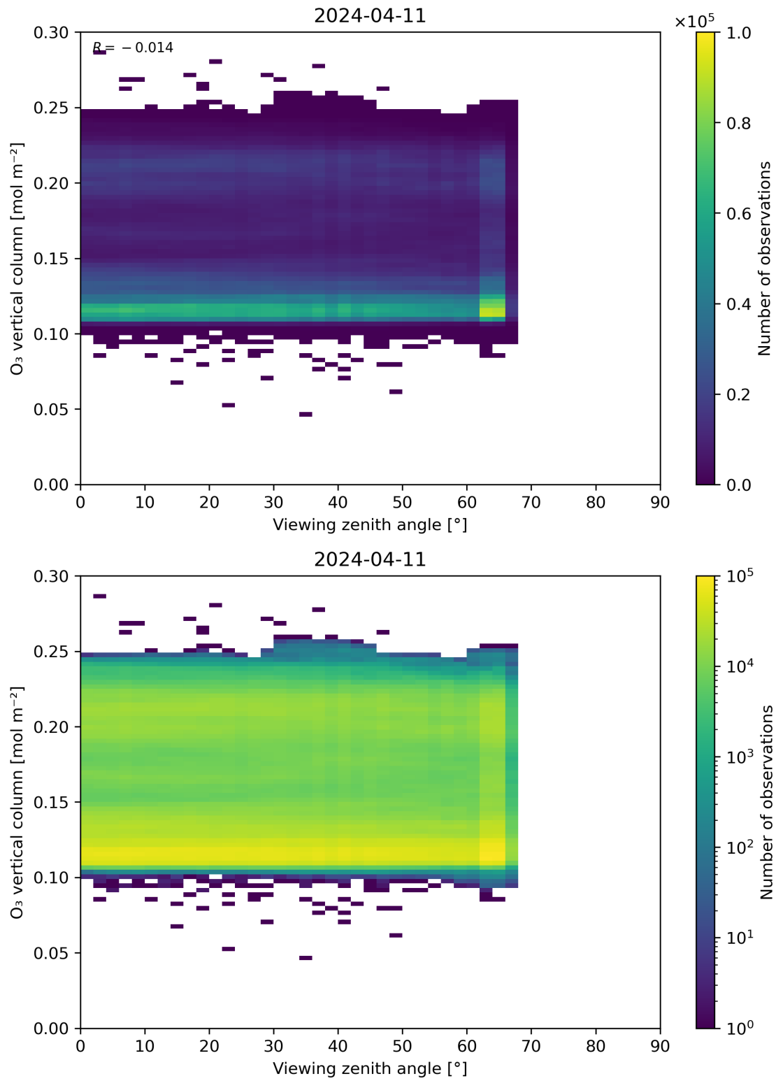
Figure 52: Scatter density plot of “Viewing zenith angle” against “O 3 vertical column” for 2024-04-10 to 2024-04-12.
