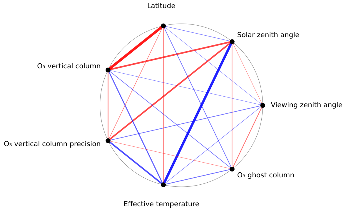
Figure 1: Map of correlation graph for 2024-04-10 to 2024-04-12.
