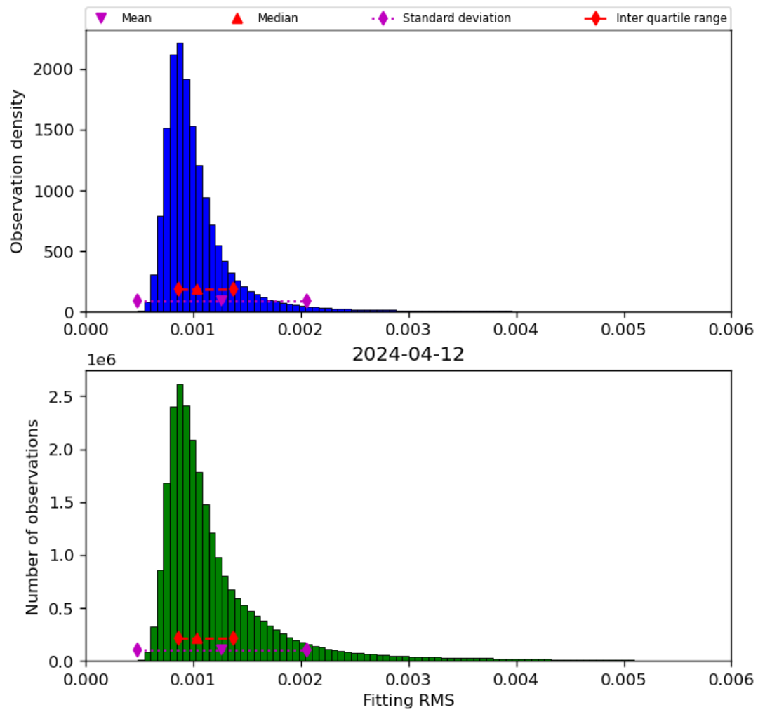
Figure 23: Histogram of “Fitting RMS” for 2024-04-11 to 2024-04-13
