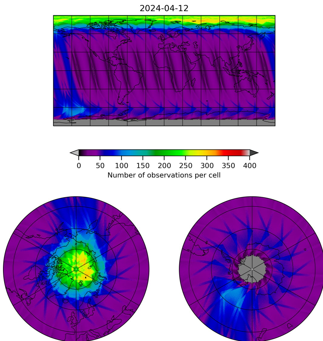
Figure 12: Map of the number of observations for 2024-04-11 to 2024-04-13
