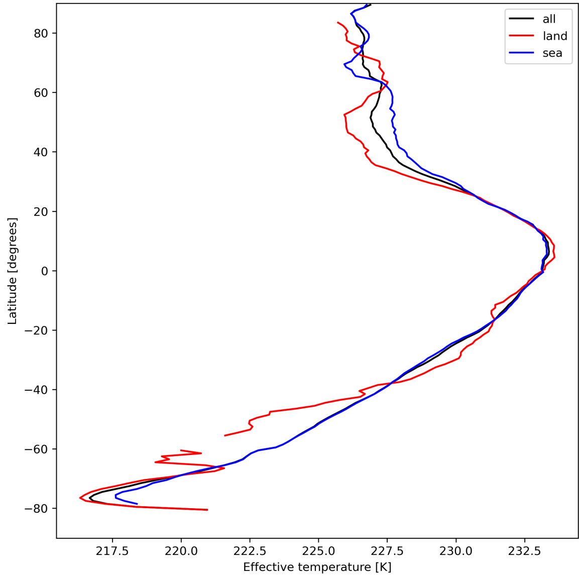
Figure 17: Zonal average of “Effective temperature” for 2024-04-11 to 2024-04-13.
