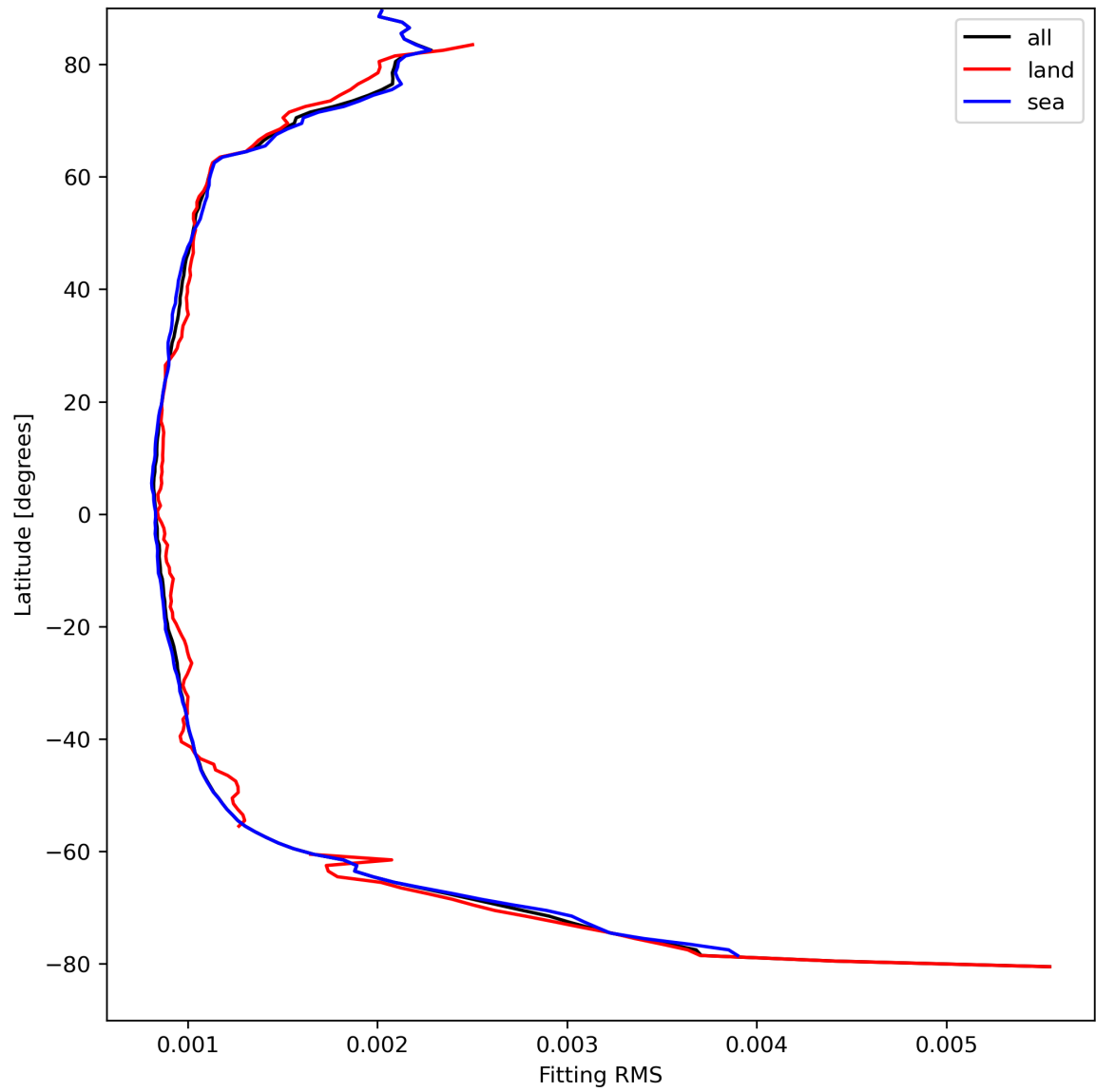
Figure 16: Zonal average of “Fitting RMS” for 2024-04-11 to 2024-04-13.
