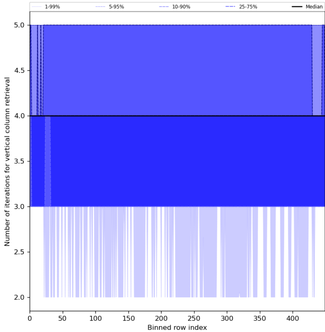
Figure 33: Along track statistics of “Number of iterations for vertical column retrieval” for 2024-04-11 to 2024-04-13
