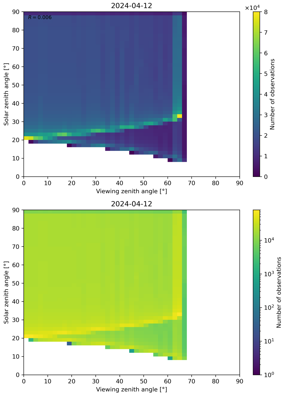
Figure 54: Scatter density plot of “Viewing zenith angle” against “Solar zenith angle” for 2024-04-11 to 2024-04-13.
