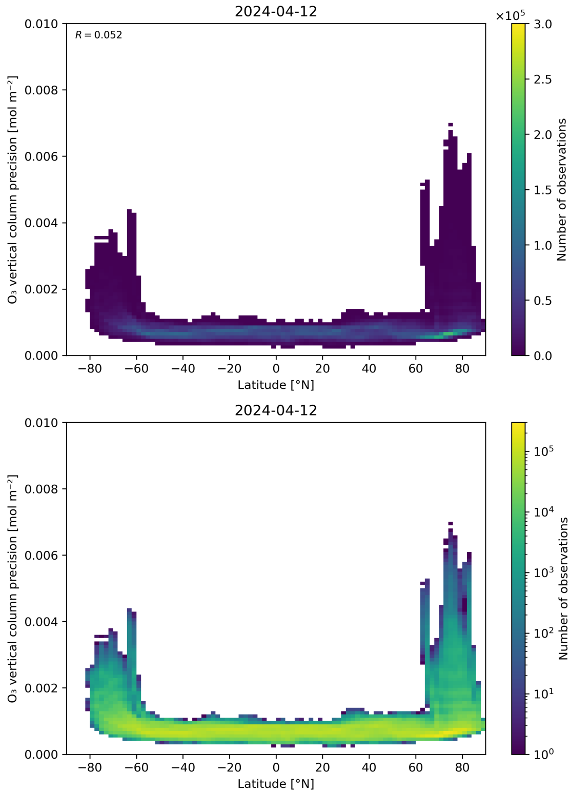
Figure 37: Scatter density plot of “Latitude” against “O 3 vertical column precision” for 2024-04-11 to 2024-04-13.
