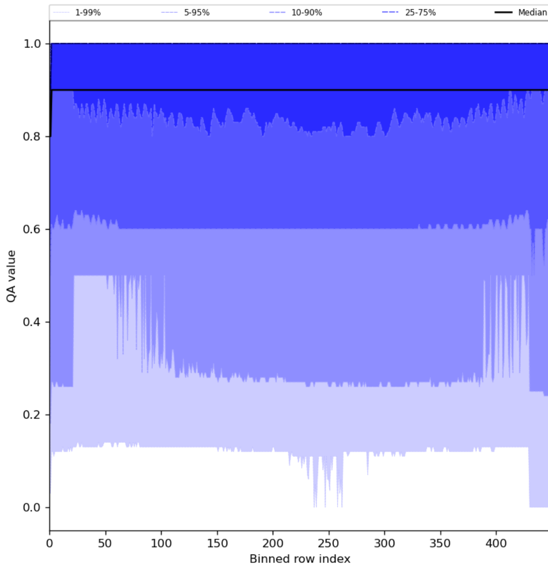
Figure 27: Along track statistics of “QA value” for 2024-04-11 to 2024-04-13
