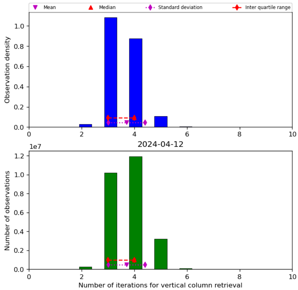
Figure 26: Histogram of “Number of iterations for vertical column retrieval” for 2024-04-11 to 2024-04-13
