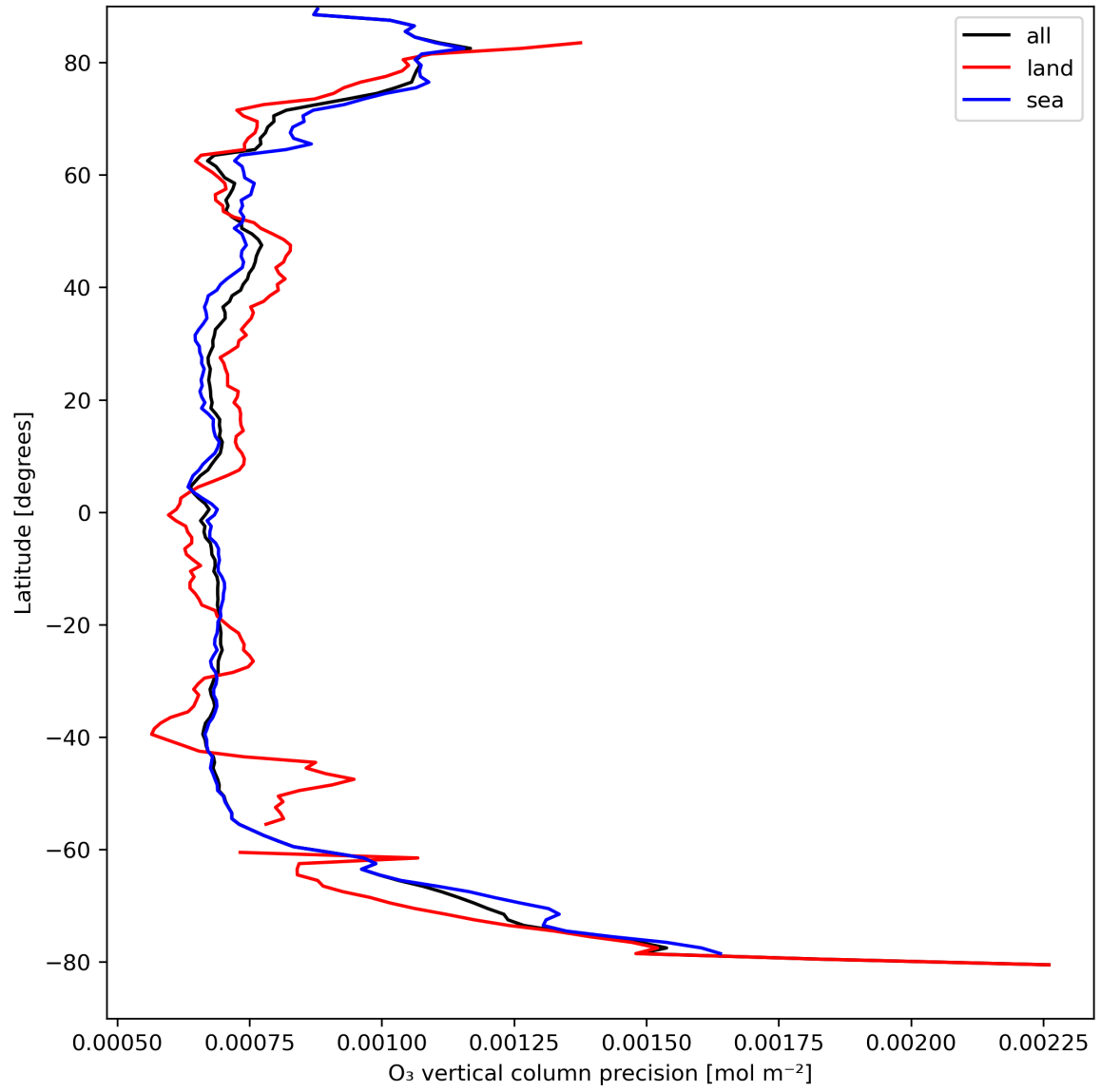
Figure 15: Zonal average of “O 3 vertical column precision” for 2024-04-11 to 2024-04-13.
