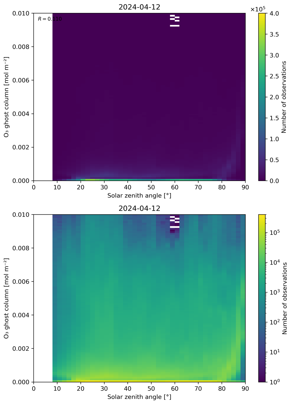
Figure 46: Scatter density plot of “Solar zenith angle” against “O 3 ghost column” for 2024-04-11 to 2024-04-13.
