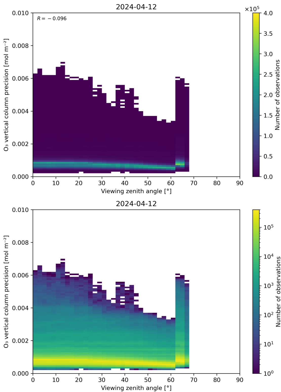
Figure 53: Scatter density plot of “Viewing zenith angle” against “O 3 vertical column precision” for 2024-04-11 to 2024-04-13.
