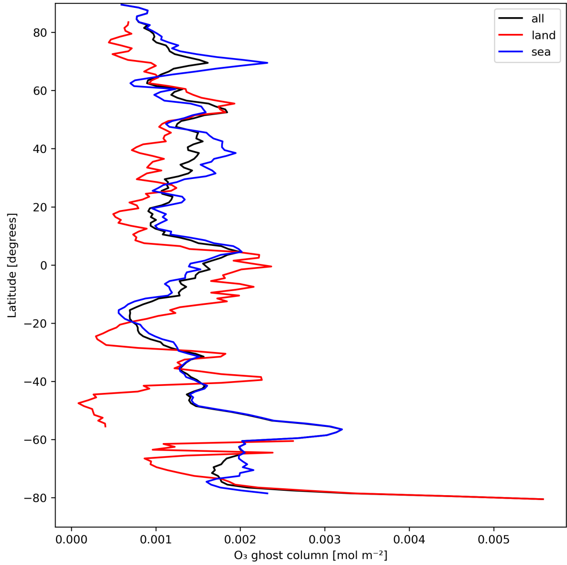
Figure 18: Zonal average of "O 3 ghost column" for 2024-04-11 to 2024-04-13.
