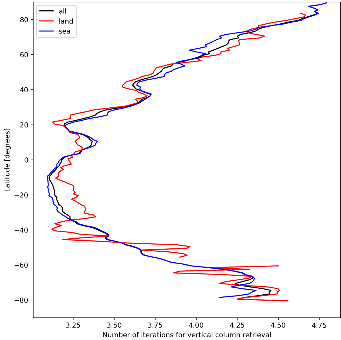
Figure 19: Zonal average of “Number of iterations for vertical column retrieval” for 2024-04-11 to 2024-04-13.
