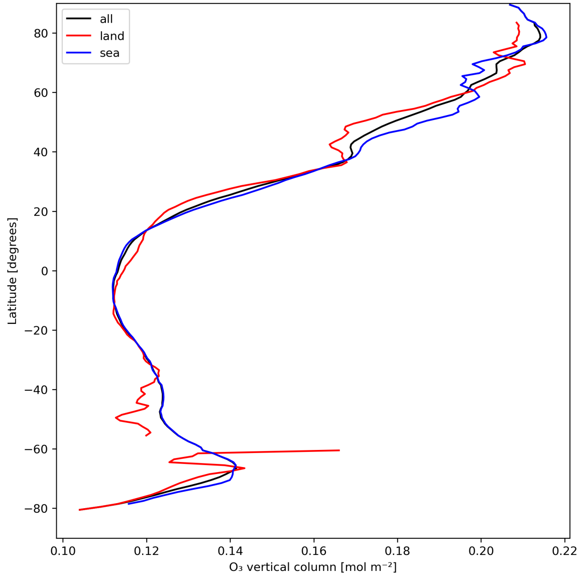
Figure 14: Zonal average of “O 3 vertical column” for 2024-04-11 to 2024-04-13.
