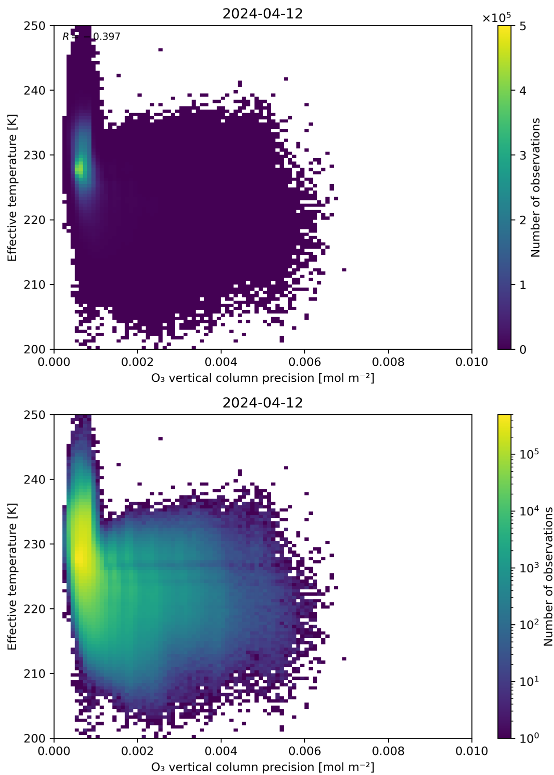
Figure 42: Scatter density plot of “O 3 vertical column precision” against “Effective temperature” for 2024-04-11 to 2024-04-13.
