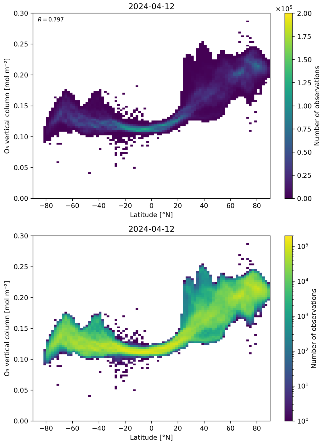
Figure 36: Scatter density plot of “Latitude” against “O 3 vertical column” for 2024-04-11 to 2024-04-13.
