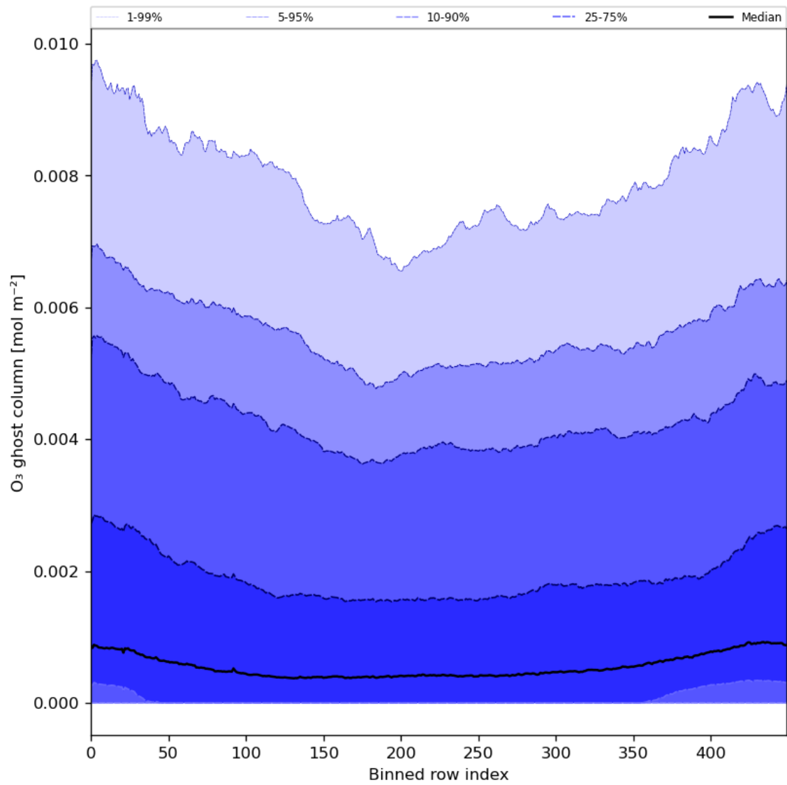
Figure 32: Along track statistics of “O 3 ghost column” for 2024-04-11 to 2024-04-13
