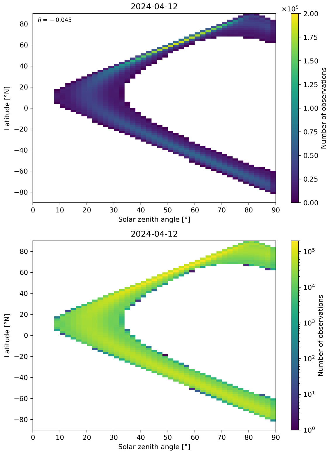
Figure 44: Scatter density plot of “Solar zenith angle” against “Latitude” for 2024-04-11 to 2024-04-13.
