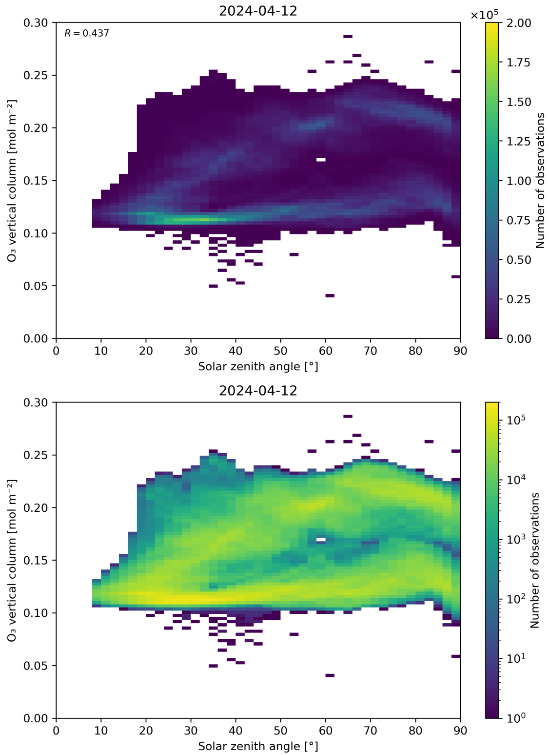
Figure 47: Scatter density plot of “Solar zenith angle” against “O 3 vertical column” for 2024-04-11 to 2024-04-13.
