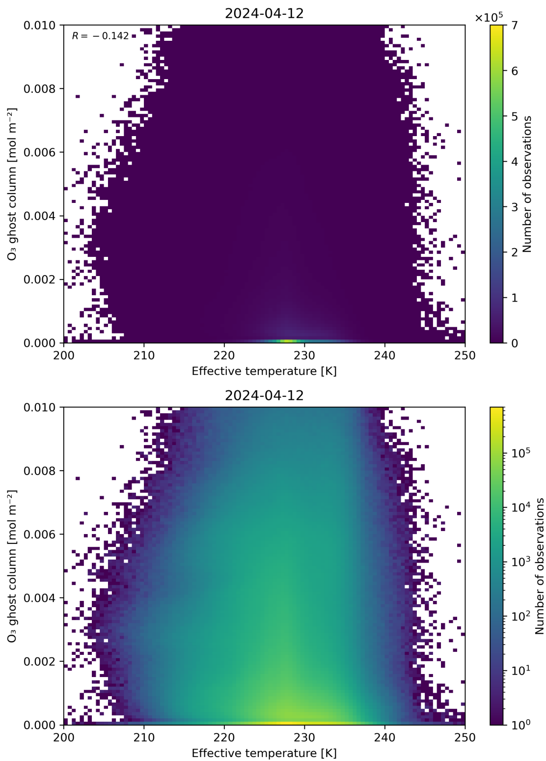
Figure 38: Scatter density plot of “Effective temperature” against “O 3 ghost column” for 2024-04-11 to 2024-04-13.
