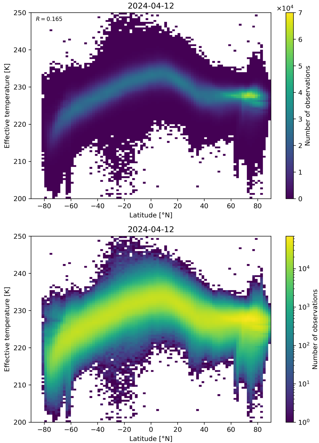
Figure 34: Scatter density plot of “Latitude” against “Effective temperature” for 2024-04-11 to 2024-04-13.
