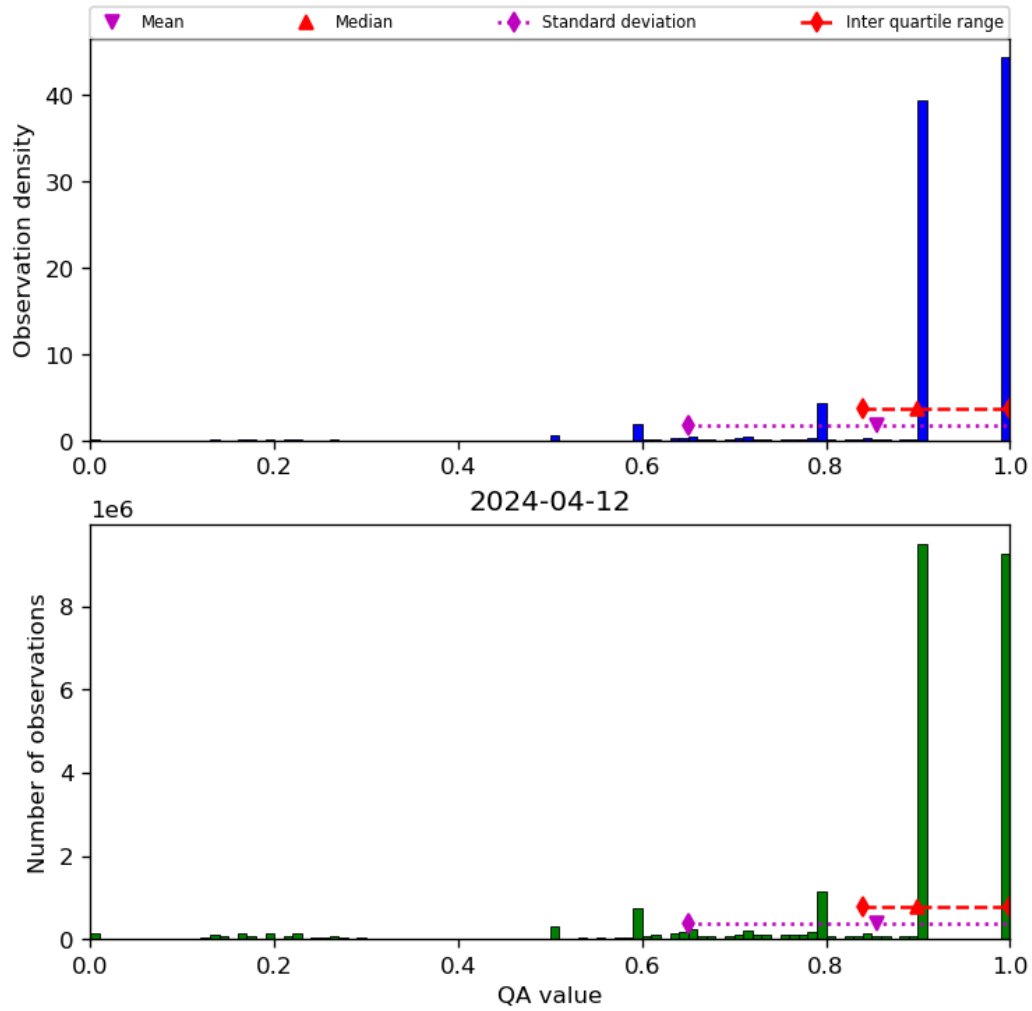
Figure 20: Histogram of “QA value” for 2024-04-11 to 2024-04-13
