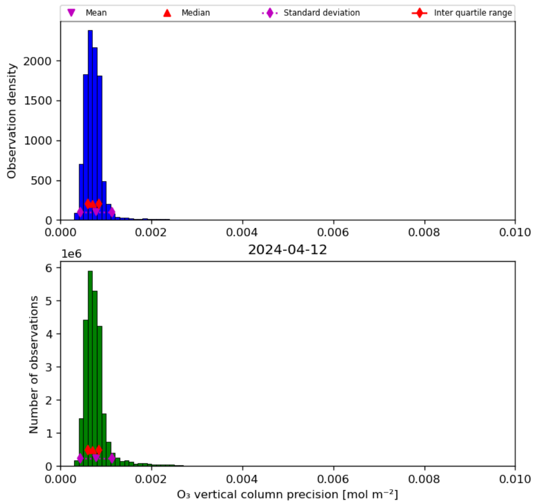
Figure 22: Histogram of “O 3 vertical column precision” for 2024-04-11 to 2024-04-13
