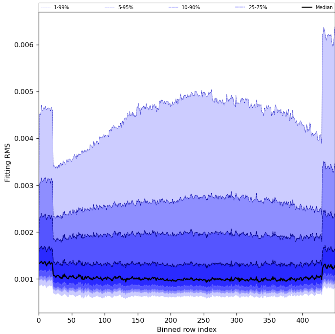
Figure 30: Along track statistics of “Fitting RMS” for 2024-04-11 to 2024-04-13
