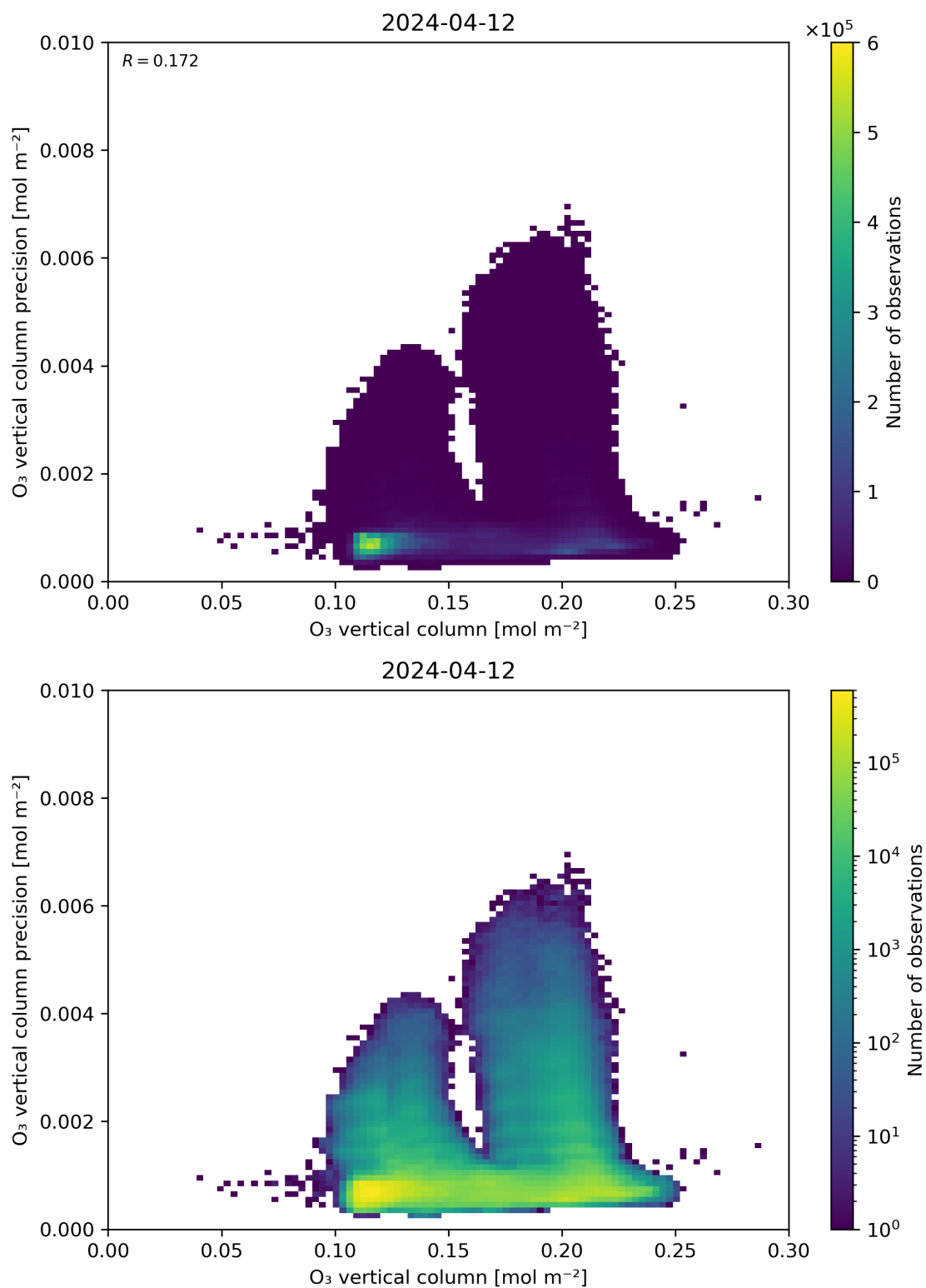
Figure 41: Scatter density plot of “O 3 vertical column” against “O 3 vertical column precision” for 2024-04-11 to 2024-04-13.
