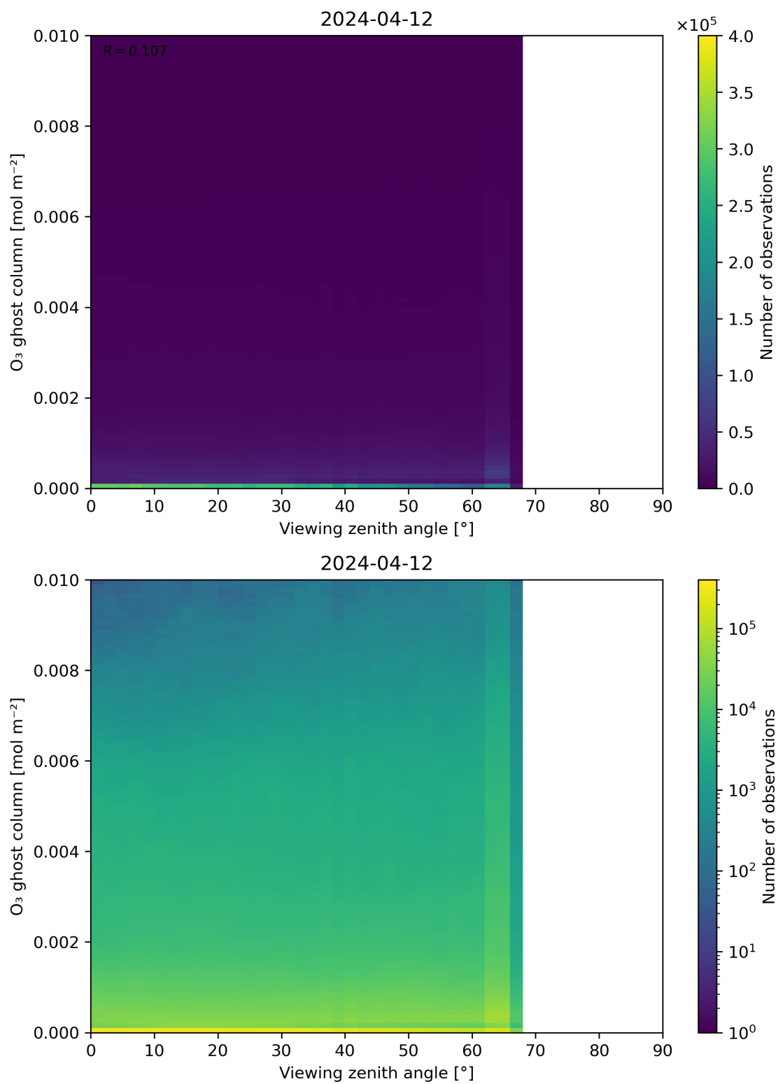
Figure 51: Scatter density plot of “Viewing zenith angle” against “O 3 ghost column” for 2024-04-11 to 2024-04-13.
