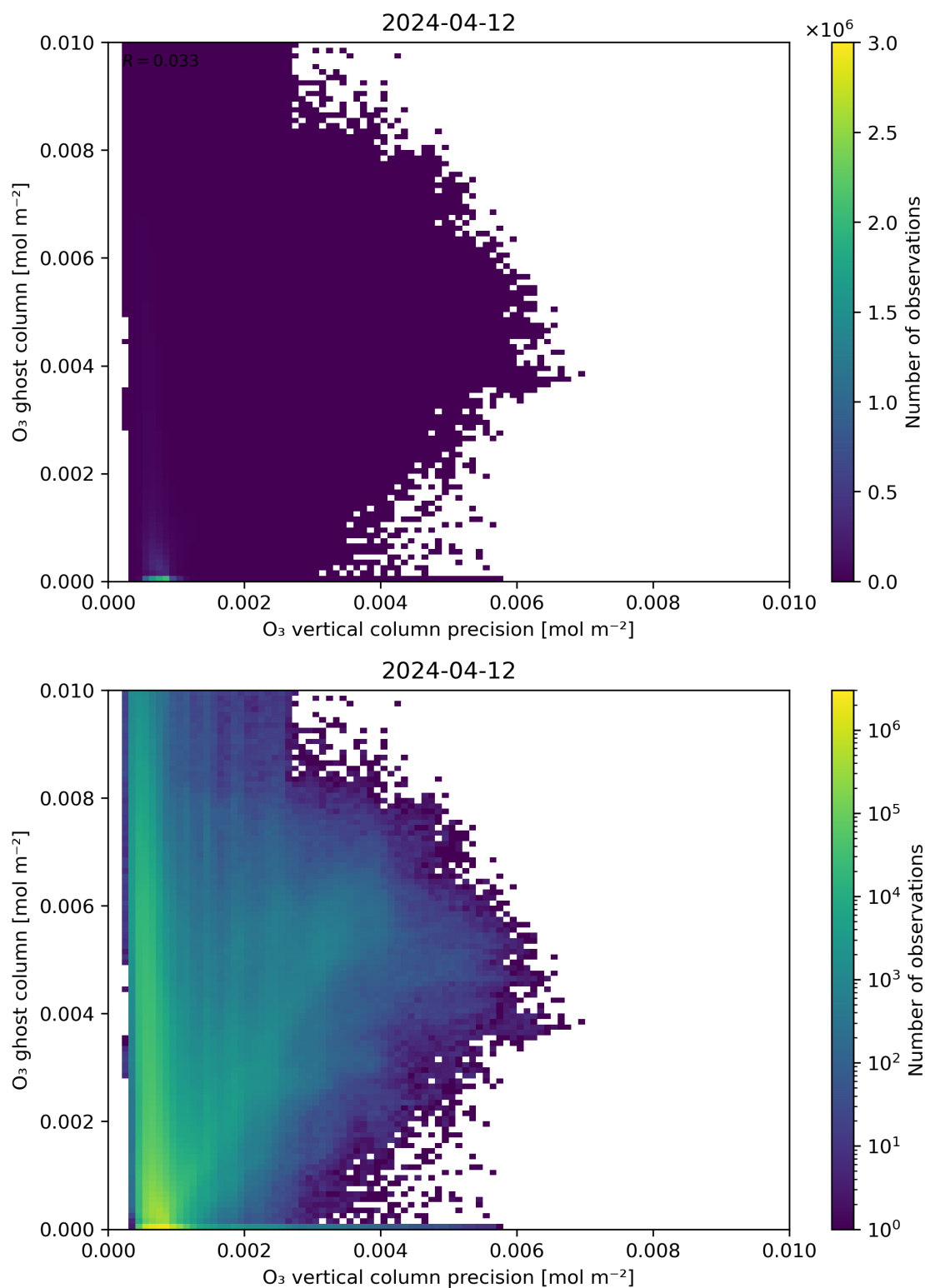
Figure 43: Scatter density plot of “ O_3 vertical column precision” against “ O_3 ghost column” for 2024-04-11 to 2024-04-13.
