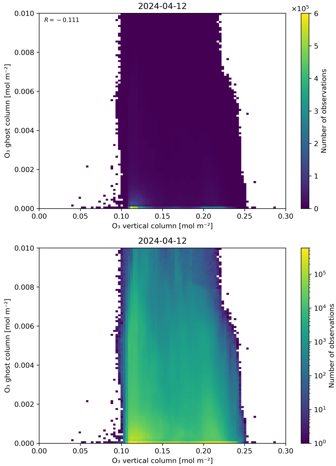
Figure 40: Scatter density plot of “O 3 vertical column” against “O 3 ghost column” for 2024-04-11 to 2024-04-13.
