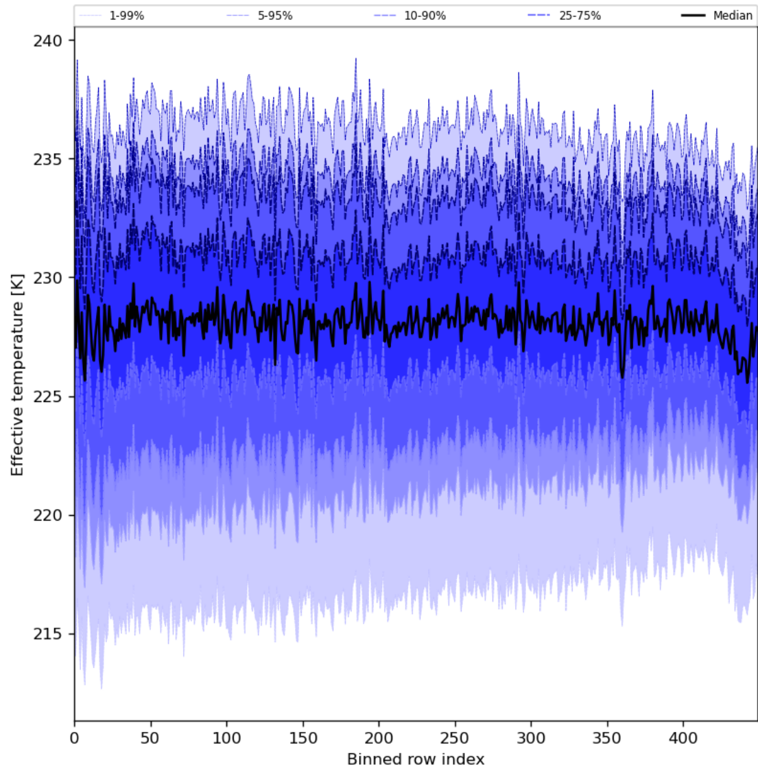
Figure 31: Along track statistics of “Effective temperature” for 2024-04-11 to 2024-04-13
