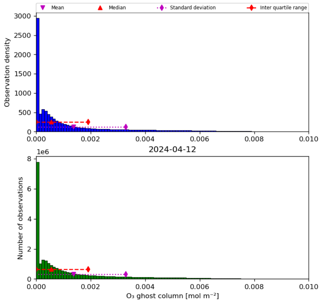
Figure 25: Histogram of “O 3 ghost column” for 2024-04-11 to 2024-04-13
