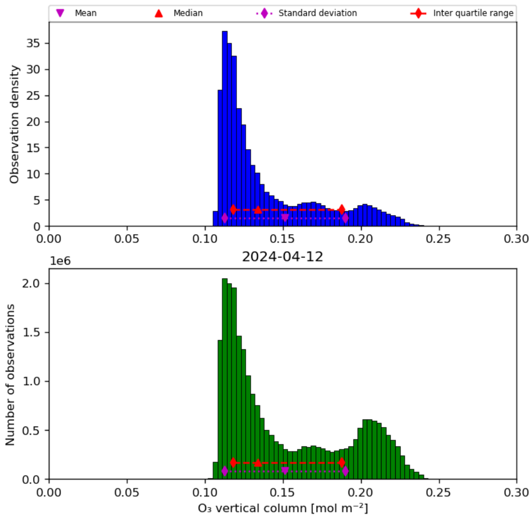
Figure 21: Histogram of “O 3 vertical column” for 2024-04-11 to 2024-04-13
