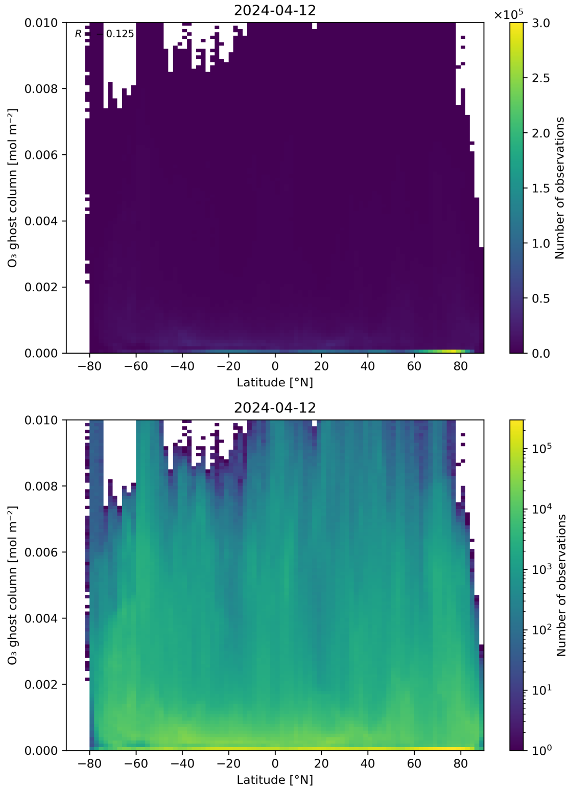
Figure 35: Scatter density plot of “Latitude” against “O 3 ghost column” for 2024-04-11 to 2024-04-13.
