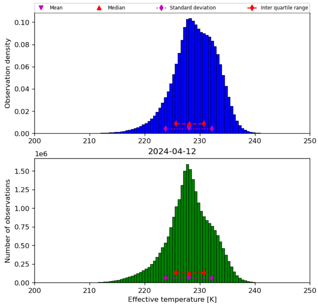
Figure 24: Histogram of “Effective temperature” for 2024-04-11 to 2024-04-13
