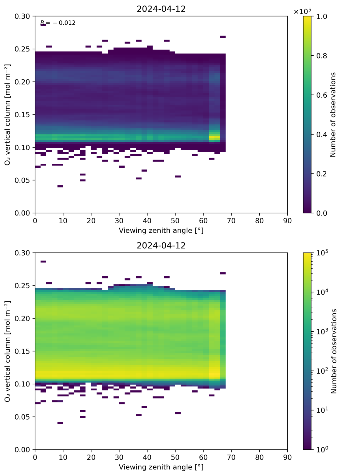
Figure 52: Scatter density plot of “Viewing zenith angle” against “O 3 vertical column” for 2024-04-11 to 2024-04-13.
