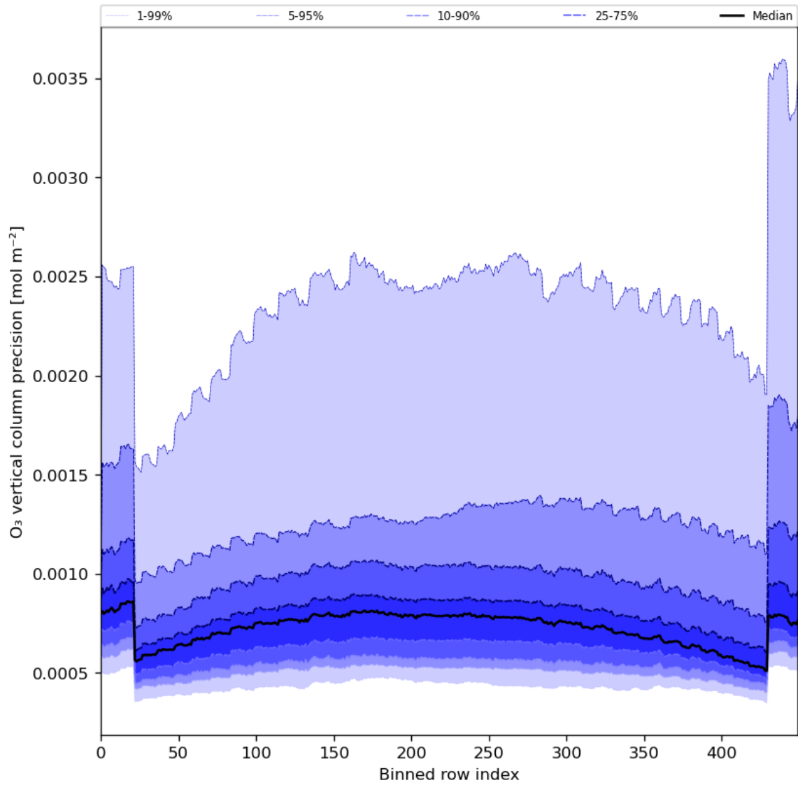
Figure 29: Along track statistics of “O 3 vertical column precision” for 2024-04-11 to 2024-04-13
