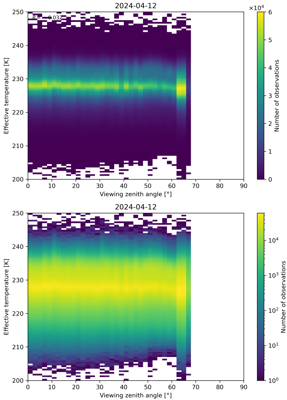
Figure 50: Scatter density plot of “Viewing zenith angle” against “Effective temperature” for 2024-04-11 to 2024-04-13.
