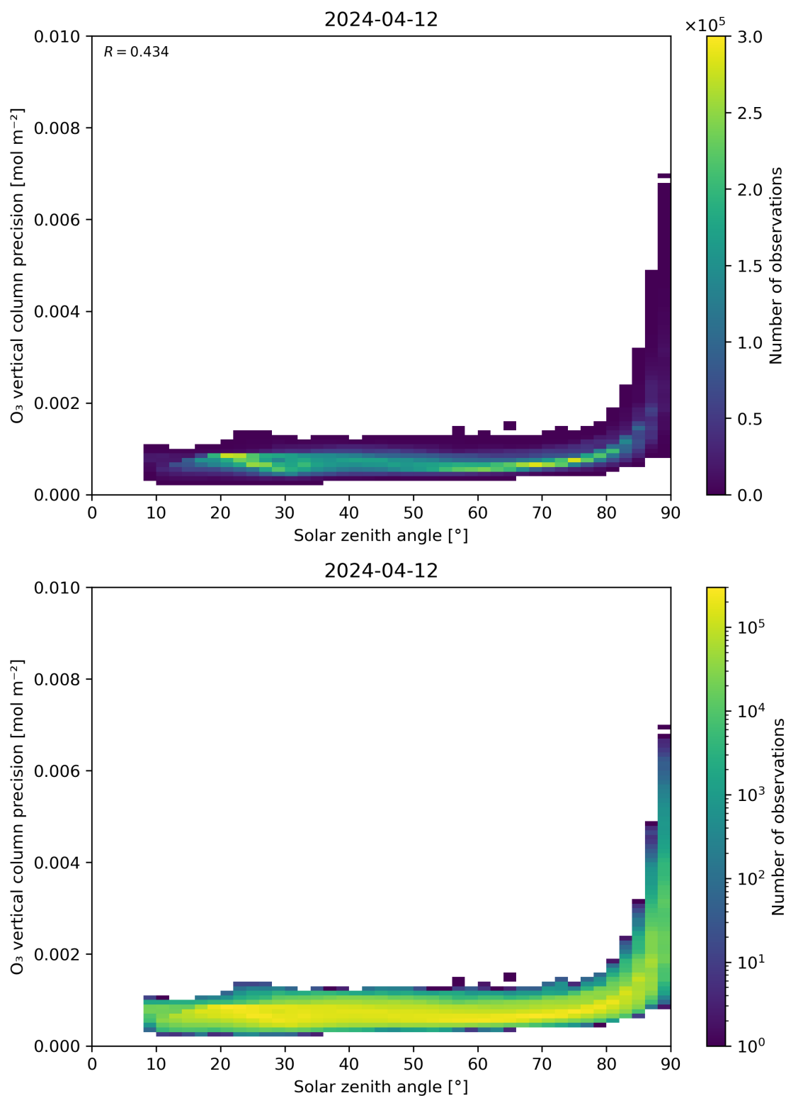
Figure 48: Scatter density plot of “Solar zenith angle” against “O 3 vertical column precision” for 2024-04-11 to 2024-04-13.
