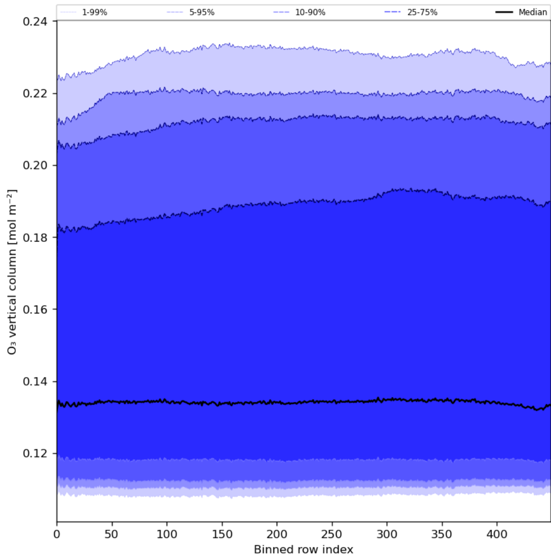
Figure 28: Along track statistics of “O 3 vertical column” for 2024-04-11 to 2024-04-13
