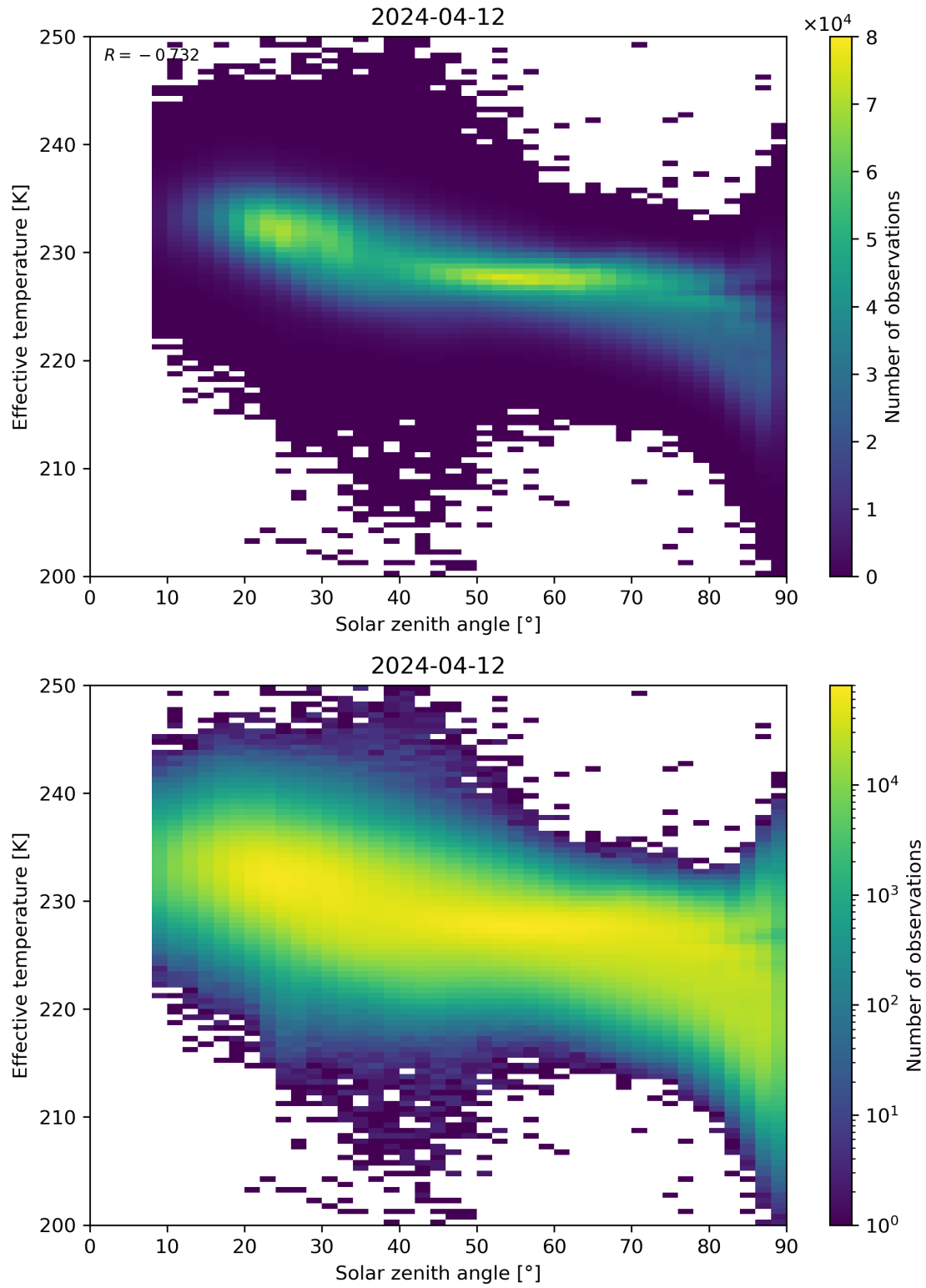
Figure 45: Scatter density plot of “Solar zenith angle” against “Effective temperature” for 2024-04-11 to 2024-04-13.
