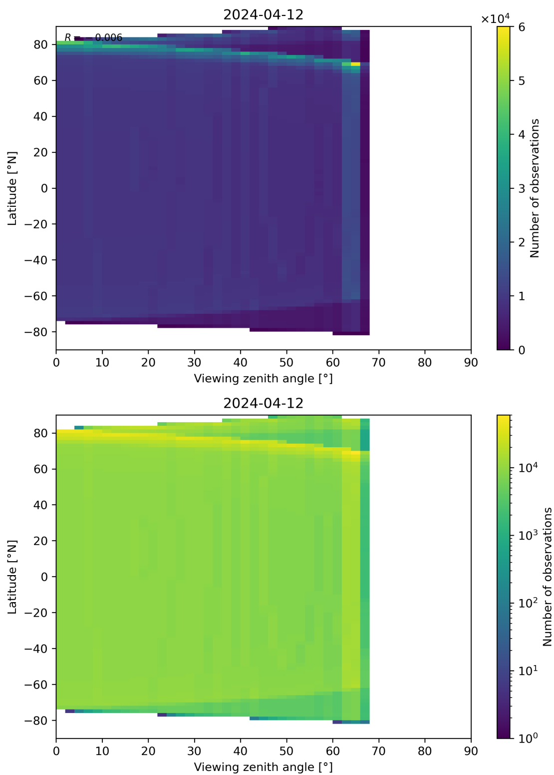
Figure 49: Scatter density plot of “Viewing zenith angle” against “Latitude” for 2024-04-11 to 2024-04-13.
