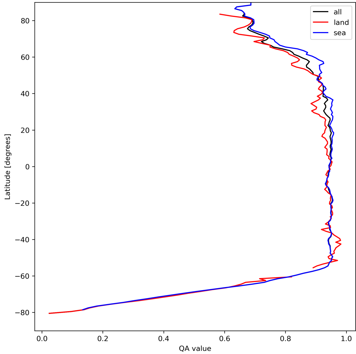
Figure 13: Zonal average of “QA value” for 2024-04-11 to 2024-04-13.
