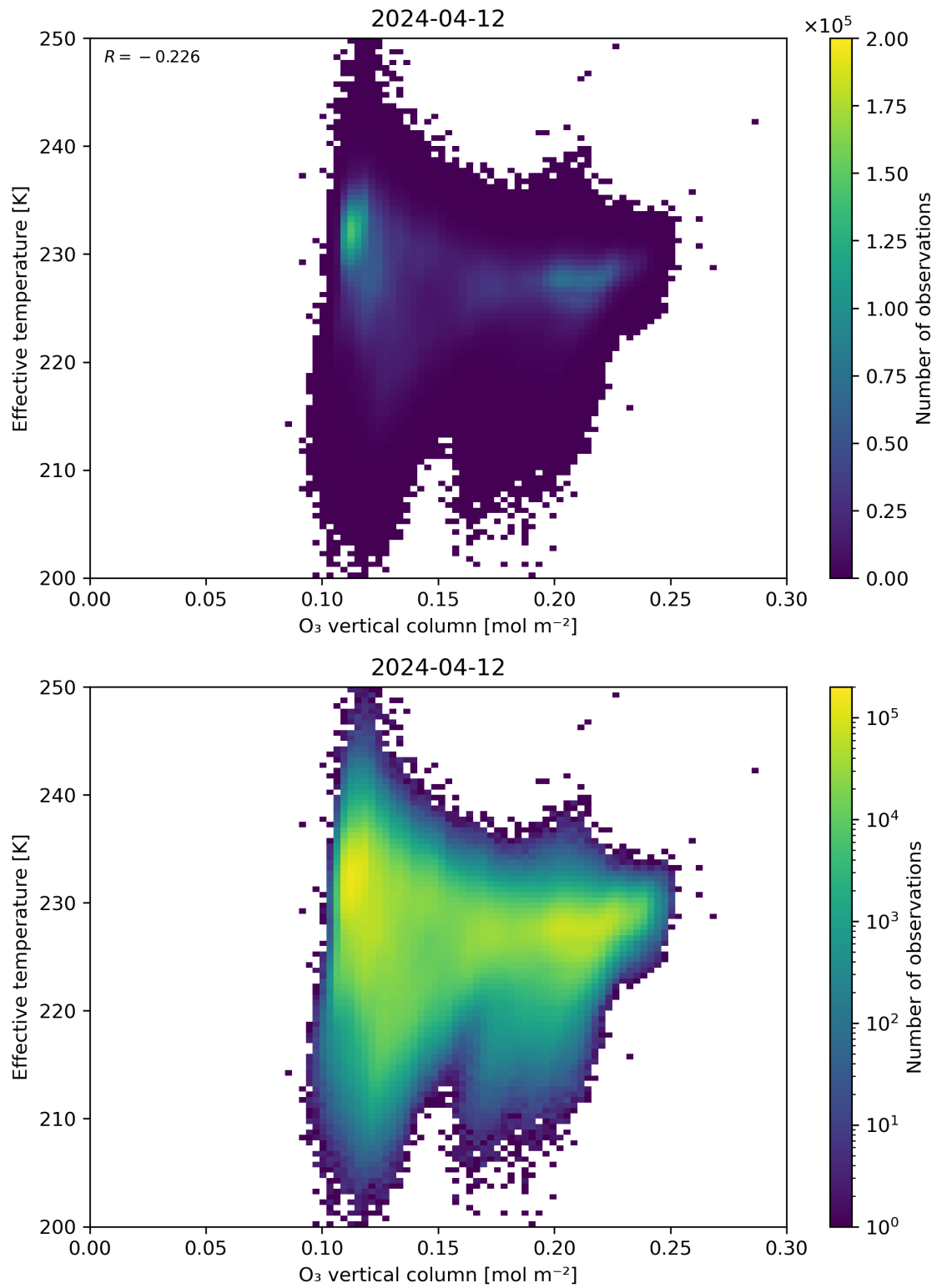
Figure 39: Scatter density plot of “O 3 vertical column” against “Effective temperature” for 2024-04-11 to 2024-04-13.
