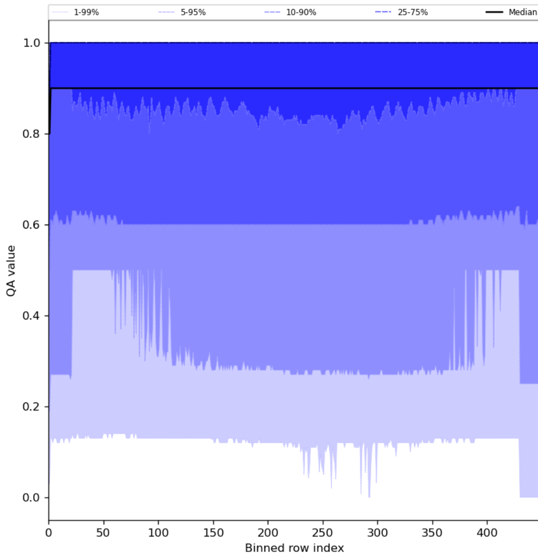
Figure 27: Along track statistics of “QA value” for 2024-04-12 to 2024-04-14
