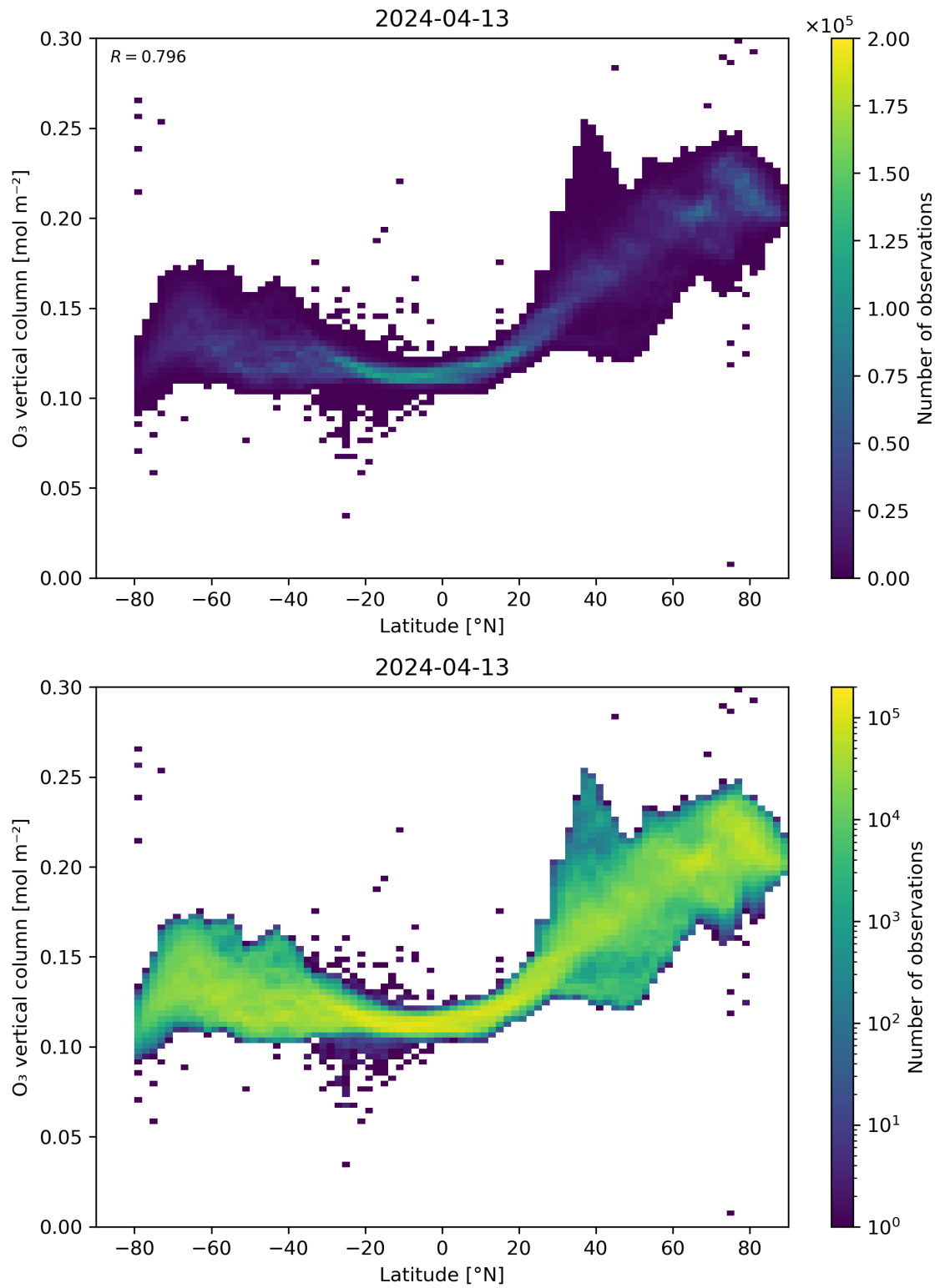
Figure 36: Scatter density plot of “Latitude” against “O 3 vertical column” for 2024-04-12 to 2024-04-14.
