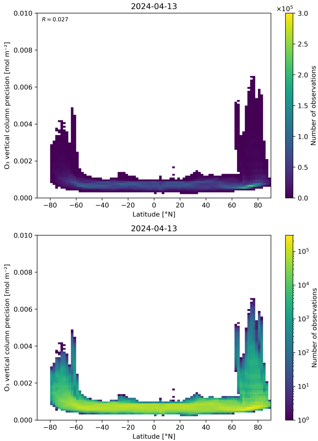
Figure 37: Scatter density plot of “Latitude” against “O 3 vertical column precision” for 2024-04-12 to 2024-04-14.
