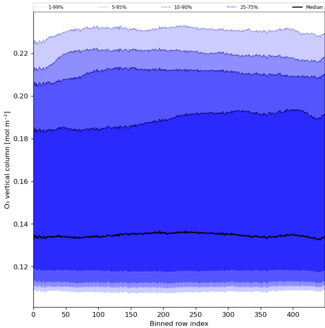
Figure 28: Along track statistics of “O 3 vertical column” for 2024-04-12 to 2024-04-14
