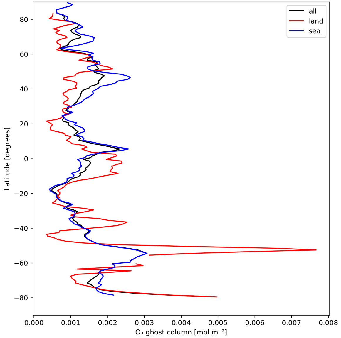
Figure 18: Zonal average of "O 3 ghost column" for 2024-04-12 to 2024-04-14.
