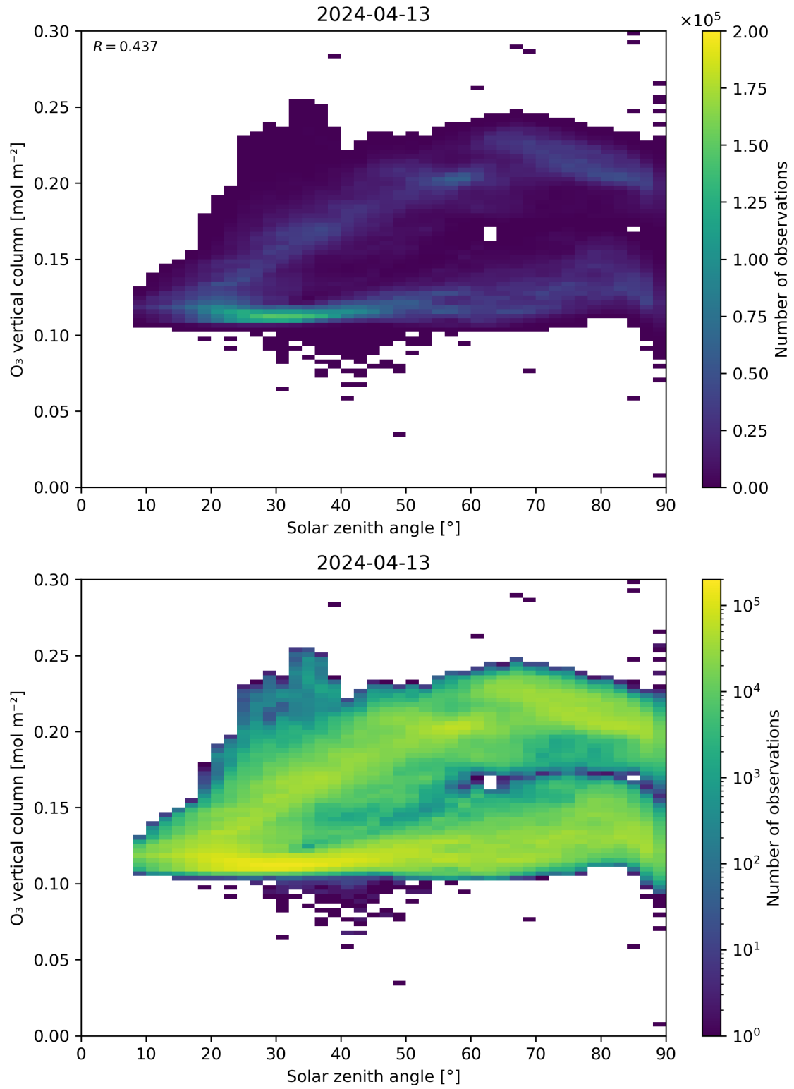
Figure 47: Scatter density plot of “Solar zenith angle” against “O 3 vertical column” for 2024-04-12 to 2024-04-14.
