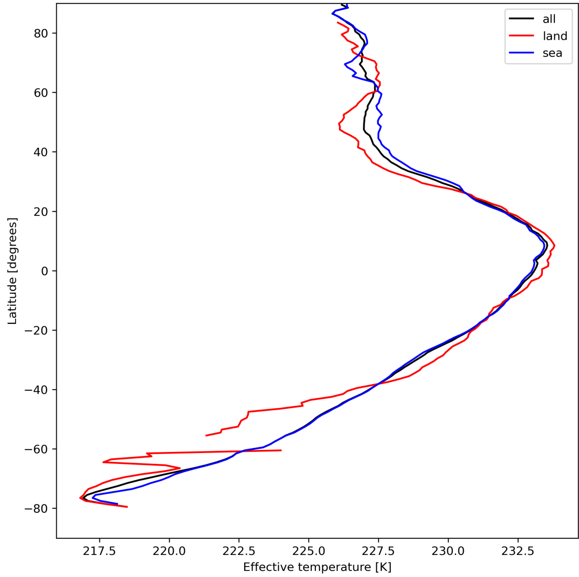
Figure 17: Zonal average of “Effective temperature” for 2024-04-12 to 2024-04-14.
