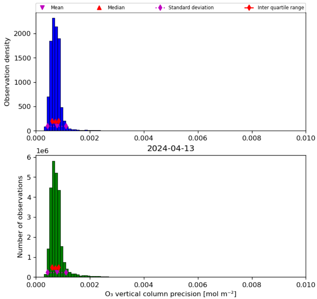
Figure 22: Histogram of “O 3 vertical column precision” for 2024-04-12 to 2024-04-14
