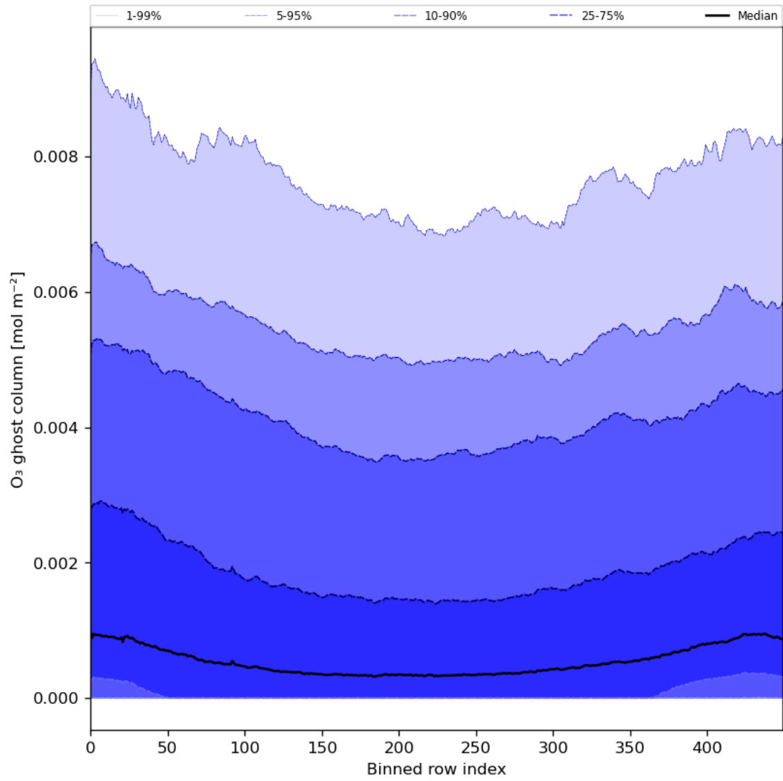
Figure 32: Along track statistics of “O 3 ghost column” for 2024-04-12 to 2024-04-14
