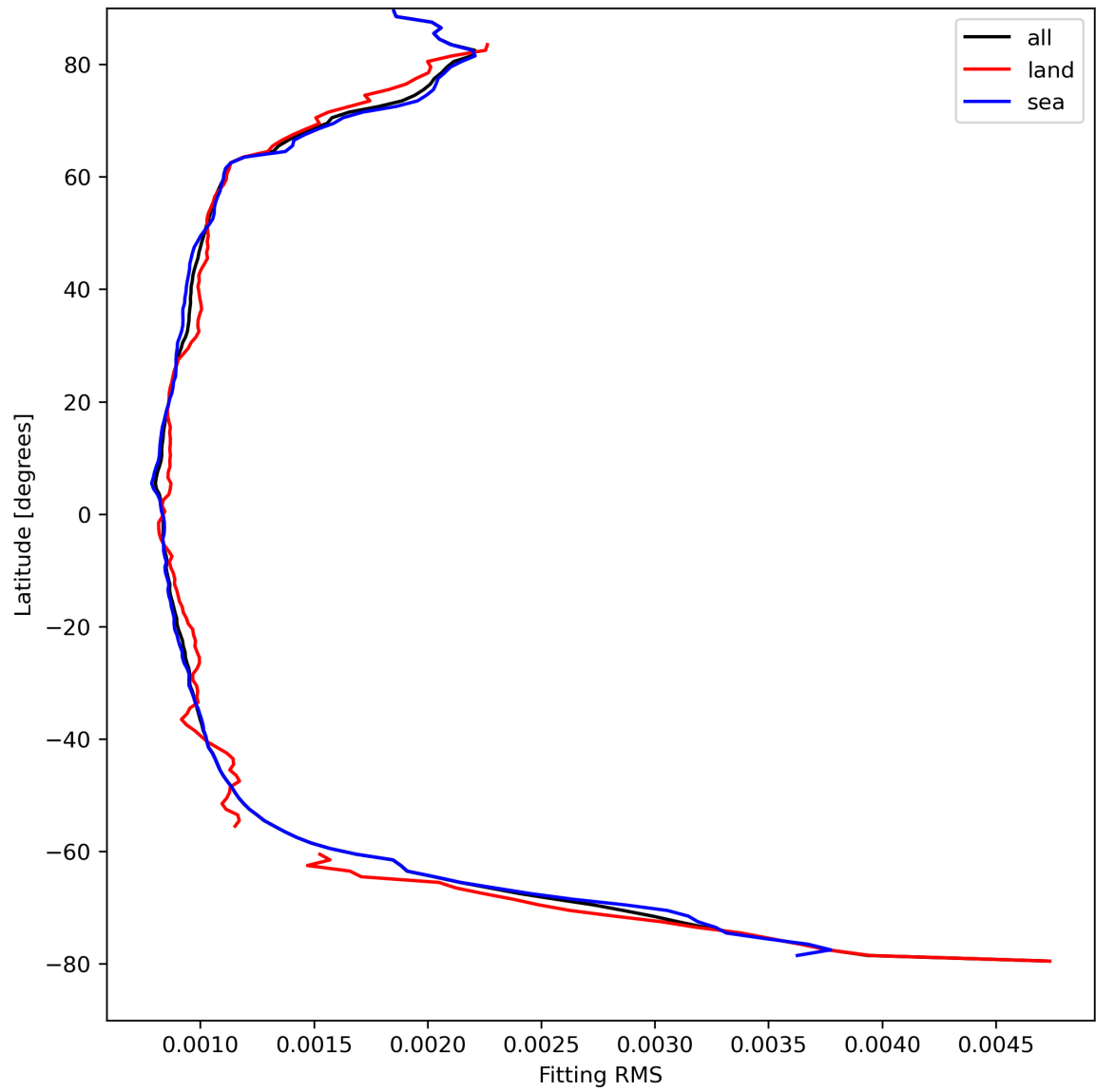
Figure 16: Zonal average of “Fitting RMS” for 2024-04-12 to 2024-04-14.
