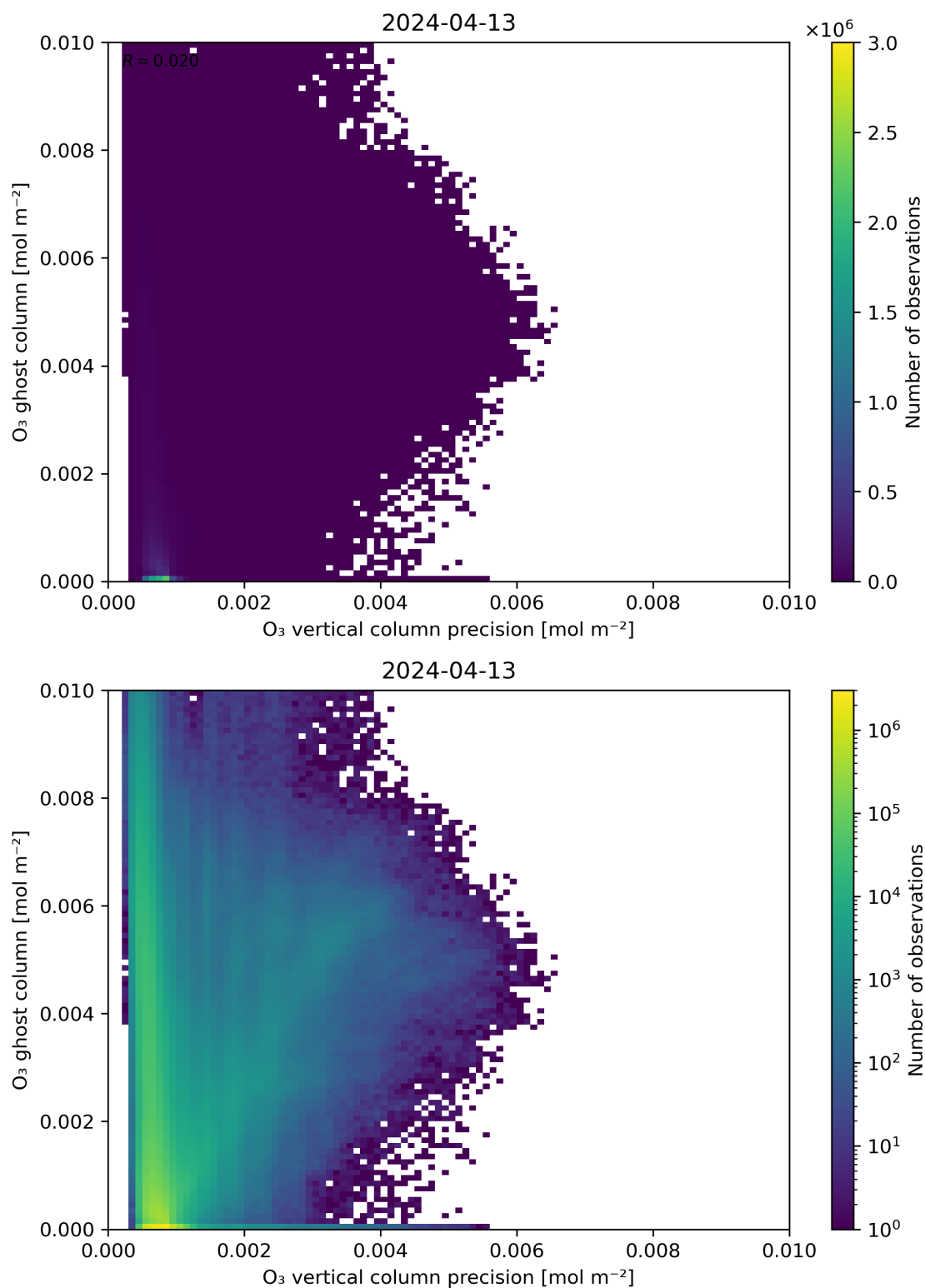
Figure 43: Scatter density plot of “ O_3 vertical column precision” against “ O_3 ghost column” for 2024-04-12 to 2024-04-14.
