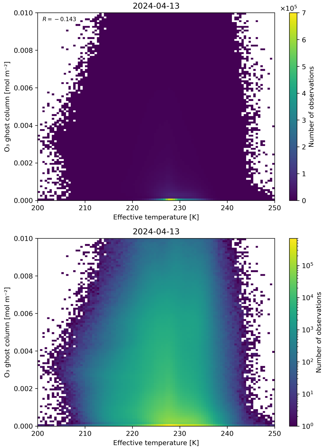
Figure 38: Scatter density plot of “Effective temperature” against “O 3 ghost column” for 2024-04-12 to 2024-04-14.
