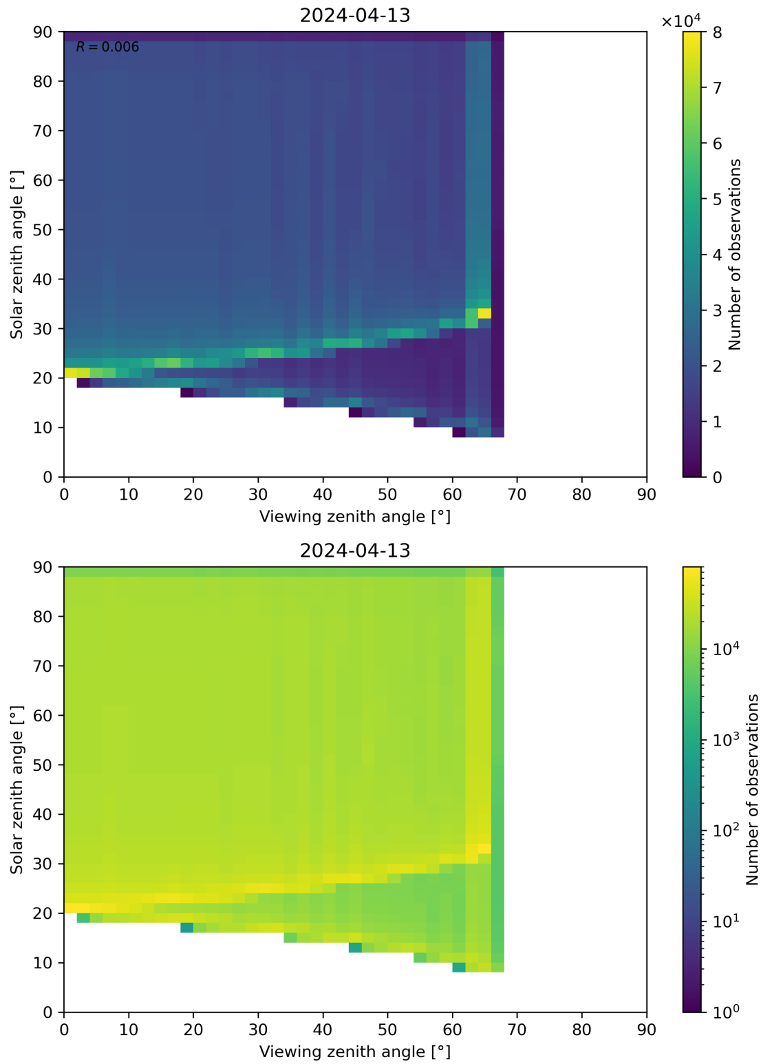
Figure 54: Scatter density plot of “Viewing zenith angle” against “Solar zenith angle” for 2024-04-12 to 2024-04-14.
