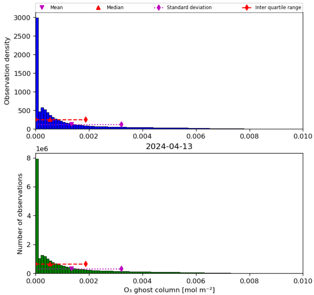
Figure 25: Histogram of “O 3 ghost column” for 2024-04-12 to 2024-04-14
