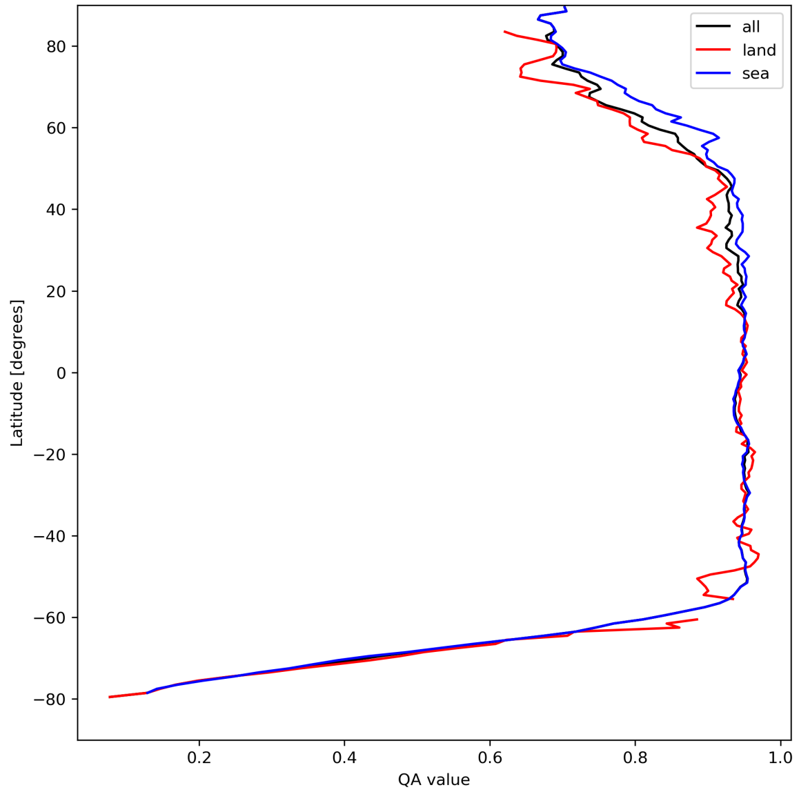
Figure 13: Zonal average of “QA value” for 2024-04-12 to 2024-04-14.
