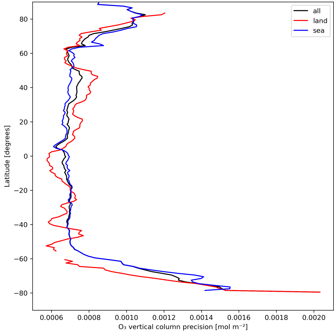
Figure 15: Zonal average of “O 3 vertical column precision” for 2024-04-12 to 2024-04-14.
