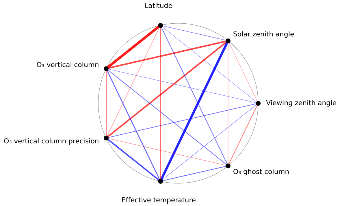
Figure 1: Map of correlation graph for 2024-04-12 to 2024-04-14.
