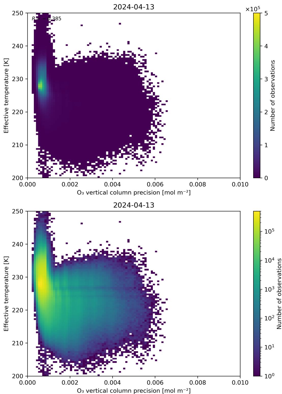
Figure 42: Scatter density plot of “O 3 vertical column precision” against “Effective temperature” for 2024-04-12 to 2024-04-14.
