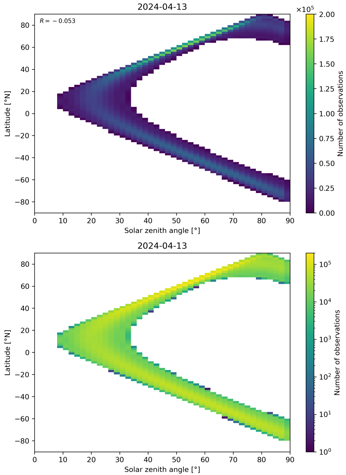
Figure 44: Scatter density plot of “Solar zenith angle” against “Latitude” for 2024-04-12 to 2024-04-14.
