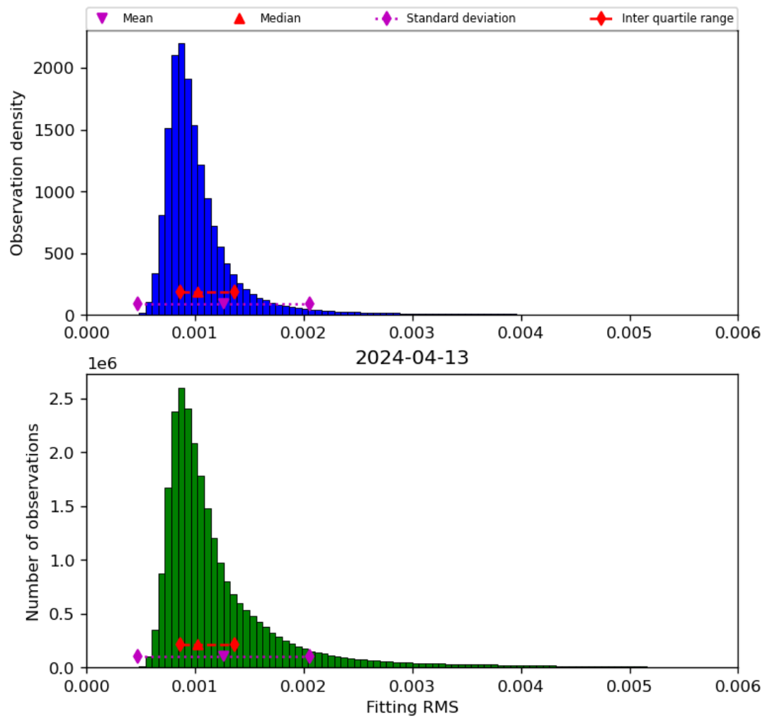
Figure 23: Histogram of "Fitting RMS" for 2024-04-12 to 2024-04-14
