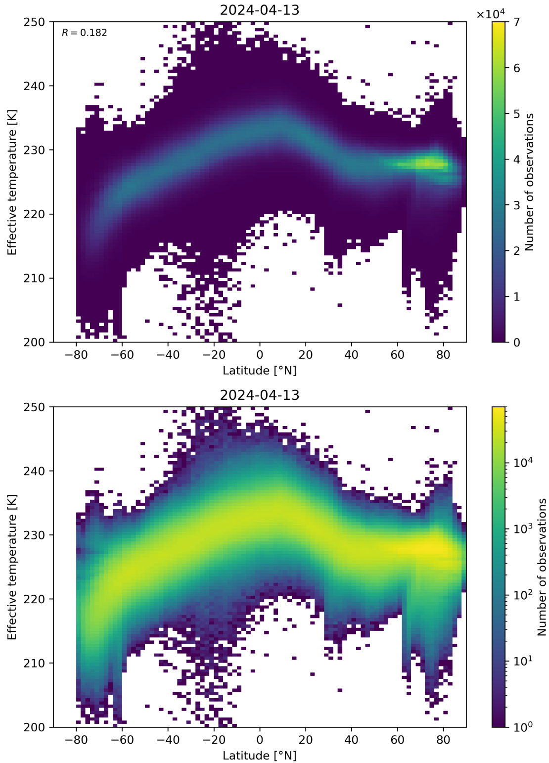
Figure 34: Scatter density plot of “Latitude” against “Effective temperature” for 2024-04-12 to 2024-04-14.
