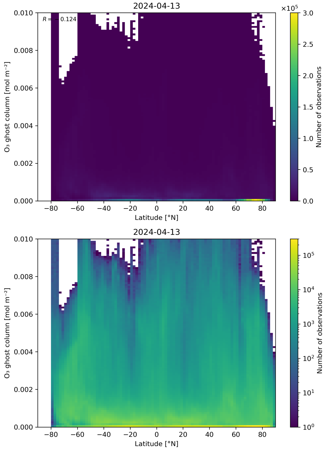
Figure 35: Scatter density plot of “Latitude” against “O 3 ghost column” for 2024-04-12 to 2024-04-14.
