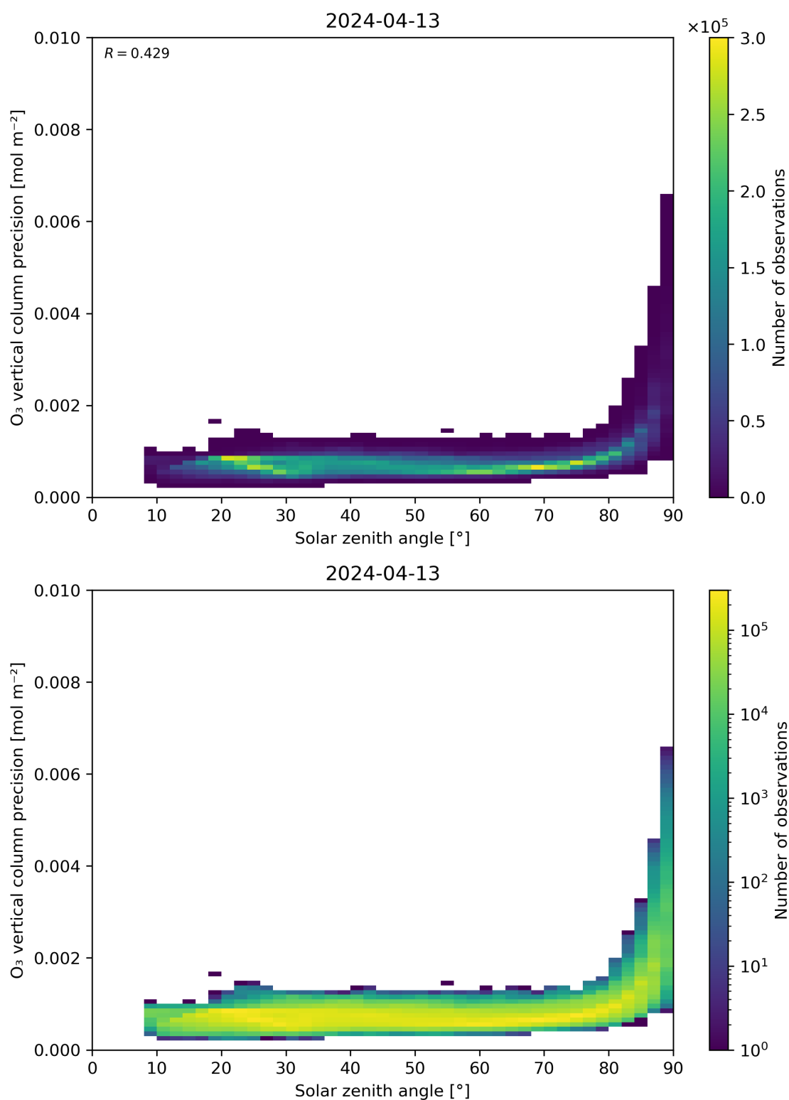
Figure 48: Scatter density plot of “Solar zenith angle” against “O 3 vertical column precision” for 2024-04-12 to 2024-04-14.
