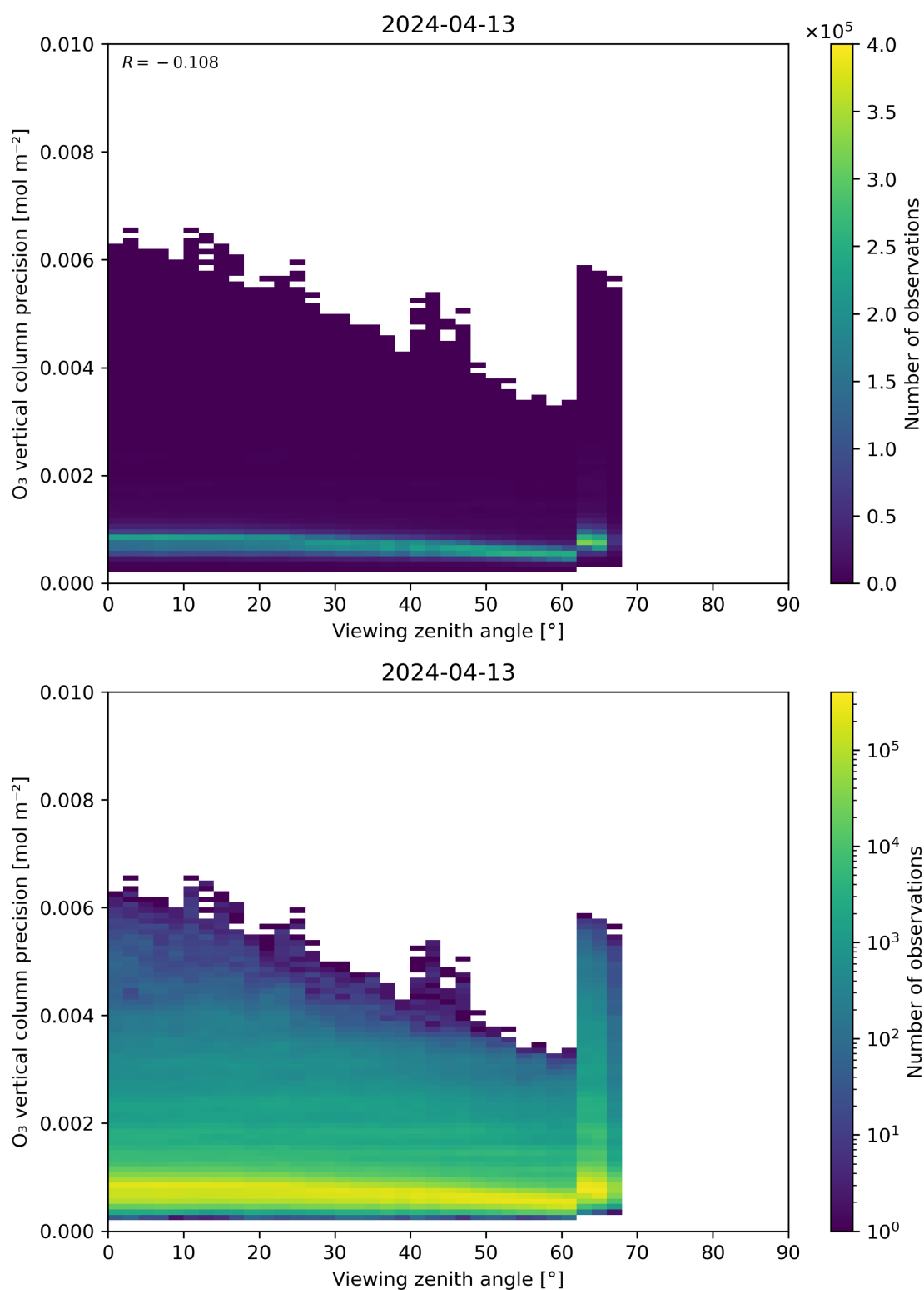
Figure 53: Scatter density plot of “Viewing zenith angle” against “O 3 vertical column precision” for 2024-04-12 to 2024-04-14.
