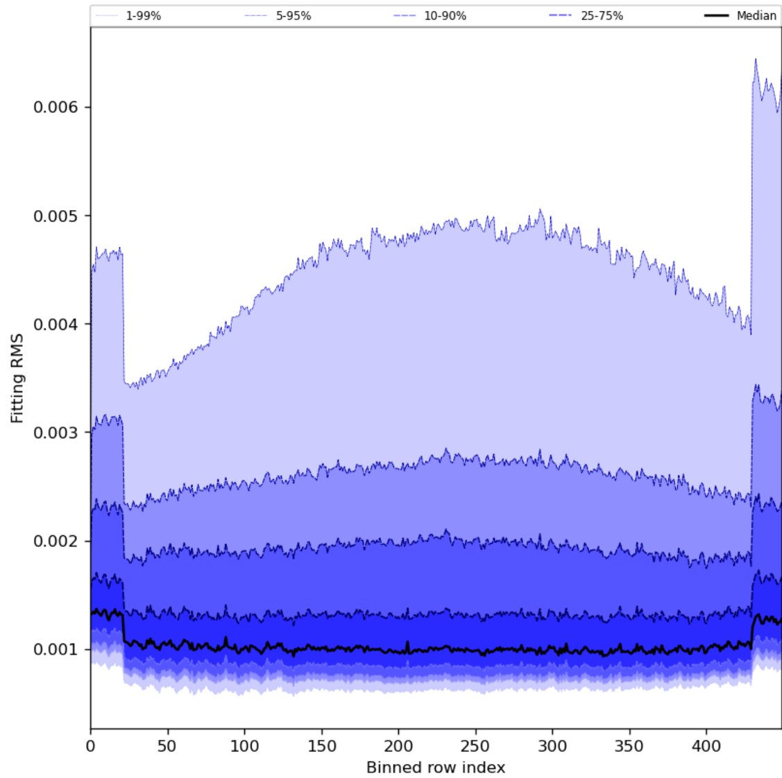
Figure 30: Along track statistics of “Fitting RMS” for 2024-04-12 to 2024-04-14
