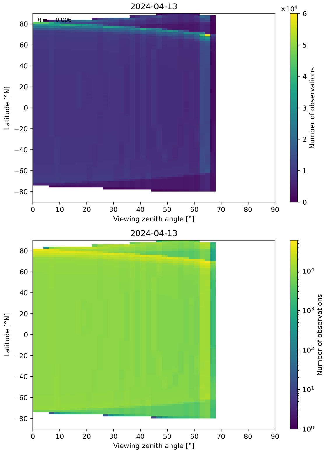
Figure 49: Scatter density plot of “Viewing zenith angle” against “Latitude” for 2024-04-12 to 2024-04-14.
