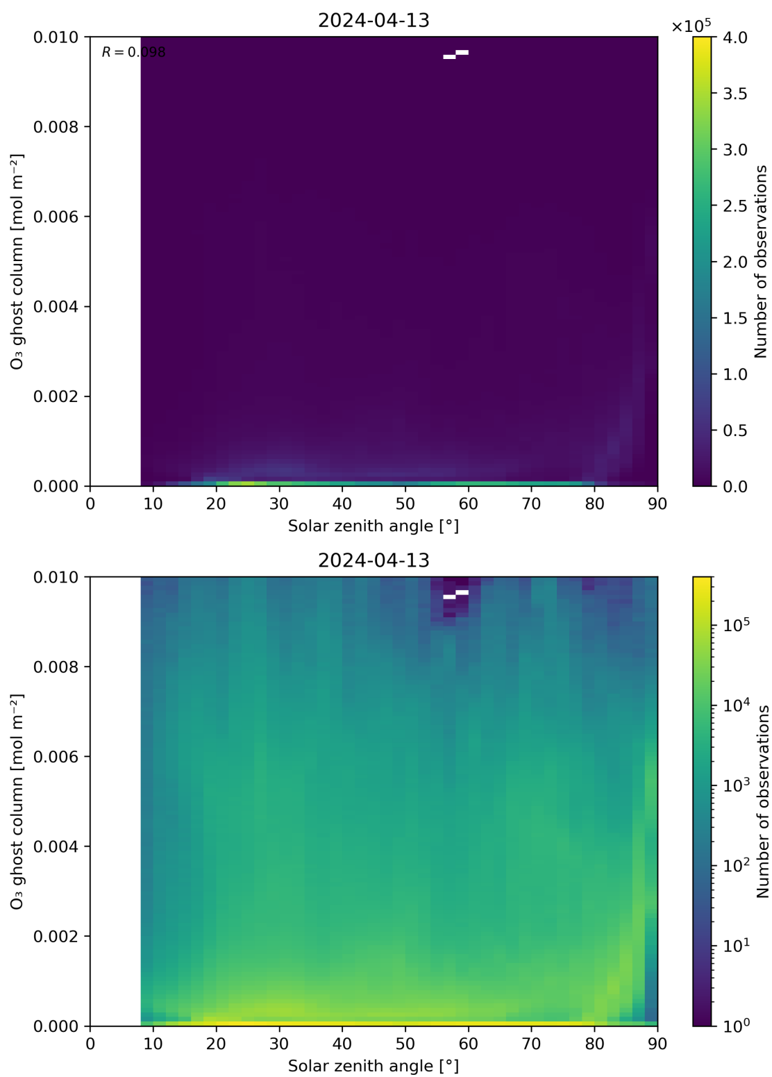
Figure 46: Scatter density plot of “Solar zenith angle” against “O 3 ghost column” for 2024-04-12 to 2024-04-14.
