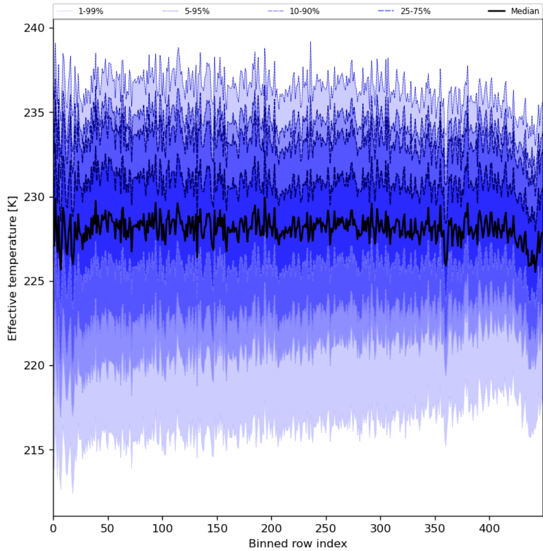
Figure 31: Along track statistics of “Effective temperature” for 2024-04-12 to 2024-04-14
