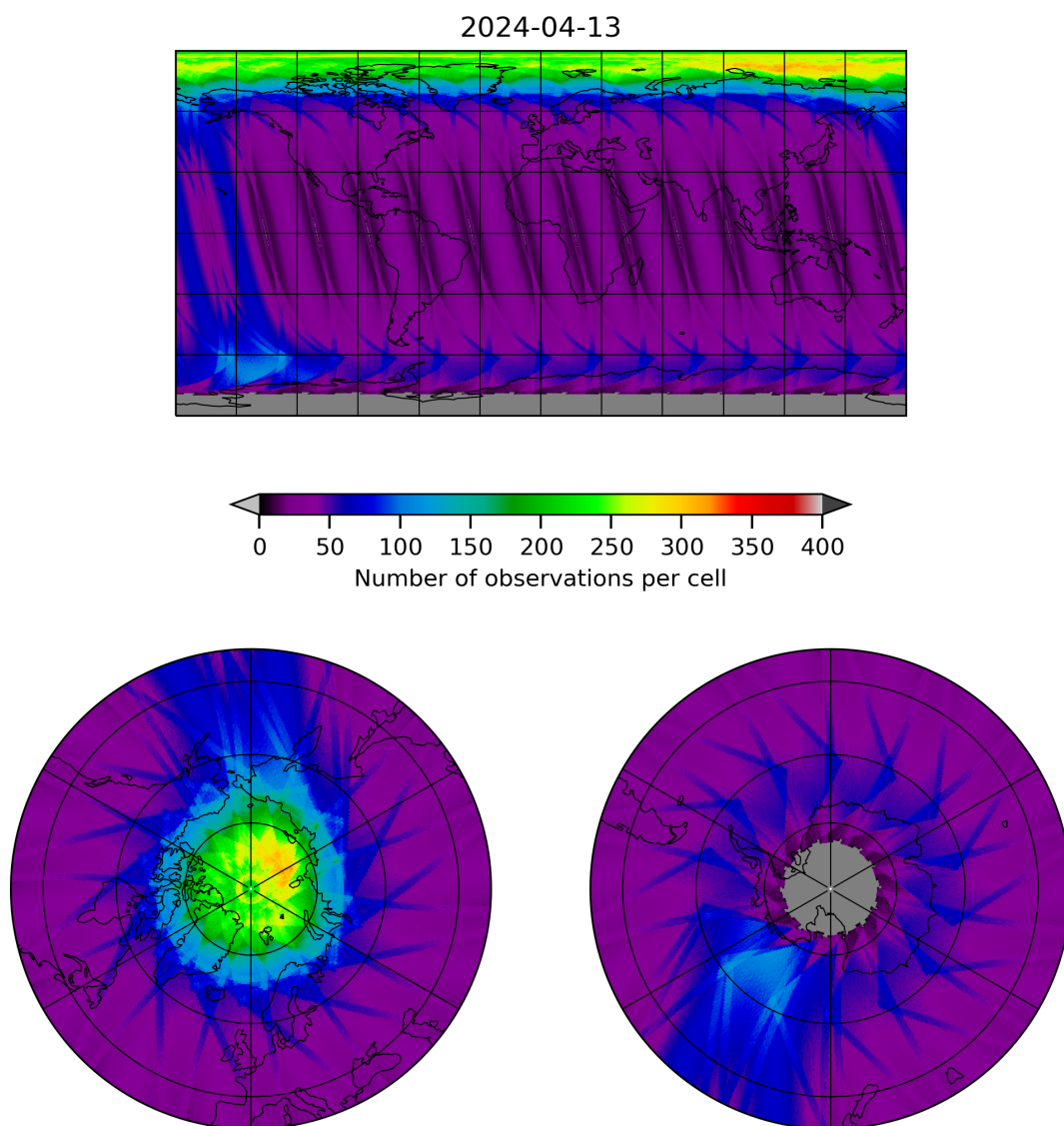
Figure 12: Map of the number of observations for 2024-04-12 to 2024-04-14
