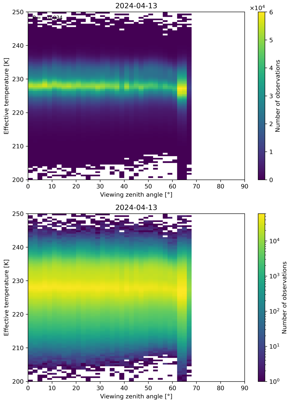
Figure 50: Scatter density plot of “Viewing zenith angle” against “Effective temperature” for 2024-04-12 to 2024-04-14.
