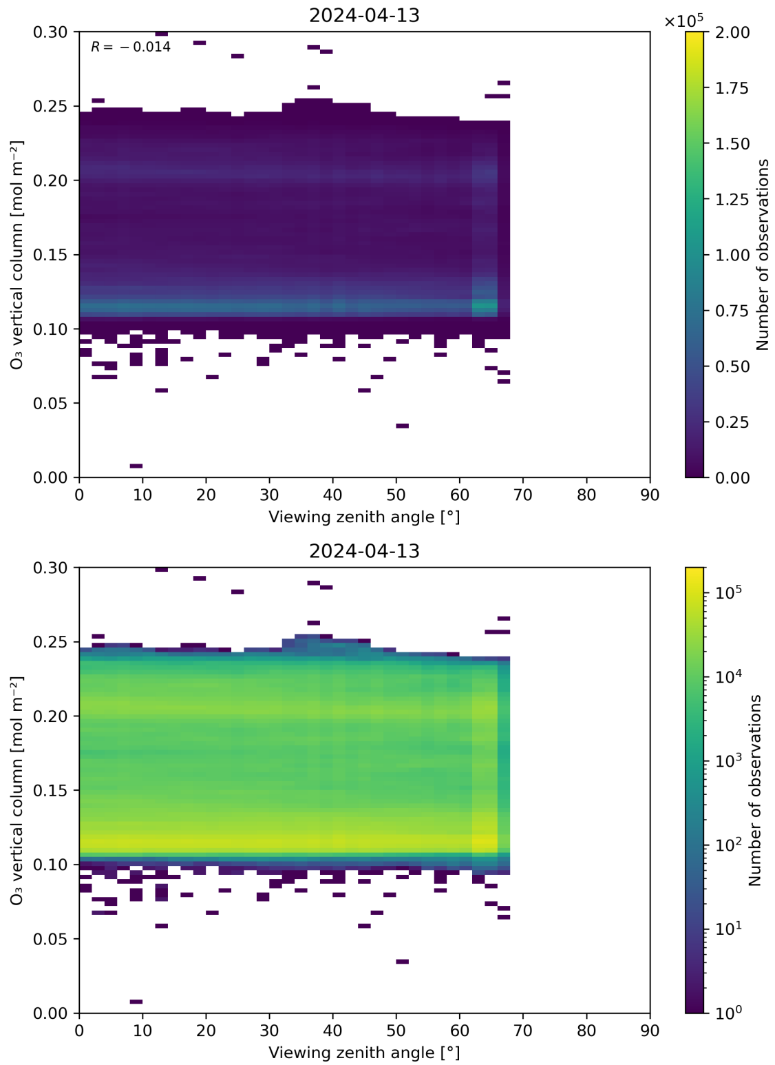
Figure 52: Scatter density plot of “Viewing zenith angle” against “O 3 vertical column” for 2024-04-12 to 2024-04-14.
