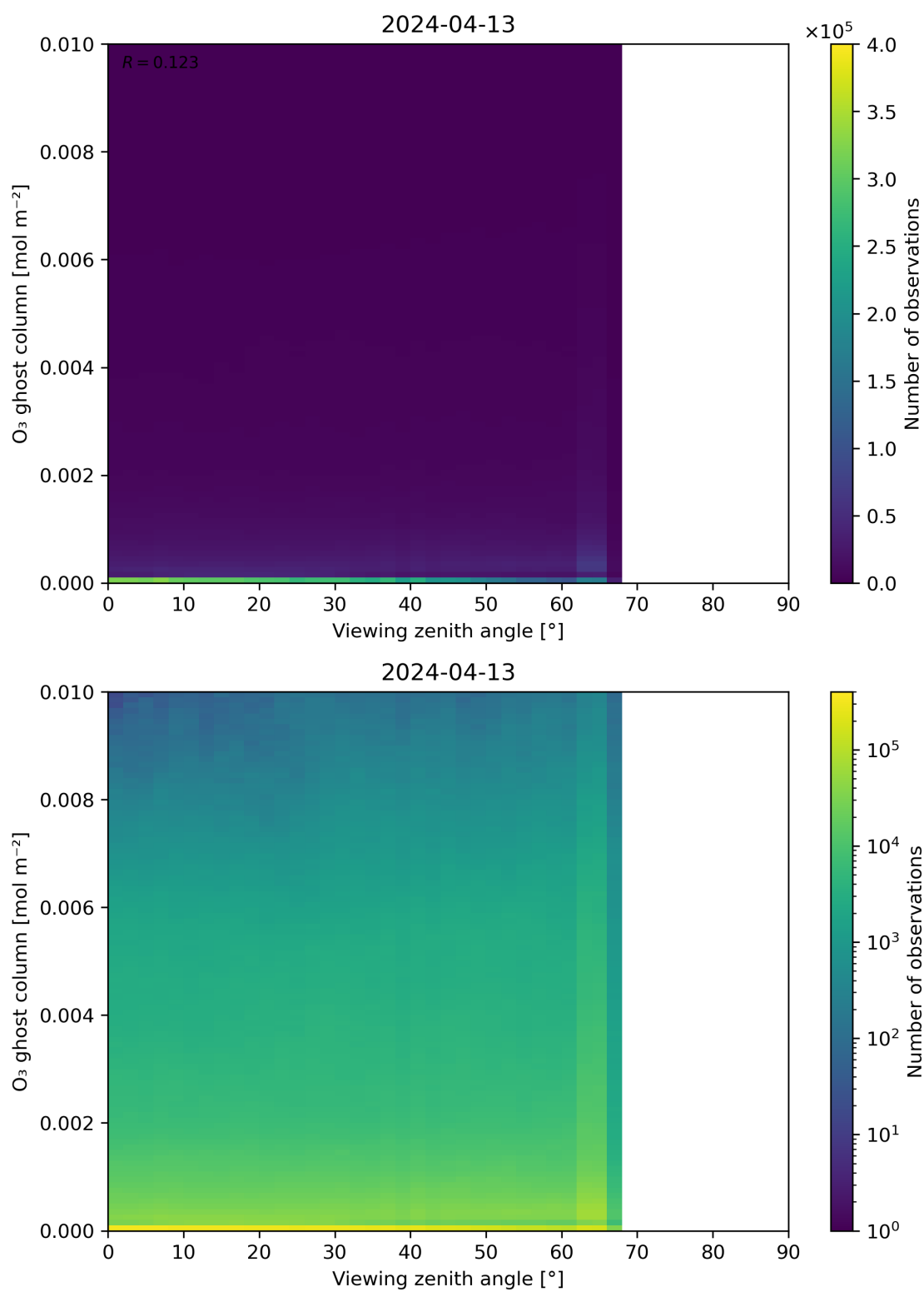
Figure 51: Scatter density plot of “Viewing zenith angle” against “O 3 ghost column” for 2024-04-12 to 2024-04-14.
