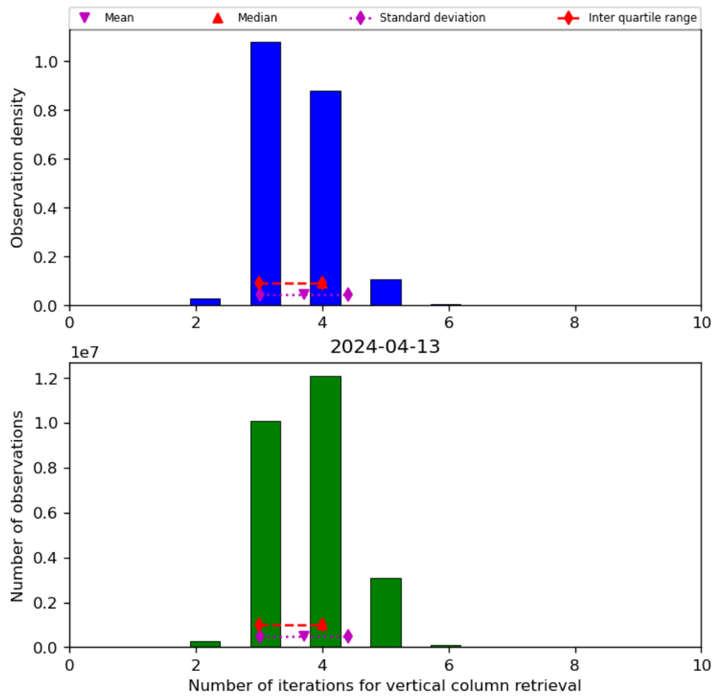
Figure 26: Histogram of “Number of iterations for vertical column retrieval” for 2024-04-12 to 2024-04-14
