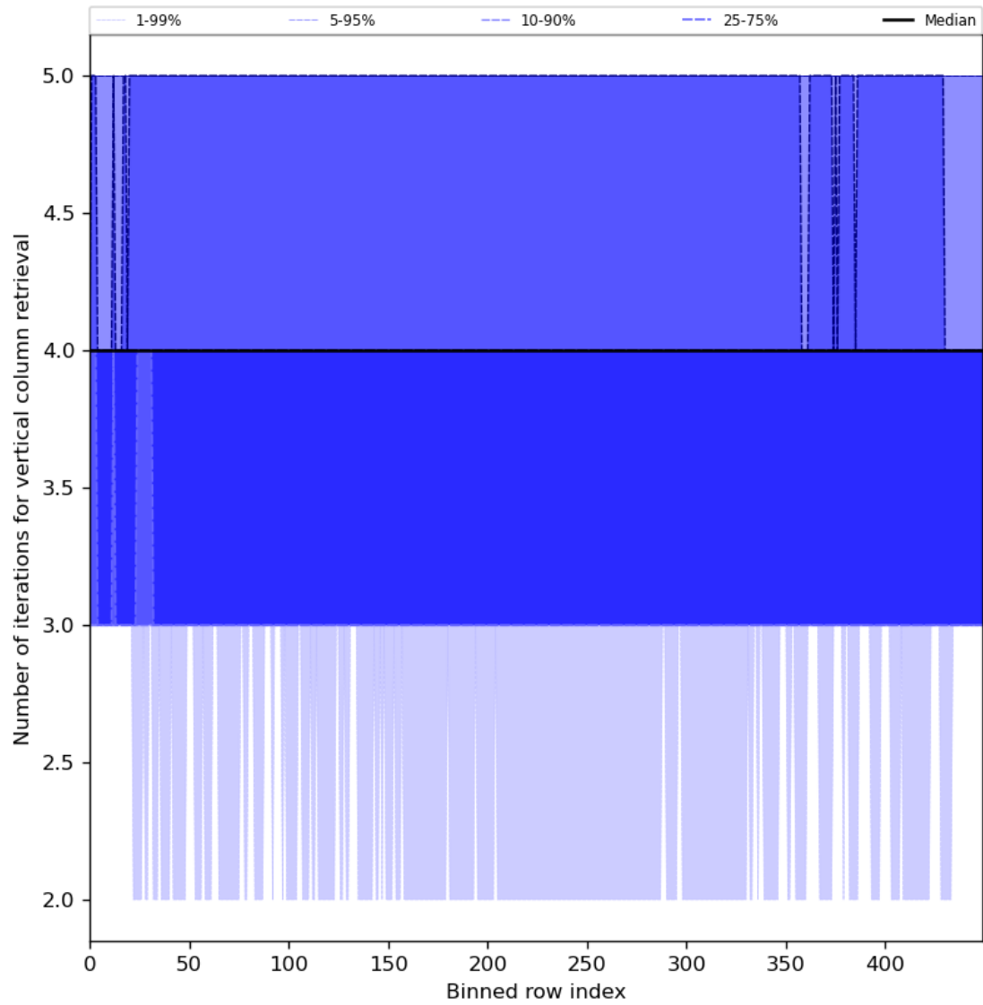
Figure 33: Along track statistics of “Number of iterations for vertical column retrieval” for 2024-04-12 to 2024-04-14
