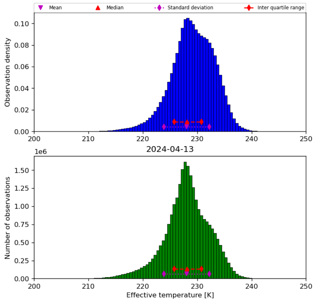
Figure 24: Histogram of “Effective temperature” for 2024-04-12 to 2024-04-14
