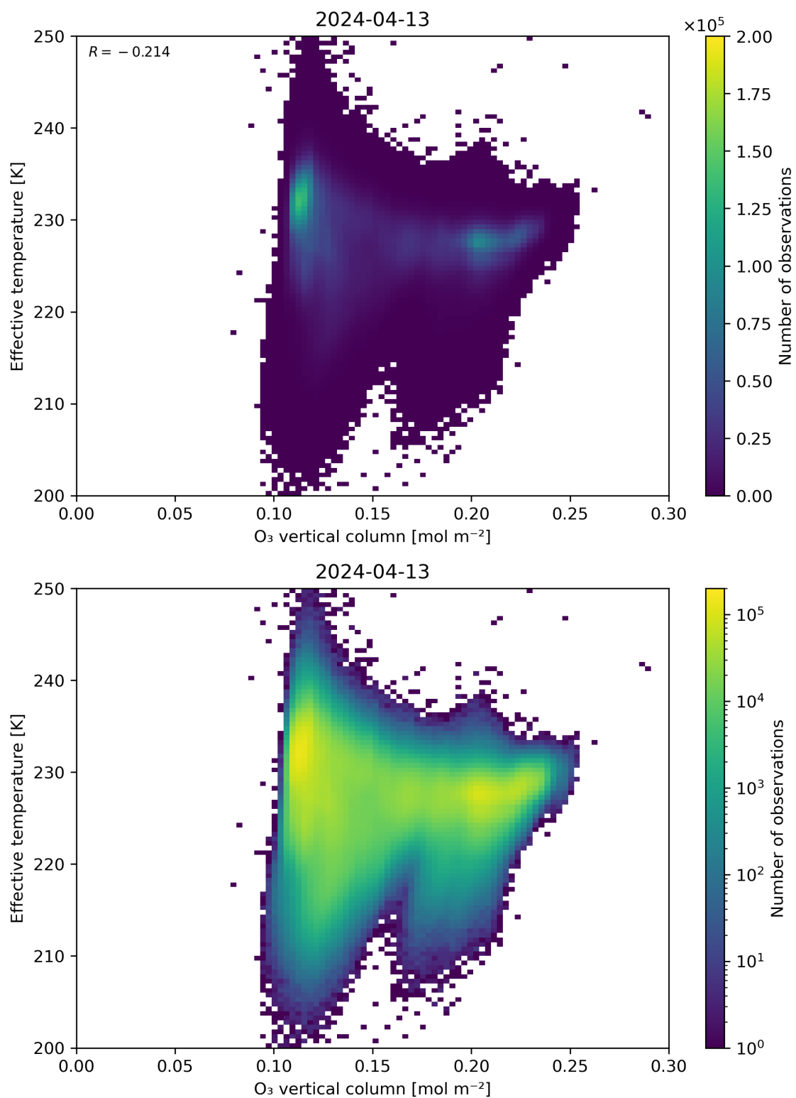
Figure 39: Scatter density plot of “O 3 vertical column” against “Effective temperature” for 2024-04-12 to 2024-04-14.
