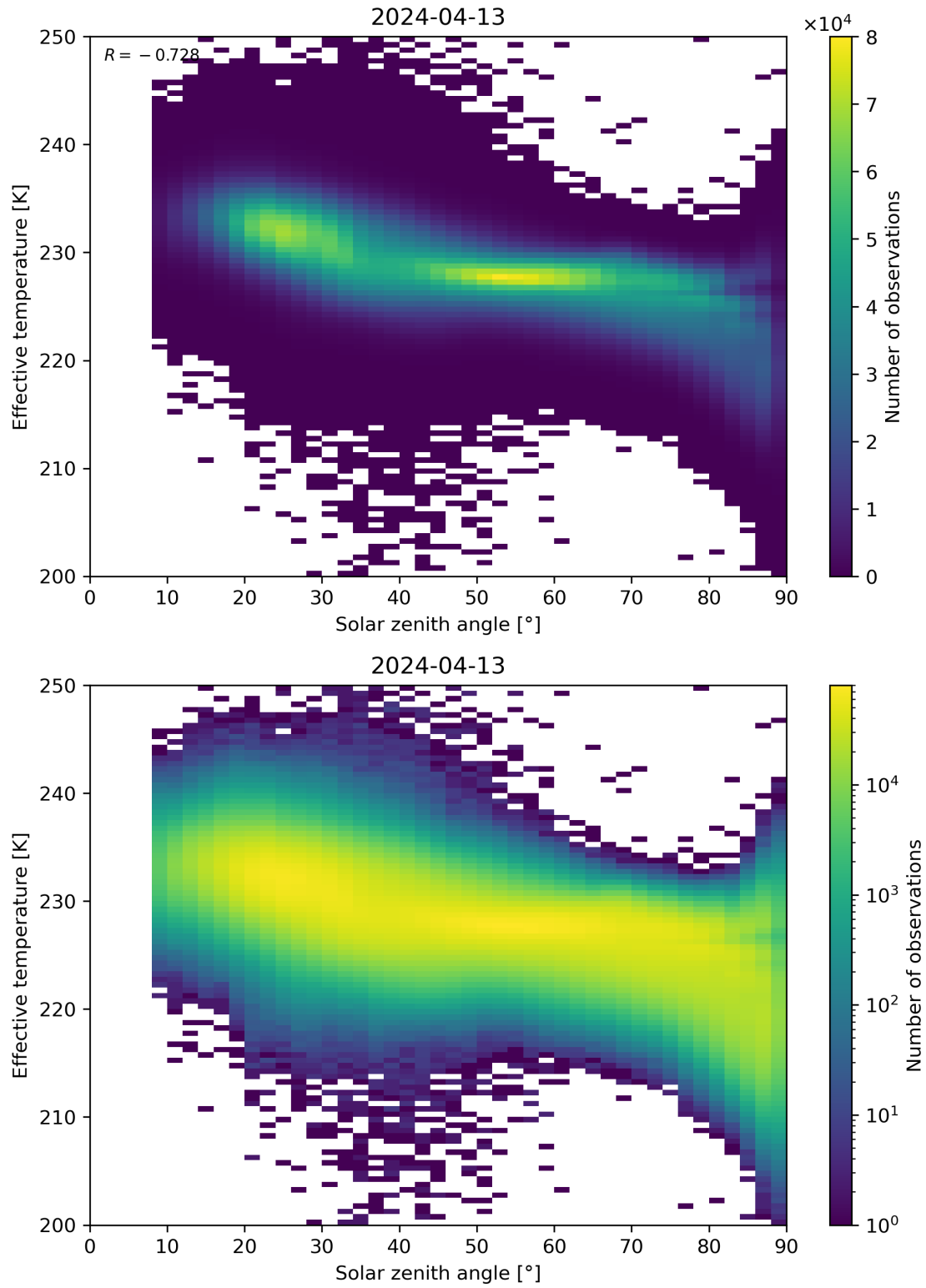
Figure 45: Scatter density plot of “Solar zenith angle” against “Effective temperature” for 2024-04-12 to 2024-04-14.
