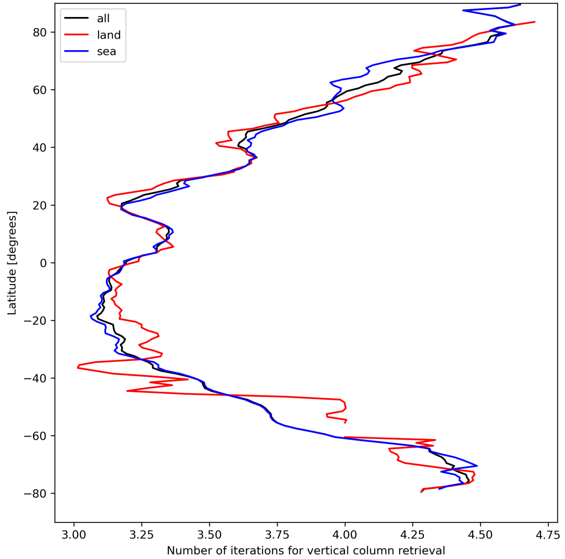
Figure 19: Zonal average of “Number of iterations for vertical column retrieval” for 2024-04-12 to 2024-04-14.
