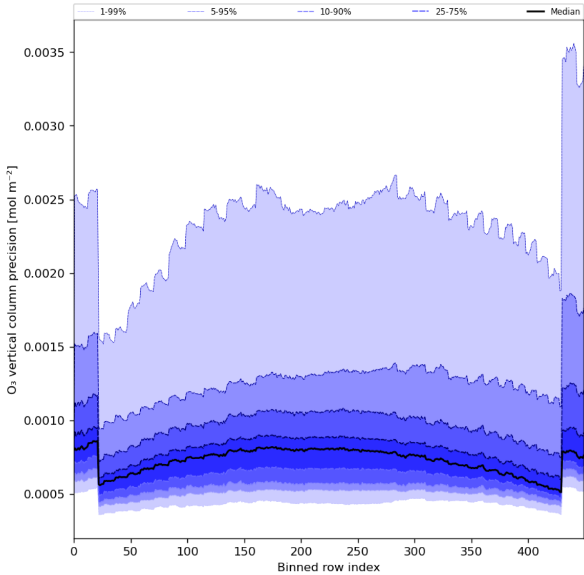
Figure 29: Along track statistics of “O 3 vertical column precision” for 2024-04-12 to 2024-04-14
