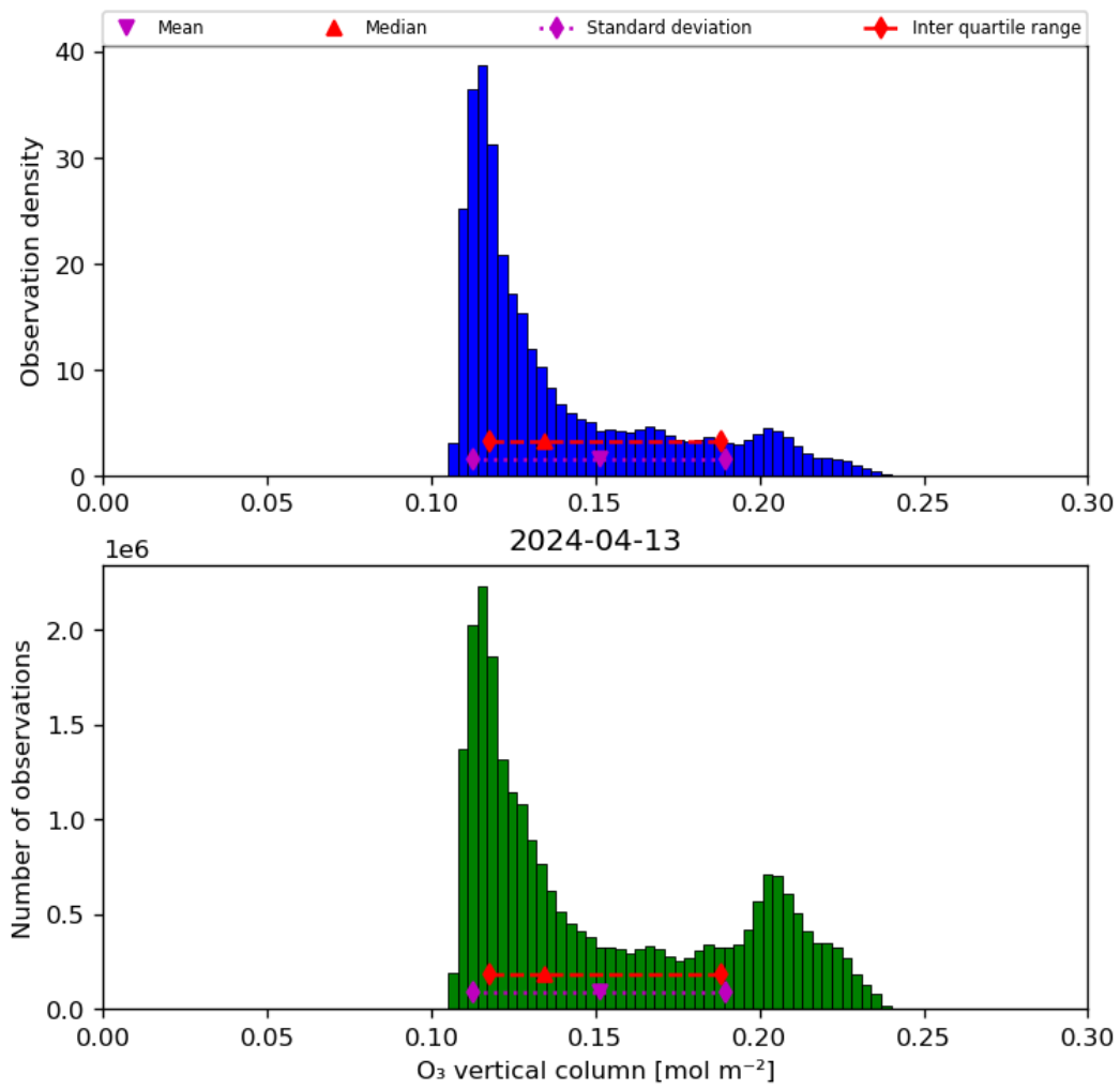
Figure 21: Histogram of “O 3 vertical column” for 2024-04-12 to 2024-04-14
