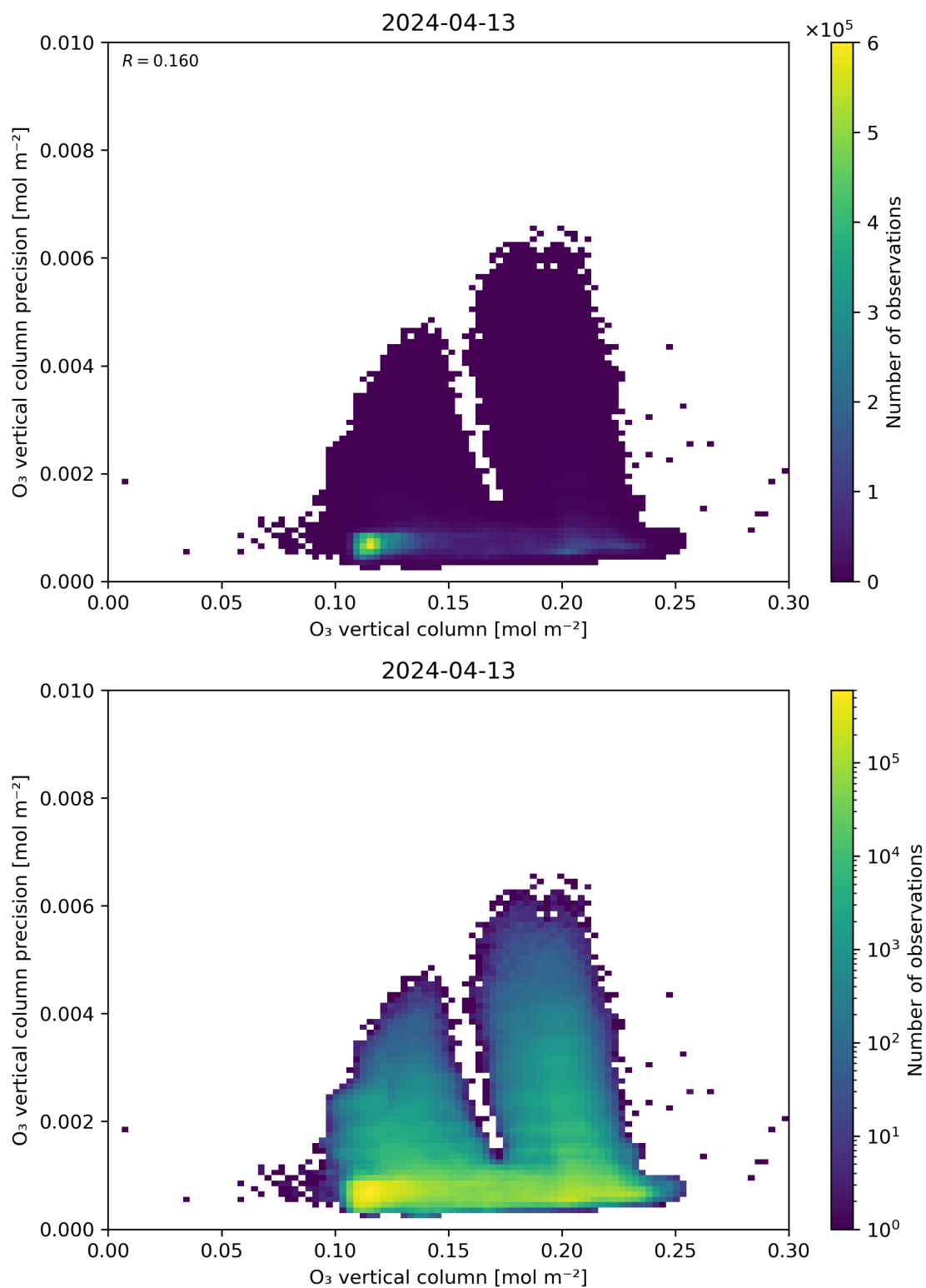
Figure 41: Scatter density plot of “O 3 vertical column” against “O 3 vertical column precision” for 2024-04-12 to 2024-04-14.
