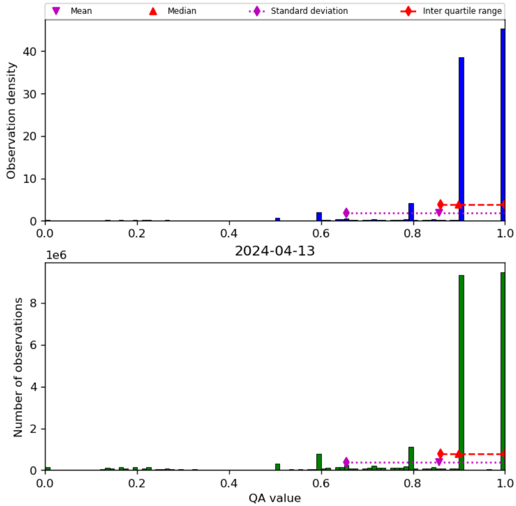
Figure 20: Histogram of “QA value” for 2024-04-12 to 2024-04-14
