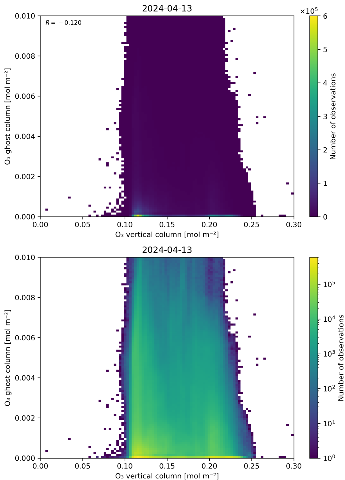
Figure 40: Scatter density plot of “O 3 vertical column” against “O 3 ghost column” for 2024-04-12 to 2024-04-14.
