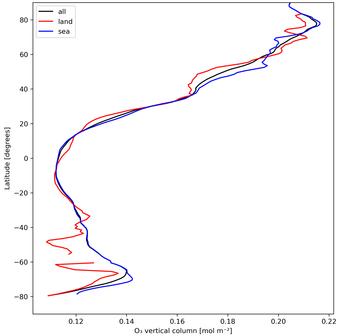
Figure 14: Zonal average of “O 3 vertical column” for 2024-04-12 to 2024-04-14.
