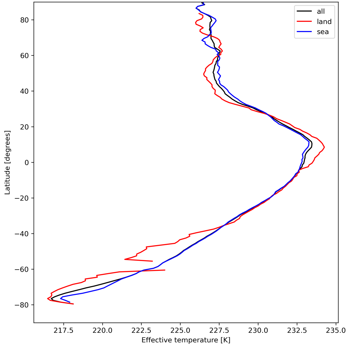
Figure 17: Zonal average of "Effective temperature" for 2024-04-13 to 2024-04-15.
