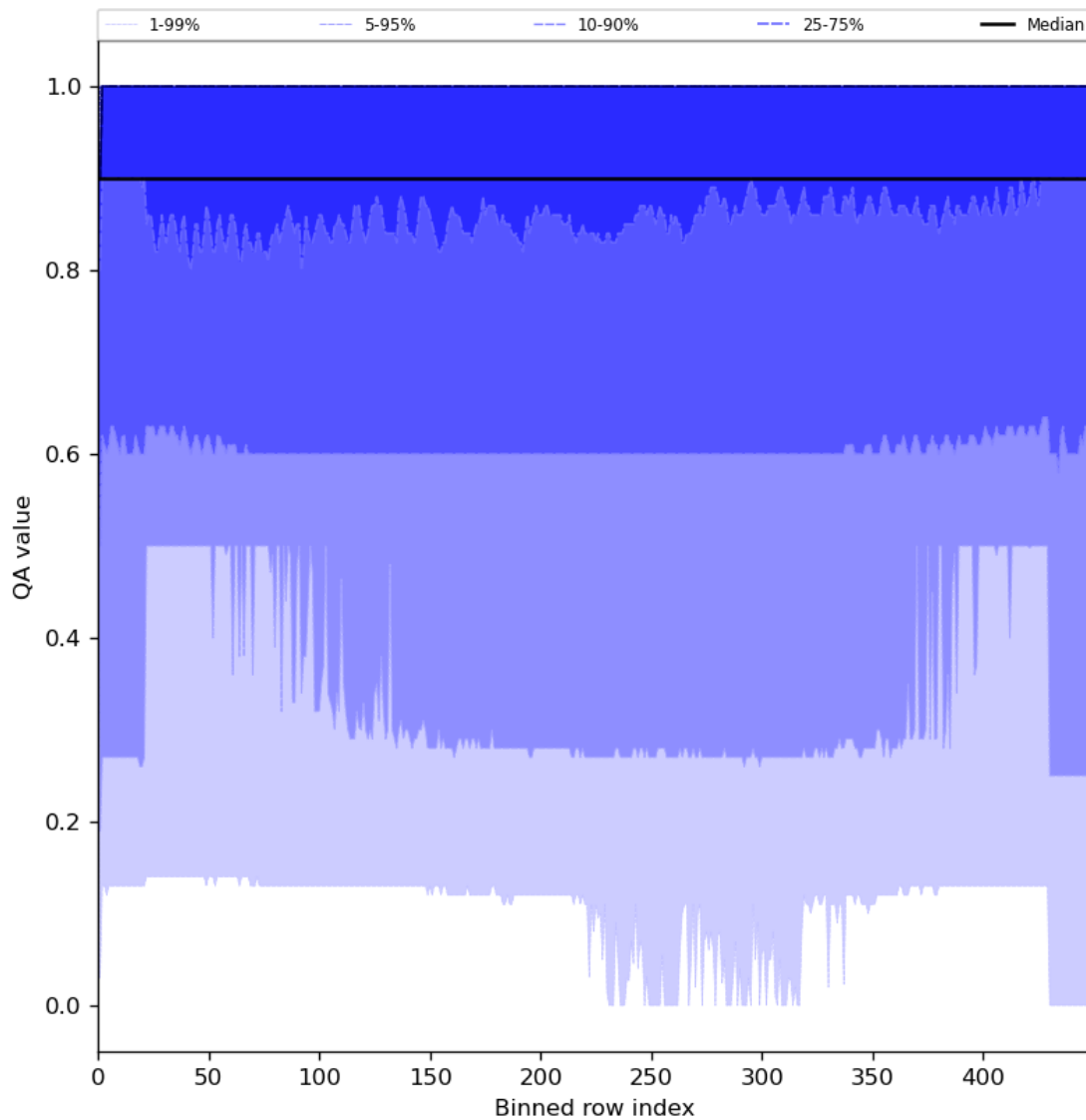
Figure 27: Along track statistics of “QA value” for 2024-04-13 to 2024-04-15
