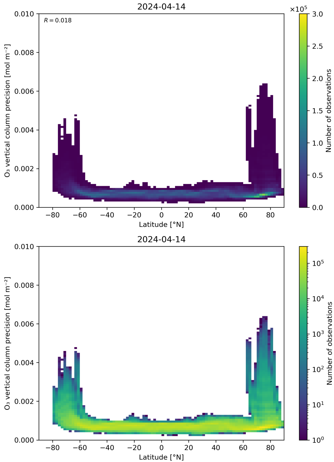
Figure 37: Scatter density plot of “Latitude” against “O 3 vertical column precision” for 2024-04-13 to 2024-04-15.
