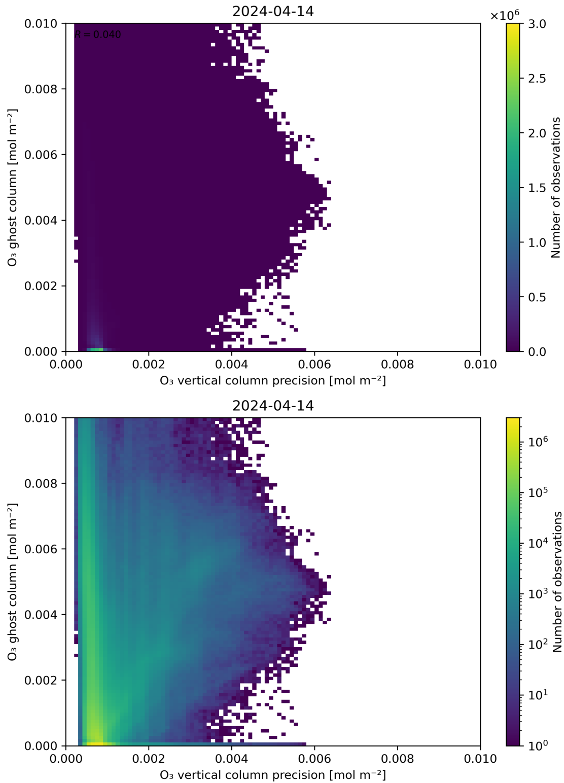
Figure 43: Scatter density plot of “ \text{O}_3 vertical column precision” against “ \text{O}_3 ghost column” for 2024-04-13 to 2024-04-15.
