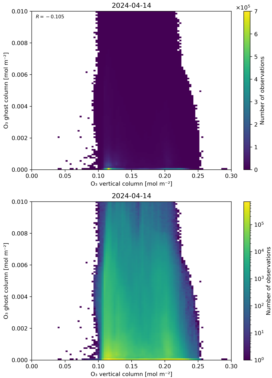
Figure 40: Scatter density plot of “O 3 vertical column” against “O 3 ghost column” for 2024-04-13 to 2024-04-15.
