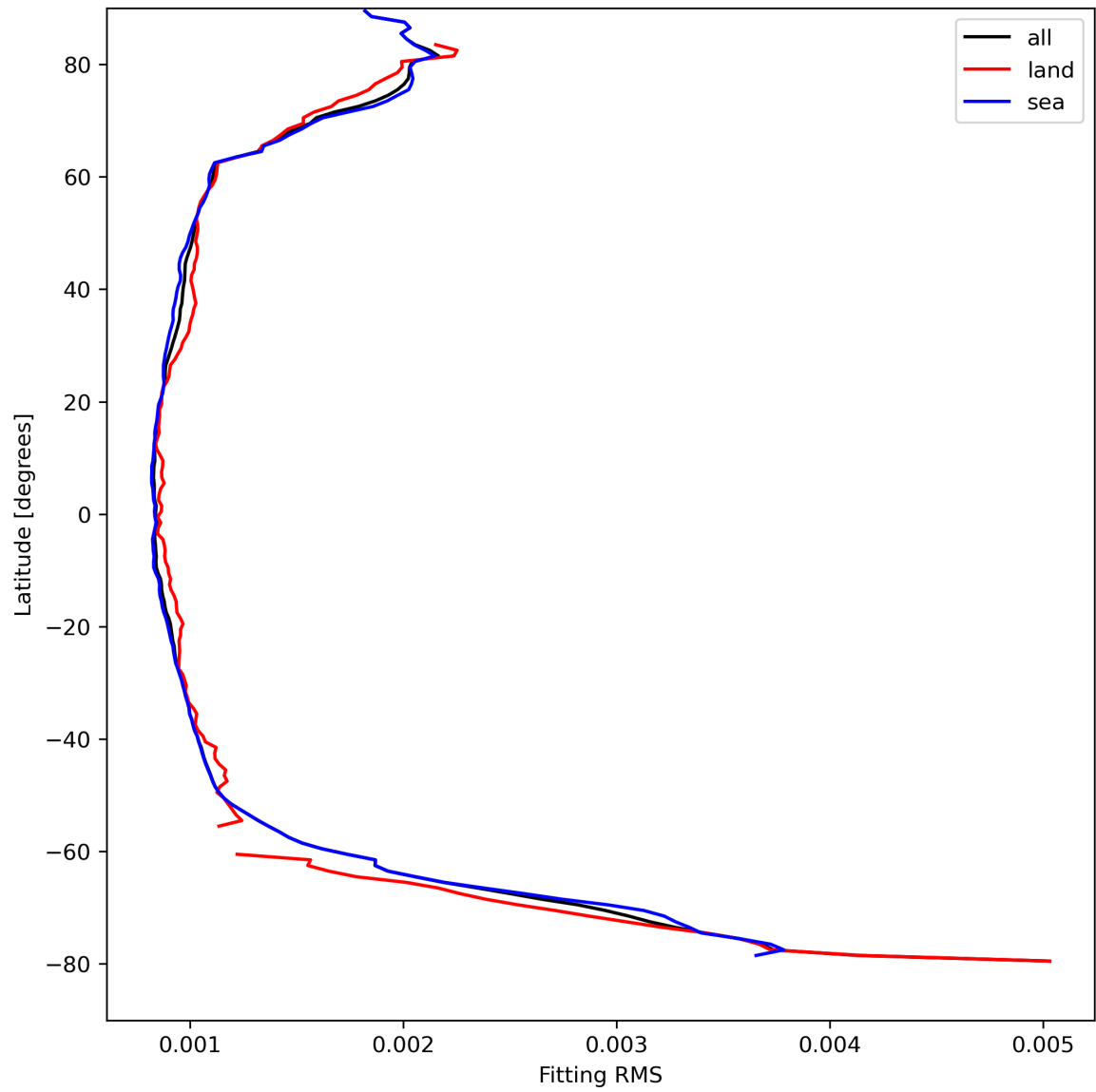
Figure 16: Zonal average of “Fitting RMS” for 2024-04-13 to 2024-04-15.
