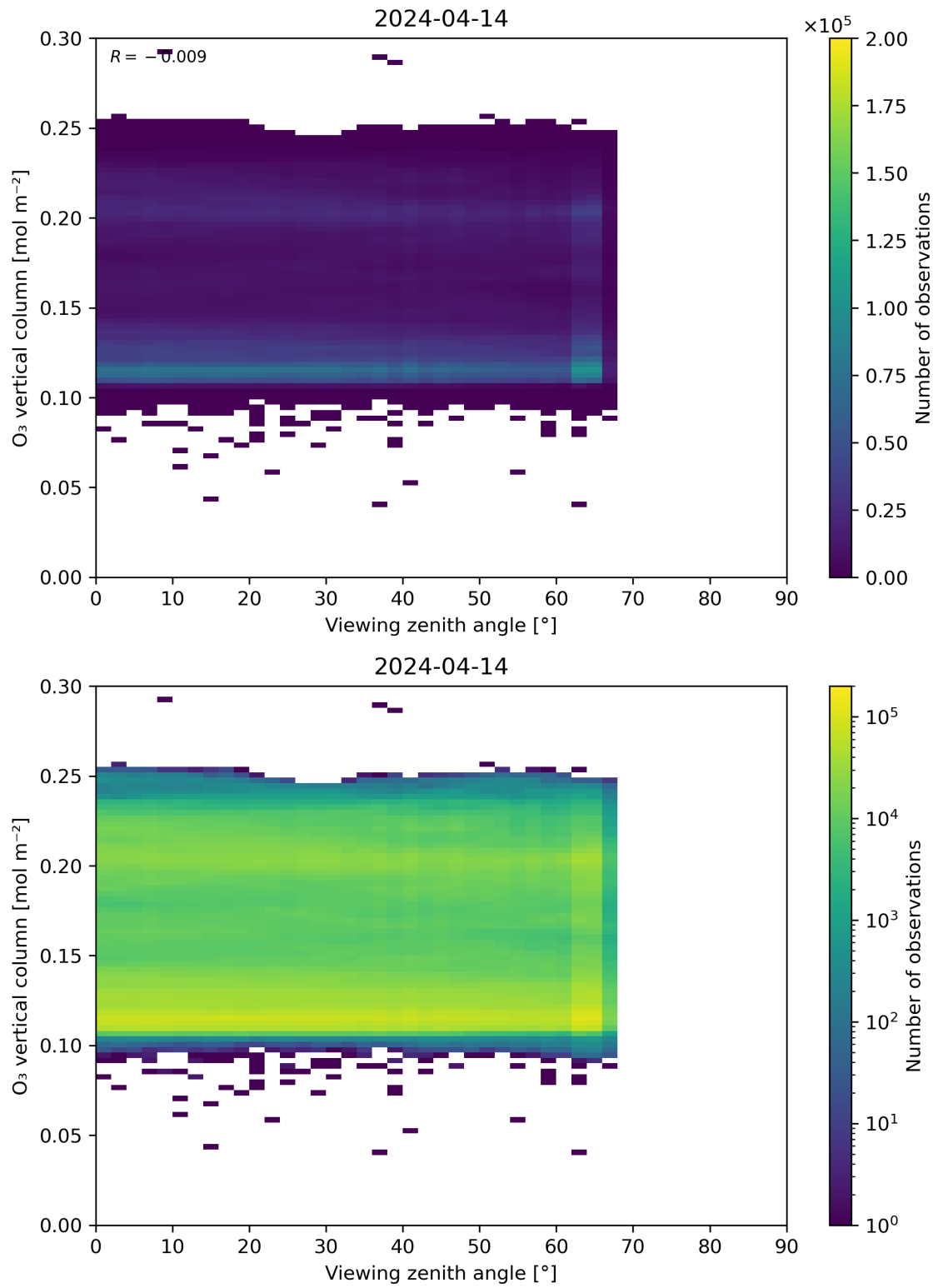
Figure 52: Scatter density plot of “Viewing zenith angle” against “O 3 vertical column” for 2024-04-13 to 2024-04-15.
