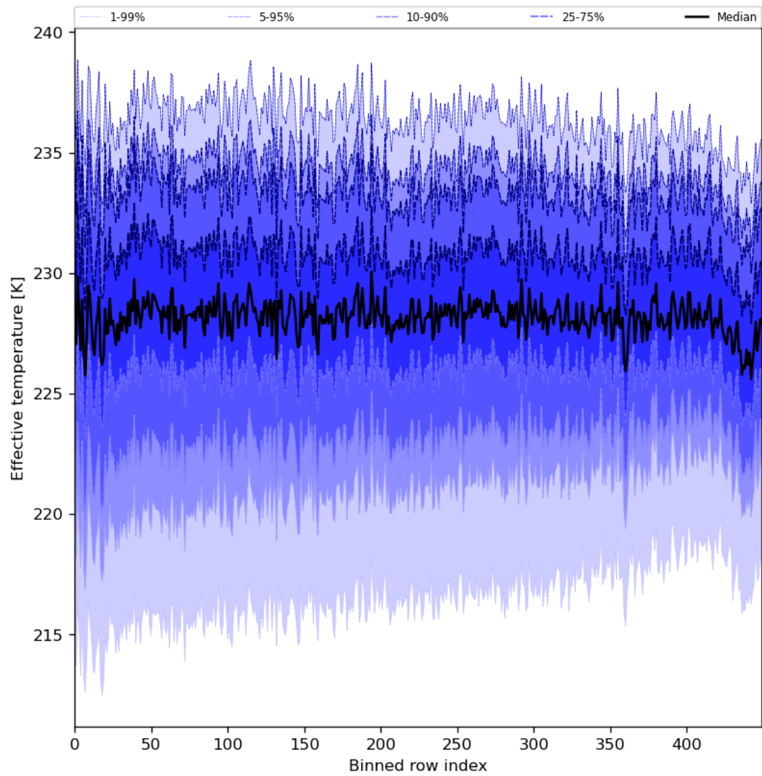
Figure 31: Along track statistics of “Effective temperature” for 2024-04-13 to 2024-04-15
