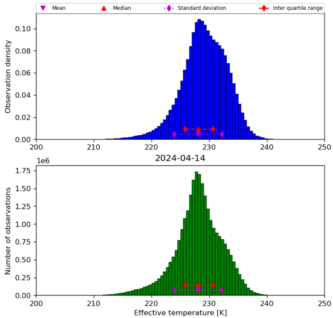
Figure 24: Histogram of “Effective temperature” for 2024-04-13 to 2024-04-15
