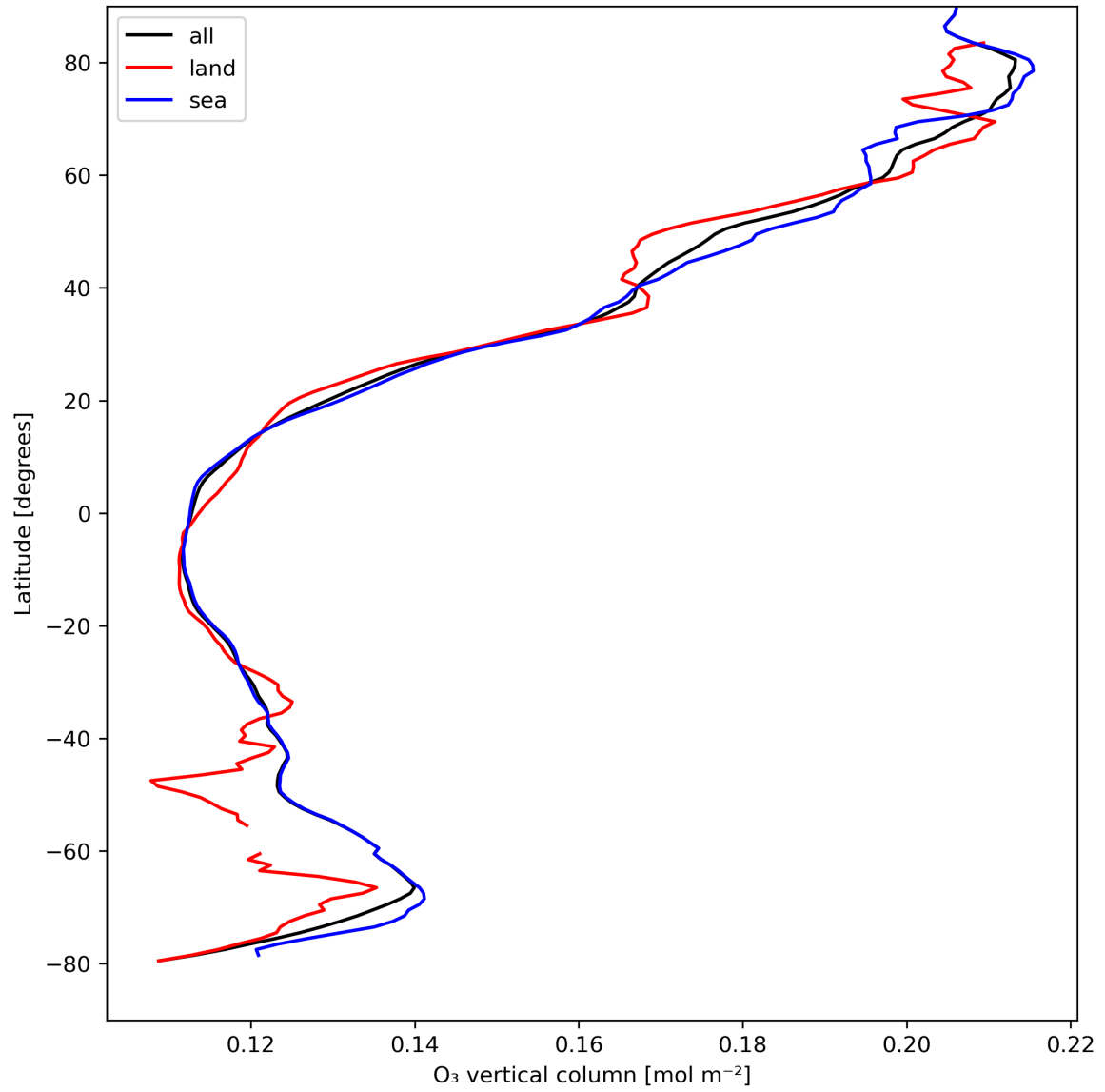
Figure 14: Zonal average of “O 3 vertical column” for 2024-04-13 to 2024-04-15.
