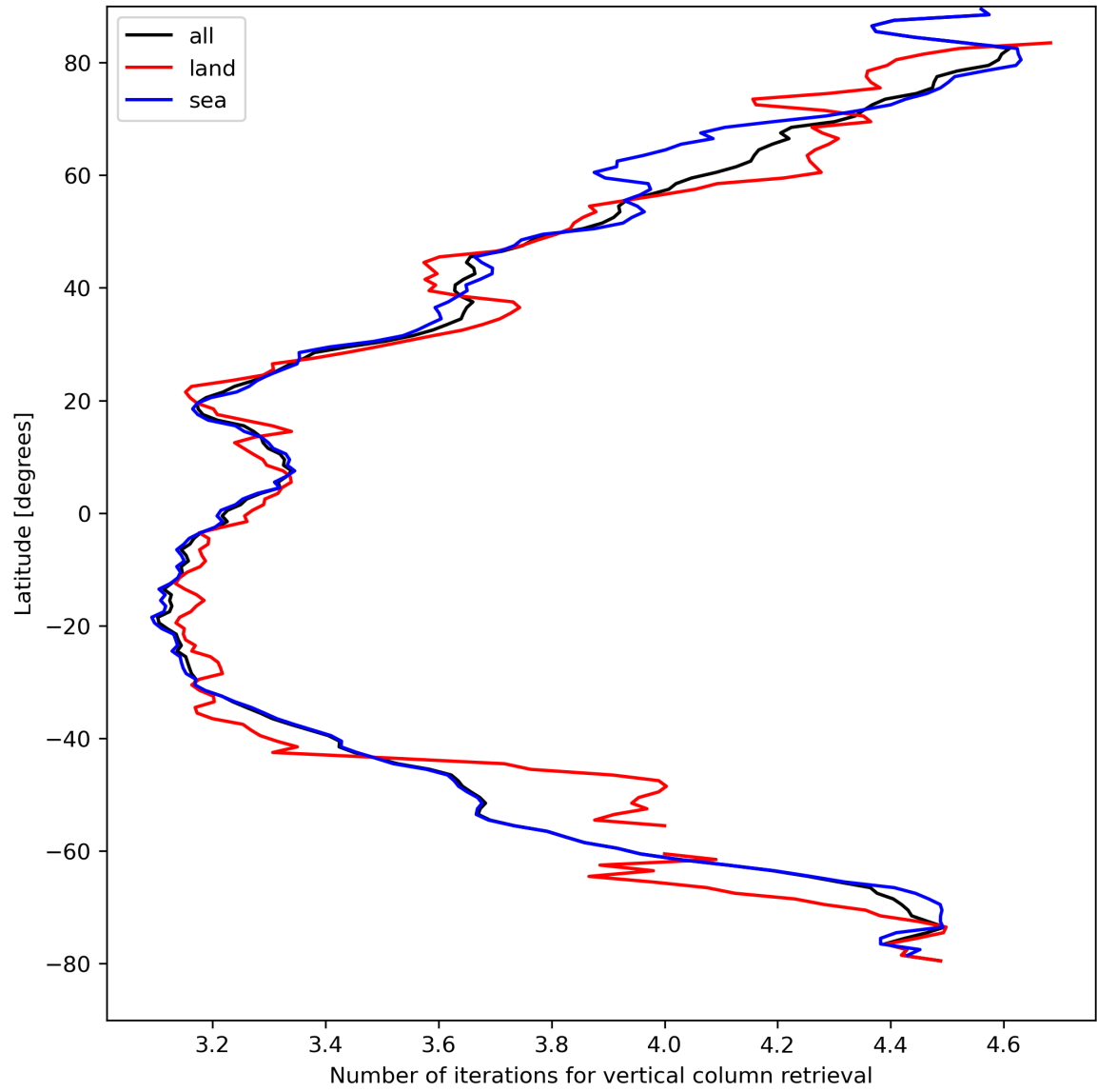
Figure 19: Zonal average of “Number of iterations for vertical column retrieval” for 2024-04-13 to 2024-04-15.
