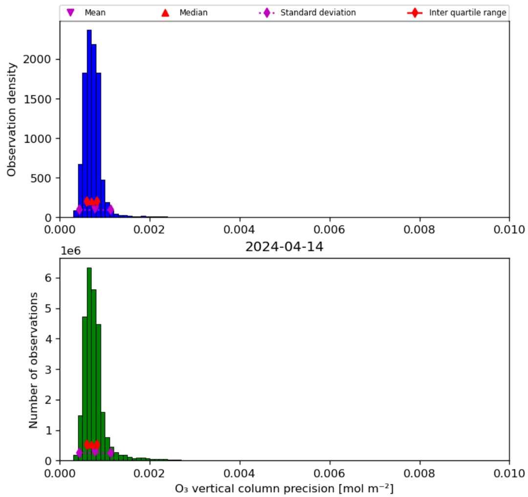
Figure 22: Histogram of “O 3 vertical column precision” for 2024-04-13 to 2024-04-15
