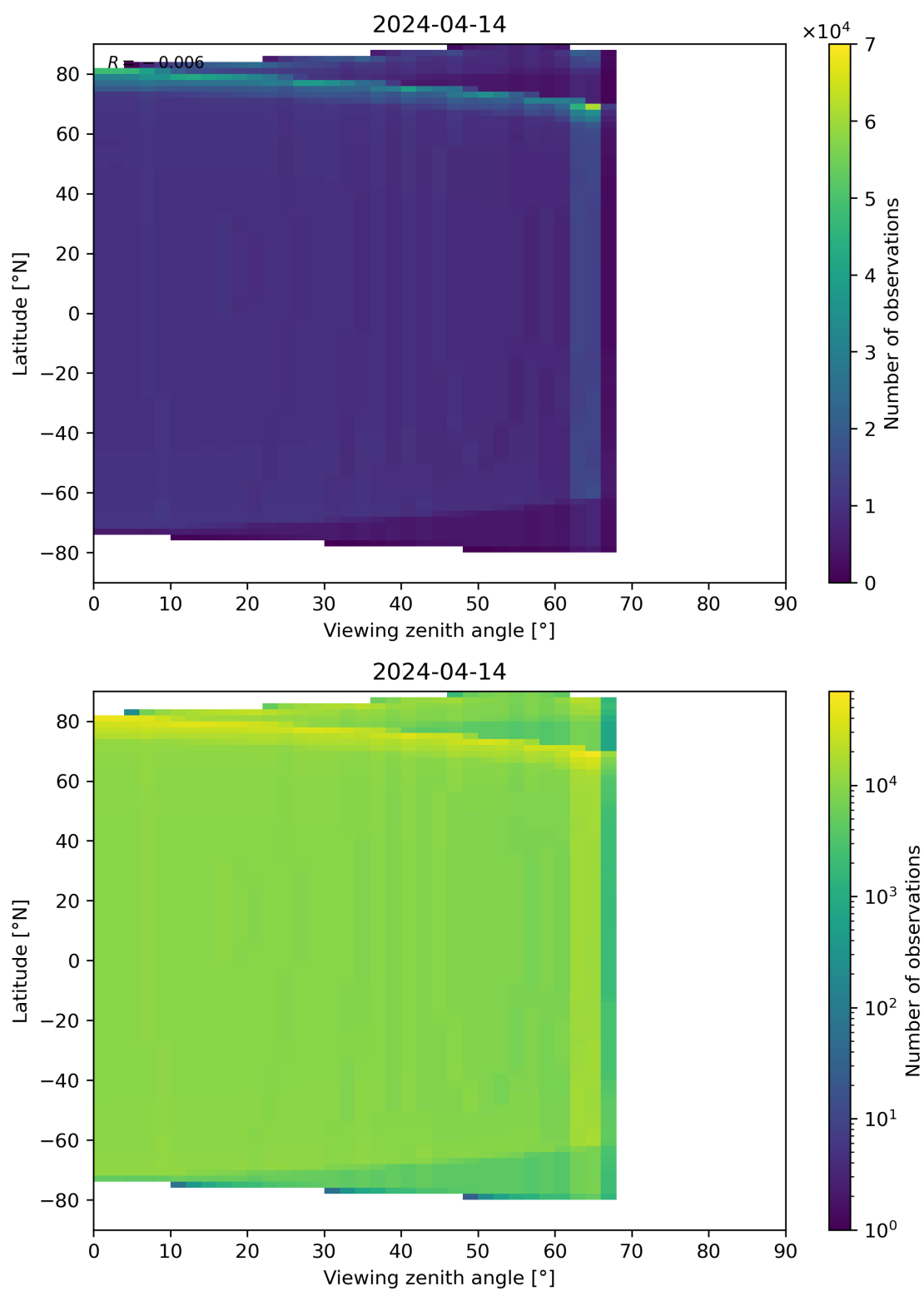
Figure 49: Scatter density plot of “Viewing zenith angle” against “Latitude” for 2024-04-13 to 2024-04-15.
