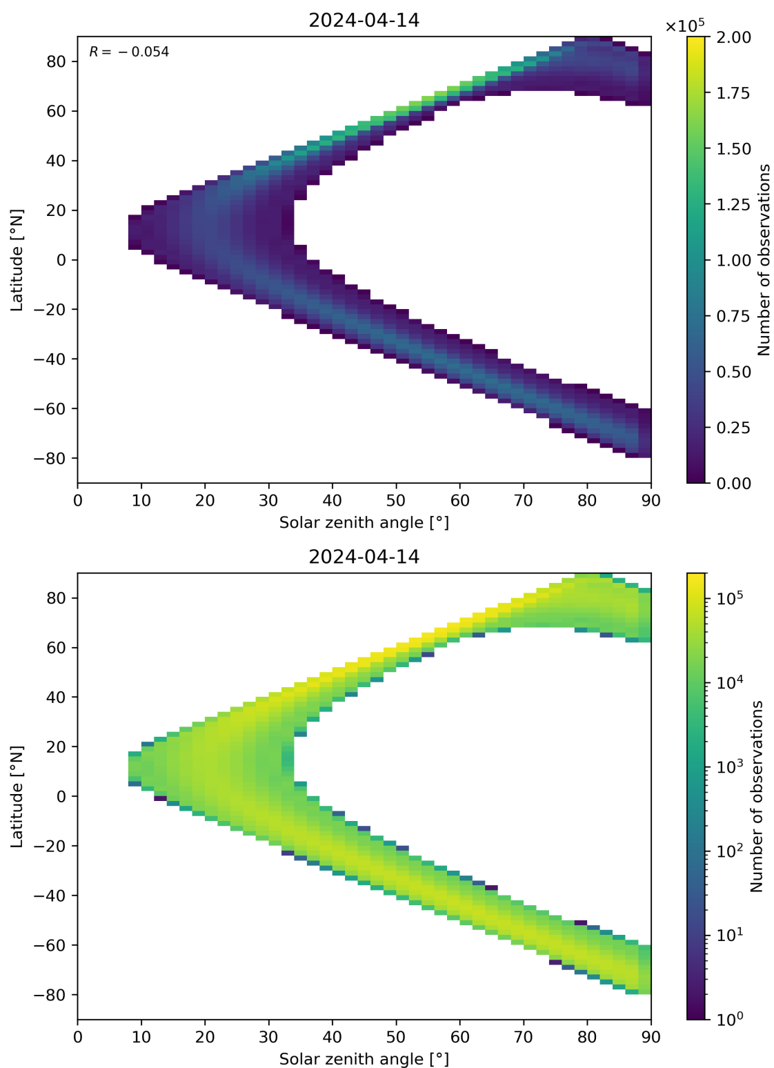
Figure 44: Scatter density plot of “Solar zenith angle” against “Latitude” for 2024-04-13 to 2024-04-15.
