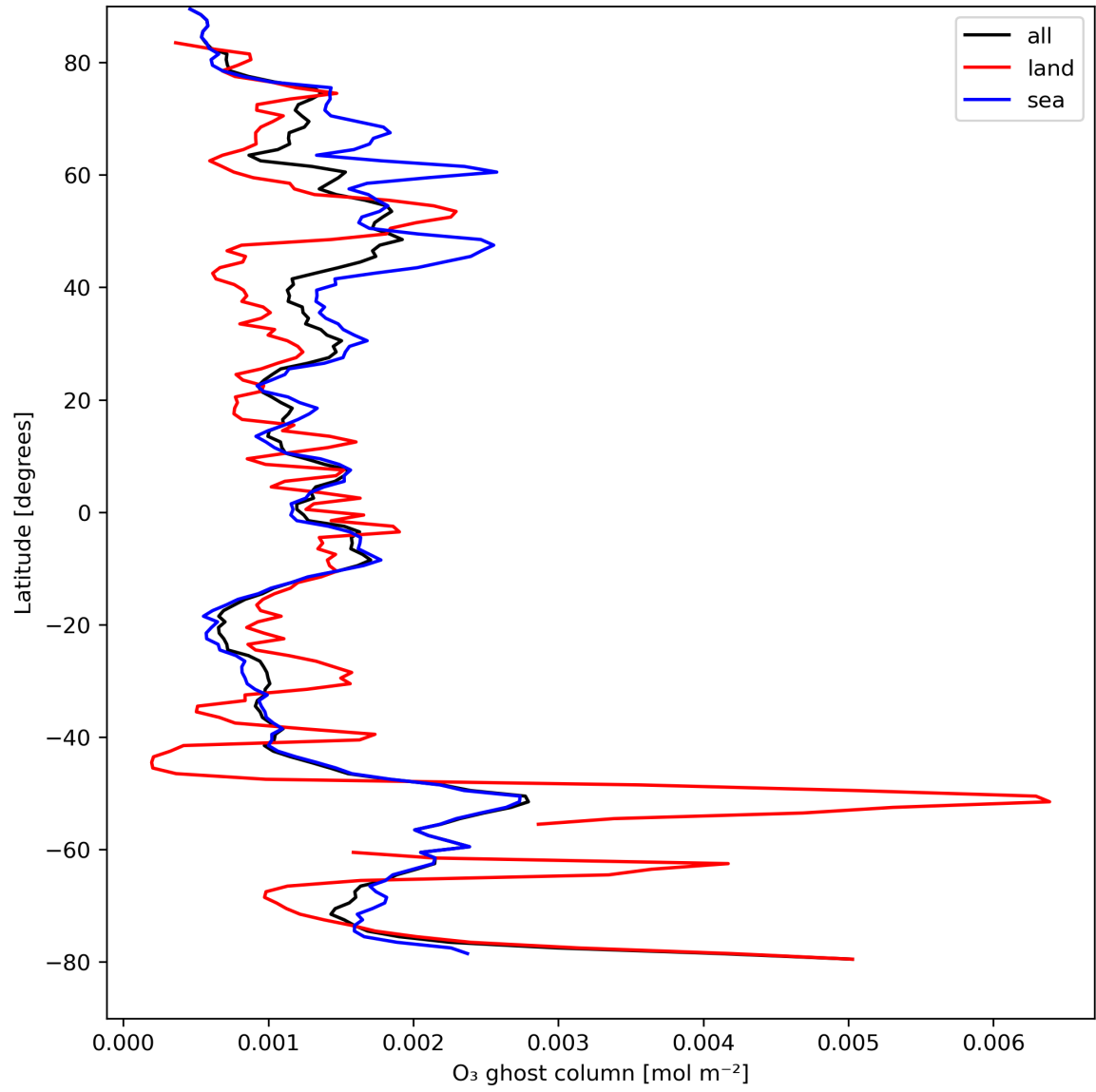
Figure 18: Zonal average of "O 3 ghost column" for 2024-04-13 to 2024-04-15.
