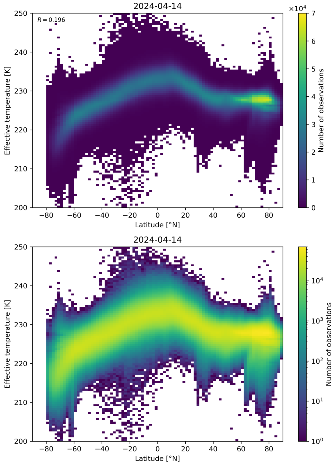
Figure 34: Scatter density plot of “Latitude” against “Effective temperature” for 2024-04-13 to 2024-04-15.
