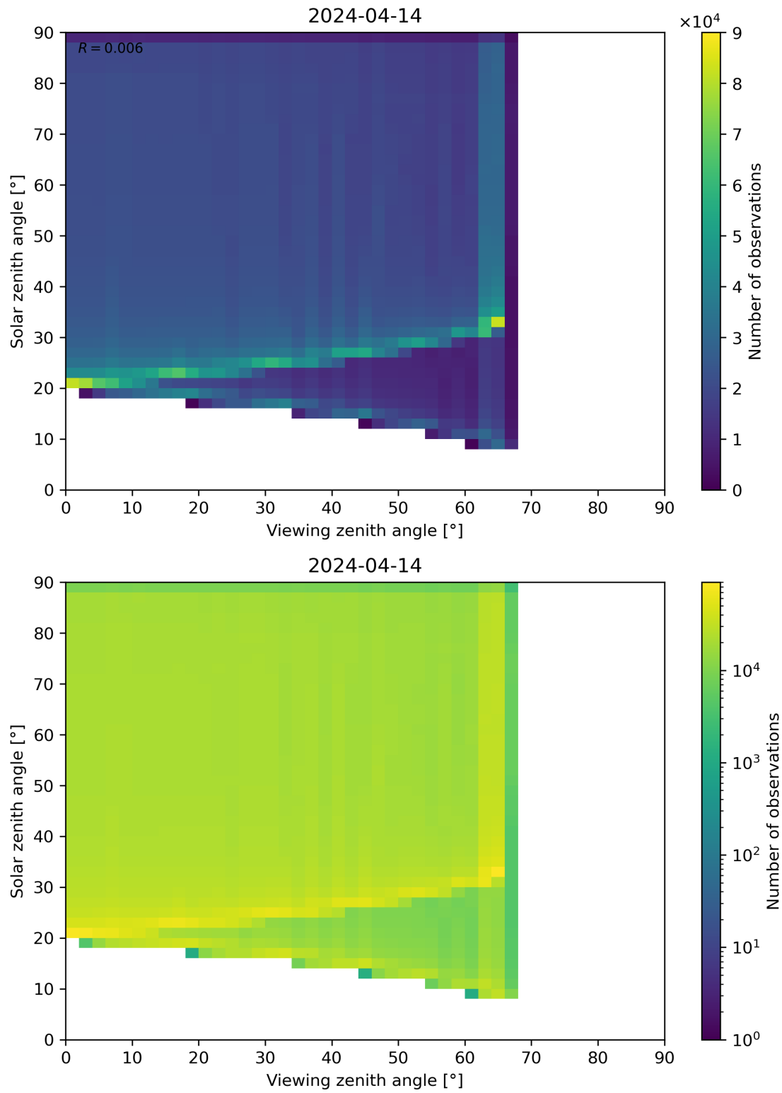
Figure 54: Scatter density plot of “Viewing zenith angle” against “Solar zenith angle” for 2024-04-13 to 2024-04-15.
