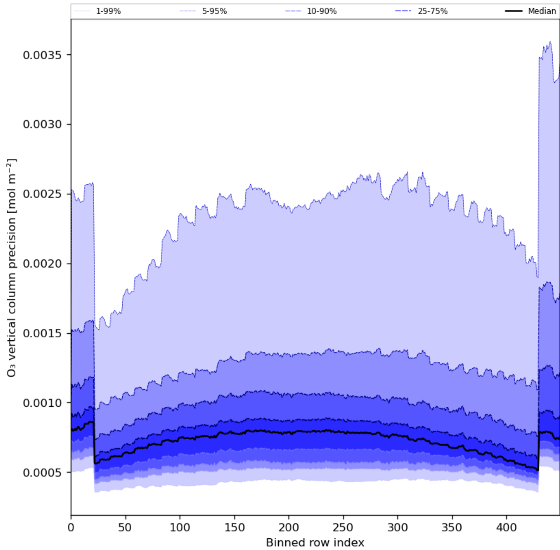
Figure 29: Along track statistics of “O 3 vertical column precision” for 2024-04-13 to 2024-04-15
