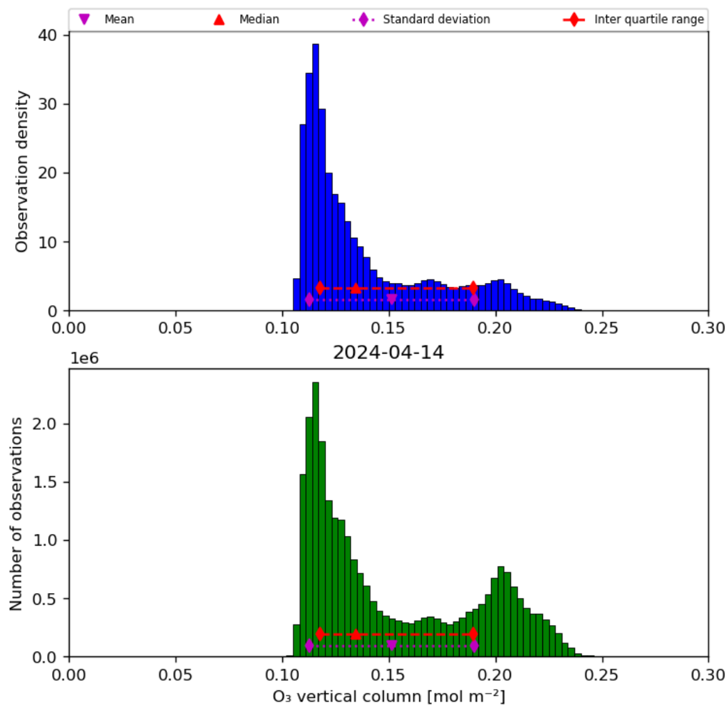
Figure 21: Histogram of “O 3 vertical column” for 2024-04-13 to 2024-04-15
