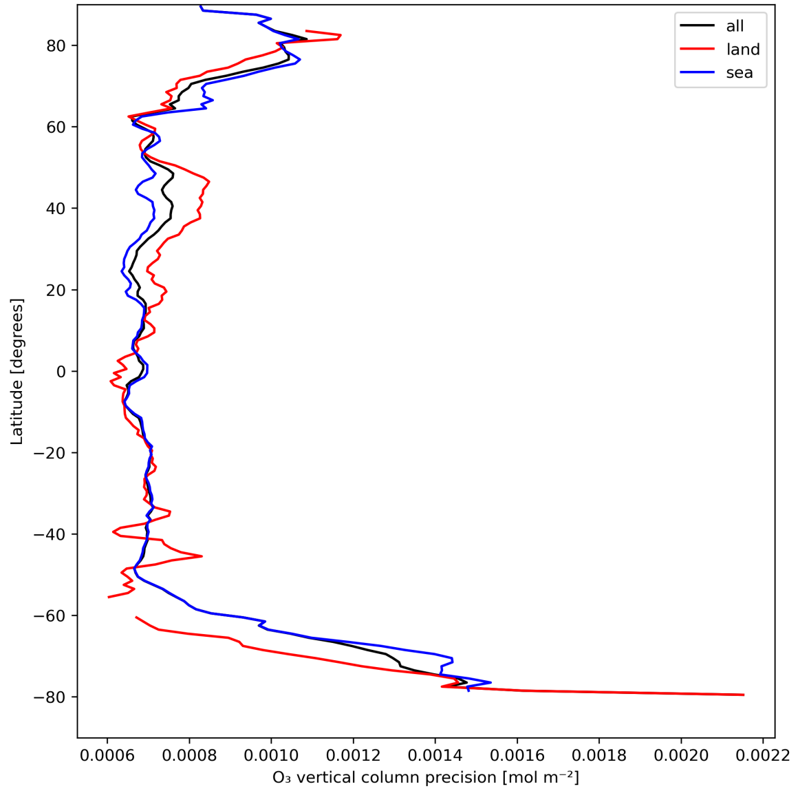
Figure 15: Zonal average of “O 3 vertical column precision” for 2024-04-13 to 2024-04-15.
