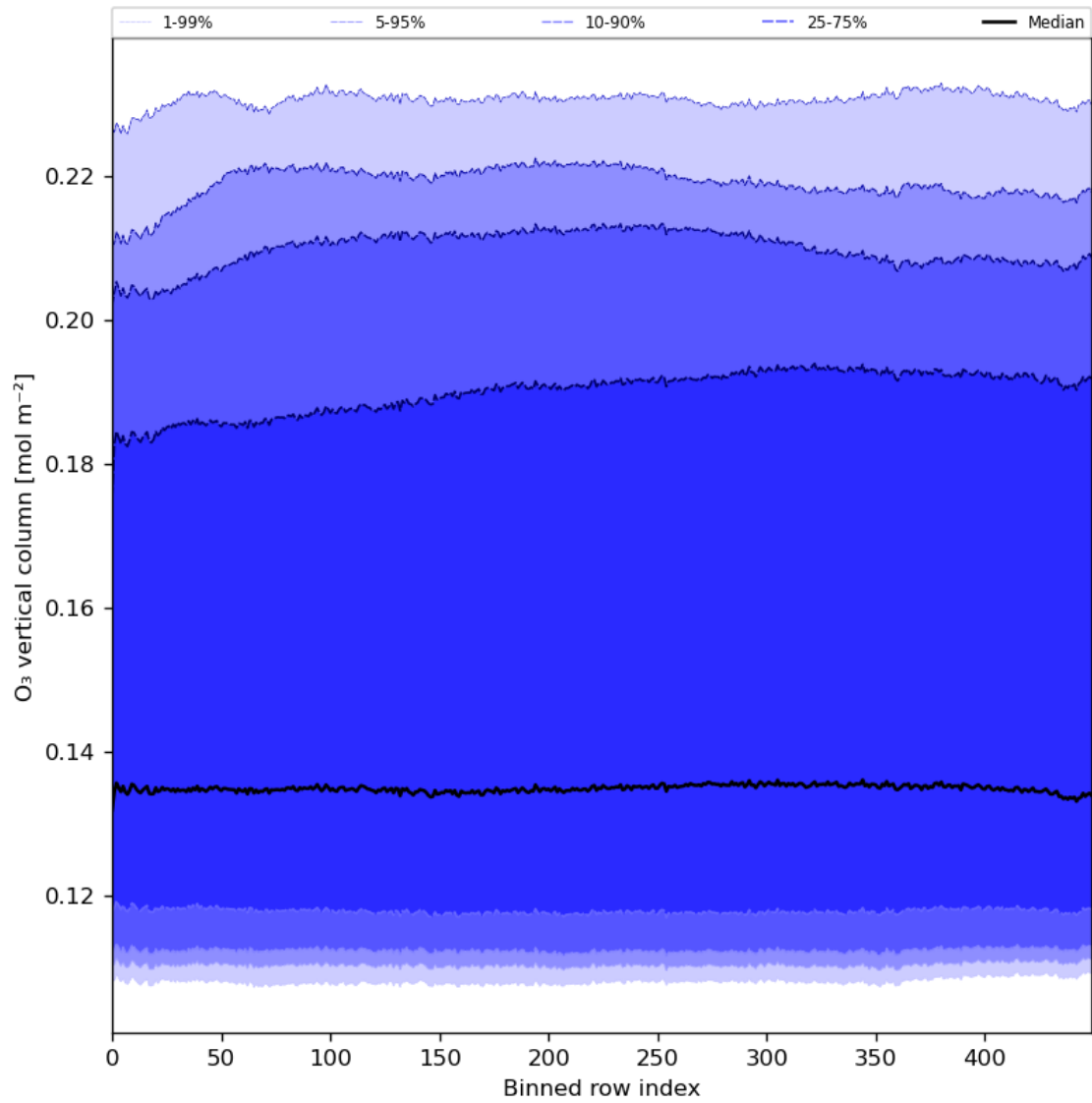
Figure 28: Along track statistics of “O 3 vertical column” for 2024-04-13 to 2024-04-15
