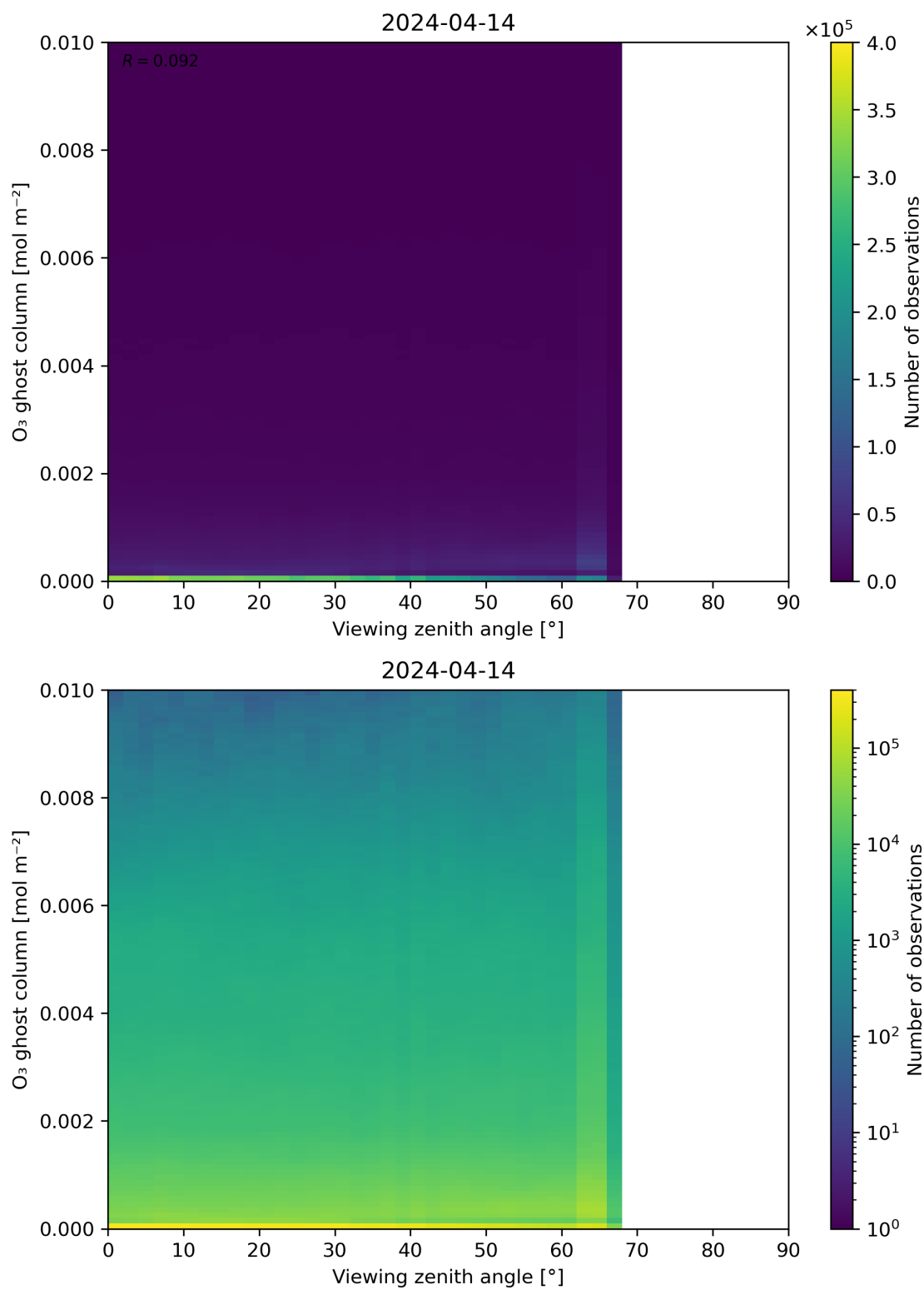
Figure 51: Scatter density plot of “Viewing zenith angle” against “O 3 ghost column” for 2024-04-13 to 2024-04-15.
