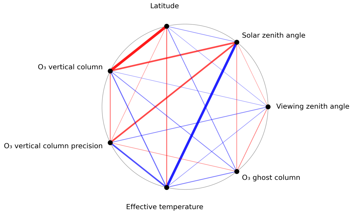
Figure 1: Map of correlation graph for 2024-04-13 to 2024-04-15.
