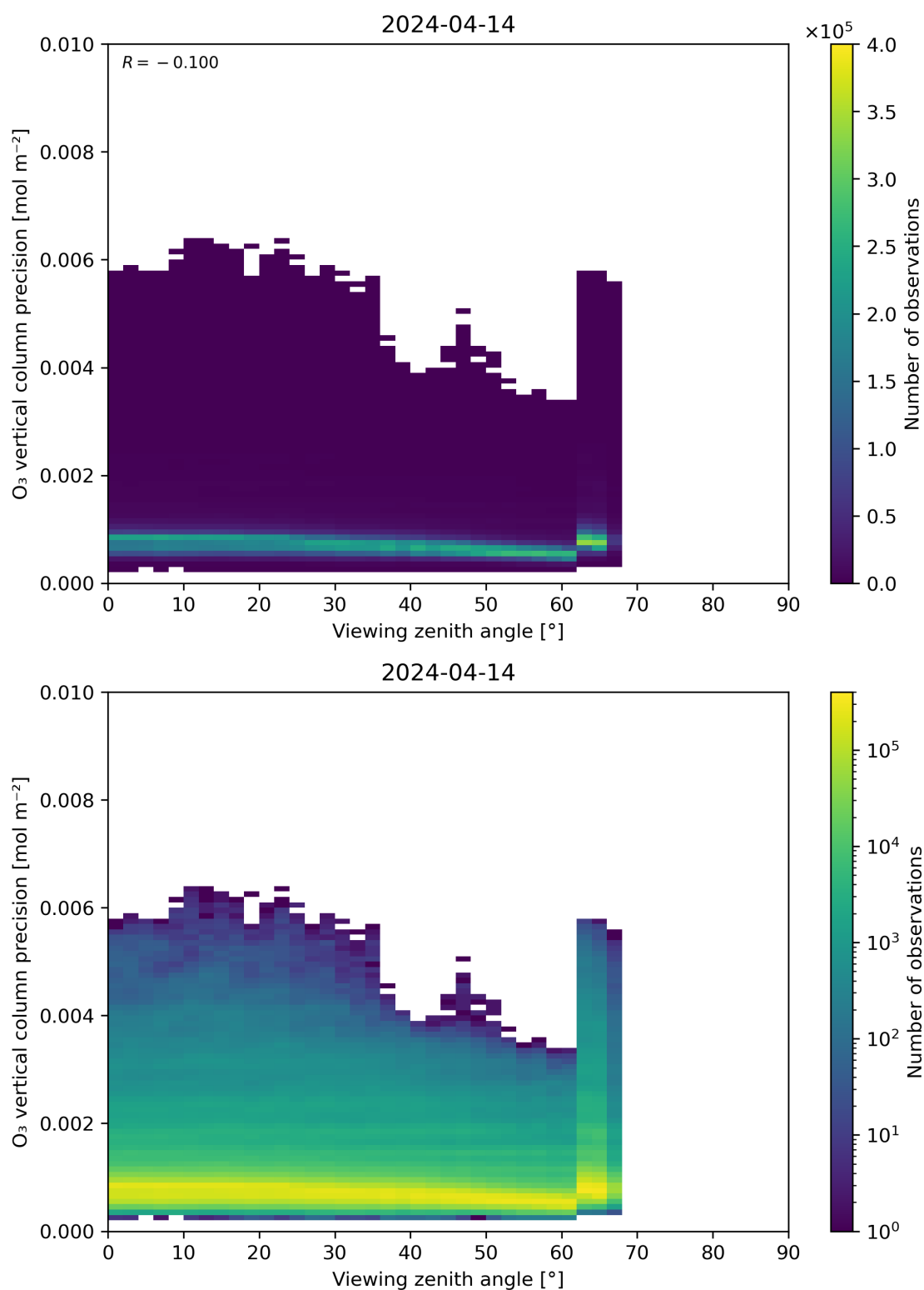
Figure 53: Scatter density plot of “Viewing zenith angle” against “O 3 vertical column precision” for 2024-04-13 to 2024-04-15.
