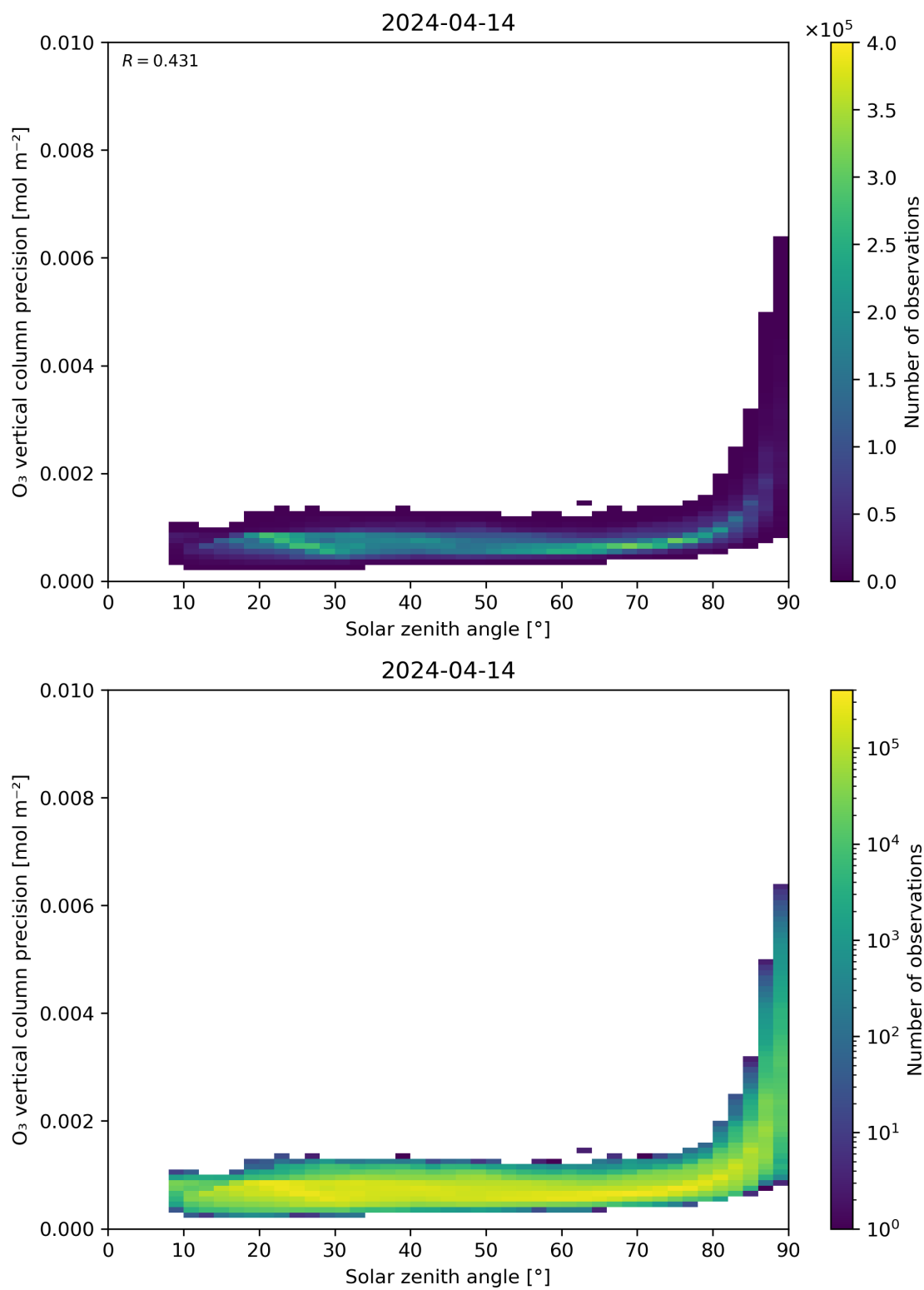
Figure 48: Scatter density plot of “Solar zenith angle” against “O 3 vertical column precision” for 2024-04-13 to 2024-04-15.
