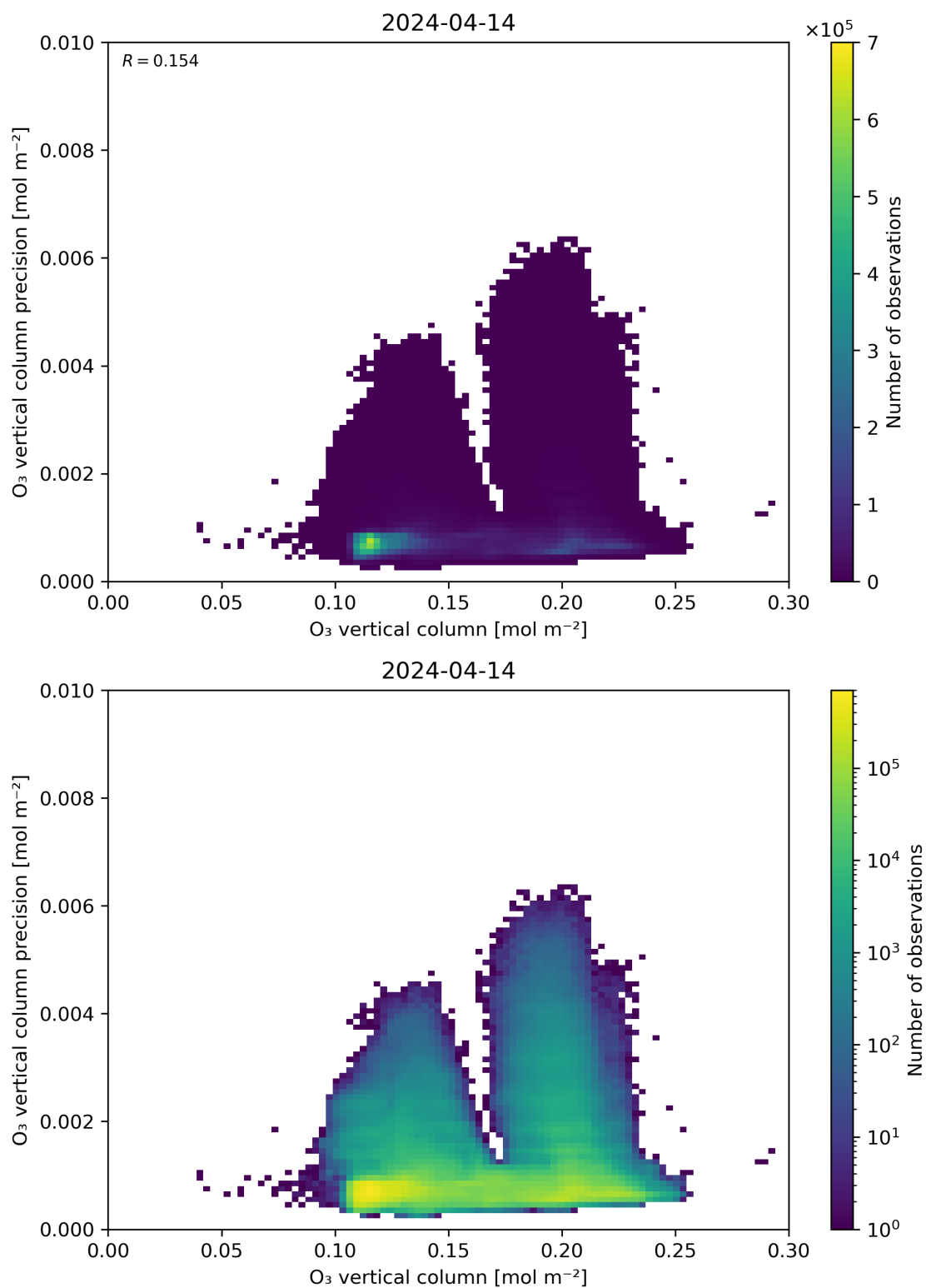
Figure 41: Scatter density plot of “O 3 vertical column” against “O 3 vertical column precision” for 2024-04-13 to 2024-04-15.
