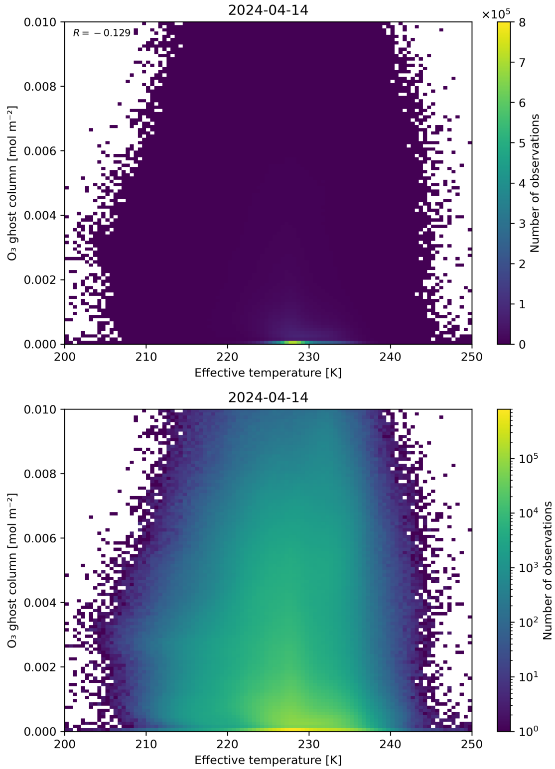
Figure 38: Scatter density plot of “Effective temperature” against “O 3 ghost column” for 2024-04-13 to 2024-04-15.
