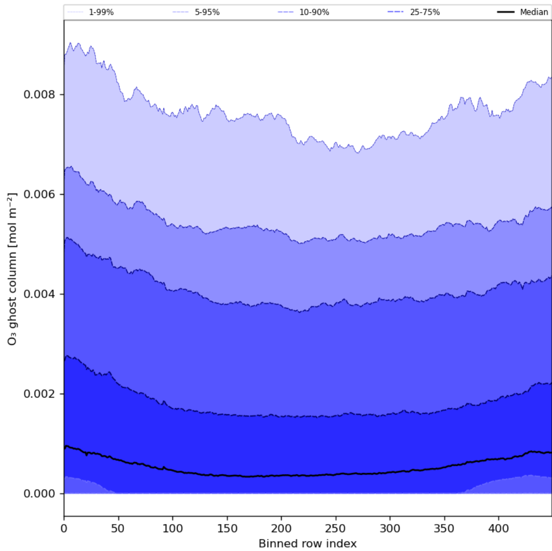
Figure 32: Along track statistics of “O 3 ghost column” for 2024-04-13 to 2024-04-15
