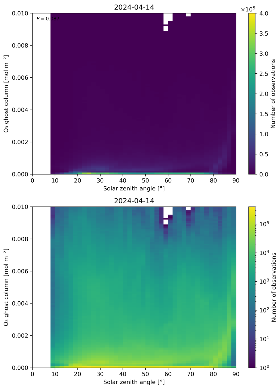
Figure 46: Scatter density plot of “Solar zenith angle” against “O 3 ghost column” for 2024-04-13 to 2024-04-15.
