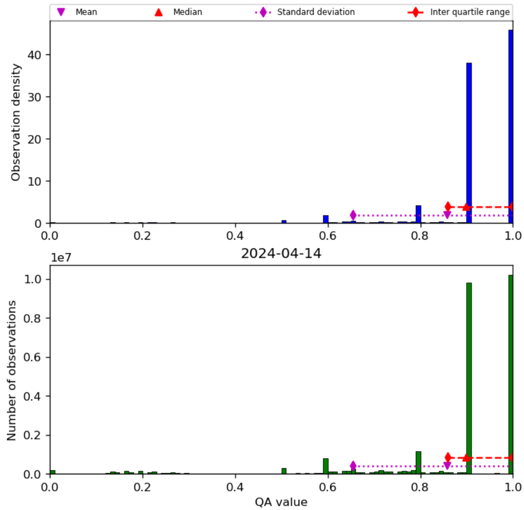
Figure 20: Histogram of “QA value” for 2024-04-13 to 2024-04-15
