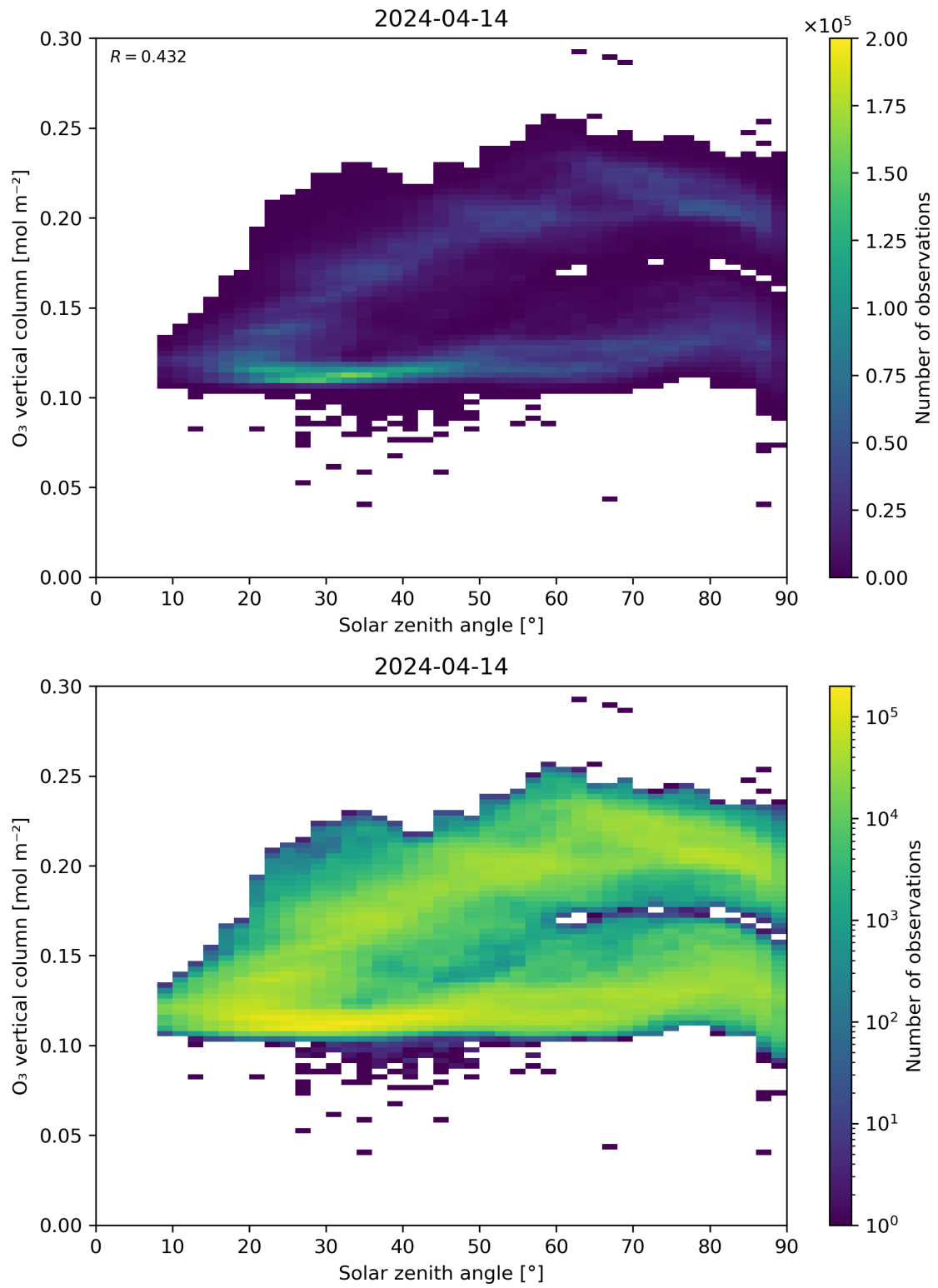
Figure 47: Scatter density plot of “Solar zenith angle” against “O 3 vertical column” for 2024-04-13 to 2024-04-15.
