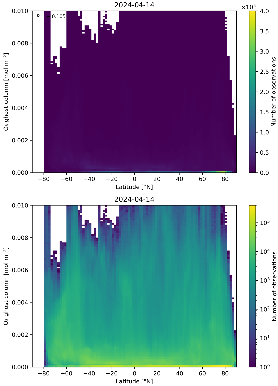
Figure 35: Scatter density plot of “Latitude” against “O 3 ghost column” for 2024-04-13 to 2024-04-15.
