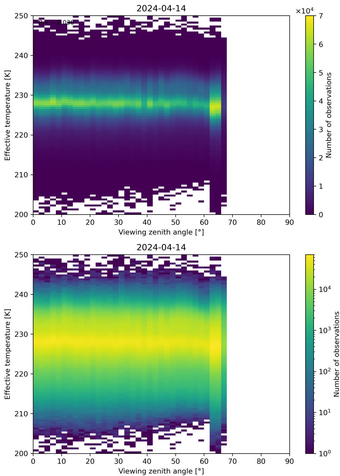
Figure 50: Scatter density plot of “Viewing zenith angle” against “Effective temperature” for 2024-04-13 to 2024-04-15.
