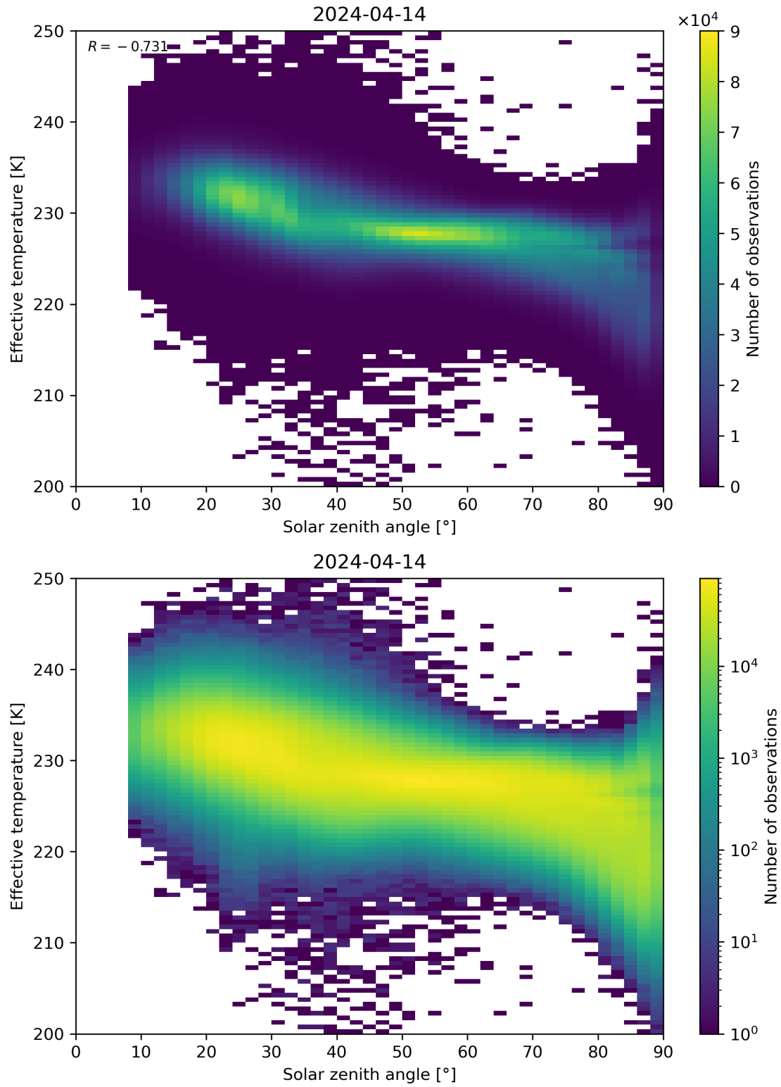
Figure 45: Scatter density plot of “Solar zenith angle” against “Effective temperature” for 2024-04-13 to 2024-04-15.
