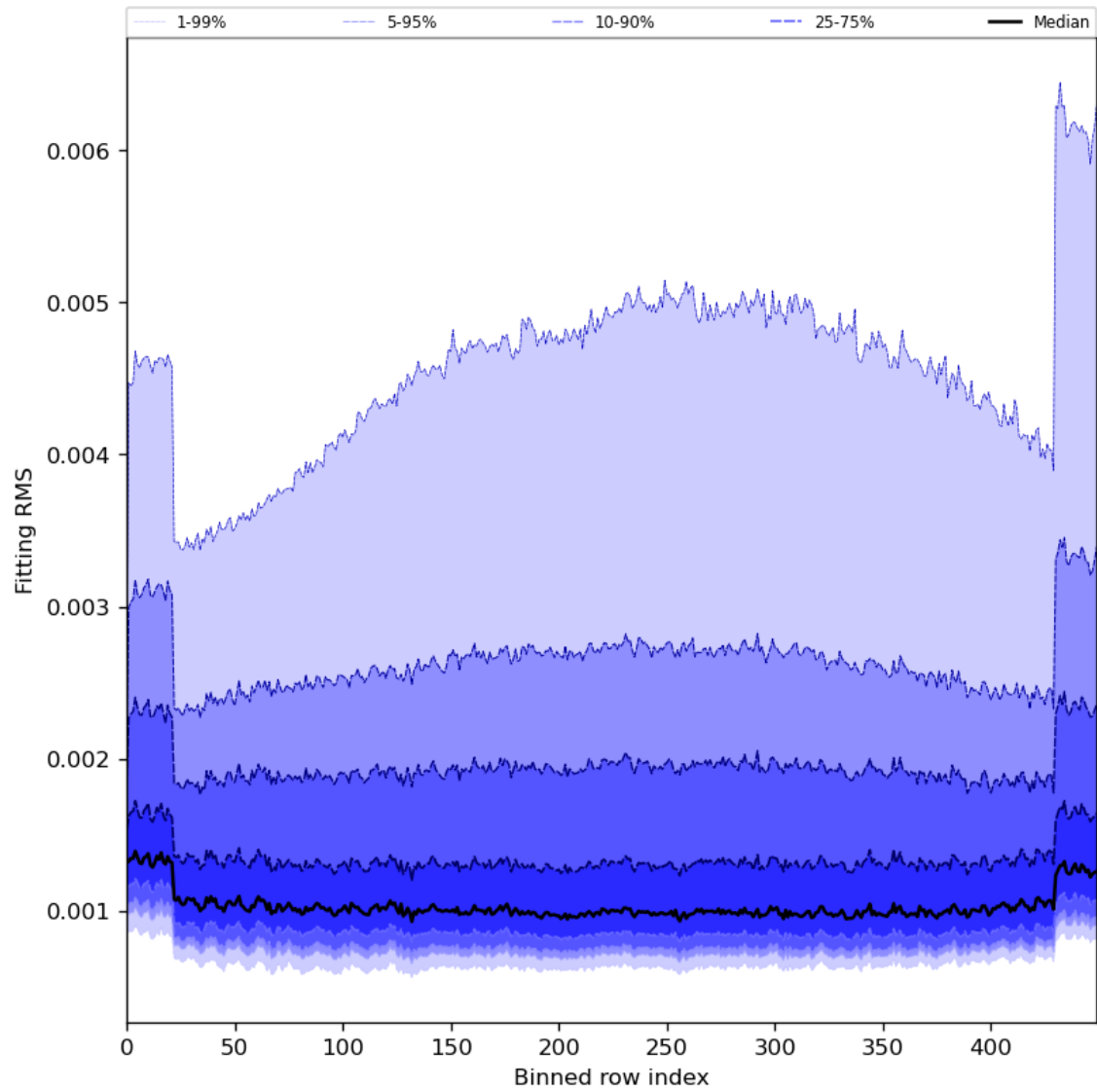
Figure 30: Along track statistics of “Fitting RMS” for 2024-04-13 to 2024-04-15
