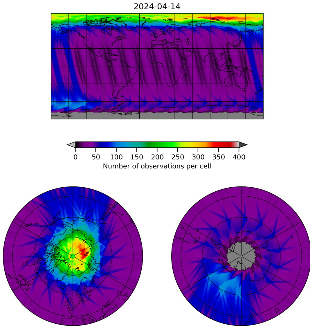
Figure 12: Map of the number of observations for 2024-04-13 to 2024-04-15
