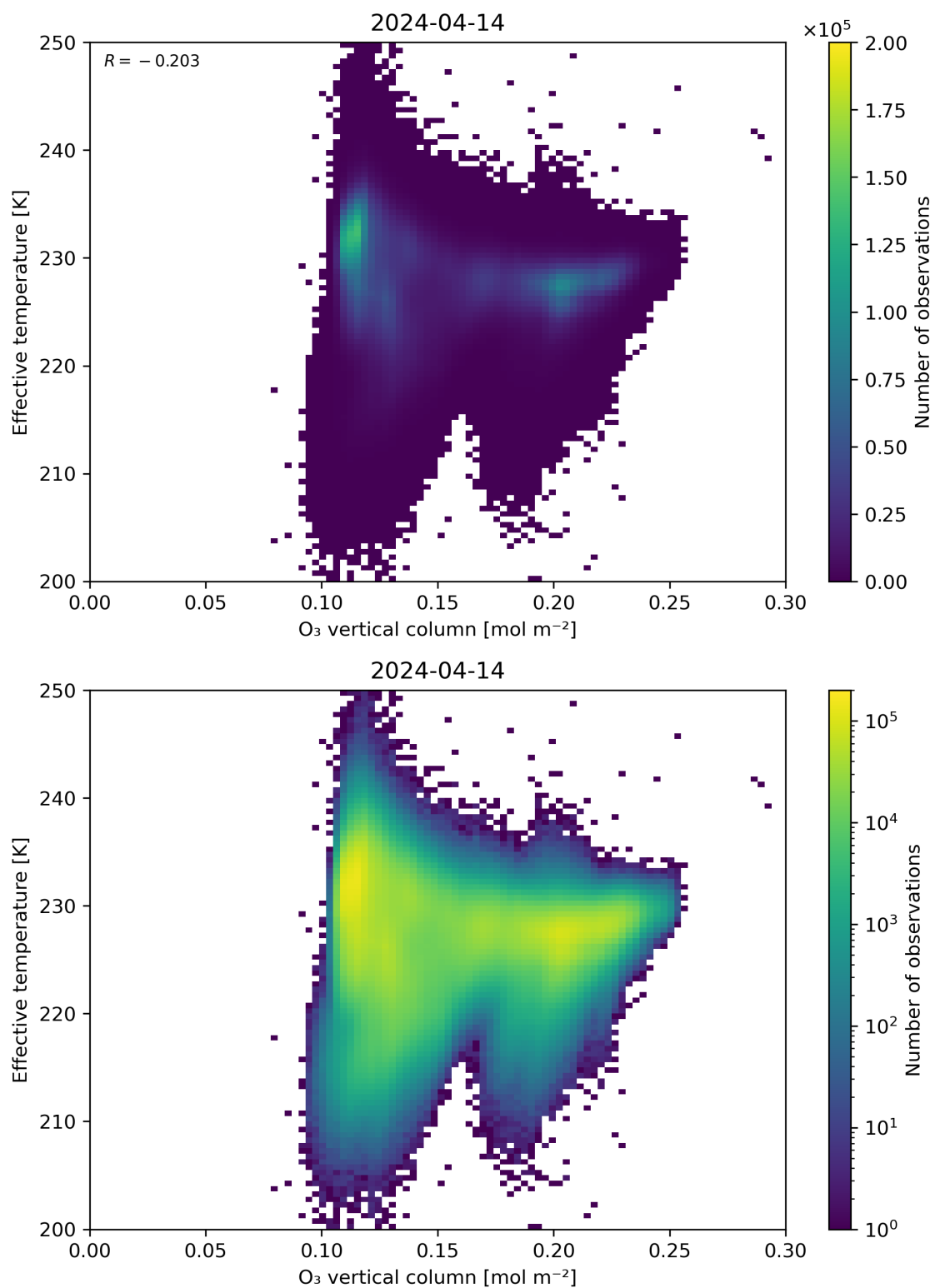
Figure 39: Scatter density plot of “O 3 vertical column” against “Effective temperature” for 2024-04-13 to 2024-04-15.
