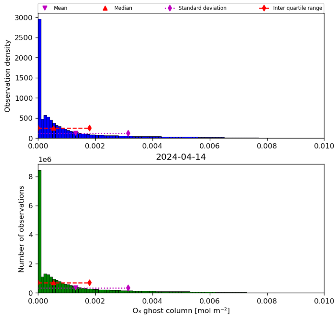
Figure 25: Histogram of “O 3 ghost column” for 2024-04-13 to 2024-04-15
