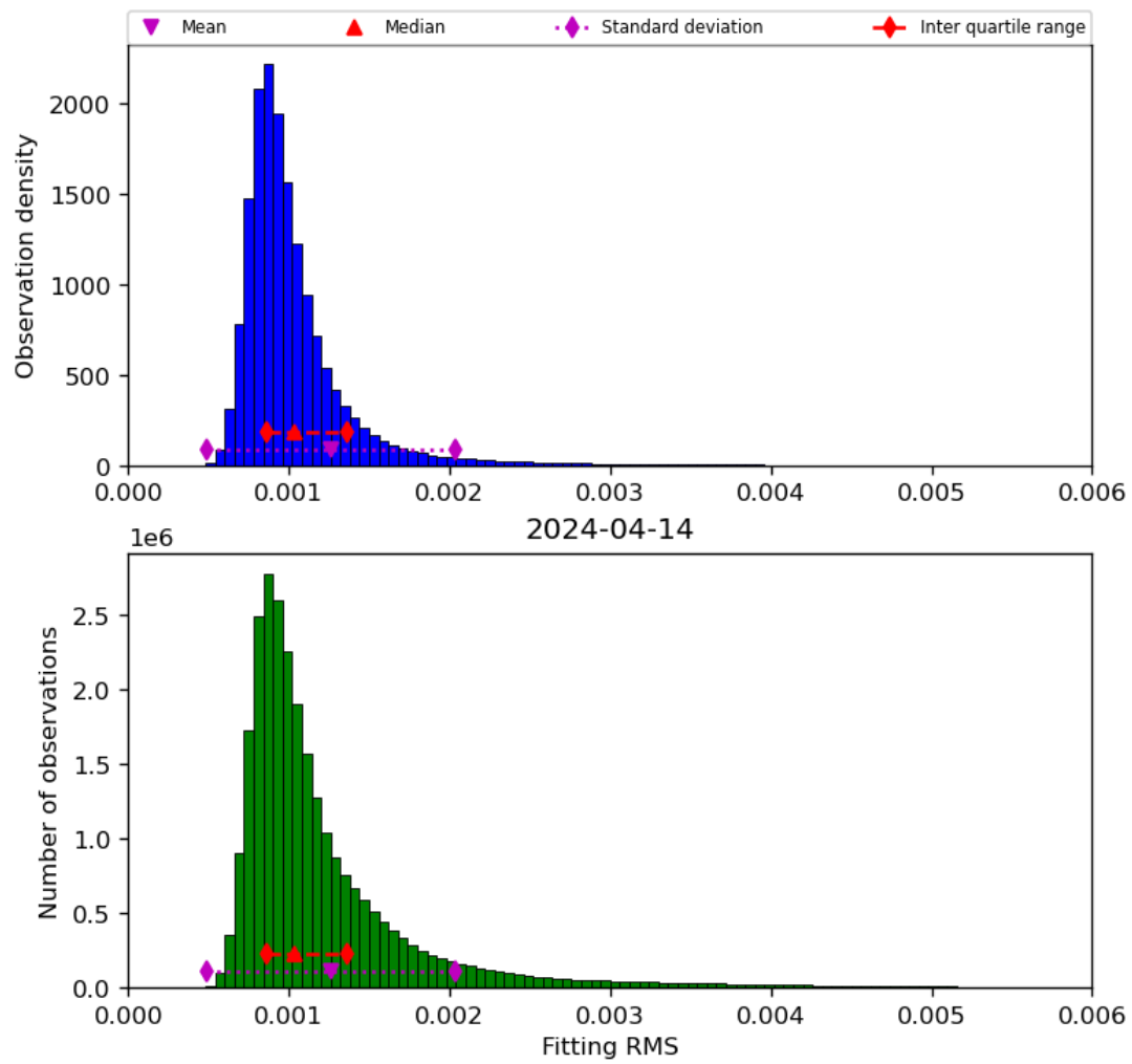
Figure 23: Histogram of "Fitting RMS" for 2024-04-13 to 2024-04-15
