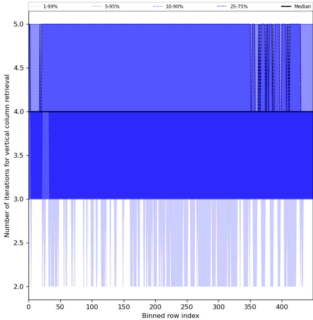
Figure 33: Along track statistics of “Number of iterations for vertical column retrieval” for 2024-04-13 to 2024-04-15
