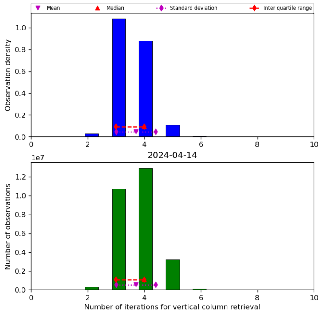
Figure 26: Histogram of “Number of iterations for vertical column retrieval” for 2024-04-13 to 2024-04-15
