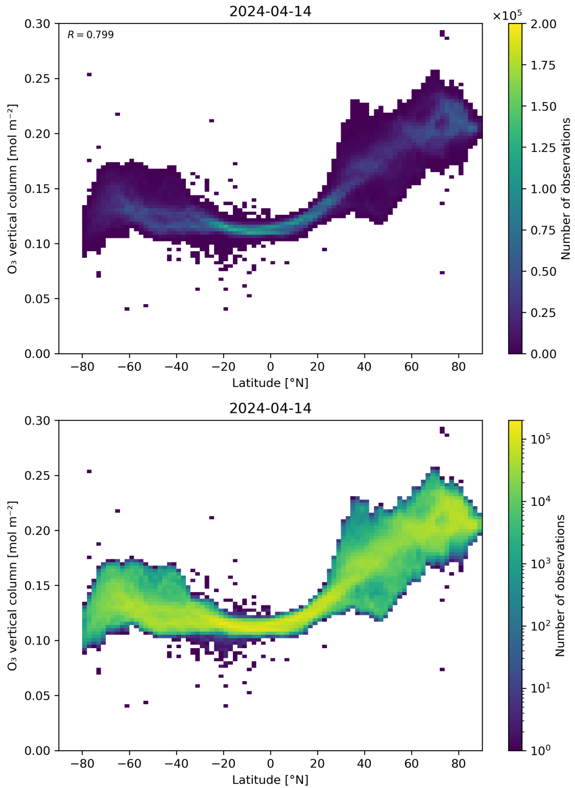
Figure 36: Scatter density plot of “Latitude” against “O 3 vertical column” for 2024-04-13 to 2024-04-15.
