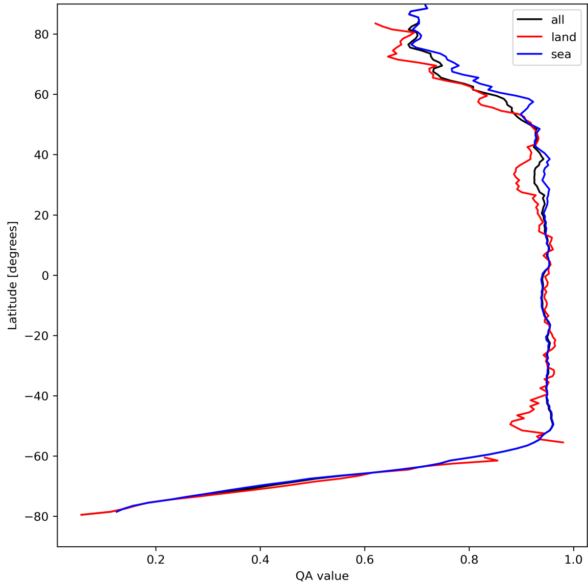
Figure 13: Zonal average of “QA value” for 2024-04-13 to 2024-04-15.
