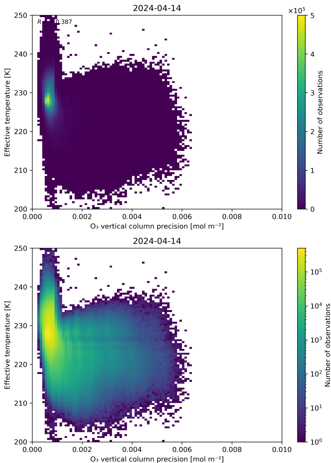
Figure 42: Scatter density plot of “O 3 vertical column precision” against “Effective temperature” for 2024-04-13 to 2024-04-15.
