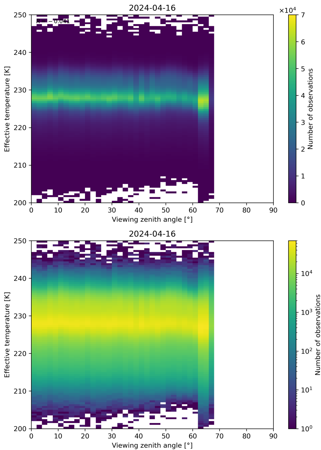
Figure 50: Scatter density plot of “Viewing zenith angle” against “Effective temperature” for 2024-04-16 to 2024-04-17.
