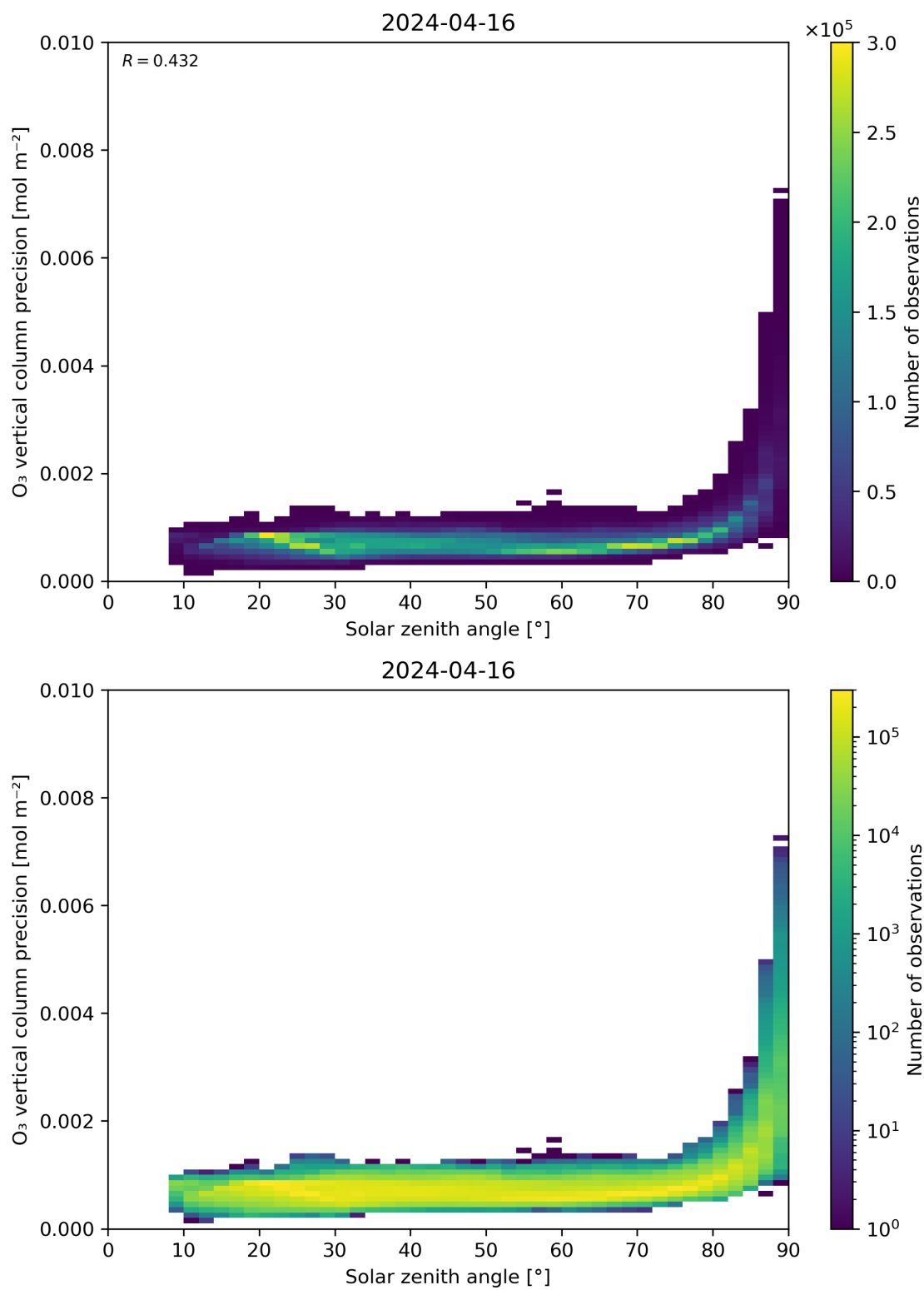
Figure 48: Scatter density plot of “Solar zenith angle” against “O 3 vertical column precision” for 2024-04-16 to 2024-04-17.
