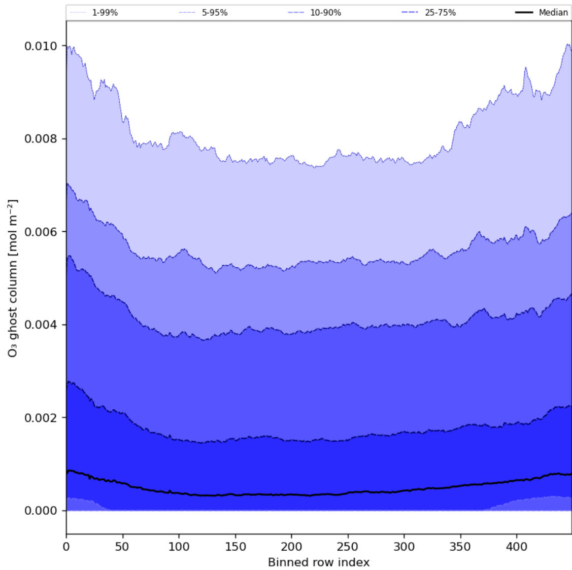
Figure 32: Along track statistics of "O 3 ghost column" for 2024-04-16 to 2024-04-17
