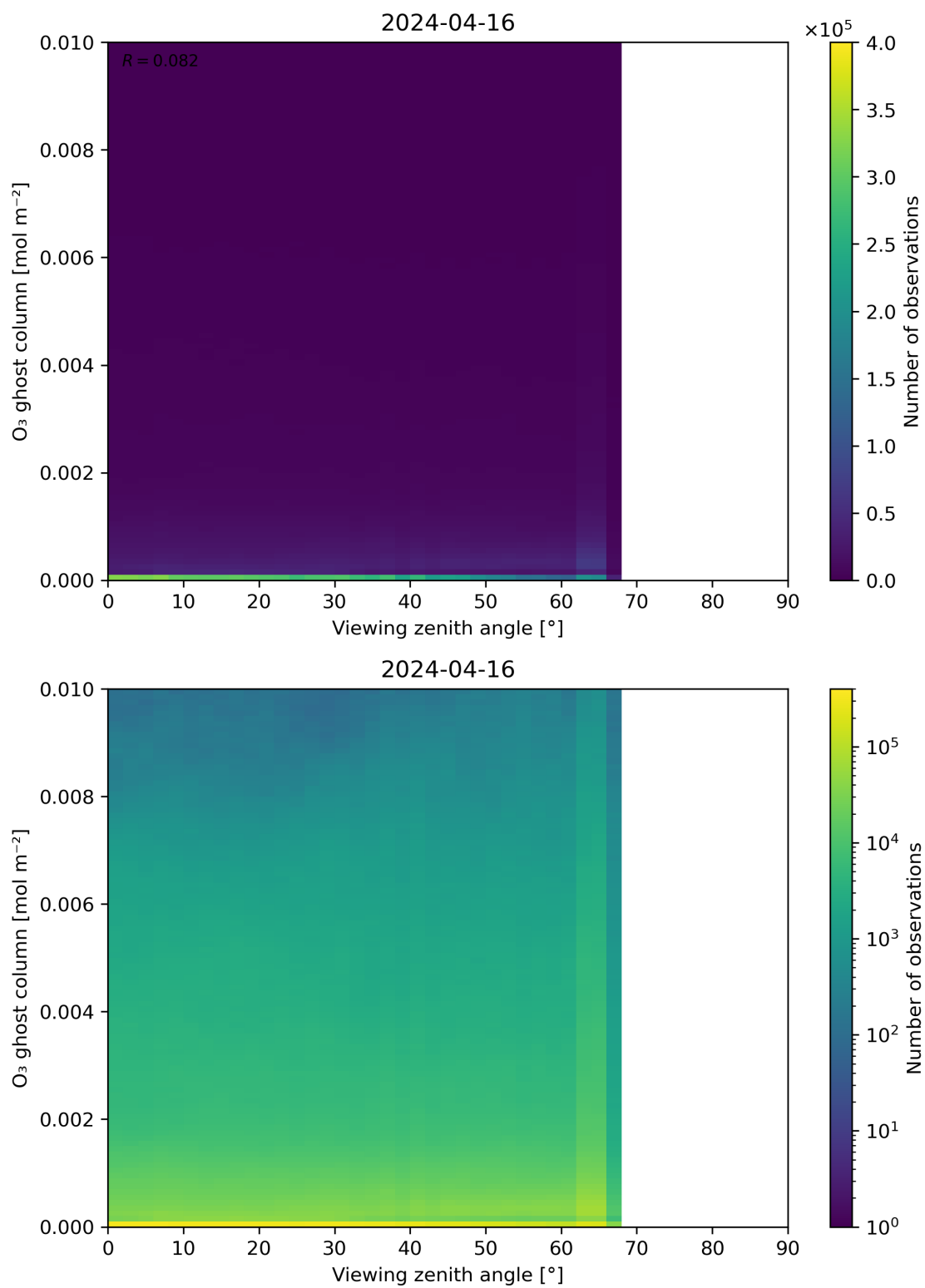
Figure 51: Scatter density plot of “Viewing zenith angle” against “O 3 ghost column” for 2024-04-16 to 2024-04-17.
