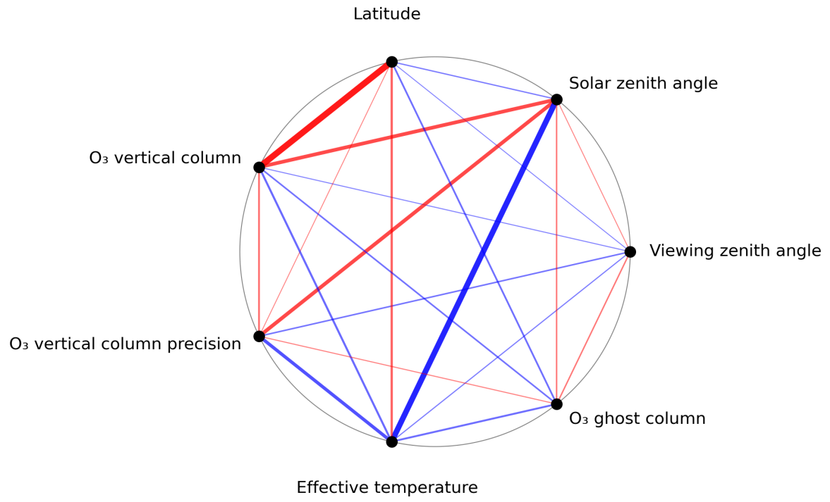
Figure 1: Map of correlation graph for 2024-04-16 to 2024-04-17.
