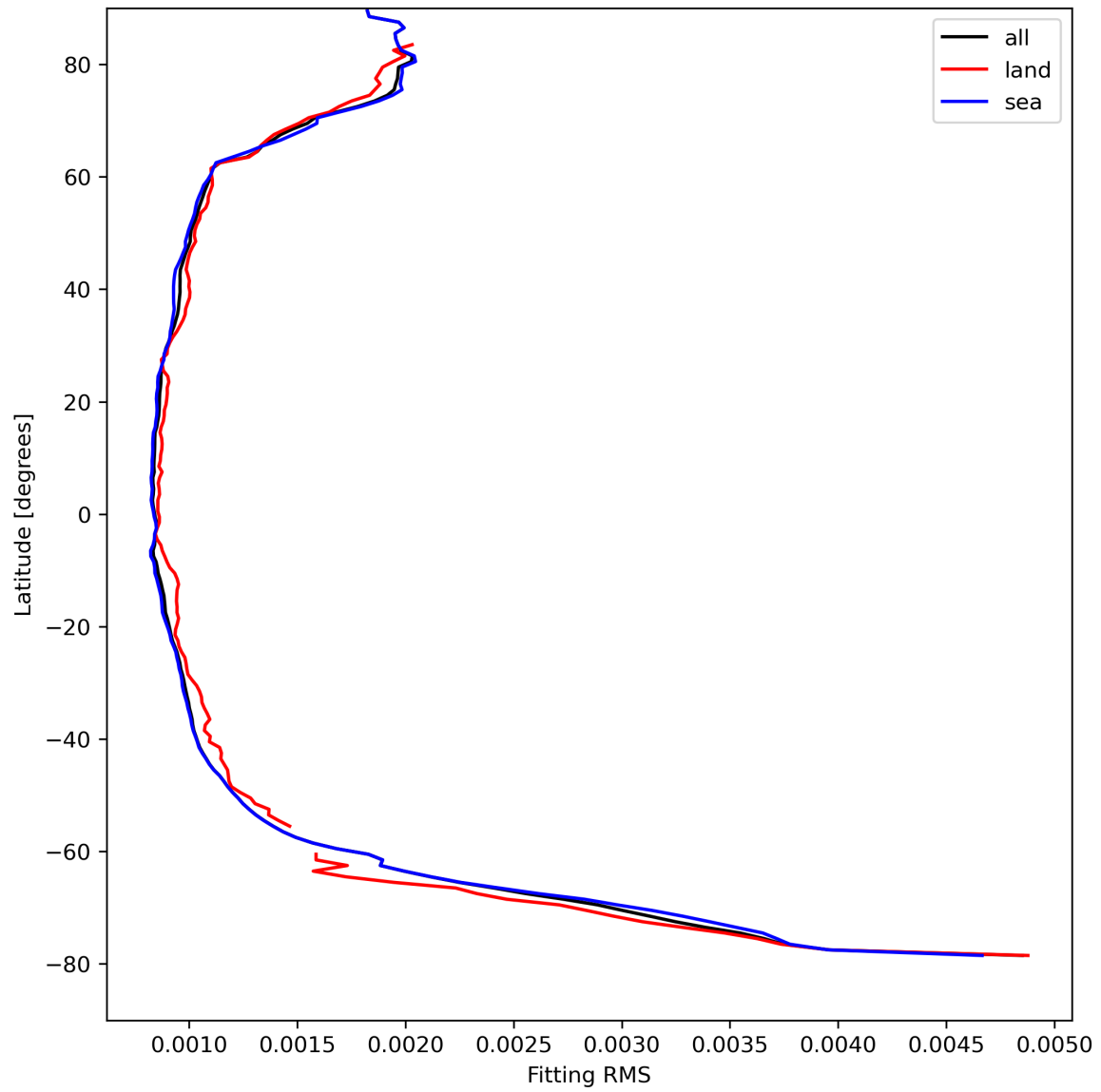
Figure 16: Zonal average of “Fitting RMS” for 2024-04-16 to 2024-04-17.
