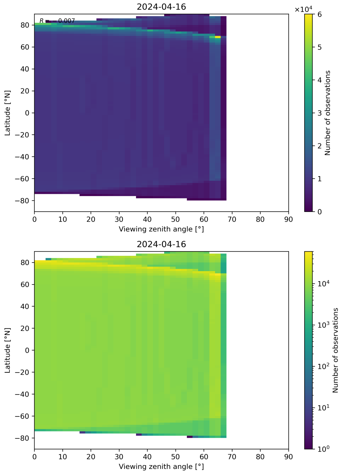
Figure 49: Scatter density plot of “Viewing zenith angle” against “Latitude” for 2024-04-16 to 2024-04-17.
