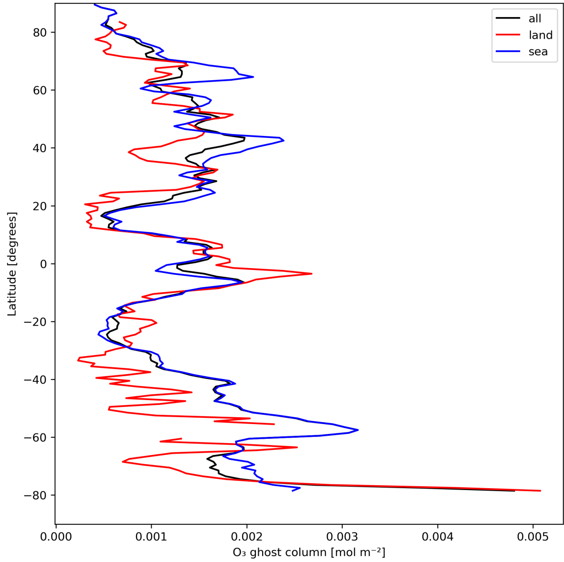
Figure 18: Zonal average of "O 3 ghost column" for 2024-04-16 to 2024-04-17.
