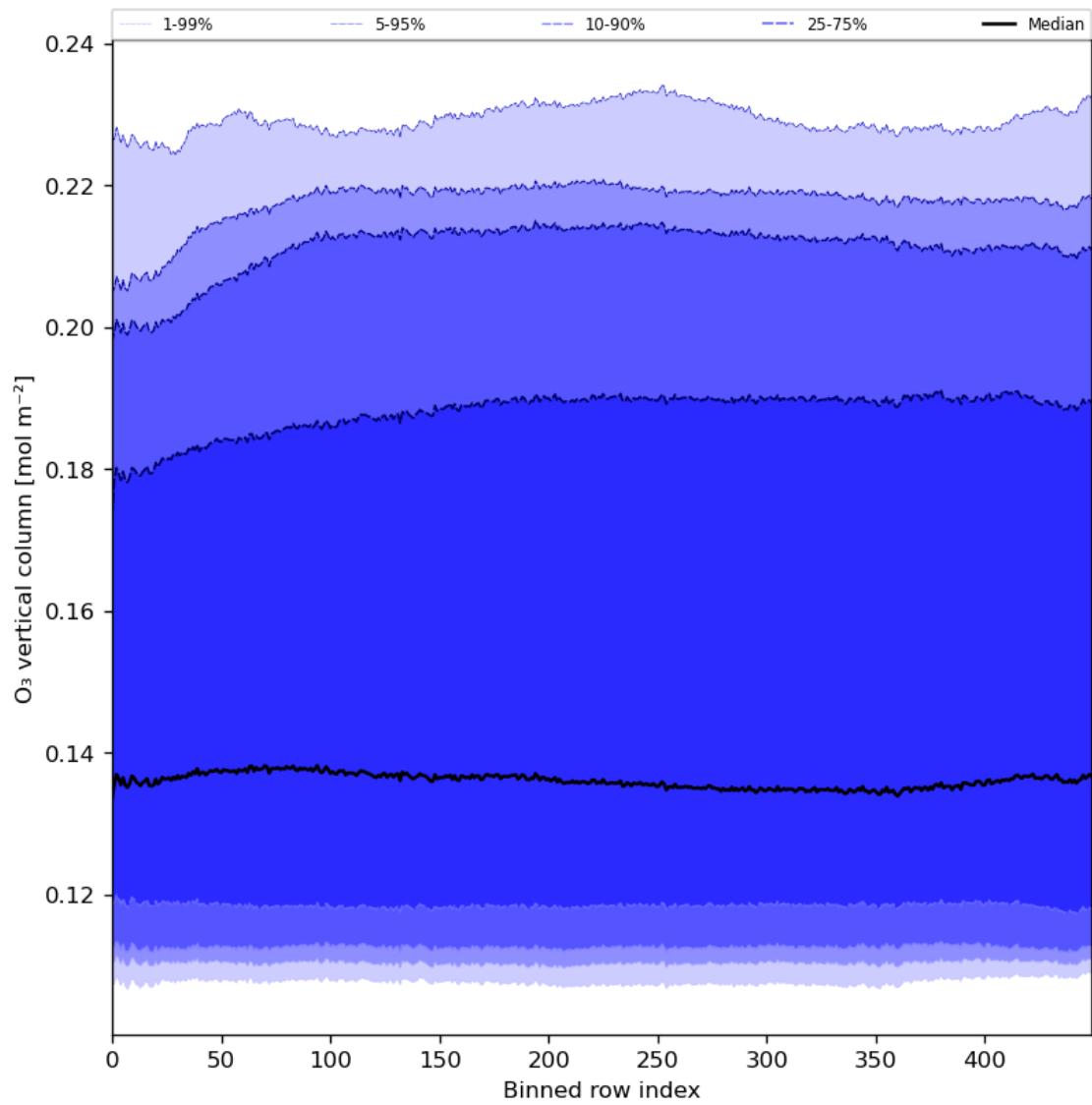
Figure 28: Along track statistics of “O 3 vertical column” for 2024-04-16 to 2024-04-17
