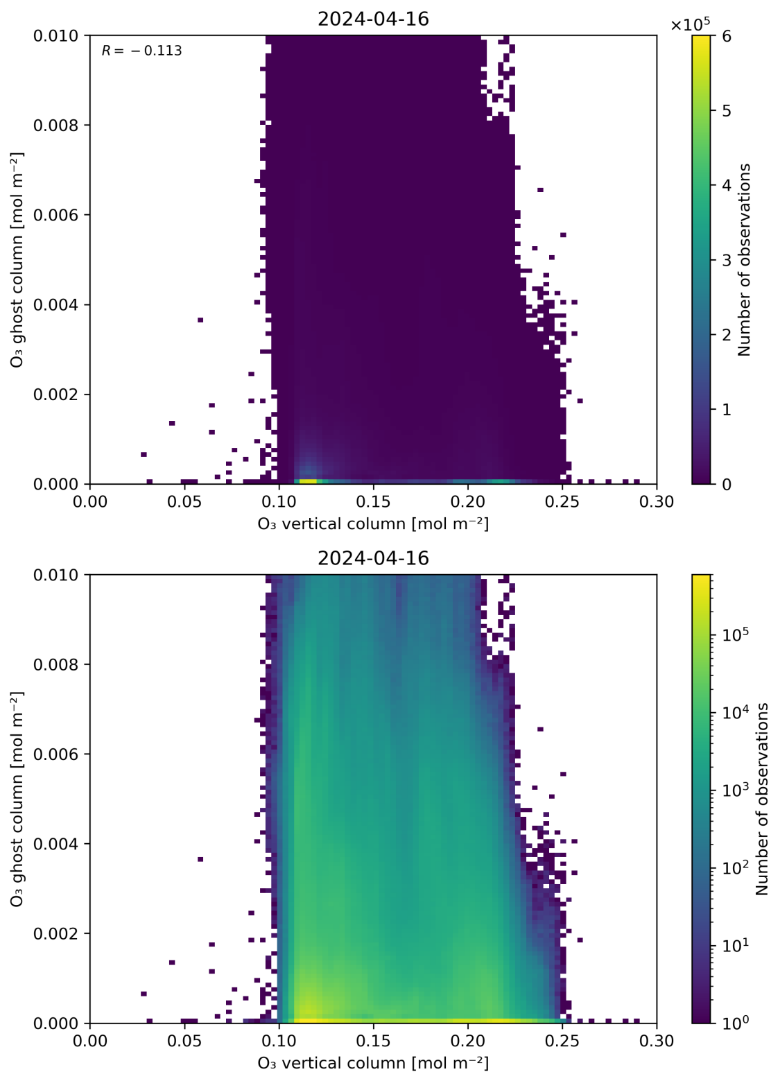
Figure 40: Scatter density plot of “O 3 vertical column” against “O 3 ghost column” for 2024-04-16 to 2024-04-17.
