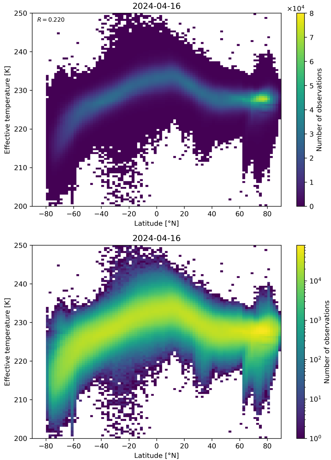
Figure 34: Scatter density plot of “Latitude” against “Effective temperature” for 2024-04-16 to 2024-04-17.
