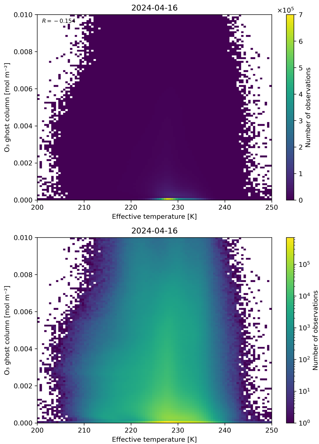
Figure 38: Scatter density plot of “Effective temperature” against “O 3 ghost column” for 2024-04-16 to 2024-04-17.
