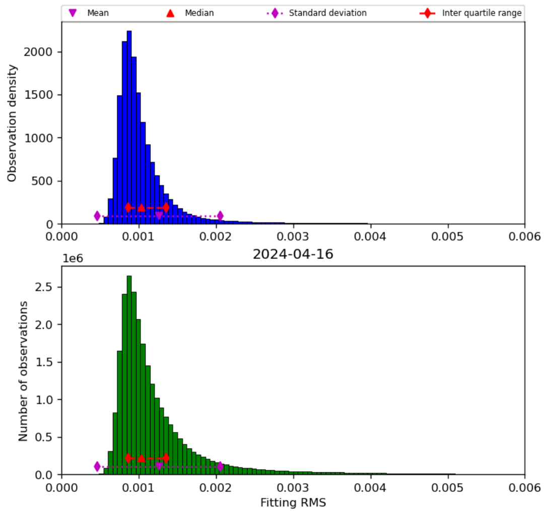
Figure 23: Histogram of “Fitting RMS” for 2024-04-16 to 2024-04-17
