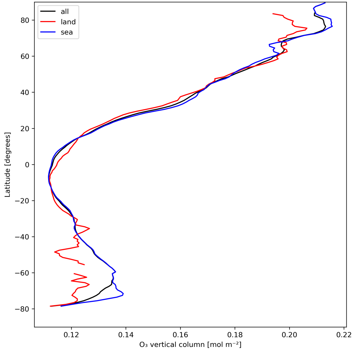
Figure 14: Zonal average of “O 3 vertical column” for 2024-04-16 to 2024-04-17.
