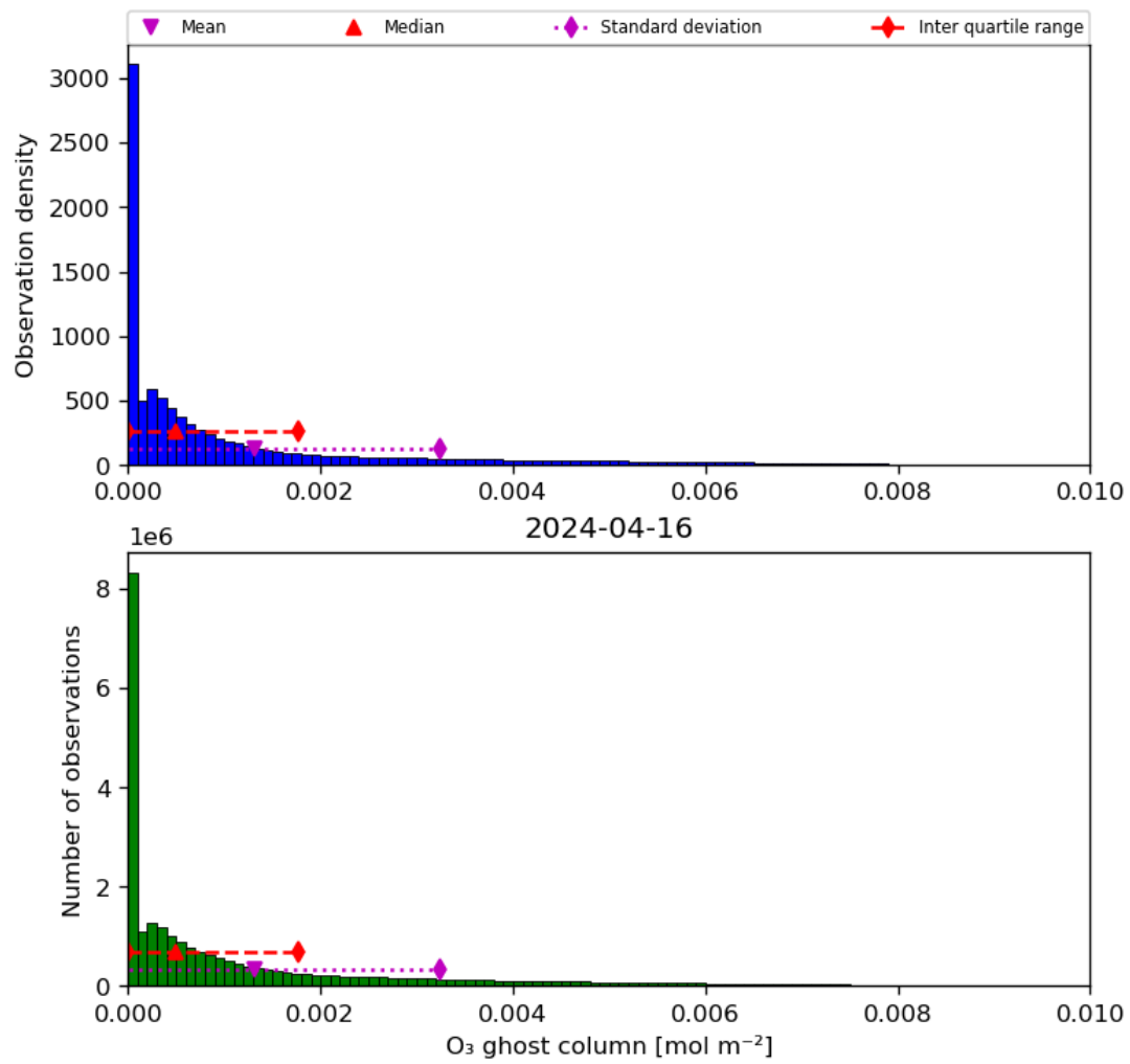
Figure 25: Histogram of “O 3 ghost column” for 2024-04-16 to 2024-04-17
