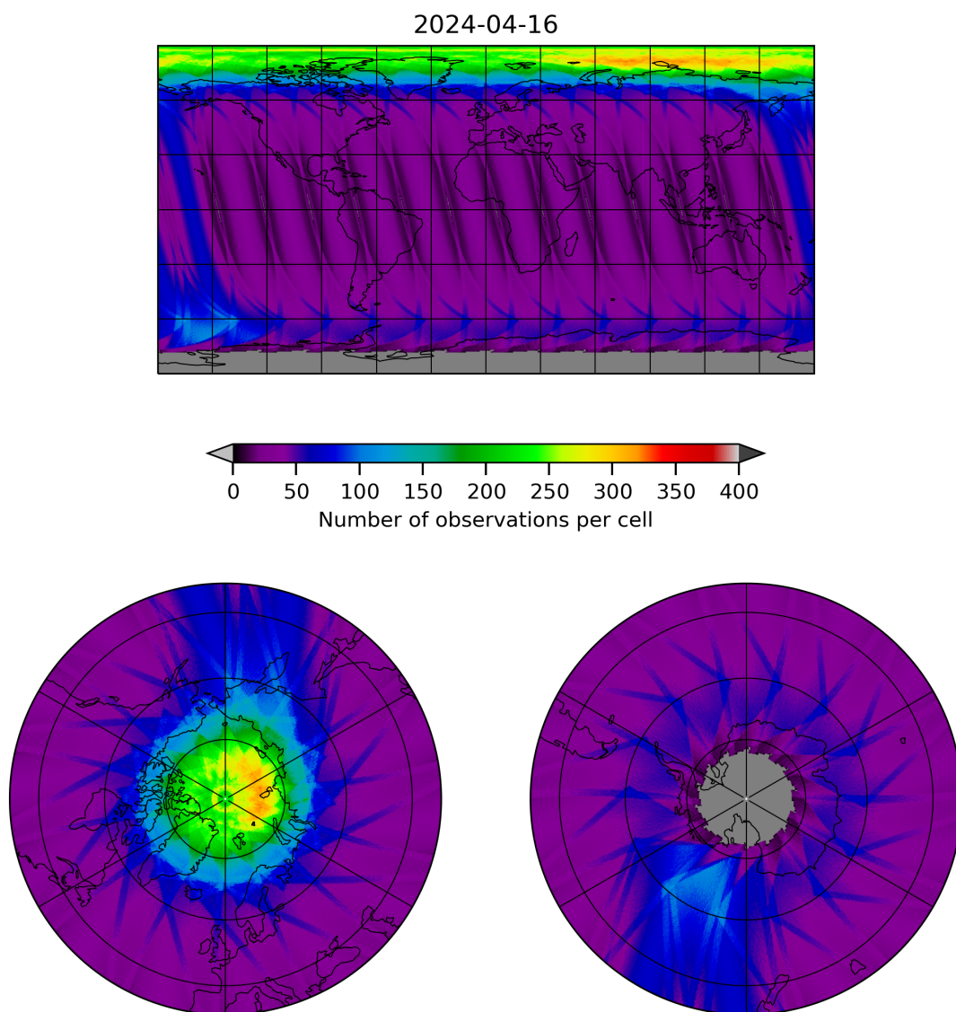
Figure 12: Map of the number of observations for 2024-04-16 to 2024-04-17
