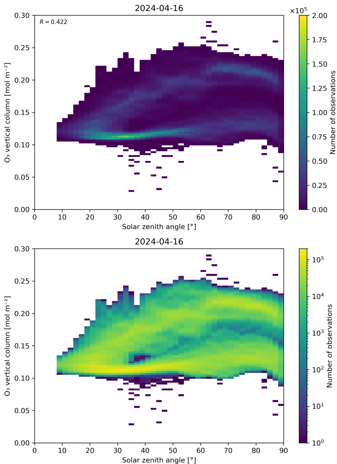
Figure 47: Scatter density plot of “Solar zenith angle” against “O 3 vertical column” for 2024-04-16 to 2024-04-17.
