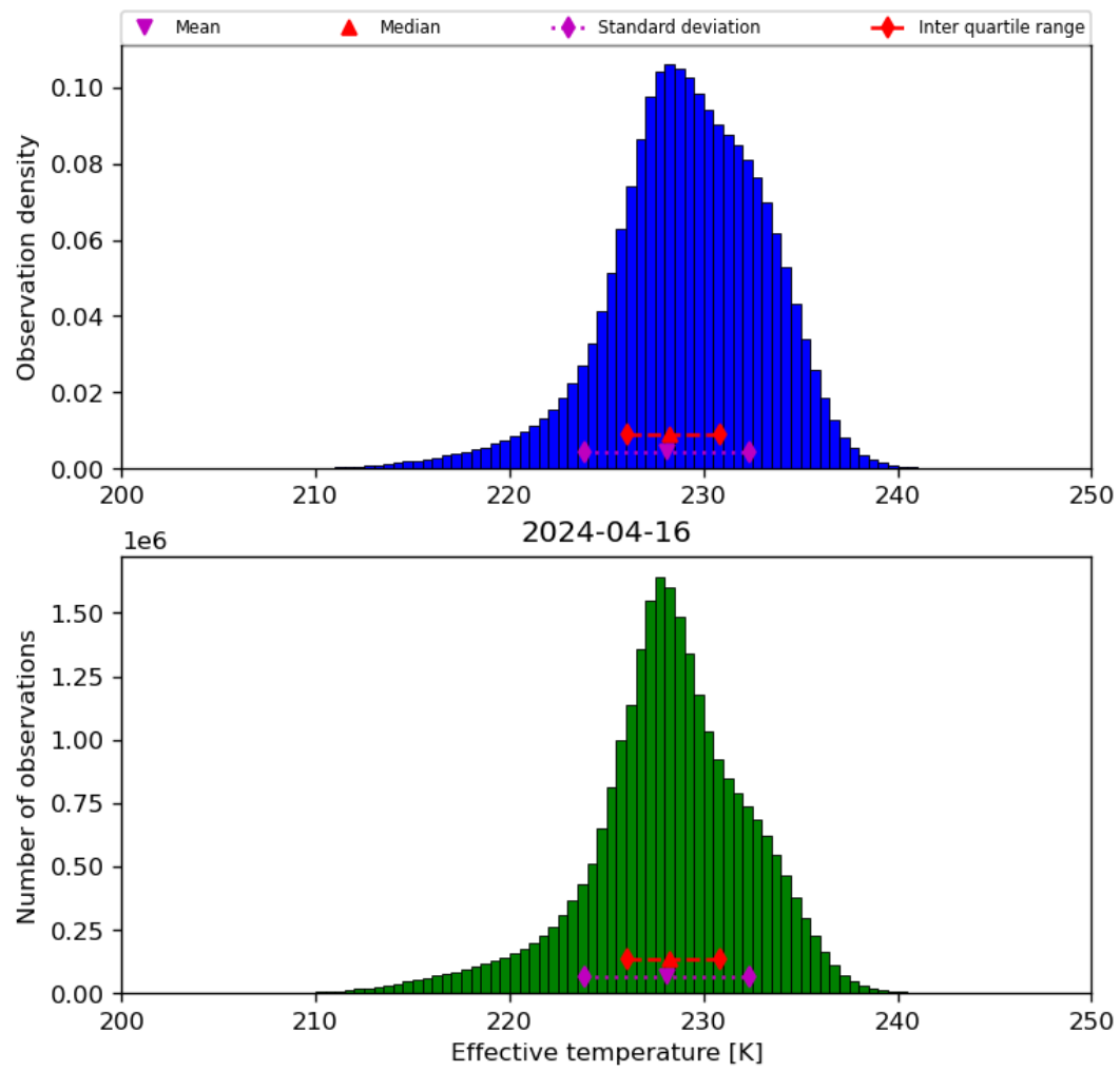
Figure 24: Histogram of “Effective temperature” for 2024-04-16 to 2024-04-17
