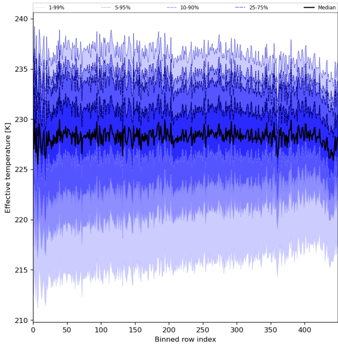
Figure 31: Along track statistics of “Effective temperature” for 2024-04-16 to 2024-04-17
