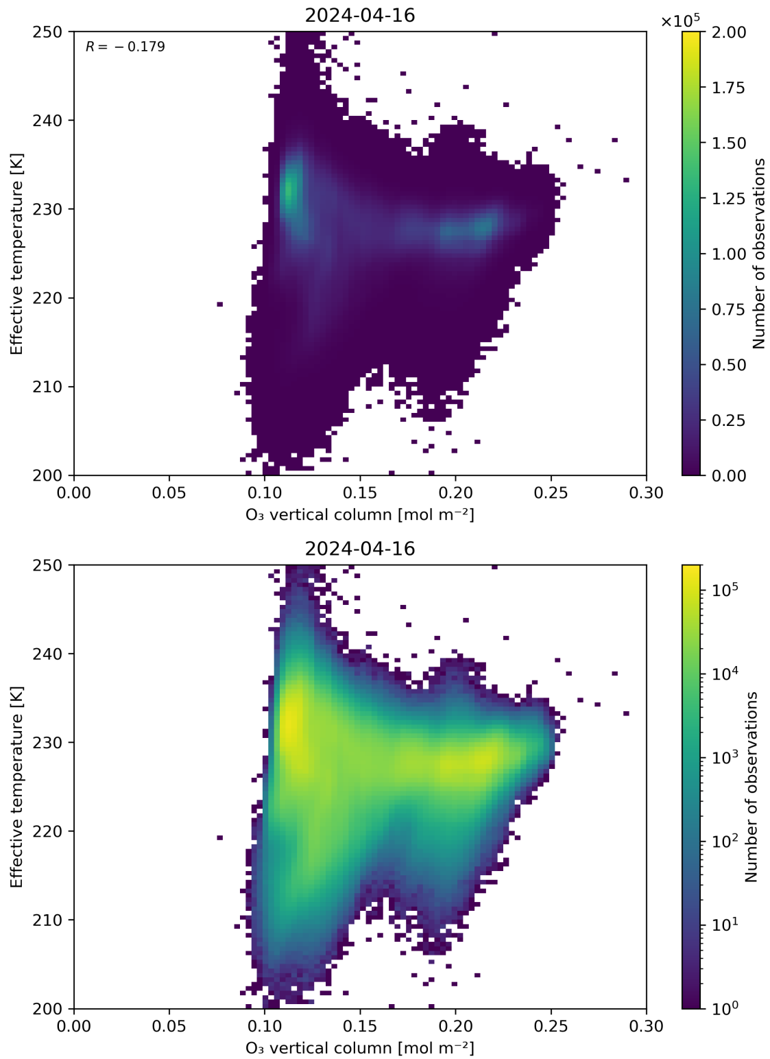
Figure 39: Scatter density plot of “O 3 vertical column” against “Effective temperature” for 2024-04-16 to 2024-04-17.
