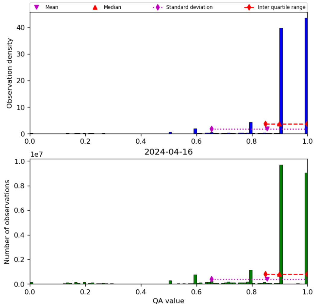
Figure 20: Histogram of “QA value” for 2024-04-16 to 2024-04-17
