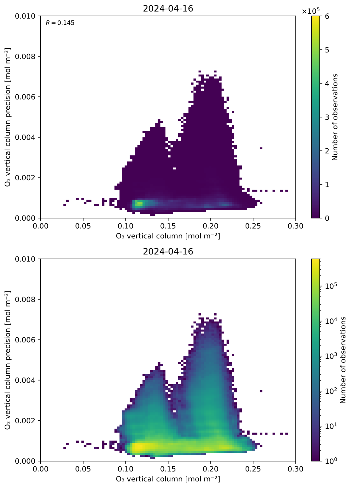
Figure 41: Scatter density plot of “O 3 vertical column” against “O 3 vertical column precision” for 2024-04-16 to 2024-04-17.
