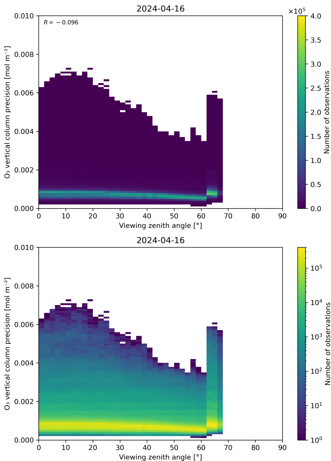
Figure 53: Scatter density plot of “Viewing zenith angle” against “O 3 vertical column precision” for 2024-04-16 to 2024-04-17.
