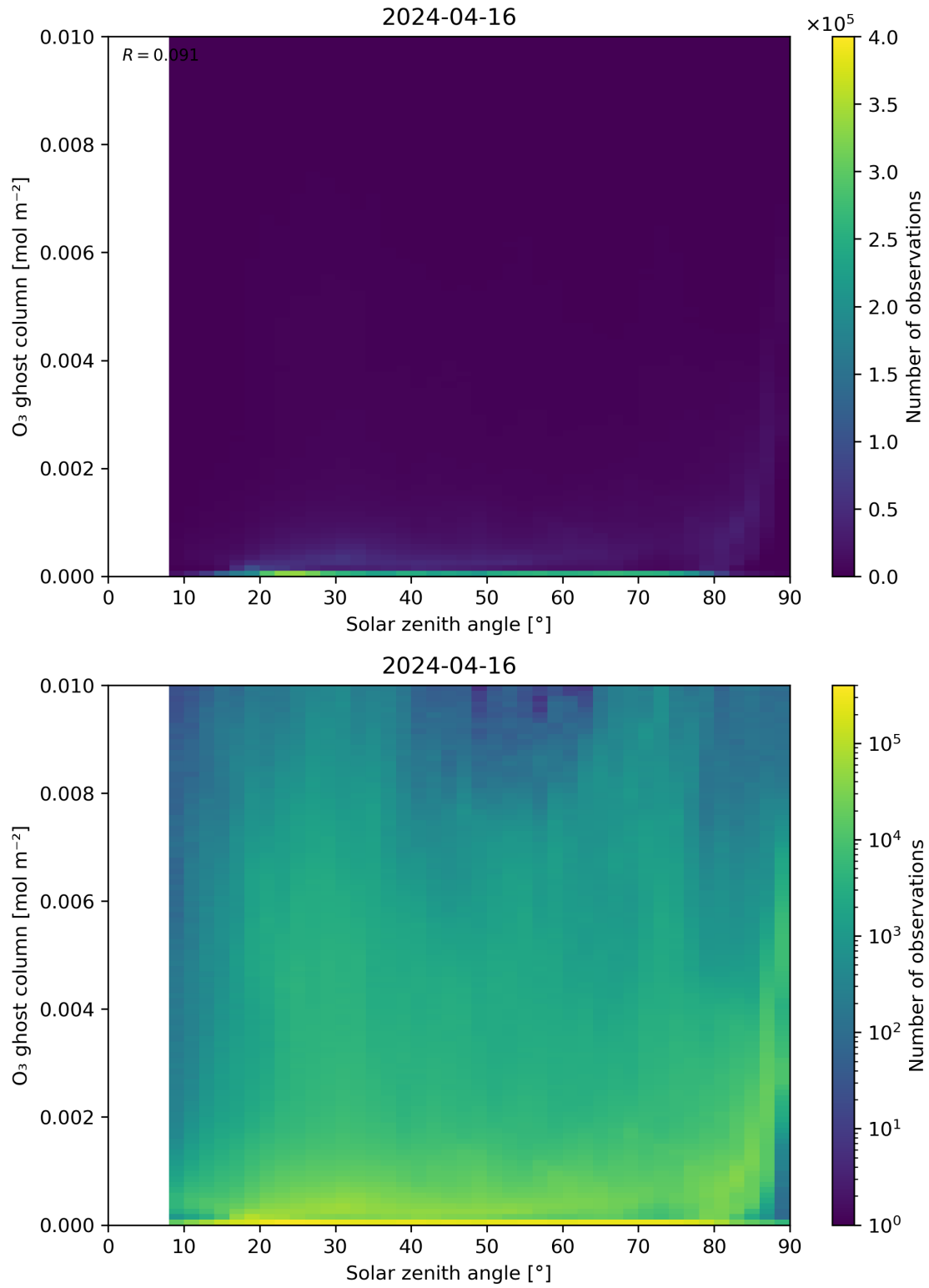
Figure 46: Scatter density plot of “Solar zenith angle” against “O 3 ghost column” for 2024-04-16 to 2024-04-17.
