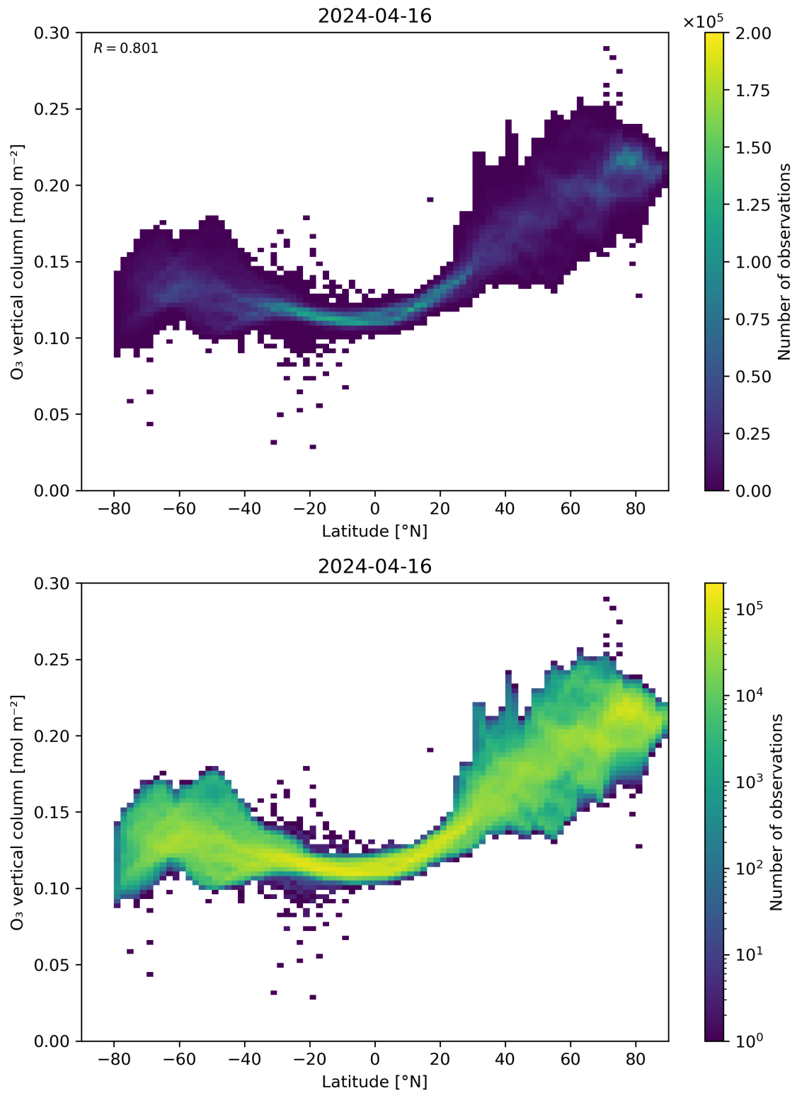
Figure 36: Scatter density plot of “Latitude” against “O 3 vertical column” for 2024-04-16 to 2024-04-17.
