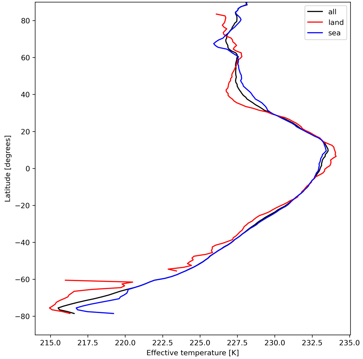
Figure 17: Zonal average of “Effective temperature” for 2024-04-16 to 2024-04-17.
