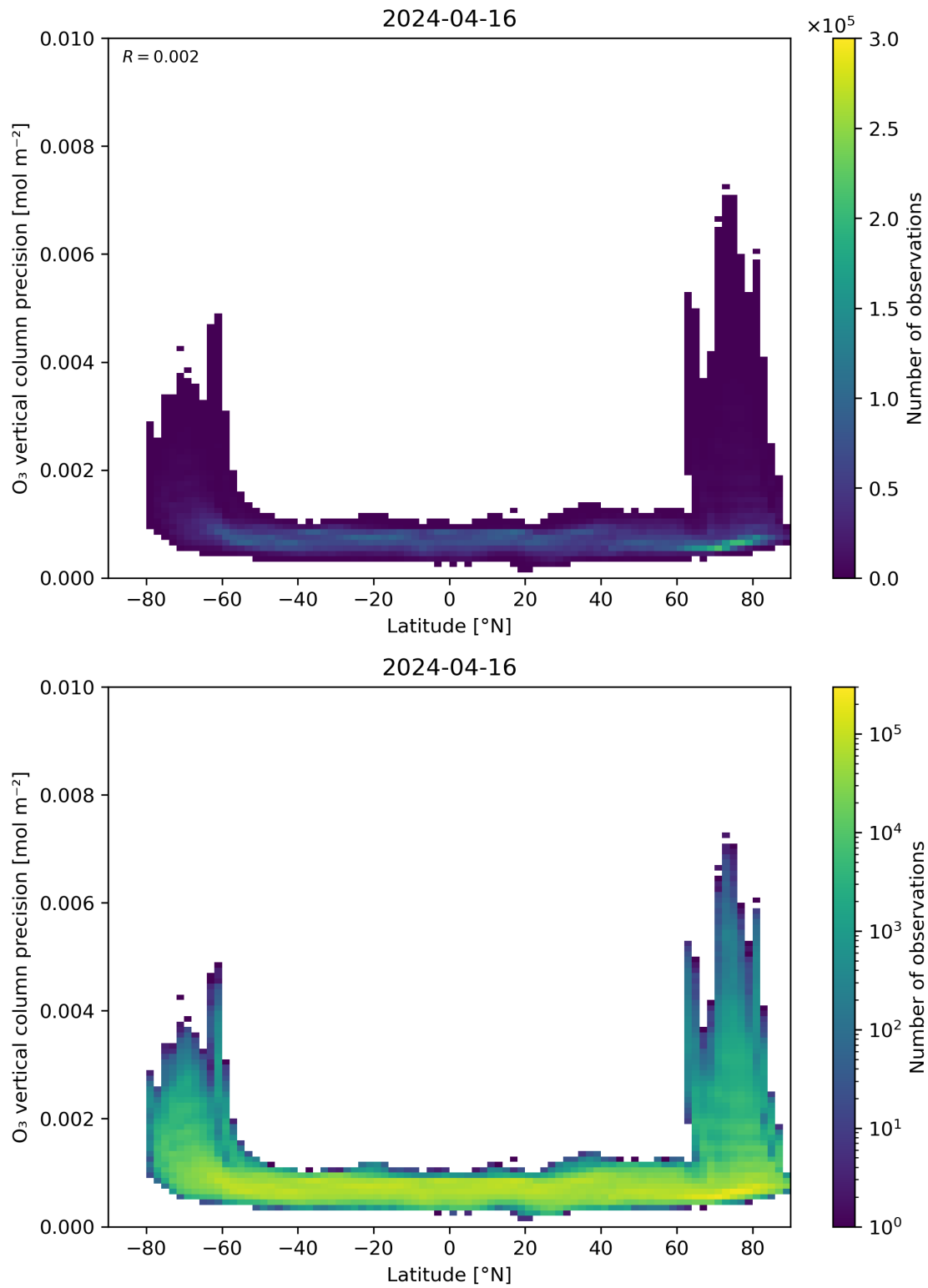
Figure 37: Scatter density plot of “Latitude” against “O 3 vertical column precision” for 2024-04-16 to 2024-04-17.
