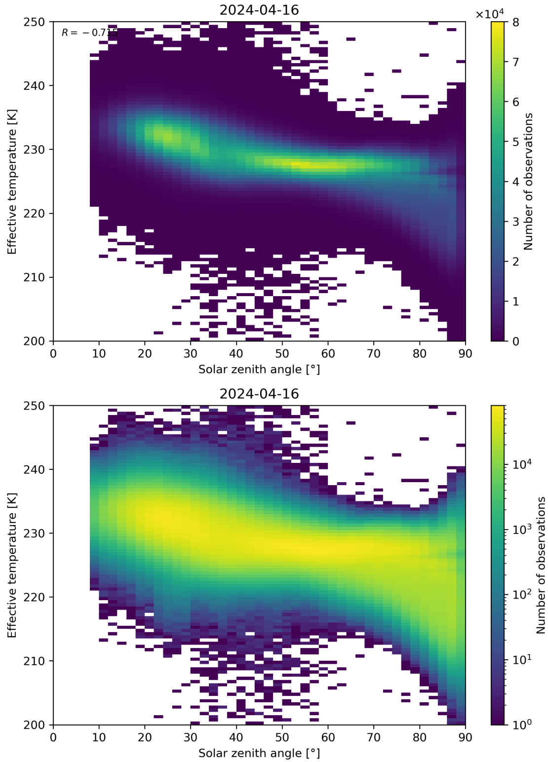
Figure 45: Scatter density plot of “Solar zenith angle” against “Effective temperature” for 2024-04-16 to 2024-04-17.
