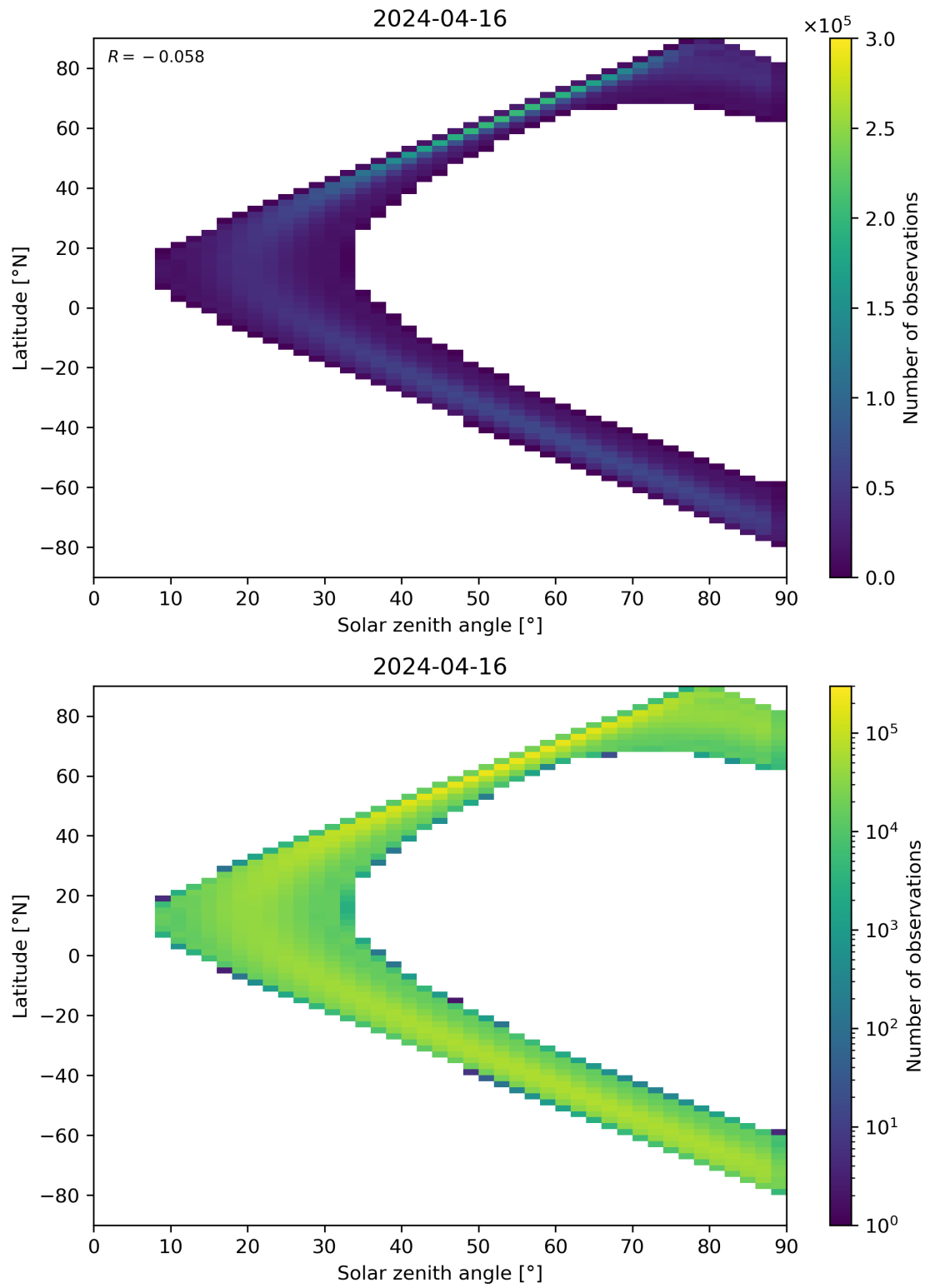
Figure 44: Scatter density plot of “Solar zenith angle” against “Latitude” for 2024-04-16 to 2024-04-17.
