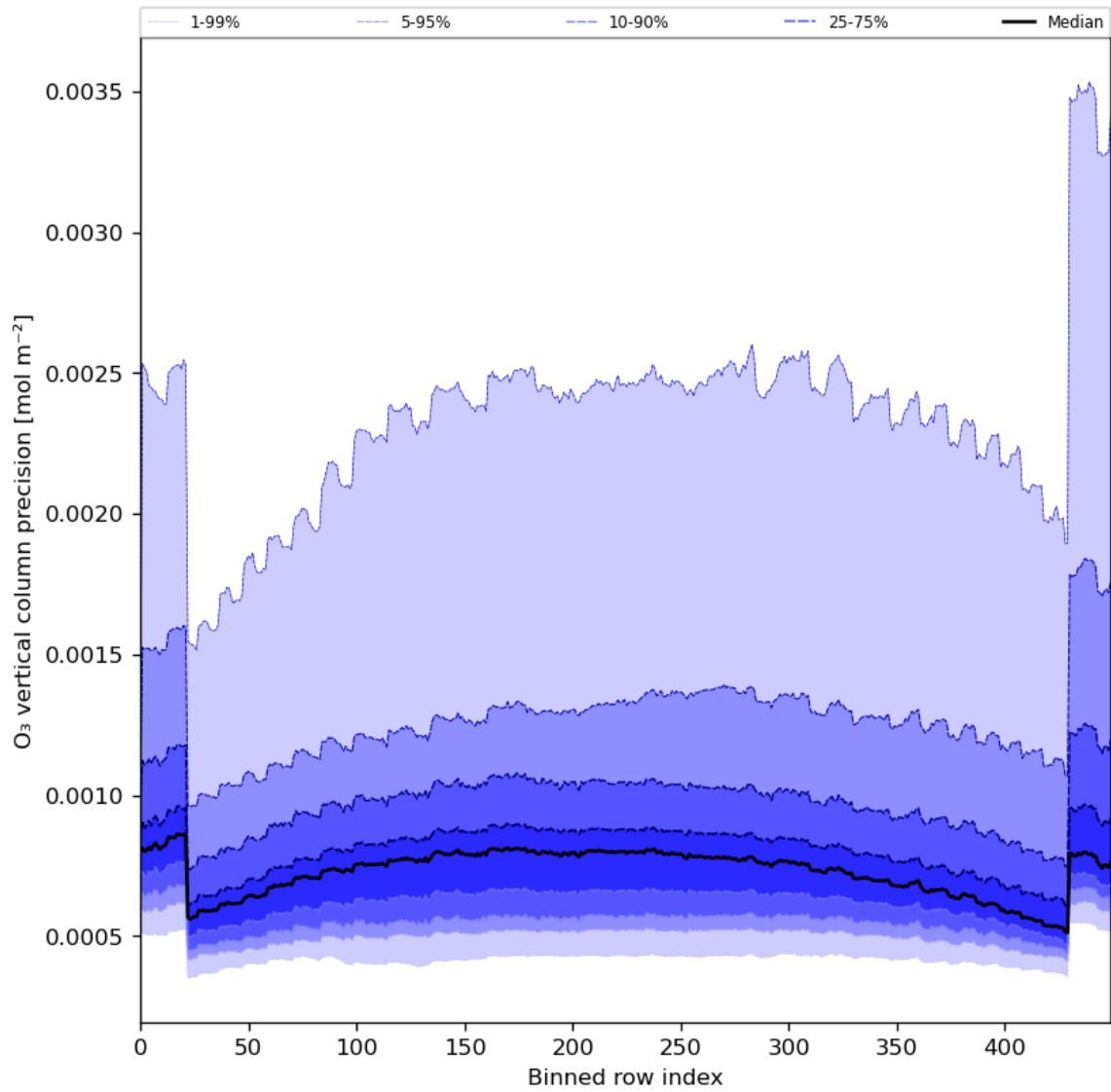
Figure 29: Along track statistics of “O 3 vertical column precision” for 2024-04-16 to 2024-04-17
