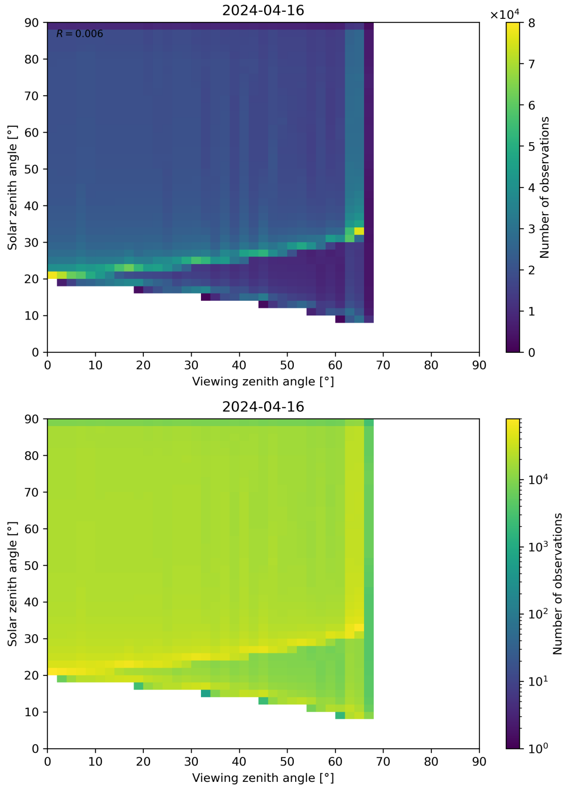
Figure 54: Scatter density plot of “Viewing zenith angle” against “Solar zenith angle” for 2024-04-16 to 2024-04-17.
