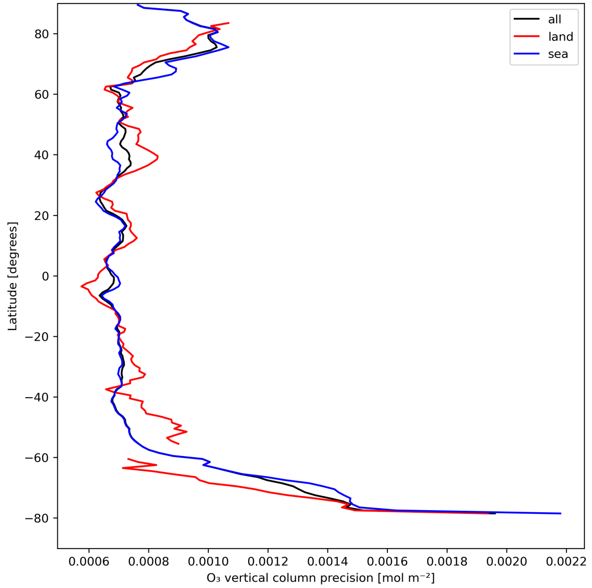
Figure 15: Zonal average of “O 3 vertical column precision” for 2024-04-16 to 2024-04-17.
