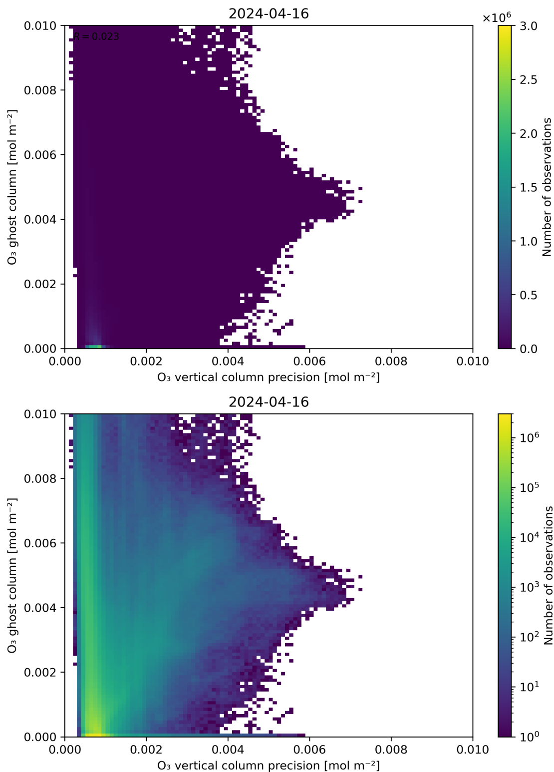
Figure 43: Scatter density plot of “ \text{O}_3 vertical column precision” against “ \text{O}_3 ghost column” for 2024-04-16 to 2024-04-17.
