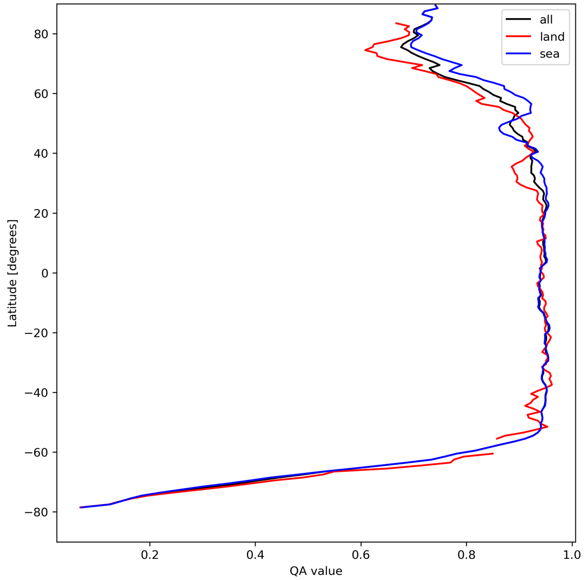
Figure 13: Zonal average of “QA value” for 2024-04-16 to 2024-04-17.
