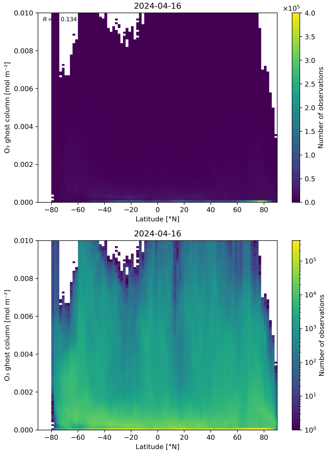
Figure 35: Scatter density plot of “Latitude” against “O 3 ghost column” for 2024-04-16 to 2024-04-17.
