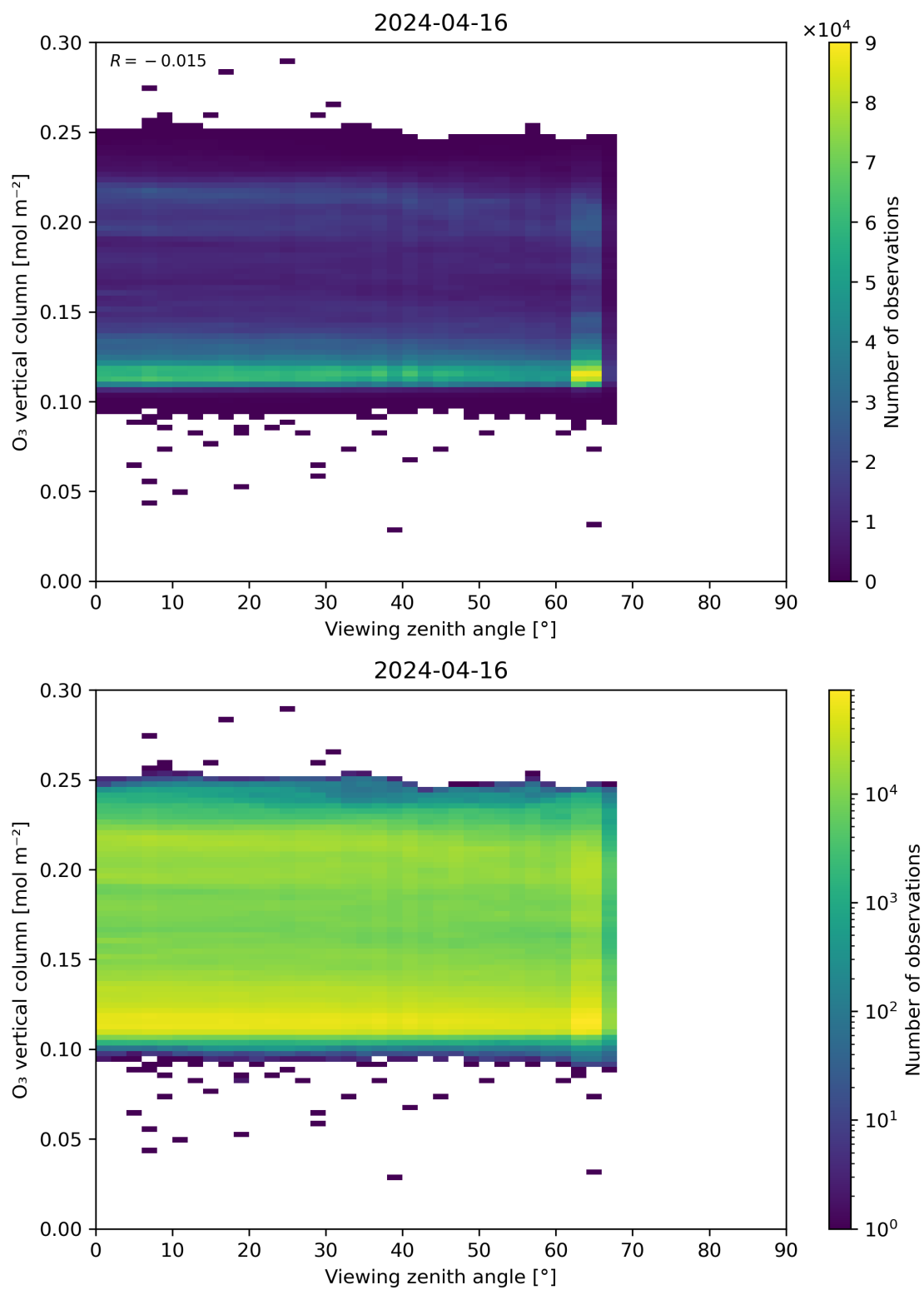
Figure 52: Scatter density plot of “Viewing zenith angle” against “O 3 vertical column” for 2024-04-16 to 2024-04-17.
