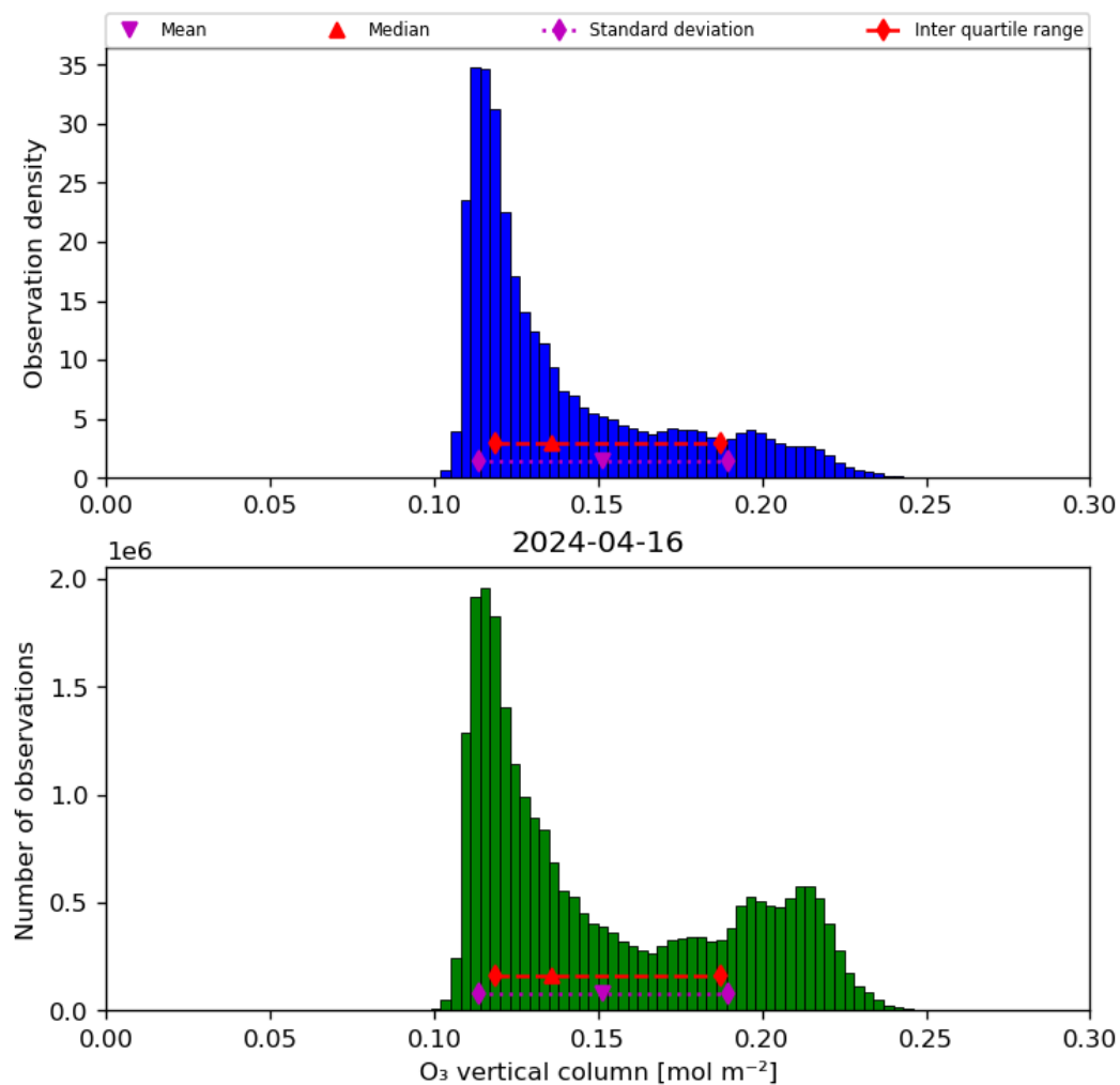
Figure 21: Histogram of “O 3 vertical column” for 2024-04-16 to 2024-04-17
