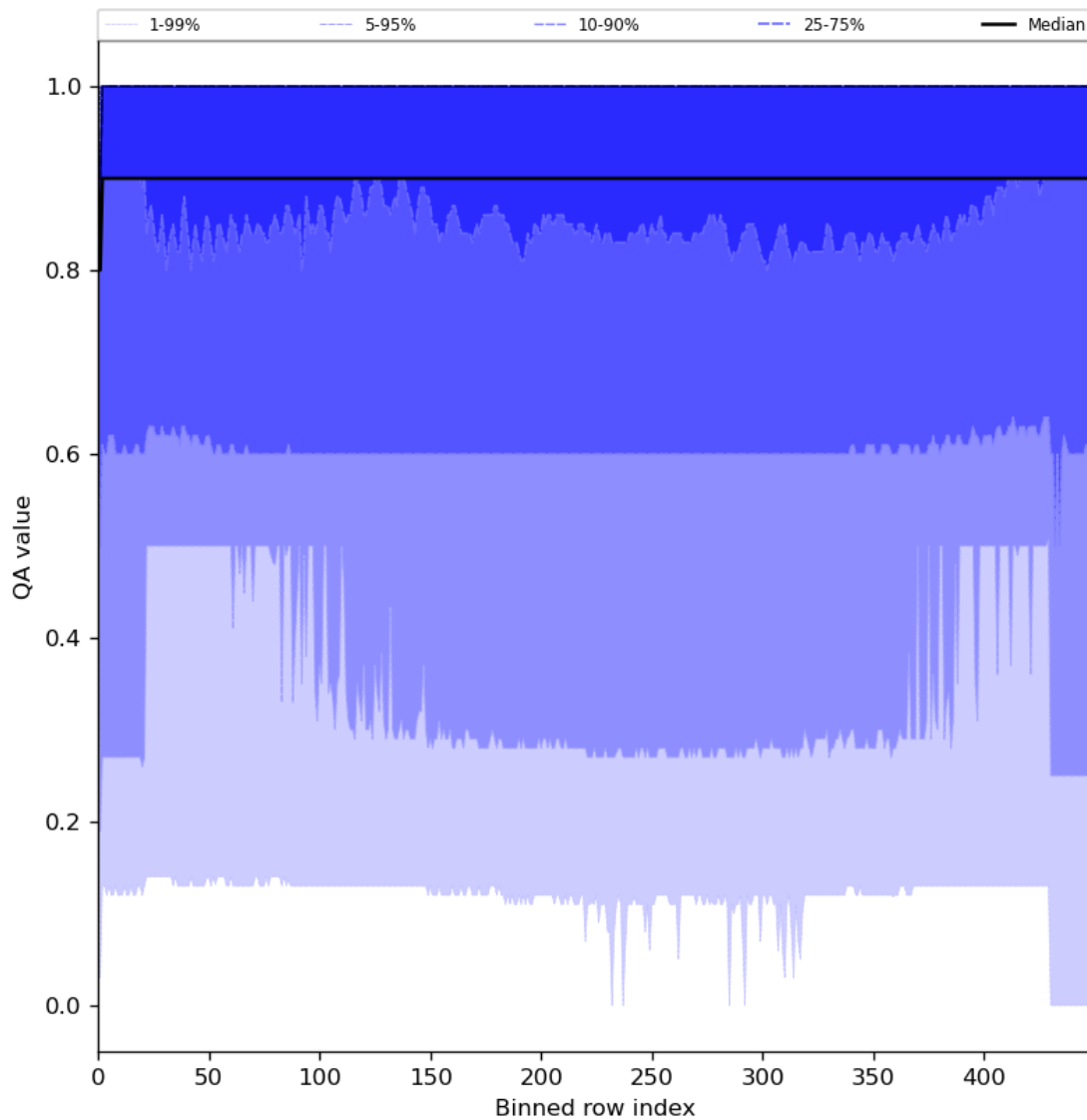
Figure 27: Along track statistics of “QA value” for 2024-04-16 to 2024-04-17
