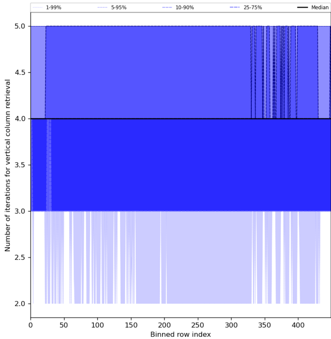
Figure 33: Along track statistics of “Number of iterations for vertical column retrieval” for 2024-04-16 to 2024-04-17
