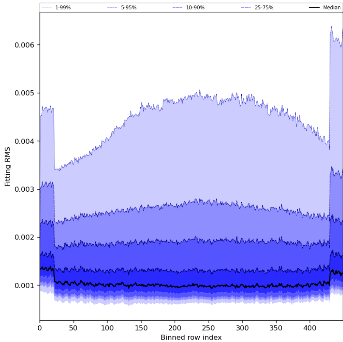
Figure 30: Along track statistics of “Fitting RMS” for 2024-04-16 to 2024-04-17
