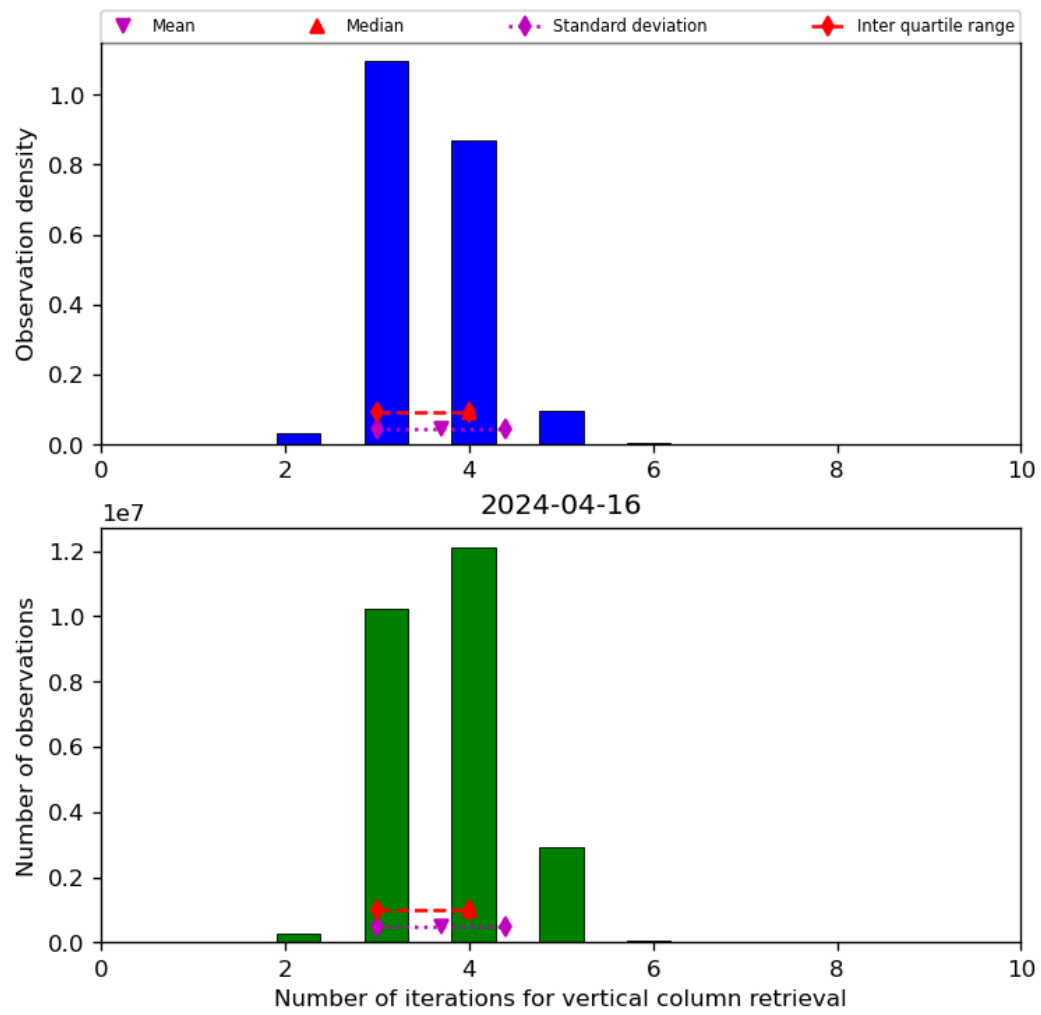
Figure 26: Histogram of “Number of iterations for vertical column retrieval” for 2024-04-16 to 2024-04-17
