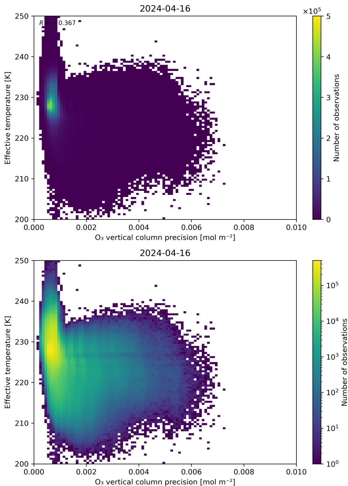
Figure 42: Scatter density plot of “O 3 vertical column precision” against “Effective temperature” for 2024-04-16 to 2024-04-17.
