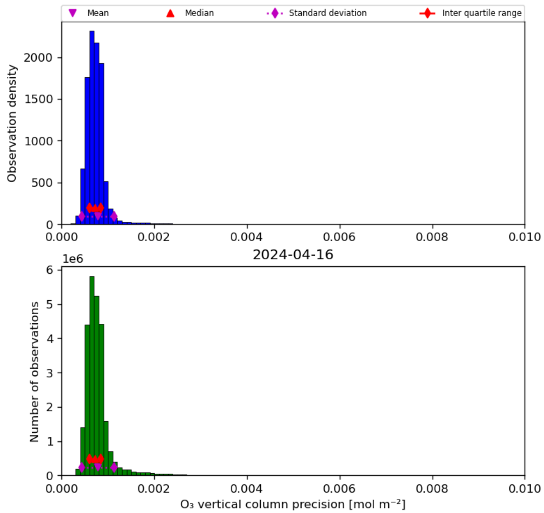
Figure 22: Histogram of “O 3 vertical column precision” for 2024-04-16 to 2024-04-17
