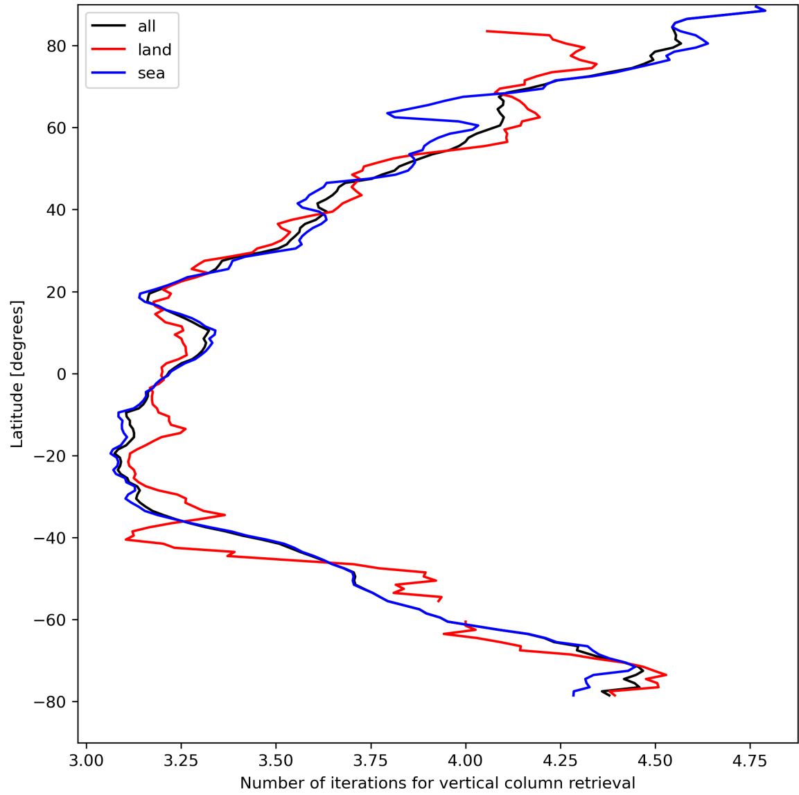
Figure 19: Zonal average of “Number of iterations for vertical column retrieval” for 2024-04-16 to 2024-04-17.
