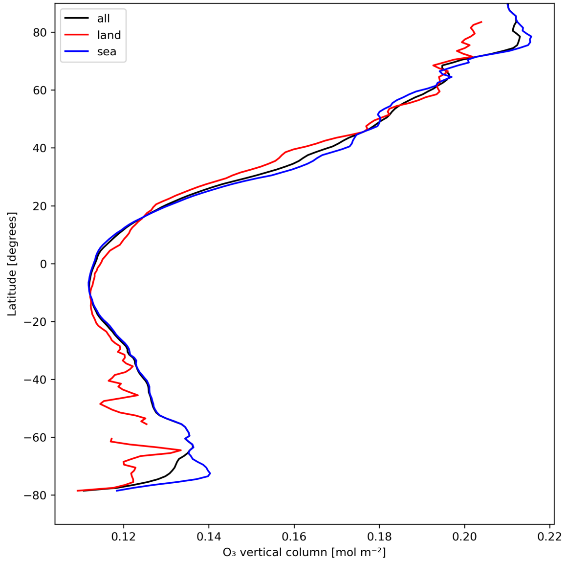
Figure 14: Zonal average of “O 3 vertical column” for 2024-04-16 to 2024-04-18.
