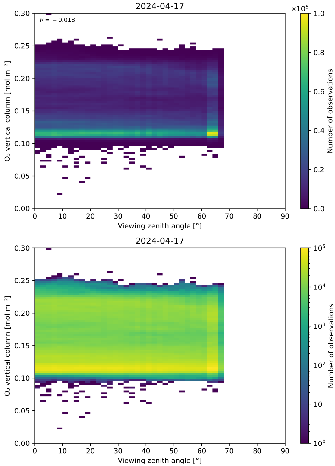
Figure 52: Scatter density plot of “Viewing zenith angle” against “O 3 vertical column” for 2024-04-16 to 2024-04-18.
