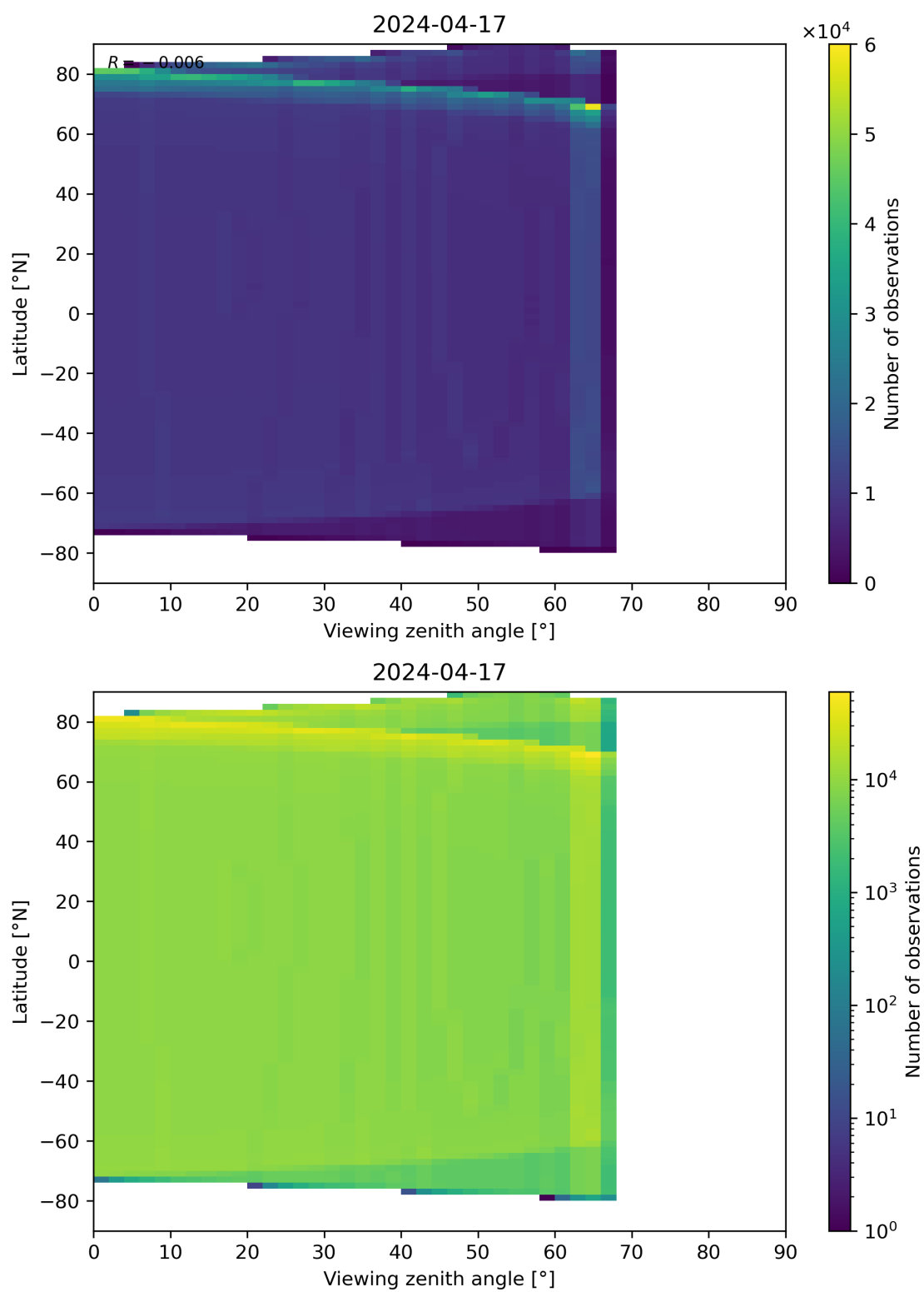
Figure 49: Scatter density plot of “Viewing zenith angle” against “Latitude” for 2024-04-16 to 2024-04-18.
