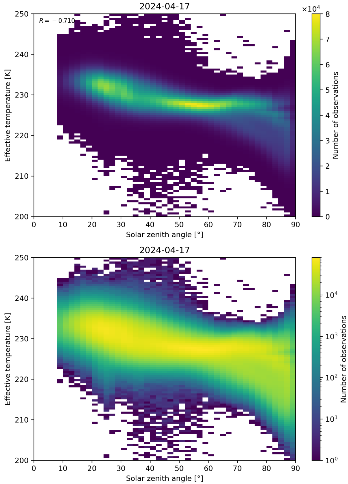
Figure 45: Scatter density plot of “Solar zenith angle” against “Effective temperature” for 2024-04-16 to 2024-04-18.
