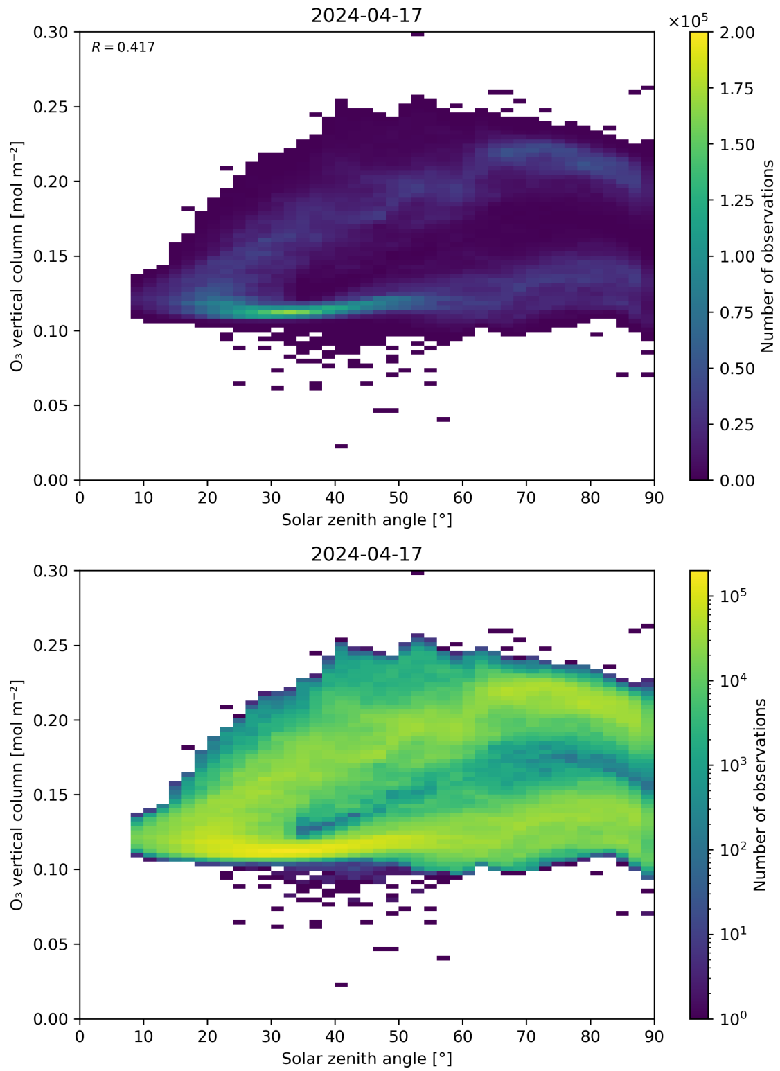
Figure 47: Scatter density plot of “Solar zenith angle” against “O 3 vertical column” for 2024-04-16 to 2024-04-18.
