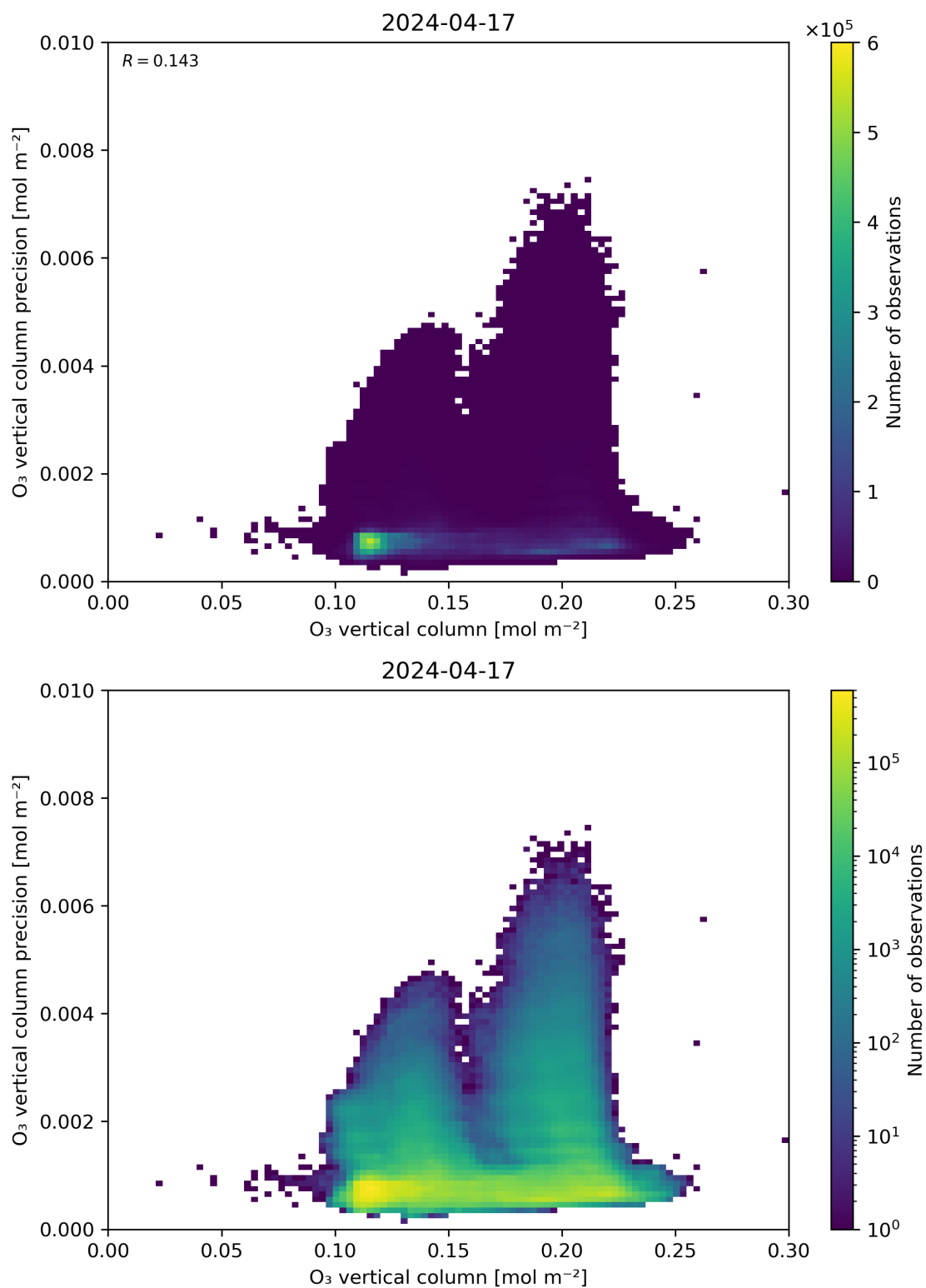
Figure 41: Scatter density plot of “O 3 vertical column” against “O 3 vertical column precision” for 2024-04-16 to 2024-04-18.
