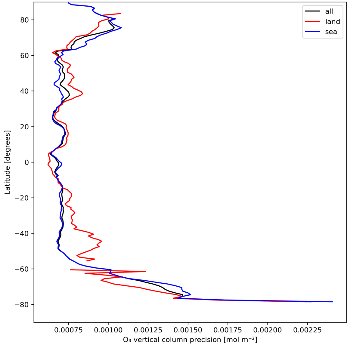
Figure 15: Zonal average of “O 3 vertical column precision” for 2024-04-16 to 2024-04-18.
