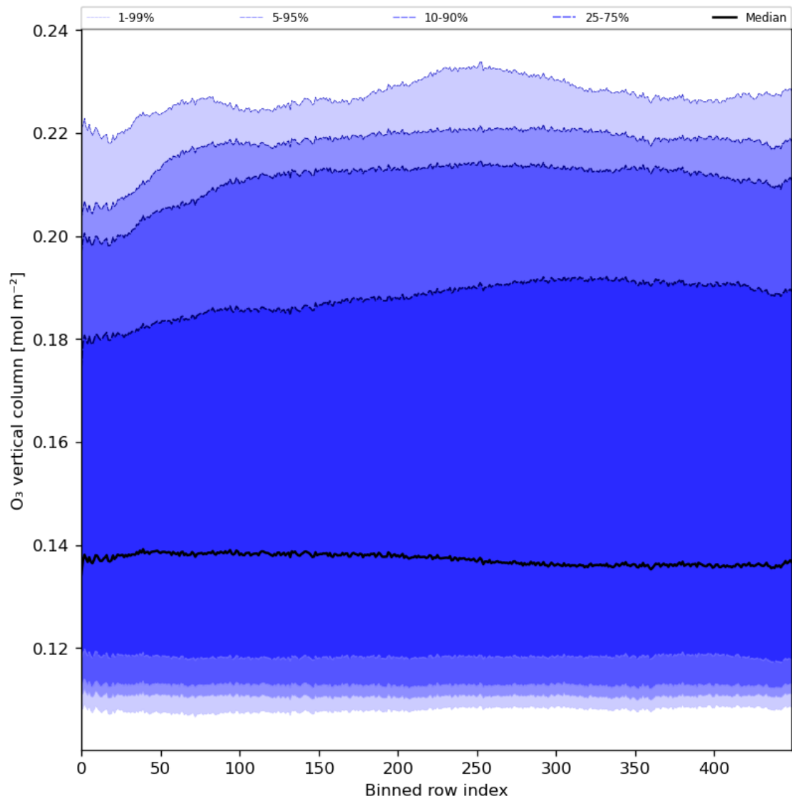
Figure 28: Along track statistics of “O 3 vertical column” for 2024-04-16 to 2024-04-18
