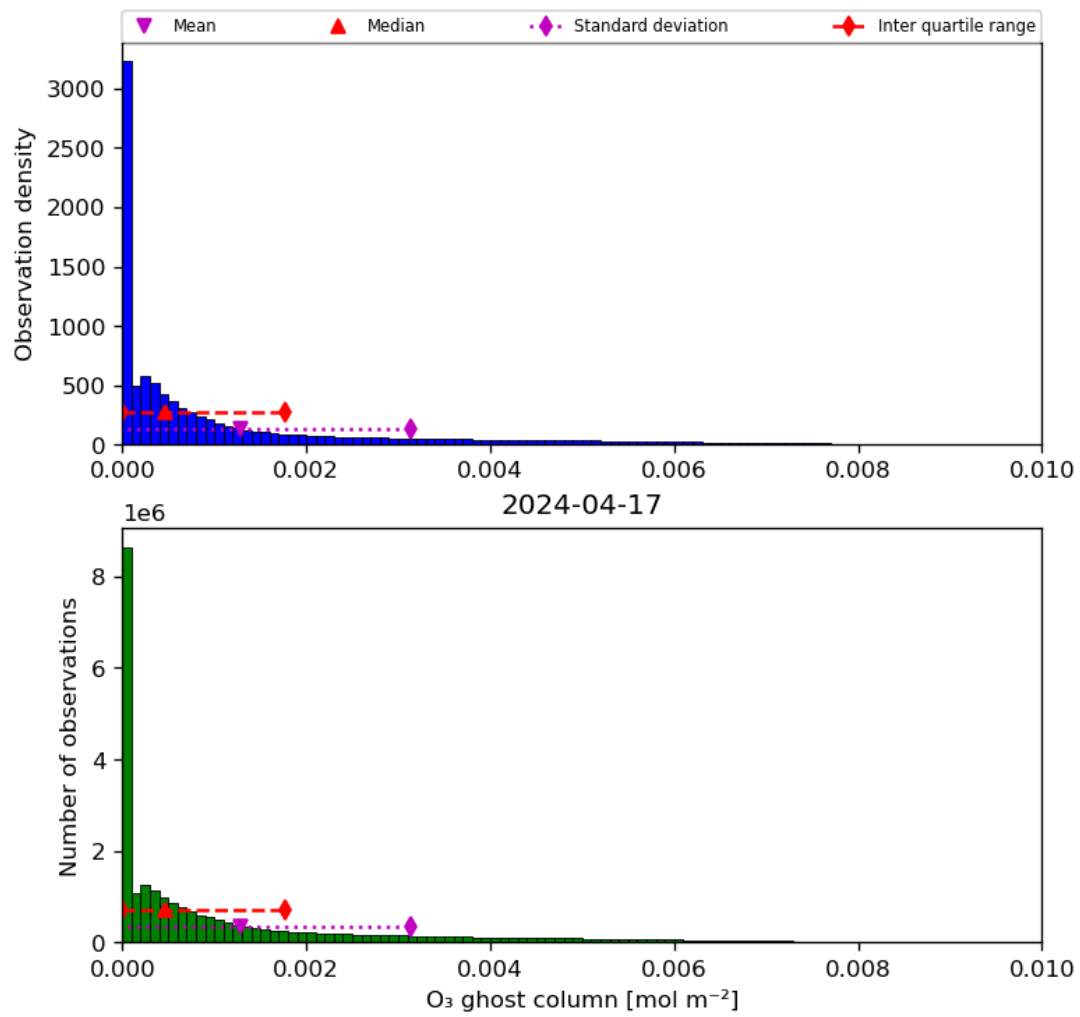
Figure 25: Histogram of "O 3 ghost column" for 2024-04-16 to 2024-04-18
