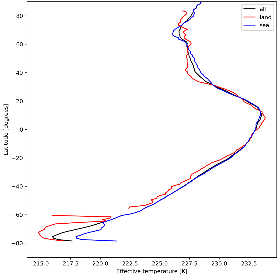
Figure 17: Zonal average of “Effective temperature” for 2024-04-16 to 2024-04-18.
