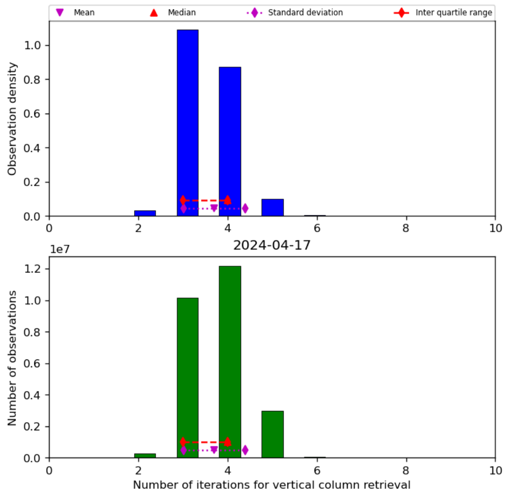
Figure 26: Histogram of “Number of iterations for vertical column retrieval” for 2024-04-16 to 2024-04-18
