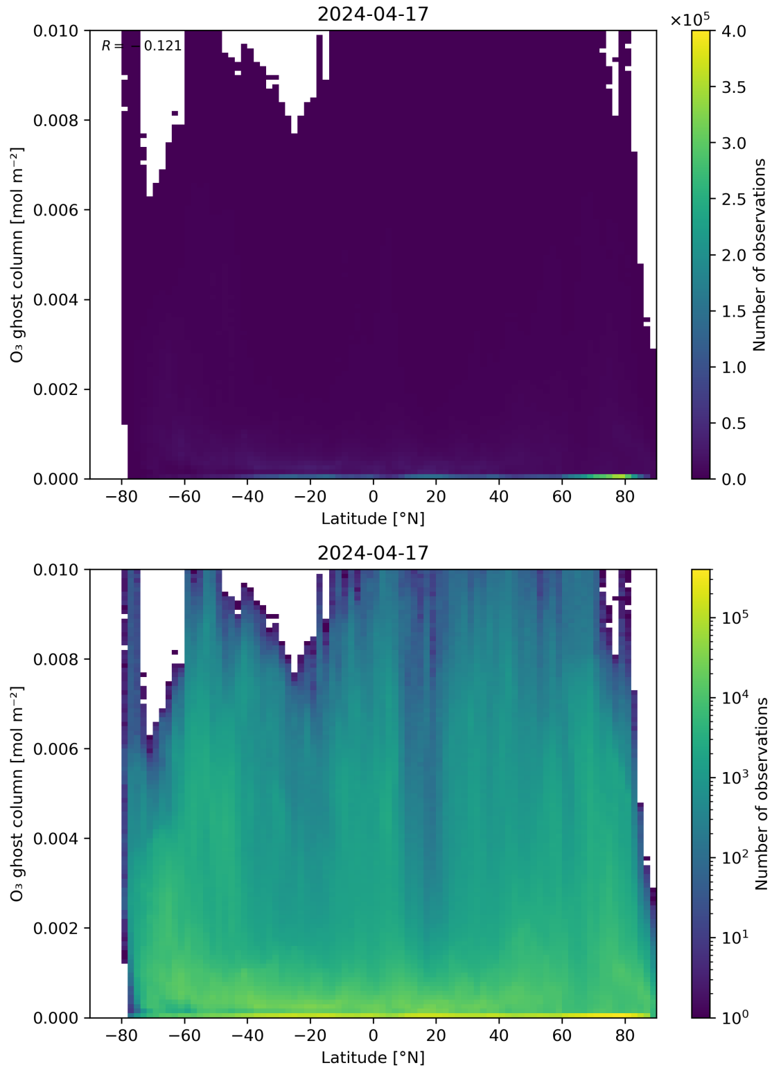
Figure 35: Scatter density plot of “Latitude” against “O 3 ghost column” for 2024-04-16 to 2024-04-18.
