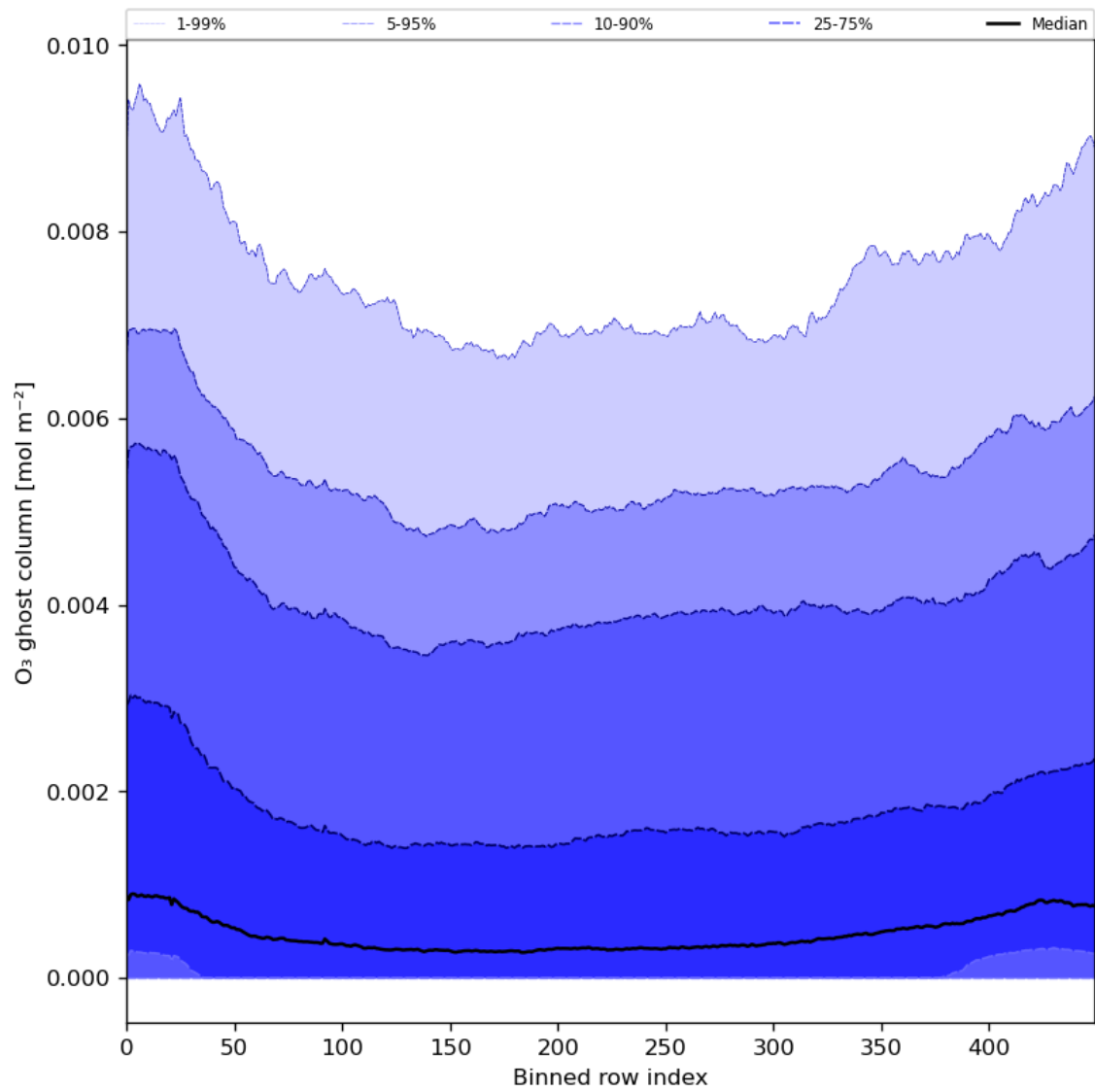
Figure 32: Along track statistics of “O 3 ghost column” for 2024-04-16 to 2024-04-18
