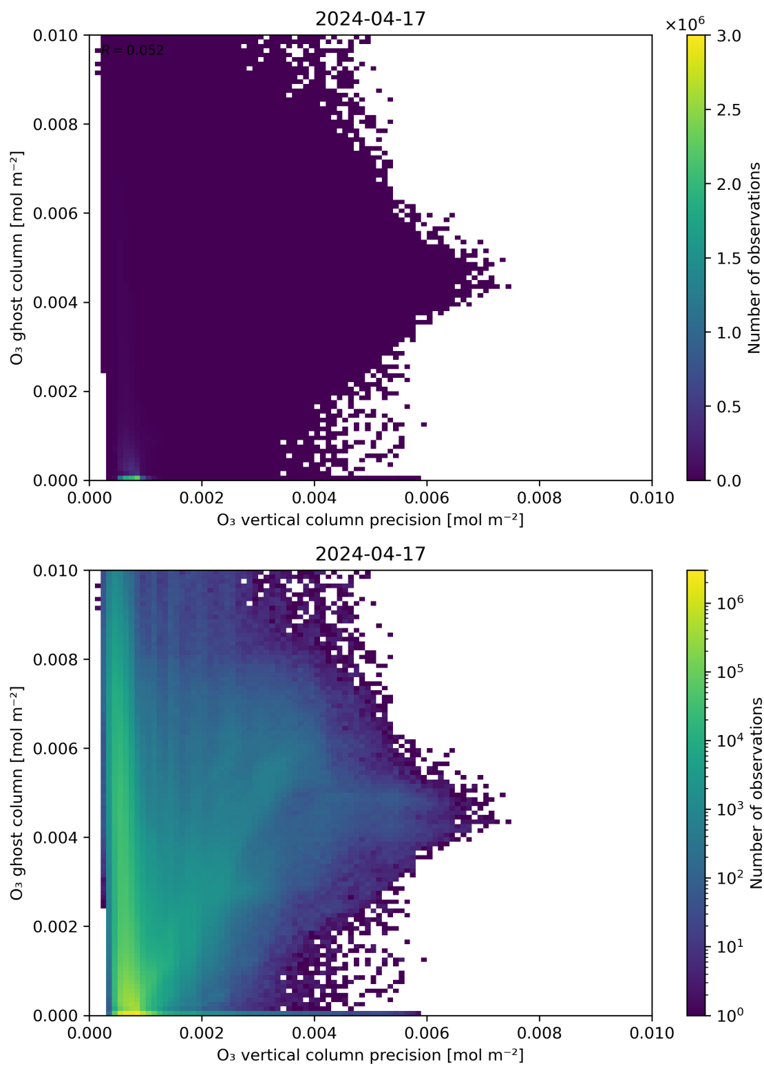
Figure 43: Scatter density plot of “ O_3 vertical column precision” against “ O_3 ghost column” for 2024-04-16 to 2024-04-18.
