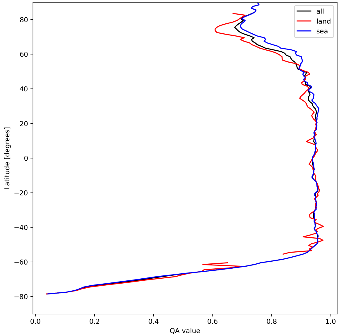
Figure 13: Zonal average of “QA value” for 2024-04-16 to 2024-04-18.
