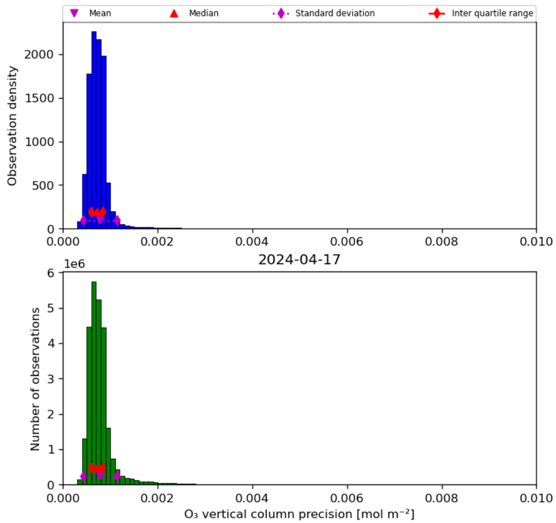
Figure 22: Histogram of “O 3 vertical column precision” for 2024-04-16 to 2024-04-18
