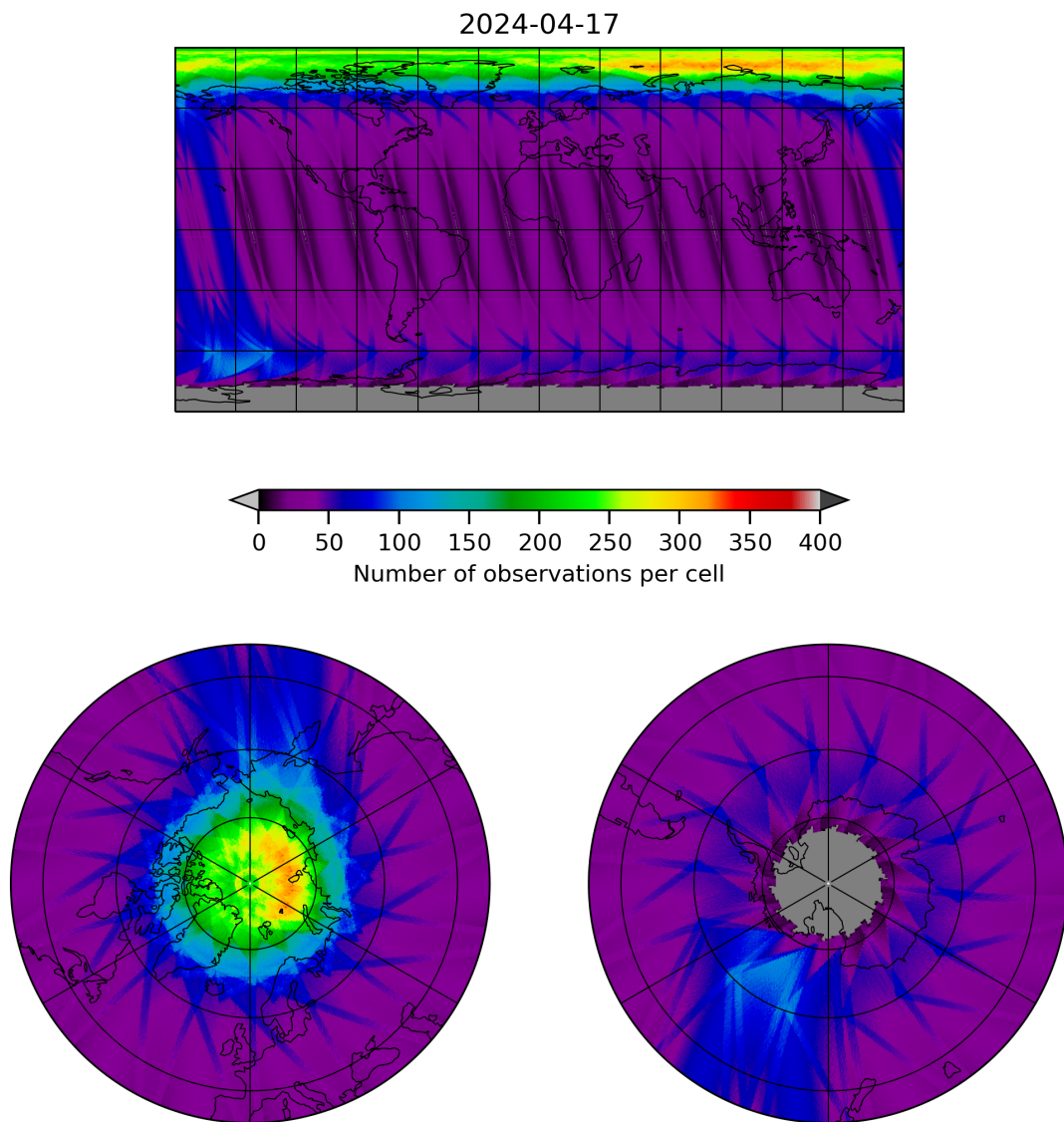
Figure 12: Map of the number of observations for 2024-04-16 to 2024-04-18
