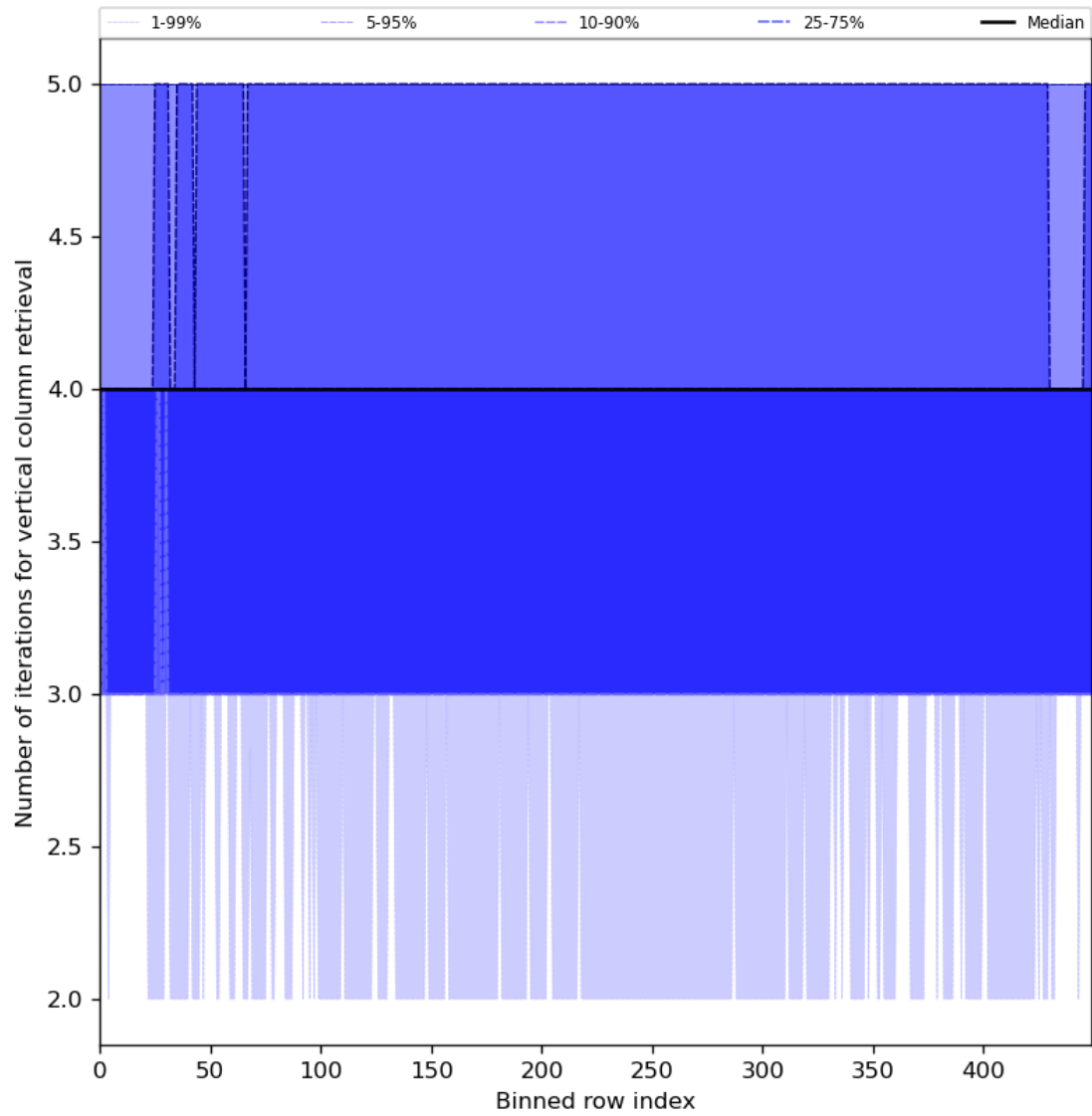
Figure 33: Along track statistics of “Number of iterations for vertical column retrieval” for 2024-04-16 to 2024-04-18
