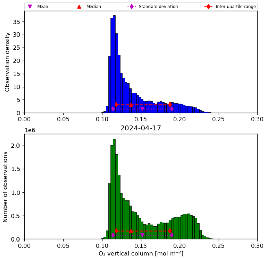
Figure 21: Histogram of “O 3 vertical column” for 2024-04-16 to 2024-04-18
