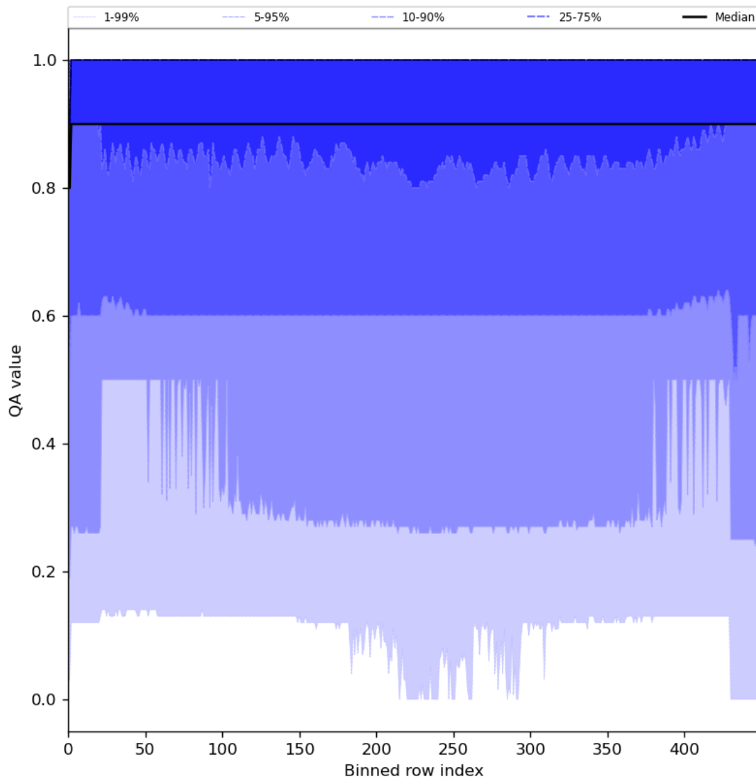
Figure 27: Along track statistics of “QA value” for 2024-04-16 to 2024-04-18
