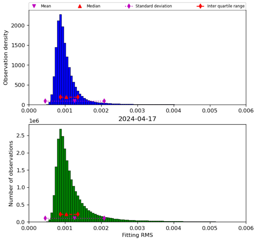
Figure 23: Histogram of “Fitting RMS” for 2024-04-16 to 2024-04-18
