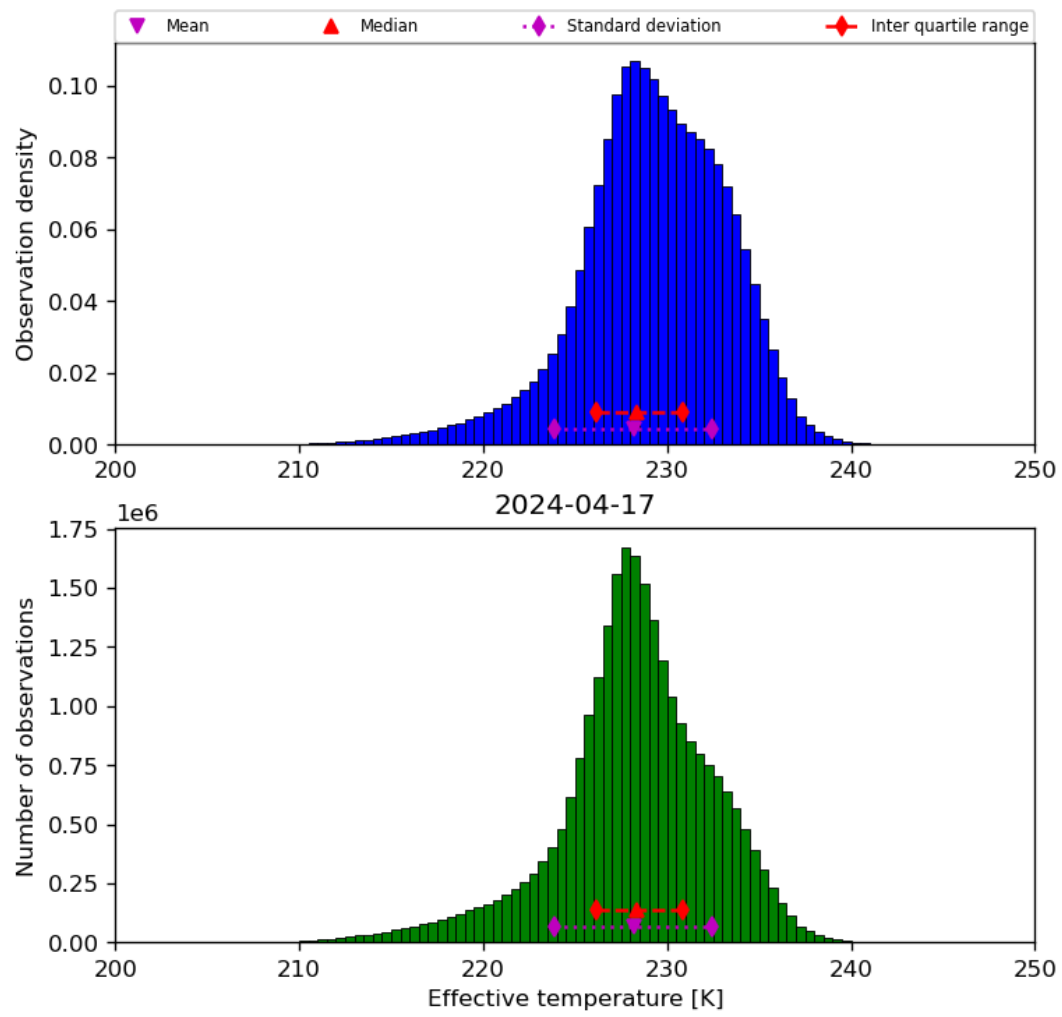
Figure 24: Histogram of “Effective temperature” for 2024-04-16 to 2024-04-18
