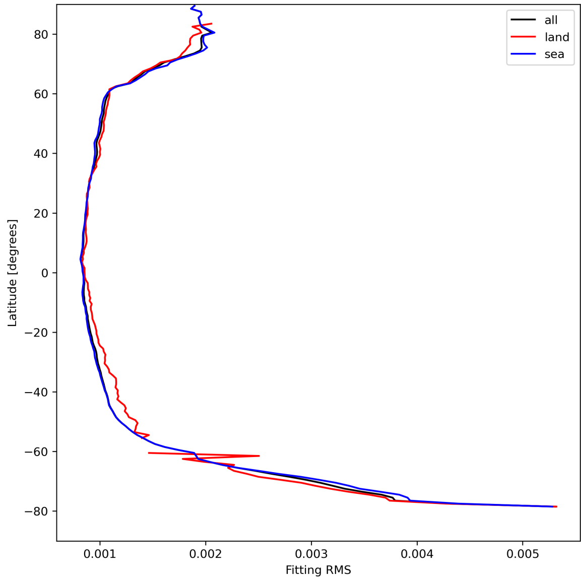
Figure 16: Zonal average of “Fitting RMS” for 2024-04-16 to 2024-04-18.
