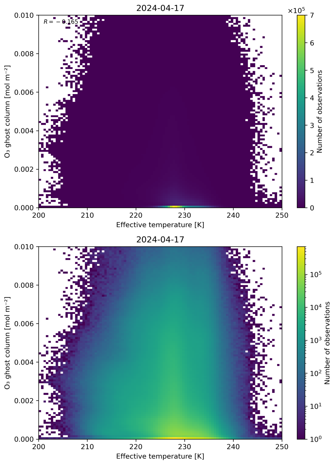
Figure 38: Scatter density plot of “Effective temperature” against “O 3 ghost column” for 2024-04-16 to 2024-04-18.
