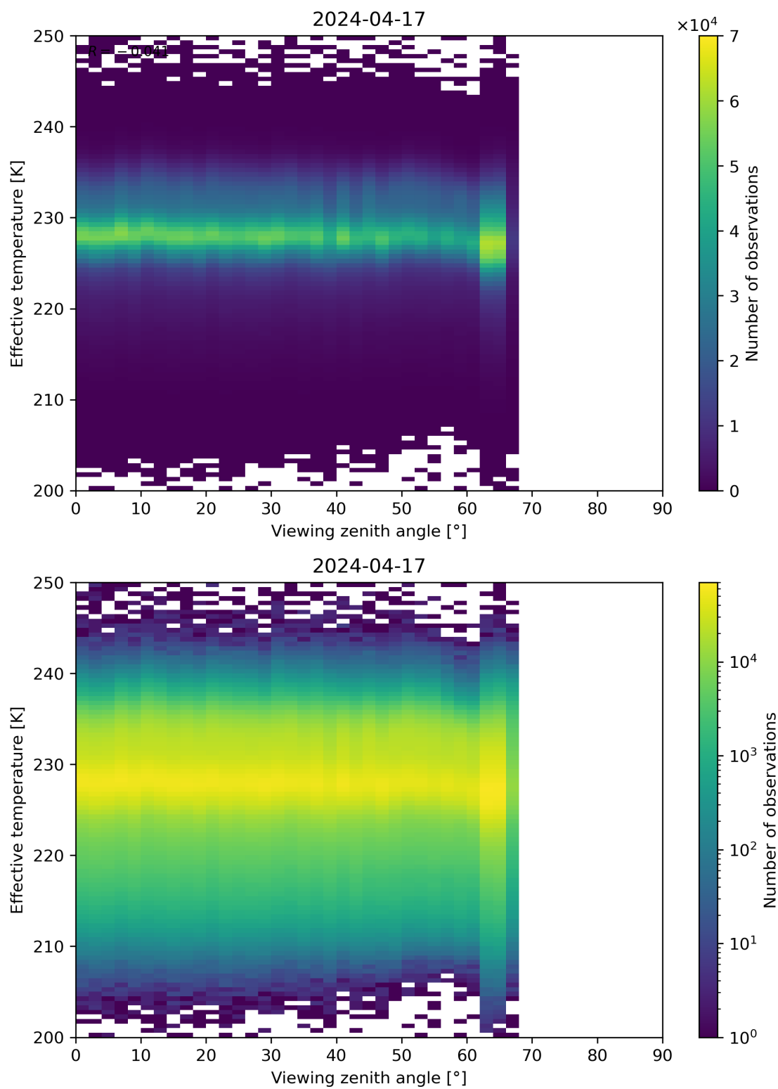
Figure 50: Scatter density plot of “Viewing zenith angle” against “Effective temperature” for 2024-04-16 to 2024-04-18.
