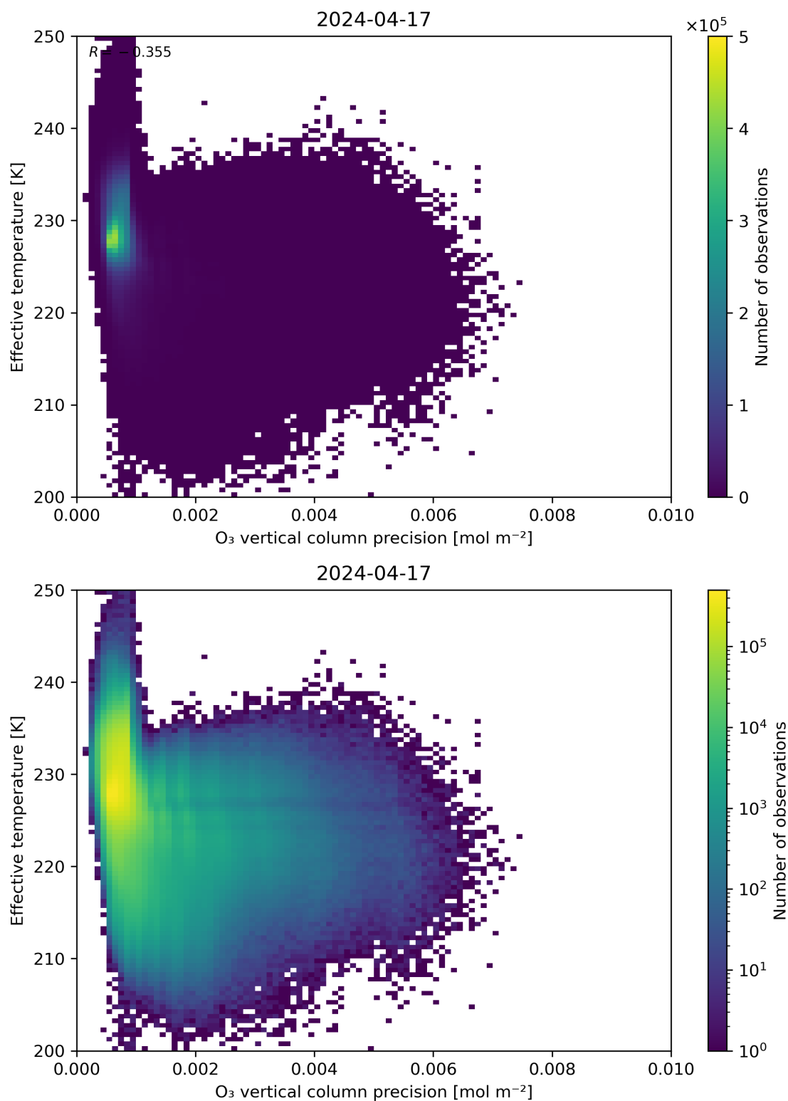
Figure 42: Scatter density plot of “O 3 vertical column precision” against “Effective temperature” for 2024-04-16 to 2024-04-18.
