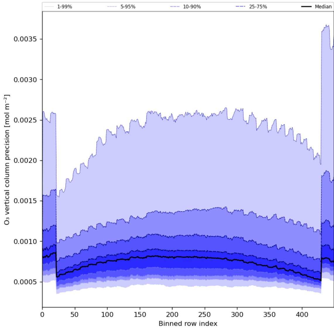
Figure 29: Along track statistics of “O 3 vertical column precision” for 2024-04-16 to 2024-04-18
