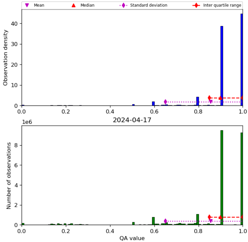
Figure 20: Histogram of “QA value” for 2024-04-16 to 2024-04-18
