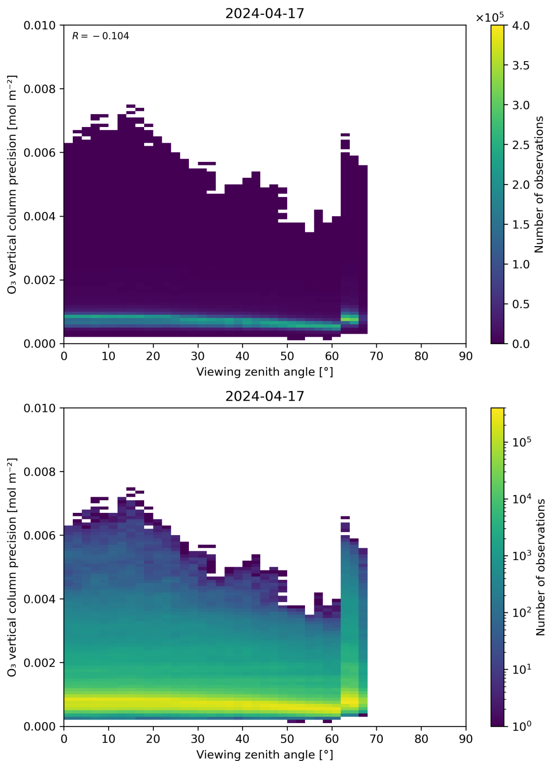
Figure 53: Scatter density plot of “Viewing zenith angle” against “O 3 vertical column precision” for 2024-04-16 to 2024-04-18.
