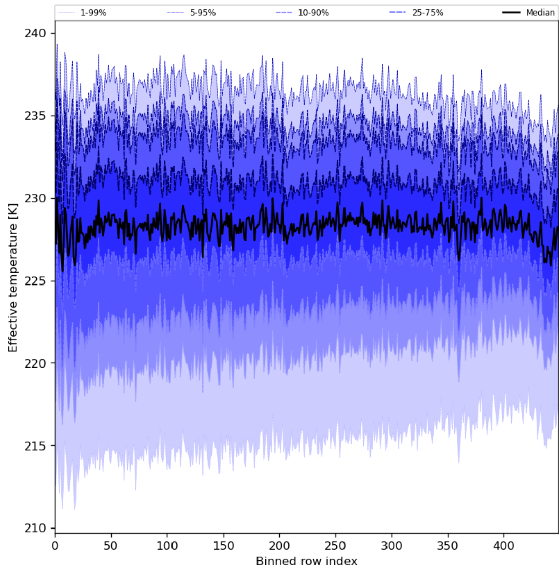
Figure 31: Along track statistics of “Effective temperature” for 2024-04-16 to 2024-04-18
