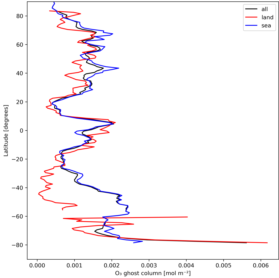
Figure 18: Zonal average of “O 3 ghost column” for 2024-04-16 to 2024-04-18.
