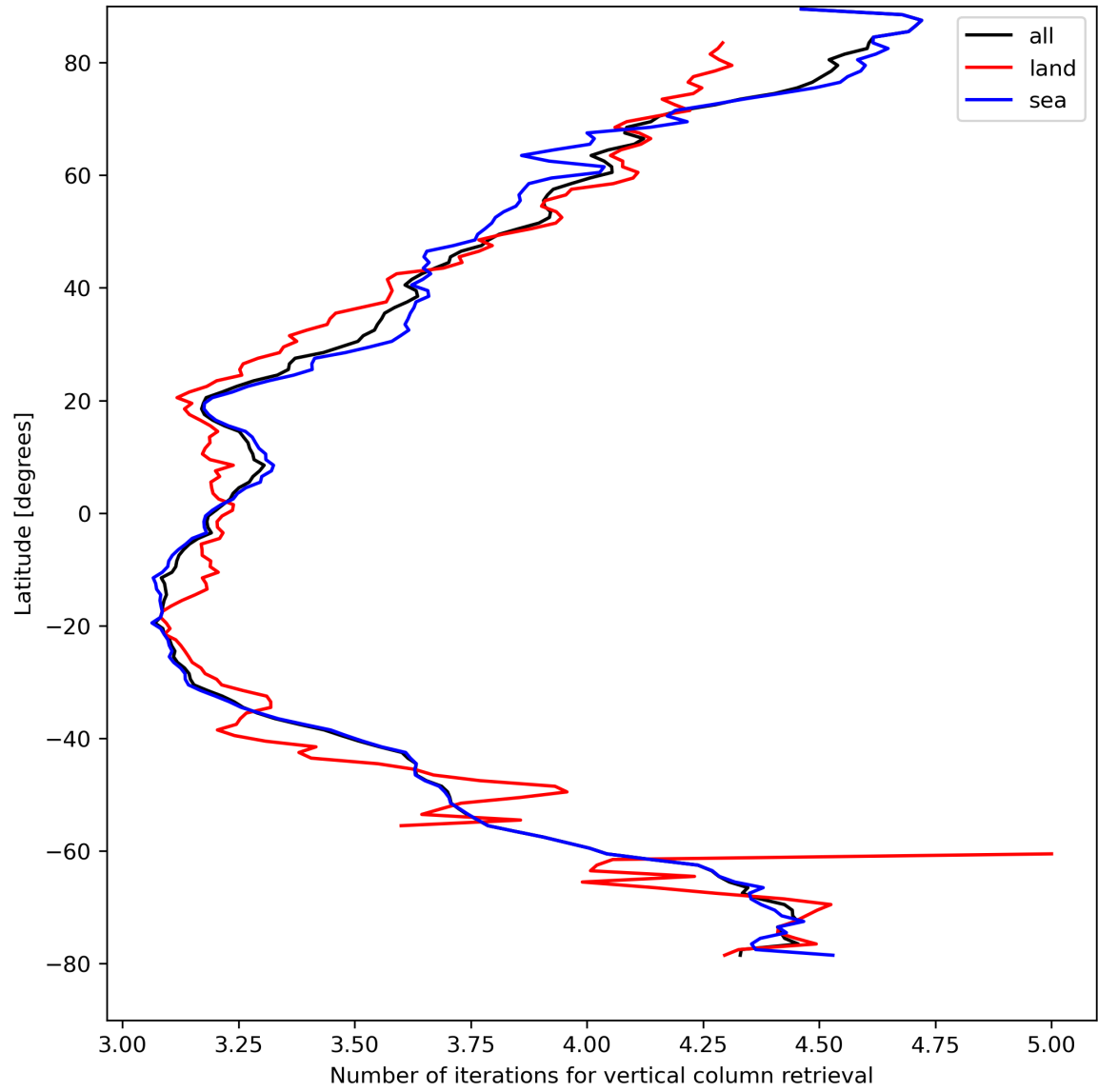
Figure 19: Zonal average of “Number of iterations for vertical column retrieval” for 2024-04-16 to 2024-04-18.
