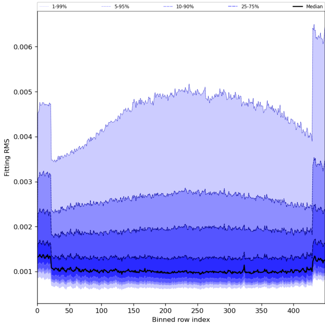
Figure 30: Along track statistics of “Fitting RMS” for 2024-04-16 to 2024-04-18
