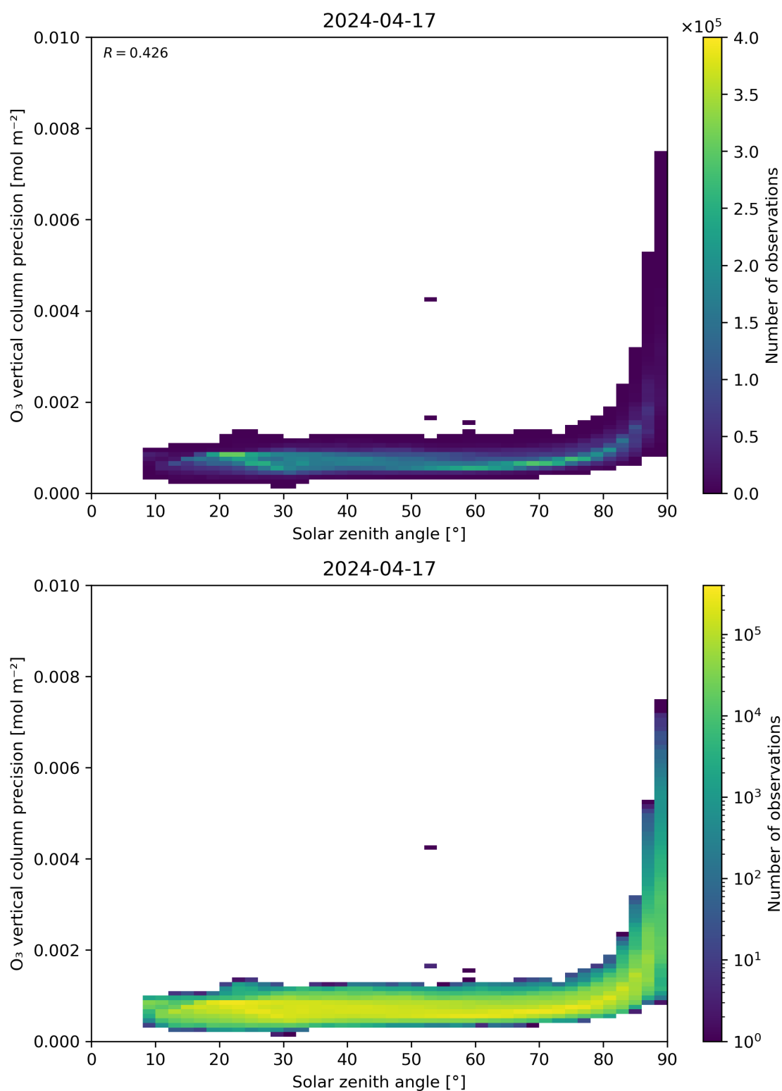
Figure 48: Scatter density plot of “Solar zenith angle” against “O 3 vertical column precision” for 2024-04-16 to 2024-04-18.
