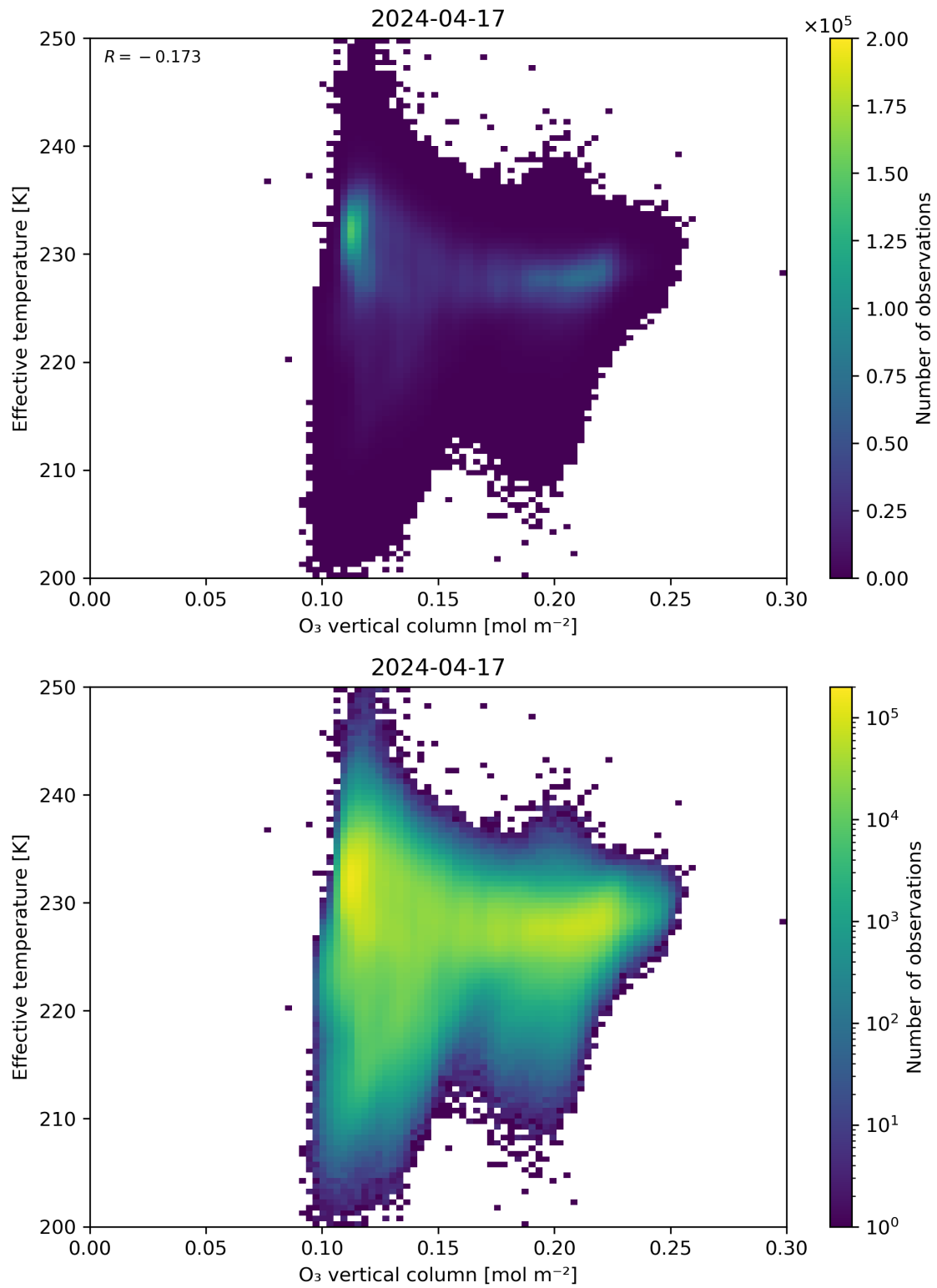
Figure 39: Scatter density plot of “O 3 vertical column” against “Effective temperature” for 2024-04-16 to 2024-04-18.
