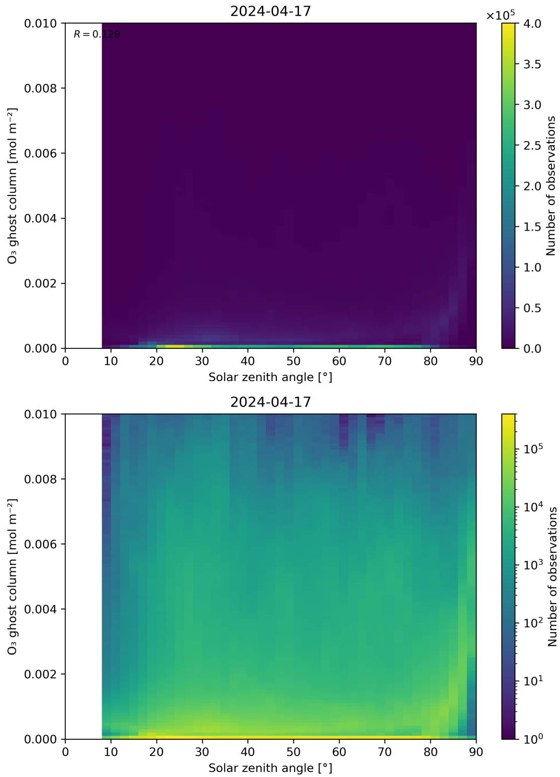
Figure 46: Scatter density plot of “Solar zenith angle” against “O 3 ghost column” for 2024-04-16 to 2024-04-18.
