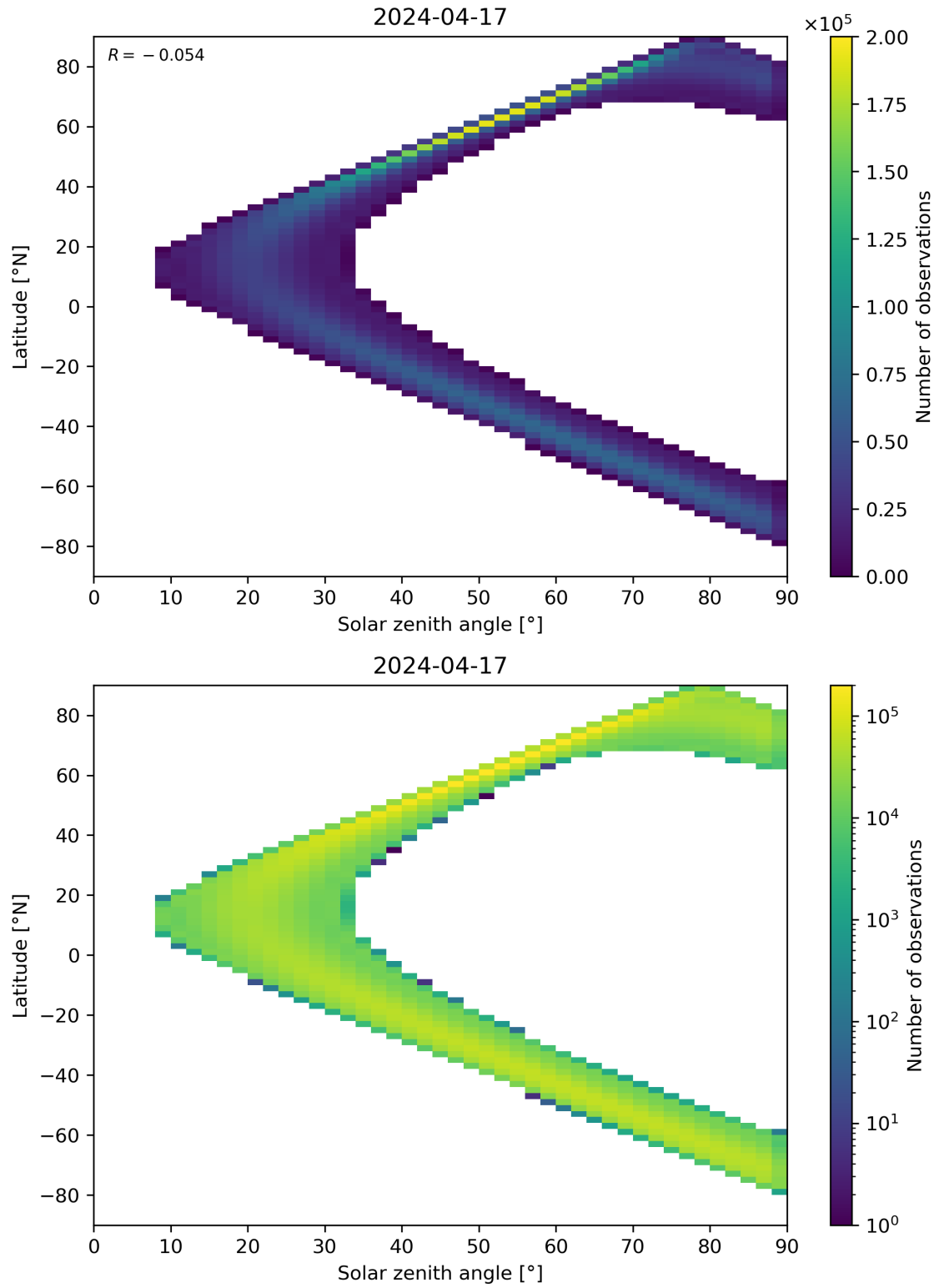
Figure 44: Scatter density plot of “Solar zenith angle” against “Latitude” for 2024-04-16 to 2024-04-18.
