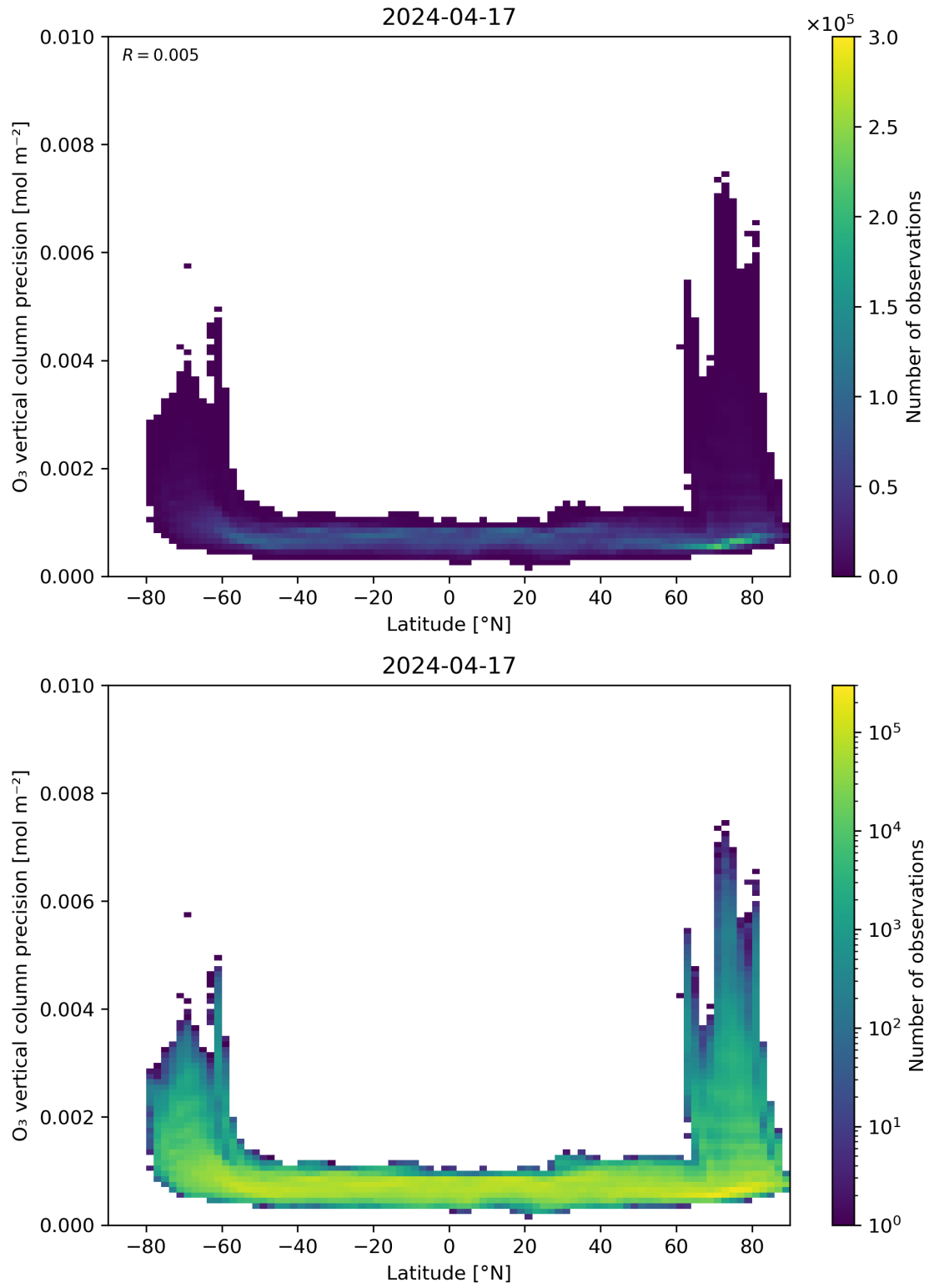
Figure 37: Scatter density plot of “Latitude” against “O 3 vertical column precision” for 2024-04-16 to 2024-04-18.
