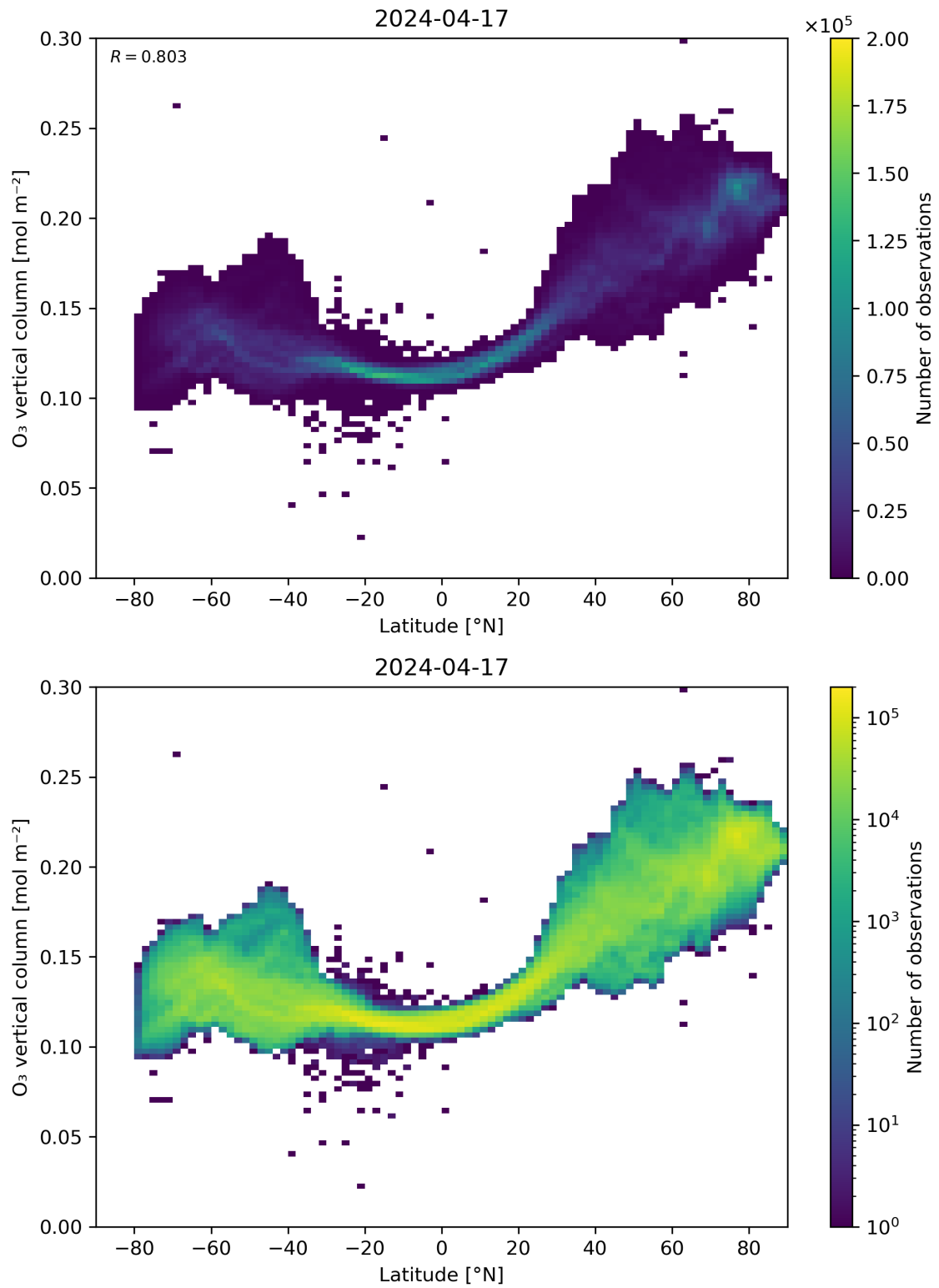
Figure 36: Scatter density plot of “Latitude” against “O 3 vertical column” for 2024-04-16 to 2024-04-18.
