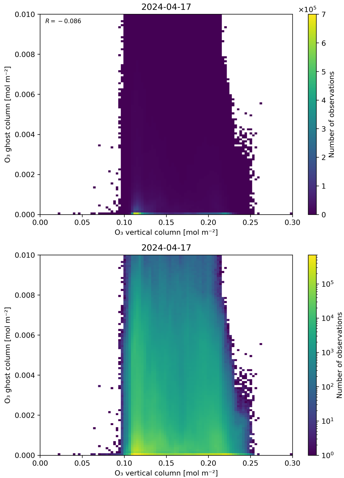
Figure 40: Scatter density plot of “O 3 vertical column” against “O 3 ghost column” for 2024-04-16 to 2024-04-18.
