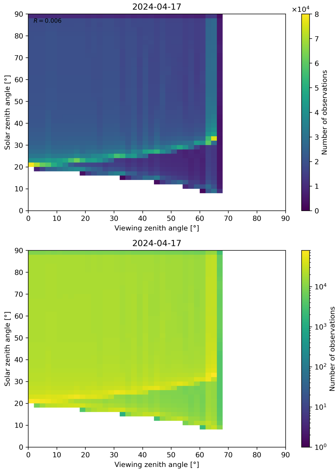
Figure 54: Scatter density plot of “Viewing zenith angle” against “Solar zenith angle” for 2024-04-16 to 2024-04-18.
