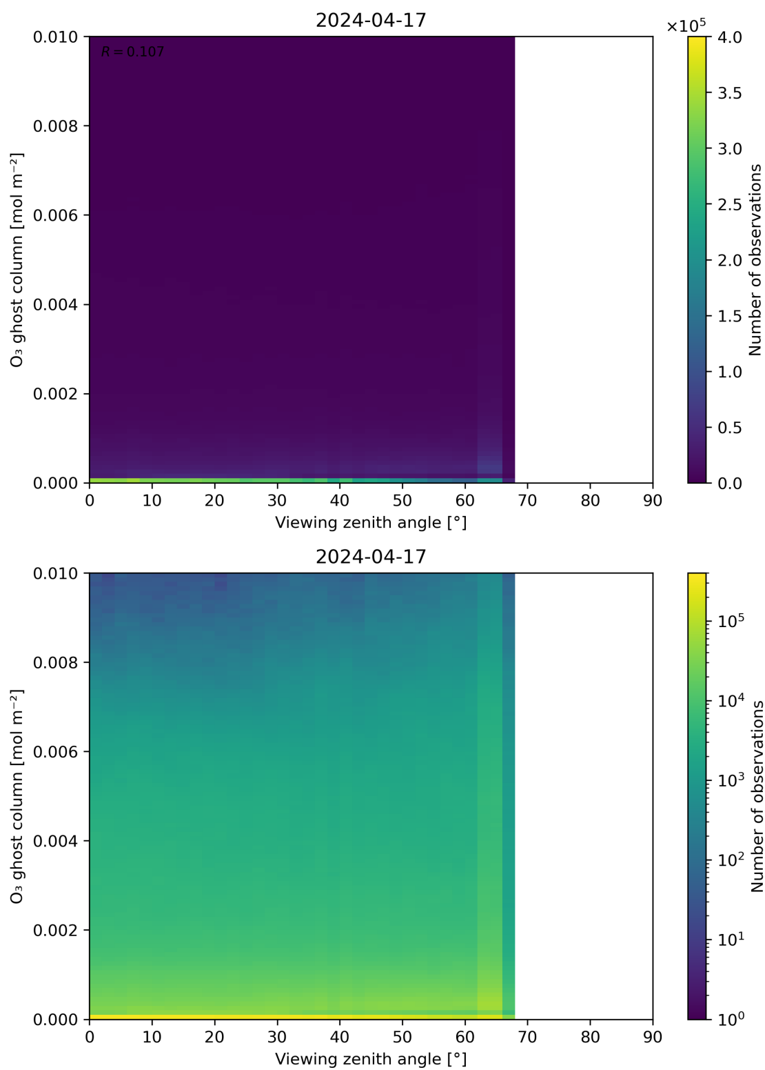
Figure 51: Scatter density plot of “Viewing zenith angle” against “O 3 ghost column” for 2024-04-16 to 2024-04-18.
