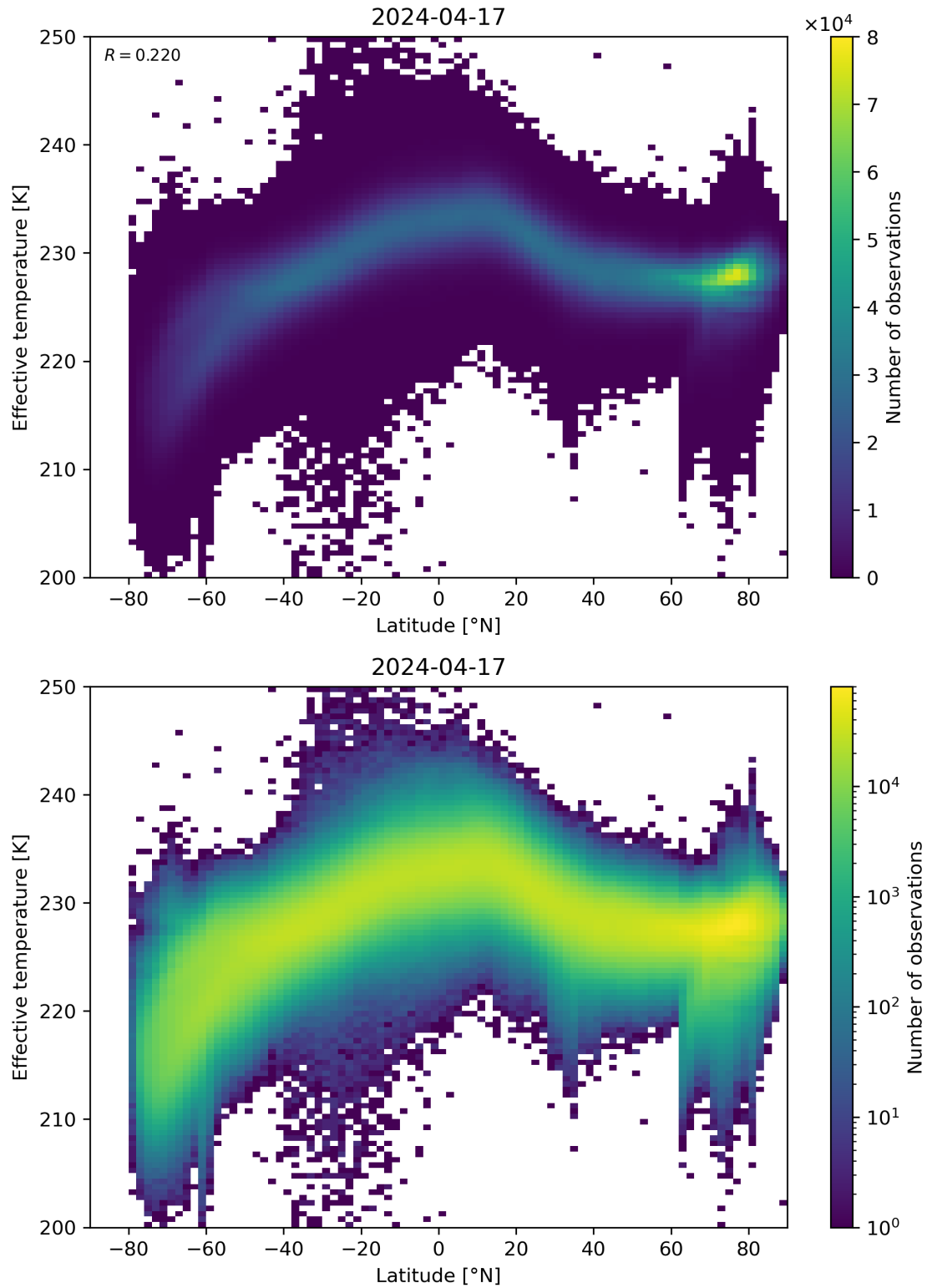
Figure 34: Scatter density plot of “Latitude” against “Effective temperature” for 2024-04-16 to 2024-04-18.
