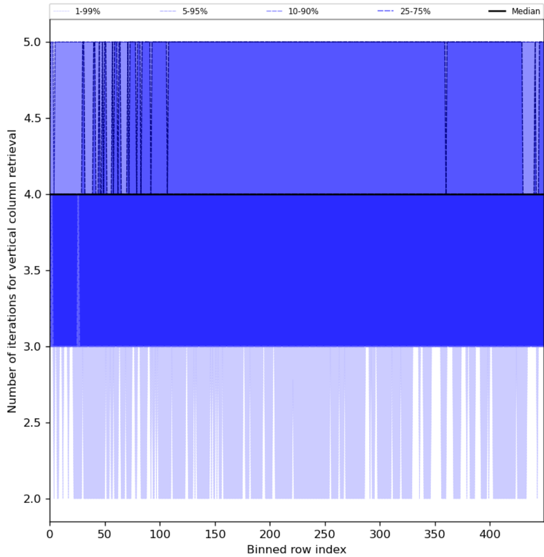
Figure 33: Along track statistics of “Number of iterations for vertical column retrieval” for 2024-04-17 to 2024-04-19
