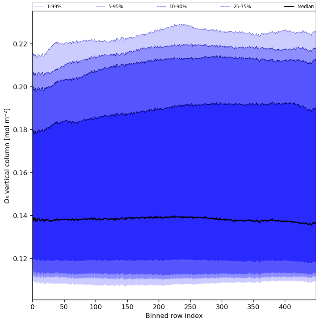
Figure 28: Along track statistics of “O 3 vertical column” for 2024-04-17 to 2024-04-19
