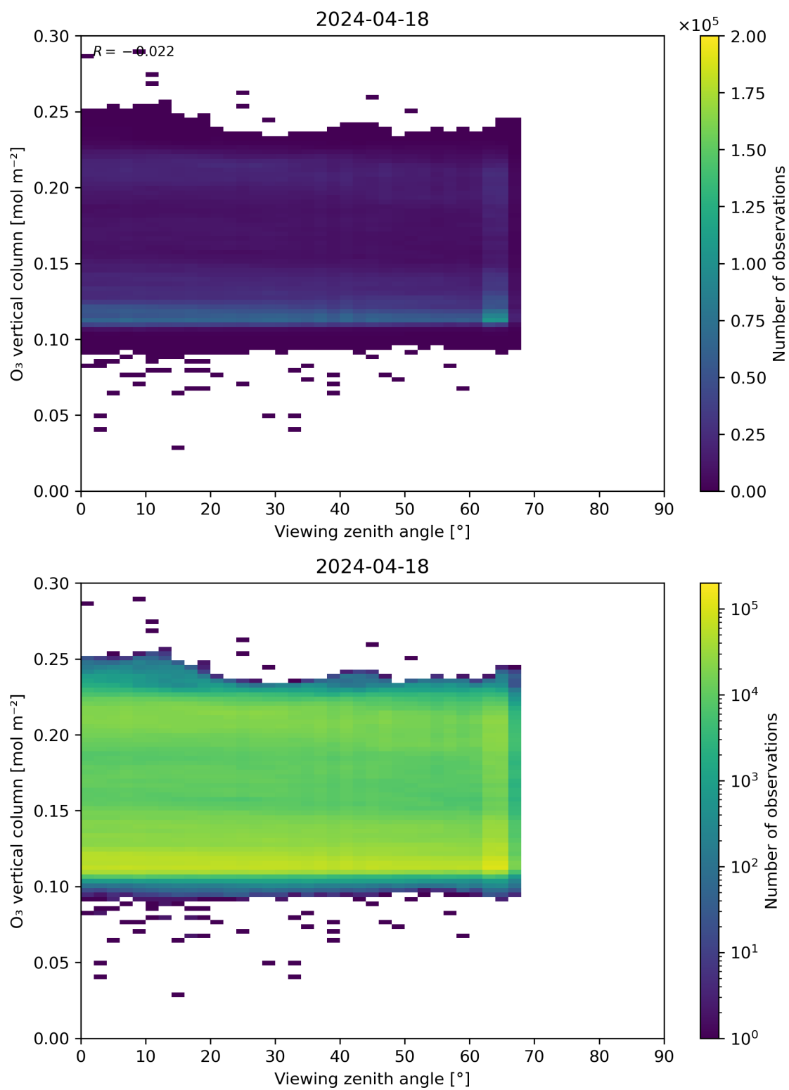
Figure 52: Scatter density plot of “Viewing zenith angle” against “O 3 vertical column” for 2024-04-17 to 2024-04-19.
