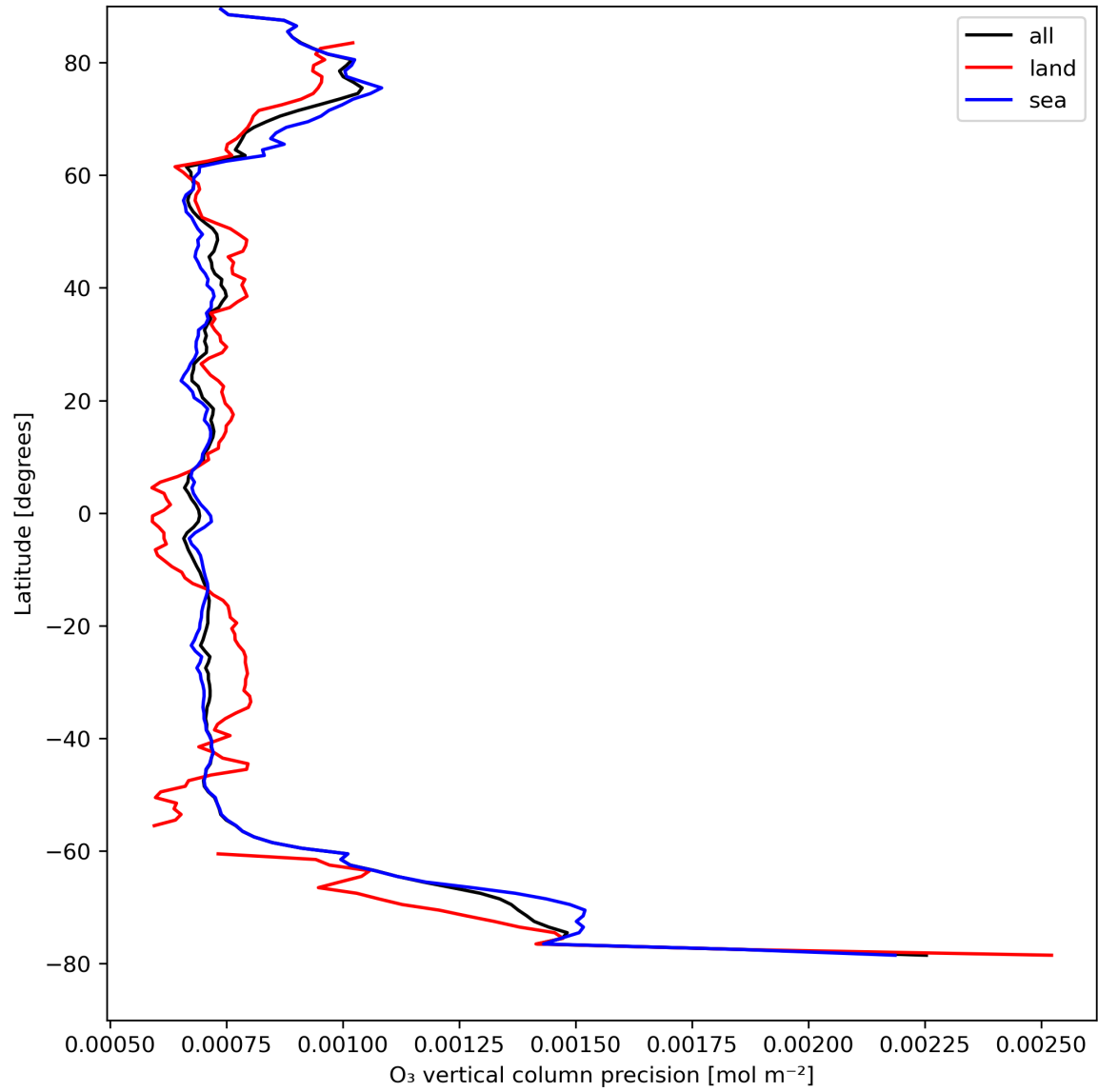
Figure 15: Zonal average of "O 3 vertical column precision" for 2024-04-17 to 2024-04-19.
