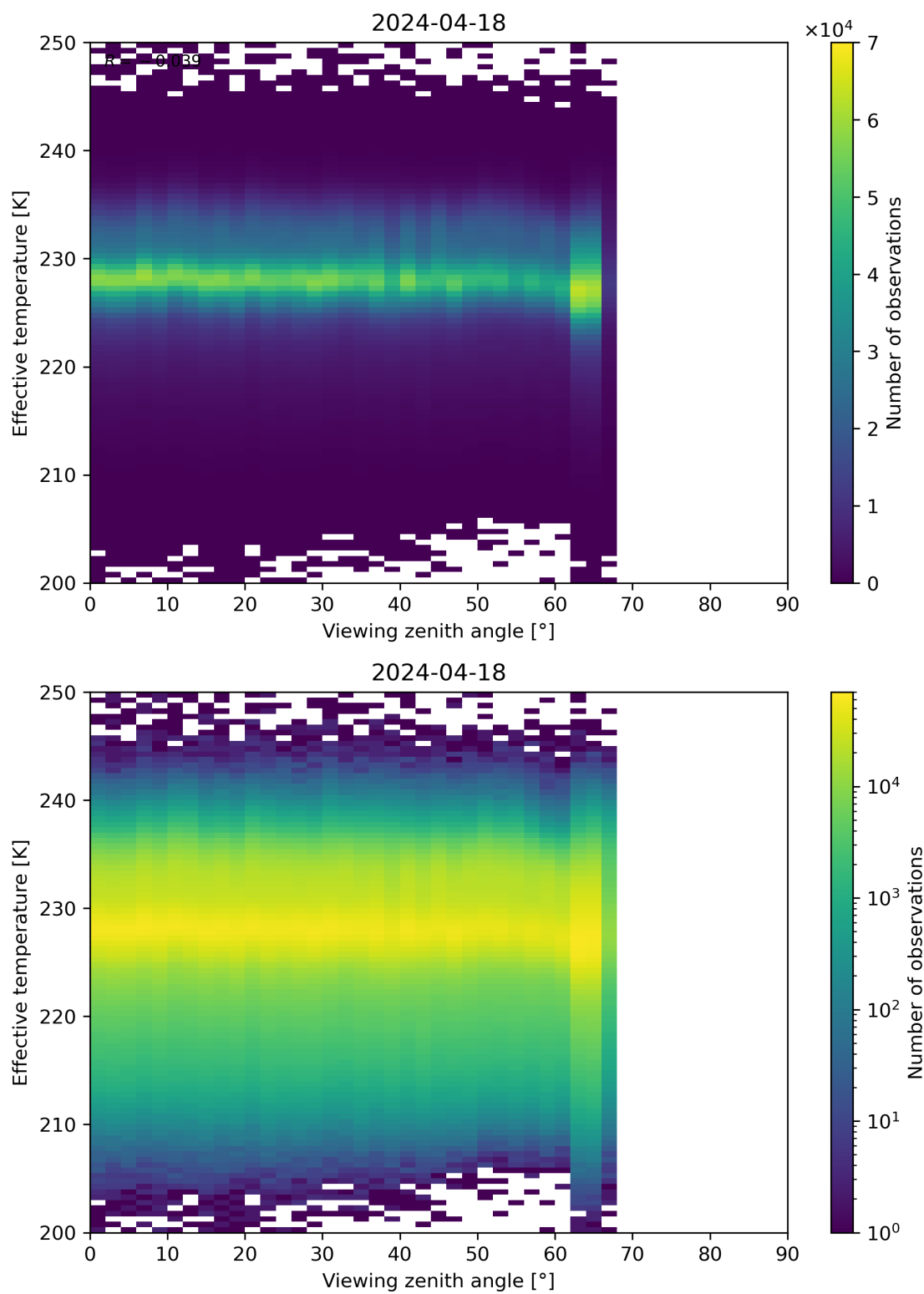
Figure 50: Scatter density plot of “Viewing zenith angle” against “Effective temperature” for 2024-04-17 to 2024-04-19.
